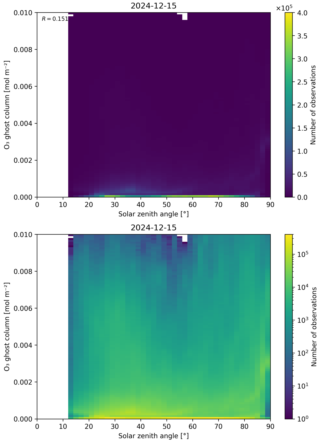
Figure 46: Scatter density plot of “Solar zenith angle” against “O 3 ghost column” for 2024-12-14 to 2024-12-16.
