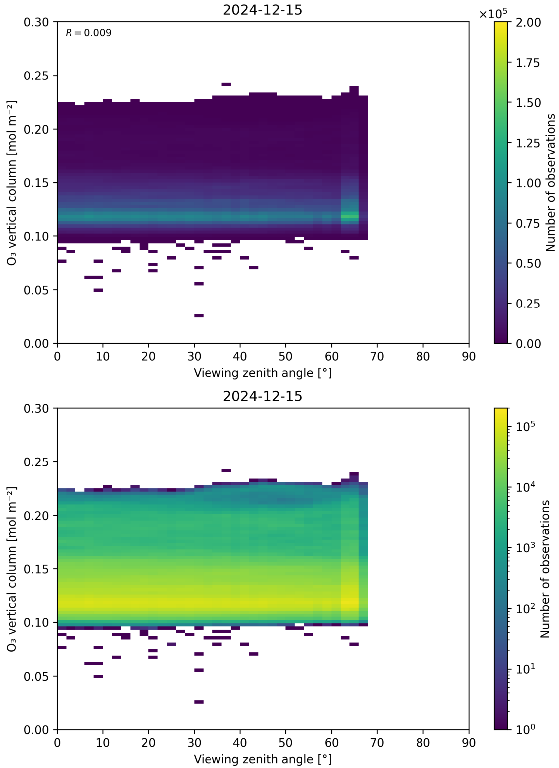
Figure 52: Scatter density plot of “Viewing zenith angle” against “O 3 vertical column” for 2024-12-14 to 2024-12-16.
