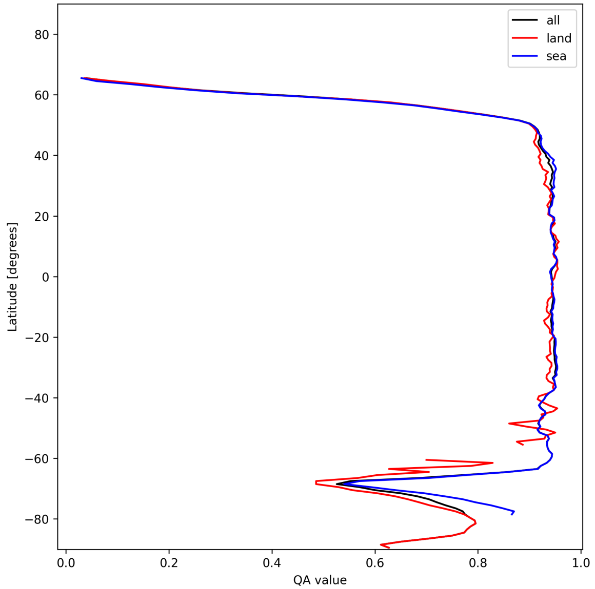
Figure 13: Zonal average of “QA value” for 2024-12-14 to 2024-12-16.
