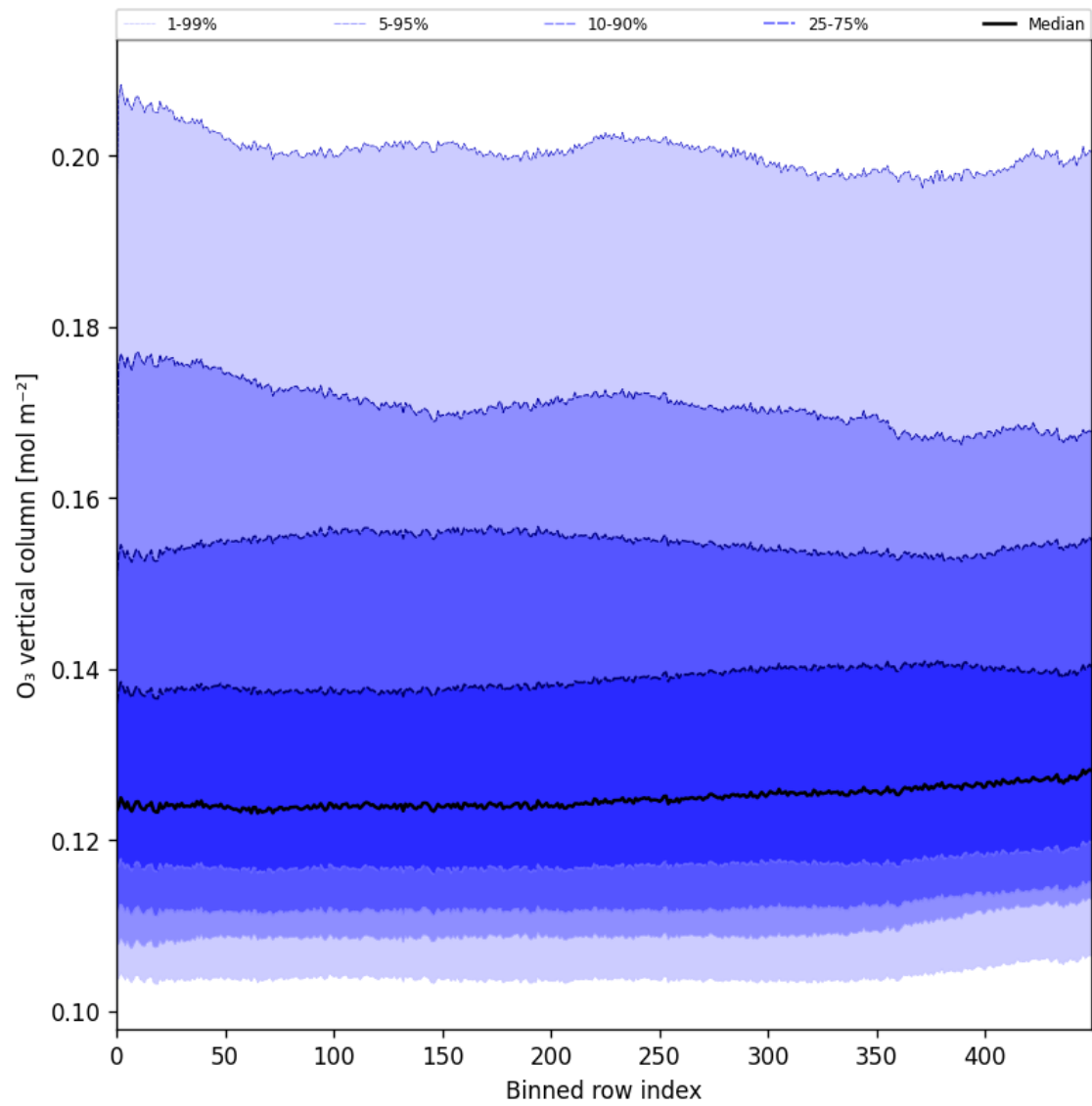
Figure 28: Along track statistics of “O 3 vertical column” for 2024-12-14 to 2024-12-16
