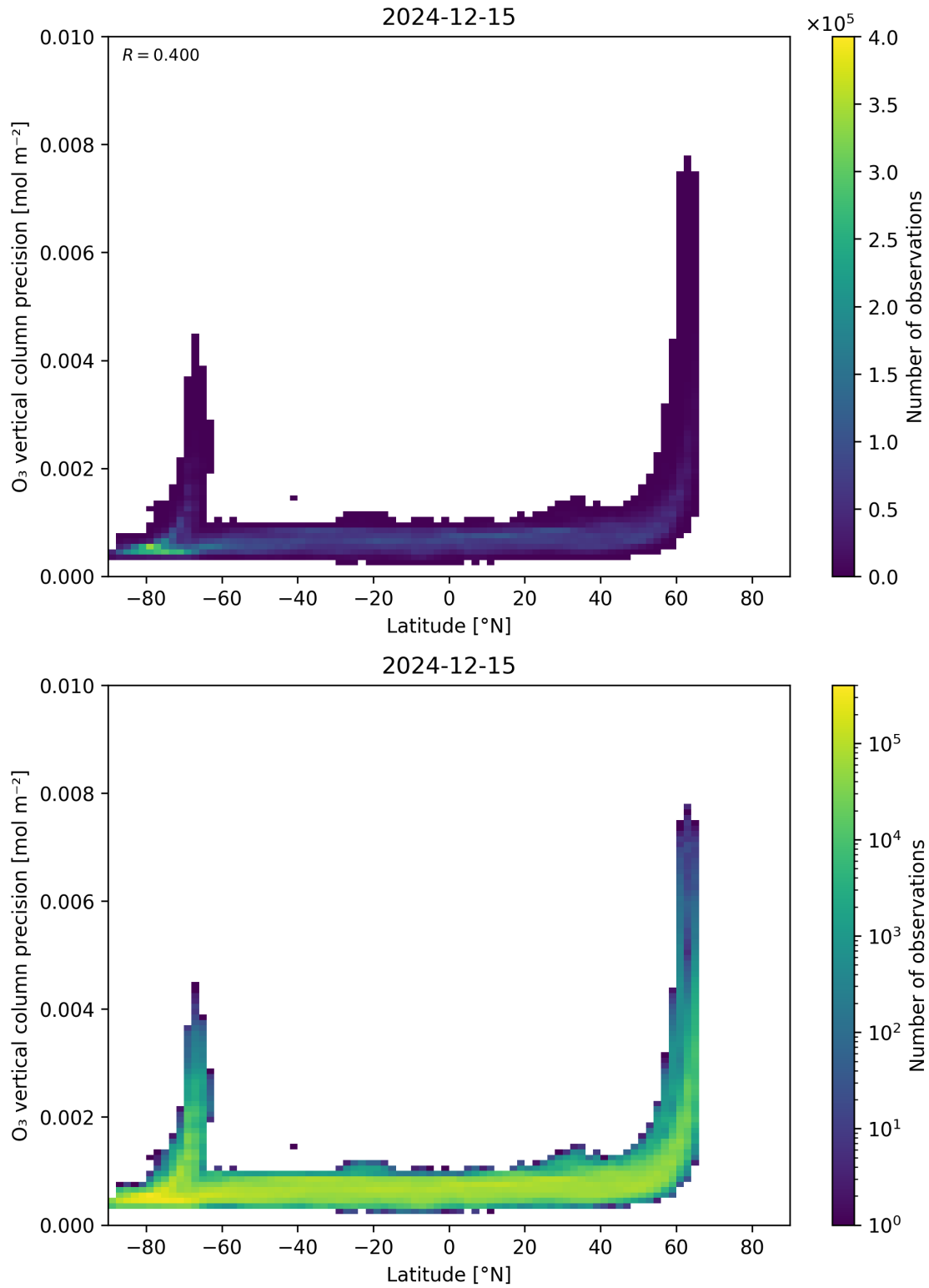
Figure 37: Scatter density plot of “Latitude” against “O 3 vertical column precision” for 2024-12-14 to 2024-12-16.
