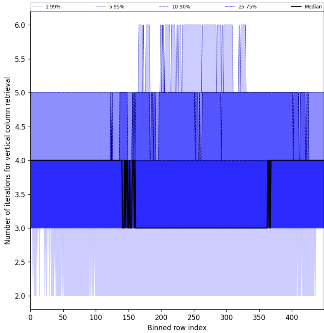
Figure 33: Along track statistics of “Number of iterations for vertical column retrieval” for 2024-12-14 to 2024-12-16
