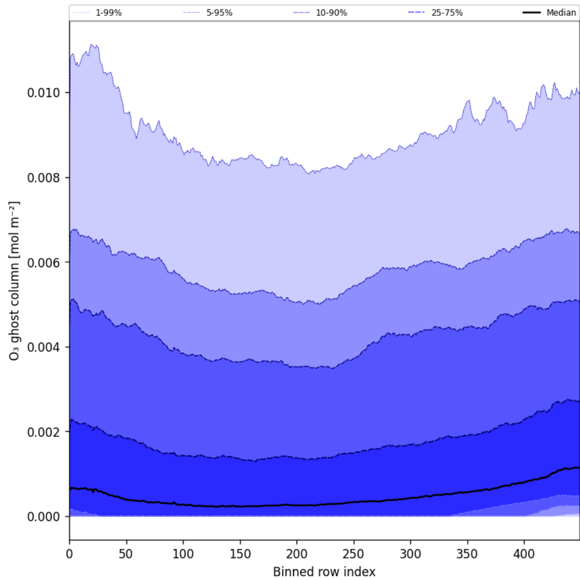
Figure 32: Along track statistics of “O 3 ghost column” for 2024-12-14 to 2024-12-16
