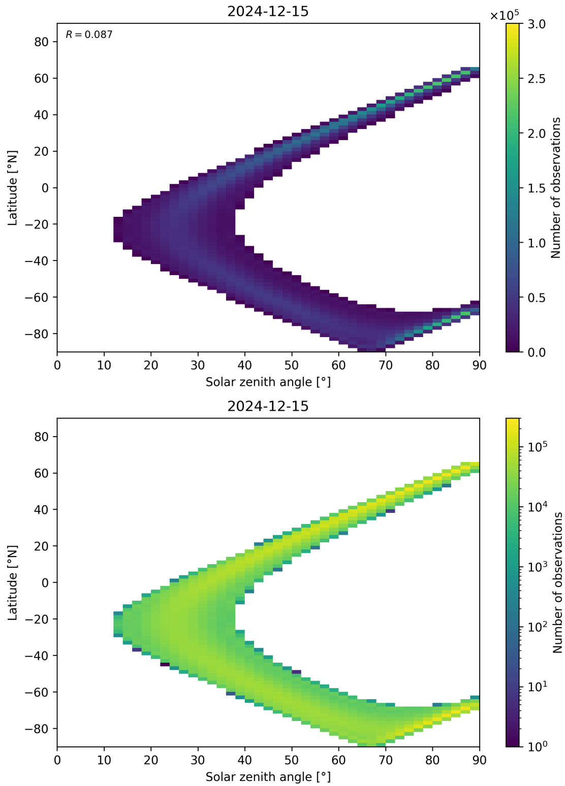
Figure 44: Scatter density plot of “Solar zenith angle” against “Latitude” for 2024-12-14 to 2024-12-16.
