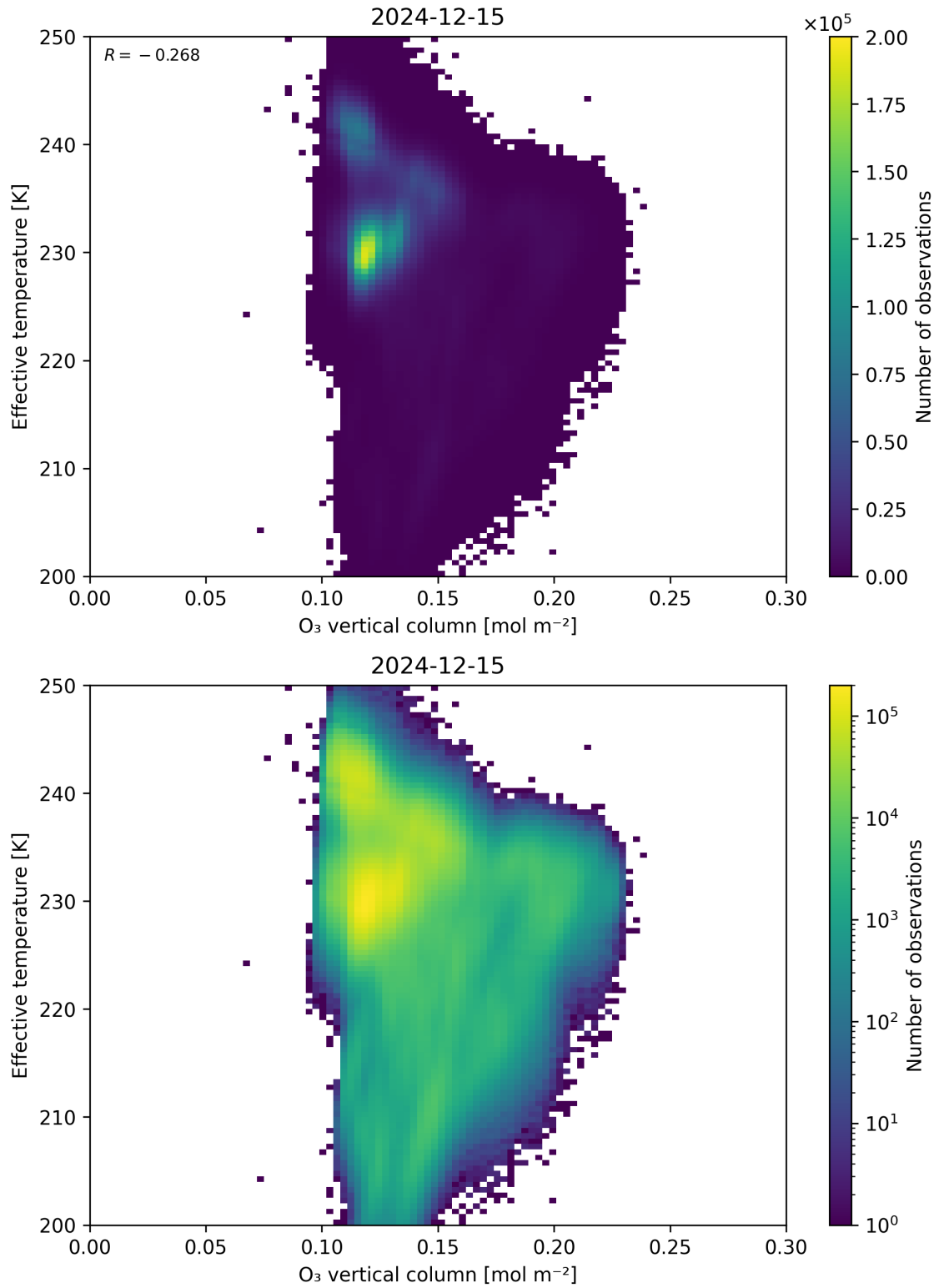
Figure 39: Scatter density plot of “O 3 vertical column” against “Effective temperature” for 2024-12-14 to 2024-12-16.
