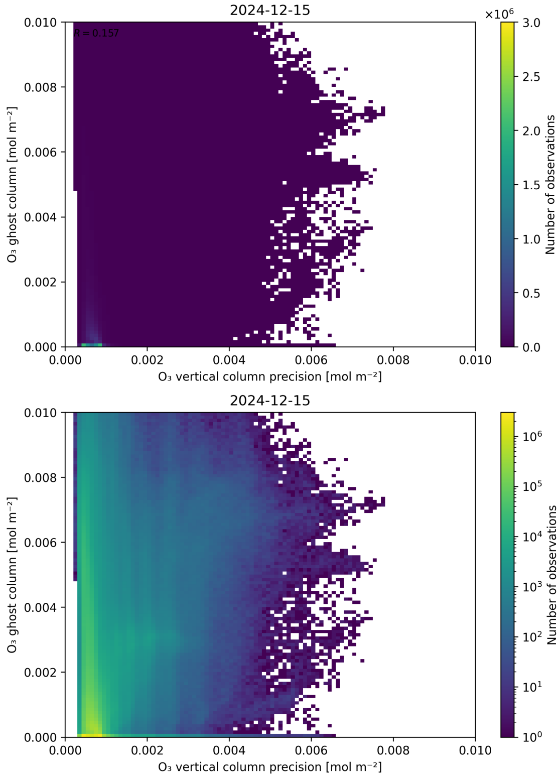
Figure 43: Scatter density plot of “ \text{O}_3 vertical column precision” against “ \text{O}_3 ghost column” for 2024-12-14 to 2024-12-16.
