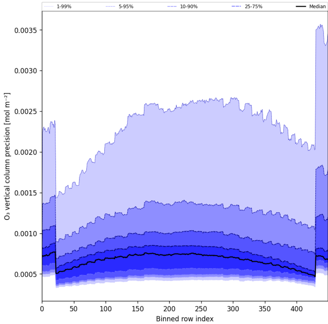
Figure 29: Along track statistics of “O 3 vertical column precision” for 2024-12-14 to 2024-12-16
