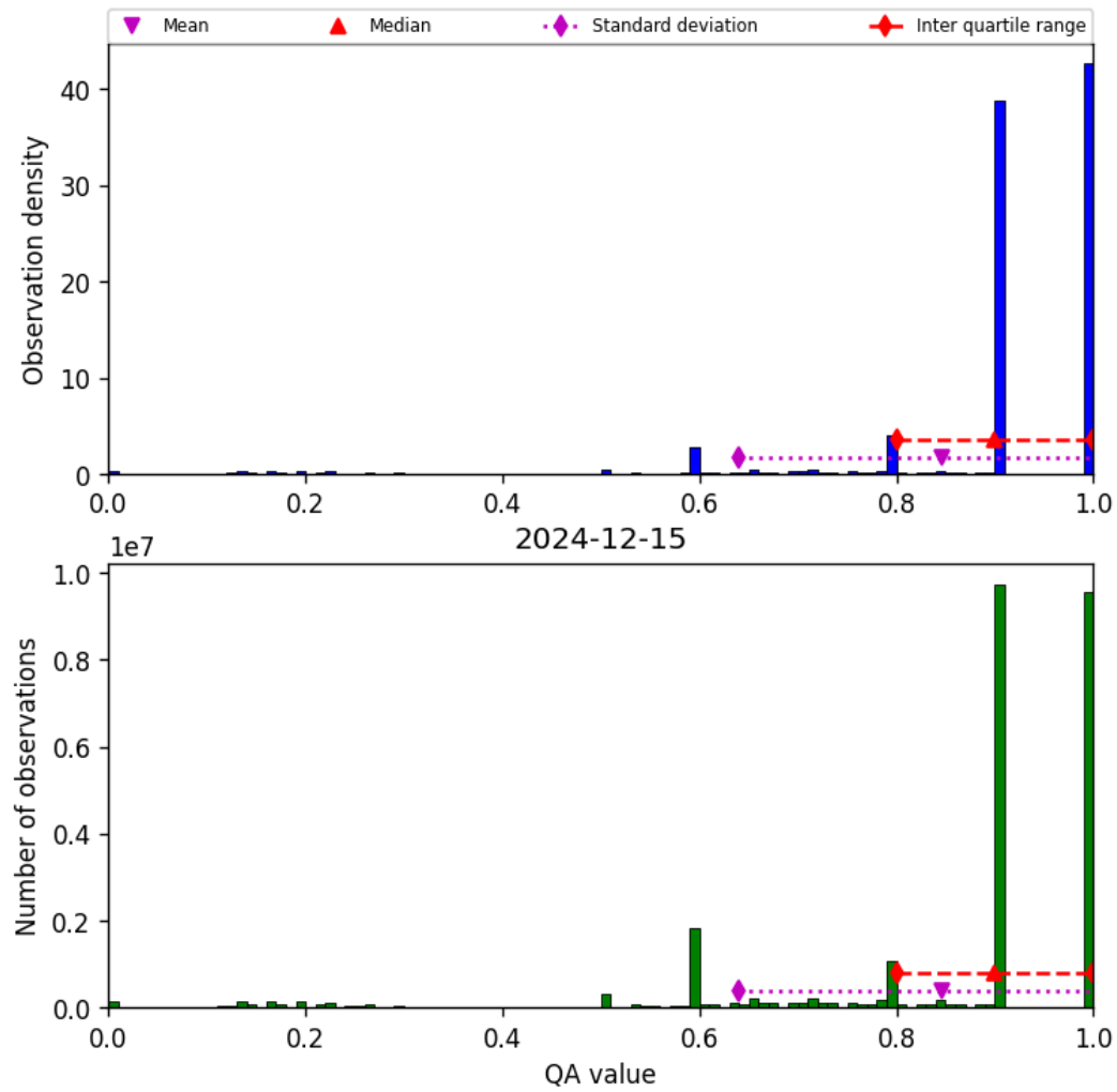
Figure 20: Histogram of “QA value” for 2024-12-14 to 2024-12-16
