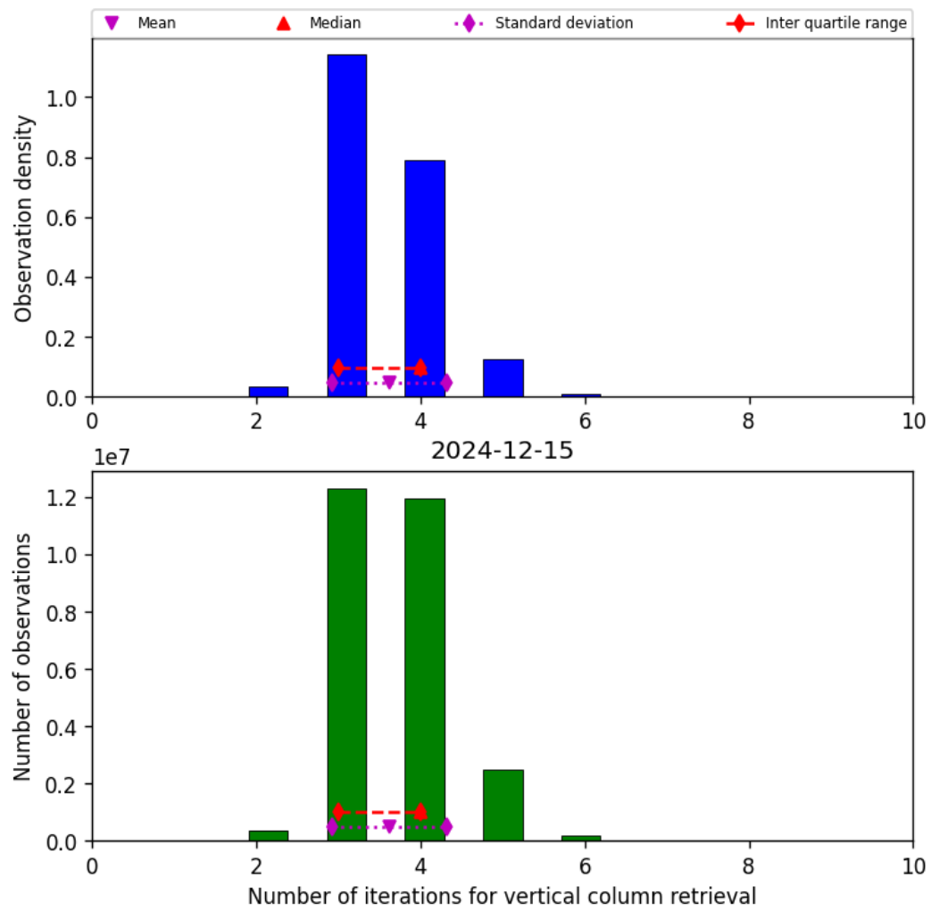
Figure 26: Histogram of “Number of iterations for vertical column retrieval” for 2024-12-14 to 2024-12-16
