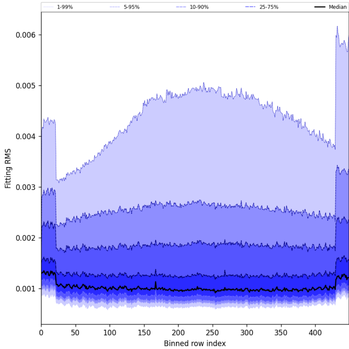
Figure 30: Along track statistics of “Fitting RMS” for 2024-12-14 to 2024-12-16
