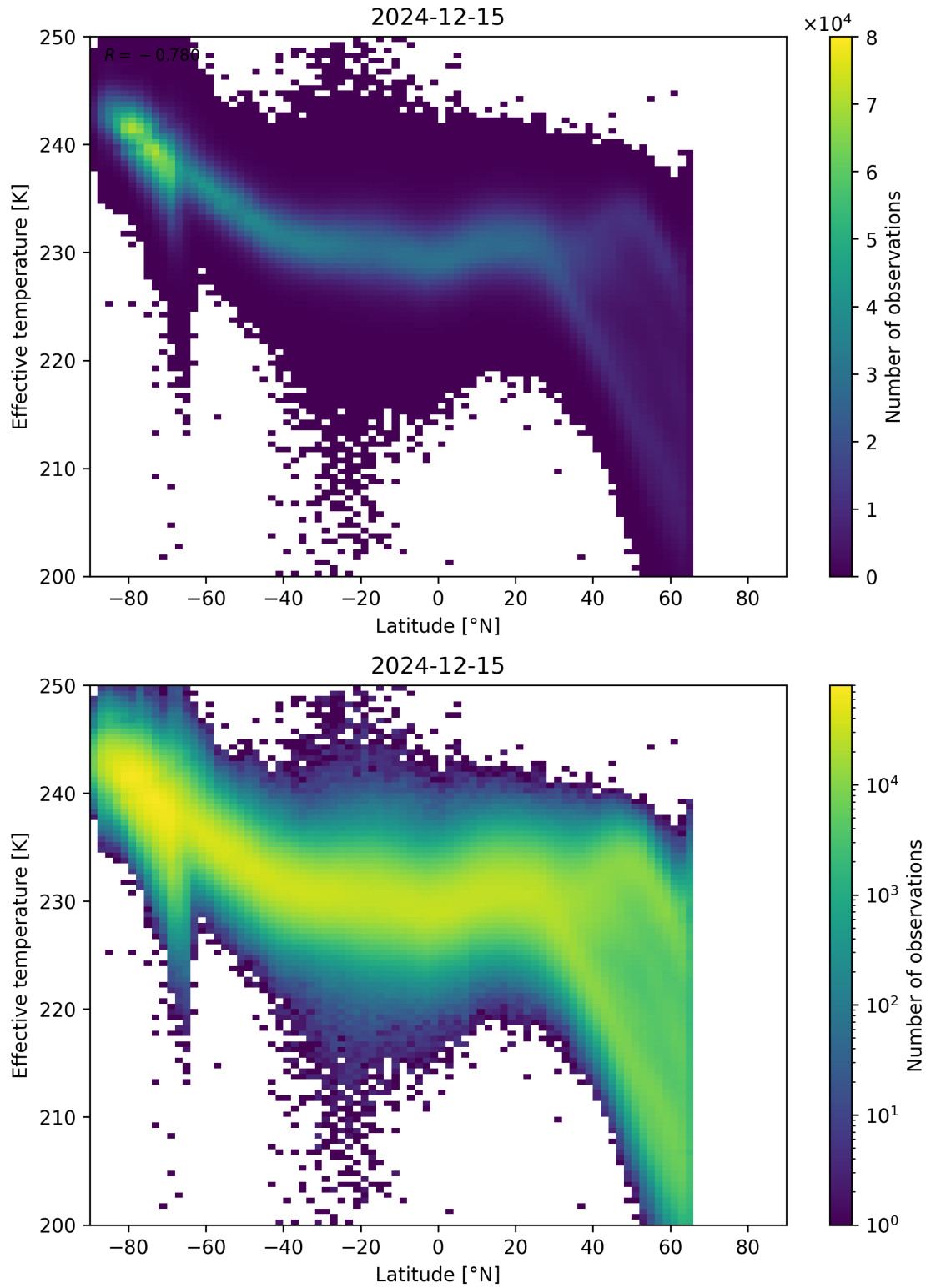
Figure 34: Scatter density plot of “Latitude” against “Effective temperature” for 2024-12-14 to 2024-12-16.
