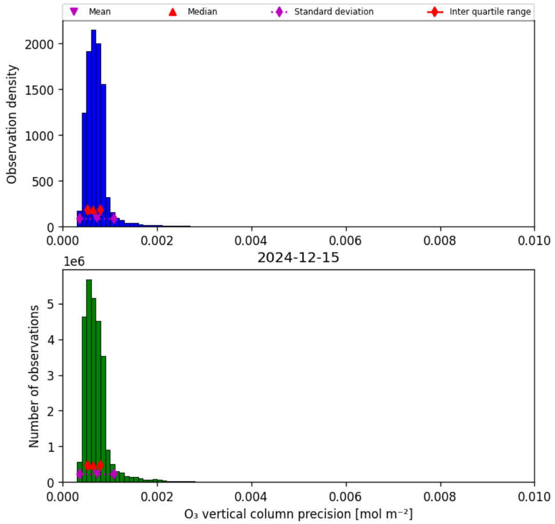
Figure 22: Histogram of “O 3 vertical column precision” for 2024-12-14 to 2024-12-16
