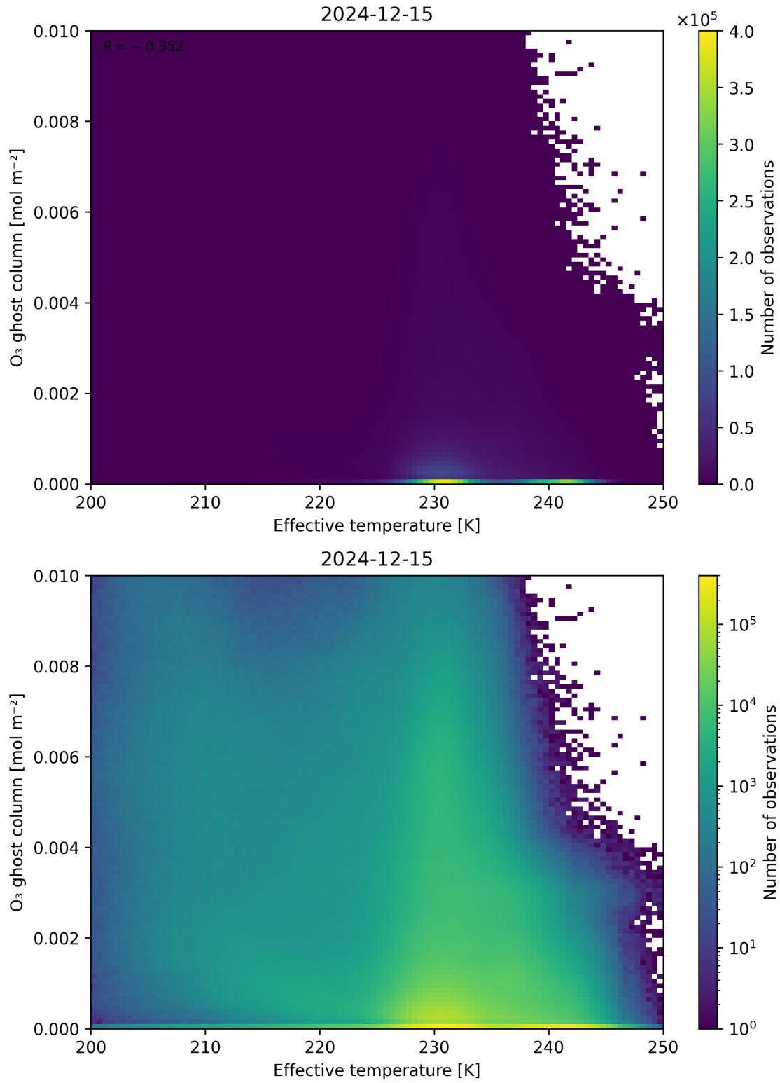
Figure 38: Scatter density plot of “Effective temperature” against “O 3 ghost column” for 2024-12-14 to 2024-12-16.
