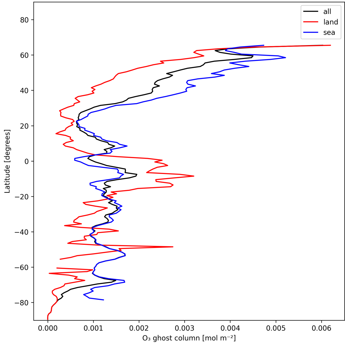
Figure 18: Zonal average of "O 3 ghost column" for 2024-12-14 to 2024-12-16.
