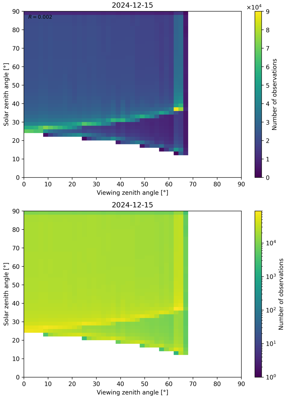
Figure 54: Scatter density plot of “Viewing zenith angle” against “Solar zenith angle” for 2024-12-14 to 2024-12-16.
