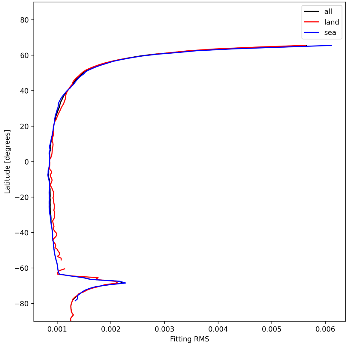
Figure 16: Zonal average of “Fitting RMS” for 2024-12-14 to 2024-12-16.
