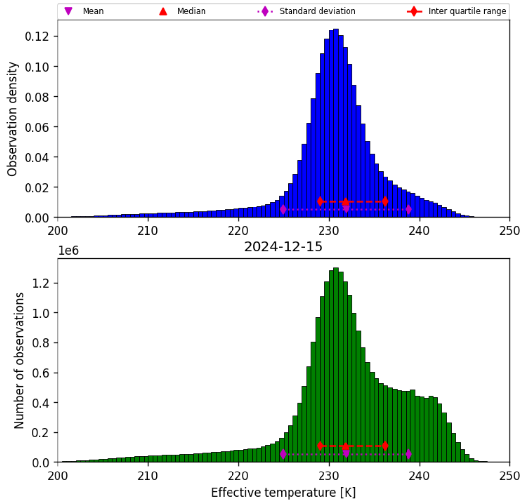
Figure 24: Histogram of “Effective temperature” for 2024-12-14 to 2024-12-16
