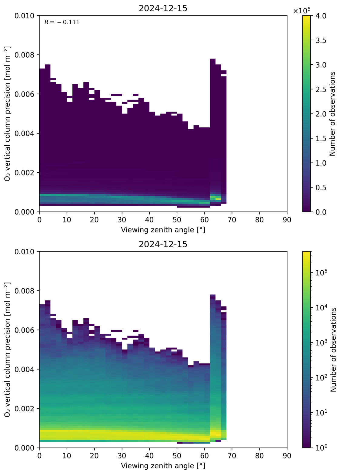
Figure 53: Scatter density plot of “Viewing zenith angle” against “O 3 vertical column precision” for 2024-12-14 to 2024-12-16.
