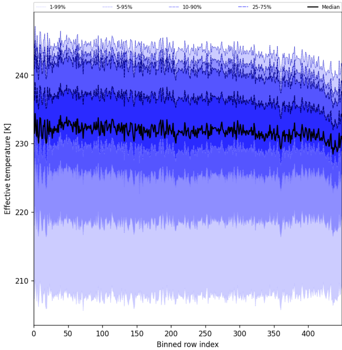
Figure 31: Along track statistics of “Effective temperature” for 2024-12-14 to 2024-12-16
