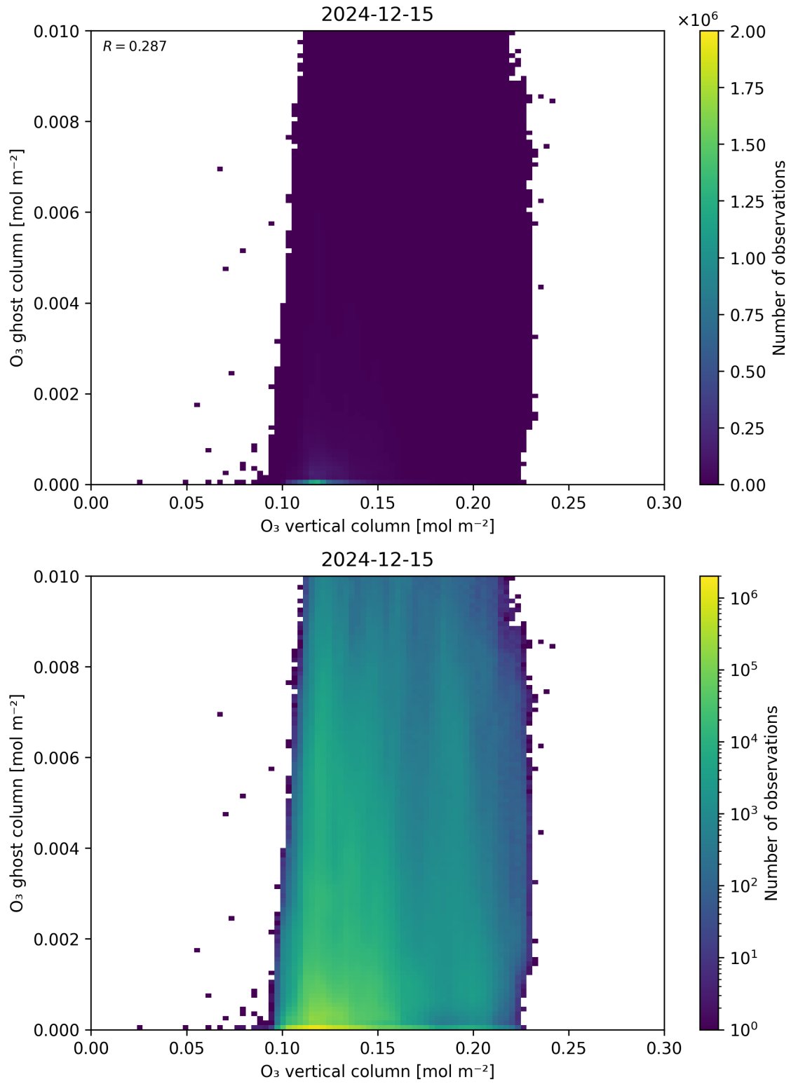
Figure 40: Scatter density plot of “O 3 vertical column” against “O 3 ghost column” for 2024-12-14 to 2024-12-16.
