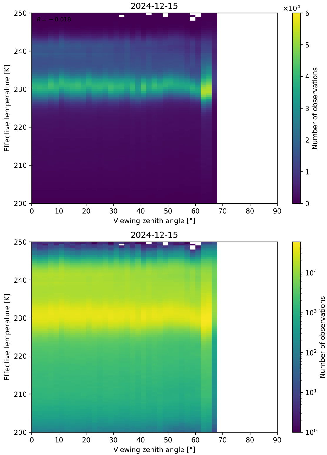
Figure 50: Scatter density plot of “Viewing zenith angle” against “Effective temperature” for 2024-12-14 to 2024-12-16.
