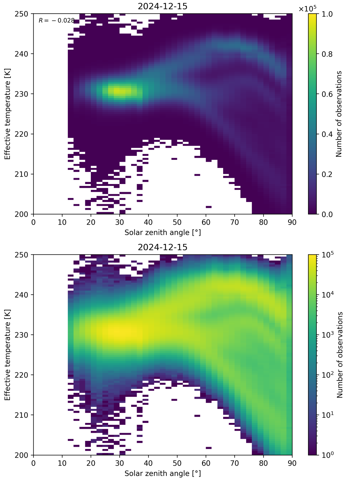
Figure 45: Scatter density plot of “Solar zenith angle” against “Effective temperature” for 2024-12-14 to 2024-12-16.
