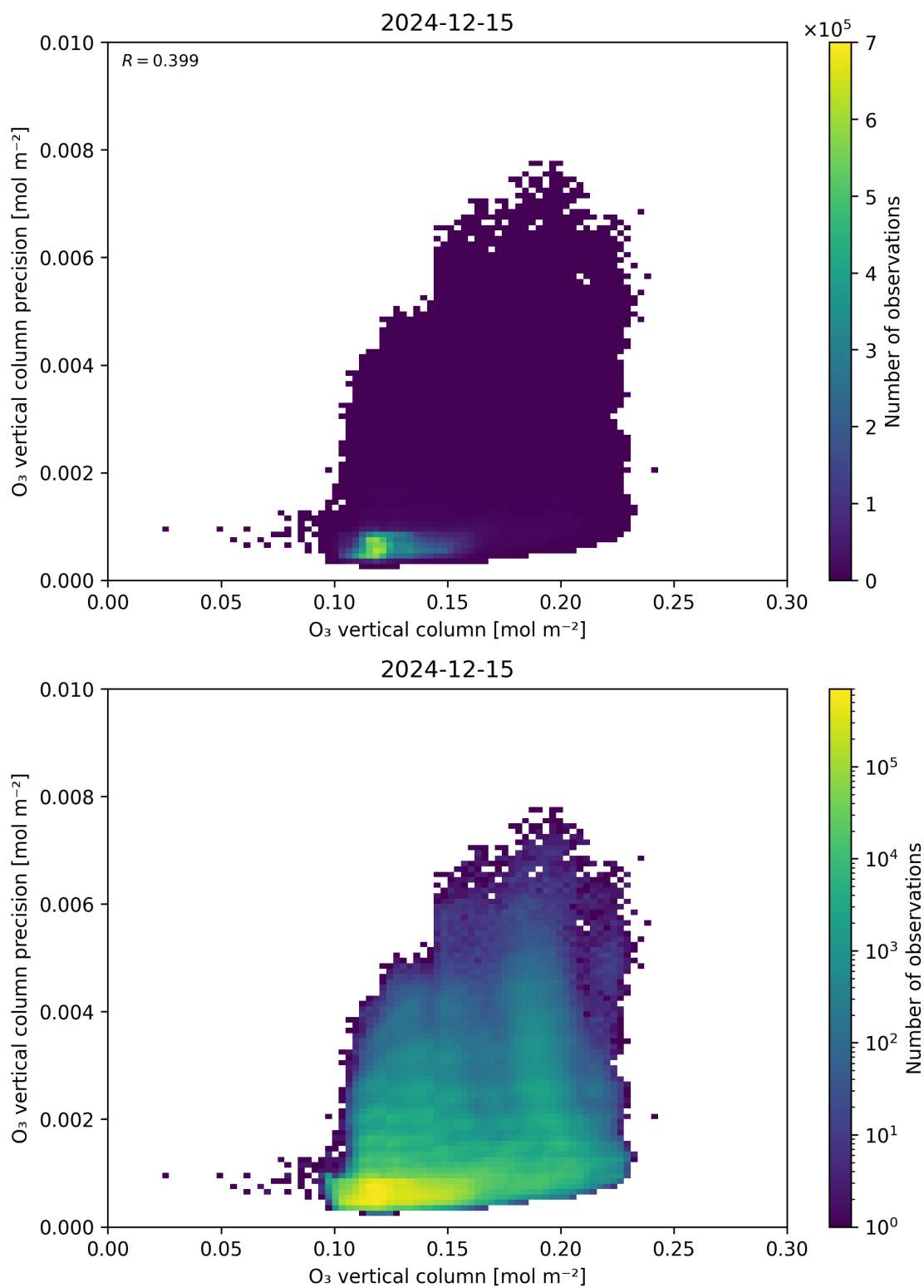
Figure 41: Scatter density plot of “O 3 vertical column” against “O 3 vertical column precision” for 2024-12-14 to 2024-12-16.
