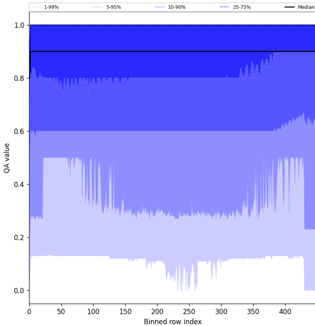
Figure 27: Along track statistics of “QA value” for 2024-12-14 to 2024-12-16
