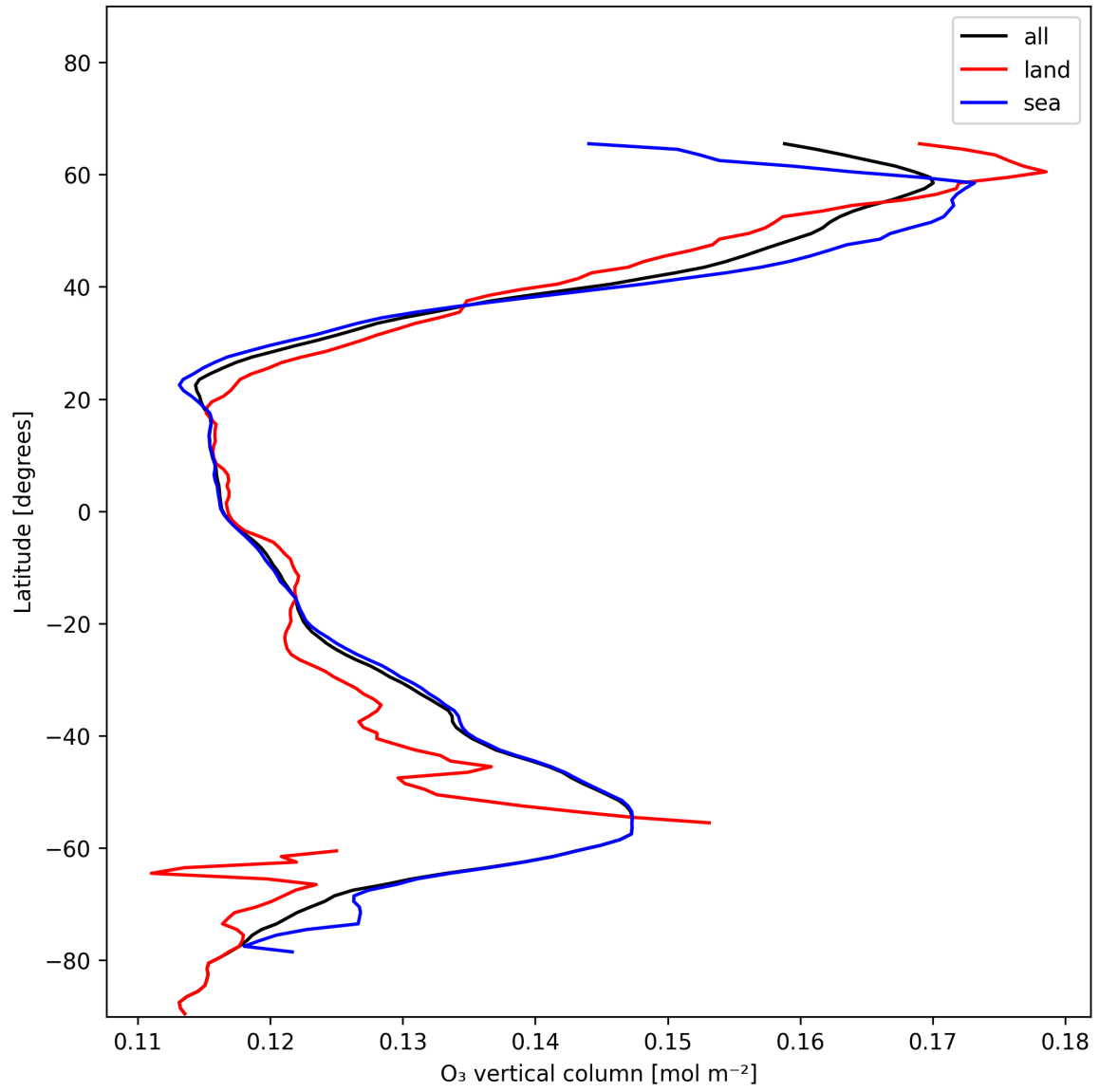
Figure 14: Zonal average of “O 3 vertical column” for 2024-12-14 to 2024-12-16.
