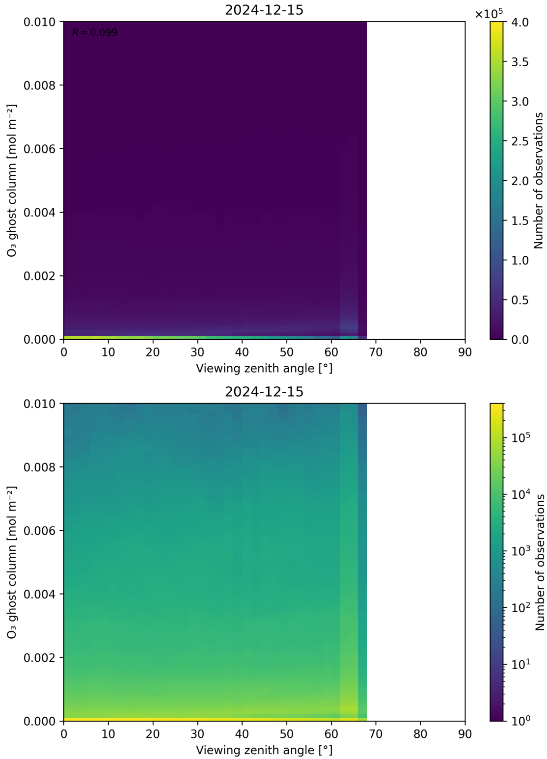
Figure 51: Scatter density plot of “Viewing zenith angle” against “O 3 ghost column” for 2024-12-14 to 2024-12-16.
