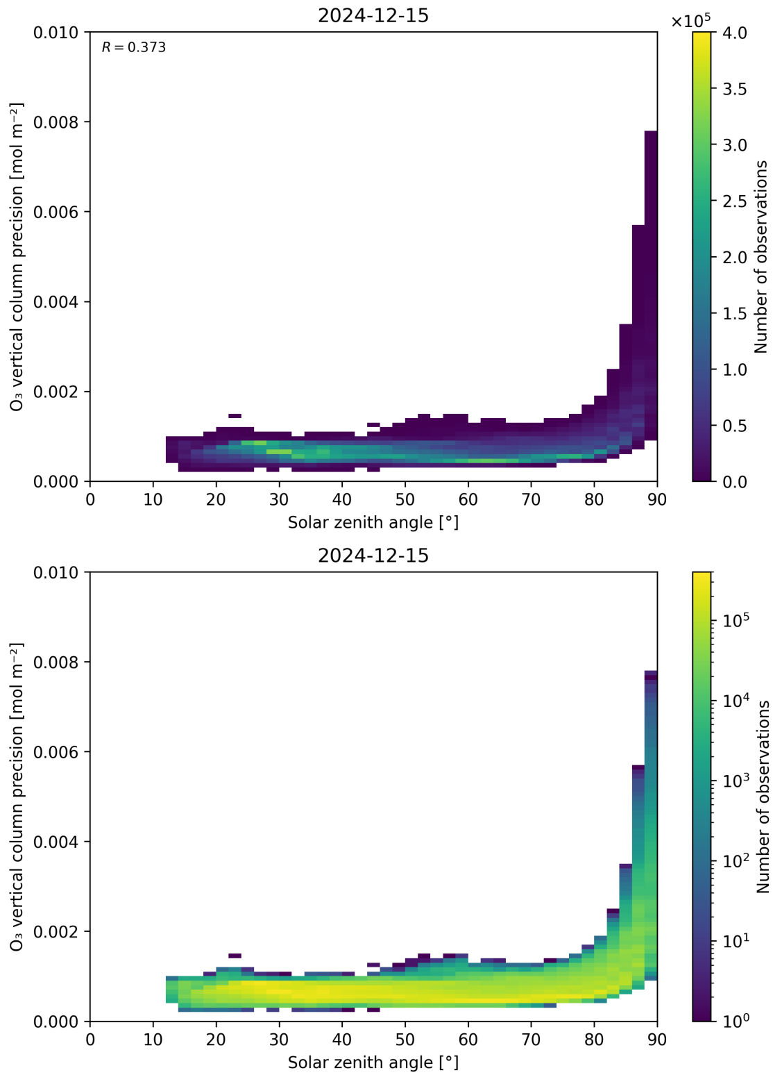
Figure 48: Scatter density plot of “Solar zenith angle” against “O 3 vertical column precision” for 2024-12-14 to 2024-12-16.
