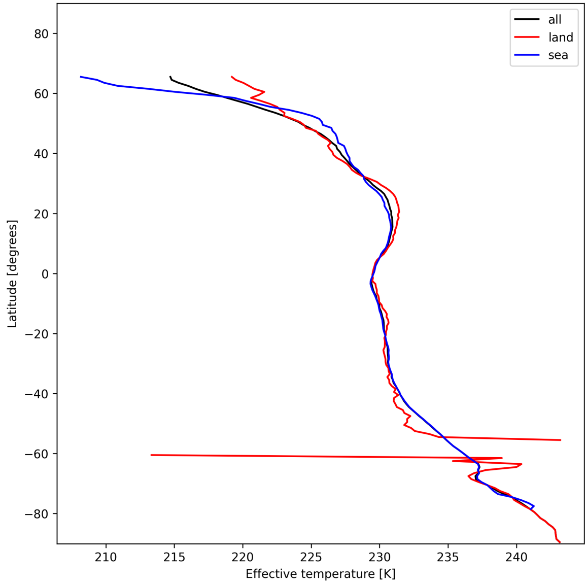
Figure 17: Zonal average of “Effective temperature” for 2024-12-14 to 2024-12-16.
