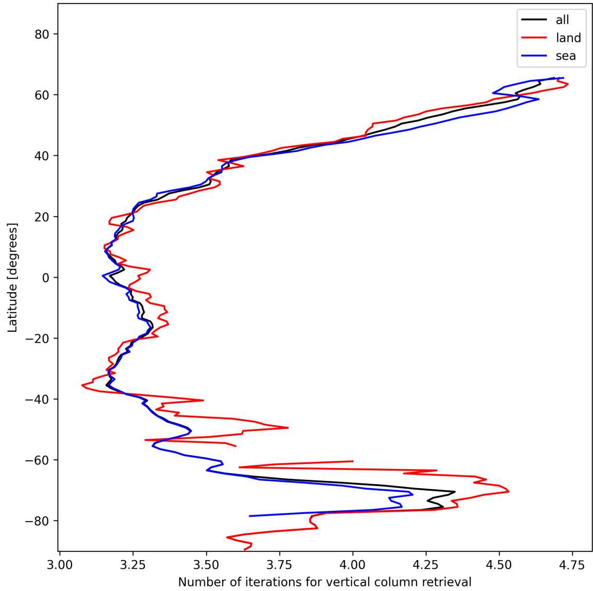
Figure 19: Zonal average of “Number of iterations for vertical column retrieval” for 2024-12-14 to 2024-12-16.
