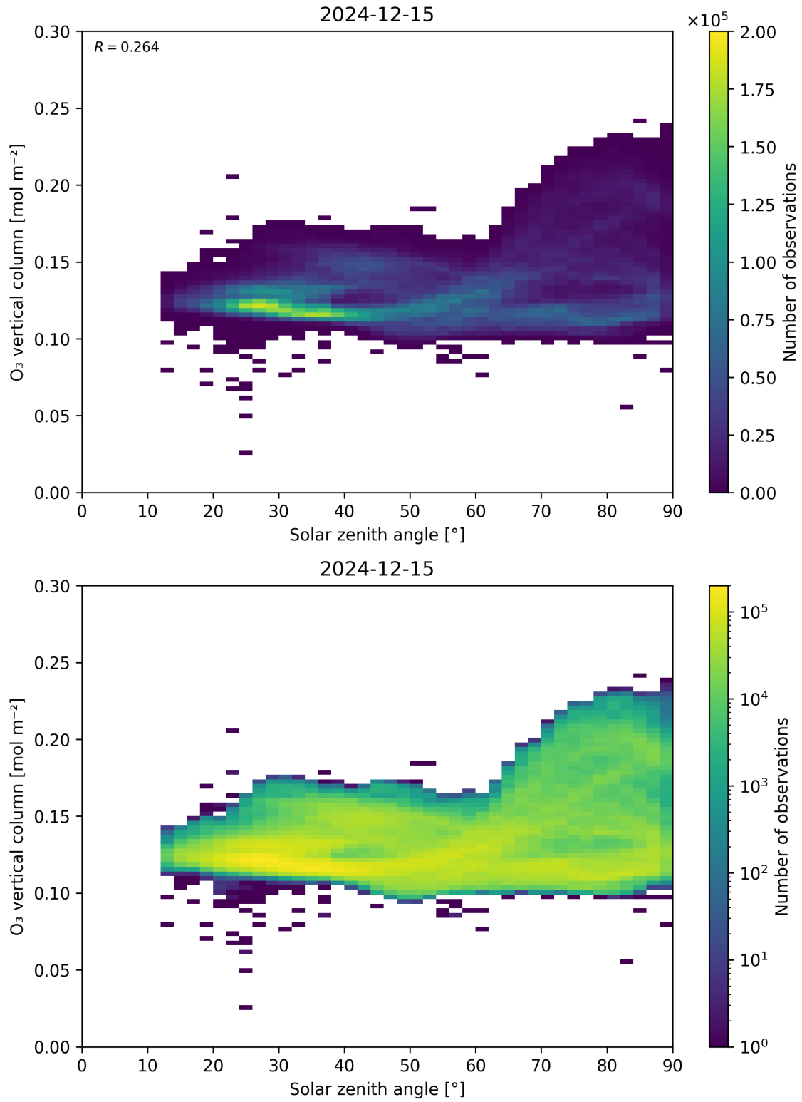
Figure 47: Scatter density plot of “Solar zenith angle” against “O 3 vertical column” for 2024-12-14 to 2024-12-16.
