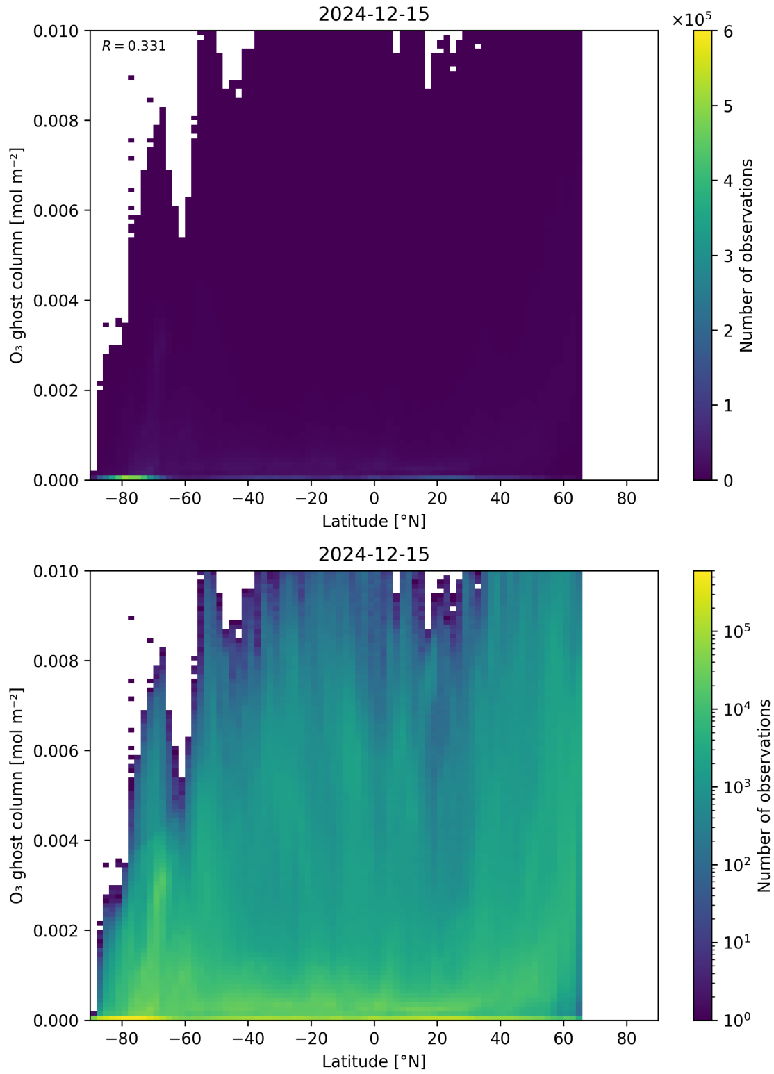
Figure 35: Scatter density plot of “Latitude” against “O 3 ghost column” for 2024-12-14 to 2024-12-16.
