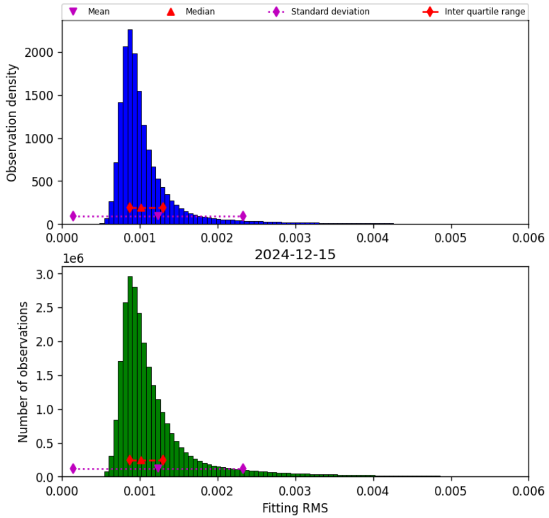
Figure 23: Histogram of “Fitting RMS” for 2024-12-14 to 2024-12-16
