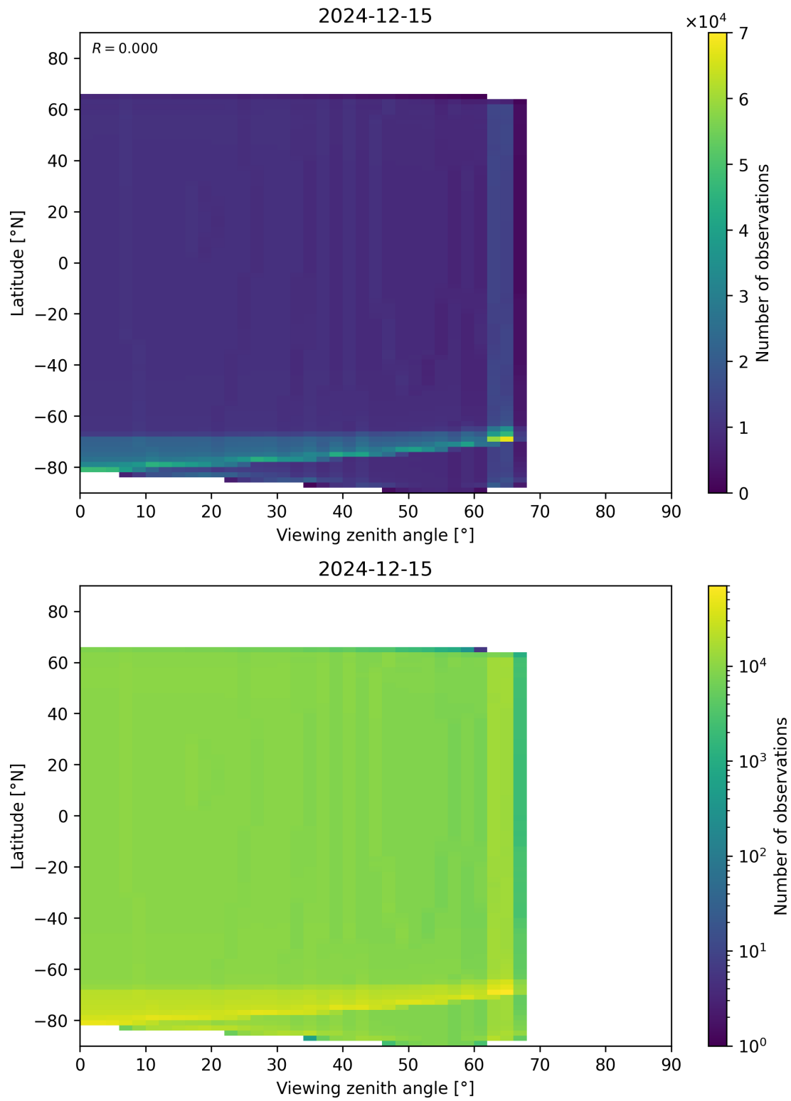
Figure 49: Scatter density plot of “Viewing zenith angle” against “Latitude” for 2024-12-14 to 2024-12-16.
