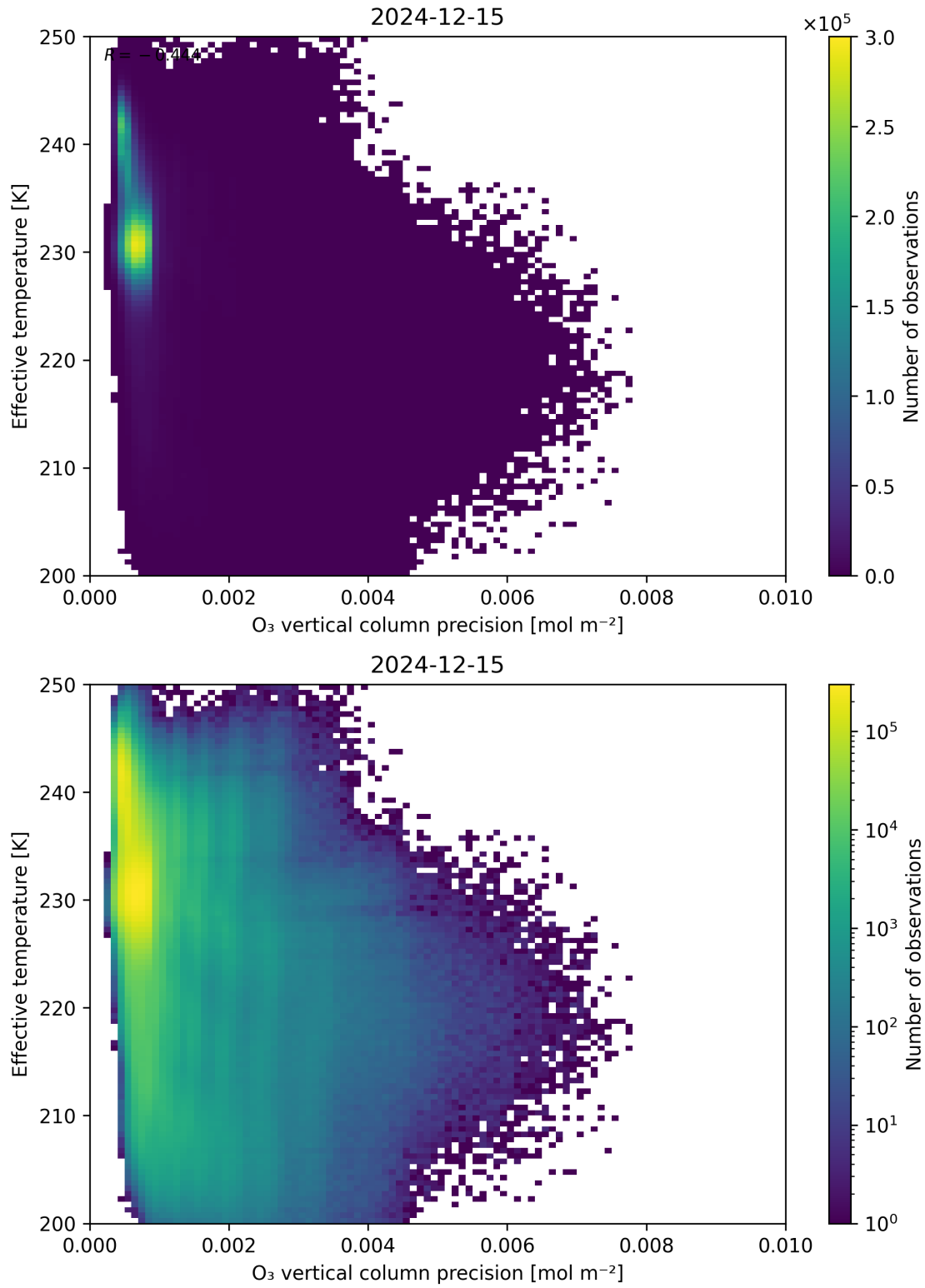
Figure 42: Scatter density plot of “O 3 vertical column precision” against “Effective temperature” for 2024-12-14 to 2024-12-16.
