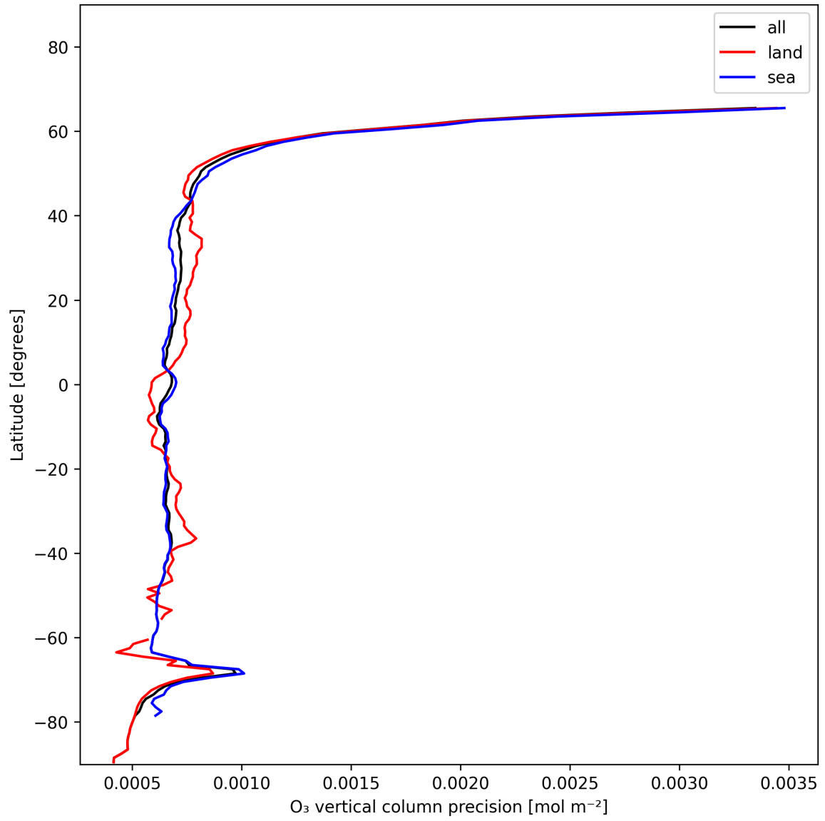
Figure 15: Zonal average of “O 3 vertical column precision” for 2024-12-14 to 2024-12-16.
