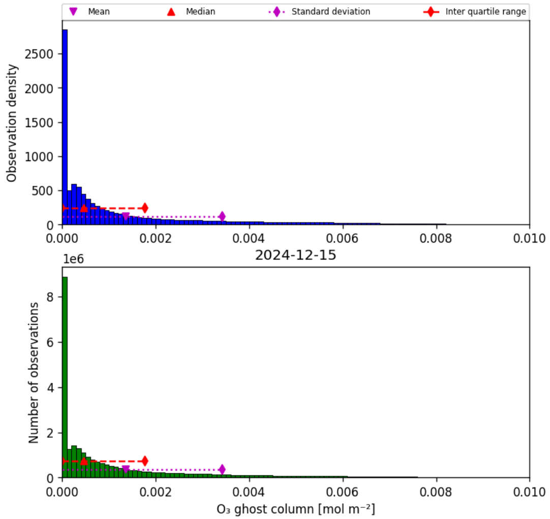
Figure 25: Histogram of "O 3 ghost column" for 2024-12-14 to 2024-12-16
