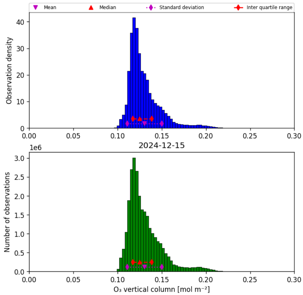
Figure 21: Histogram of “O 3 vertical column” for 2024-12-14 to 2024-12-16
