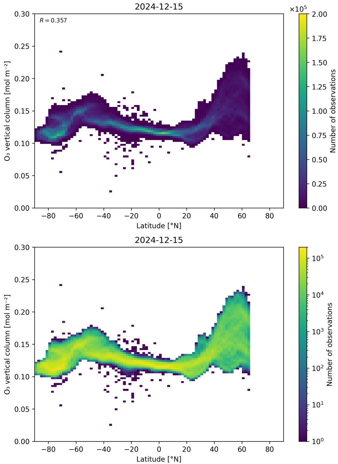
Figure 36: Scatter density plot of “Latitude” against “O 3 vertical column” for 2024-12-14 to 2024-12-16.
