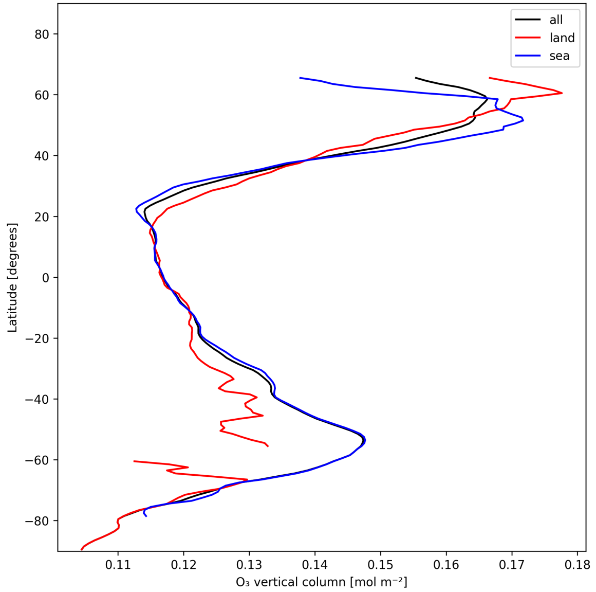
Figure 14: Zonal average of “O 3 vertical column” for 2024-12-16 to 2024-12-17.
