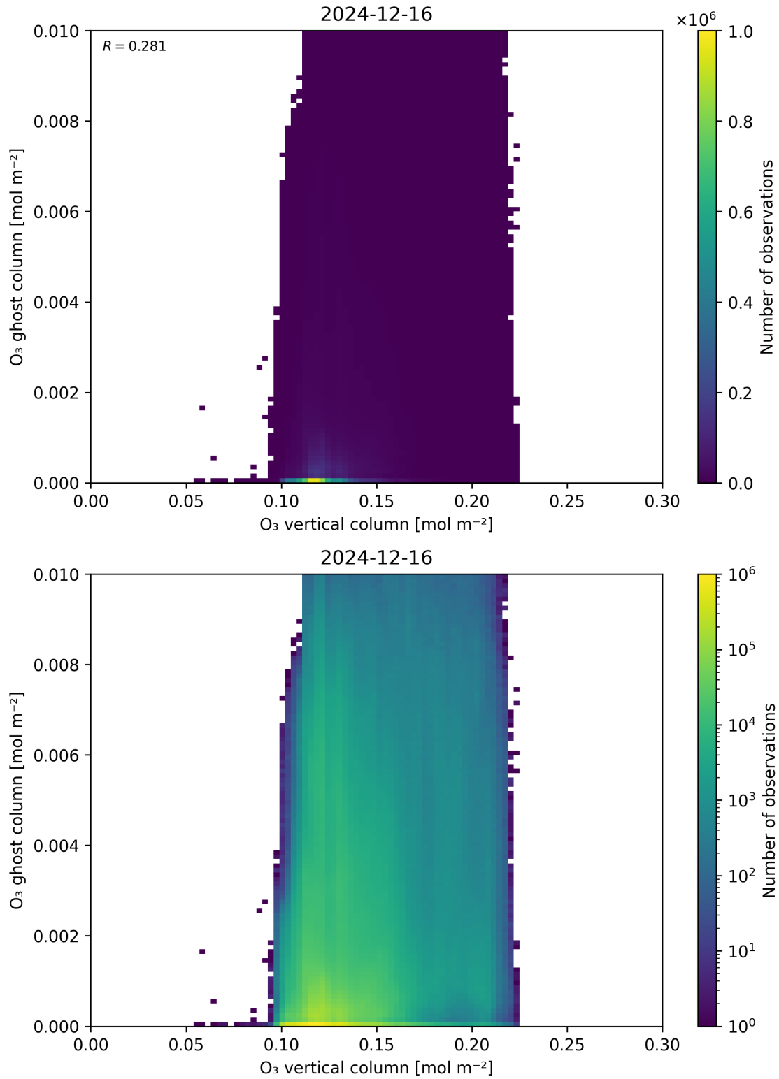
Figure 40: Scatter density plot of “O 3 vertical column” against “O 3 ghost column” for 2024-12-16 to 2024-12-17.
