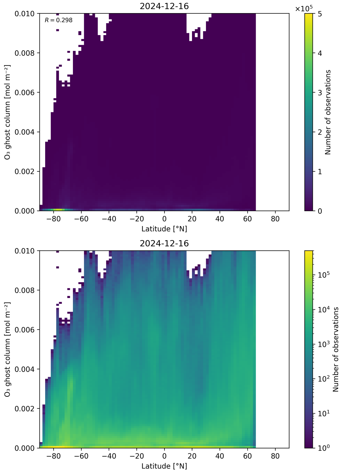
Figure 35: Scatter density plot of “Latitude” against “O 3 ghost column” for 2024-12-16 to 2024-12-17.
