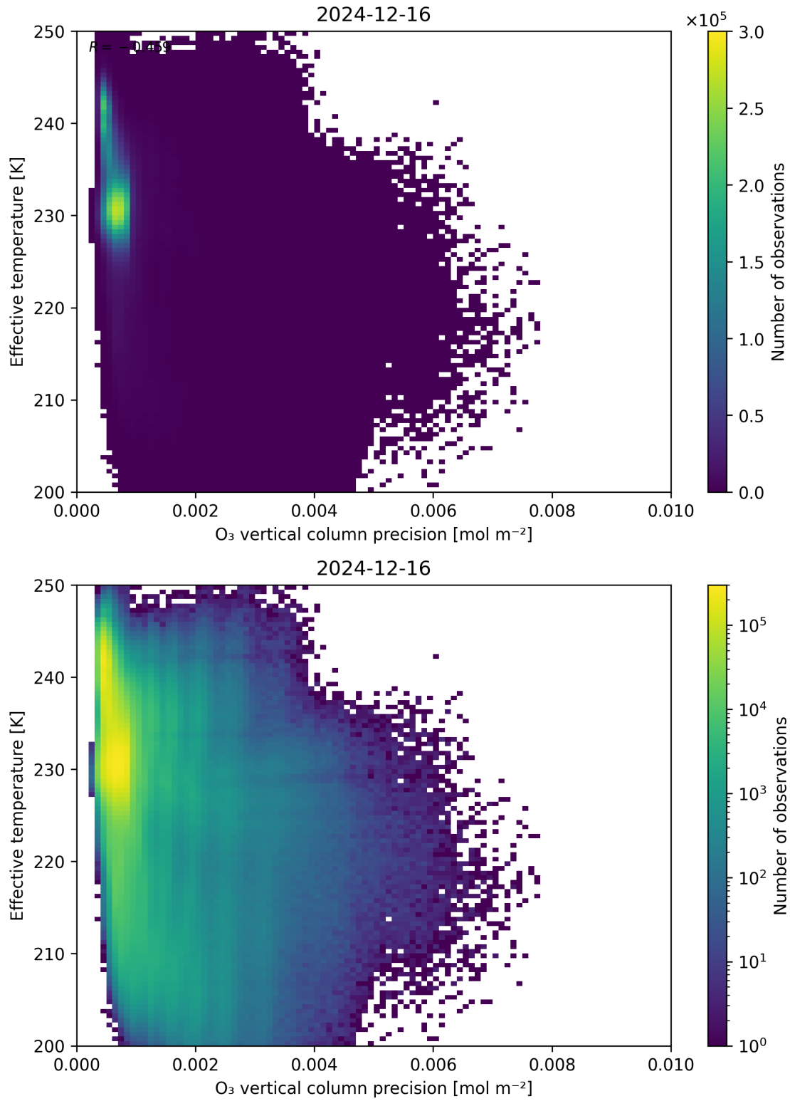
Figure 42: Scatter density plot of “O 3 vertical column precision” against “Effective temperature” for 2024-12-16 to 2024-12-17.
