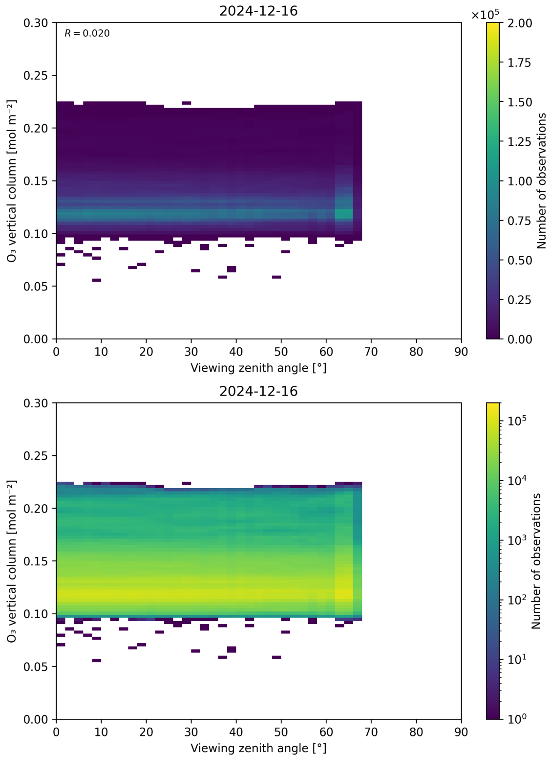
Figure 52: Scatter density plot of “Viewing zenith angle” against “O 3 vertical column” for 2024-12-16 to 2024-12-17.
