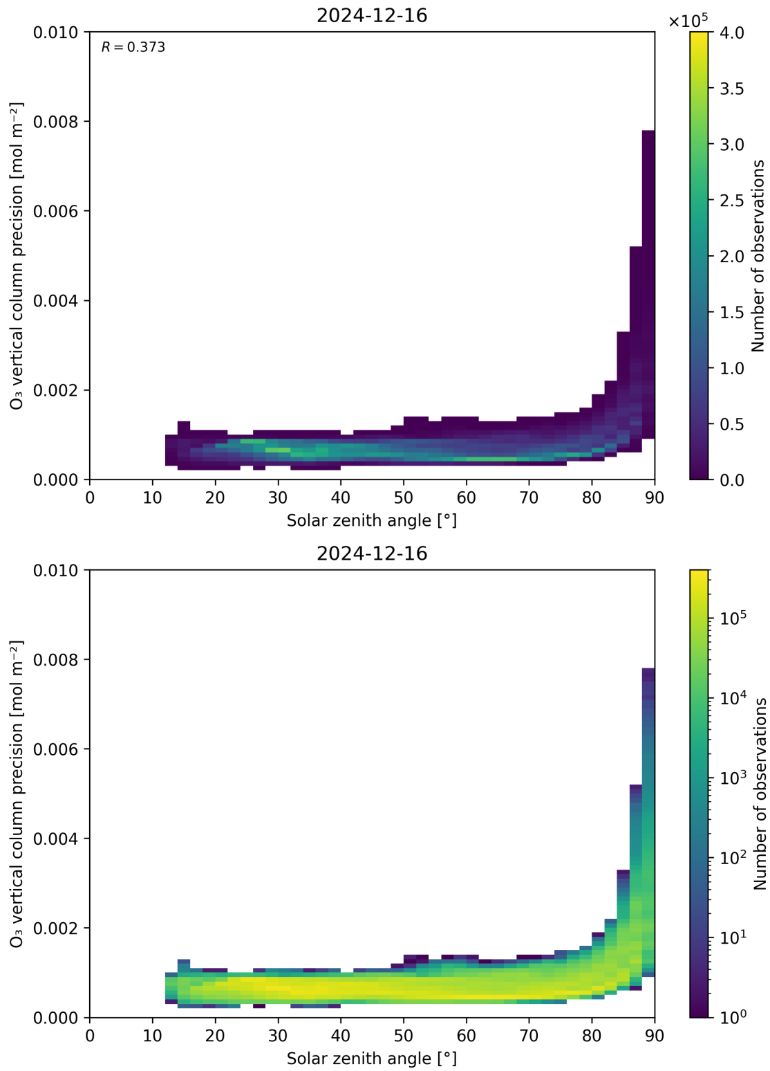
Figure 48: Scatter density plot of “Solar zenith angle” against “O 3 vertical column precision” for 2024-12-16 to 2024-12-17.
