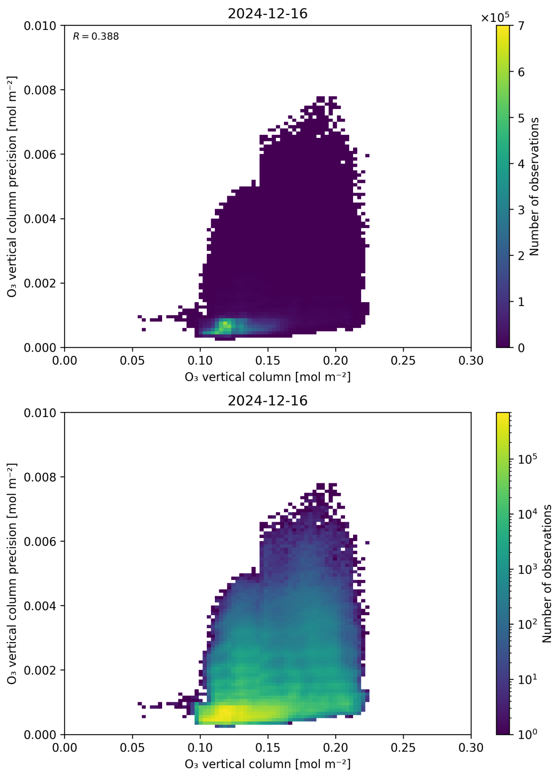
Figure 41: Scatter density plot of “O 3 vertical column” against “O 3 vertical column precision” for 2024-12-16 to 2024-12-17.
