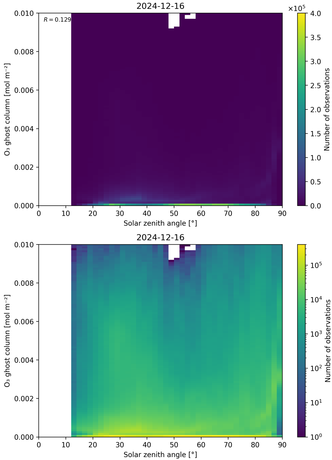
Figure 46: Scatter density plot of “Solar zenith angle” against “O 3 ghost column” for 2024-12-16 to 2024-12-17.
