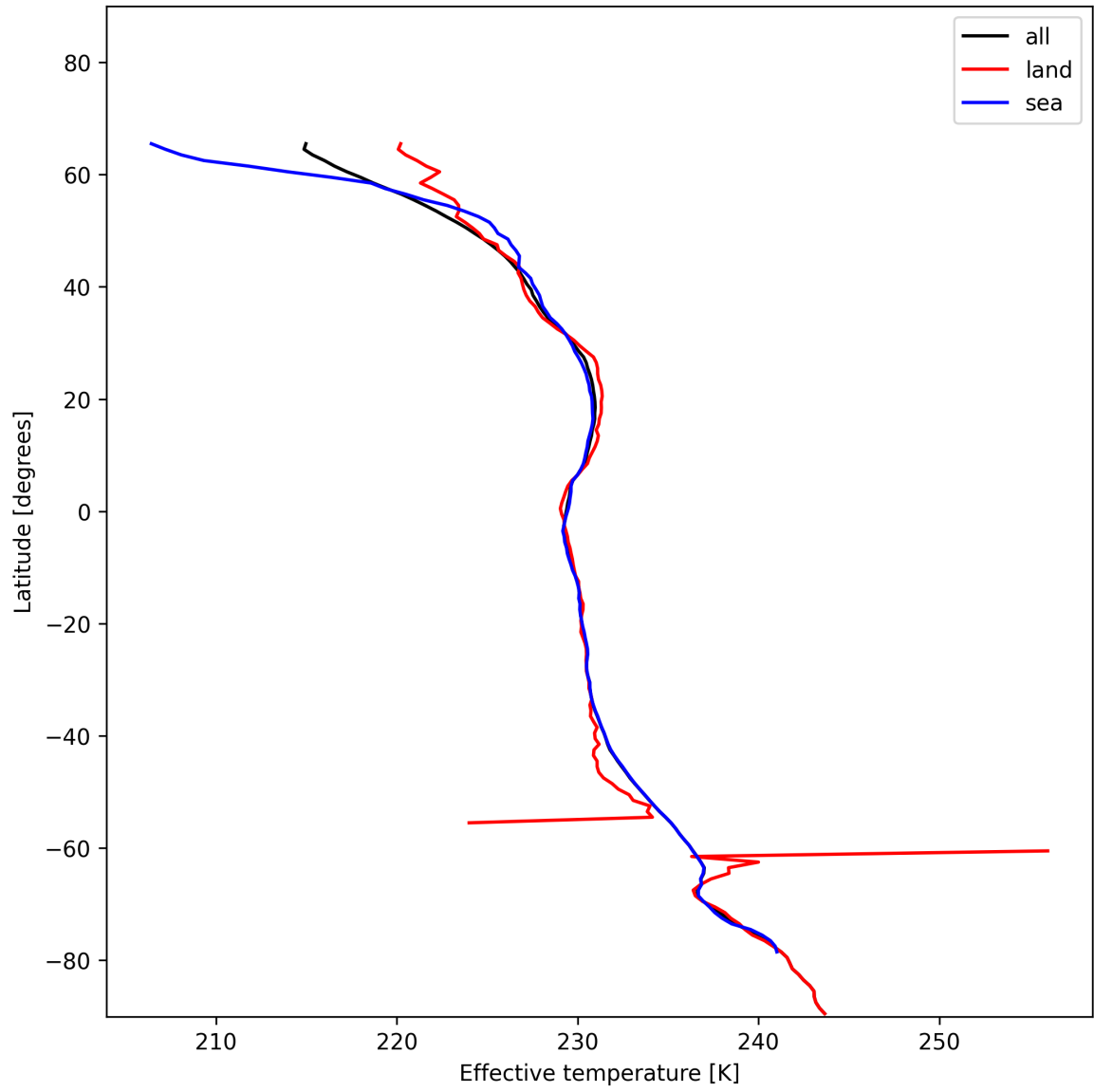
Figure 17: Zonal average of “Effective temperature” for 2024-12-16 to 2024-12-17.
