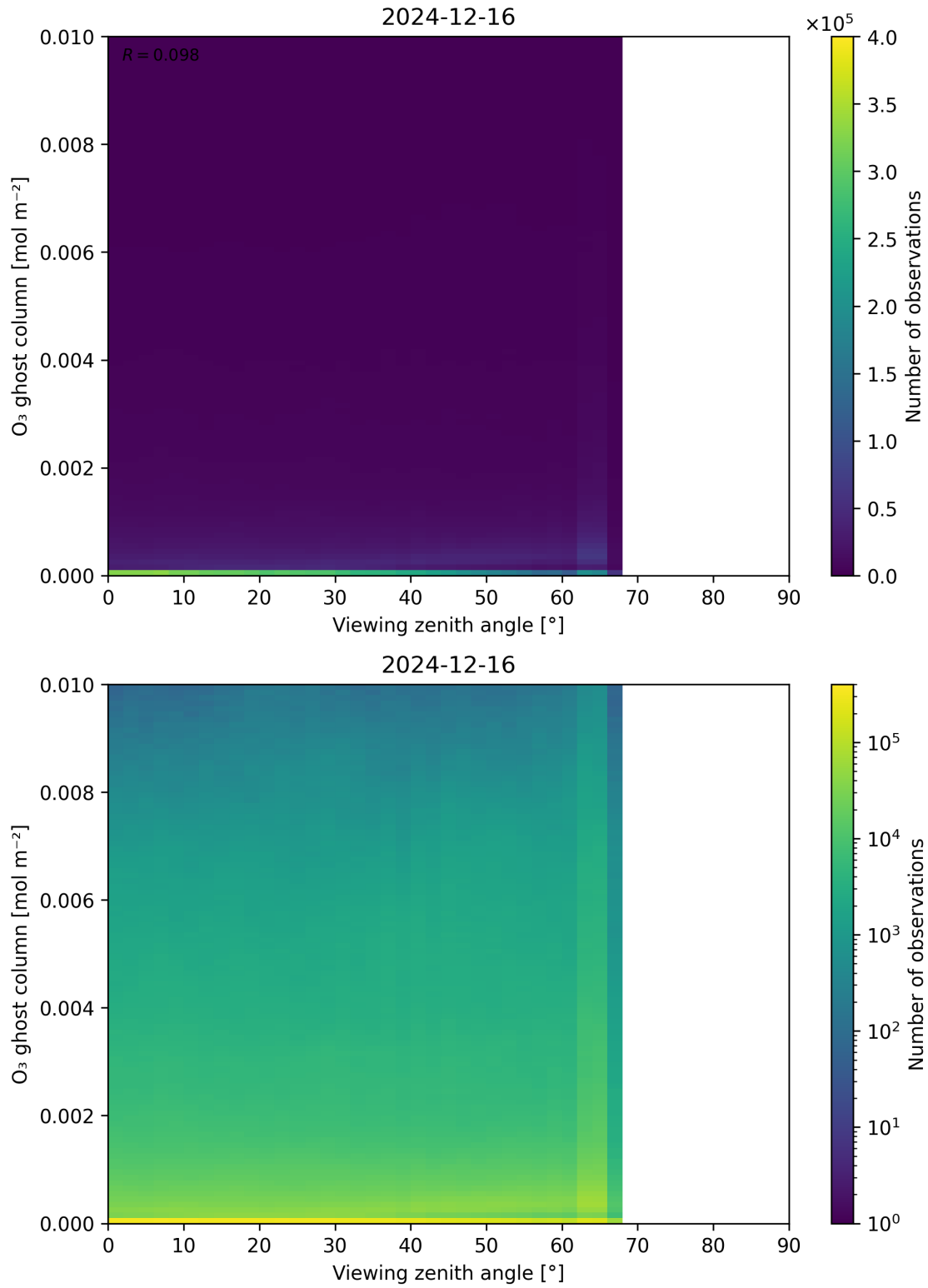
Figure 51: Scatter density plot of “Viewing zenith angle” against “O 3 ghost column” for 2024-12-16 to 2024-12-17.
