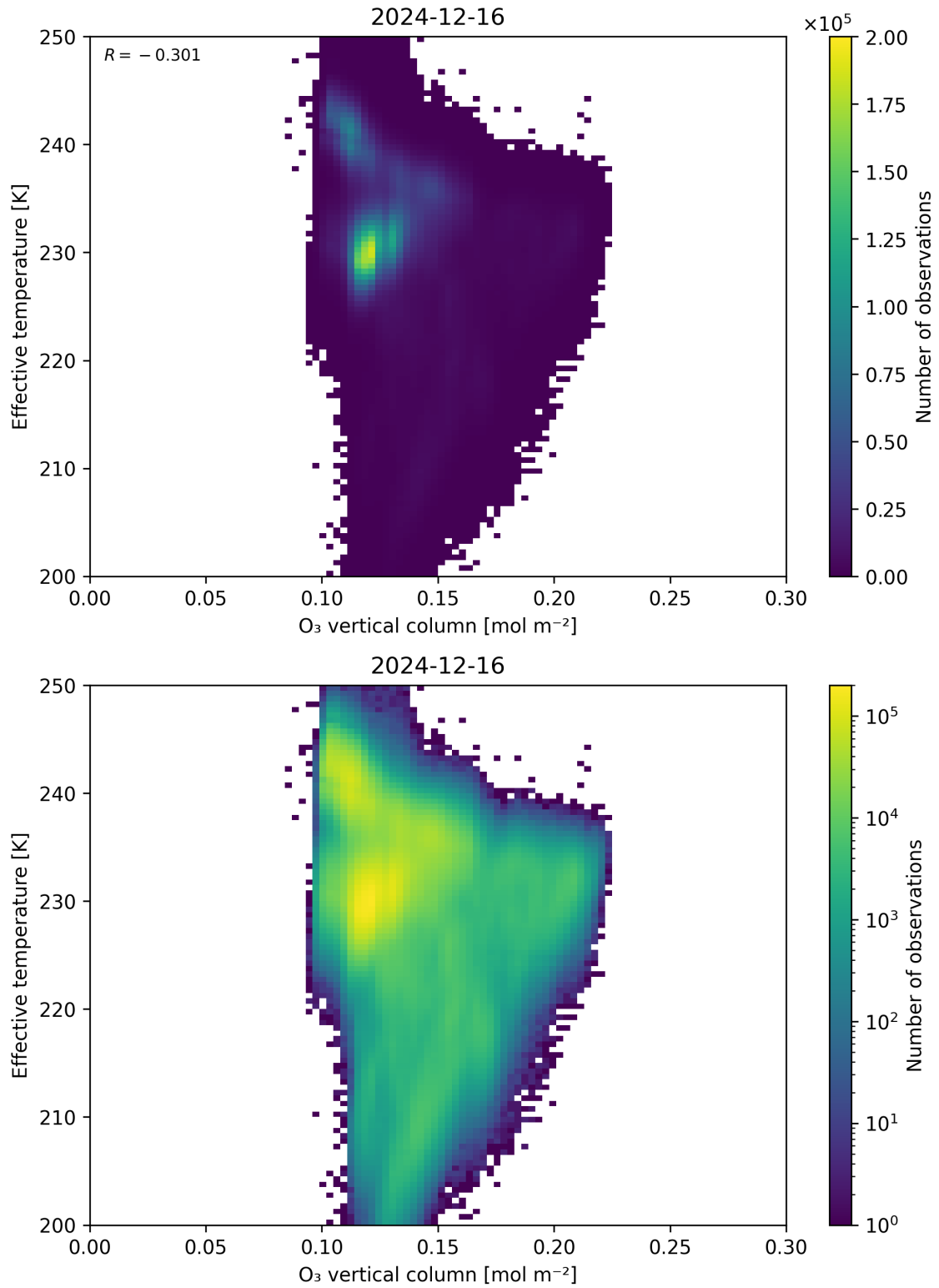
Figure 39: Scatter density plot of “O 3 vertical column” against “Effective temperature” for 2024-12-16 to 2024-12-17.
