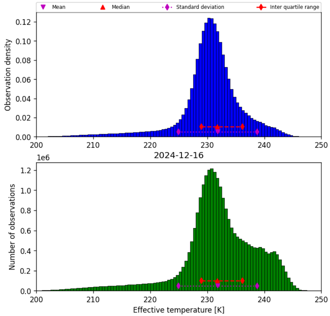
Figure 24: Histogram of “Effective temperature” for 2024-12-16 to 2024-12-17
