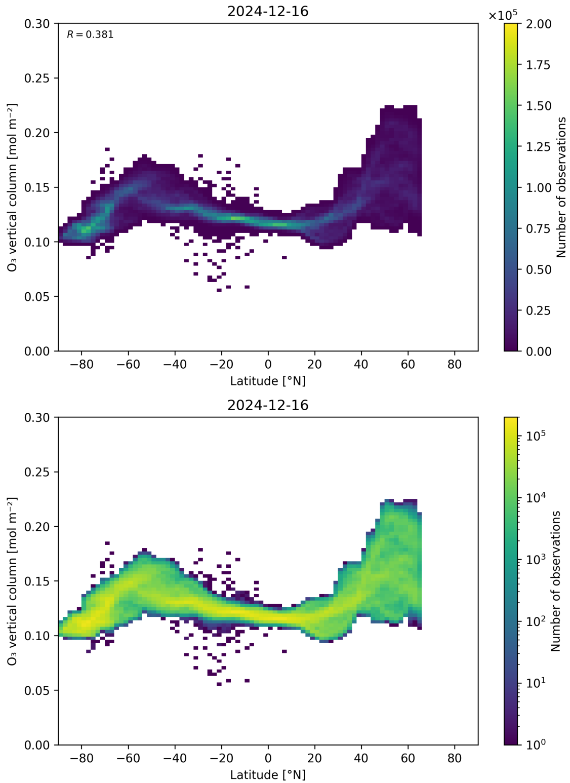
Figure 36: Scatter density plot of “Latitude” against “O 3 vertical column” for 2024-12-16 to 2024-12-17.
