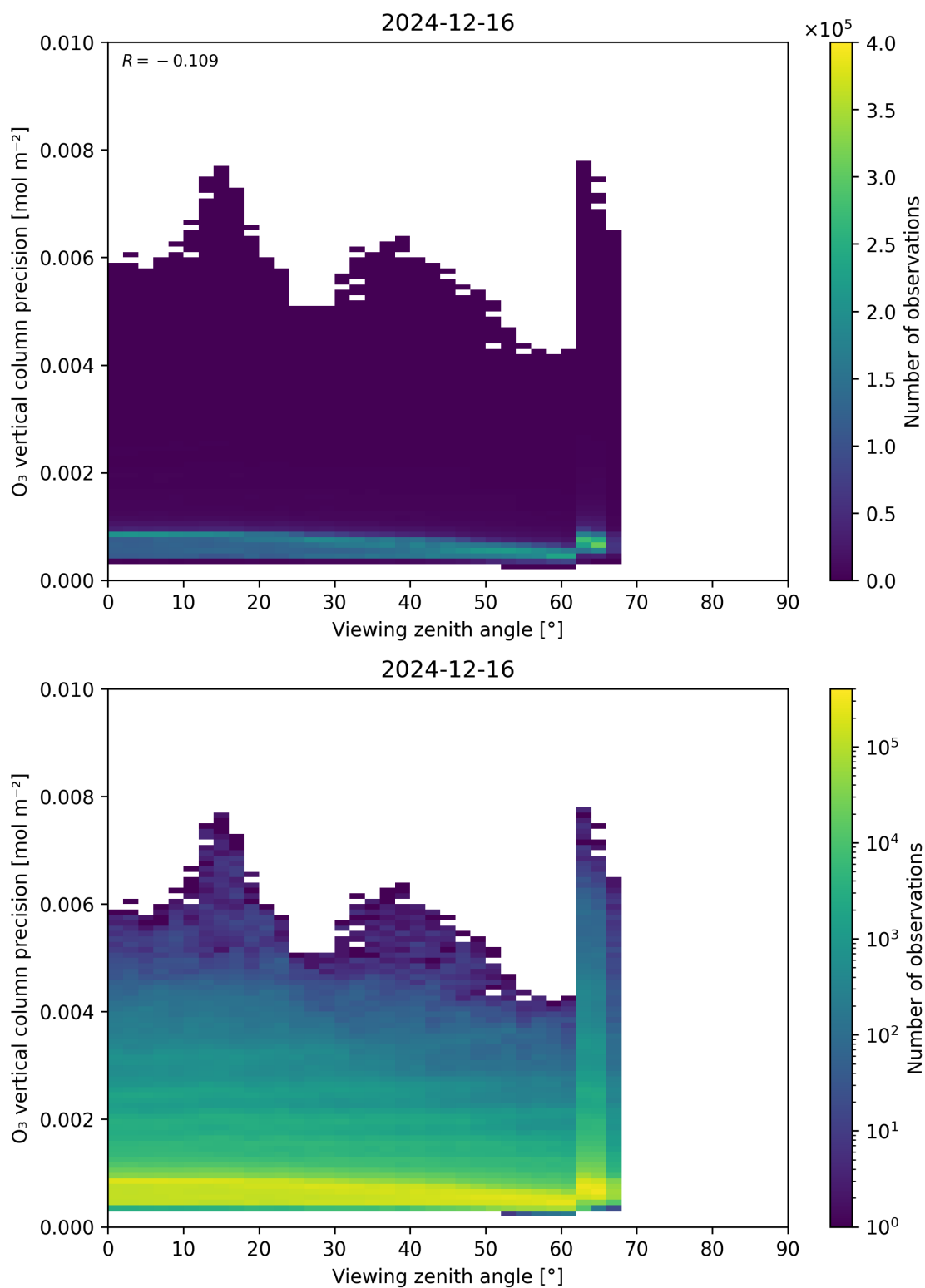
Figure 53: Scatter density plot of “Viewing zenith angle” against “O 3 vertical column precision” for 2024-12-16 to 2024-12-17.
