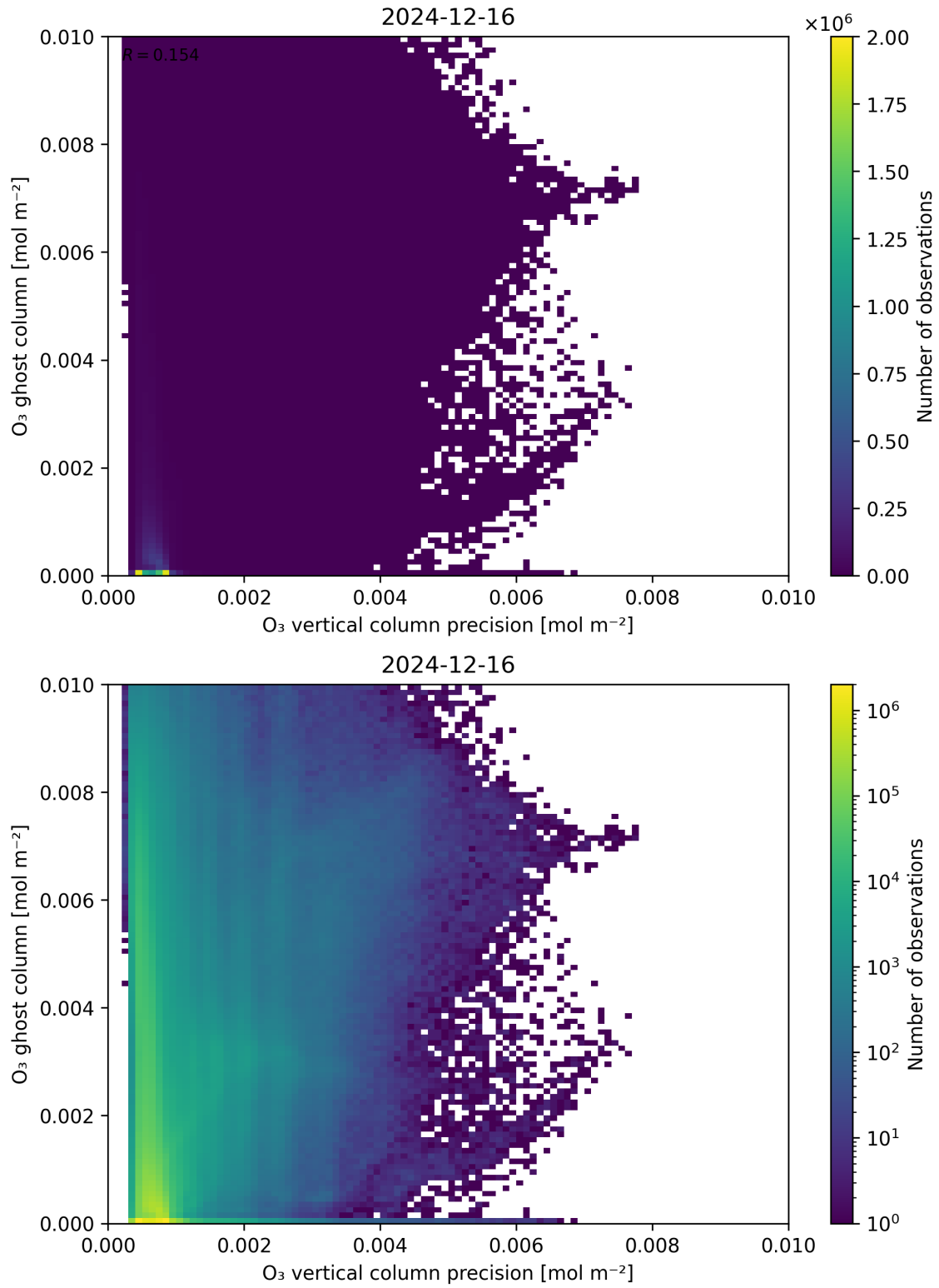
Figure 43: Scatter density plot of “ O_3 vertical column precision” against “ O_3 ghost column” for 2024-12-16 to 2024-12-17.
