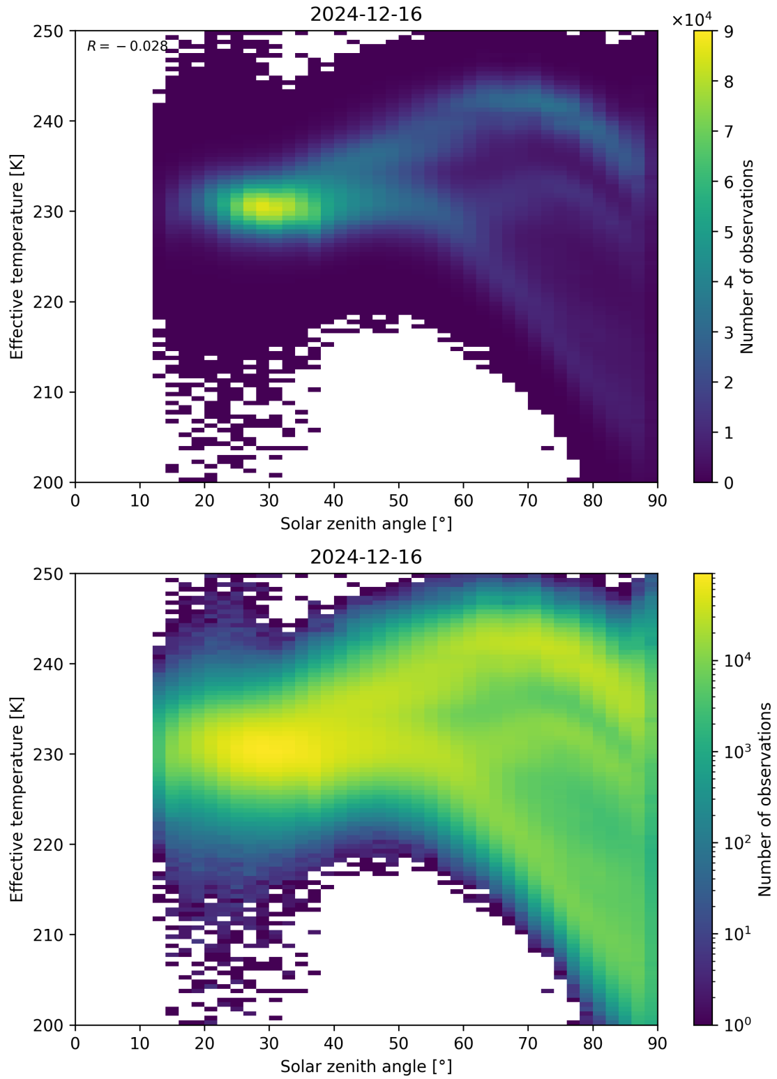
Figure 45: Scatter density plot of “Solar zenith angle” against “Effective temperature” for 2024-12-16 to 2024-12-17.
