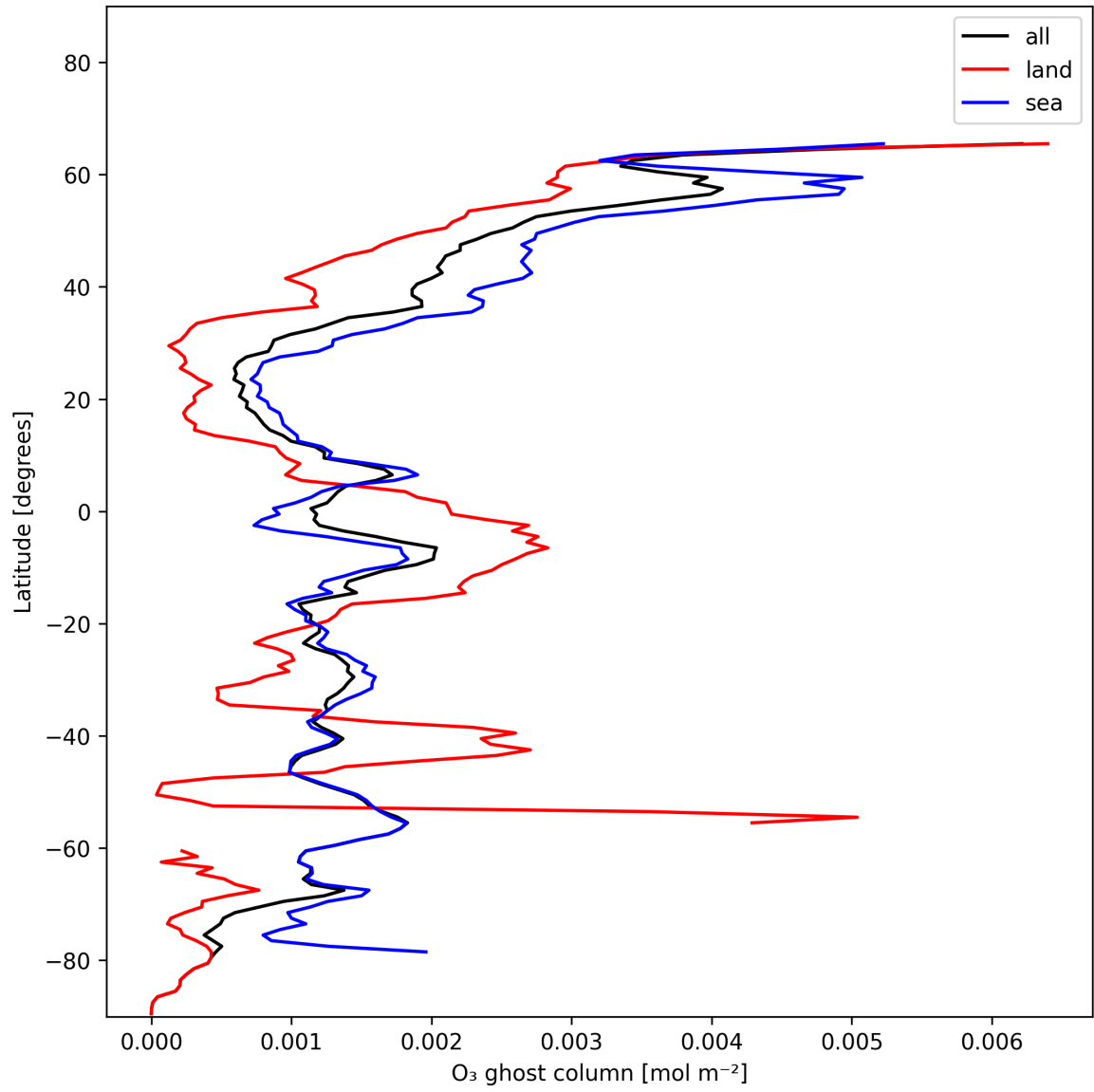
Figure 18: Zonal average of “O 3 ghost column” for 2024-12-16 to 2024-12-17.
