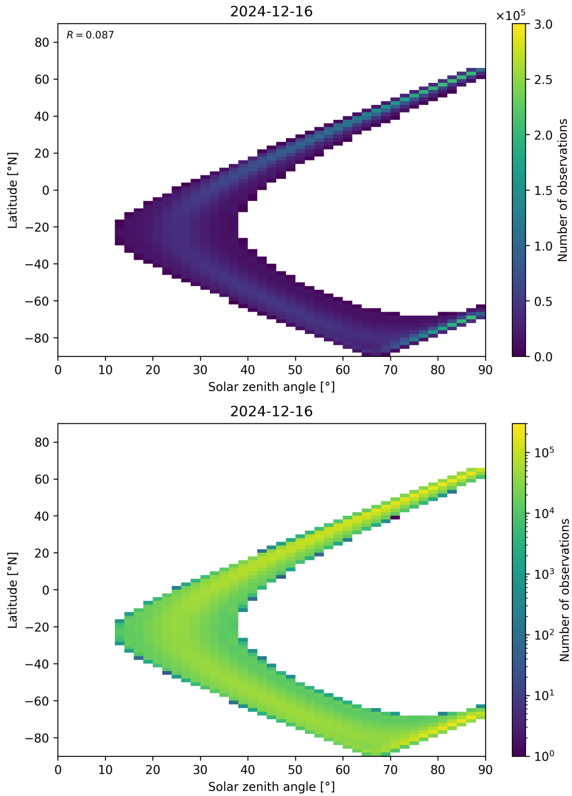
Figure 44: Scatter density plot of “Solar zenith angle” against “Latitude” for 2024-12-16 to 2024-12-17.
