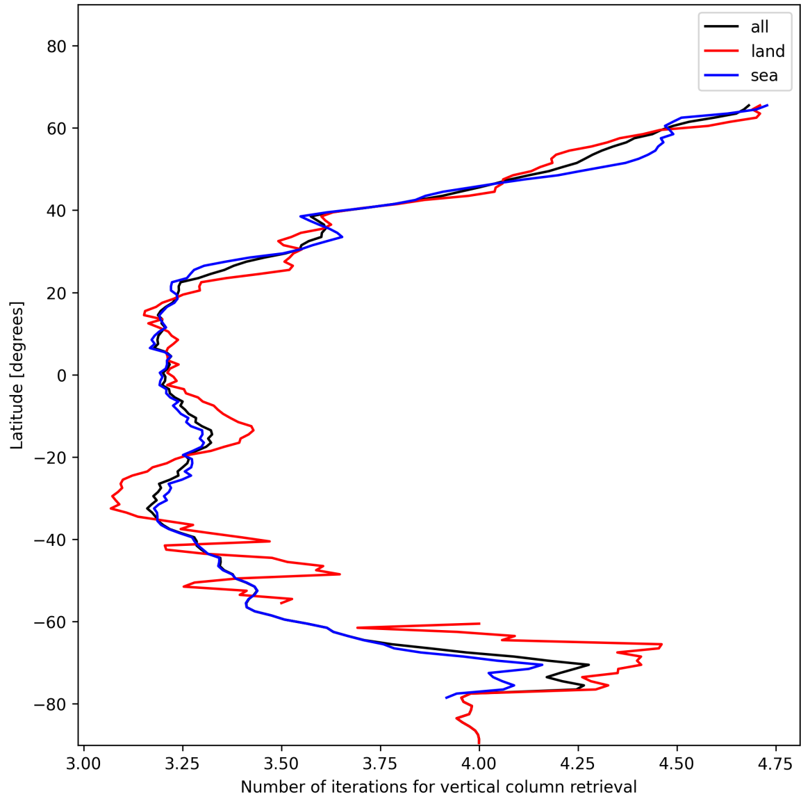
Figure 19: Zonal average of “Number of iterations for vertical column retrieval” for 2024-12-16 to 2024-12-17.
