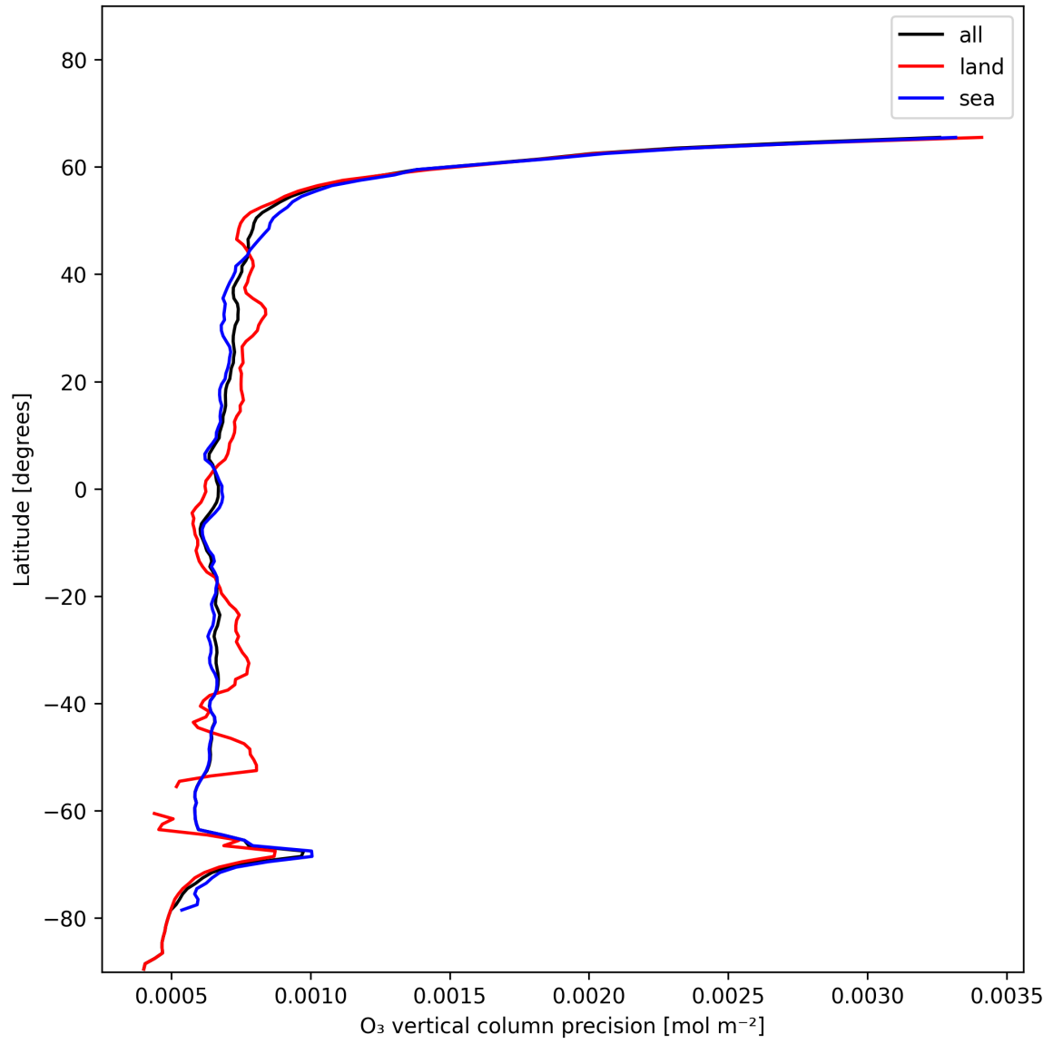
Figure 15: Zonal average of “O 3 vertical column precision” for 2024-12-16 to 2024-12-17.
