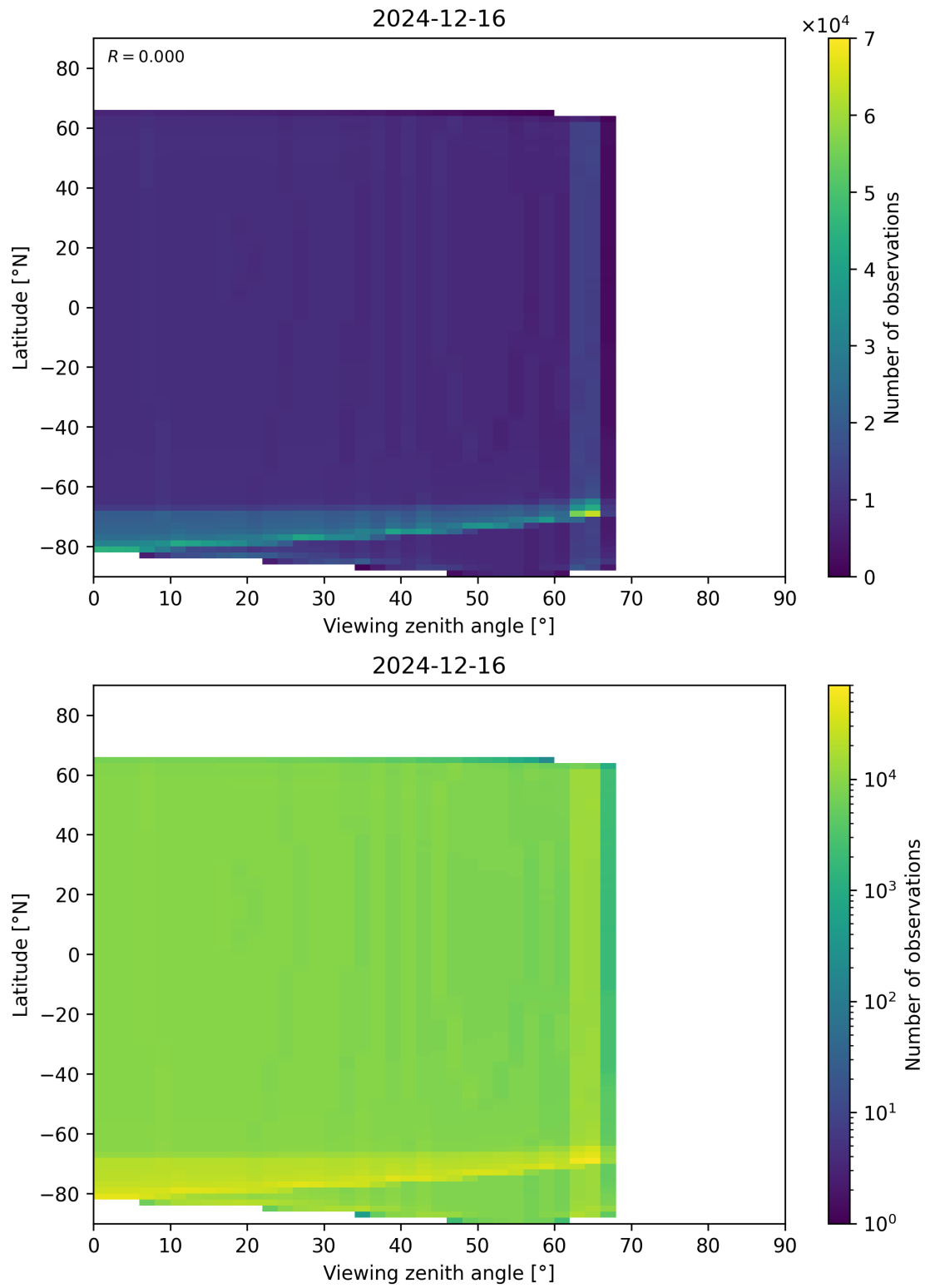
Figure 49: Scatter density plot of “Viewing zenith angle” against “Latitude” for 2024-12-16 to 2024-12-17.
