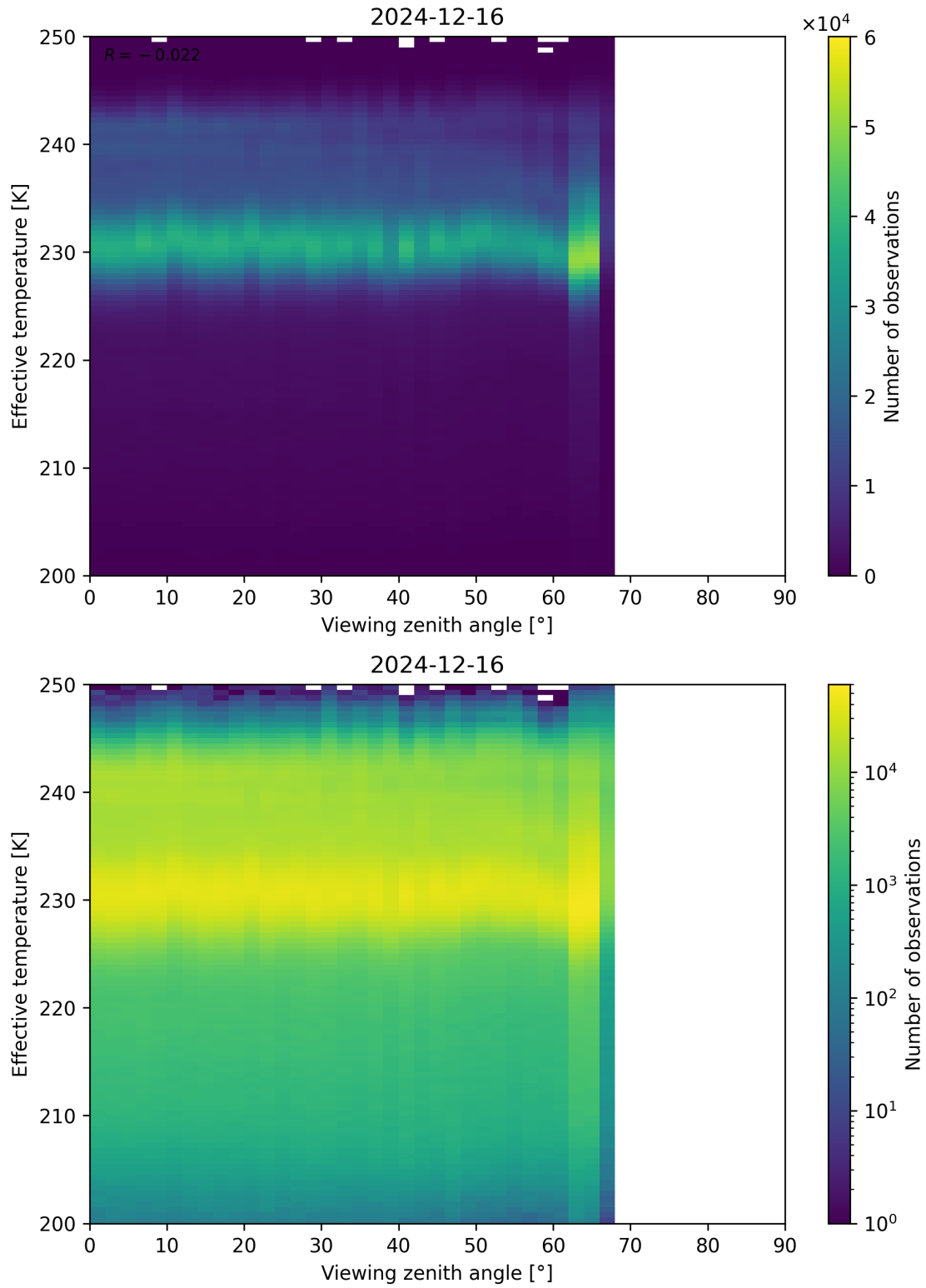
Figure 50: Scatter density plot of “Viewing zenith angle” against “Effective temperature” for 2024-12-16 to 2024-12-17.
