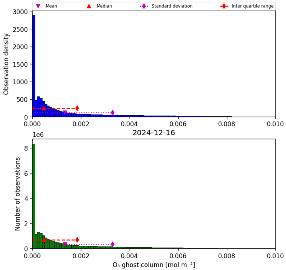
Figure 25: Histogram of “O 3 ghost column” for 2024-12-16 to 2024-12-17
