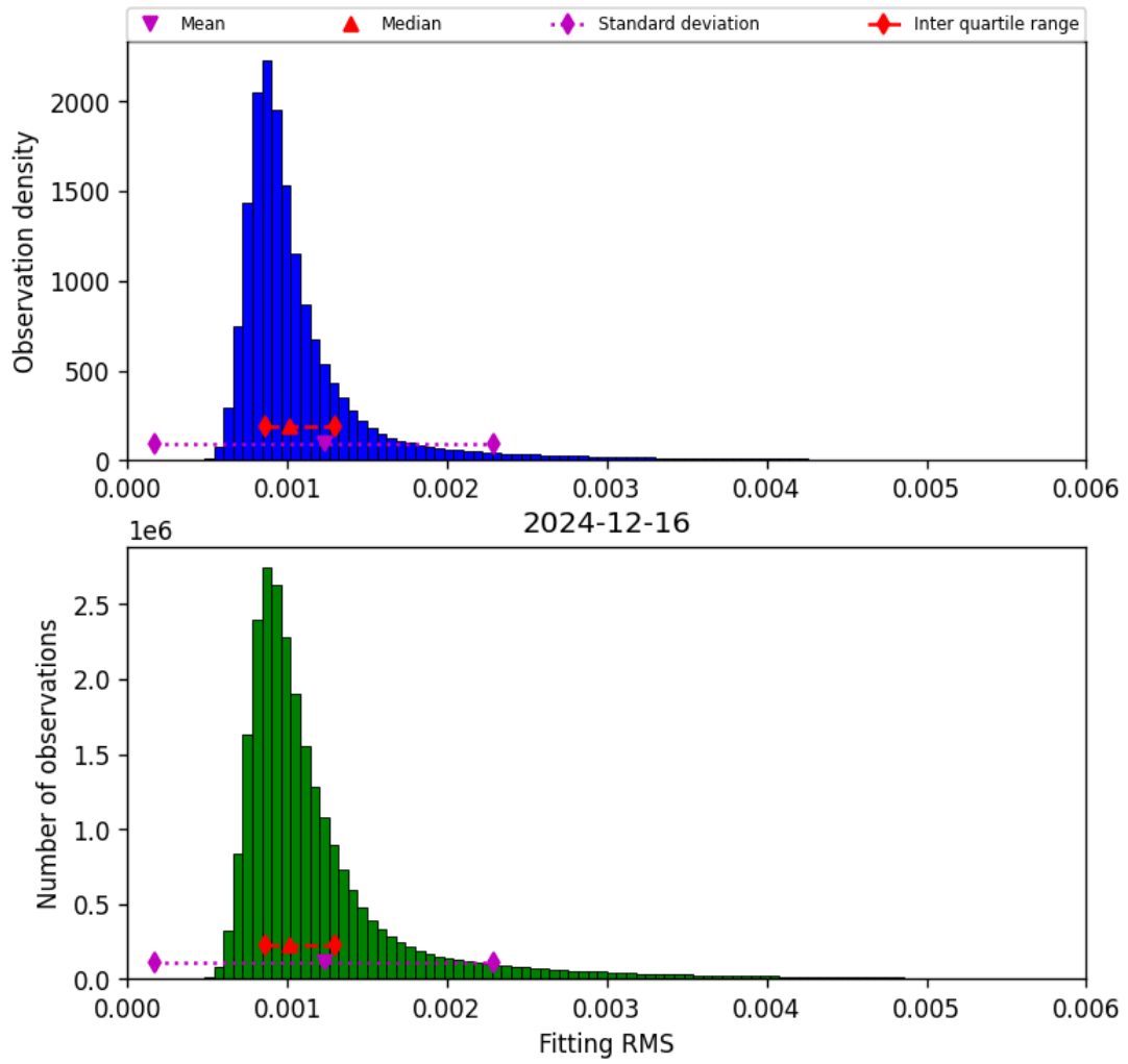
Figure 23: Histogram of “Fitting RMS” for 2024-12-16 to 2024-12-17
