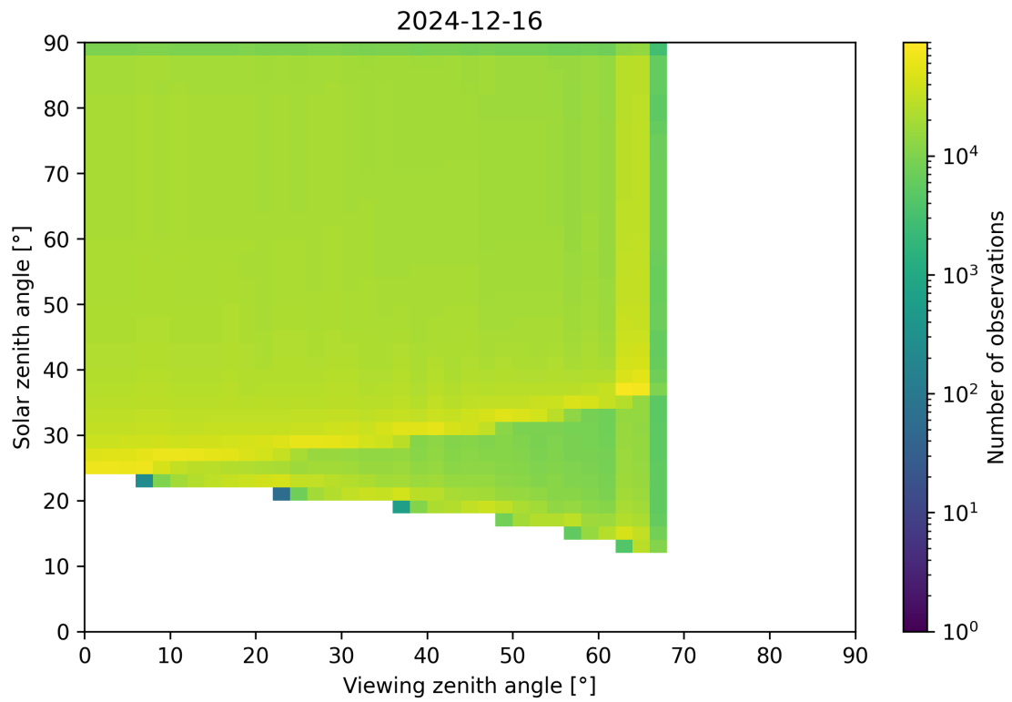
Figure 54: Scatter density plot of “Viewing zenith angle” against “Solar zenith angle” for 2024-12-16 to 2024-12-17.
