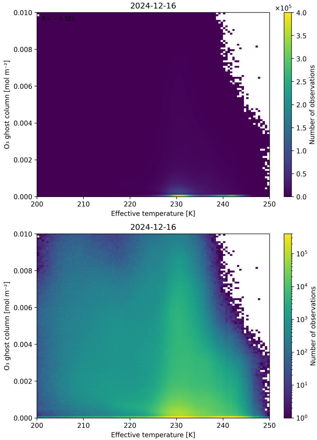
Figure 38: Scatter density plot of “Effective temperature” against “O 3 ghost column” for 2024-12-16 to 2024-12-17.
