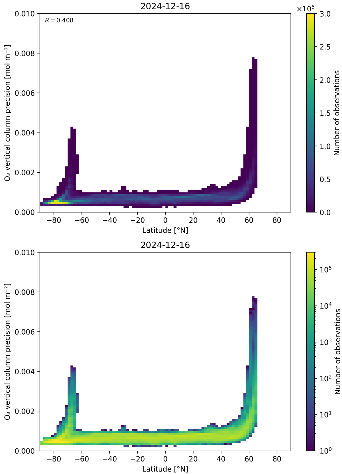
Figure 37: Scatter density plot of “Latitude” against “O 3 vertical column precision” for 2024-12-16 to 2024-12-17.
