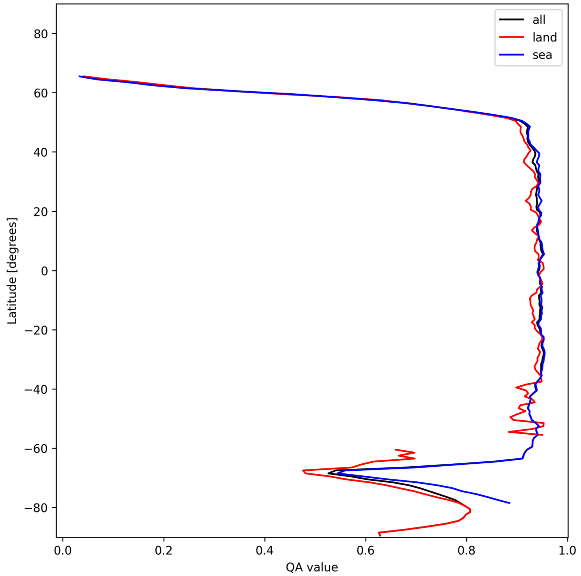
Figure 13: Zonal average of “QA value” for 2024-12-16 to 2024-12-17.
