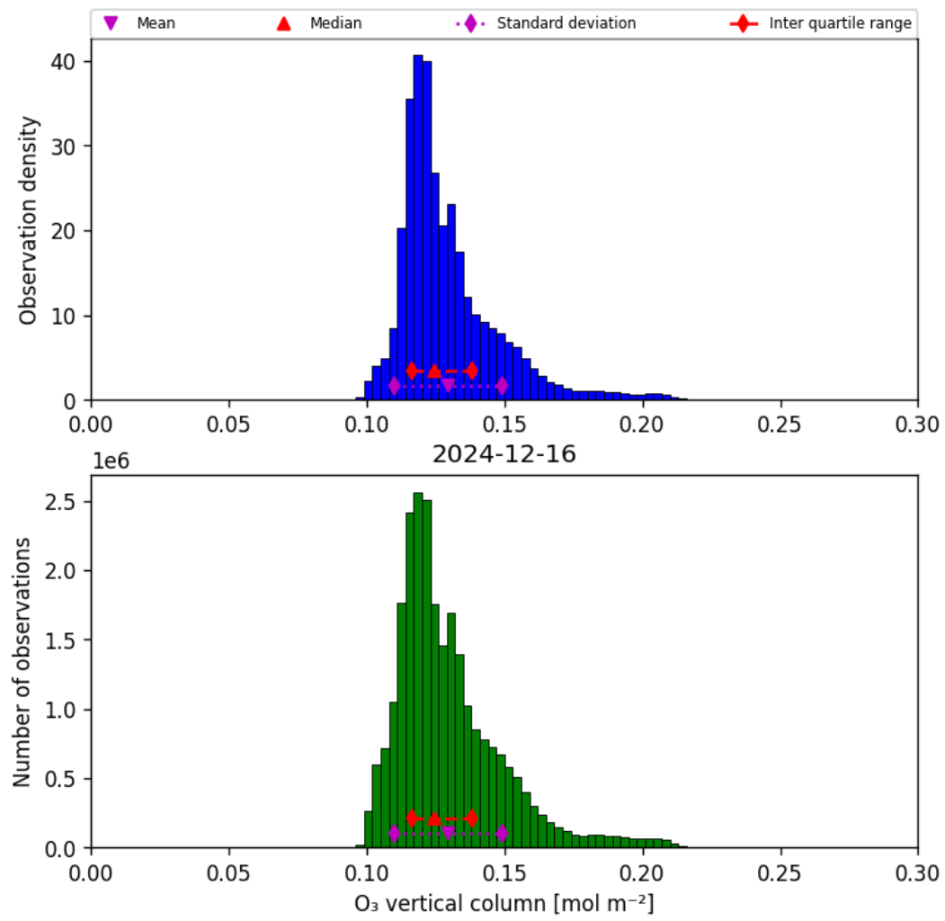
Figure 21: Histogram of “O 3 vertical column” for 2024-12-16 to 2024-12-17
