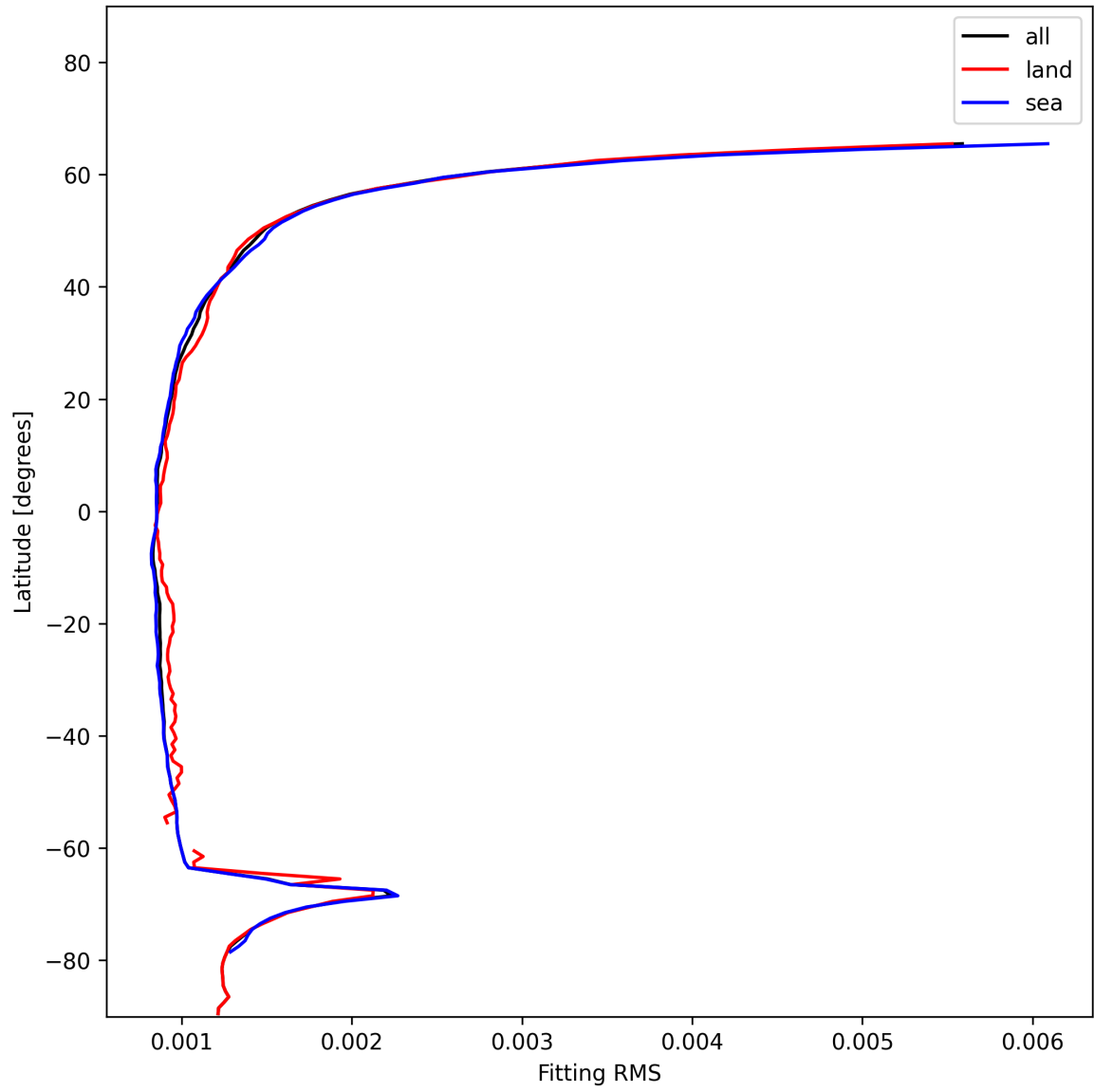
Figure 16: Zonal average of “Fitting RMS” for 2024-12-16 to 2024-12-17.
