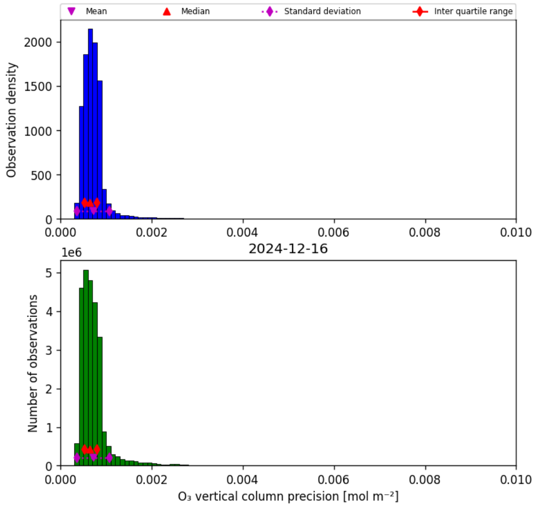
Figure 22: Histogram of “O 3 vertical column precision” for 2024-12-16 to 2024-12-17
