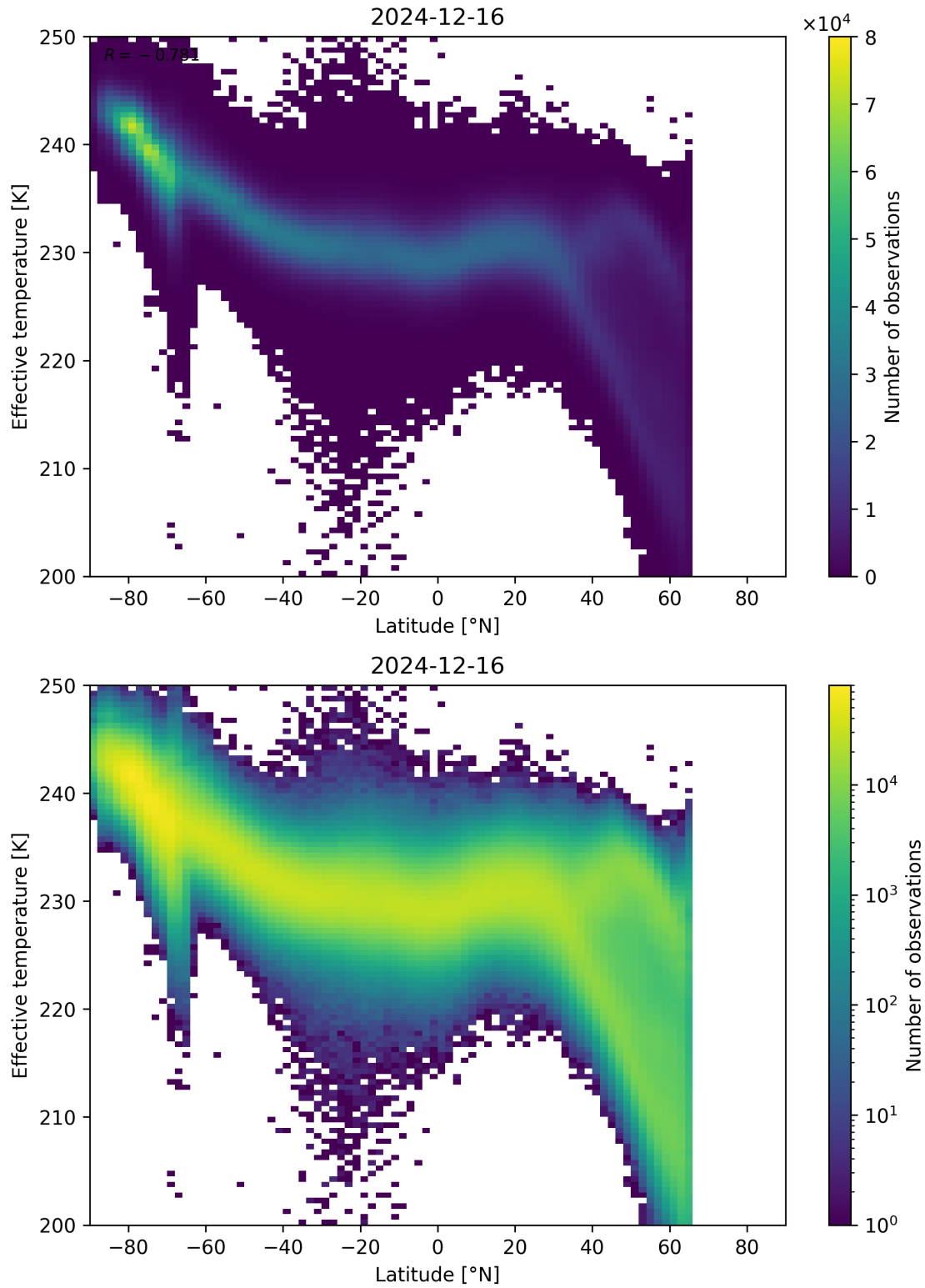
Figure 34: Scatter density plot of “Latitude” against “Effective temperature” for 2024-12-16 to 2024-12-17.
