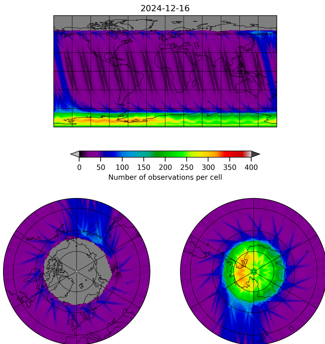
Figure 12: Map of the number of observations for 2024-12-16 to 2024-12-17
