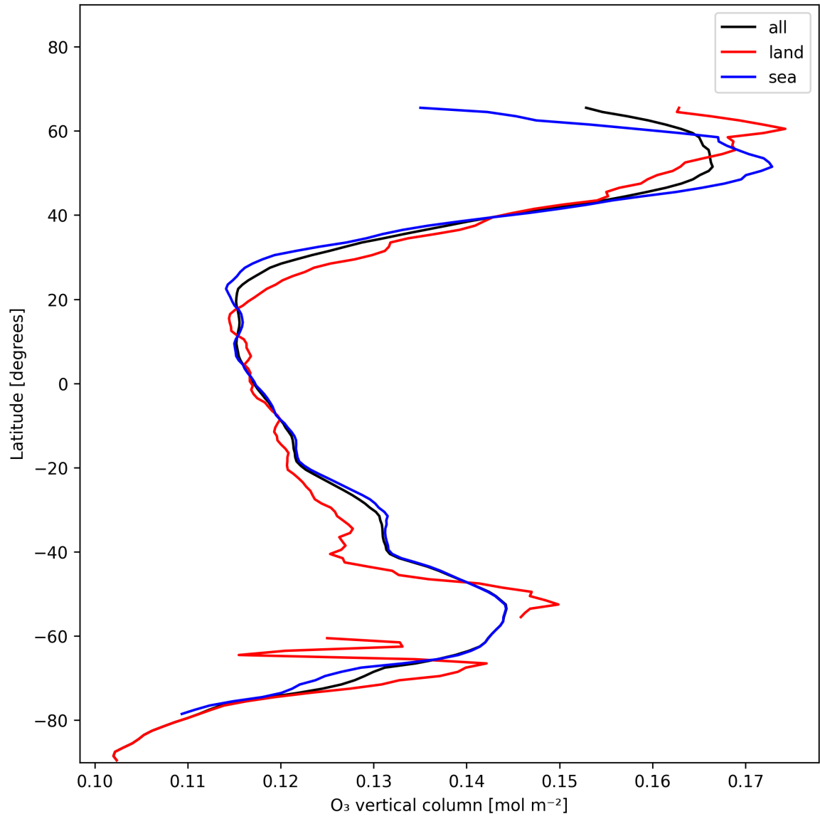
Figure 14: Zonal average of “O 3 vertical column” for 2024-12-17 to 2024-12-19.
