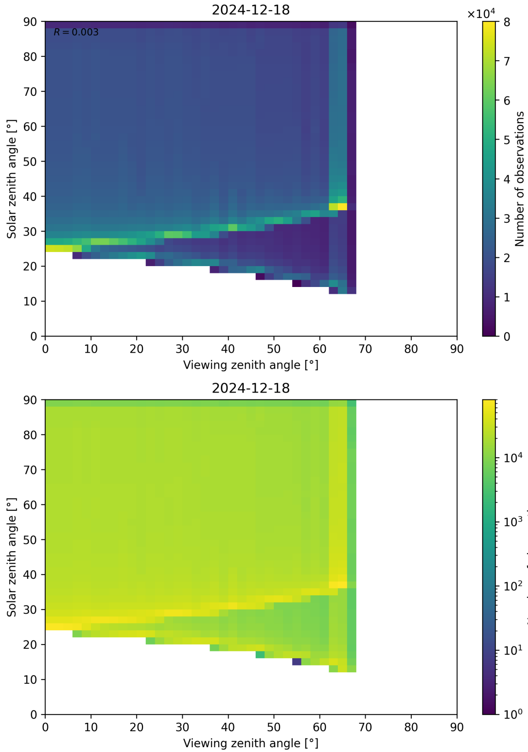
Figure 54: Scatter density plot of “Viewing zenith angle” against “Solar zenith angle” for 2024-12-17 to 2024-12-19.
