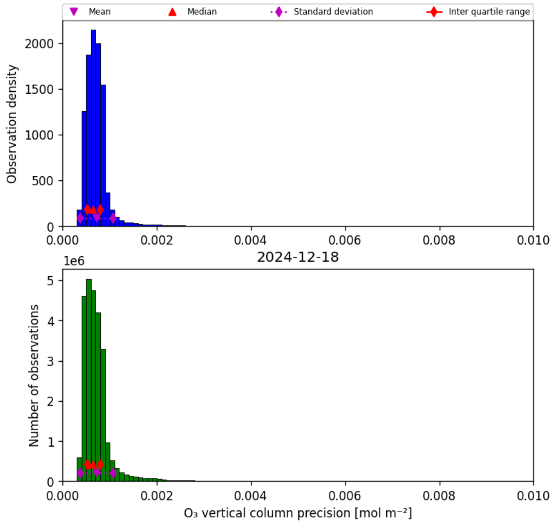
Figure 22: Histogram of “O 3 vertical column precision” for 2024-12-17 to 2024-12-19
