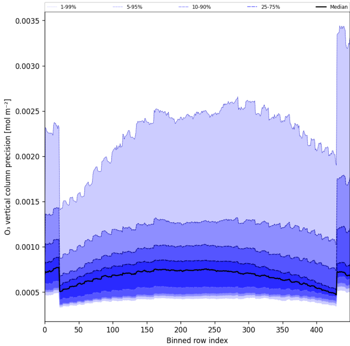
Figure 29: Along track statistics of “O 3 vertical column precision” for 2024-12-17 to 2024-12-19
