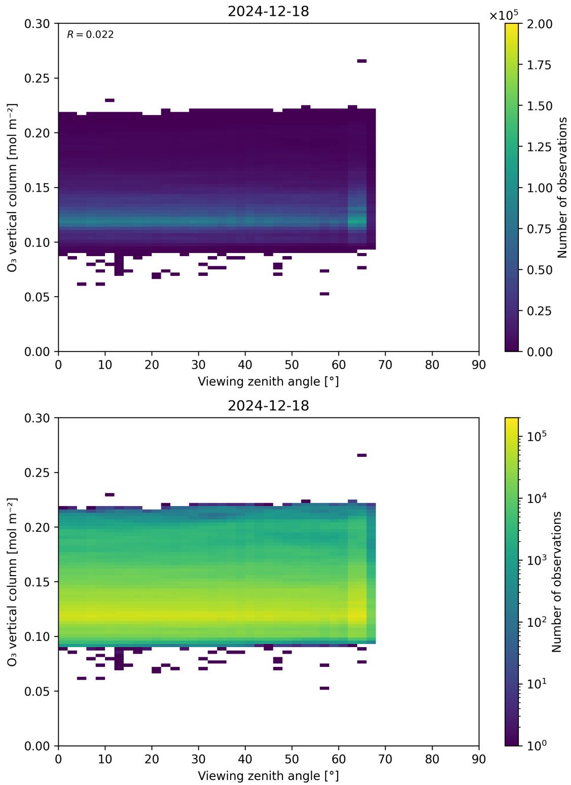
Figure 52: Scatter density plot of “Viewing zenith angle” against “O 3 vertical column” for 2024-12-17 to 2024-12-19.
