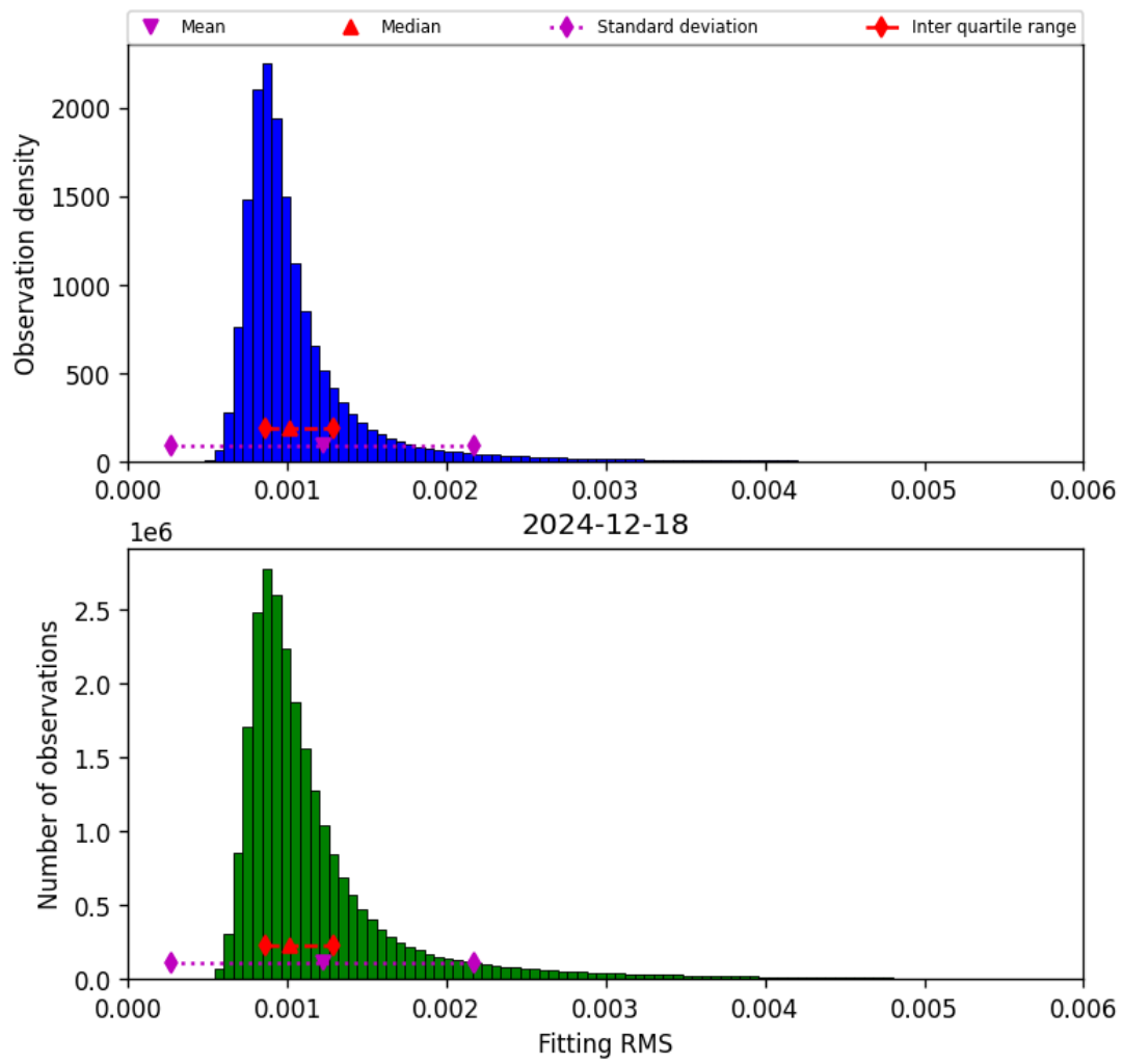
Figure 23: Histogram of “Fitting RMS” for 2024-12-17 to 2024-12-19
