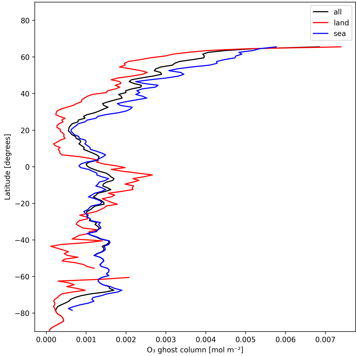
Figure 18: Zonal average of “O 3 ghost column” for 2024-12-17 to 2024-12-19.
