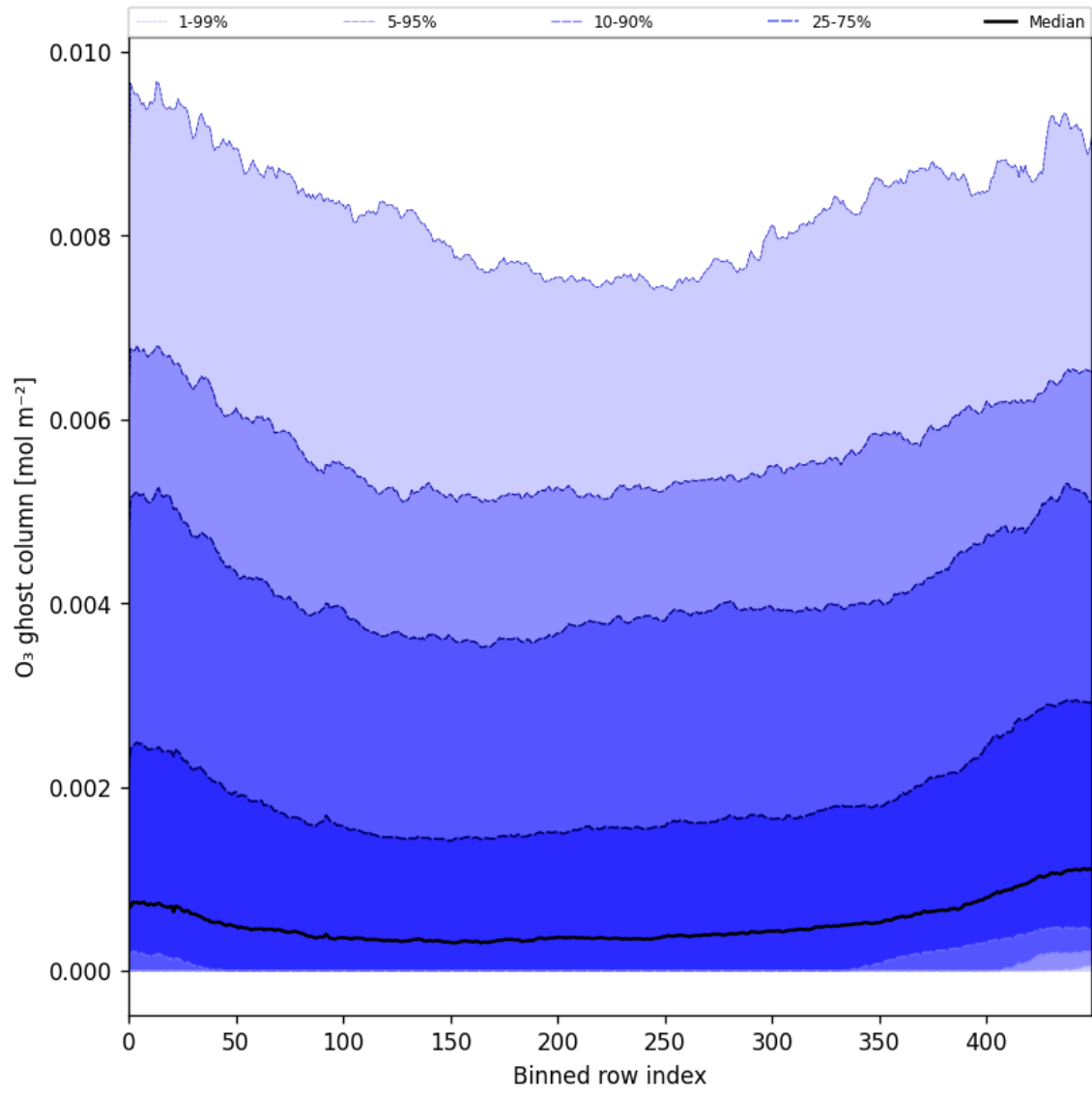
Figure 32: Along track statistics of “O 3 ghost column” for 2024-12-17 to 2024-12-19
