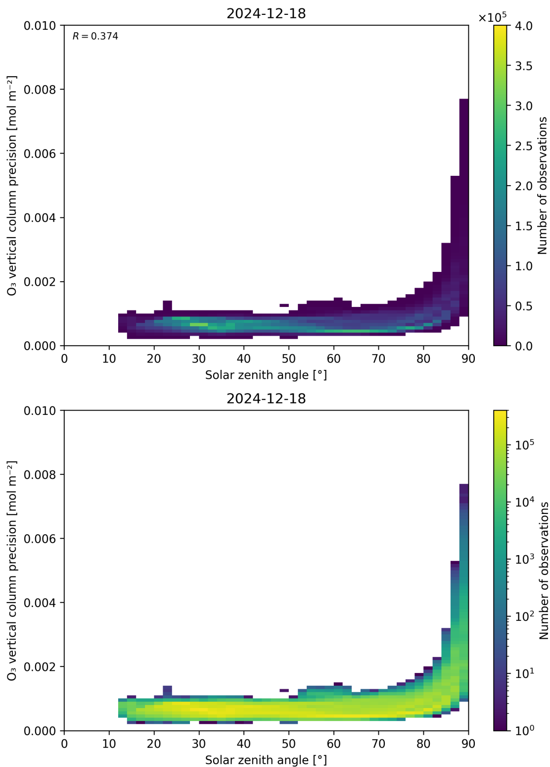
Figure 48: Scatter density plot of “Solar zenith angle” against “O 3 vertical column precision” for 2024-12-17 to 2024-12-19.
