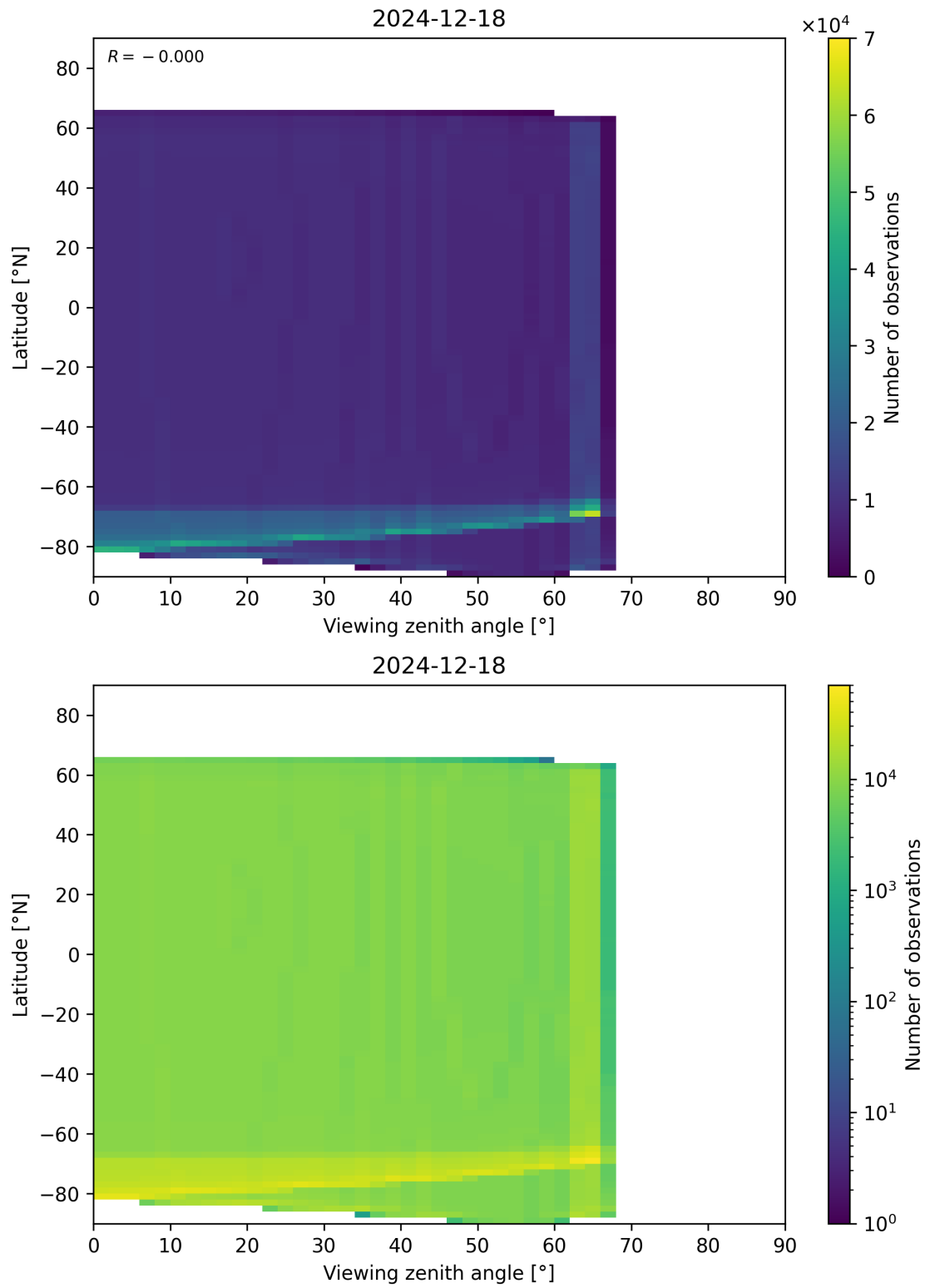
Figure 49: Scatter density plot of “Viewing zenith angle” against “Latitude” for 2024-12-17 to 2024-12-19.
