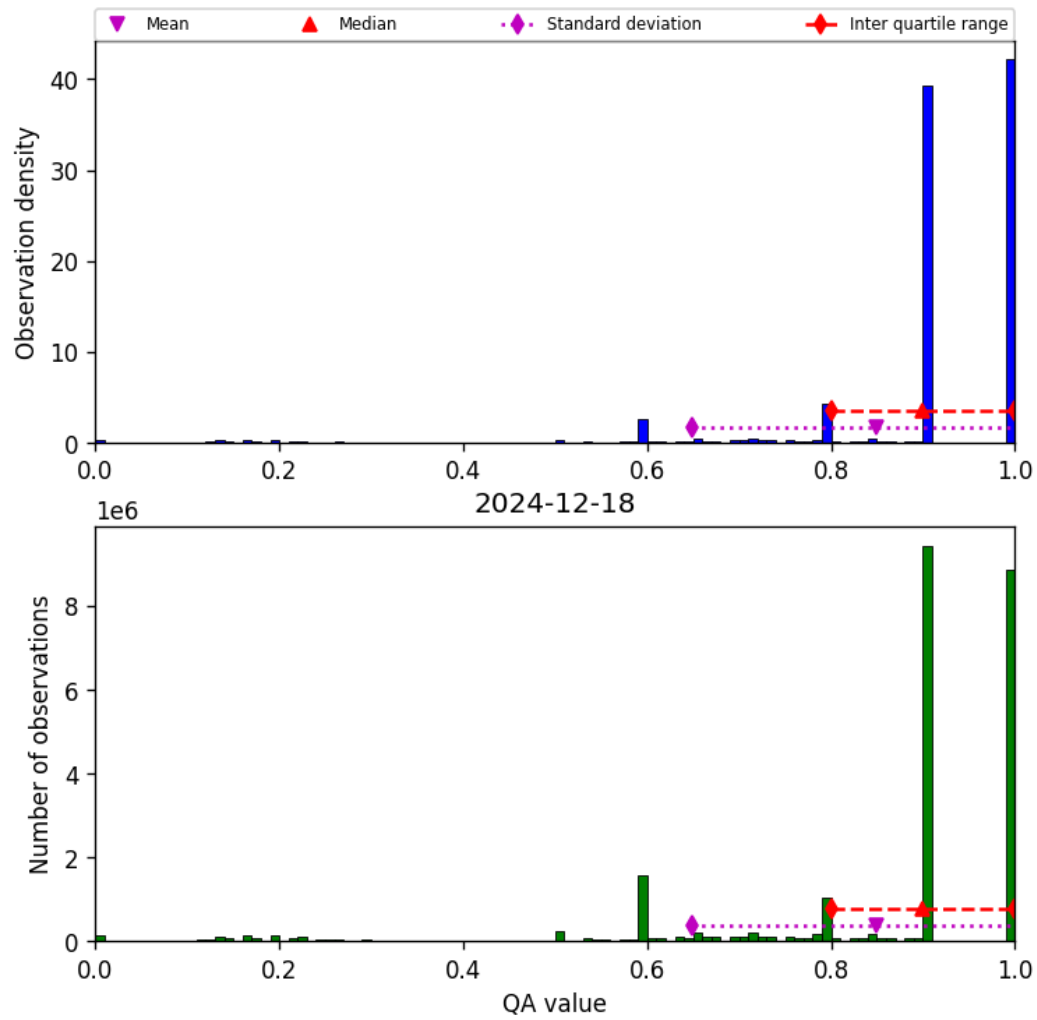
Figure 20: Histogram of “QA value” for 2024-12-17 to 2024-12-19
