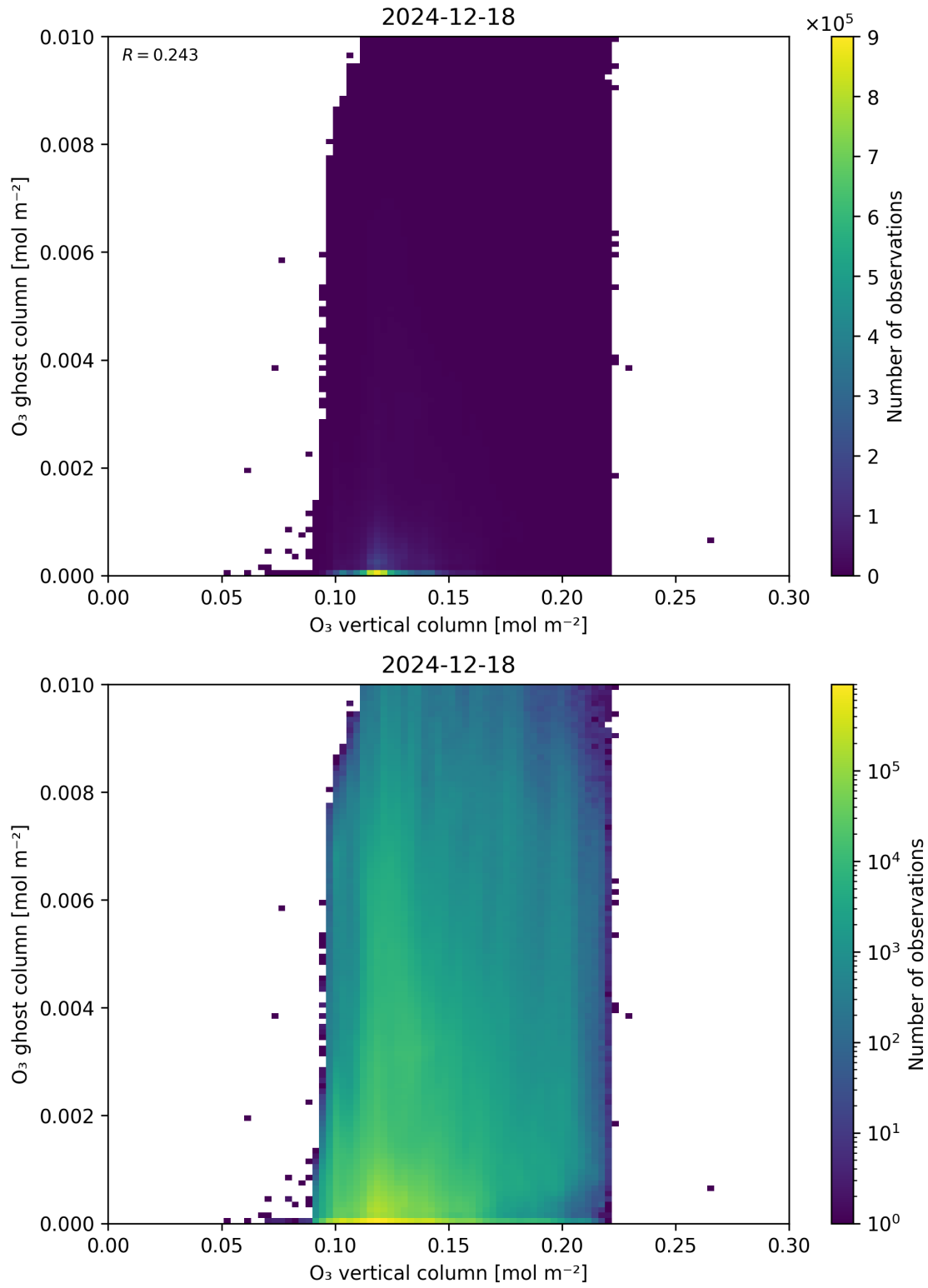
Figure 40: Scatter density plot of “O 3 vertical column” against “O 3 ghost column” for 2024-12-17 to 2024-12-19.
