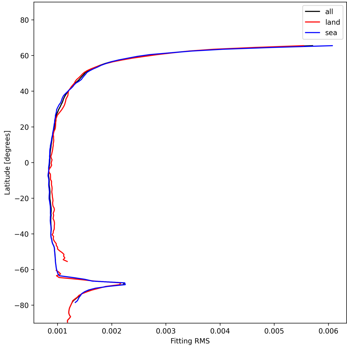
Figure 16: Zonal average of “Fitting RMS” for 2024-12-17 to 2024-12-19.
