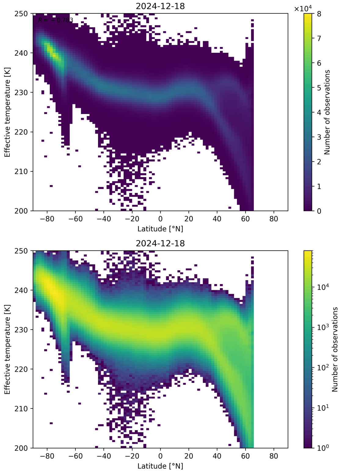
Figure 34: Scatter density plot of “Latitude” against “Effective temperature” for 2024-12-17 to 2024-12-19.
