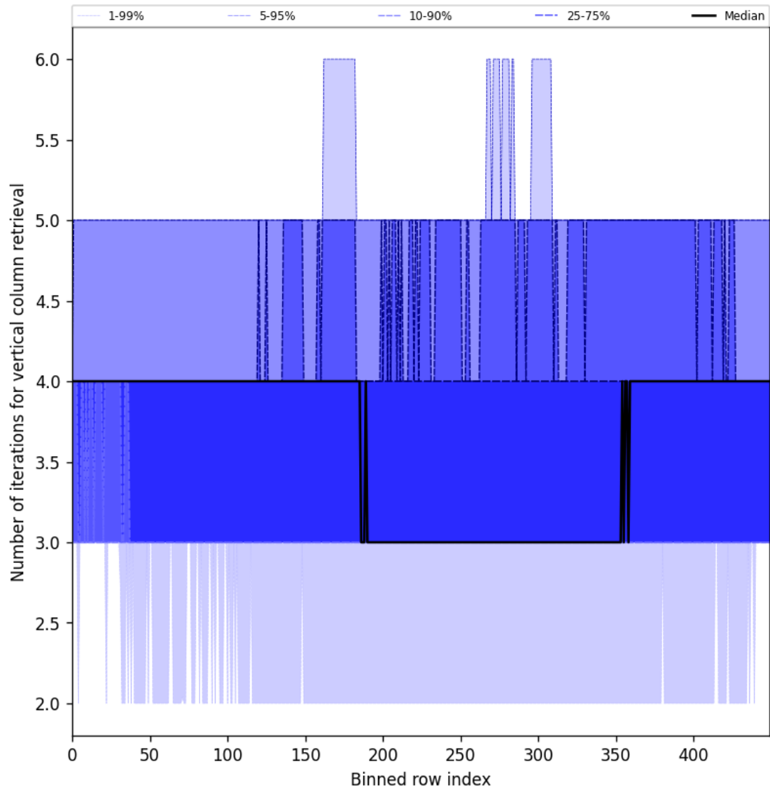
Figure 33: Along track statistics of “Number of iterations for vertical column retrieval” for 2024-12-17 to 2024-12-19
