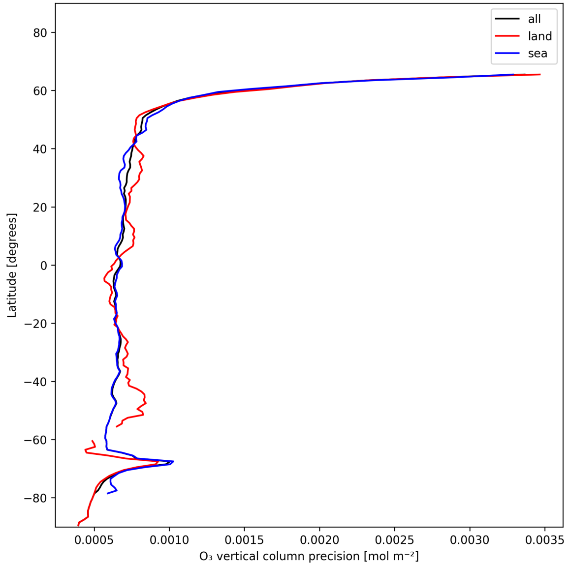
Figure 15: Zonal average of “O 3 vertical column precision” for 2024-12-17 to 2024-12-19.
