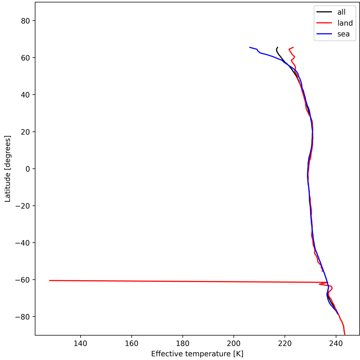
Figure 17: Zonal average of "Effective temperature" for 2024-12-17 to 2024-12-19.
