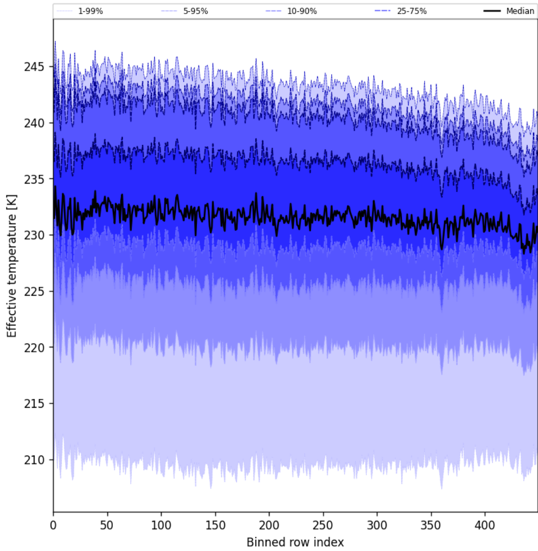
Figure 31: Along track statistics of “Effective temperature” for 2024-12-17 to 2024-12-19
