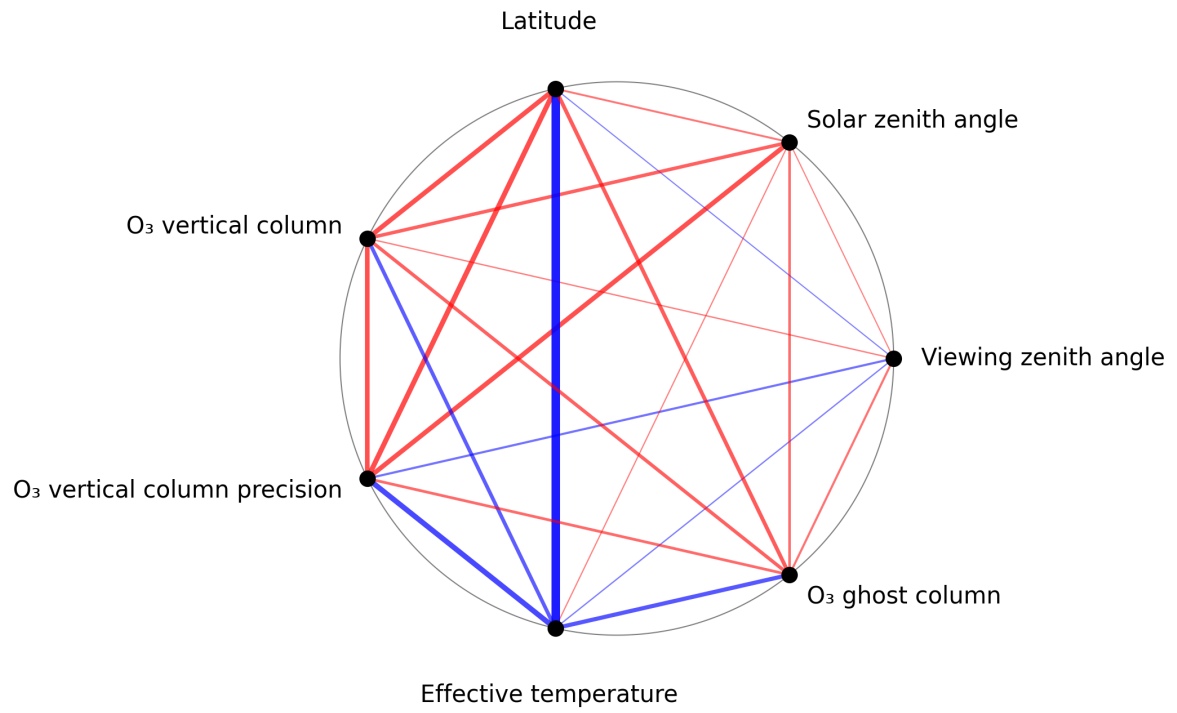
Figure 1: Map of correlation graph for 2024-12-17 to 2024-12-19.
