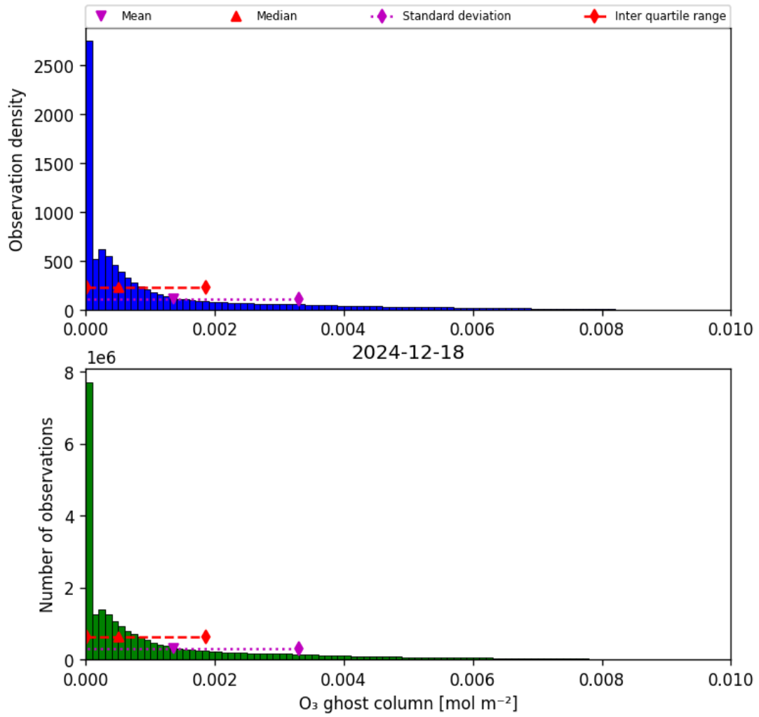
Figure 25: Histogram of “O 3 ghost column” for 2024-12-17 to 2024-12-19
