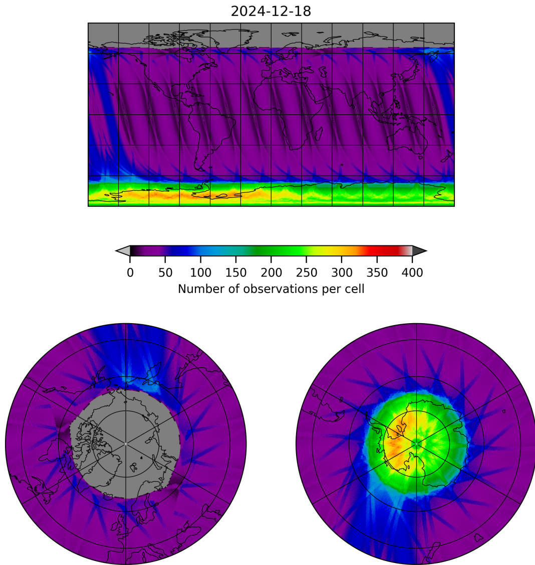
Figure 12: Map of the number of observations for 2024-12-17 to 2024-12-19
