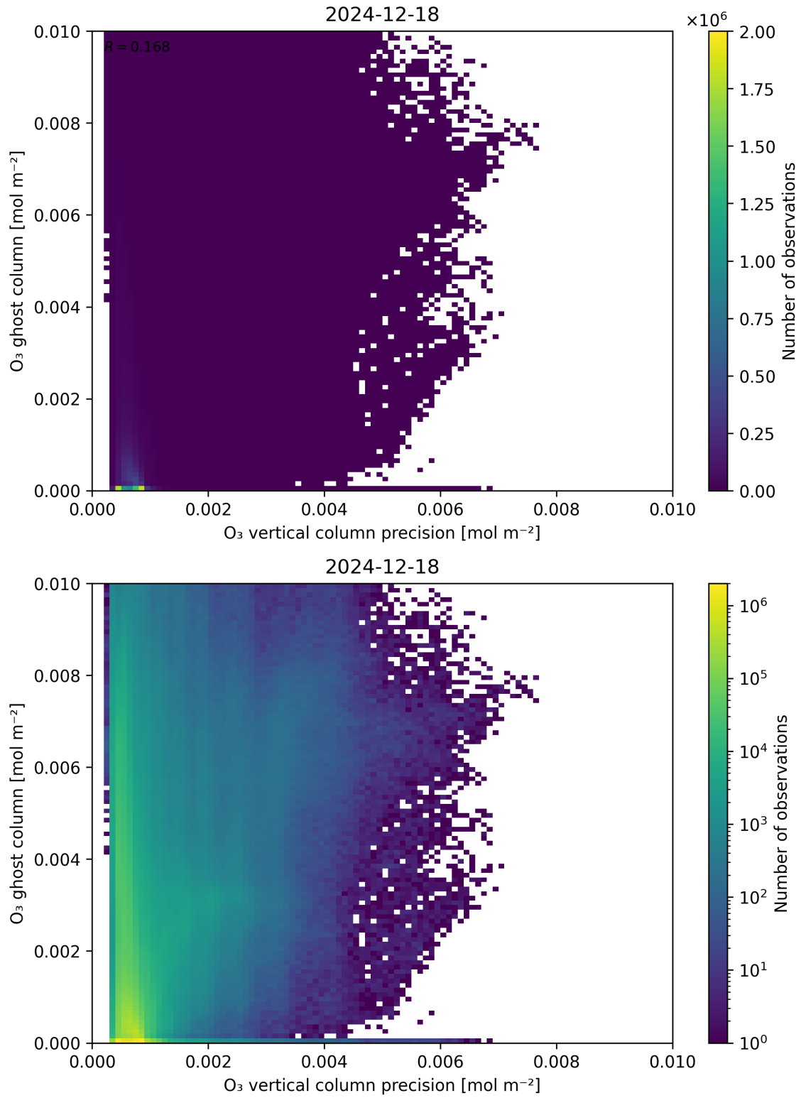
Figure 43: Scatter density plot of “ \text{O}_3 vertical column precision” against “ \text{O}_3 ghost column” for 2024-12-17 to 2024-12-19.
