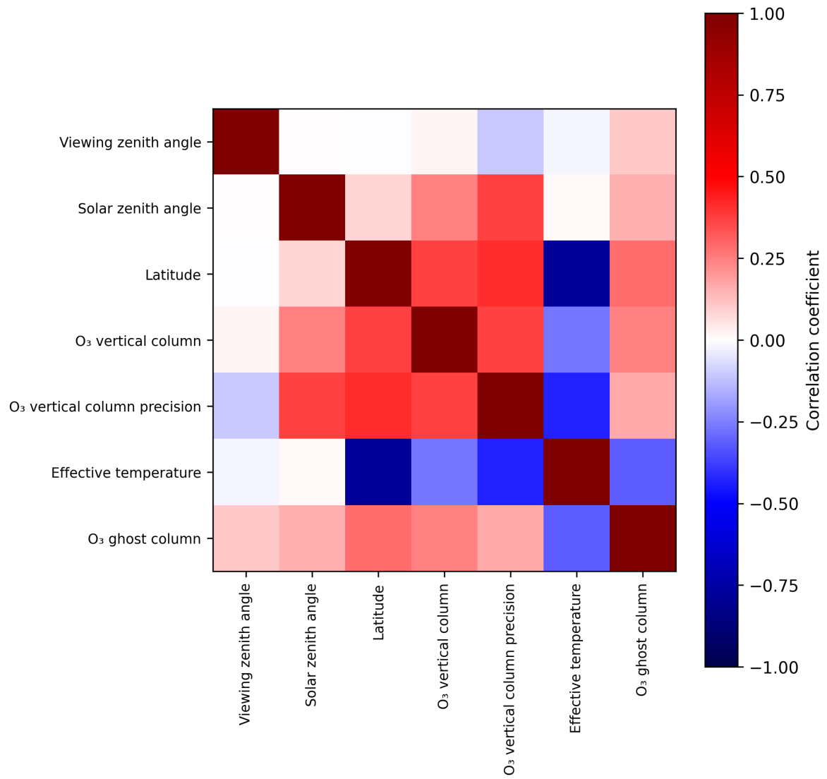
Figure 2: Map of correlation matrix for 2024-12-17 to 2024-12-19.
