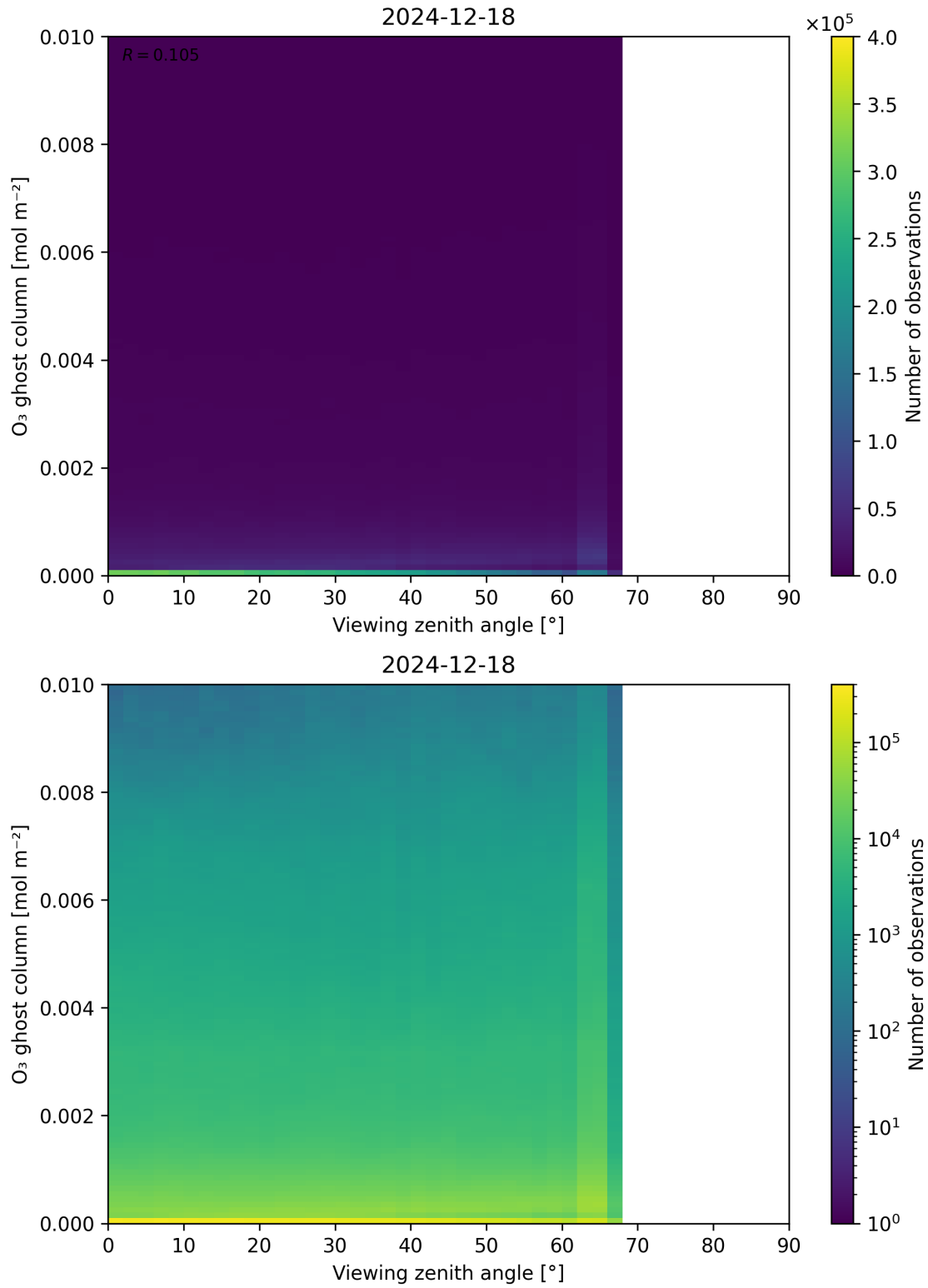
Figure 51: Scatter density plot of “Viewing zenith angle” against “O 3 ghost column” for 2024-12-17 to 2024-12-19.
