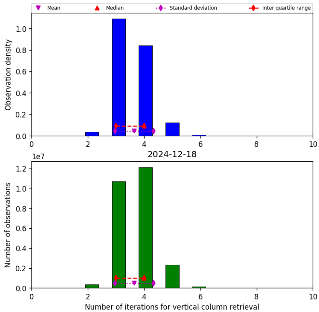
Figure 26: Histogram of “Number of iterations for vertical column retrieval” for 2024-12-17 to 2024-12-19
