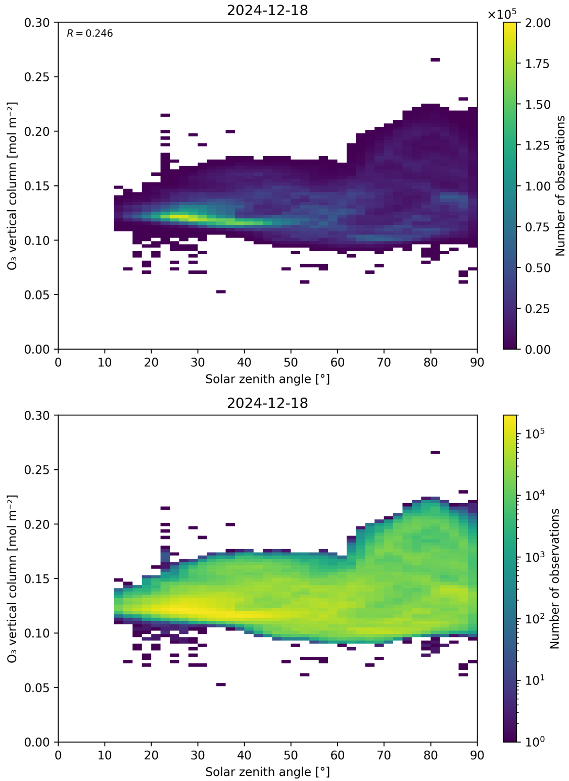
Figure 47: Scatter density plot of “Solar zenith angle” against “O 3 vertical column” for 2024-12-17 to 2024-12-19.
