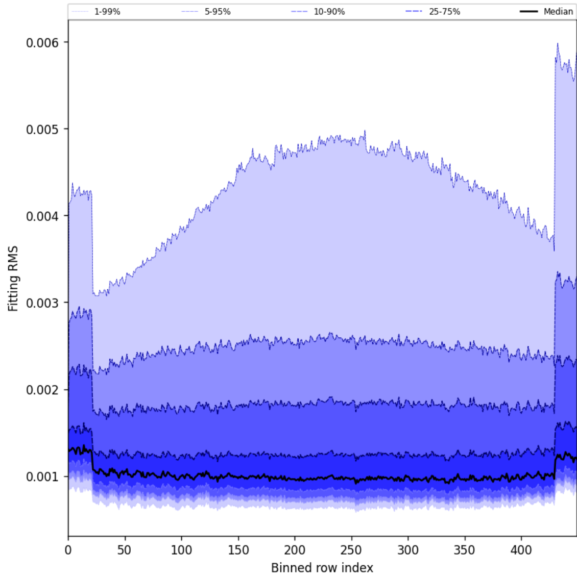
Figure 30: Along track statistics of “Fitting RMS” for 2024-12-17 to 2024-12-19
