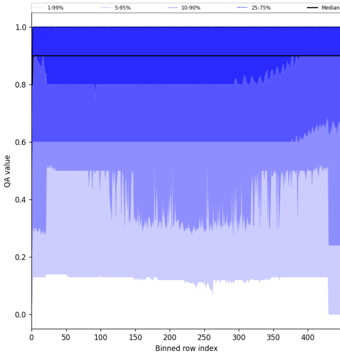
Figure 27: Along track statistics of “QA value” for 2024-12-17 to 2024-12-19
