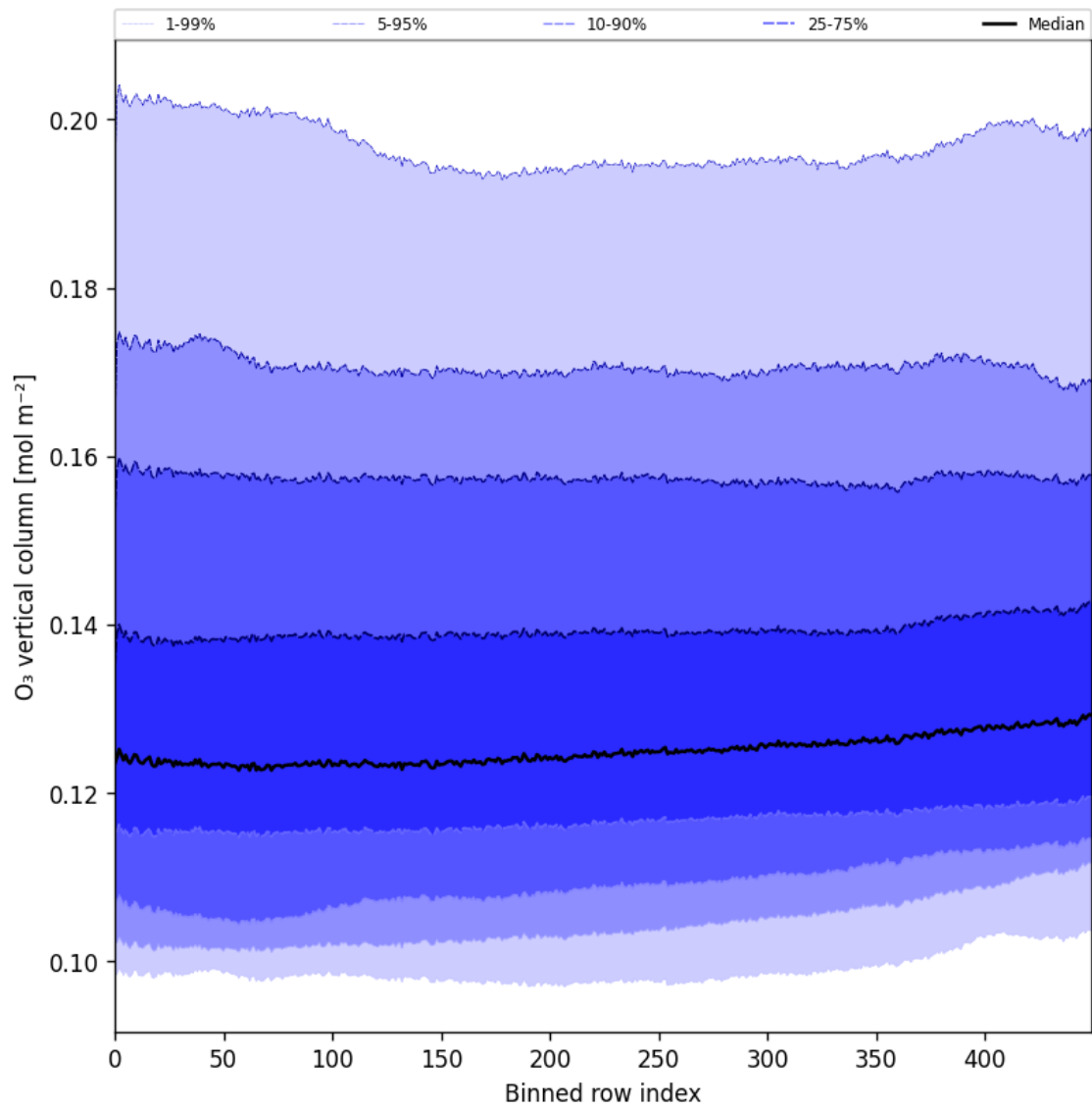
Figure 28: Along track statistics of “O 3 vertical column” for 2024-12-17 to 2024-12-19
