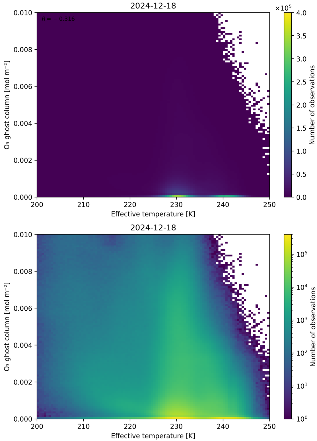
Figure 38: Scatter density plot of “Effective temperature” against “O 3 ghost column” for 2024-12-17 to 2024-12-19.
