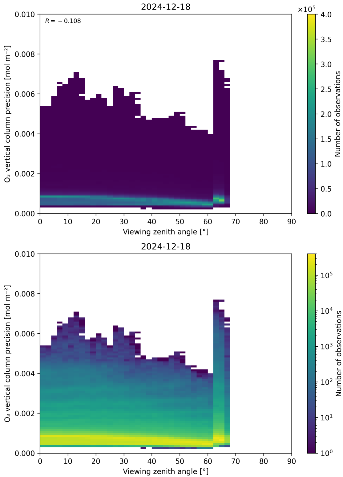
Figure 53: Scatter density plot of “Viewing zenith angle” against “O 3 vertical column precision” for 2024-12-17 to 2024-12-19.
