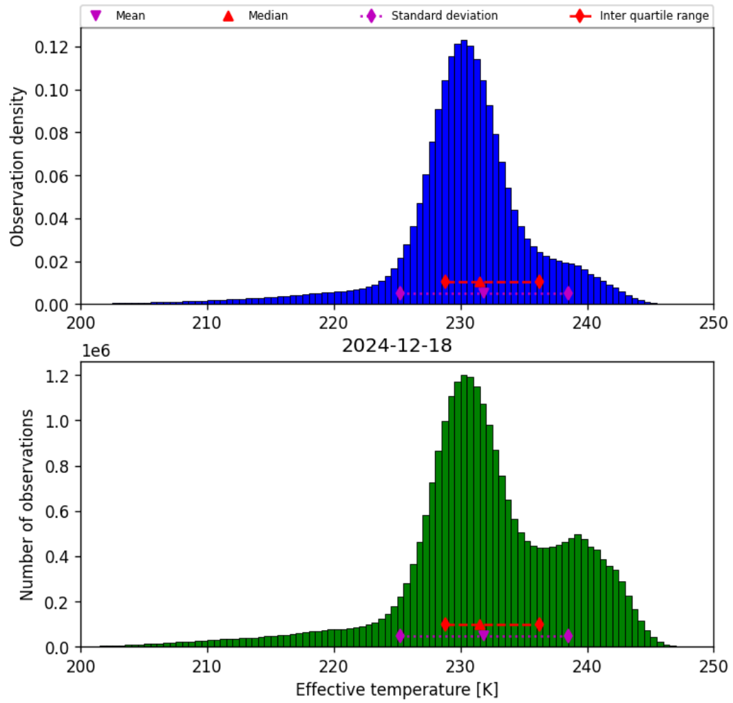
Figure 24: Histogram of “Effective temperature” for 2024-12-17 to 2024-12-19
