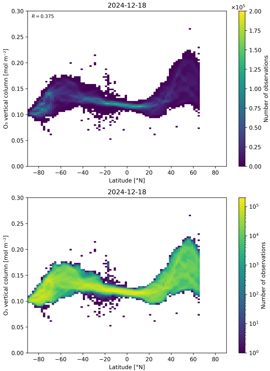
Figure 36: Scatter density plot of “Latitude” against “O 3 vertical column” for 2024-12-17 to 2024-12-19.
