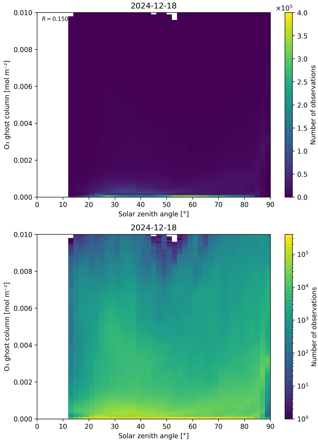
Figure 46: Scatter density plot of “Solar zenith angle” against “O 3 ghost column” for 2024-12-17 to 2024-12-19.
