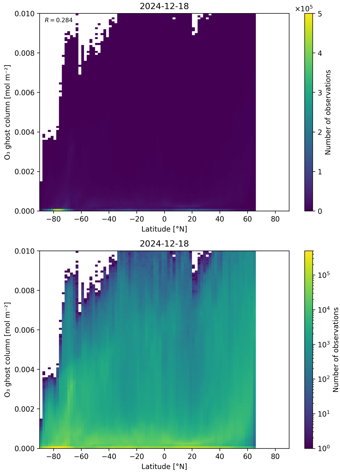
Figure 35: Scatter density plot of “Latitude” against “O 3 ghost column” for 2024-12-17 to 2024-12-19.
