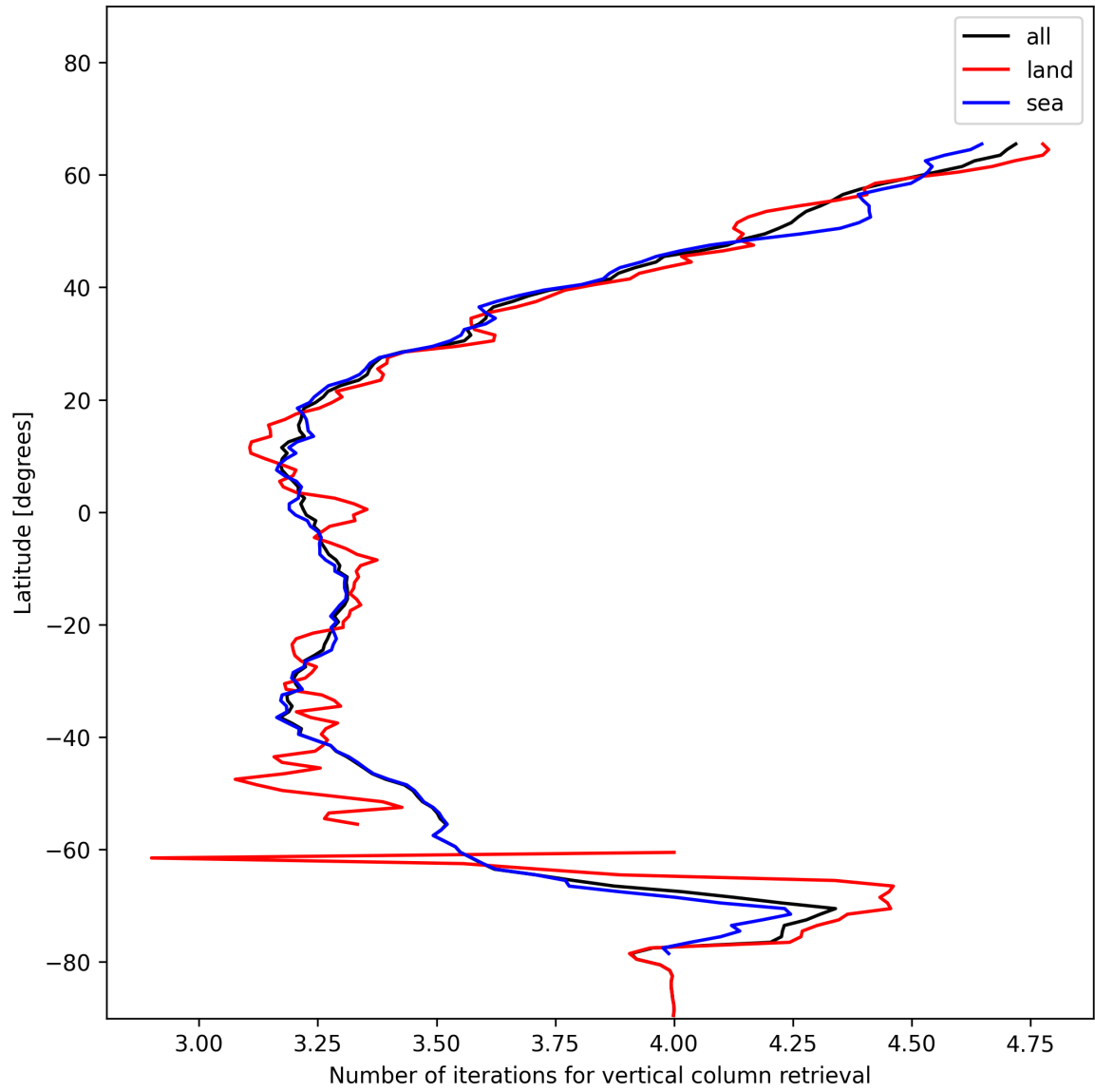
Figure 19: Zonal average of “Number of iterations for vertical column retrieval” for 2024-12-17 to 2024-12-19.
