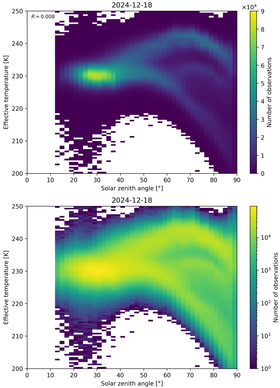
Figure 45: Scatter density plot of “Solar zenith angle” against “Effective temperature” for 2024-12-17 to 2024-12-19.
