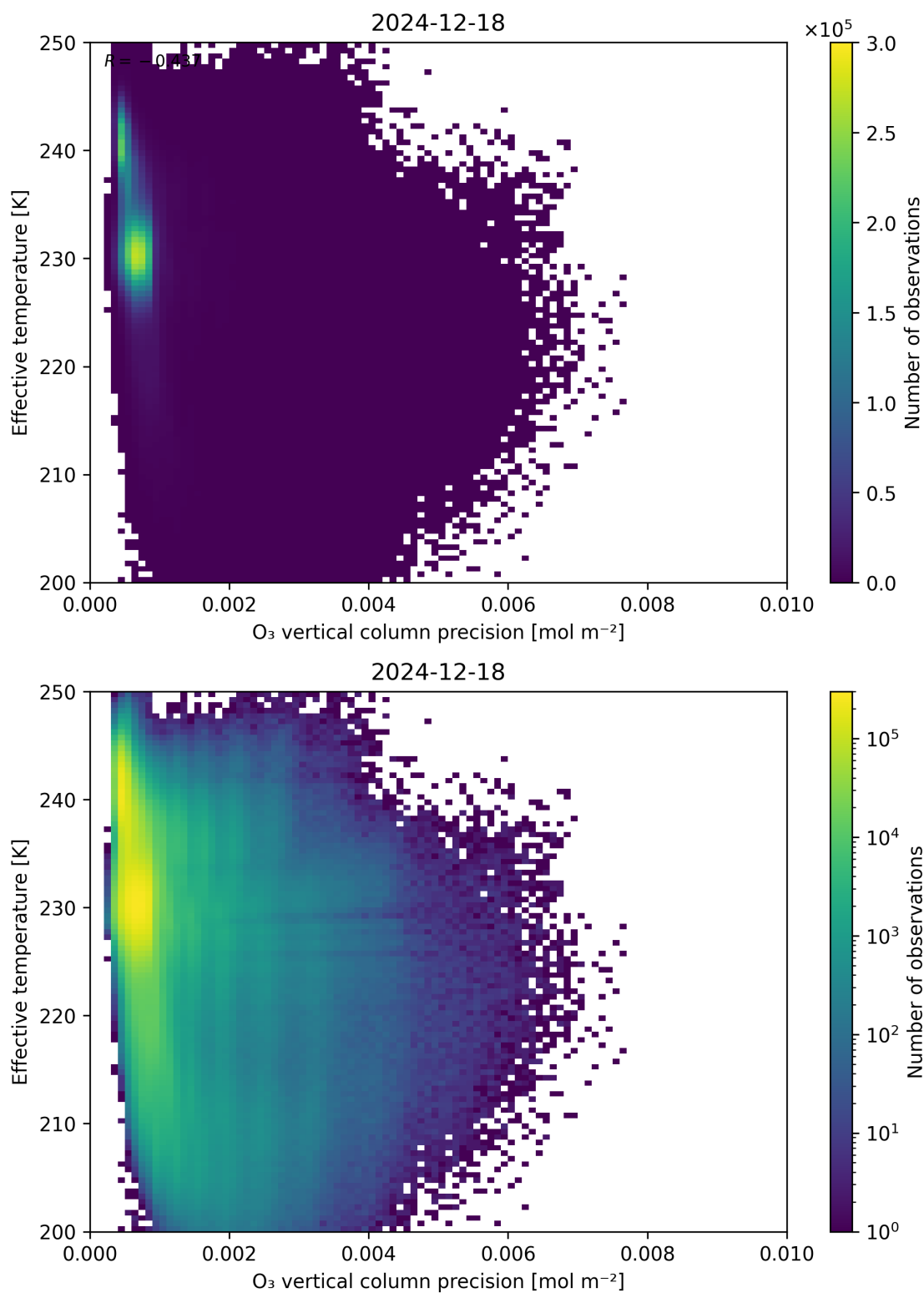
Figure 42: Scatter density plot of “O 3 vertical column precision” against “Effective temperature” for 2024-12-17 to 2024-12-19.
