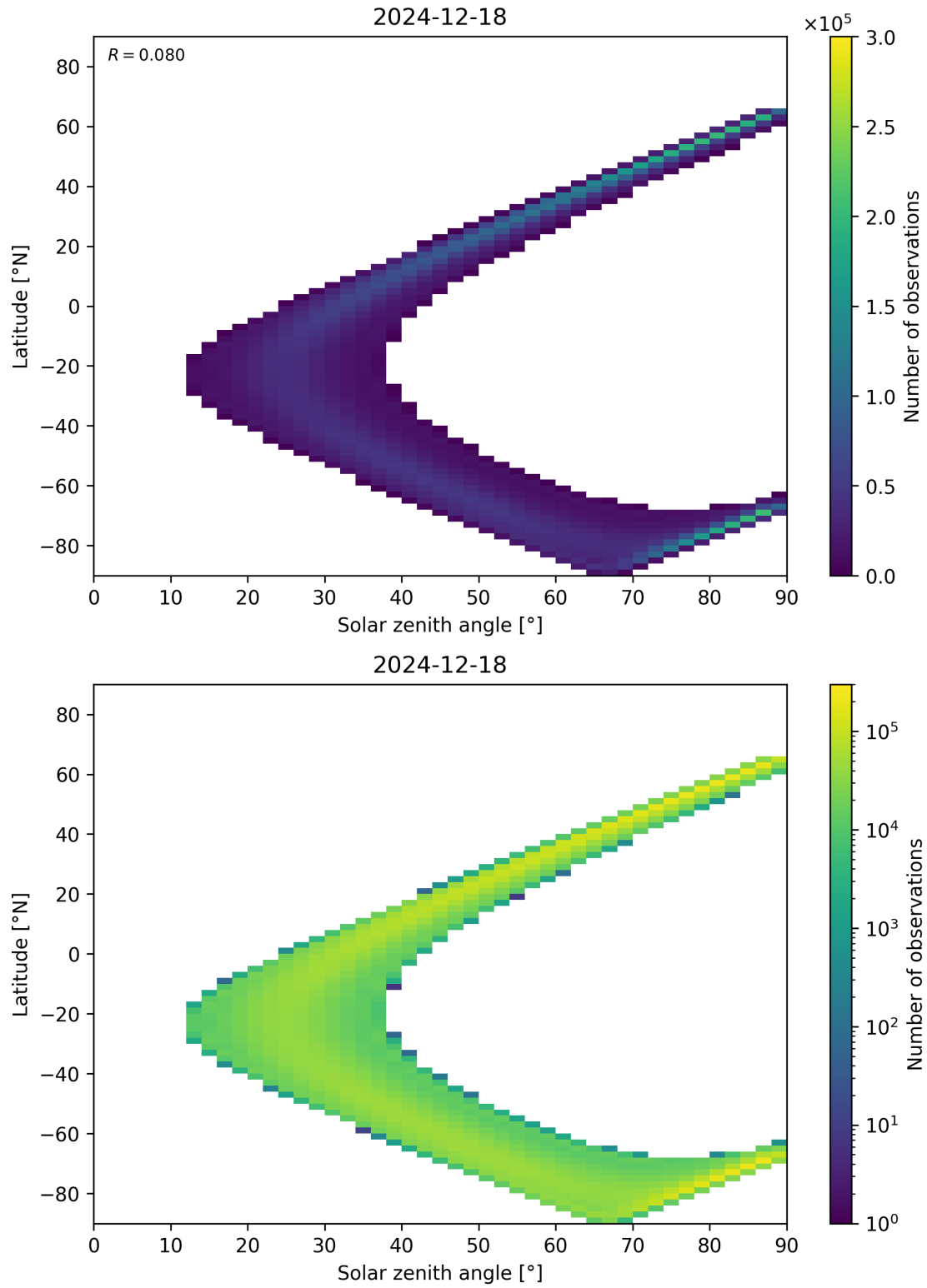
Figure 44: Scatter density plot of “Solar zenith angle” against “Latitude” for 2024-12-17 to 2024-12-19.
