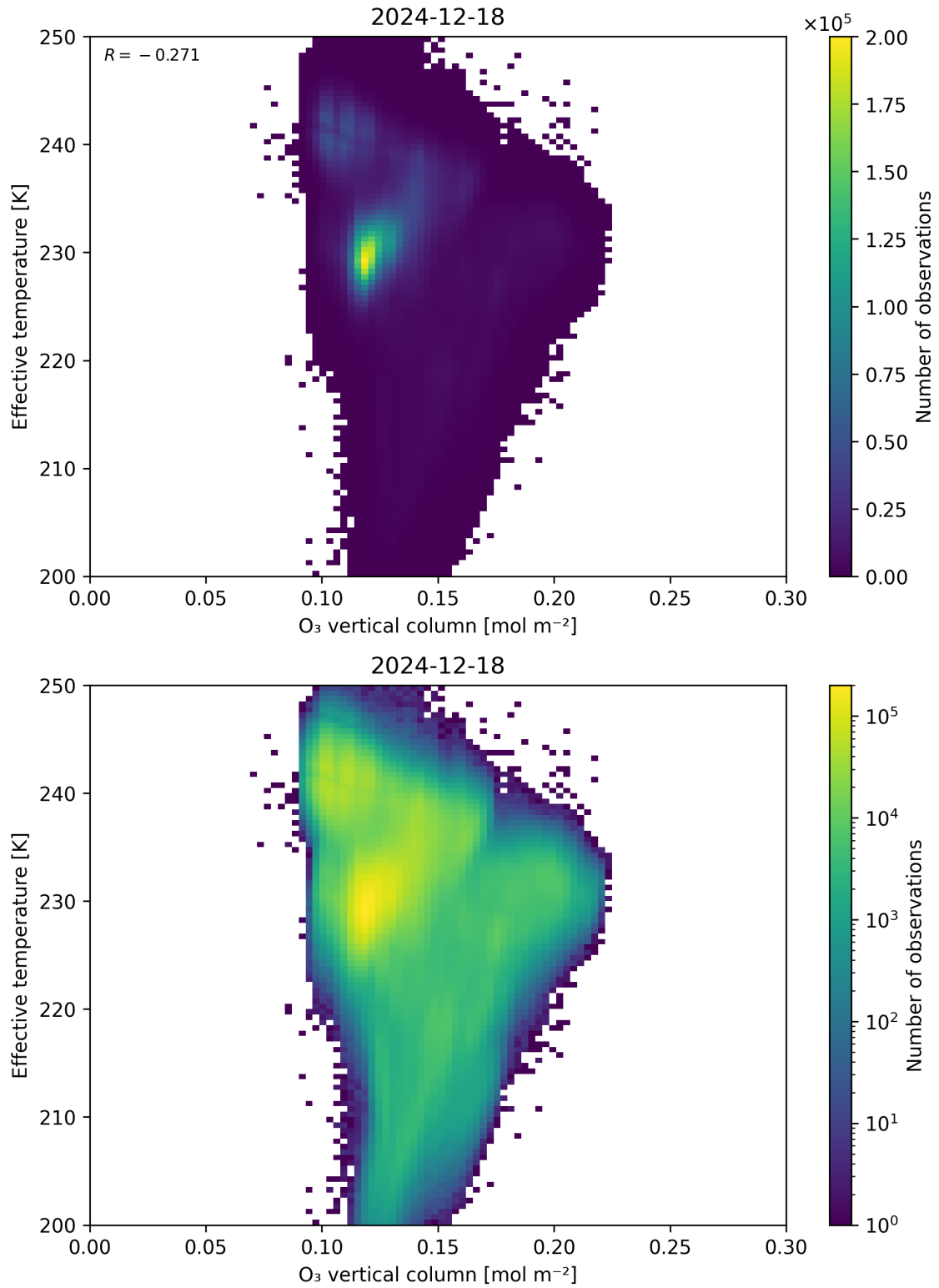
Figure 39: Scatter density plot of “O 3 vertical column” against “Effective temperature” for 2024-12-17 to 2024-12-19.
