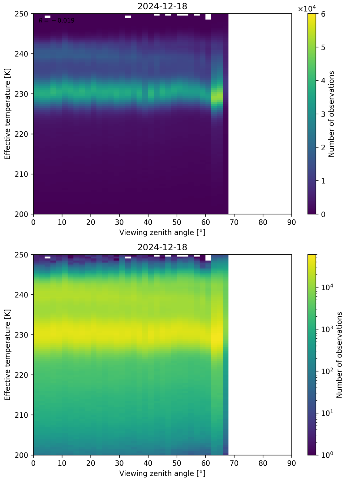
Figure 50: Scatter density plot of “Viewing zenith angle” against “Effective temperature” for 2024-12-17 to 2024-12-19.
