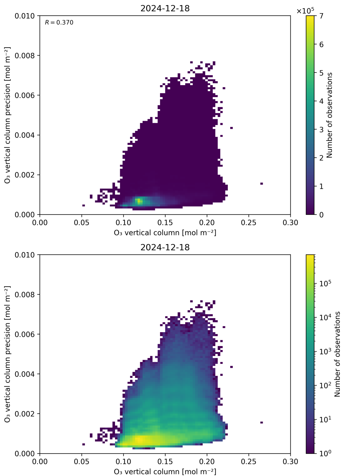
Figure 41: Scatter density plot of “O 3 vertical column” against “O 3 vertical column precision” for 2024-12-17 to 2024-12-19.
