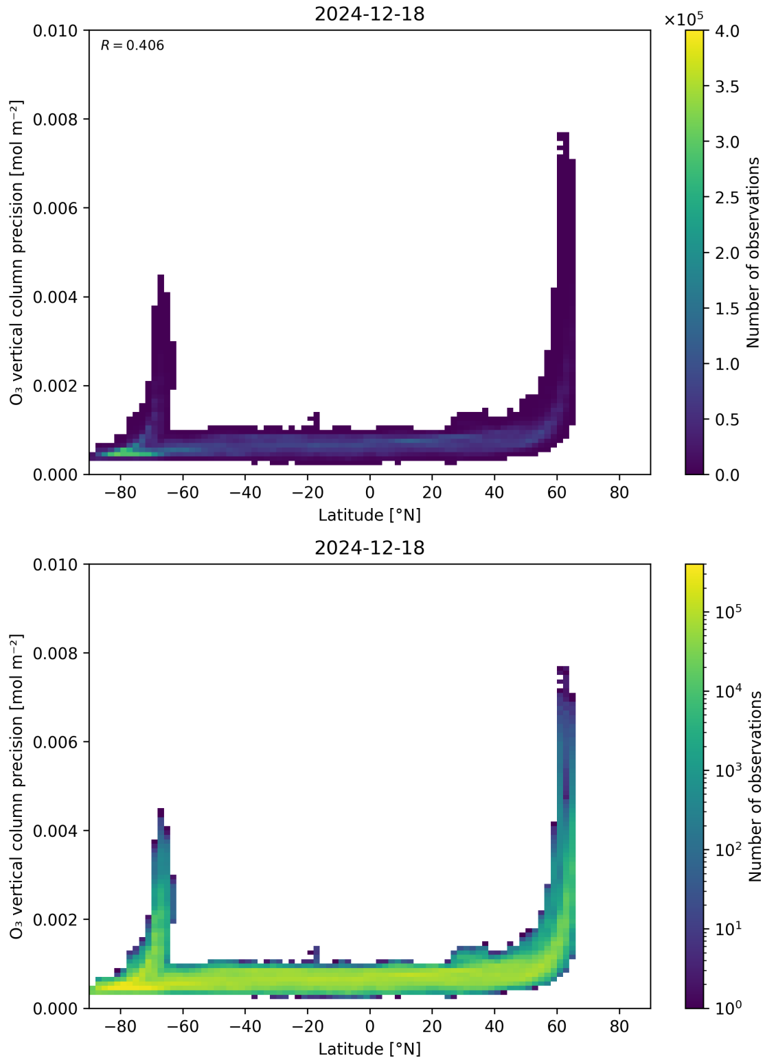
Figure 37: Scatter density plot of “Latitude” against “O 3 vertical column precision” for 2024-12-17 to 2024-12-19.
