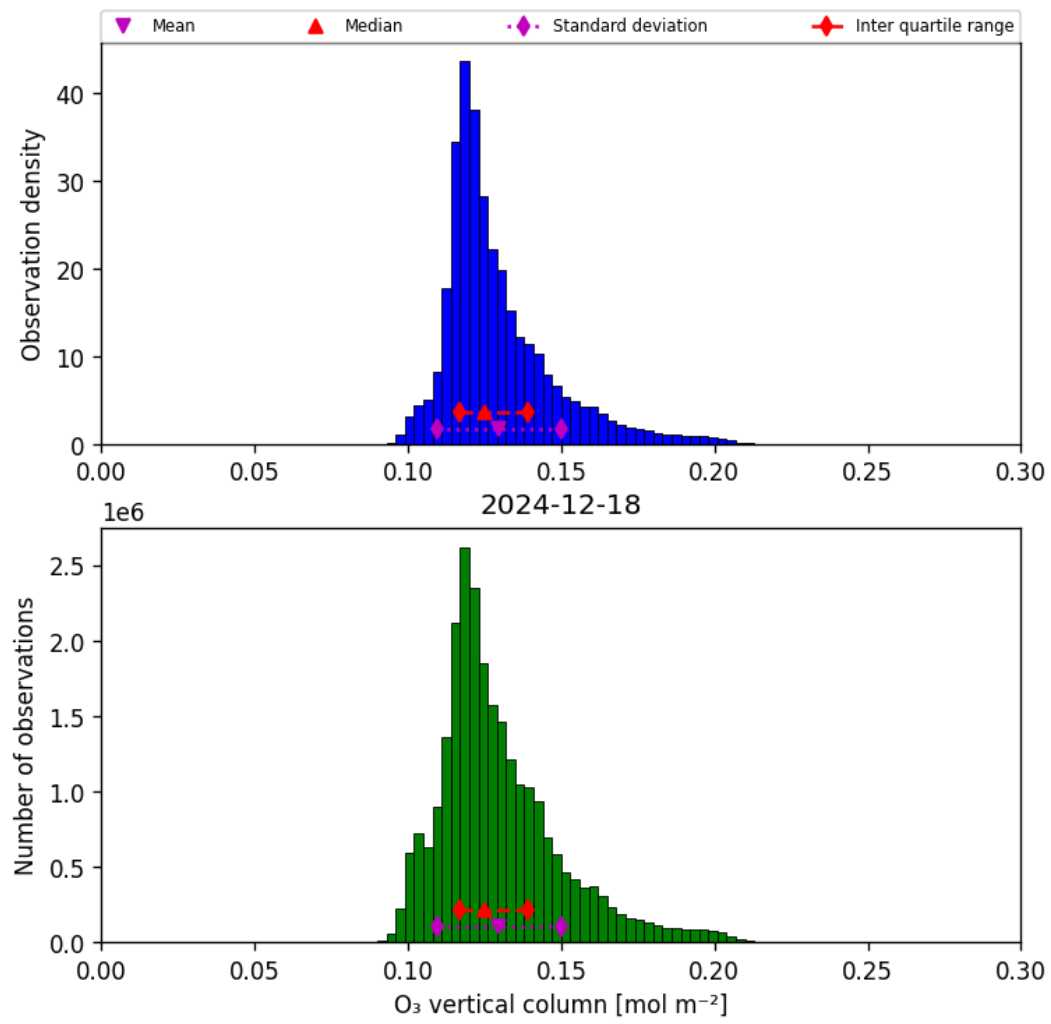
Figure 21: Histogram of “O 3 vertical column” for 2024-12-17 to 2024-12-19
