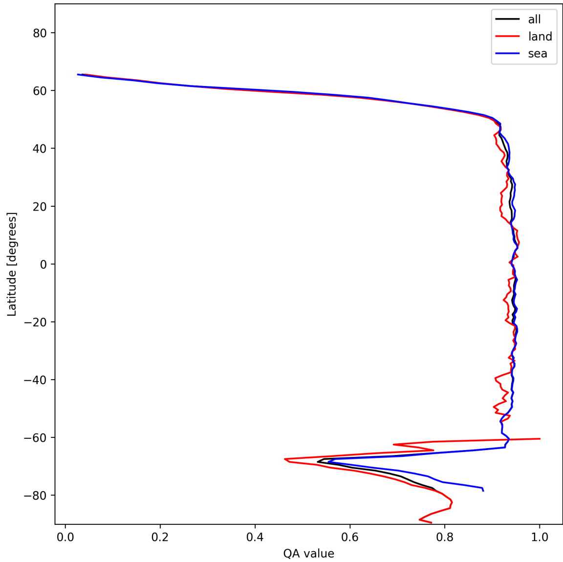
Figure 13: Zonal average of “QA value” for 2024-12-17 to 2024-12-19.
