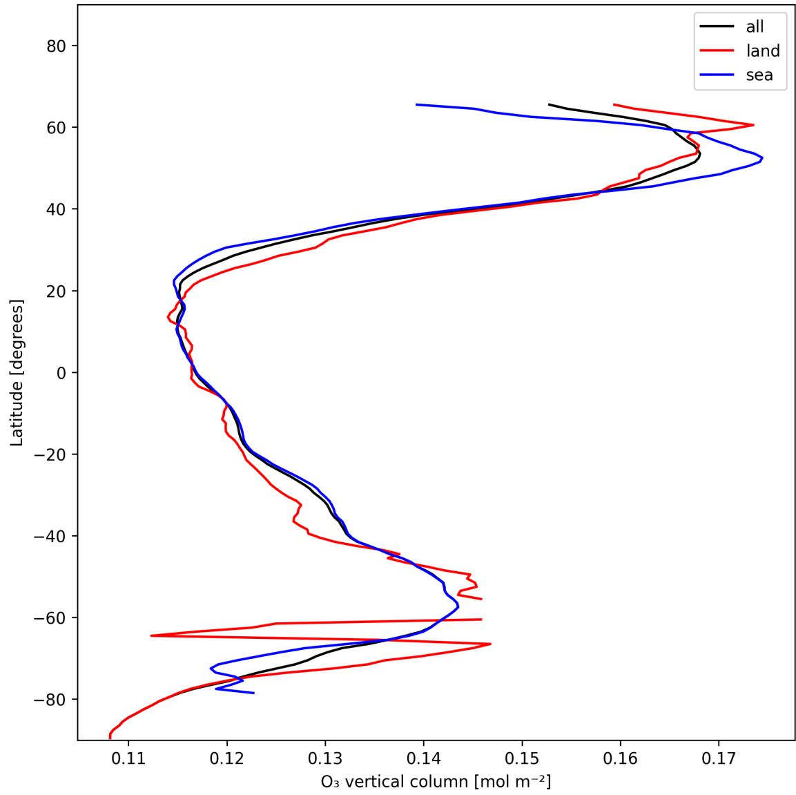
Figure 14: Zonal average of “O 3 vertical column” for 2024-12-18 to 2024-12-20.
