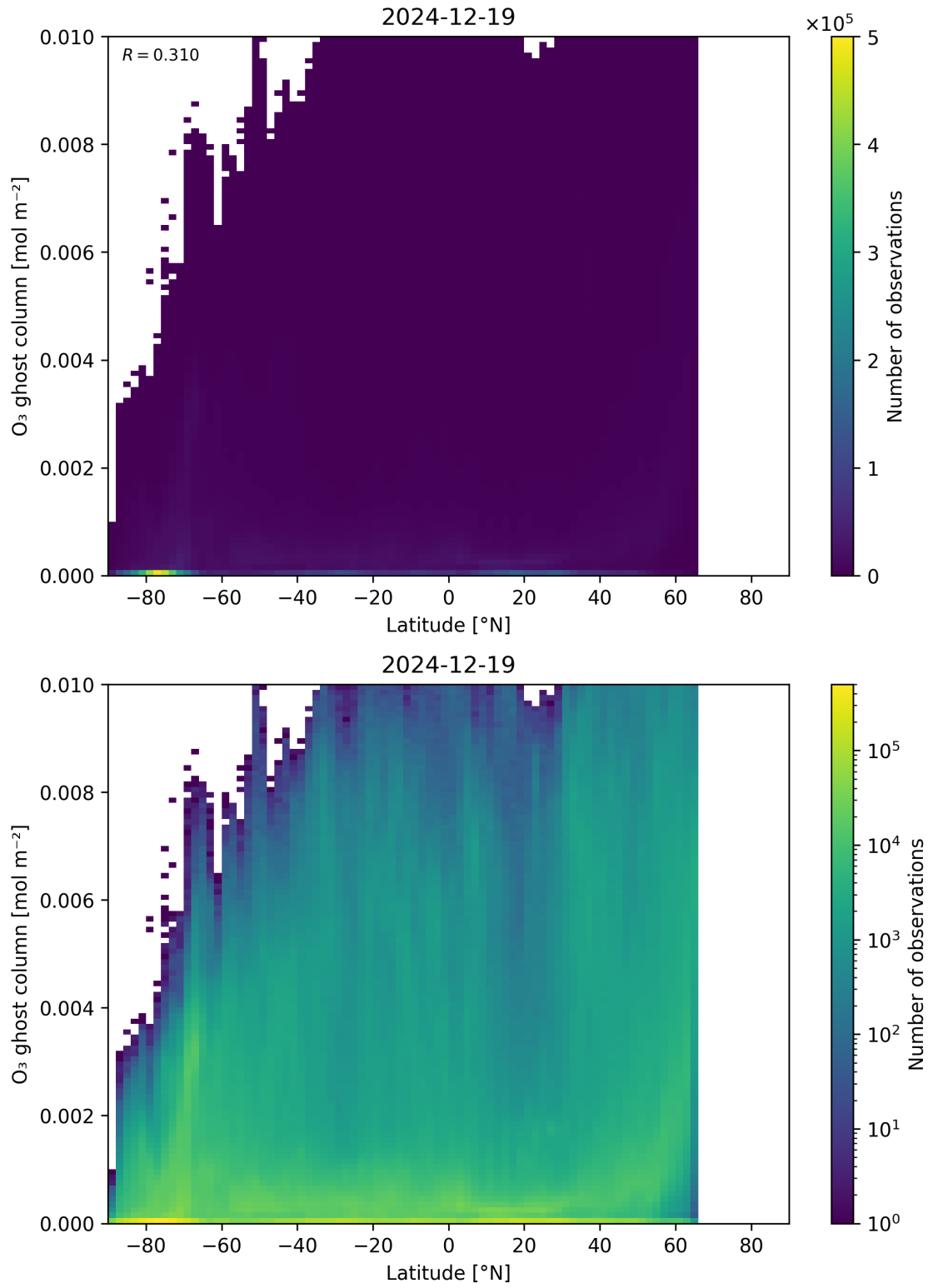
Figure 35: Scatter density plot of “Latitude” against “O 3 ghost column” for 2024-12-18 to 2024-12-20.
