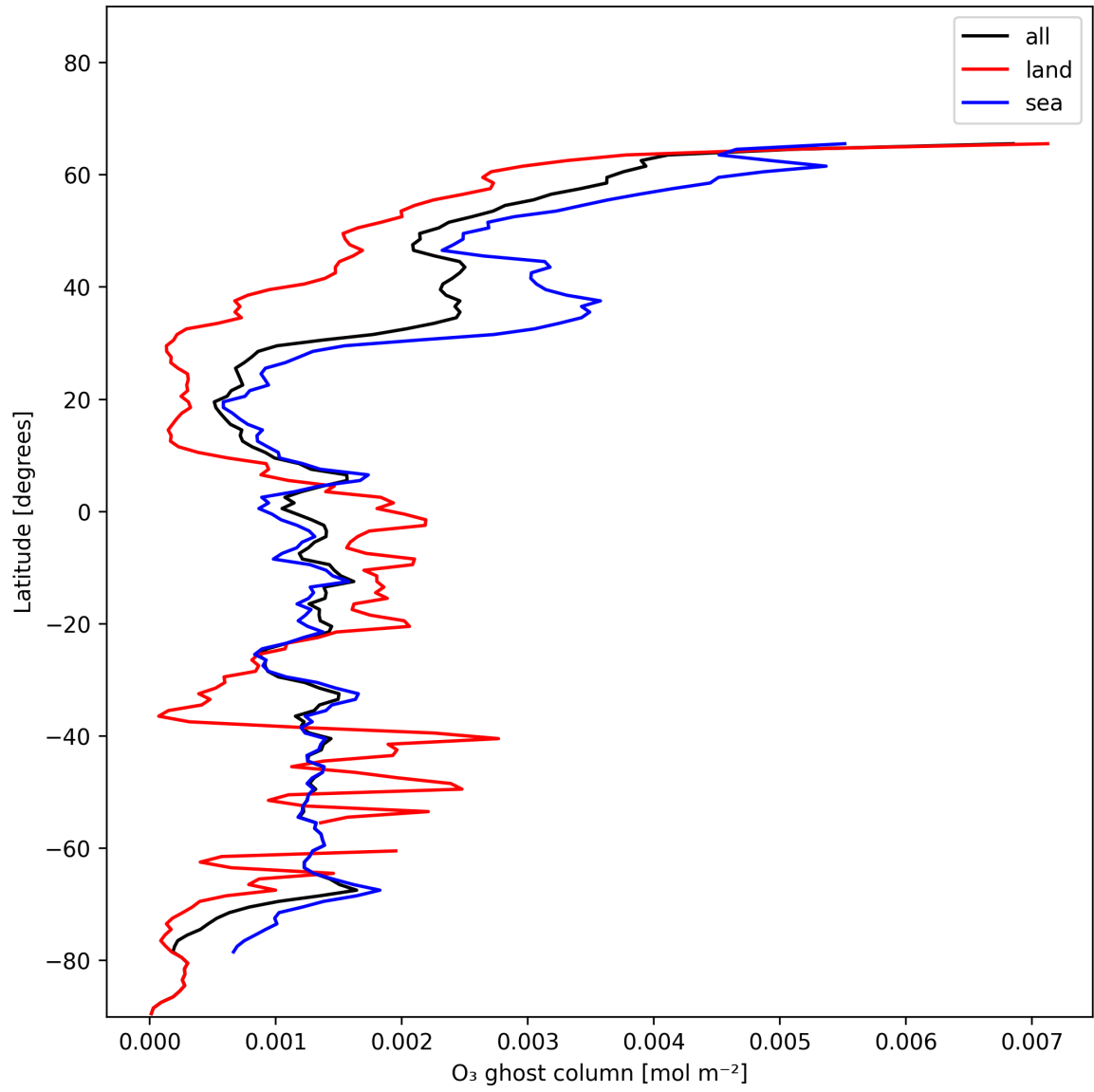
Figure 18: Zonal average of “O 3 ghost column” for 2024-12-18 to 2024-12-20.
