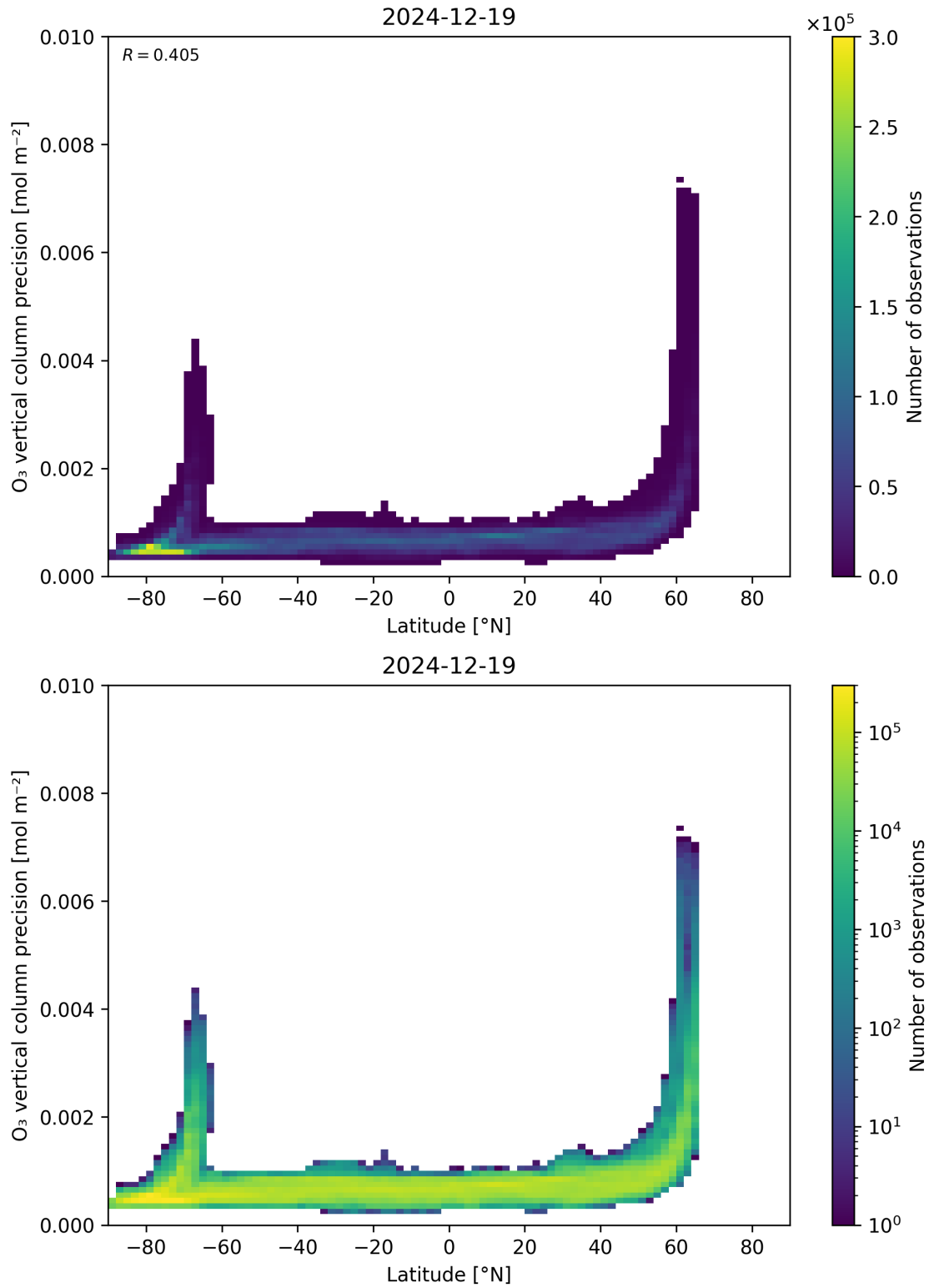
Figure 37: Scatter density plot of “Latitude” against “O 3 vertical column precision” for 2024-12-18 to 2024-12-20.
