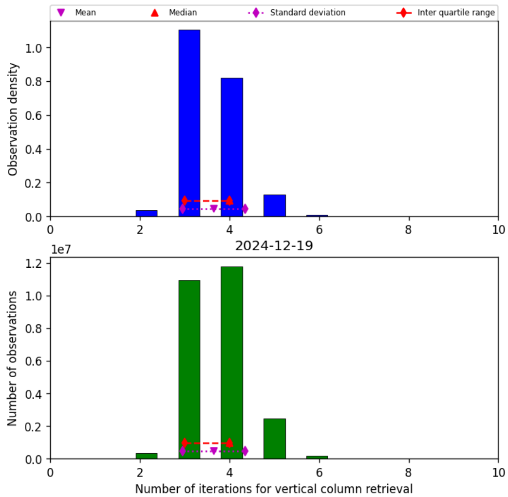
Figure 26: Histogram of “Number of iterations for vertical column retrieval” for 2024-12-18 to 2024-12-20
