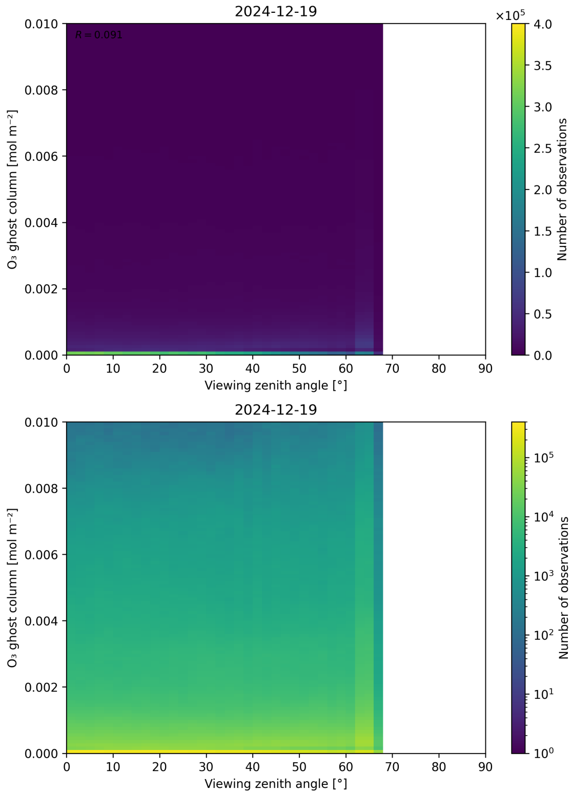
Figure 51: Scatter density plot of “Viewing zenith angle” against “O 3 ghost column” for 2024-12-18 to 2024-12-20.
