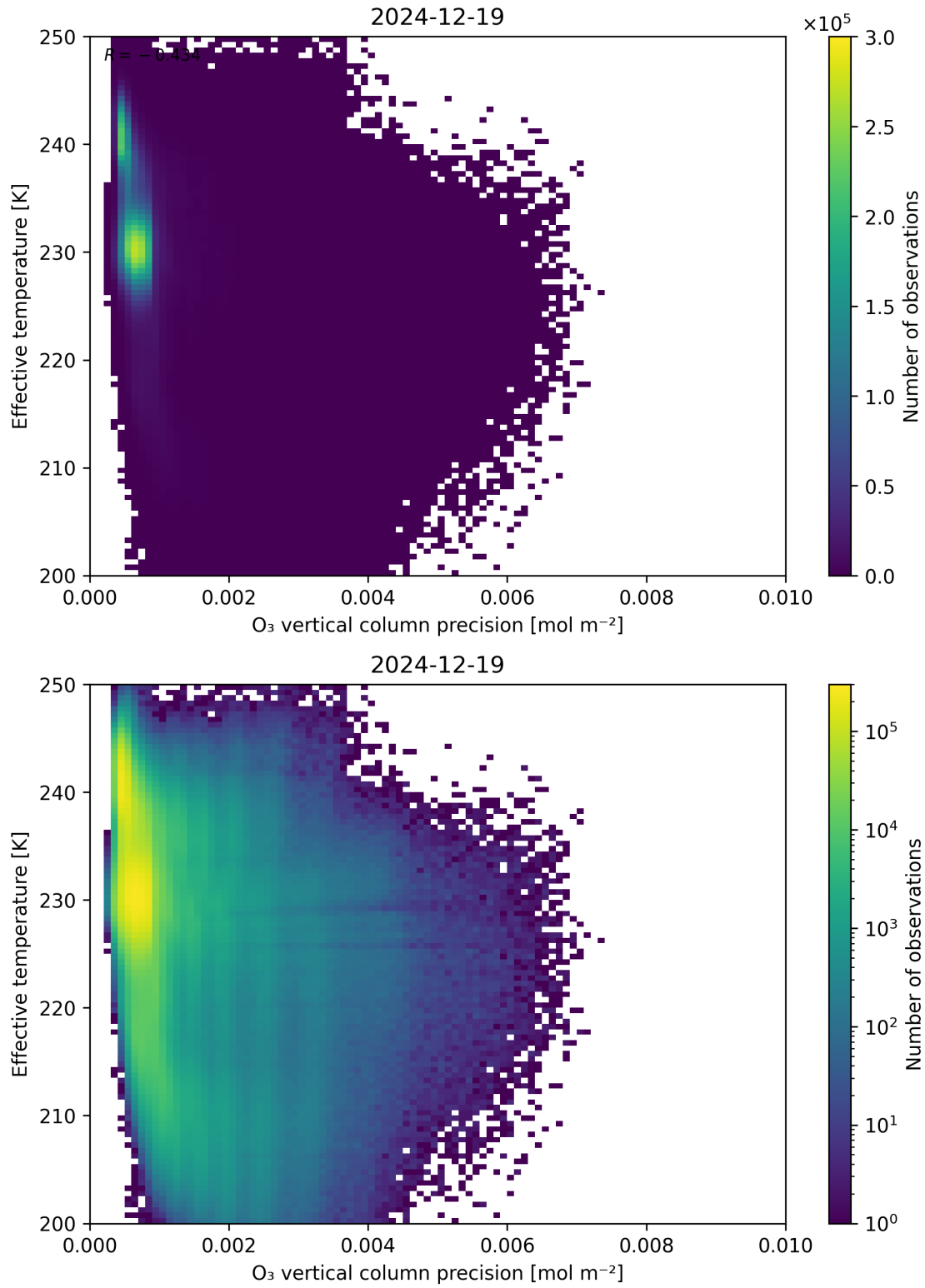
Figure 42: Scatter density plot of “O 3 vertical column precision” against “Effective temperature” for 2024-12-18 to 2024-12-20.
