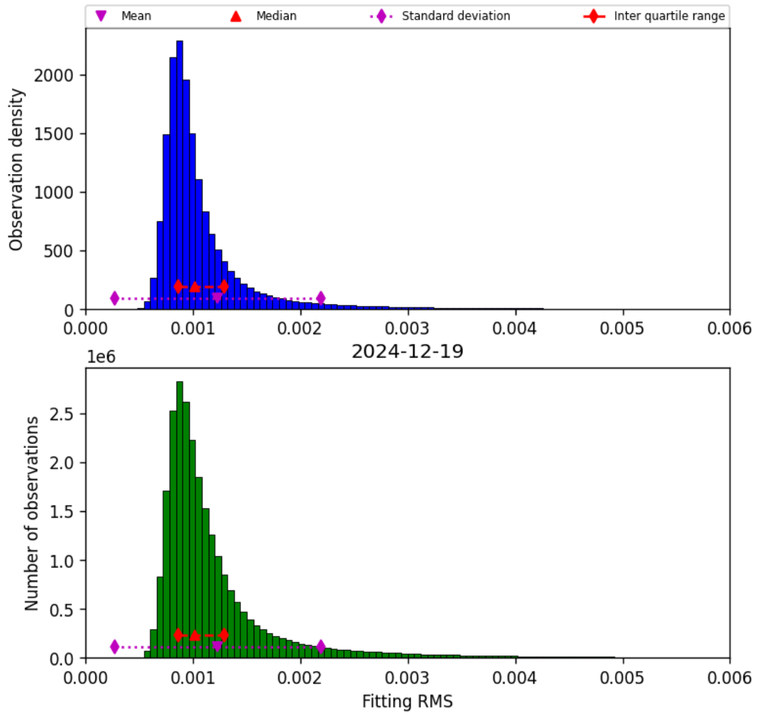
Figure 23: Histogram of “Fitting RMS” for 2024-12-18 to 2024-12-20
