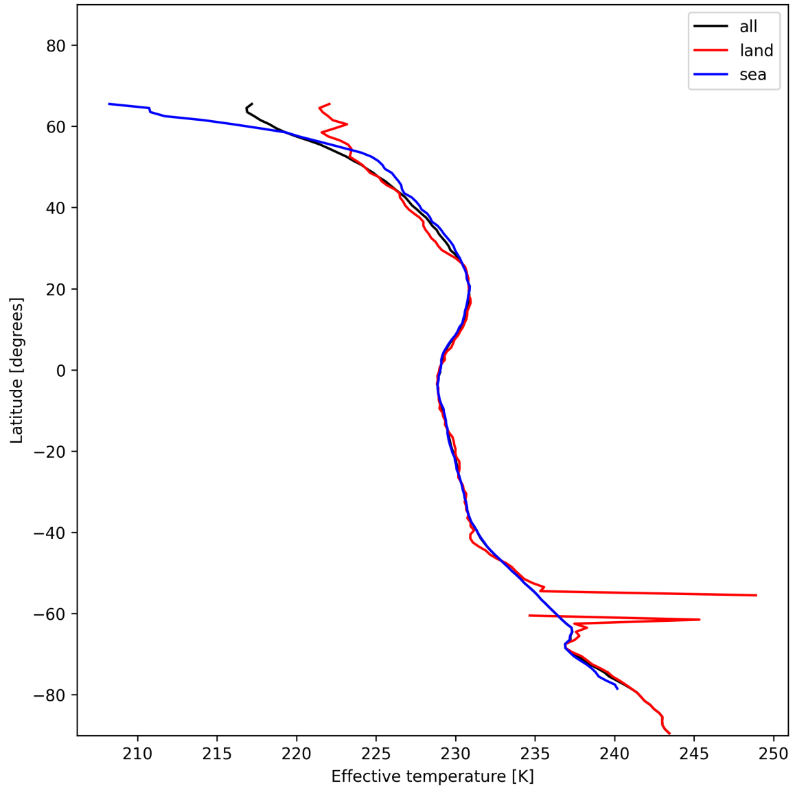
Figure 17: Zonal average of “Effective temperature” for 2024-12-18 to 2024-12-20.
