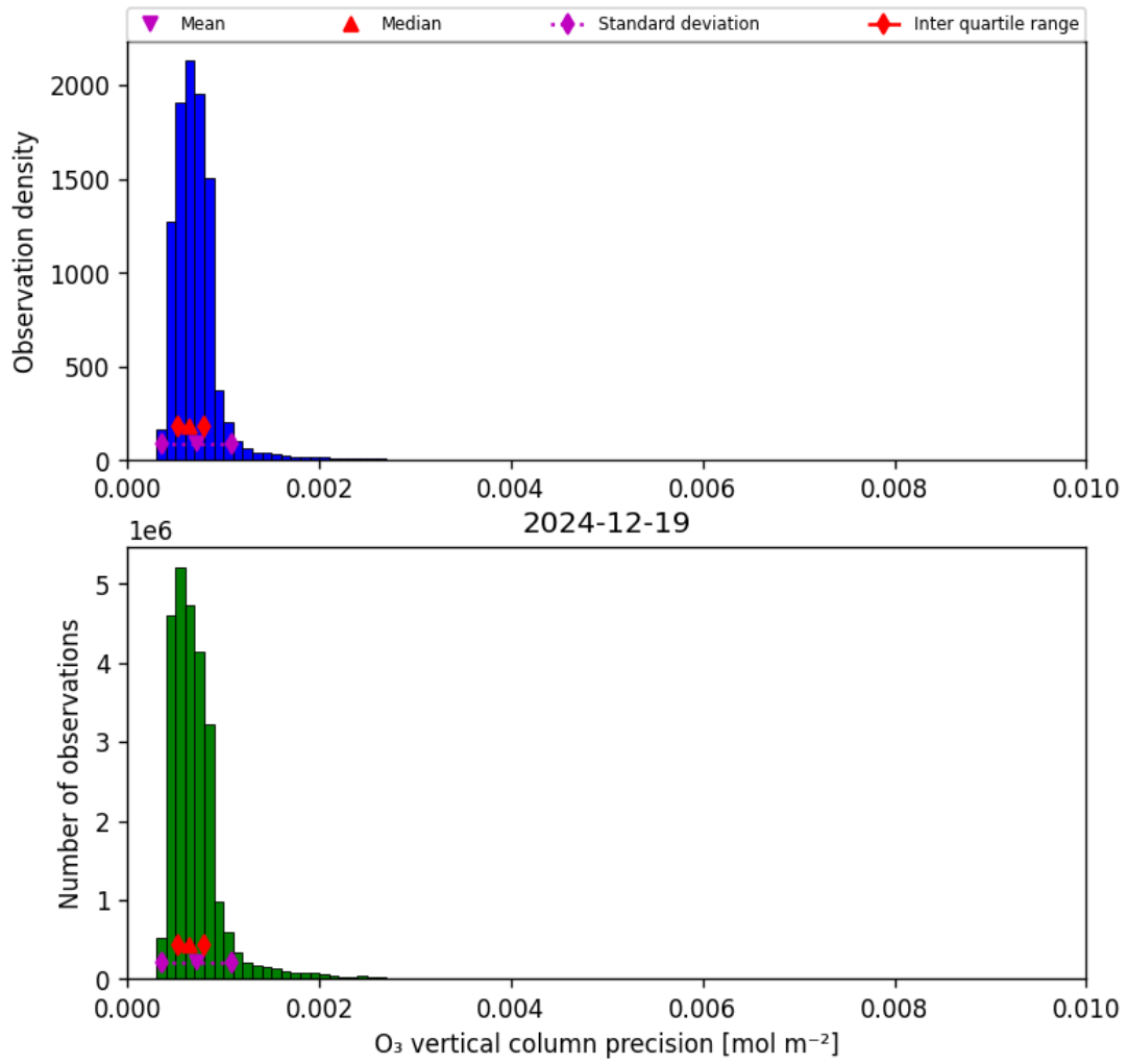
Figure 22: Histogram of “O 3 vertical column precision” for 2024-12-18 to 2024-12-20
