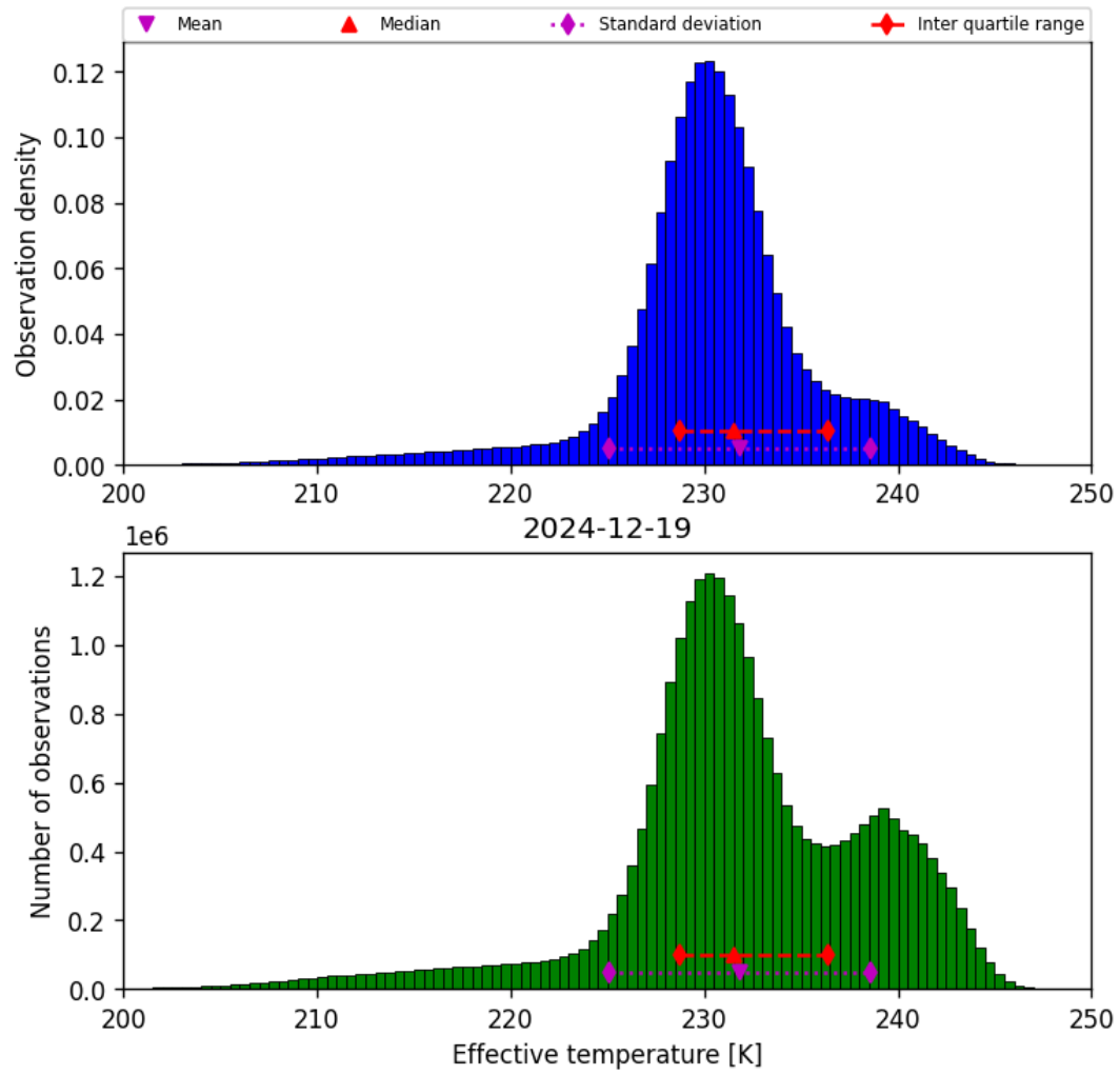
Figure 24: Histogram of “Effective temperature” for 2024-12-18 to 2024-12-20
