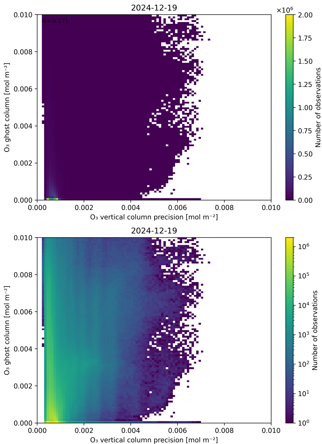
Figure 43: Scatter density plot of “O 3 vertical column precision” against “O 3 ghost column” for 2024-12-18 to 2024-12-20.
