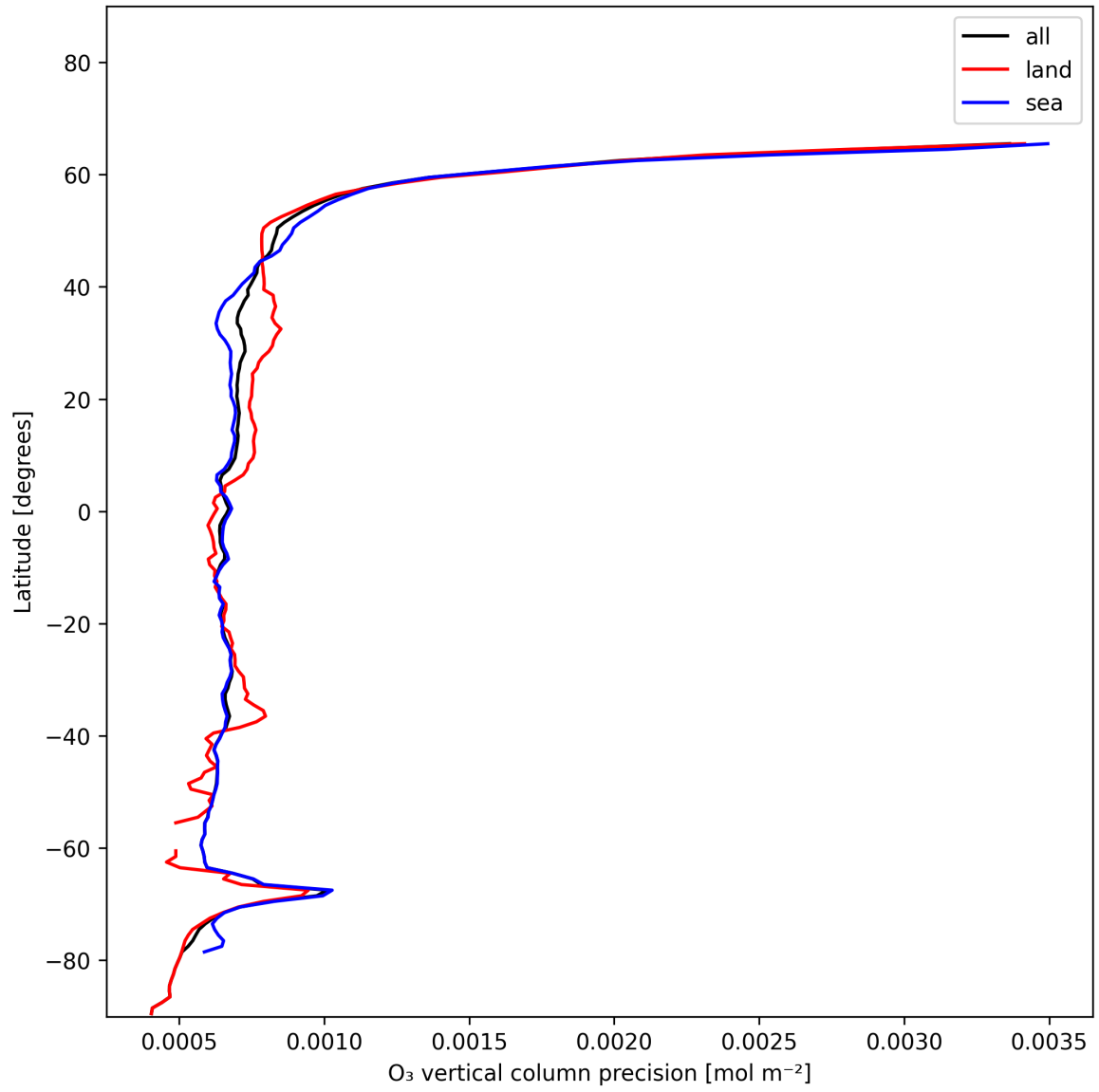
Figure 15: Zonal average of “O 3 vertical column precision” for 2024-12-18 to 2024-12-20.
