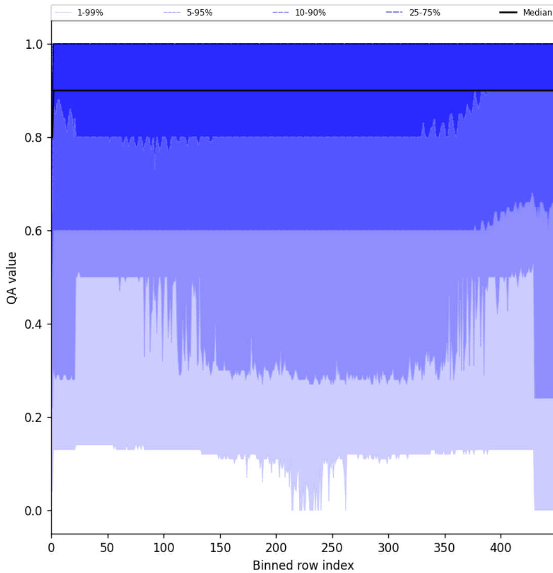
Figure 27: Along track statistics of “QA value” for 2024-12-18 to 2024-12-20
