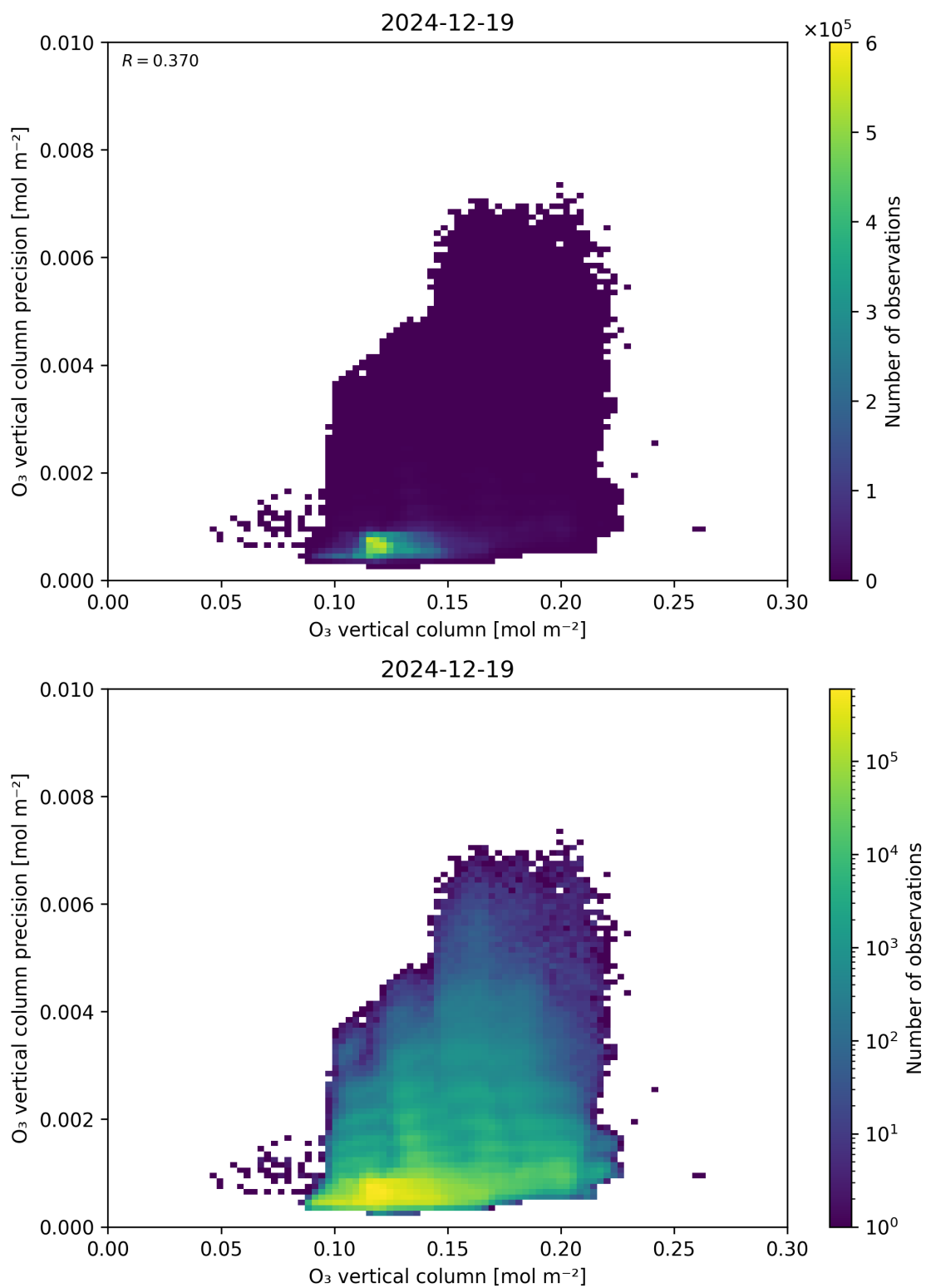
Figure 41: Scatter density plot of “O 3 vertical column” against “O 3 vertical column precision” for 2024-12-18 to 2024-12-20.
