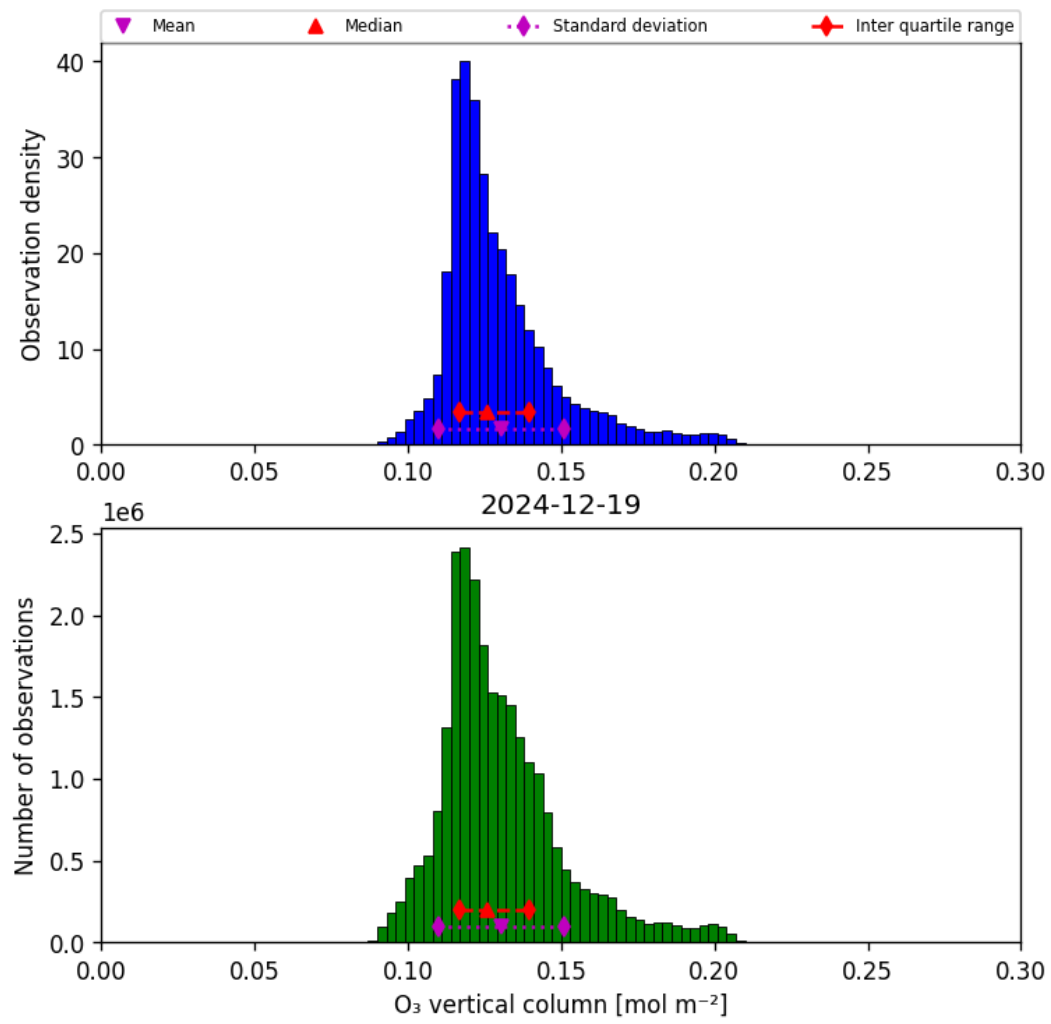
Figure 21: Histogram of “O 3 vertical column” for 2024-12-18 to 2024-12-20
