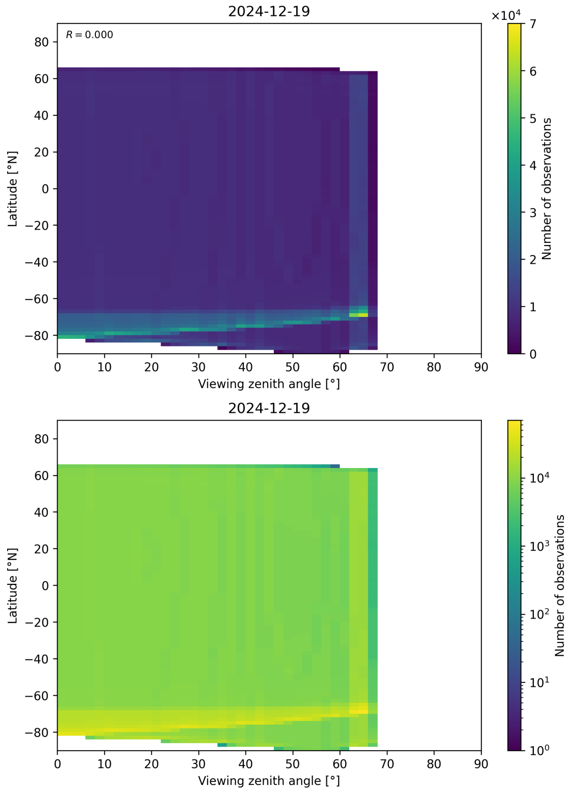
Figure 49: Scatter density plot of “Viewing zenith angle” against “Latitude” for 2024-12-18 to 2024-12-20.
