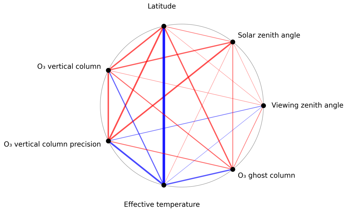
Figure 1: Map of correlation graph for 2024-12-18 to 2024-12-20.
