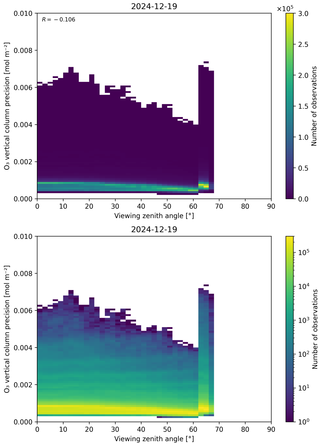
Figure 53: Scatter density plot of “Viewing zenith angle” against “O 3 vertical column precision” for 2024-12-18 to 2024-12-20.
