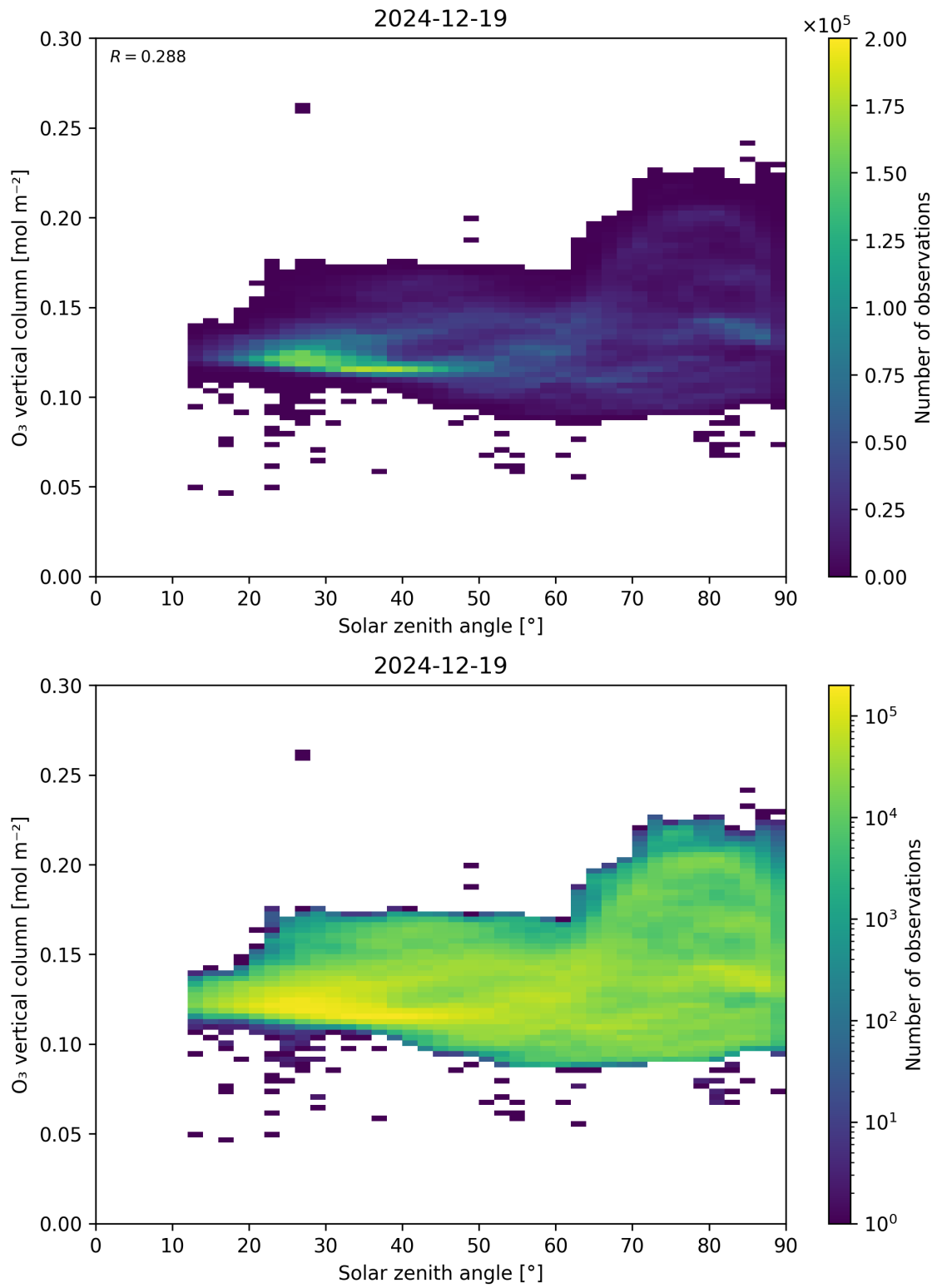
Figure 47: Scatter density plot of “Solar zenith angle” against “O 3 vertical column” for 2024-12-18 to 2024-12-20.
