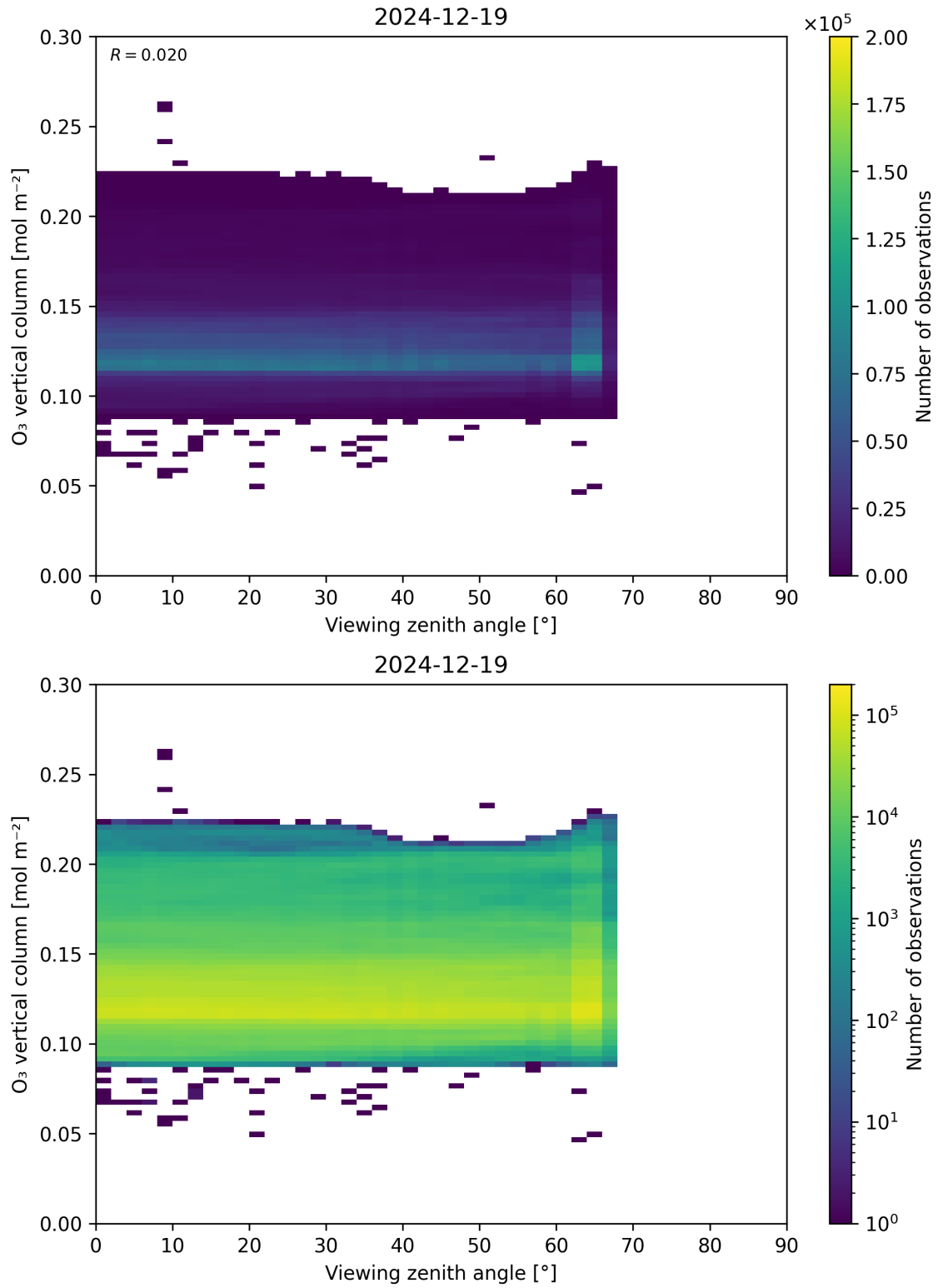
Figure 52: Scatter density plot of “Viewing zenith angle” against “O 3 vertical column” for 2024-12-18 to 2024-12-20.
