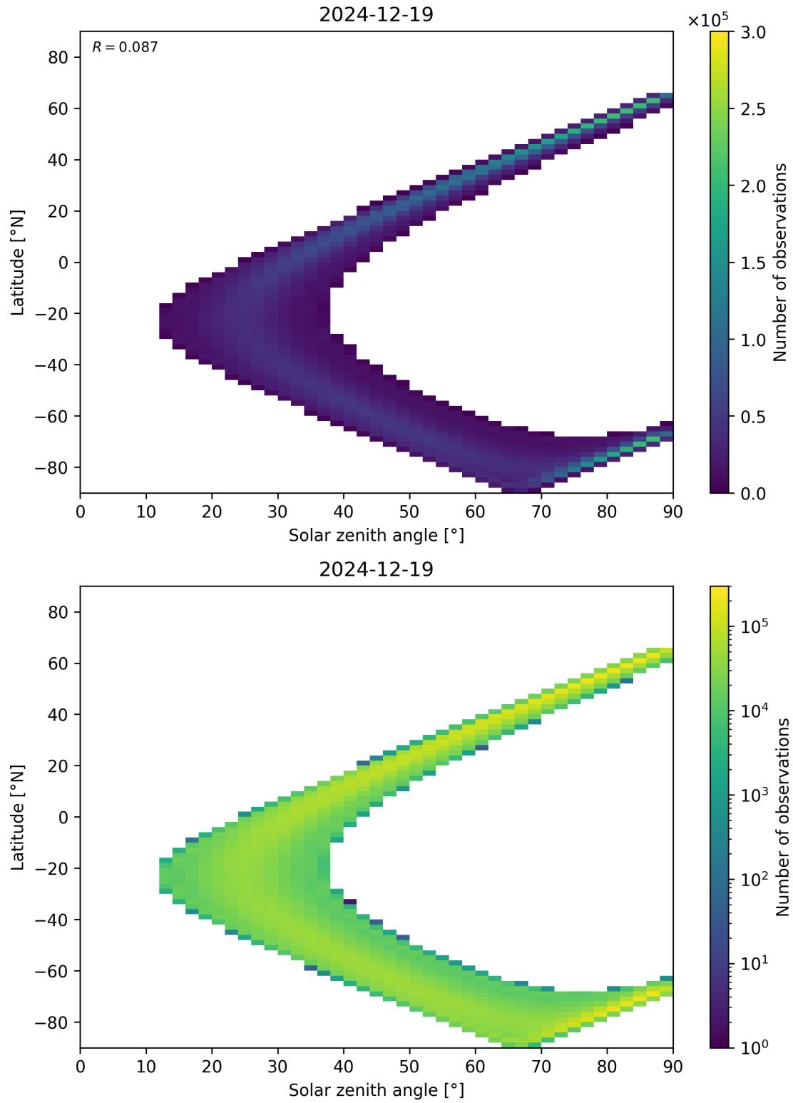
Figure 44: Scatter density plot of “Solar zenith angle” against “Latitude” for 2024-12-18 to 2024-12-20.
