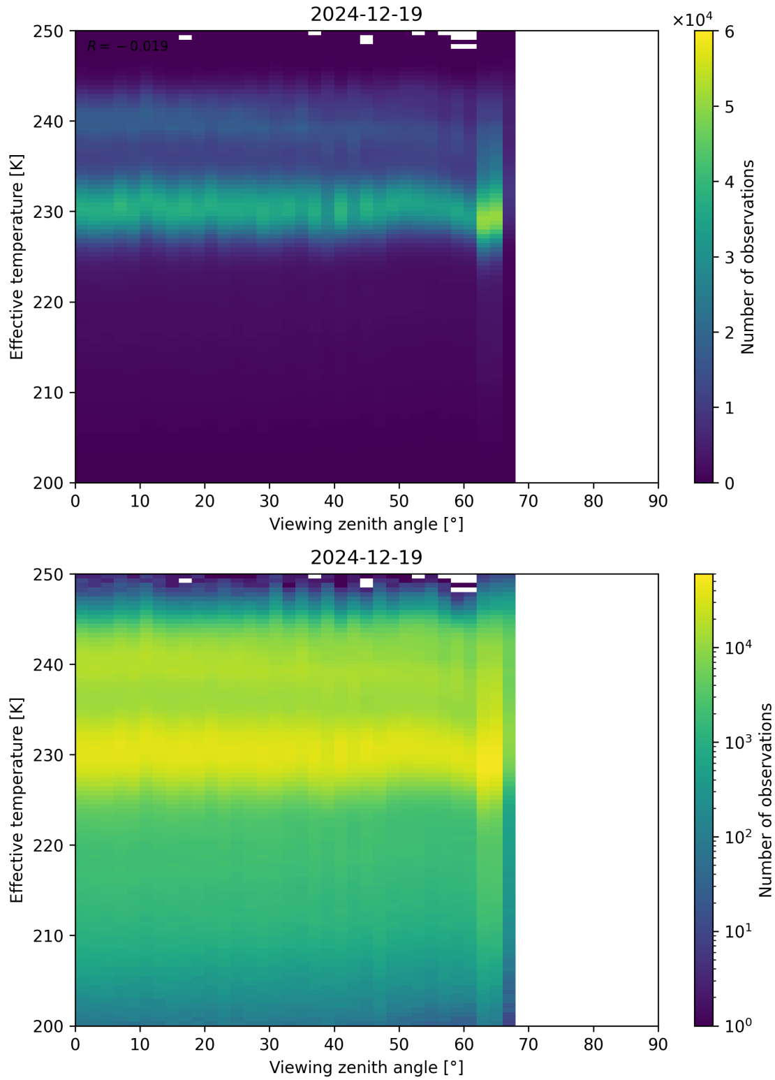
Figure 50: Scatter density plot of “Viewing zenith angle” against “Effective temperature” for 2024-12-18 to 2024-12-20.
