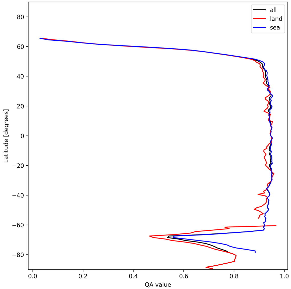
Figure 13: Zonal average of “QA value” for 2024-12-18 to 2024-12-20.
