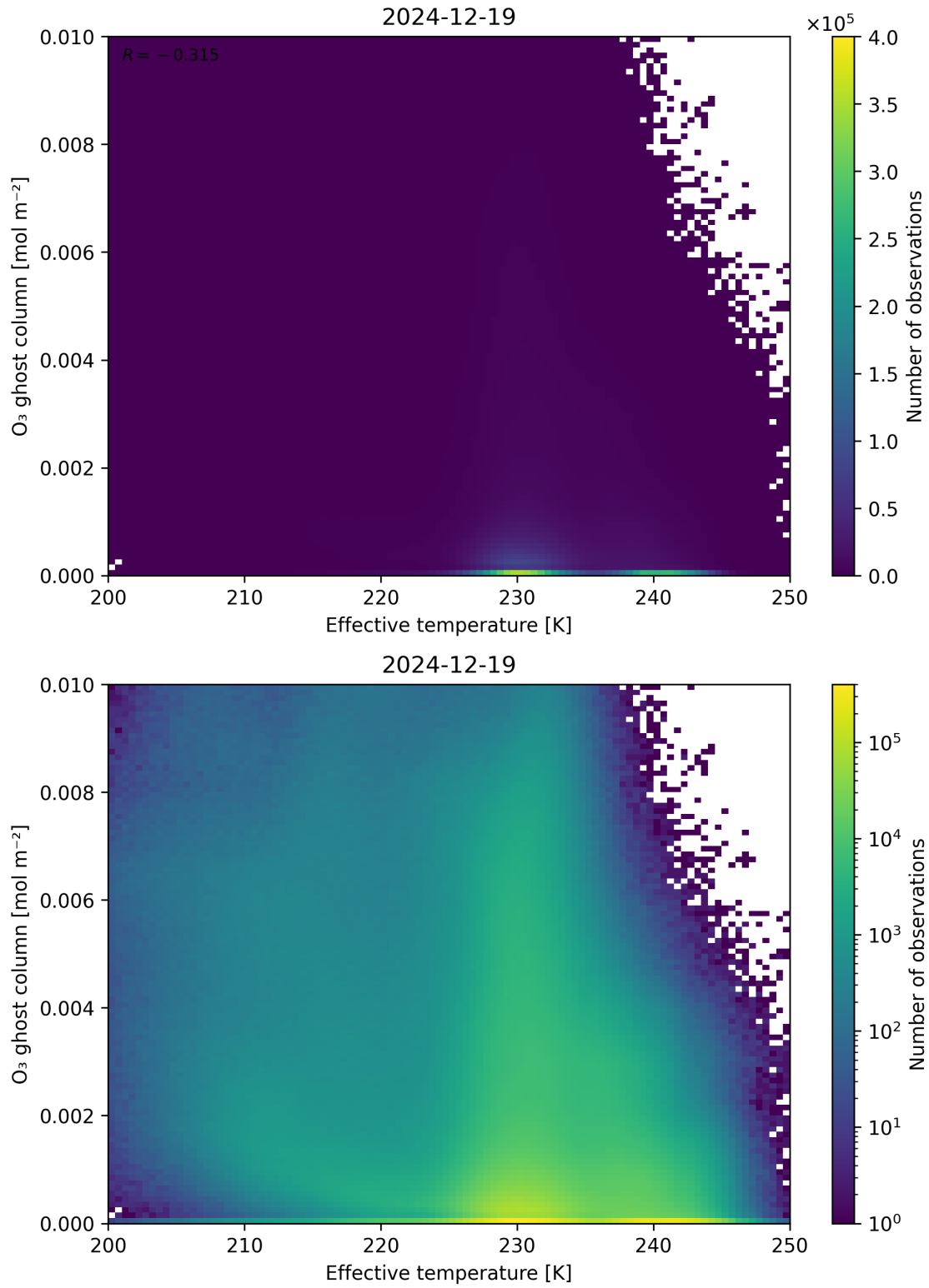
Figure 38: Scatter density plot of “Effective temperature” against “O 3 ghost column” for 2024-12-18 to 2024-12-20.
