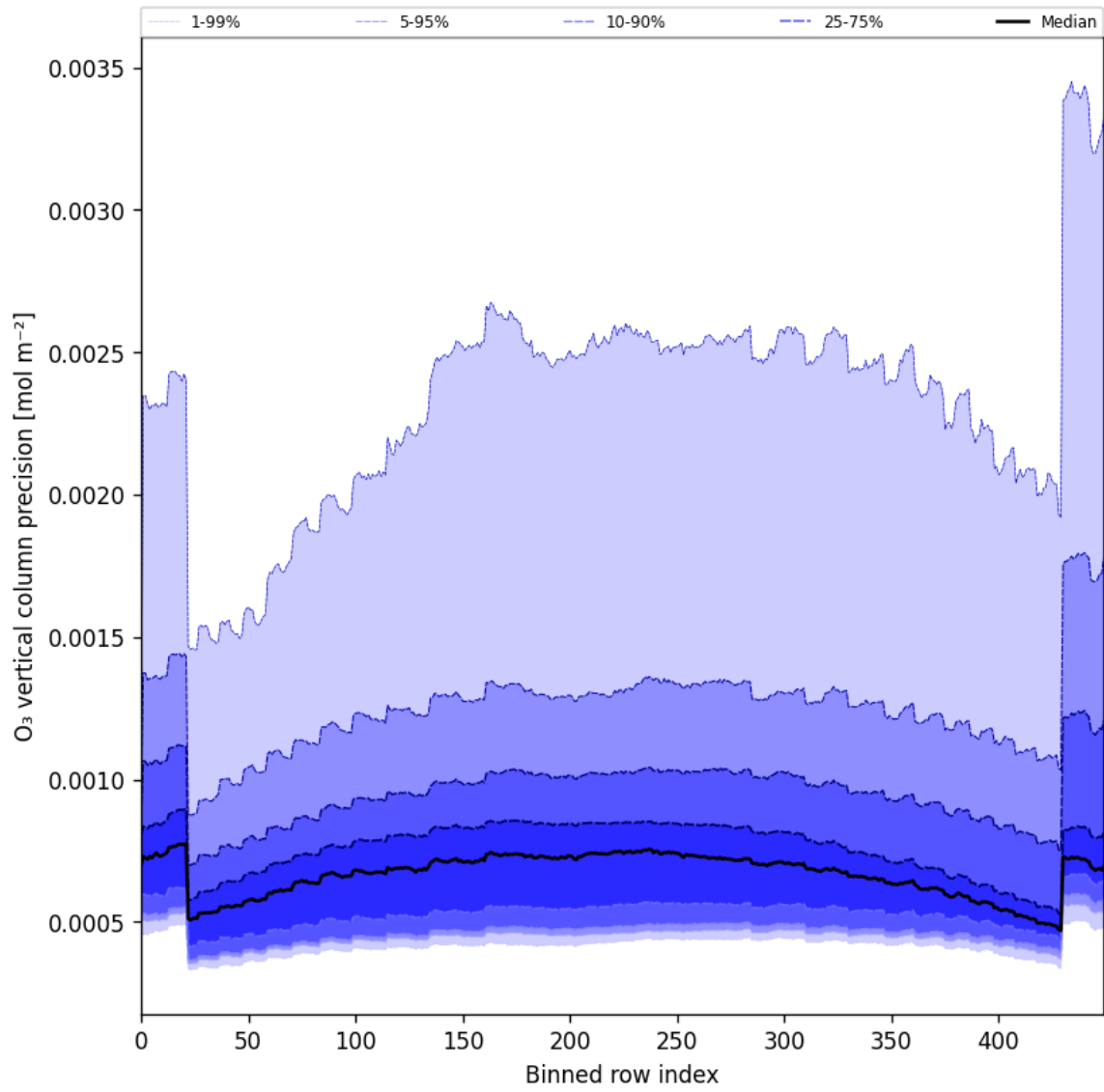
Figure 29: Along track statistics of “O 3 vertical column precision” for 2024-12-18 to 2024-12-20
