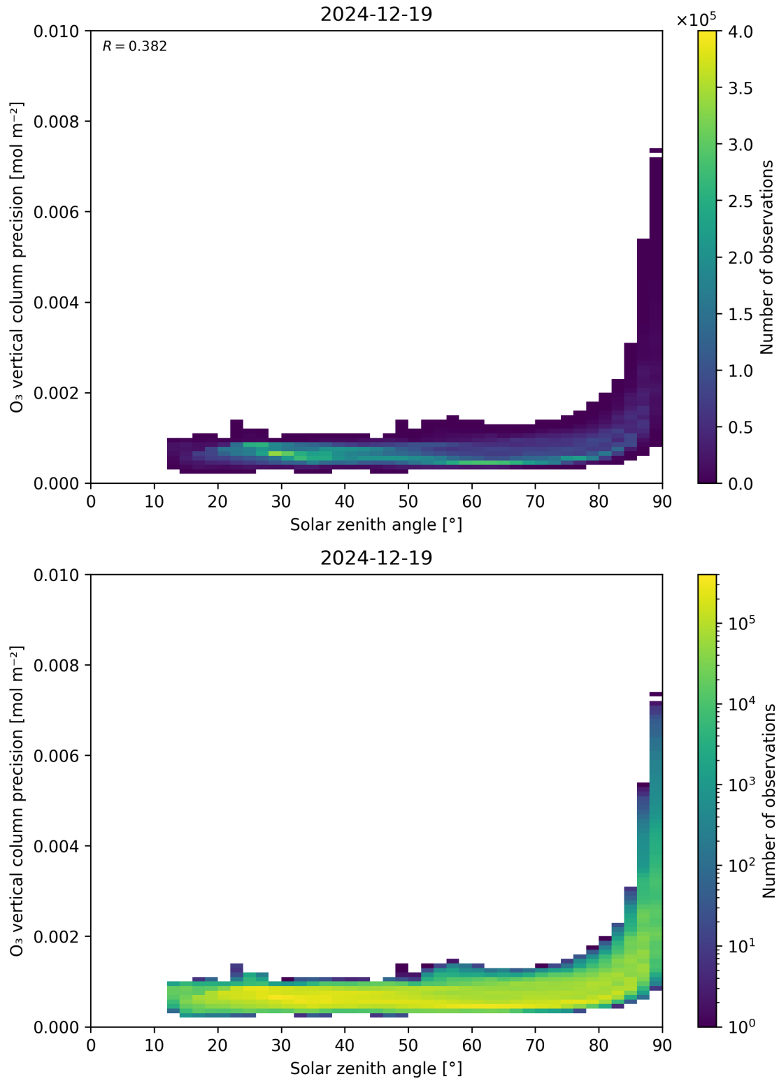
Figure 48: Scatter density plot of “Solar zenith angle” against “O 3 vertical column precision” for 2024-12-18 to 2024-12-20.
