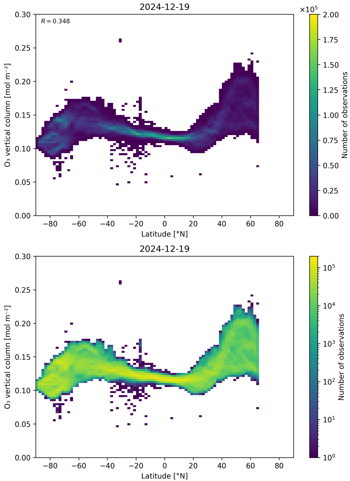
Figure 36: Scatter density plot of “Latitude” against “O 3 vertical column” for 2024-12-18 to 2024-12-20.
