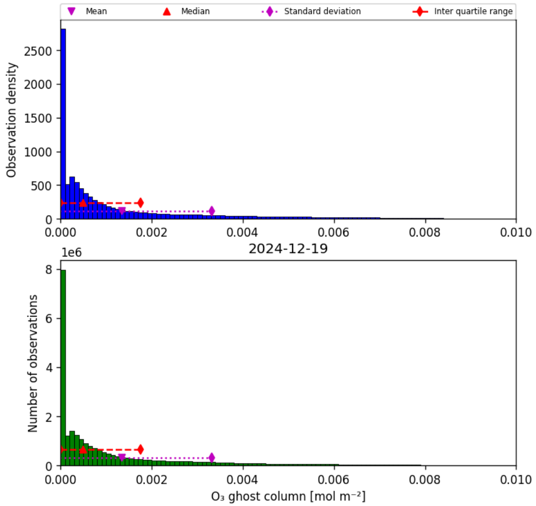
Figure 25: Histogram of “O 3 ghost column” for 2024-12-18 to 2024-12-20
