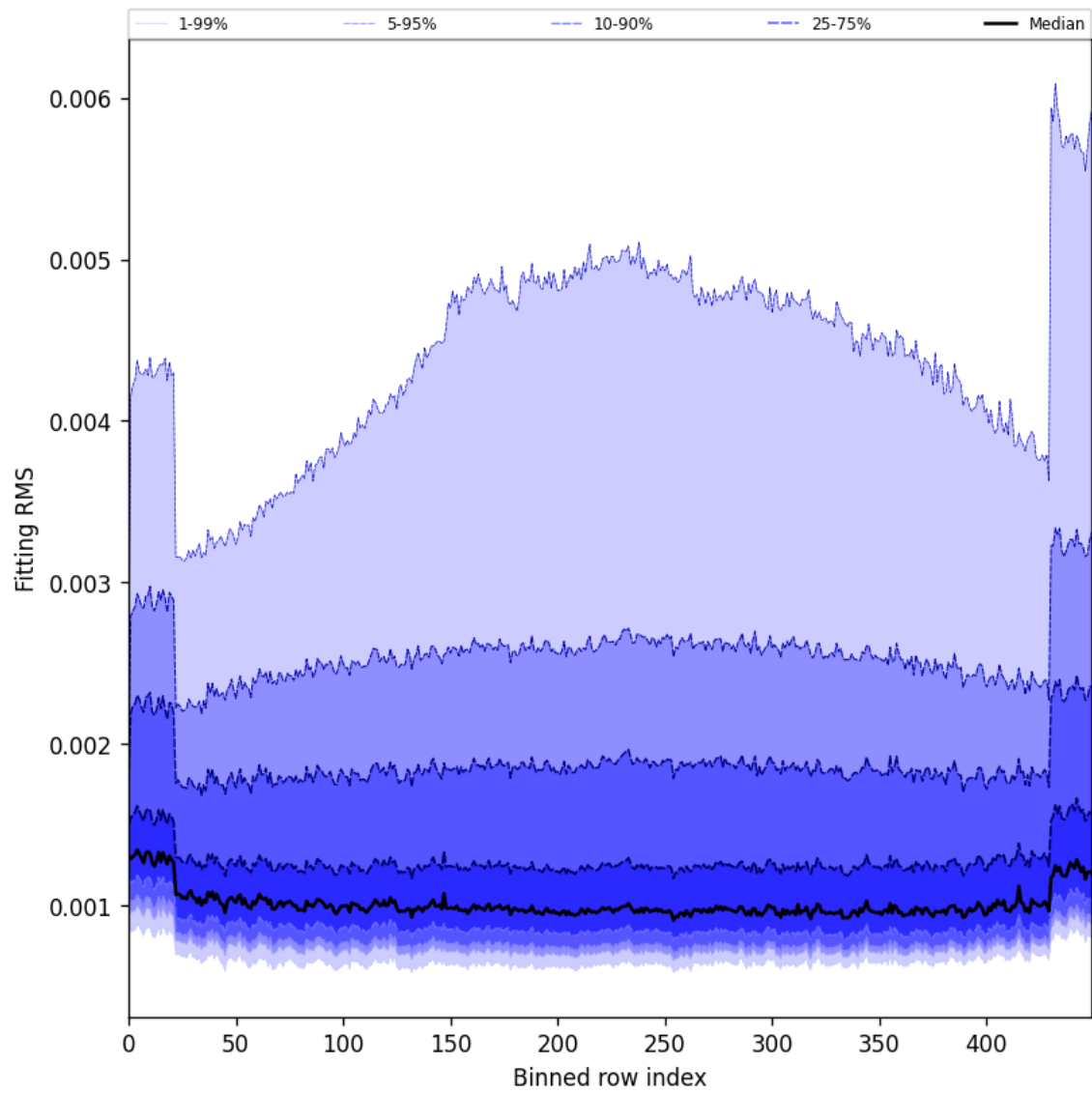
Figure 30: Along track statistics of “Fitting RMS” for 2024-12-18 to 2024-12-20
