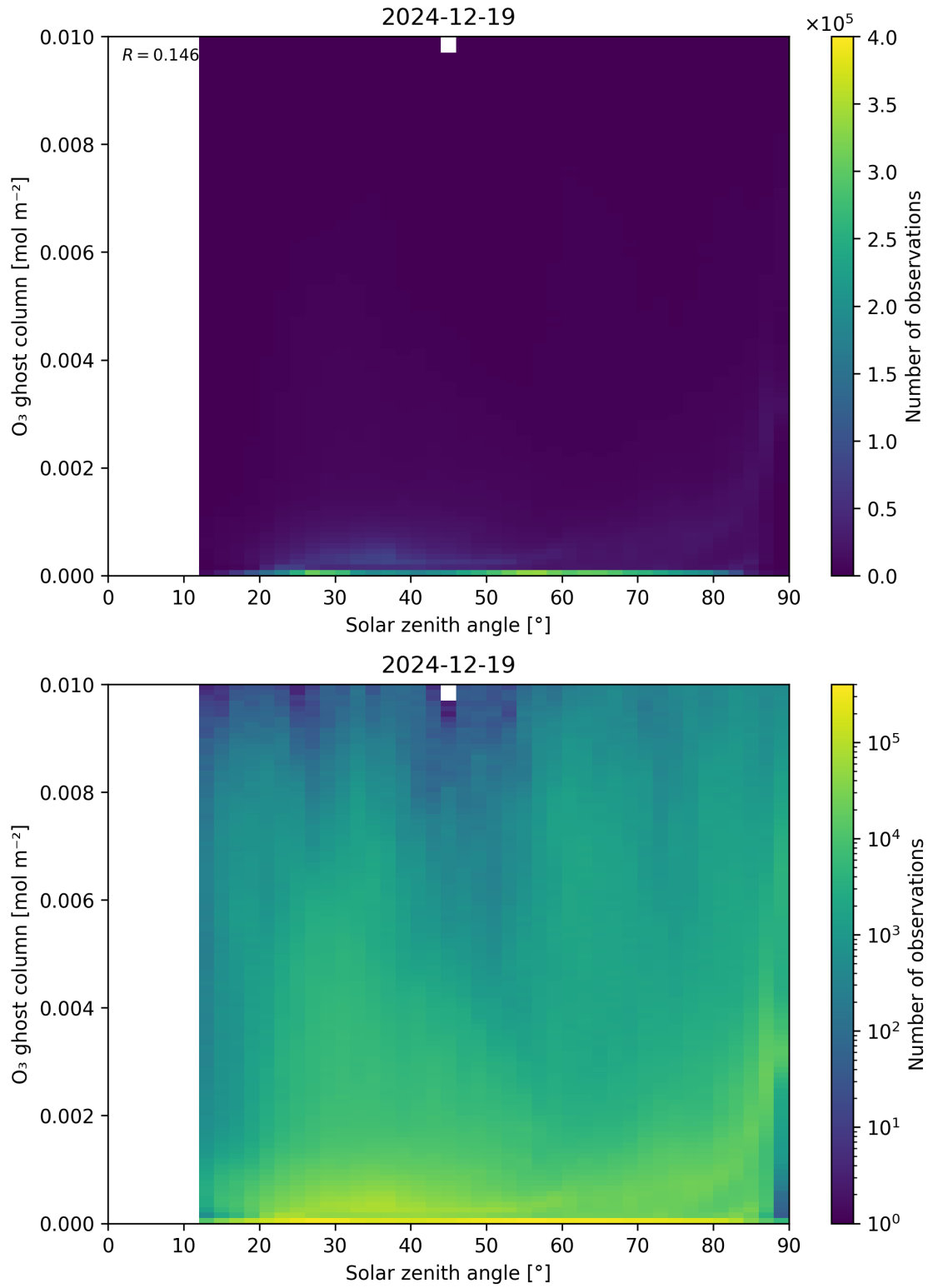
Figure 46: Scatter density plot of “Solar zenith angle” against “O 3 ghost column” for 2024-12-18 to 2024-12-20.
