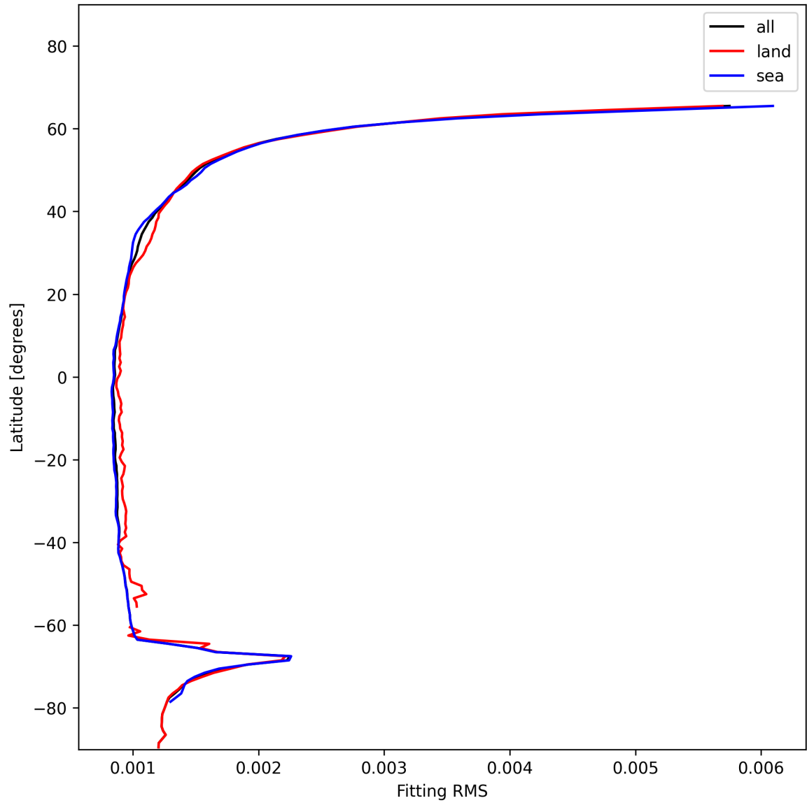
Figure 16: Zonal average of “Fitting RMS” for 2024-12-18 to 2024-12-20.
