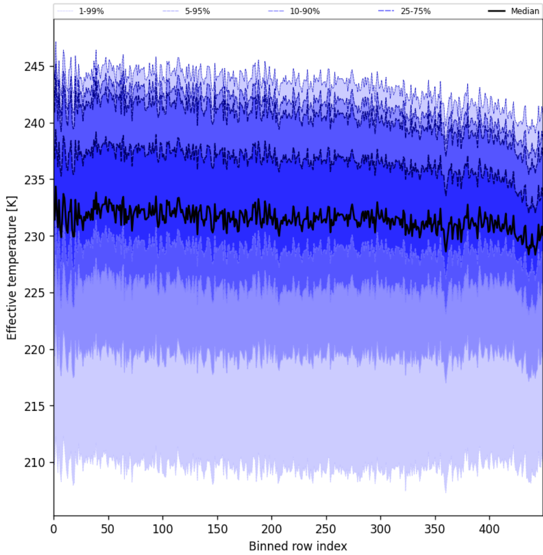
Figure 31: Along track statistics of “Effective temperature” for 2024-12-18 to 2024-12-20
