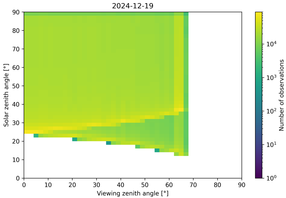
Figure 54: Scatter density plot of “Viewing zenith angle” against “Solar zenith angle” for 2024-12-18 to 2024-12-20.
