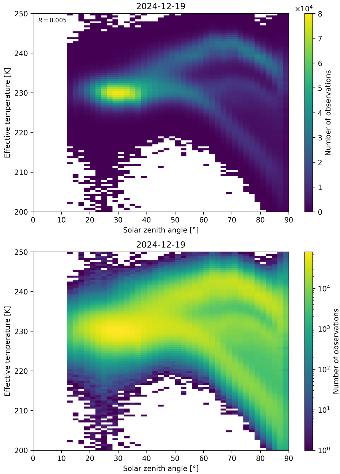
Figure 45: Scatter density plot of “Solar zenith angle” against “Effective temperature” for 2024-12-18 to 2024-12-20.
