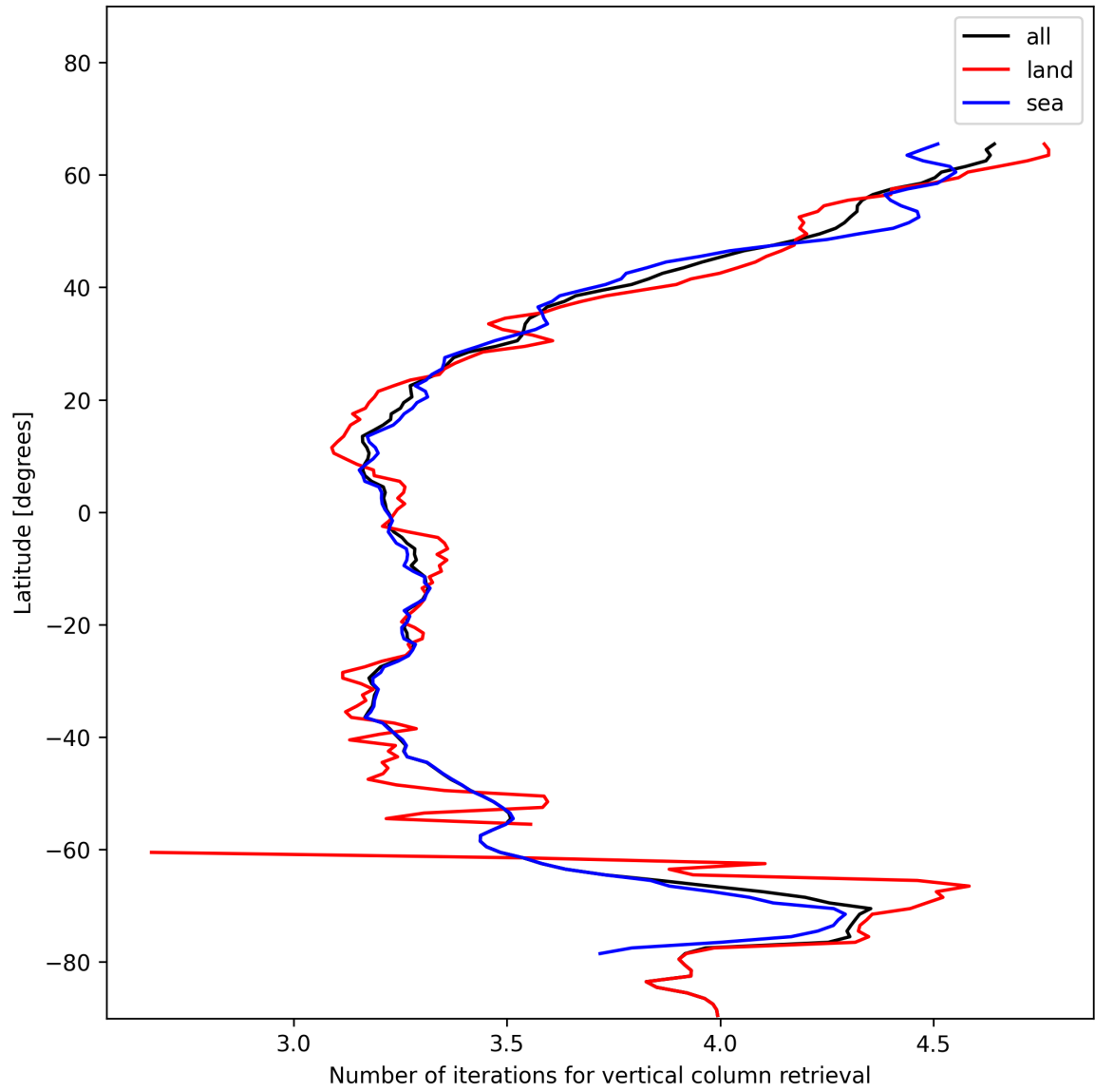
Figure 19: Zonal average of “Number of iterations for vertical column retrieval” for 2024-12-18 to 2024-12-20.
