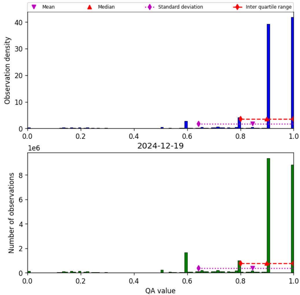
Figure 20: Histogram of “QA value” for 2024-12-18 to 2024-12-20
