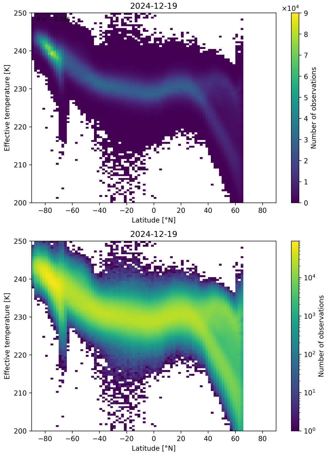
Figure 34: Scatter density plot of “Latitude” against “Effective temperature” for 2024-12-18 to 2024-12-20.
