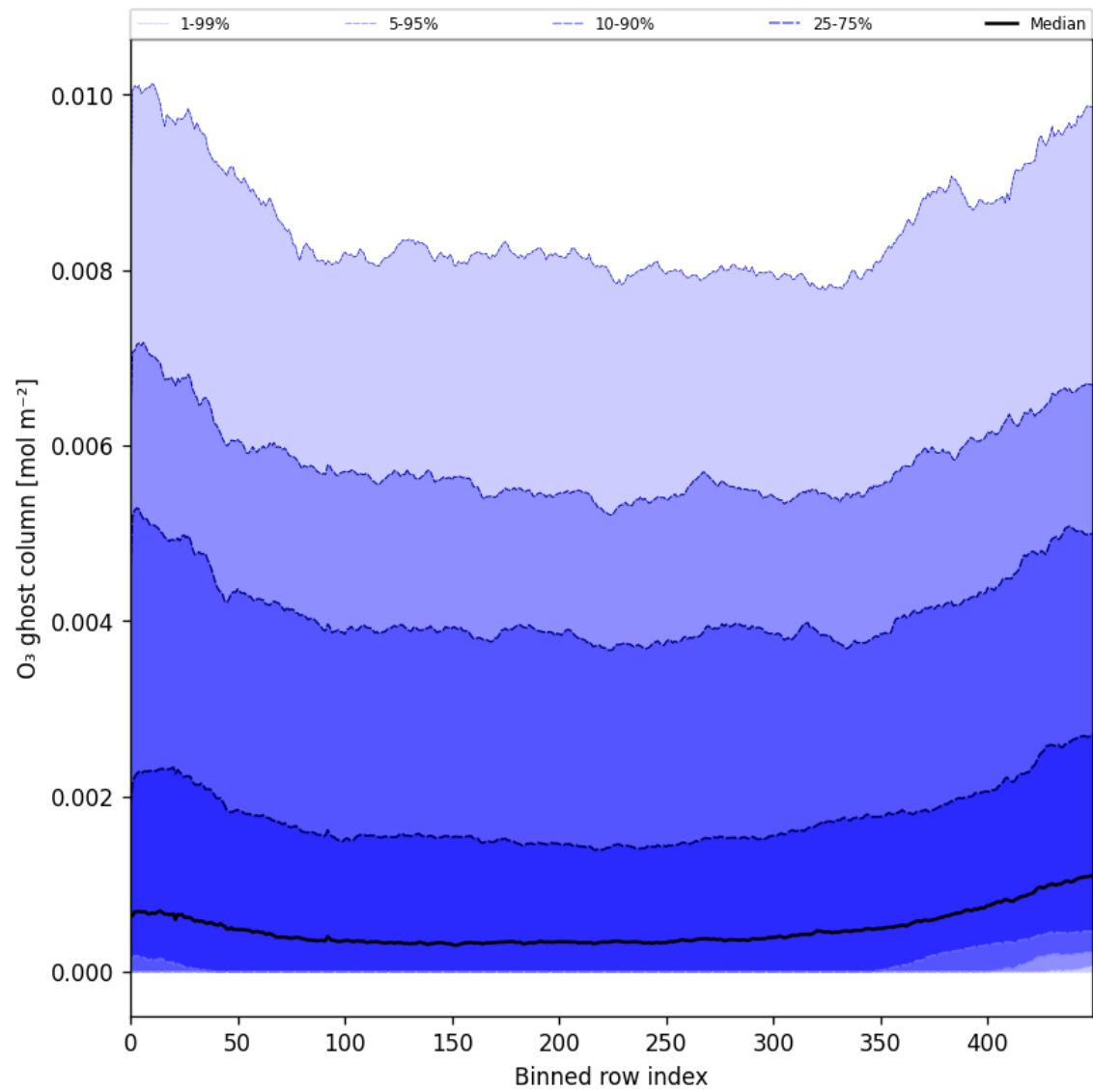
Figure 32: Along track statistics of “O 3 ghost column” for 2024-12-18 to 2024-12-20
