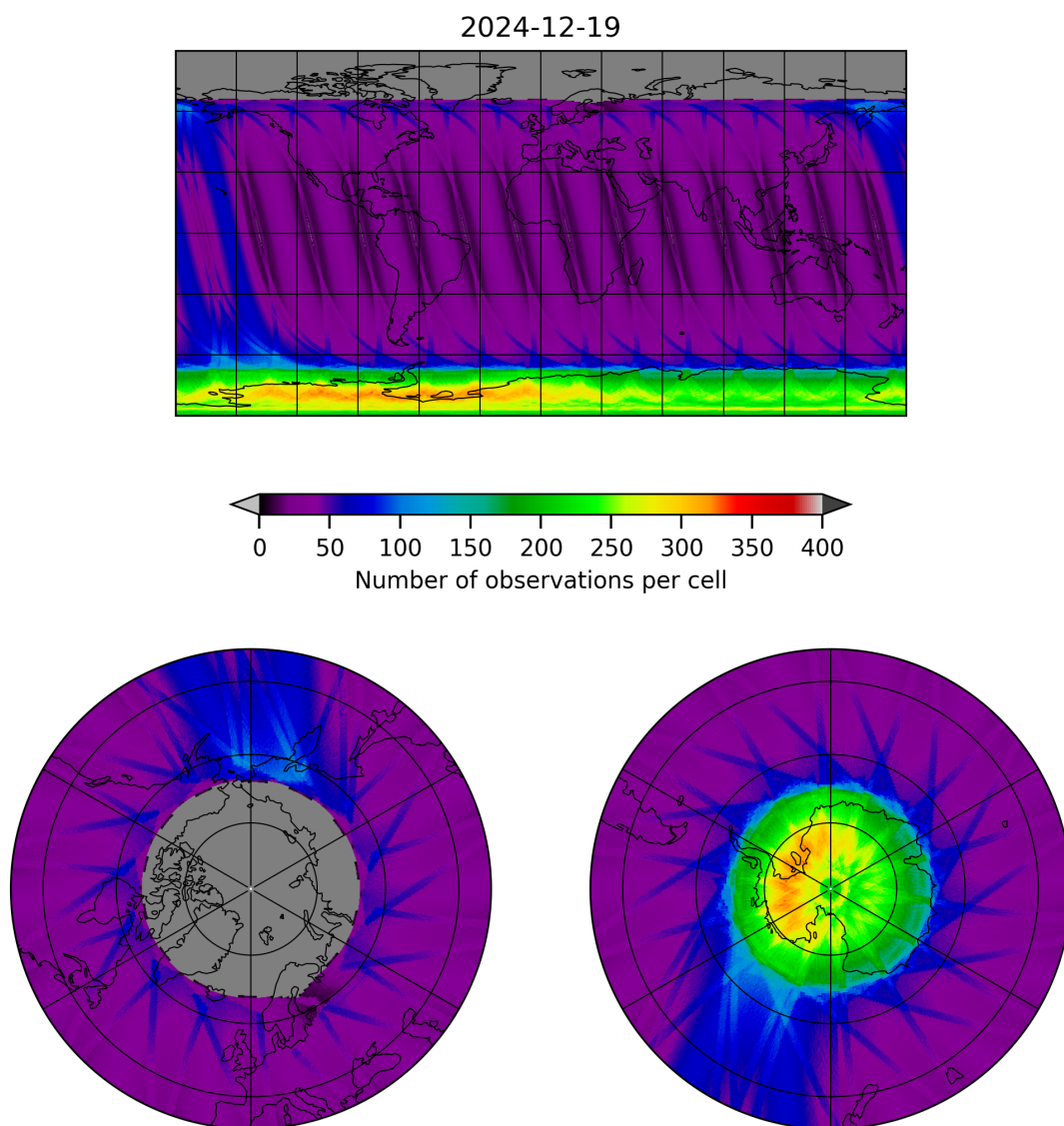
Figure 12: Map of the number of observations for 2024-12-18 to 2024-12-20
