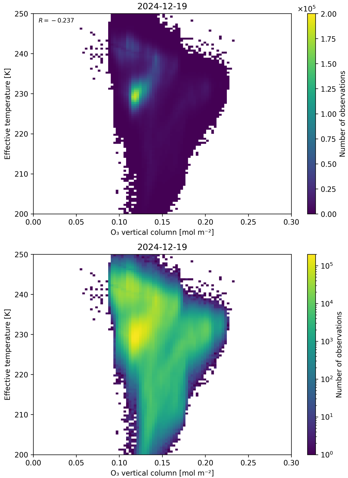
Figure 39: Scatter density plot of “O 3 vertical column” against “Effective temperature” for 2024-12-18 to 2024-12-20.
