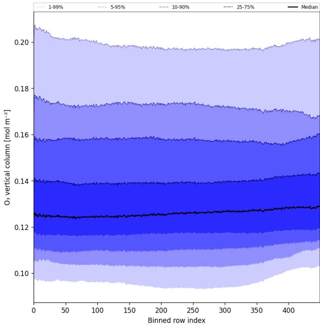
Figure 28: Along track statistics of “O 3 vertical column” for 2024-12-18 to 2024-12-20
