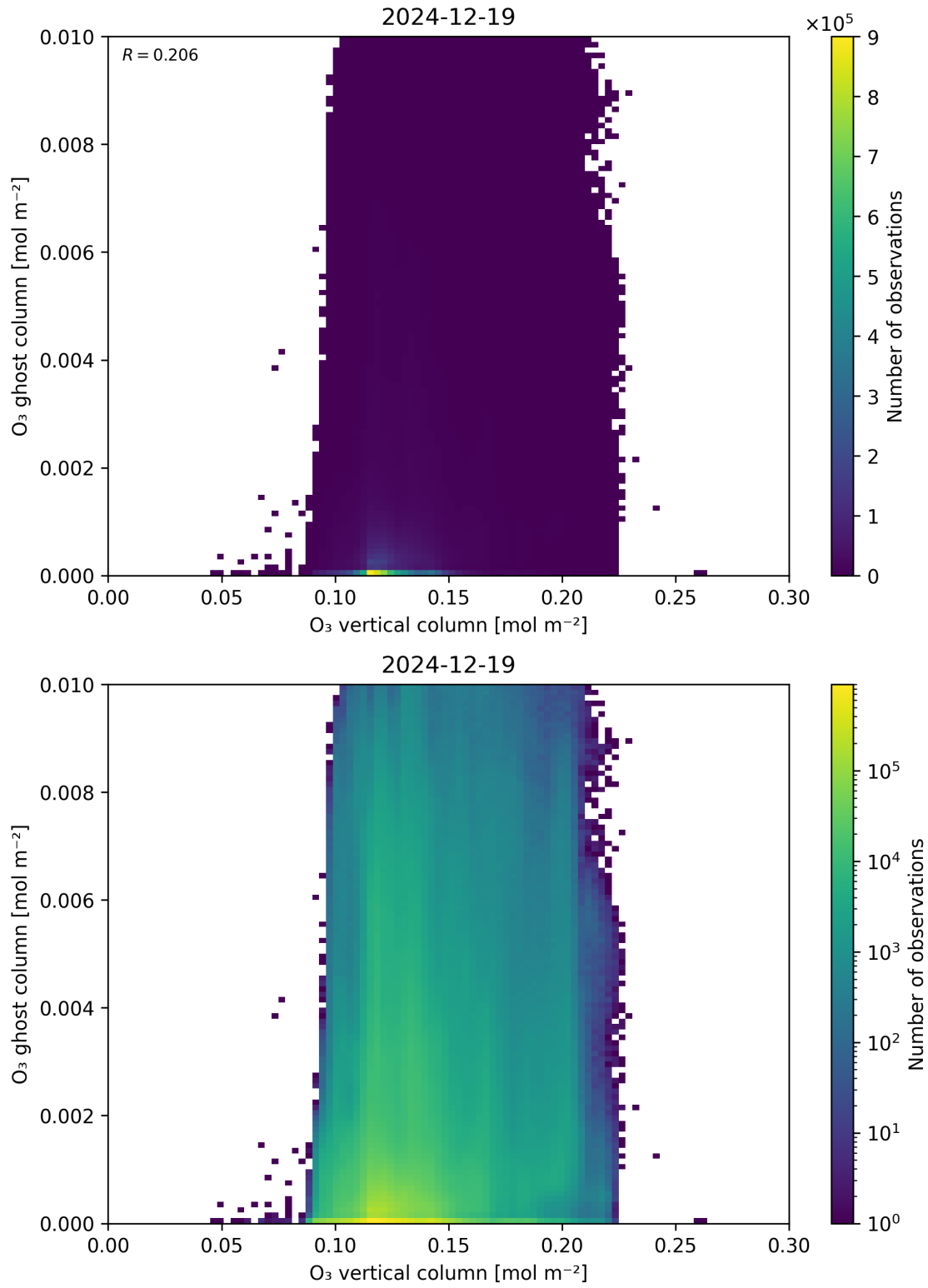
Figure 40: Scatter density plot of “O 3 vertical column” against “O 3 ghost column” for 2024-12-18 to 2024-12-20.
