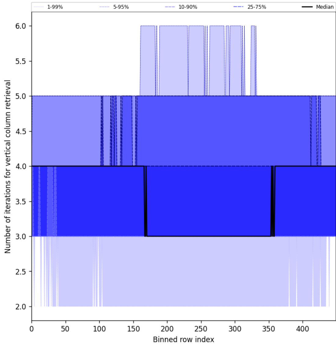
Figure 33: Along track statistics of “Number of iterations for vertical column retrieval” for 2024-12-18 to 2024-12-20
