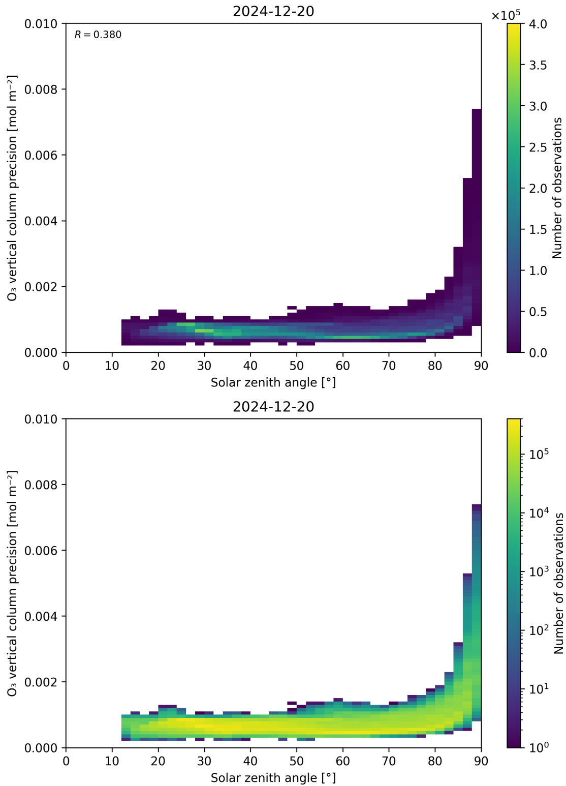
Figure 48: Scatter density plot of “Solar zenith angle” against “O 3 vertical column precision” for 2024-12-19 to 2024-12-21.
