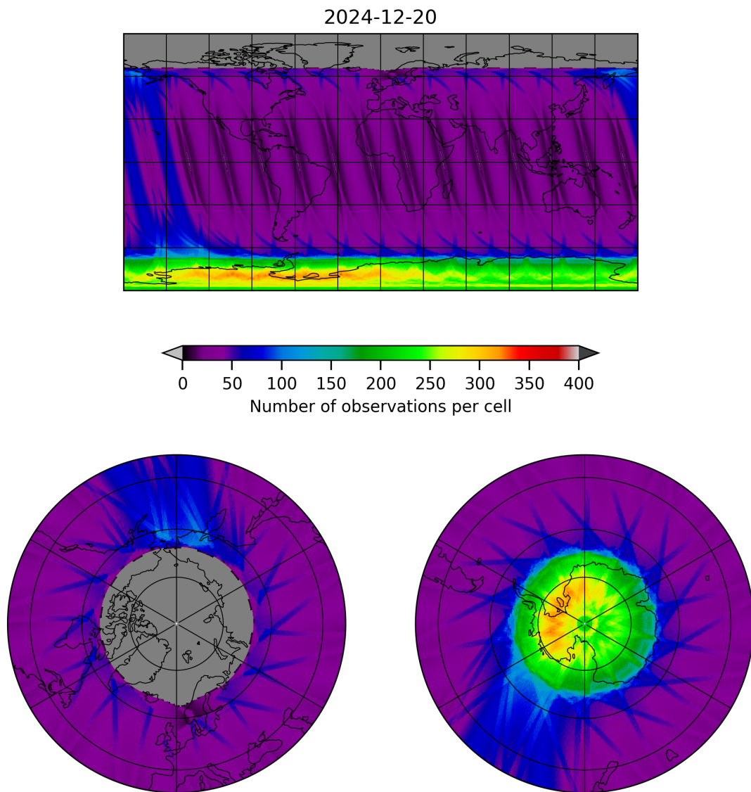
Figure 12: Map of the number of observations for 2024-12-19 to 2024-12-21
