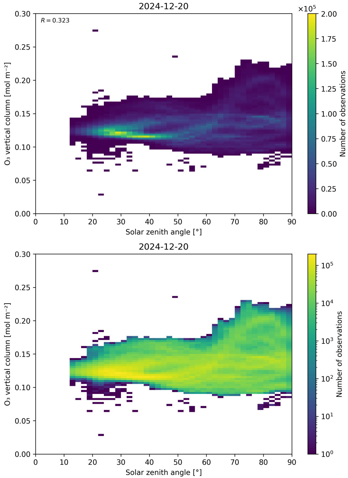
Figure 47: Scatter density plot of “Solar zenith angle” against “O 3 vertical column” for 2024-12-19 to 2024-12-21.
