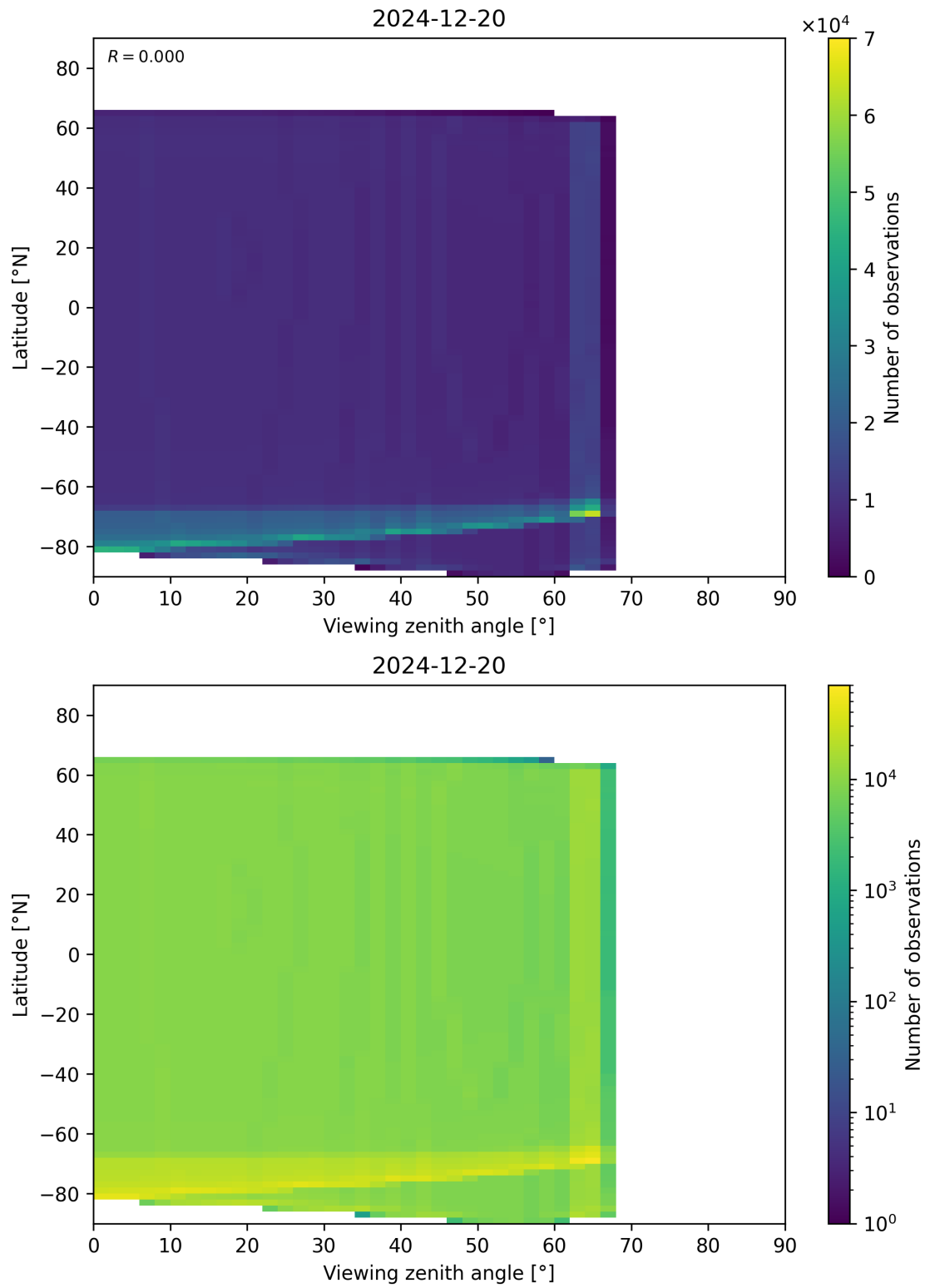
Figure 49: Scatter density plot of “Viewing zenith angle” against “Latitude” for 2024-12-19 to 2024-12-21.
