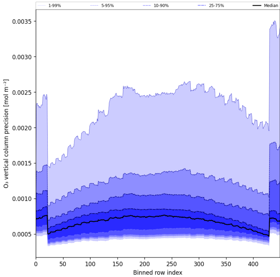
Figure 29: Along track statistics of “O 3 vertical column precision” for 2024-12-19 to 2024-12-21
