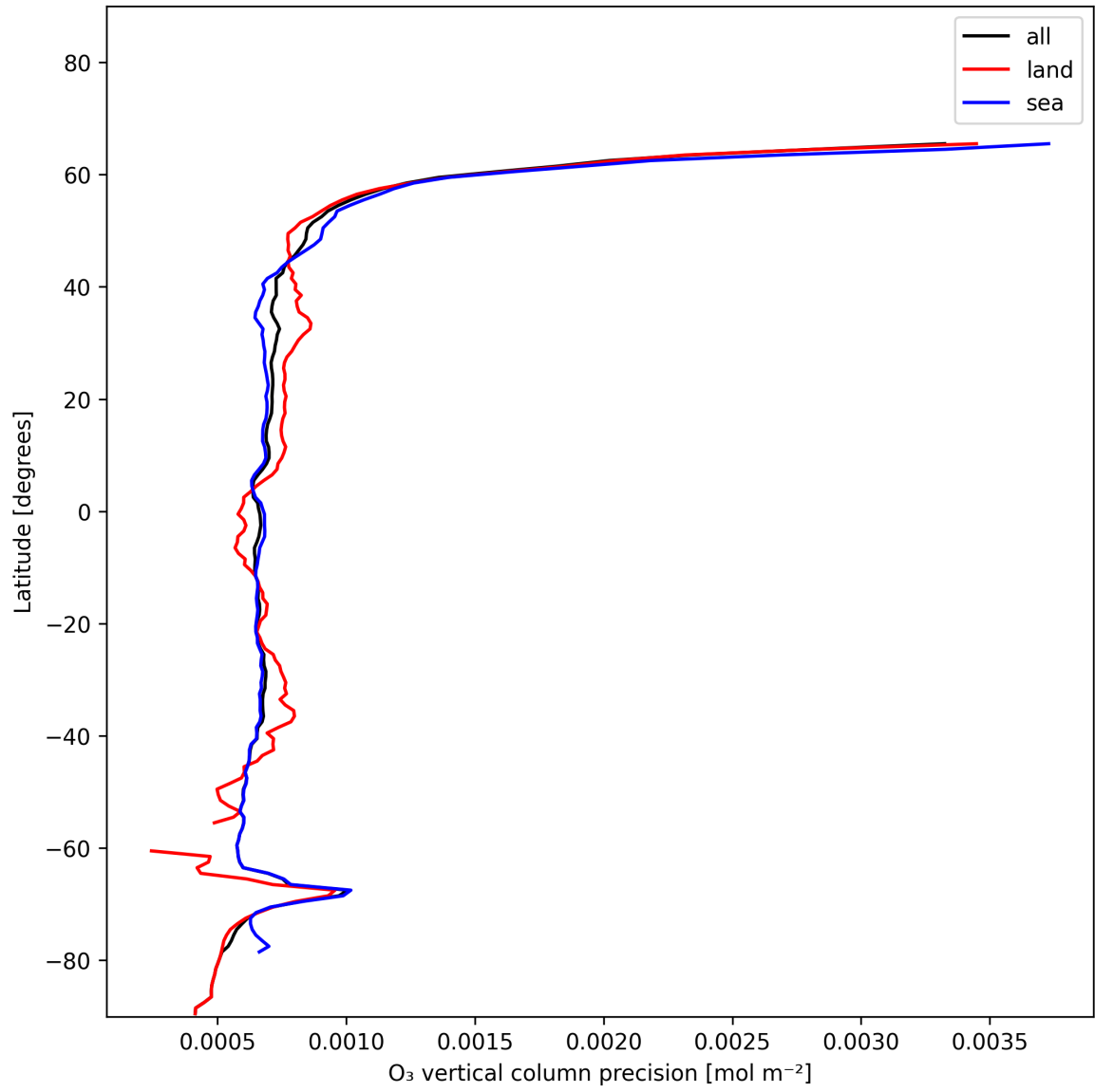
Figure 15: Zonal average of “O 3 vertical column precision” for 2024-12-19 to 2024-12-21.
