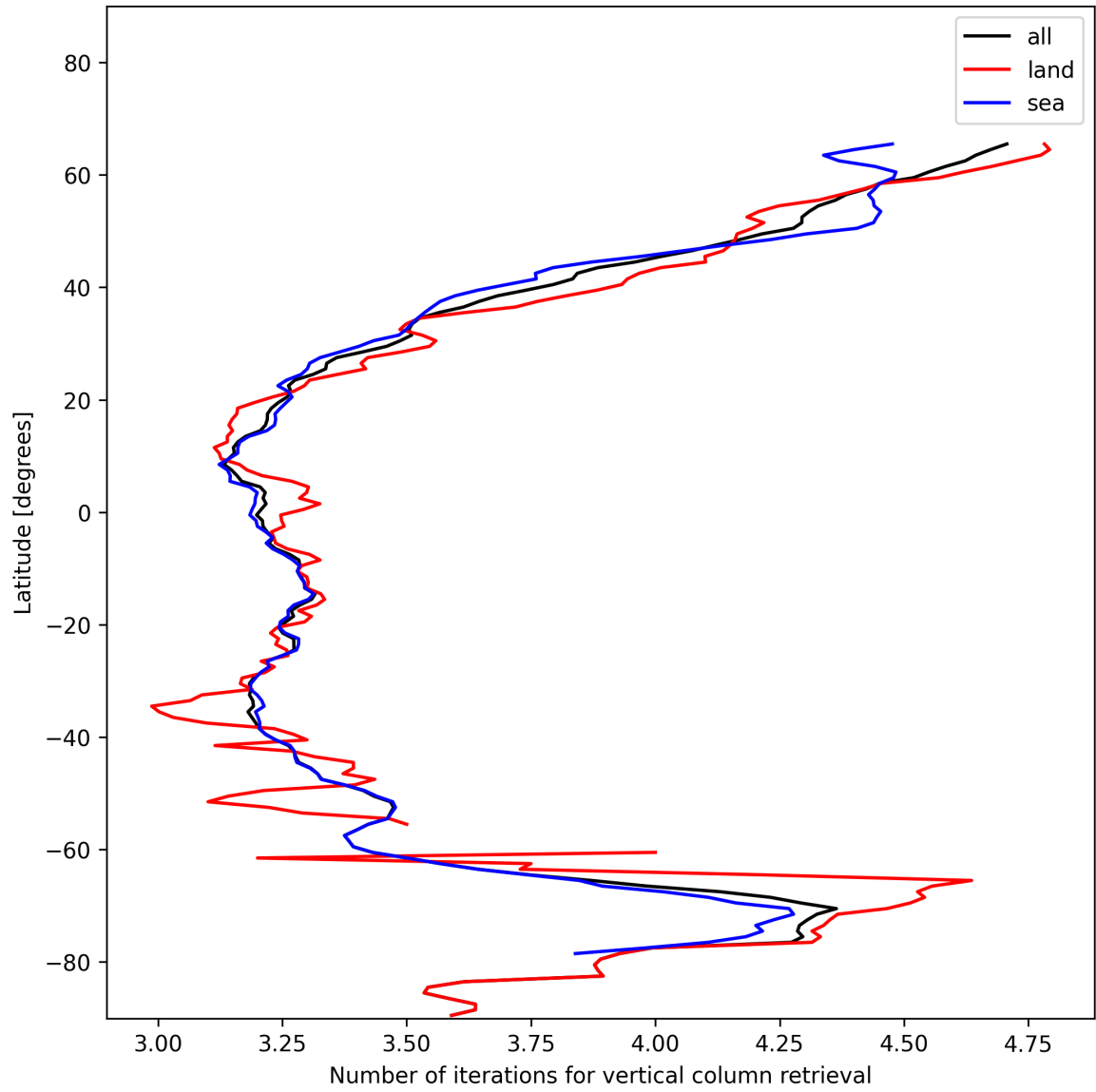
Figure 19: Zonal average of “Number of iterations for vertical column retrieval” for 2024-12-19 to 2024-12-21.
