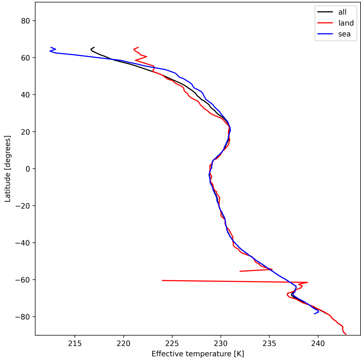
Figure 17: Zonal average of "Effective temperature" for 2024-12-19 to 2024-12-21.
