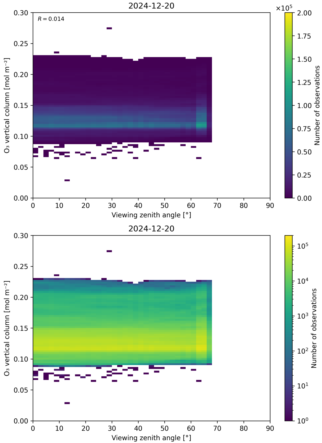
Figure 52: Scatter density plot of “Viewing zenith angle” against “O 3 vertical column” for 2024-12-19 to 2024-12-21.
