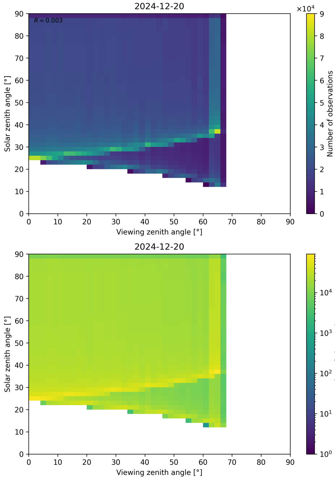
Figure 54: Scatter density plot of “Viewing zenith angle” against “Solar zenith angle” for 2024-12-19 to 2024-12-21.
