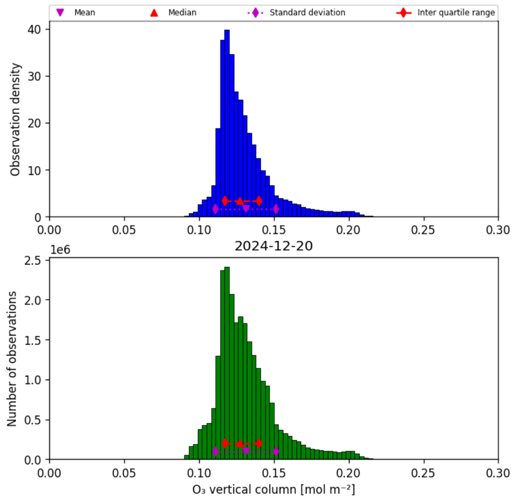
Figure 21: Histogram of “O 3 vertical column” for 2024-12-19 to 2024-12-21
