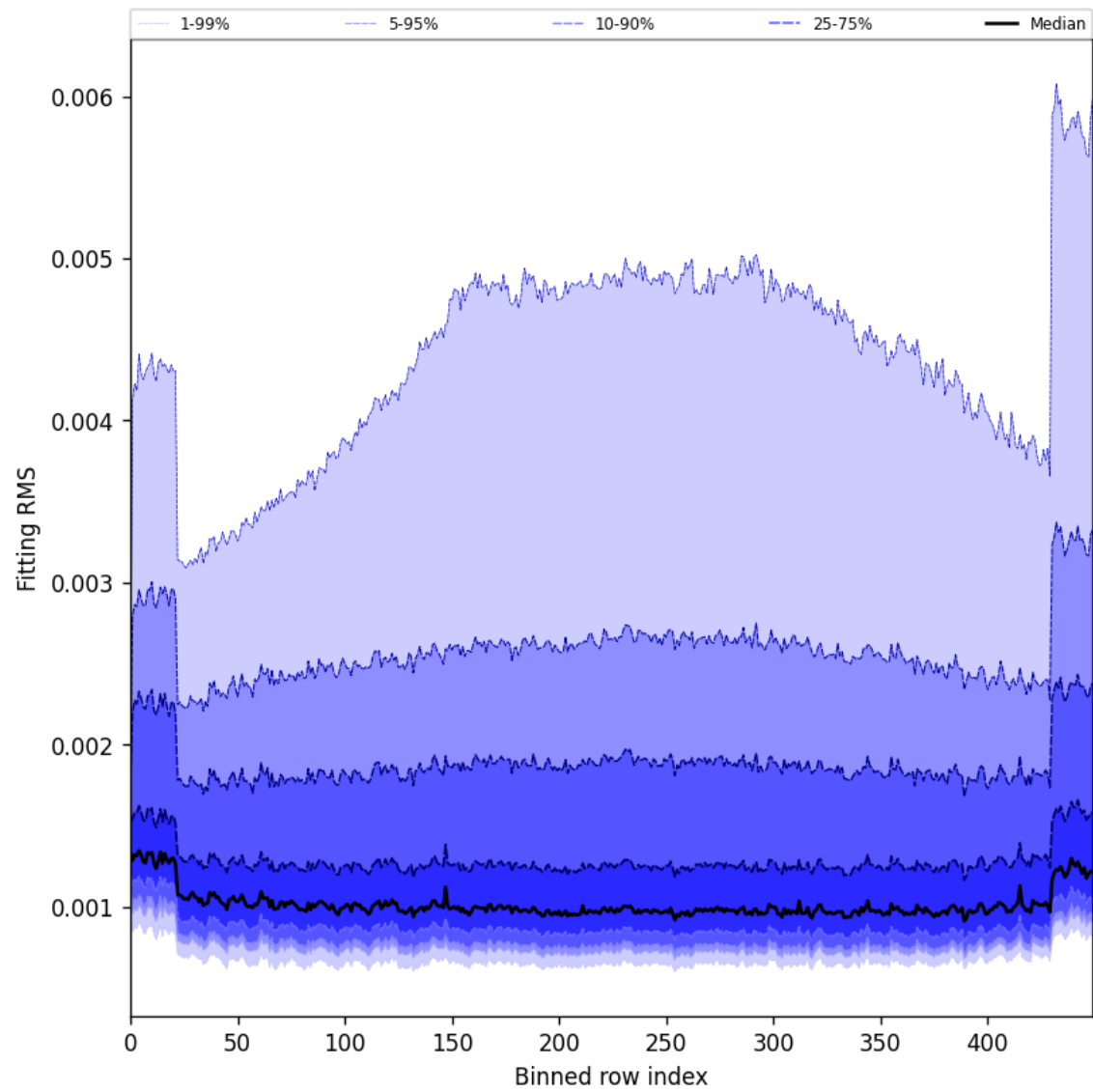
Figure 30: Along track statistics of “Fitting RMS” for 2024-12-19 to 2024-12-21
