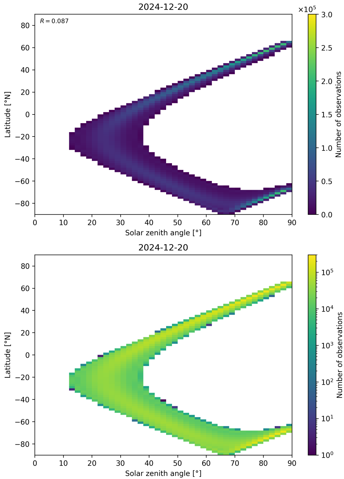
Figure 44: Scatter density plot of “Solar zenith angle” against “Latitude” for 2024-12-19 to 2024-12-21.
