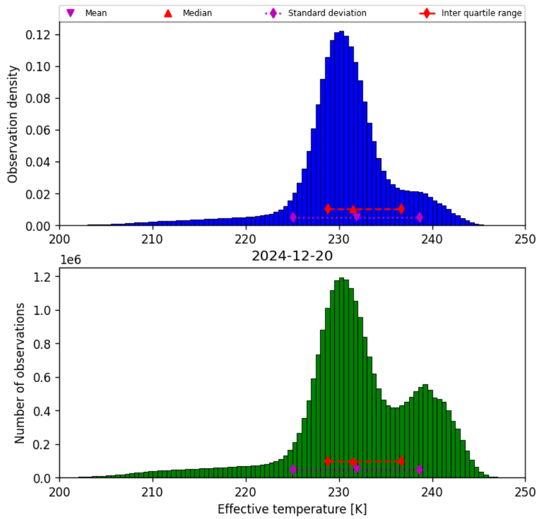
Figure 24: Histogram of “Effective temperature” for 2024-12-19 to 2024-12-21
