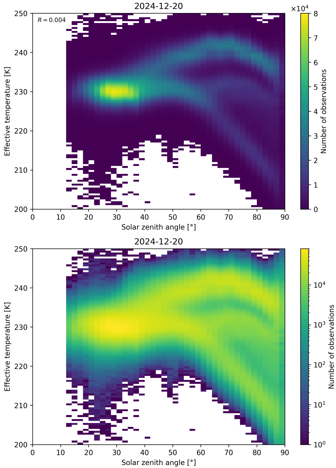
Figure 45: Scatter density plot of “Solar zenith angle” against “Effective temperature” for 2024-12-19 to 2024-12-21.
