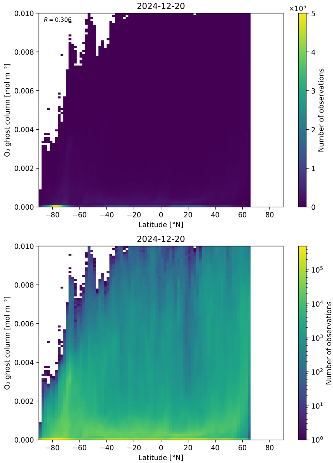
Figure 35: Scatter density plot of “Latitude” against “O 3 ghost column” for 2024-12-19 to 2024-12-21.
