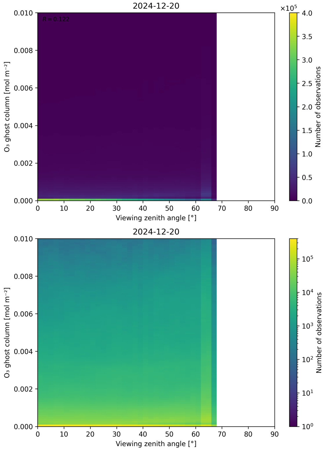
Figure 51: Scatter density plot of “Viewing zenith angle” against “O 3 ghost column” for 2024-12-19 to 2024-12-21.
