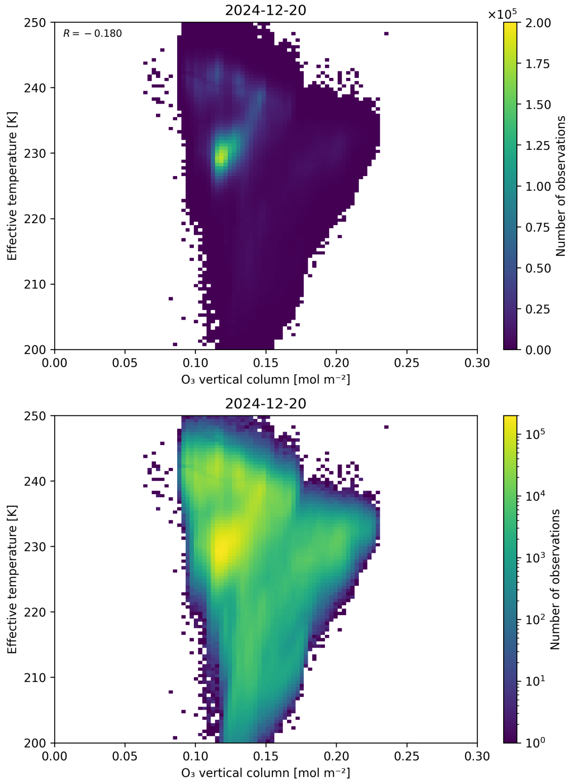
Figure 39: Scatter density plot of “O 3 vertical column” against “Effective temperature” for 2024-12-19 to 2024-12-21.
