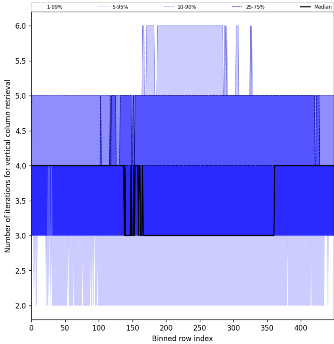
Figure 33: Along track statistics of “Number of iterations for vertical column retrieval” for 2024-12-19 to 2024-12-21
