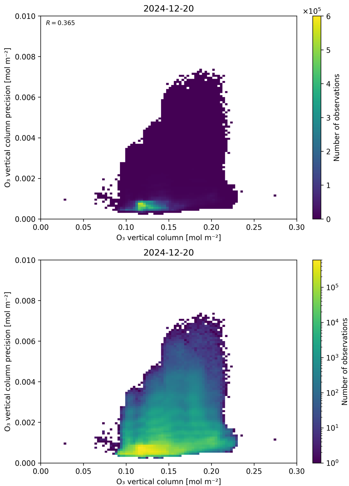
Figure 41: Scatter density plot of “O 3 vertical column” against “O 3 vertical column precision” for 2024-12-19 to 2024-12-21.
