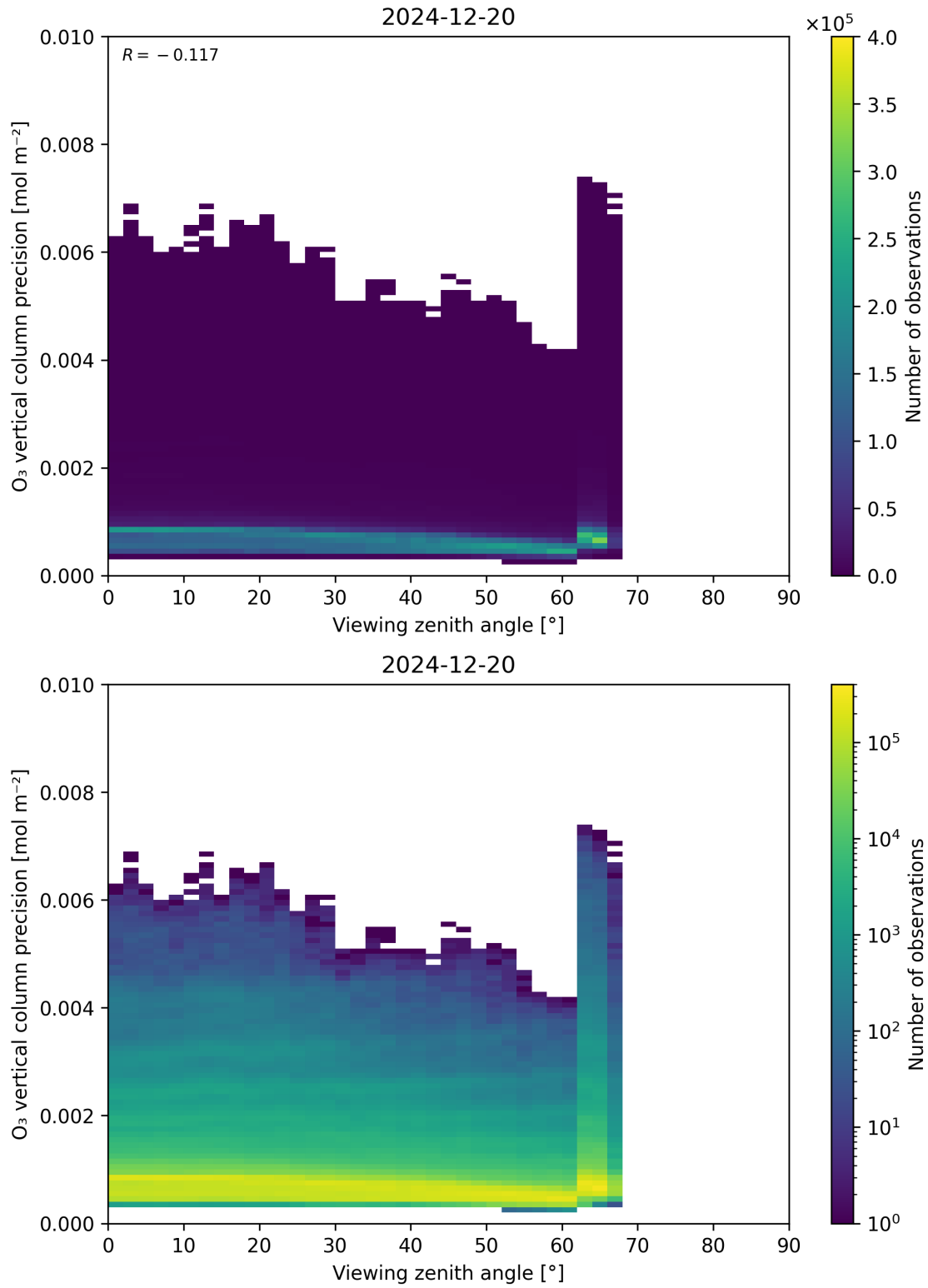
Figure 53: Scatter density plot of “Viewing zenith angle” against “O 3 vertical column precision” for 2024-12-19 to 2024-12-21.
