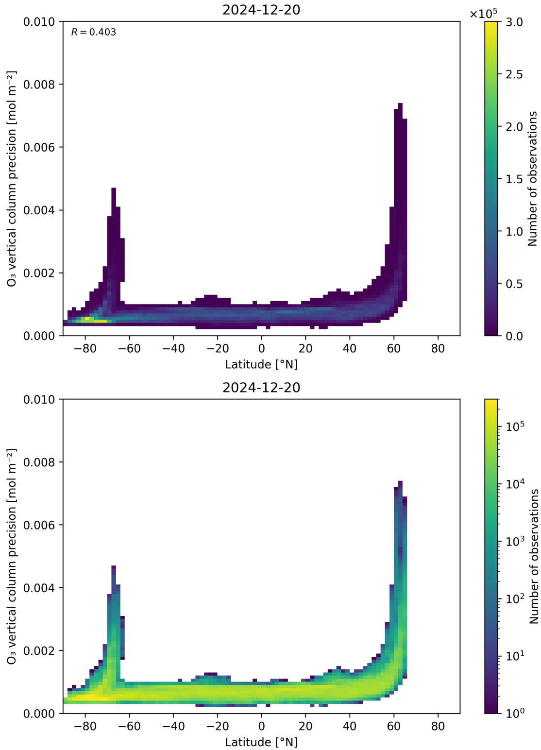
Figure 37: Scatter density plot of “Latitude” against “O 3 vertical column precision” for 2024-12-19 to 2024-12-21.
