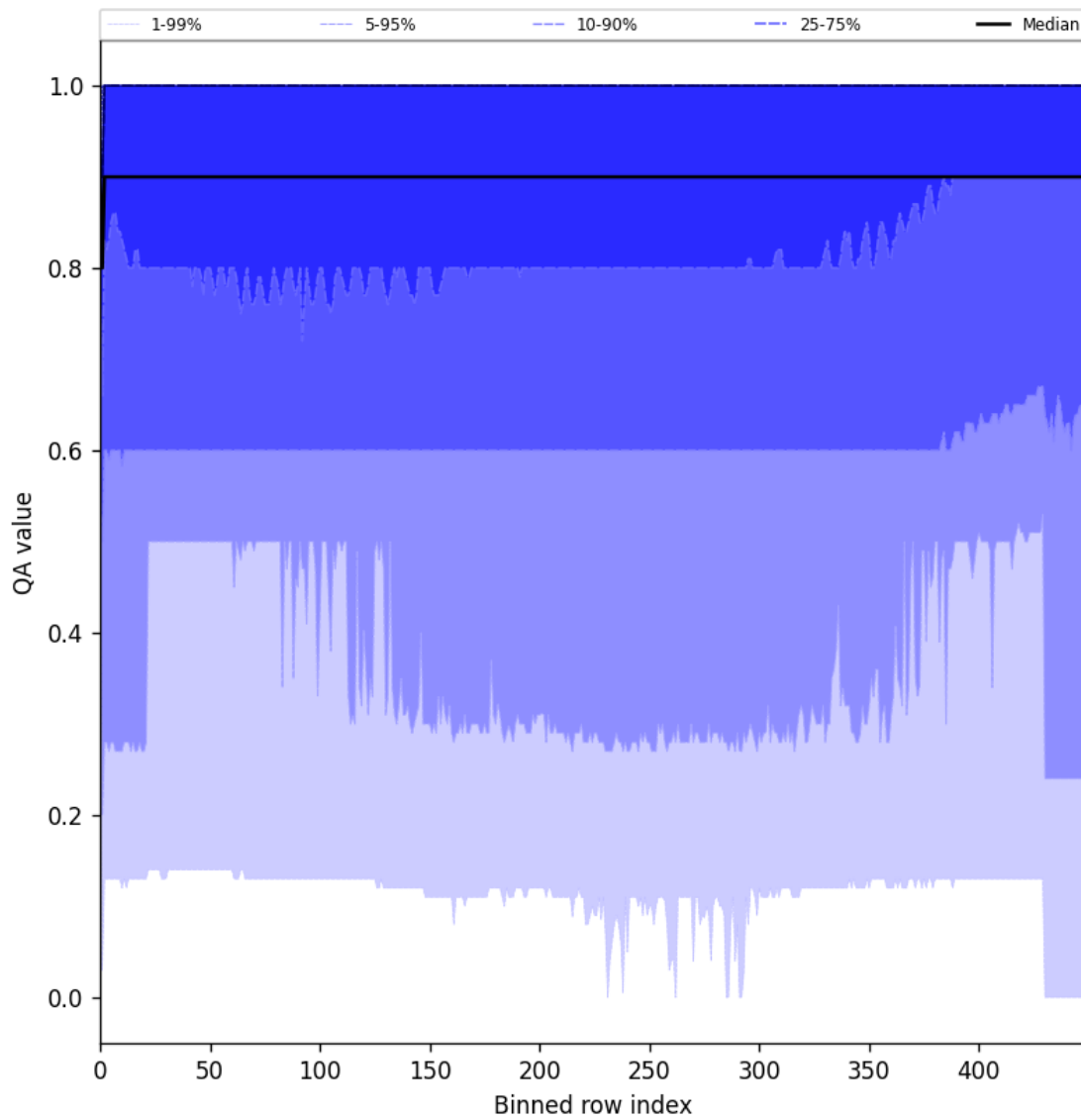
Figure 27: Along track statistics of “QA value” for 2024-12-19 to 2024-12-21
