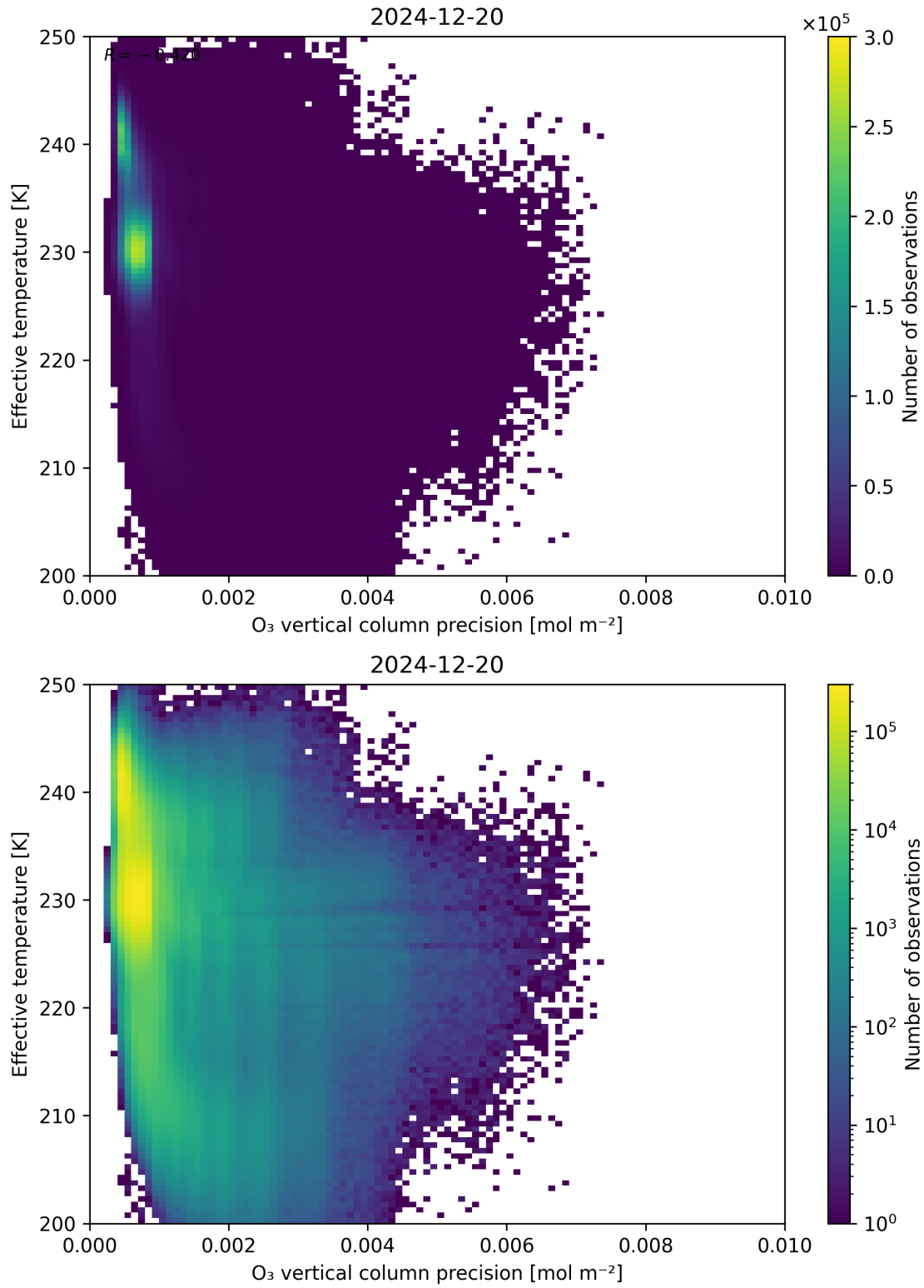
Figure 42: Scatter density plot of “O 3 vertical column precision” against “Effective temperature” for 2024-12-19 to 2024-12-21.
