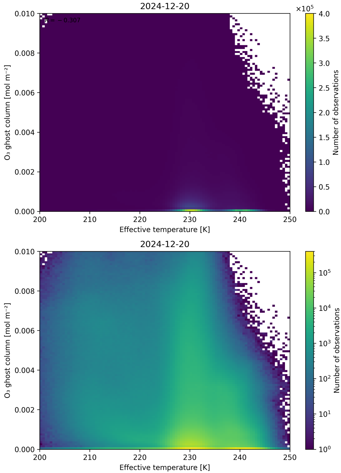
Figure 38: Scatter density plot of “Effective temperature” against “O 3 ghost column” for 2024-12-19 to 2024-12-21.
