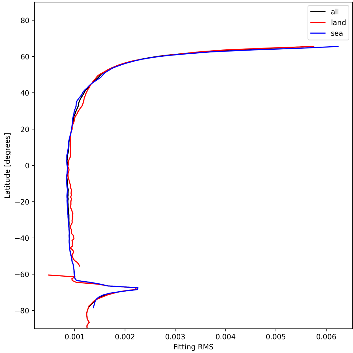
Figure 16: Zonal average of “Fitting RMS” for 2024-12-19 to 2024-12-21.
