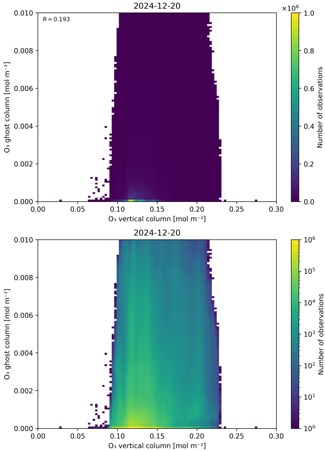
Figure 40: Scatter density plot of “O 3 vertical column” against “O 3 ghost column” for 2024-12-19 to 2024-12-21.
