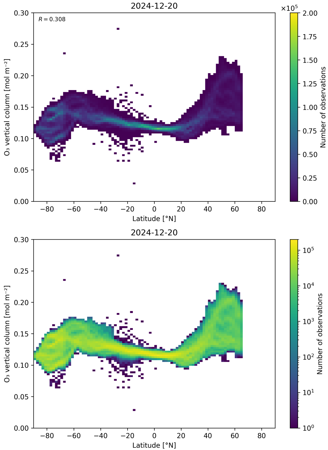
Figure 36: Scatter density plot of “Latitude” against “O 3 vertical column” for 2024-12-19 to 2024-12-21.
