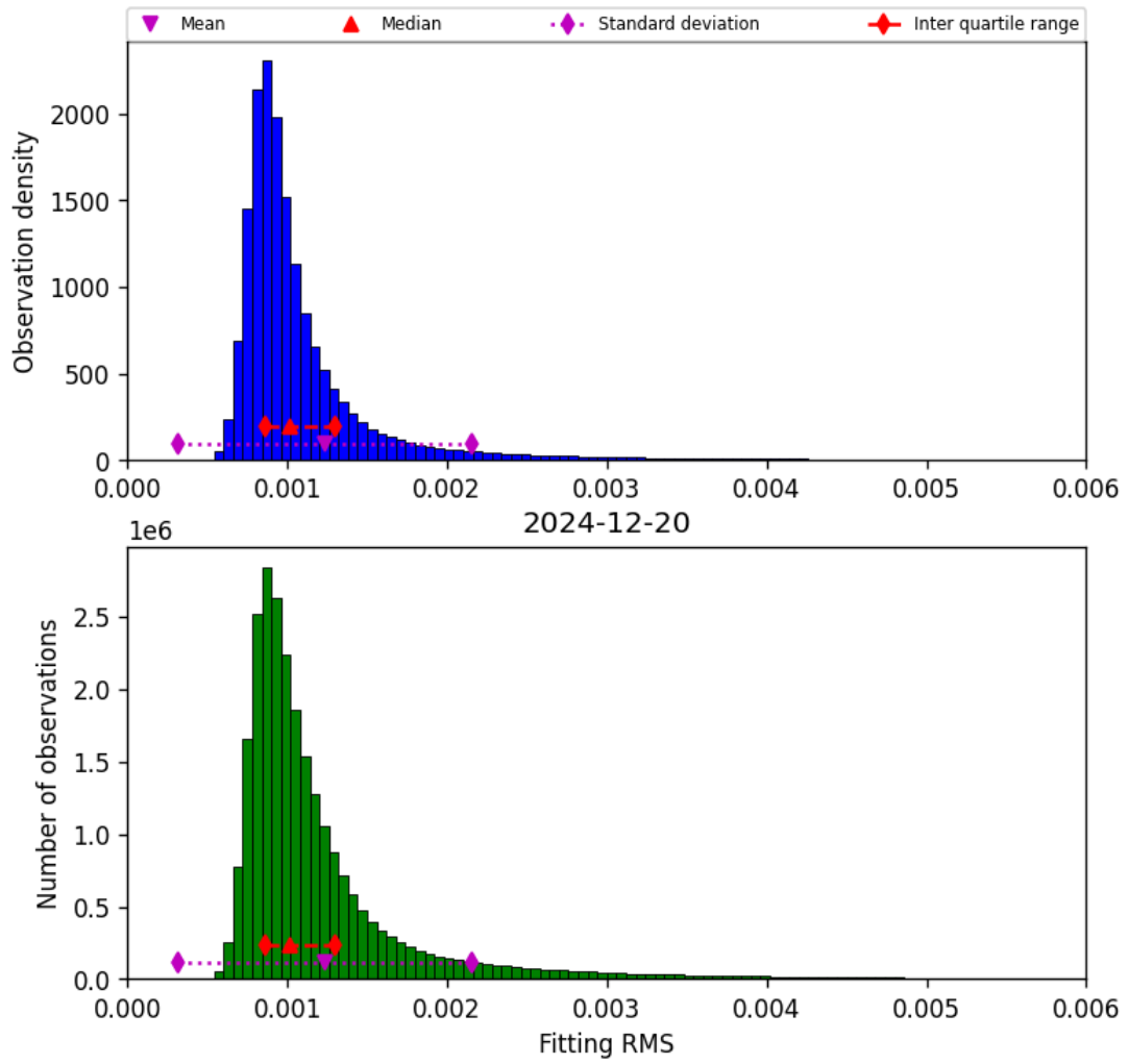
Figure 23: Histogram of “Fitting RMS” for 2024-12-19 to 2024-12-21
