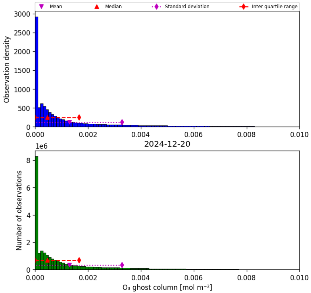
Figure 25: Histogram of “O 3 ghost column” for 2024-12-19 to 2024-12-21
