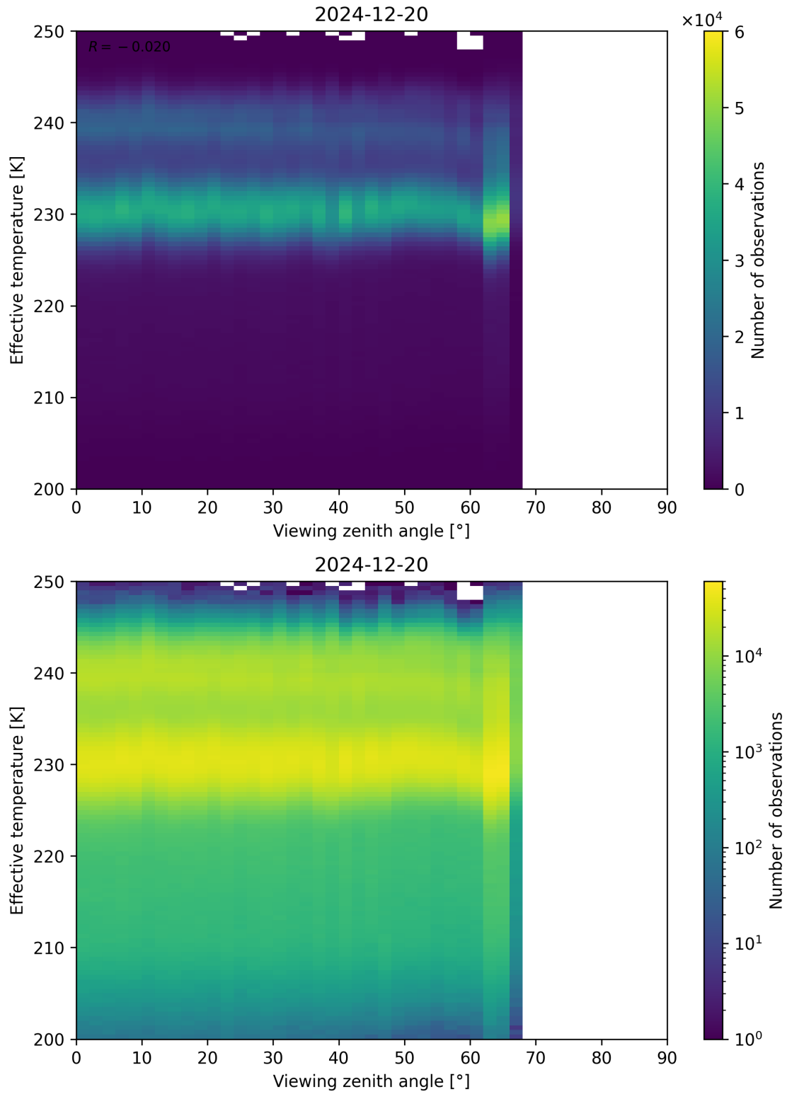
Figure 50: Scatter density plot of “Viewing zenith angle” against “Effective temperature” for 2024-12-19 to 2024-12-21.
