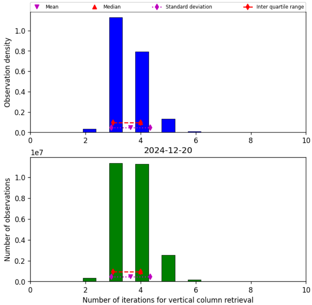
Figure 26: Histogram of “Number of iterations for vertical column retrieval” for 2024-12-19 to 2024-12-21
