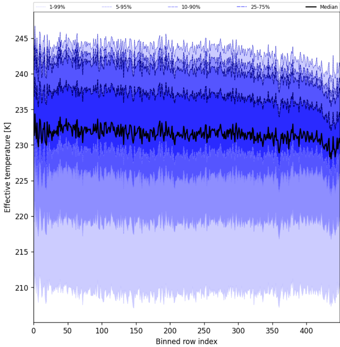
Figure 31: Along track statistics of “Effective temperature” for 2024-12-19 to 2024-12-21
