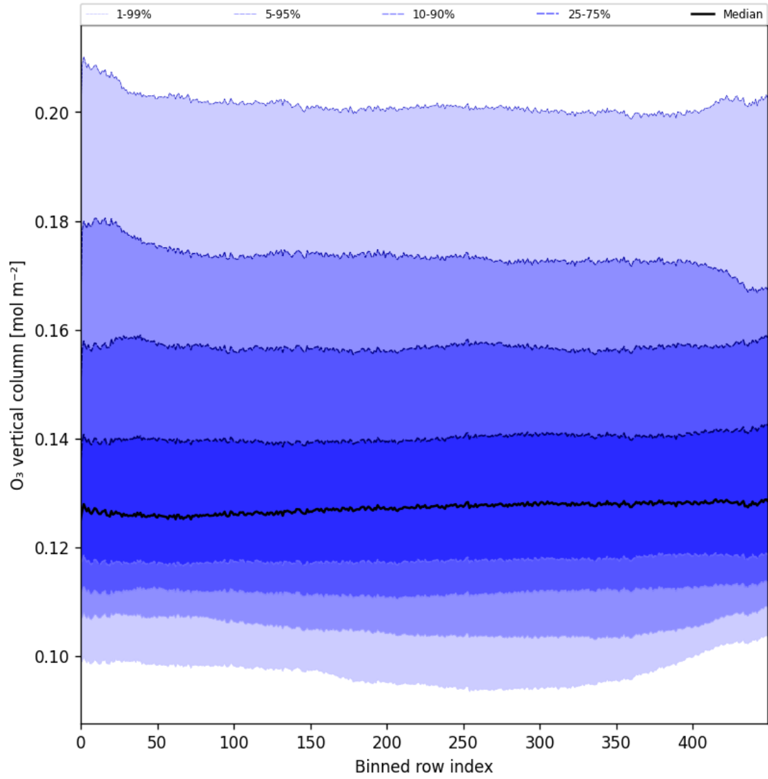
Figure 28: Along track statistics of “O 3 vertical column” for 2024-12-19 to 2024-12-21
