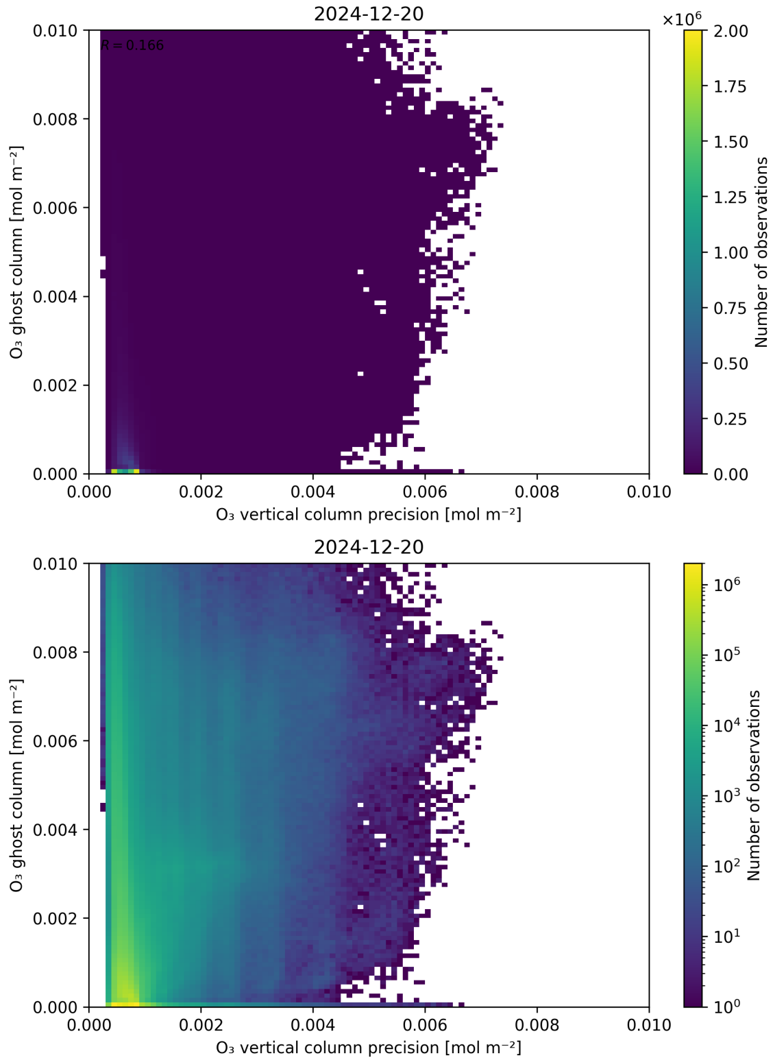
Figure 43: Scatter density plot of “ \text{O}_3 vertical column precision” against “ \text{O}_3 ghost column” for 2024-12-19 to 2024-12-21.
