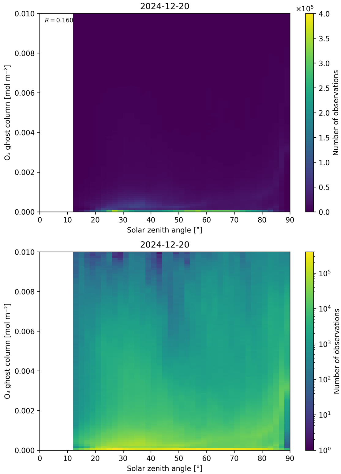
Figure 46: Scatter density plot of “Solar zenith angle” against “O 3 ghost column” for 2024-12-19 to 2024-12-21.
