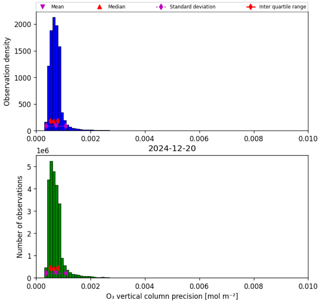
Figure 22: Histogram of “O 3 vertical column precision” for 2024-12-19 to 2024-12-21
