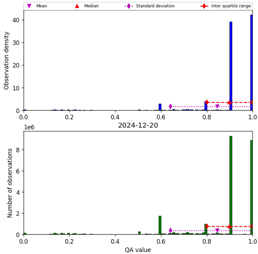
Figure 20: Histogram of “QA value” for 2024-12-19 to 2024-12-21
