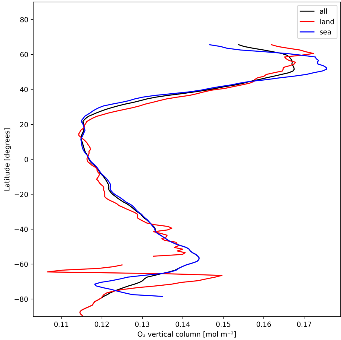
Figure 14: Zonal average of “O 3 vertical column” for 2024-12-19 to 2024-12-21.
