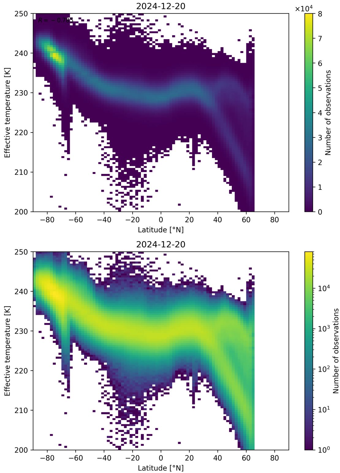
Figure 34: Scatter density plot of “Latitude” against “Effective temperature” for 2024-12-19 to 2024-12-21.
