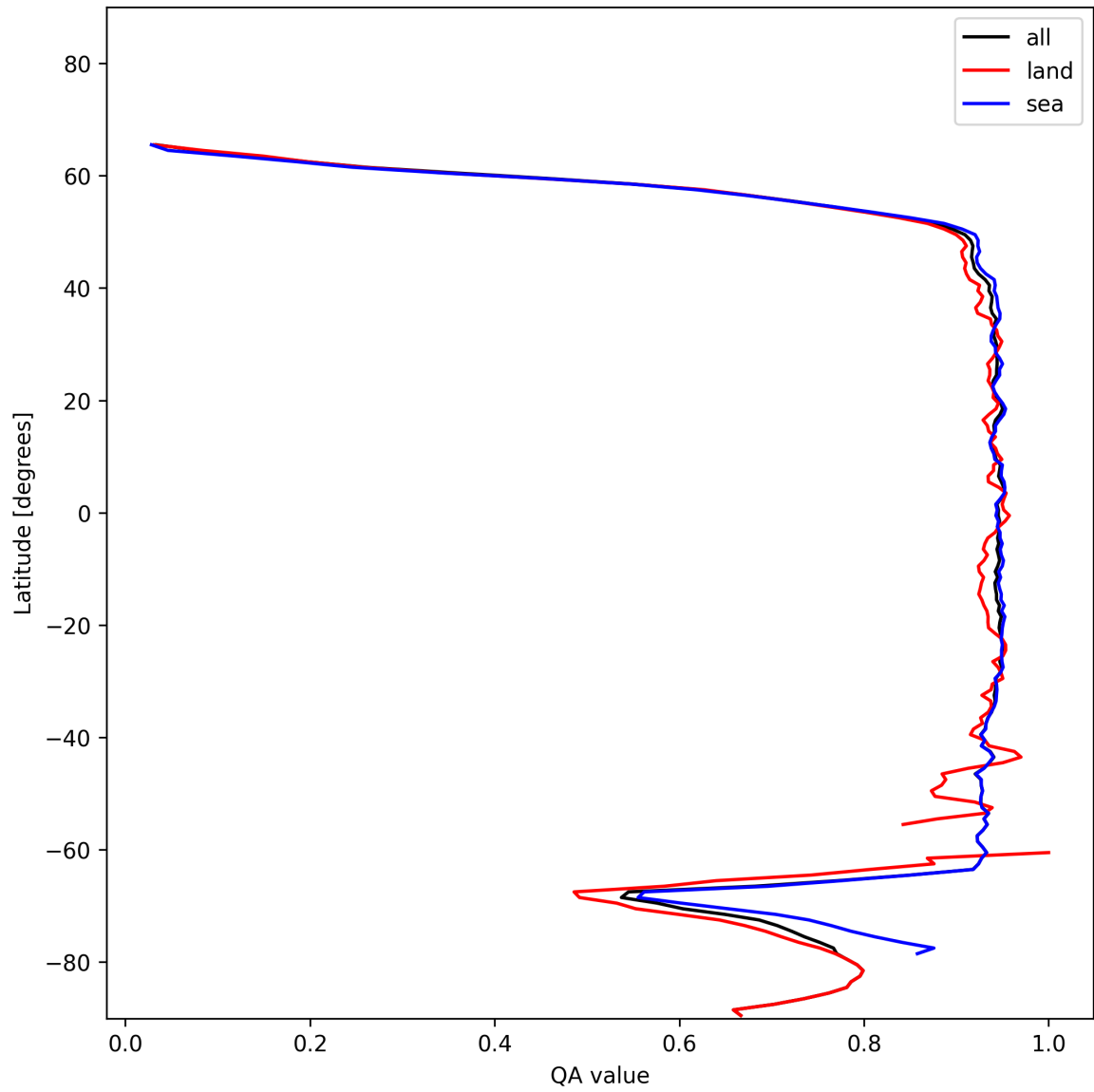
Figure 13: Zonal average of “QA value” for 2024-12-19 to 2024-12-21.
