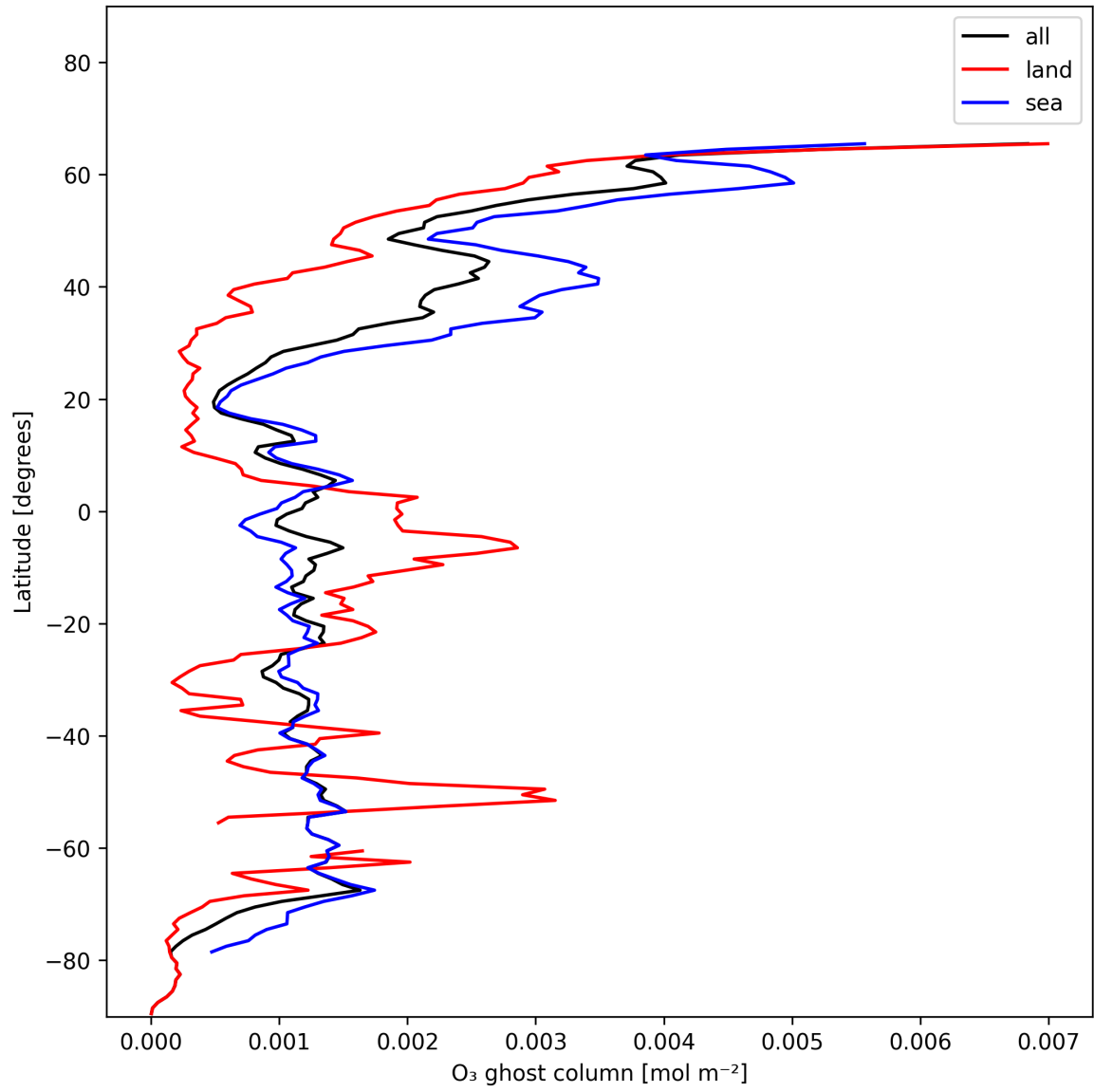
Figure 18: Zonal average of “O 3 ghost column” for 2024-12-19 to 2024-12-21.
