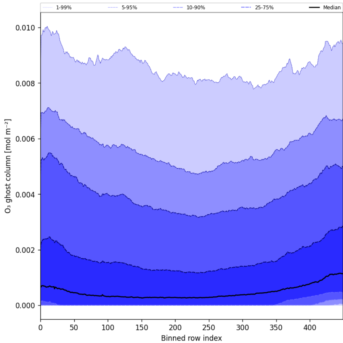
Figure 32: Along track statistics of “O 3 ghost column” for 2024-12-19 to 2024-12-21
