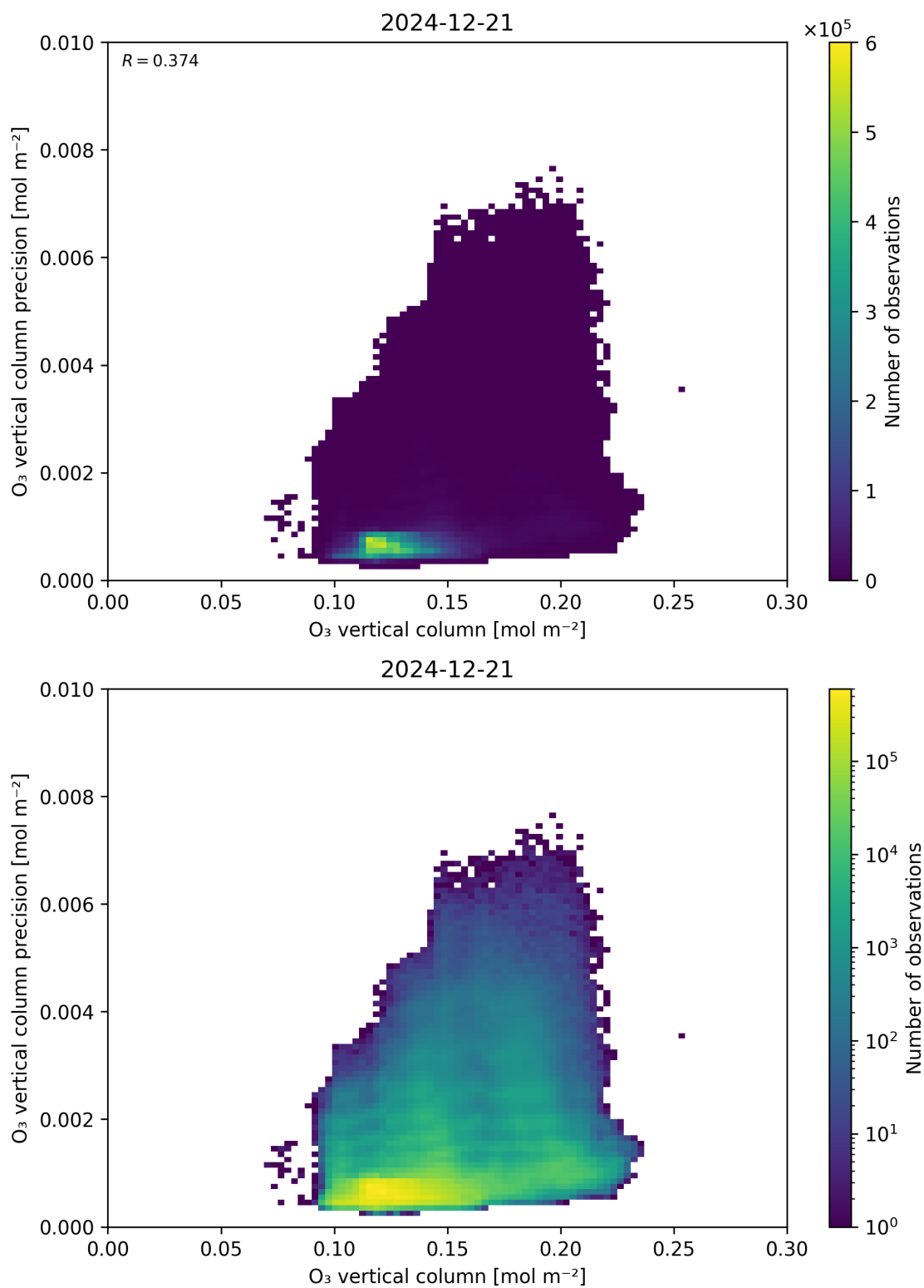
Figure 41: Scatter density plot of “O 3 vertical column” against “O 3 vertical column precision” for 2024-12-20 to 2024-12-22.
