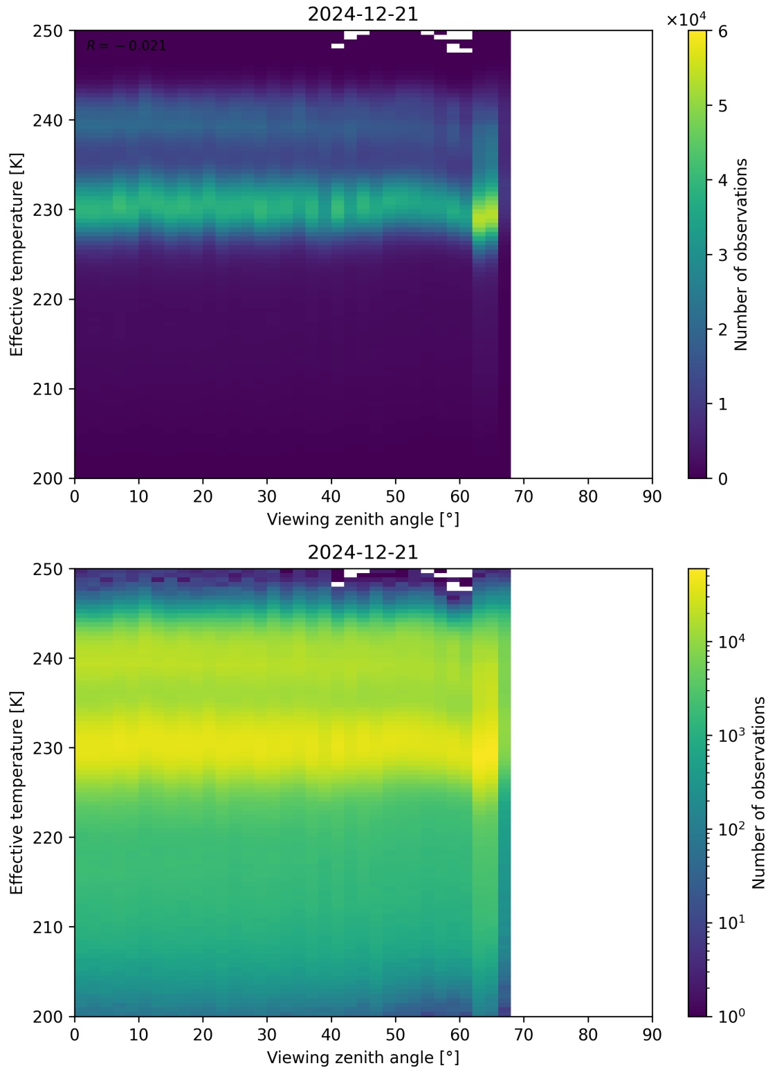
Figure 50: Scatter density plot of “Viewing zenith angle” against “Effective temperature” for 2024-12-20 to 2024-12-22.
