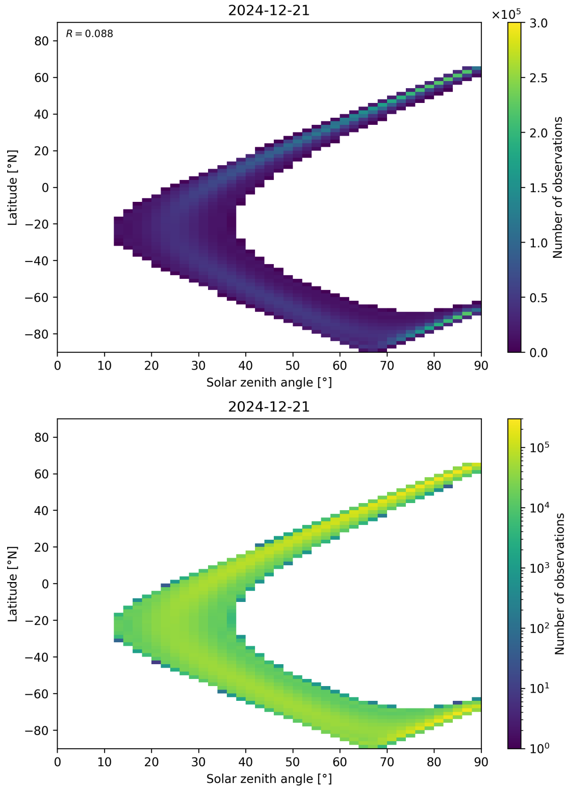
Figure 44: Scatter density plot of “Solar zenith angle” against “Latitude” for 2024-12-20 to 2024-12-22.
