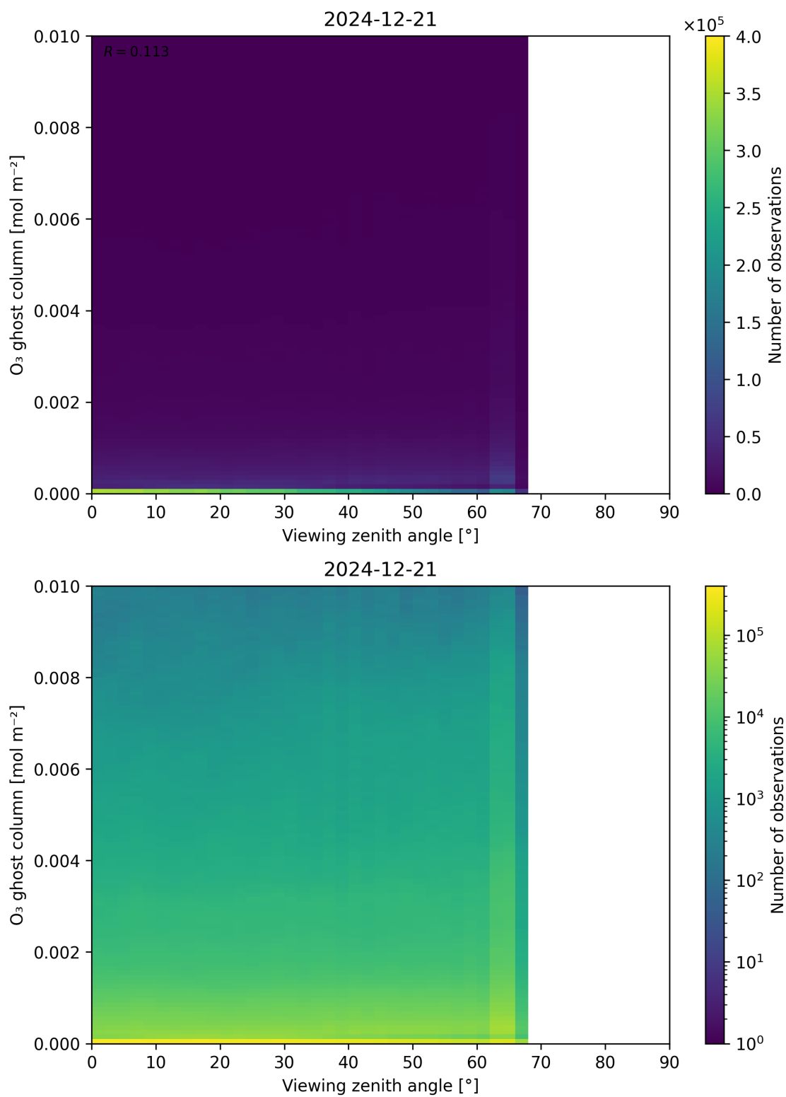
Figure 51: Scatter density plot of “Viewing zenith angle” against “O 3 ghost column” for 2024-12-20 to 2024-12-22.
