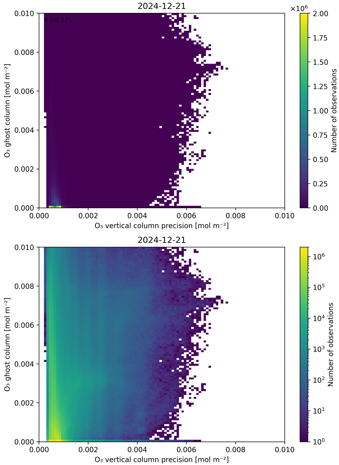
Figure 43: Scatter density plot of “ \text{O}_3 vertical column precision” against “ \text{O}_3 ghost column” for 2024-12-20 to 2024-12-22.
