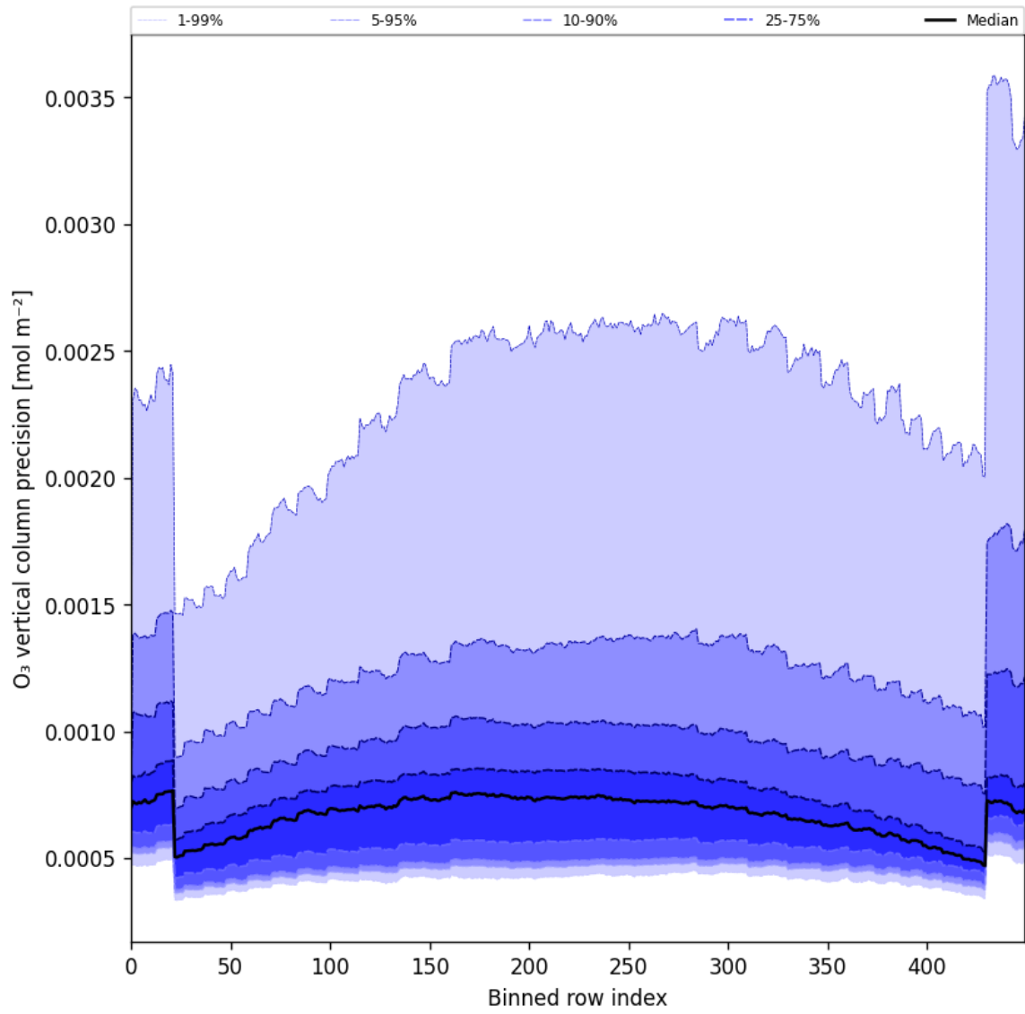
Figure 29: Along track statistics of “O 3 vertical column precision” for 2024-12-20 to 2024-12-22
