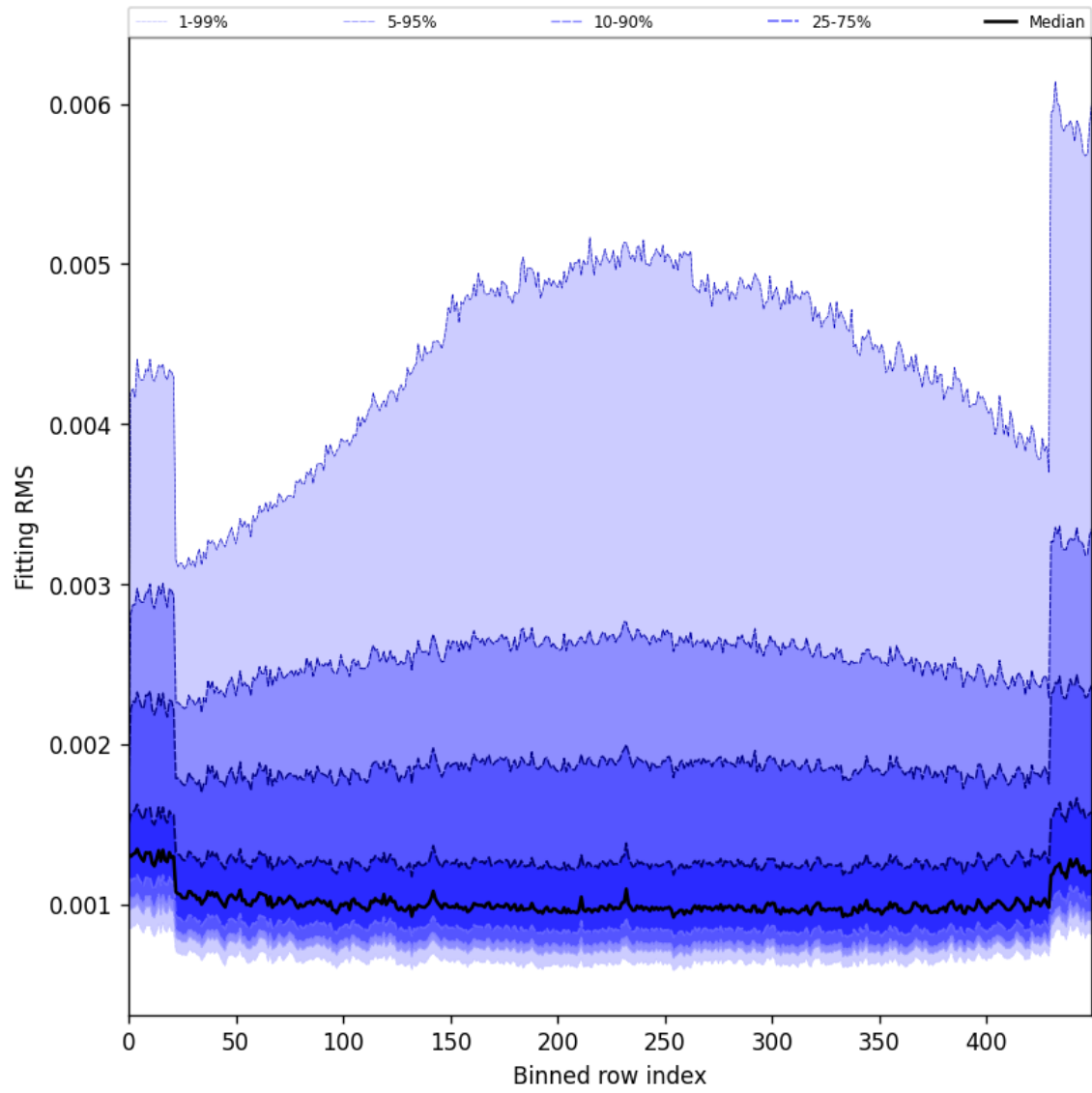
Figure 30: Along track statistics of “Fitting RMS” for 2024-12-20 to 2024-12-22
