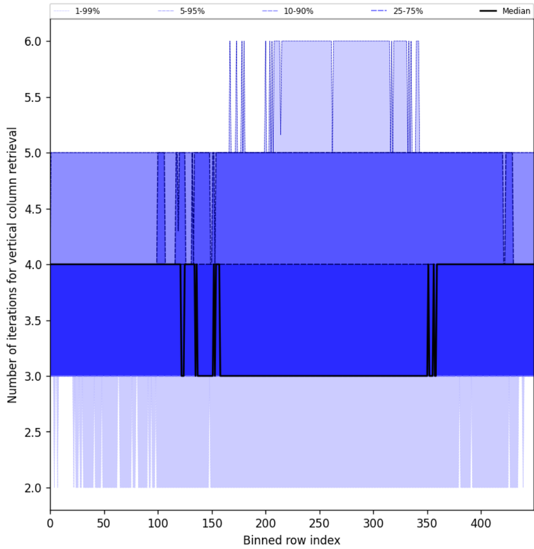
Figure 33: Along track statistics of “Number of iterations for vertical column retrieval” for 2024-12-20 to 2024-12-22
