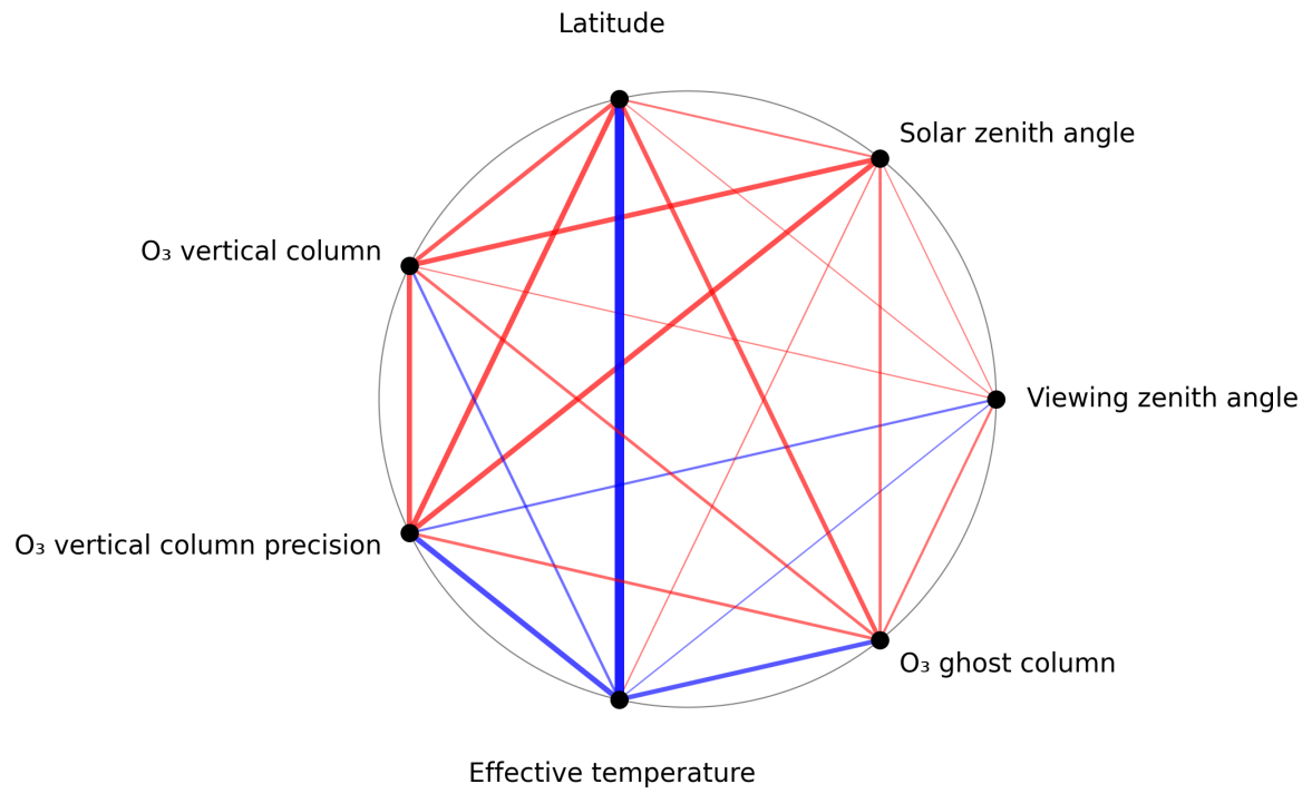
Figure 1: Map of correlation graph for 2024-12-20 to 2024-12-22.
