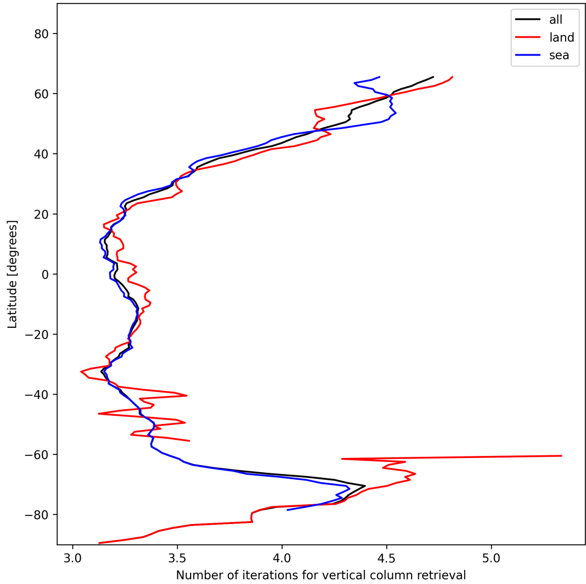
Figure 19: Zonal average of “Number of iterations for vertical column retrieval” for 2024-12-20 to 2024-12-22.
