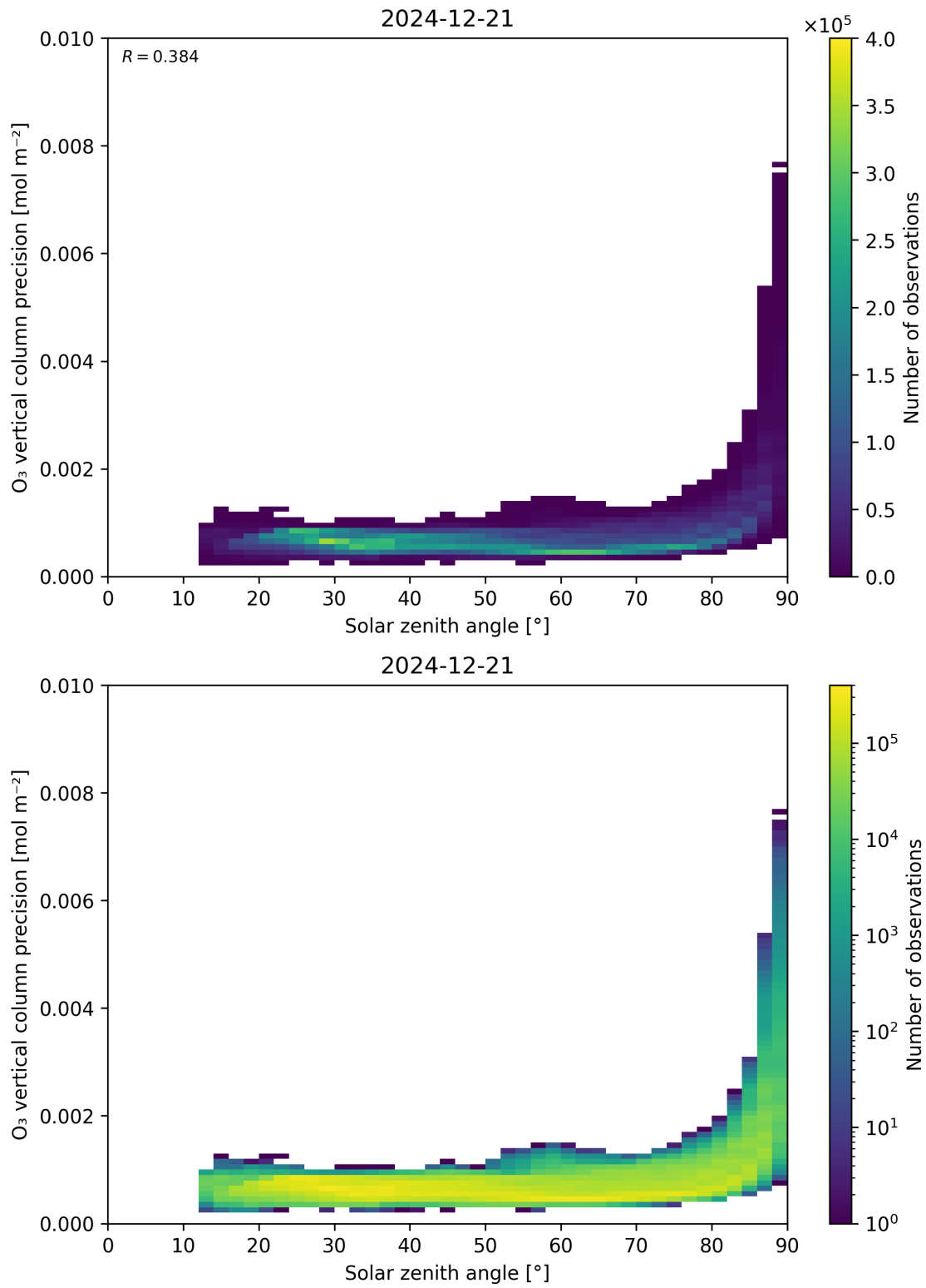
Figure 48: Scatter density plot of “Solar zenith angle” against “O 3 vertical column precision” for 2024-12-20 to 2024-12-22.
