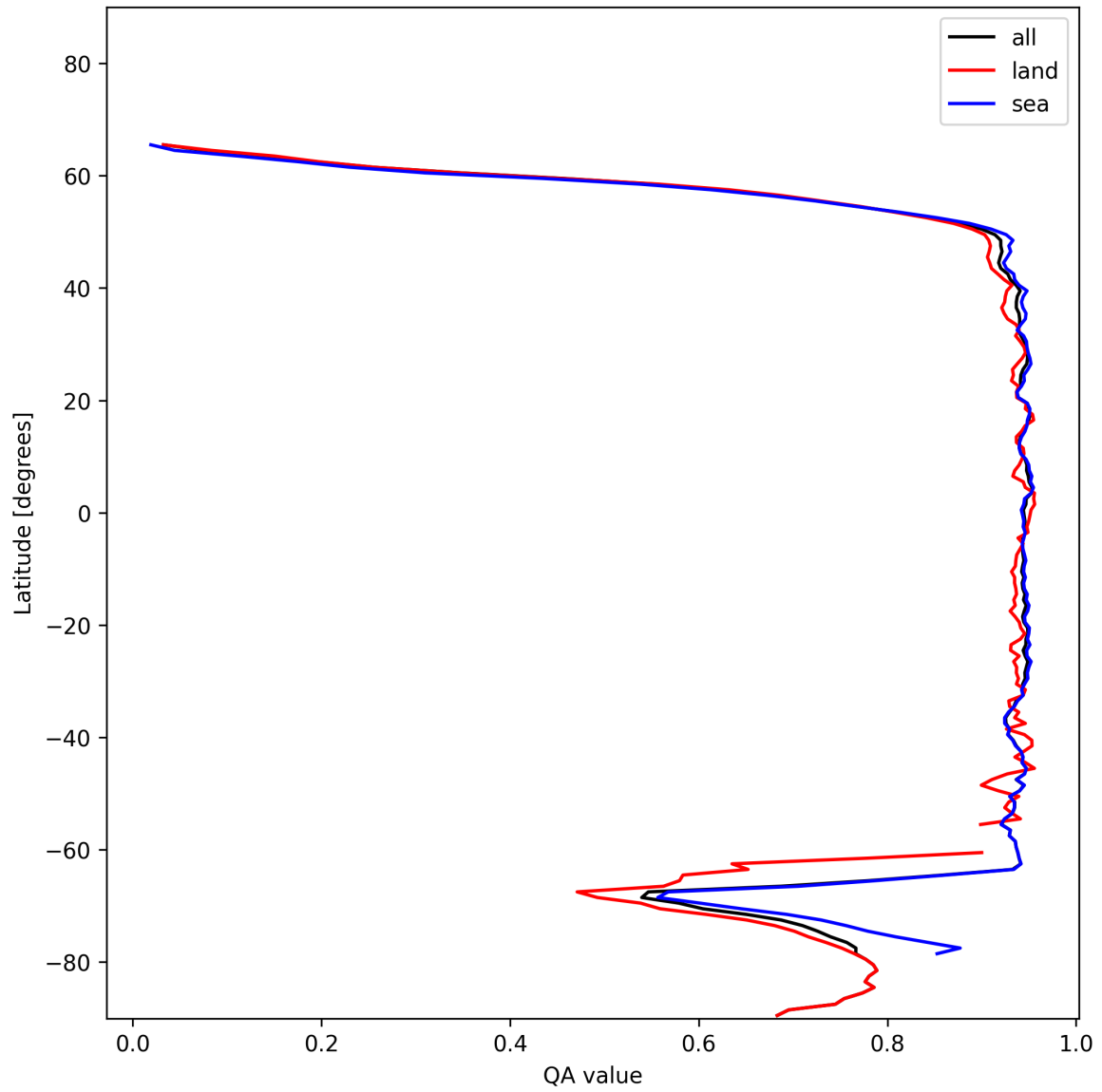
Figure 13: Zonal average of “QA value” for 2024-12-20 to 2024-12-22.
