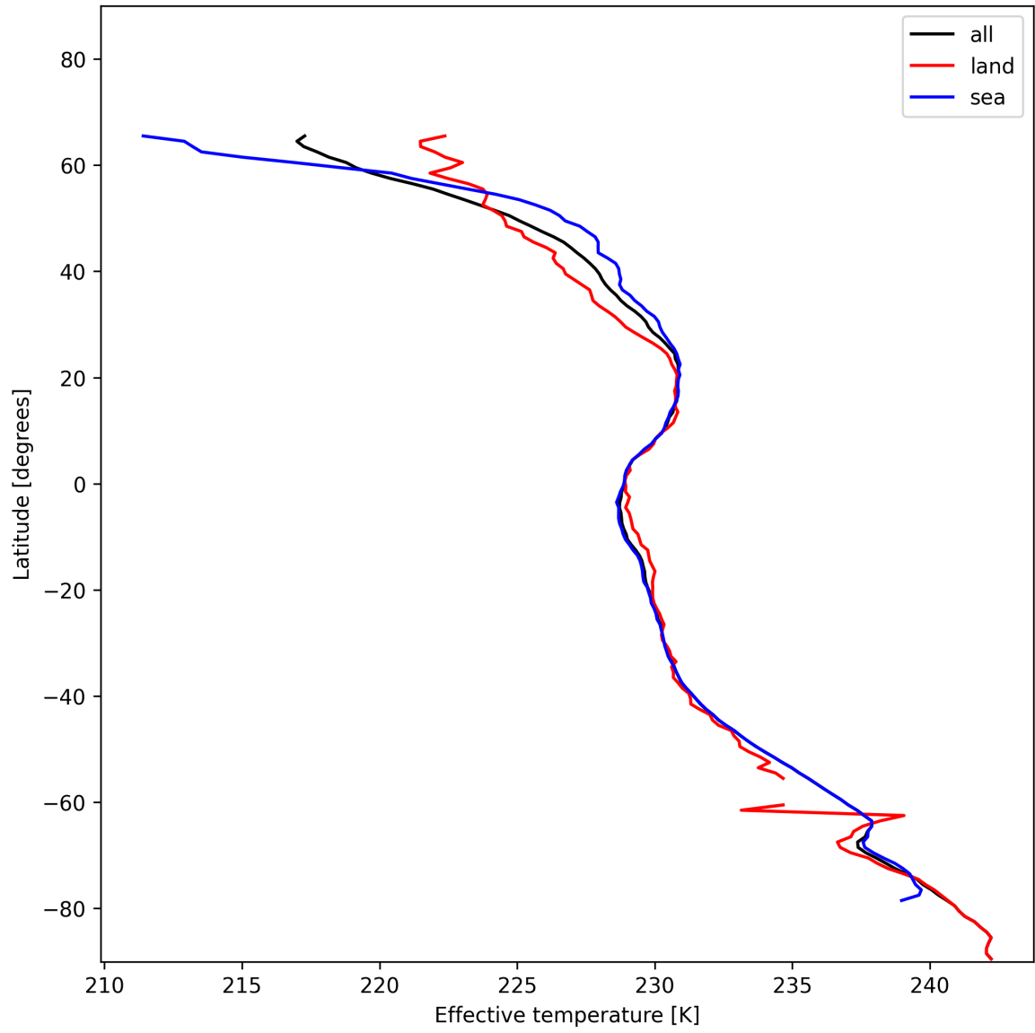
Figure 17: Zonal average of "Effective temperature" for 2024-12-20 to 2024-12-22.
