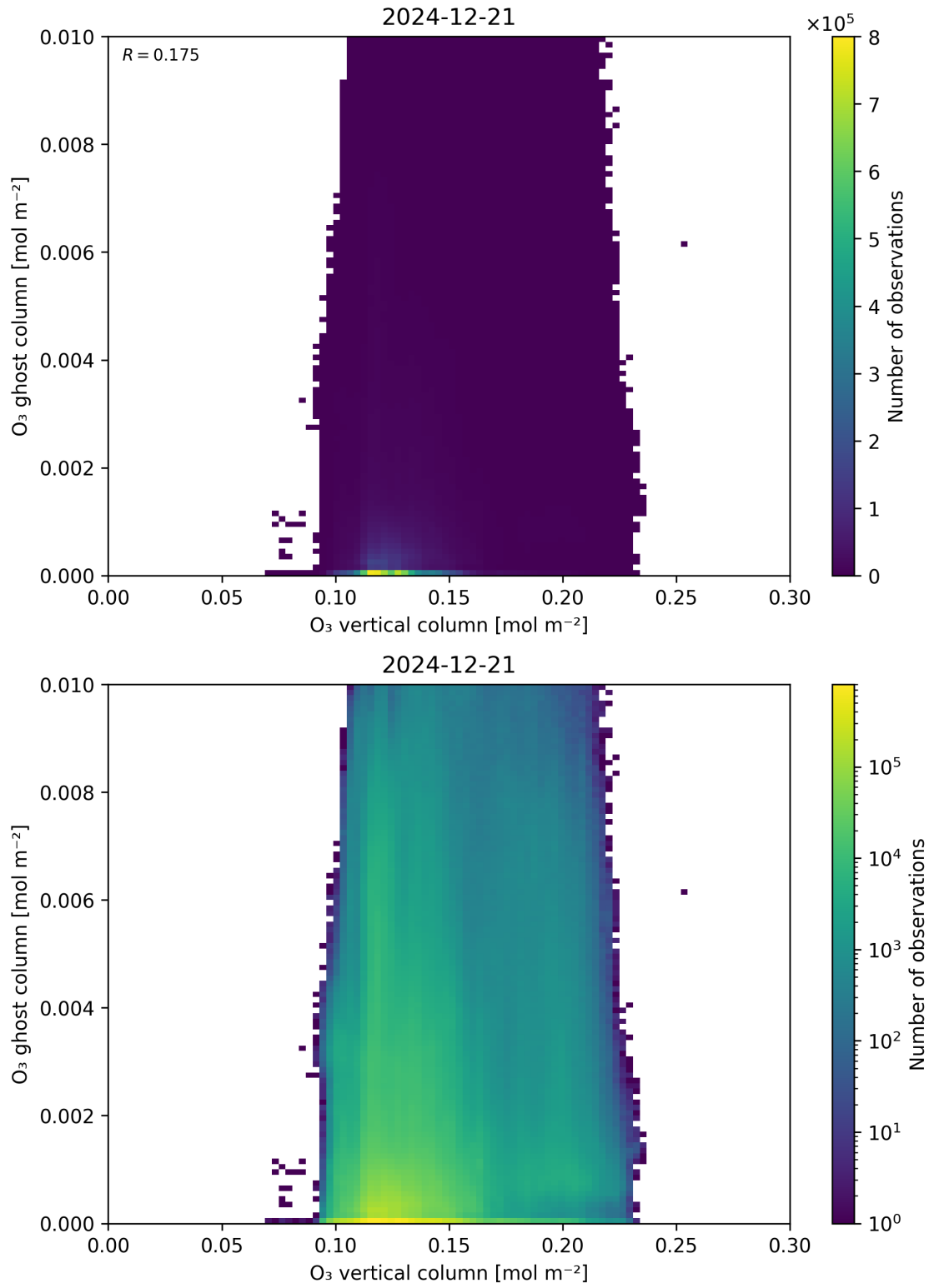
Figure 40: Scatter density plot of “O 3 vertical column” against “O 3 ghost column” for 2024-12-20 to 2024-12-22.
