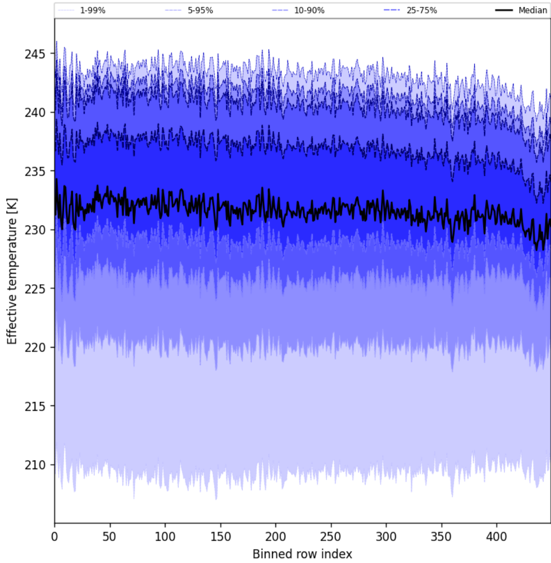
Figure 31: Along track statistics of “Effective temperature” for 2024-12-20 to 2024-12-22
