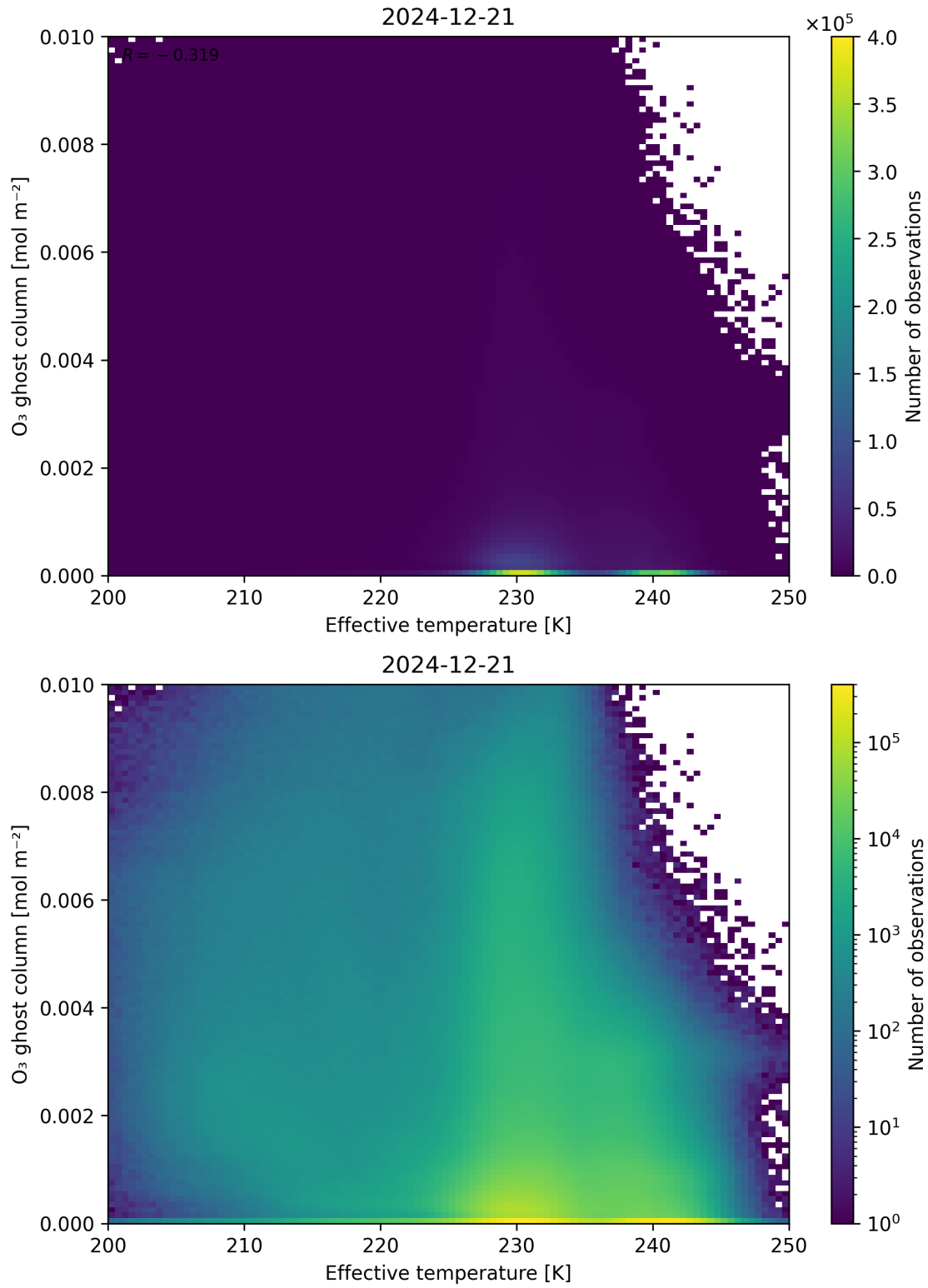
Figure 38: Scatter density plot of “Effective temperature” against “O 3 ghost column” for 2024-12-20 to 2024-12-22.
