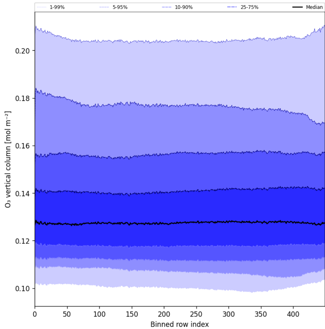
Figure 28: Along track statistics of "O 3 vertical column" for 2024-12-20 to 2024-12-22
