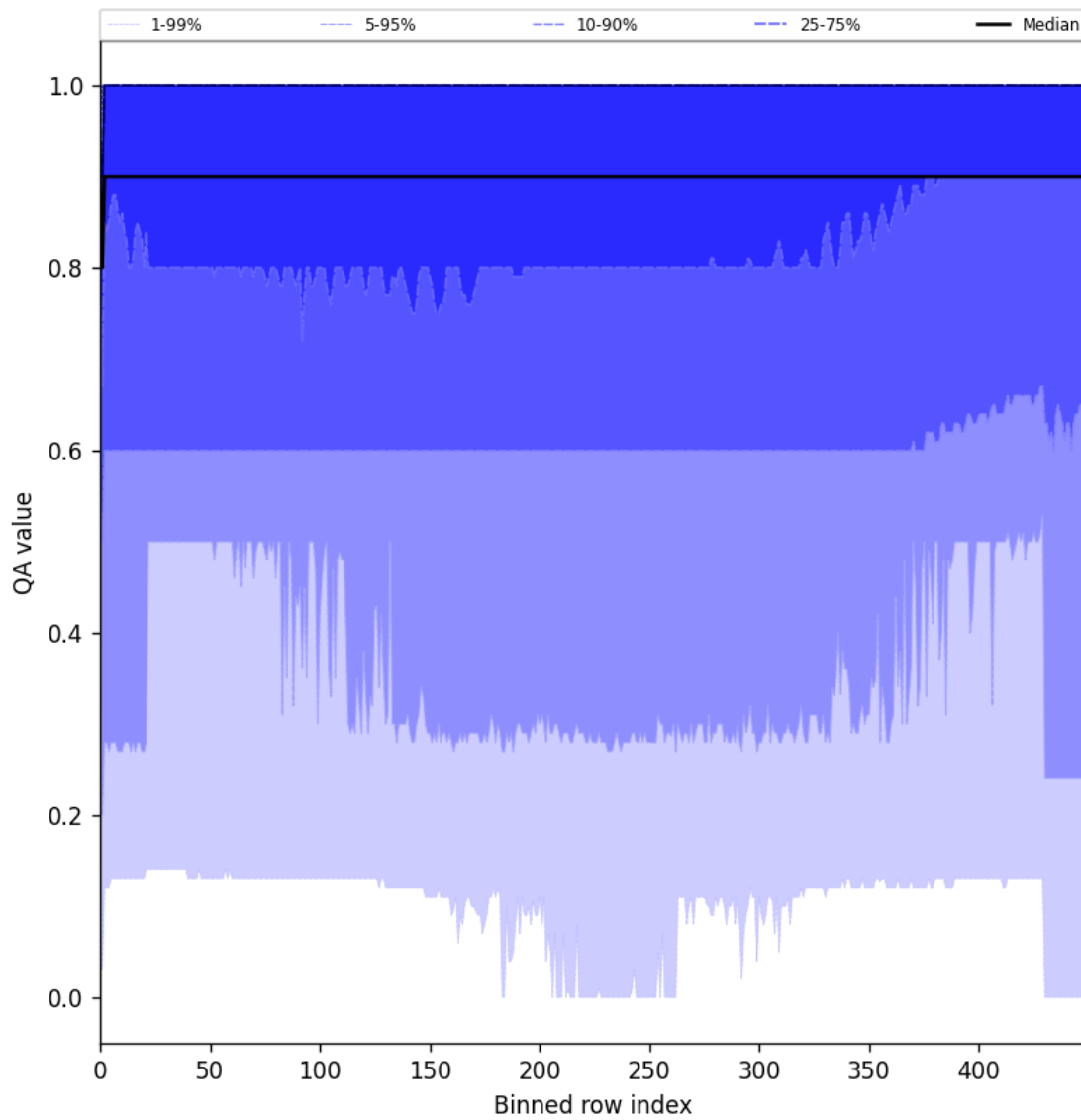
Figure 27: Along track statistics of “QA value” for 2024-12-20 to 2024-12-22
