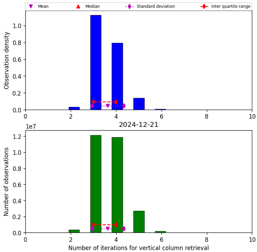
Figure 26: Histogram of “Number of iterations for vertical column retrieval” for 2024-12-20 to 2024-12-22
