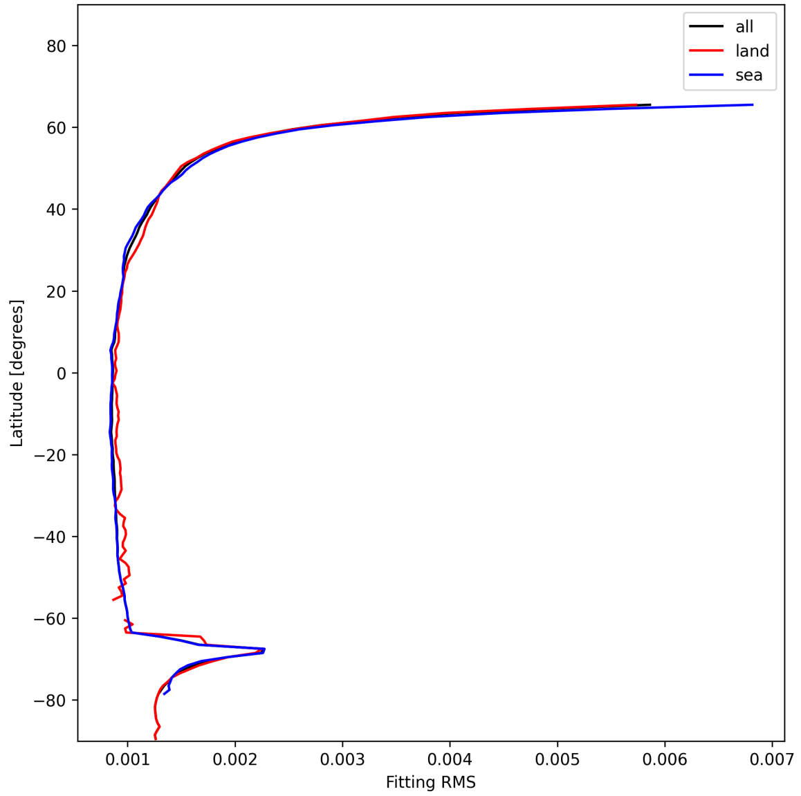
Figure 16: Zonal average of “Fitting RMS” for 2024-12-20 to 2024-12-22.
