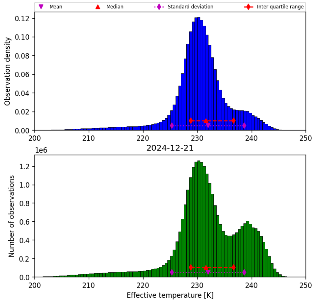
Figure 24: Histogram of “Effective temperature” for 2024-12-20 to 2024-12-22
