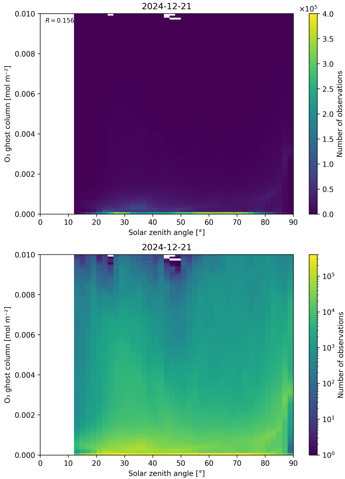
Figure 46: Scatter density plot of “Solar zenith angle” against “O 3 ghost column” for 2024-12-20 to 2024-12-22.
