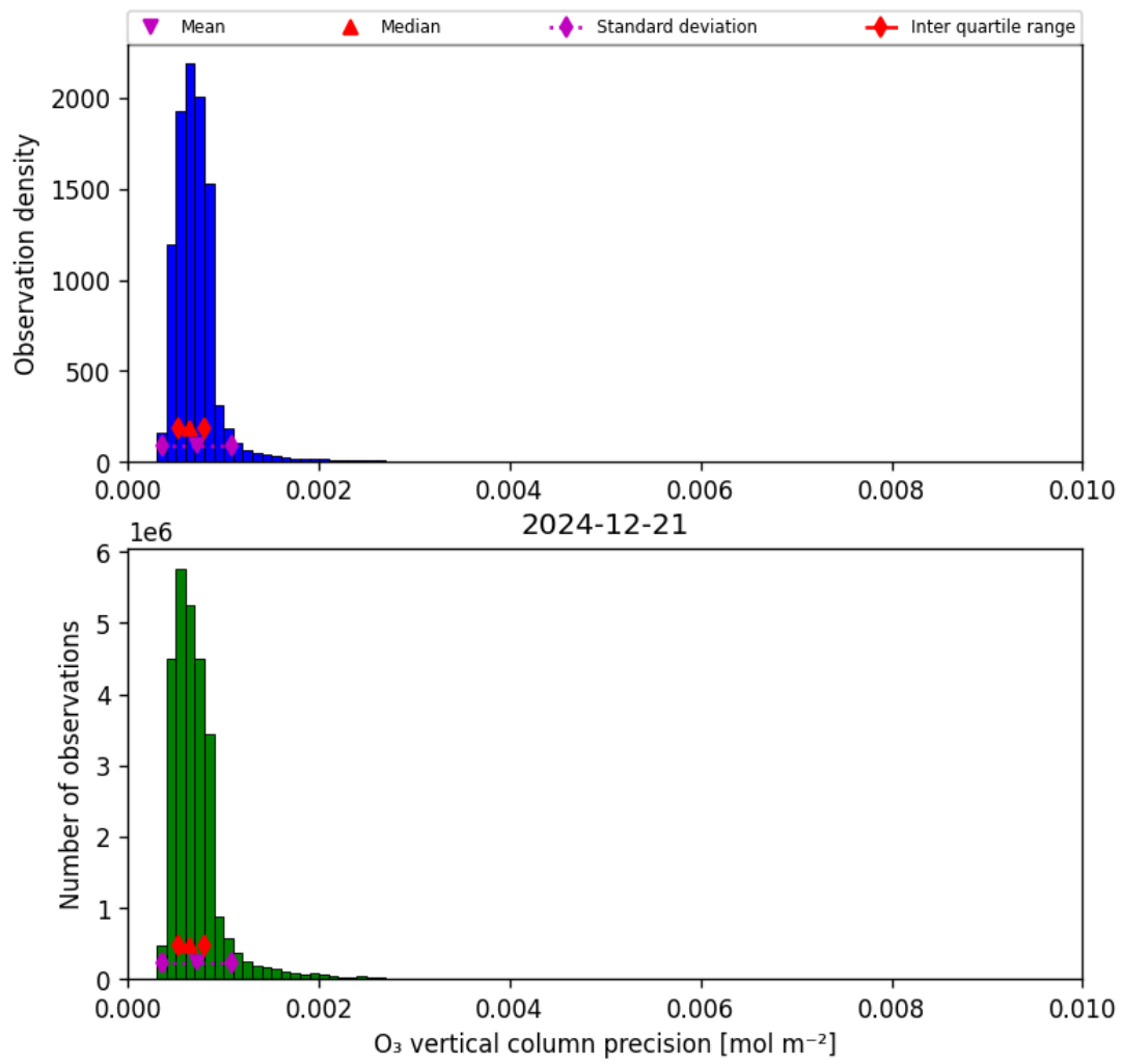
Figure 22: Histogram of “O 3 vertical column precision” for 2024-12-20 to 2024-12-22
