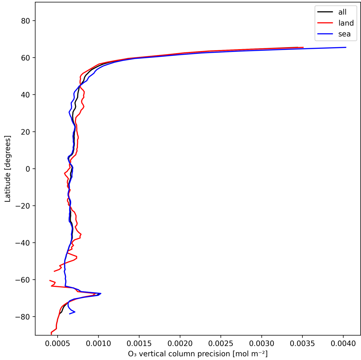
Figure 15: Zonal average of “O 3 vertical column precision” for 2024-12-20 to 2024-12-22.
