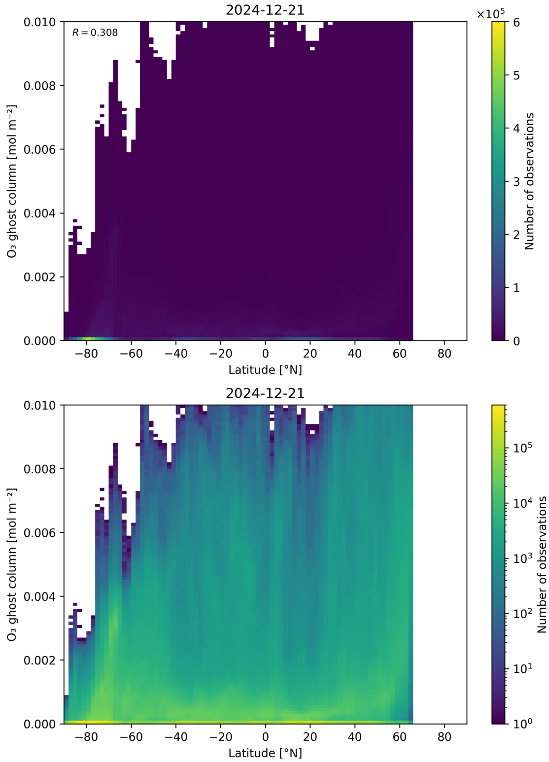
Figure 35: Scatter density plot of “Latitude” against “O 3 ghost column” for 2024-12-20 to 2024-12-22.
