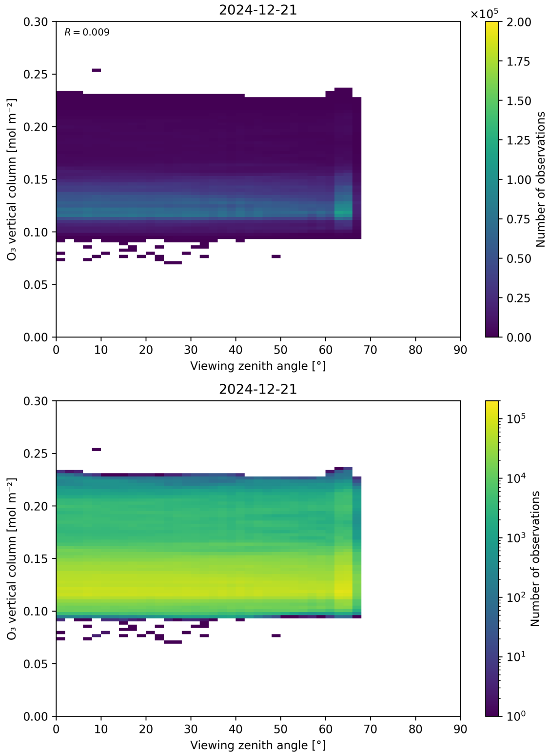
Figure 52: Scatter density plot of “Viewing zenith angle” against “O 3 vertical column” for 2024-12-20 to 2024-12-22.
