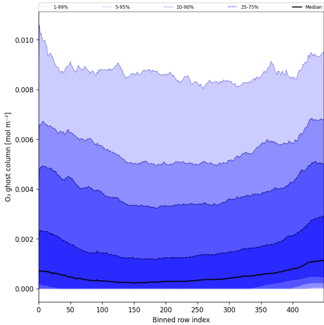
Figure 32: Along track statistics of “O 3 ghost column” for 2024-12-20 to 2024-12-22
