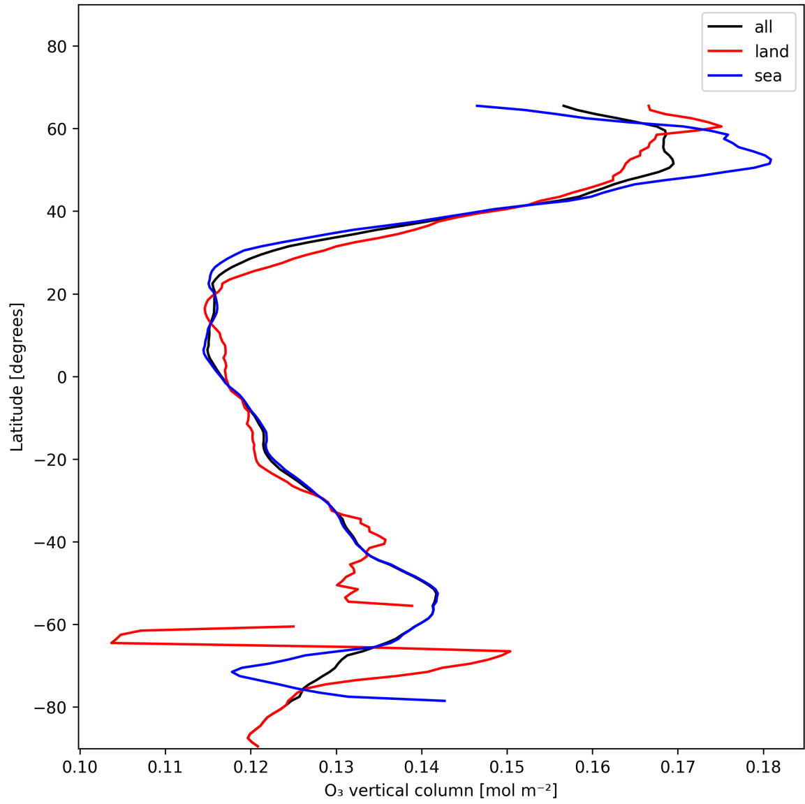
Figure 14: Zonal average of “O 3 vertical column” for 2024-12-20 to 2024-12-22.
