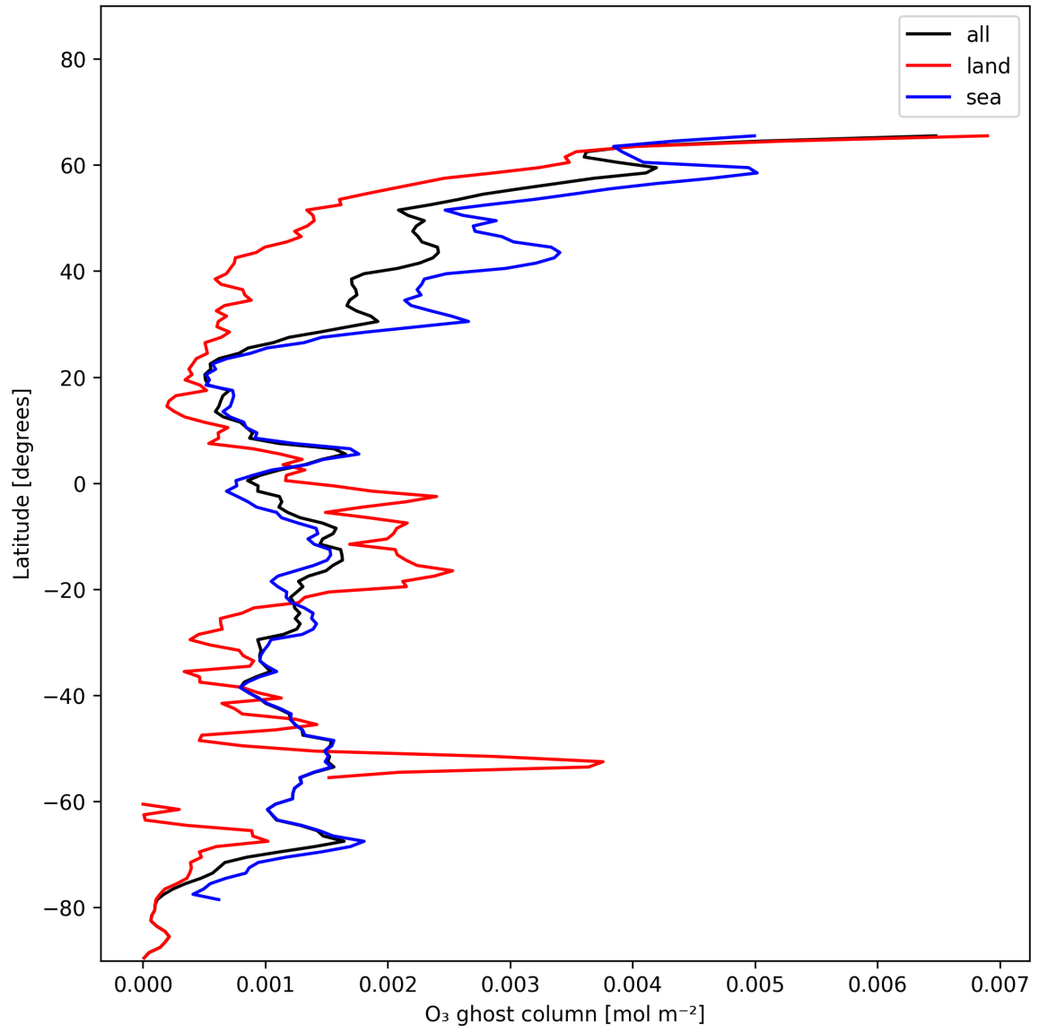
Figure 18: Zonal average of “O 3 ghost column” for 2024-12-20 to 2024-12-22.
