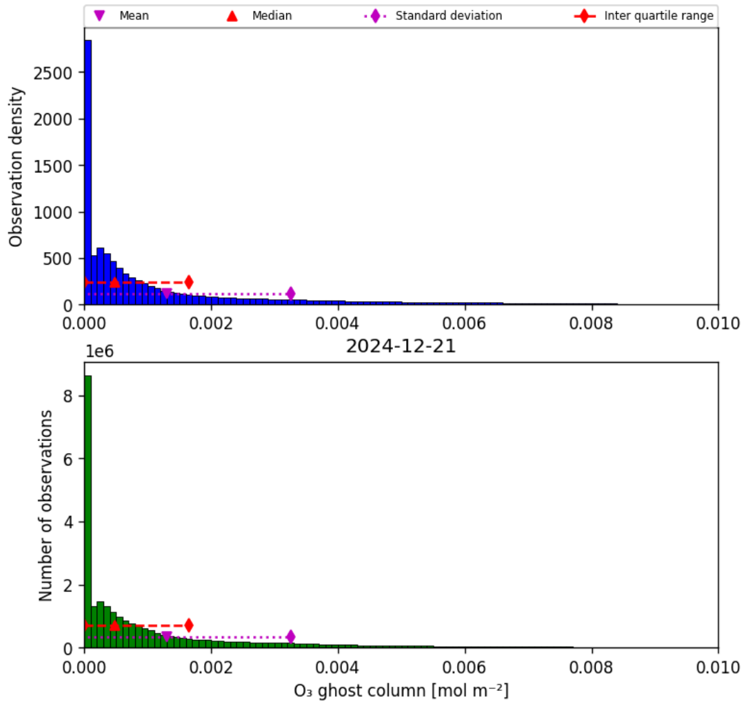
Figure 25: Histogram of "O 3 ghost column" for 2024-12-20 to 2024-12-22
