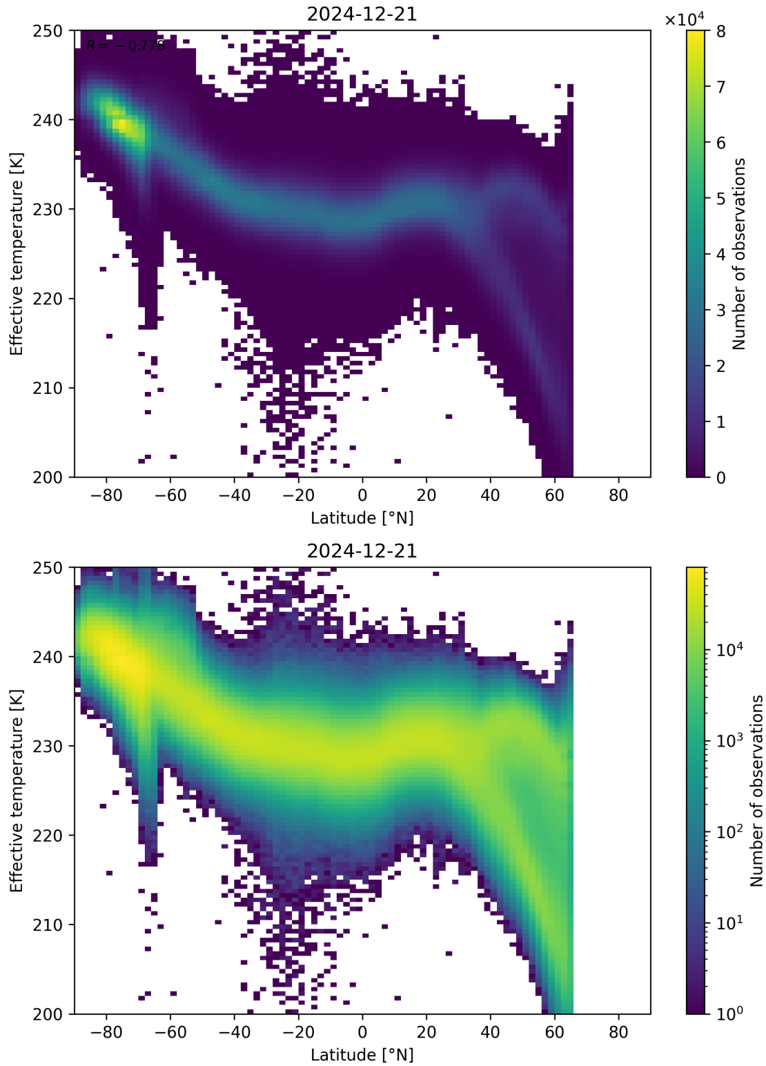
Figure 34: Scatter density plot of “Latitude” against “Effective temperature” for 2024-12-20 to 2024-12-22.
