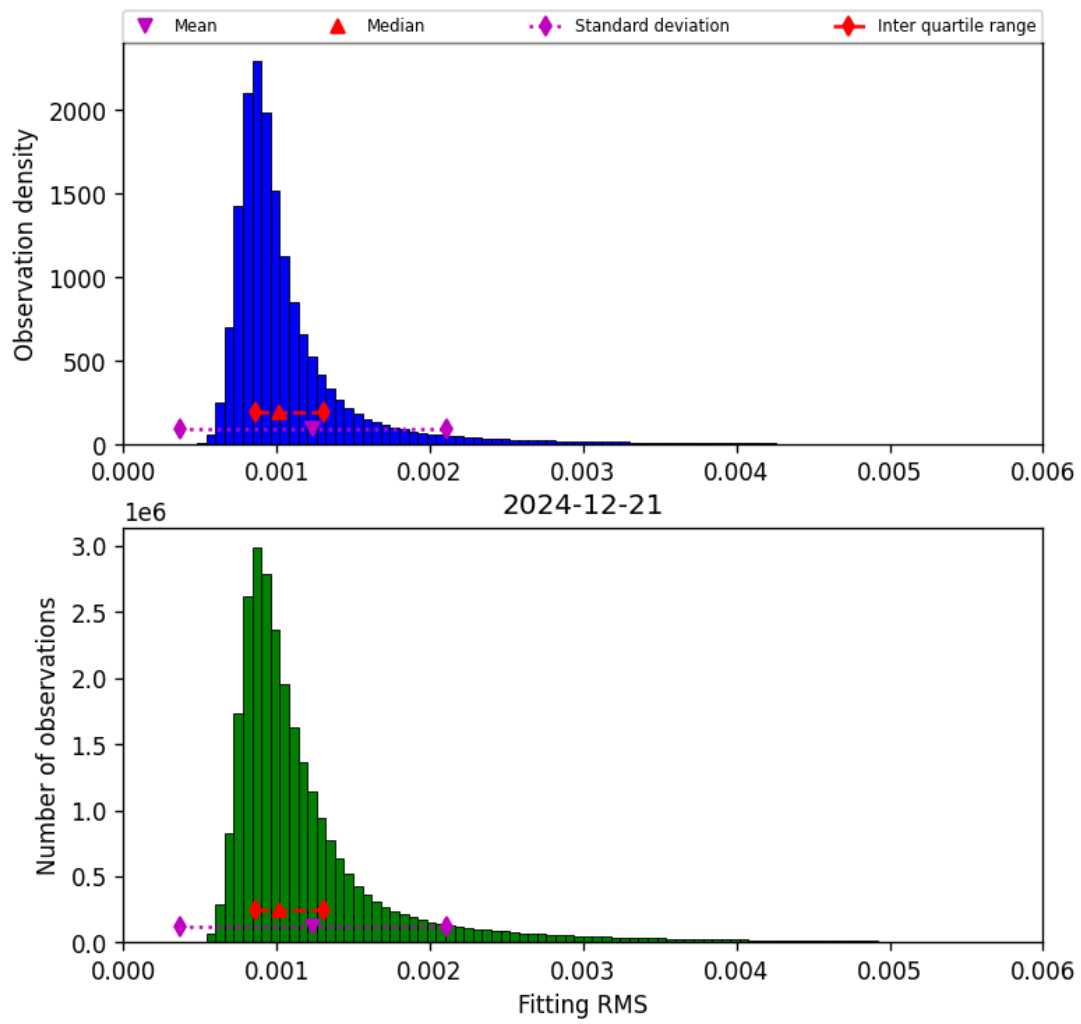
Figure 23: Histogram of “Fitting RMS” for 2024-12-20 to 2024-12-22
