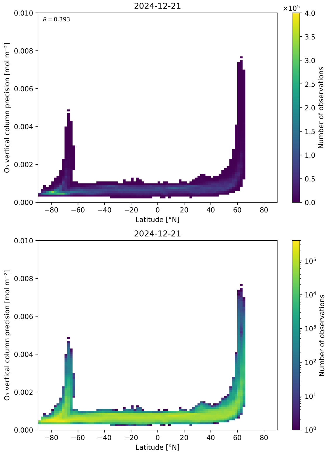
Figure 37: Scatter density plot of “Latitude” against “O 3 vertical column precision” for 2024-12-20 to 2024-12-22.
