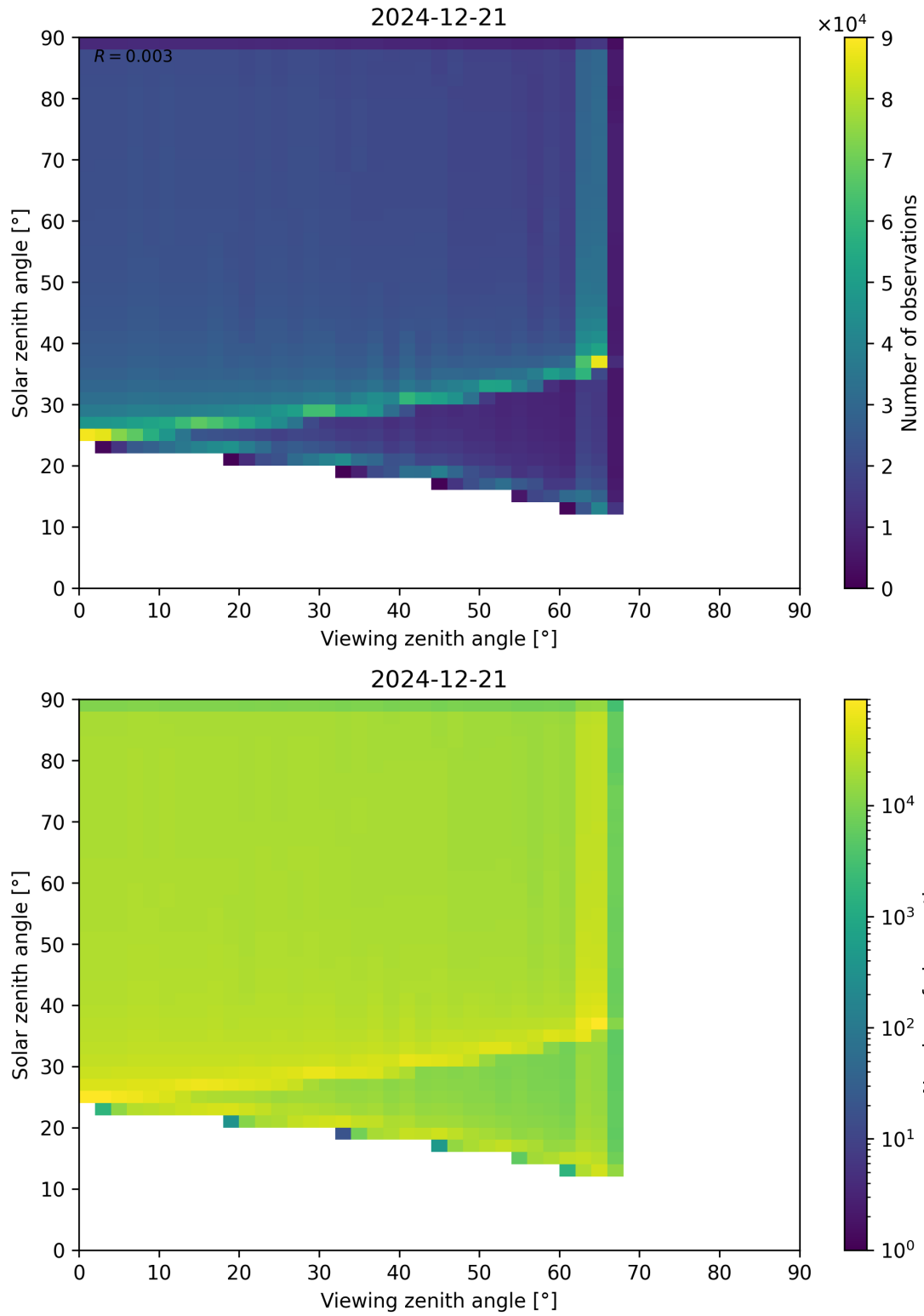
Figure 54: Scatter density plot of “Viewing zenith angle” against “Solar zenith angle” for 2024-12-20 to 2024-12-22.
