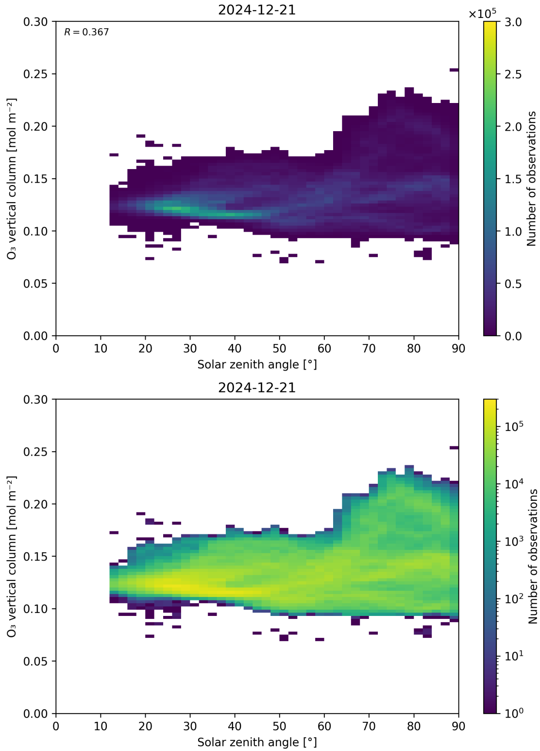
Figure 47: Scatter density plot of “Solar zenith angle” against “O 3 vertical column” for 2024-12-20 to 2024-12-22.
