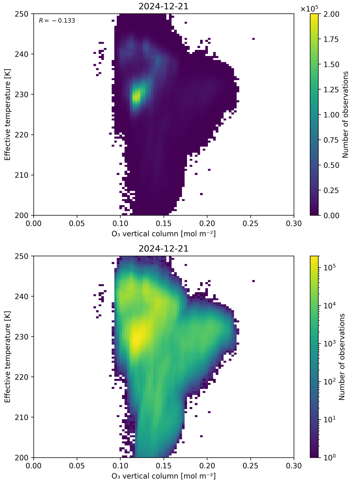
Figure 39: Scatter density plot of “O 3 vertical column” against “Effective temperature” for 2024-12-20 to 2024-12-22.
