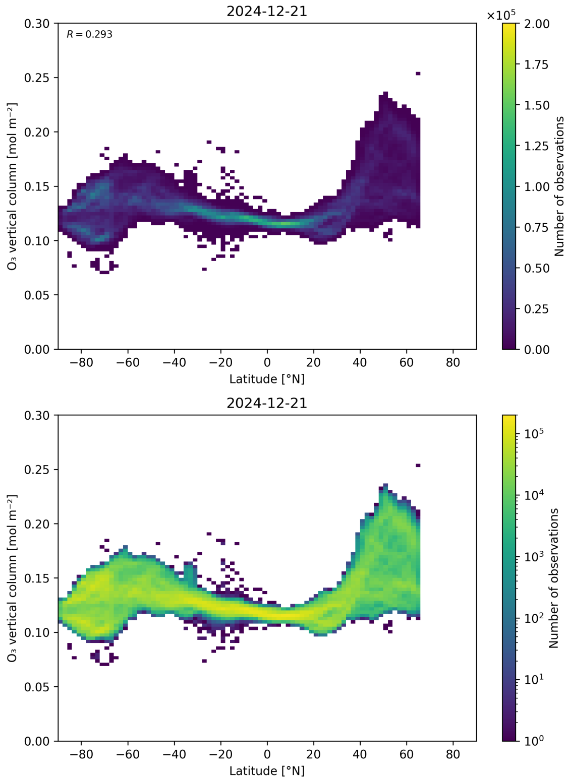
Figure 36: Scatter density plot of “Latitude” against “O 3 vertical column” for 2024-12-20 to 2024-12-22.
