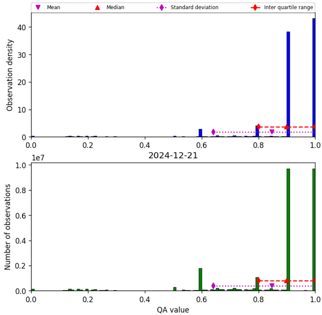
Figure 20: Histogram of “QA value” for 2024-12-20 to 2024-12-22
