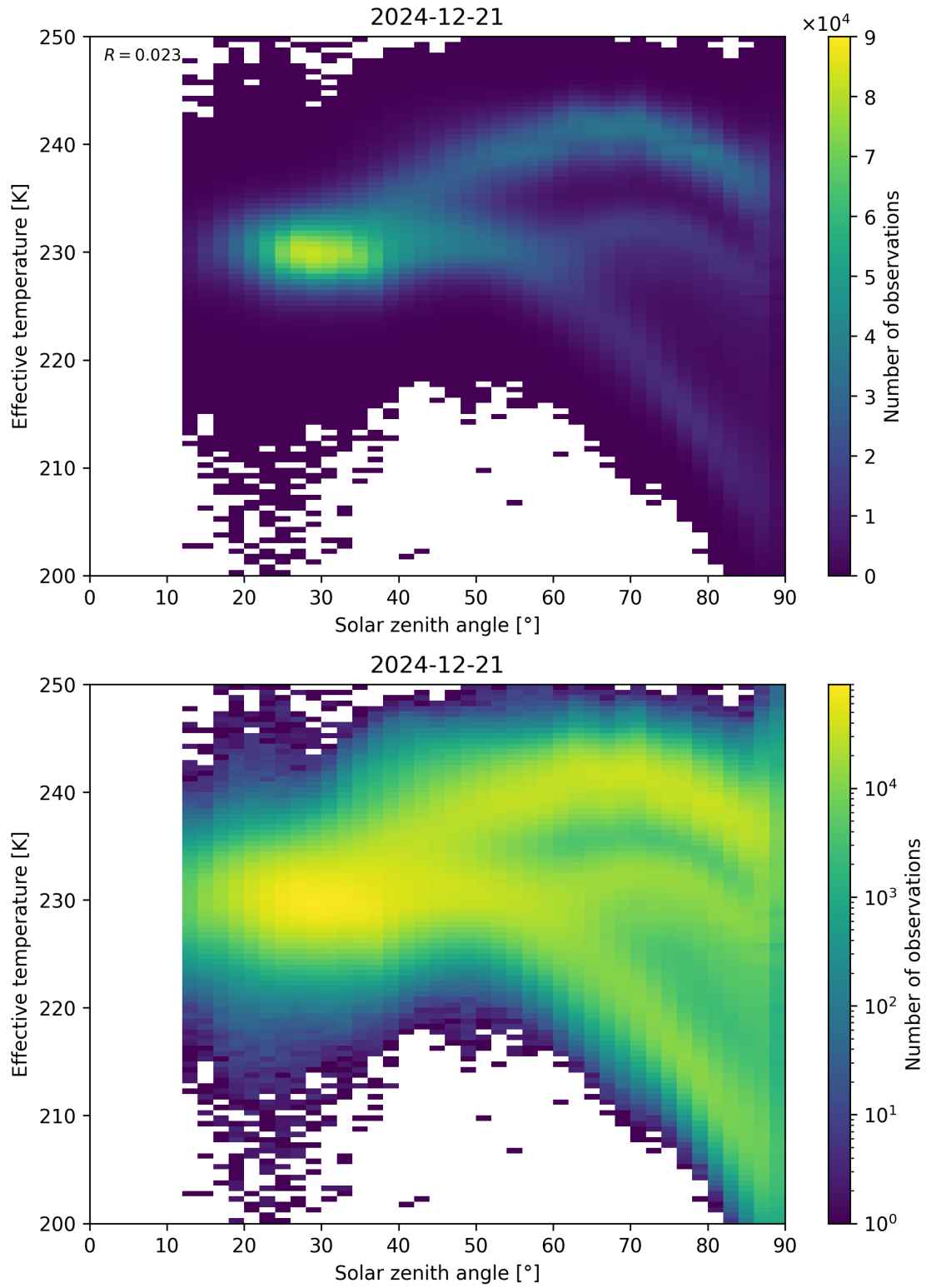
Figure 45: Scatter density plot of “Solar zenith angle” against “Effective temperature” for 2024-12-20 to 2024-12-22.
