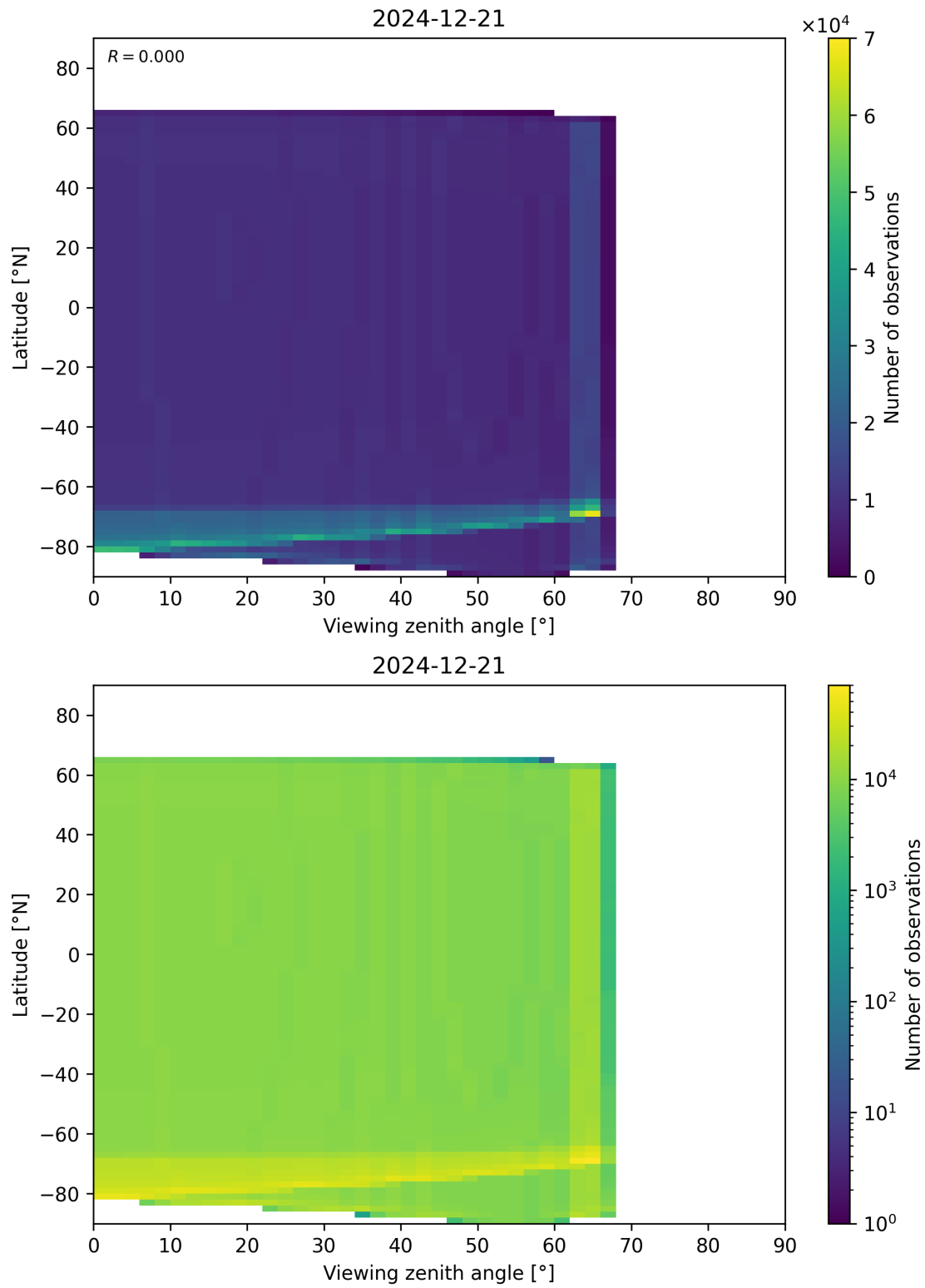
Figure 49: Scatter density plot of “Viewing zenith angle” against “Latitude” for 2024-12-20 to 2024-12-22.
