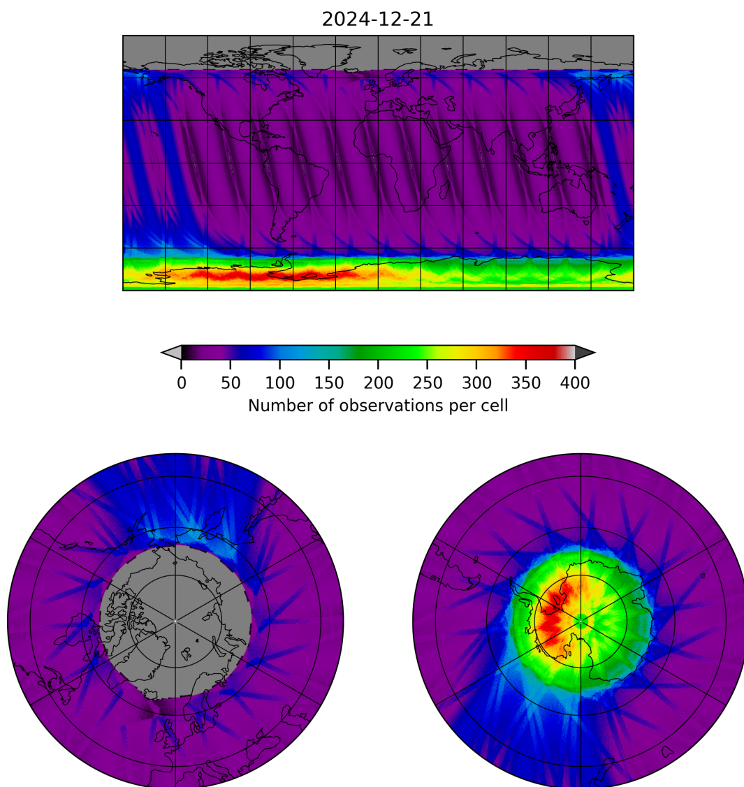
Figure 12: Map of the number of observations for 2024-12-20 to 2024-12-22
