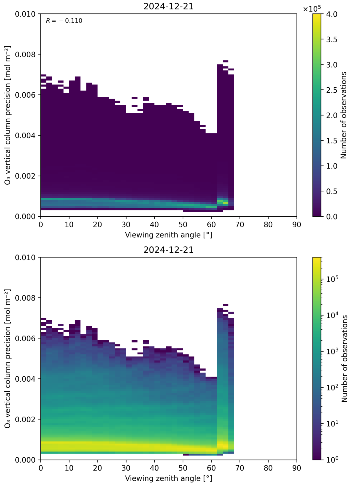
Figure 53: Scatter density plot of “Viewing zenith angle” against “O 3 vertical column precision” for 2024-12-20 to 2024-12-22.
