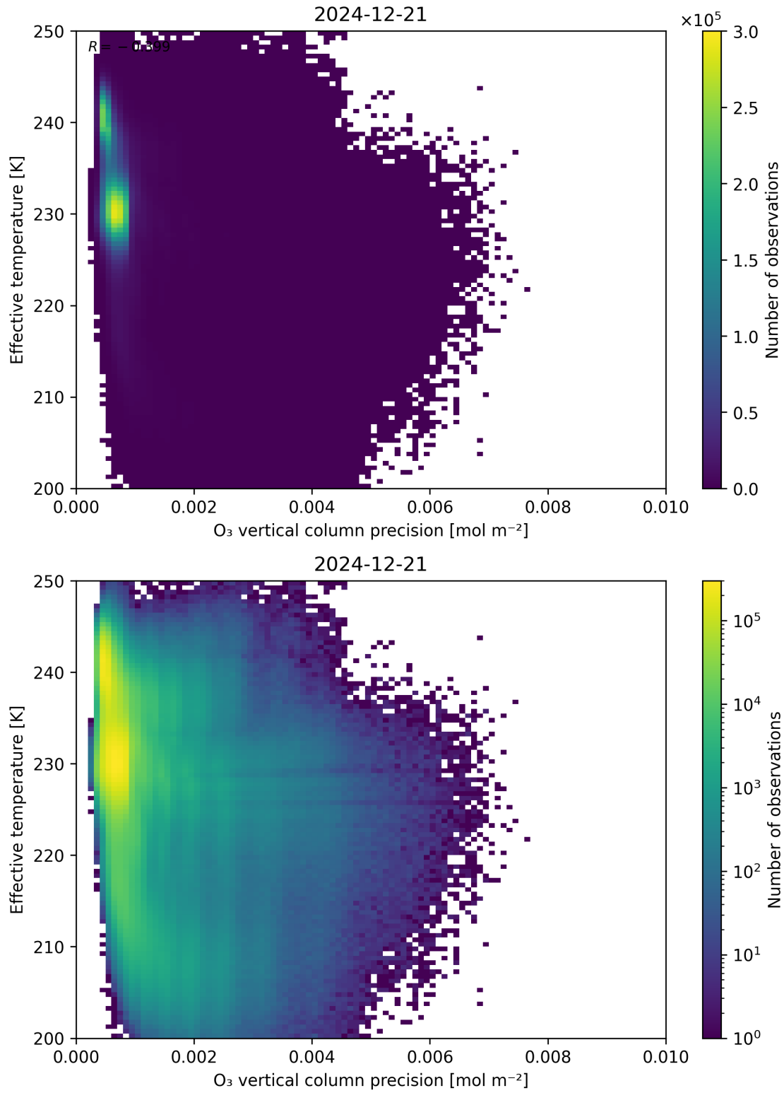
Figure 42: Scatter density plot of “O 3 vertical column precision” against “Effective temperature” for 2024-12-20 to 2024-12-22.
