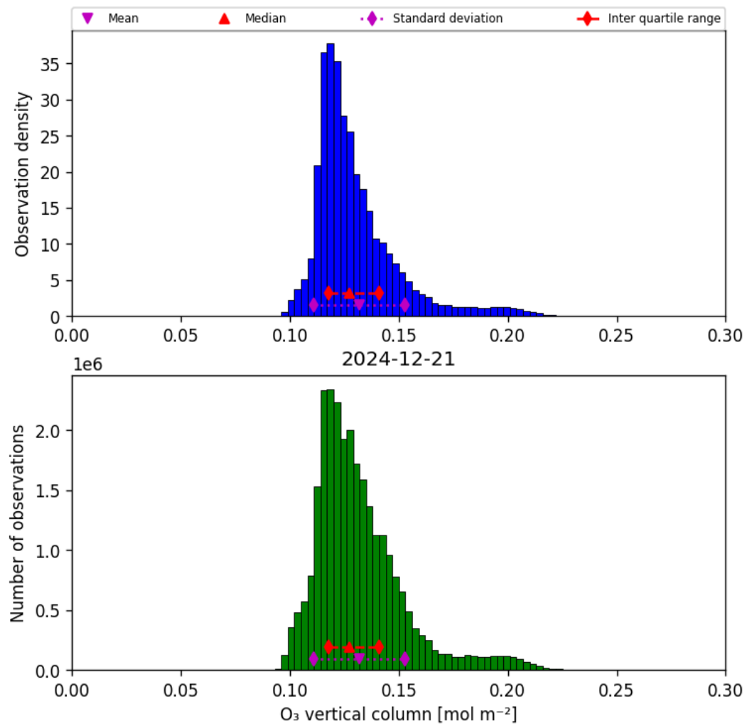
Figure 21: Histogram of “O 3 vertical column” for 2024-12-20 to 2024-12-22
