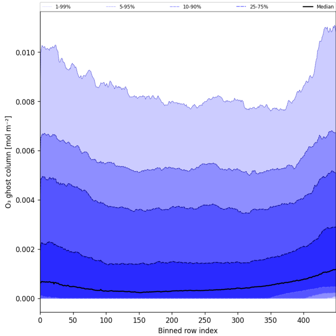
Figure 32: Along track statistics of “O 3 ghost column” for 2024-12-22 to 2024-12-23
