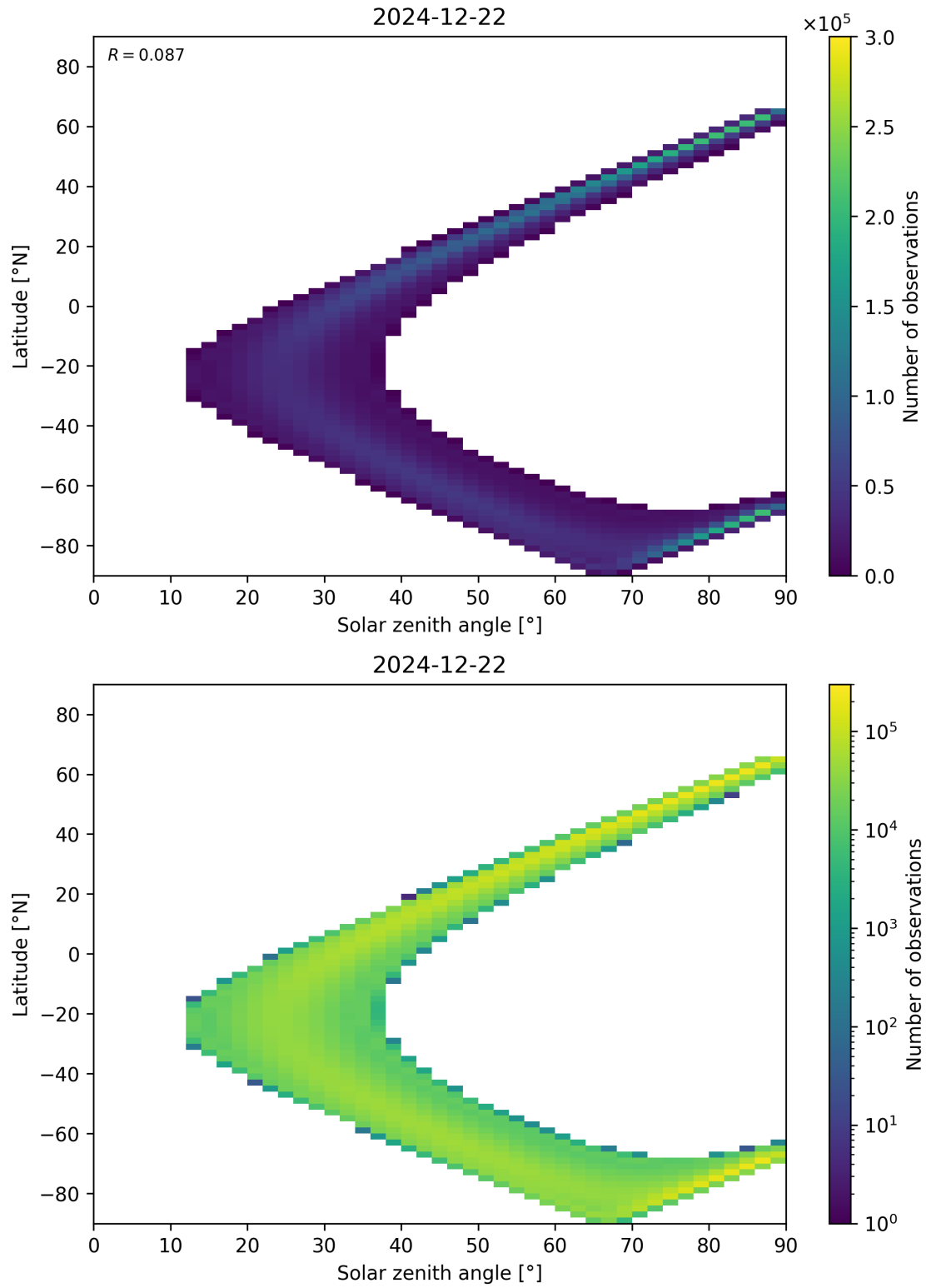
Figure 44: Scatter density plot of “Solar zenith angle” against “Latitude” for 2024-12-22 to 2024-12-23.
