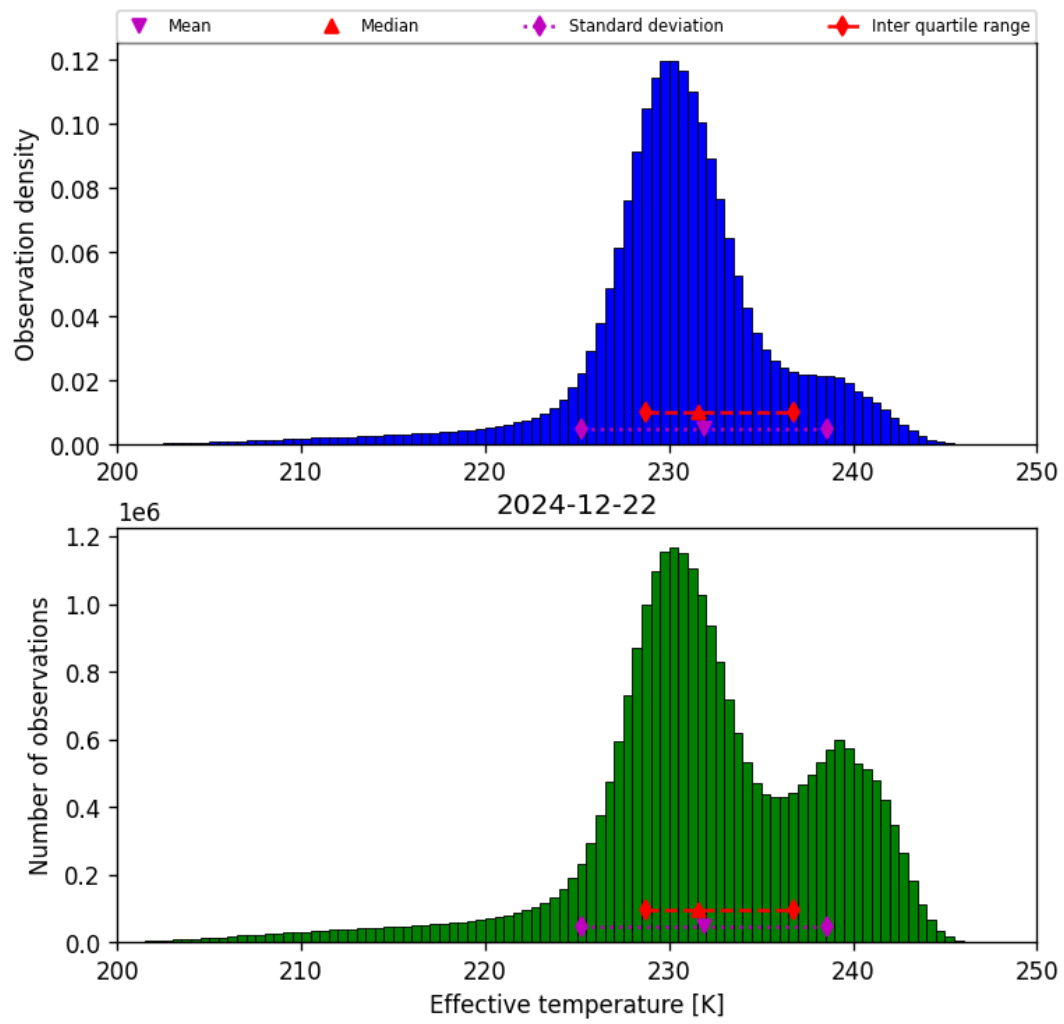
Figure 24: Histogram of “Effective temperature” for 2024-12-22 to 2024-12-23
