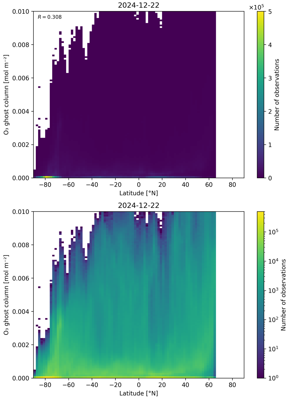
Figure 35: Scatter density plot of “Latitude” against “O 3 ghost column” for 2024-12-22 to 2024-12-23.
