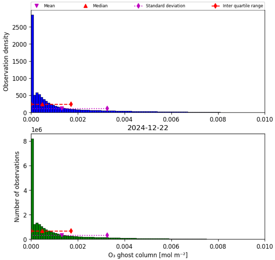
Figure 25: Histogram of “O 3 ghost column” for 2024-12-22 to 2024-12-23
