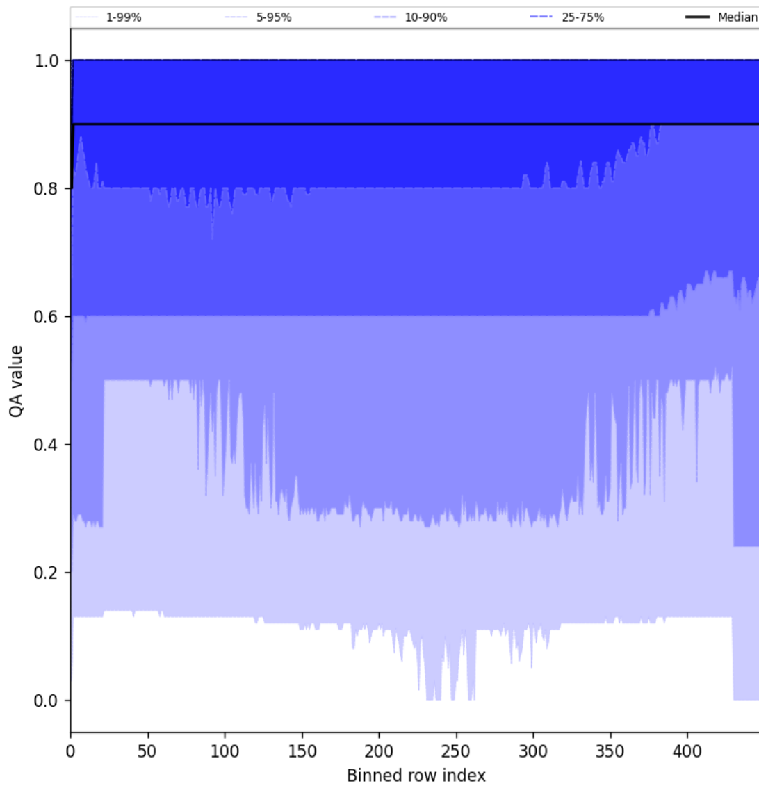
Figure 27: Along track statistics of “QA value” for 2024-12-22 to 2024-12-23
