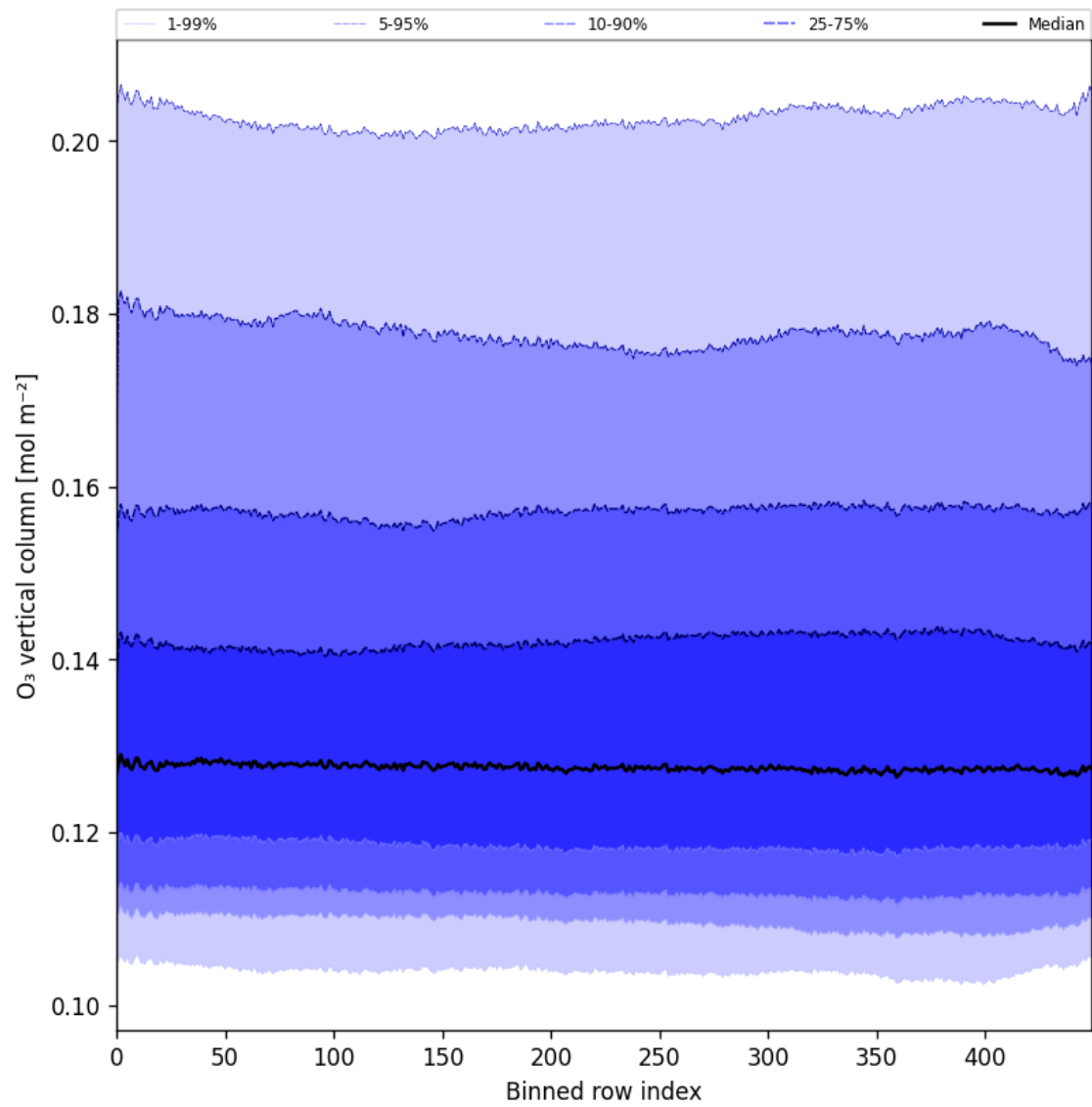
Figure 28: Along track statistics of “O 3 vertical column” for 2024-12-22 to 2024-12-23
