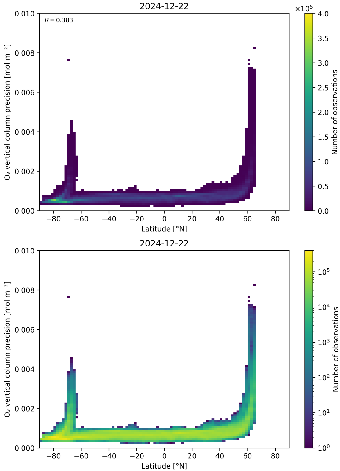
Figure 37: Scatter density plot of “Latitude” against “O 3 vertical column precision” for 2024-12-22 to 2024-12-23.
