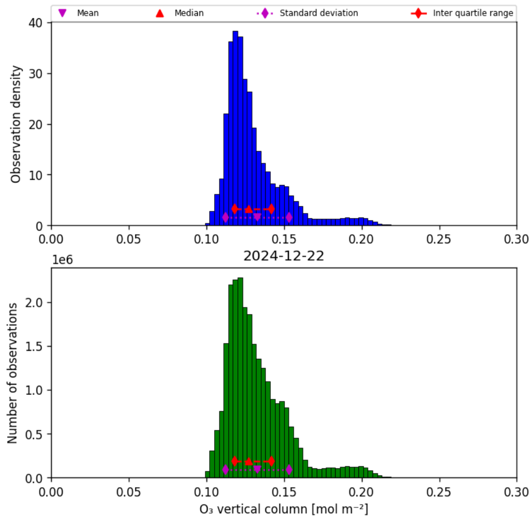
Figure 21: Histogram of “O 3 vertical column” for 2024-12-22 to 2024-12-23
