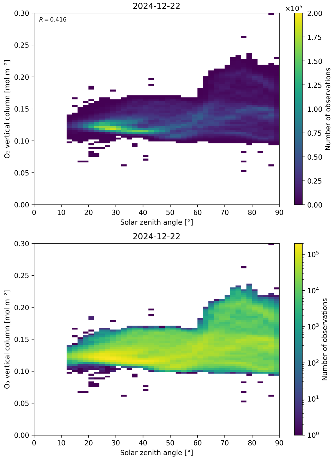
Figure 47: Scatter density plot of “Solar zenith angle” against “O 3 vertical column” for 2024-12-22 to 2024-12-23.
