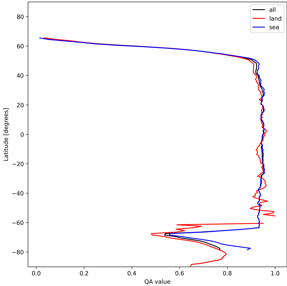
Figure 13: Zonal average of “QA value” for 2024-12-22 to 2024-12-23.
