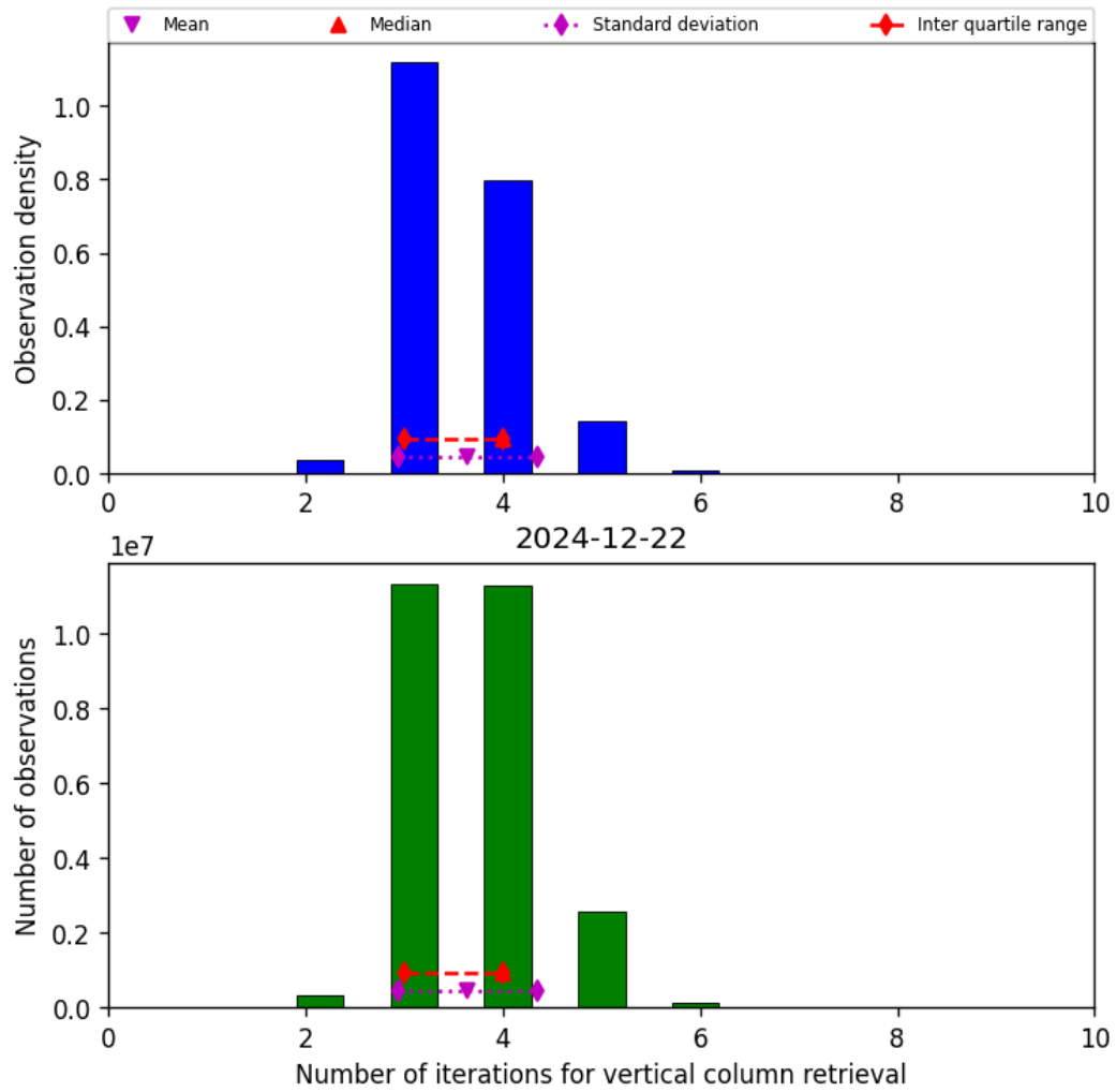
Figure 26: Histogram of “Number of iterations for vertical column retrieval” for 2024-12-22 to 2024-12-23
