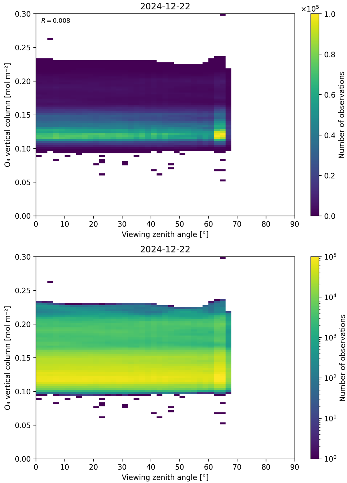
Figure 52: Scatter density plot of “Viewing zenith angle” against “O 3 vertical column” for 2024-12-22 to 2024-12-23.
