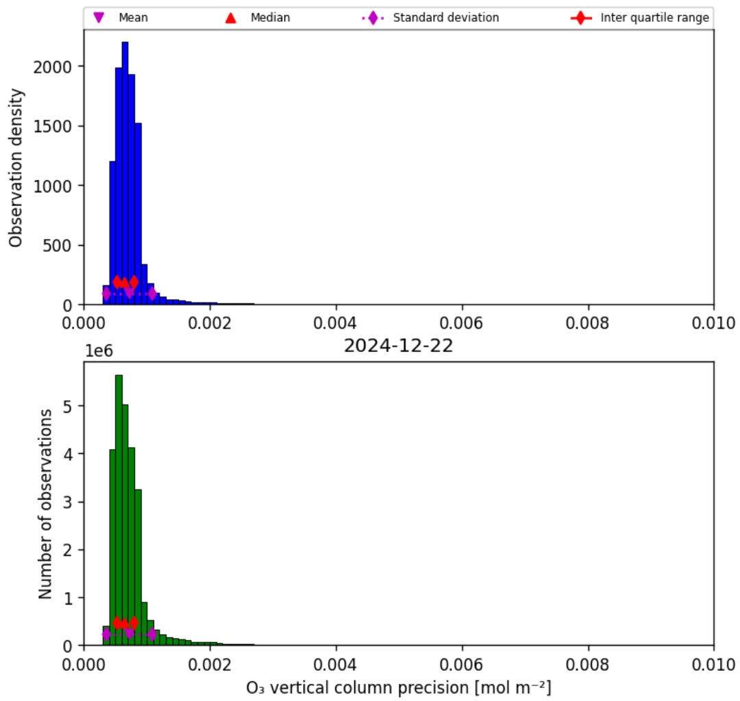
Figure 22: Histogram of “O 3 vertical column precision” for 2024-12-22 to 2024-12-23
