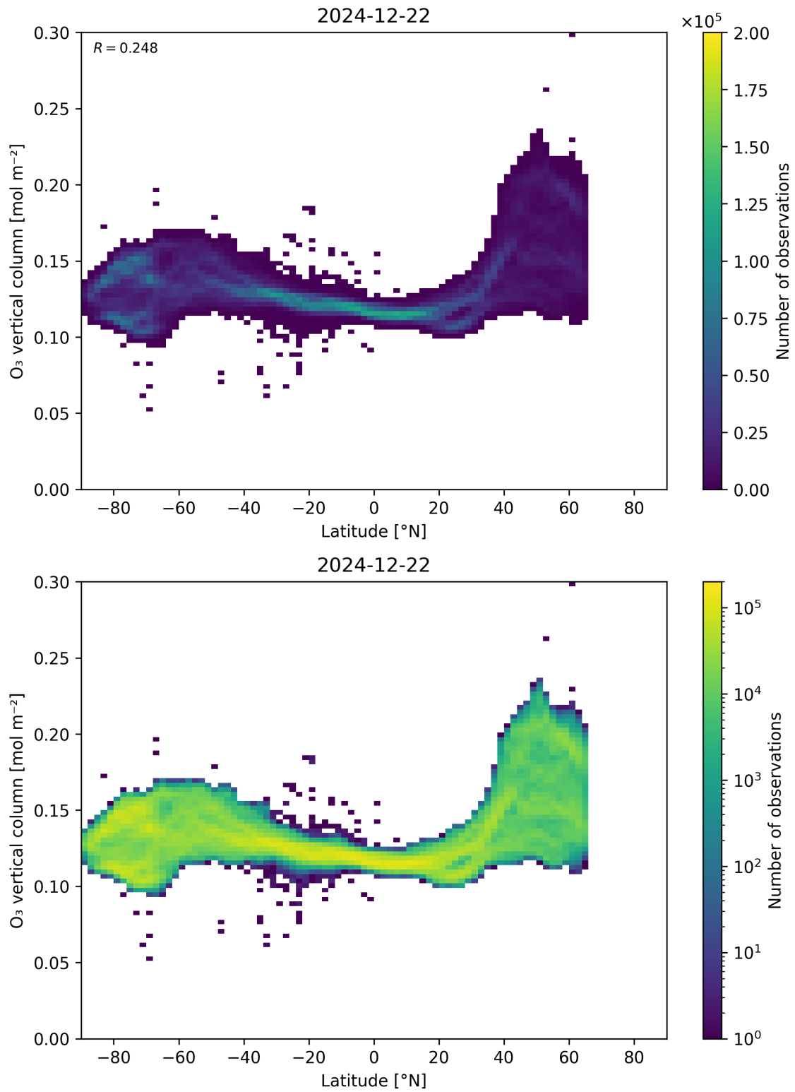
Figure 36: Scatter density plot of “Latitude” against “O 3 vertical column” for 2024-12-22 to 2024-12-23.
