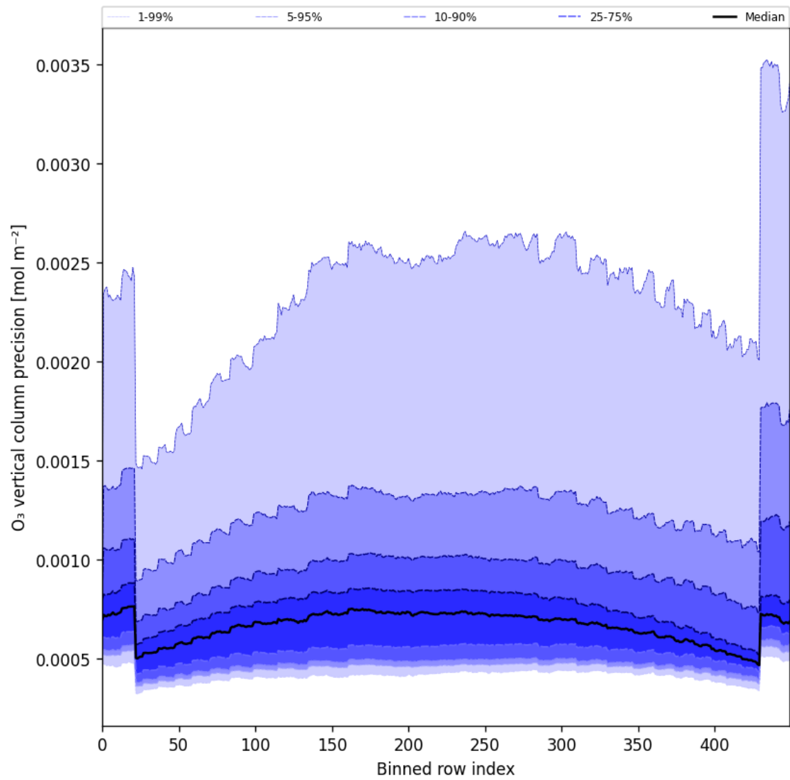
Figure 29: Along track statistics of “O 3 vertical column precision” for 2024-12-22 to 2024-12-23
