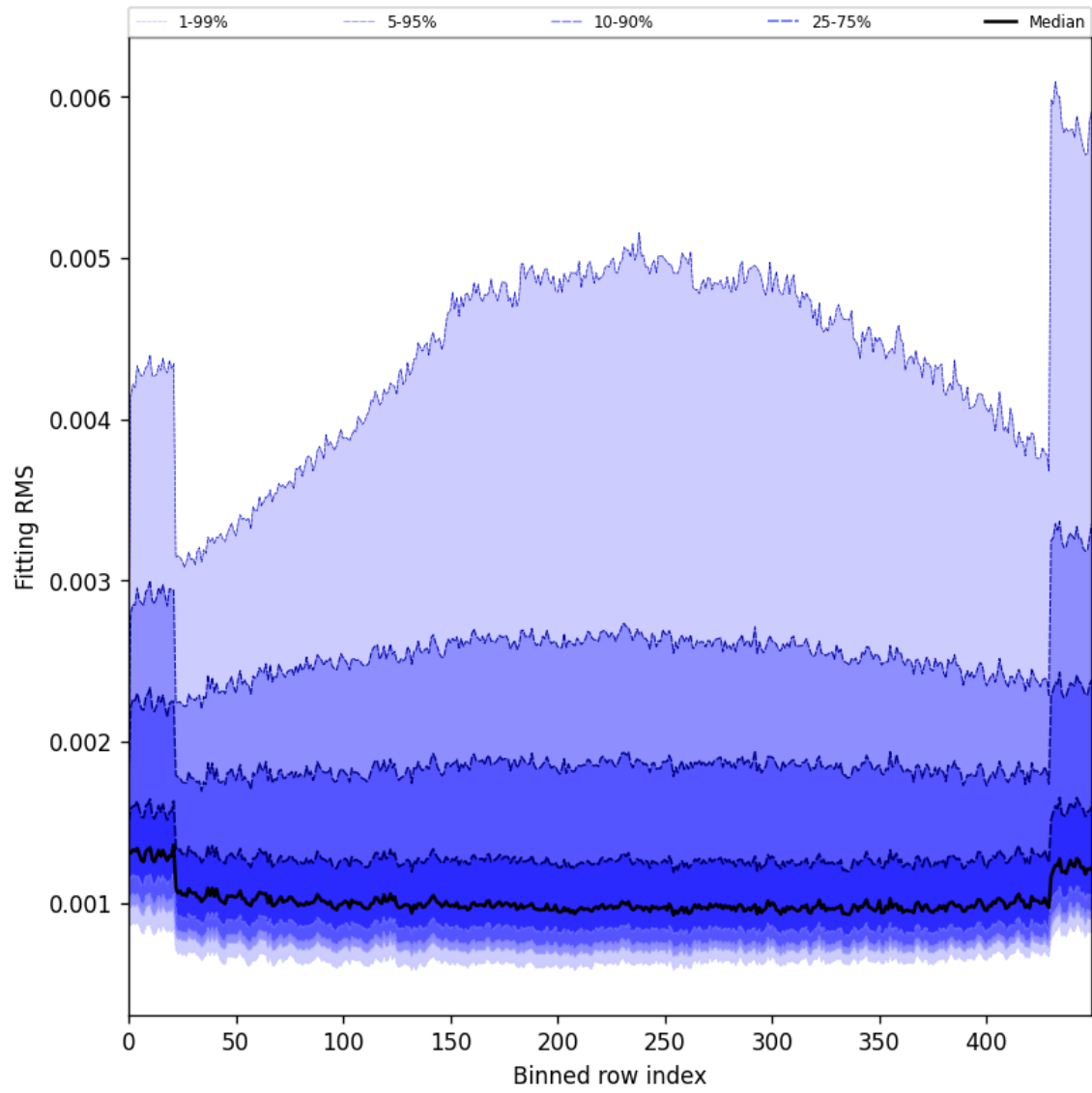
Figure 30: Along track statistics of “Fitting RMS” for 2024-12-22 to 2024-12-23
