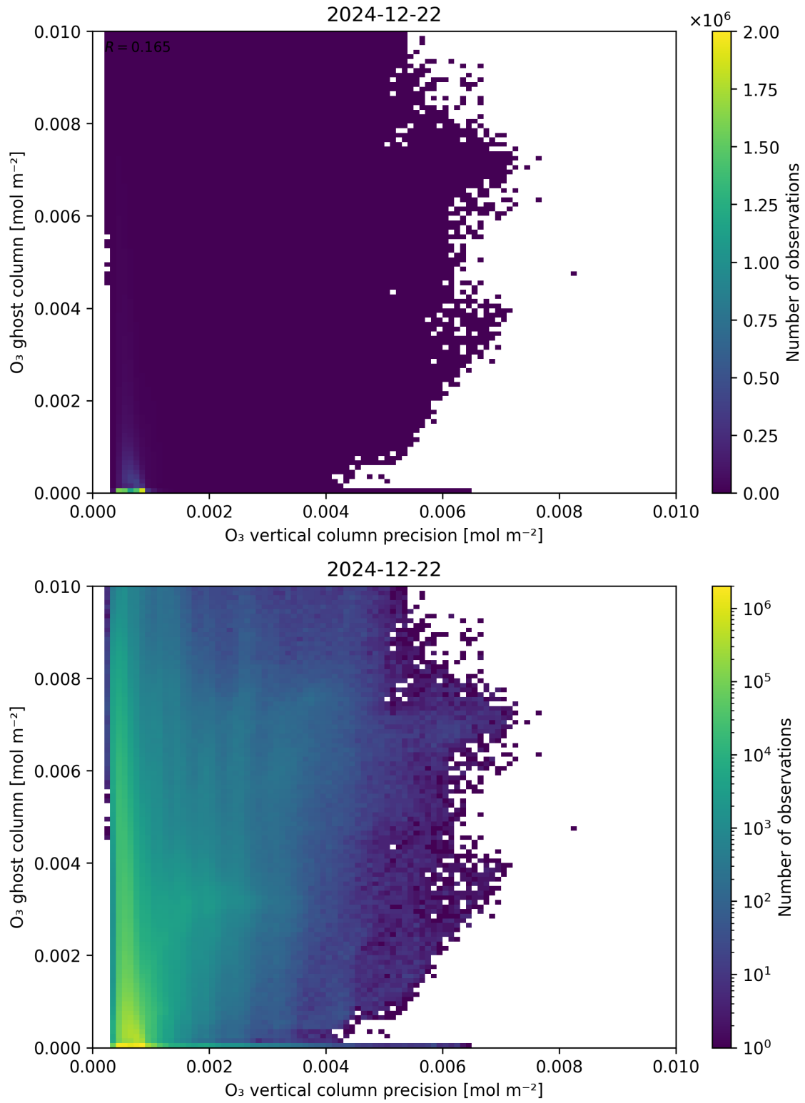
Figure 43: Scatter density plot of “ \text{O}_3 vertical column precision” against “ \text{O}_3 ghost column” for 2024-12-22 to 2024-12-23.
