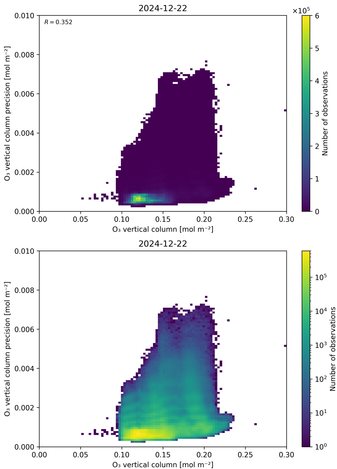
Figure 41: Scatter density plot of “O 3 vertical column” against “O 3 vertical column precision” for 2024-12-22 to 2024-12-23.
