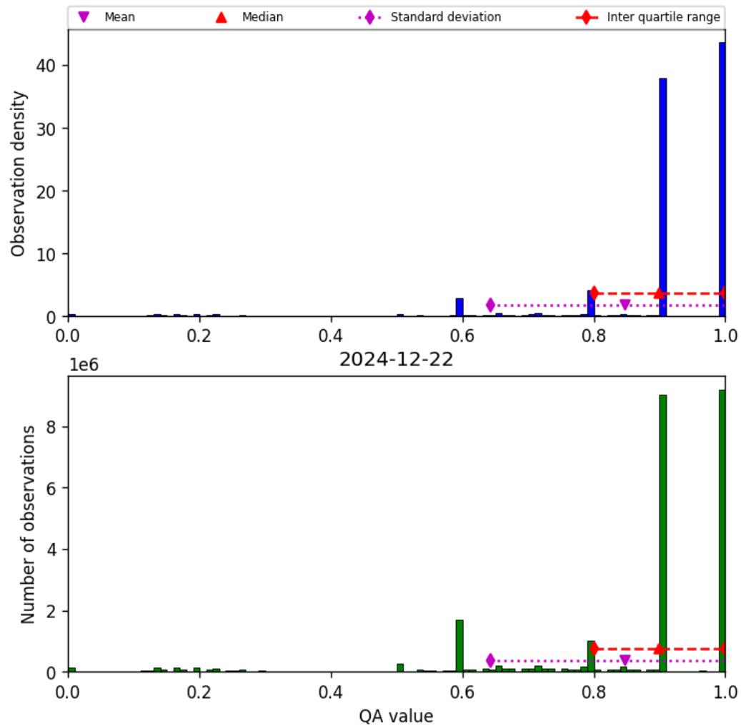
Figure 20: Histogram of “QA value” for 2024-12-22 to 2024-12-23
