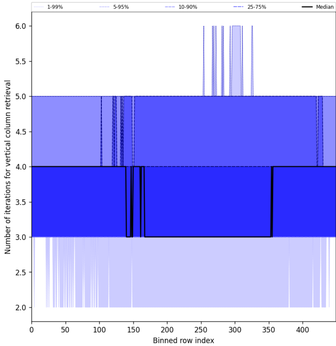
Figure 33: Along track statistics of “Number of iterations for vertical column retrieval” for 2024-12-22 to 2024-12-23
