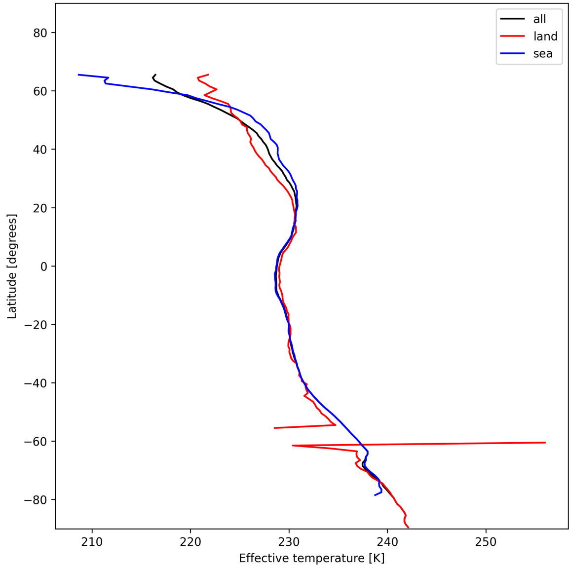
Figure 17: Zonal average of "Effective temperature" for 2024-12-22 to 2024-12-23.
