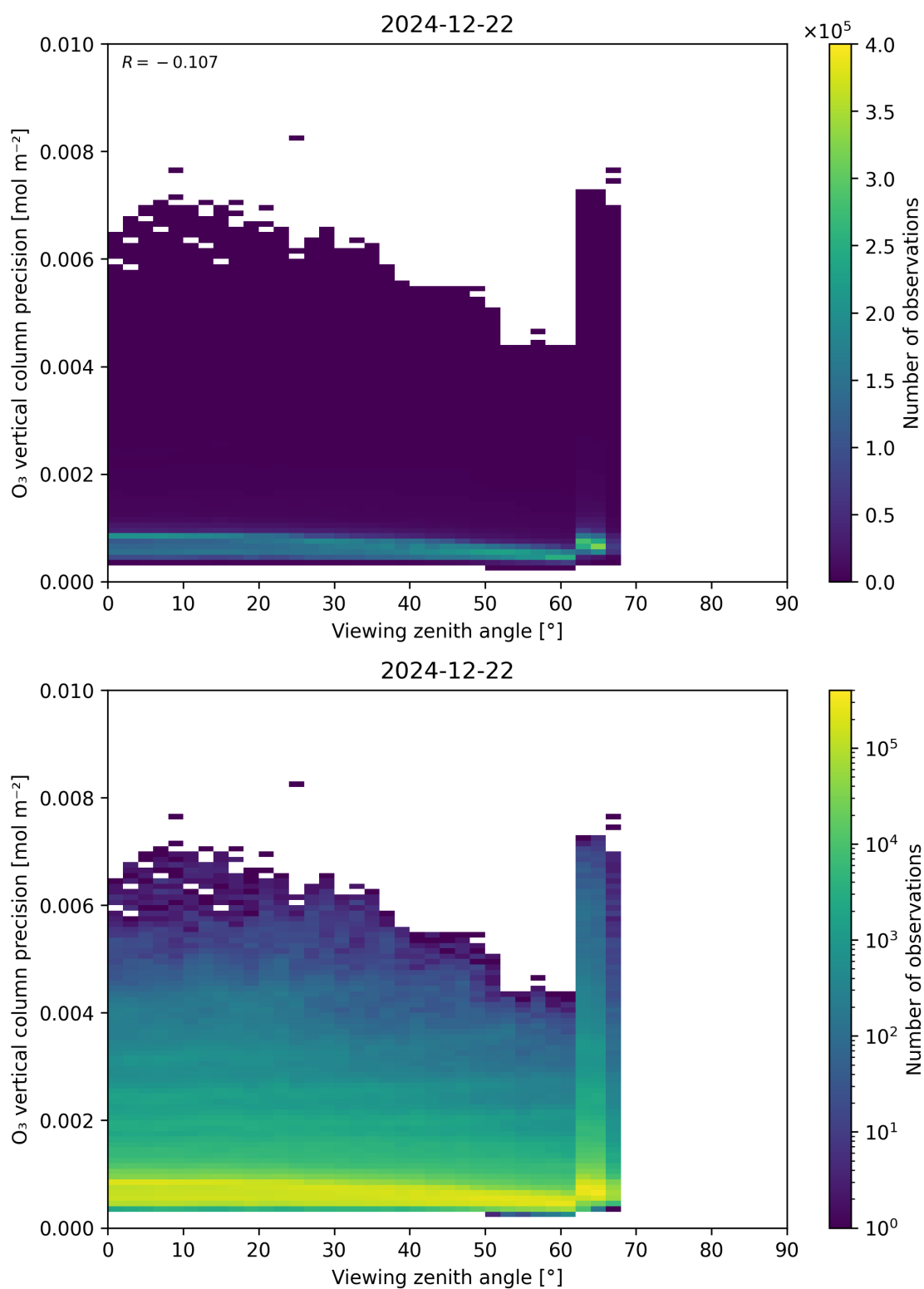
Figure 53: Scatter density plot of “Viewing zenith angle” against “O 3 vertical column precision” for 2024-12-22 to 2024-12-23.
