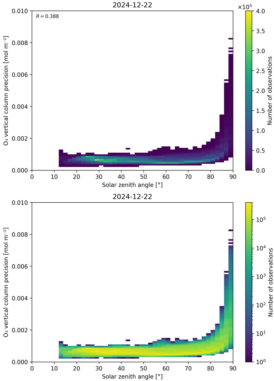
Figure 48: Scatter density plot of “Solar zenith angle” against “O 3 vertical column precision” for 2024-12-22 to 2024-12-23.
