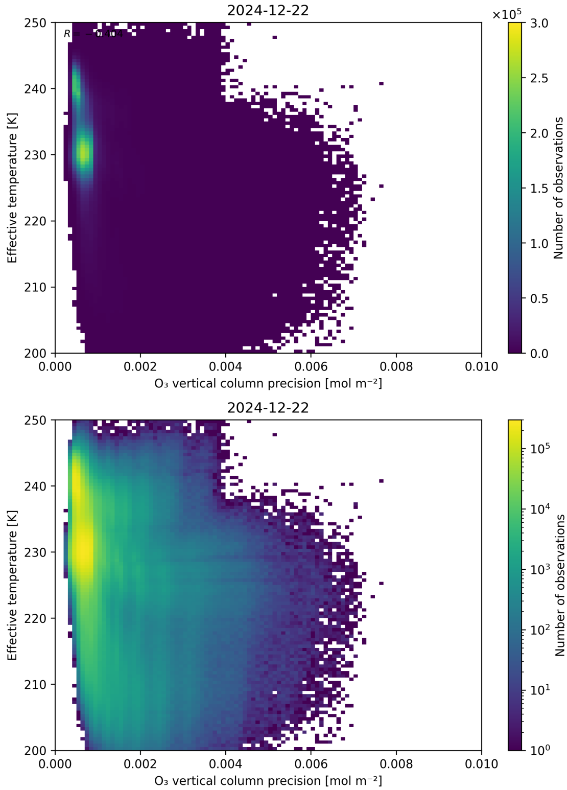
Figure 42: Scatter density plot of “O 3 vertical column precision” against “Effective temperature” for 2024-12-22 to 2024-12-23.
