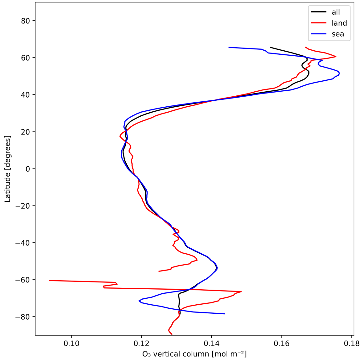
Figure 14: Zonal average of “O 3 vertical column” for 2024-12-22 to 2024-12-23.
