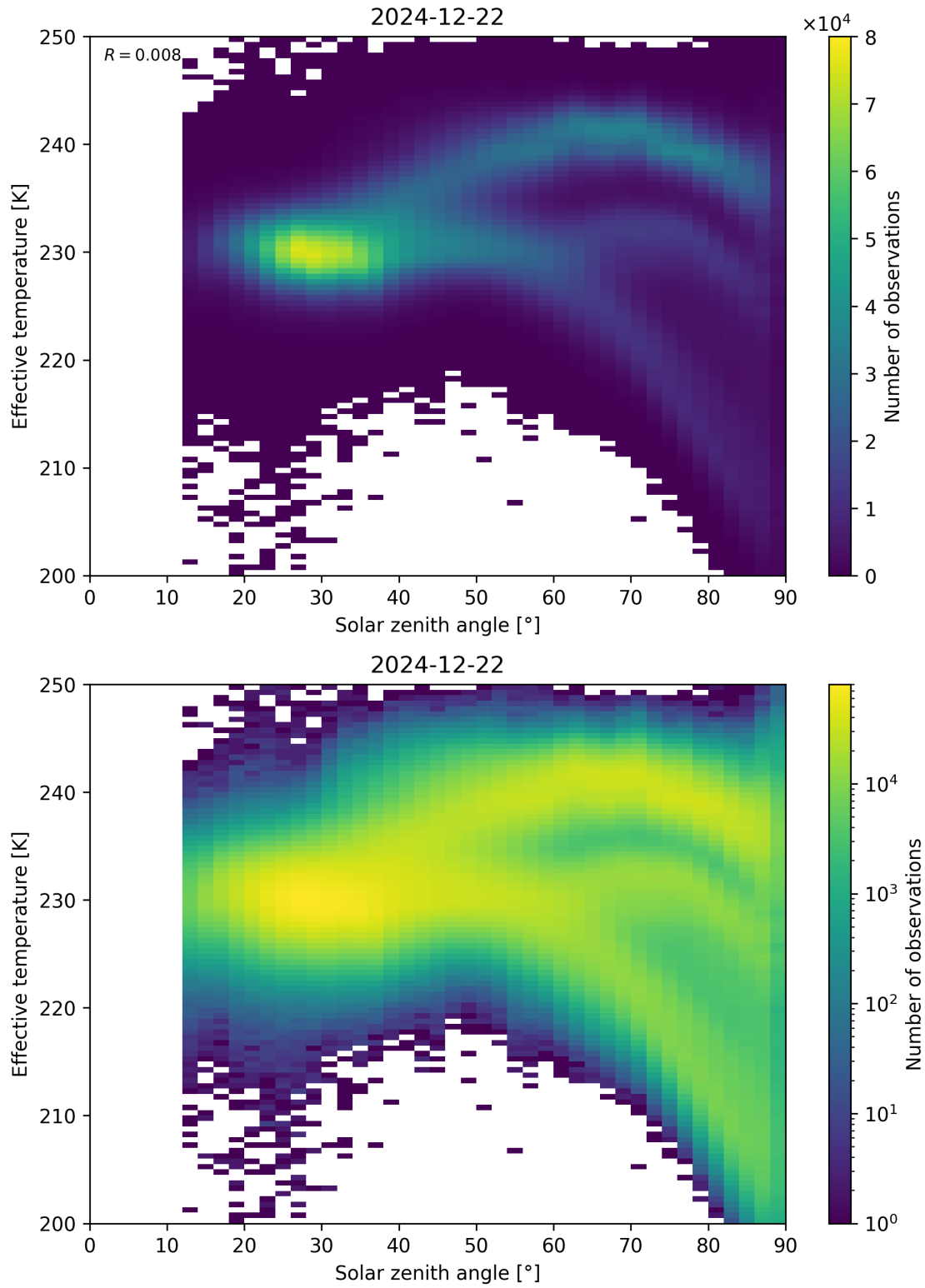
Figure 45: Scatter density plot of “Solar zenith angle” against “Effective temperature” for 2024-12-22 to 2024-12-23.
