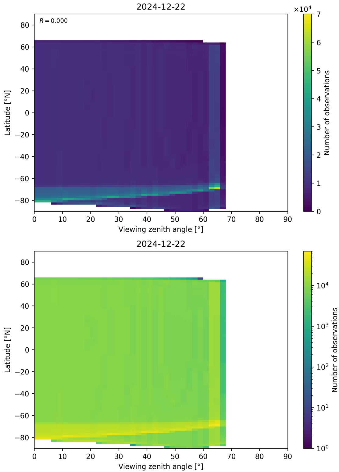
Figure 49: Scatter density plot of “Viewing zenith angle” against “Latitude” for 2024-12-22 to 2024-12-23.
