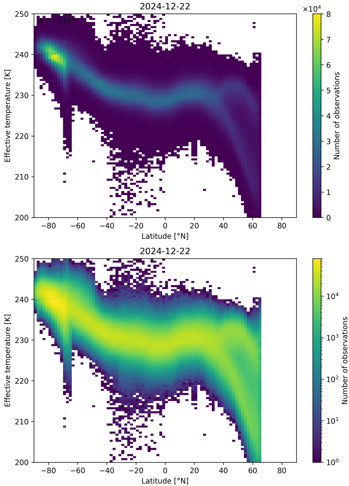
Figure 34: Scatter density plot of “Latitude” against “Effective temperature” for 2024-12-22 to 2024-12-23.
