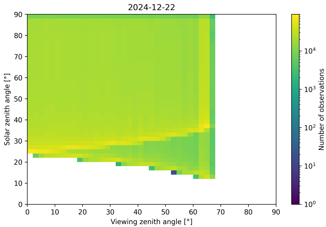
Figure 54: Scatter density plot of “Viewing zenith angle” against “Solar zenith angle” for 2024-12-22 to 2024-12-23.
