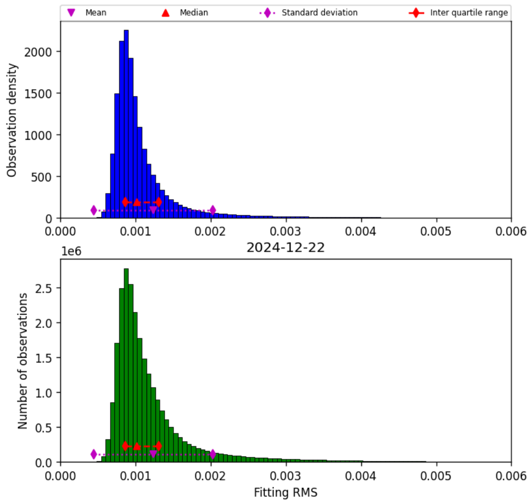
Figure 23: Histogram of “Fitting RMS” for 2024-12-22 to 2024-12-23
