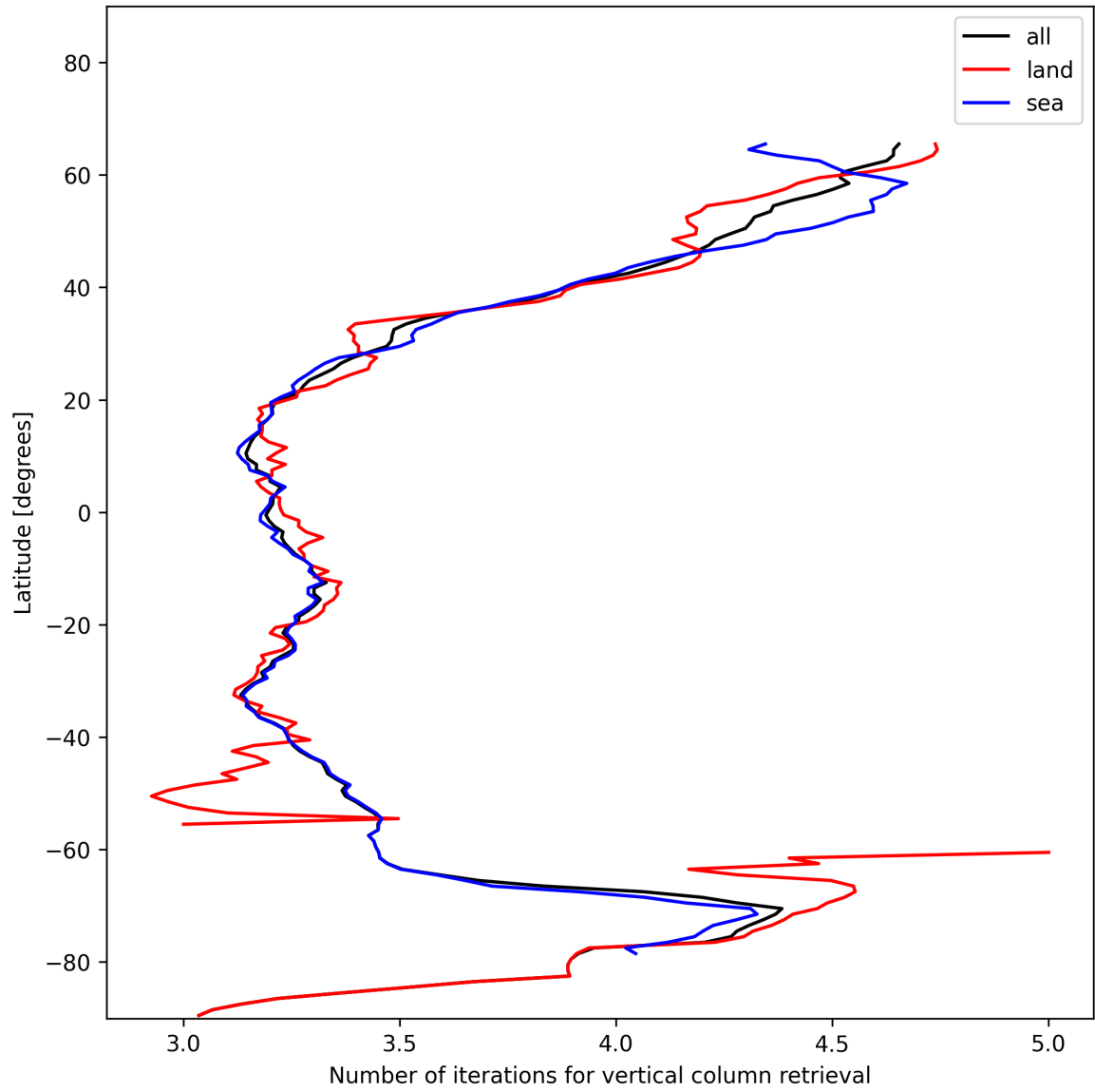
Figure 19: Zonal average of “Number of iterations for vertical column retrieval” for 2024-12-22 to 2024-12-23.
