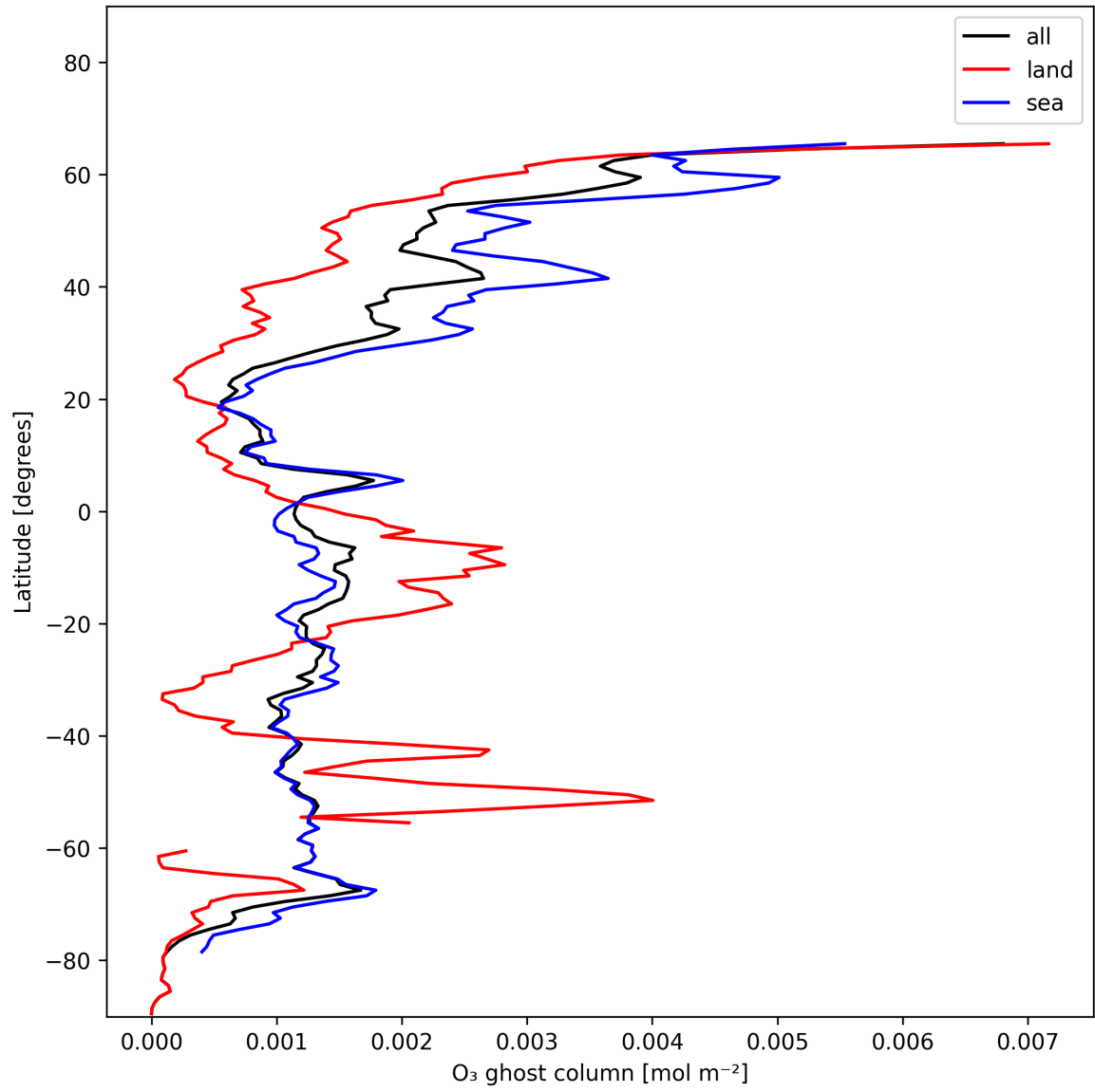
Figure 18: Zonal average of “O 3 ghost column” for 2024-12-22 to 2024-12-23.
