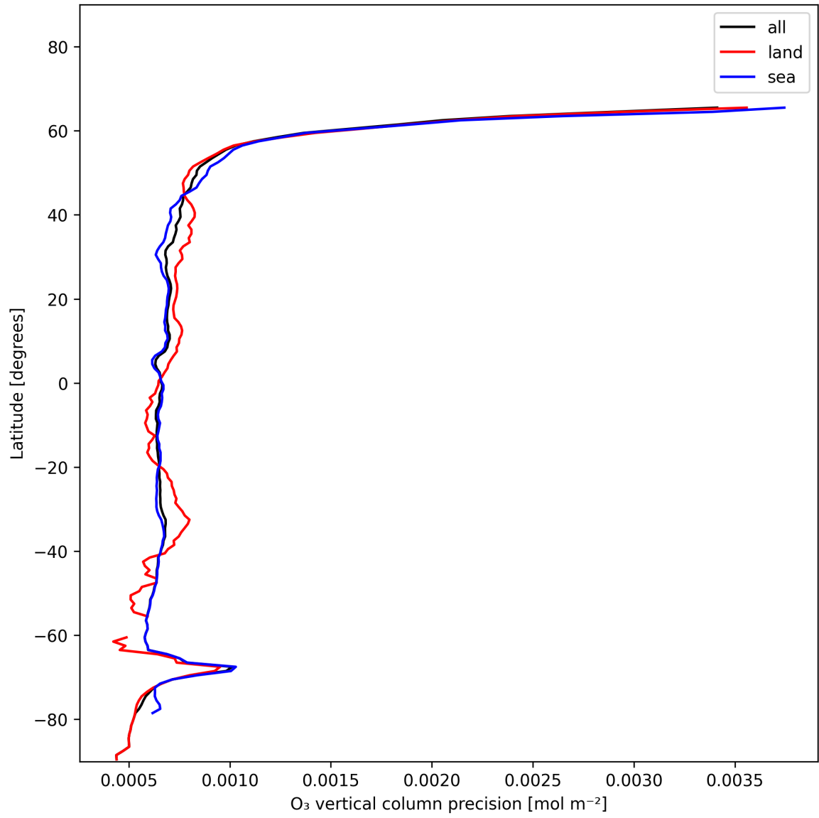
Figure 15: Zonal average of “O 3 vertical column precision” for 2024-12-22 to 2024-12-23.
