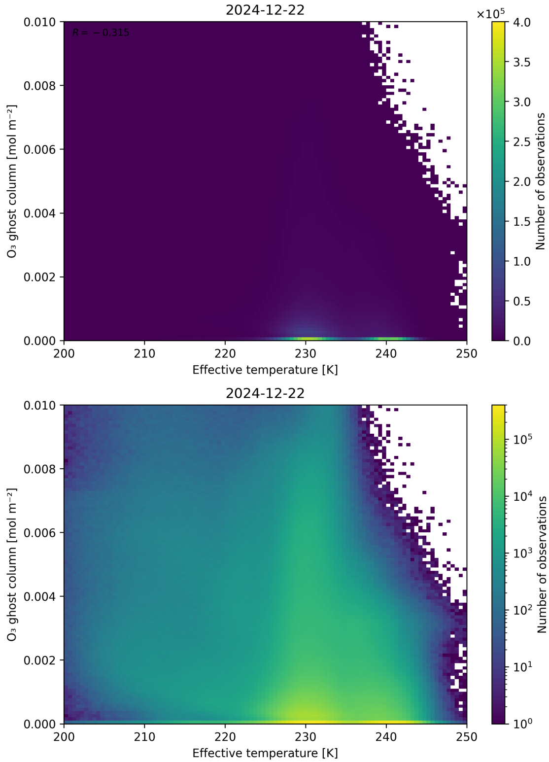
Figure 38: Scatter density plot of “Effective temperature” against “O 3 ghost column” for 2024-12-22 to 2024-12-23.
