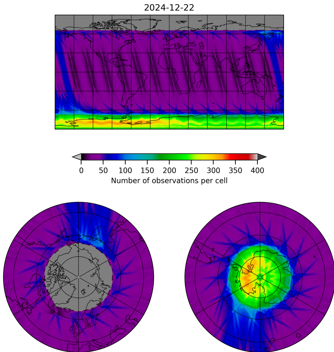
Figure 12: Map of the number of observations for 2024-12-22 to 2024-12-23
