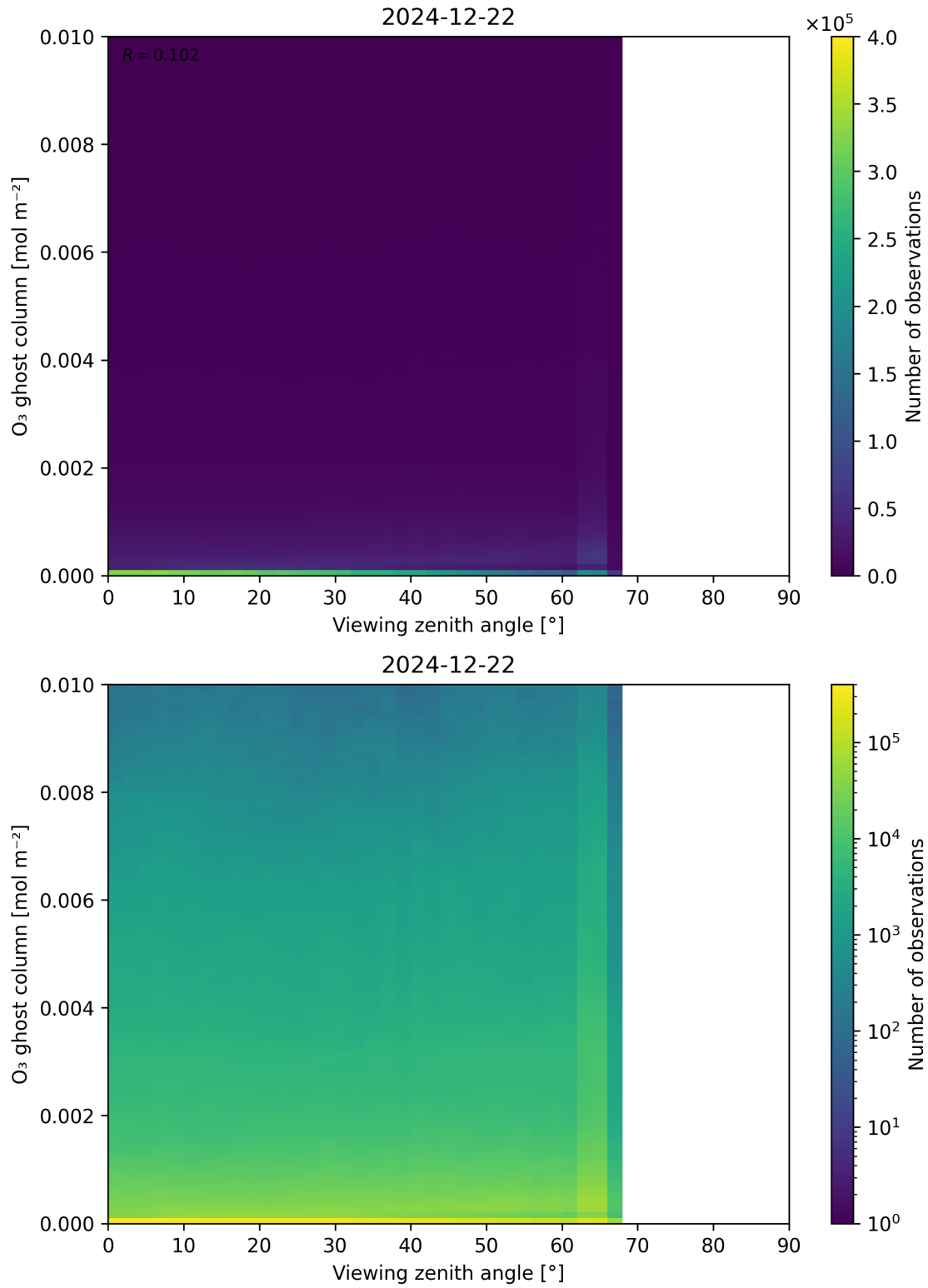
Figure 51: Scatter density plot of “Viewing zenith angle” against “O 3 ghost column” for 2024-12-22 to 2024-12-23.
