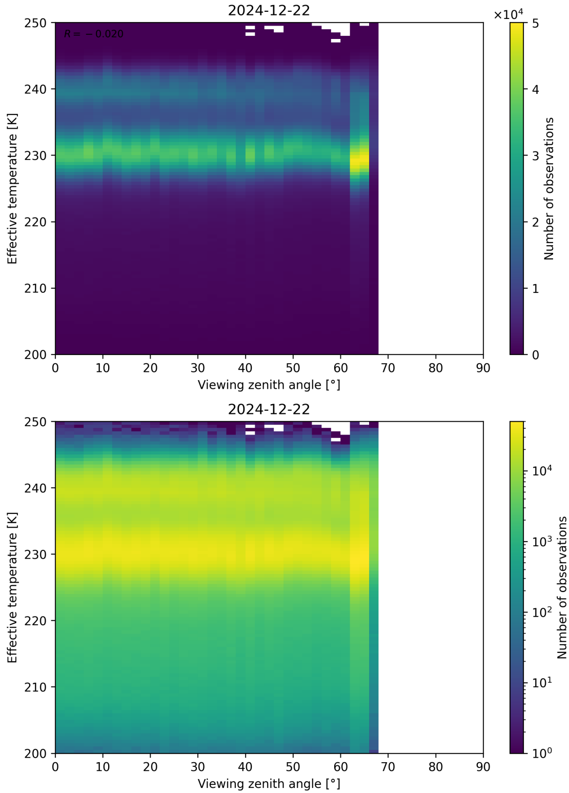
Figure 50: Scatter density plot of “Viewing zenith angle” against “Effective temperature” for 2024-12-22 to 2024-12-23.
