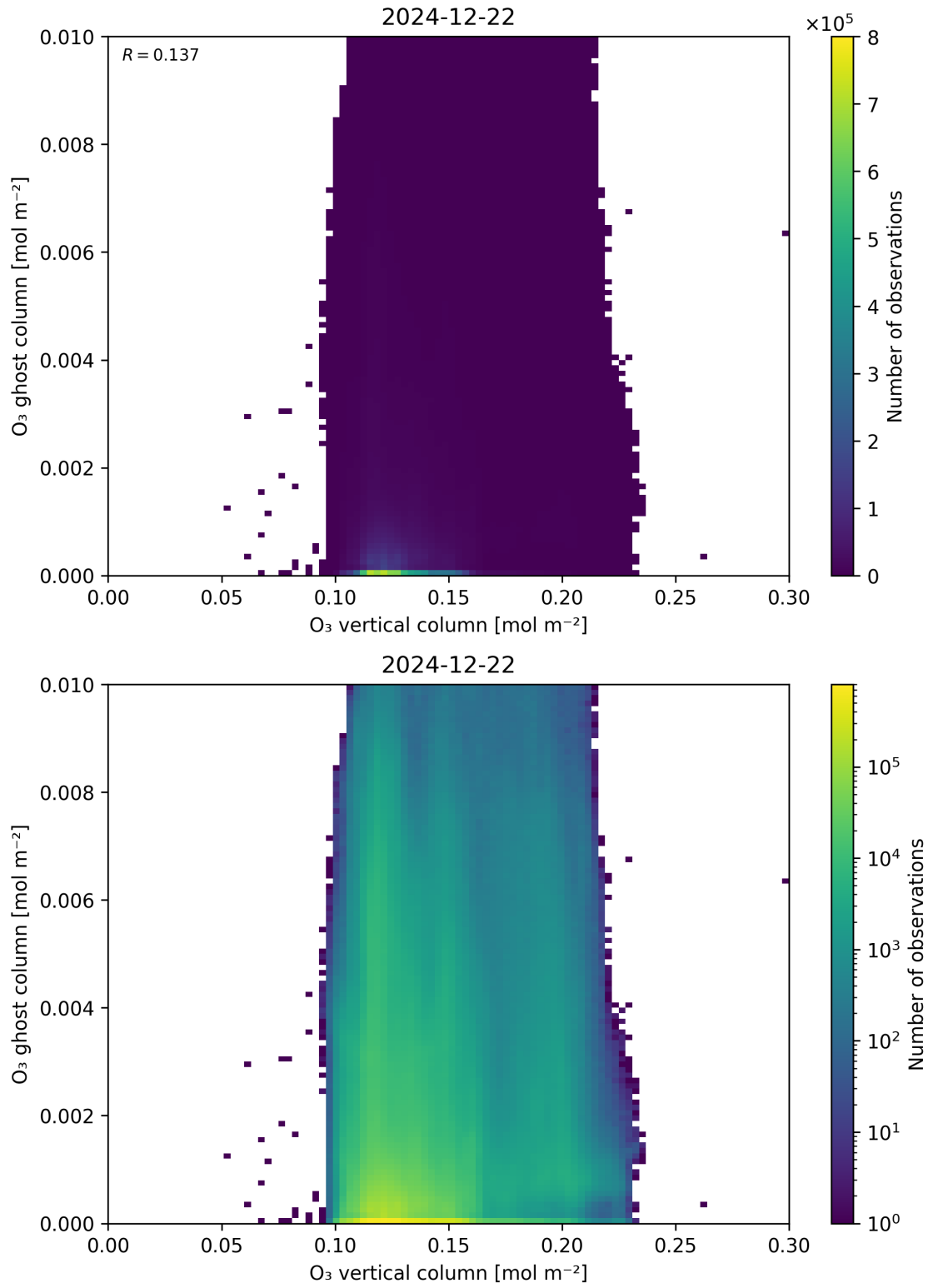
Figure 40: Scatter density plot of “O 3 vertical column” against “O 3 ghost column” for 2024-12-22 to 2024-12-23.
