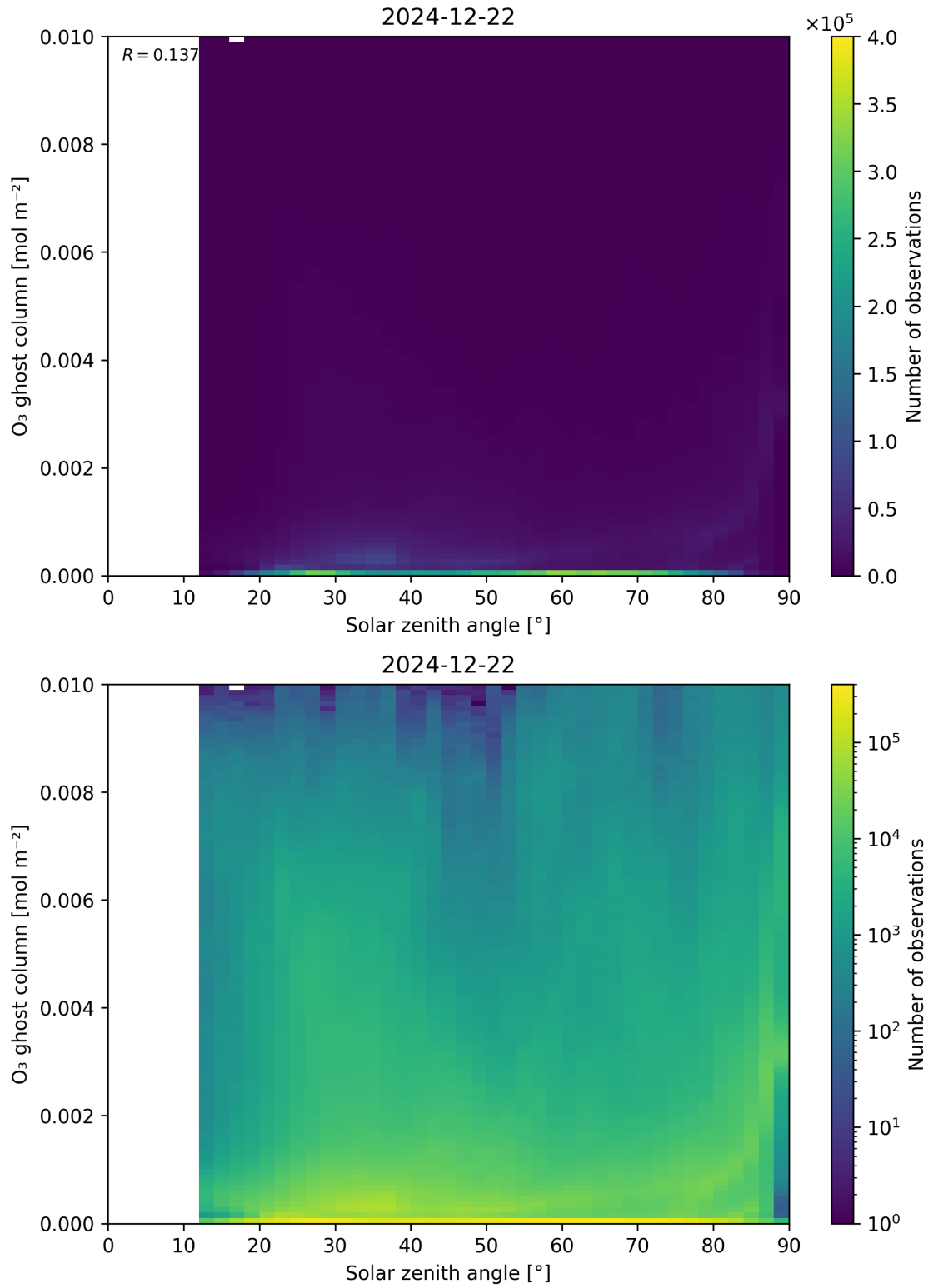
Figure 46: Scatter density plot of “Solar zenith angle” against “O 3 ghost column” for 2024-12-22 to 2024-12-23.
