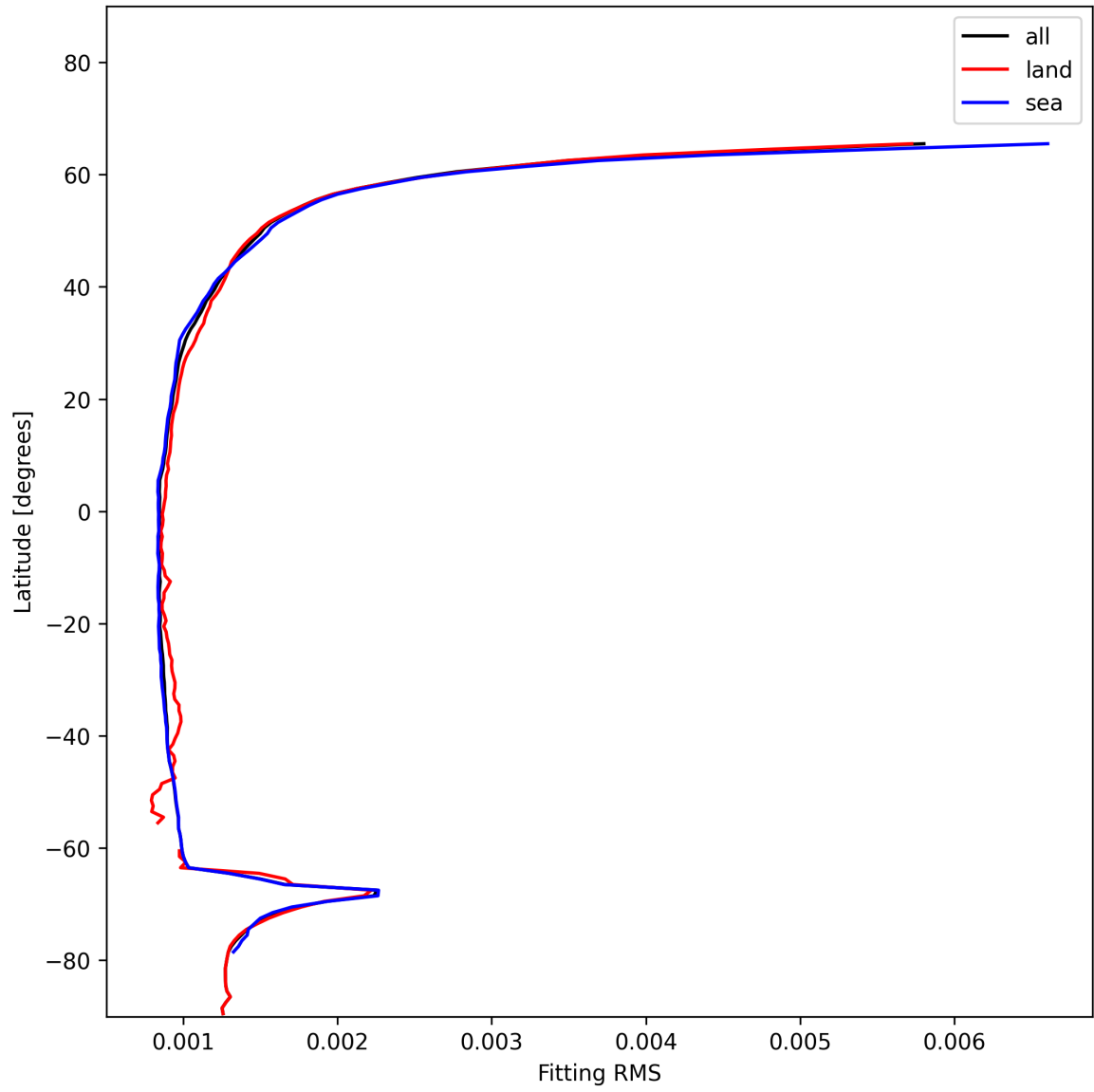
Figure 16: Zonal average of “Fitting RMS” for 2024-12-22 to 2024-12-23.
