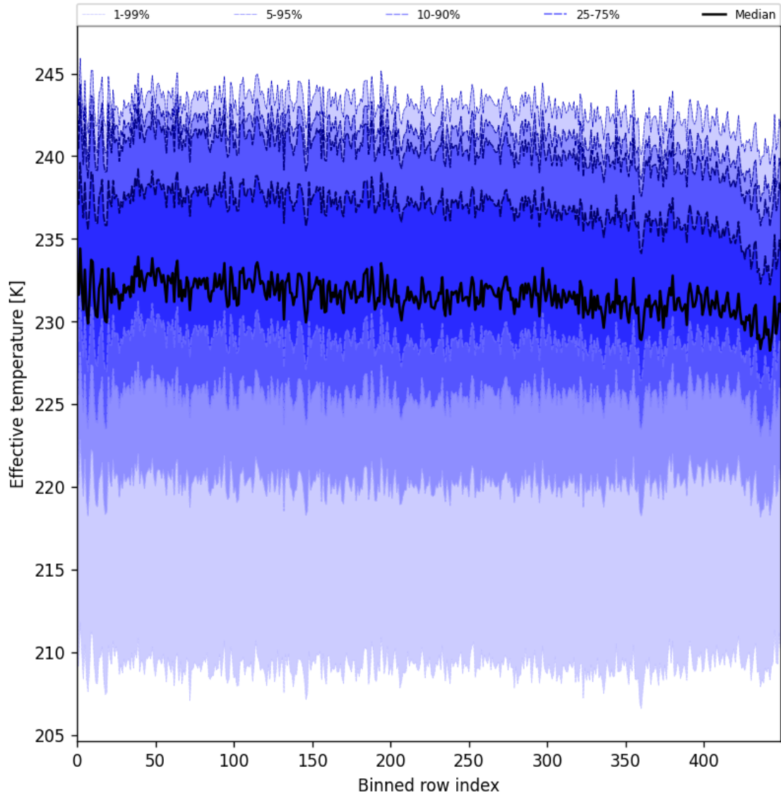
Figure 31: Along track statistics of “Effective temperature” for 2024-12-22 to 2024-12-23
