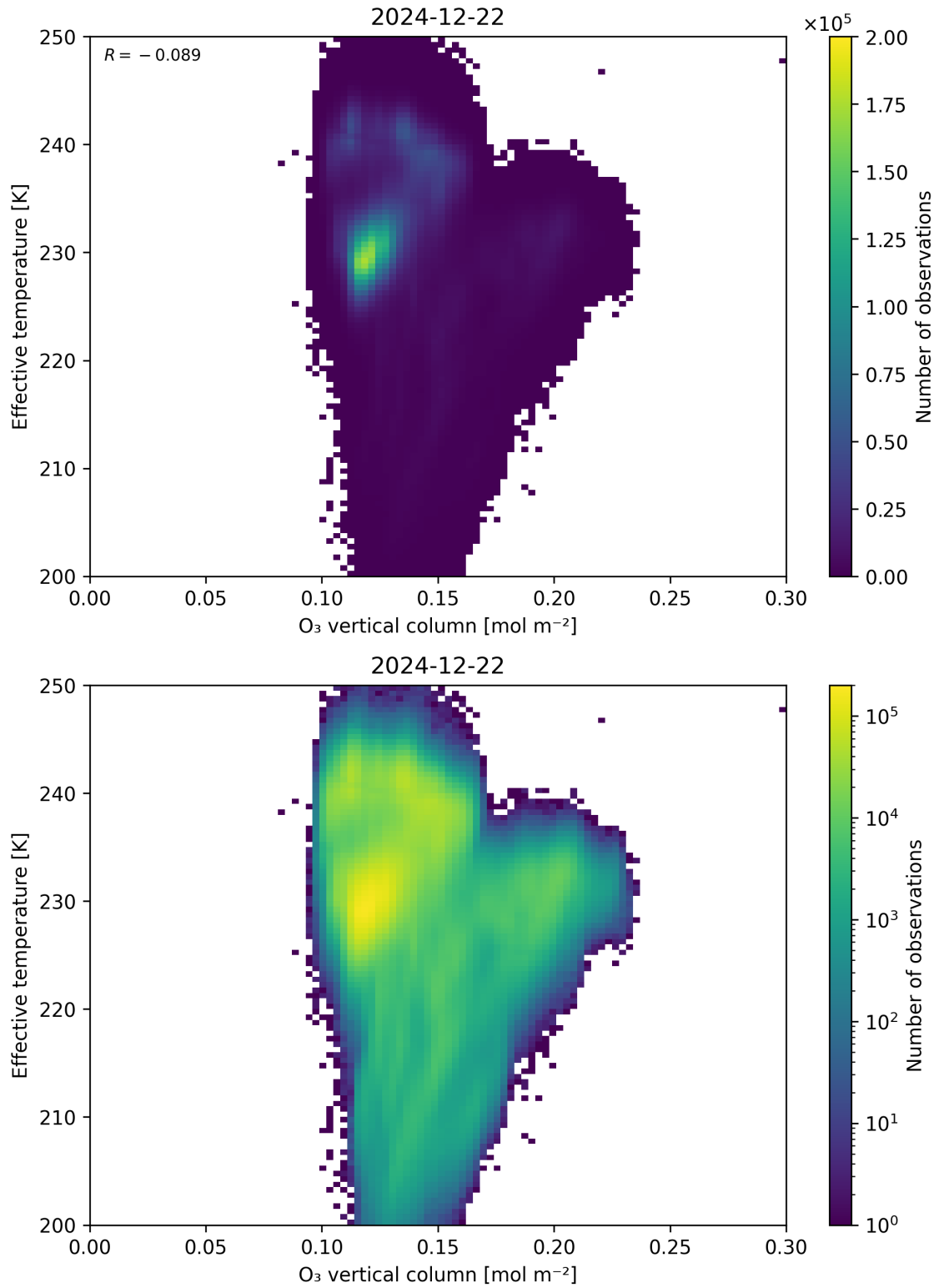
Figure 39: Scatter density plot of “O 3 vertical column” against “Effective temperature” for 2024-12-22 to 2024-12-23.
