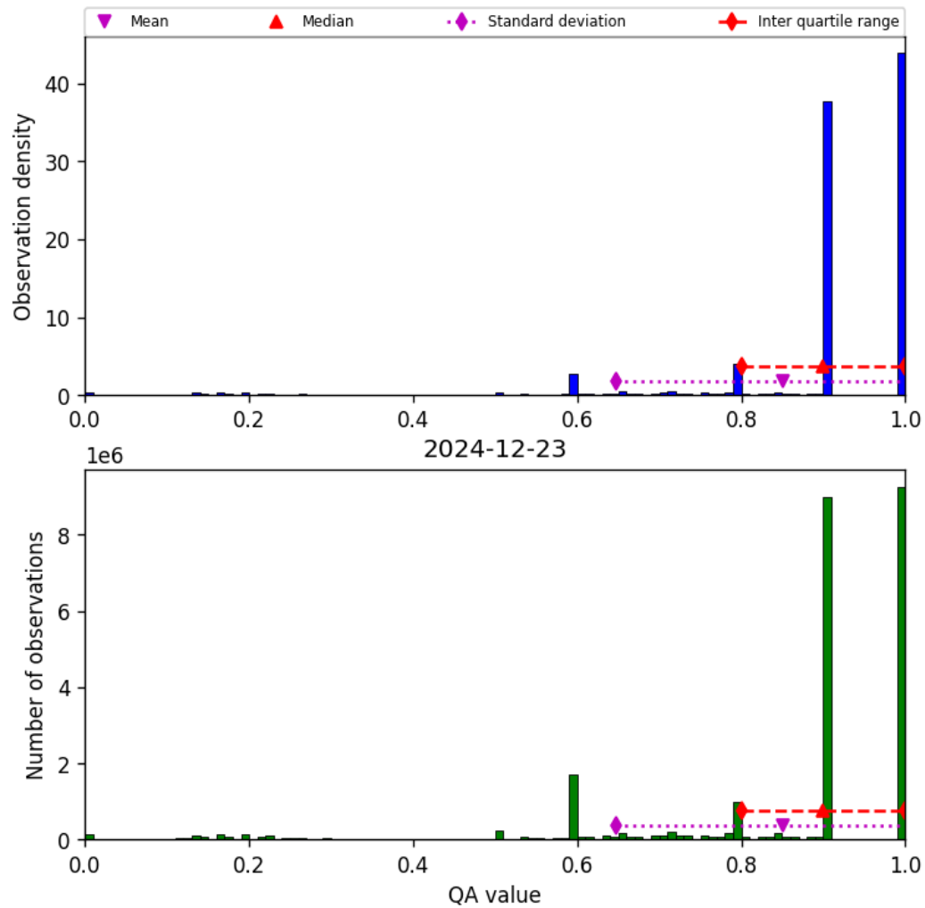
Figure 20: Histogram of “QA value” for 2024-12-22 to 2024-12-24
