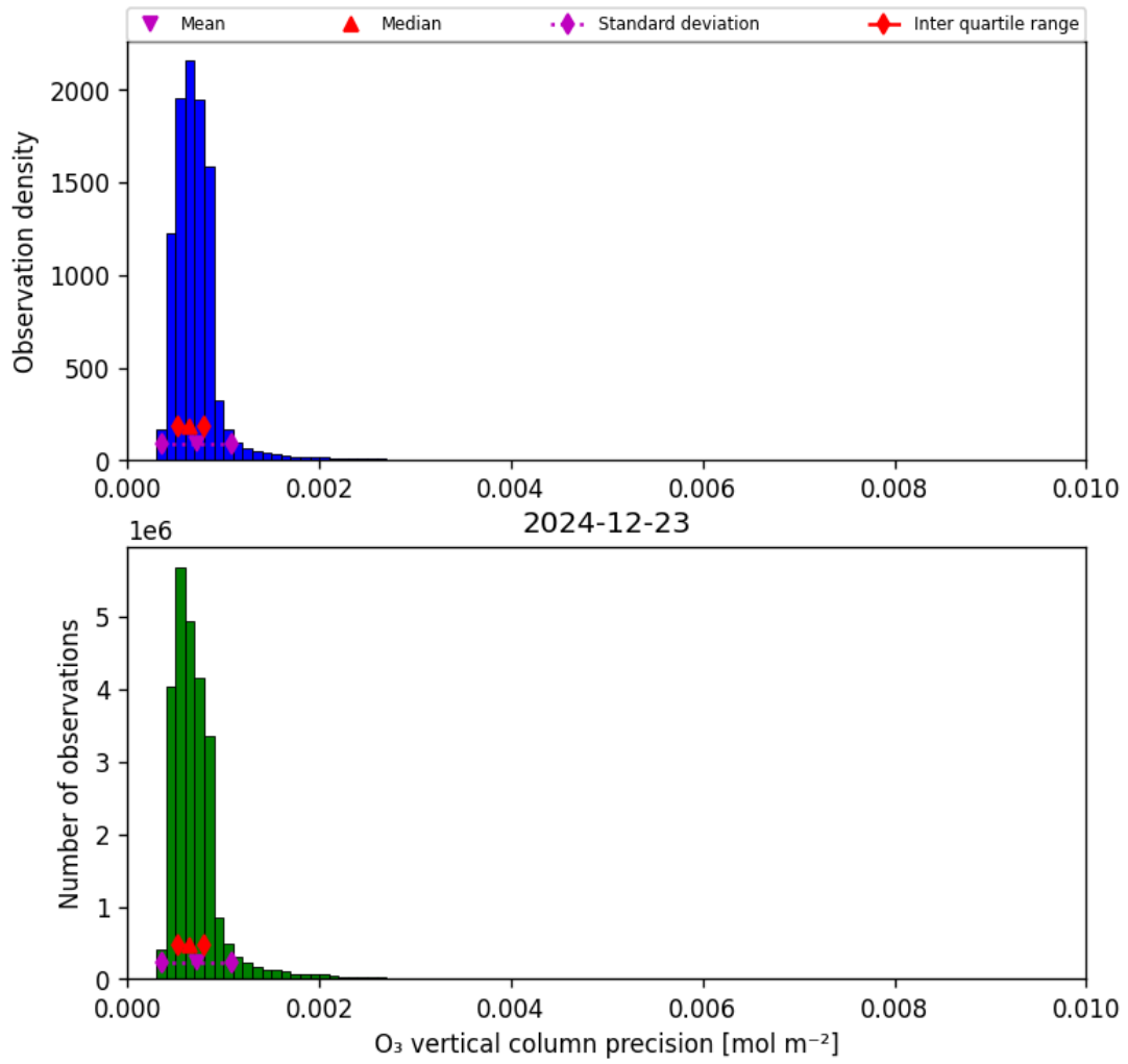
Figure 22: Histogram of “O 3 vertical column precision” for 2024-12-22 to 2024-12-24
