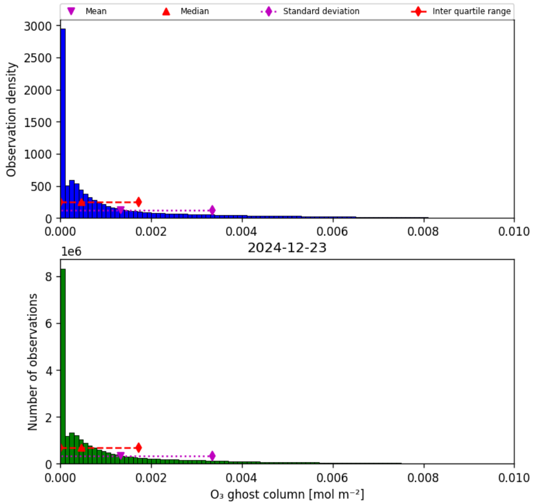
Figure 25: Histogram of “O 3 ghost column” for 2024-12-22 to 2024-12-24
