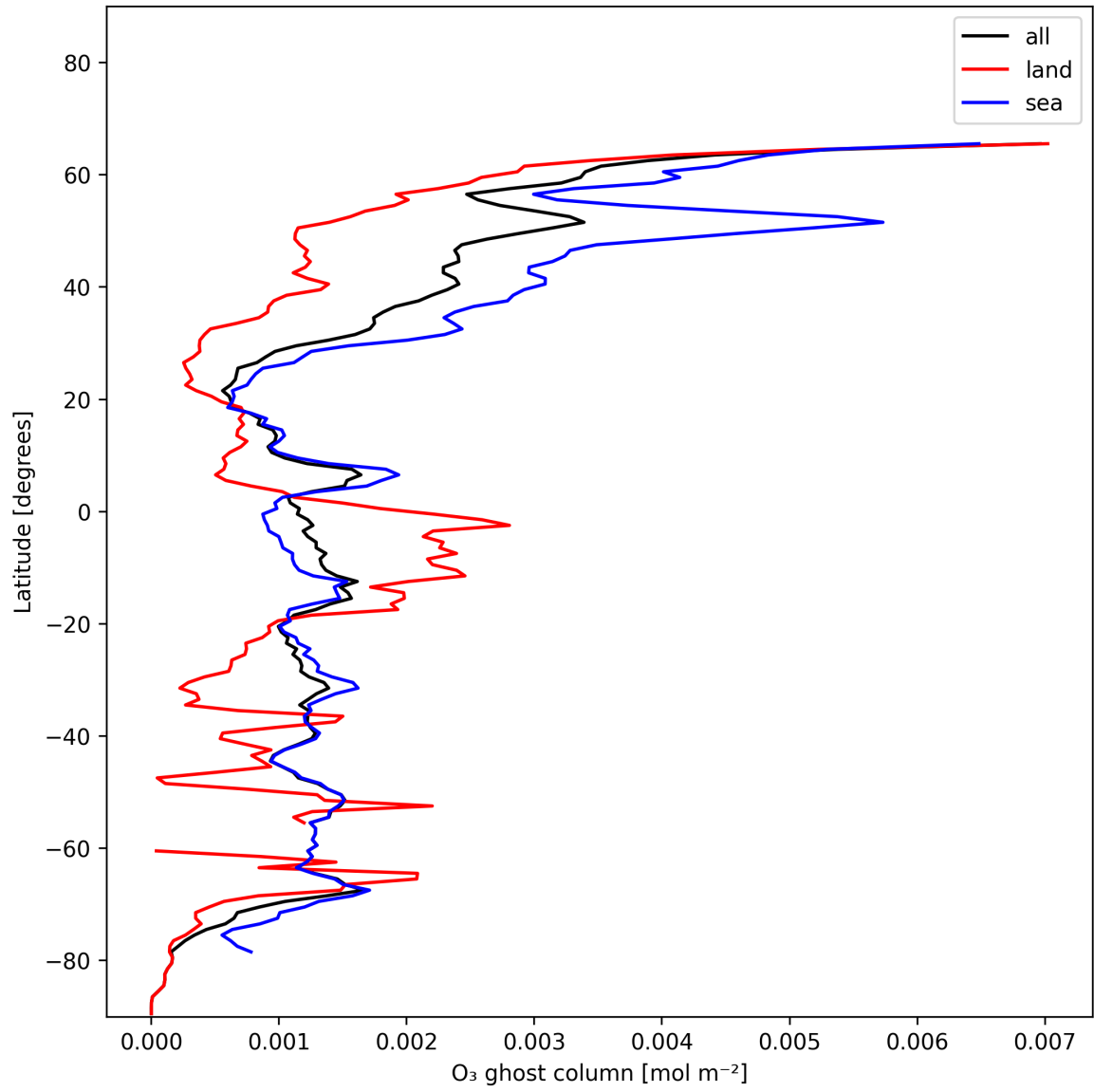
Figure 18: Zonal average of “O 3 ghost column” for 2024-12-22 to 2024-12-24.
