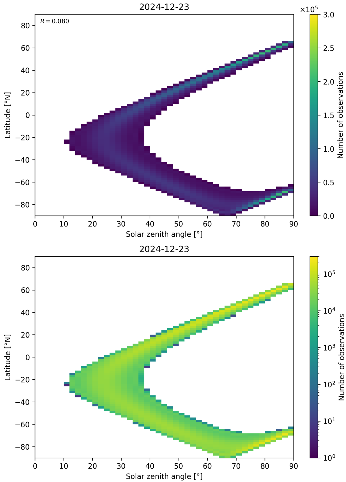
Figure 44: Scatter density plot of “Solar zenith angle” against “Latitude” for 2024-12-22 to 2024-12-24.
