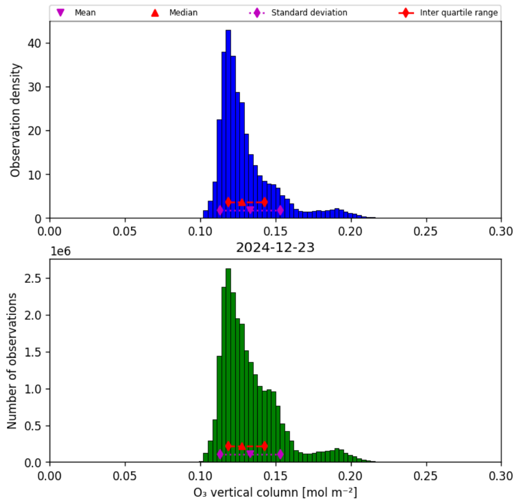
Figure 21: Histogram of “O 3 vertical column” for 2024-12-22 to 2024-12-24
