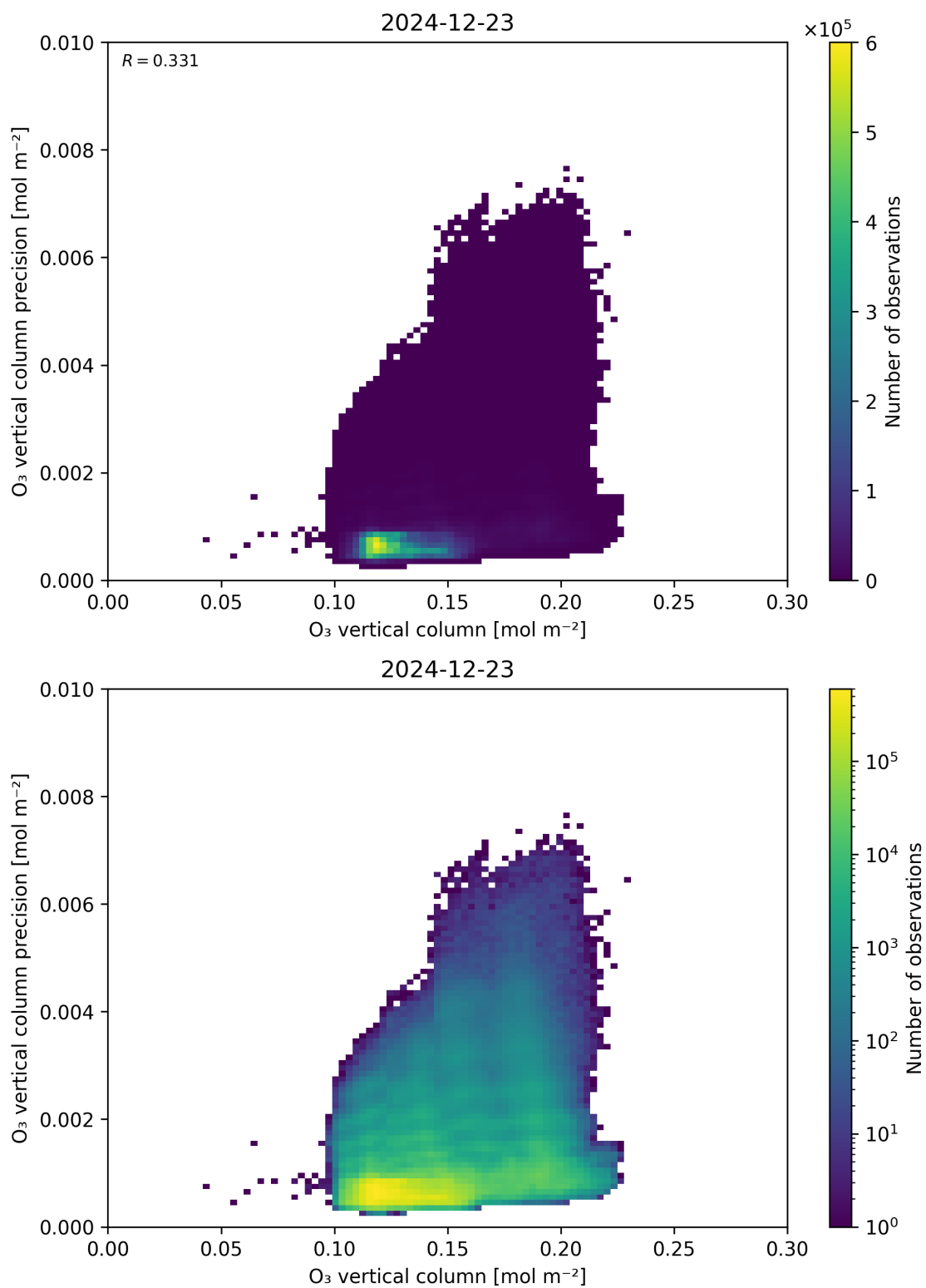
Figure 41: Scatter density plot of “O 3 vertical column” against “O 3 vertical column precision” for 2024-12-22 to 2024-12-24.
