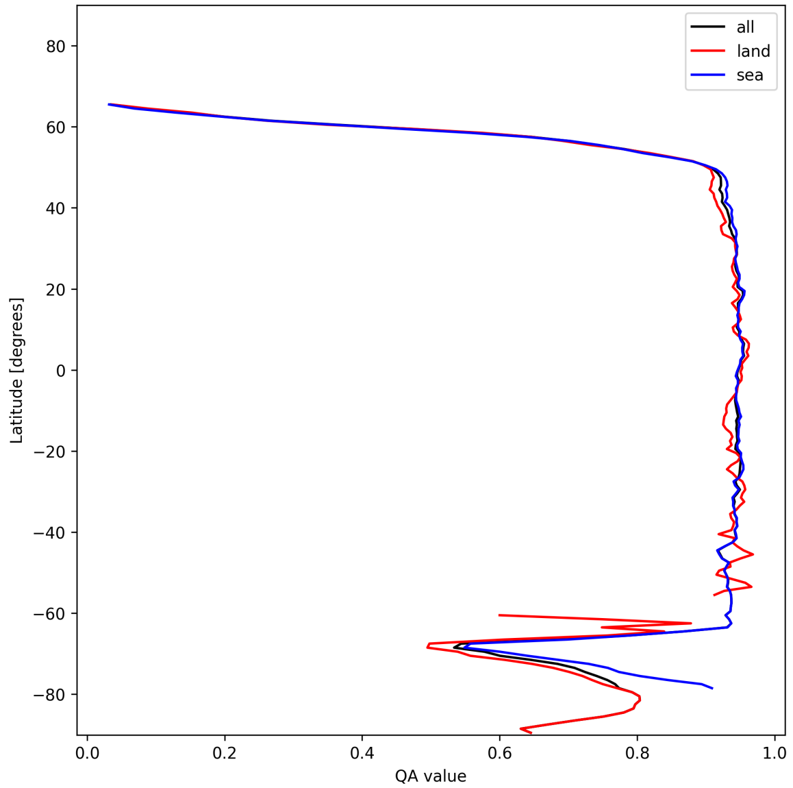
Figure 13: Zonal average of “QA value” for 2024-12-22 to 2024-12-24.
