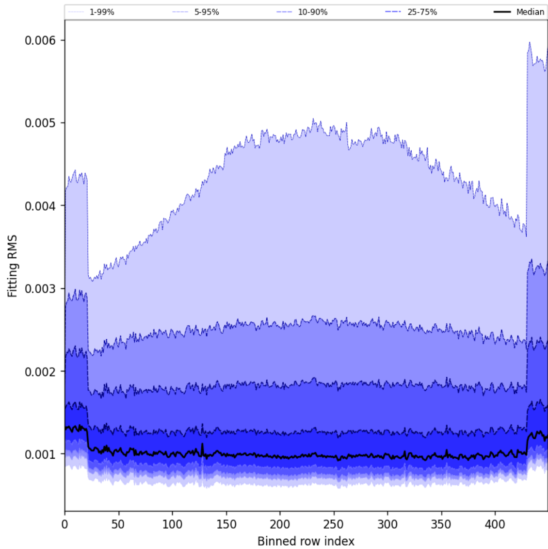
Figure 30: Along track statistics of “Fitting RMS” for 2024-12-22 to 2024-12-24
