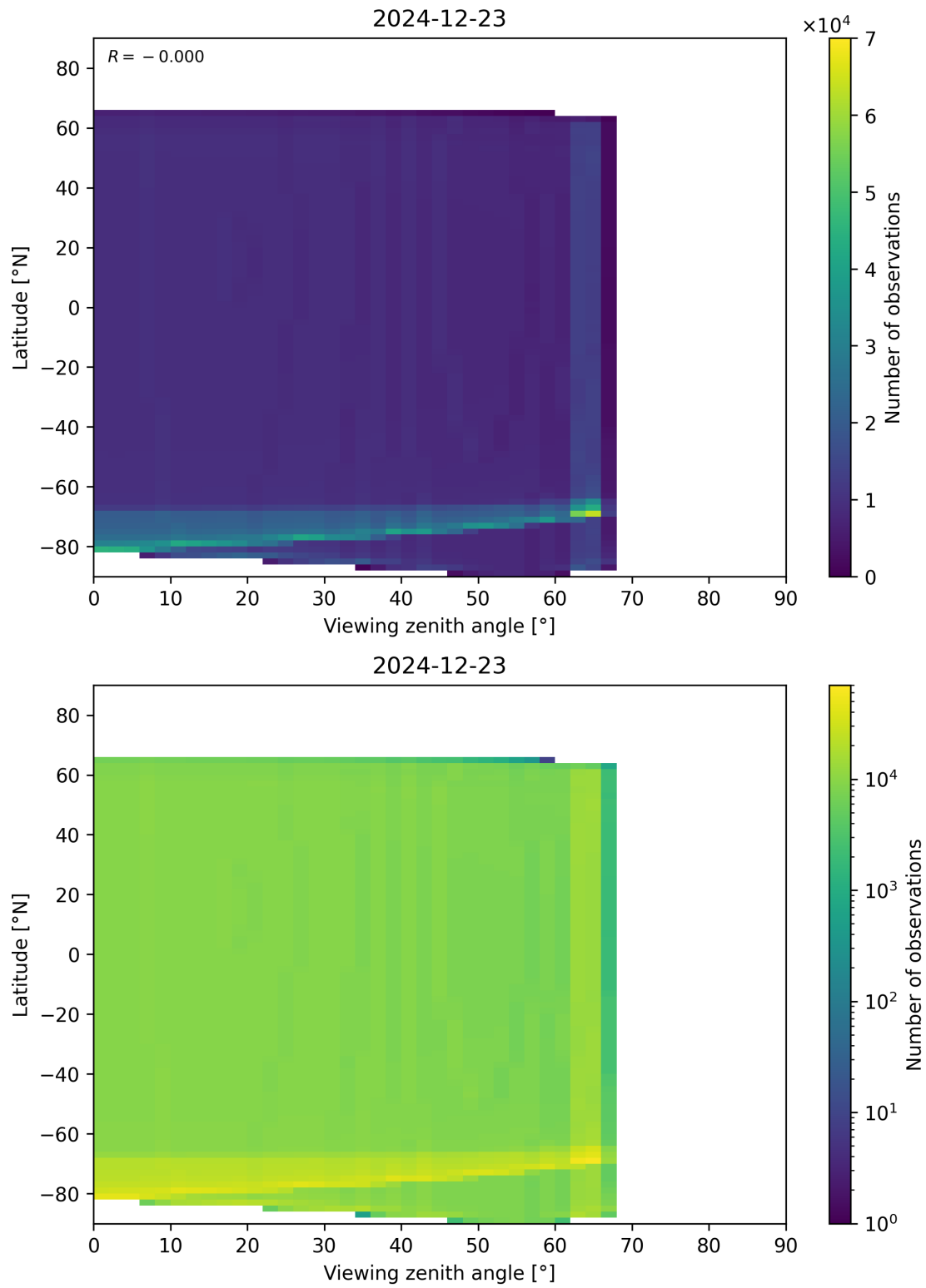
Figure 49: Scatter density plot of “Viewing zenith angle” against “Latitude” for 2024-12-22 to 2024-12-24.
