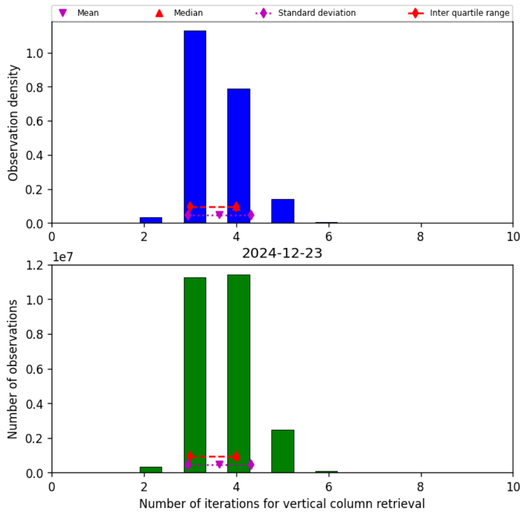
Figure 26: Histogram of “Number of iterations for vertical column retrieval” for 2024-12-22 to 2024-12-24
