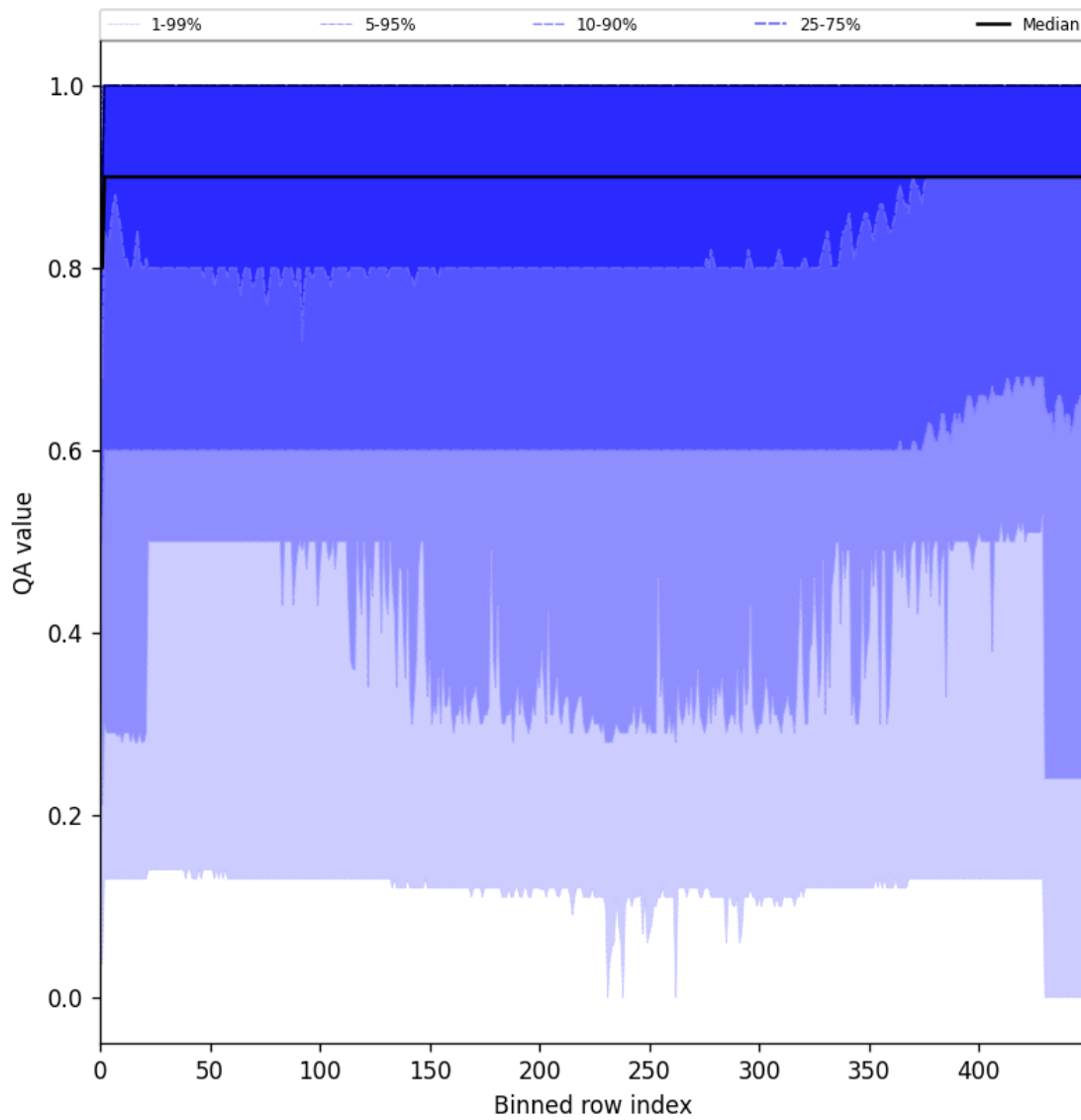
Figure 27: Along track statistics of “QA value” for 2024-12-22 to 2024-12-24
