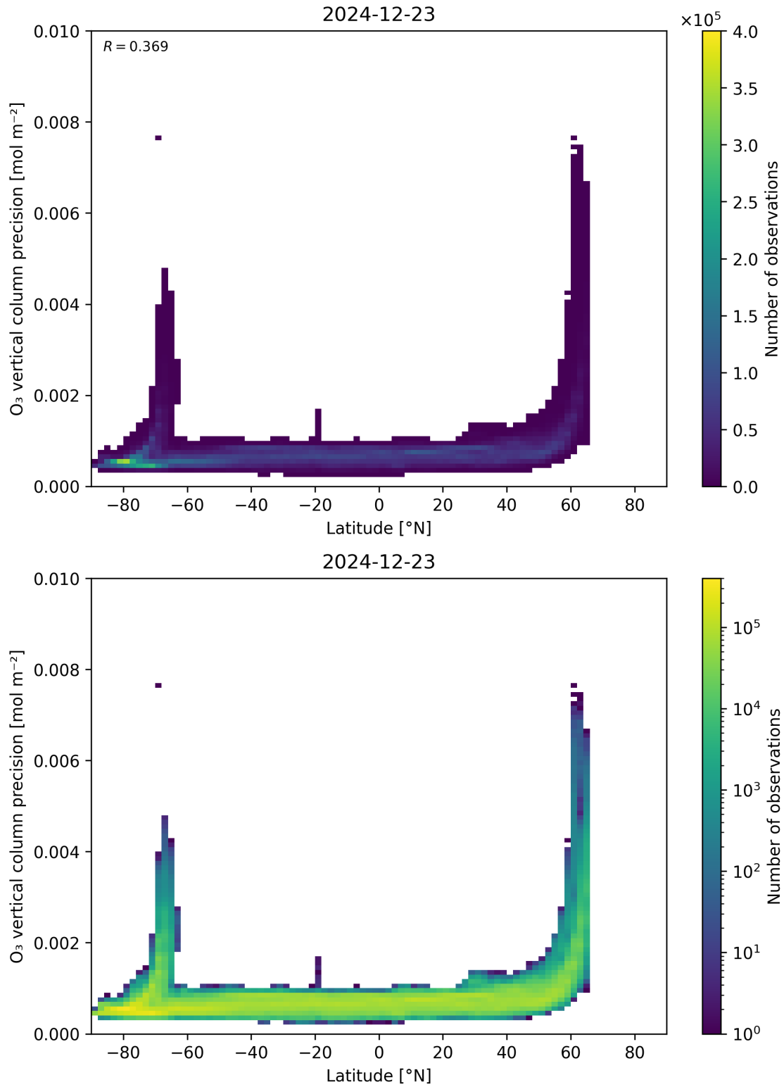
Figure 37: Scatter density plot of “Latitude” against “O 3 vertical column precision” for 2024-12-22 to 2024-12-24.
