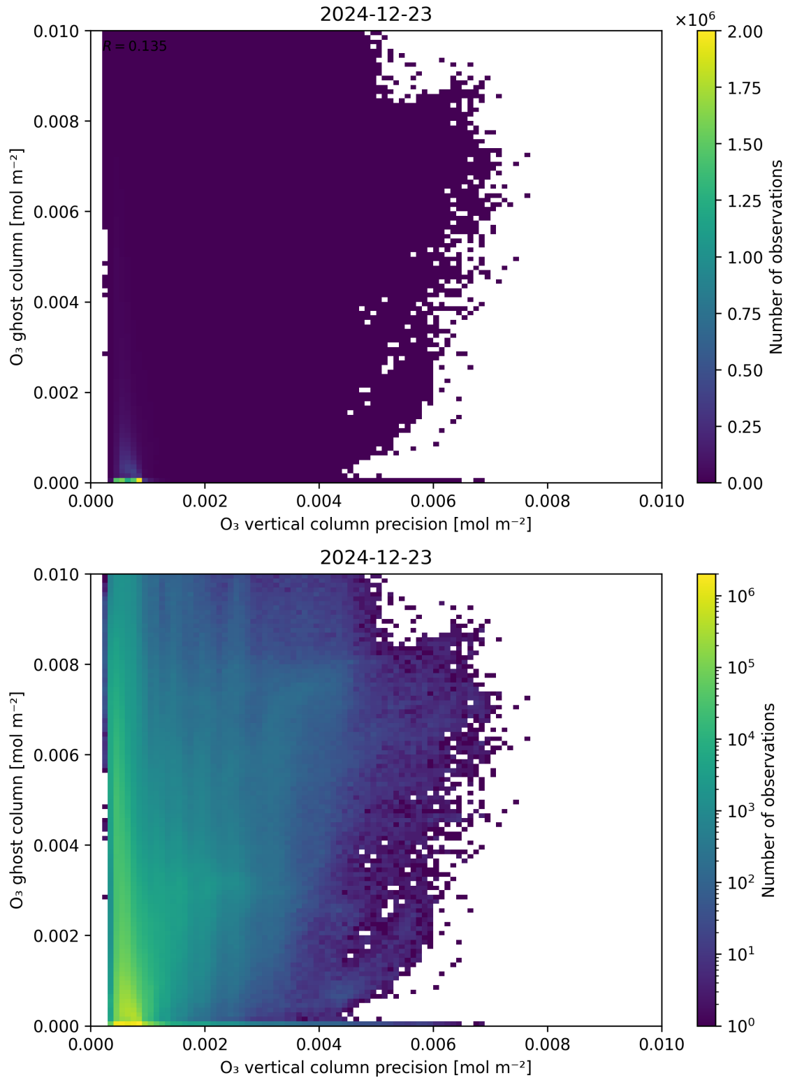
Figure 43: Scatter density plot of “O 3 vertical column precision” against “O 3 ghost column” for 2024-12-22 to 2024-12-24.
