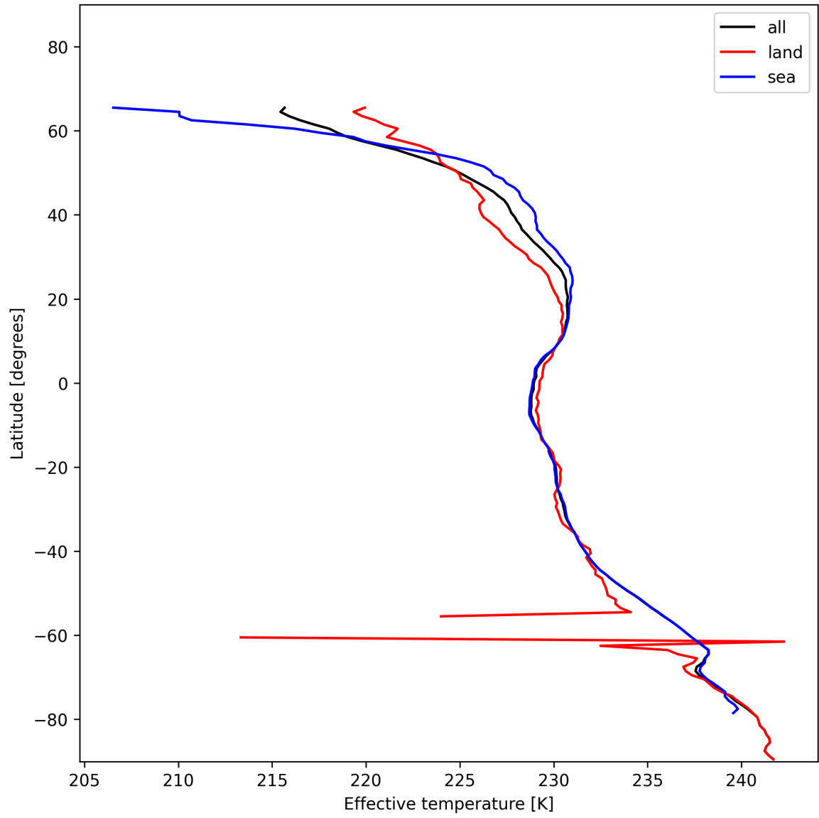
Figure 17: Zonal average of “Effective temperature” for 2024-12-22 to 2024-12-24.
