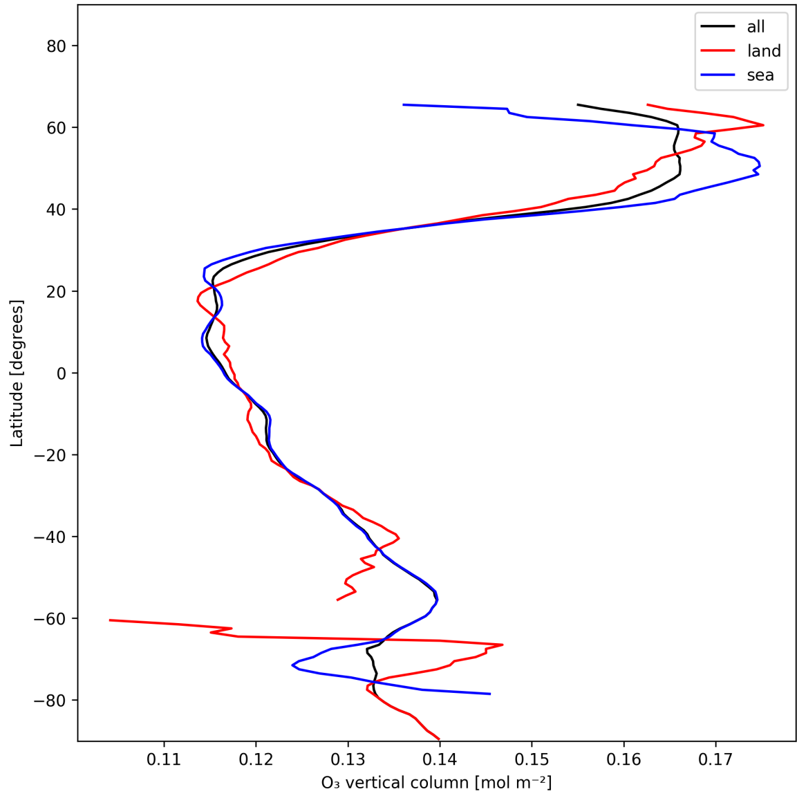
Figure 14: Zonal average of “O 3 vertical column” for 2024-12-22 to 2024-12-24.
