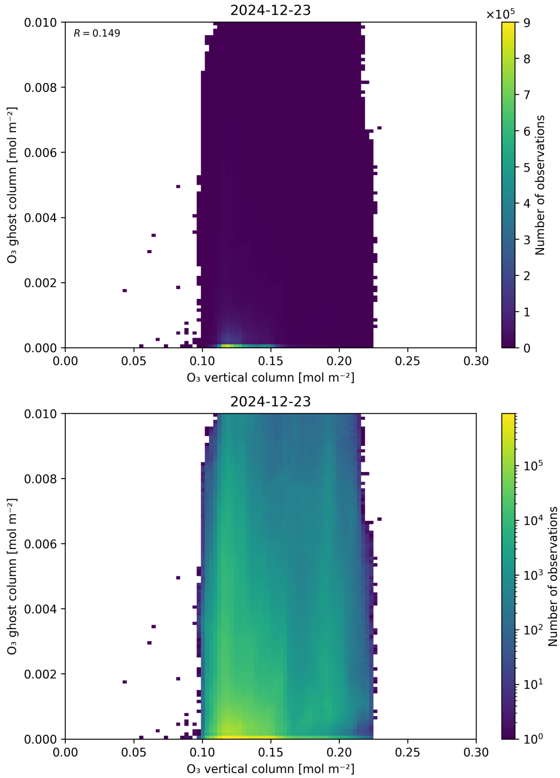
Figure 40: Scatter density plot of “O 3 vertical column” against “O 3 ghost column” for 2024-12-22 to 2024-12-24.
