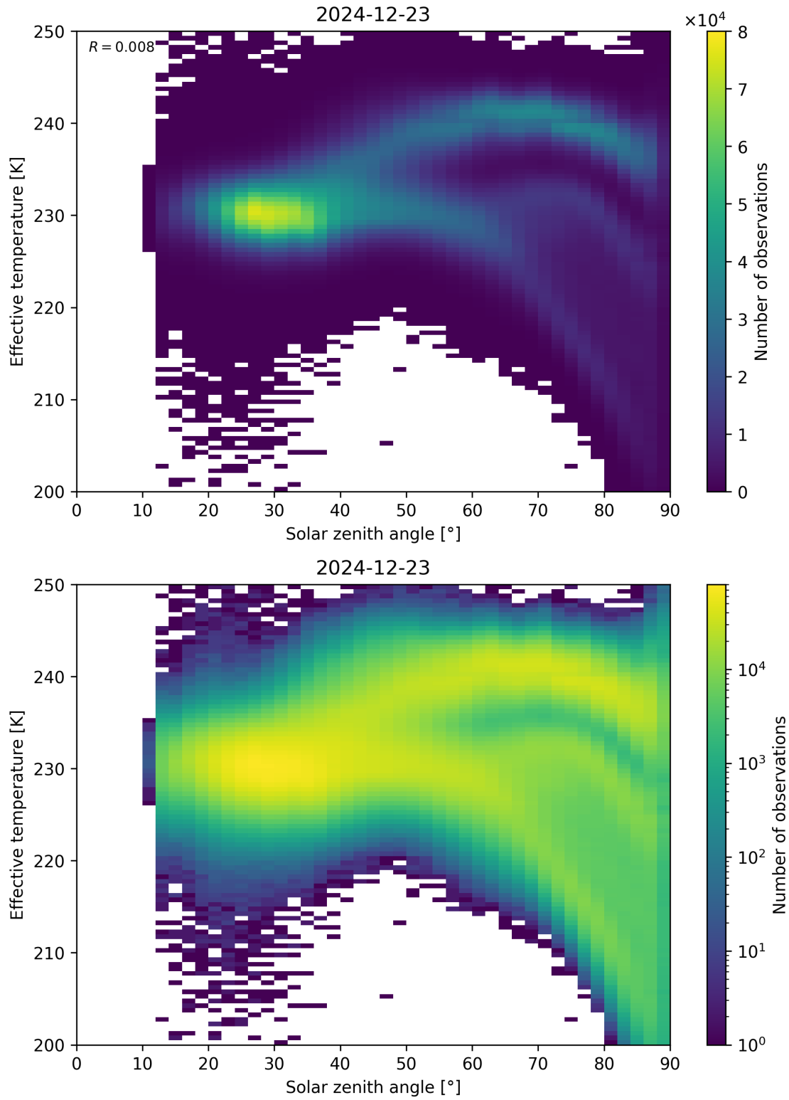
Figure 45: Scatter density plot of “Solar zenith angle” against “Effective temperature” for 2024-12-22 to 2024-12-24.
