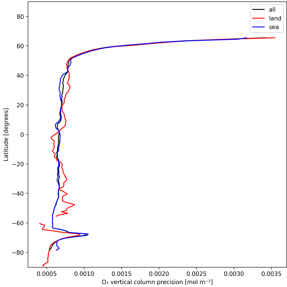
Figure 15: Zonal average of “O 3 vertical column precision” for 2024-12-22 to 2024-12-24.
