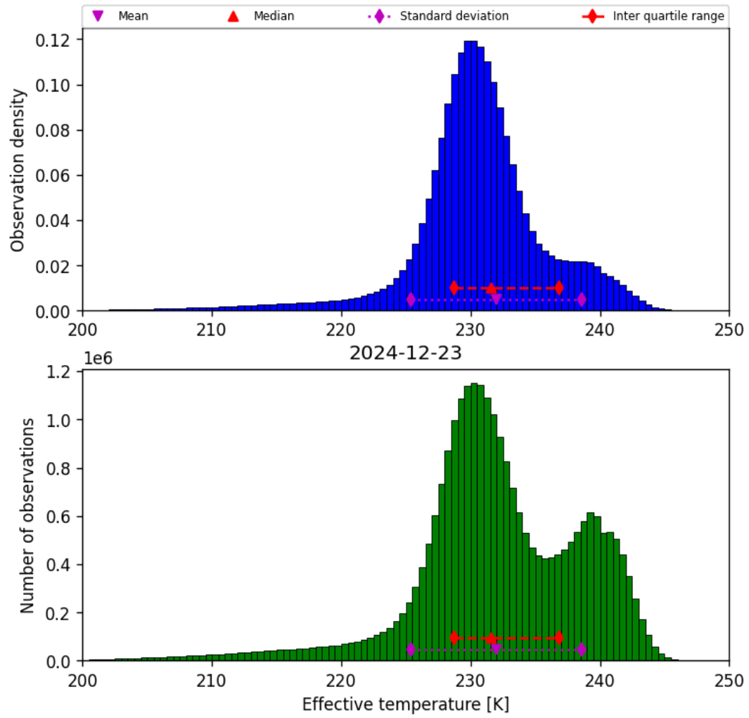
Figure 24: Histogram of “Effective temperature” for 2024-12-22 to 2024-12-24
