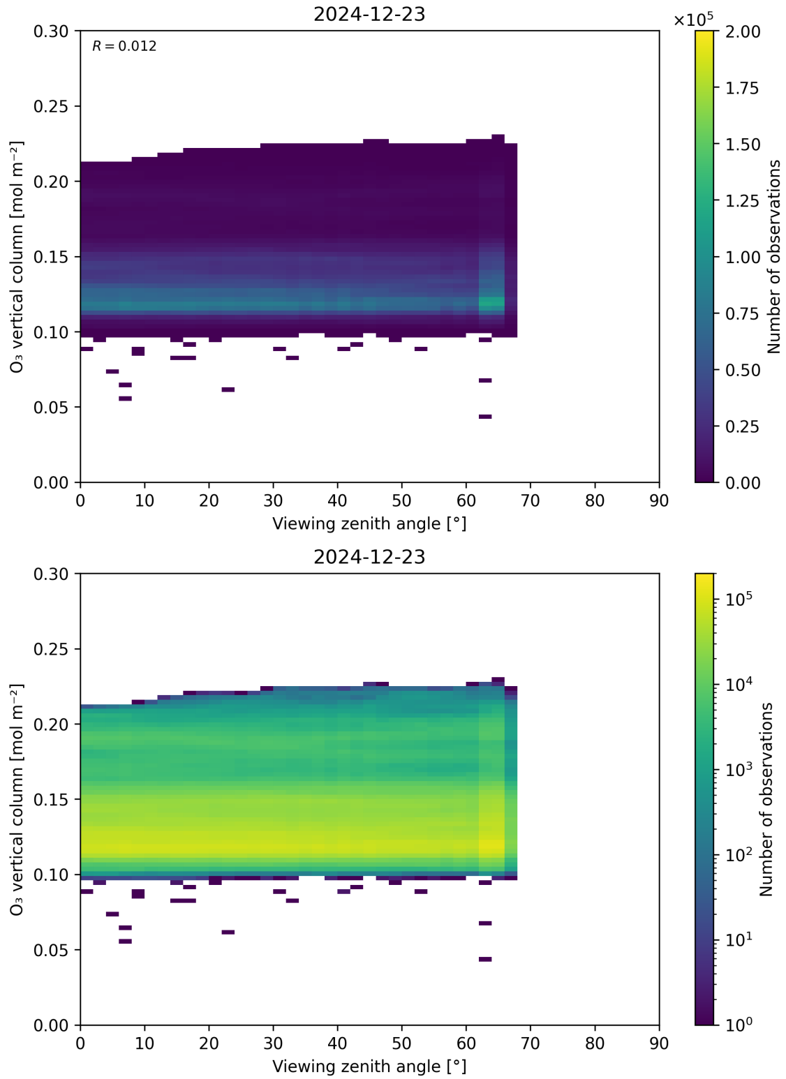
Figure 52: Scatter density plot of “Viewing zenith angle” against “O 3 vertical column” for 2024-12-22 to 2024-12-24.
