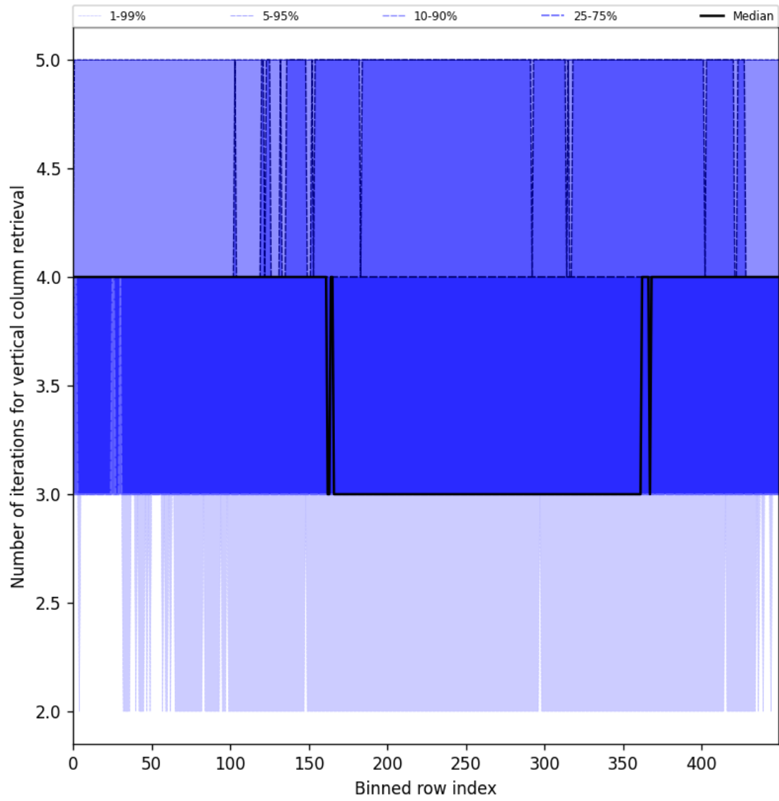
Figure 33: Along track statistics of “Number of iterations for vertical column retrieval” for 2024-12-22 to 2024-12-24
