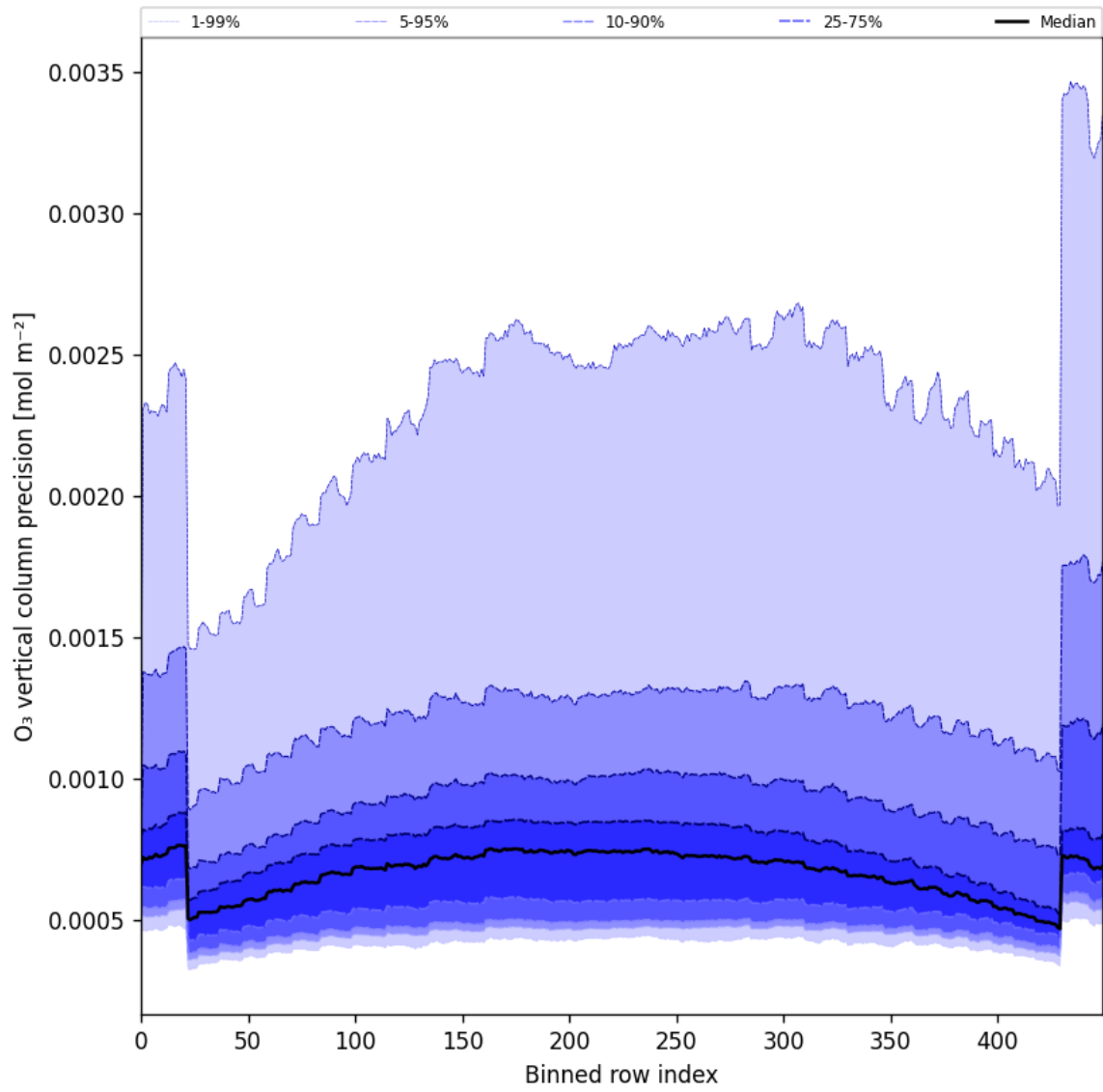
Figure 29: Along track statistics of “O 3 vertical column precision” for 2024-12-22 to 2024-12-24
