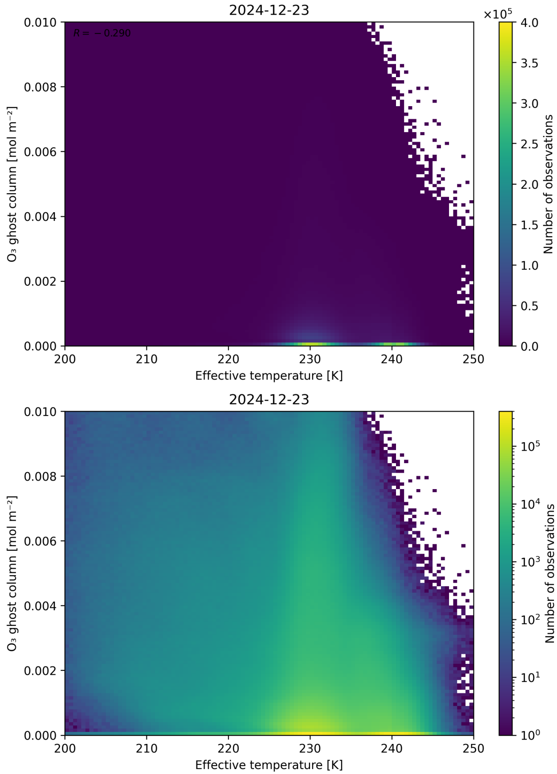
Figure 38: Scatter density plot of “Effective temperature” against “O 3 ghost column” for 2024-12-22 to 2024-12-24.
