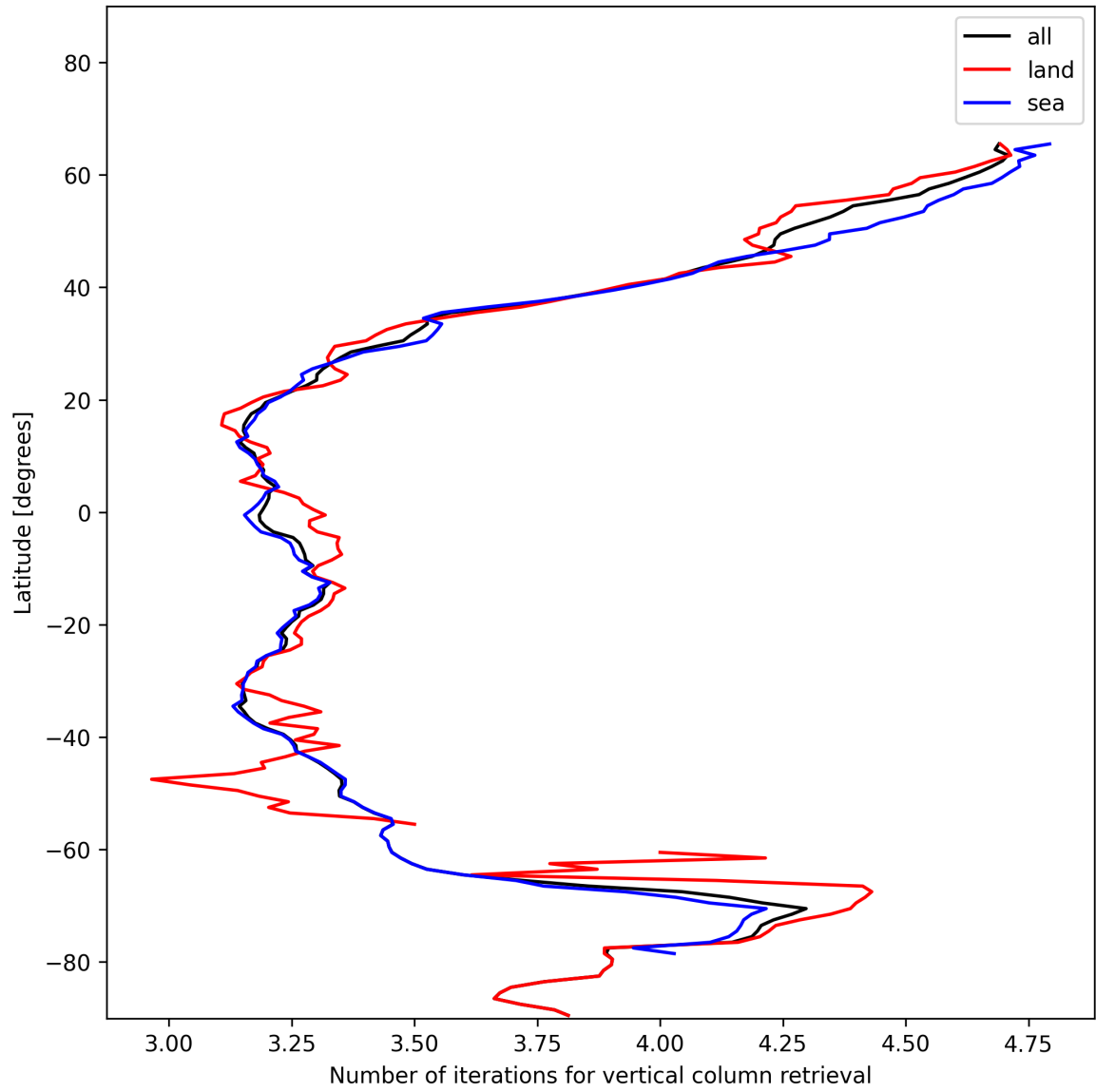
Figure 19: Zonal average of “Number of iterations for vertical column retrieval” for 2024-12-22 to 2024-12-24.
