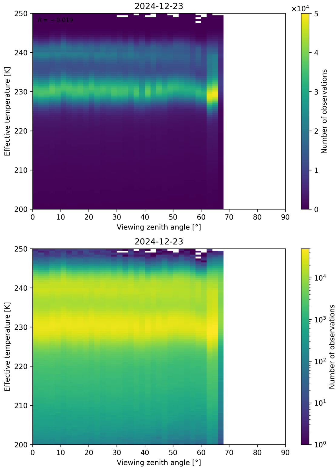
Figure 50: Scatter density plot of “Viewing zenith angle” against “Effective temperature” for 2024-12-22 to 2024-12-24.
