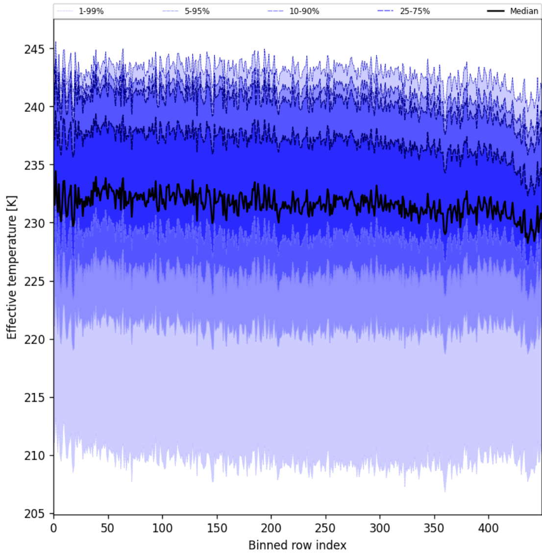
Figure 31: Along track statistics of “Effective temperature” for 2024-12-22 to 2024-12-24
