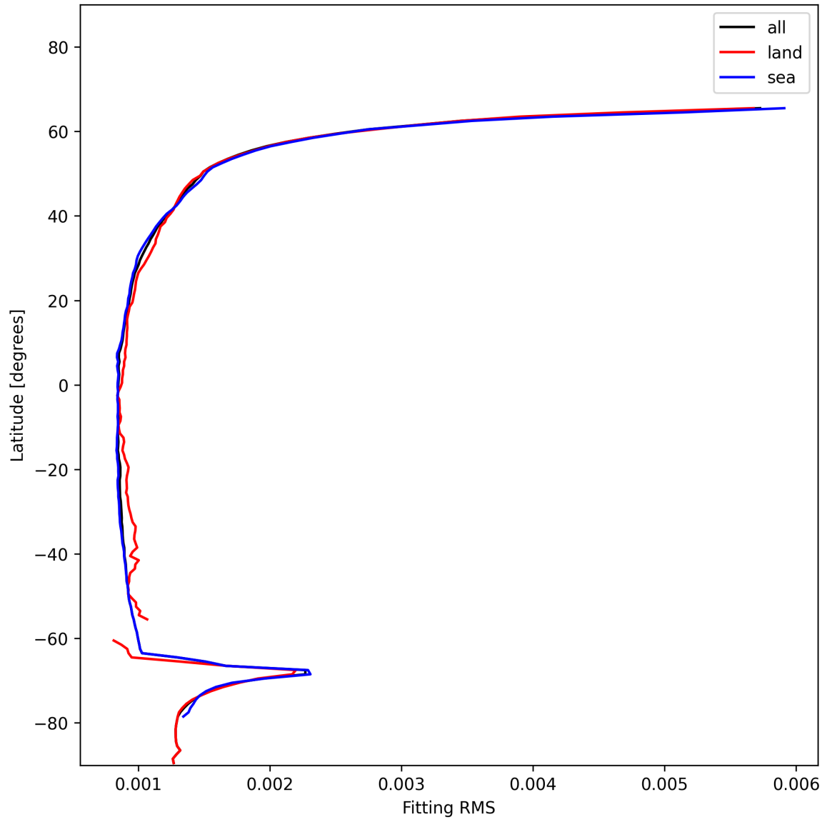
Figure 16: Zonal average of “Fitting RMS” for 2024-12-22 to 2024-12-24.
