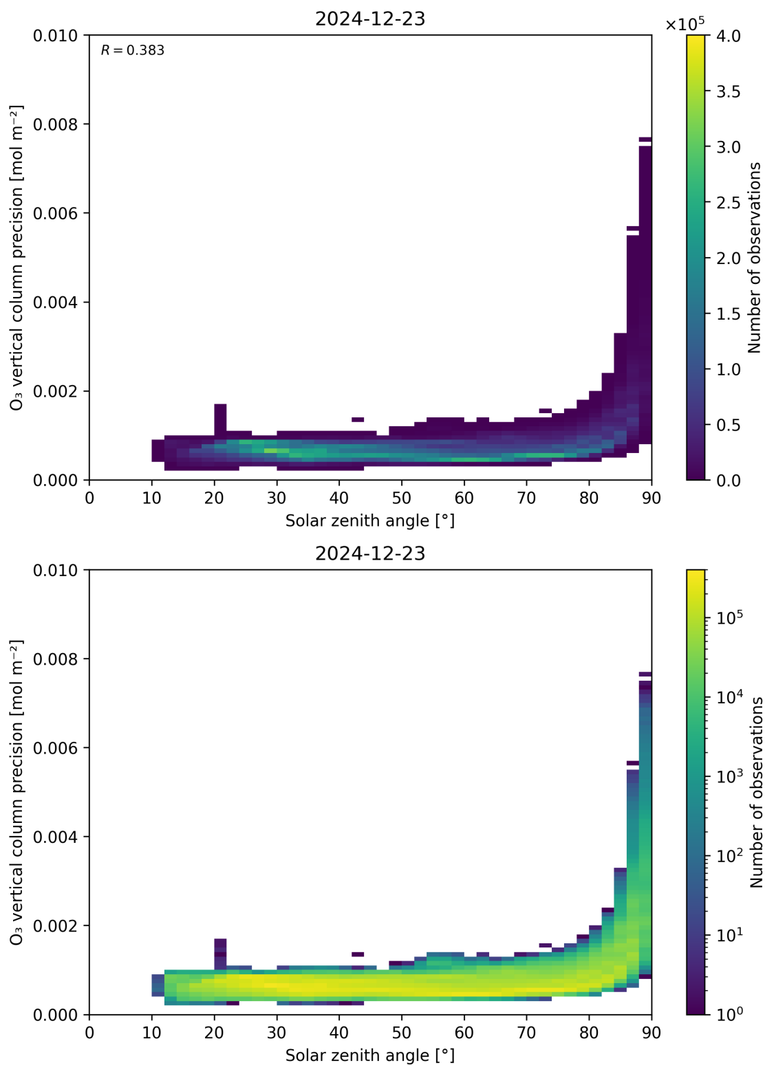
Figure 48: Scatter density plot of “Solar zenith angle” against “O 3 vertical column precision” for 2024-12-22 to 2024-12-24.
