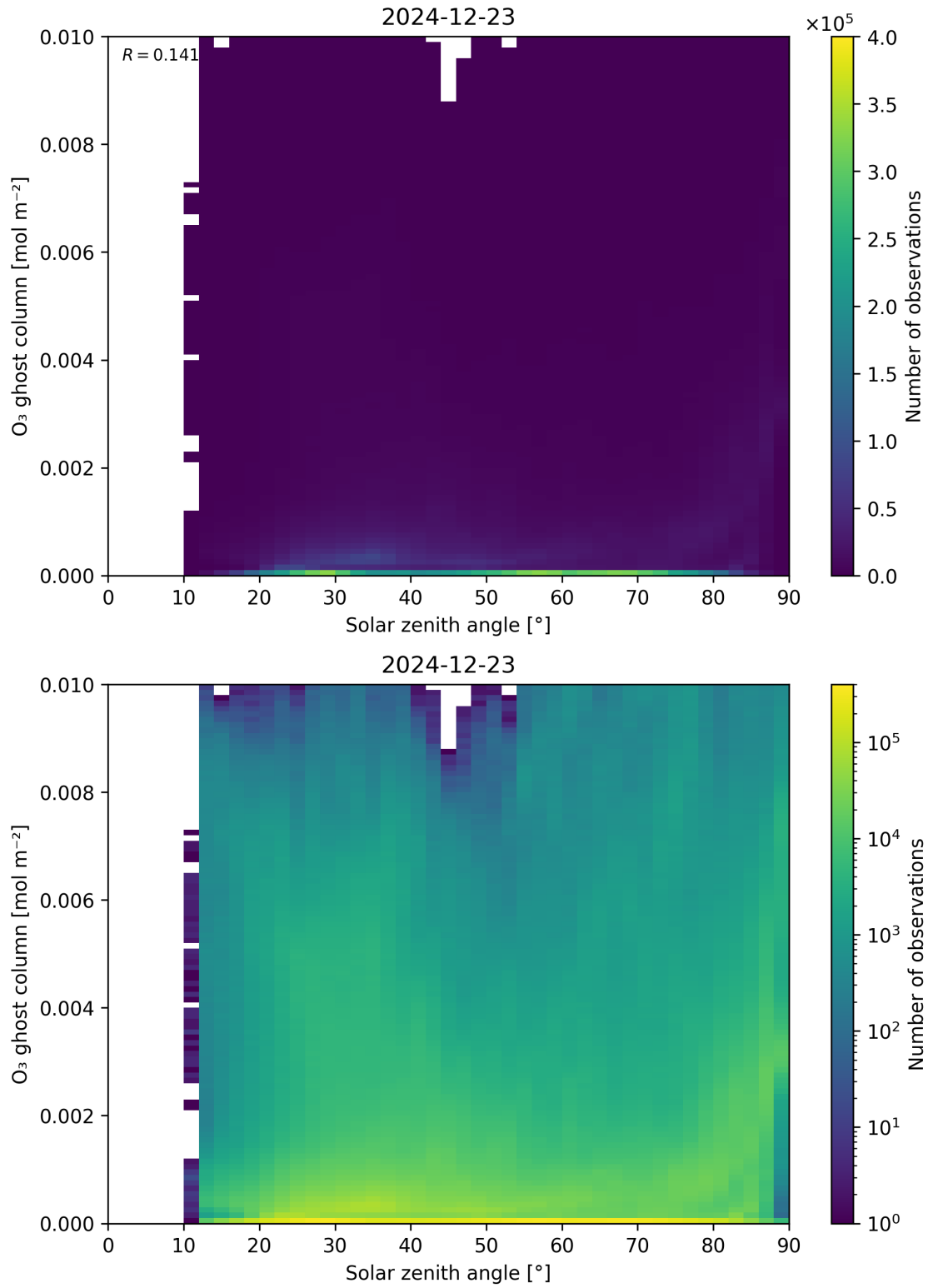
Figure 46: Scatter density plot of “Solar zenith angle” against “O 3 ghost column” for 2024-12-22 to 2024-12-24.
