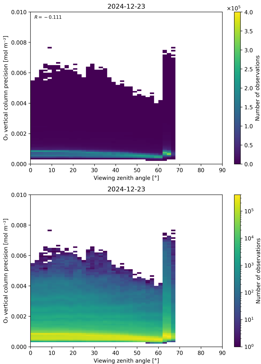
Figure 53: Scatter density plot of “Viewing zenith angle” against “O 3 vertical column precision” for 2024-12-22 to 2024-12-24.
