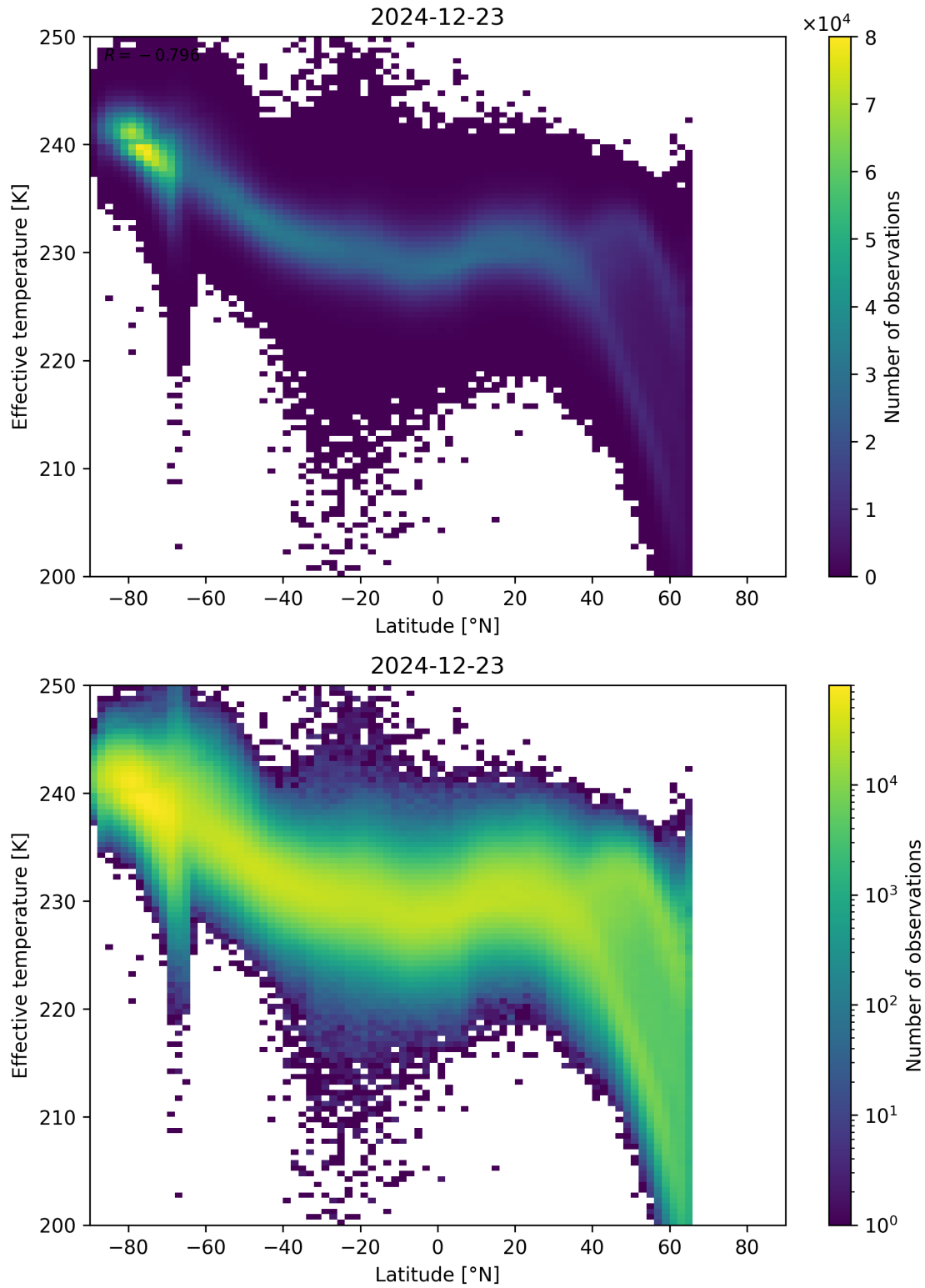
Figure 34: Scatter density plot of “Latitude” against “Effective temperature” for 2024-12-22 to 2024-12-24.
