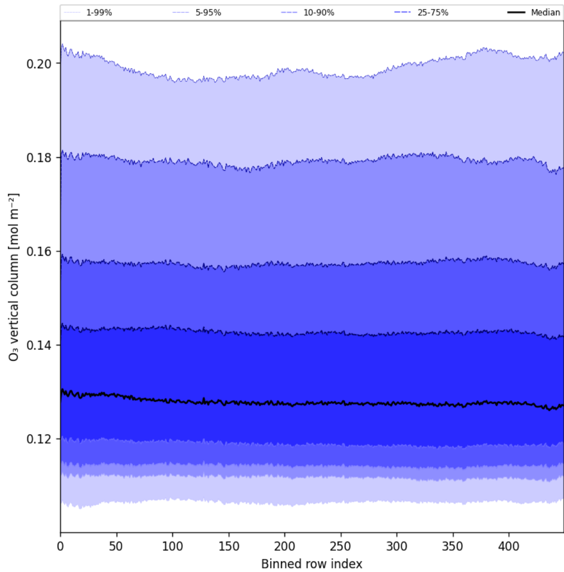
Figure 28: Along track statistics of “O 3 vertical column” for 2024-12-22 to 2024-12-24
