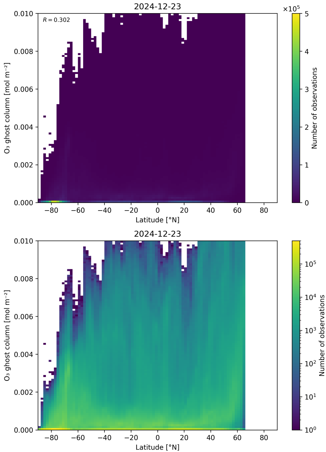
Figure 35: Scatter density plot of “Latitude” against “O 3 ghost column” for 2024-12-22 to 2024-12-24.
