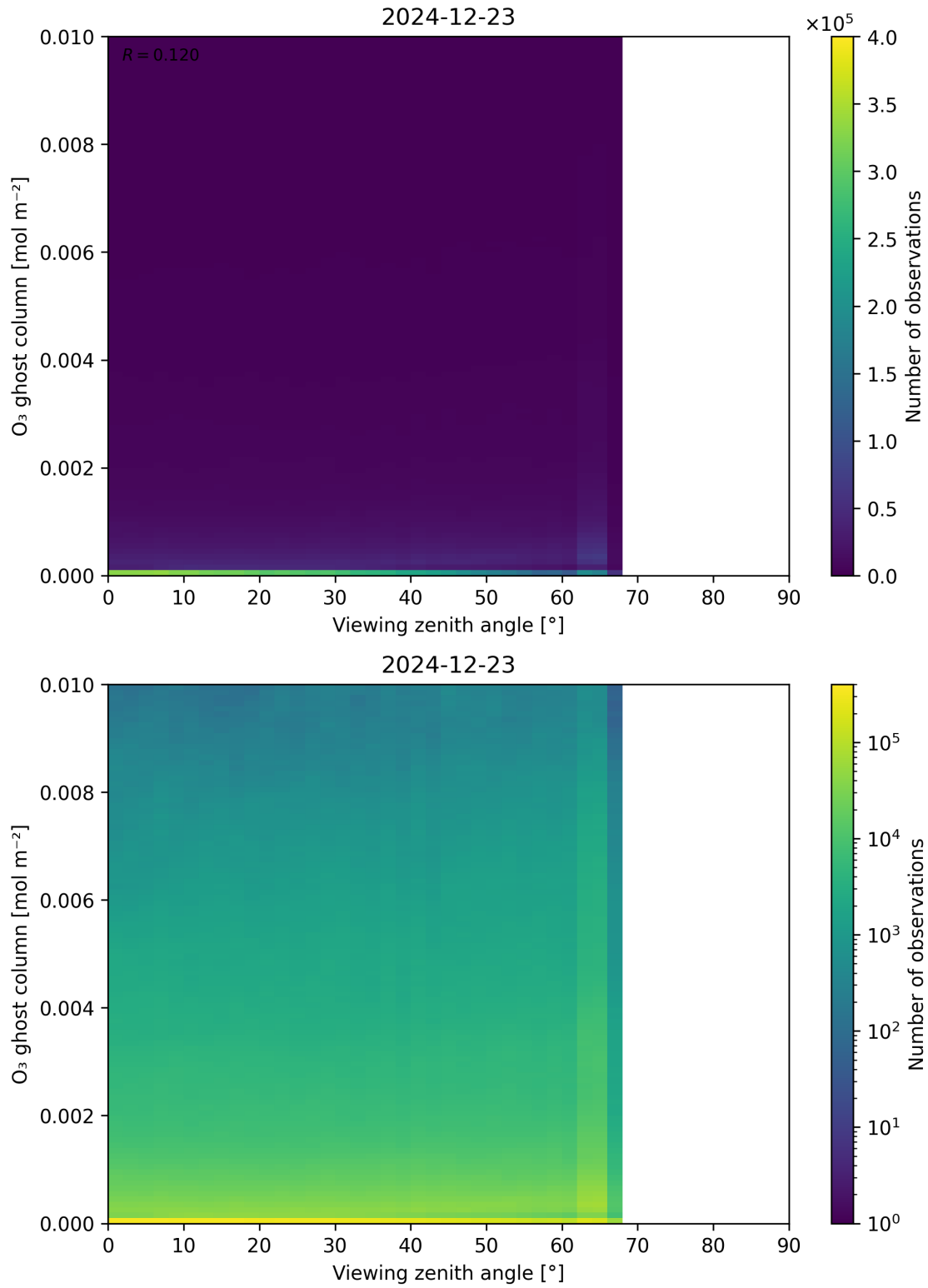
Figure 51: Scatter density plot of “Viewing zenith angle” against “O 3 ghost column” for 2024-12-22 to 2024-12-24.
