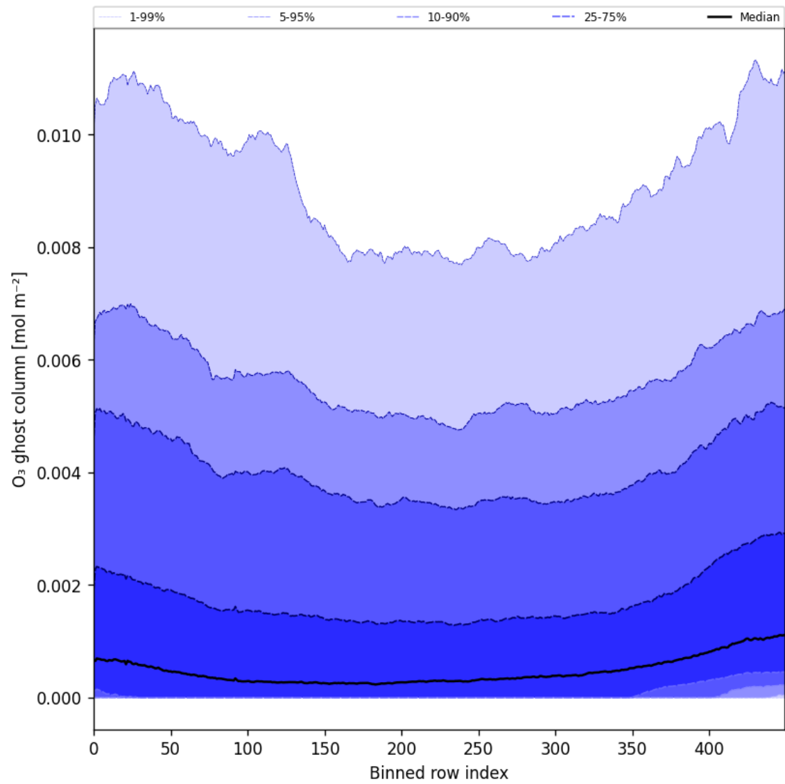
Figure 32: Along track statistics of “O 3 ghost column” for 2024-12-22 to 2024-12-24
