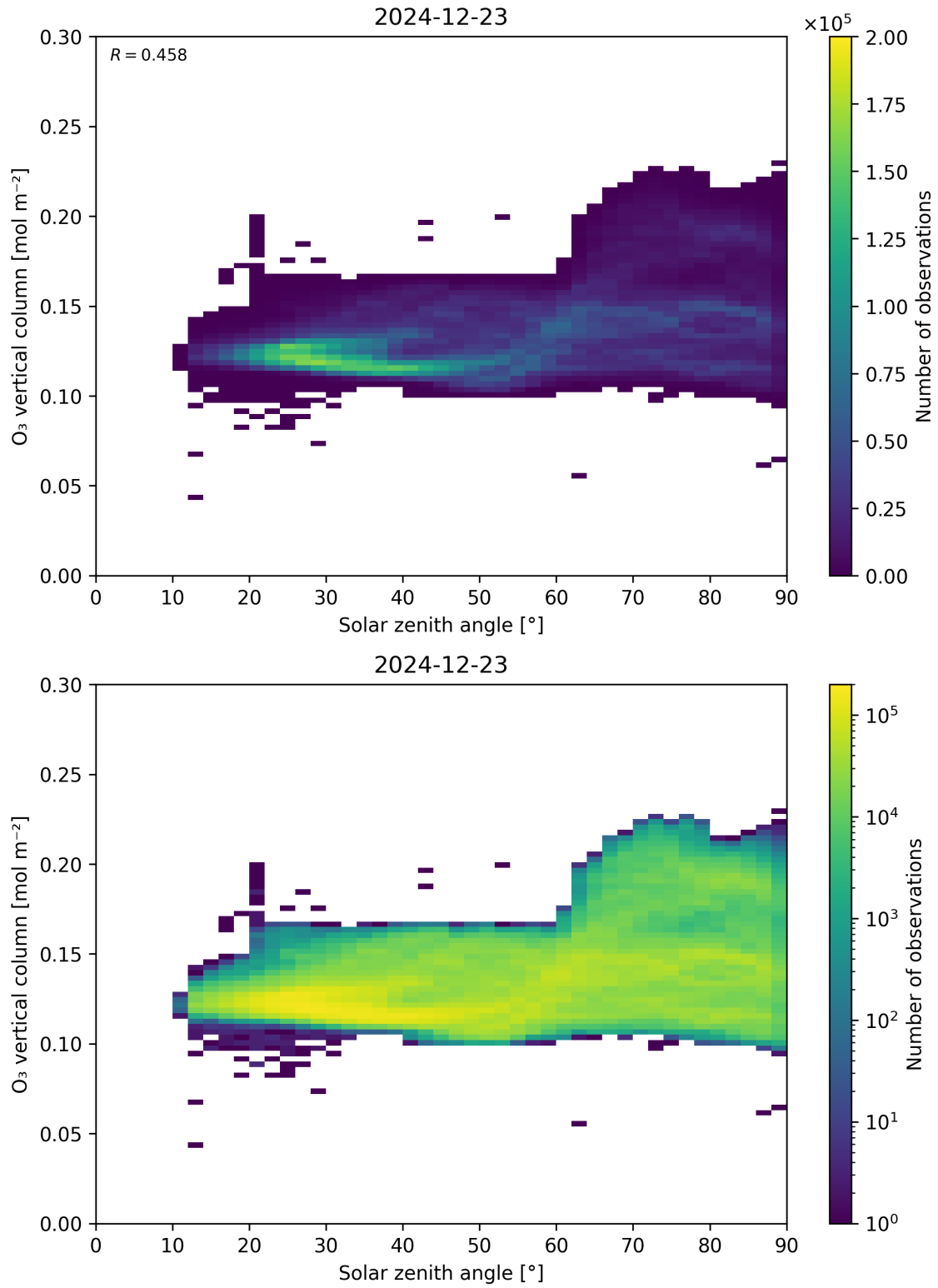
Figure 47: Scatter density plot of “Solar zenith angle” against “O 3 vertical column” for 2024-12-22 to 2024-12-24.
