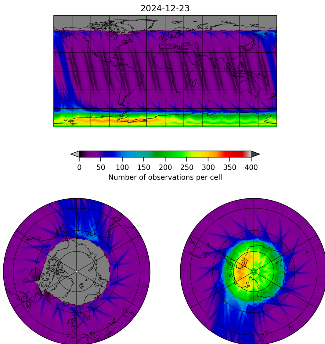
Figure 12: Map of the number of observations for 2024-12-22 to 2024-12-24
