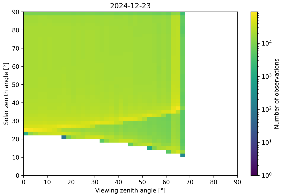
Figure 54: Scatter density plot of “Viewing zenith angle” against “Solar zenith angle” for 2024-12-22 to 2024-12-24.
