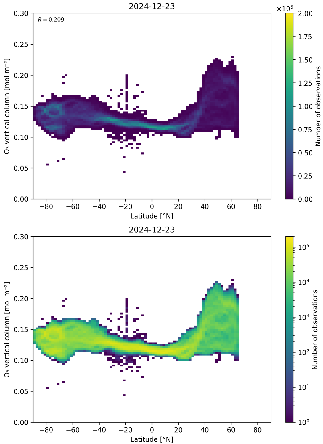
Figure 36: Scatter density plot of “Latitude” against “O 3 vertical column” for 2024-12-22 to 2024-12-24.
