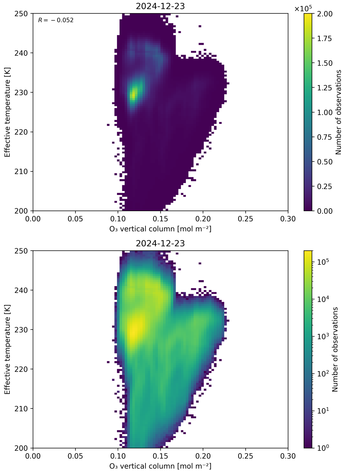
Figure 39: Scatter density plot of “O 3 vertical column” against “Effective temperature” for 2024-12-22 to 2024-12-24.
