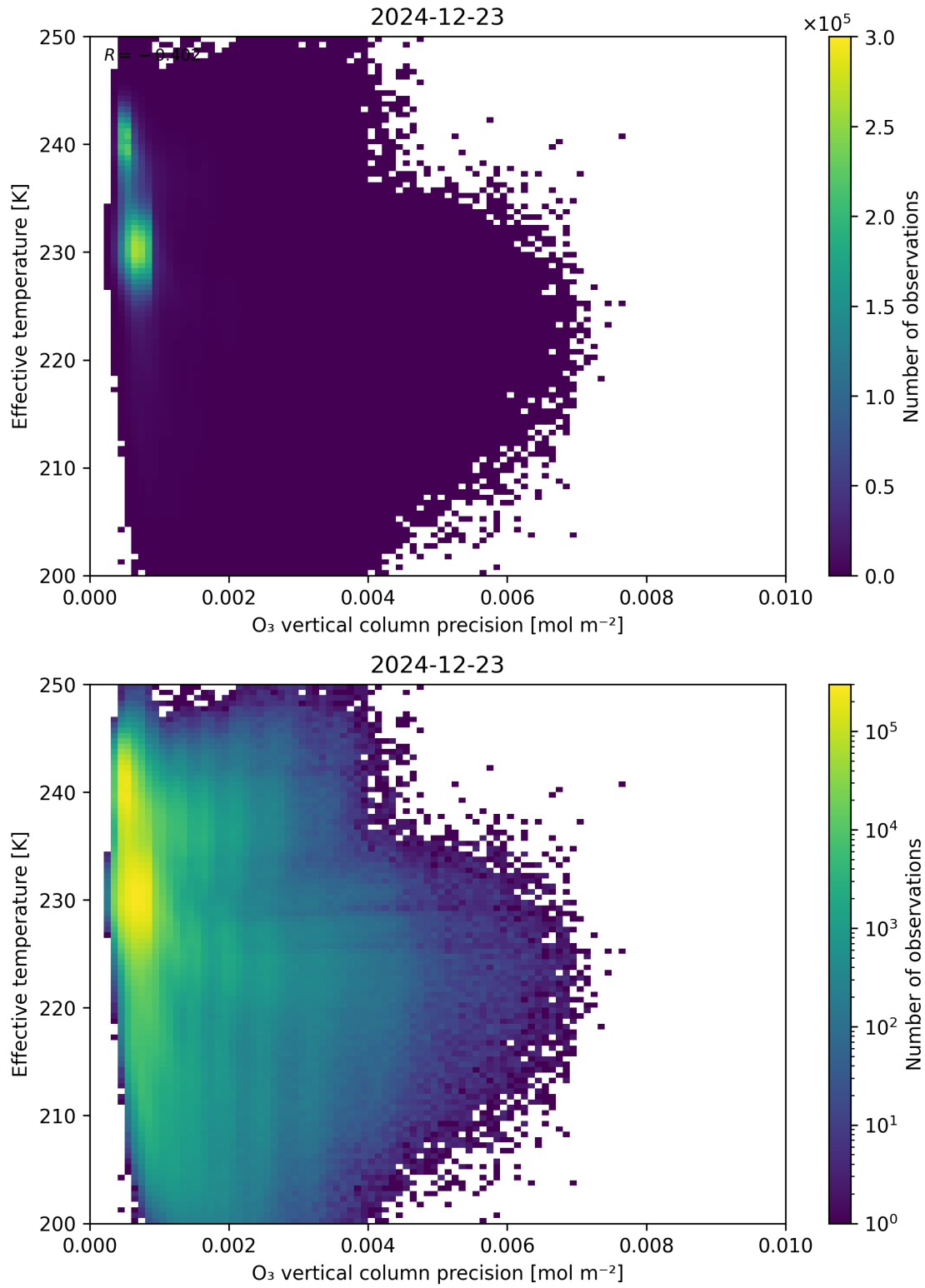
Figure 42: Scatter density plot of “O 3 vertical column precision” against “Effective temperature” for 2024-12-22 to 2024-12-24.
