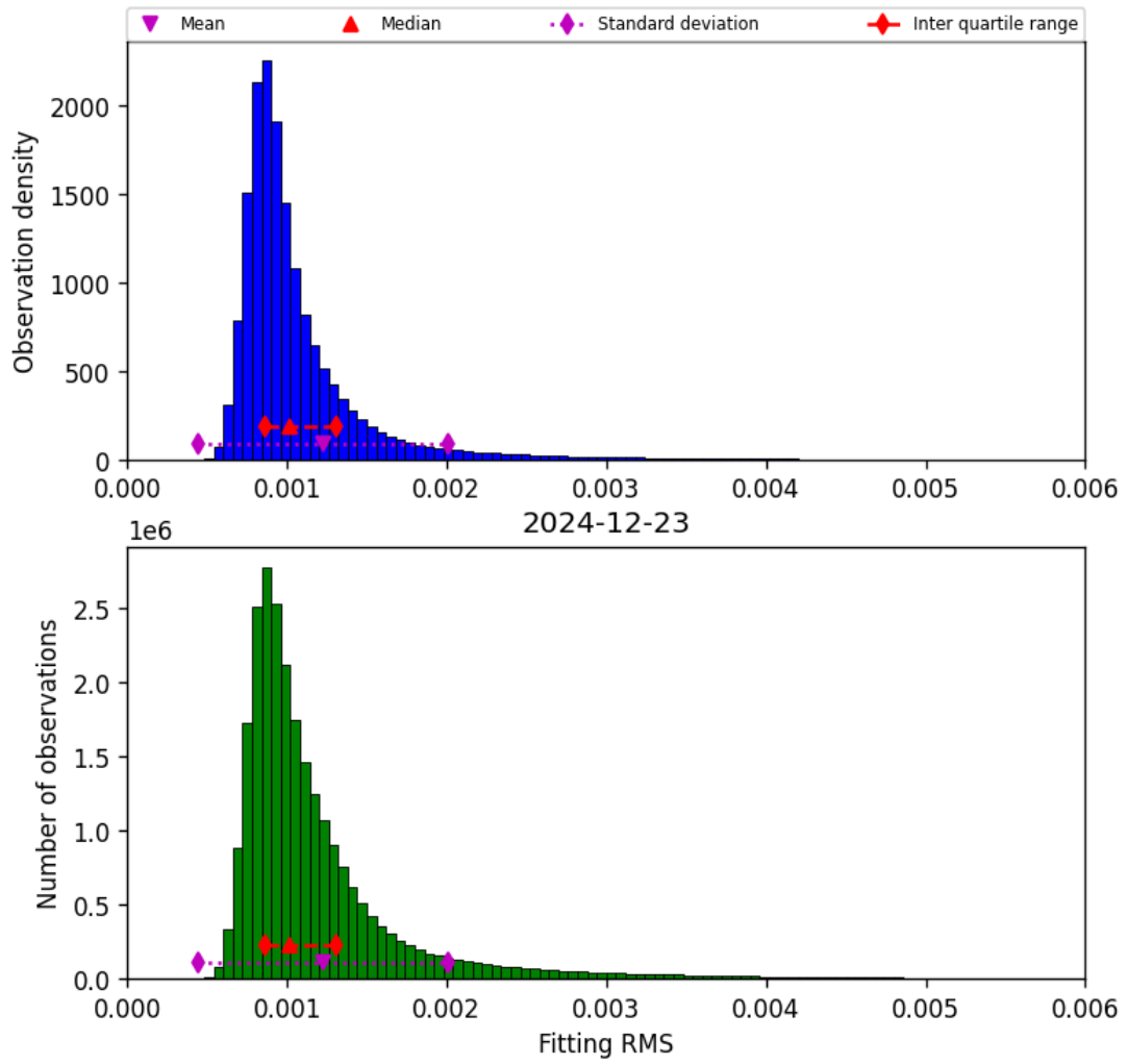
Figure 23: Histogram of “Fitting RMS” for 2024-12-22 to 2024-12-24
