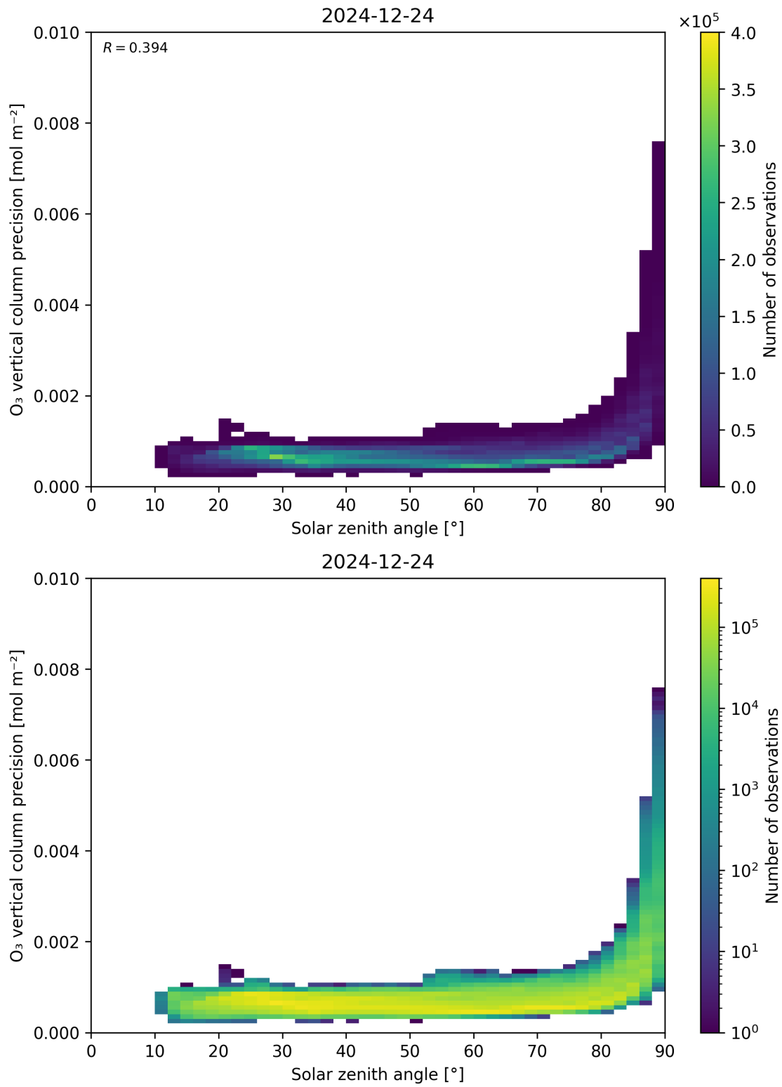
Figure 48: Scatter density plot of “Solar zenith angle” against “O 3 vertical column precision” for 2024-12-23 to 2024-12-25.
