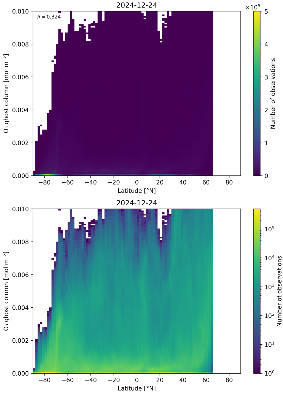
Figure 35: Scatter density plot of “Latitude” against “O 3 ghost column” for 2024-12-23 to 2024-12-25.
