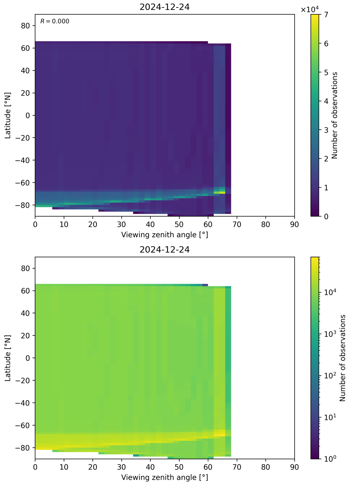
Figure 49: Scatter density plot of “Viewing zenith angle” against “Latitude” for 2024-12-23 to 2024-12-25.
