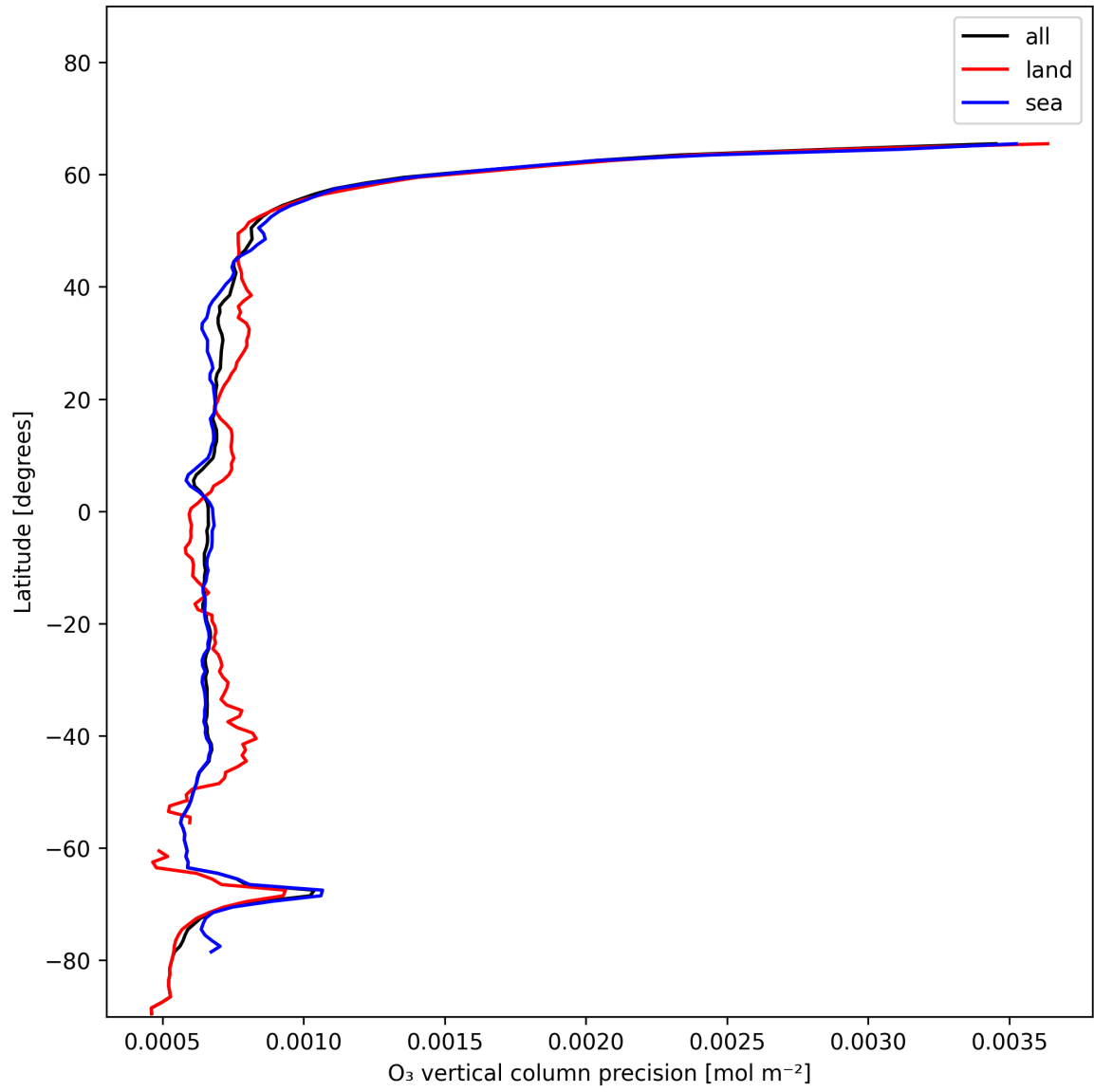
Figure 15: Zonal average of “O 3 vertical column precision” for 2024-12-23 to 2024-12-25.
