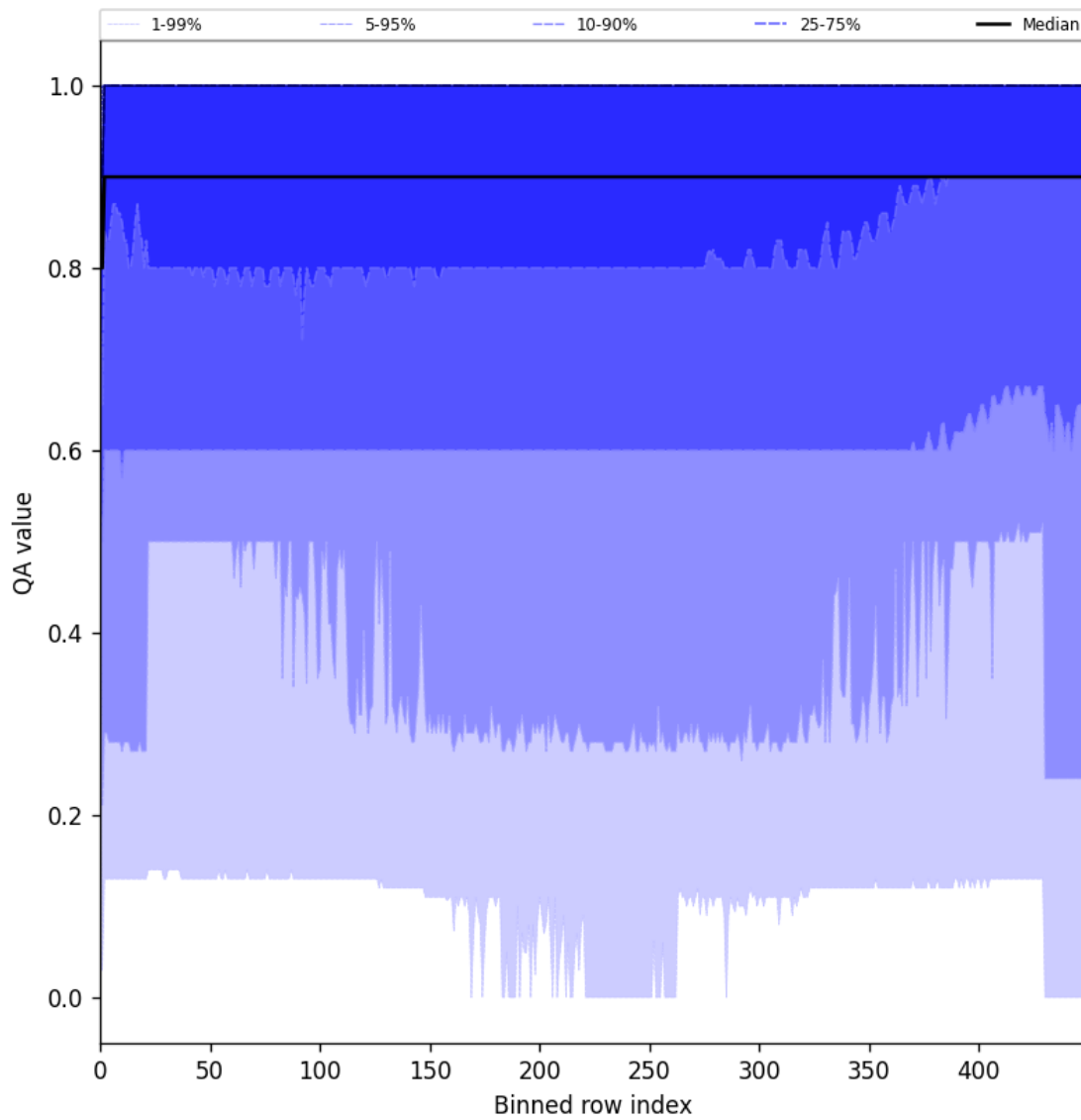
Figure 27: Along track statistics of “QA value” for 2024-12-23 to 2024-12-25
