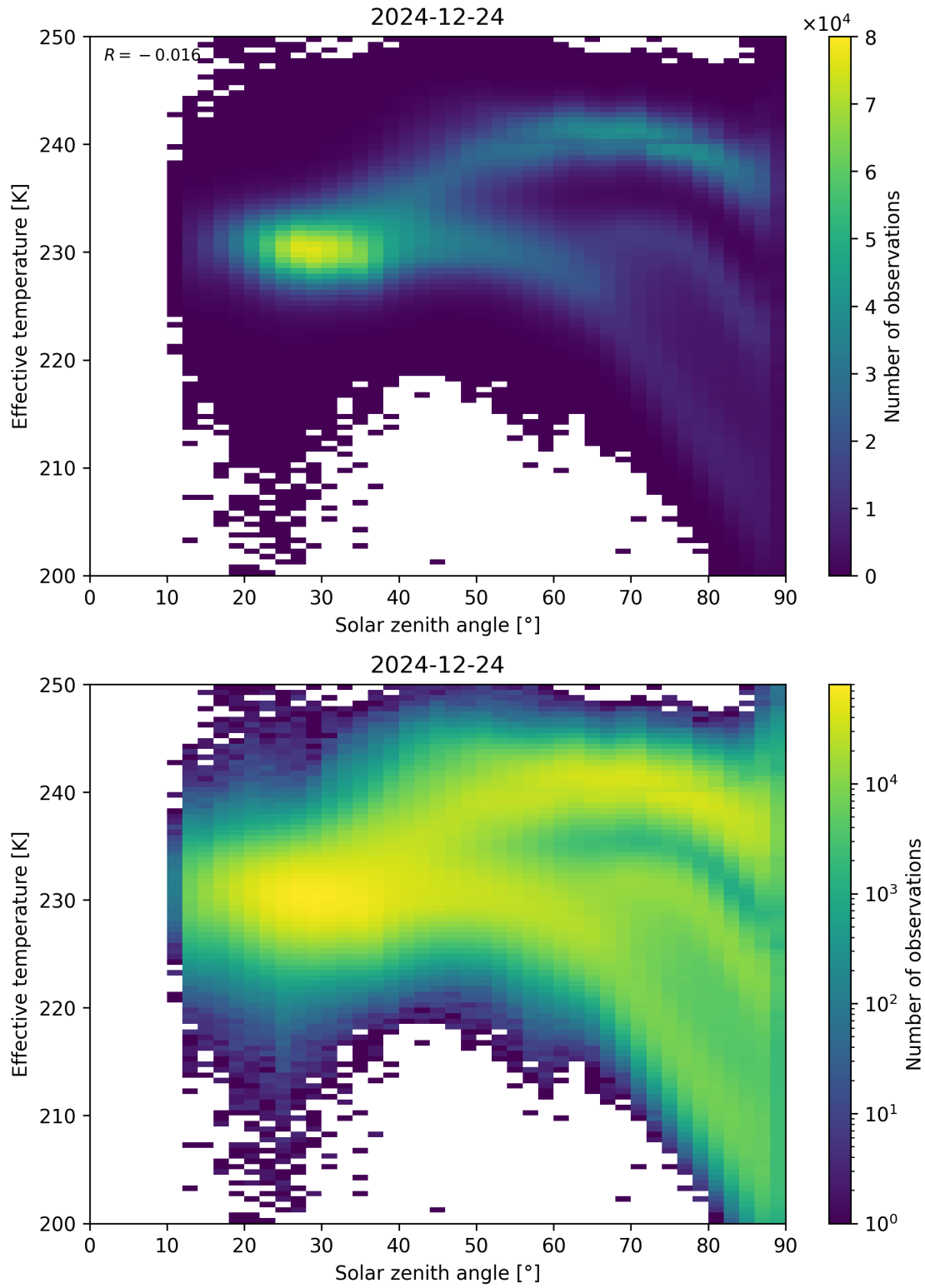
Figure 45: Scatter density plot of “Solar zenith angle” against “Effective temperature” for 2024-12-23 to 2024-12-25.
