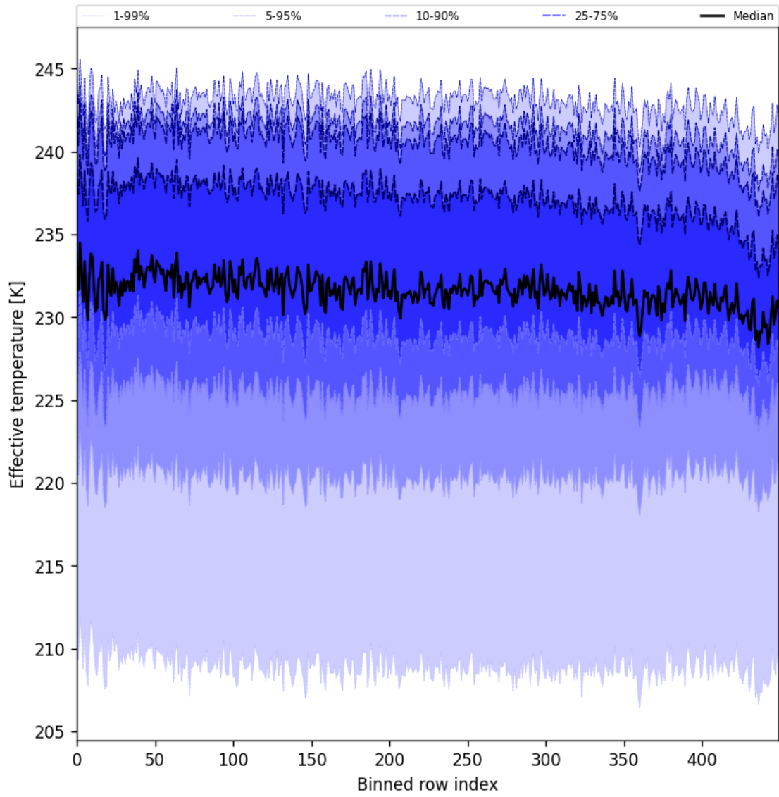
Figure 31: Along track statistics of “Effective temperature” for 2024-12-23 to 2024-12-25
