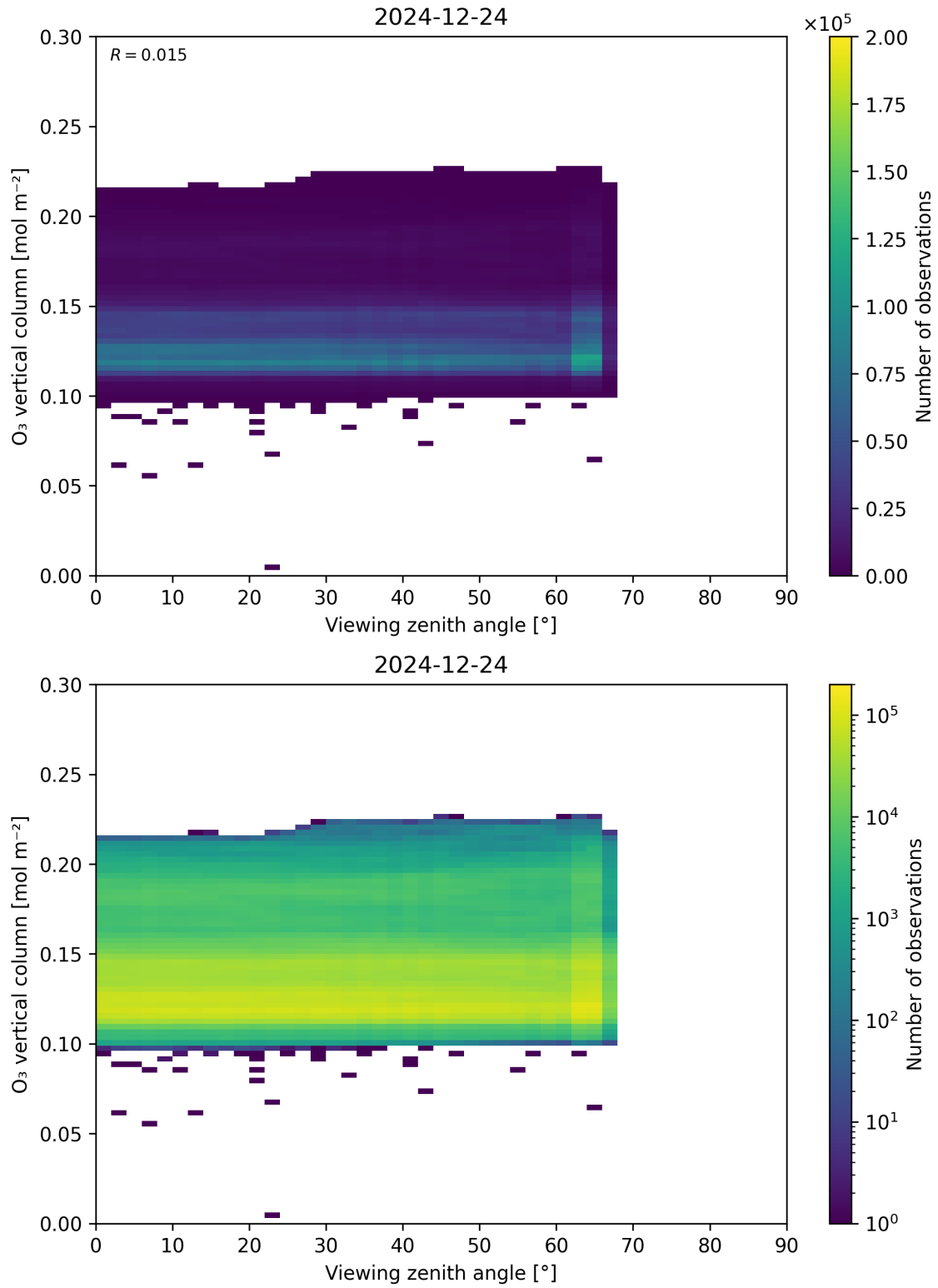
Figure 52: Scatter density plot of “Viewing zenith angle” against “O 3 vertical column” for 2024-12-23 to 2024-12-25.
