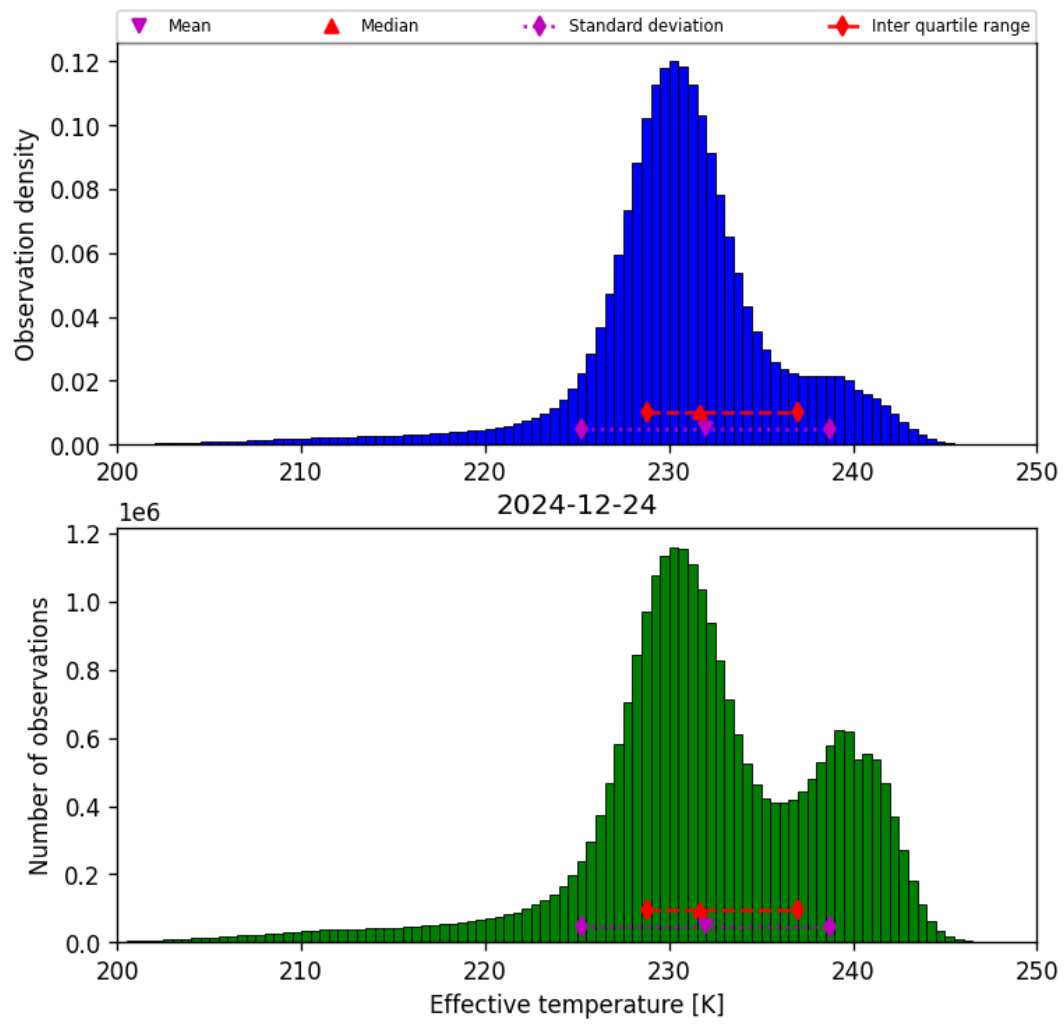
Figure 24: Histogram of “Effective temperature” for 2024-12-23 to 2024-12-25
