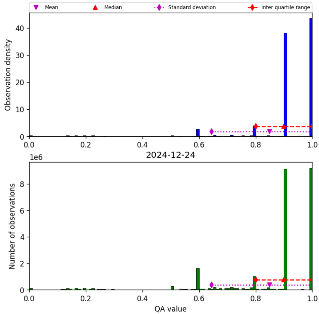
Figure 20: Histogram of “QA value” for 2024-12-23 to 2024-12-25
