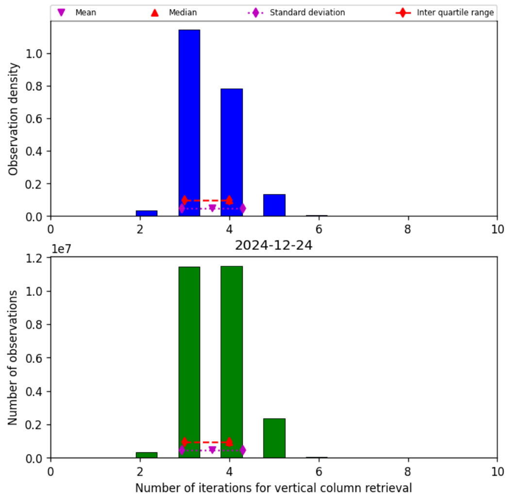
Figure 26: Histogram of “Number of iterations for vertical column retrieval” for 2024-12-23 to 2024-12-25
