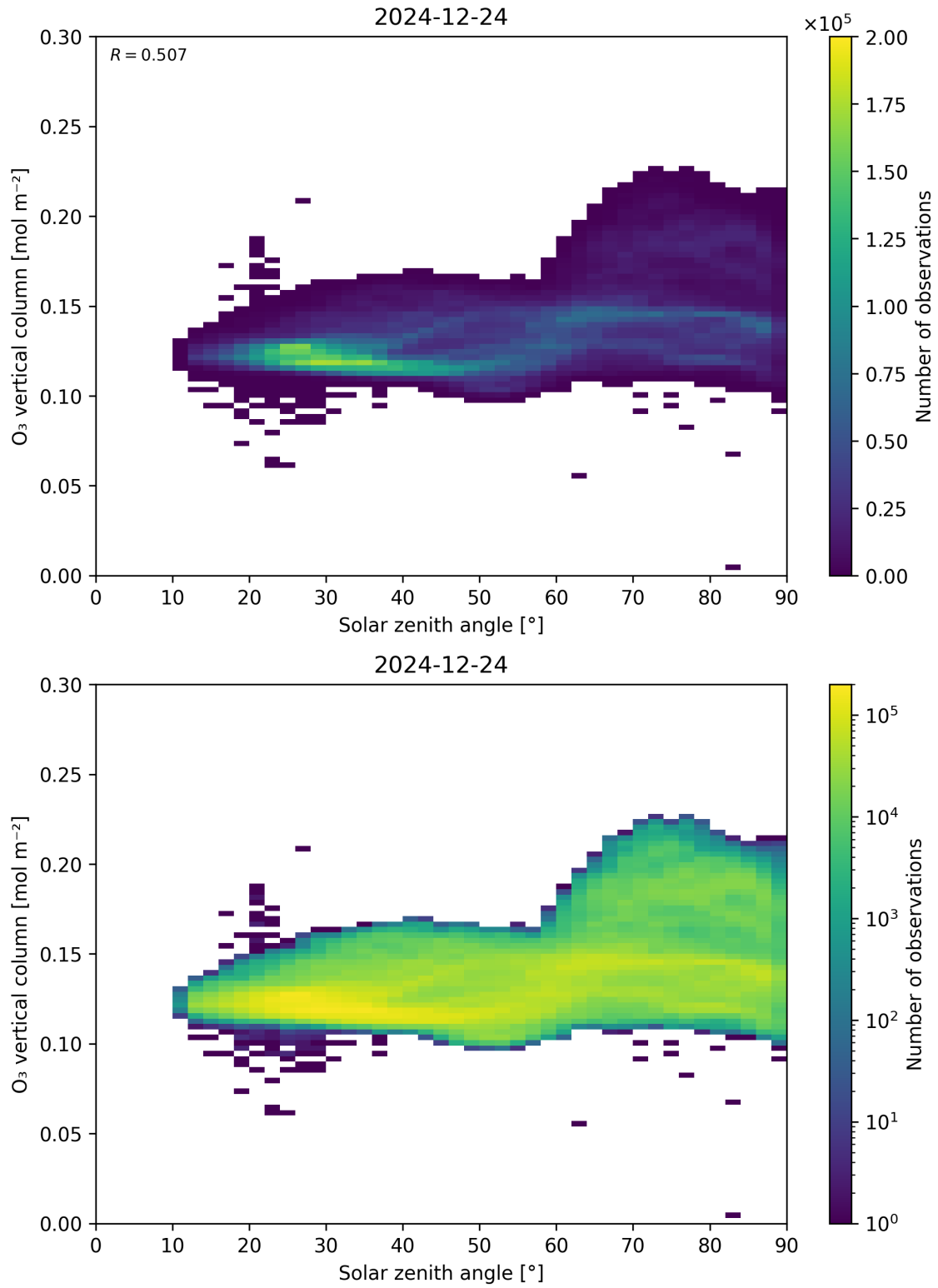
Figure 47: Scatter density plot of “Solar zenith angle” against “O 3 vertical column” for 2024-12-23 to 2024-12-25.
