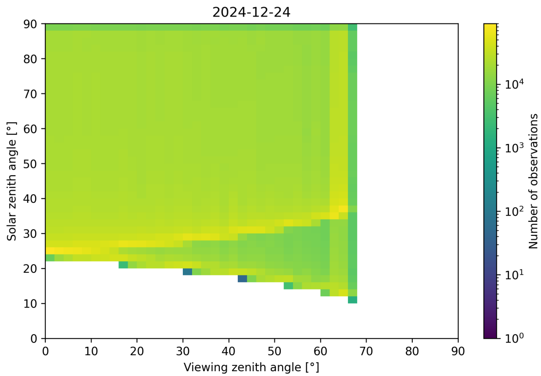
Figure 54: Scatter density plot of “Viewing zenith angle” against “Solar zenith angle” for 2024-12-23 to 2024-12-25.
