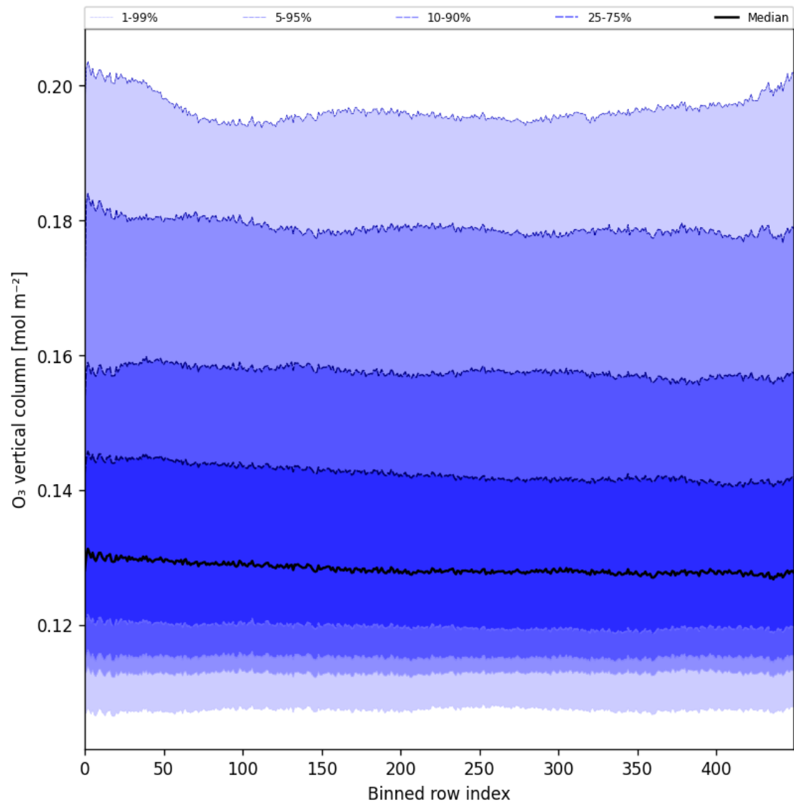
Figure 28: Along track statistics of “O 3 vertical column” for 2024-12-23 to 2024-12-25
