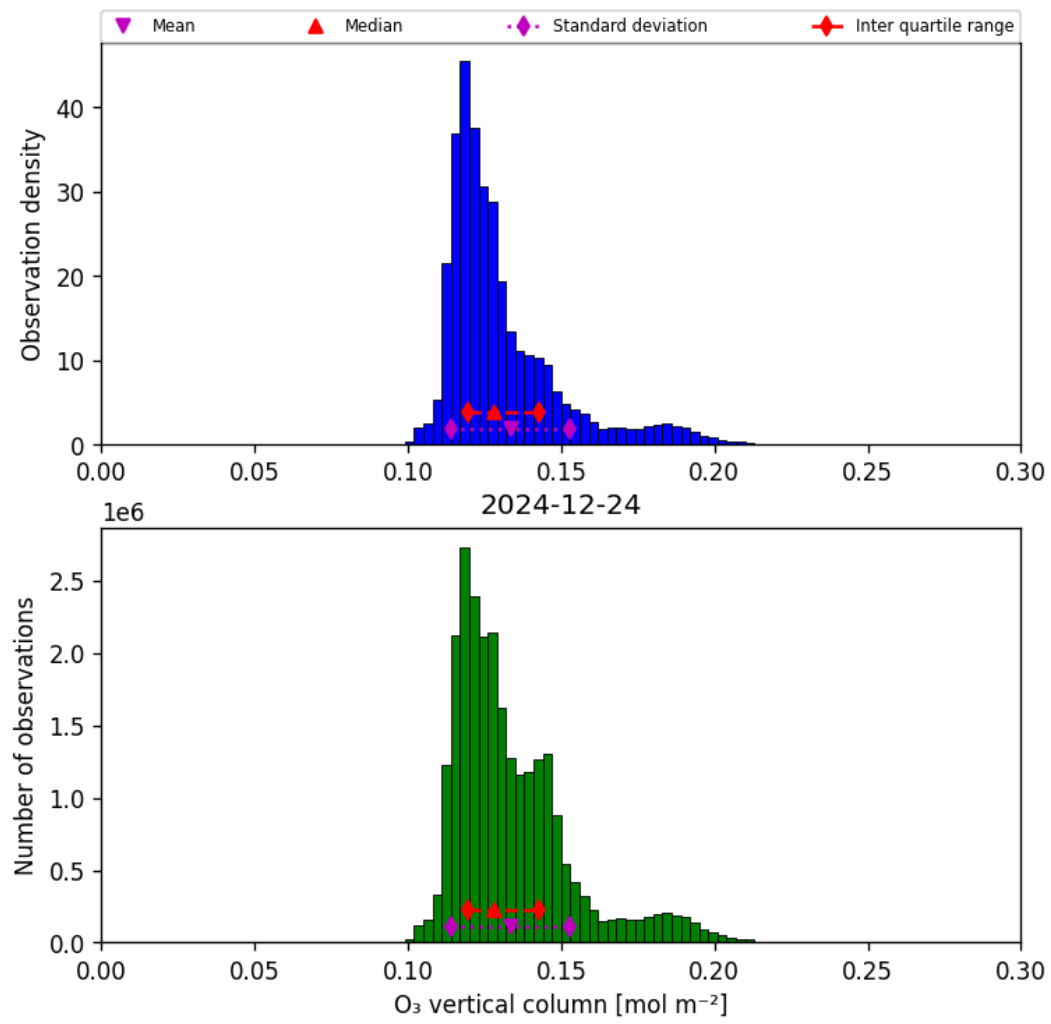
Figure 21: Histogram of “O 3 vertical column” for 2024-12-23 to 2024-12-25
