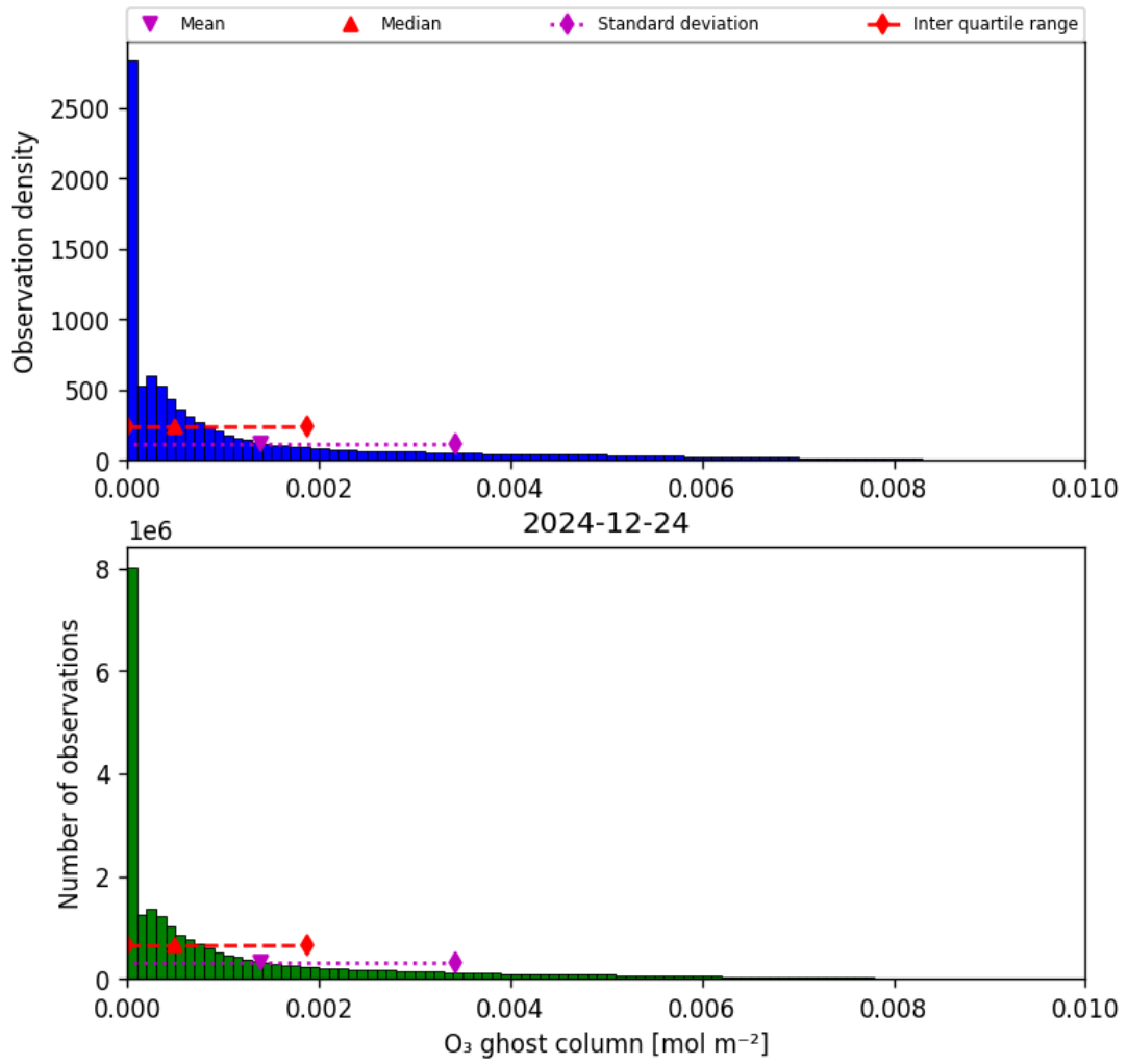
Figure 25: Histogram of “O 3 ghost column” for 2024-12-23 to 2024-12-25
