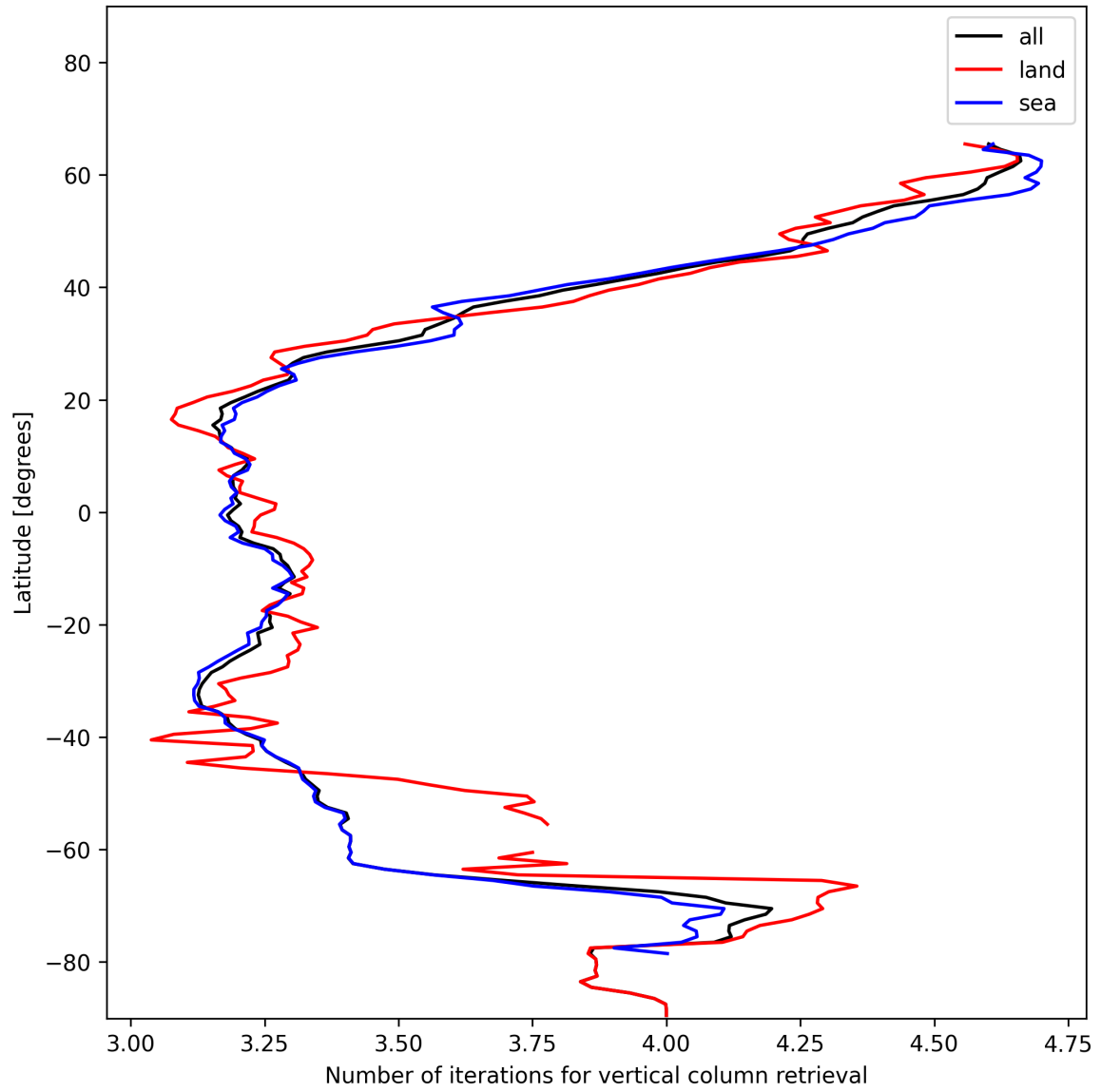
Figure 19: Zonal average of “Number of iterations for vertical column retrieval” for 2024-12-23 to 2024-12-25.
