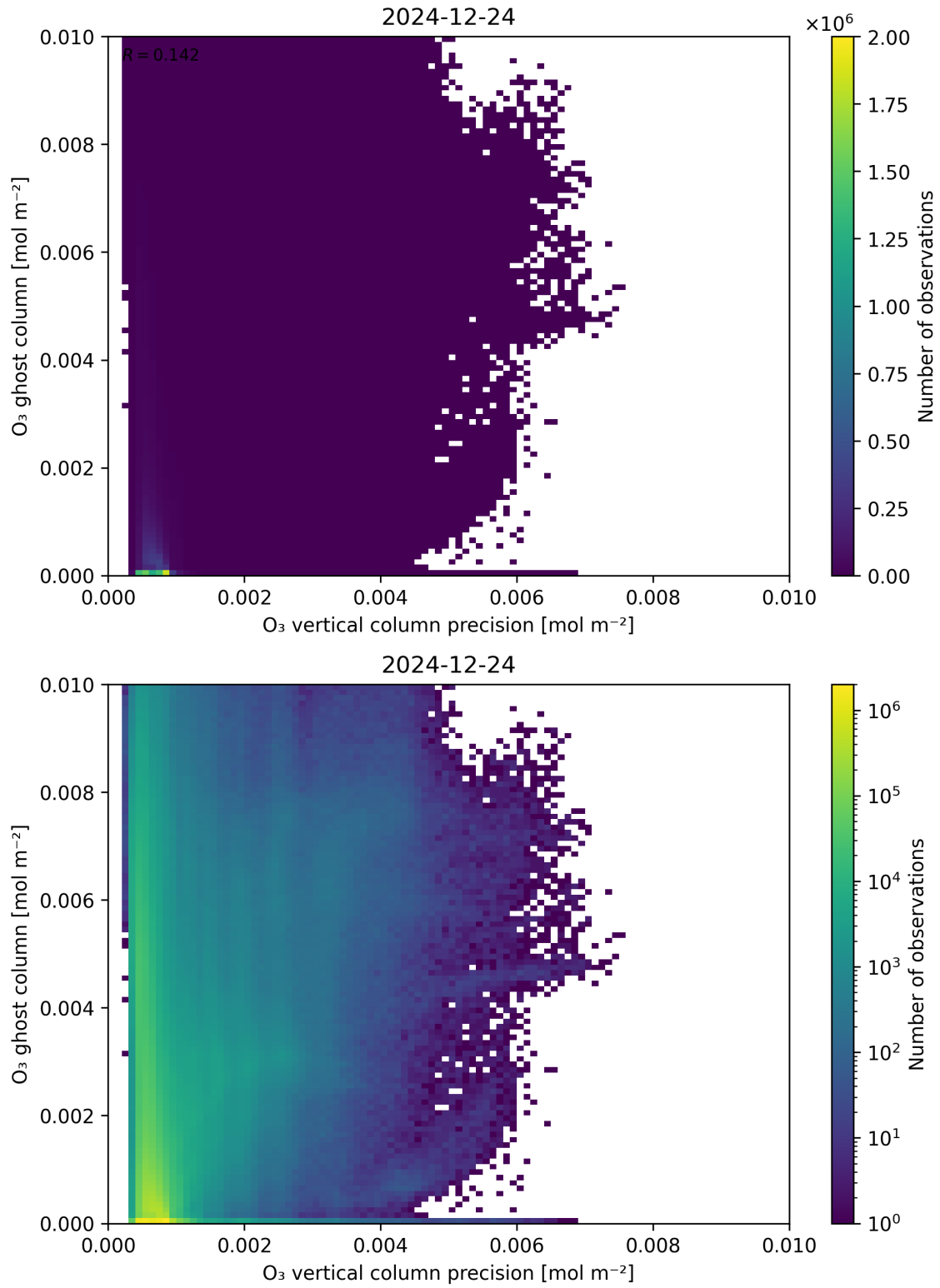
Figure 43: Scatter density plot of “ \text{O}_3 vertical column precision” against “ \text{O}_3 ghost column” for 2024-12-23 to 2024-12-25.
