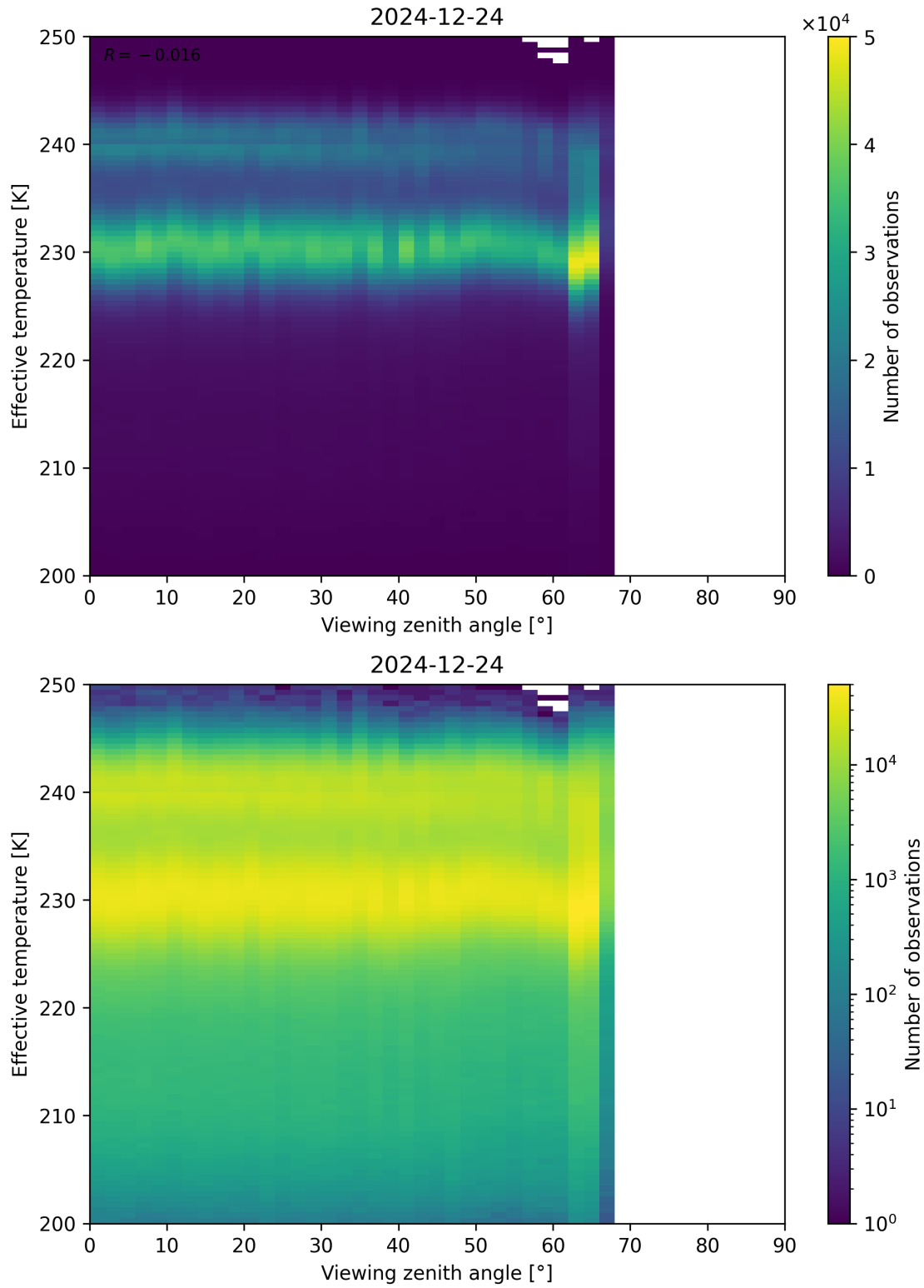
Figure 50: Scatter density plot of “Viewing zenith angle” against “Effective temperature” for 2024-12-23 to 2024-12-25.
