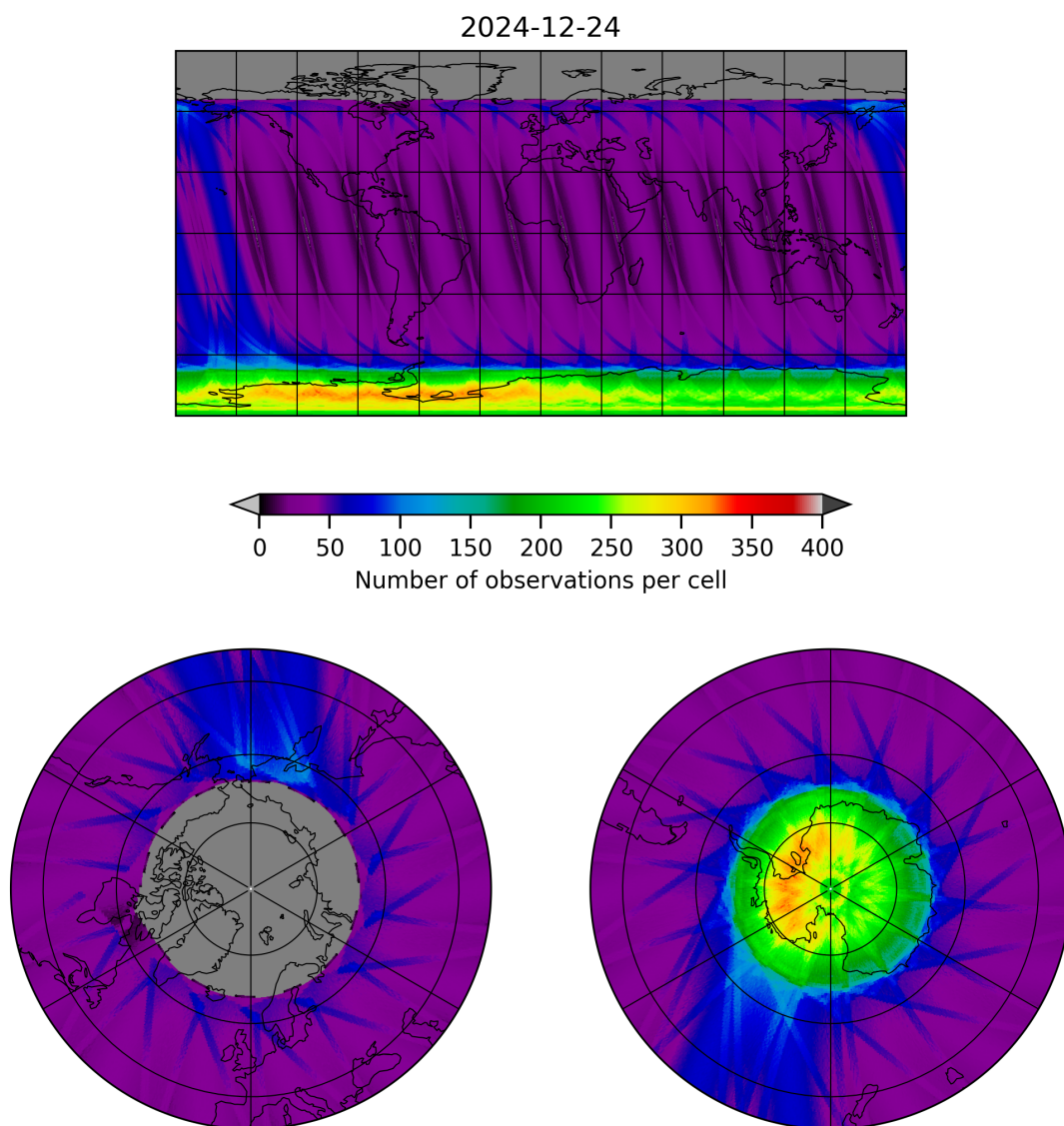
Figure 12: Map of the number of observations for 2024-12-23 to 2024-12-25
