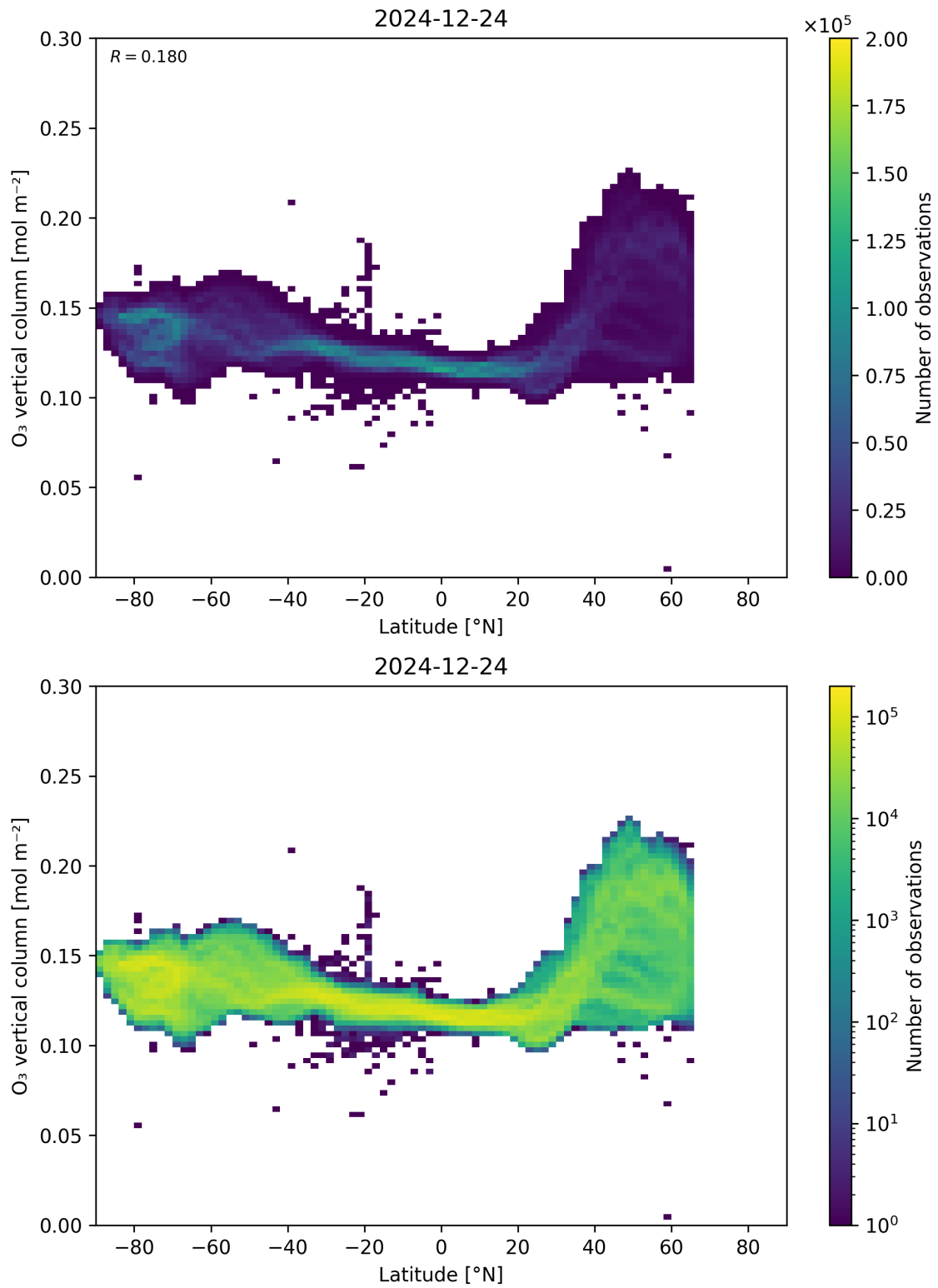
Figure 36: Scatter density plot of “Latitude” against “O 3 vertical column” for 2024-12-23 to 2024-12-25.
