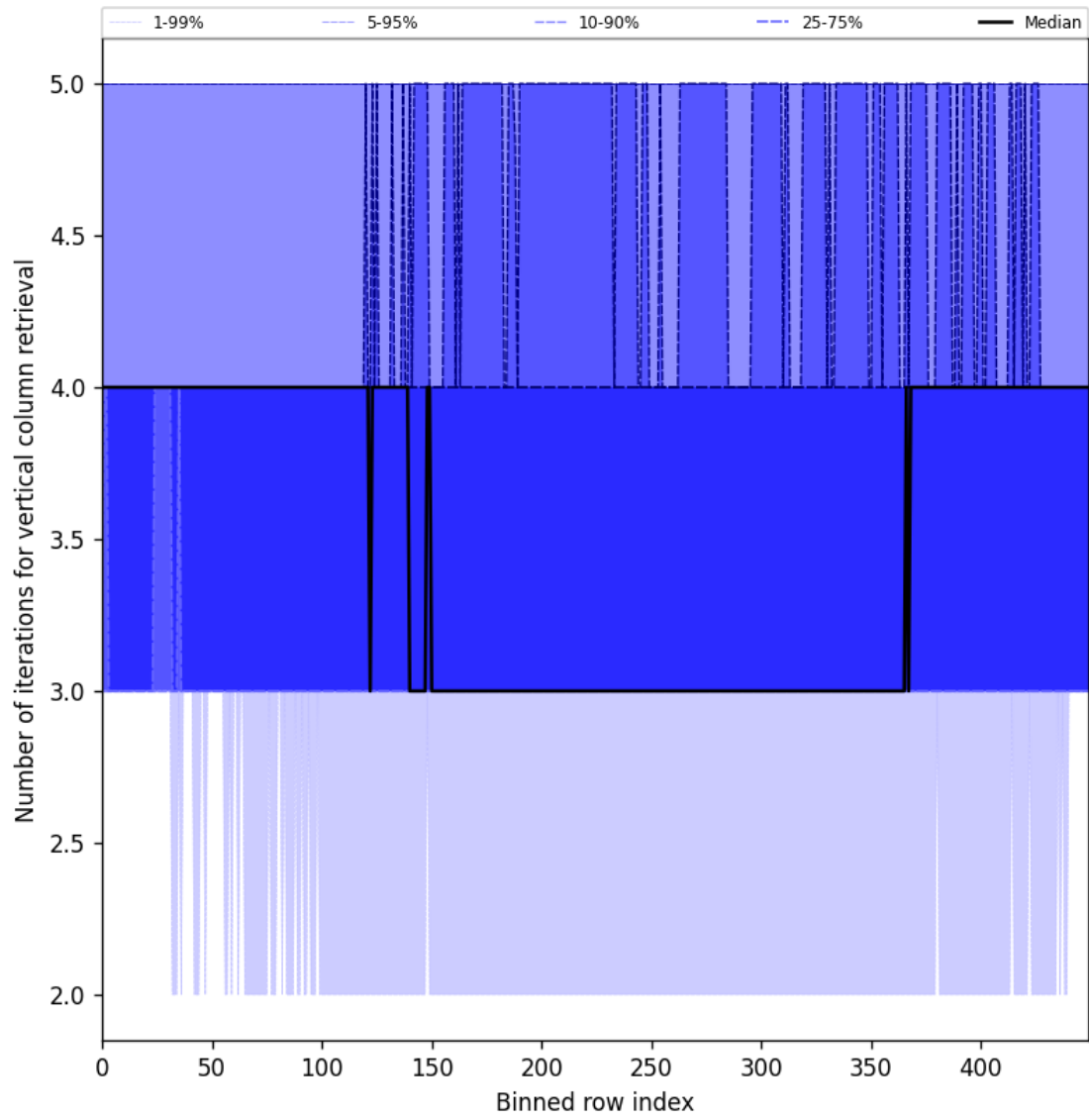
Figure 33: Along track statistics of “Number of iterations for vertical column retrieval” for 2024-12-23 to 2024-12-25
