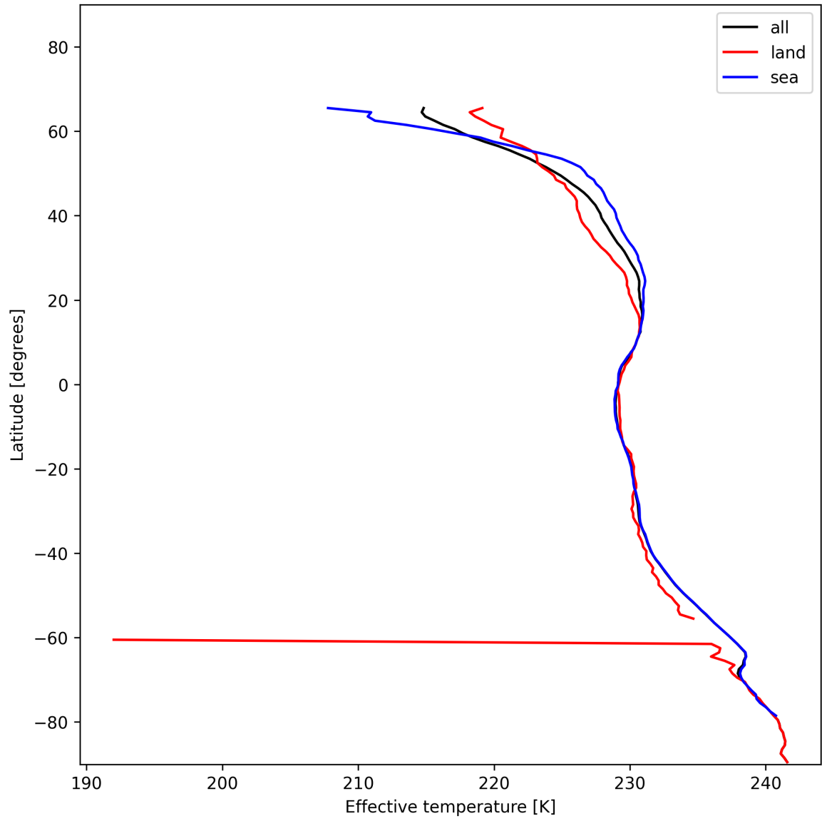
Figure 17: Zonal average of “Effective temperature” for 2024-12-23 to 2024-12-25.
