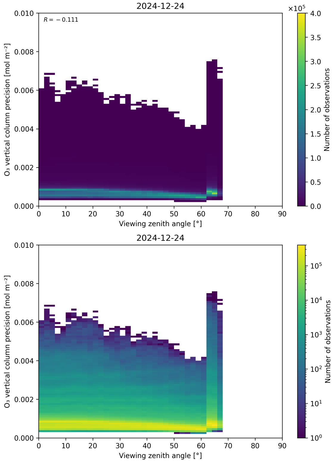
Figure 53: Scatter density plot of “Viewing zenith angle” against “O 3 vertical column precision” for 2024-12-23 to 2024-12-25.
