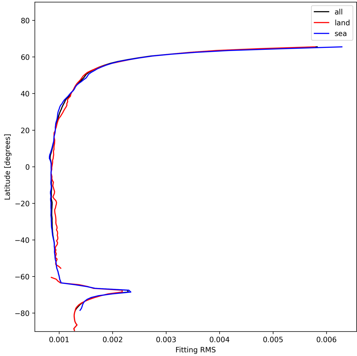
Figure 16: Zonal average of “Fitting RMS” for 2024-12-23 to 2024-12-25.
