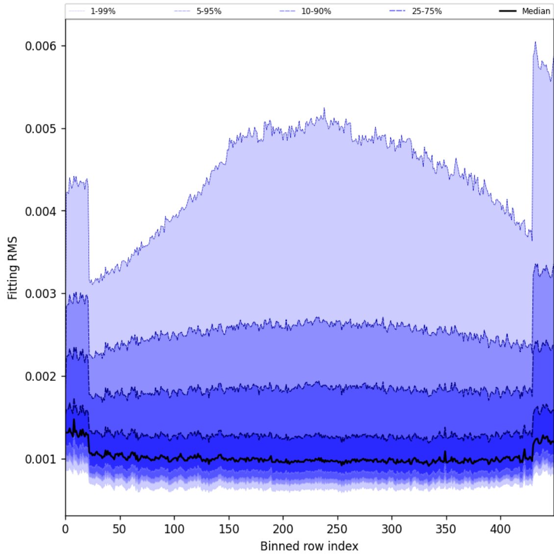
Figure 30: Along track statistics of “Fitting RMS” for 2024-12-23 to 2024-12-25
