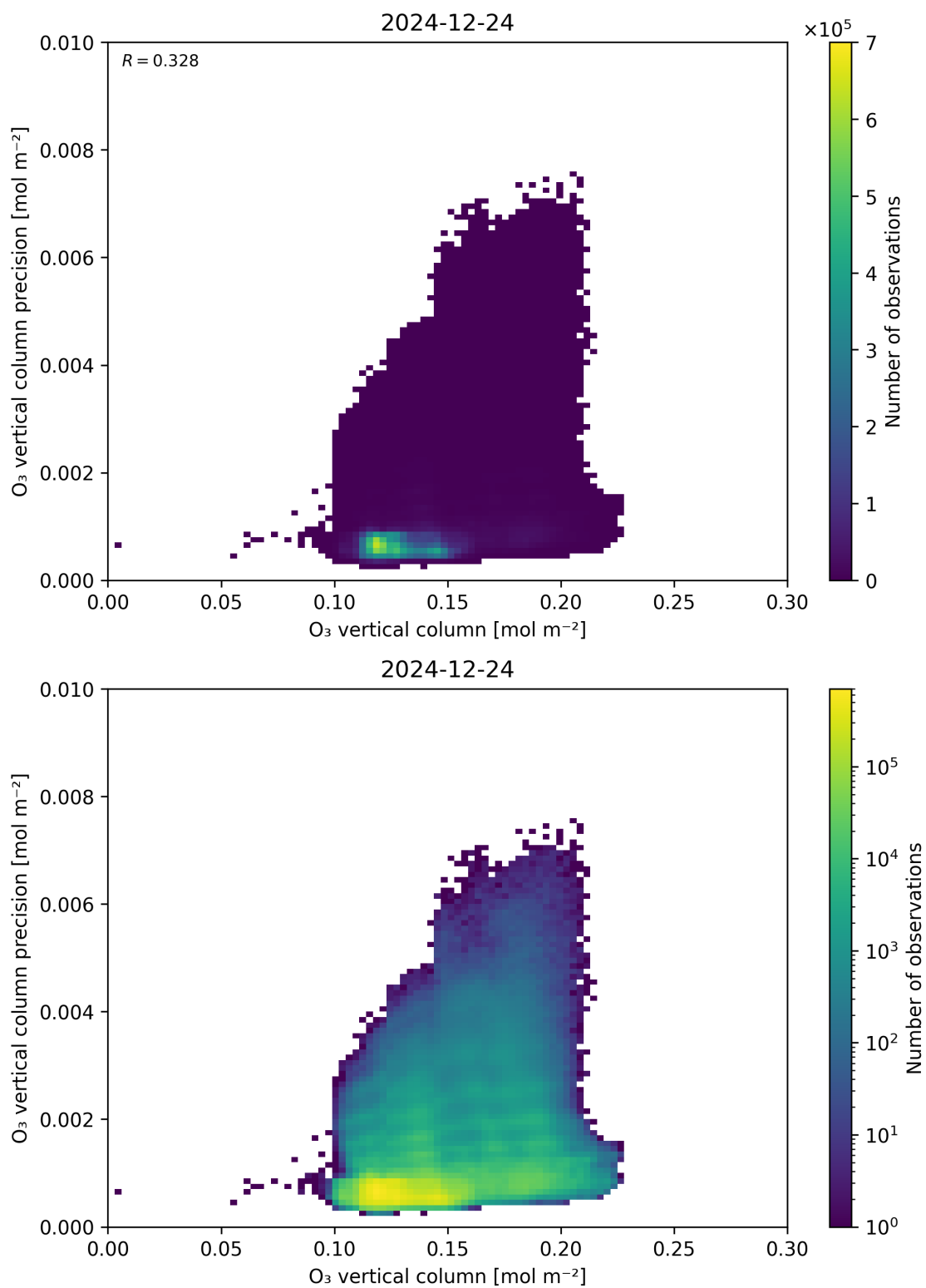
Figure 41: Scatter density plot of “O 3 vertical column” against “O 3 vertical column precision” for 2024-12-23 to 2024-12-25.
