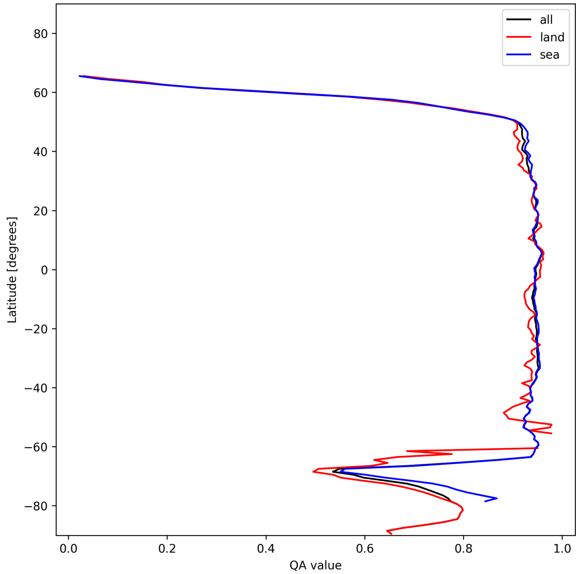
Figure 13: Zonal average of “QA value” for 2024-12-23 to 2024-12-25.
