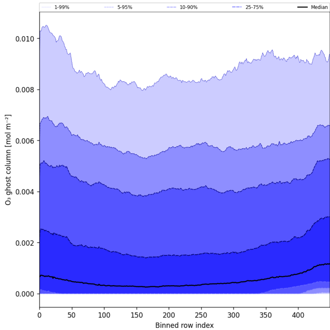
Figure 32: Along track statistics of “O 3 ghost column” for 2024-12-23 to 2024-12-25
