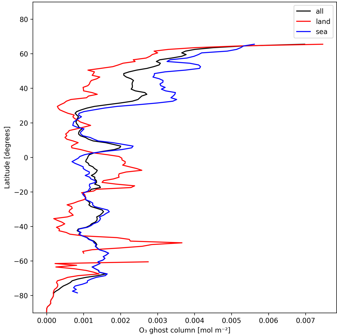
Figure 18: Zonal average of “O 3 ghost column” for 2024-12-23 to 2024-12-25.
