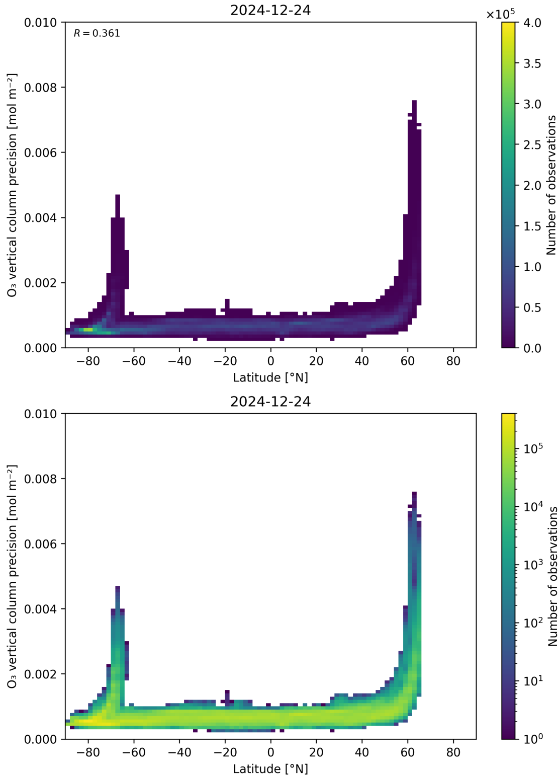
Figure 37: Scatter density plot of “Latitude” against “O 3 vertical column precision” for 2024-12-23 to 2024-12-25.
