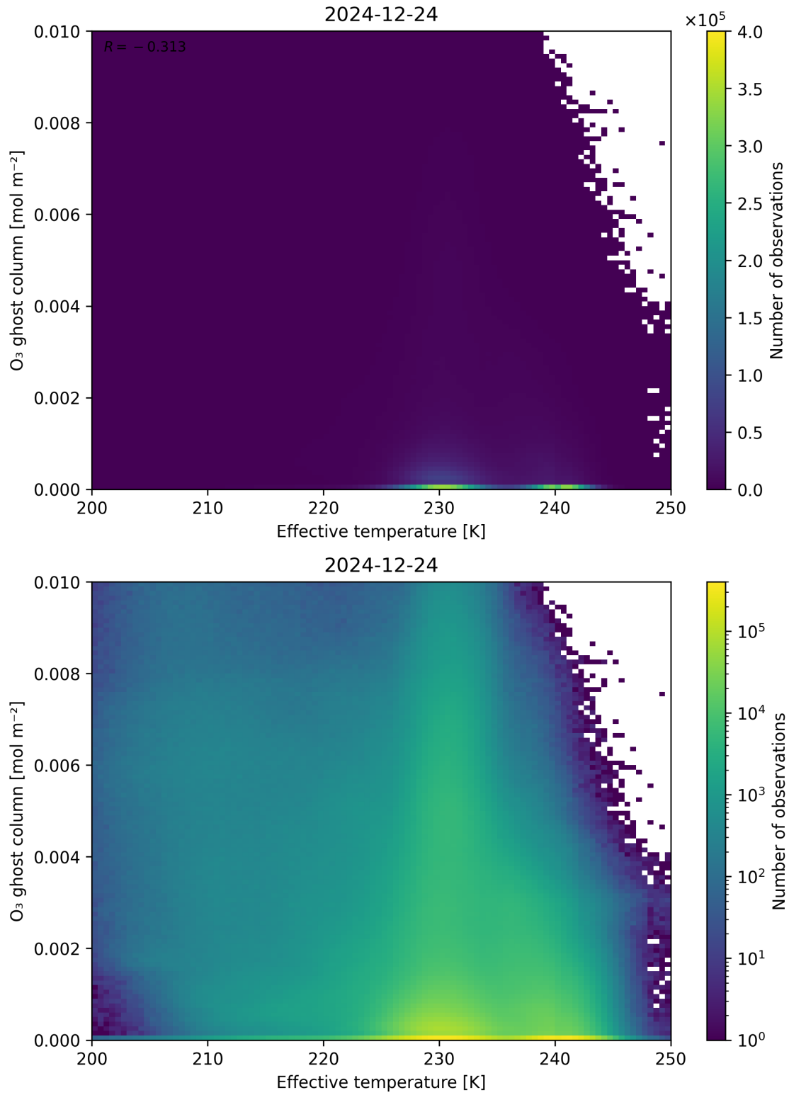
Figure 38: Scatter density plot of “Effective temperature” against “O 3 ghost column” for 2024-12-23 to 2024-12-25.
