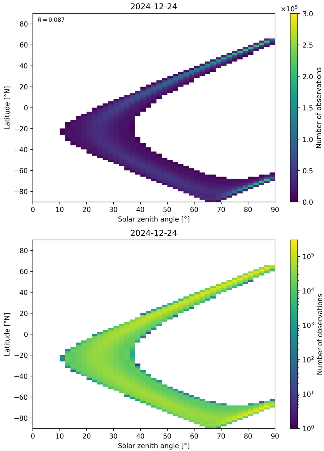
Figure 44: Scatter density plot of “Solar zenith angle” against “Latitude” for 2024-12-23 to 2024-12-25.
