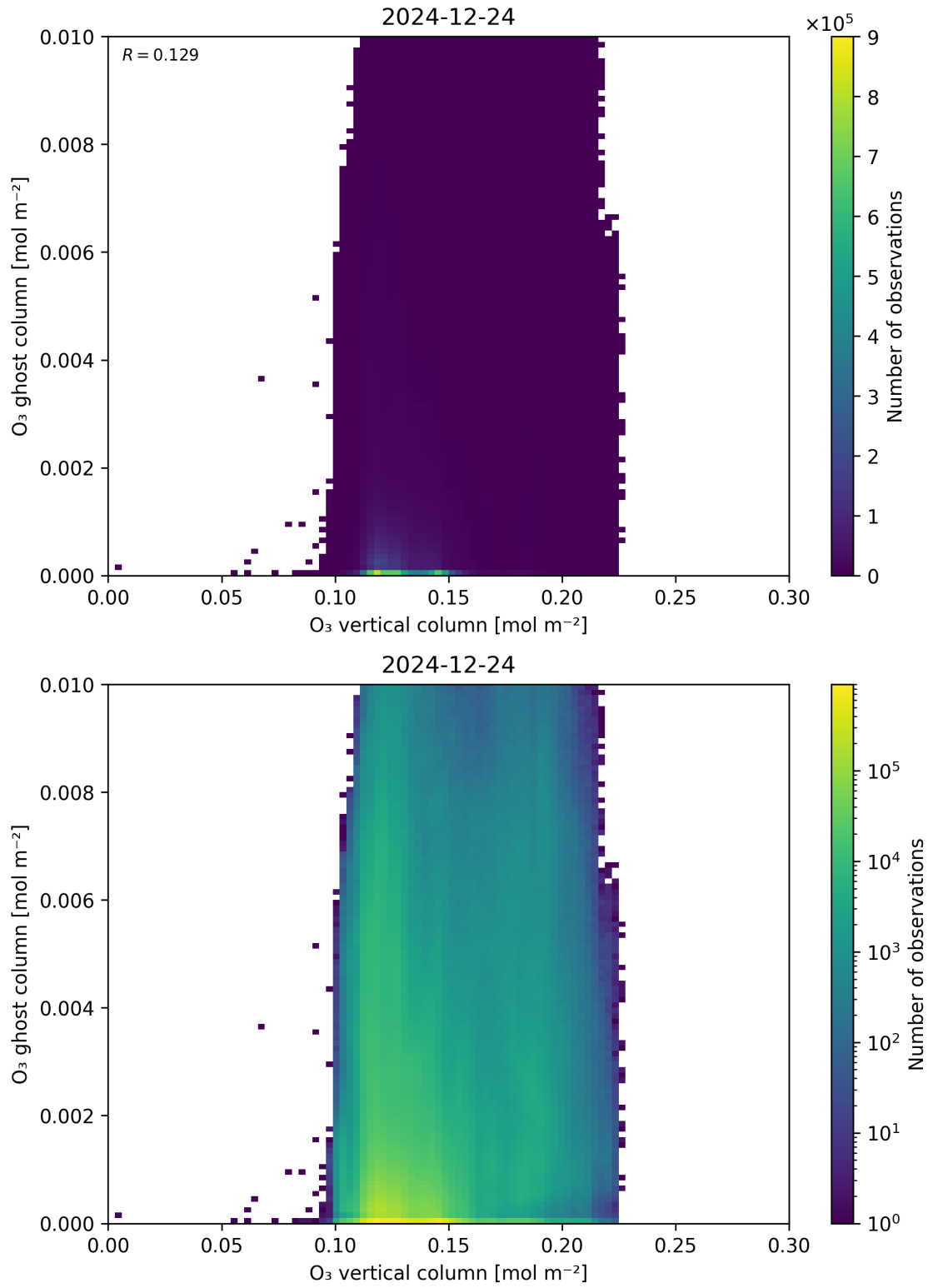
Figure 40: Scatter density plot of “O 3 vertical column” against “O 3 ghost column” for 2024-12-23 to 2024-12-25.
