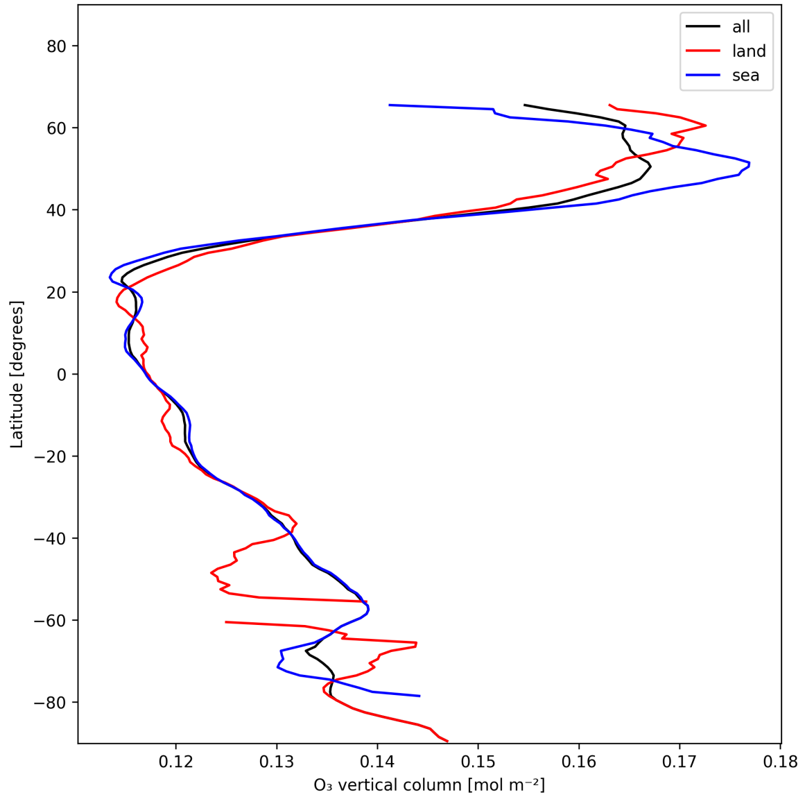
Figure 14: Zonal average of “O 3 vertical column” for 2024-12-23 to 2024-12-25.
