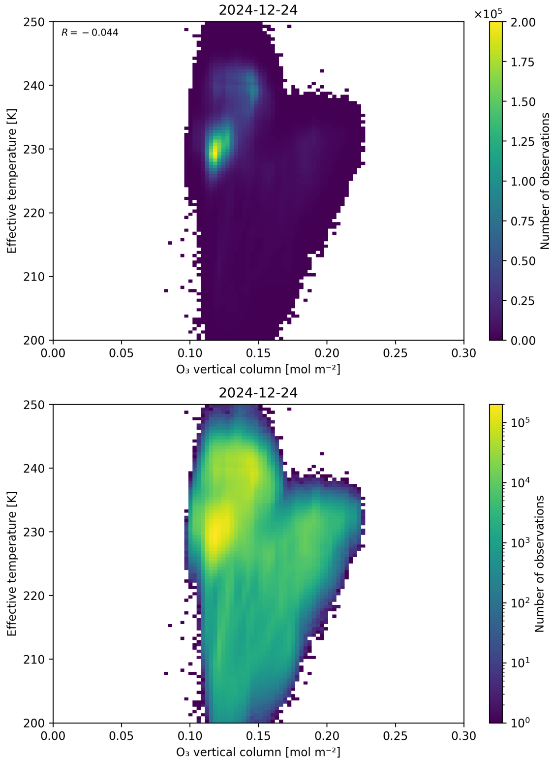
Figure 39: Scatter density plot of “O 3 vertical column” against “Effective temperature” for 2024-12-23 to 2024-12-25.
