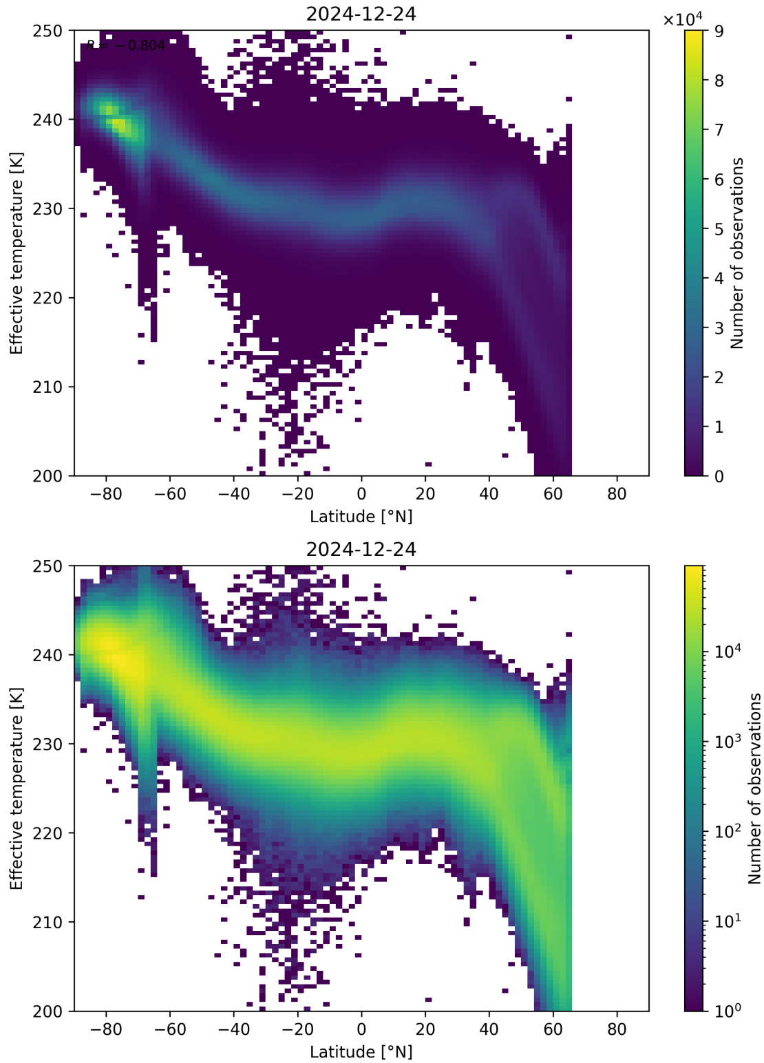
Figure 34: Scatter density plot of “Latitude” against “Effective temperature” for 2024-12-23 to 2024-12-25.
