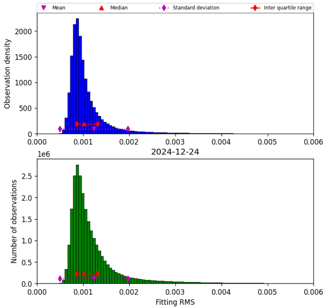
Figure 23: Histogram of “Fitting RMS” for 2024-12-23 to 2024-12-25
