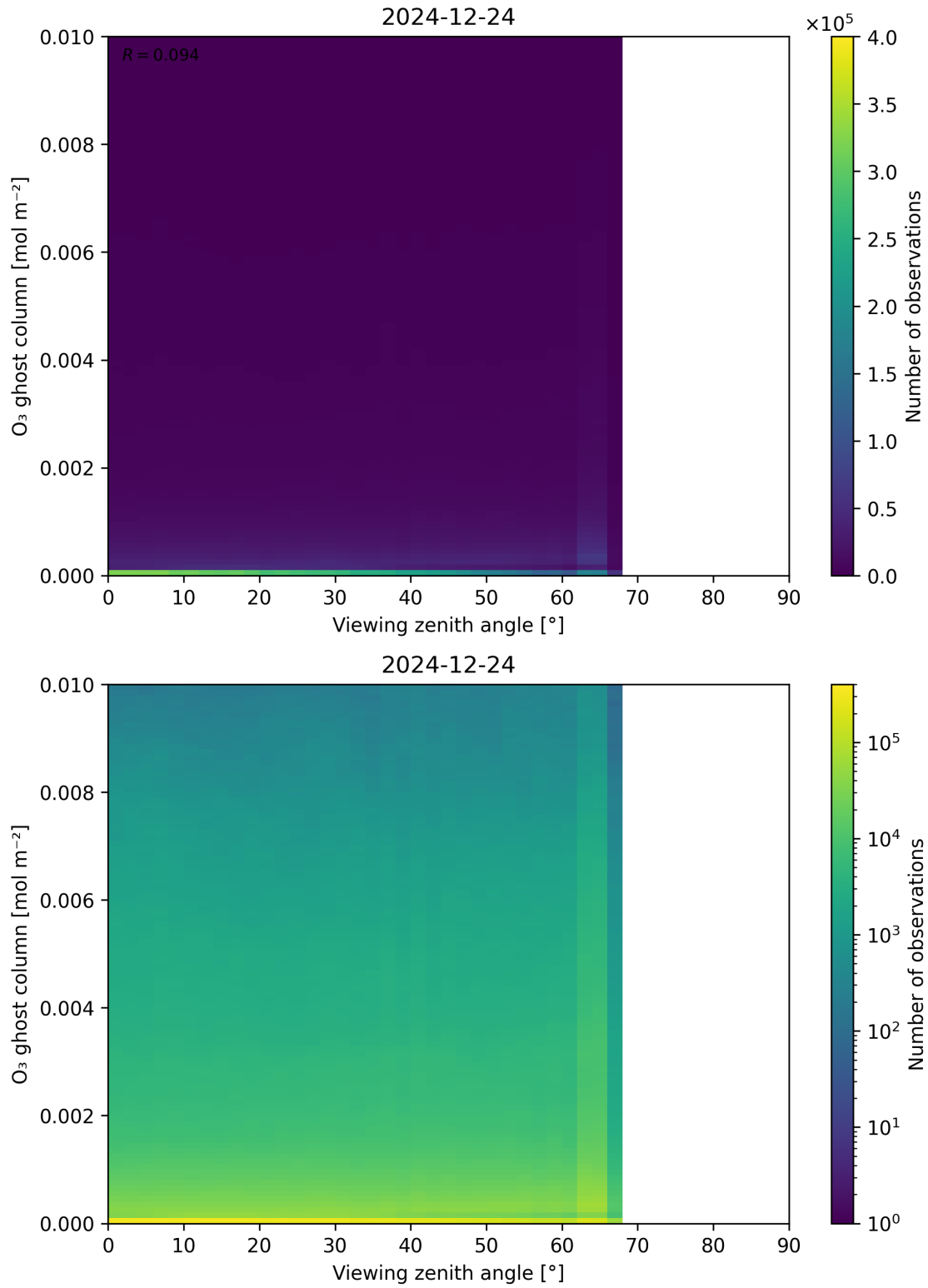
Figure 51: Scatter density plot of “Viewing zenith angle” against “O 3 ghost column” for 2024-12-23 to 2024-12-25.
