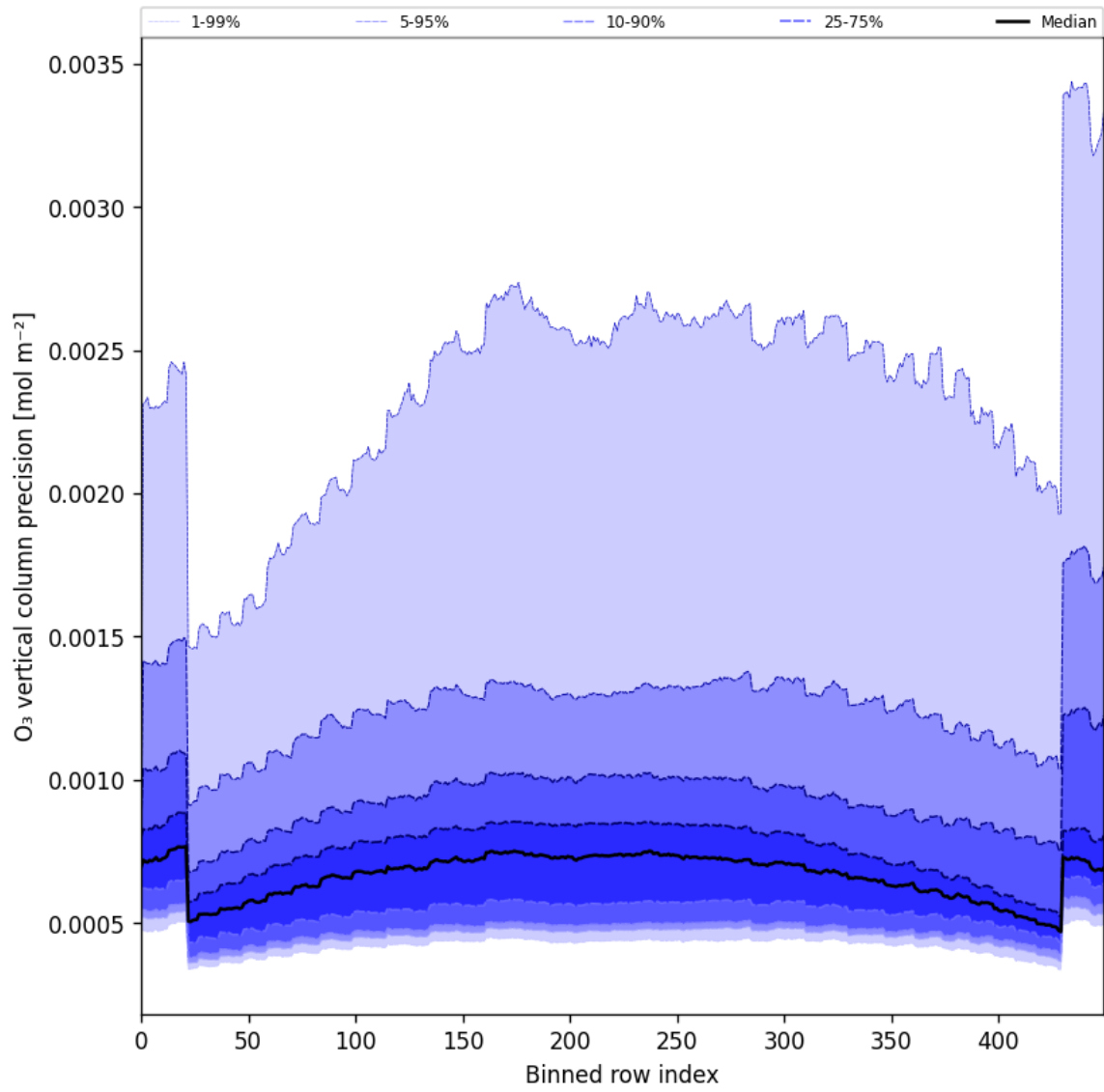
Figure 29: Along track statistics of “O 3 vertical column precision” for 2024-12-23 to 2024-12-25
