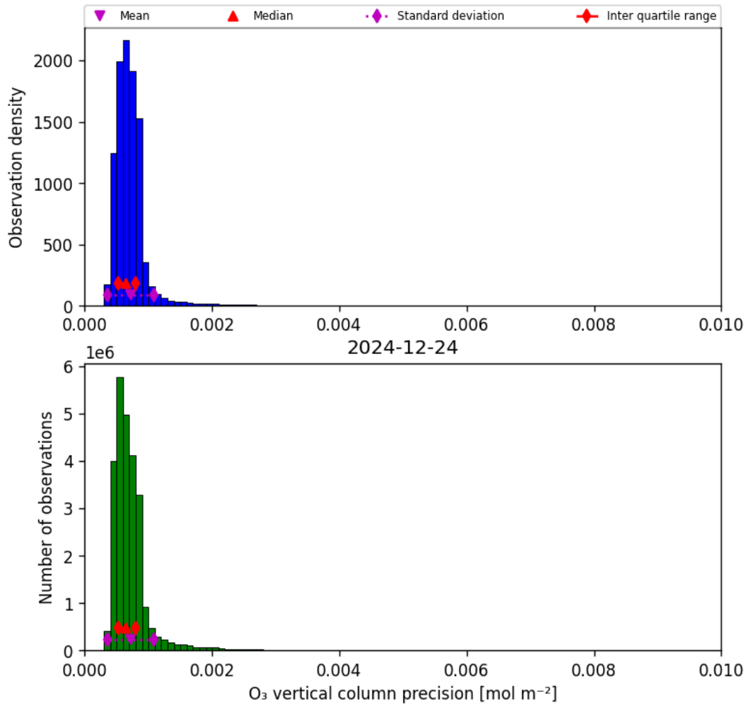
Figure 22: Histogram of “O 3 vertical column precision” for 2024-12-23 to 2024-12-25
