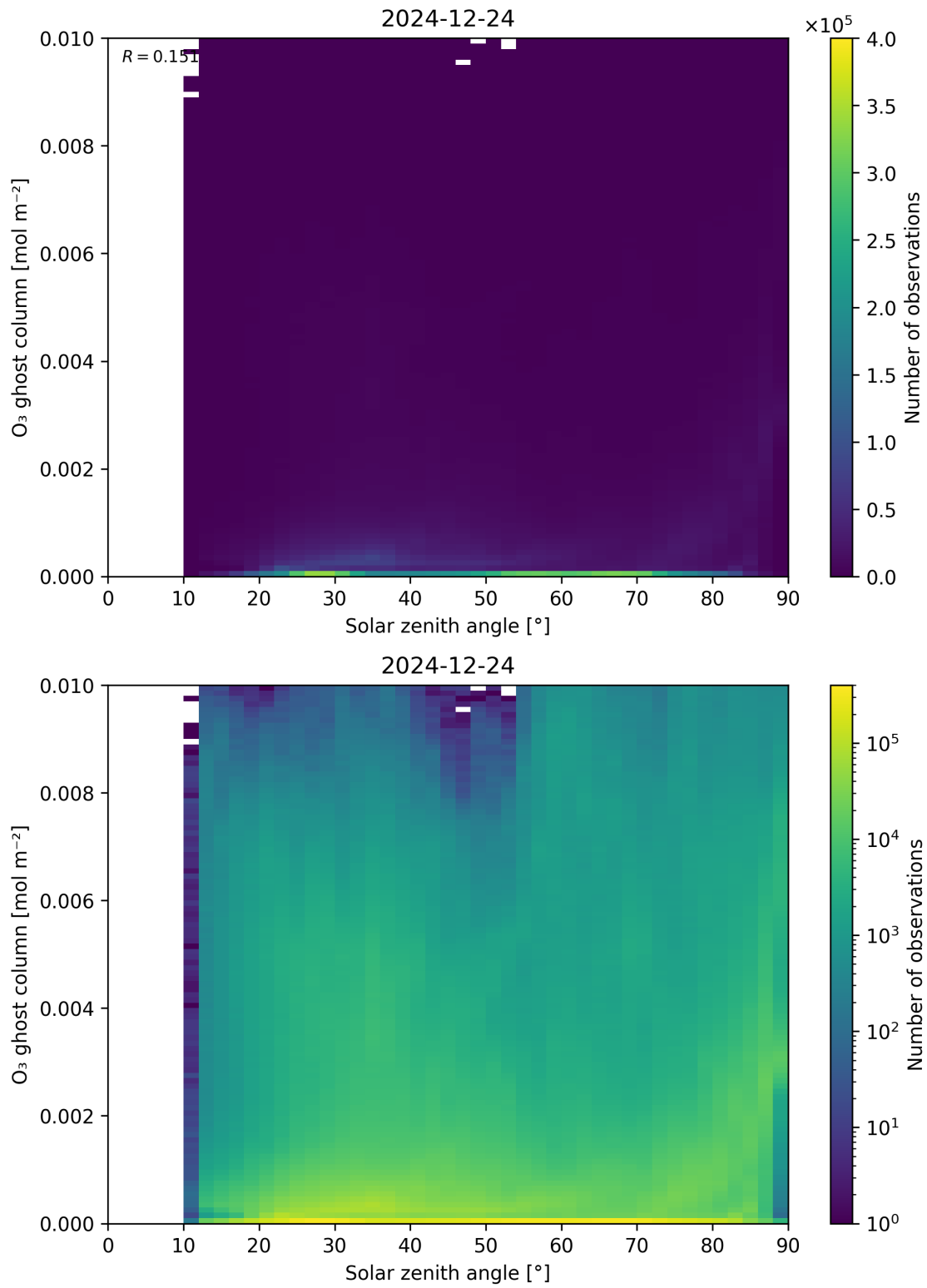
Figure 46: Scatter density plot of “Solar zenith angle” against “O 3 ghost column” for 2024-12-23 to 2024-12-25.
