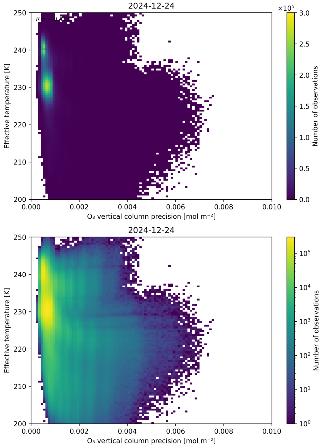
Figure 42: Scatter density plot of “O 3 vertical column precision” against “Effective temperature” for 2024-12-23 to 2024-12-25.
