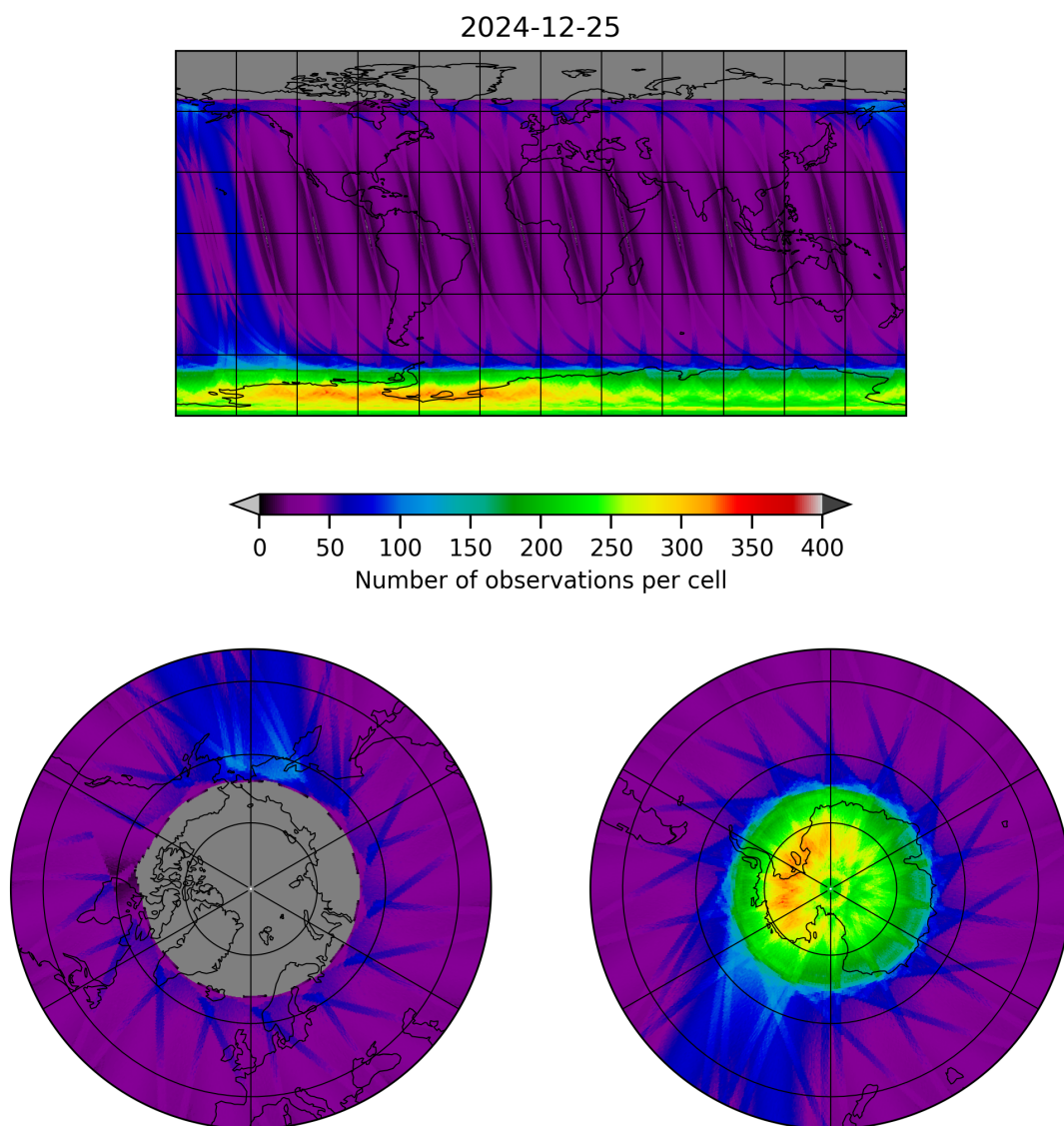
Figure 12: Map of the number of observations for 2024-12-24 to 2024-12-26
