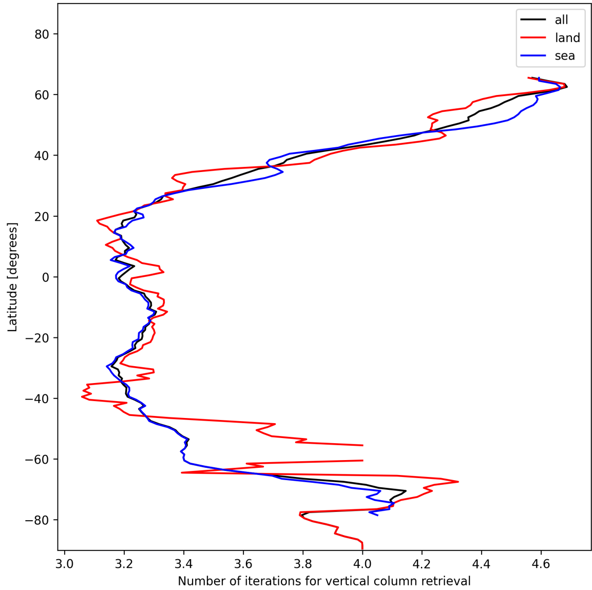
Figure 19: Zonal average of “Number of iterations for vertical column retrieval” for 2024-12-24 to 2024-12-26.
