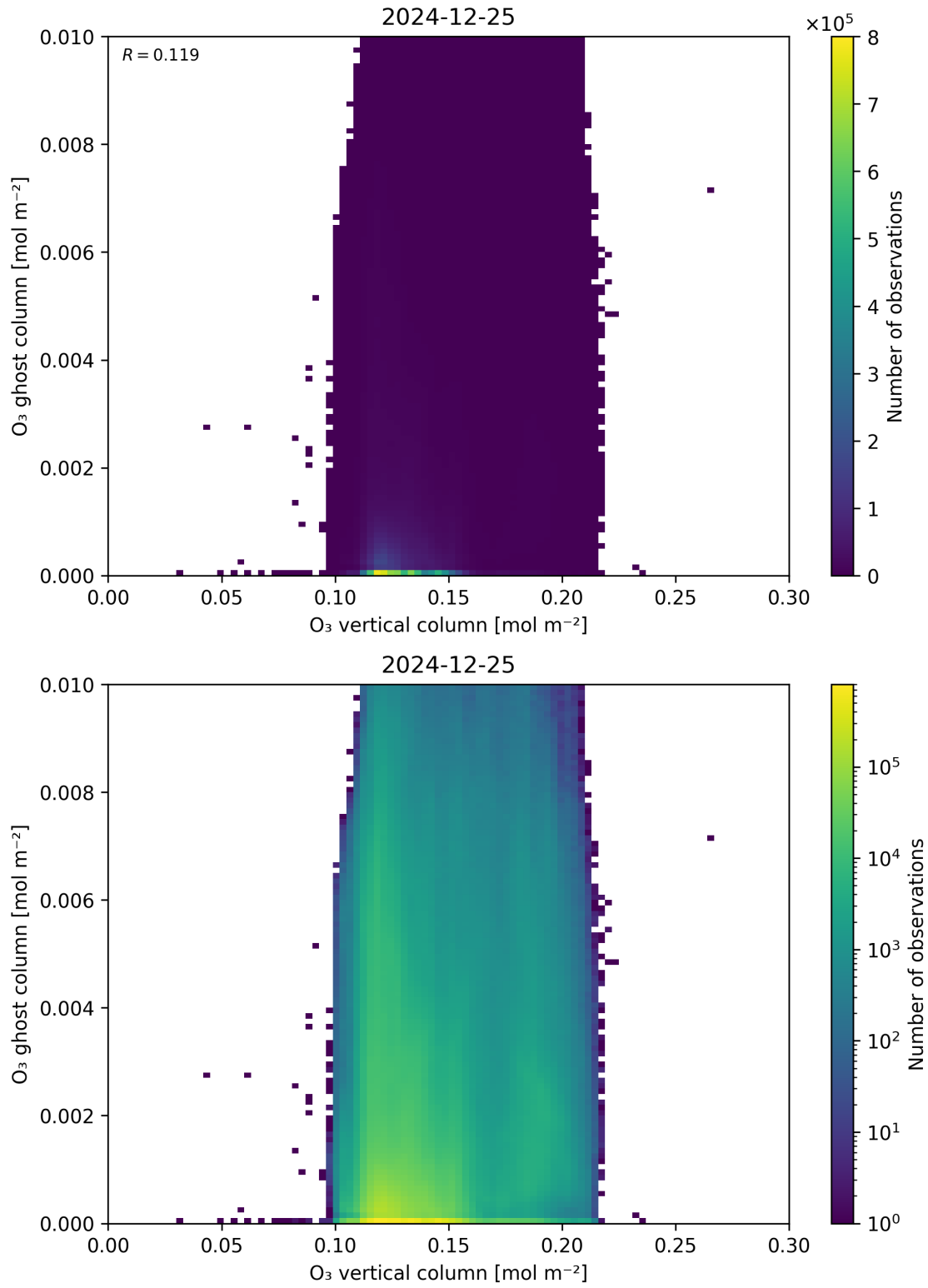
Figure 40: Scatter density plot of “O 3 vertical column” against “O 3 ghost column” for 2024-12-24 to 2024-12-26.
