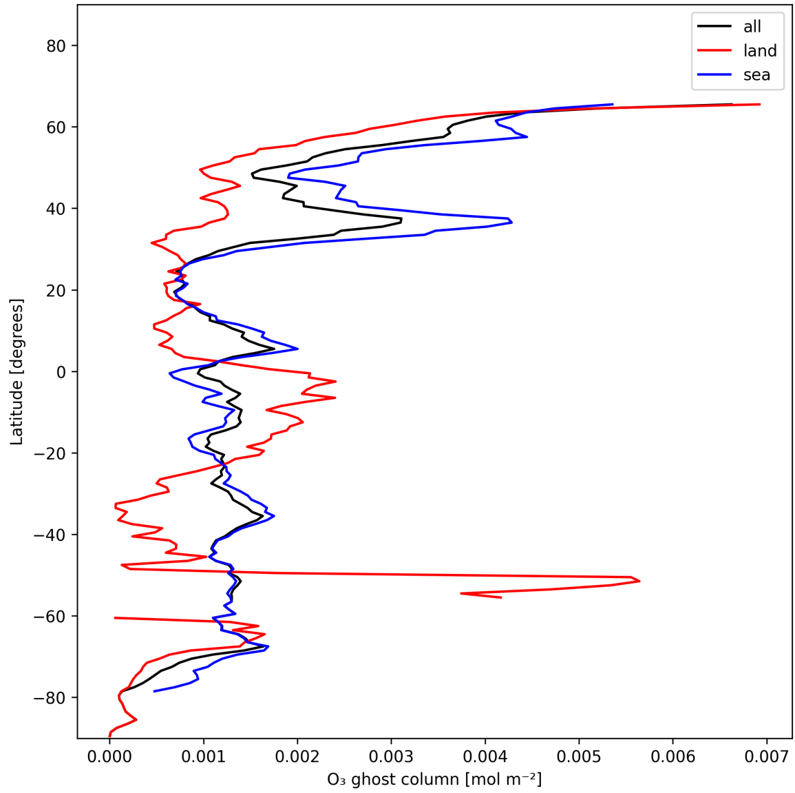
Figure 18: Zonal average of "O 3 ghost column" for 2024-12-24 to 2024-12-26.
