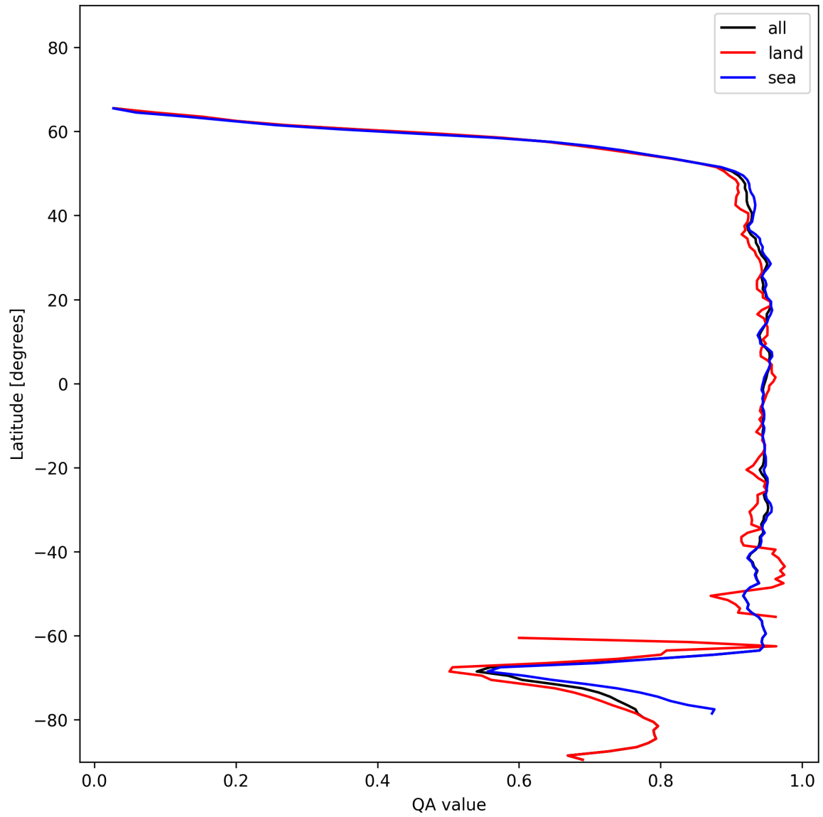
Figure 13: Zonal average of “QA value” for 2024-12-24 to 2024-12-26.
