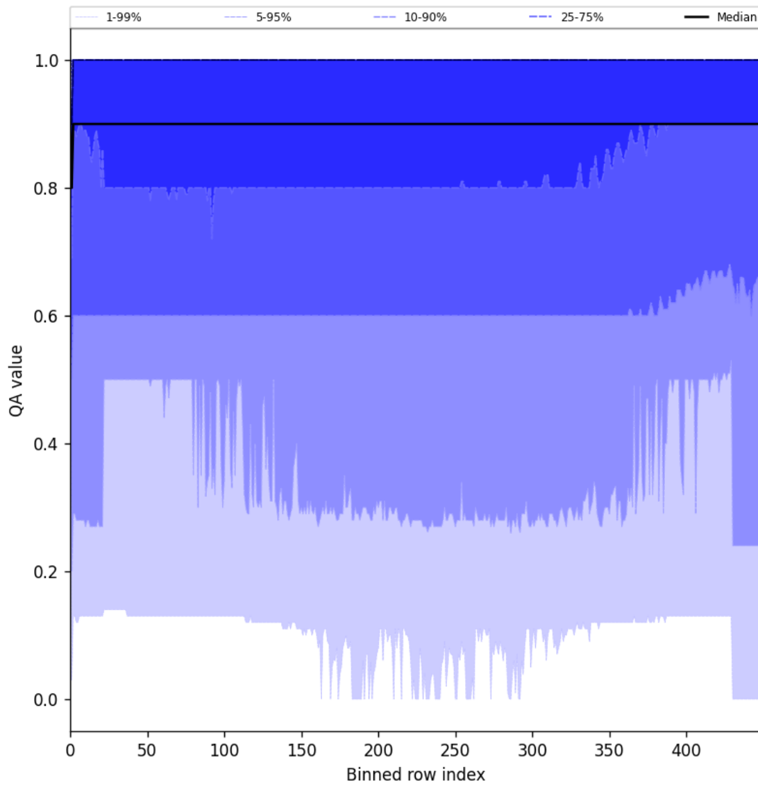
Figure 27: Along track statistics of “QA value” for 2024-12-24 to 2024-12-26
