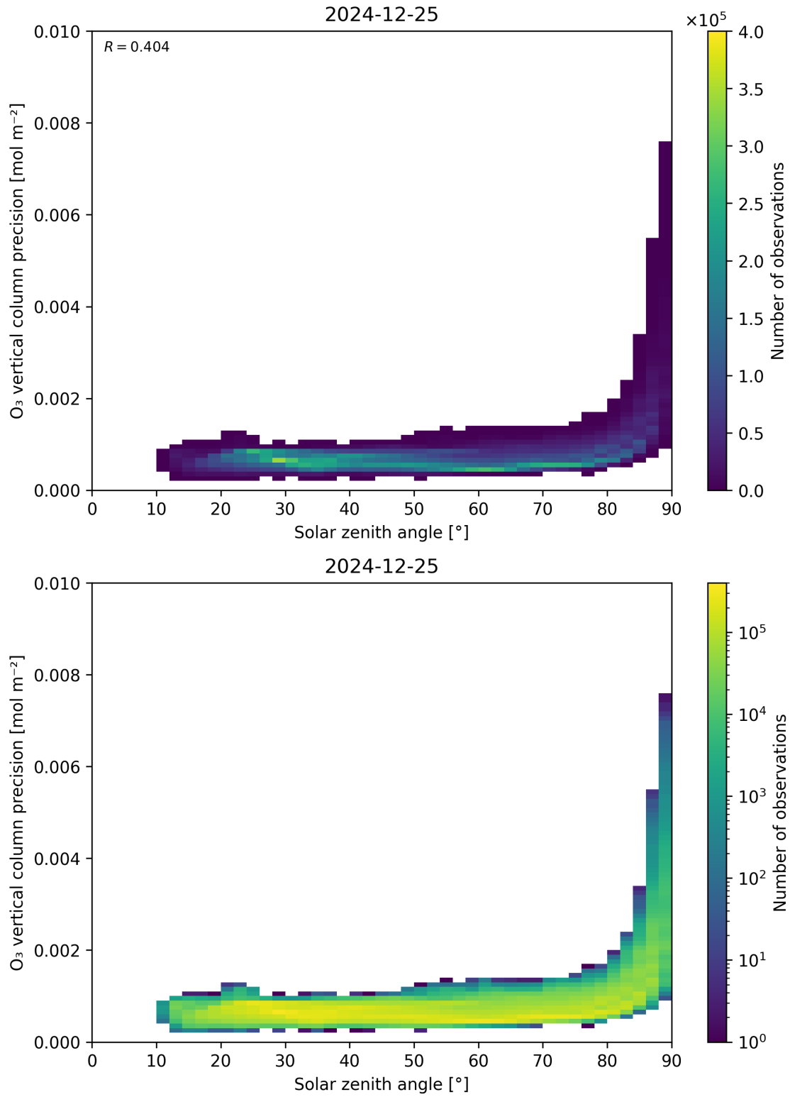
Figure 48: Scatter density plot of “Solar zenith angle” against “O 3 vertical column precision” for 2024-12-24 to 2024-12-26.
