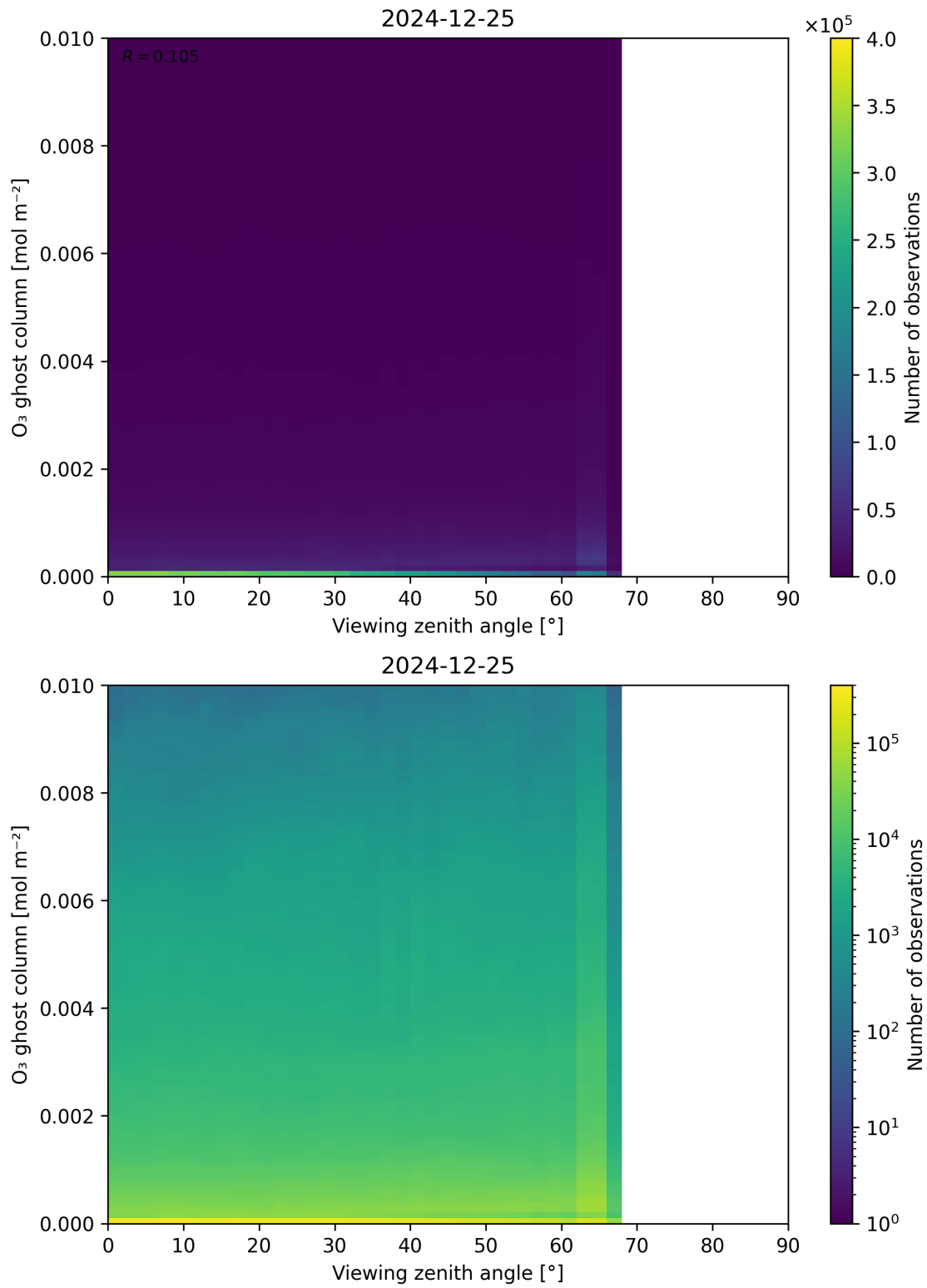
Figure 51: Scatter density plot of “Viewing zenith angle” against “O 3 ghost column” for 2024-12-24 to 2024-12-26.
