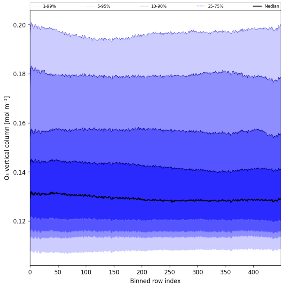
Figure 28: Along track statistics of “O 3 vertical column” for 2024-12-24 to 2024-12-26
