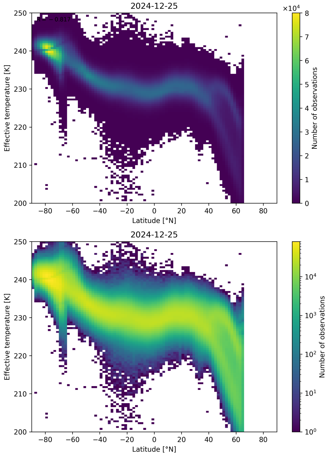
Figure 34: Scatter density plot of “Latitude” against “Effective temperature” for 2024-12-24 to 2024-12-26.
