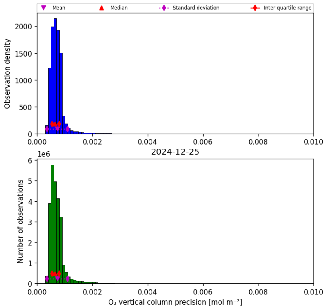
Figure 22: Histogram of “O 3 vertical column precision” for 2024-12-24 to 2024-12-26
