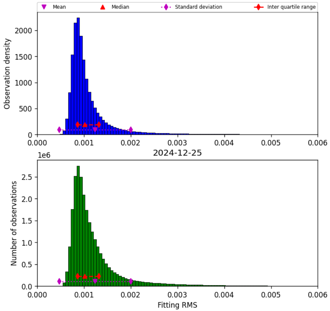
Figure 23: Histogram of “Fitting RMS” for 2024-12-24 to 2024-12-26
