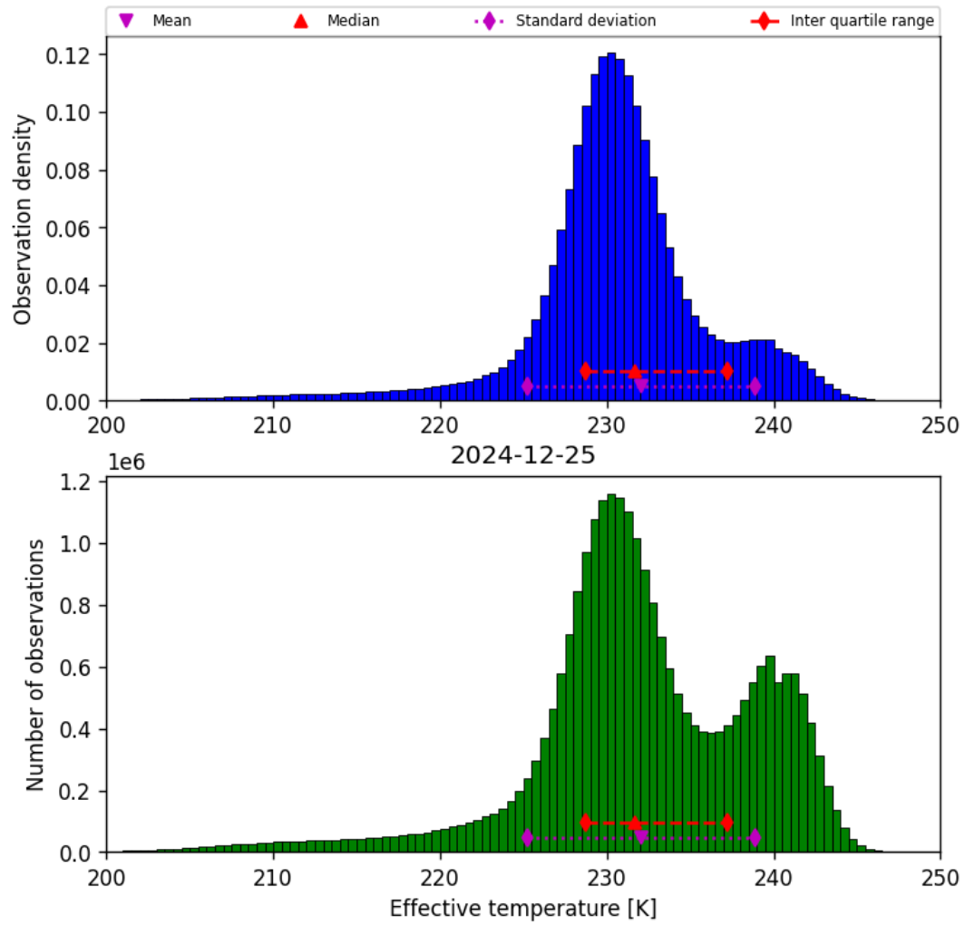
Figure 24: Histogram of “Effective temperature” for 2024-12-24 to 2024-12-26
