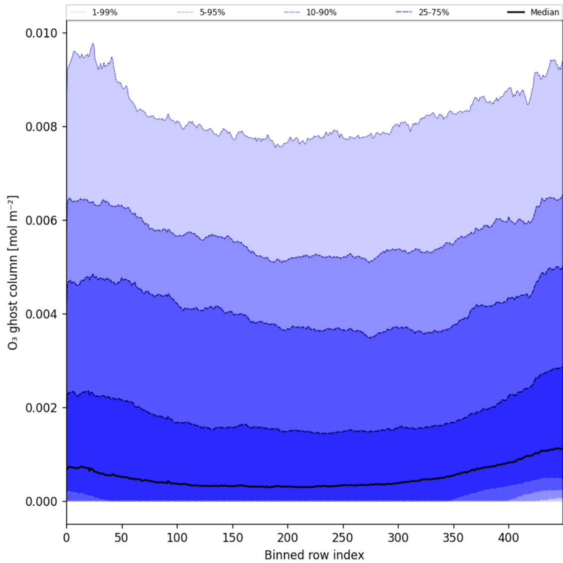
Figure 32: Along track statistics of “O 3 ghost column” for 2024-12-24 to 2024-12-26
