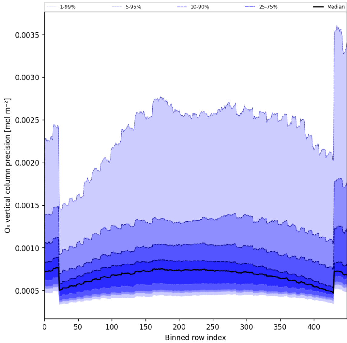
Figure 29: Along track statistics of “O 3 vertical column precision” for 2024-12-24 to 2024-12-26
