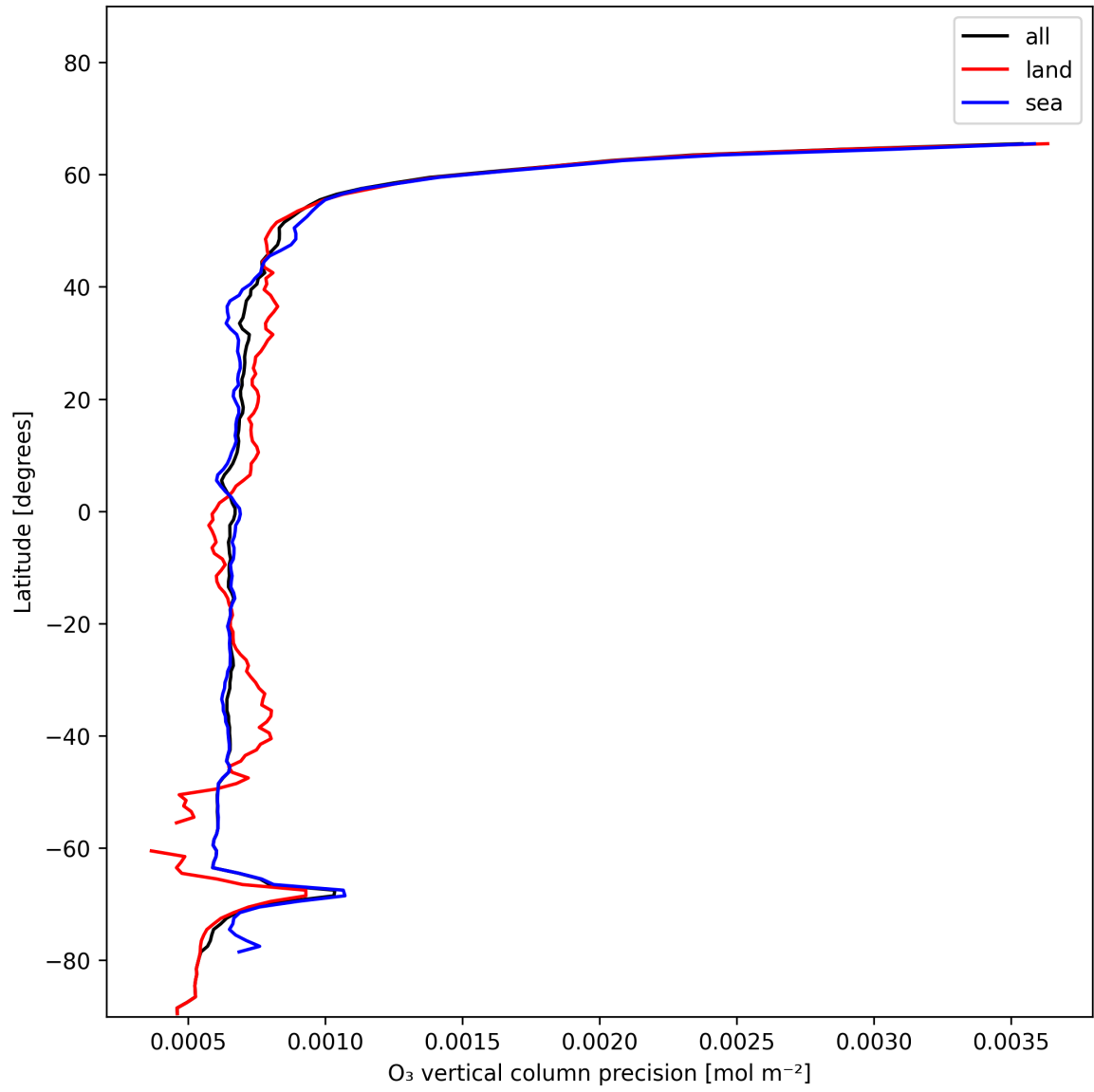
Figure 15: Zonal average of “O 3 vertical column precision” for 2024-12-24 to 2024-12-26.
