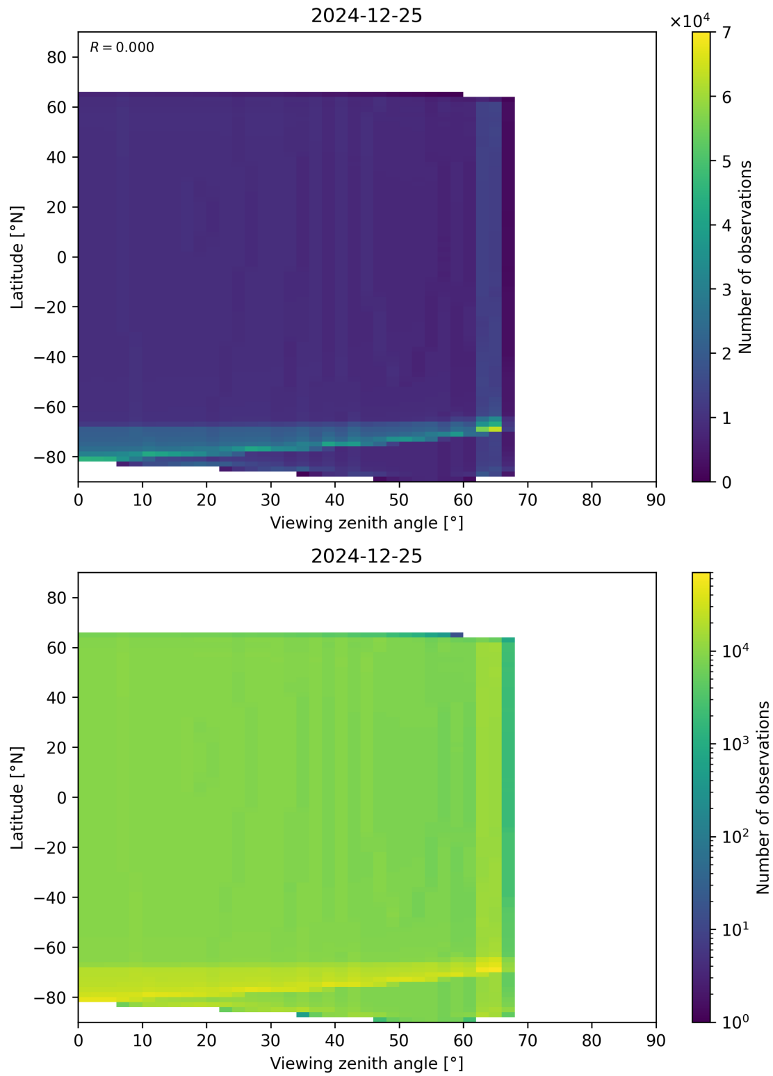
Figure 49: Scatter density plot of “Viewing zenith angle” against “Latitude” for 2024-12-24 to 2024-12-26.
