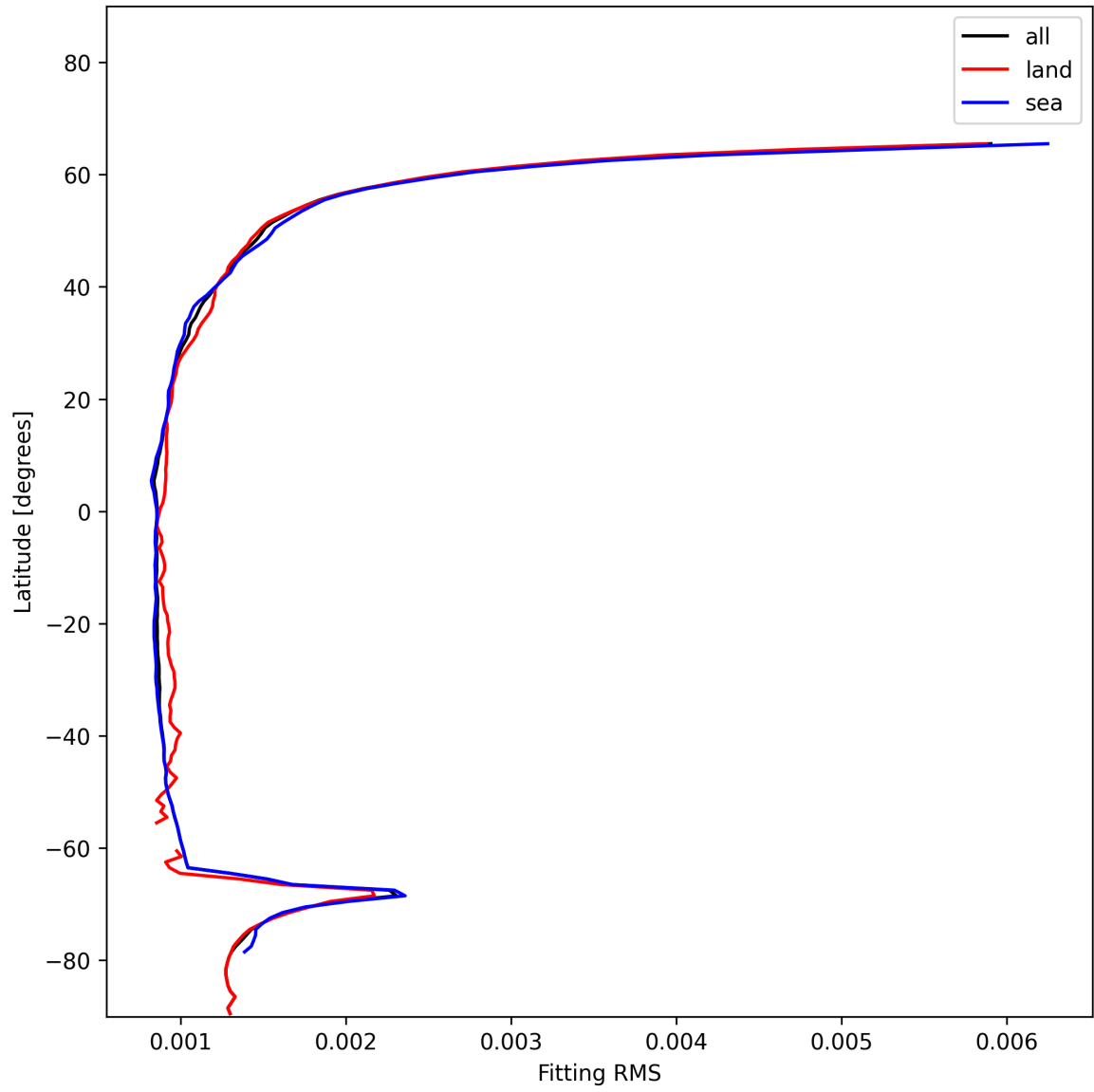
Figure 16: Zonal average of “Fitting RMS” for 2024-12-24 to 2024-12-26.
