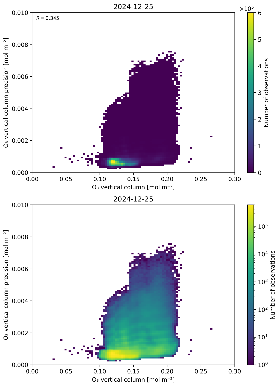
Figure 41: Scatter density plot of “O 3 vertical column” against “O 3 vertical column precision” for 2024-12-24 to 2024-12-26.
