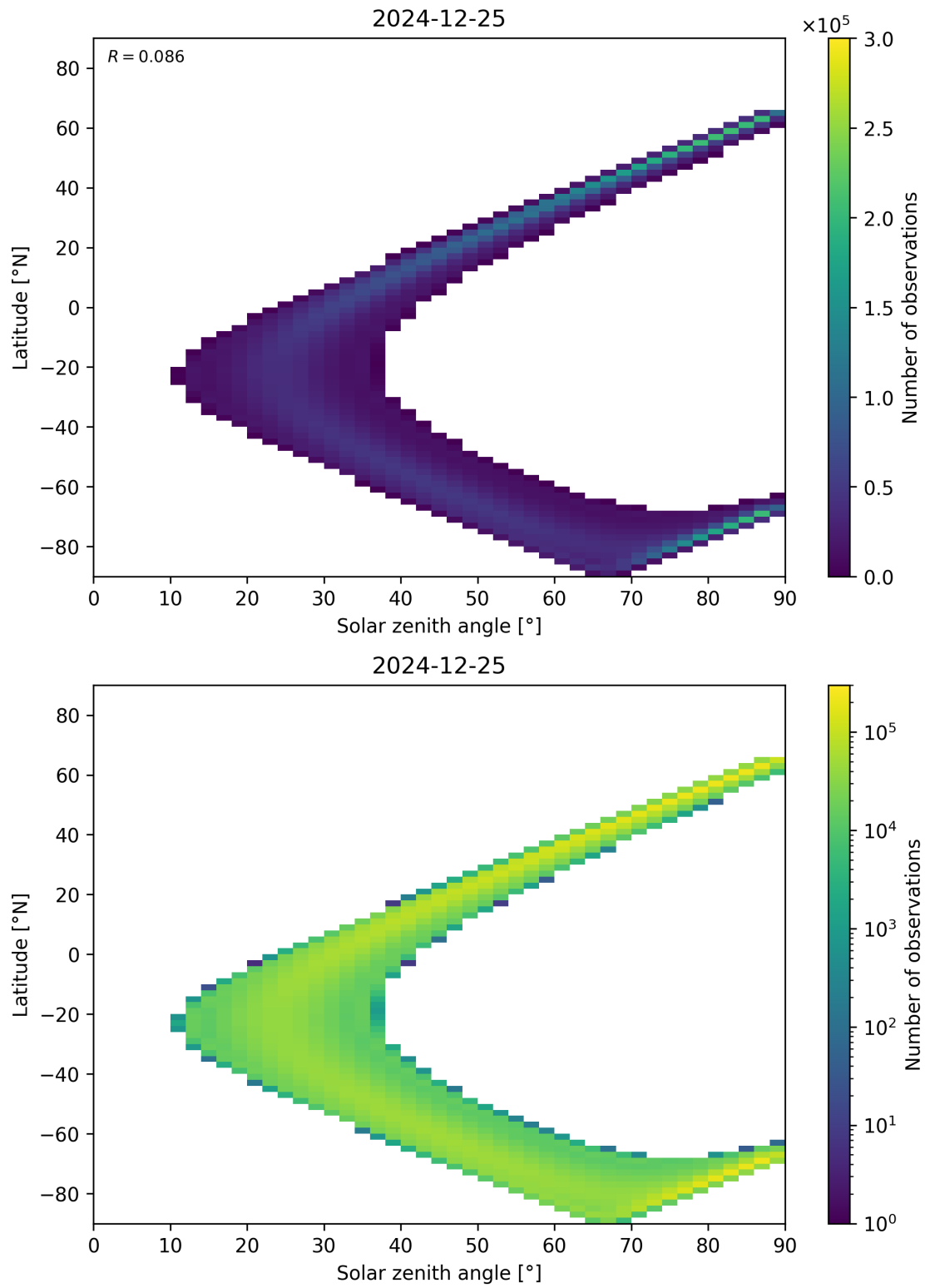
Figure 44: Scatter density plot of “Solar zenith angle” against “Latitude” for 2024-12-24 to 2024-12-26.
