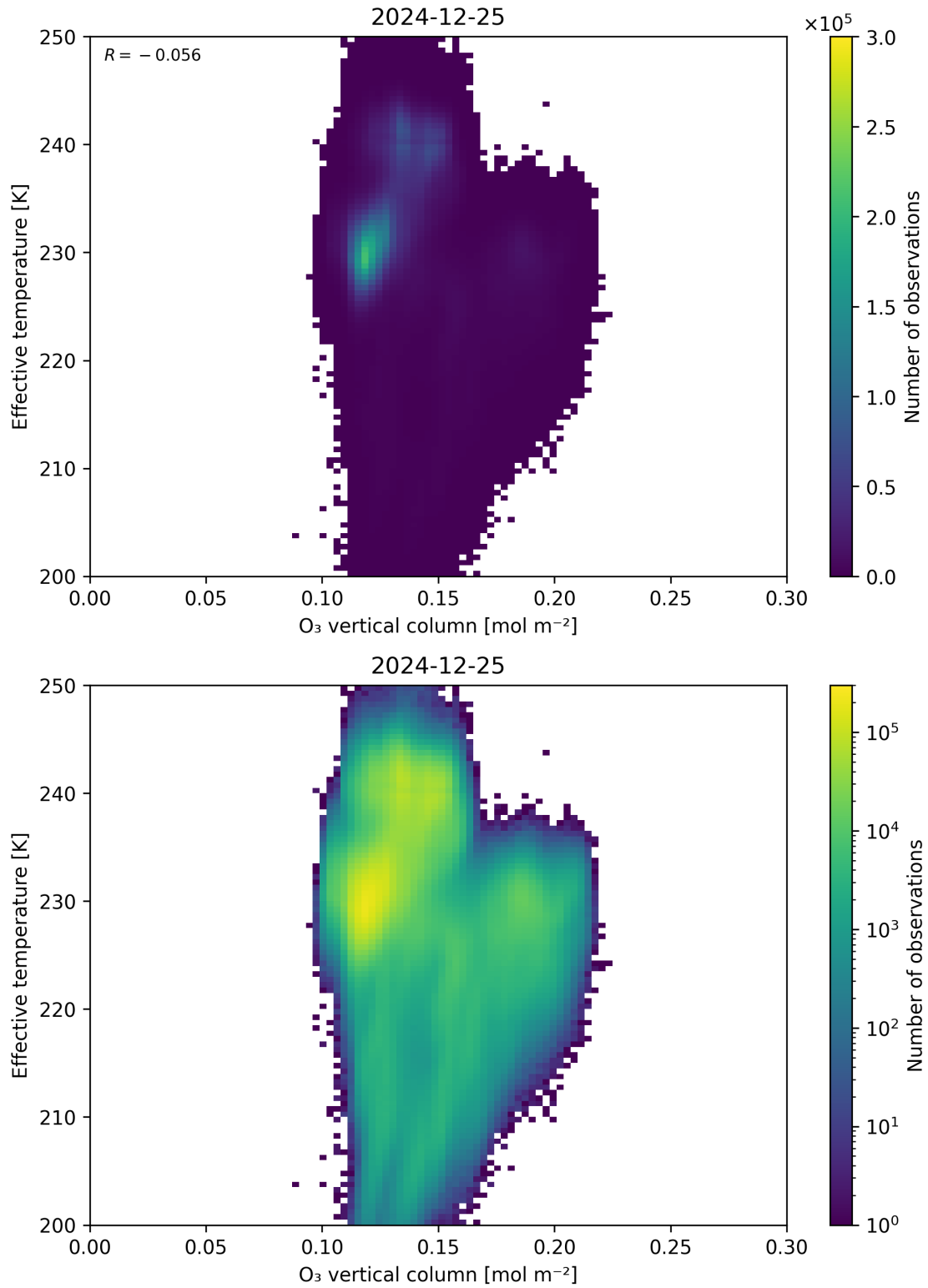
Figure 39: Scatter density plot of “O 3 vertical column” against “Effective temperature” for 2024-12-24 to 2024-12-26.
