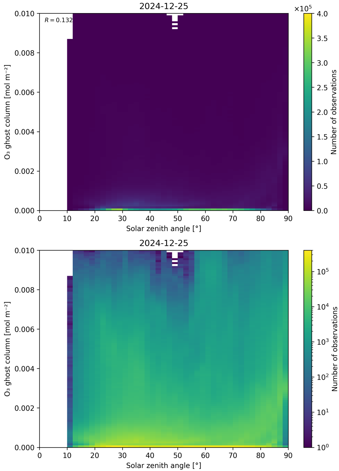
Figure 46: Scatter density plot of “Solar zenith angle” against “O 3 ghost column” for 2024-12-24 to 2024-12-26.
