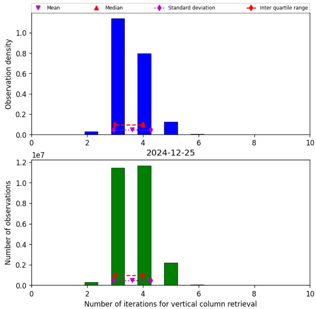
Figure 26: Histogram of “Number of iterations for vertical column retrieval” for 2024-12-24 to 2024-12-26
