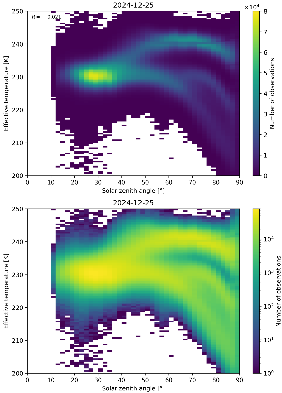
Figure 45: Scatter density plot of “Solar zenith angle” against “Effective temperature” for 2024-12-24 to 2024-12-26.
