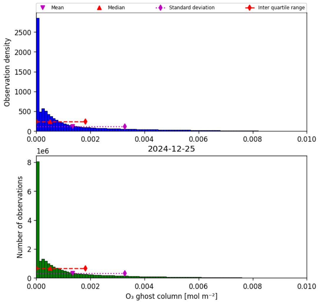
Figure 25: Histogram of “O 3 ghost column” for 2024-12-24 to 2024-12-26
