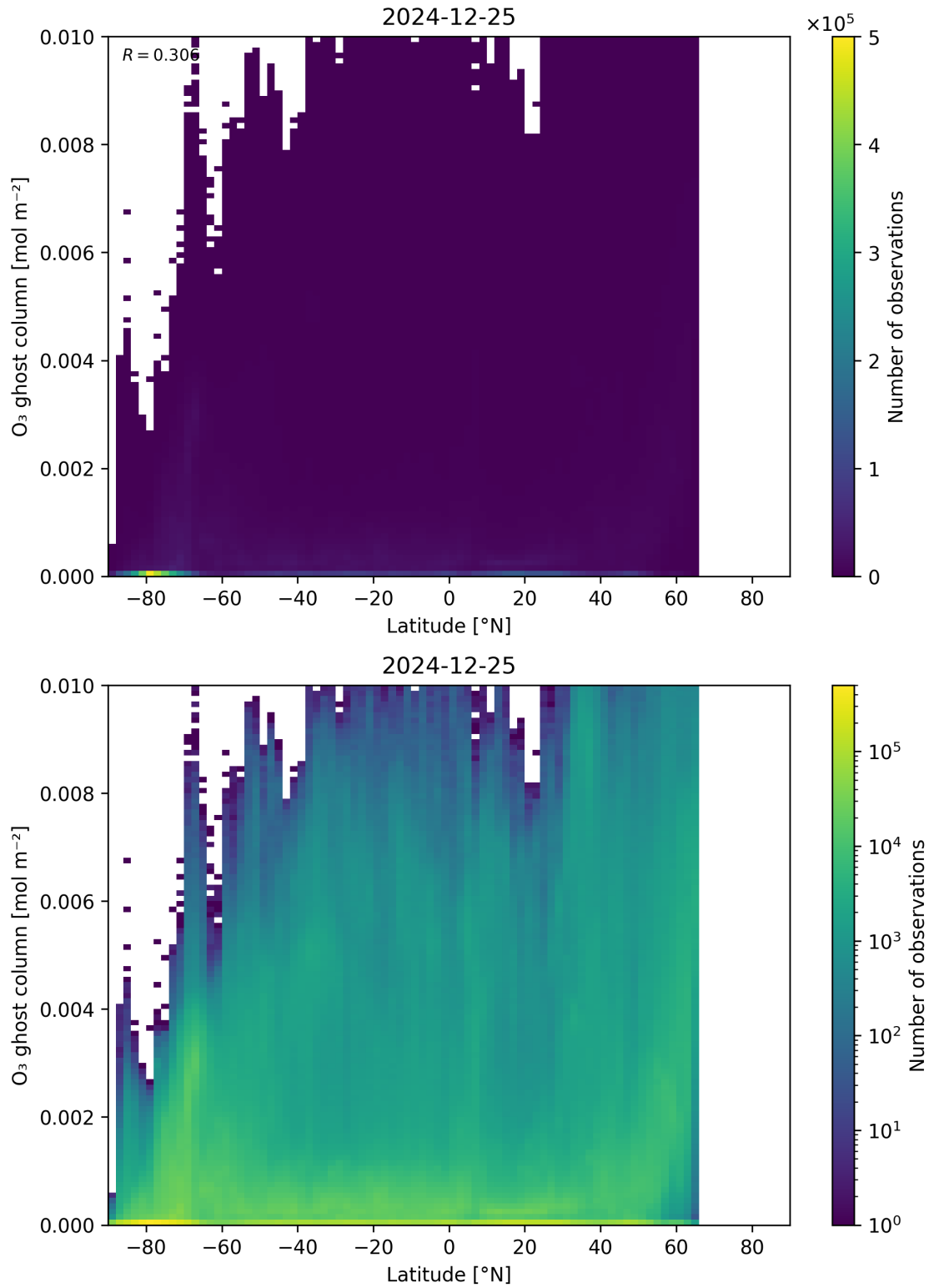
Figure 35: Scatter density plot of “Latitude” against “O 3 ghost column” for 2024-12-24 to 2024-12-26.
