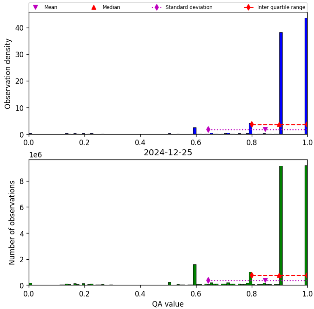
Figure 20: Histogram of “QA value” for 2024-12-24 to 2024-12-26
