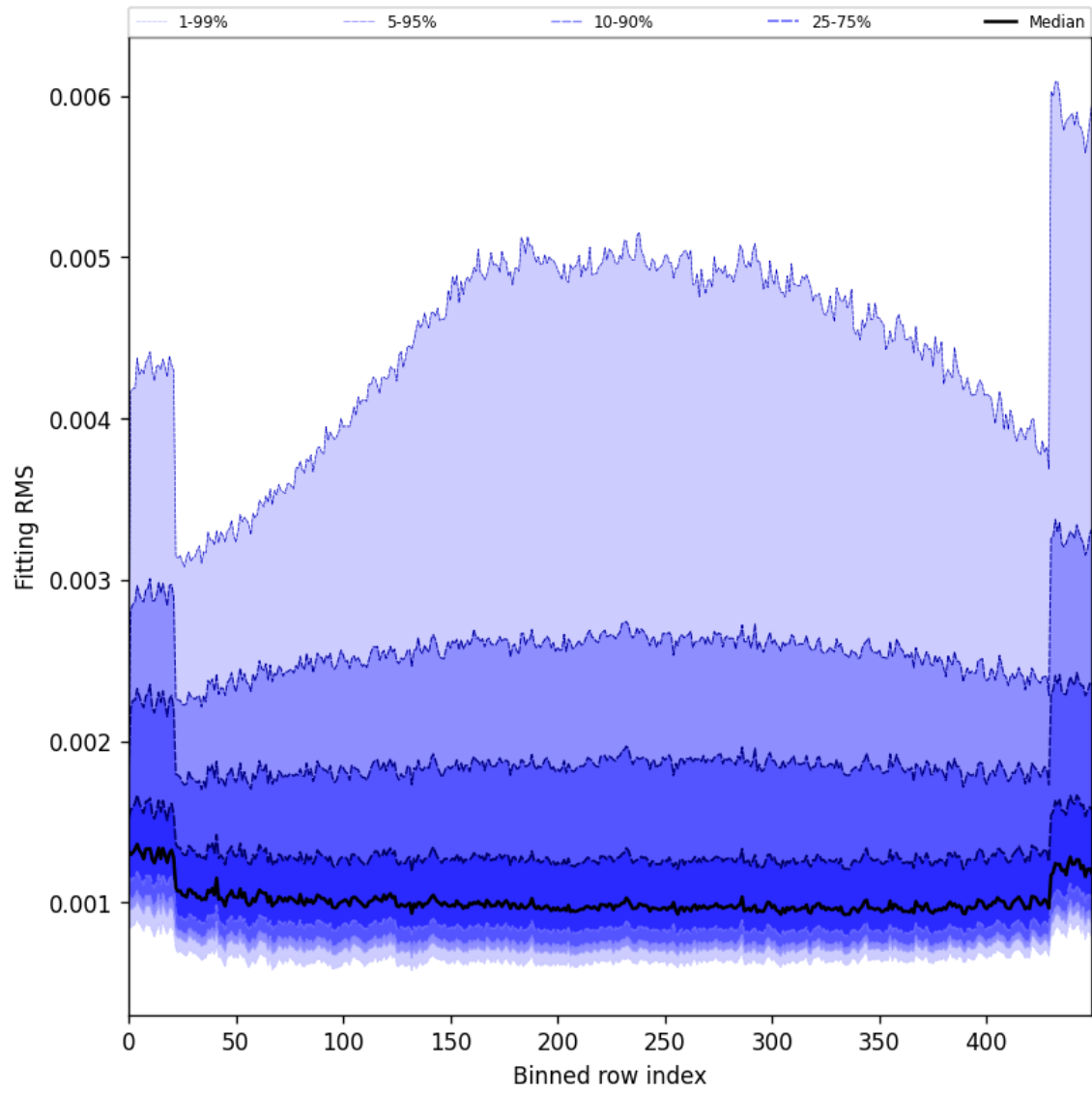
Figure 30: Along track statistics of “Fitting RMS” for 2024-12-24 to 2024-12-26
