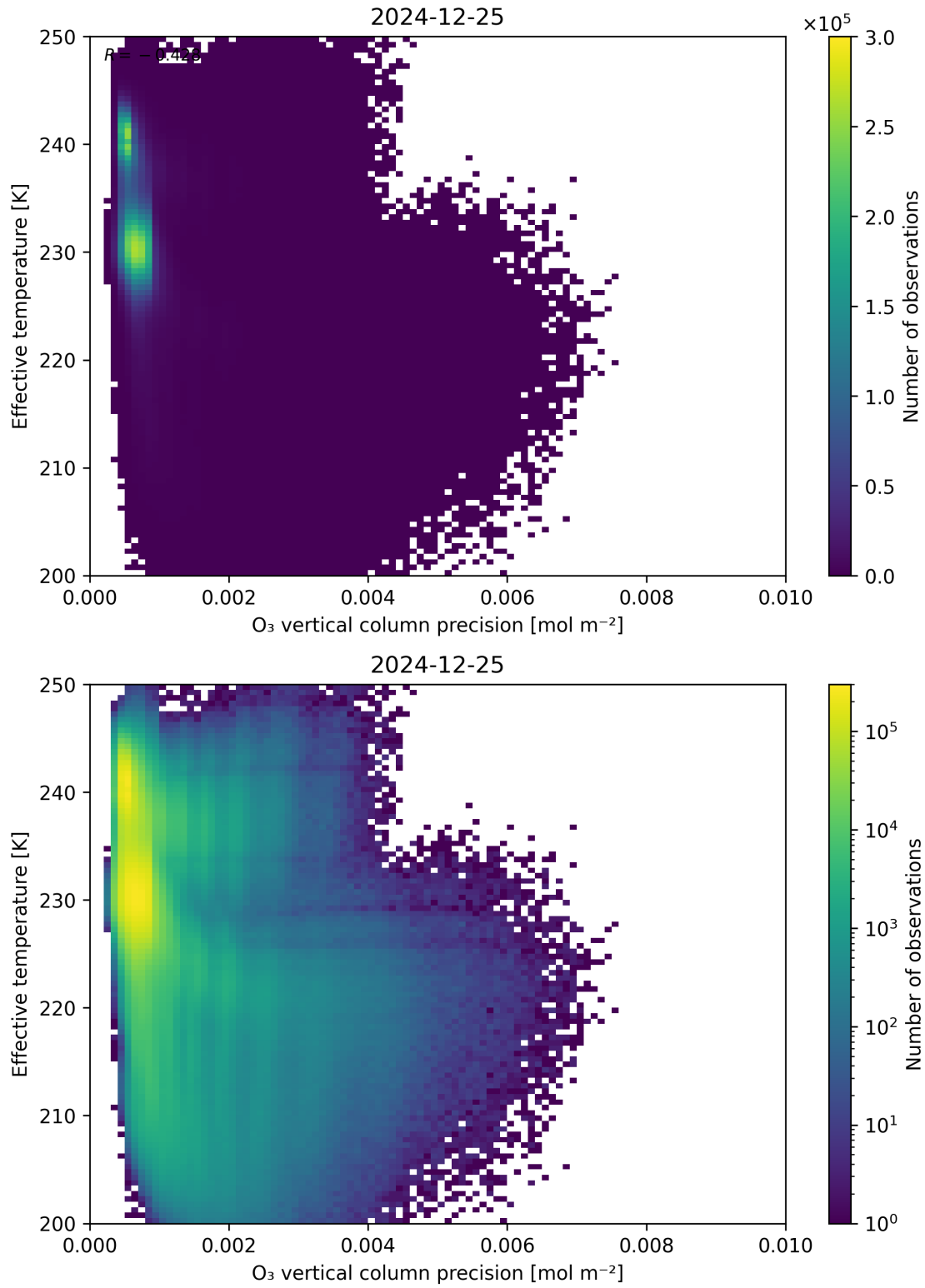
Figure 42: Scatter density plot of “O 3 vertical column precision” against “Effective temperature” for 2024-12-24 to 2024-12-26.
