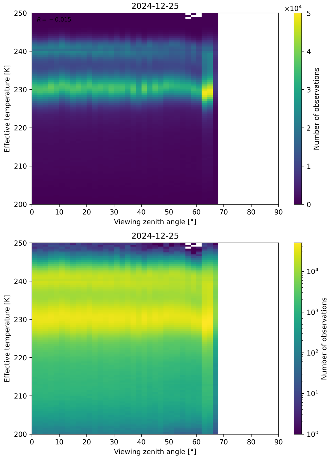
Figure 50: Scatter density plot of “Viewing zenith angle” against “Effective temperature” for 2024-12-24 to 2024-12-26.
