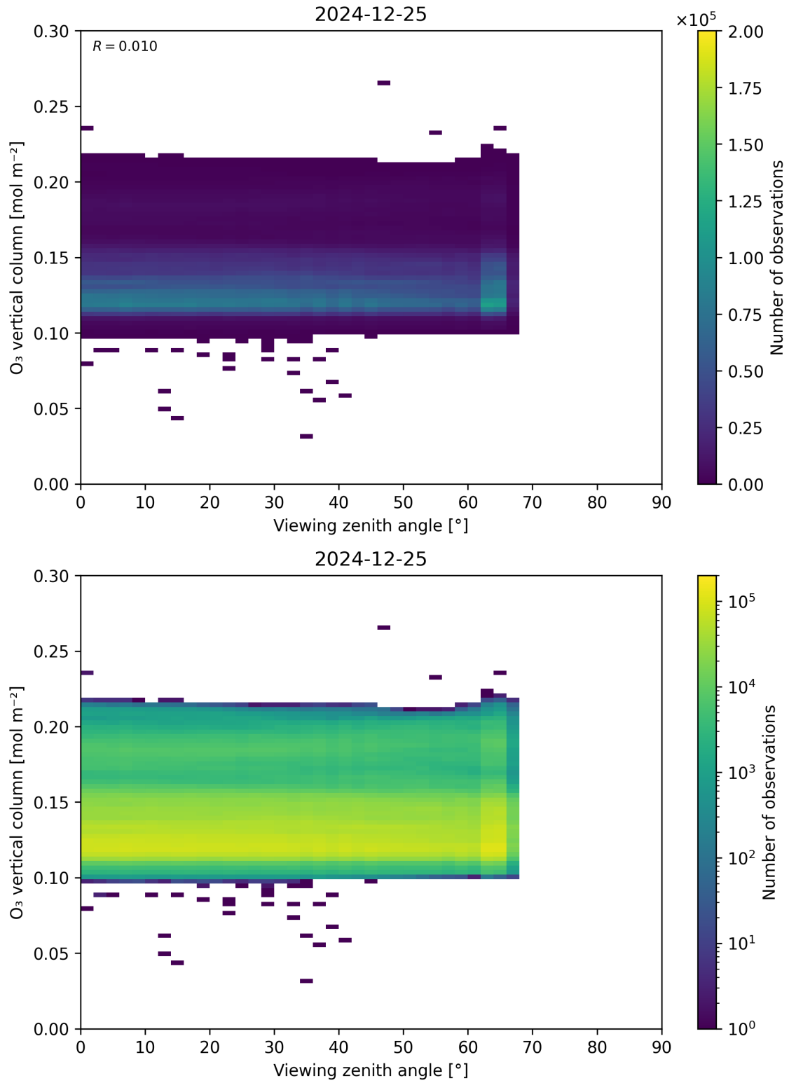
Figure 52: Scatter density plot of “Viewing zenith angle” against “O 3 vertical column” for 2024-12-24 to 2024-12-26.
