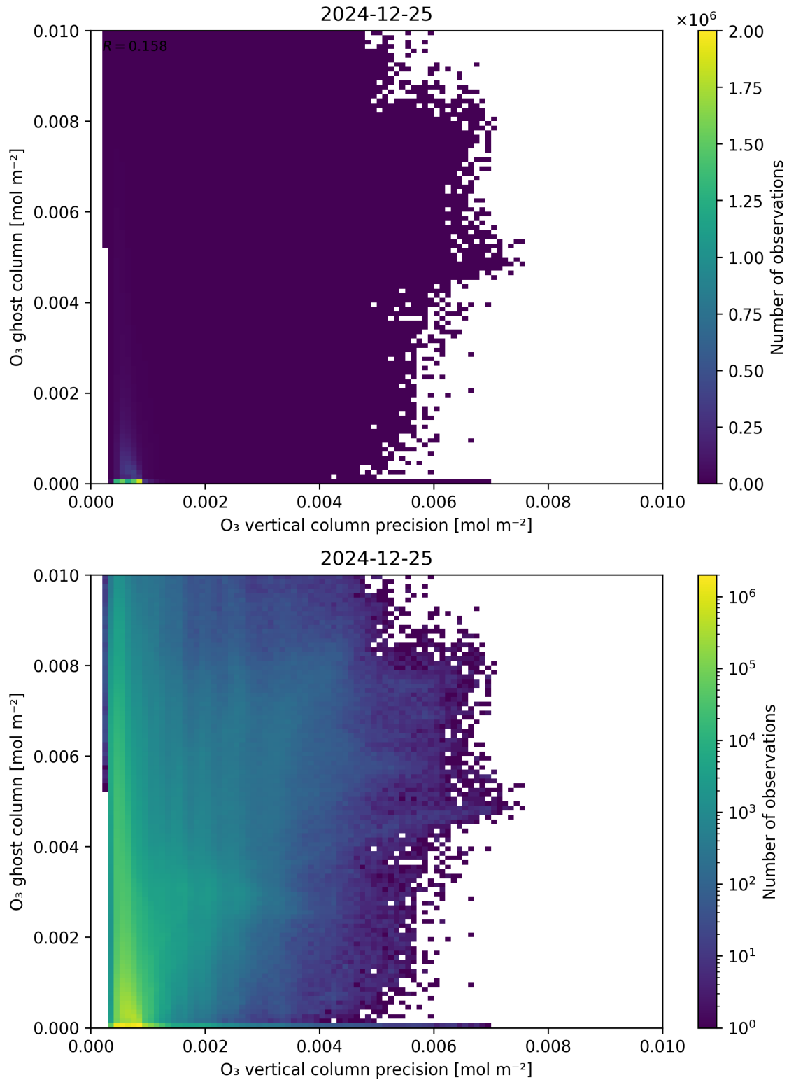
Figure 43: Scatter density plot of “ \text{O}_3 vertical column precision” against “ \text{O}_3 ghost column” for 2024-12-24 to 2024-12-26.
