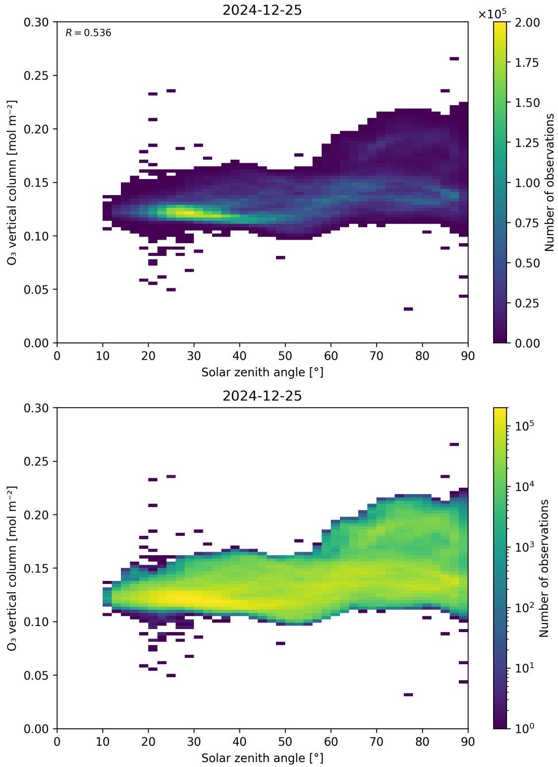
Figure 47: Scatter density plot of “Solar zenith angle” against “O 3 vertical column” for 2024-12-24 to 2024-12-26.
