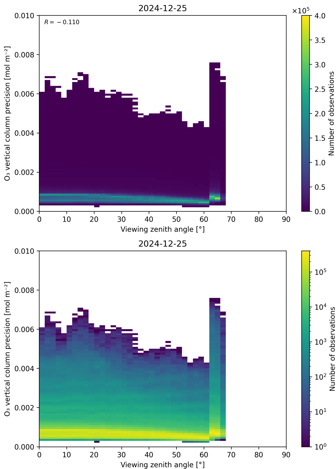
Figure 53: Scatter density plot of “Viewing zenith angle” against “O 3 vertical column precision” for 2024-12-24 to 2024-12-26.
