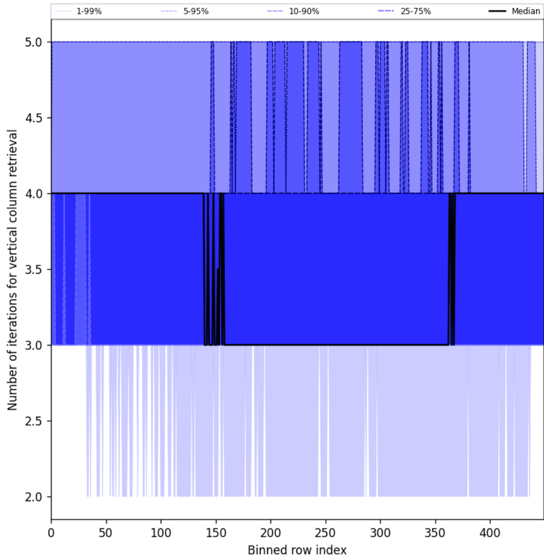
Figure 33: Along track statistics of “Number of iterations for vertical column retrieval” for 2024-12-24 to 2024-12-26
