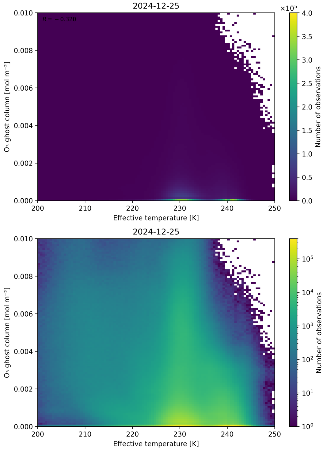
Figure 38: Scatter density plot of “Effective temperature” against “O 3 ghost column” for 2024-12-24 to 2024-12-26.
