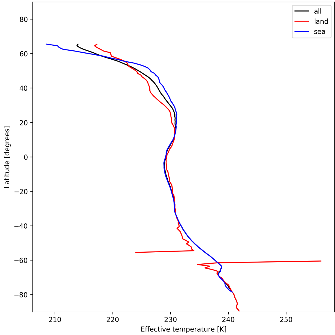
Figure 17: Zonal average of “Effective temperature” for 2024-12-24 to 2024-12-26.
