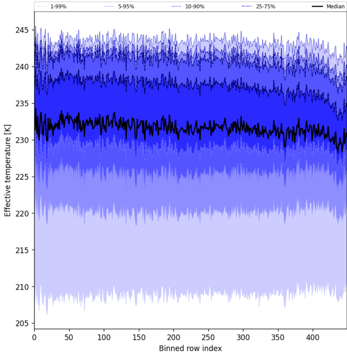
Figure 31: Along track statistics of “Effective temperature” for 2024-12-24 to 2024-12-26
