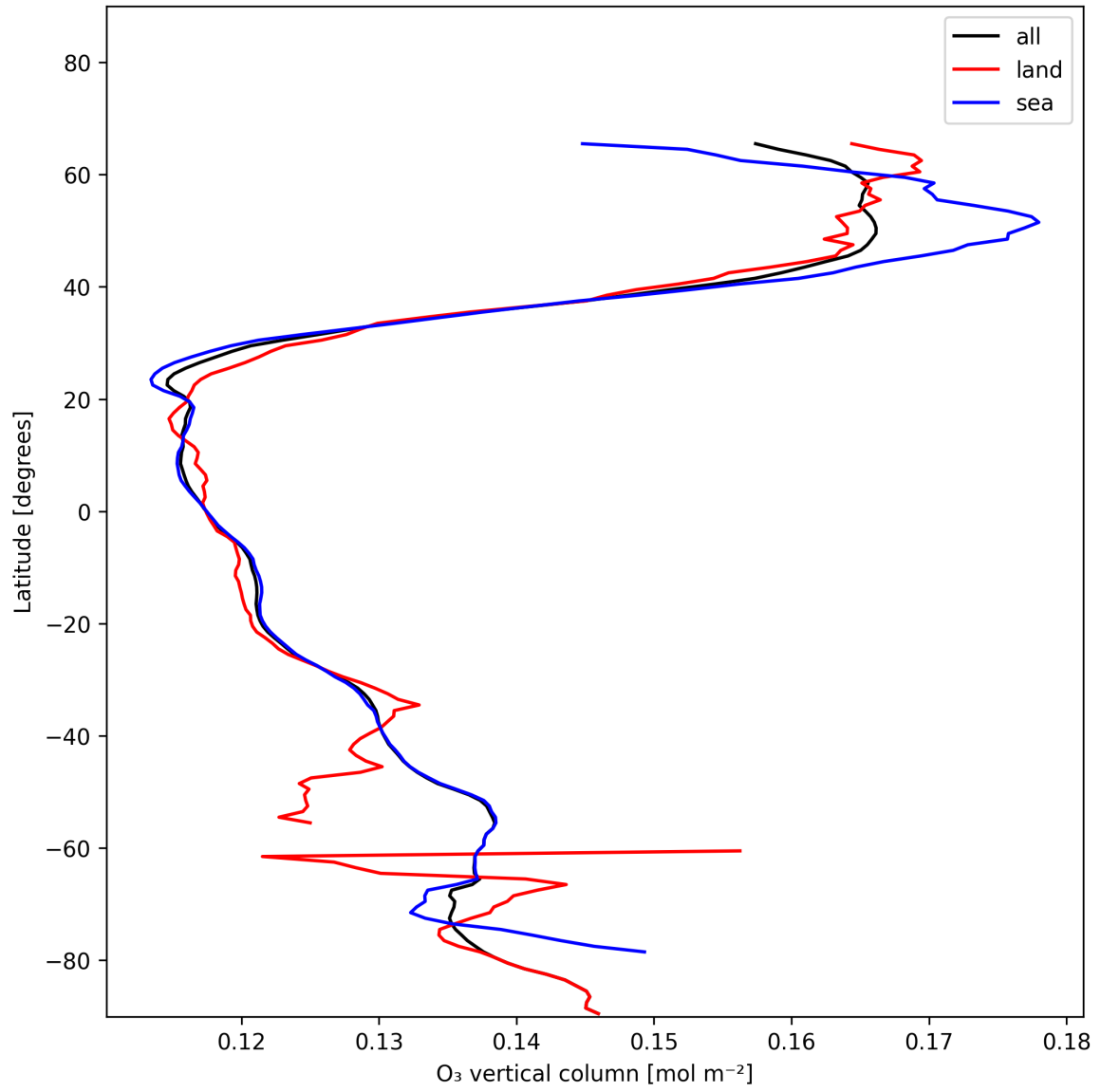
Figure 14: Zonal average of “O 3 vertical column” for 2024-12-24 to 2024-12-26.
