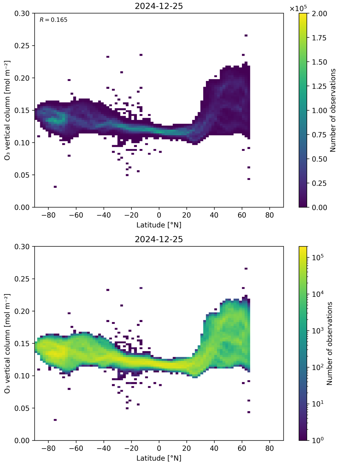
Figure 36: Scatter density plot of “Latitude” against “O 3 vertical column” for 2024-12-24 to 2024-12-26.
