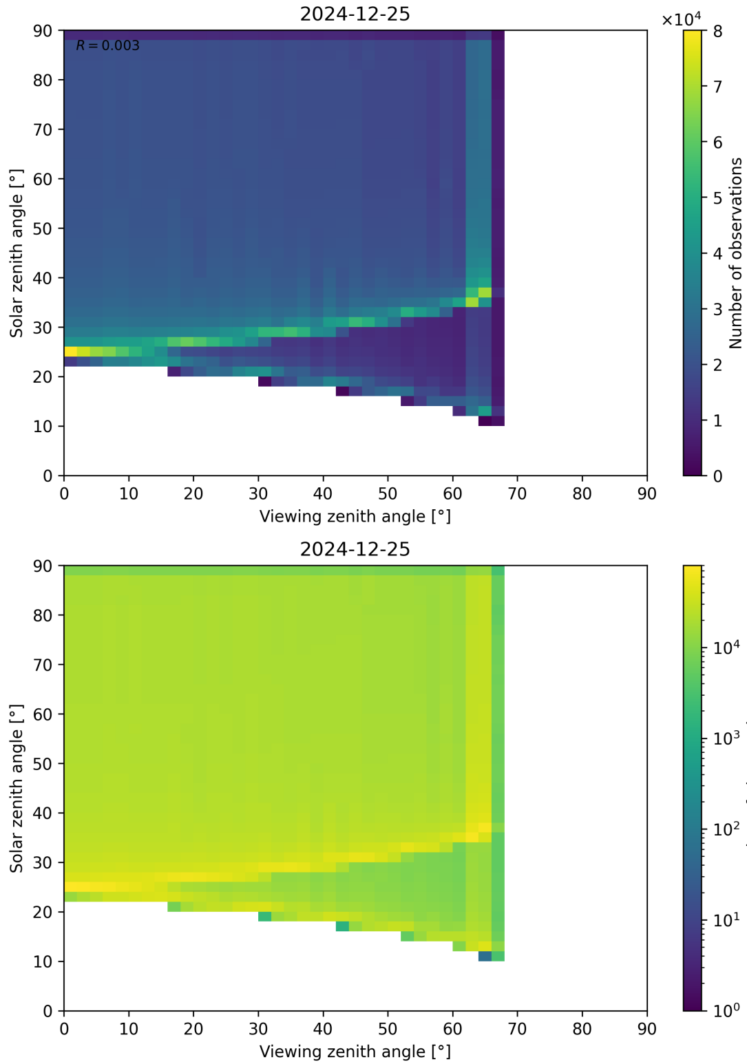
Figure 54: Scatter density plot of “Viewing zenith angle” against “Solar zenith angle” for 2024-12-24 to 2024-12-26.
