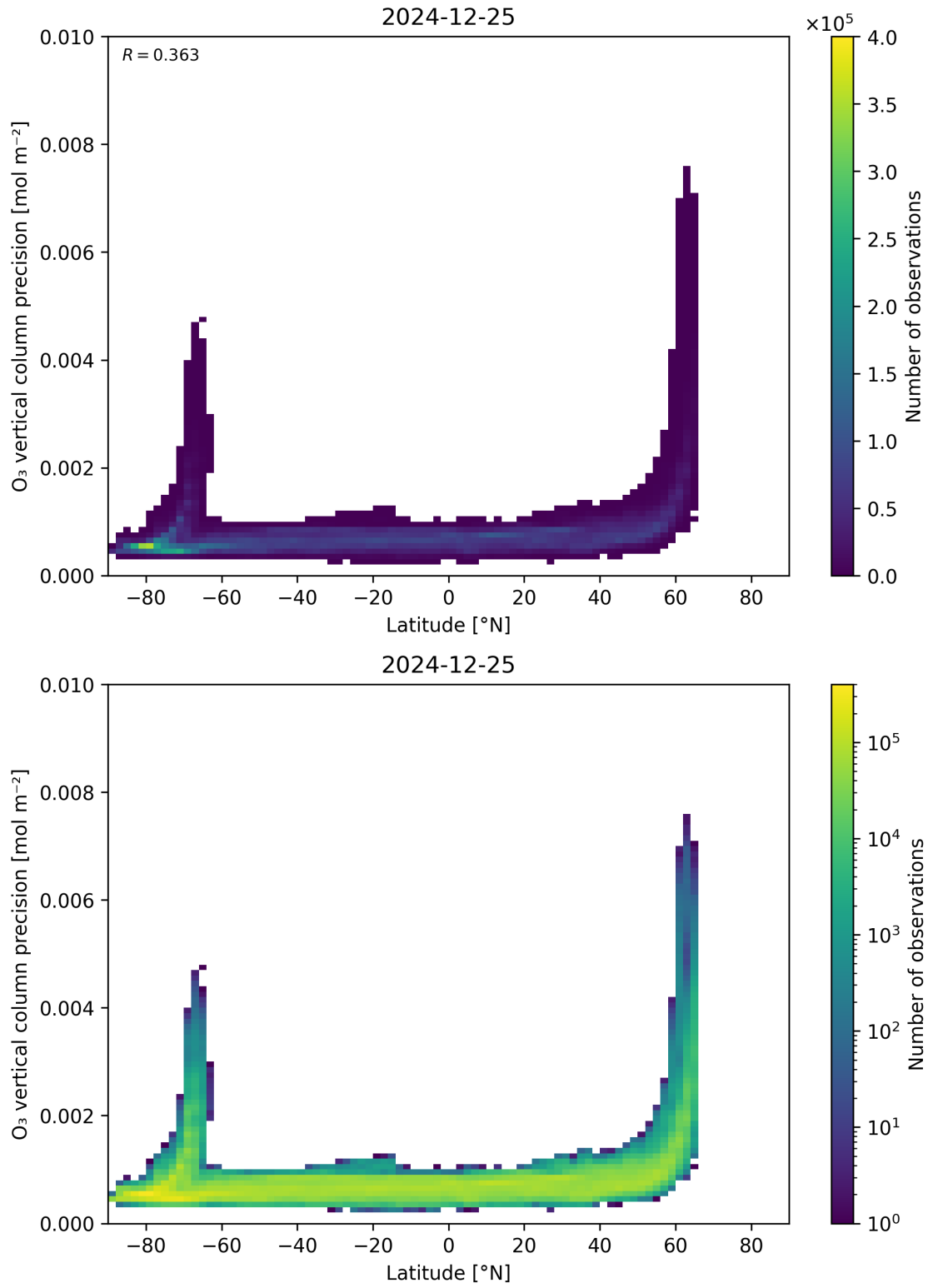
Figure 37: Scatter density plot of “Latitude” against “O 3 vertical column precision” for 2024-12-24 to 2024-12-26.
