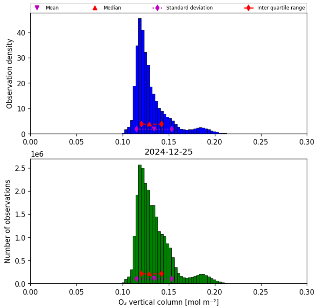
Figure 21: Histogram of “O 3 vertical column” for 2024-12-24 to 2024-12-26
