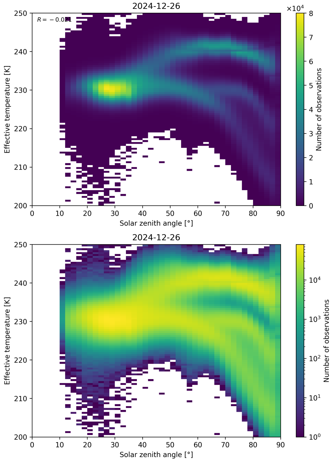
Figure 45: Scatter density plot of “Solar zenith angle” against “Effective temperature” for 2024-12-25 to 2024-12-27.
