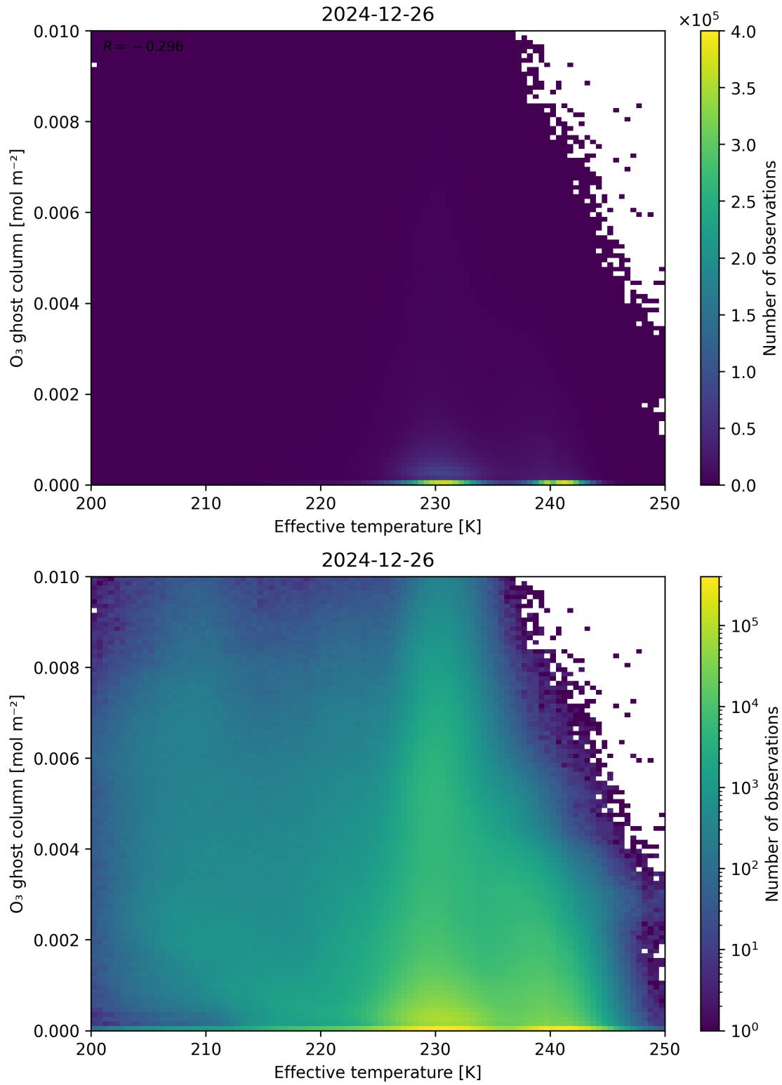
Figure 38: Scatter density plot of “Effective temperature” against “O 3 ghost column” for 2024-12-25 to 2024-12-27.
