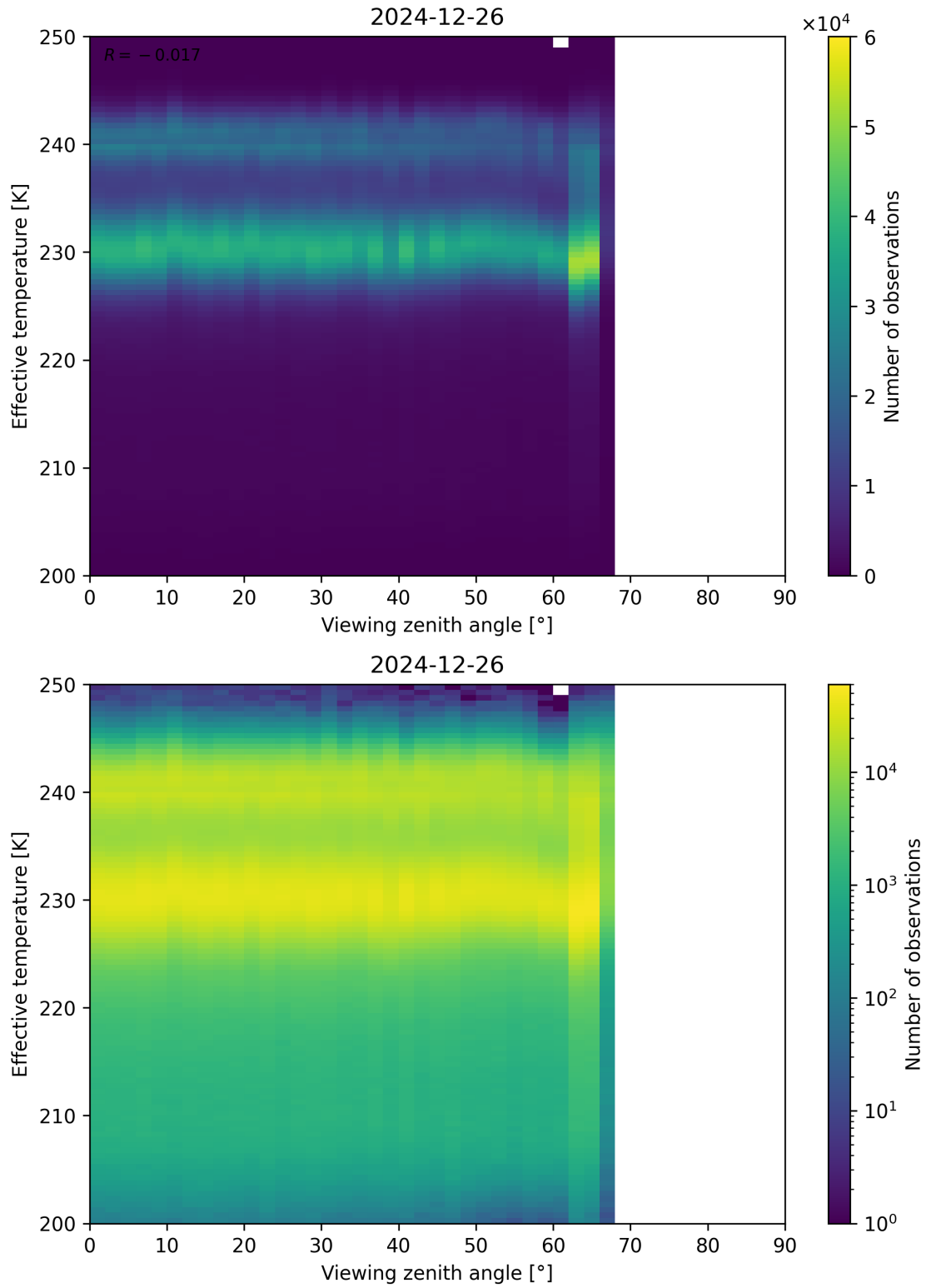
Figure 50: Scatter density plot of “Viewing zenith angle” against “Effective temperature” for 2024-12-25 to 2024-12-27.
