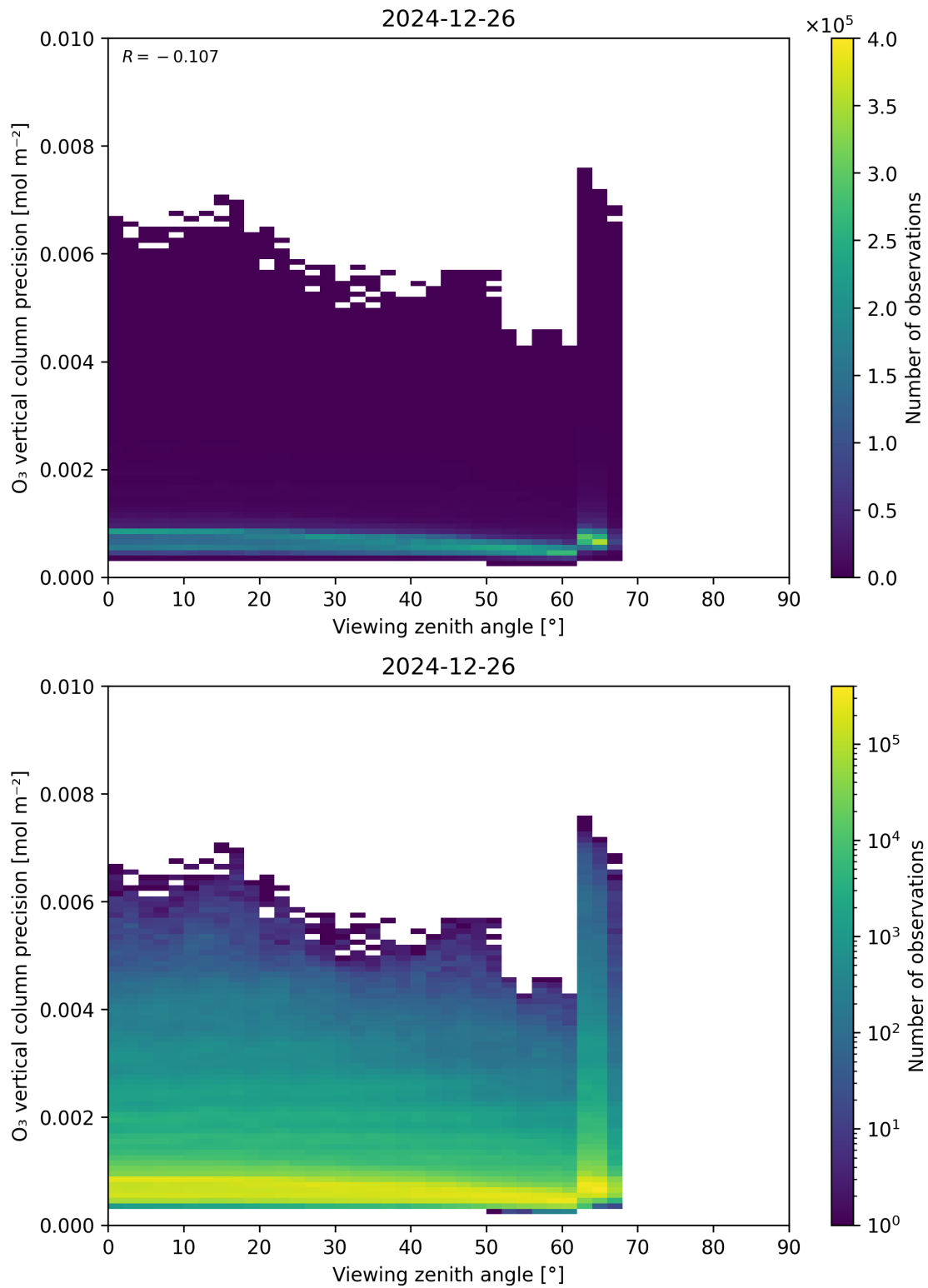
Figure 53: Scatter density plot of “Viewing zenith angle” against “O 3 vertical column precision” for 2024-12-25 to 2024-12-27.
