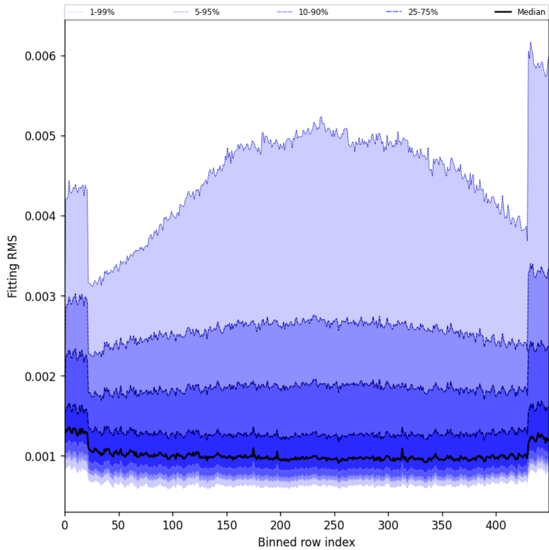
Figure 30: Along track statistics of “Fitting RMS” for 2024-12-25 to 2024-12-27
