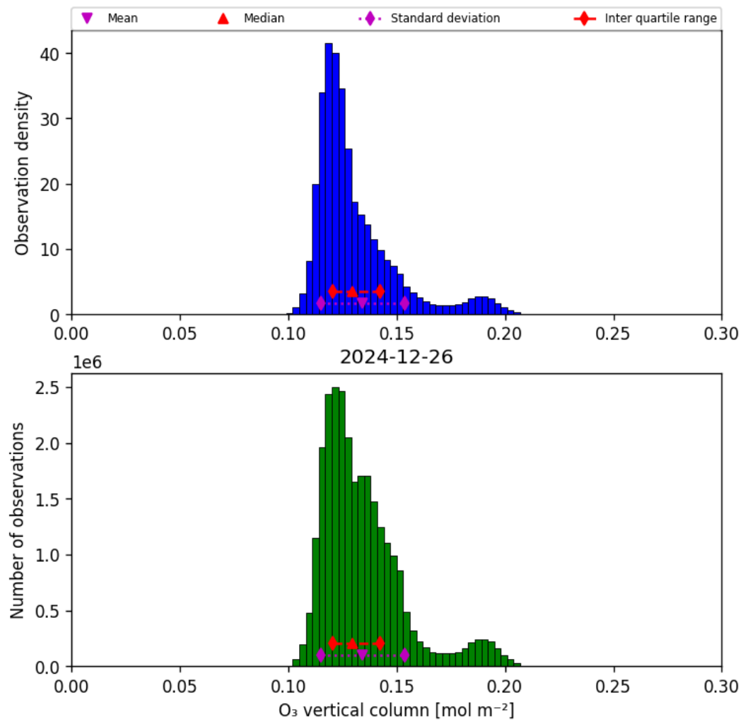
Figure 21: Histogram of “O 3 vertical column” for 2024-12-25 to 2024-12-27
