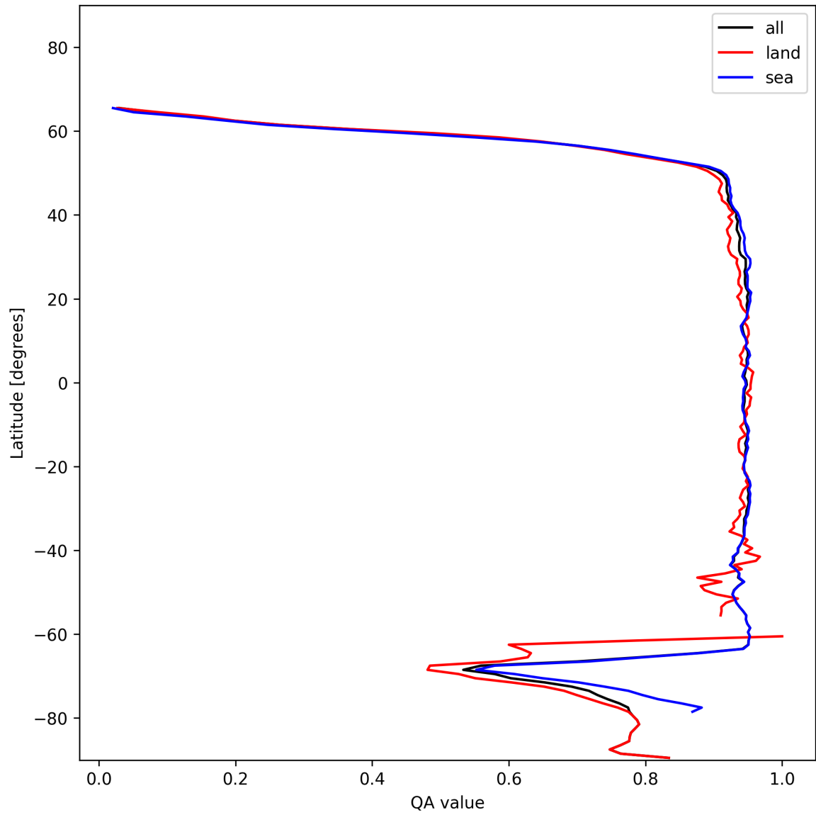
Figure 13: Zonal average of “QA value” for 2024-12-25 to 2024-12-27.
