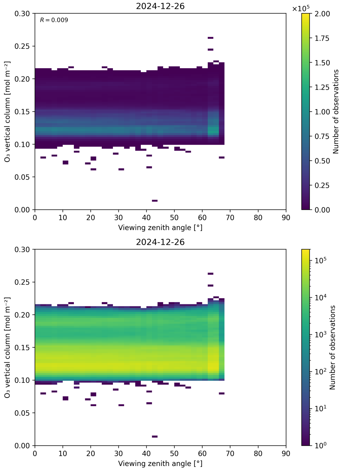
Figure 52: Scatter density plot of “Viewing zenith angle” against “O 3 vertical column” for 2024-12-25 to 2024-12-27.
