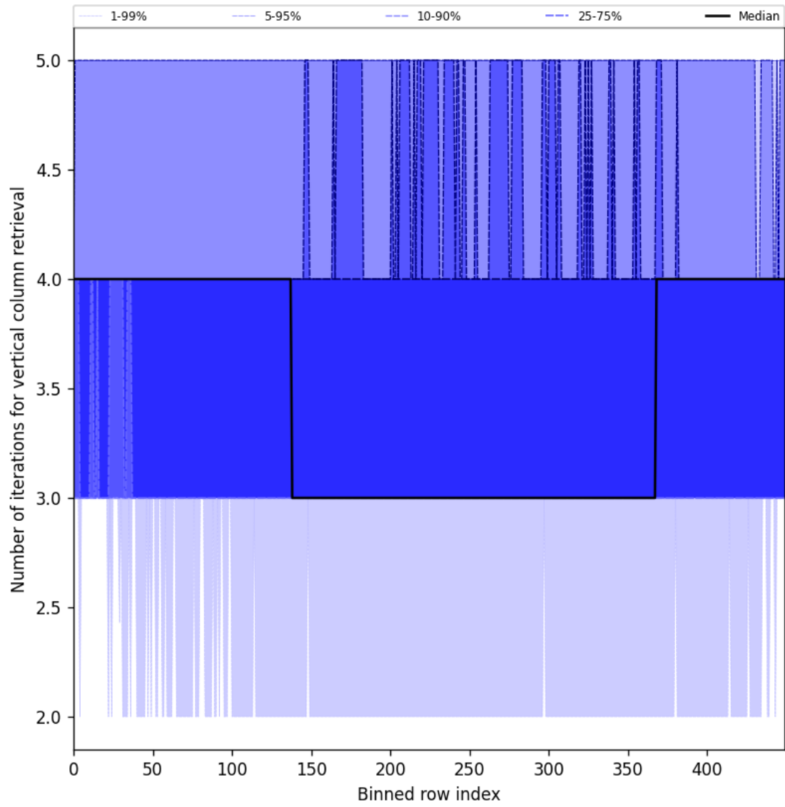
Figure 33: Along track statistics of “Number of iterations for vertical column retrieval” for 2024-12-25 to 2024-12-27
