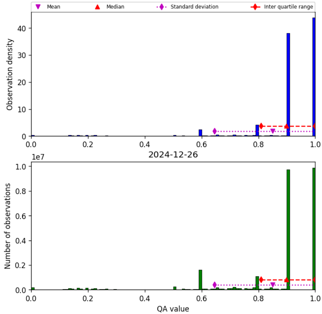
Figure 20: Histogram of “QA value” for 2024-12-25 to 2024-12-27
