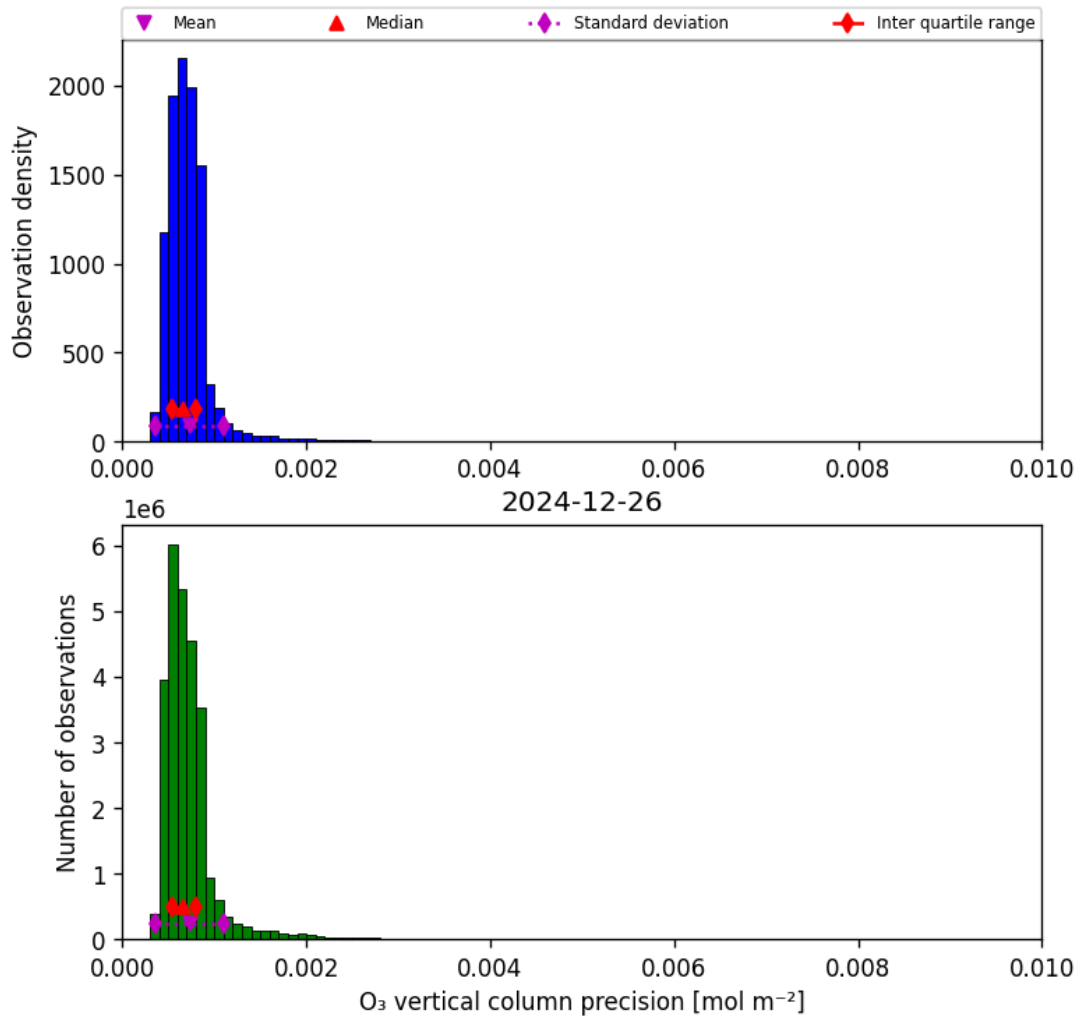
Figure 22: Histogram of "O 3 vertical column precision" for 2024-12-25 to 2024-12-27
