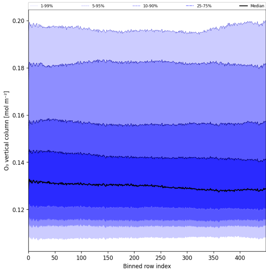
Figure 28: Along track statistics of “O 3 vertical column” for 2024-12-25 to 2024-12-27
