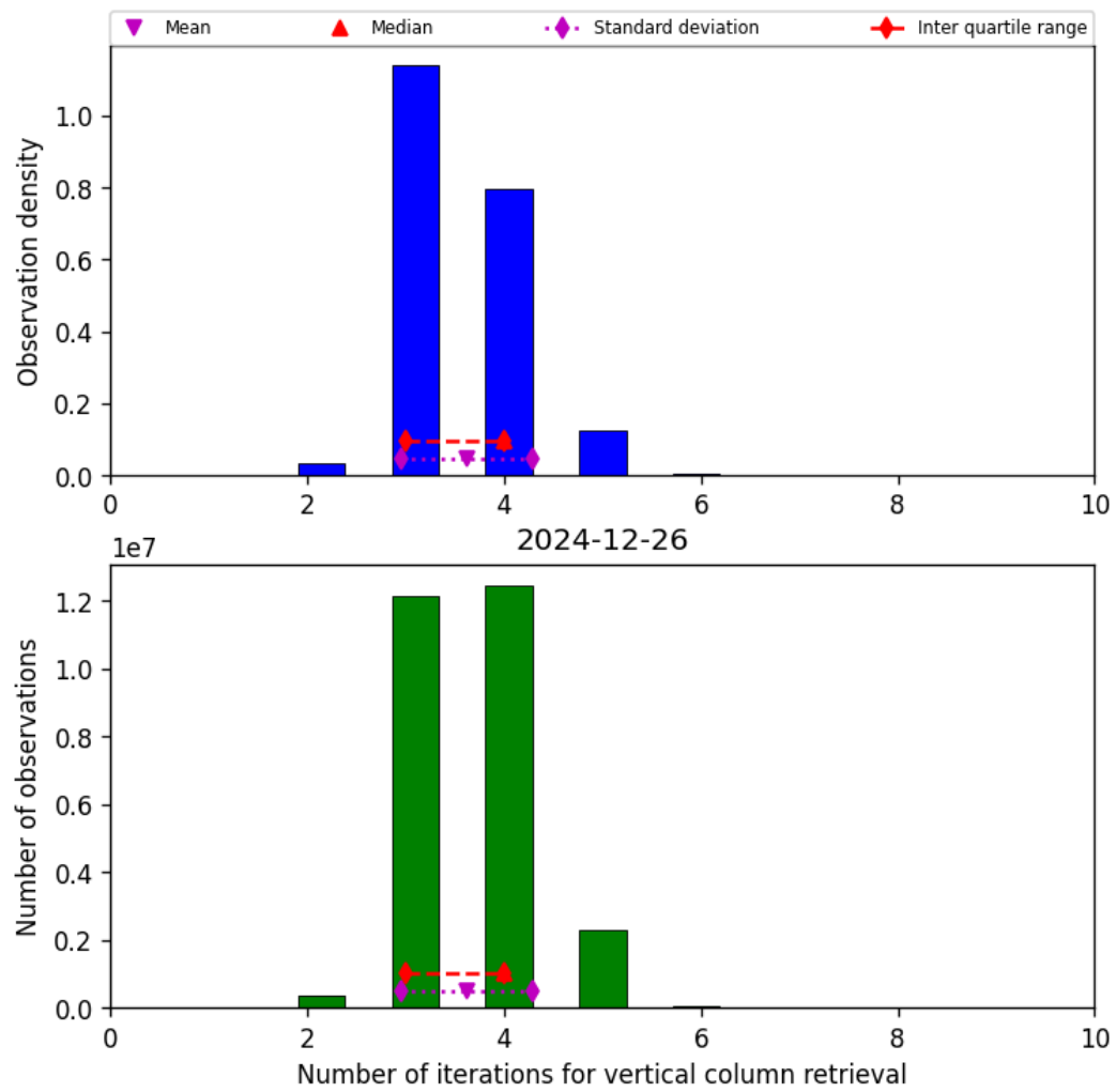
Figure 26: Histogram of “Number of iterations for vertical column retrieval” for 2024-12-25 to 2024-12-27
