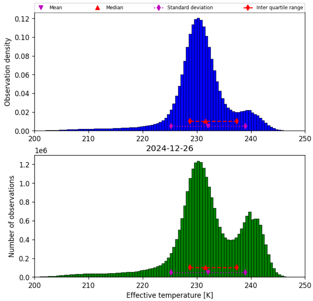
Figure 24: Histogram of “Effective temperature” for 2024-12-25 to 2024-12-27
