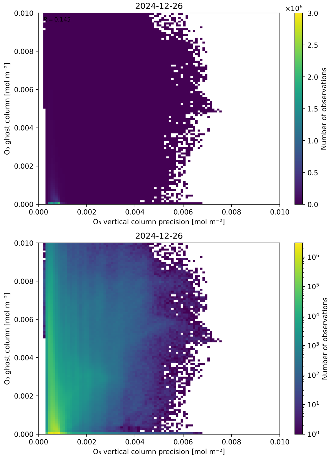
Figure 43: Scatter density plot of “ \text{O}_3 vertical column precision” against “ \text{O}_3 ghost column” for 2024-12-25 to 2024-12-27.
