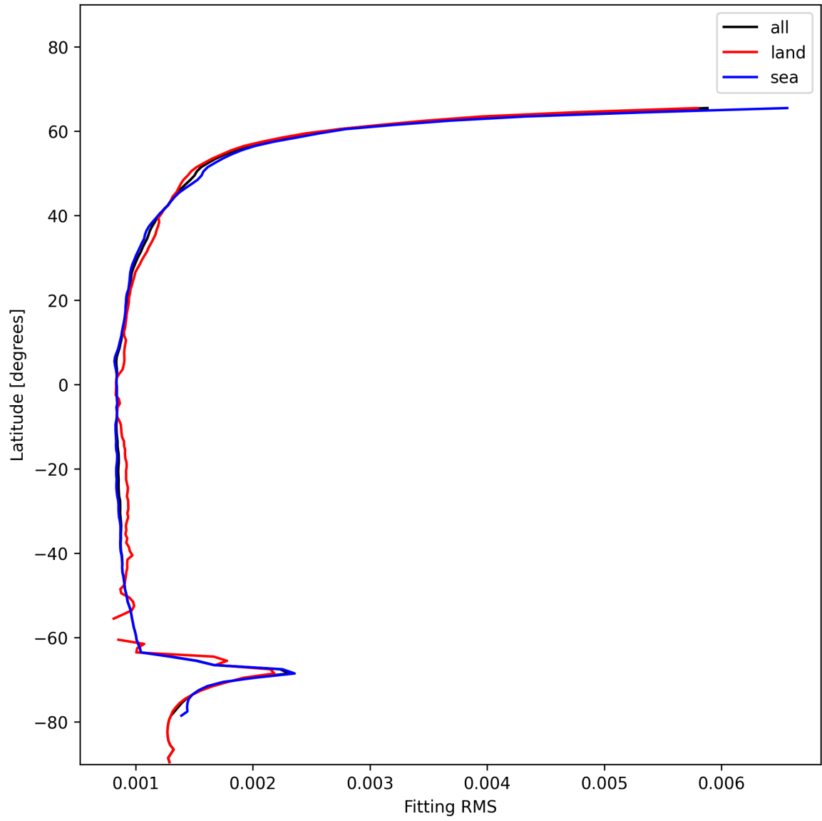
Figure 16: Zonal average of “Fitting RMS” for 2024-12-25 to 2024-12-27.
