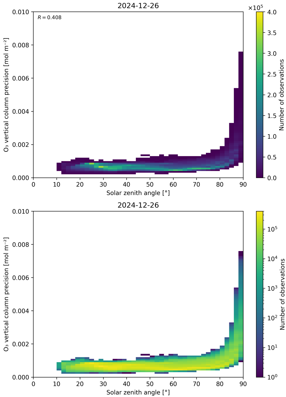
Figure 48: Scatter density plot of “Solar zenith angle” against “O 3 vertical column precision” for 2024-12-25 to 2024-12-27.
