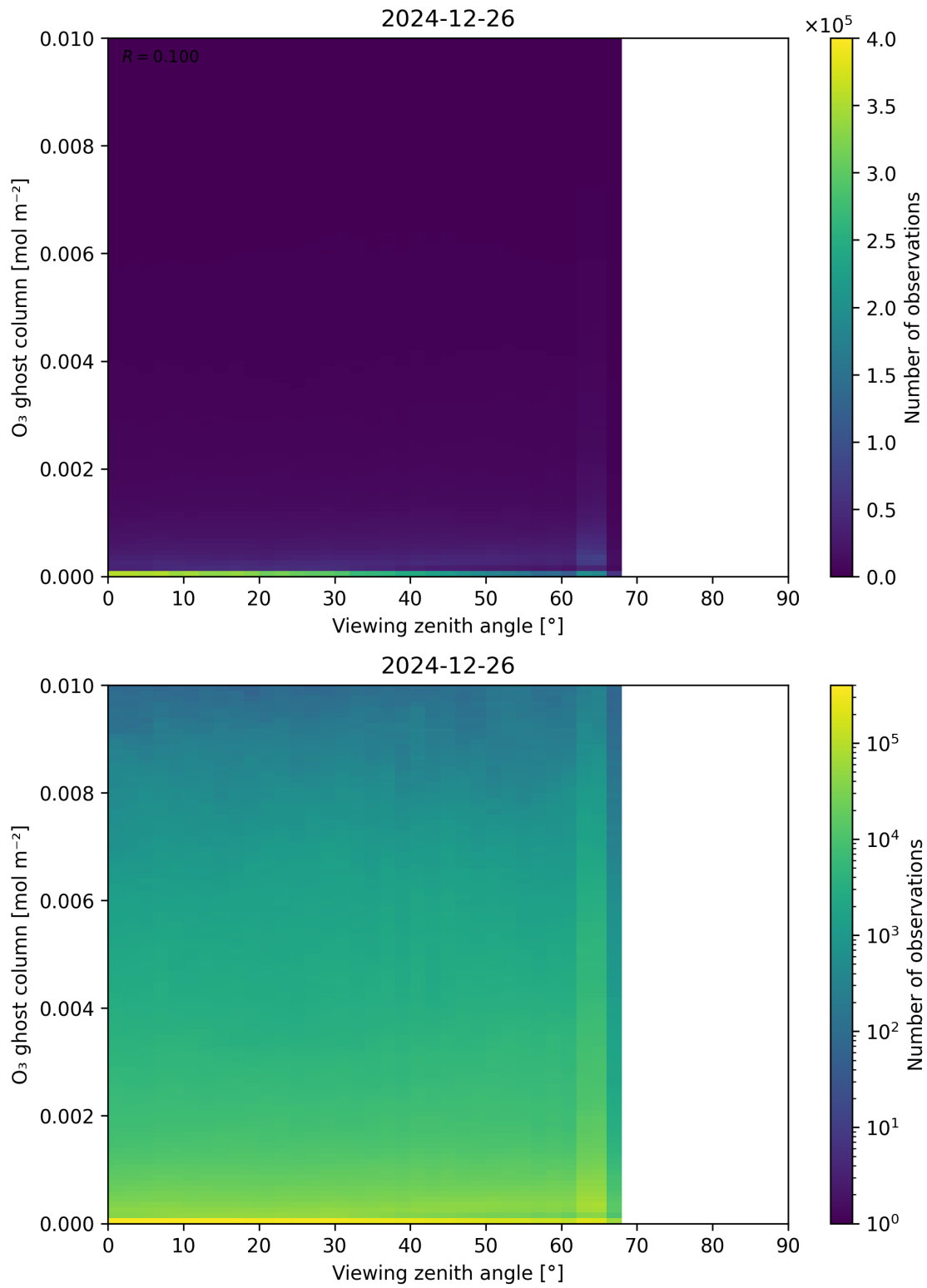
Figure 51: Scatter density plot of “Viewing zenith angle” against “O 3 ghost column” for 2024-12-25 to 2024-12-27.
