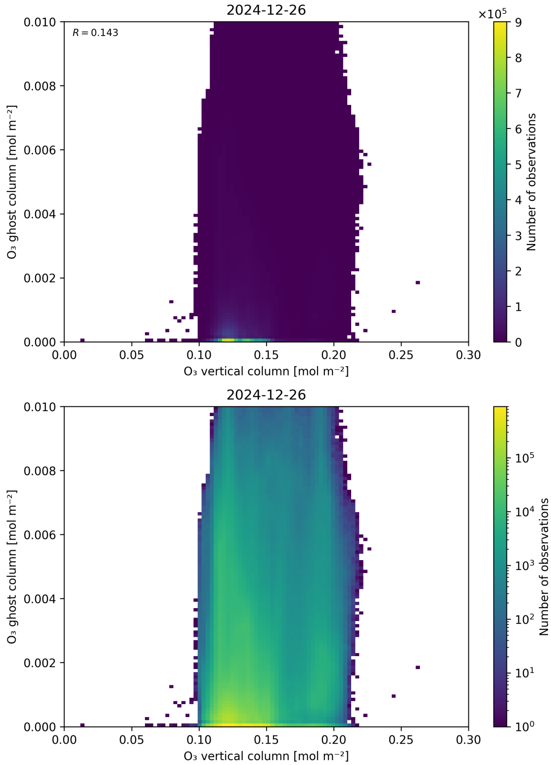
Figure 40: Scatter density plot of “O 3 vertical column” against “O 3 ghost column” for 2024-12-25 to 2024-12-27.
