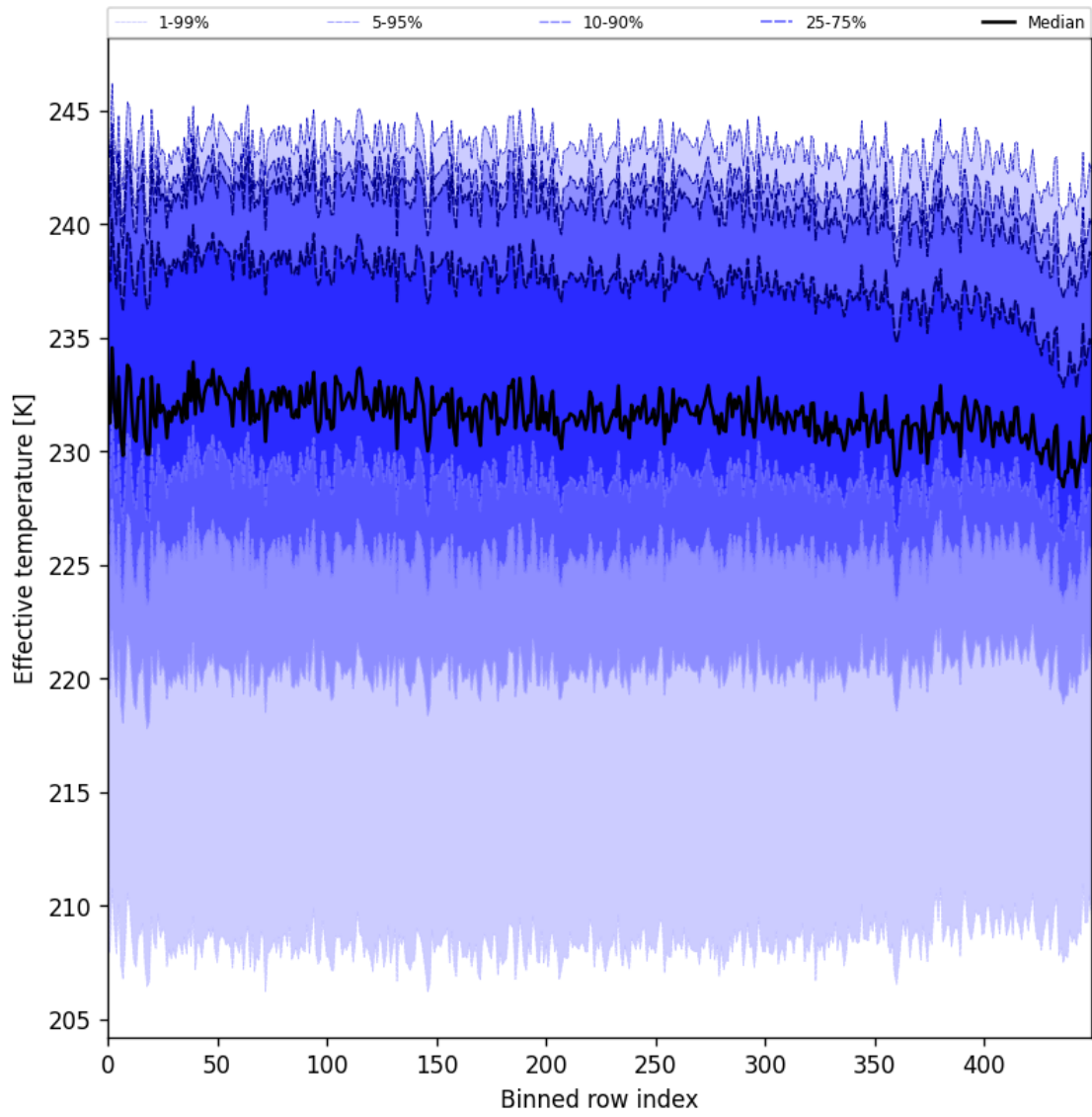
Figure 31: Along track statistics of “Effective temperature” for 2024-12-25 to 2024-12-27
