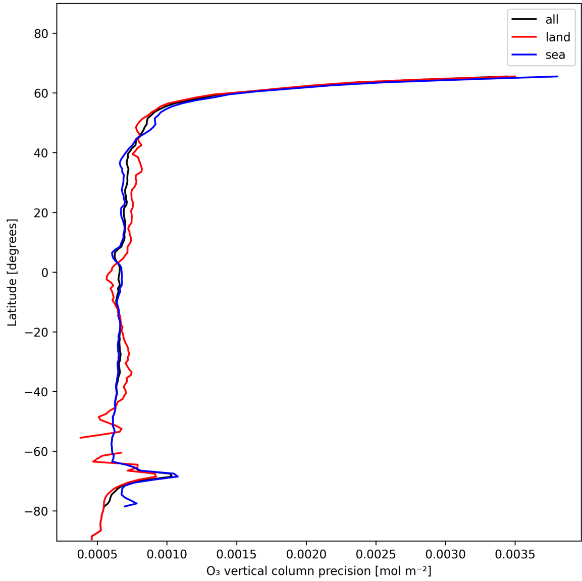
Figure 15: Zonal average of “O 3 vertical column precision” for 2024-12-25 to 2024-12-27.
