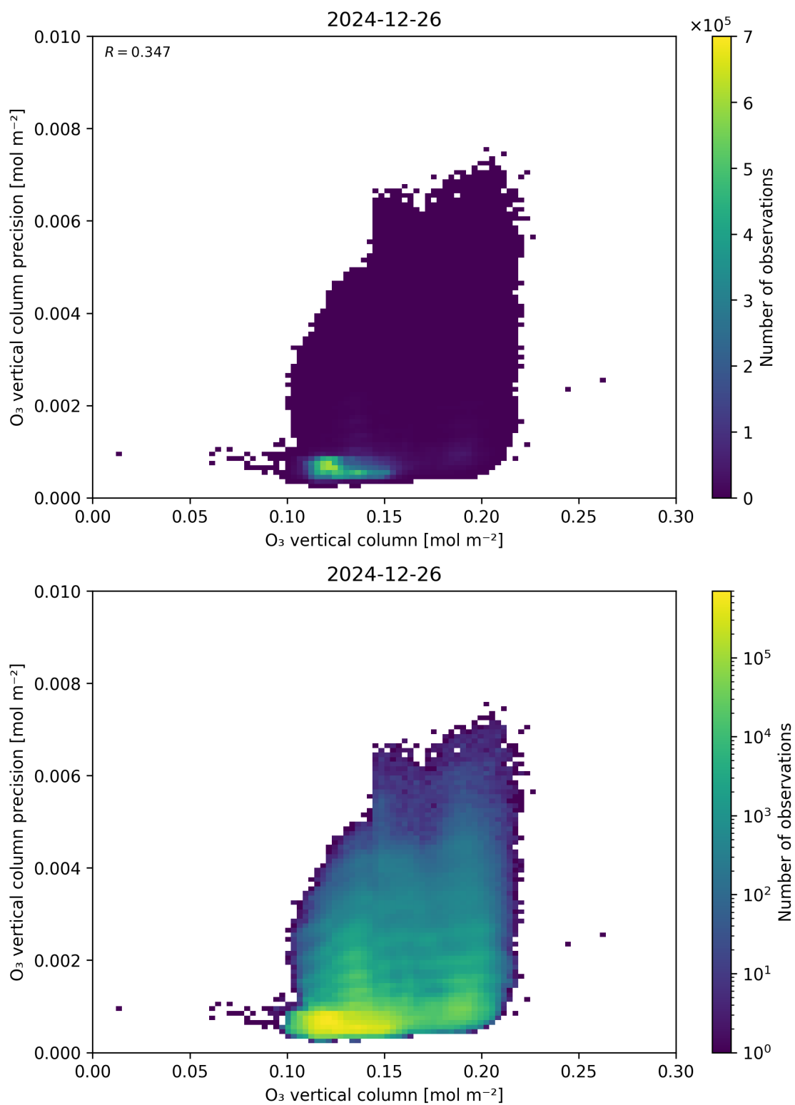
Figure 41: Scatter density plot of “O 3 vertical column” against “O 3 vertical column precision” for 2024-12-25 to 2024-12-27.
