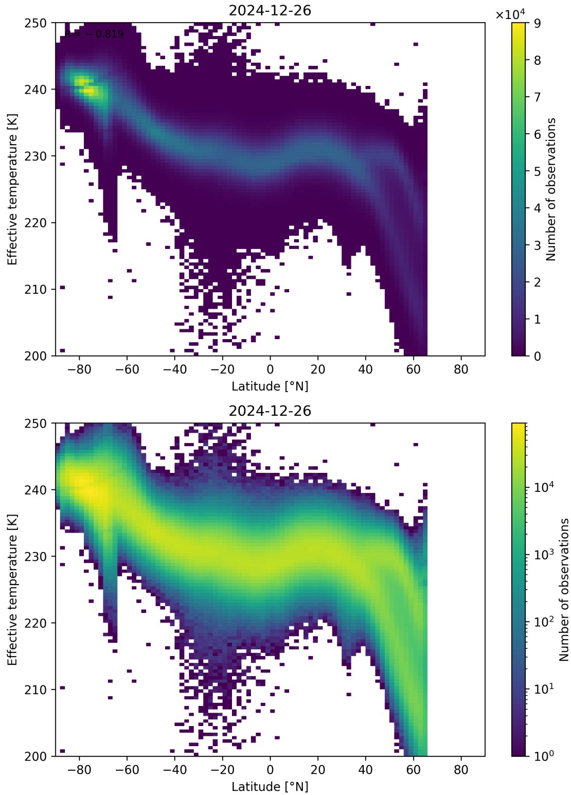
Figure 34: Scatter density plot of “Latitude” against “Effective temperature” for 2024-12-25 to 2024-12-27.
