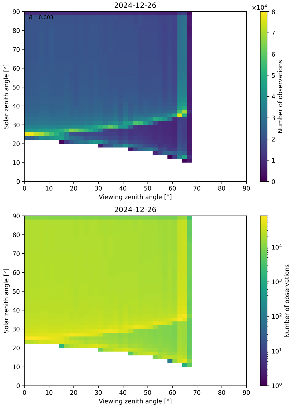
Figure 54: Scatter density plot of “Viewing zenith angle” against “Solar zenith angle” for 2024-12-25 to 2024-12-27.
