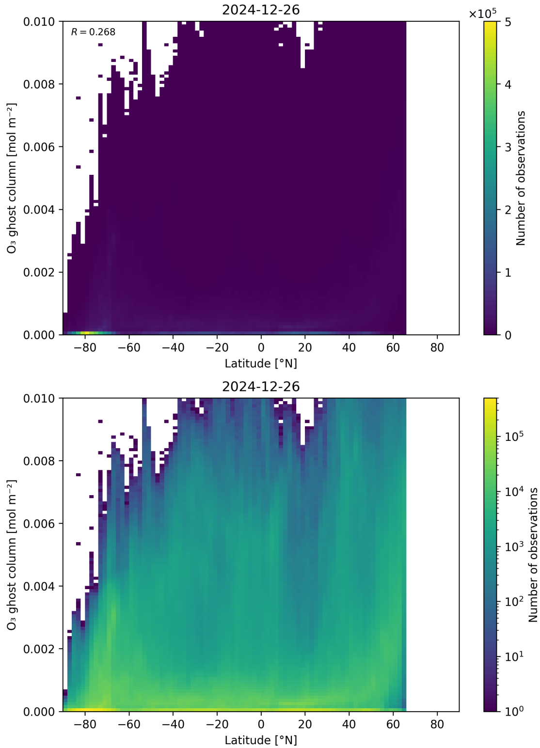
Figure 35: Scatter density plot of “Latitude” against “O 3 ghost column” for 2024-12-25 to 2024-12-27.
