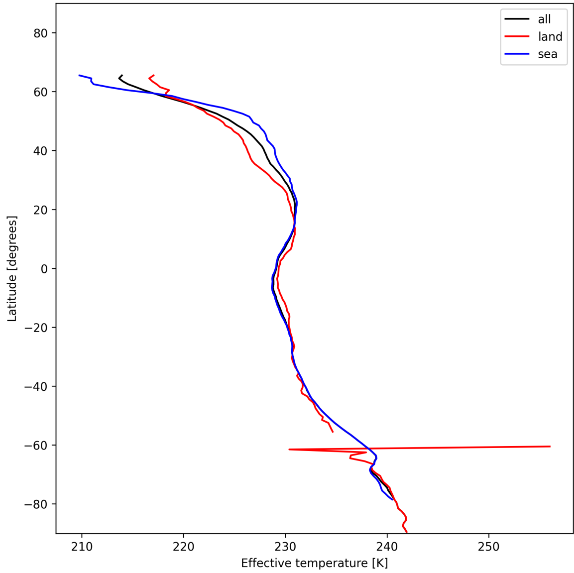
Figure 17: Zonal average of “Effective temperature” for 2024-12-25 to 2024-12-27.
