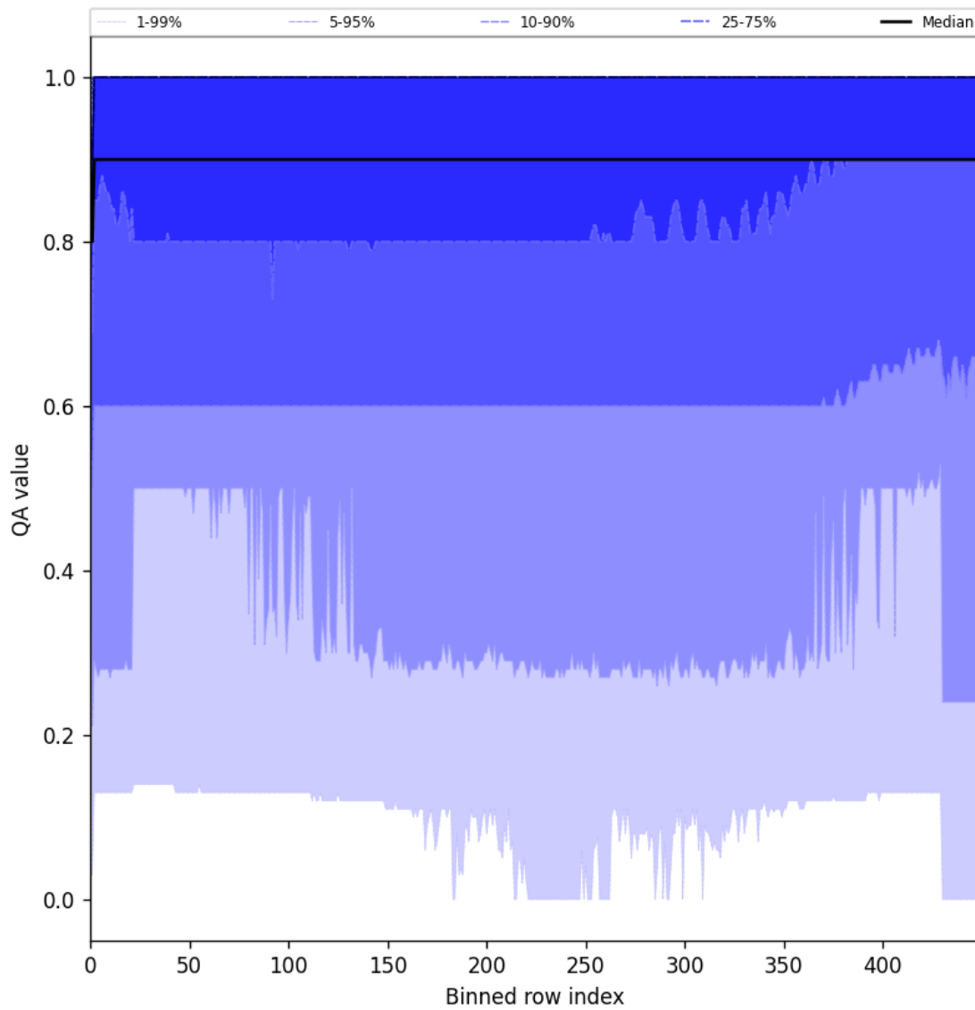
Figure 27: Along track statistics of “QA value” for 2024-12-25 to 2024-12-27
