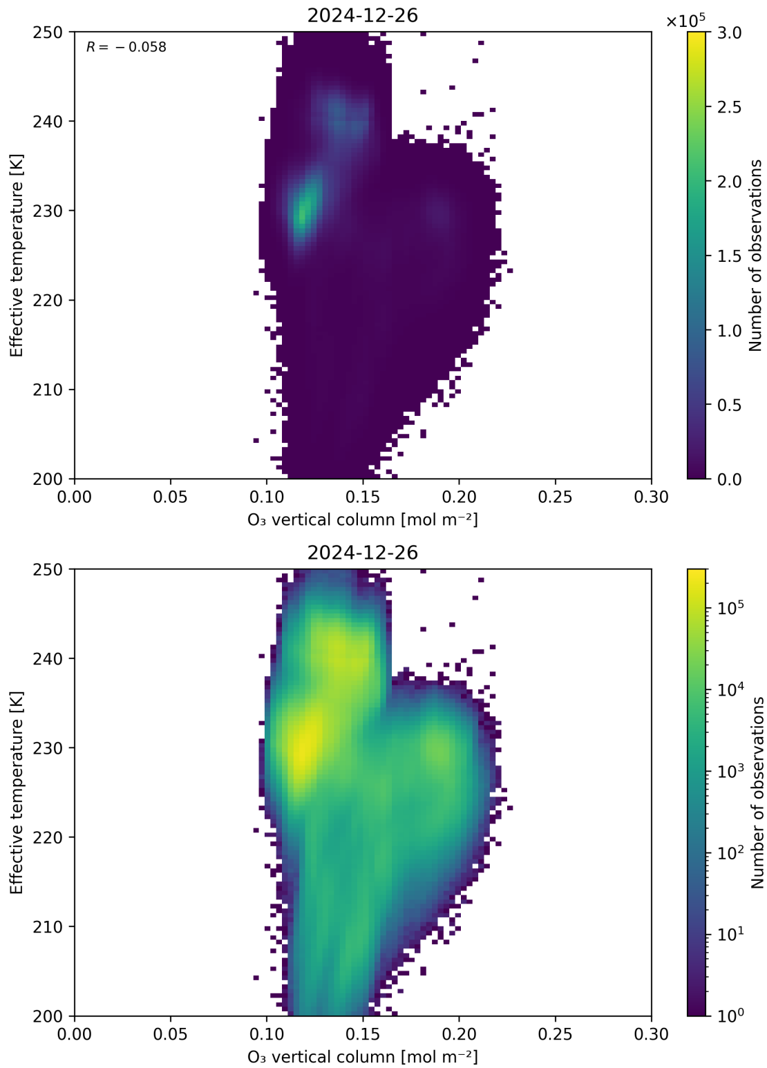
Figure 39: Scatter density plot of “O 3 vertical column” against “Effective temperature” for 2024-12-25 to 2024-12-27.
