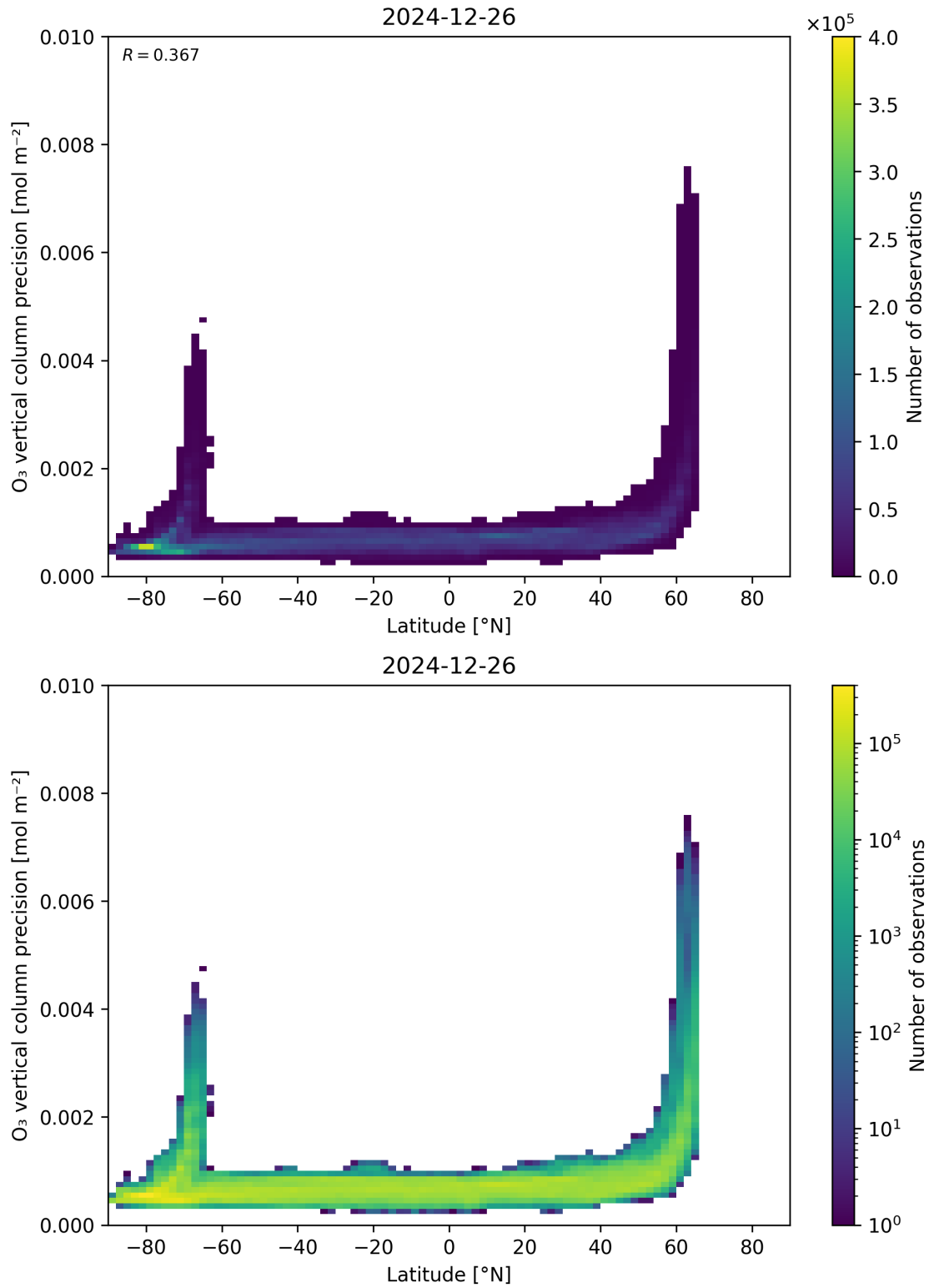
Figure 37: Scatter density plot of “Latitude” against “O 3 vertical column precision” for 2024-12-25 to 2024-12-27.
