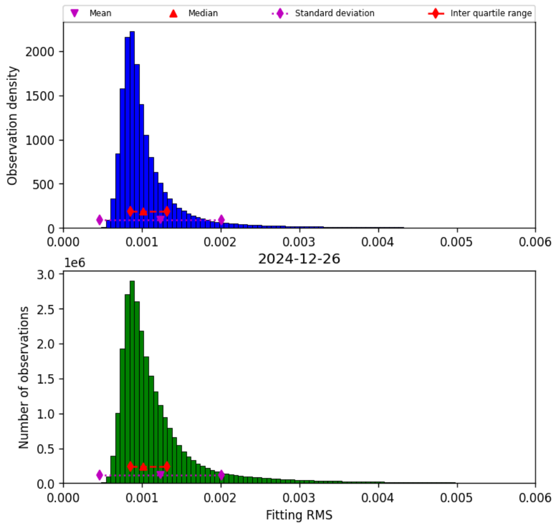
Figure 23: Histogram of “Fitting RMS” for 2024-12-25 to 2024-12-27
