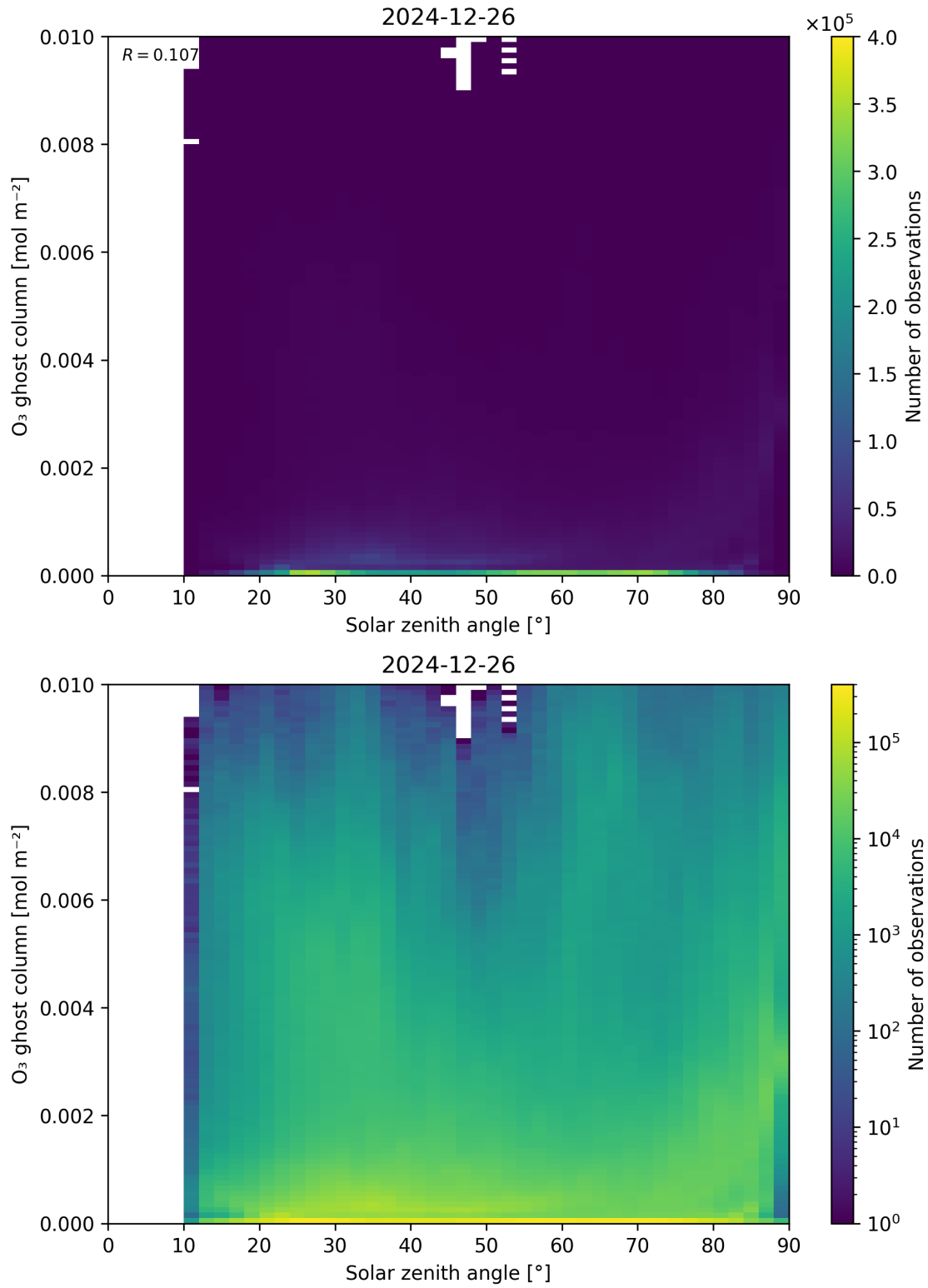
Figure 46: Scatter density plot of “Solar zenith angle” against “O 3 ghost column” for 2024-12-25 to 2024-12-27.
