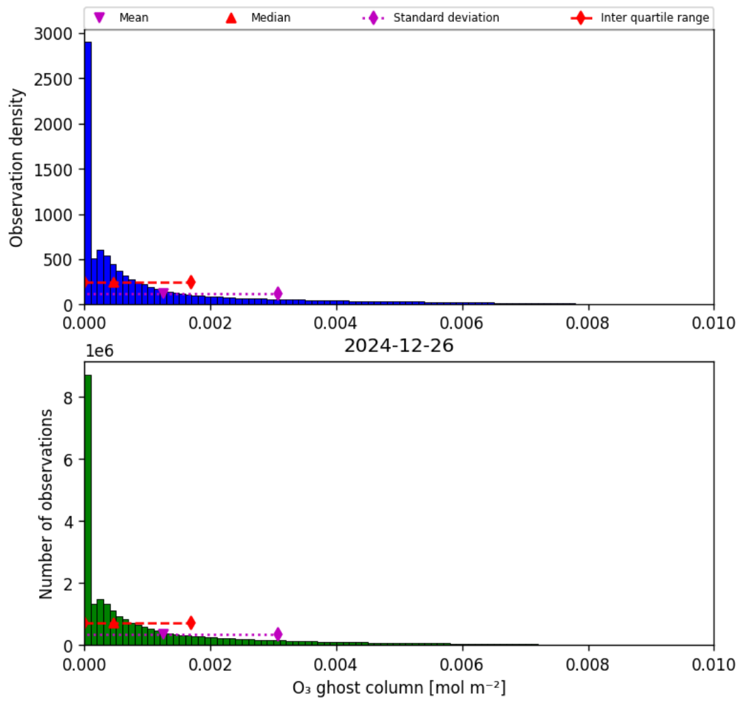
Figure 25: Histogram of “O 3 ghost column” for 2024-12-25 to 2024-12-27
