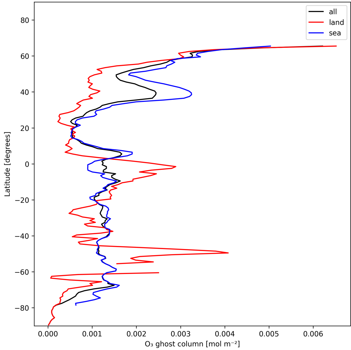
Figure 18: Zonal average of "O 3 ghost column" for 2024-12-25 to 2024-12-27.
