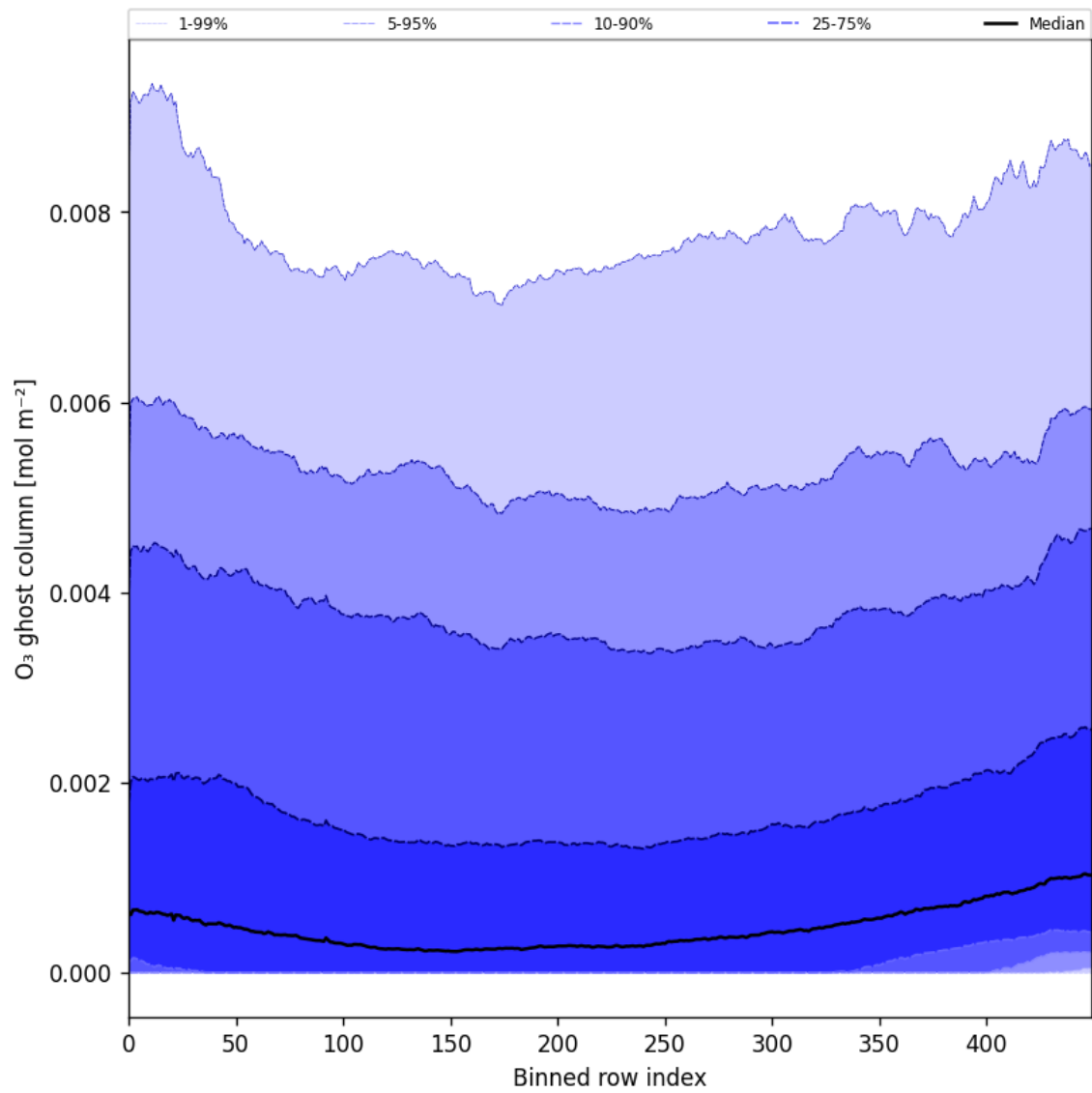
Figure 32: Along track statistics of “O 3 ghost column” for 2024-12-25 to 2024-12-27
