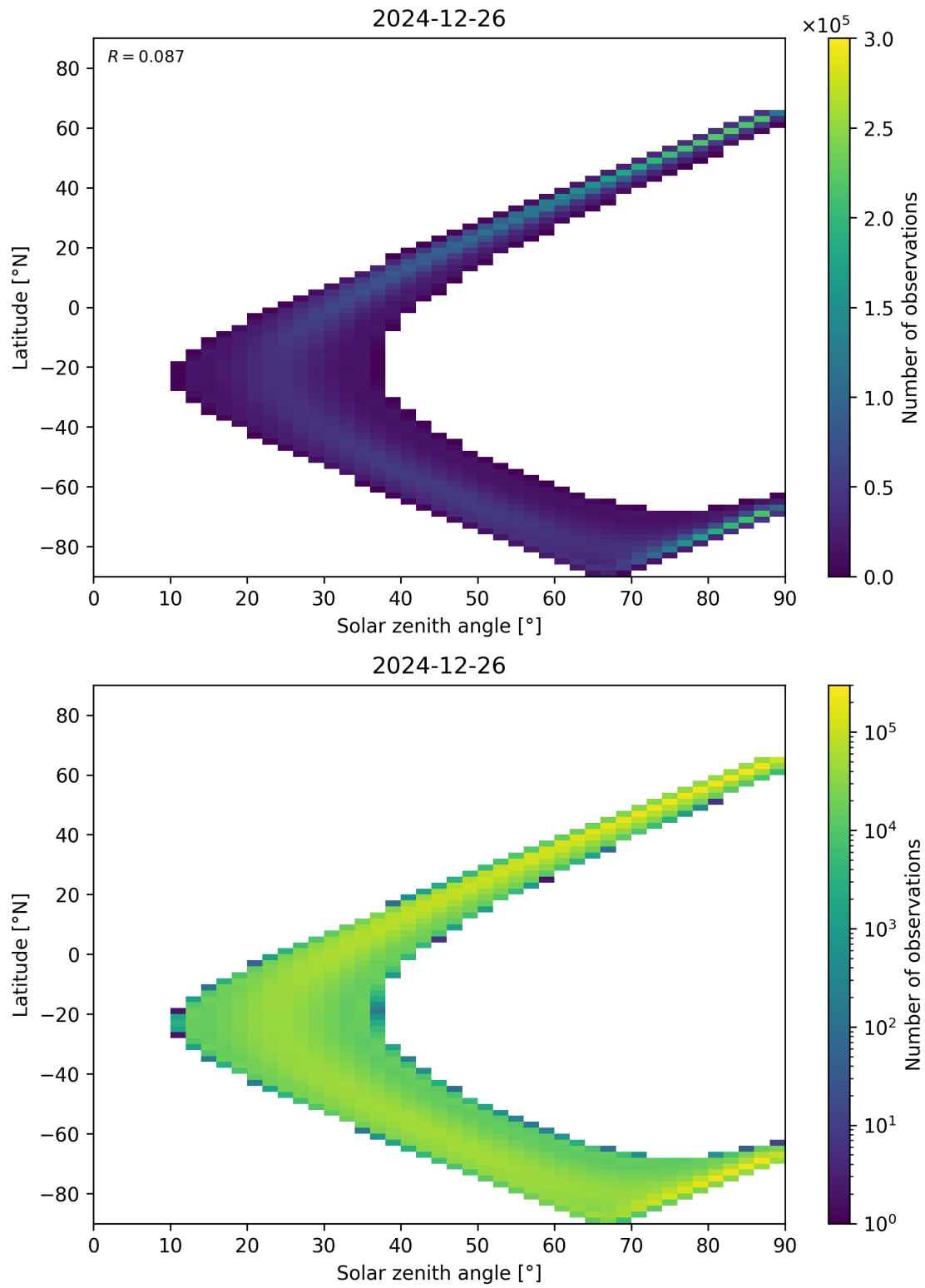
Figure 44: Scatter density plot of “Solar zenith angle” against “Latitude” for 2024-12-25 to 2024-12-27.
