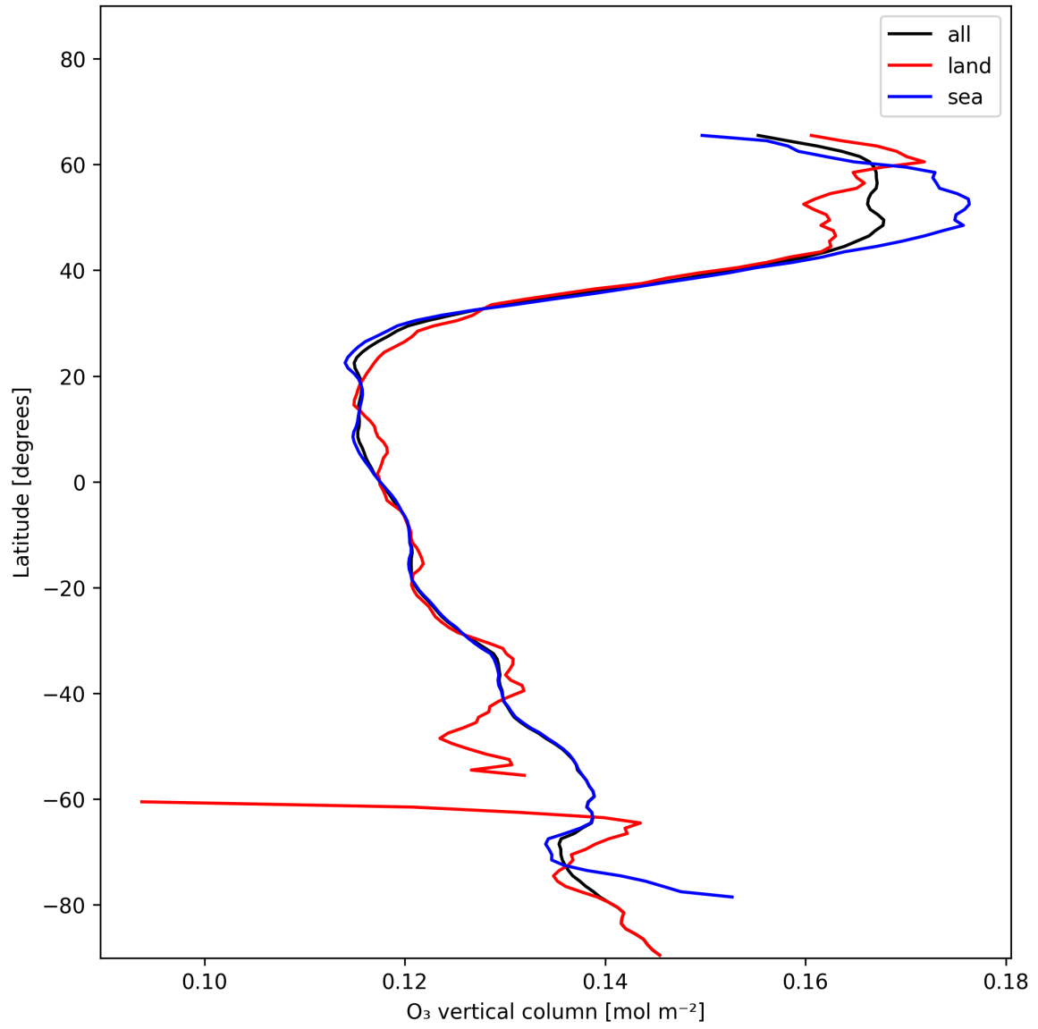
Figure 14: Zonal average of “O 3 vertical column” for 2024-12-25 to 2024-12-27.
