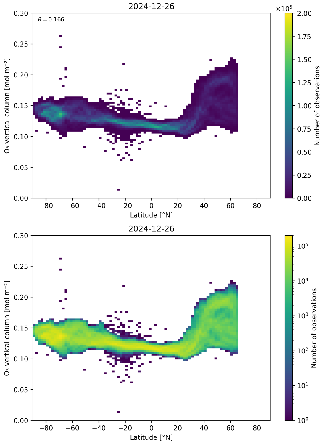
Figure 36: Scatter density plot of “Latitude” against “O 3 vertical column” for 2024-12-25 to 2024-12-27.
