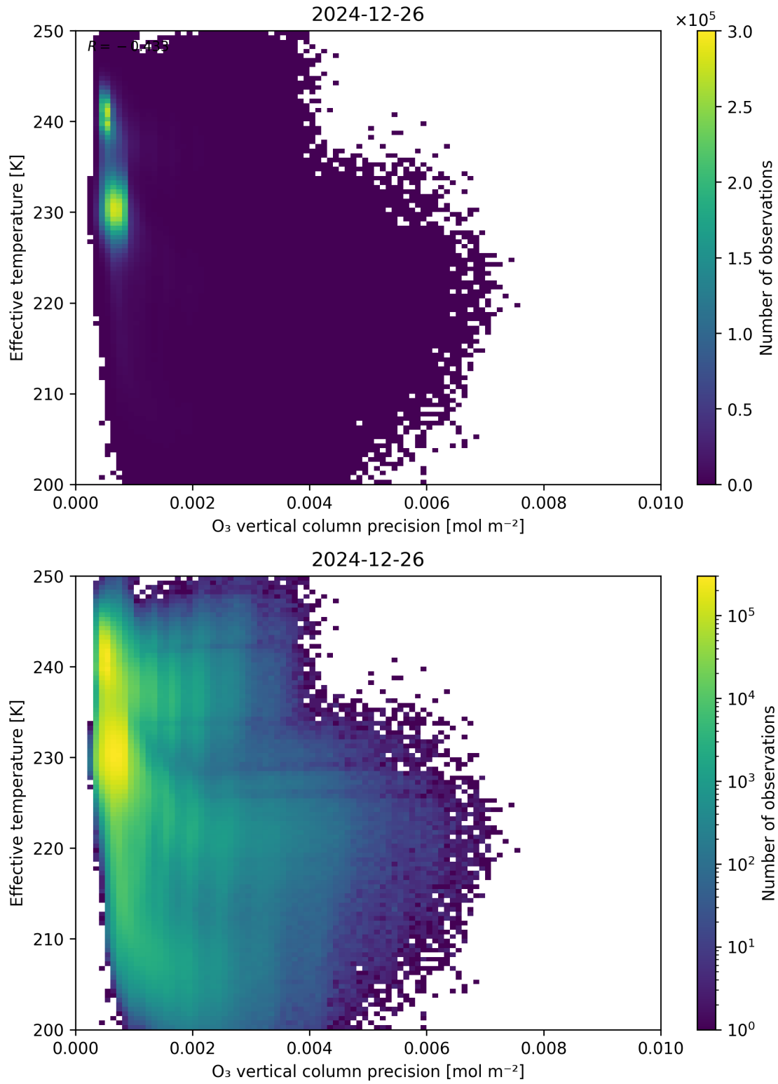
Figure 42: Scatter density plot of “O 3 vertical column precision” against “Effective temperature” for 2024-12-25 to 2024-12-27.
