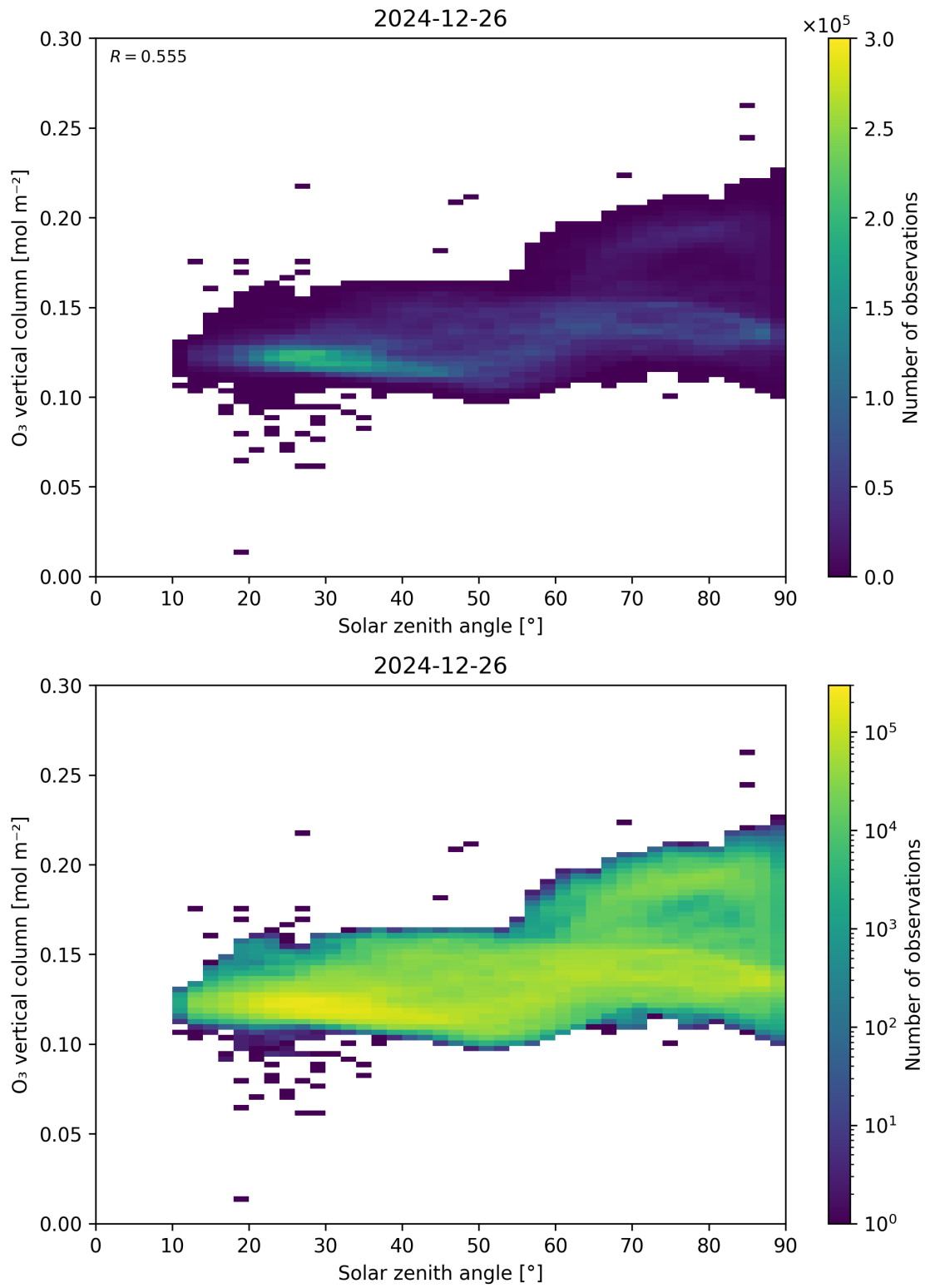
Figure 47: Scatter density plot of “Solar zenith angle” against “O 3 vertical column” for 2024-12-25 to 2024-12-27.
