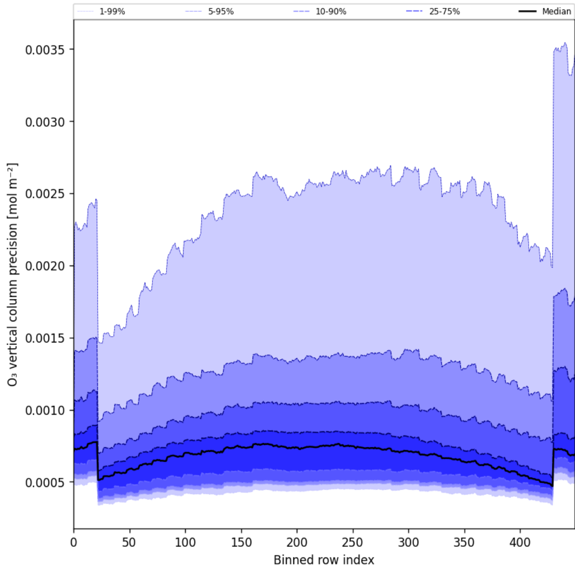
Figure 29: Along track statistics of “O 3 vertical column precision” for 2024-12-25 to 2024-12-27
