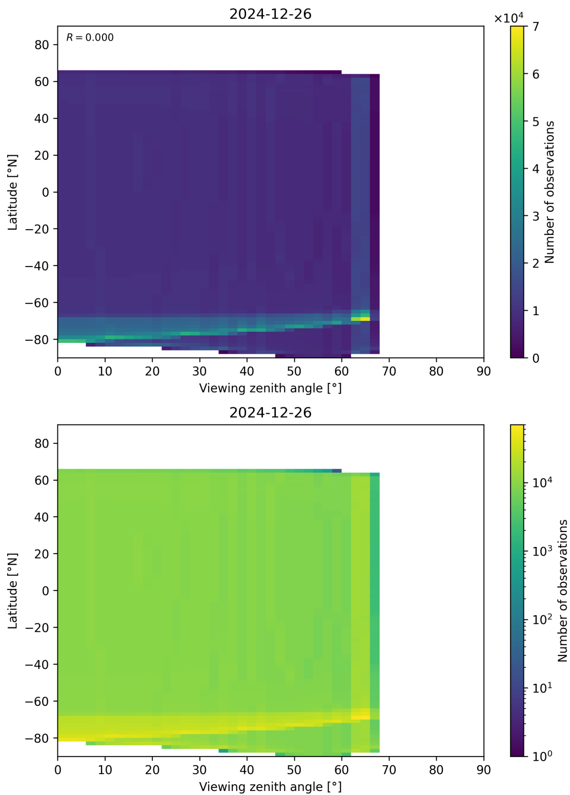
Figure 49: Scatter density plot of “Viewing zenith angle” against “Latitude” for 2024-12-25 to 2024-12-27.
