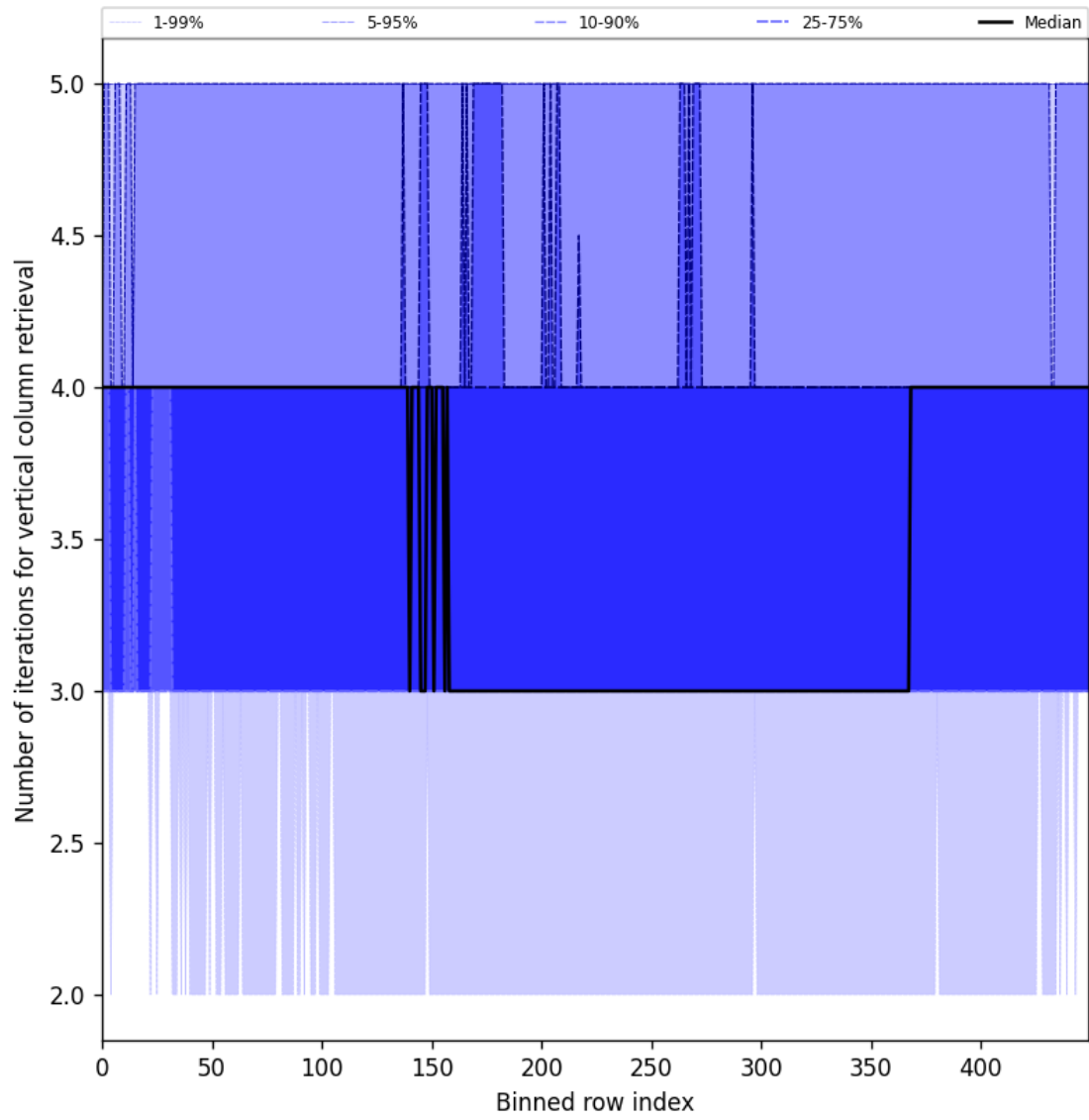
Figure 33: Along track statistics of “Number of iterations for vertical column retrieval” for 2024-12-27 to 2024-12-28
