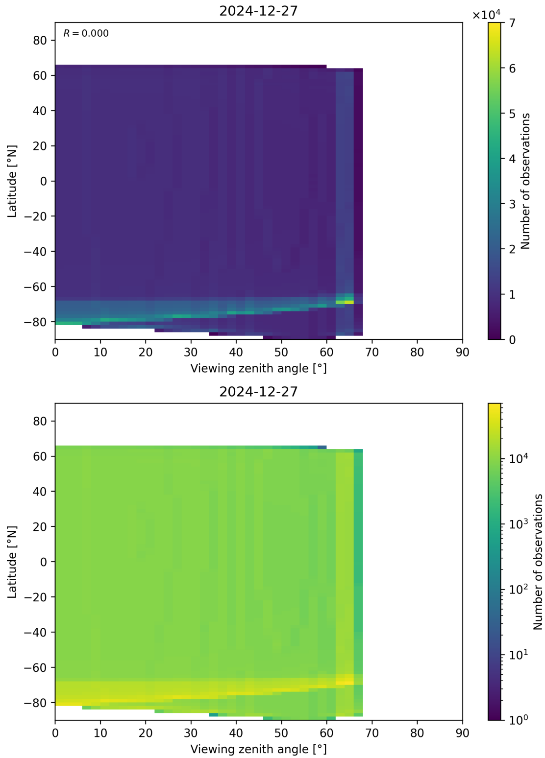
Figure 49: Scatter density plot of “Viewing zenith angle” against “Latitude” for 2024-12-27 to 2024-12-28.
