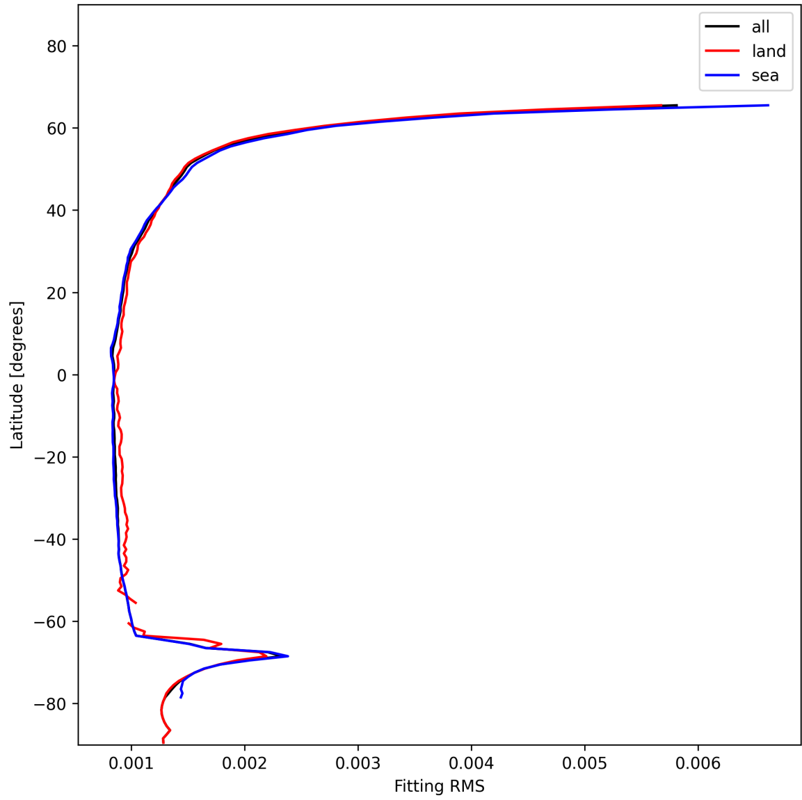
Figure 16: Zonal average of “Fitting RMS” for 2024-12-27 to 2024-12-28.
