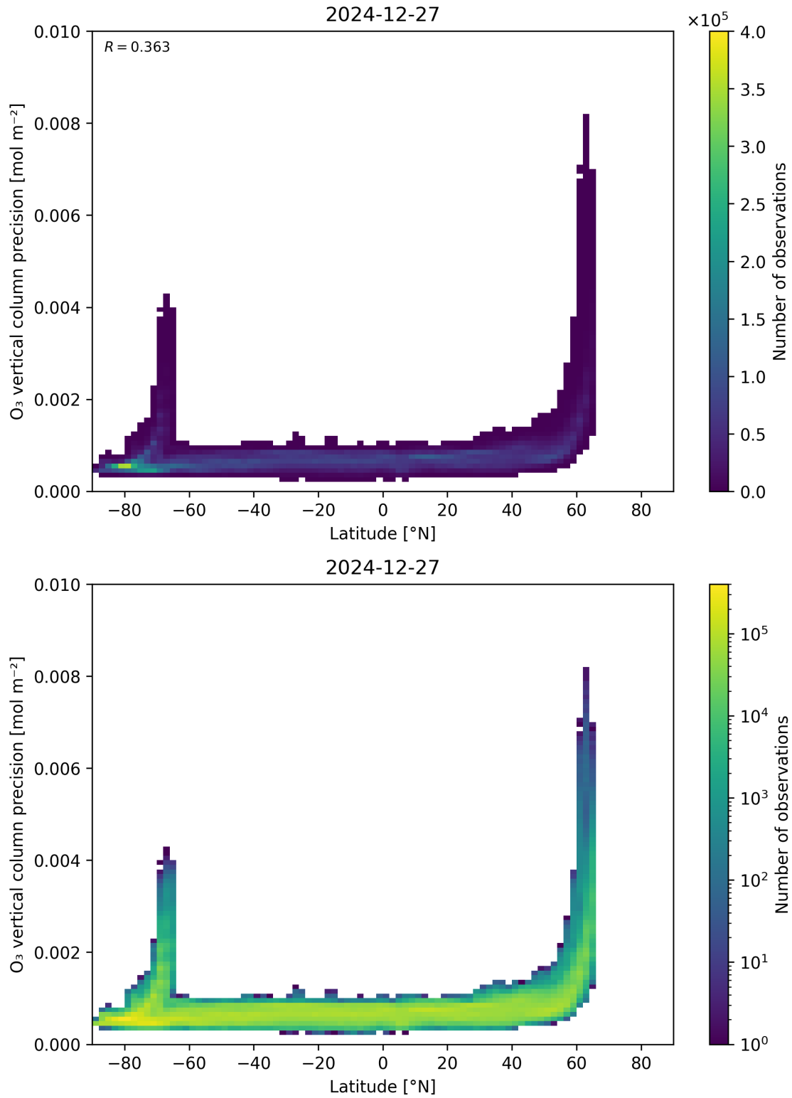
Figure 37: Scatter density plot of “Latitude” against “O 3 vertical column precision” for 2024-12-27 to 2024-12-28.
