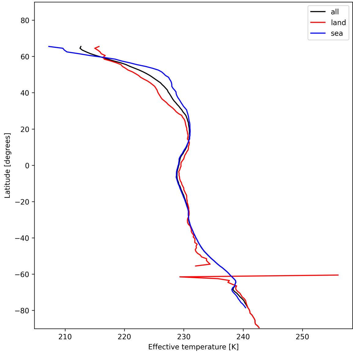
Figure 17: Zonal average of “Effective temperature” for 2024-12-27 to 2024-12-28.
