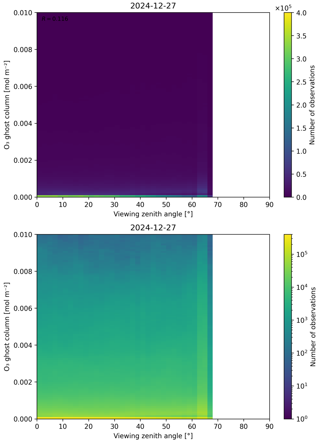
Figure 51: Scatter density plot of “Viewing zenith angle” against “O 3 ghost column” for 2024-12-27 to 2024-12-28.
