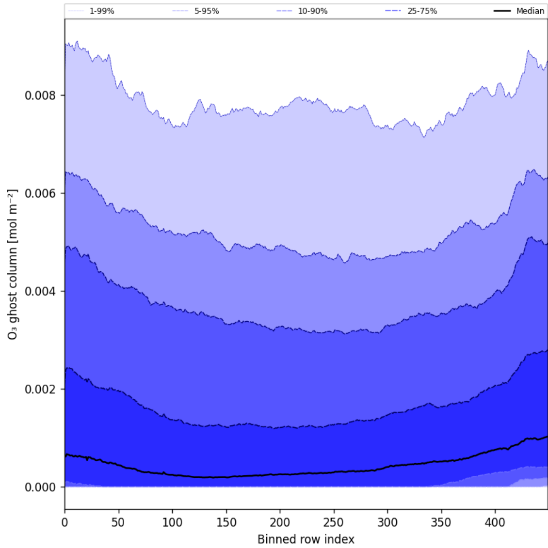
Figure 32: Along track statistics of “O 3 ghost column” for 2024-12-27 to 2024-12-28
