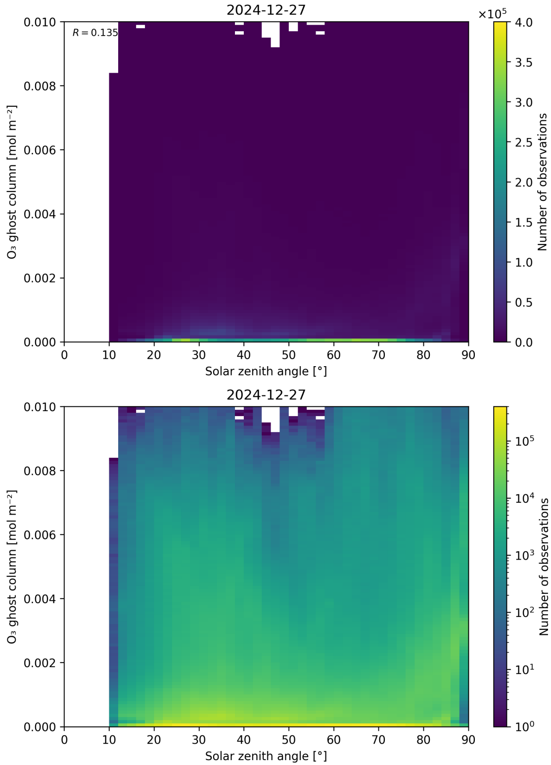
Figure 46: Scatter density plot of “Solar zenith angle” against “O 3 ghost column” for 2024-12-27 to 2024-12-28.
