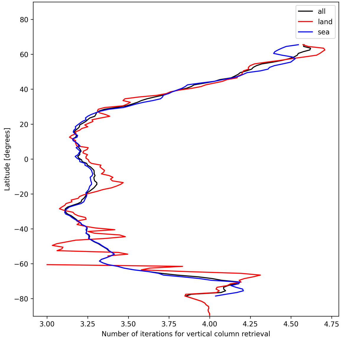
Figure 19: Zonal average of “Number of iterations for vertical column retrieval” for 2024-12-27 to 2024-12-28.
