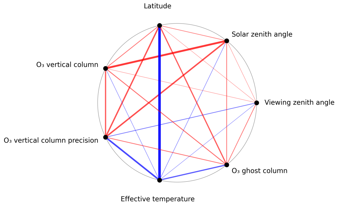
Figure 1: Map of correlation graph for 2024-12-27 to 2024-12-28.
