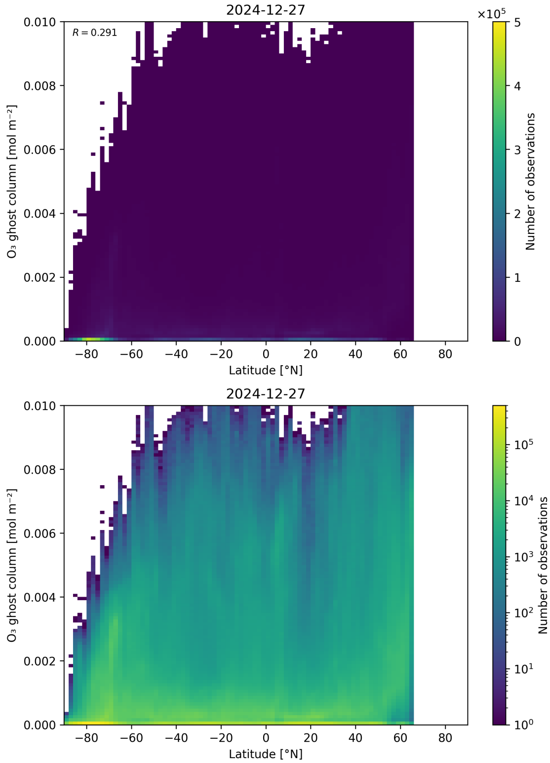
Figure 35: Scatter density plot of “Latitude” against “O 3 ghost column” for 2024-12-27 to 2024-12-28.
