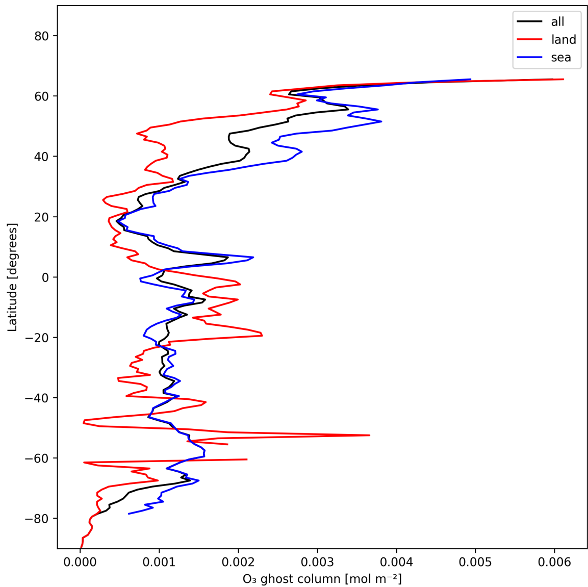
Figure 18: Zonal average of “O 3 ghost column” for 2024-12-27 to 2024-12-28.
