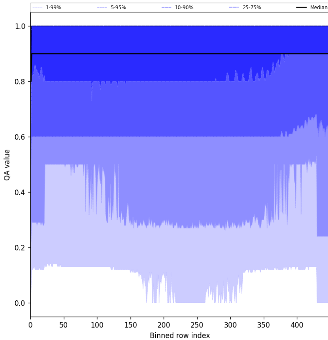
Figure 27: Along track statistics of “QA value” for 2024-12-27 to 2024-12-28
