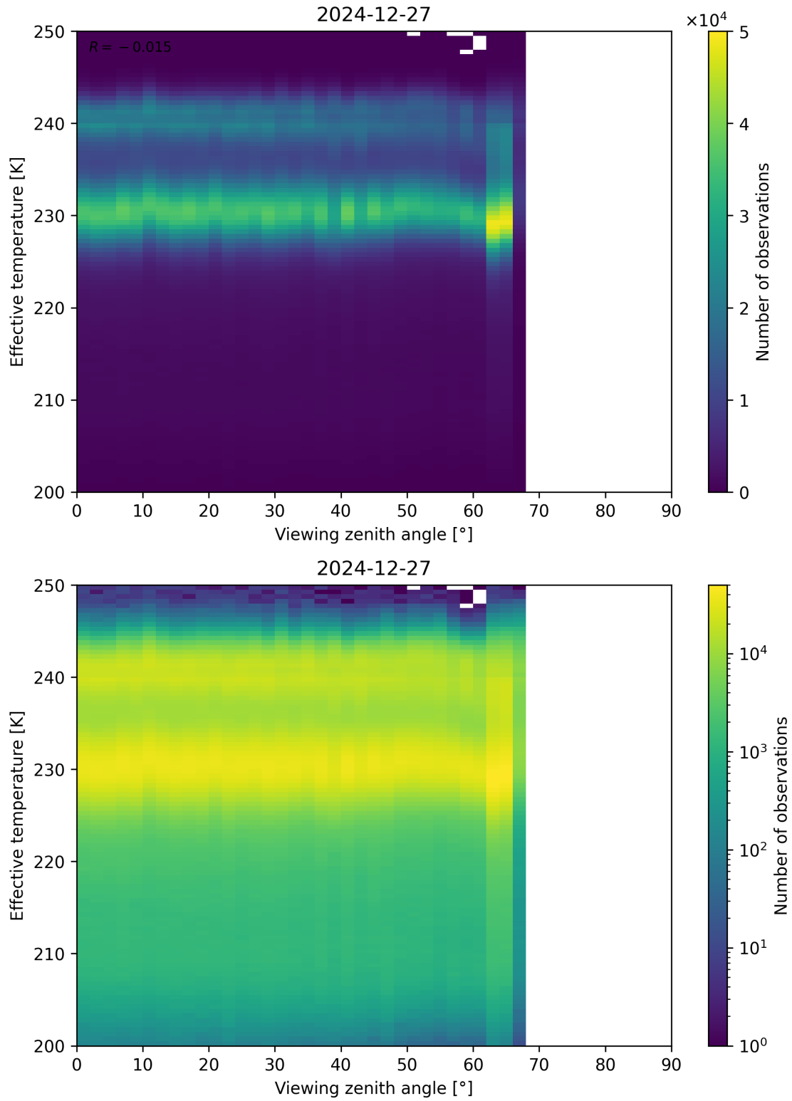
Figure 50: Scatter density plot of “Viewing zenith angle” against “Effective temperature” for 2024-12-27 to 2024-12-28.
