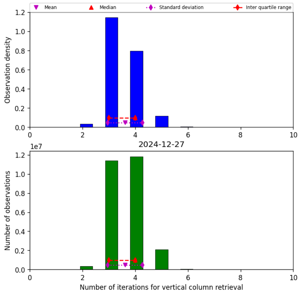
Figure 26: Histogram of “Number of iterations for vertical column retrieval” for 2024-12-27 to 2024-12-28
