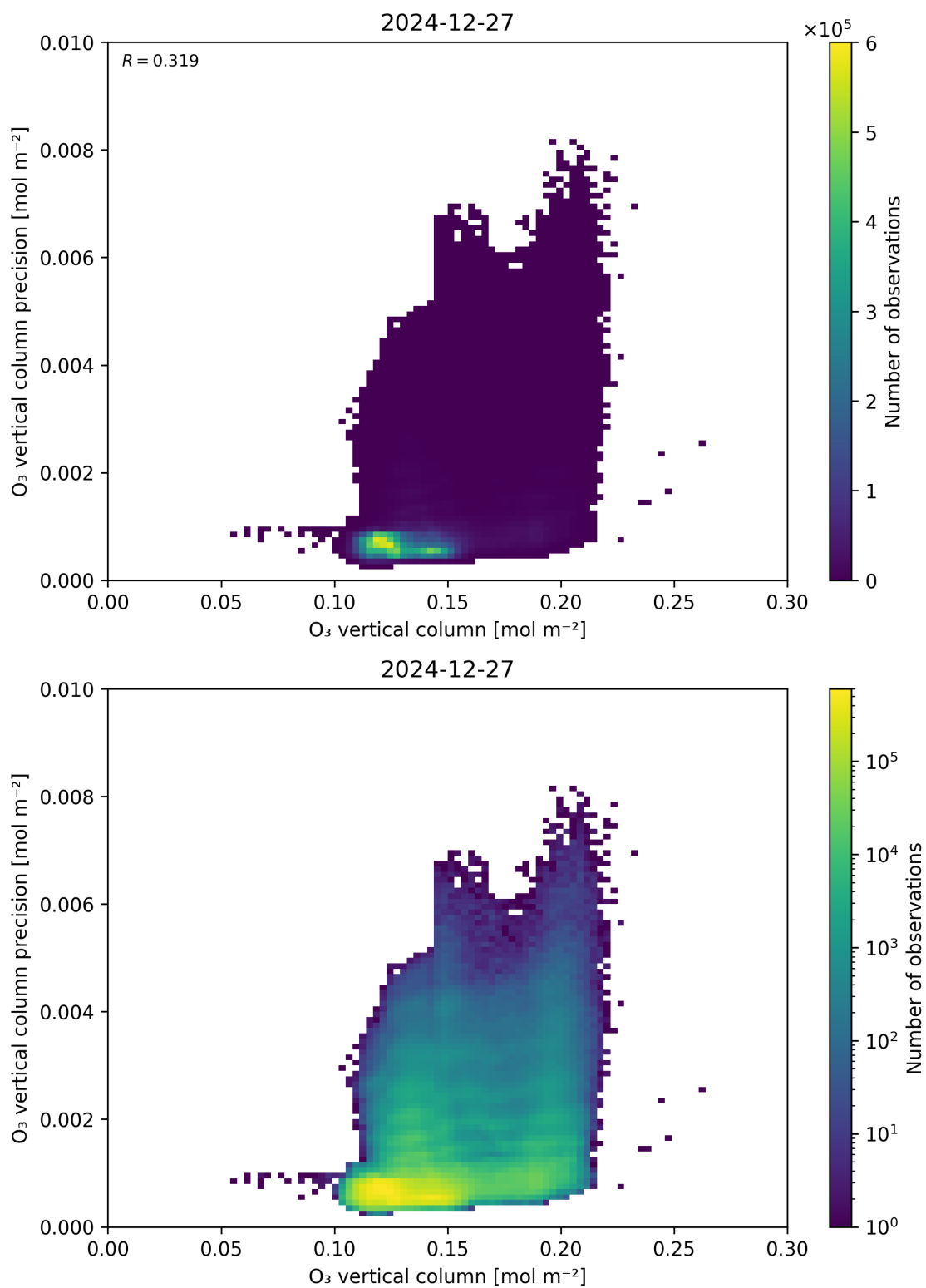
Figure 41: Scatter density plot of “O 3 vertical column” against “O 3 vertical column precision” for 2024-12-27 to 2024-12-28.
