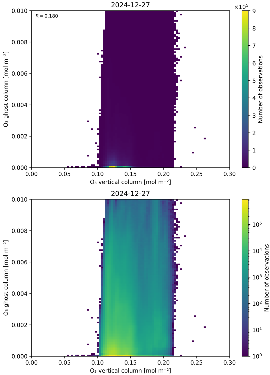
Figure 40: Scatter density plot of “O 3 vertical column” against “O 3 ghost column” for 2024-12-27 to 2024-12-28.
