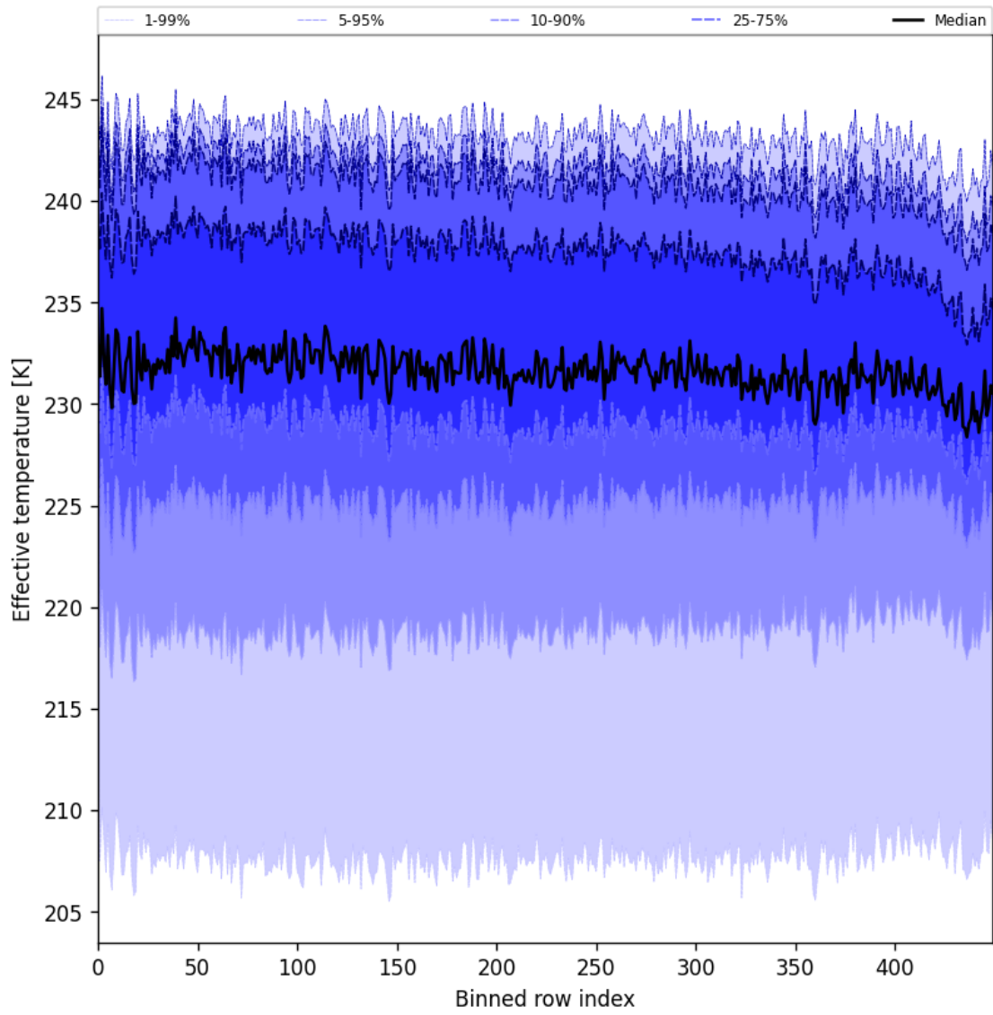
Figure 31: Along track statistics of “Effective temperature” for 2024-12-27 to 2024-12-28
