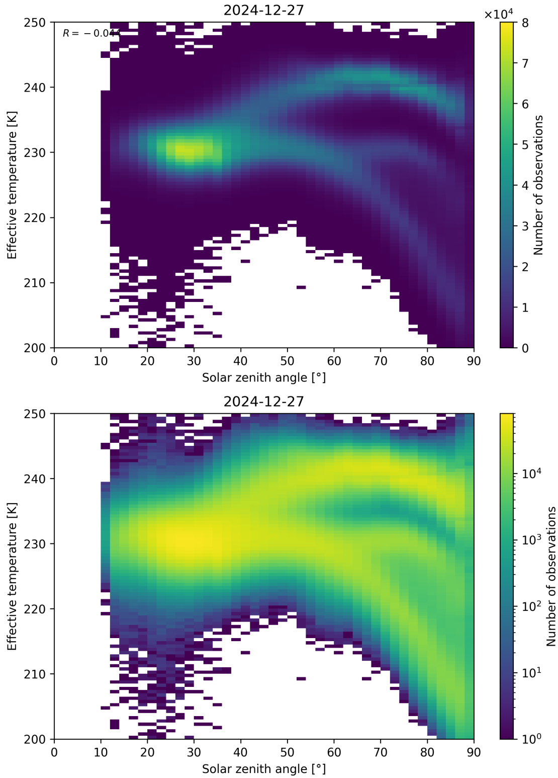
Figure 45: Scatter density plot of “Solar zenith angle” against “Effective temperature” for 2024-12-27 to 2024-12-28.
