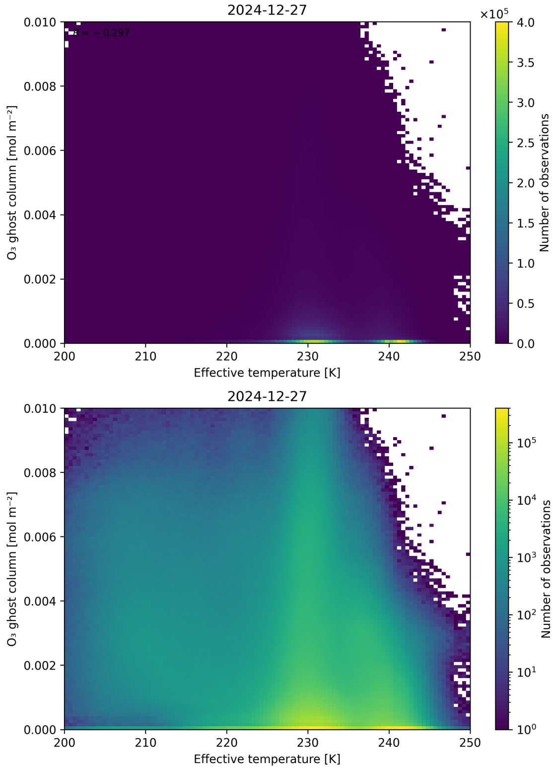
Figure 38: Scatter density plot of “Effective temperature” against “O 3 ghost column” for 2024-12-27 to 2024-12-28.
