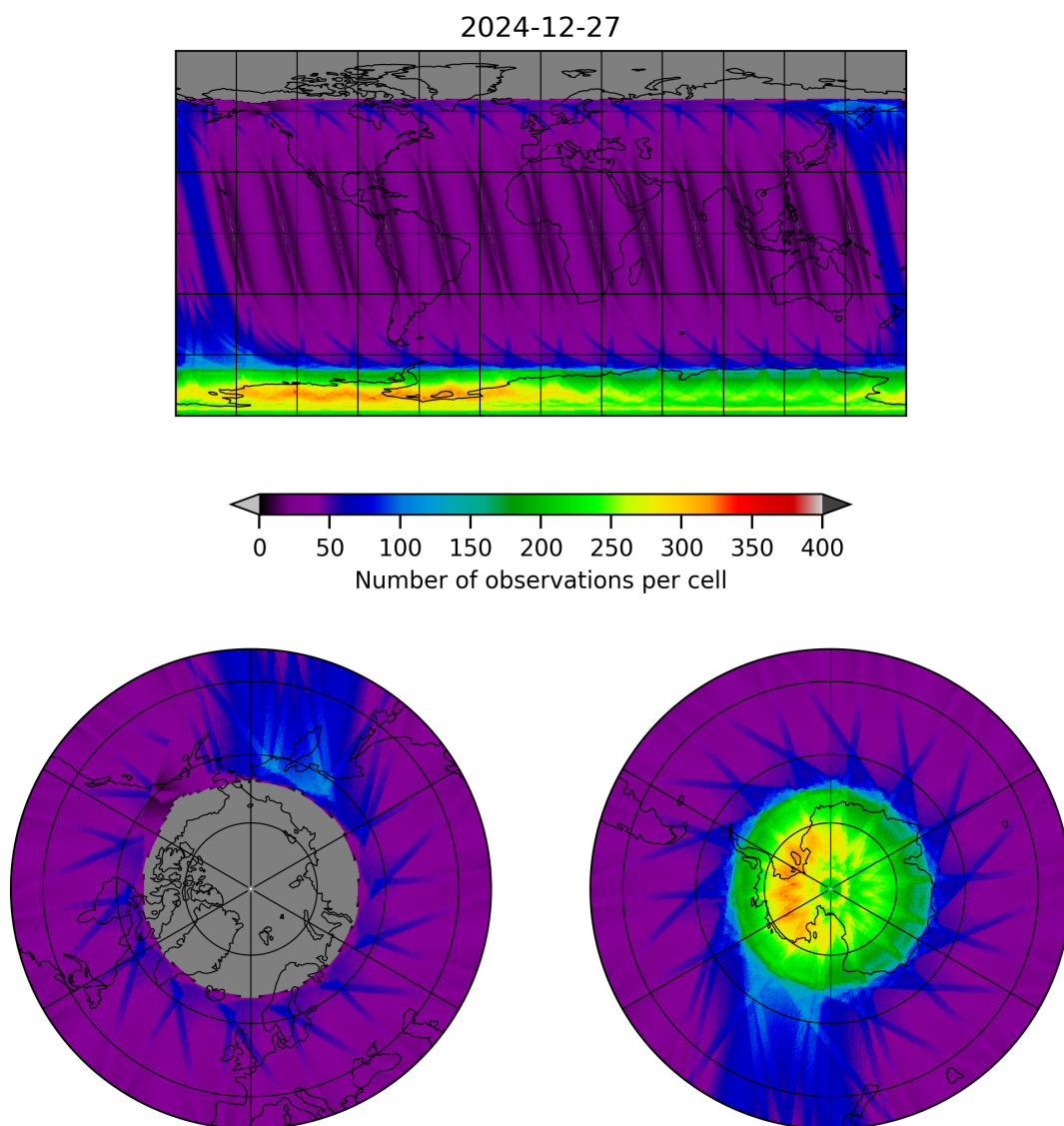
Figure 12: Map of the number of observations for 2024-12-27 to 2024-12-28
