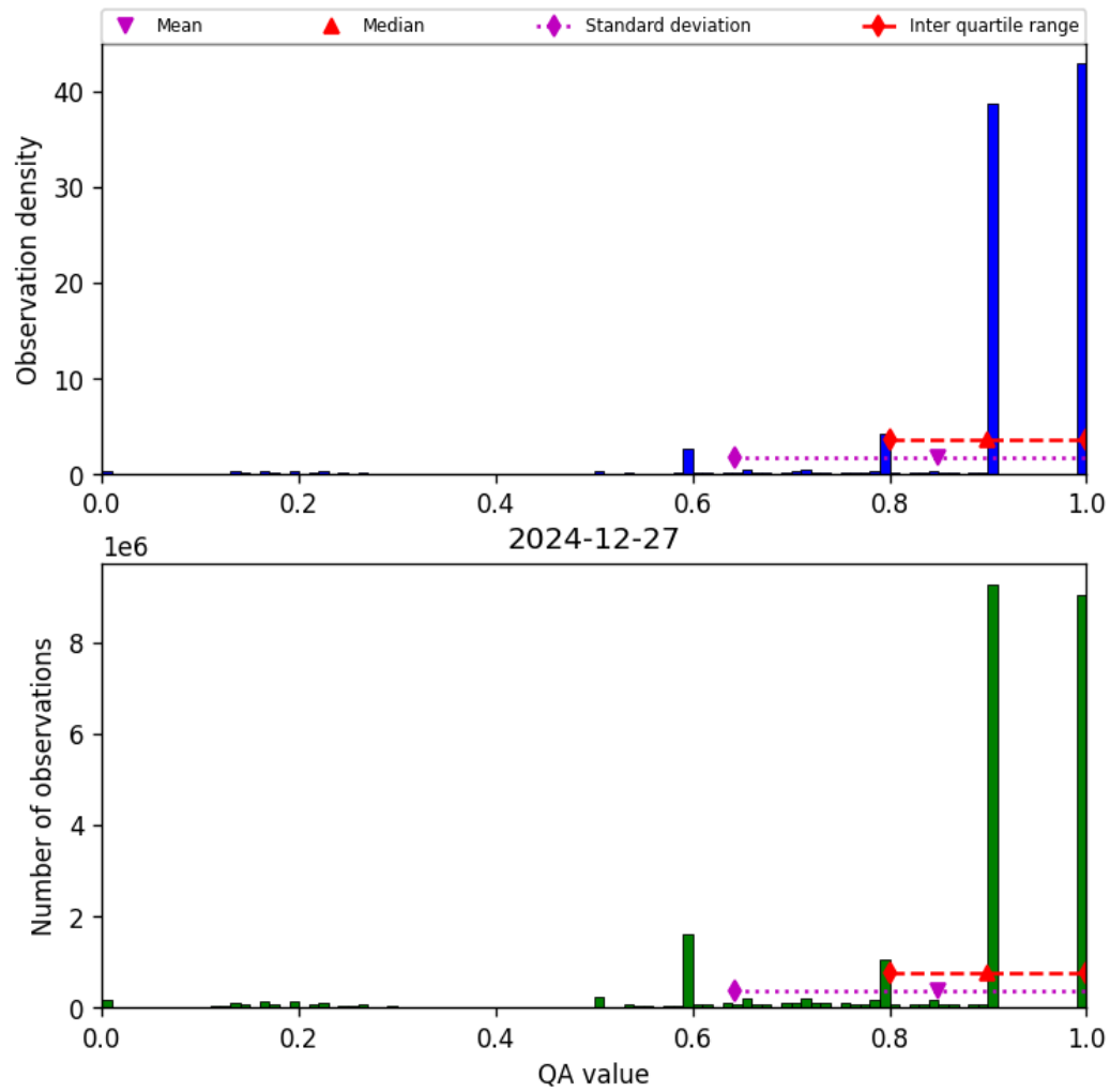
Figure 20: Histogram of “QA value” for 2024-12-27 to 2024-12-28
