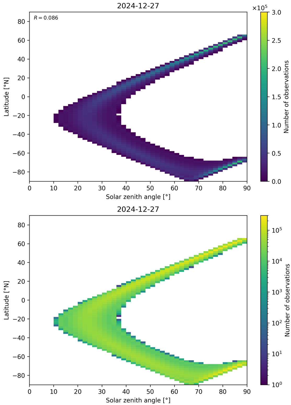
Figure 44: Scatter density plot of “Solar zenith angle” against “Latitude” for 2024-12-27 to 2024-12-28.
