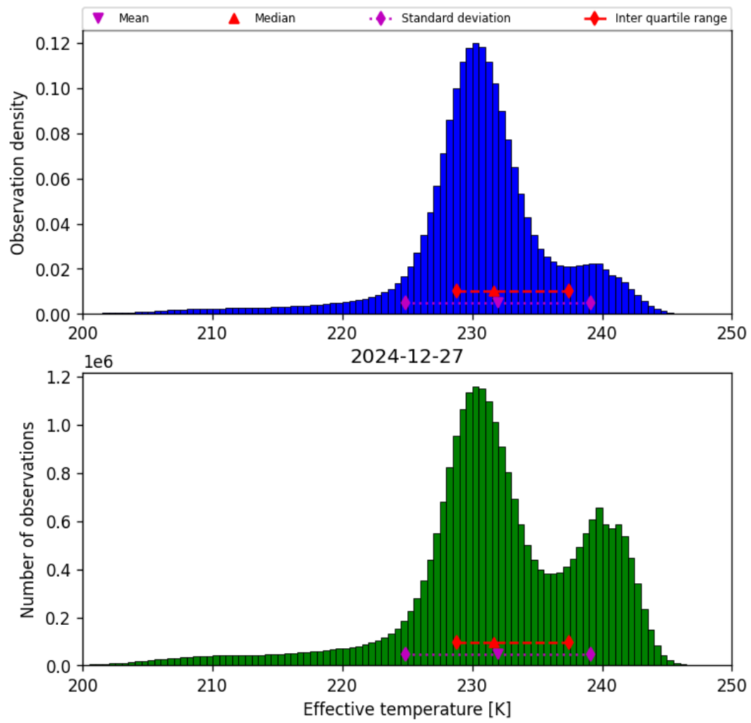
Figure 24: Histogram of “Effective temperature” for 2024-12-27 to 2024-12-28
