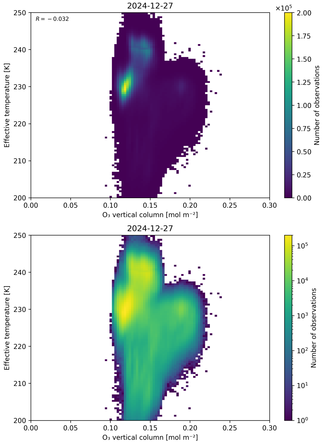
Figure 39: Scatter density plot of “O 3 vertical column” against “Effective temperature” for 2024-12-27 to 2024-12-28.
