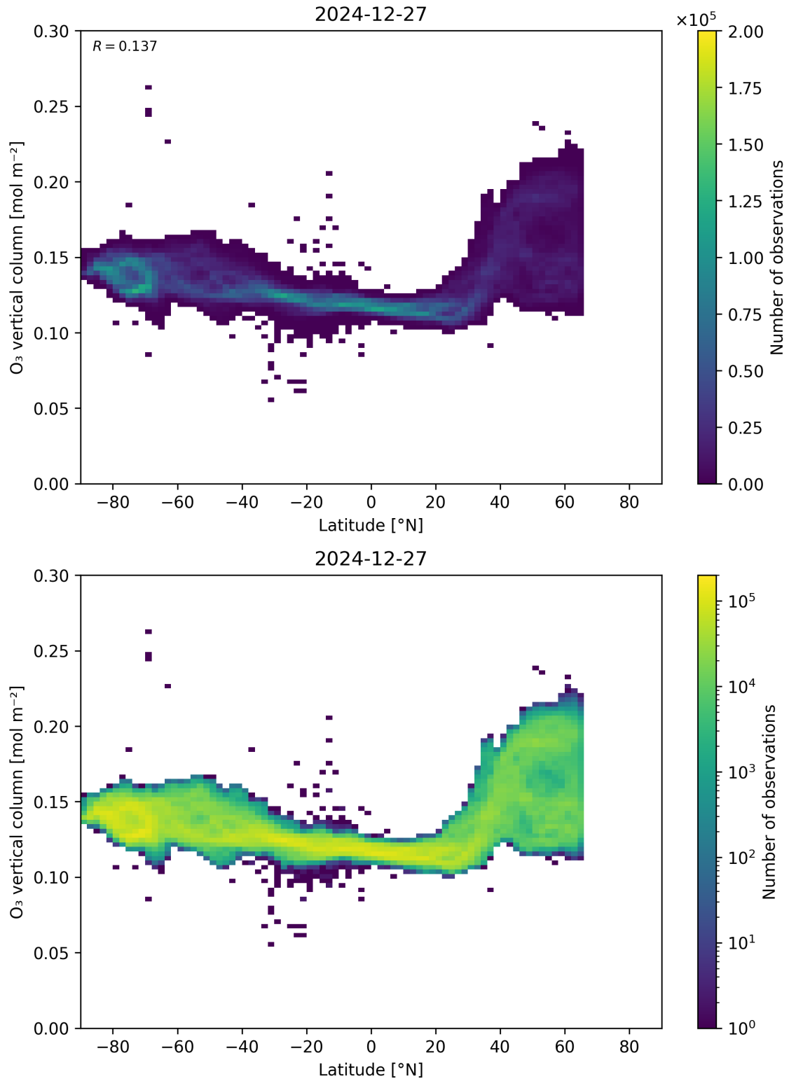
Figure 36: Scatter density plot of “Latitude” against “O 3 vertical column” for 2024-12-27 to 2024-12-28.
