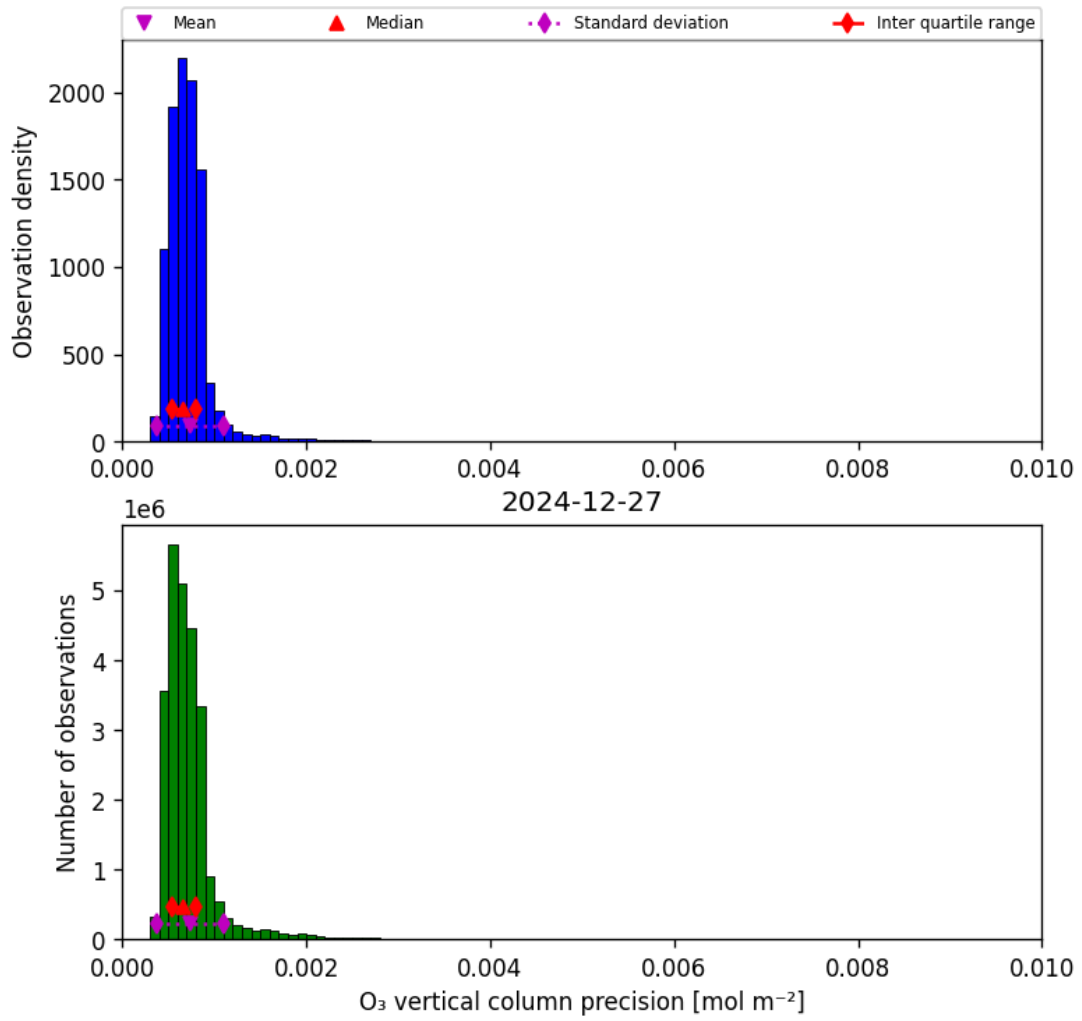
Figure 22: Histogram of “O 3 vertical column precision” for 2024-12-27 to 2024-12-28
