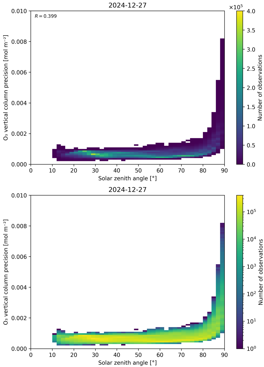
Figure 48: Scatter density plot of “Solar zenith angle” against “O 3 vertical column precision” for 2024-12-27 to 2024-12-28.
