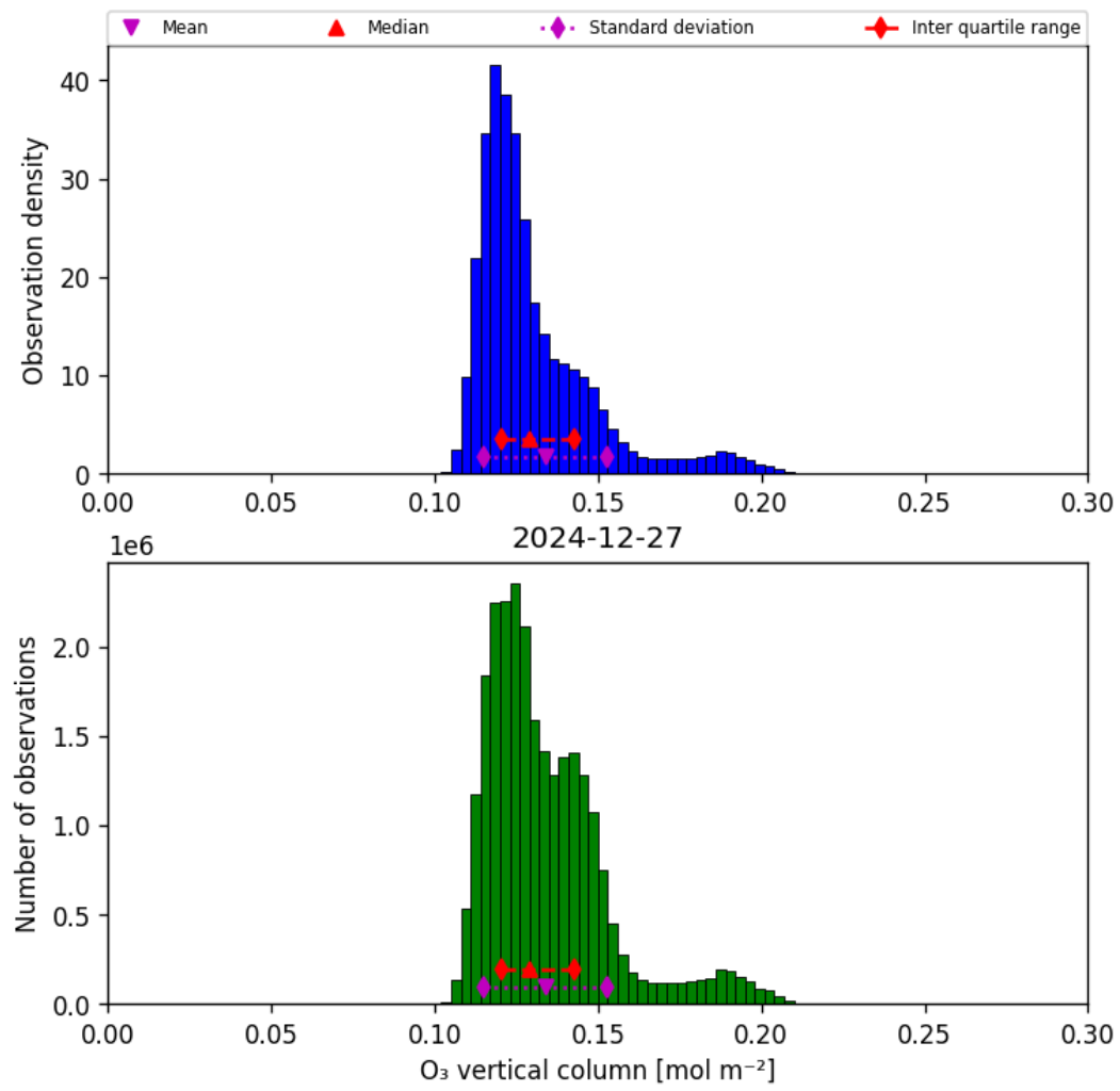
Figure 21: Histogram of “O 3 vertical column” for 2024-12-27 to 2024-12-28
