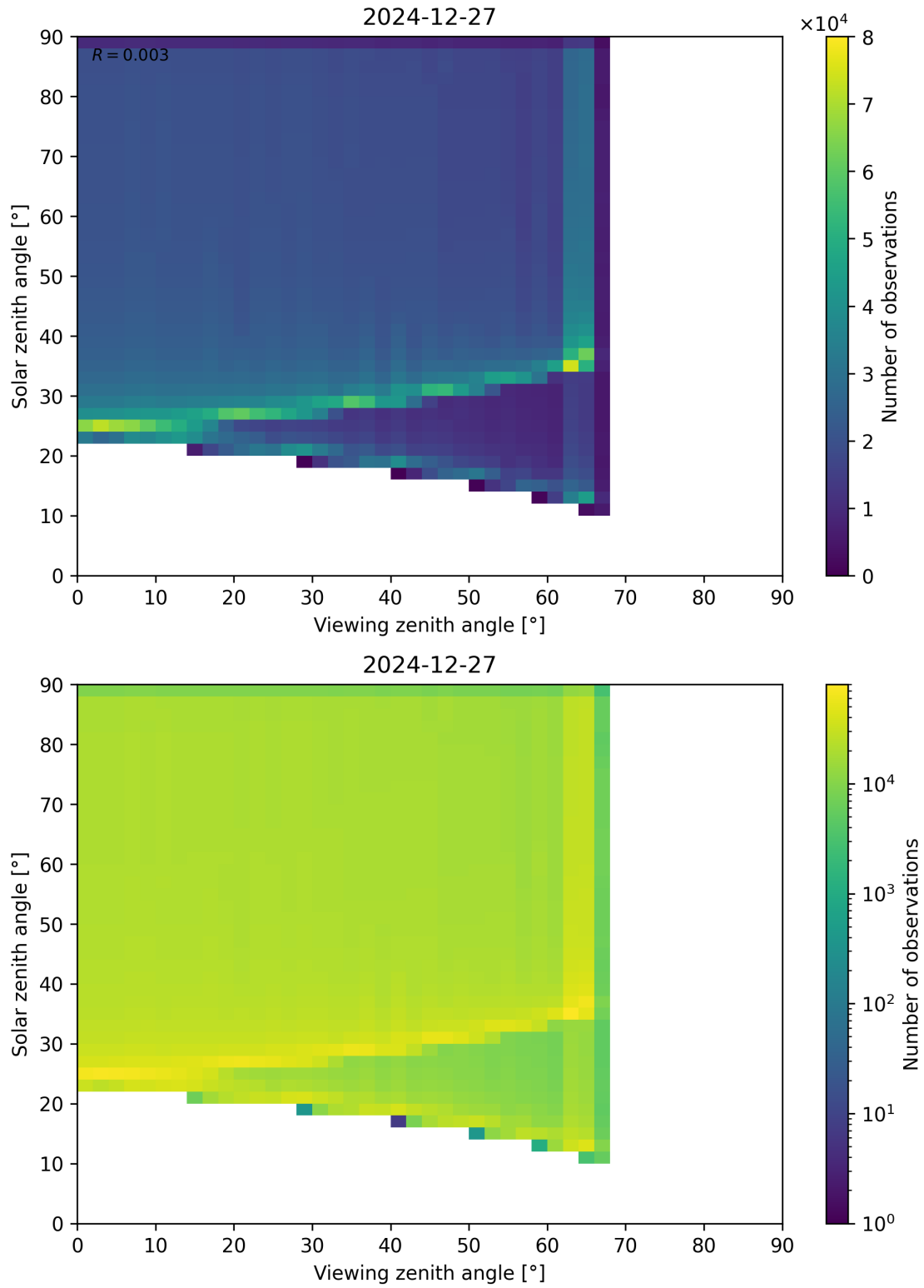
Figure 54: Scatter density plot of “Viewing zenith angle” against “Solar zenith angle” for 2024-12-27 to 2024-12-28.
