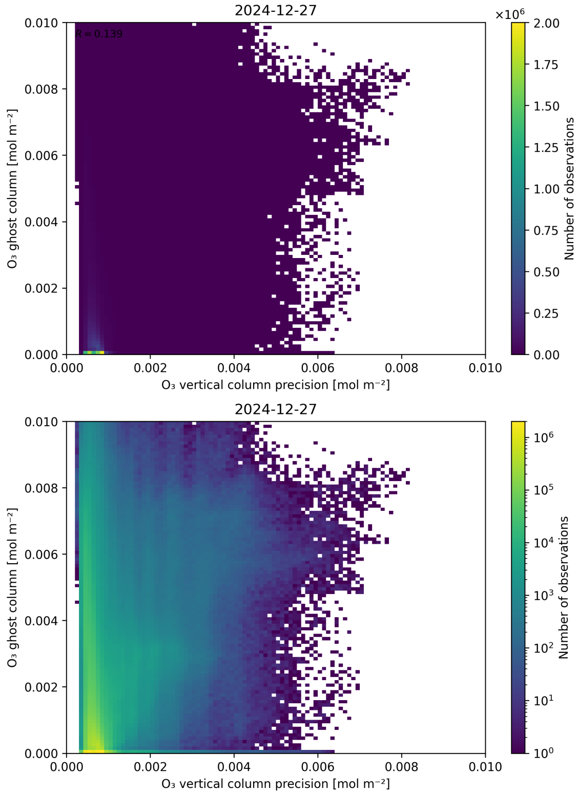
Figure 43: Scatter density plot of “ \text{O}_3 vertical column precision” against “ \text{O}_3 ghost column” for 2024-12-27 to 2024-12-28.
