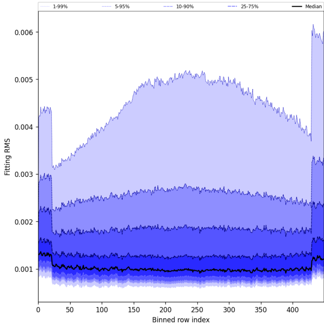
Figure 30: Along track statistics of “Fitting RMS” for 2024-12-27 to 2024-12-28
