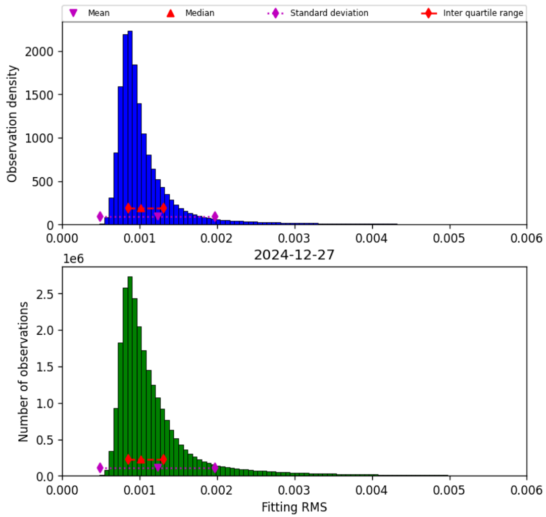
Figure 23: Histogram of “Fitting RMS” for 2024-12-27 to 2024-12-28
