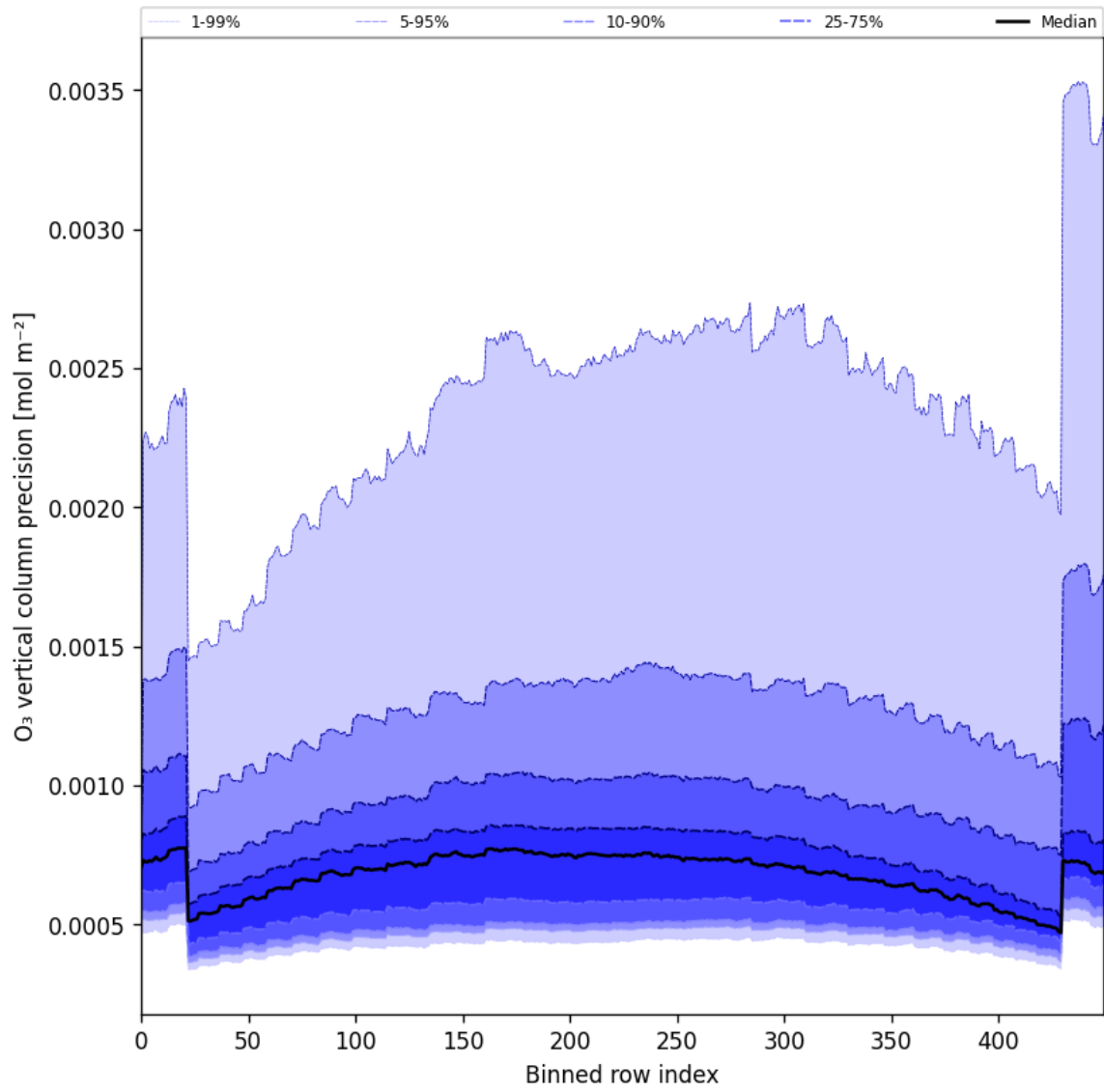
Figure 29: Along track statistics of “O 3 vertical column precision” for 2024-12-27 to 2024-12-28
