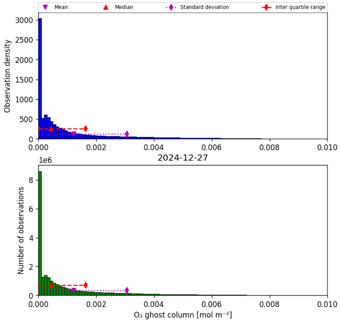
Figure 25: Histogram of “O 3 ghost column” for 2024-12-27 to 2024-12-28
