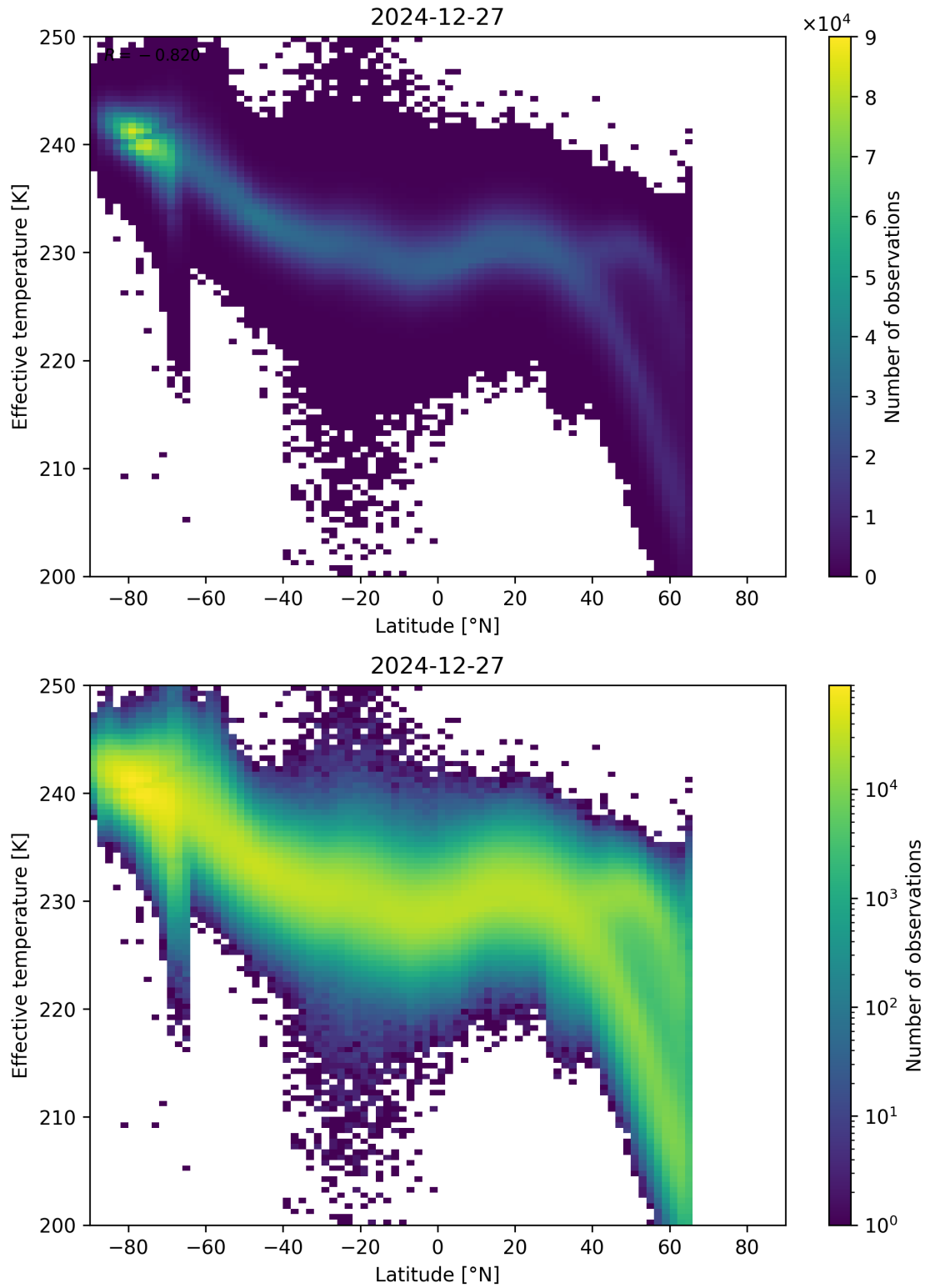
Figure 34: Scatter density plot of “Latitude” against “Effective temperature” for 2024-12-27 to 2024-12-28.
