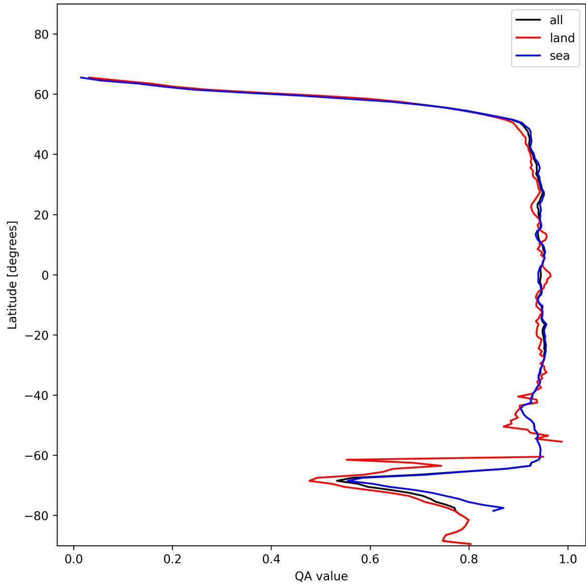
Figure 13: Zonal average of “QA value” for 2024-12-27 to 2024-12-28.
