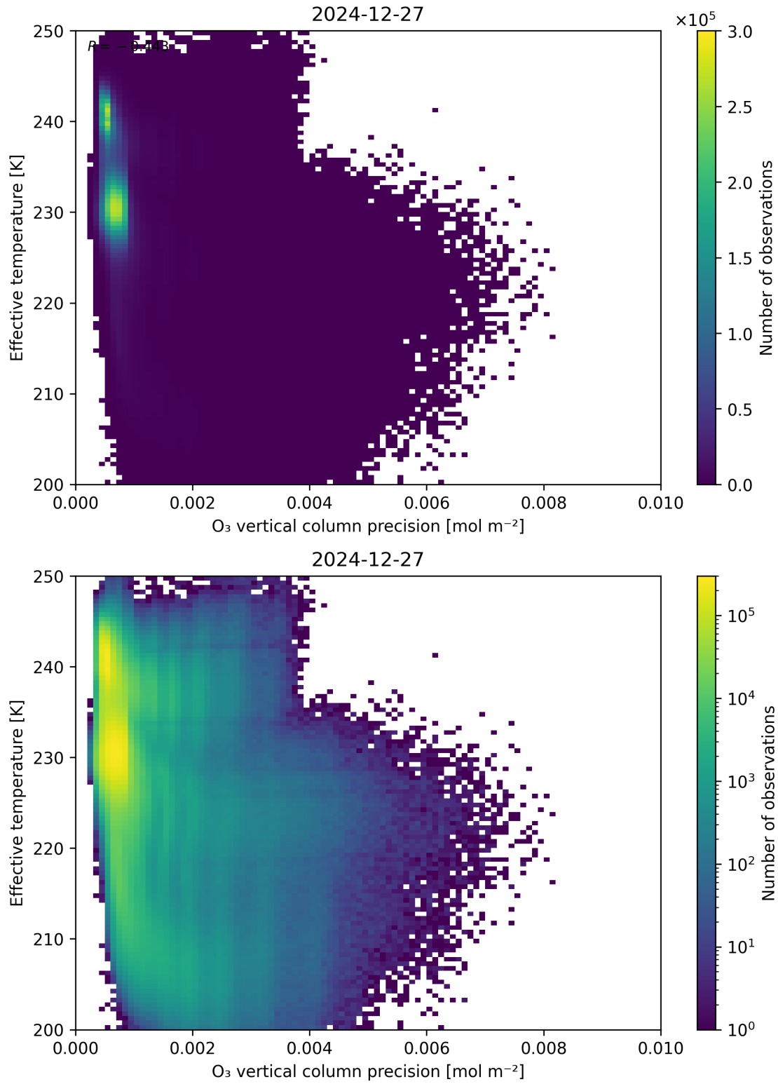
Figure 42: Scatter density plot of “O 3 vertical column precision” against “Effective temperature” for 2024-12-27 to 2024-12-28.
