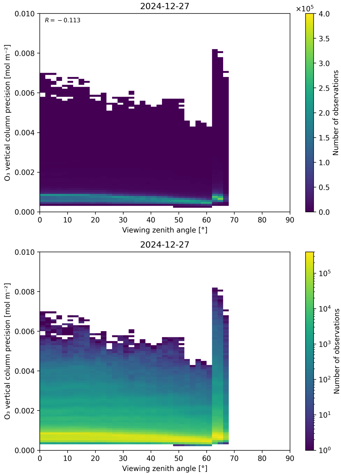
Figure 53: Scatter density plot of “Viewing zenith angle” against “O 3 vertical column precision” for 2024-12-27 to 2024-12-28.
