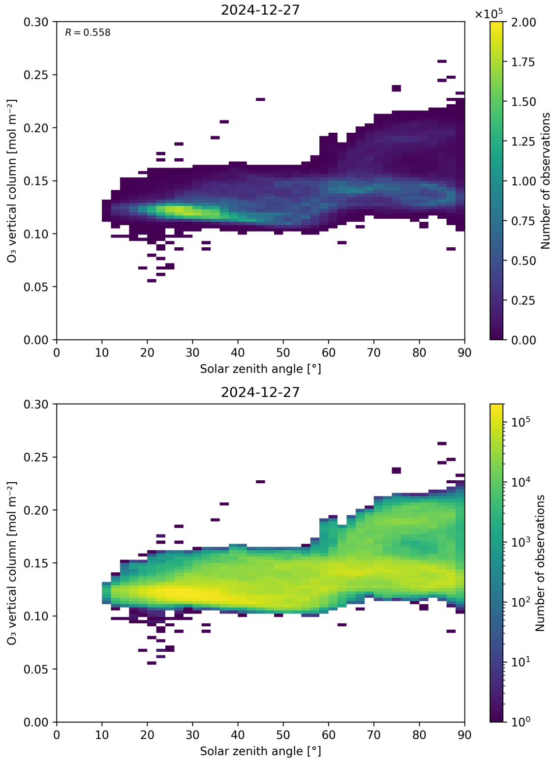
Figure 47: Scatter density plot of “Solar zenith angle” against “O 3 vertical column” for 2024-12-27 to 2024-12-28.
