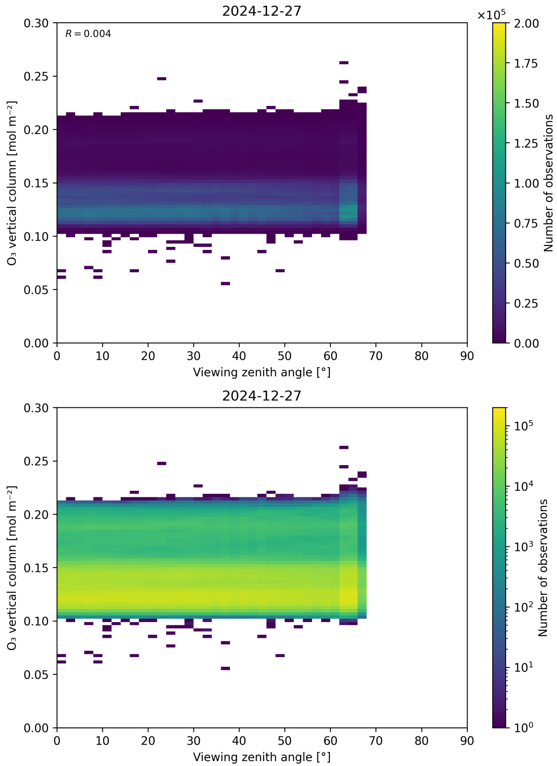
Figure 52: Scatter density plot of “Viewing zenith angle” against “O 3 vertical column” for 2024-12-27 to 2024-12-28.
