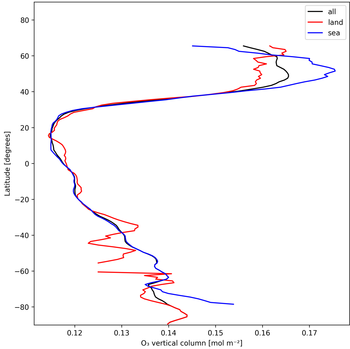
Figure 14: Zonal average of “O 3 vertical column” for 2024-12-27 to 2024-12-28.
