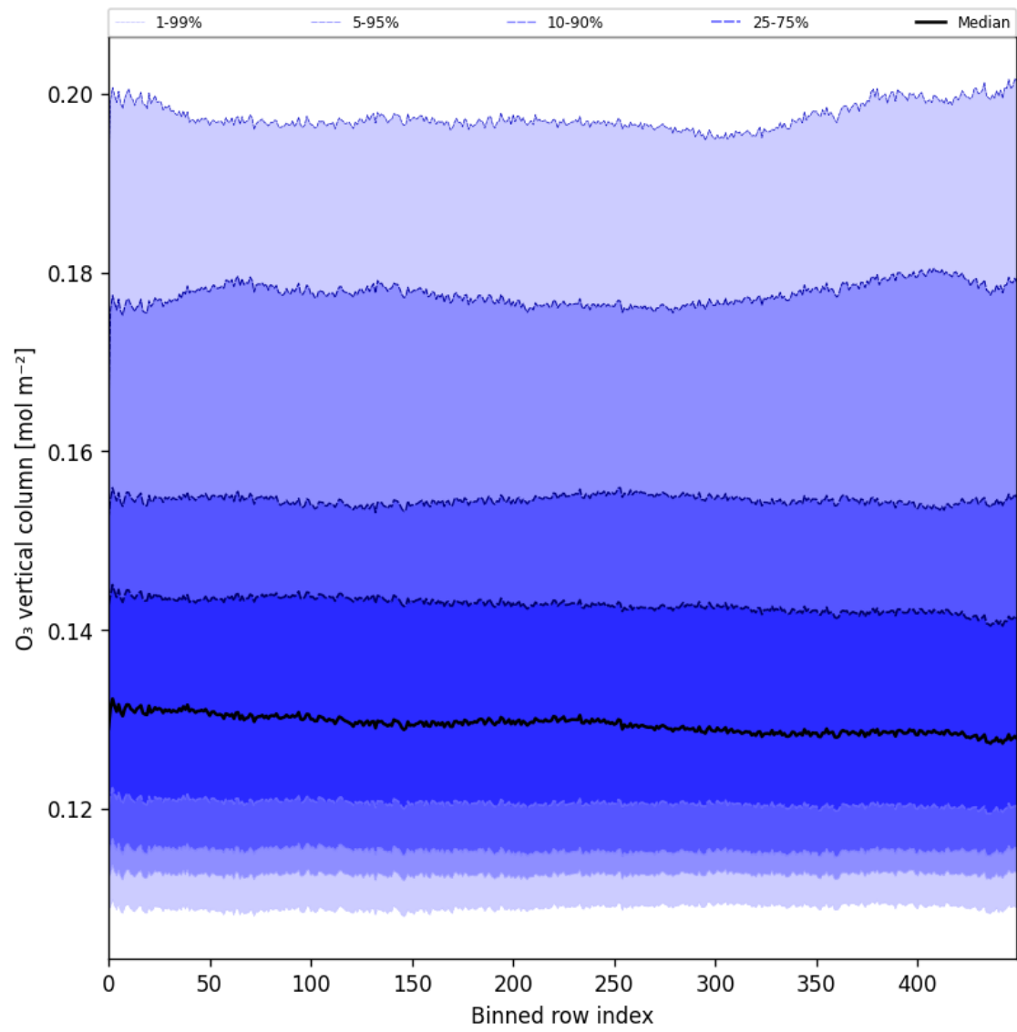
Figure 28: Along track statistics of “O 3 vertical column” for 2024-12-27 to 2024-12-28
