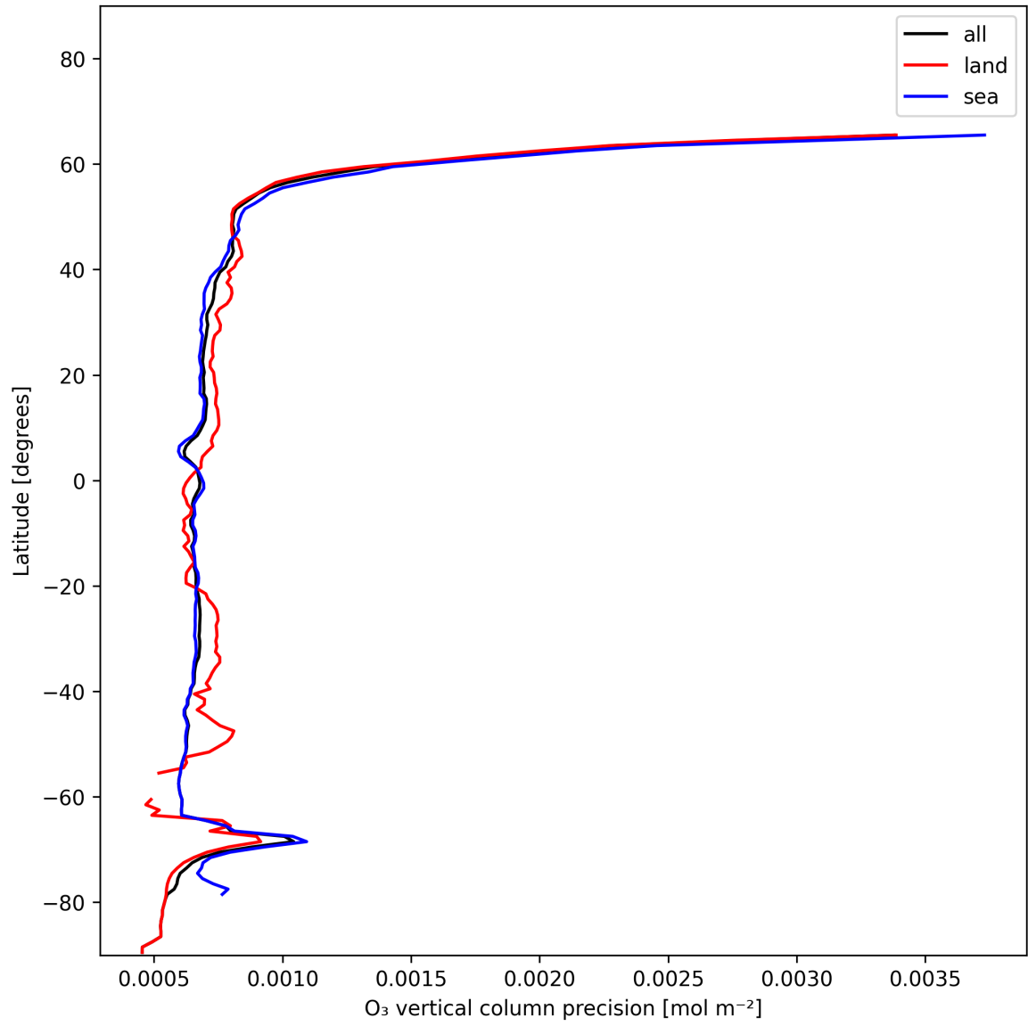
Figure 15: Zonal average of "O 3 vertical column precision" for 2024-12-27 to 2024-12-28.
