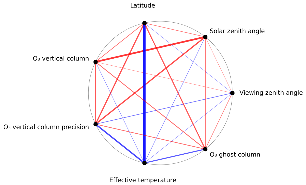
Figure 1: Map of correlation graph for 2024-12-27 to 2024-12-29.
