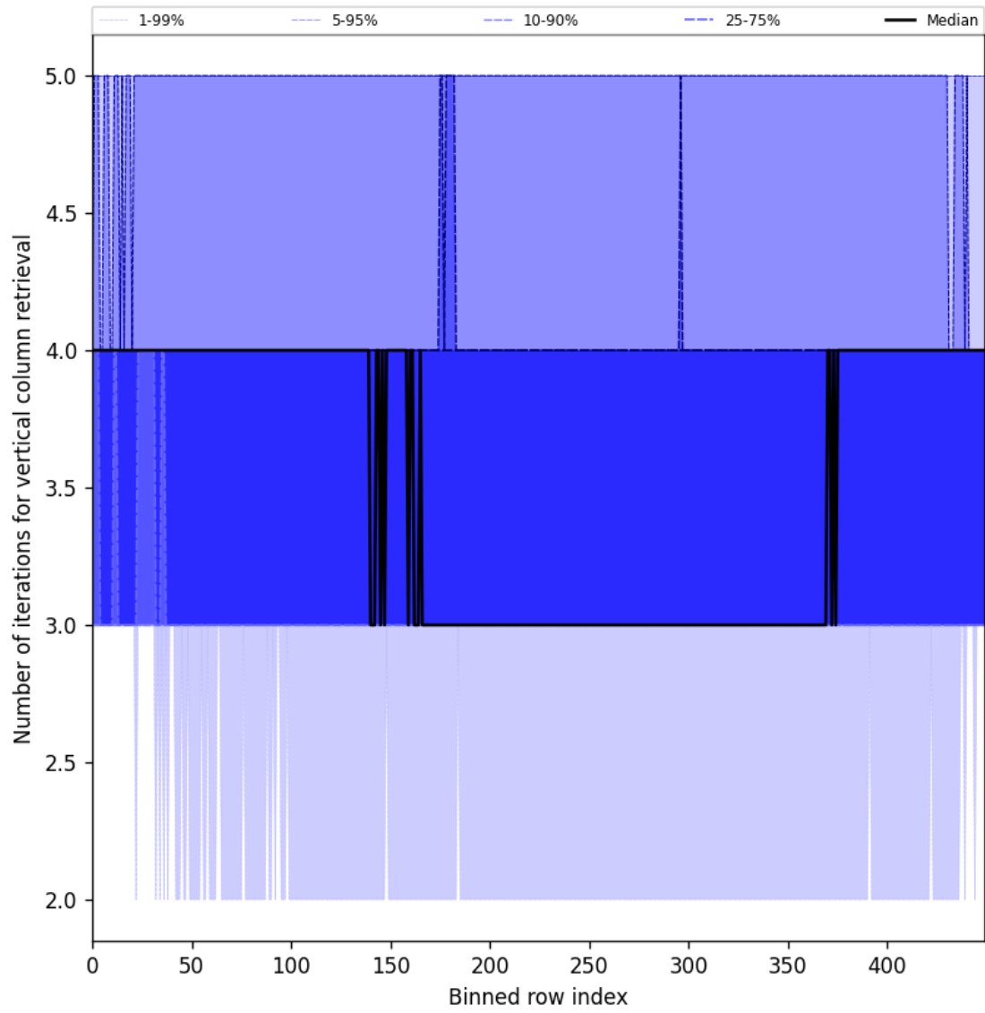
Figure 33: Along track statistics of “Number of iterations for vertical column retrieval” for 2024-12-27 to 2024-12-29
