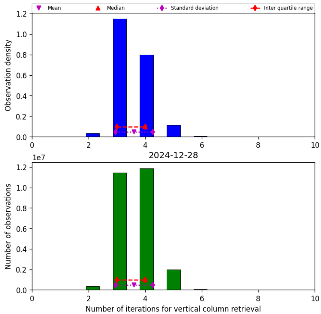
Figure 26: Histogram of “Number of iterations for vertical column retrieval” for 2024-12-27 to 2024-12-29
