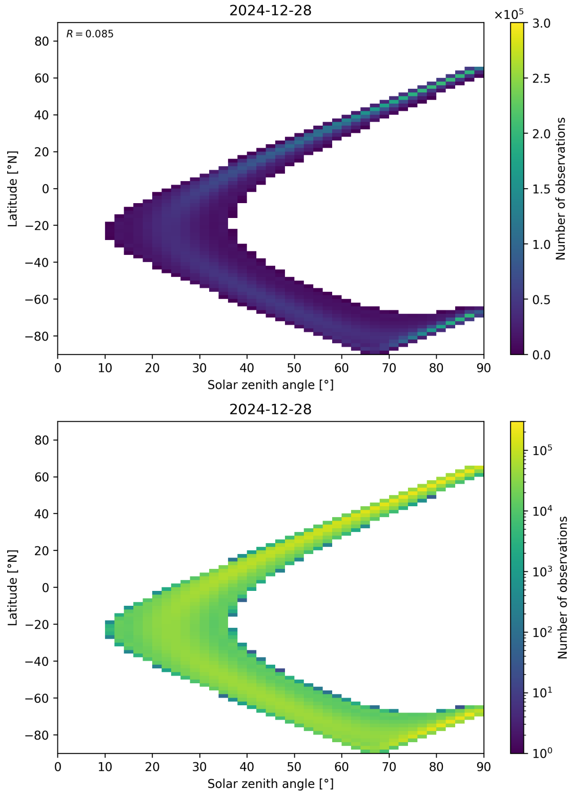
Figure 44: Scatter density plot of “Solar zenith angle” against “Latitude” for 2024-12-27 to 2024-12-29.
