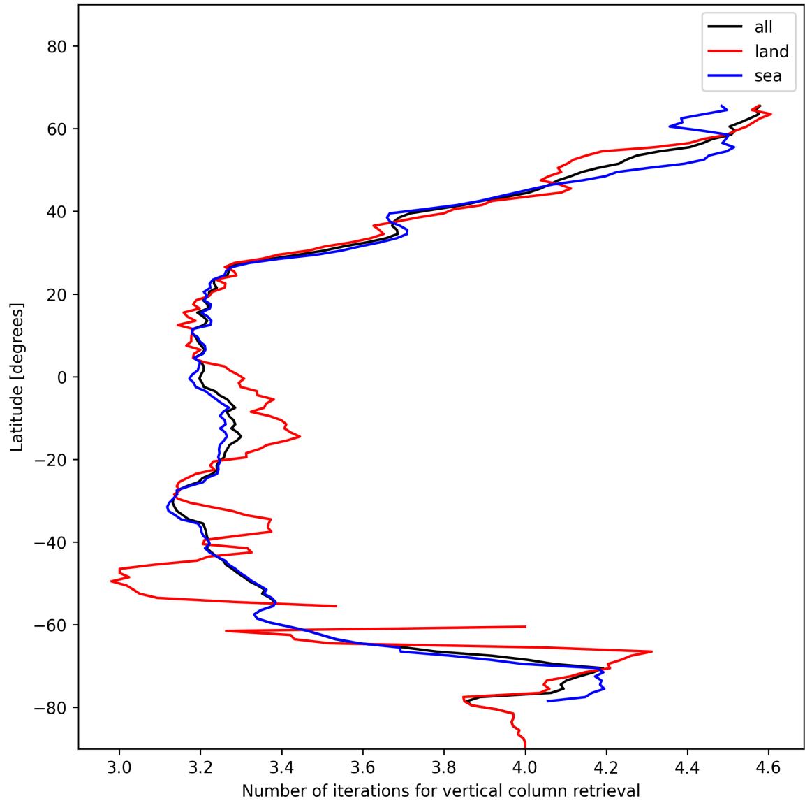
Figure 19: Zonal average of “Number of iterations for vertical column retrieval” for 2024-12-27 to 2024-12-29.
