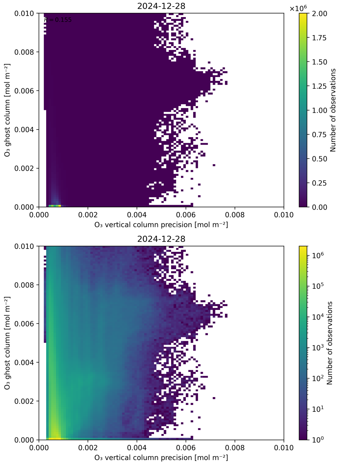
Figure 43: Scatter density plot of “ \text{O}_3 vertical column precision” against “ \text{O}_3 ghost column” for 2024-12-27 to 2024-12-29.
