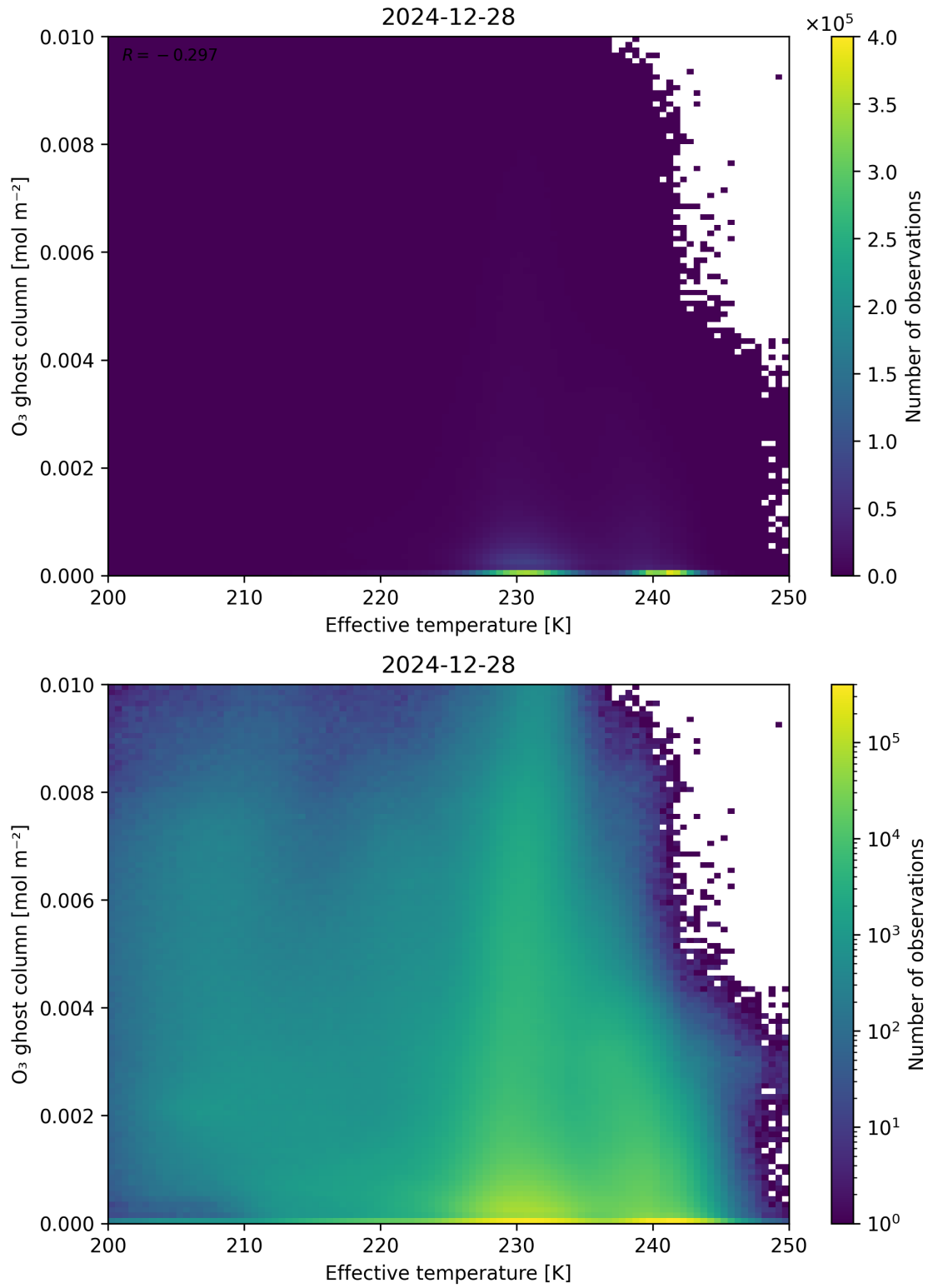
Figure 38: Scatter density plot of “Effective temperature” against “O 3 ghost column” for 2024-12-27 to 2024-12-29.
