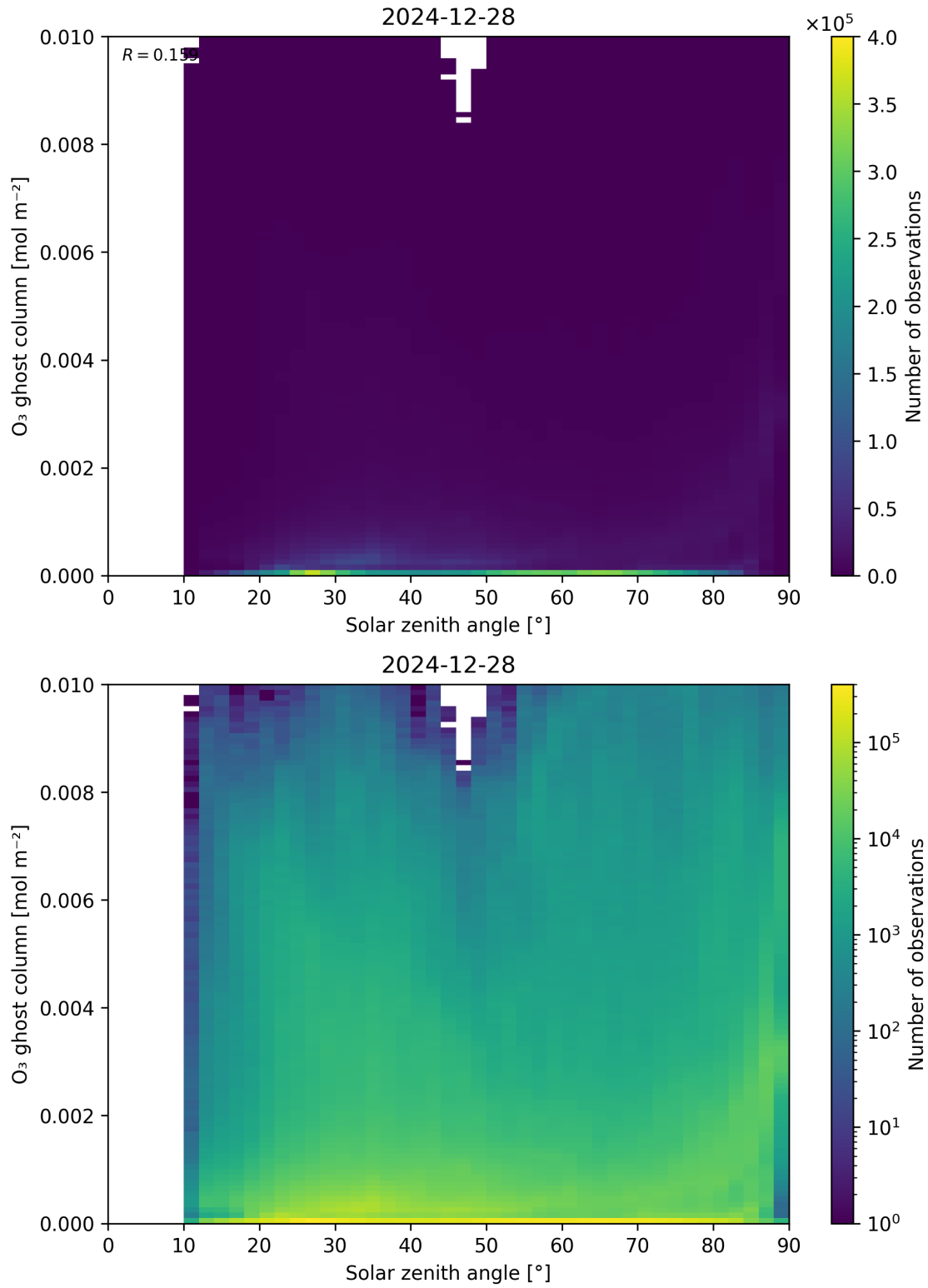
Figure 46: Scatter density plot of “Solar zenith angle” against “O 3 ghost column” for 2024-12-27 to 2024-12-29.
