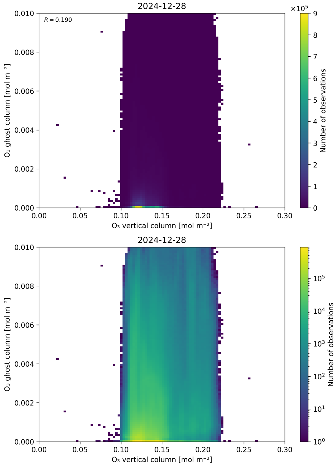
Figure 40: Scatter density plot of “O 3 vertical column” against “O 3 ghost column” for 2024-12-27 to 2024-12-29.
