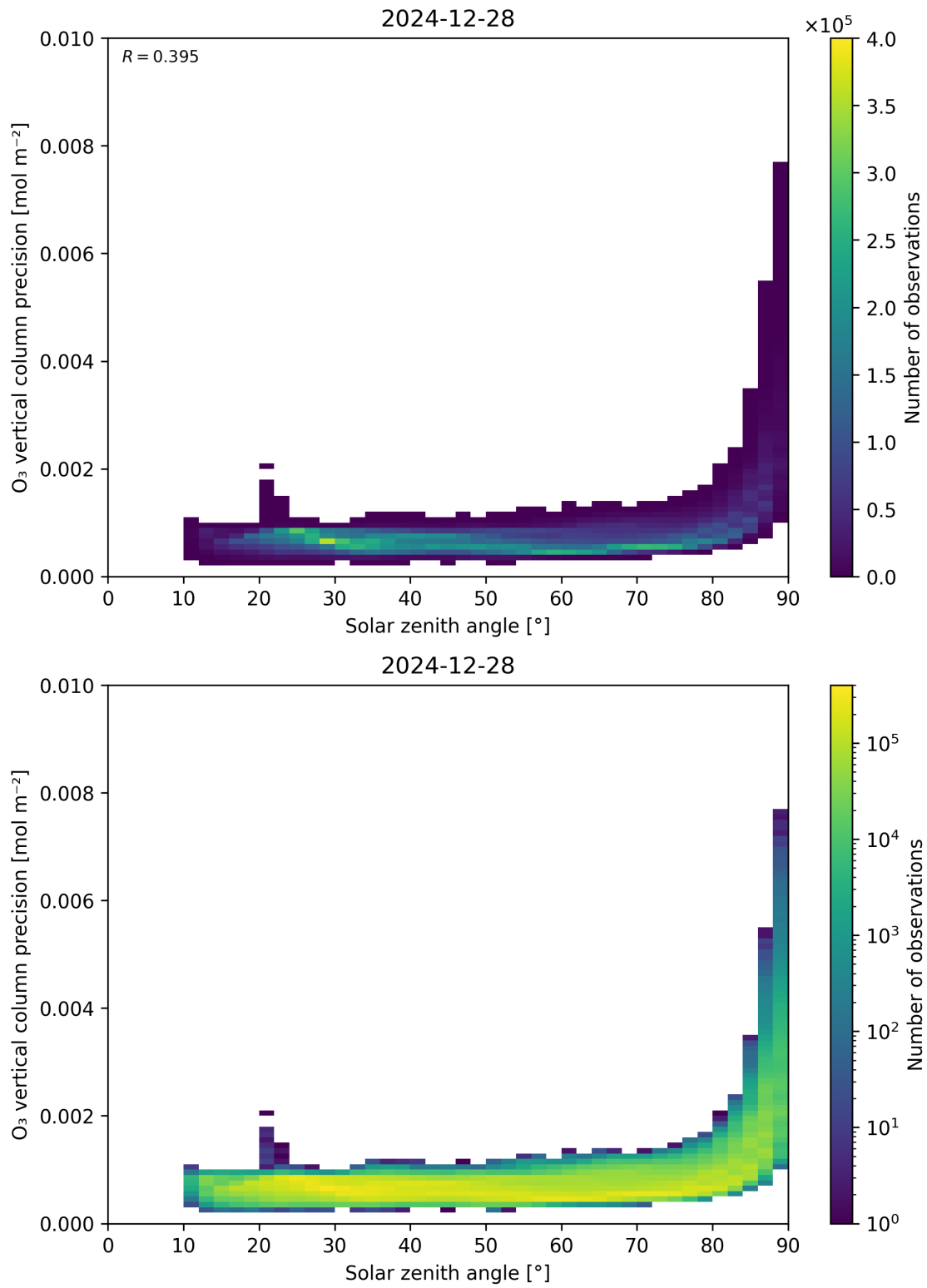
Figure 48: Scatter density plot of “Solar zenith angle” against “O 3 vertical column precision” for 2024-12-27 to 2024-12-29.
