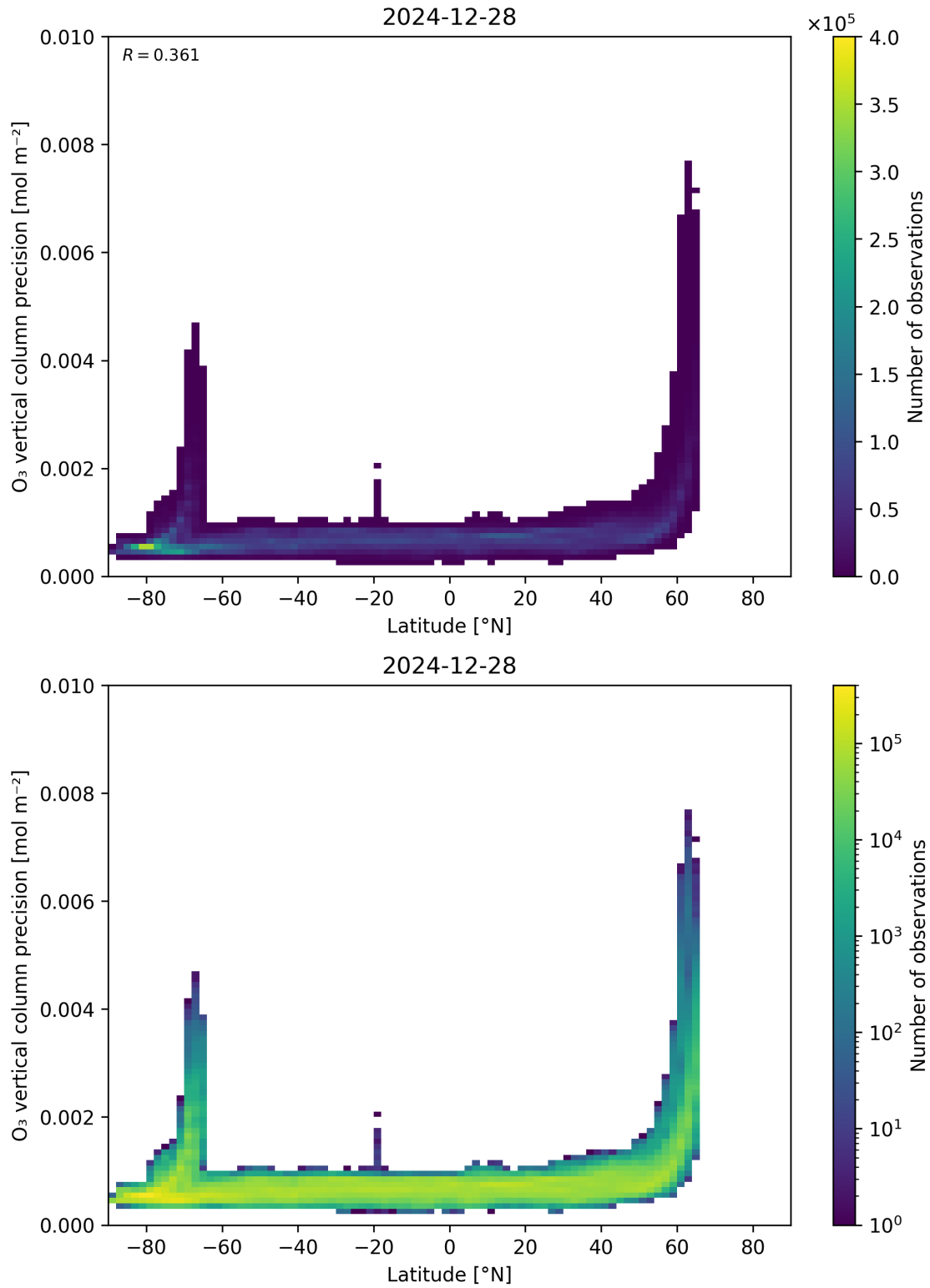
Figure 37: Scatter density plot of “Latitude” against “O 3 vertical column precision” for 2024-12-27 to 2024-12-29.
