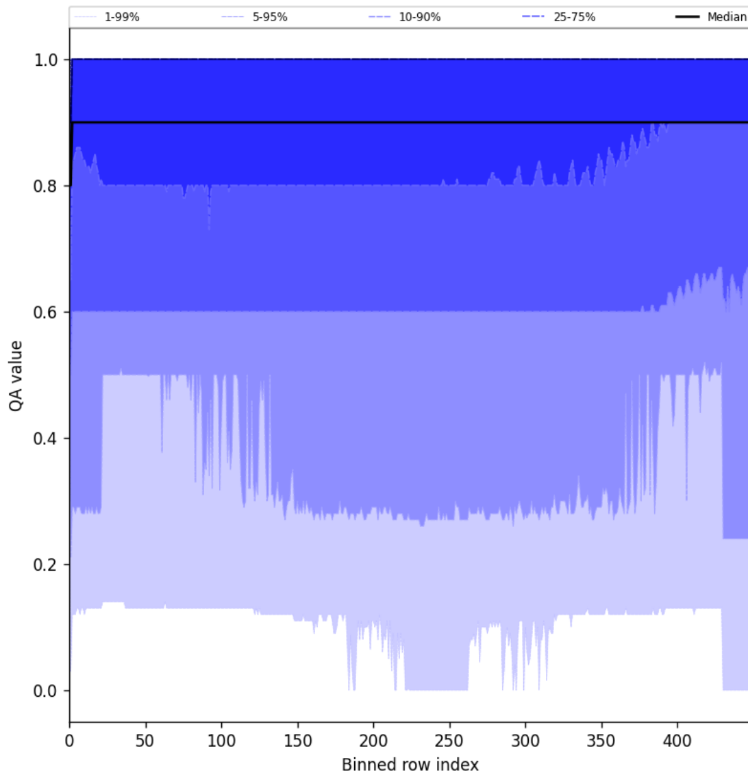
Figure 27: Along track statistics of “QA value” for 2024-12-27 to 2024-12-29
