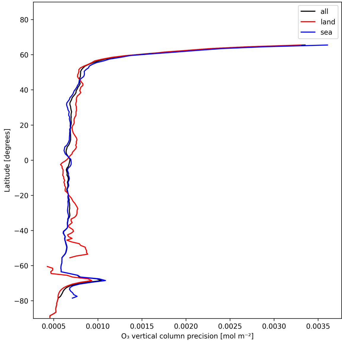
Figure 15: Zonal average of “O 3 vertical column precision” for 2024-12-27 to 2024-12-29.
