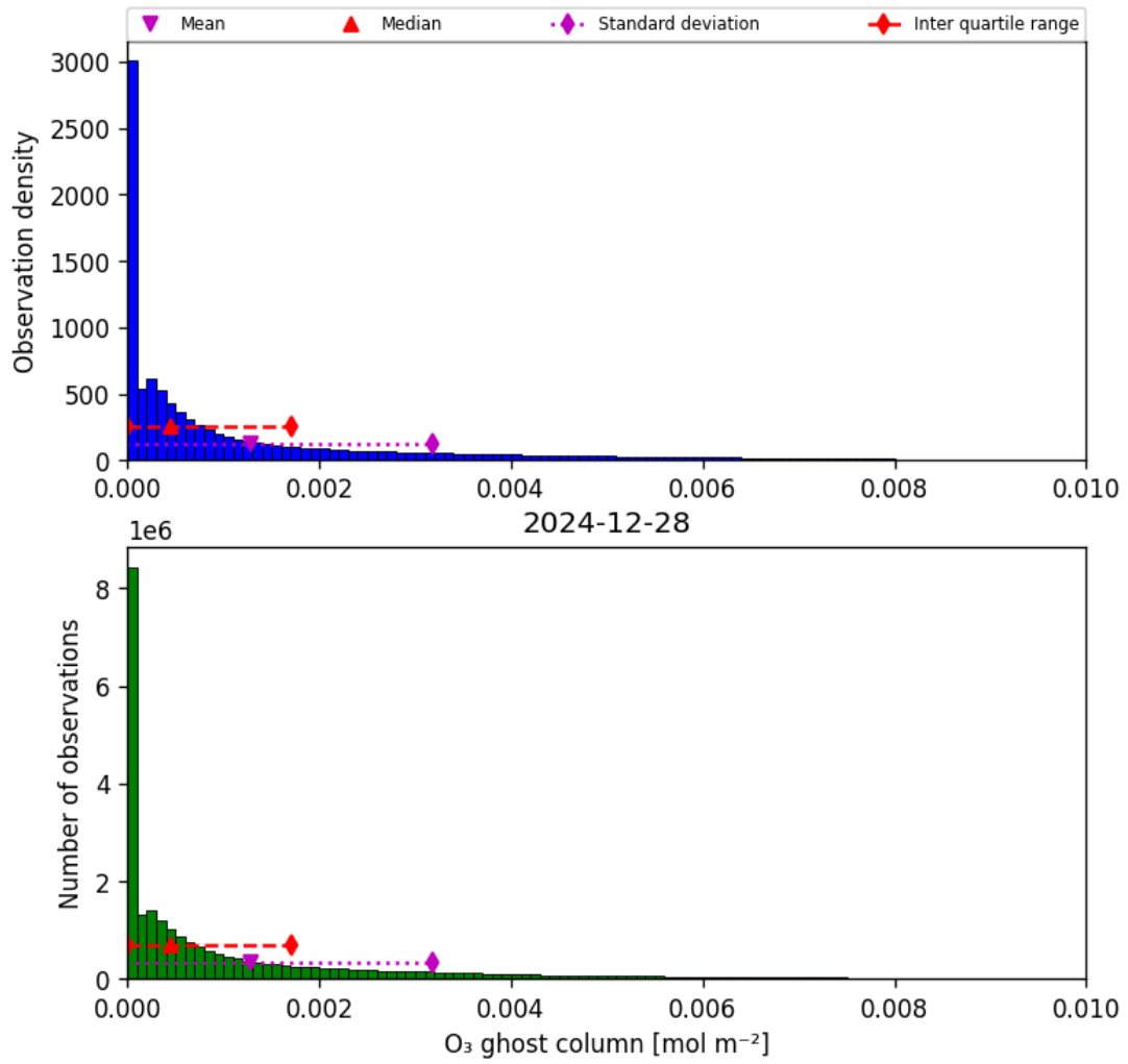
Figure 25: Histogram of “O 3 ghost column” for 2024-12-27 to 2024-12-29
