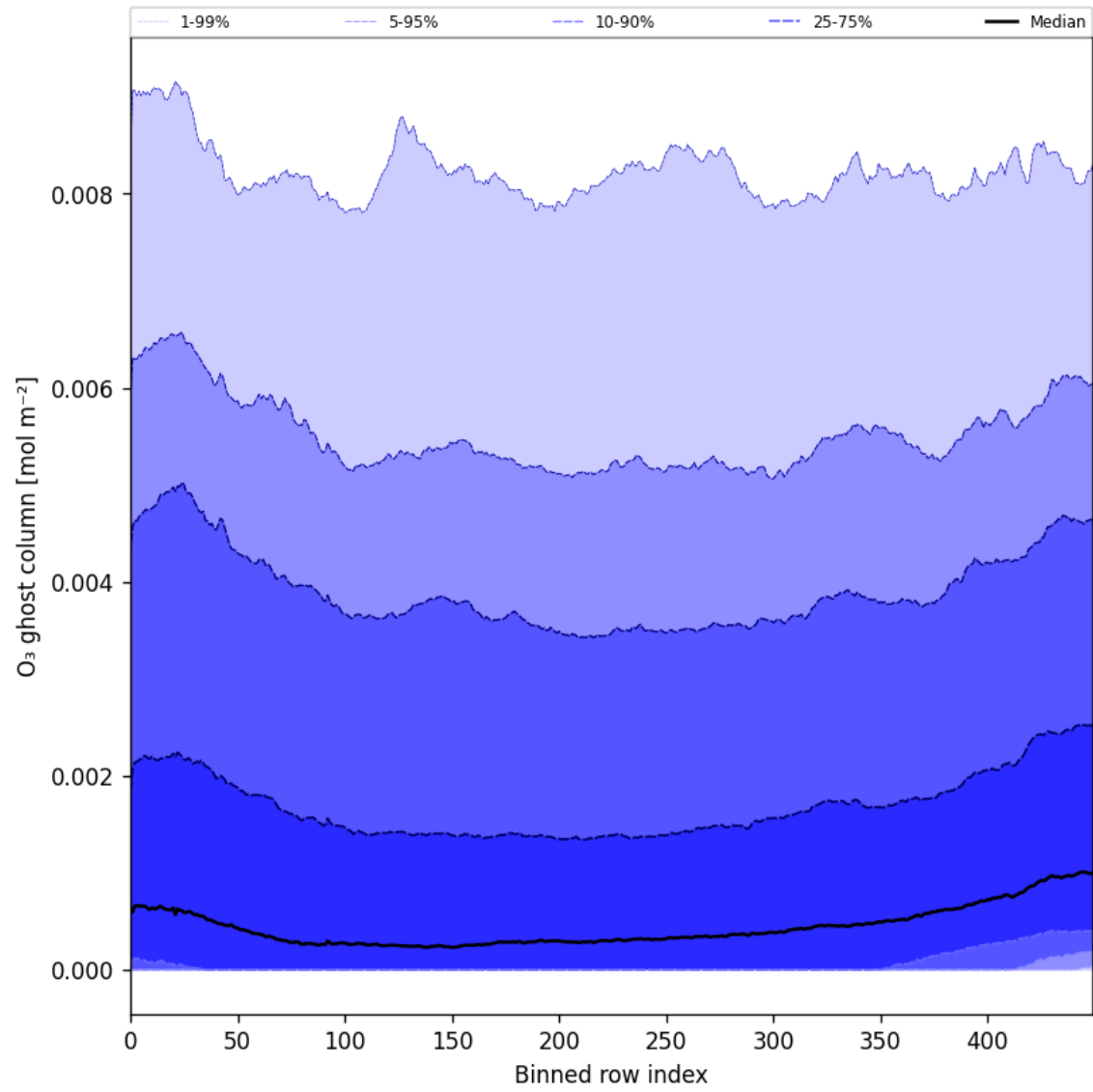
Figure 32: Along track statistics of “O 3 ghost column” for 2024-12-27 to 2024-12-29
