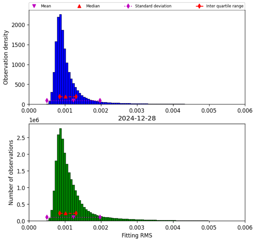
Figure 23: Histogram of “Fitting RMS” for 2024-12-27 to 2024-12-29
