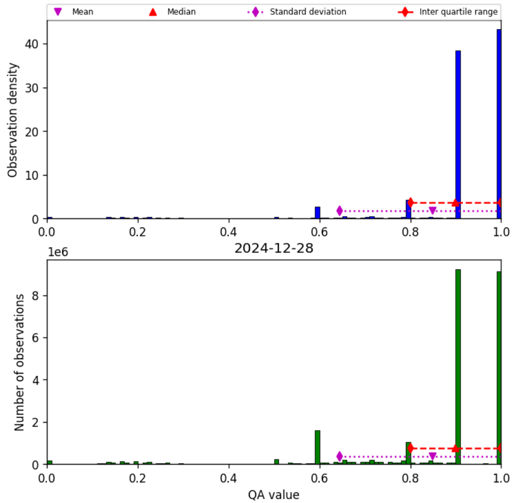
Figure 20: Histogram of “QA value” for 2024-12-27 to 2024-12-29
