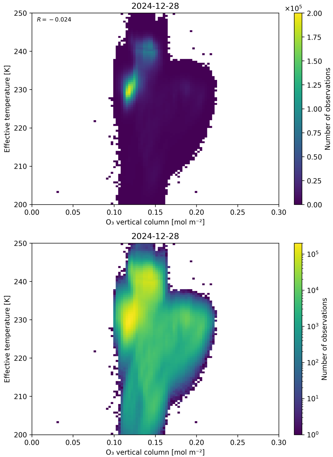
Figure 39: Scatter density plot of “O 3 vertical column” against “Effective temperature” for 2024-12-27 to 2024-12-29.
