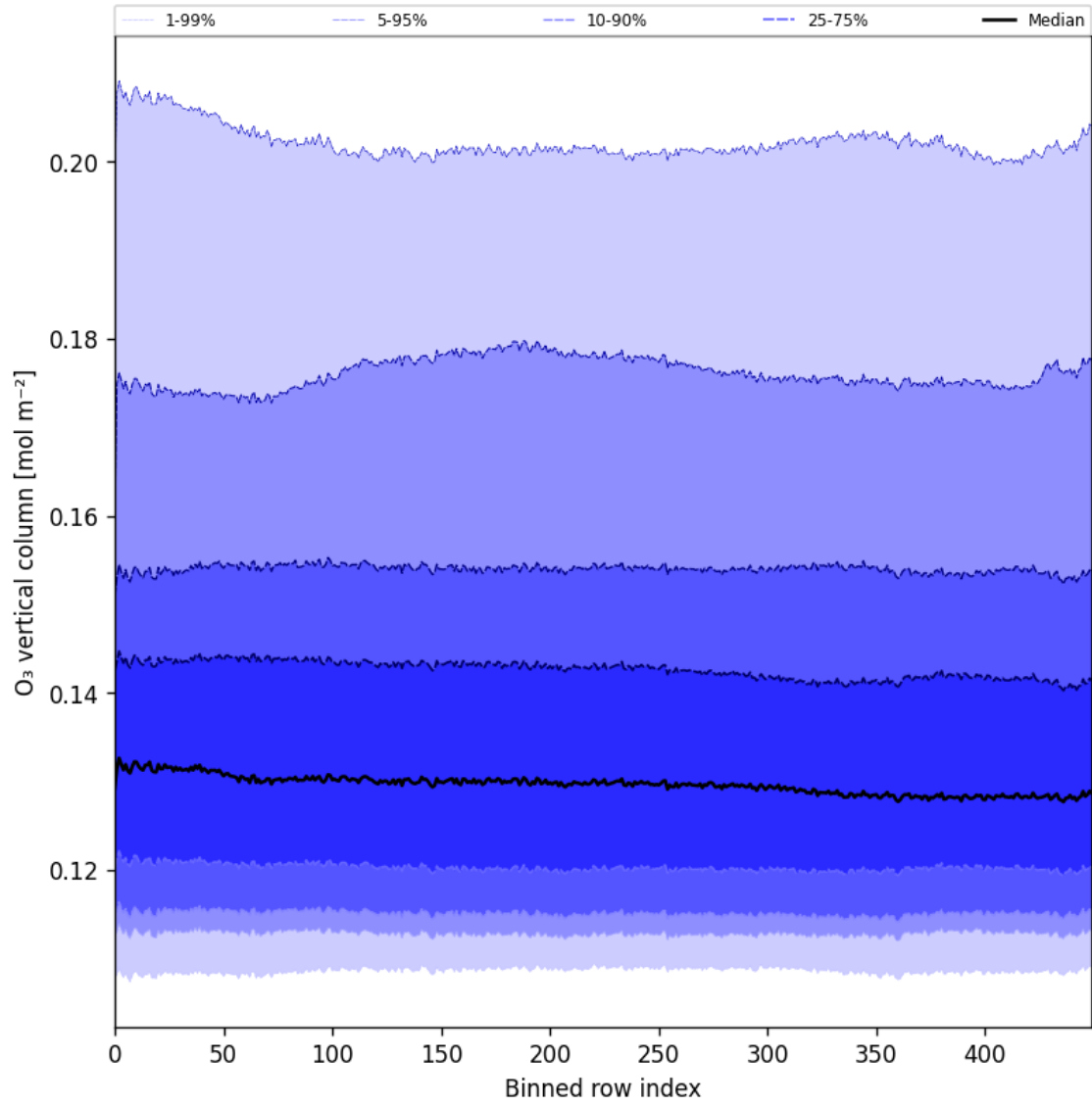
Figure 28: Along track statistics of “O 3 vertical column” for 2024-12-27 to 2024-12-29
