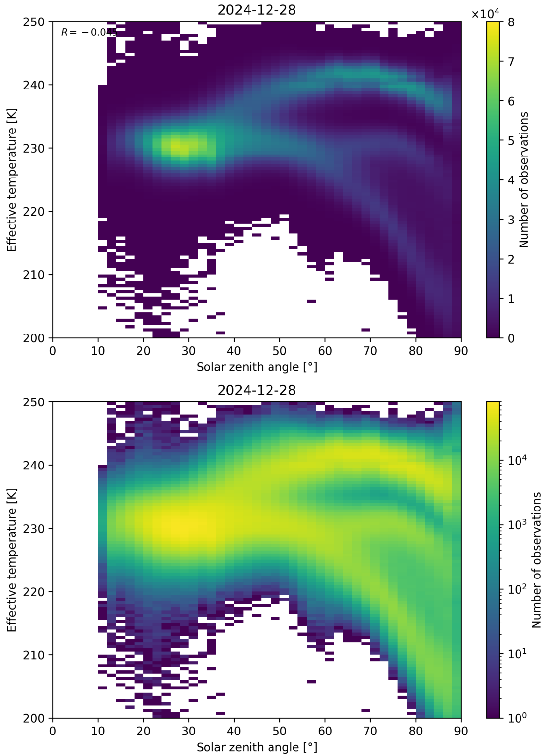
Figure 45: Scatter density plot of “Solar zenith angle” against “Effective temperature” for 2024-12-27 to 2024-12-29.
