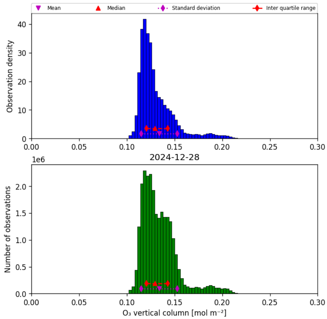
Figure 21: Histogram of “O 3 vertical column” for 2024-12-27 to 2024-12-29
