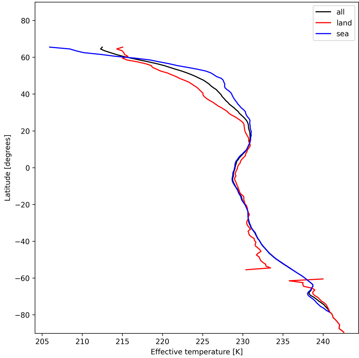
Figure 17: Zonal average of “Effective temperature” for 2024-12-27 to 2024-12-29.
