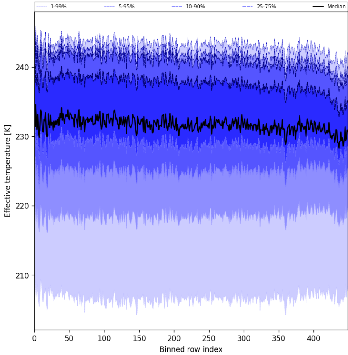
Figure 31: Along track statistics of “Effective temperature” for 2024-12-27 to 2024-12-29
