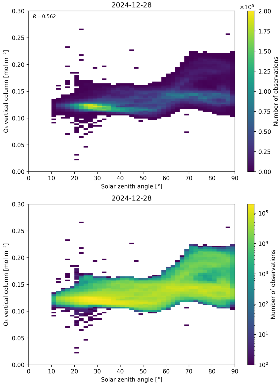
Figure 47: Scatter density plot of “Solar zenith angle” against “O 3 vertical column” for 2024-12-27 to 2024-12-29.
