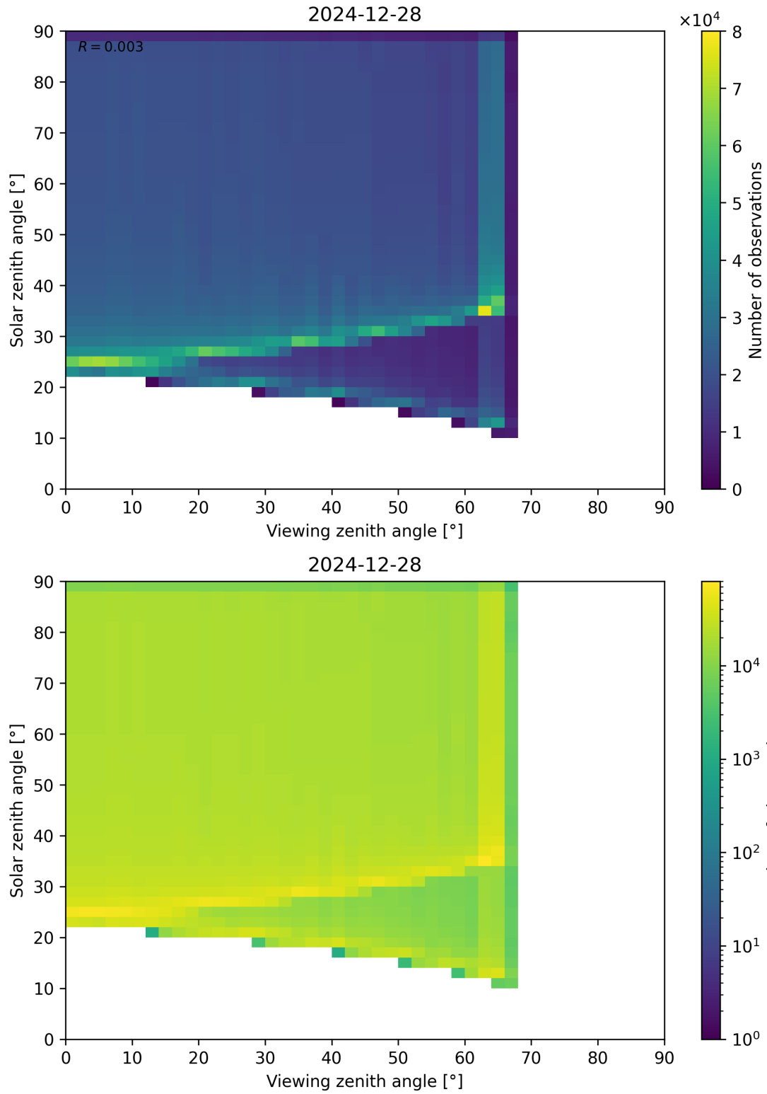
Figure 54: Scatter density plot of “Viewing zenith angle” against “Solar zenith angle” for 2024-12-27 to 2024-12-29.
