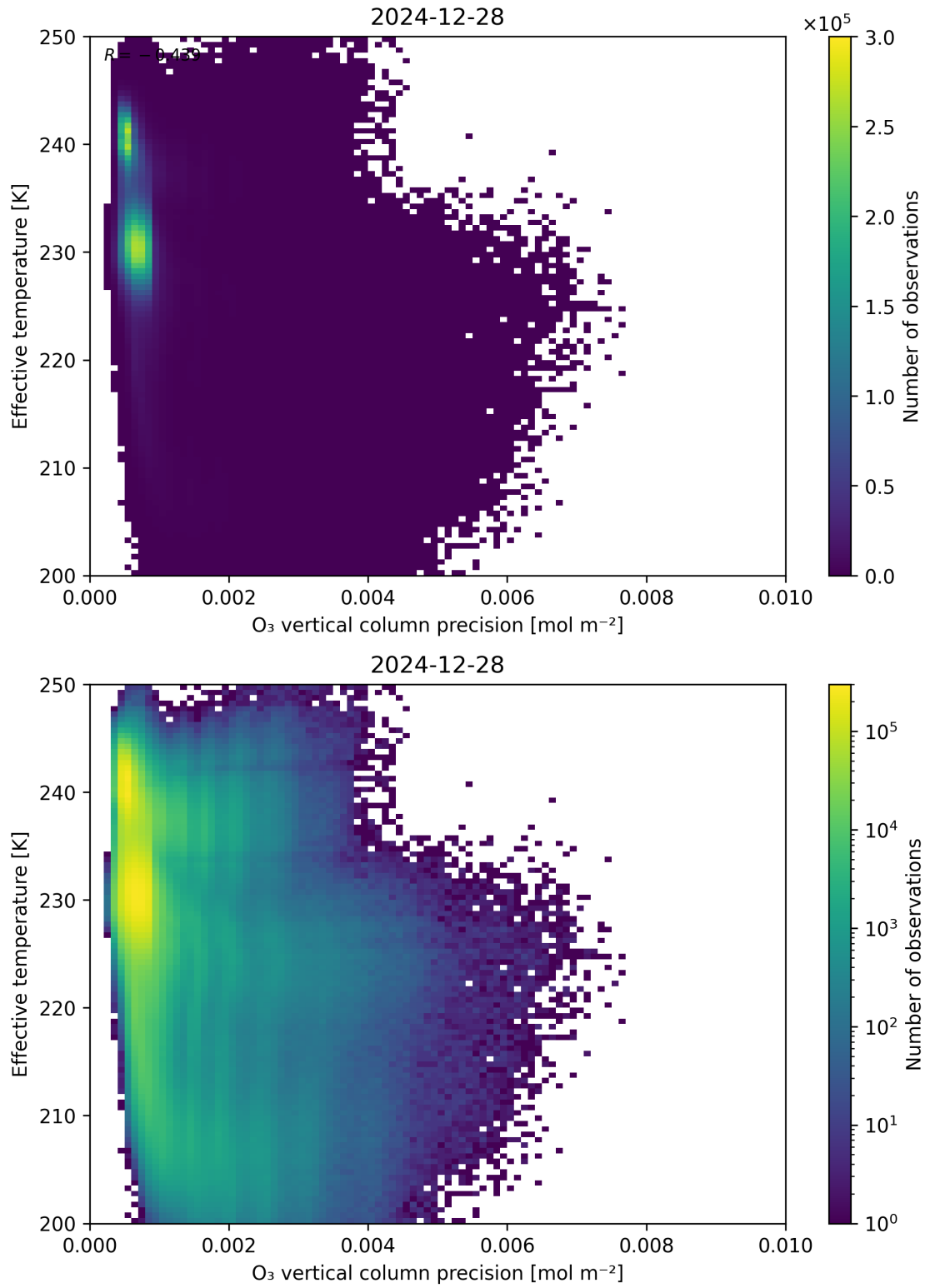
Figure 42: Scatter density plot of “O 3 vertical column precision” against “Effective temperature” for 2024-12-27 to 2024-12-29.
