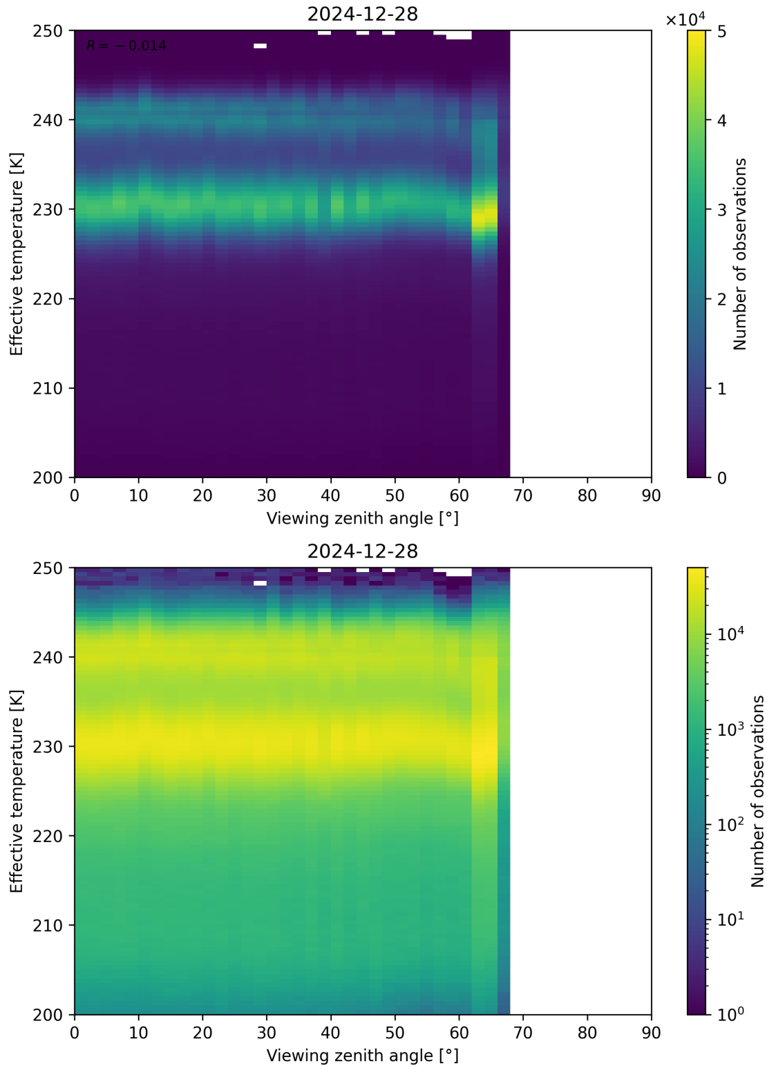
Figure 50: Scatter density plot of “Viewing zenith angle” against “Effective temperature” for 2024-12-27 to 2024-12-29.
