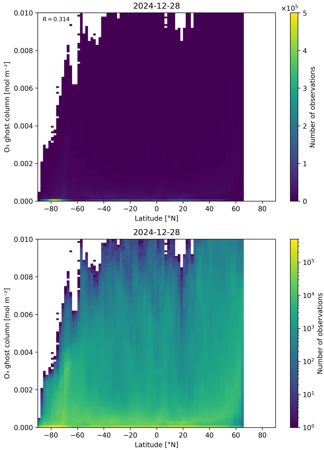
Figure 35: Scatter density plot of “Latitude” against “O 3 ghost column” for 2024-12-27 to 2024-12-29.
