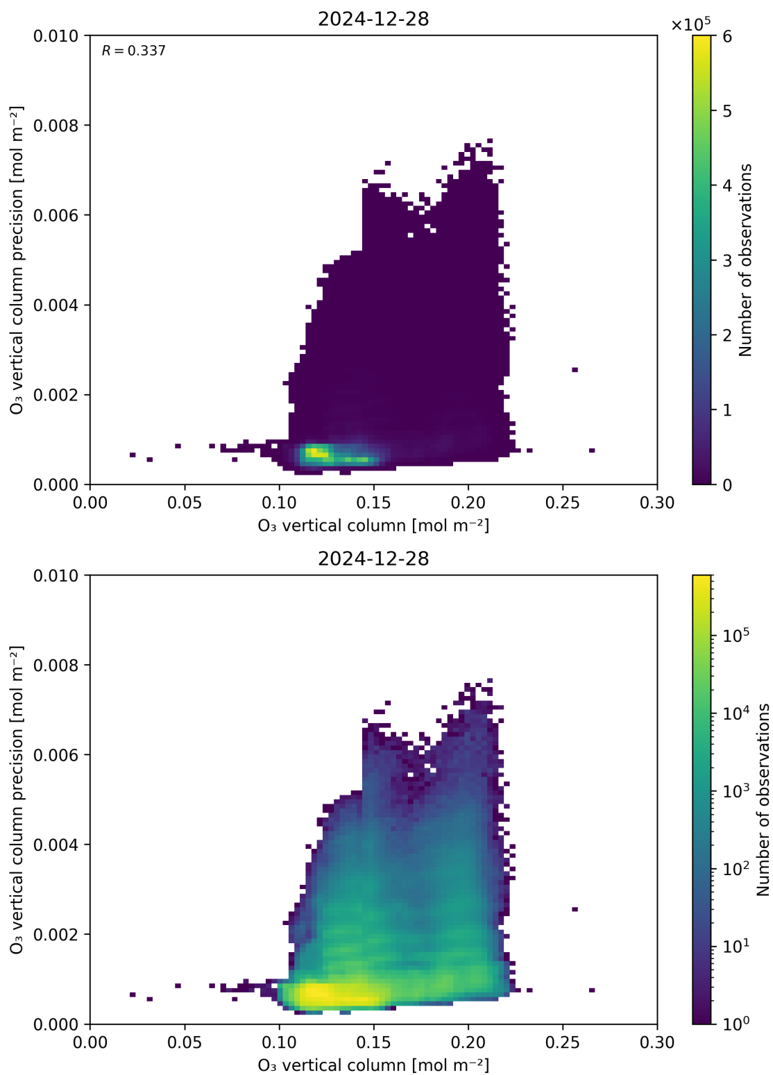
Figure 41: Scatter density plot of “O 3 vertical column” against “O 3 vertical column precision” for 2024-12-27 to 2024-12-29.
