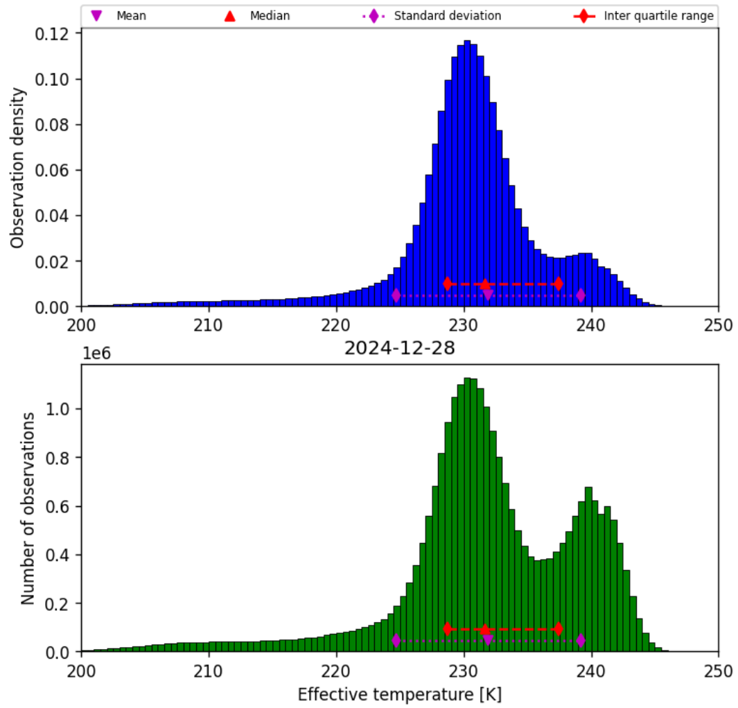
Figure 24: Histogram of “Effective temperature” for 2024-12-27 to 2024-12-29
