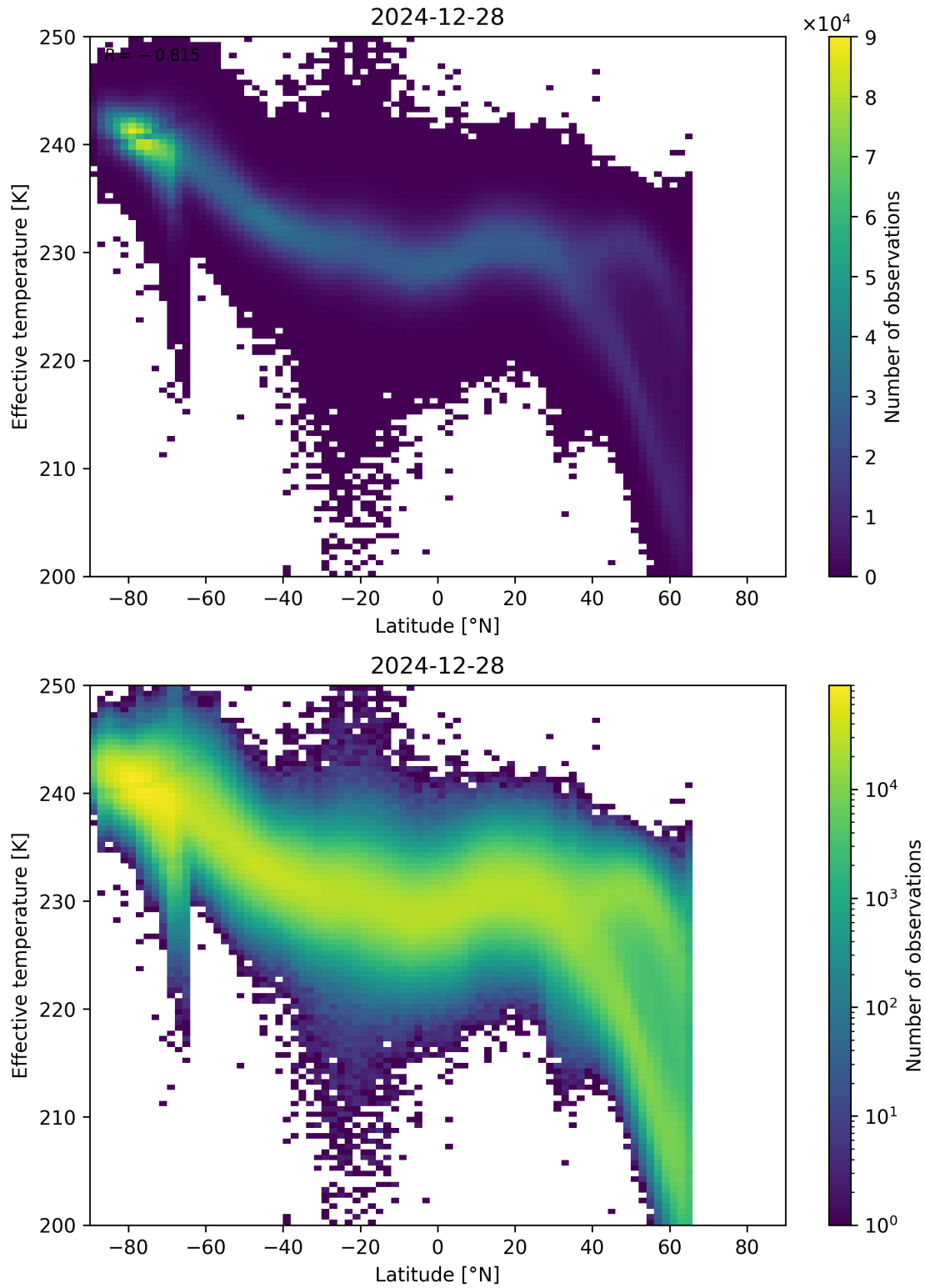
Figure 34: Scatter density plot of “Latitude” against “Effective temperature” for 2024-12-27 to 2024-12-29.
