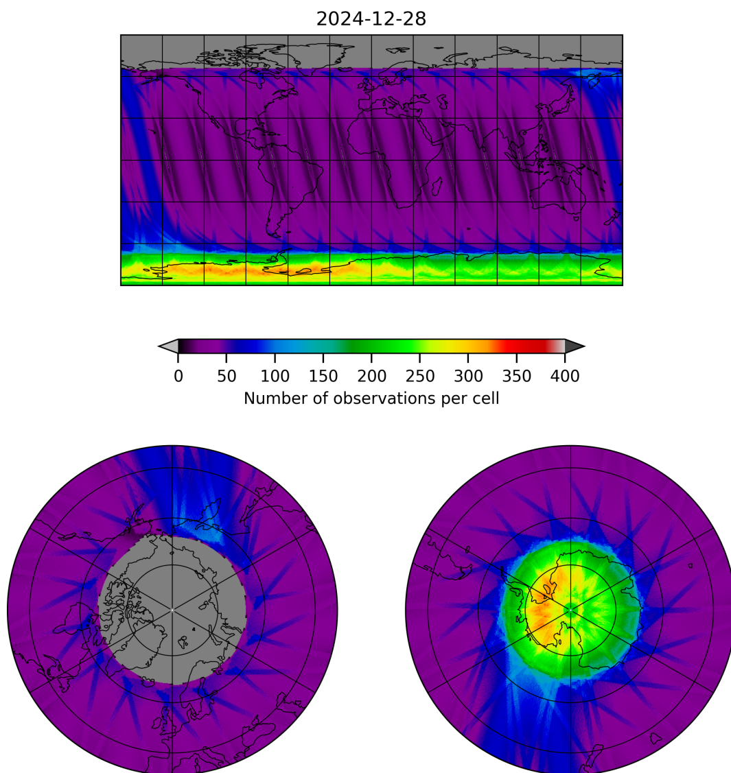
Figure 12: Map of the number of observations for 2024-12-27 to 2024-12-29
