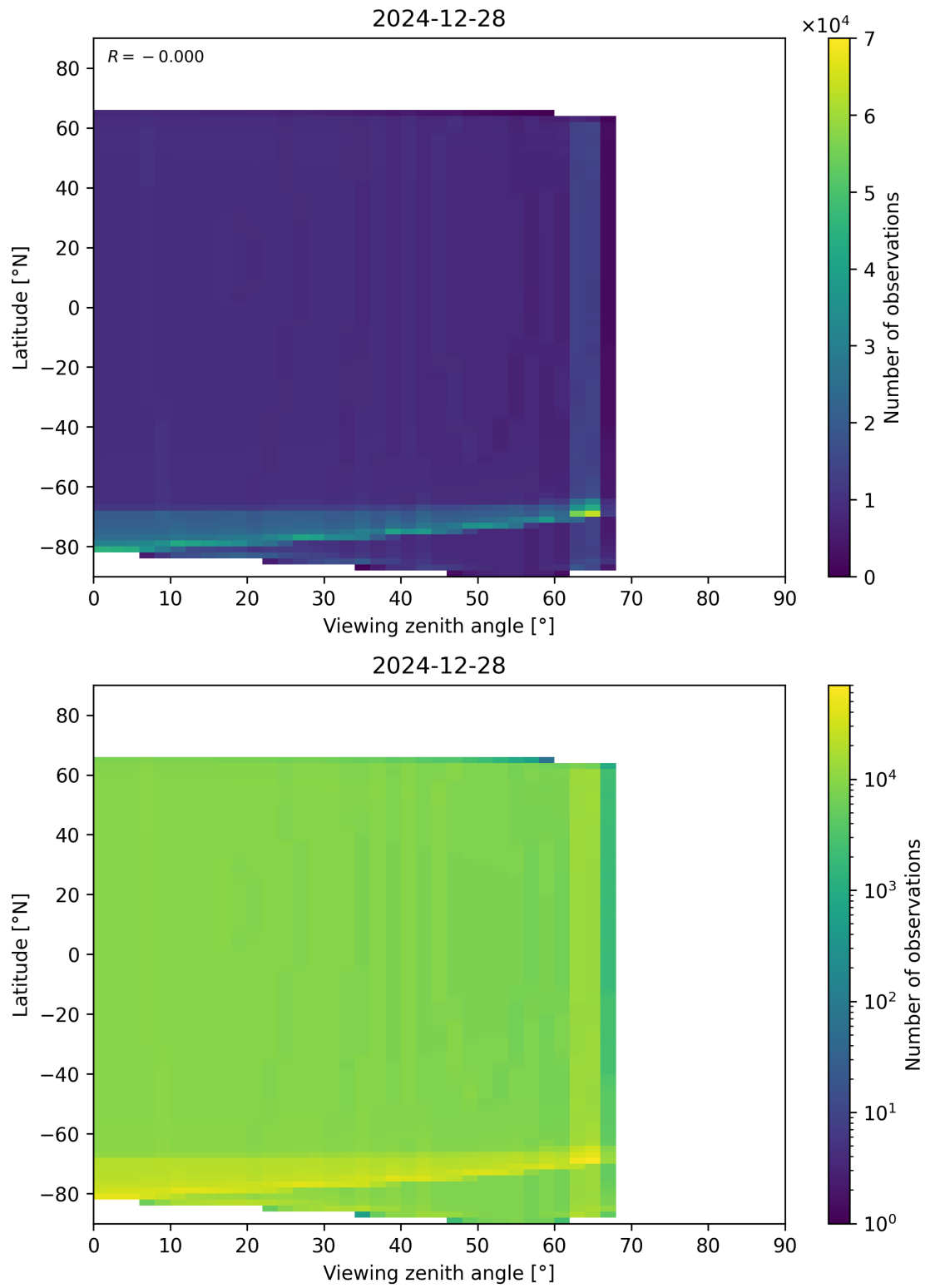
Figure 49: Scatter density plot of “Viewing zenith angle” against “Latitude” for 2024-12-27 to 2024-12-29.
