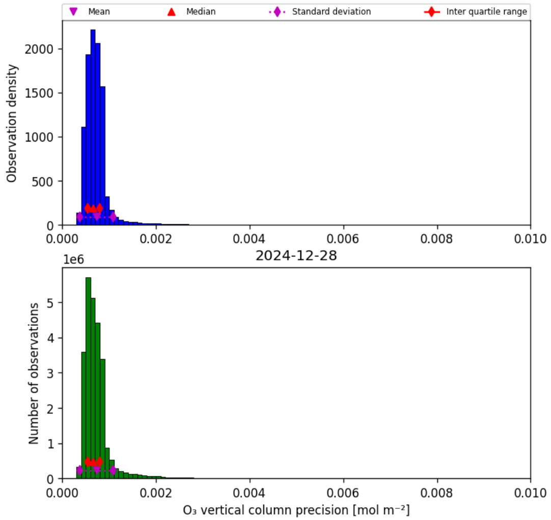
Figure 22: Histogram of “O 3 vertical column precision” for 2024-12-27 to 2024-12-29
