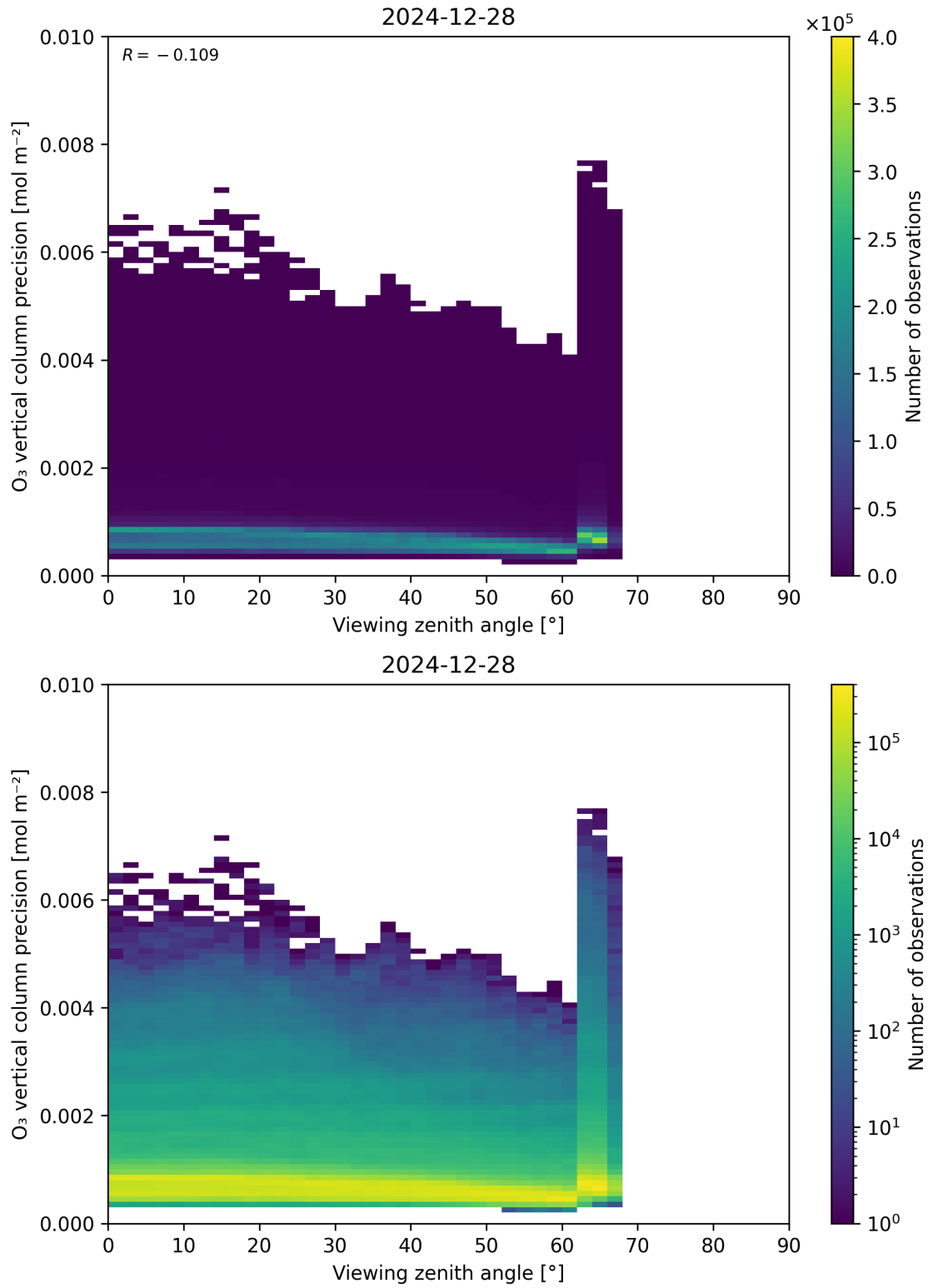
Figure 53: Scatter density plot of “Viewing zenith angle” against “O 3 vertical column precision” for 2024-12-27 to 2024-12-29.
