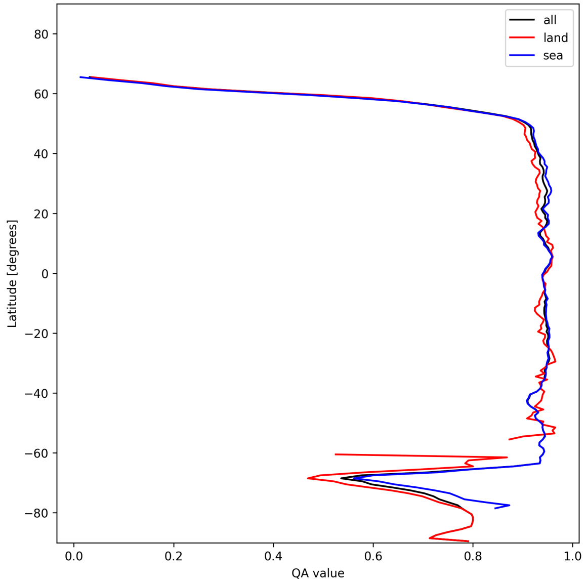
Figure 13: Zonal average of “QA value” for 2024-12-27 to 2024-12-29.
