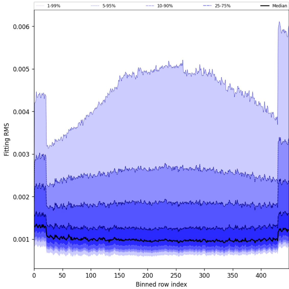
Figure 30: Along track statistics of “Fitting RMS” for 2024-12-27 to 2024-12-29
