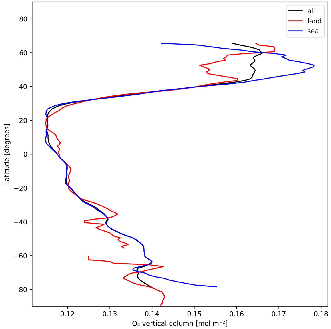
Figure 14: Zonal average of “O 3 vertical column” for 2024-12-27 to 2024-12-29.
