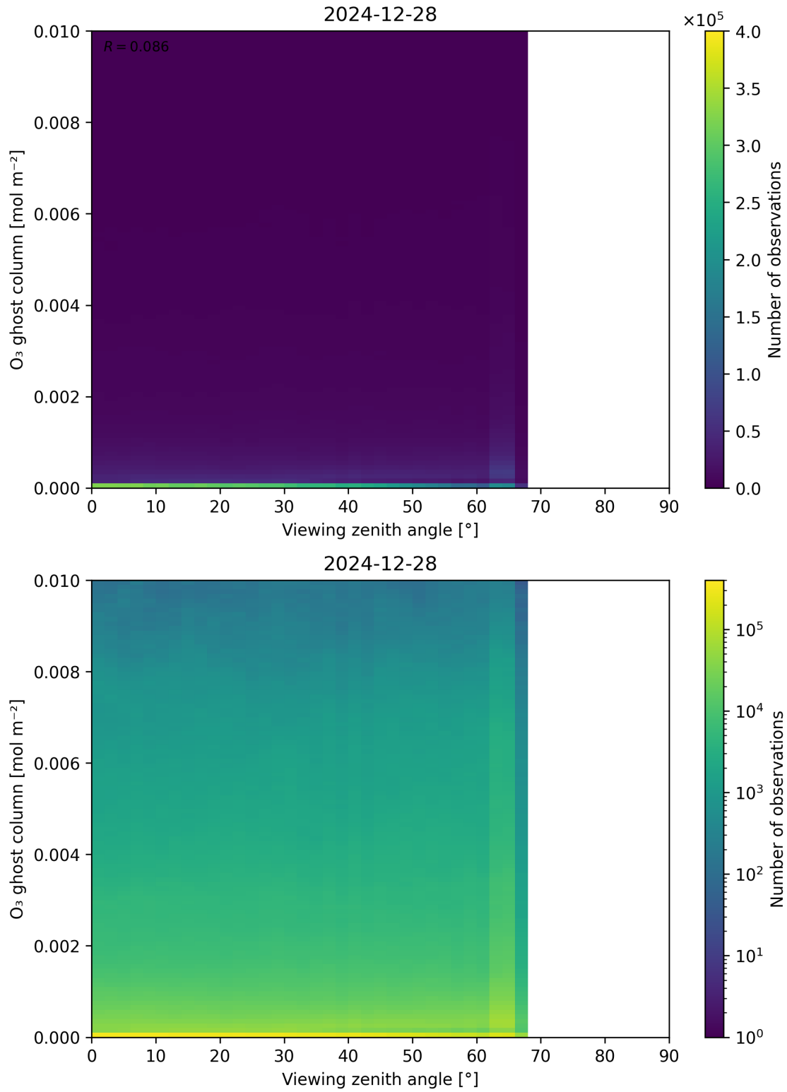
Figure 51: Scatter density plot of “Viewing zenith angle” against “O 3 ghost column” for 2024-12-27 to 2024-12-29.
