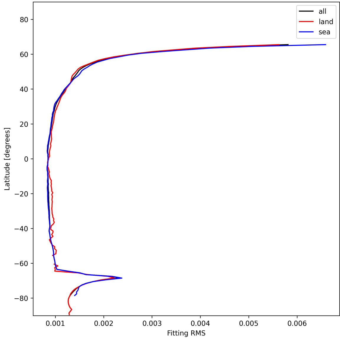
Figure 16: Zonal average of “Fitting RMS” for 2024-12-27 to 2024-12-29.
