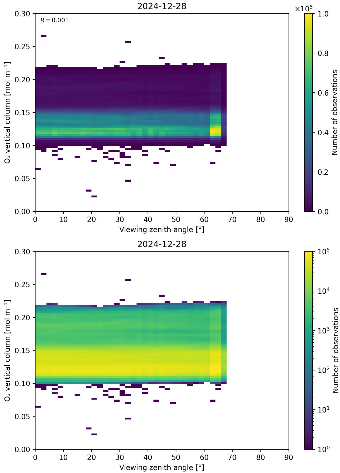
Figure 52: Scatter density plot of “Viewing zenith angle” against “O 3 vertical column” for 2024-12-27 to 2024-12-29.
