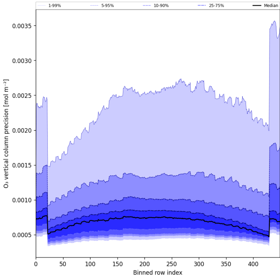
Figure 29: Along track statistics of “O 3 vertical column precision” for 2024-12-27 to 2024-12-29
