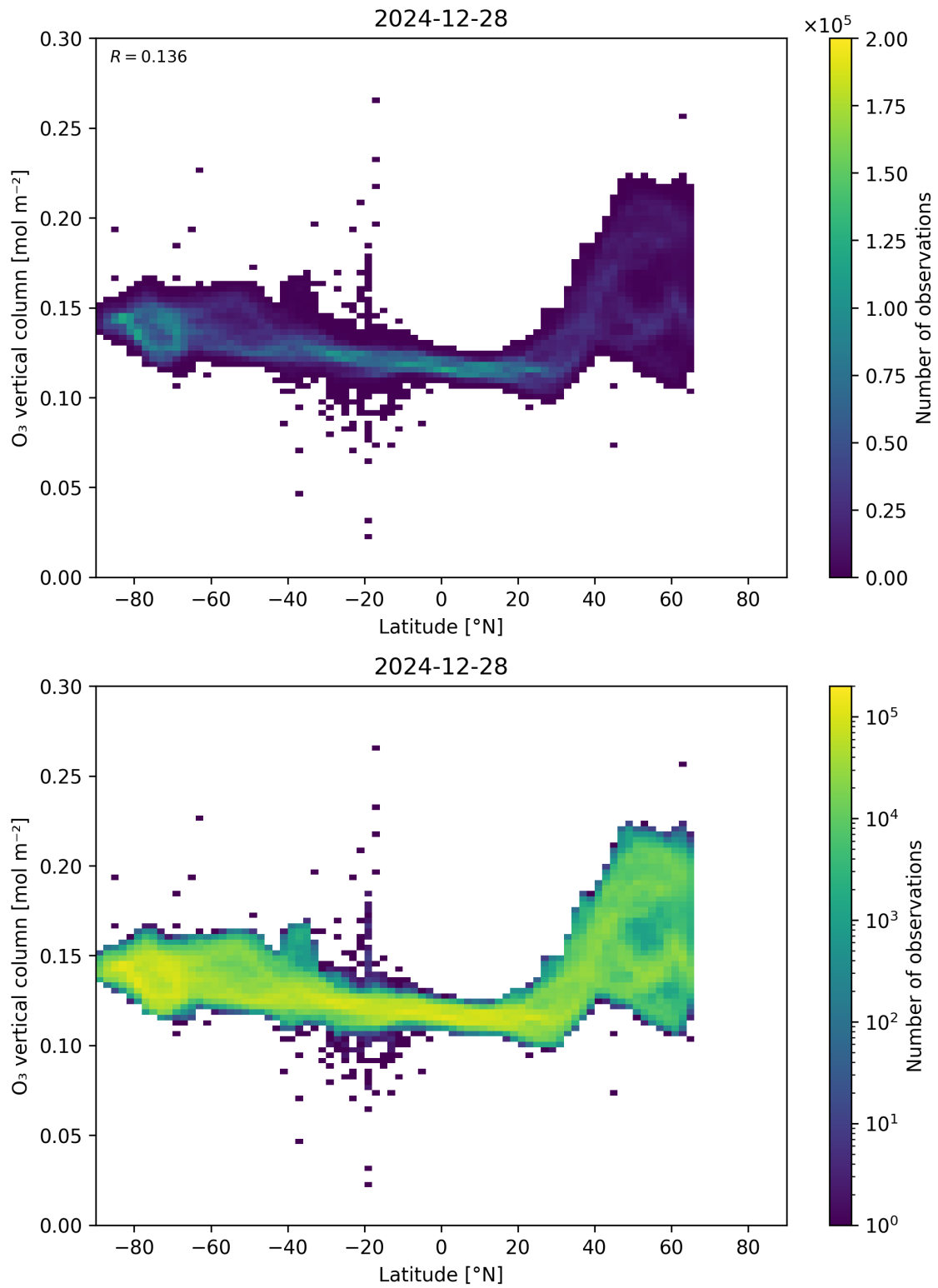
Figure 36: Scatter density plot of “Latitude” against “O 3 vertical column” for 2024-12-27 to 2024-12-29.
