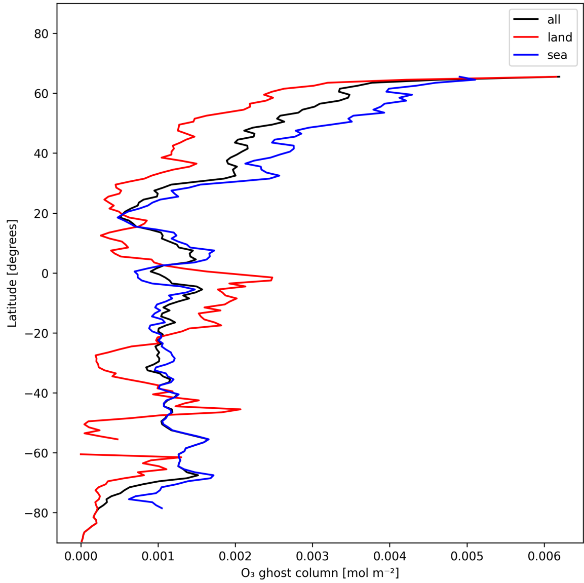
Figure 18: Zonal average of “O 3 ghost column” for 2024-12-27 to 2024-12-29.
