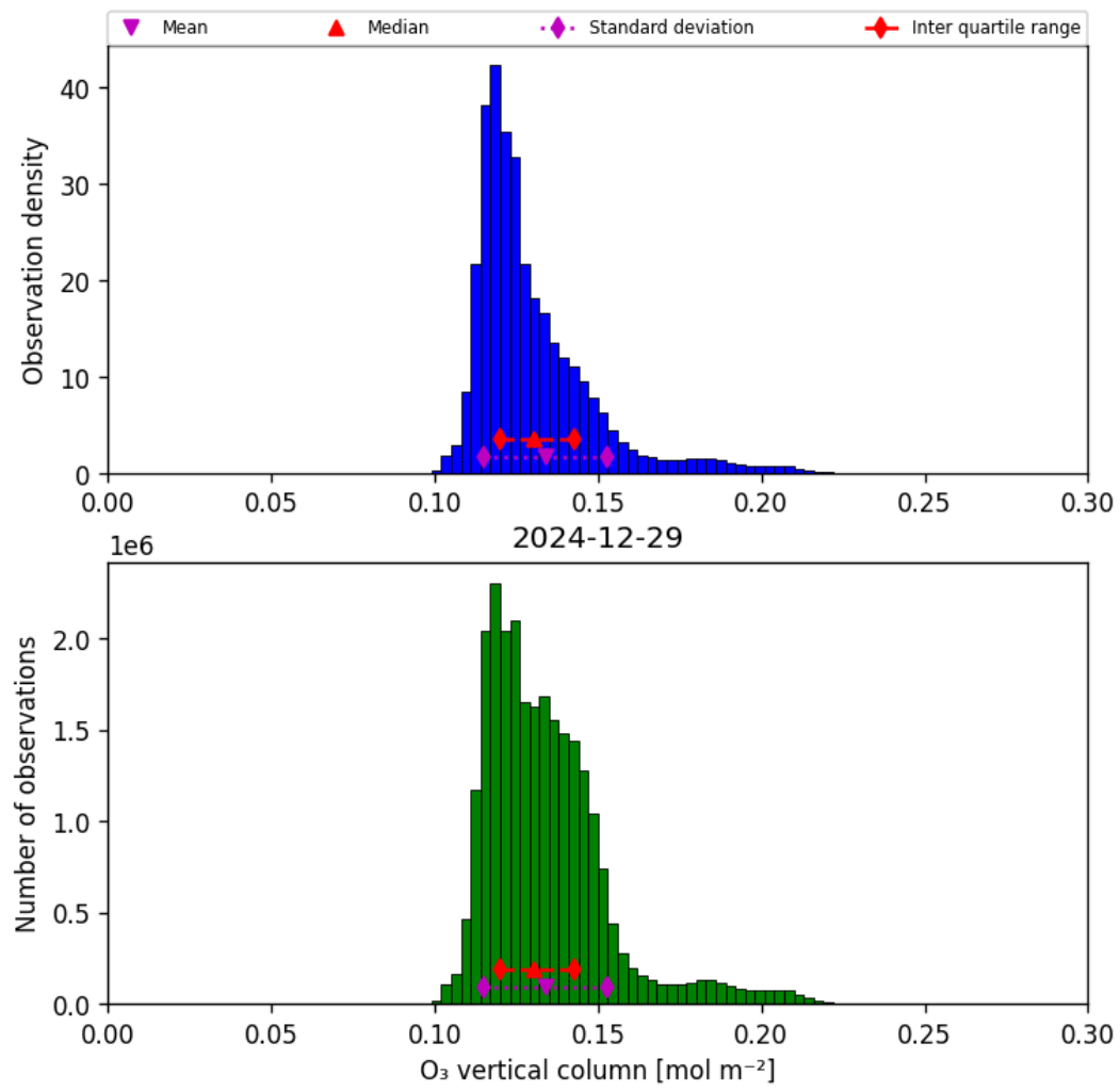
Figure 21: Histogram of “O 3 vertical column” for 2024-12-28 to 2024-12-30
