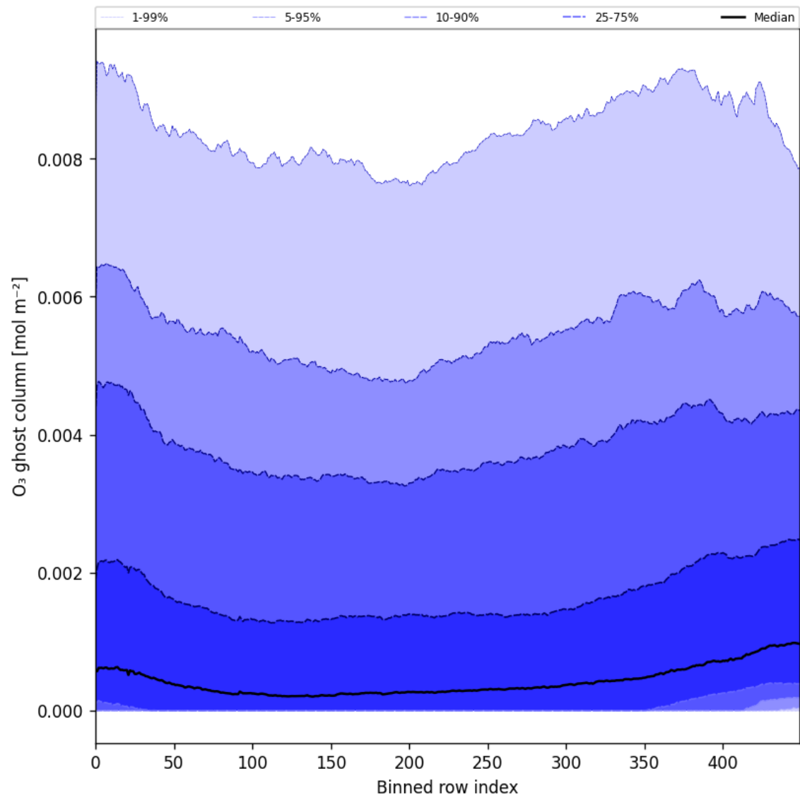
Figure 32: Along track statistics of “O 3 ghost column” for 2024-12-28 to 2024-12-30
