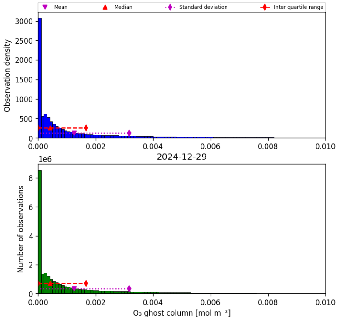
Figure 25: Histogram of “O 3 ghost column” for 2024-12-28 to 2024-12-30
