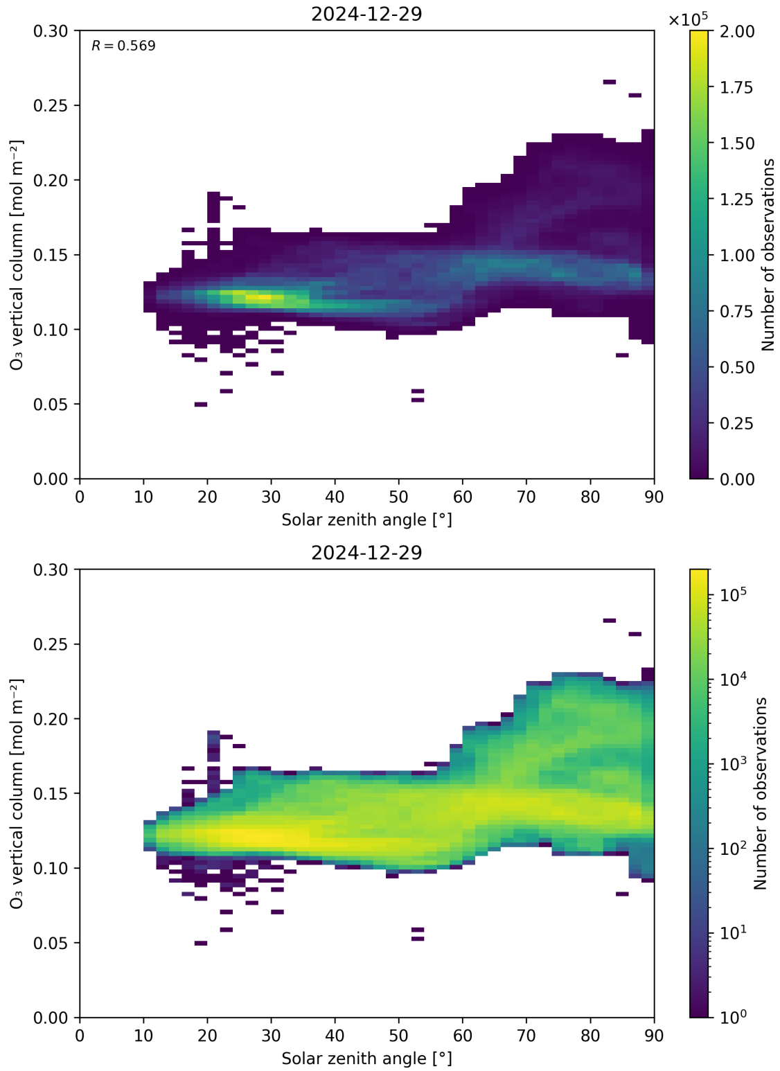
Figure 47: Scatter density plot of “Solar zenith angle” against “O 3 vertical column” for 2024-12-28 to 2024-12-30.
