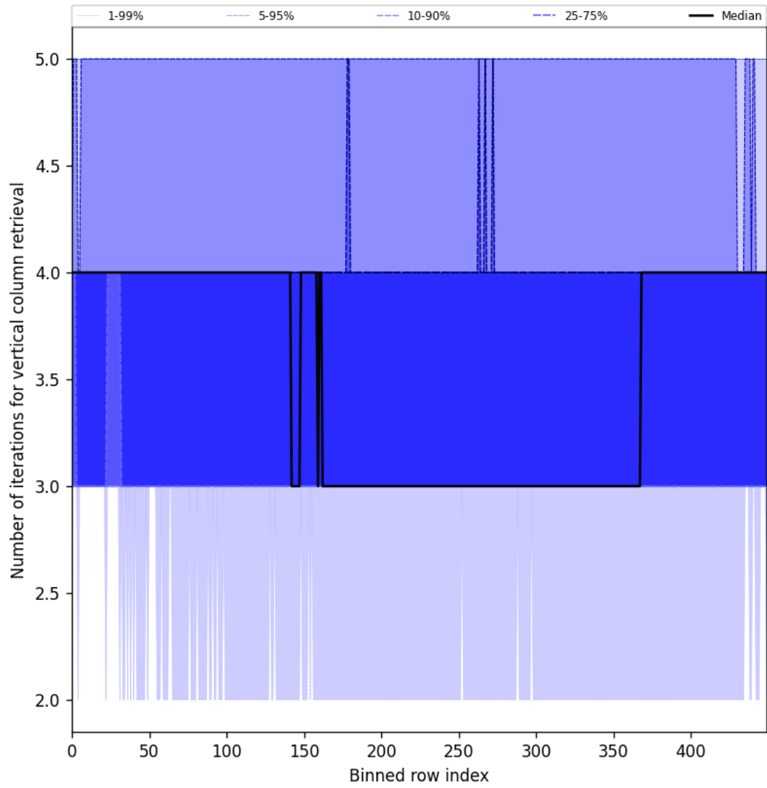
Figure 33: Along track statistics of “Number of iterations for vertical column retrieval” for 2024-12-28 to 2024-12-30
