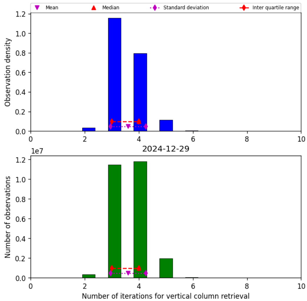
Figure 26: Histogram of “Number of iterations for vertical column retrieval” for 2024-12-28 to 2024-12-30
