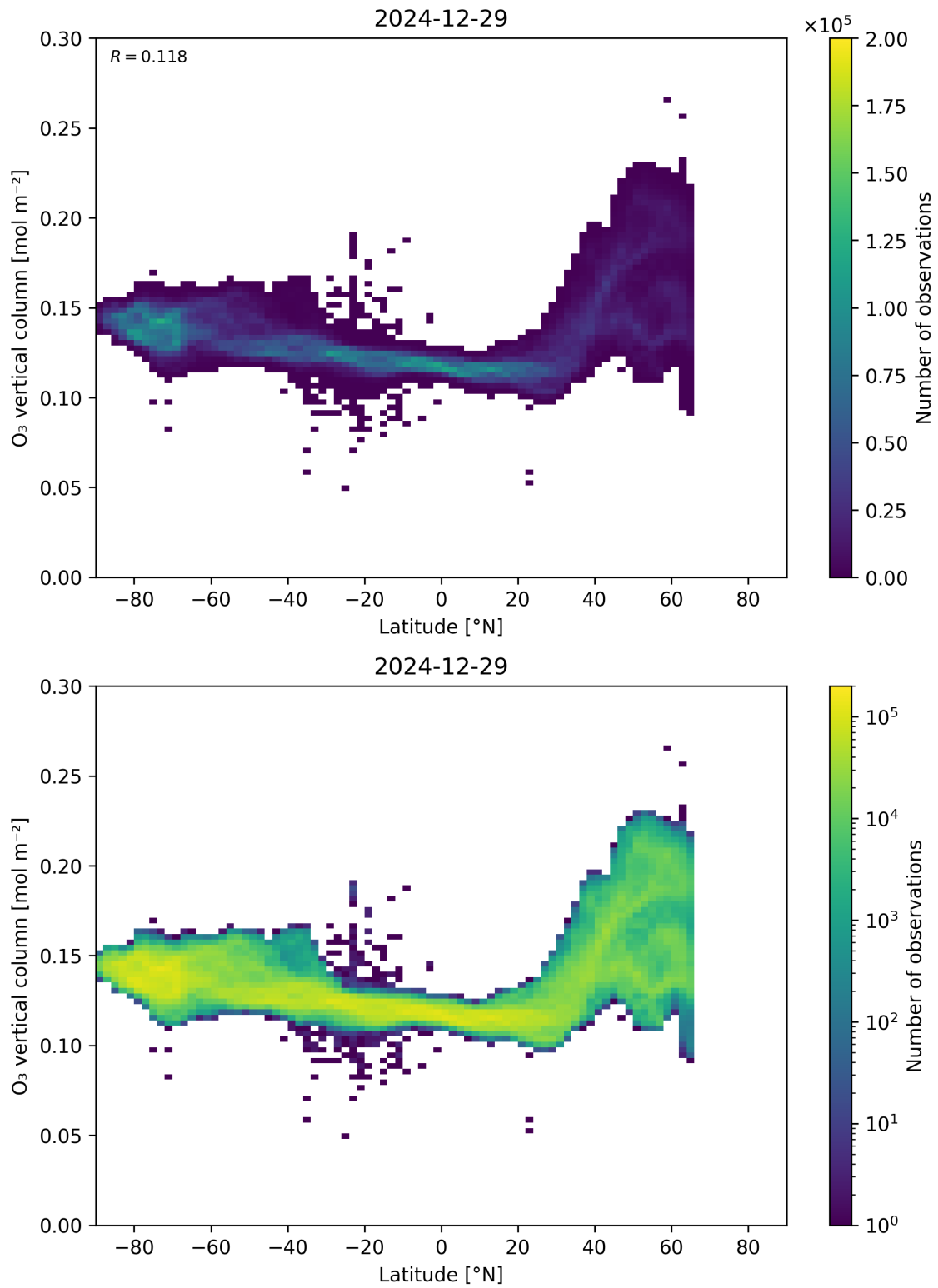
Figure 36: Scatter density plot of “Latitude” against “O 3 vertical column” for 2024-12-28 to 2024-12-30.
