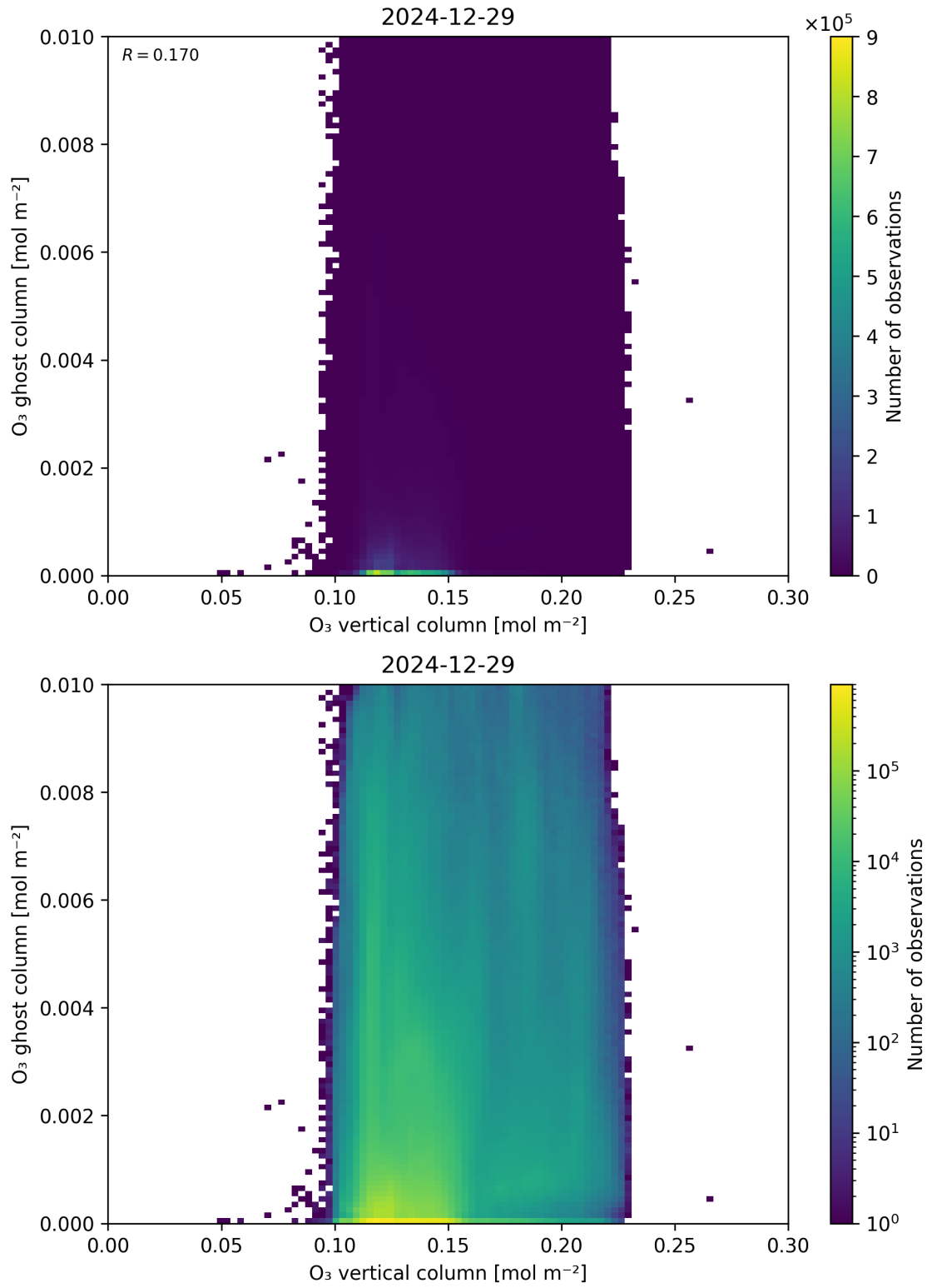
Figure 40: Scatter density plot of “O 3 vertical column” against “O 3 ghost column” for 2024-12-28 to 2024-12-30.
