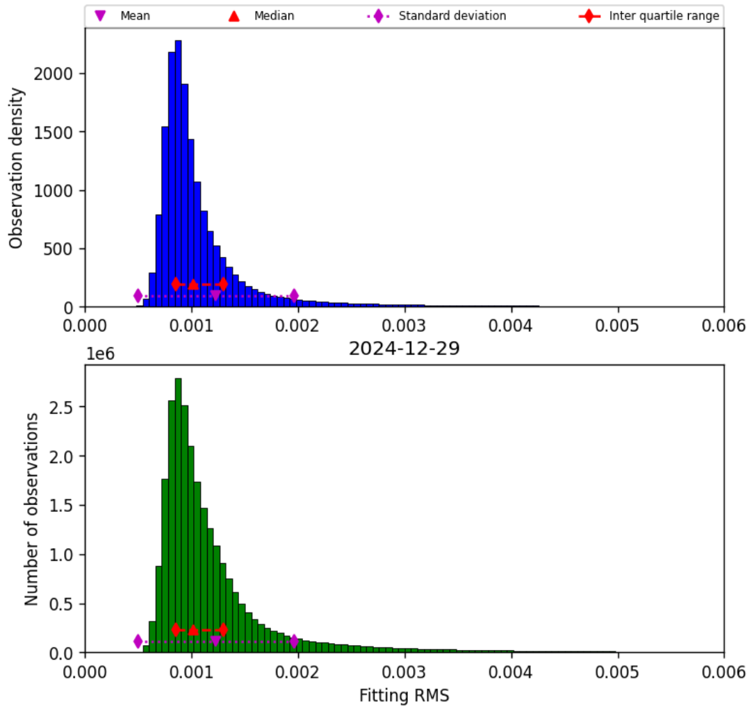
Figure 23: Histogram of “Fitting RMS” for 2024-12-28 to 2024-12-30
