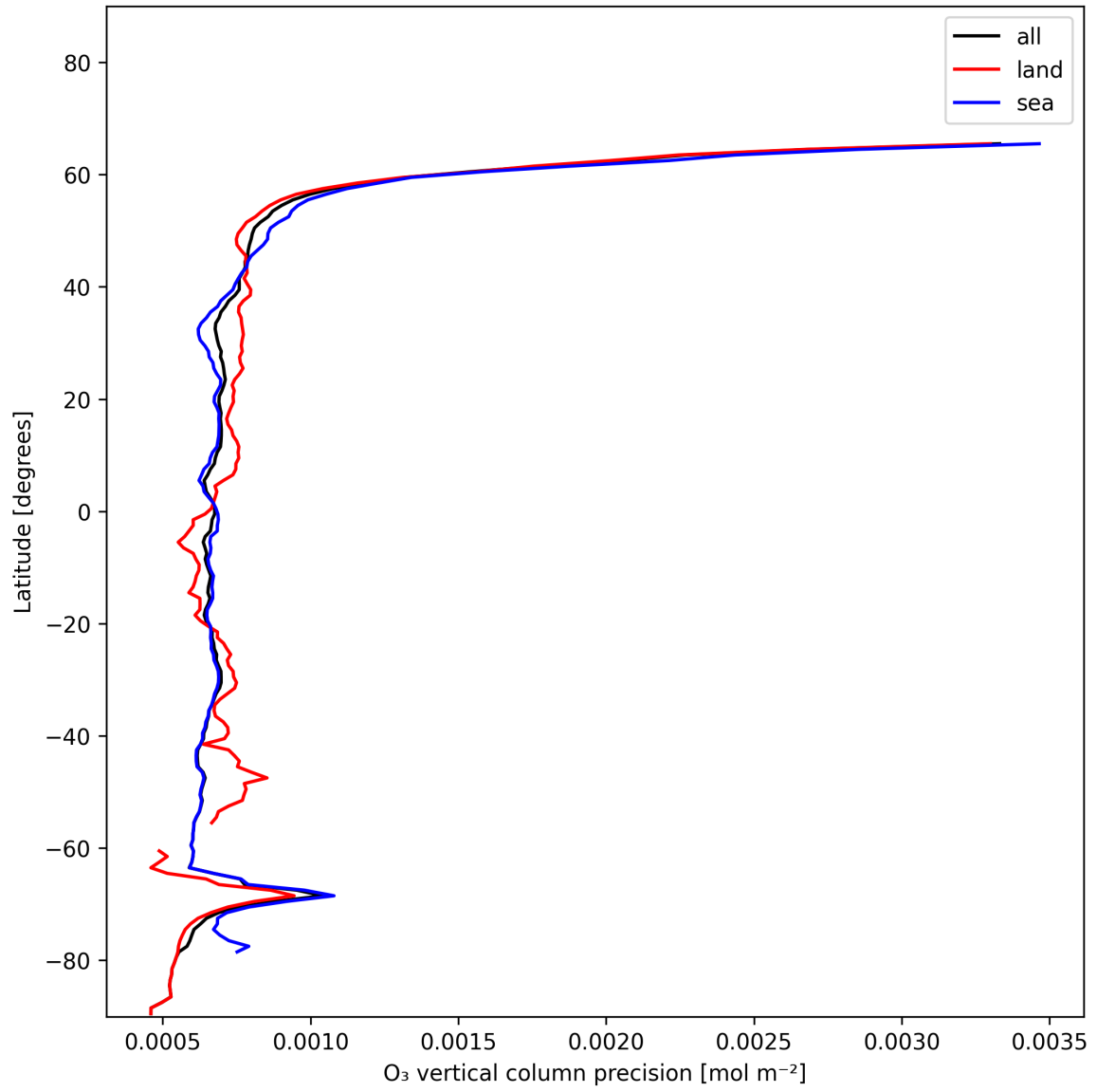
Figure 15: Zonal average of “O 3 vertical column precision” for 2024-12-28 to 2024-12-30.
