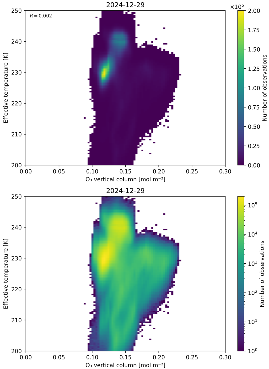
Figure 39: Scatter density plot of “O 3 vertical column” against “Effective temperature” for 2024-12-28 to 2024-12-30.
