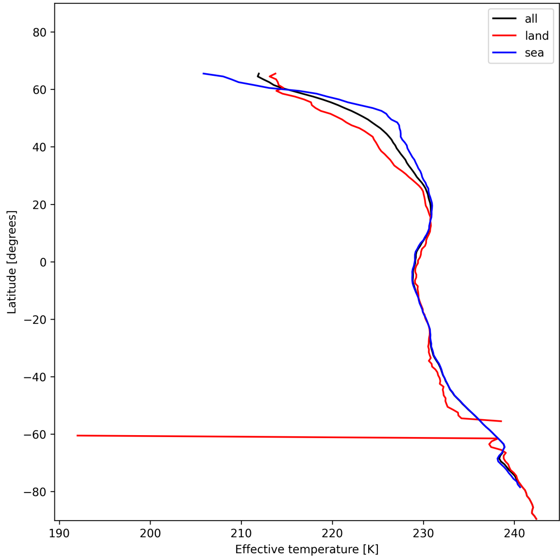
Figure 17: Zonal average of "Effective temperature" for 2024-12-28 to 2024-12-30.
