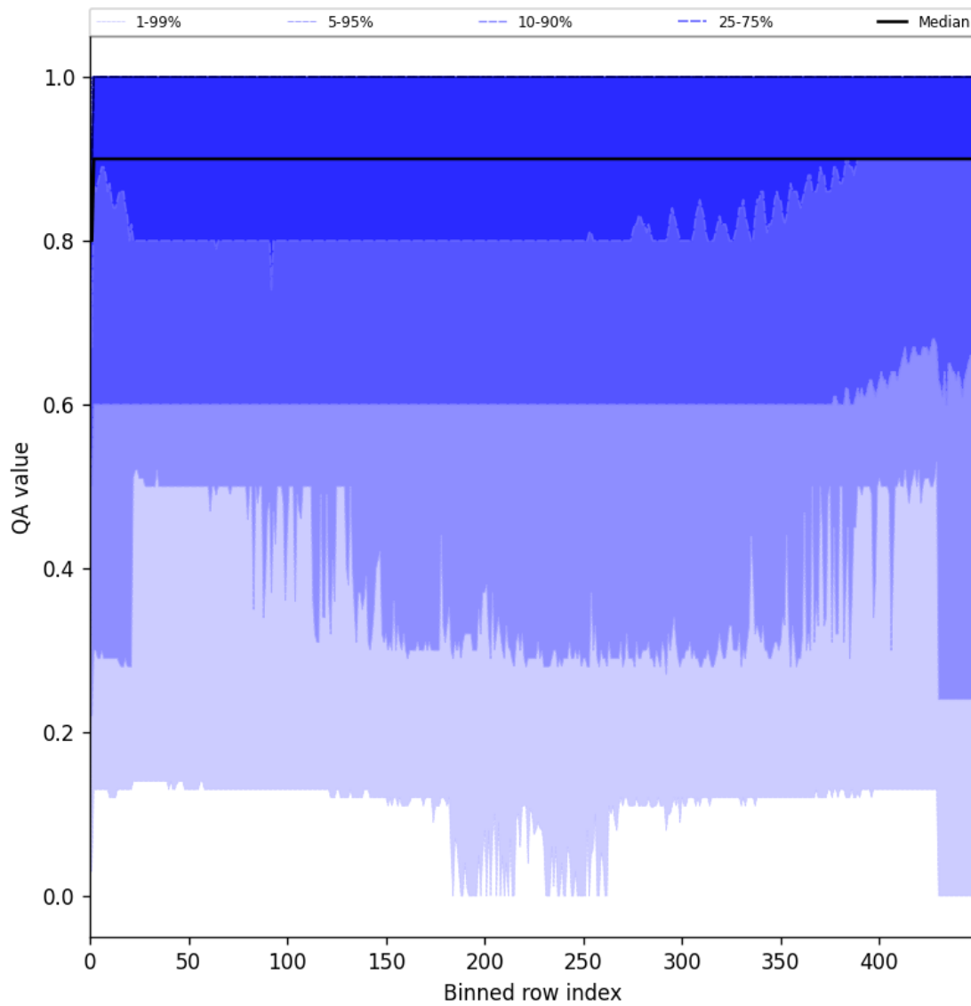
Figure 27: Along track statistics of “QA value” for 2024-12-28 to 2024-12-30
