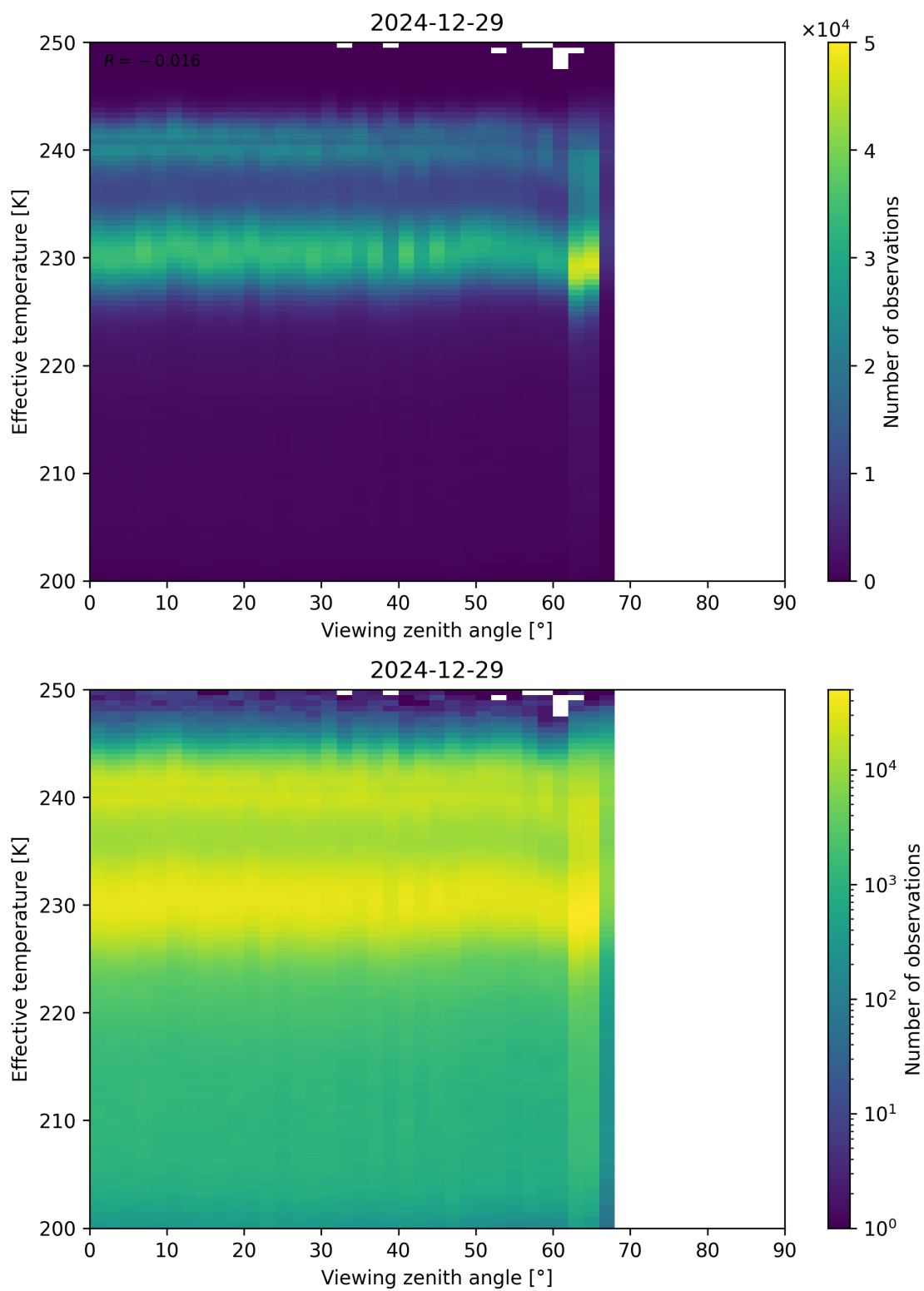
Figure 50: Scatter density plot of “Viewing zenith angle” against “Effective temperature” for 2024-12-28 to 2024-12-30.
