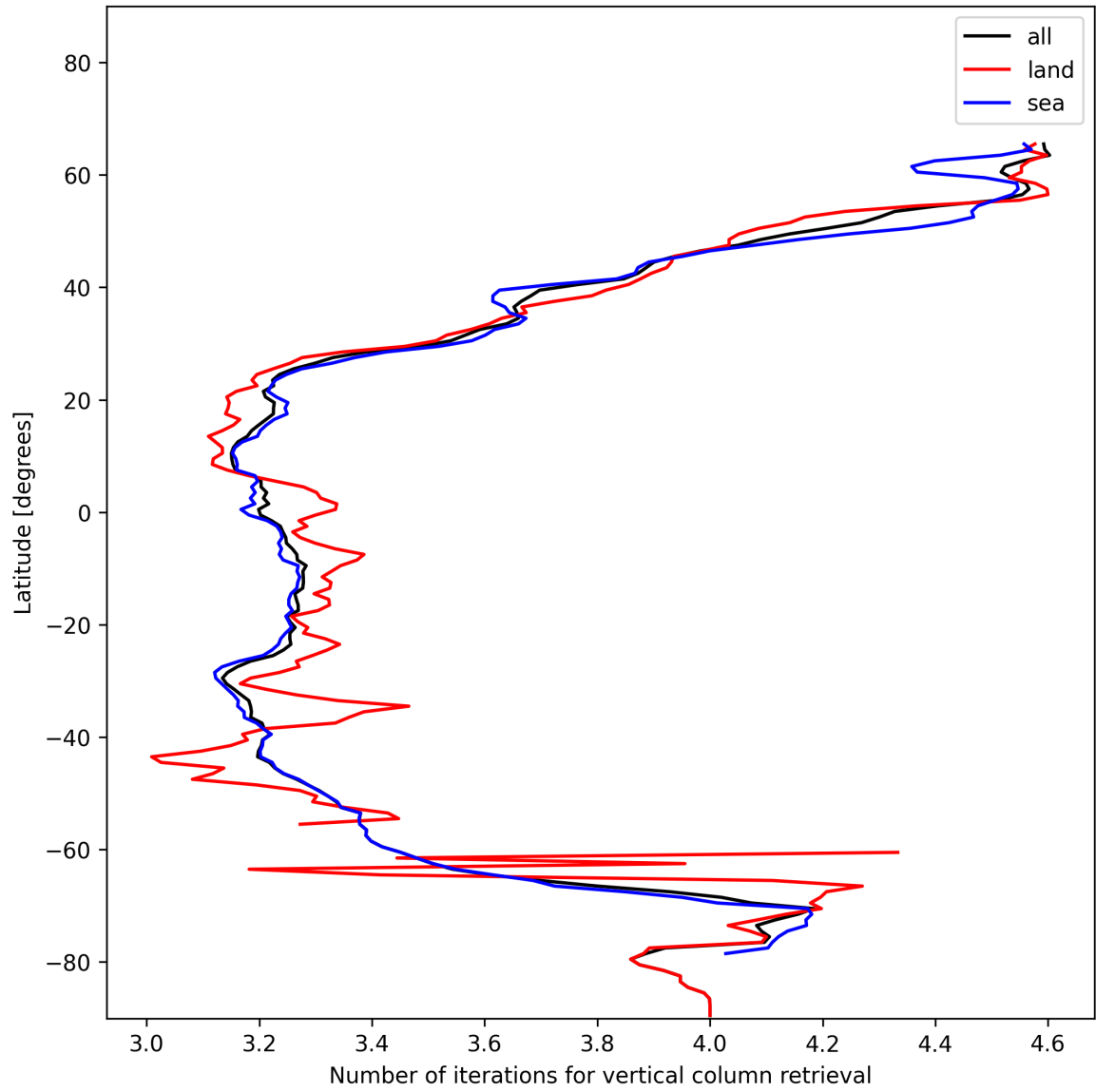
Figure 19: Zonal average of “Number of iterations for vertical column retrieval” for 2024-12-28 to 2024-12-30.
