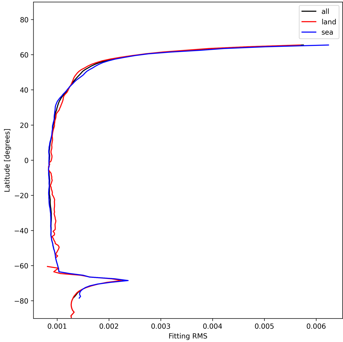
Figure 16: Zonal average of “Fitting RMS” for 2024-12-28 to 2024-12-30.
