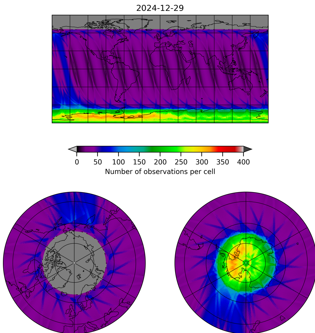
Figure 12: Map of the number of observations for 2024-12-28 to 2024-12-30
