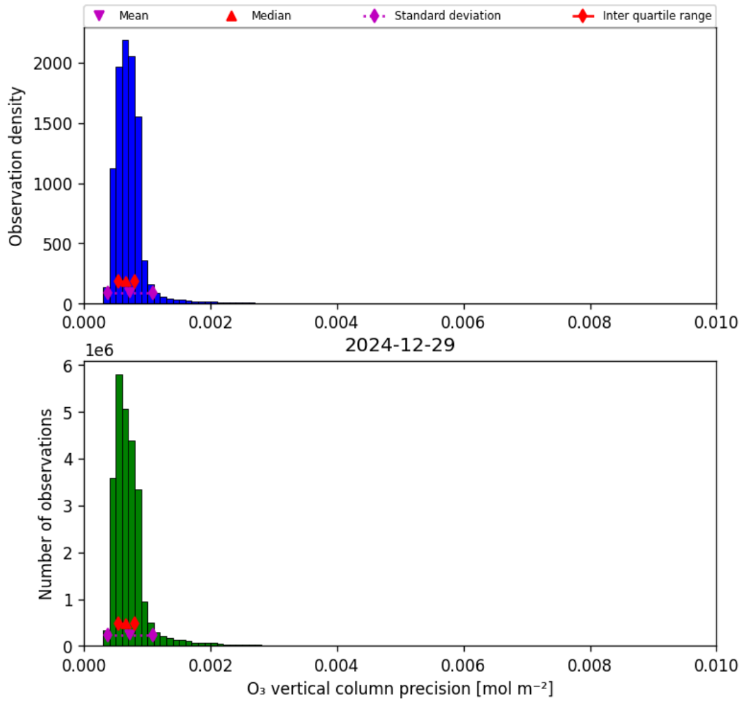
Figure 22: Histogram of “O 3 vertical column precision” for 2024-12-28 to 2024-12-30
