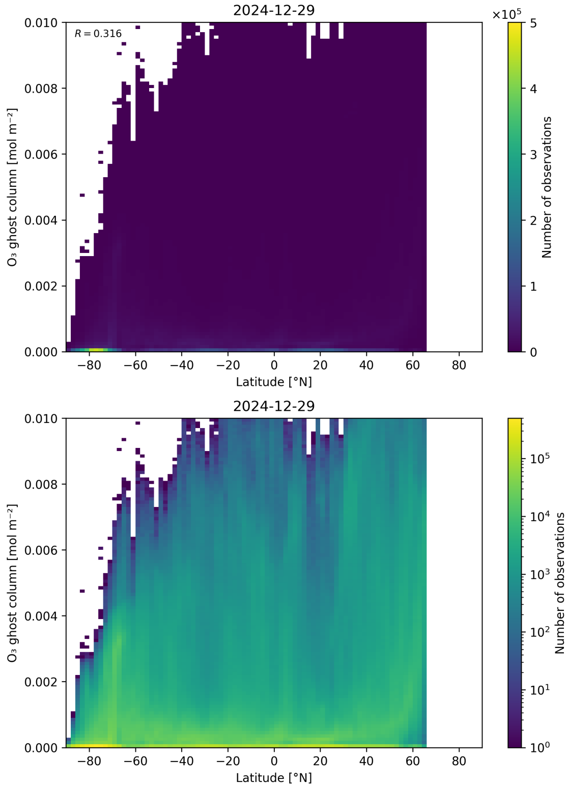
Figure 35: Scatter density plot of “Latitude” against “O 3 ghost column” for 2024-12-28 to 2024-12-30.
