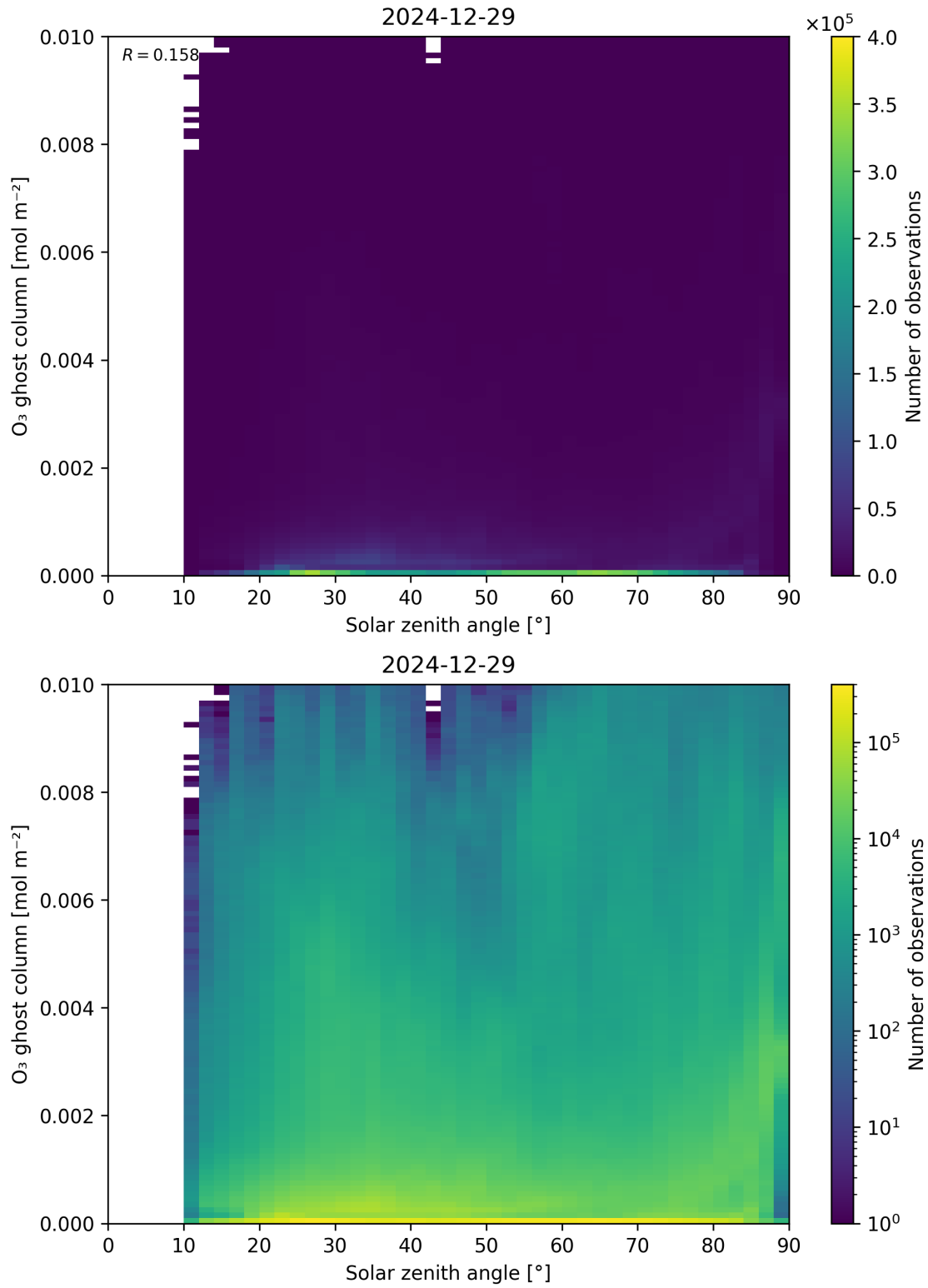
Figure 46: Scatter density plot of “Solar zenith angle” against “O 3 ghost column” for 2024-12-28 to 2024-12-30.
