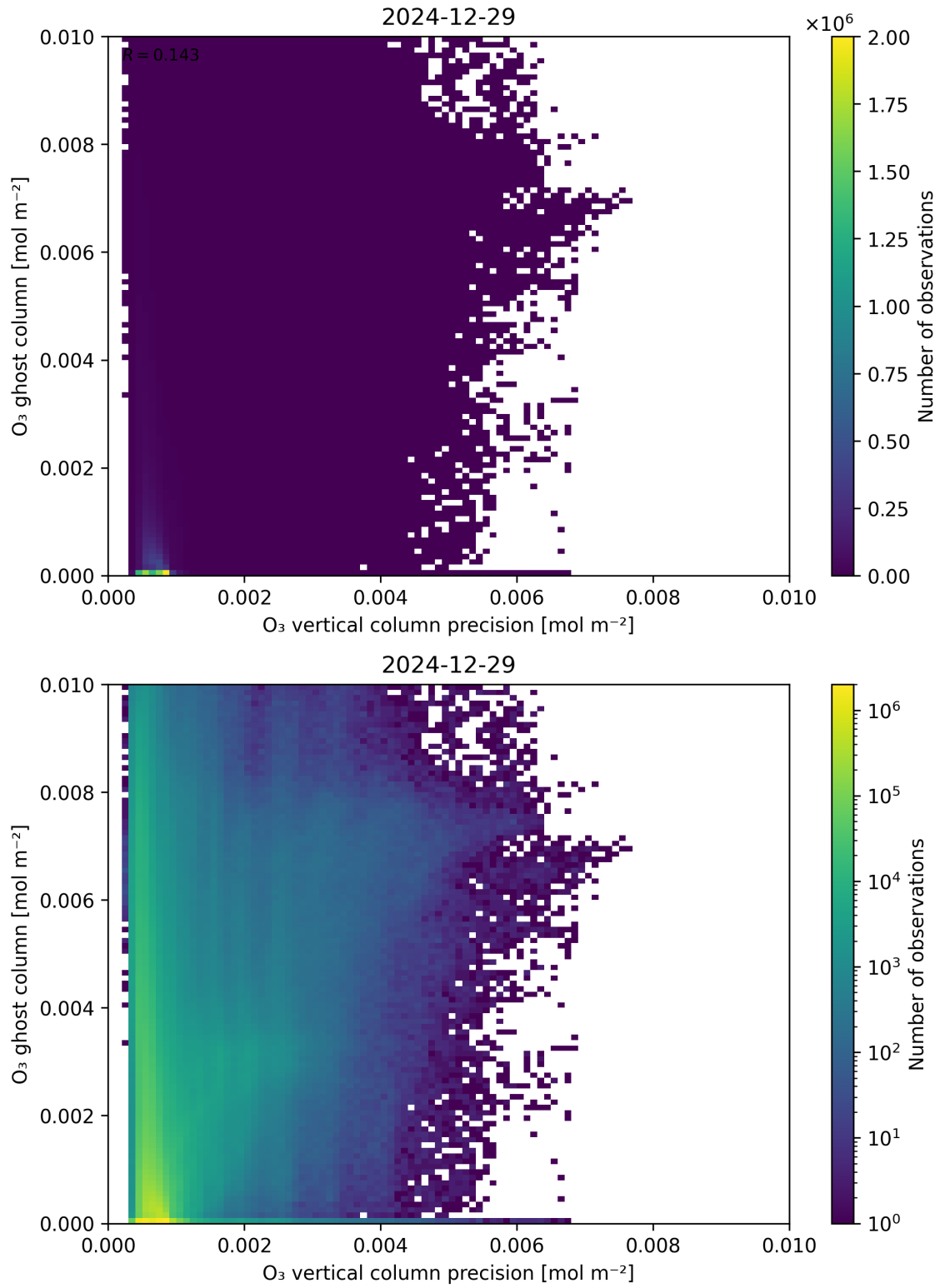
Figure 43: Scatter density plot of “ \text{O}_3 vertical column precision” against “ \text{O}_3 ghost column” for 2024-12-28 to 2024-12-30.
