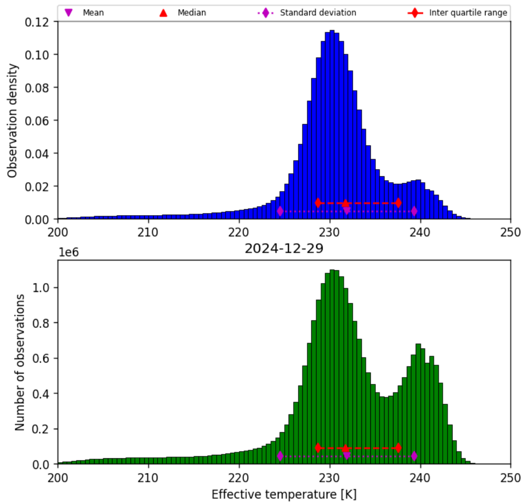
Figure 24: Histogram of “Effective temperature” for 2024-12-28 to 2024-12-30
