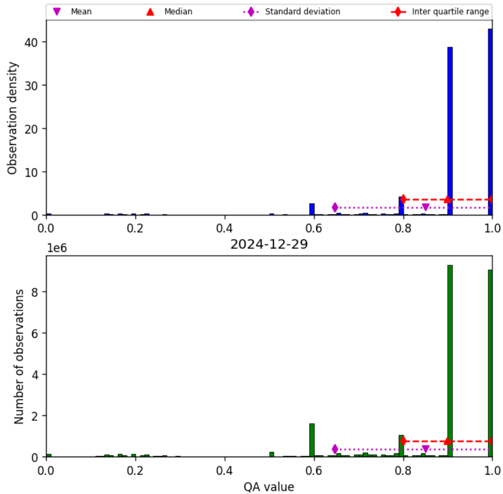
Figure 20: Histogram of “QA value” for 2024-12-28 to 2024-12-30
