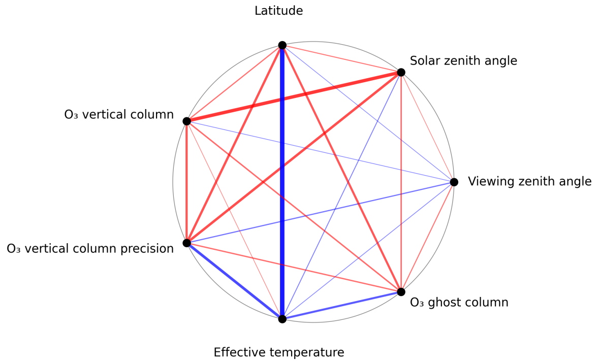
Figure 1: Map of correlation graph for 2024-12-28 to 2024-12-30.
