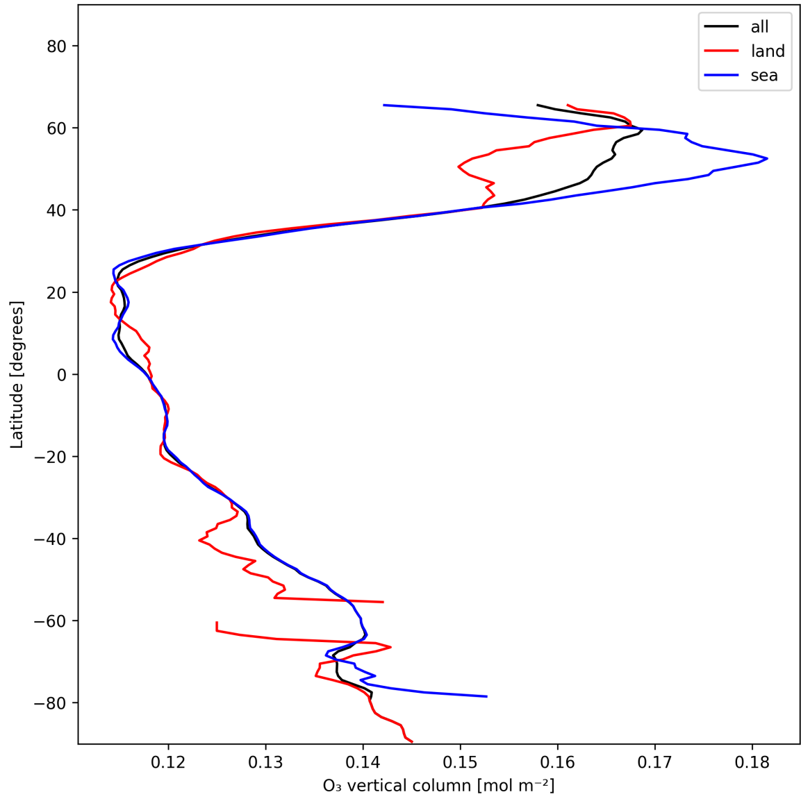
Figure 14: Zonal average of “O 3 vertical column” for 2024-12-28 to 2024-12-30.
