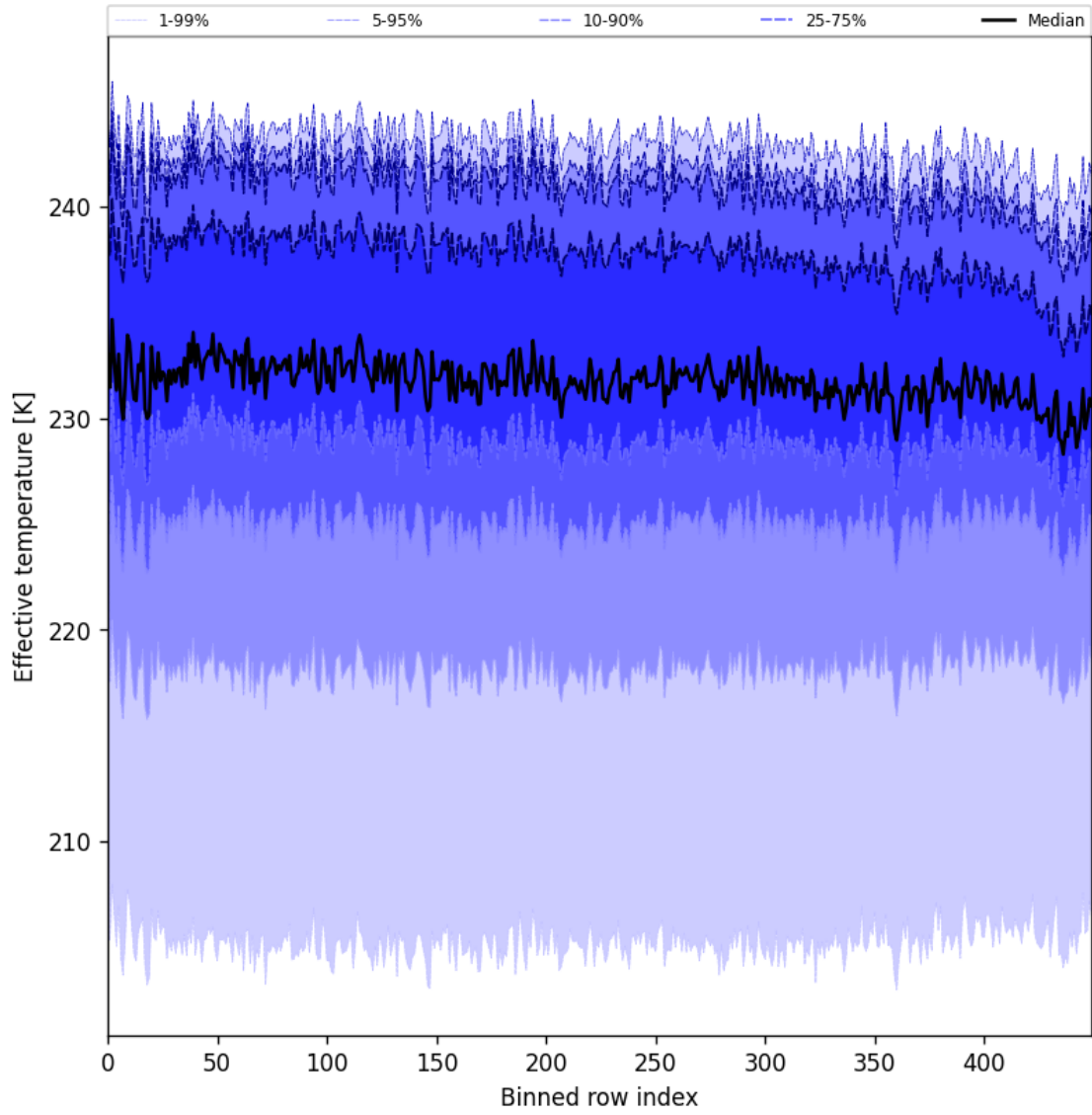
Figure 31: Along track statistics of “Effective temperature” for 2024-12-28 to 2024-12-30
