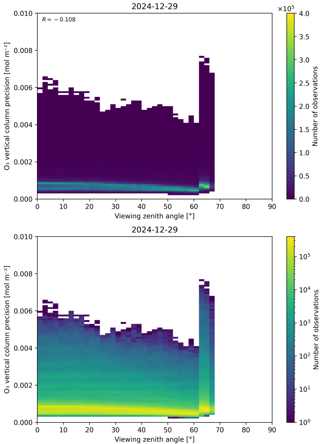
Figure 53: Scatter density plot of “Viewing zenith angle” against “O 3 vertical column precision” for 2024-12-28 to 2024-12-30.
