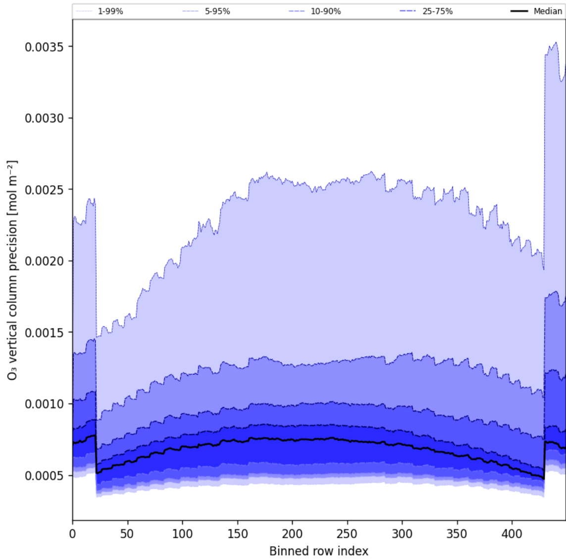
Figure 29: Along track statistics of “O 3 vertical column precision” for 2024-12-28 to 2024-12-30
