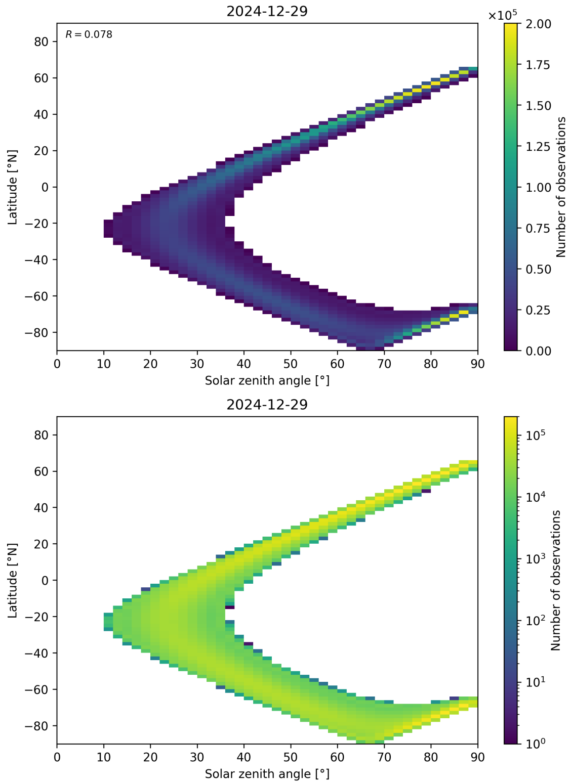
Figure 44: Scatter density plot of “Solar zenith angle” against “Latitude” for 2024-12-28 to 2024-12-30.
