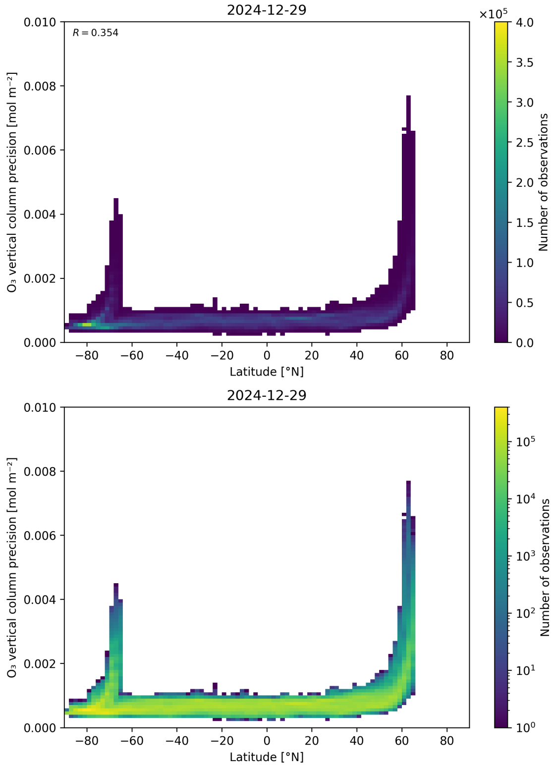
Figure 37: Scatter density plot of “Latitude” against “O 3 vertical column precision” for 2024-12-28 to 2024-12-30.
