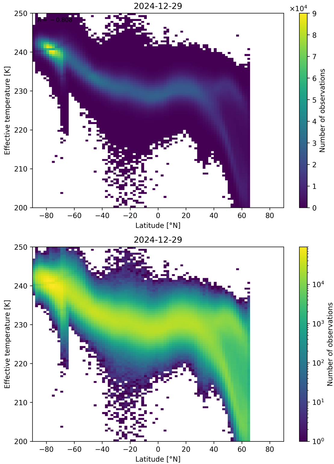
Figure 34: Scatter density plot of “Latitude” against “Effective temperature” for 2024-12-28 to 2024-12-30.
