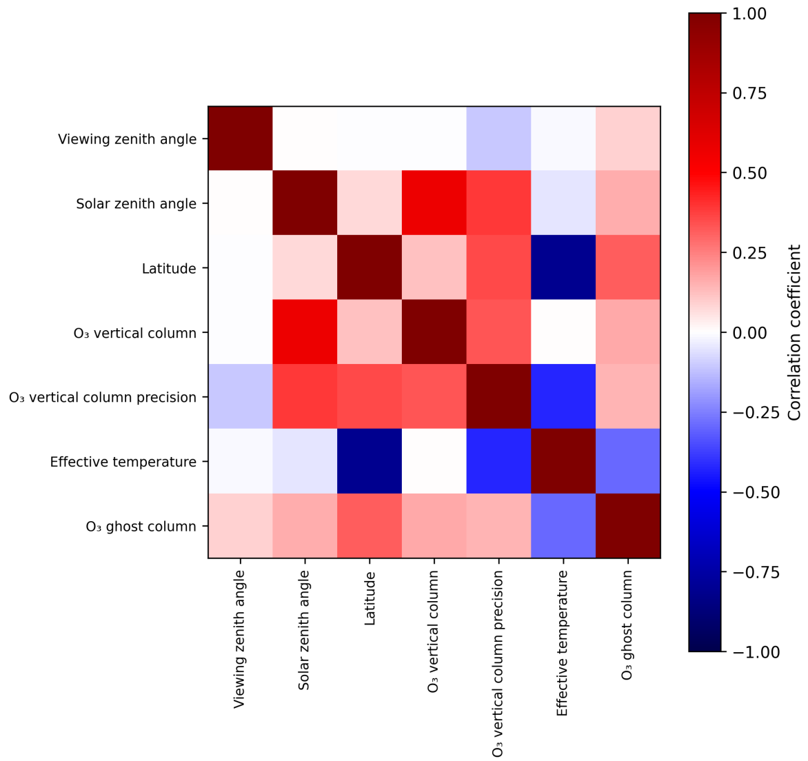
Figure 2: Map of correlation matrix for 2024-12-28 to 2024-12-30.
