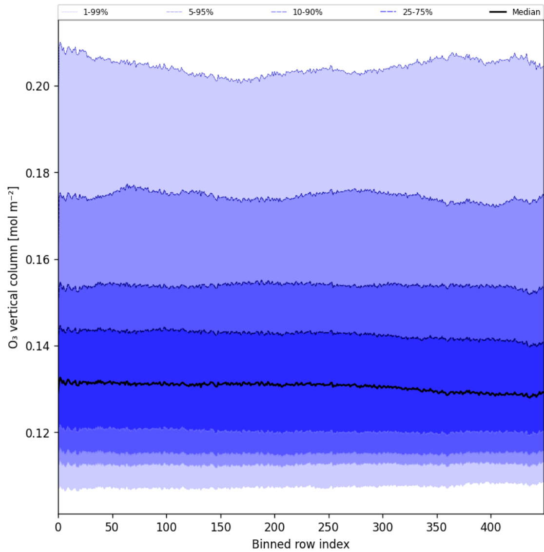
Figure 28: Along track statistics of “O 3 vertical column” for 2024-12-28 to 2024-12-30
