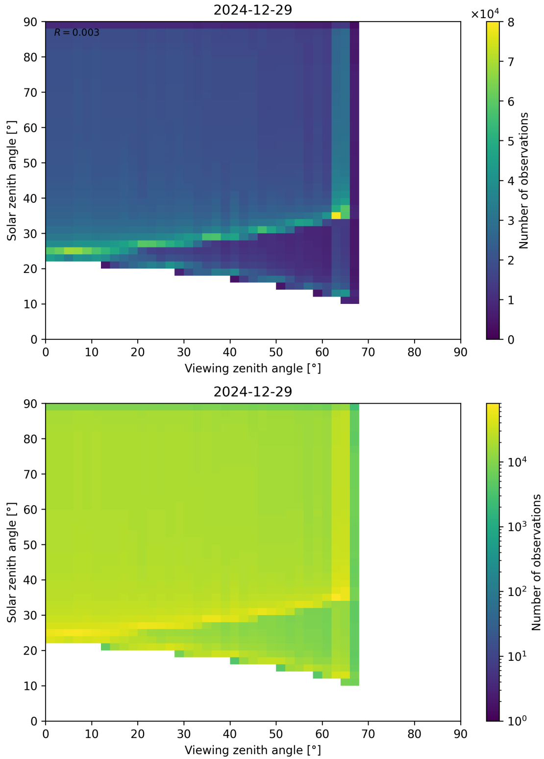
Figure 54: Scatter density plot of “Viewing zenith angle” against “Solar zenith angle” for 2024-12-28 to 2024-12-30.
