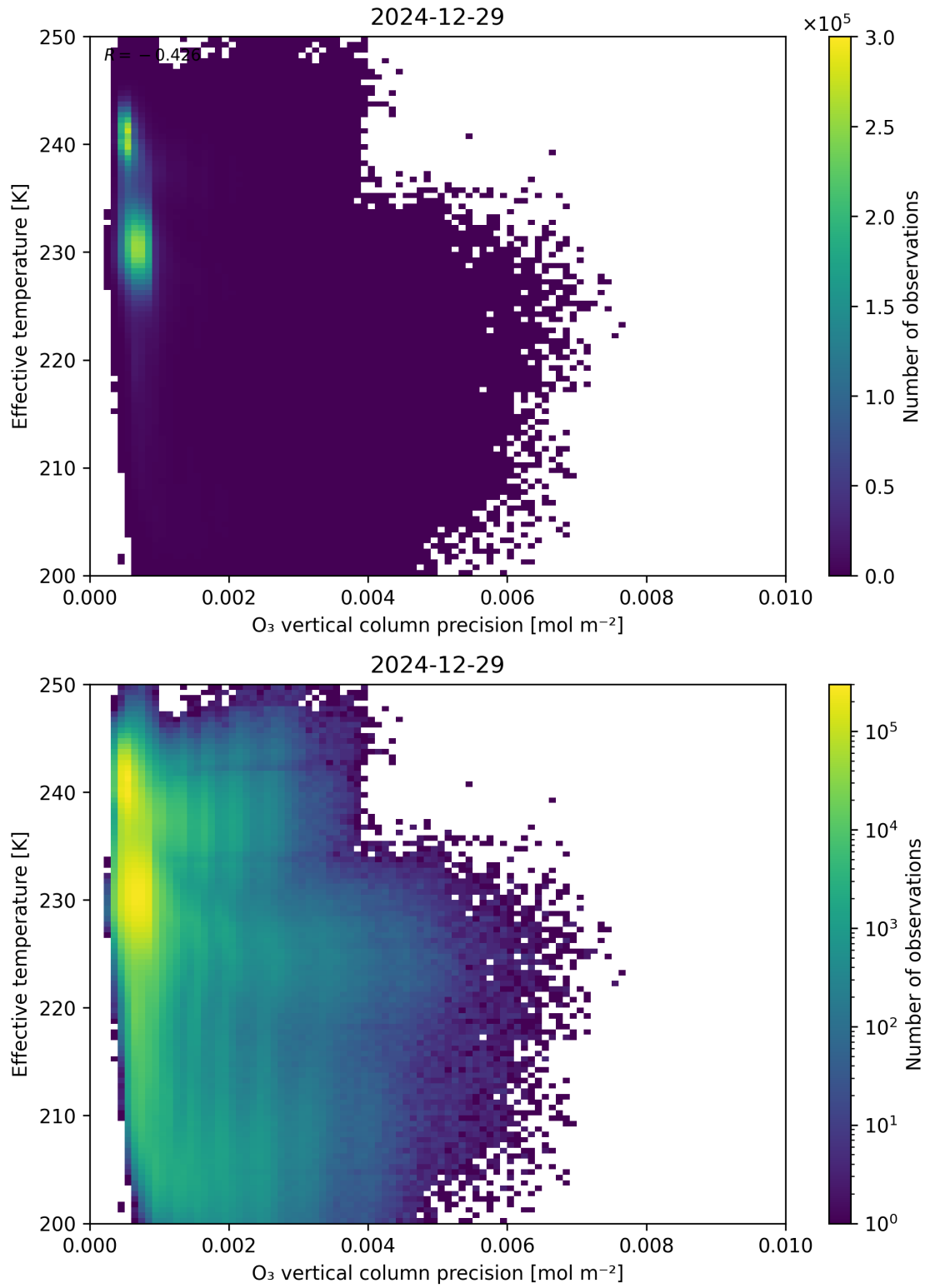
Figure 42: Scatter density plot of “O 3 vertical column precision” against “Effective temperature” for 2024-12-28 to 2024-12-30.
