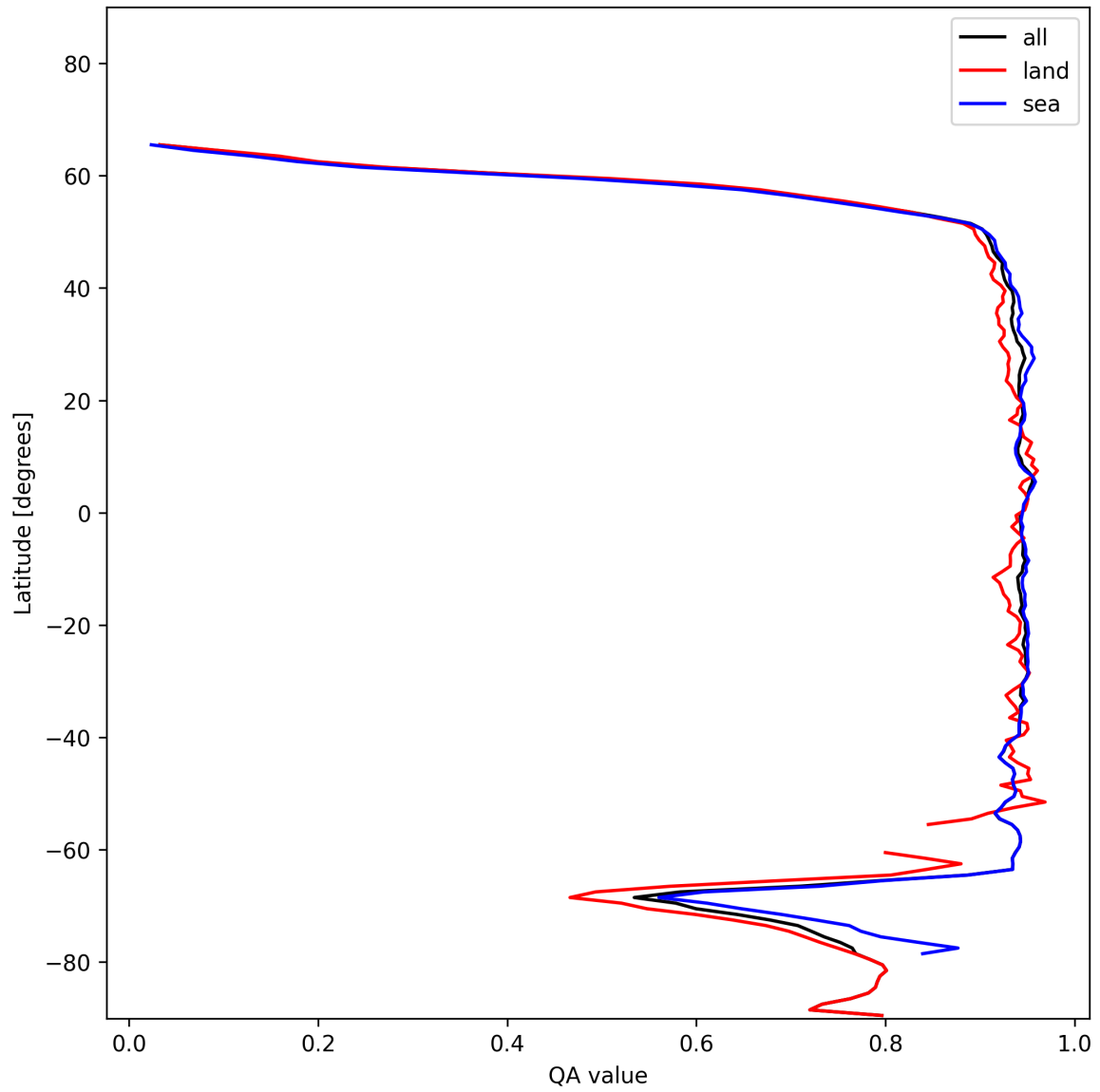
Figure 13: Zonal average of “QA value” for 2024-12-28 to 2024-12-30.
