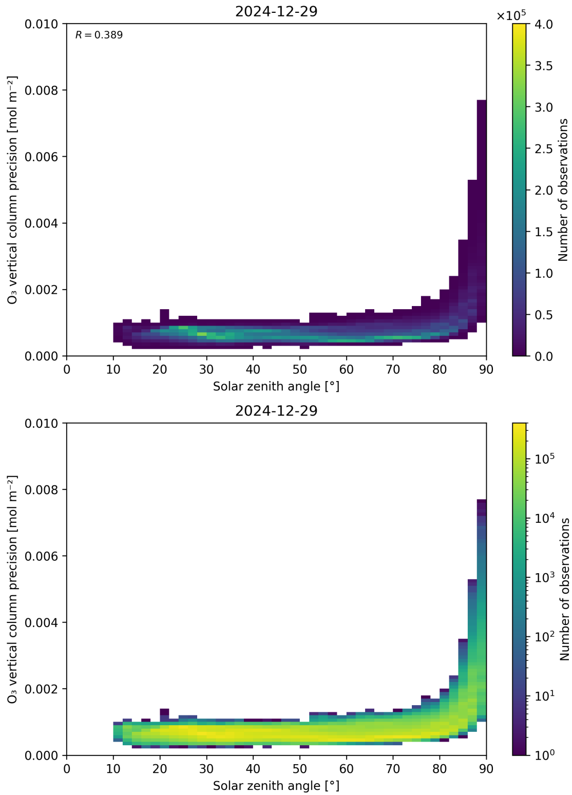
Figure 48: Scatter density plot of “Solar zenith angle” against “O 3 vertical column precision” for 2024-12-28 to 2024-12-30.
