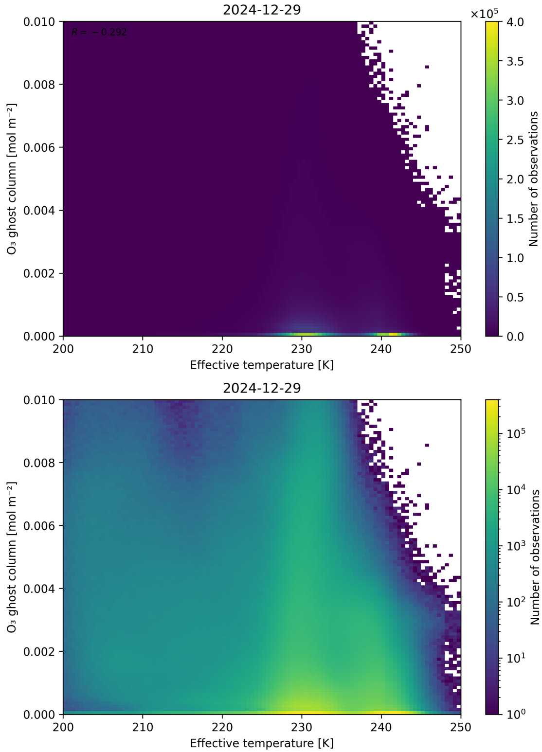
Figure 38: Scatter density plot of “Effective temperature” against “O 3 ghost column” for 2024-12-28 to 2024-12-30.
