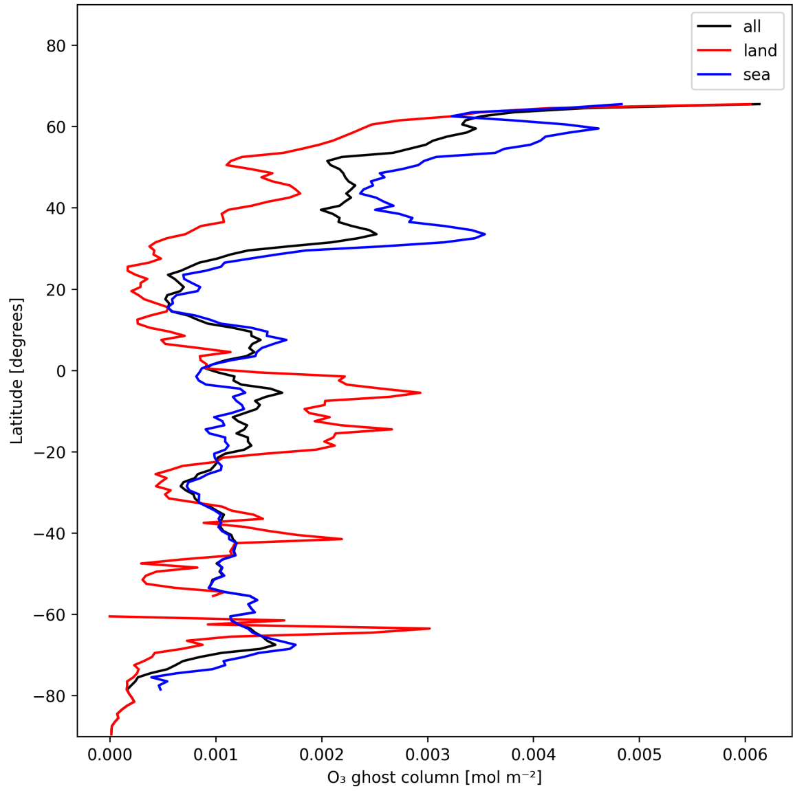
Figure 18: Zonal average of “O 3 ghost column” for 2024-12-28 to 2024-12-30.
