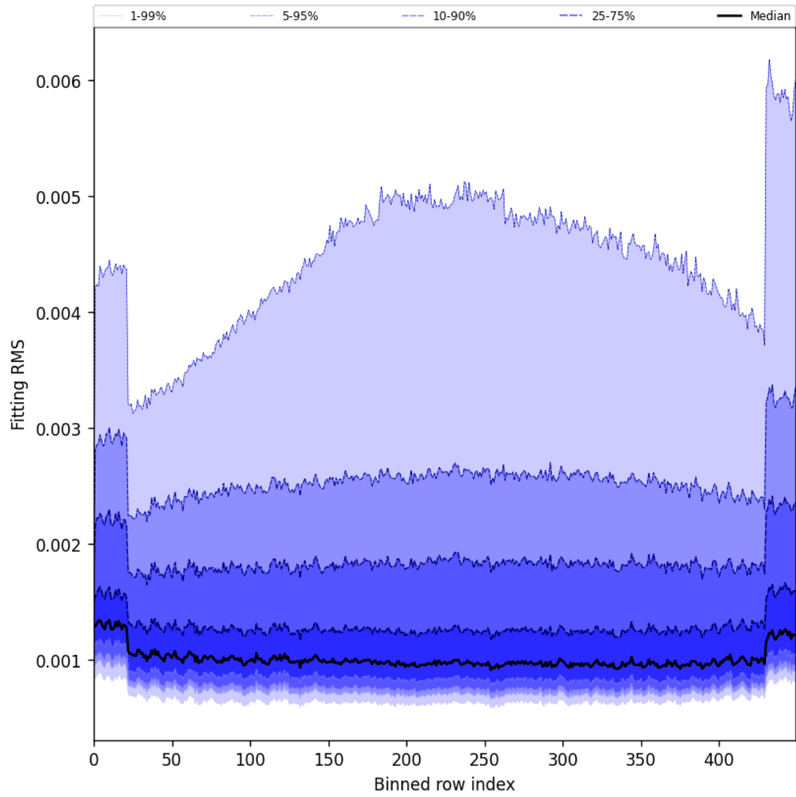
Figure 30: Along track statistics of “Fitting RMS” for 2024-12-28 to 2024-12-30
