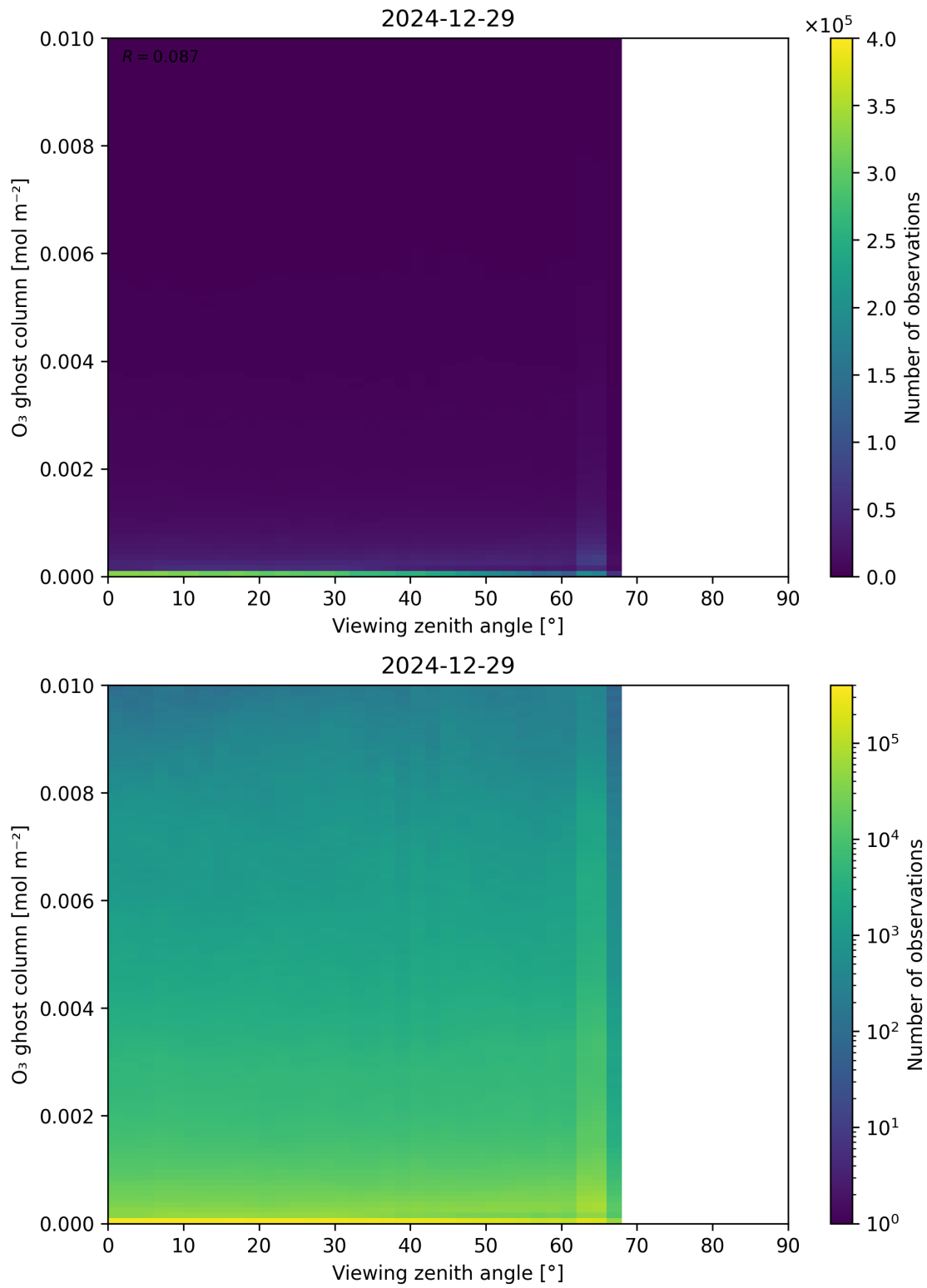
Figure 51: Scatter density plot of “Viewing zenith angle” against “O 3 ghost column” for 2024-12-28 to 2024-12-30.
