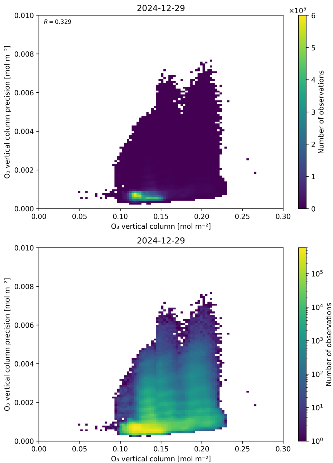
Figure 41: Scatter density plot of “O 3 vertical column” against “O 3 vertical column precision” for 2024-12-28 to 2024-12-30.
