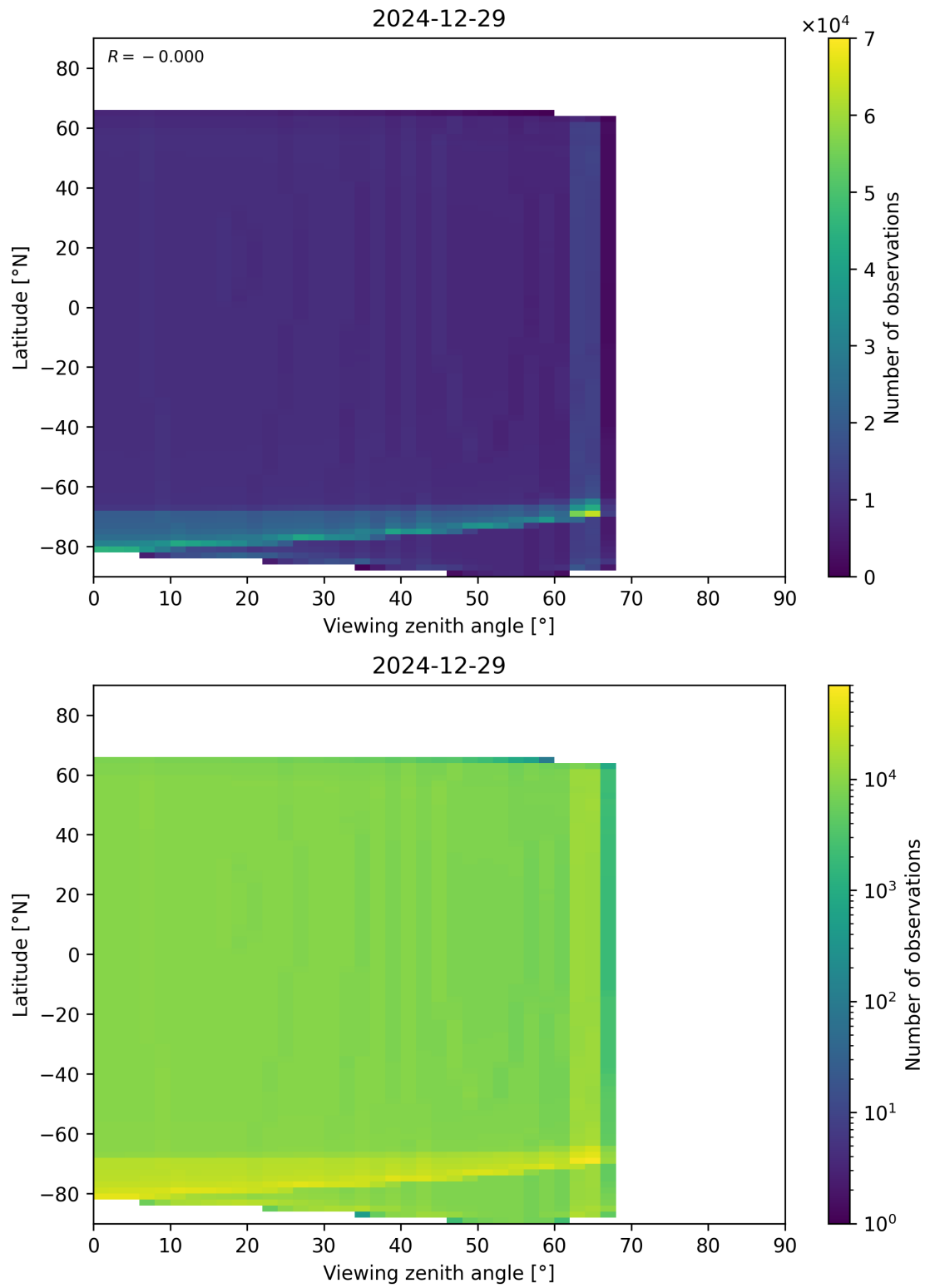
Figure 49: Scatter density plot of “Viewing zenith angle” against “Latitude” for 2024-12-28 to 2024-12-30.
