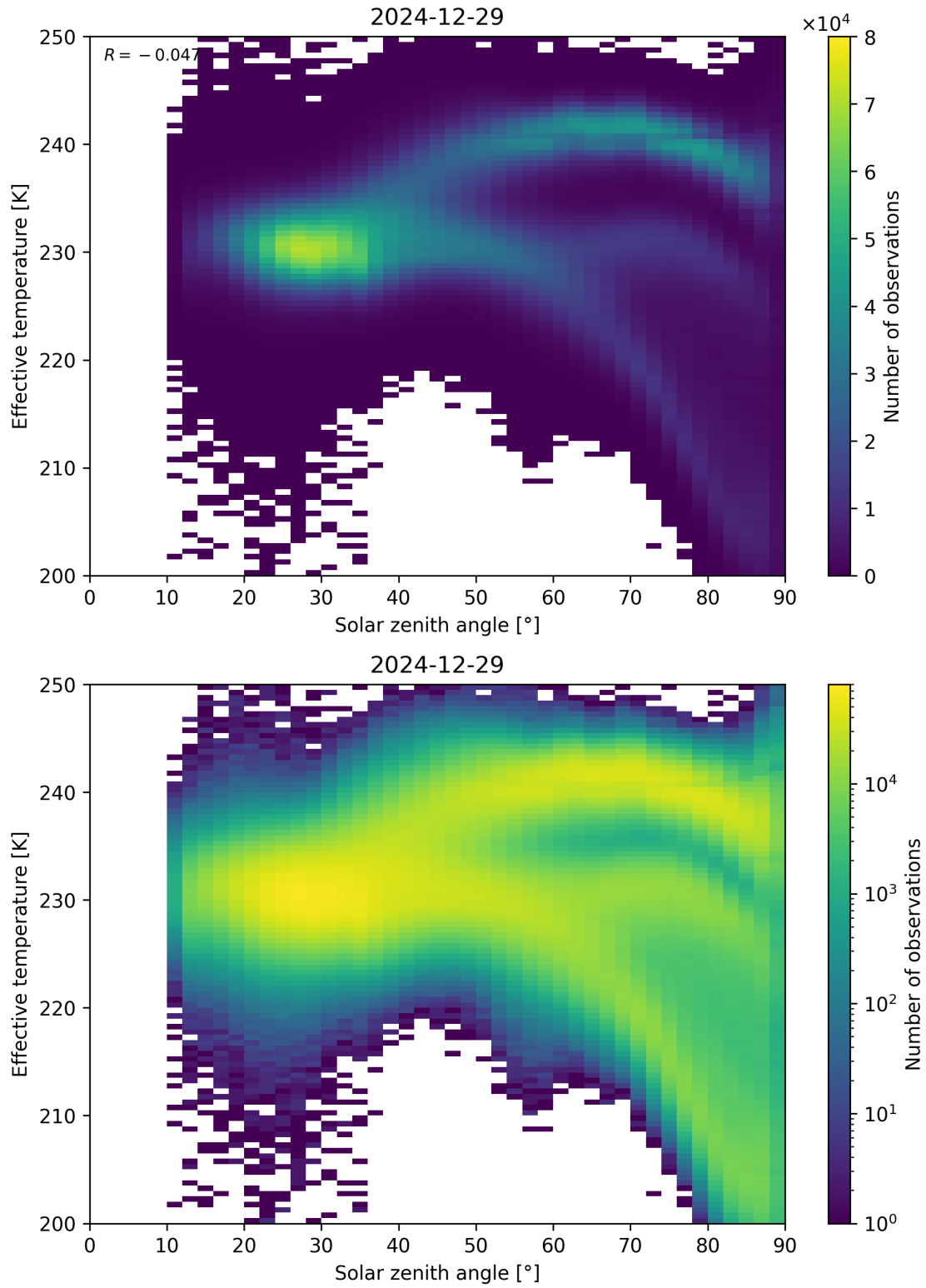
Figure 45: Scatter density plot of “Solar zenith angle” against “Effective temperature” for 2024-12-28 to 2024-12-30.
