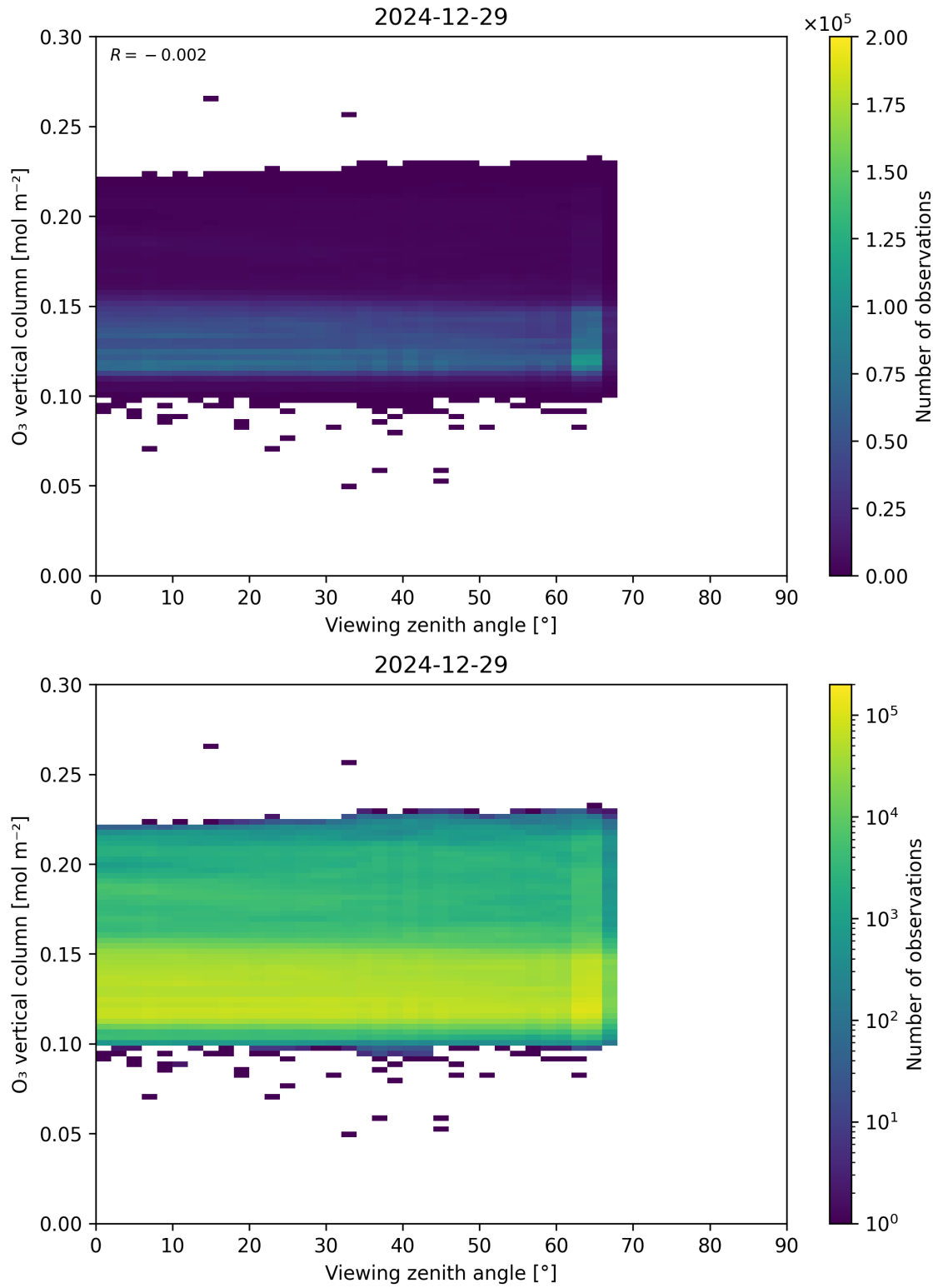
Figure 52: Scatter density plot of “Viewing zenith angle” against “O 3 vertical column” for 2024-12-28 to 2024-12-30.
