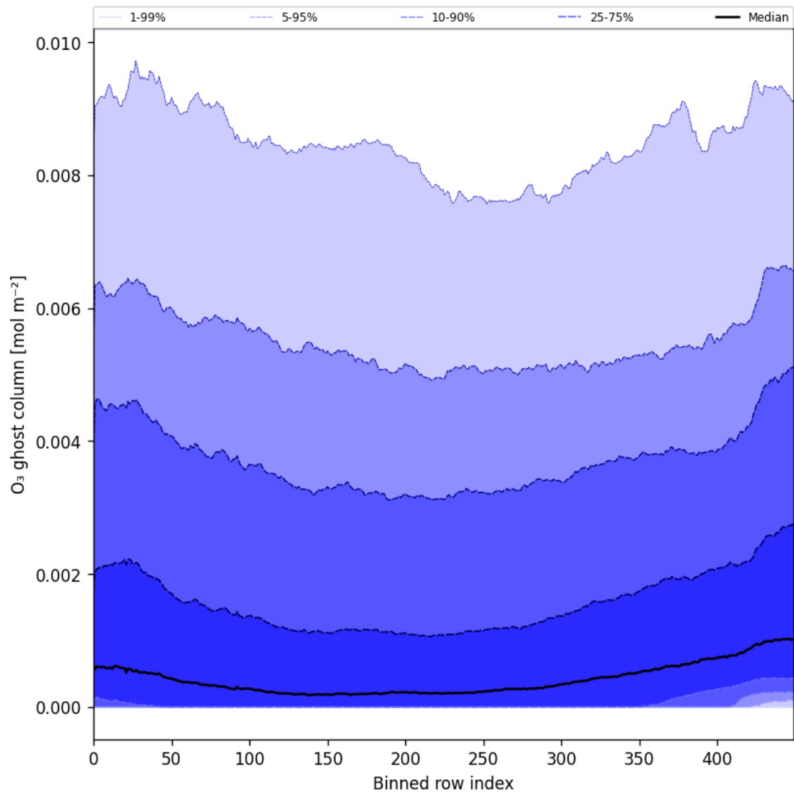
Figure 32: Along track statistics of “O 3 ghost column” for 2024-12-29 to 2024-12-31
