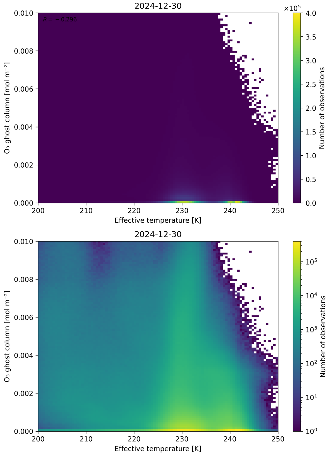
Figure 38: Scatter density plot of “Effective temperature” against “O 3 ghost column” for 2024-12-29 to 2024-12-31.
