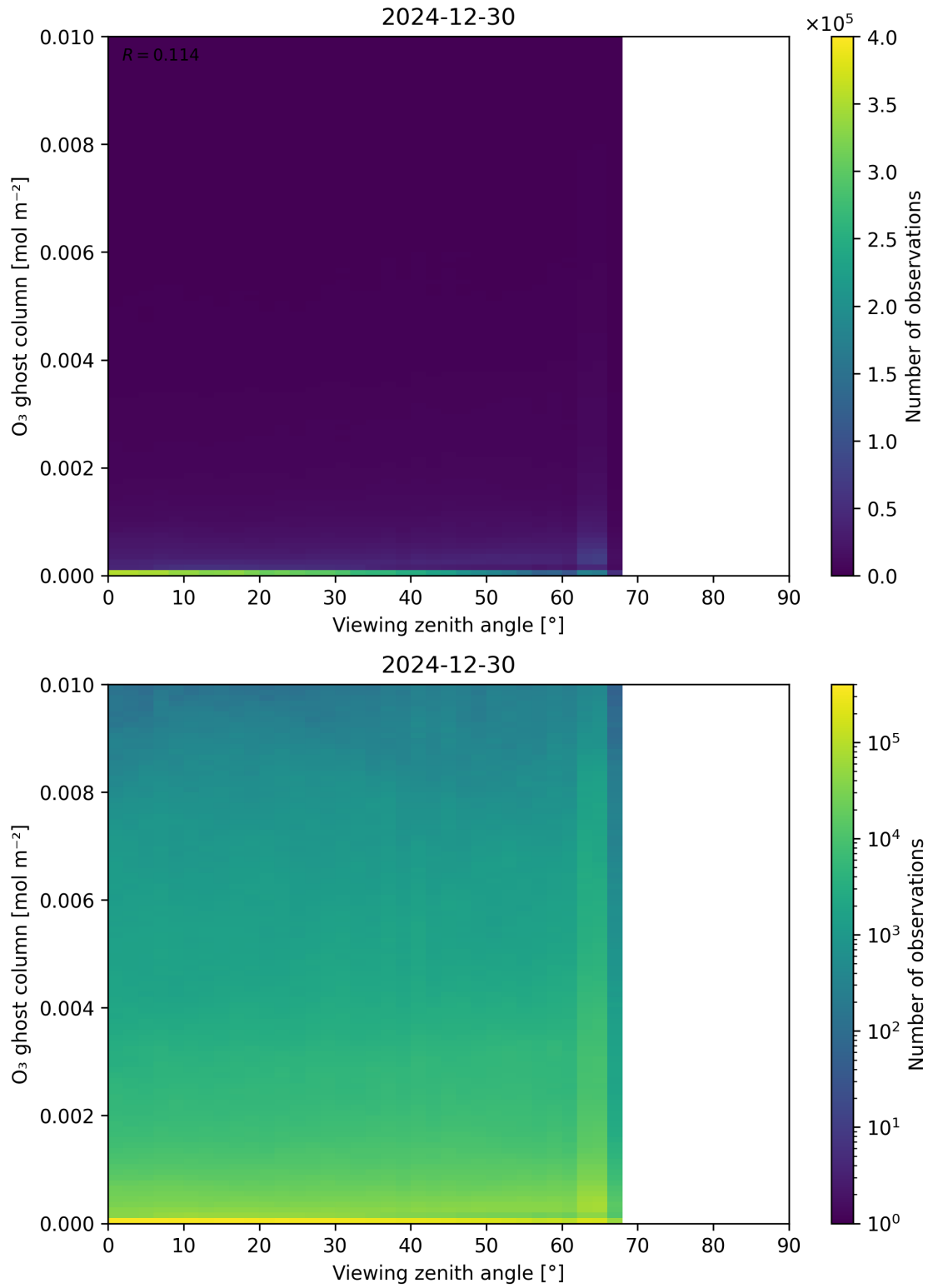
Figure 51: Scatter density plot of “Viewing zenith angle” against “O 3 ghost column” for 2024-12-29 to 2024-12-31.
