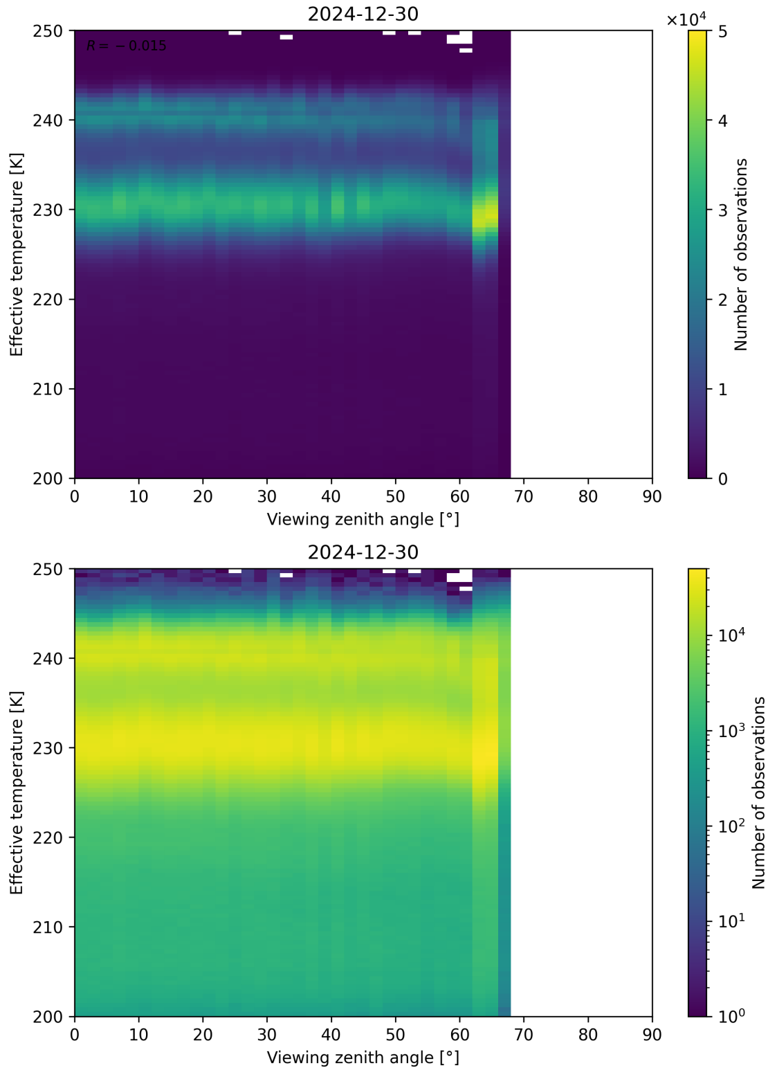
Figure 50: Scatter density plot of “Viewing zenith angle” against “Effective temperature” for 2024-12-29 to 2024-12-31.
