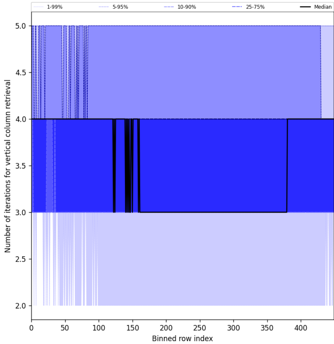
Figure 33: Along track statistics of “Number of iterations for vertical column retrieval” for 2024-12-29 to 2024-12-31
