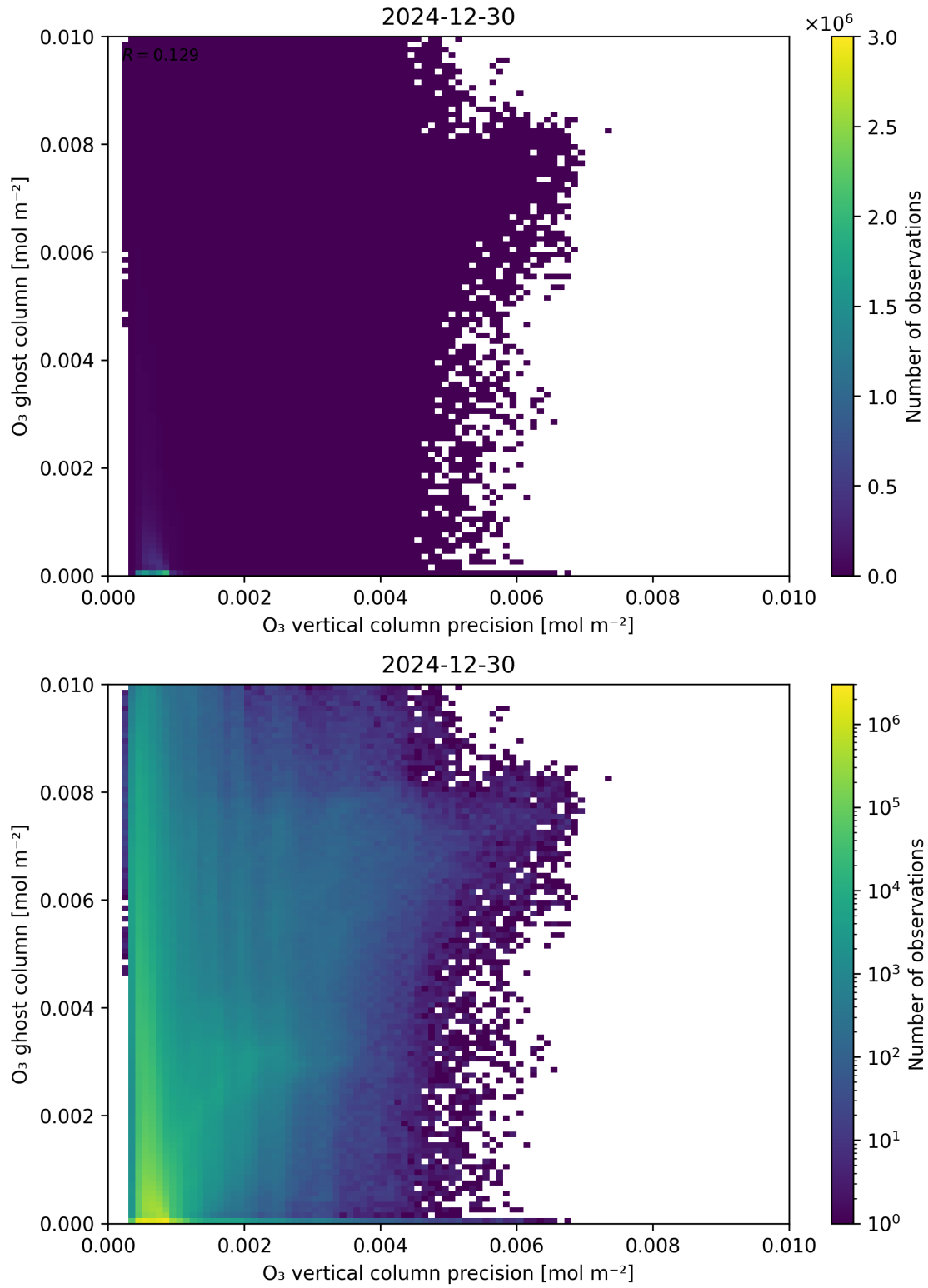
Figure 43: Scatter density plot of “ O_3 vertical column precision” against “ O_3 ghost column” for 2024-12-29 to 2024-12-31.
