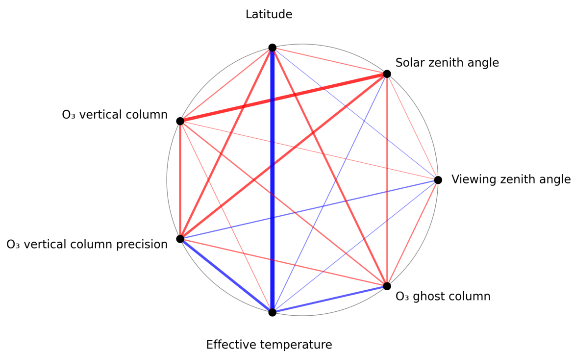
Figure 1: Map of correlation graph for 2024-12-29 to 2024-12-31.
