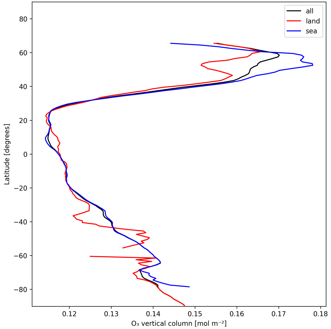
Figure 14: Zonal average of “O 3 vertical column” for 2024-12-29 to 2024-12-31.
