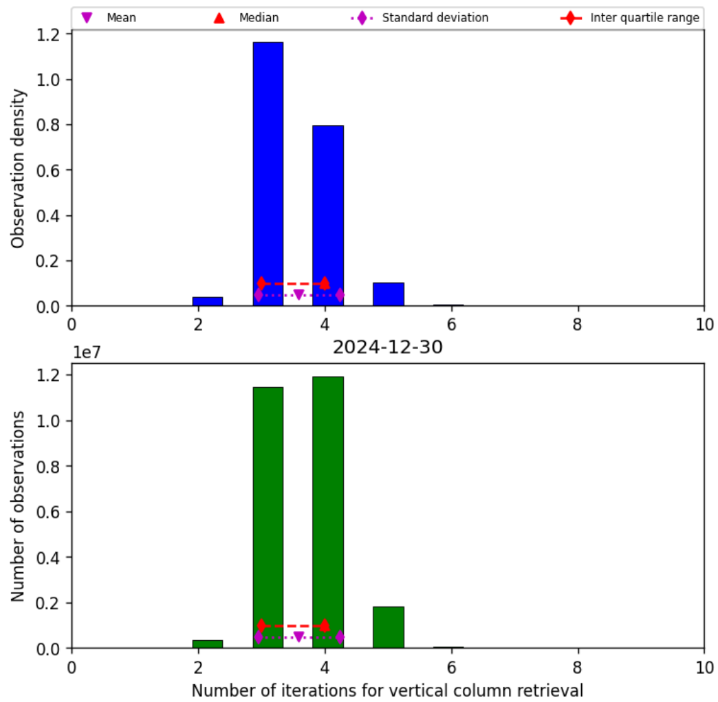
Figure 26: Histogram of “Number of iterations for vertical column retrieval” for 2024-12-29 to 2024-12-31
