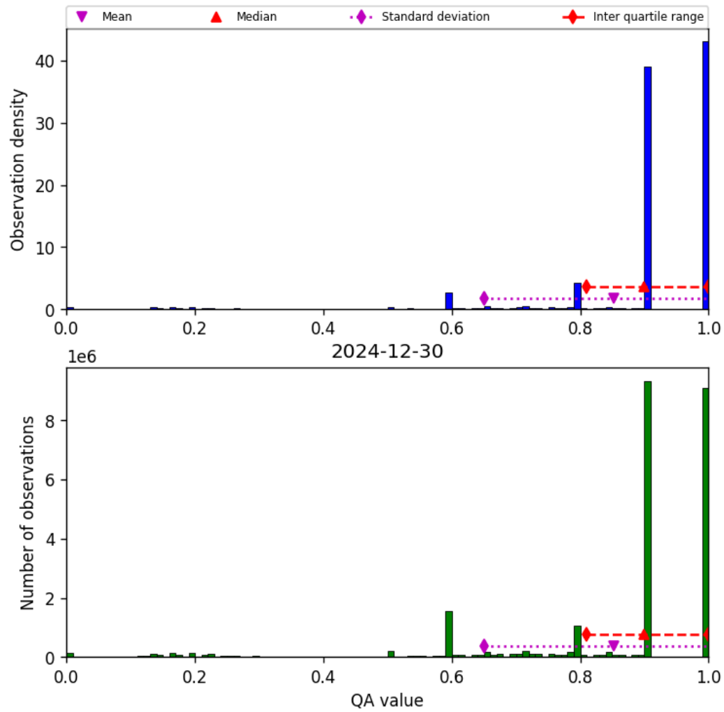
Figure 20: Histogram of “QA value” for 2024-12-29 to 2024-12-31
