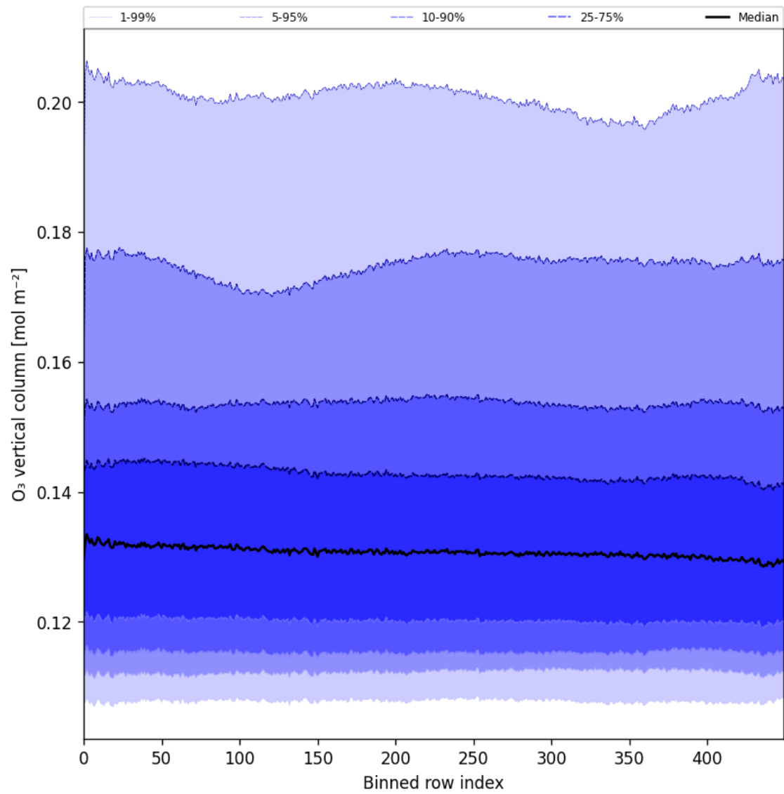
Figure 28: Along track statistics of “O 3 vertical column” for 2024-12-29 to 2024-12-31
