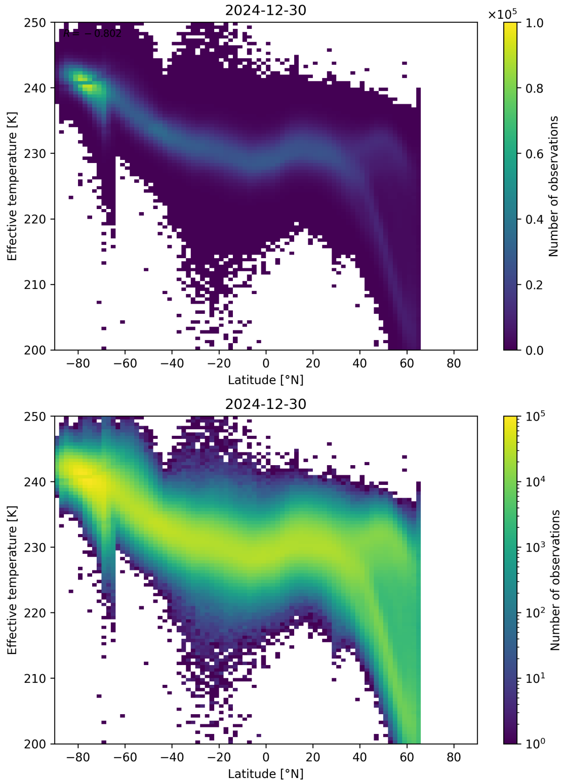
Figure 34: Scatter density plot of “Latitude” against “Effective temperature” for 2024-12-29 to 2024-12-31.
