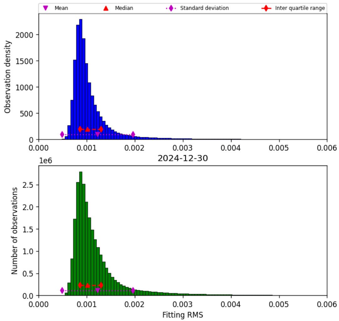
Figure 23: Histogram of “Fitting RMS” for 2024-12-29 to 2024-12-31
