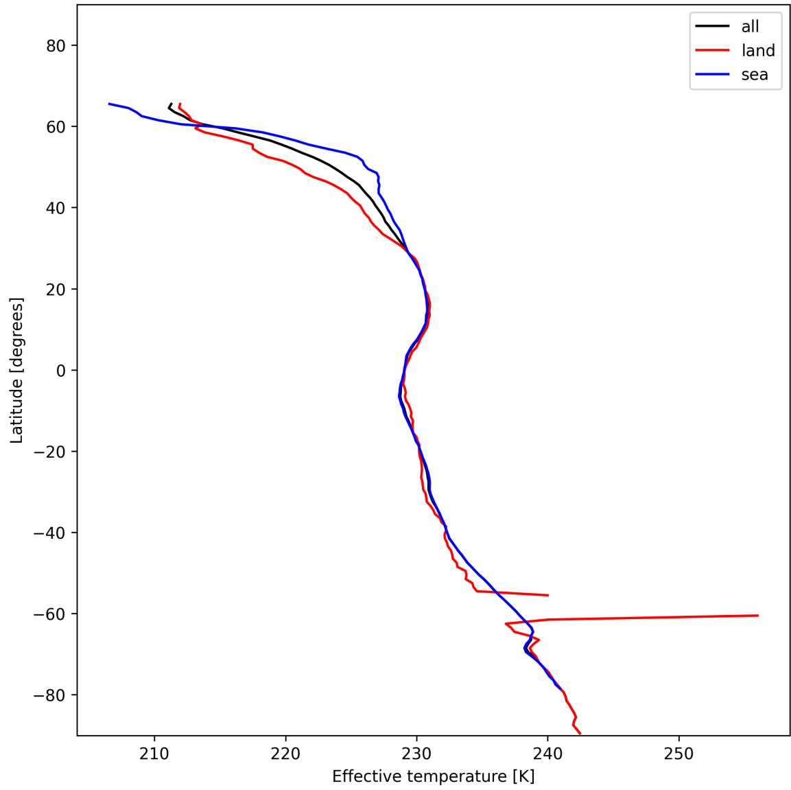
Figure 17: Zonal average of “Effective temperature” for 2024-12-29 to 2024-12-31.
