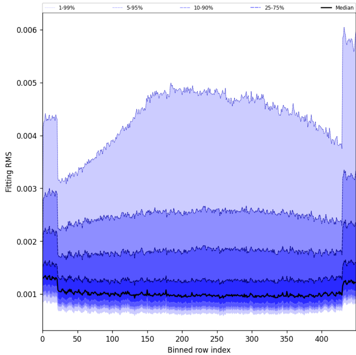
Figure 30: Along track statistics of “Fitting RMS” for 2024-12-29 to 2024-12-31
