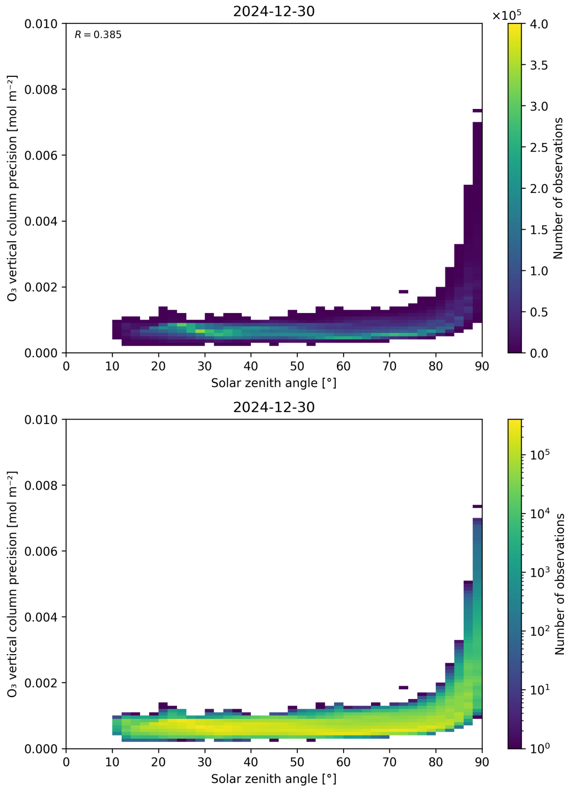
Figure 48: Scatter density plot of “Solar zenith angle” against “O 3 vertical column precision” for 2024-12-29 to 2024-12-31.
