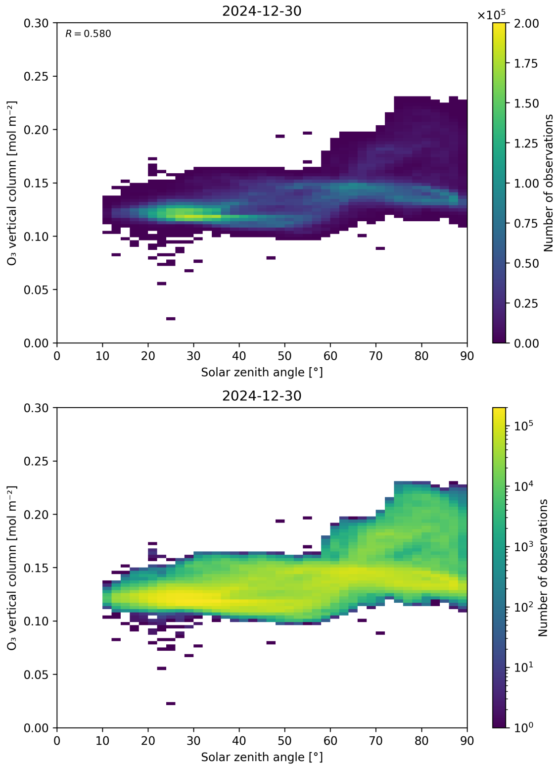
Figure 47: Scatter density plot of “Solar zenith angle” against “O 3 vertical column” for 2024-12-29 to 2024-12-31.
