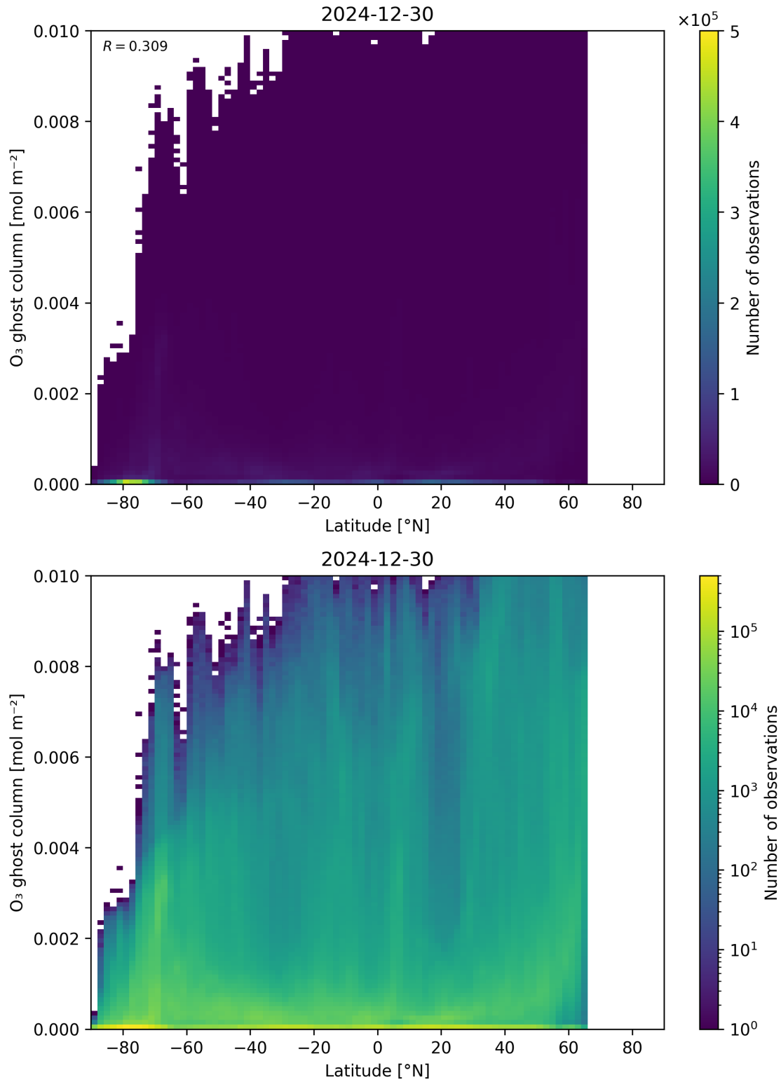
Figure 35: Scatter density plot of “Latitude” against “O 3 ghost column” for 2024-12-29 to 2024-12-31.
