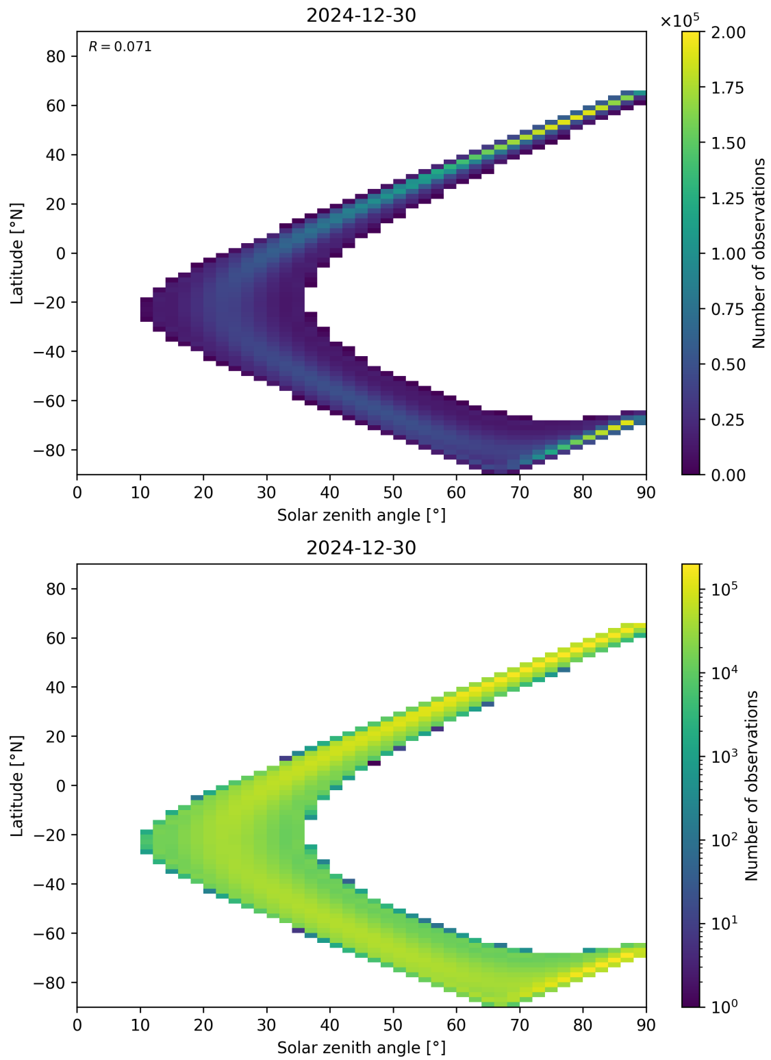
Figure 44: Scatter density plot of “Solar zenith angle” against “Latitude” for 2024-12-29 to 2024-12-31.
