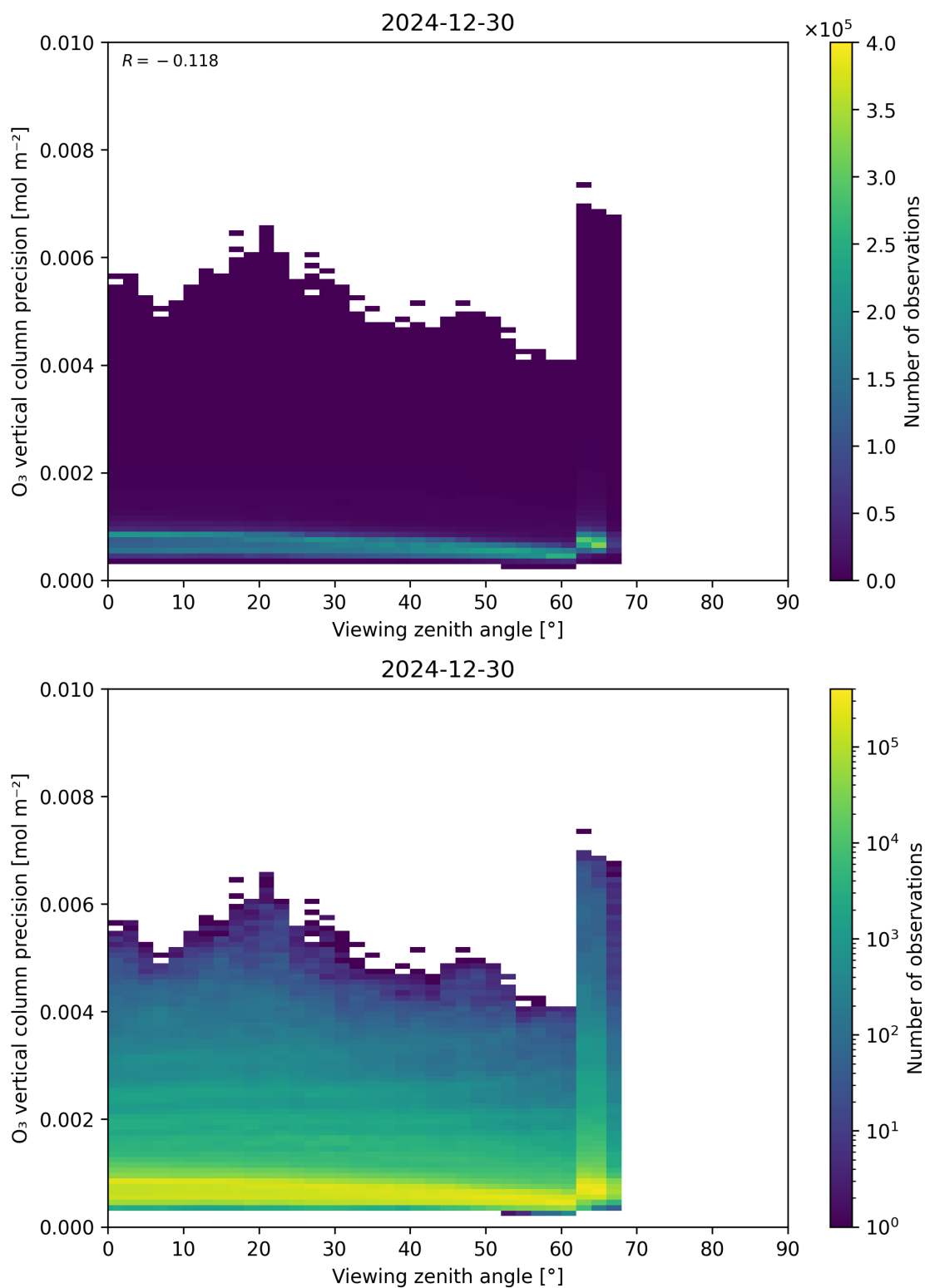
Figure 53: Scatter density plot of “Viewing zenith angle” against “O 3 vertical column precision” for 2024-12-29 to 2024-12-31.
