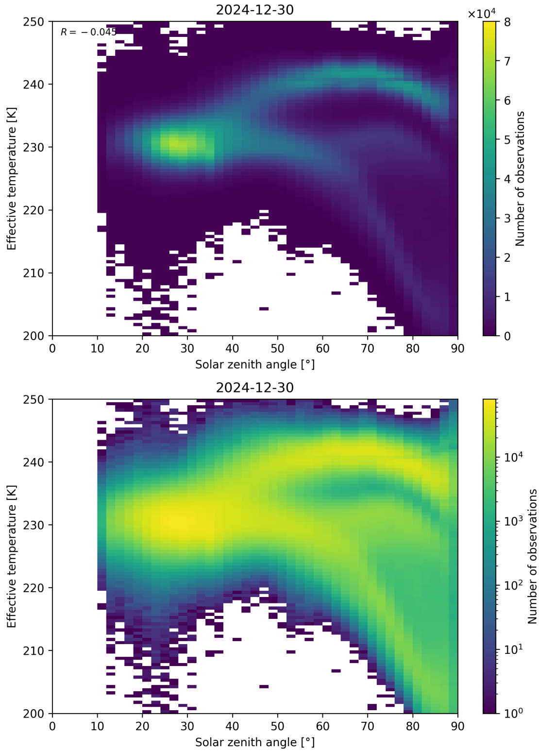
Figure 45: Scatter density plot of “Solar zenith angle” against “Effective temperature” for 2024-12-29 to 2024-12-31.
