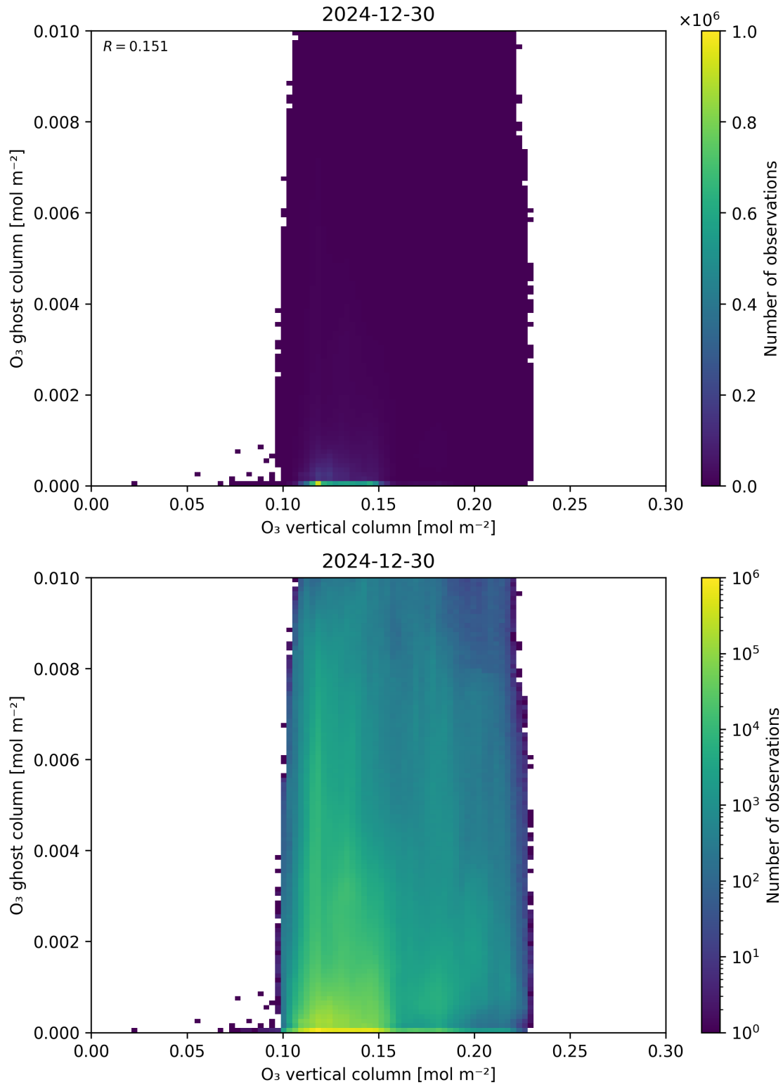
Figure 40: Scatter density plot of “O 3 vertical column” against “O 3 ghost column” for 2024-12-29 to 2024-12-31.
