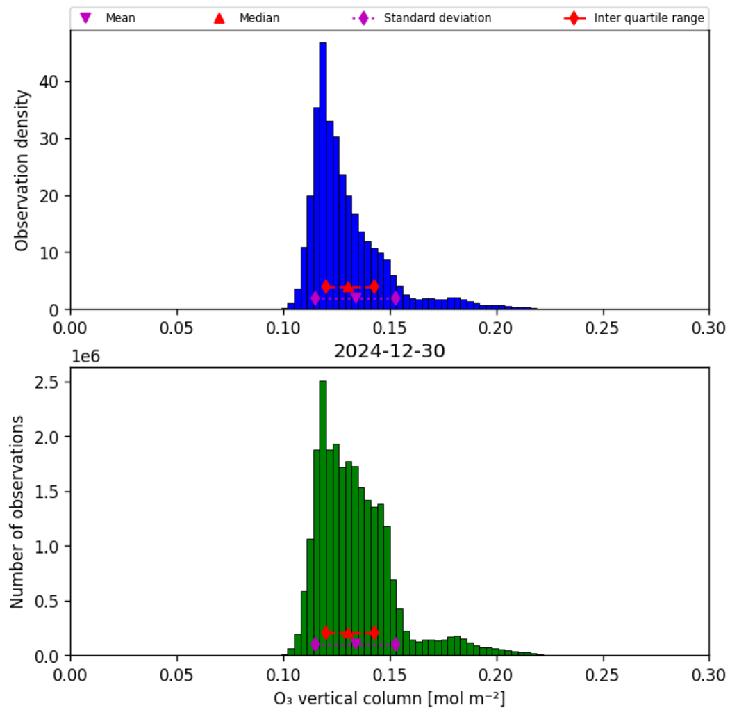
Figure 21: Histogram of “O 3 vertical column” for 2024-12-29 to 2024-12-31
