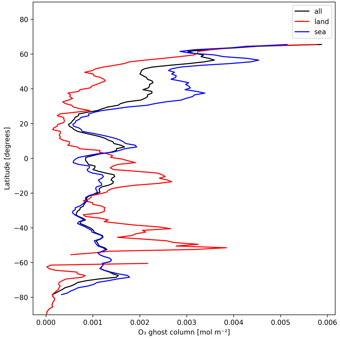
Figure 18: Zonal average of “O 3 ghost column” for 2024-12-29 to 2024-12-31.
