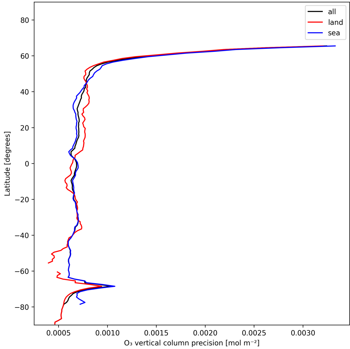
Figure 15: Zonal average of "O 3 vertical column precision" for 2024-12-29 to 2024-12-31.
