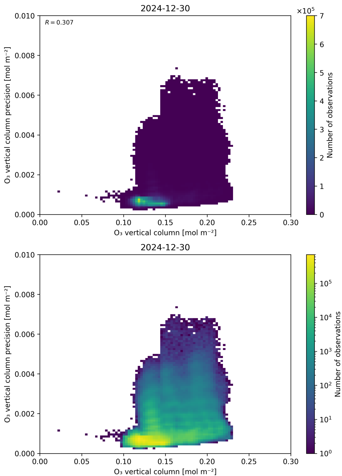
Figure 41: Scatter density plot of “O 3 vertical column” against “O 3 vertical column precision” for 2024-12-29 to 2024-12-31.
