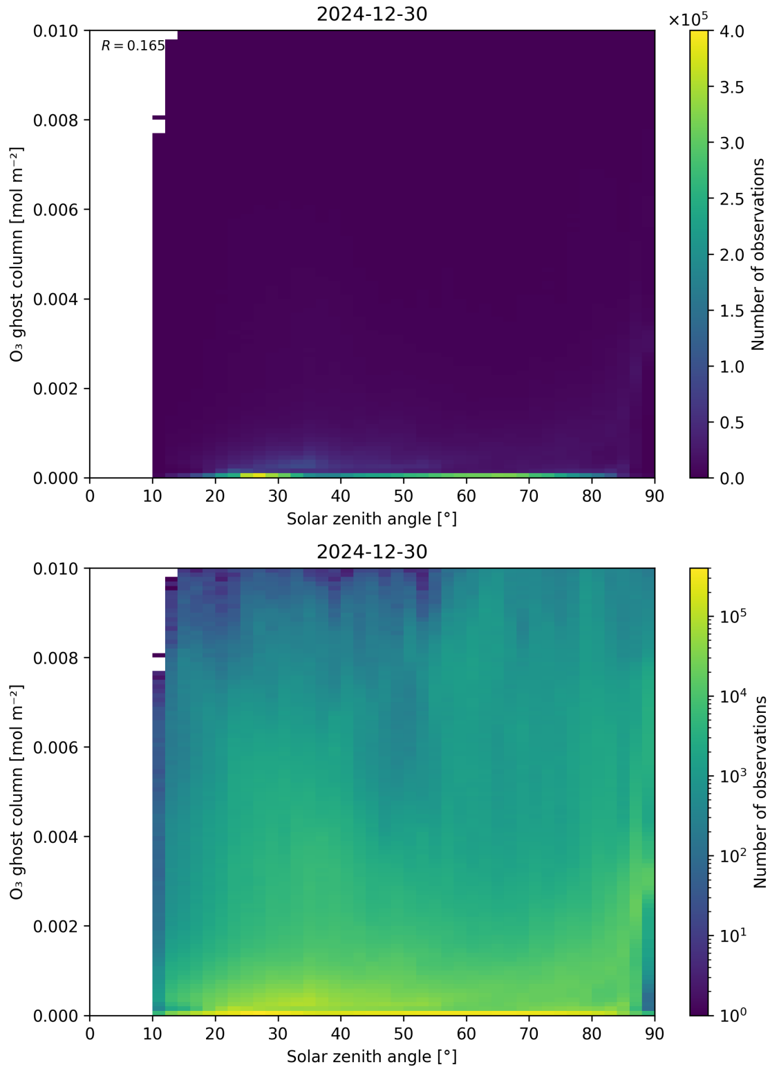
Figure 46: Scatter density plot of “Solar zenith angle” against “O 3 ghost column” for 2024-12-29 to 2024-12-31.
