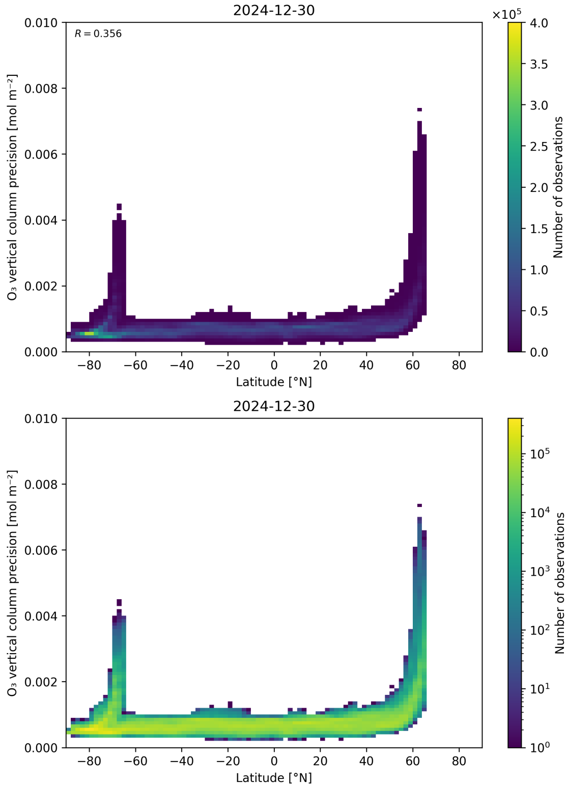
Figure 37: Scatter density plot of “Latitude” against “O 3 vertical column precision” for 2024-12-29 to 2024-12-31.
