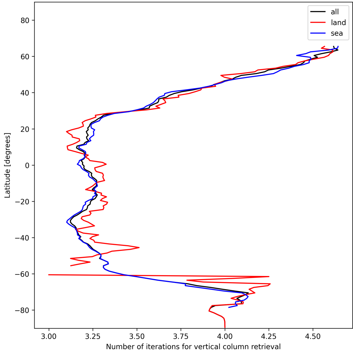
Figure 19: Zonal average of “Number of iterations for vertical column retrieval” for 2024-12-29 to 2024-12-31.
