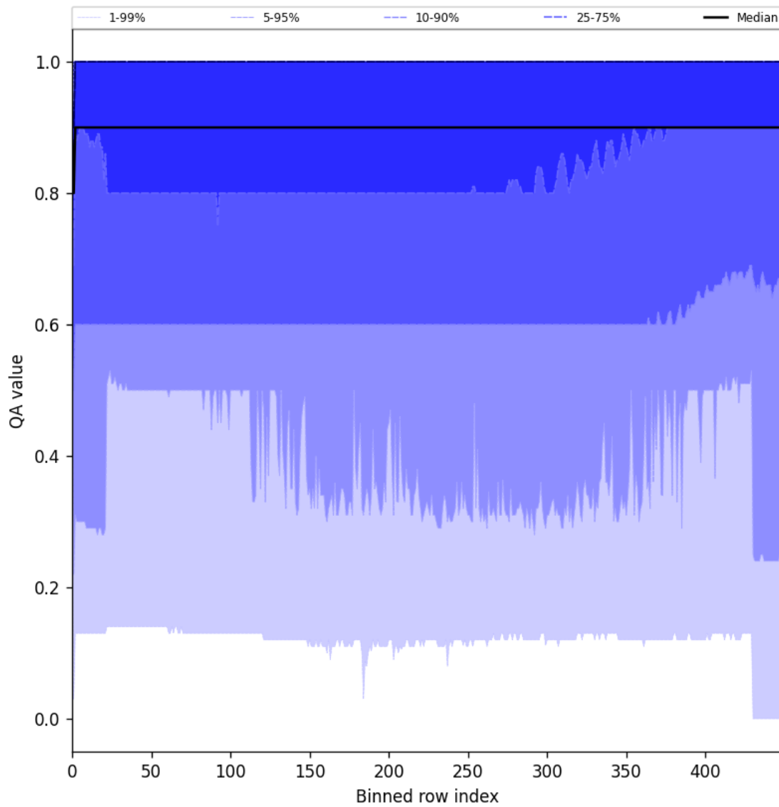
Figure 27: Along track statistics of “QA value” for 2024-12-29 to 2024-12-31
