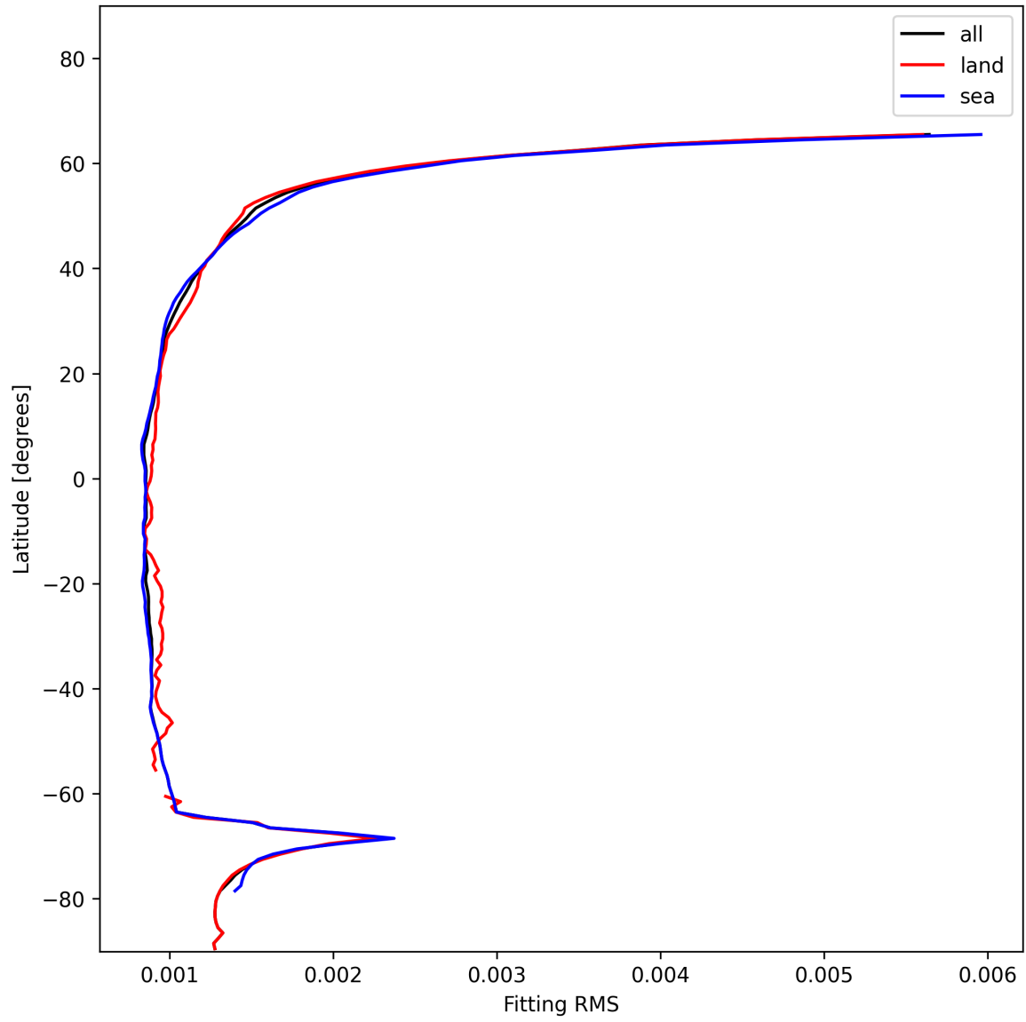
Figure 16: Zonal average of “Fitting RMS” for 2024-12-29 to 2024-12-31.
