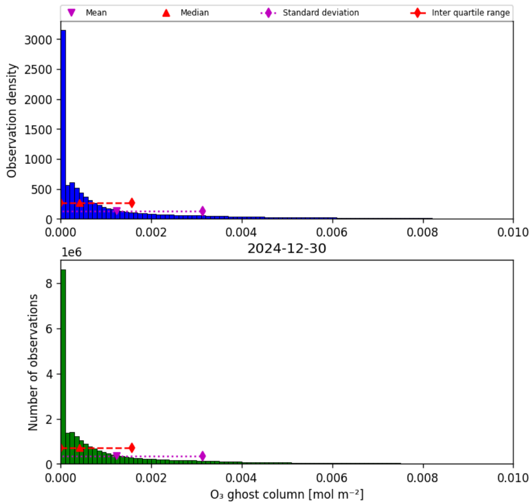
Figure 25: Histogram of “O 3 ghost column” for 2024-12-29 to 2024-12-31
