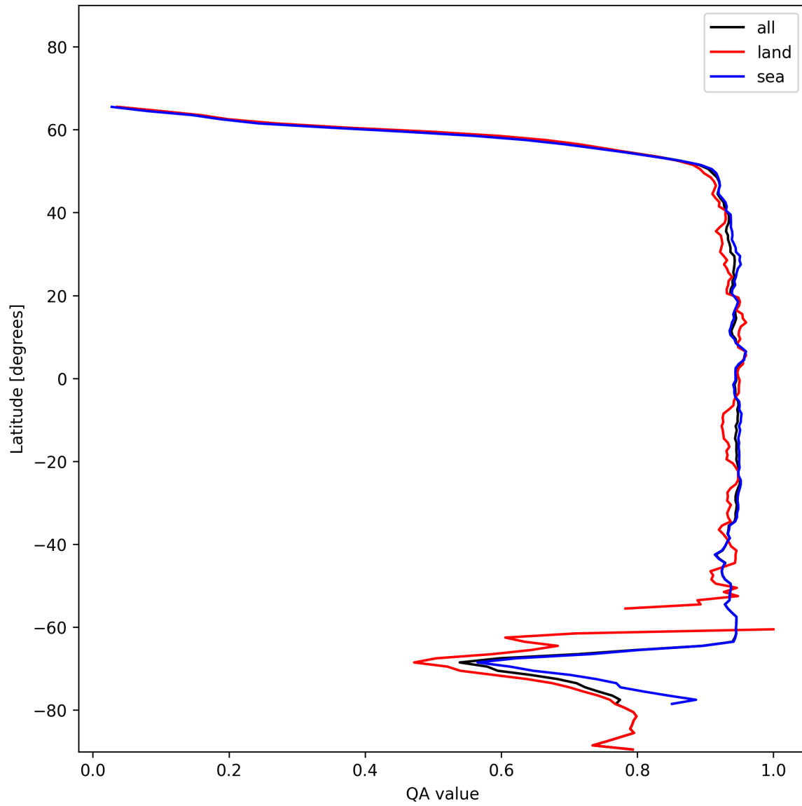
Figure 13: Zonal average of “QA value” for 2024-12-29 to 2024-12-31.
