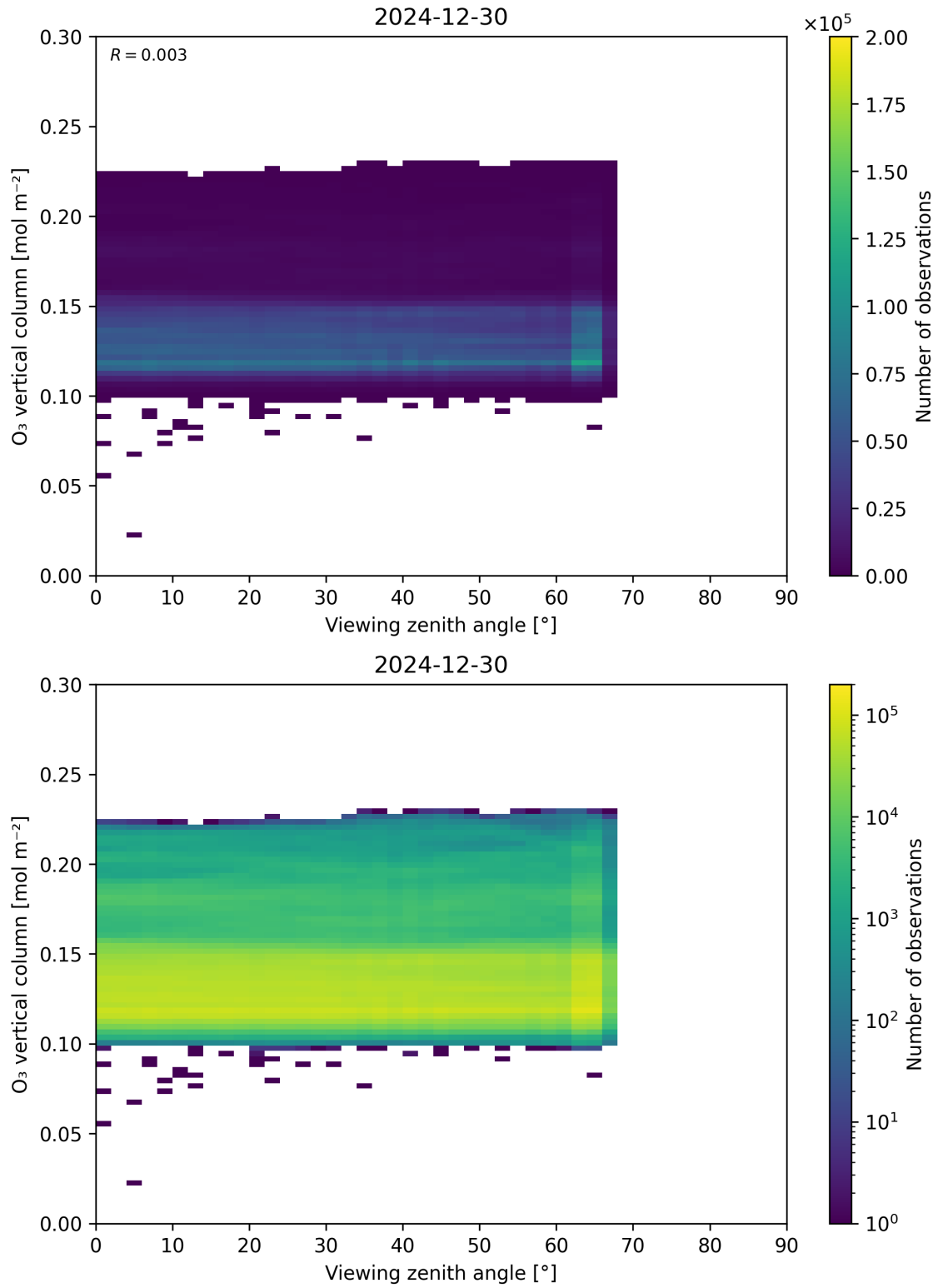
Figure 52: Scatter density plot of “Viewing zenith angle” against “O 3 vertical column” for 2024-12-29 to 2024-12-31.
