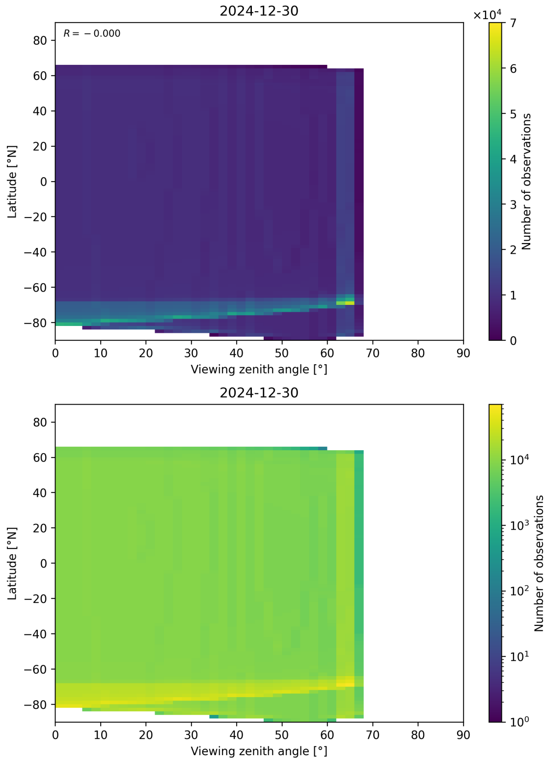
Figure 49: Scatter density plot of “Viewing zenith angle” against “Latitude” for 2024-12-29 to 2024-12-31.
