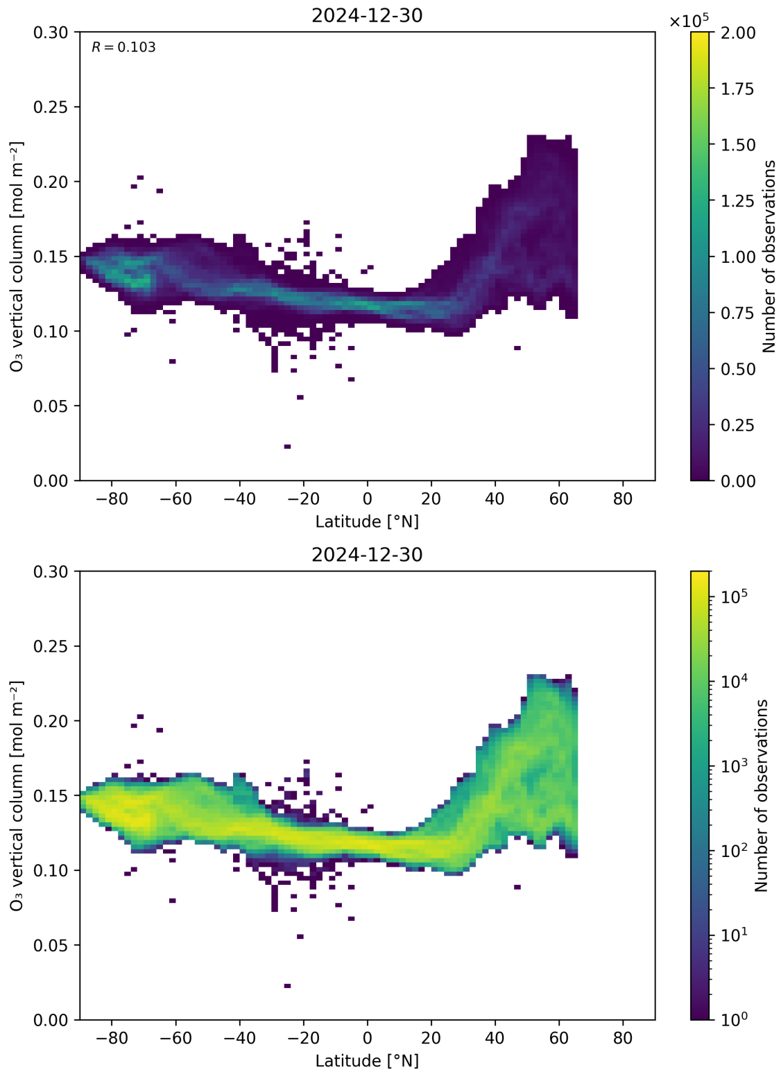
Figure 36: Scatter density plot of “Latitude” against “O 3 vertical column” for 2024-12-29 to 2024-12-31.
