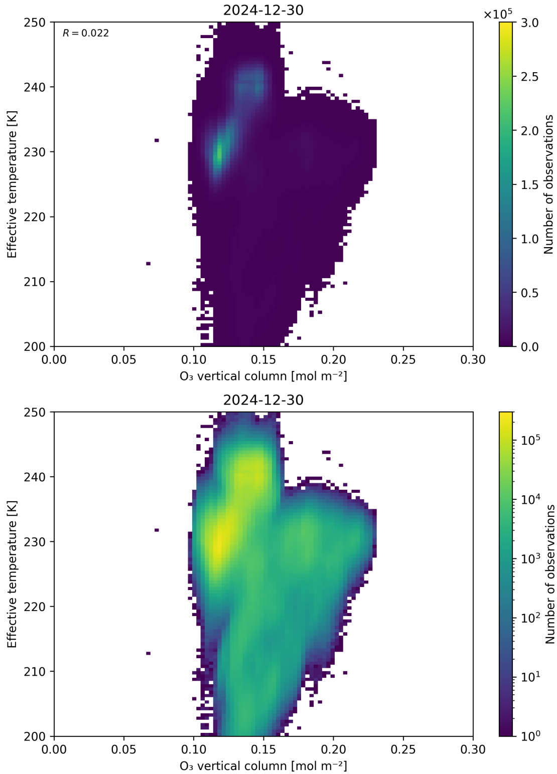
Figure 39: Scatter density plot of “O 3 vertical column” against “Effective temperature” for 2024-12-29 to 2024-12-31.
