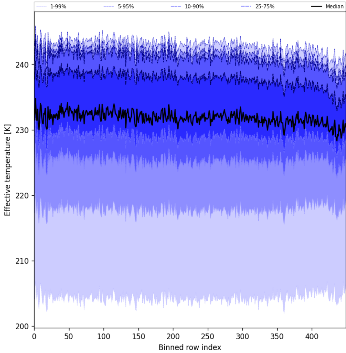
Figure 31: Along track statistics of “Effective temperature” for 2024-12-29 to 2024-12-31
