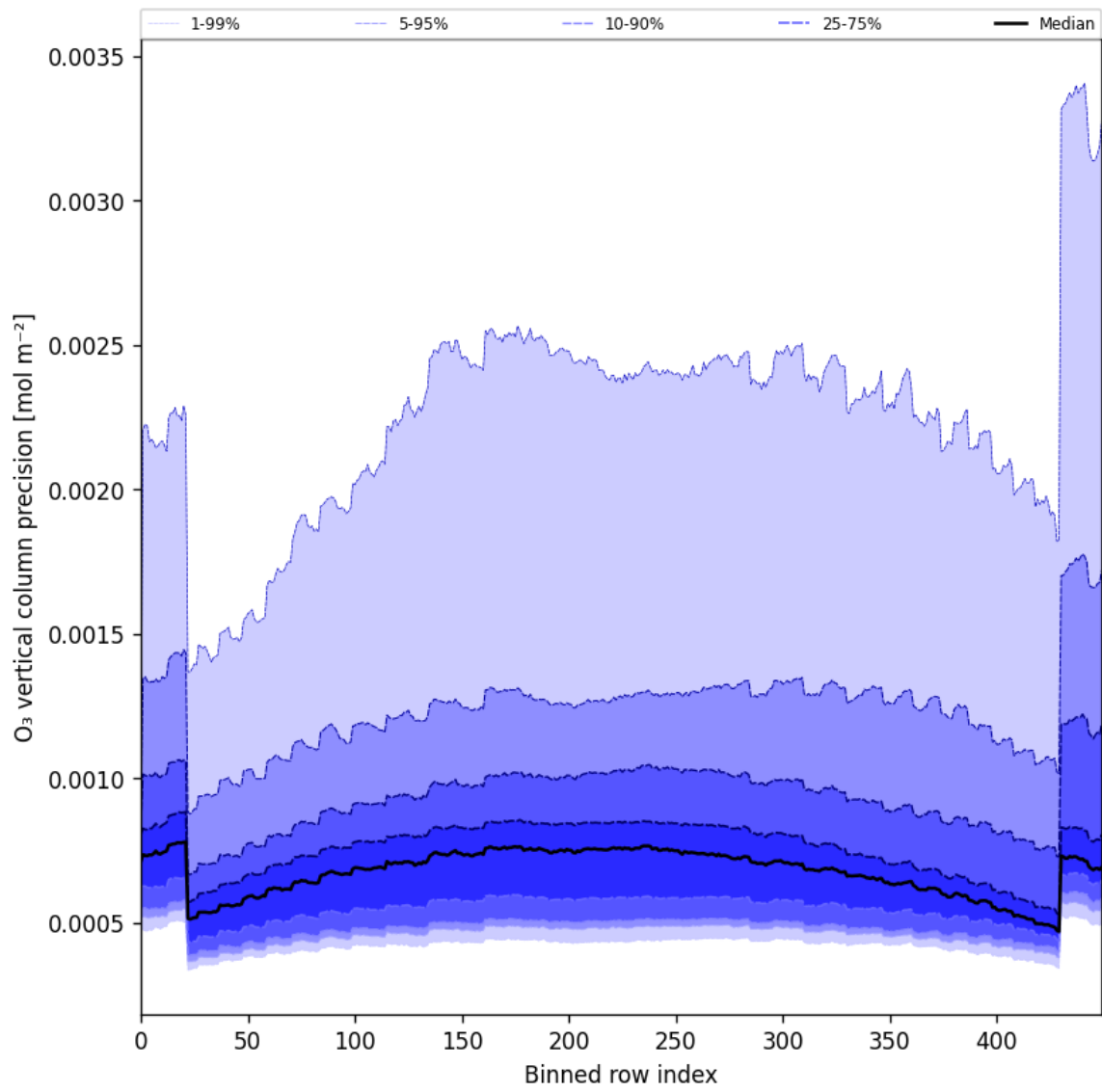
Figure 29: Along track statistics of “O 3 vertical column precision” for 2024-12-29 to 2024-12-31
