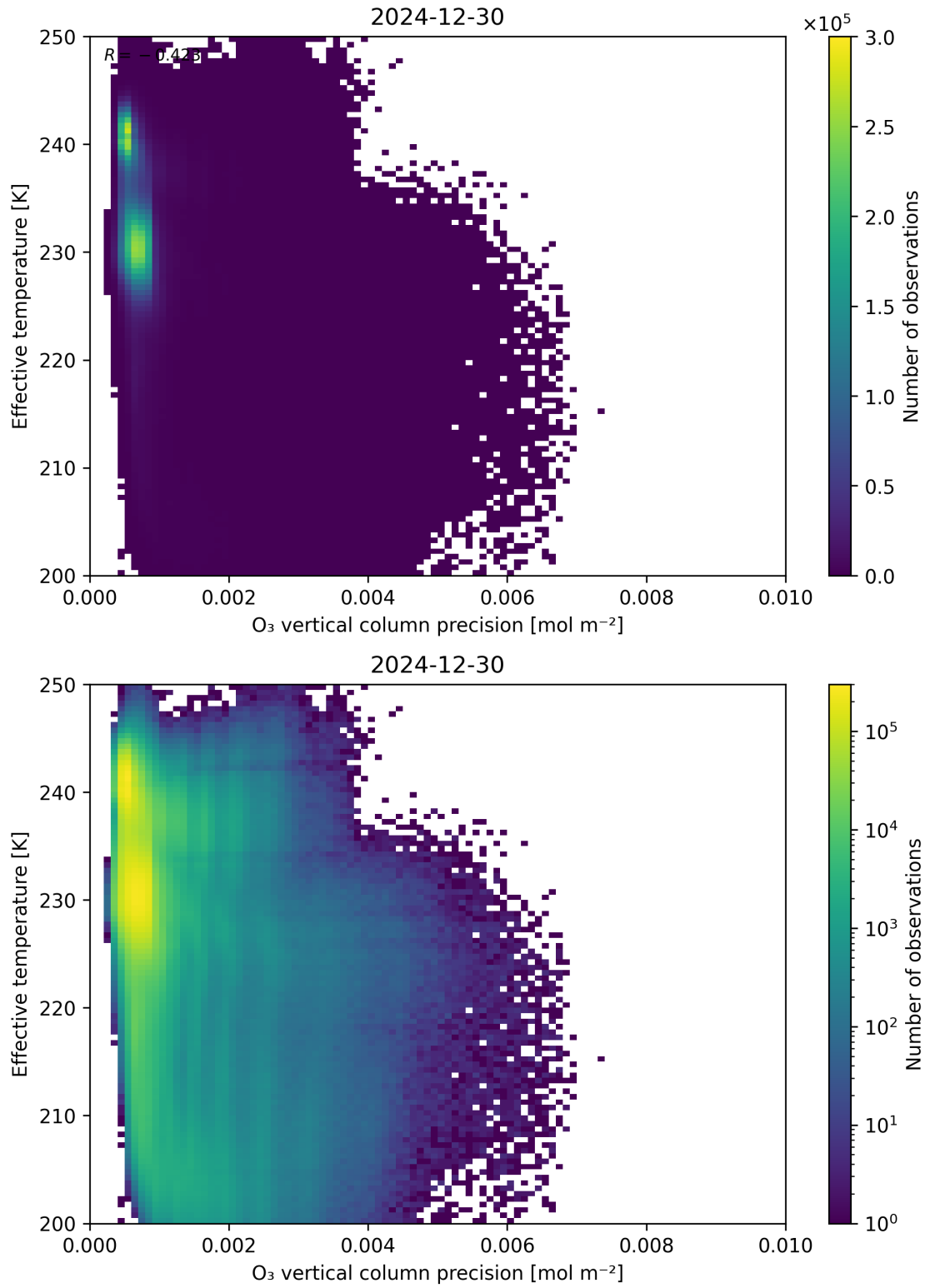
Figure 42: Scatter density plot of “O 3 vertical column precision” against “Effective temperature” for 2024-12-29 to 2024-12-31.
