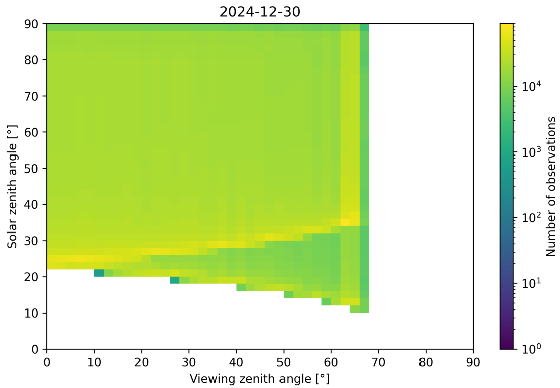
Figure 54: Scatter density plot of “Viewing zenith angle” against “Solar zenith angle” for 2024-12-29 to 2024-12-31.
