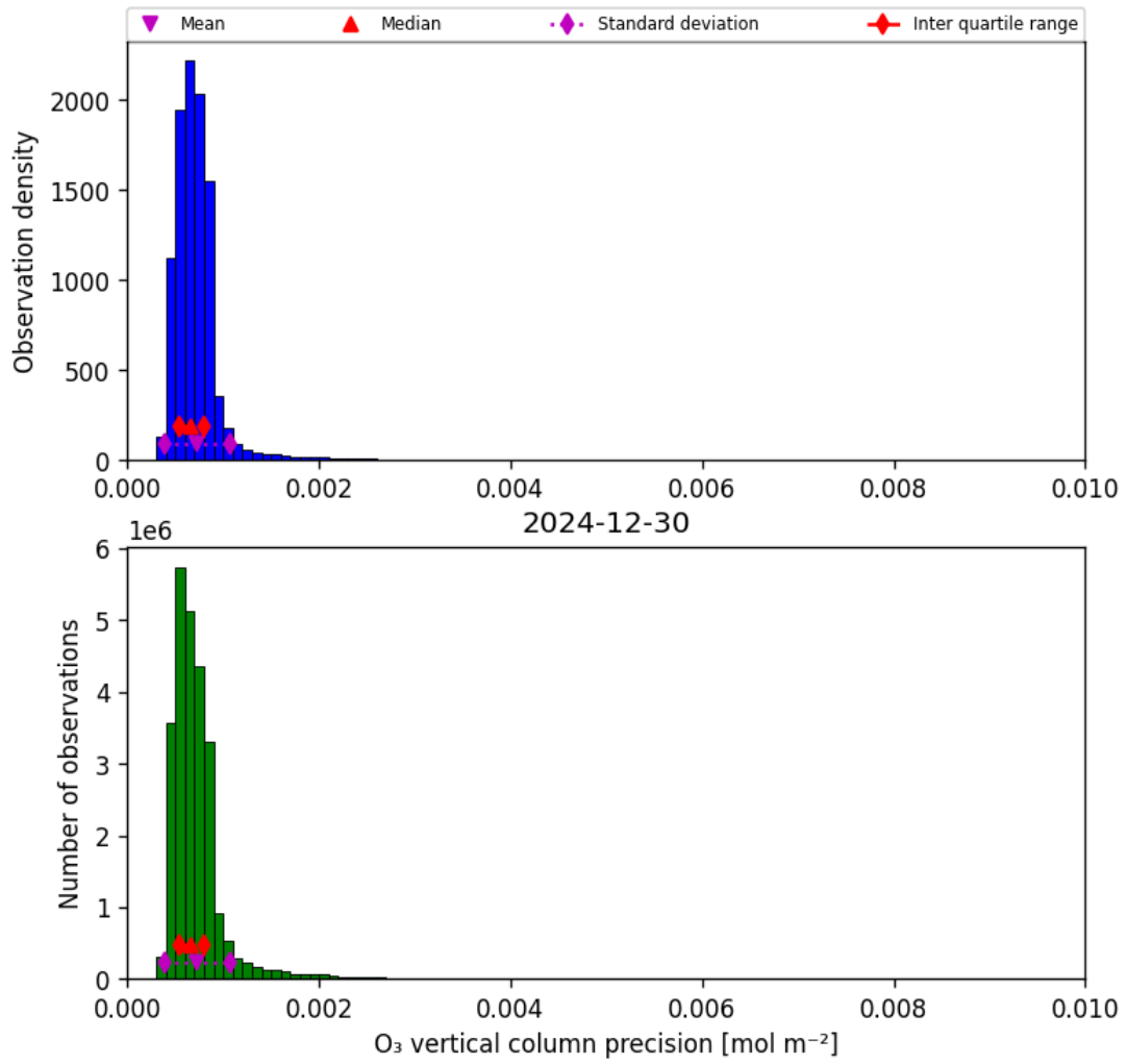
Figure 22: Histogram of “O 3 vertical column precision” for 2024-12-29 to 2024-12-31
