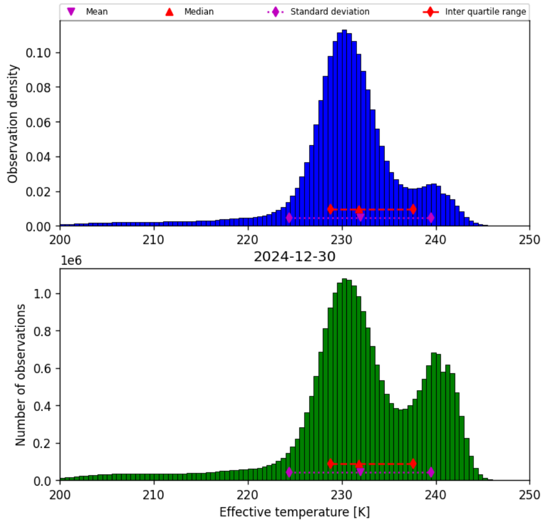
Figure 24: Histogram of “Effective temperature” for 2024-12-29 to 2024-12-31
