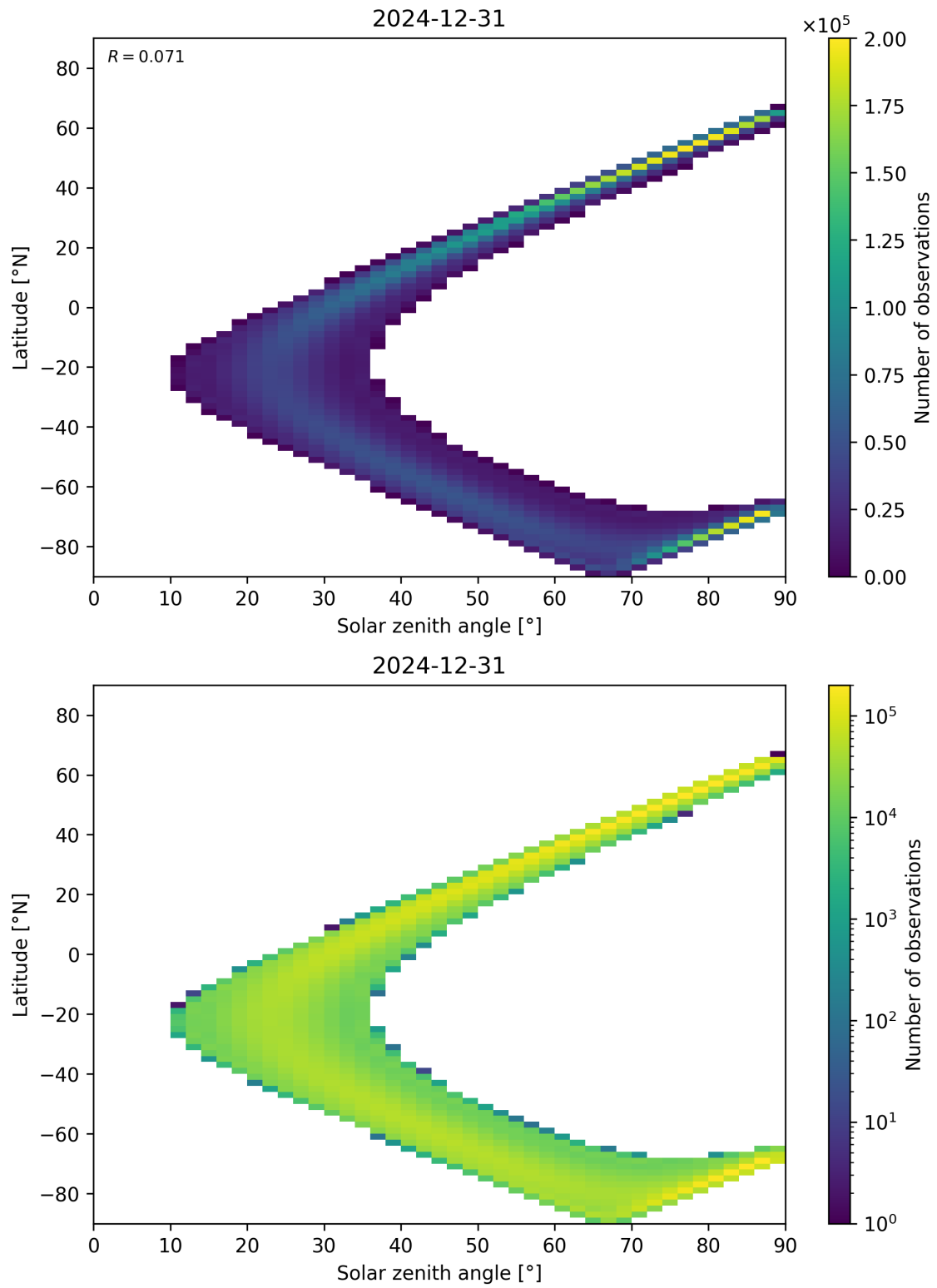
Figure 44: Scatter density plot of “Solar zenith angle” against “Latitude” for 2024-12-30 to 2025-01-01.
