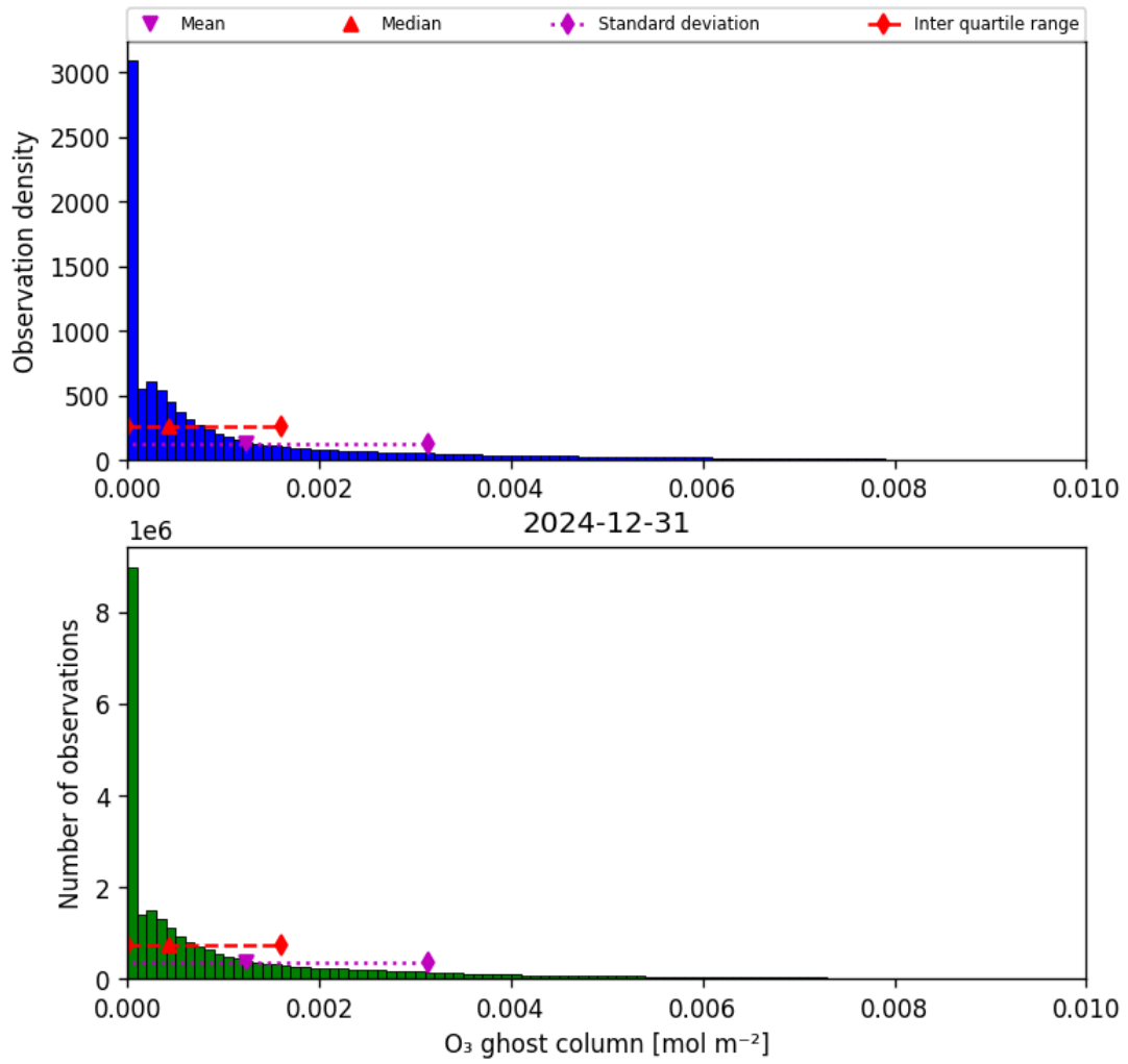
Figure 25: Histogram of “O 3 ghost column” for 2024-12-30 to 2025-01-01
