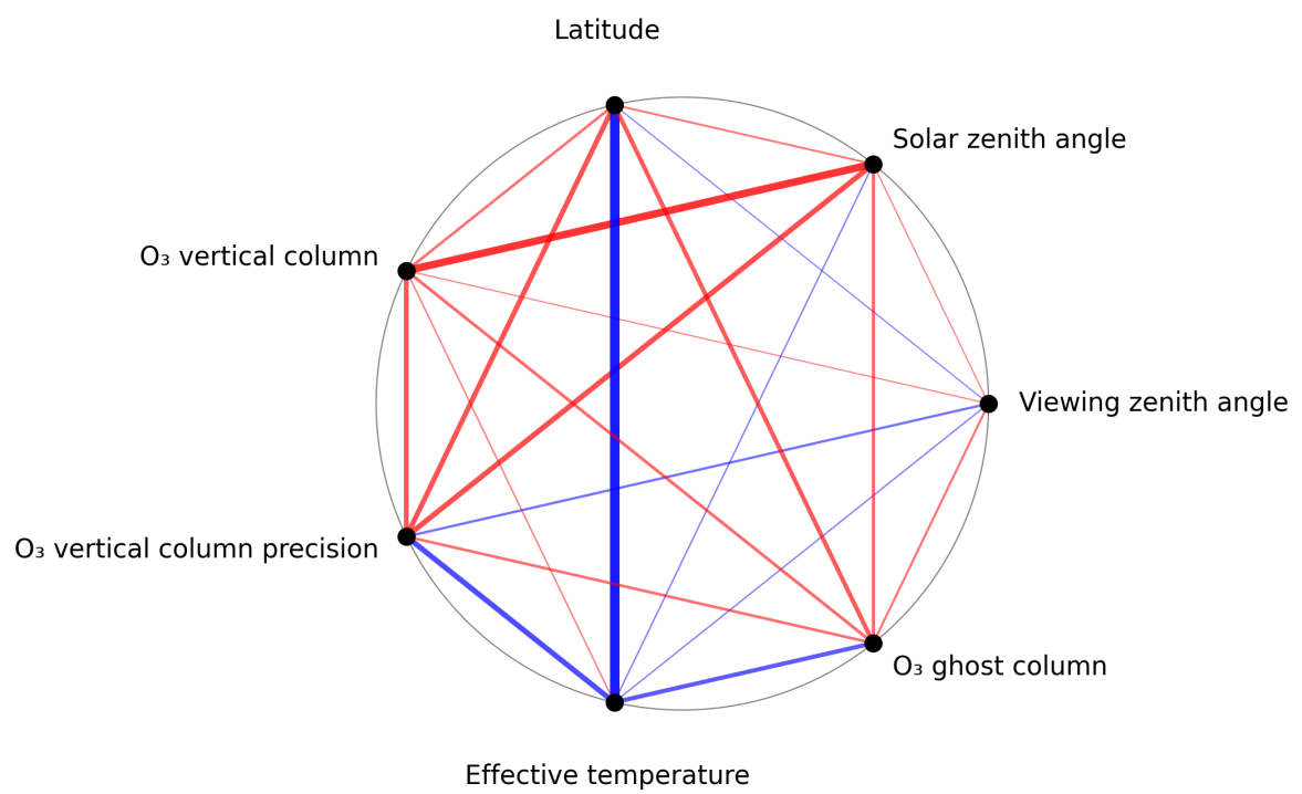
Figure 1: Map of correlation graph for 2024-12-30 to 2025-01-01.
