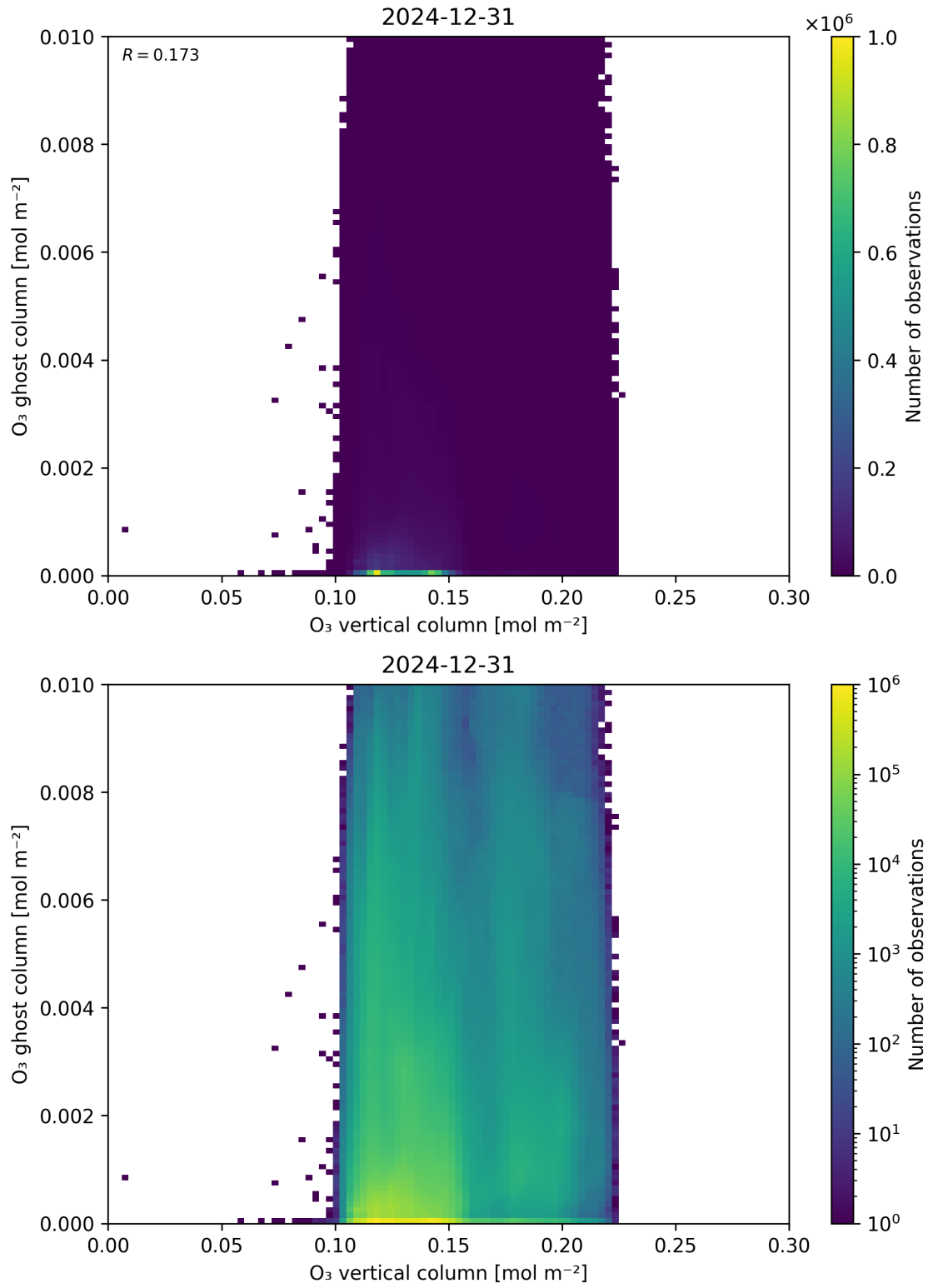
Figure 40: Scatter density plot of “O 3 vertical column” against “O 3 ghost column” for 2024-12-30 to 2025-01-01.
