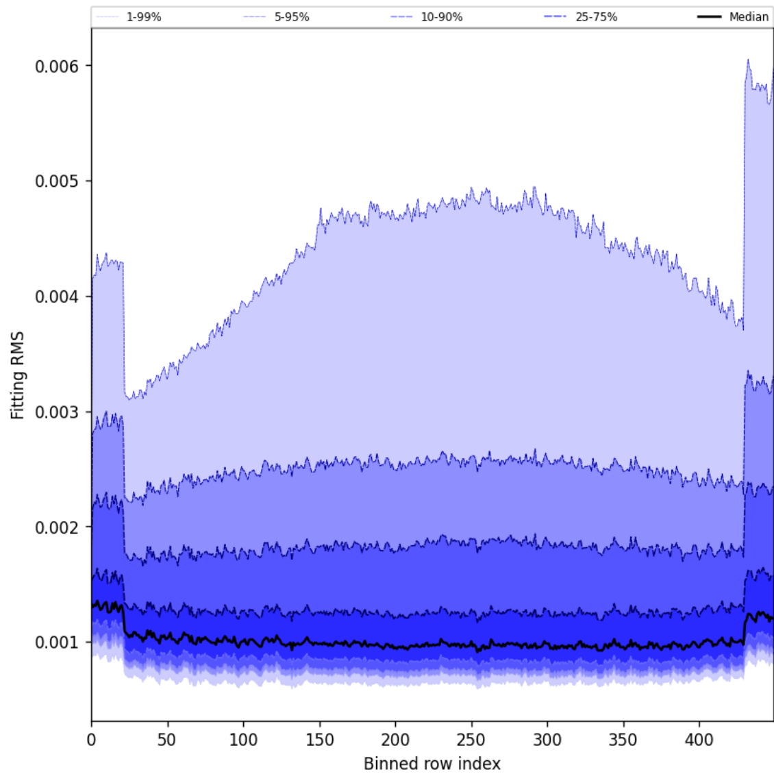
Figure 30: Along track statistics of “Fitting RMS” for 2024-12-30 to 2025-01-01
