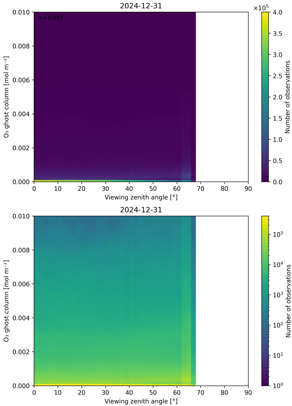
Figure 51: Scatter density plot of “Viewing zenith angle” against “O 3 ghost column” for 2024-12-30 to 2025-01-01.
