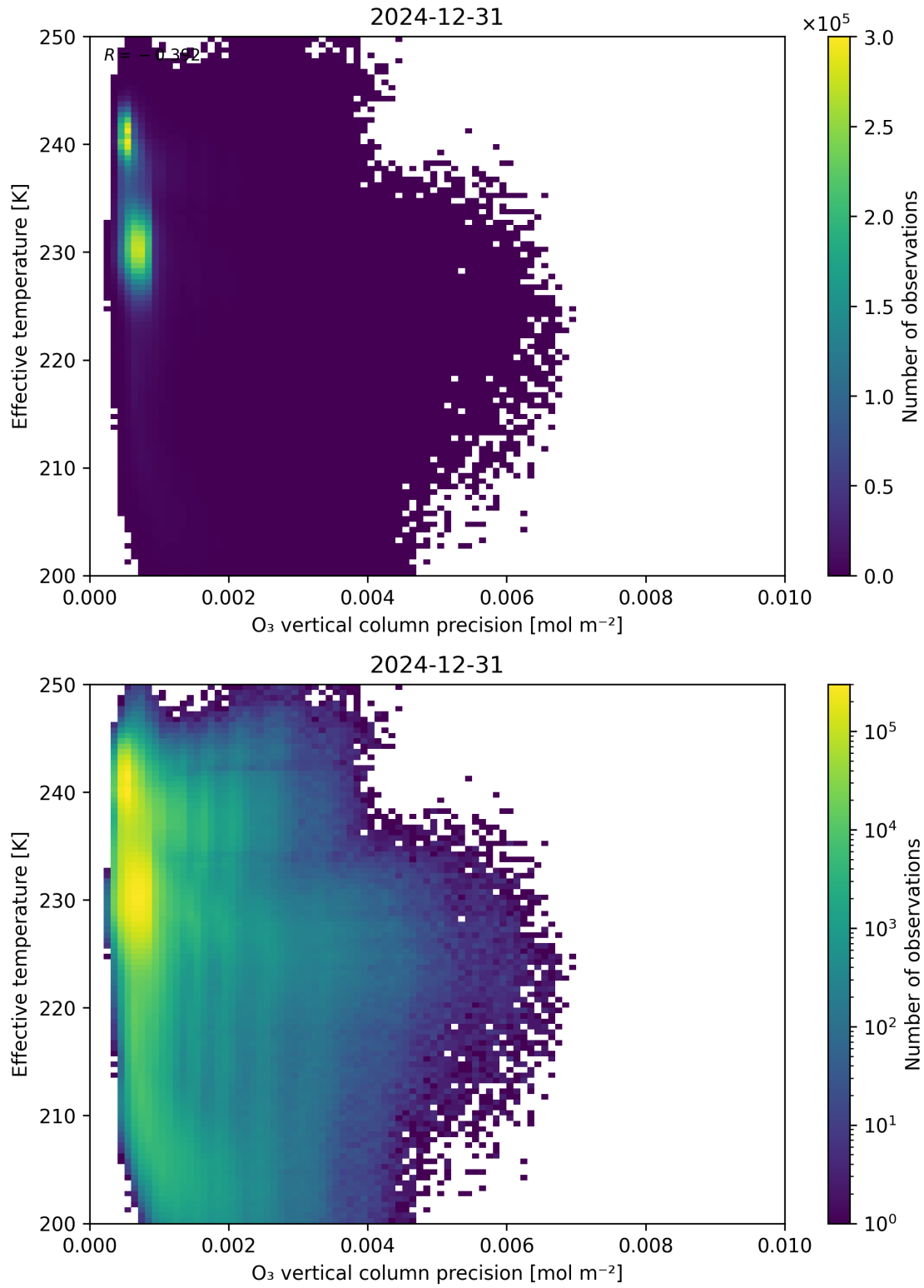
Figure 42: Scatter density plot of “O 3 vertical column precision” against “Effective temperature” for 2024-12-30 to 2025-01-01.
