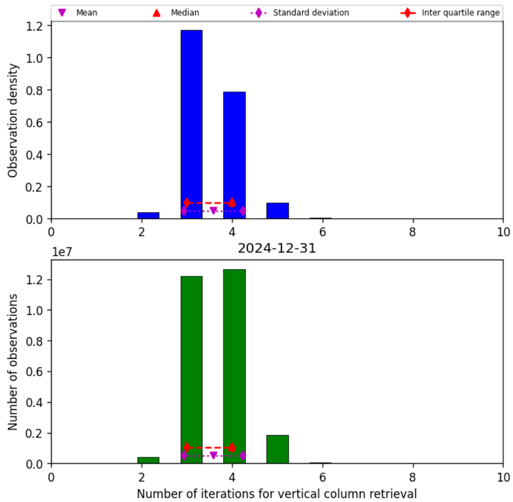
Figure 26: Histogram of “Number of iterations for vertical column retrieval” for 2024-12-30 to 2025-01-01
