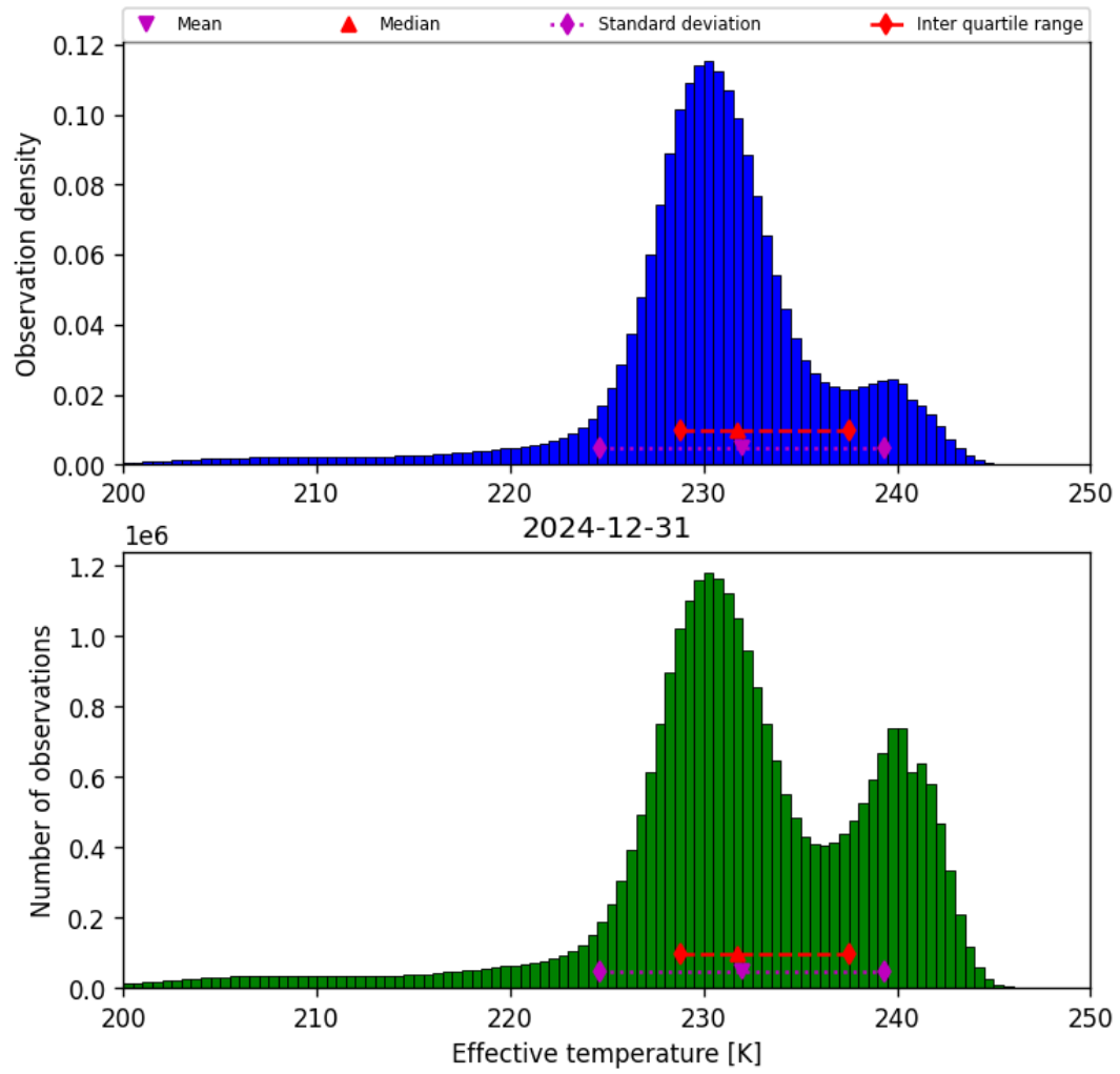
Figure 24: Histogram of “Effective temperature” for 2024-12-30 to 2025-01-01
