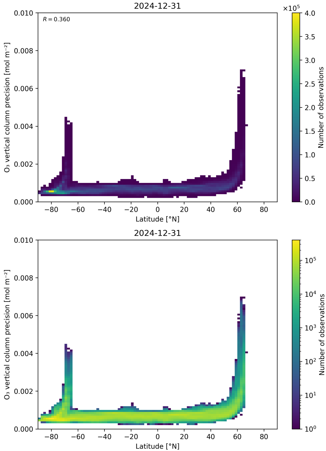
Figure 37: Scatter density plot of “Latitude” against “O 3 vertical column precision” for 2024-12-30 to 2025-01-01.
