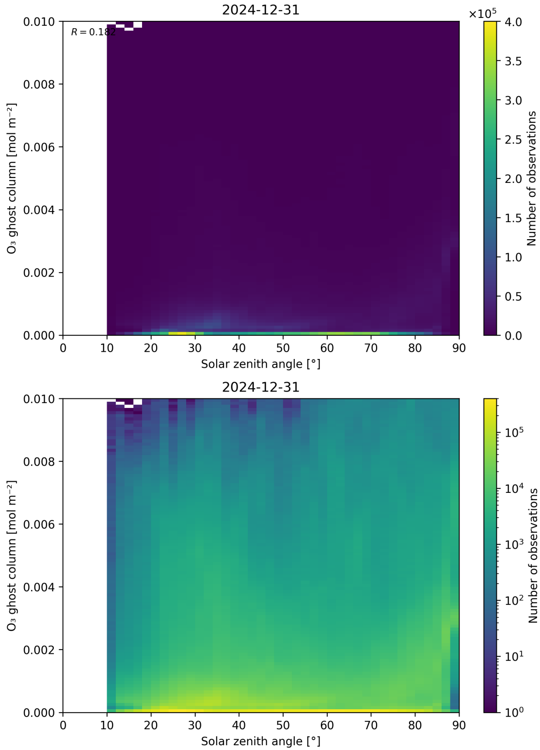
Figure 46: Scatter density plot of “Solar zenith angle” against “O 3 ghost column” for 2024-12-30 to 2025-01-01.
