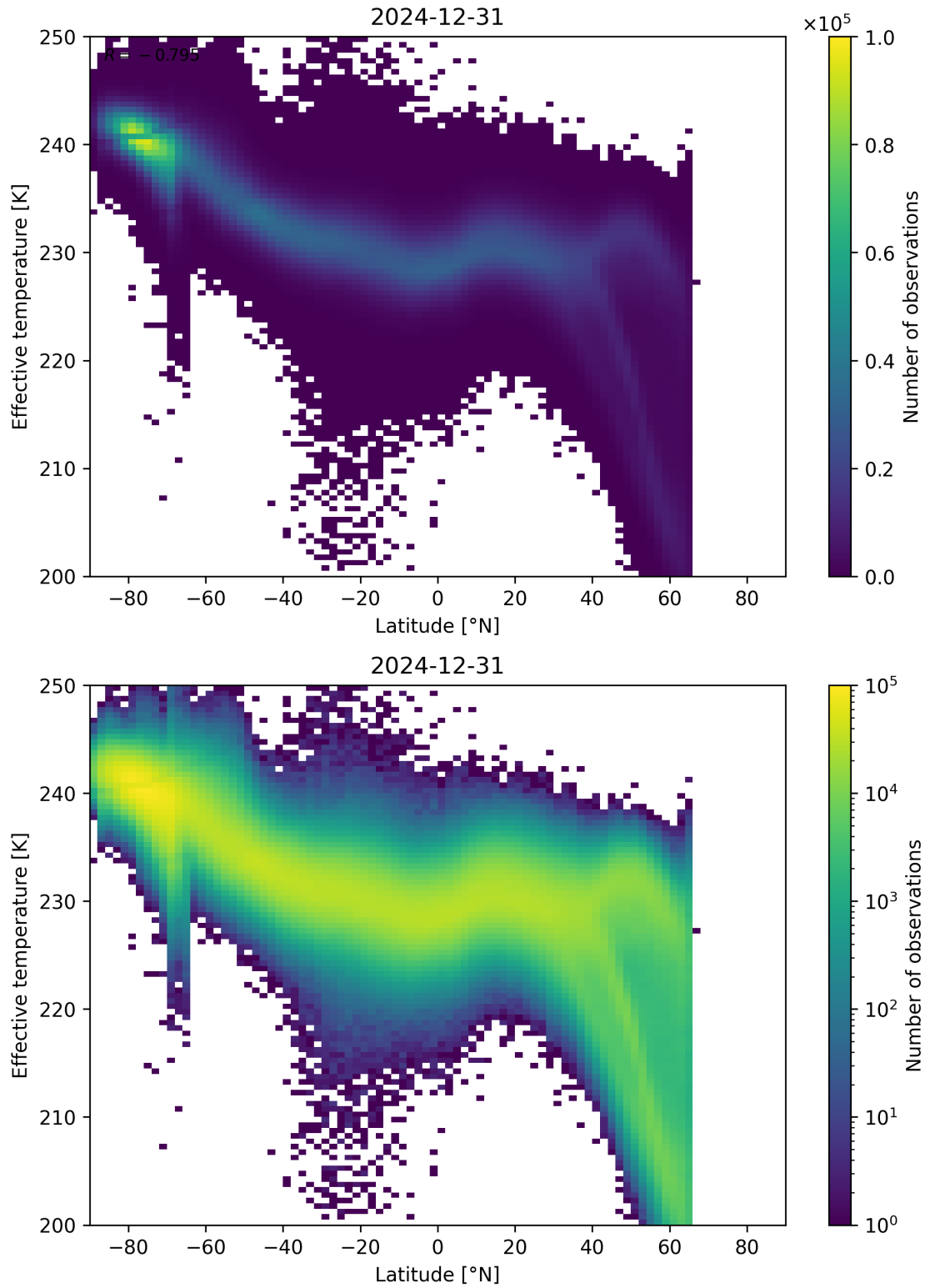
Figure 34: Scatter density plot of “Latitude” against “Effective temperature” for 2024-12-30 to 2025-01-01.
