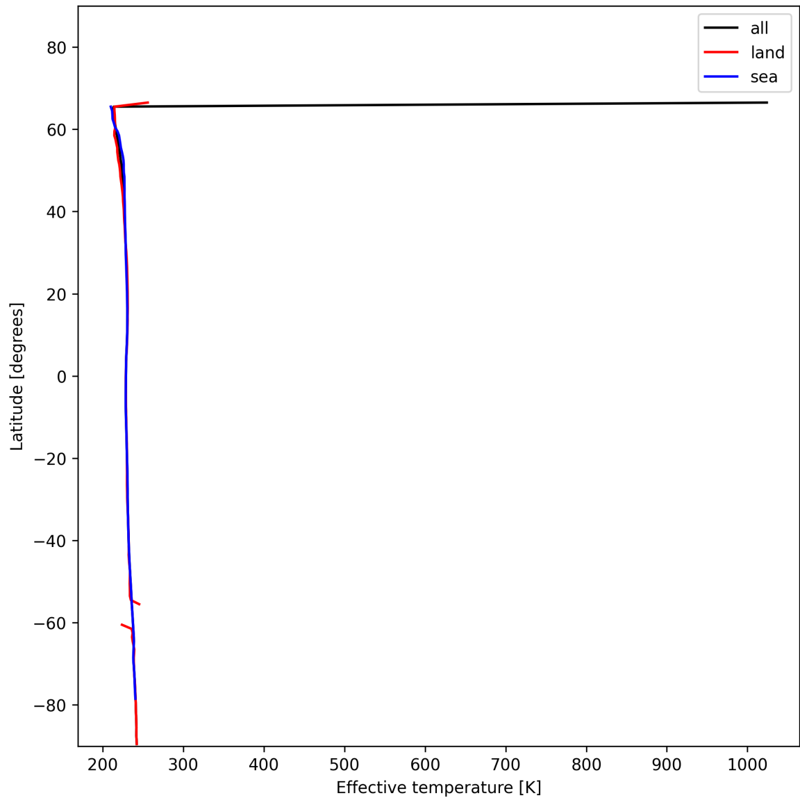
Figure 17: Zonal average of “Effective temperature” for 2024-12-30 to 2025-01-01.
