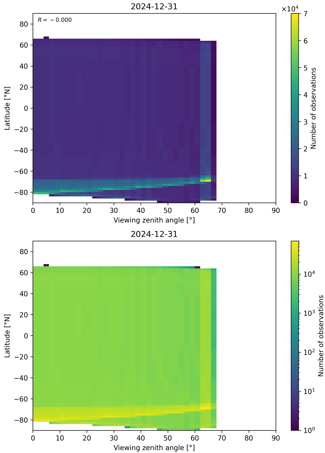
Figure 49: Scatter density plot of “Viewing zenith angle” against “Latitude” for 2024-12-30 to 2025-01-01.
