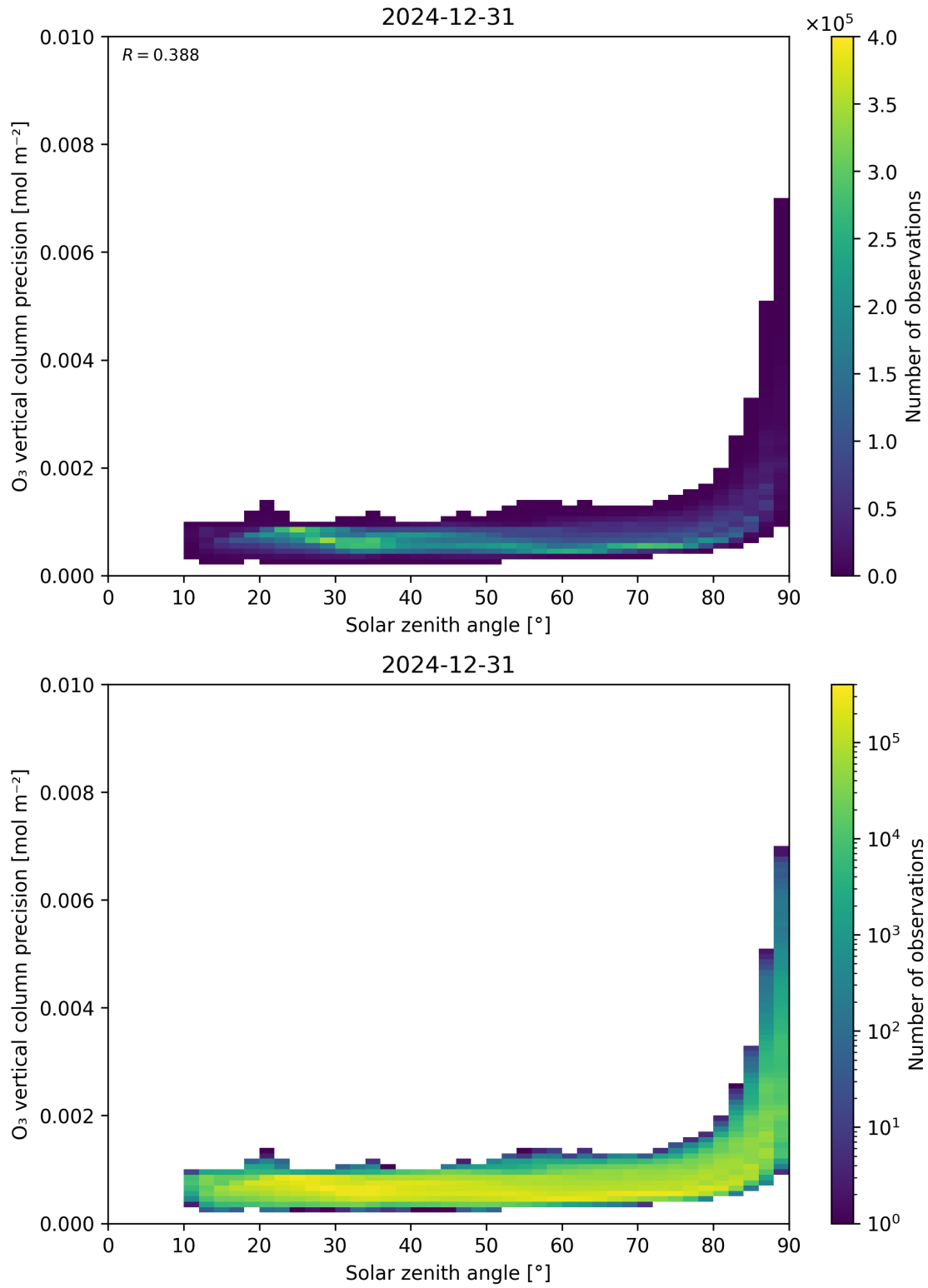
Figure 48: Scatter density plot of “Solar zenith angle” against “O 3 vertical column precision” for 2024-12-30 to 2025-01-01.
