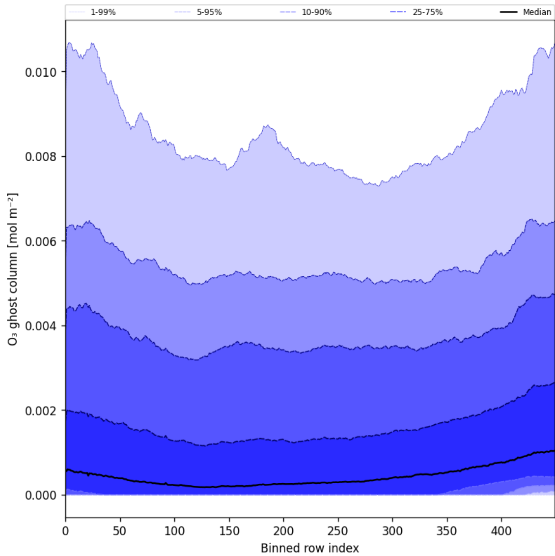
Figure 32: Along track statistics of “O 3 ghost column” for 2024-12-30 to 2025-01-01
