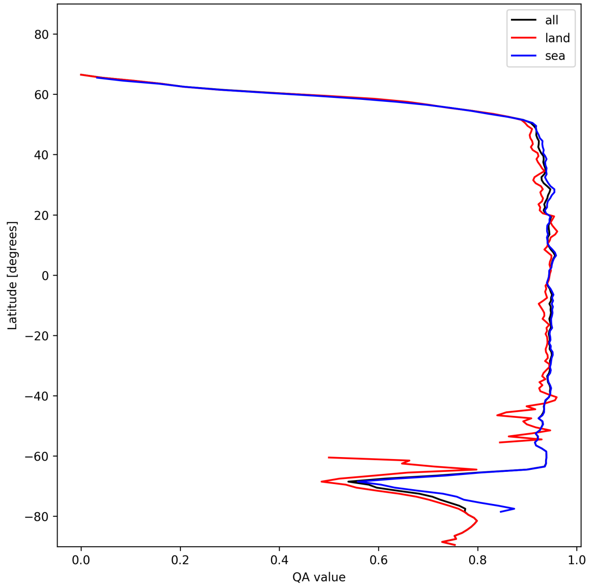
Figure 13: Zonal average of “QA value” for 2024-12-30 to 2025-01-01.
