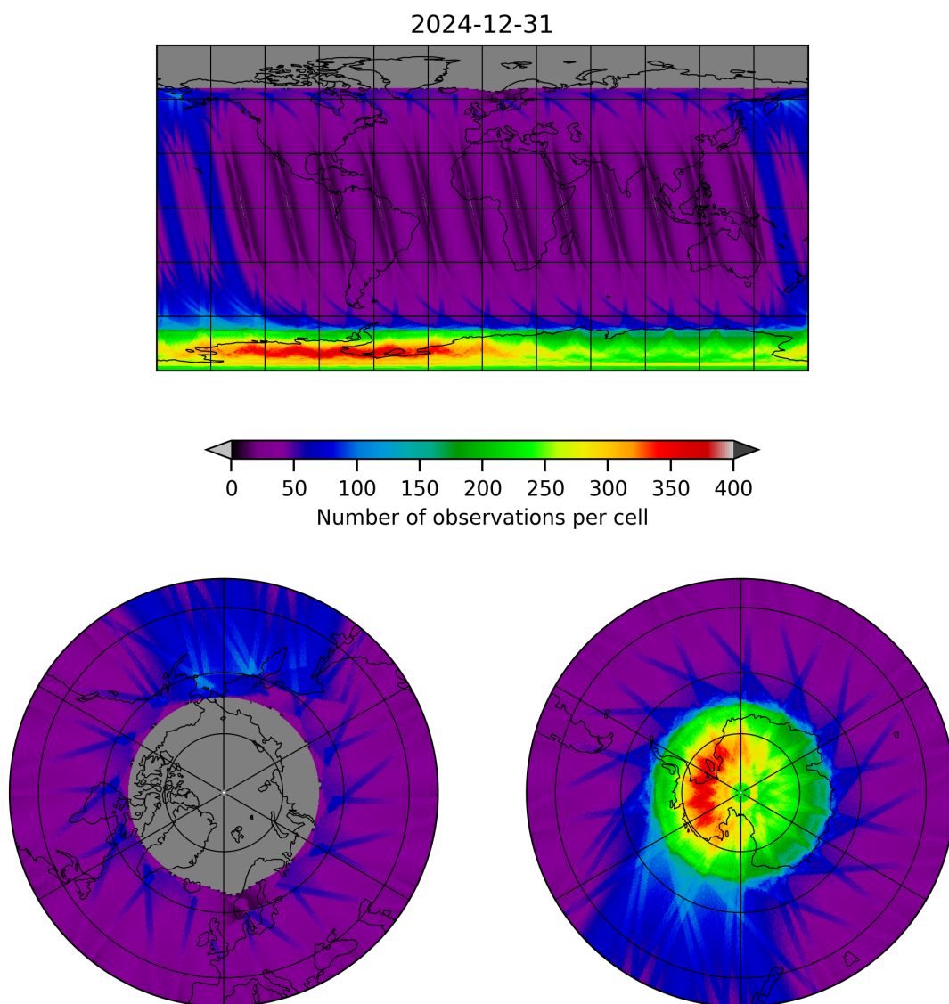
Figure 12: Map of the number of observations for 2024-12-30 to 2025-01-01
