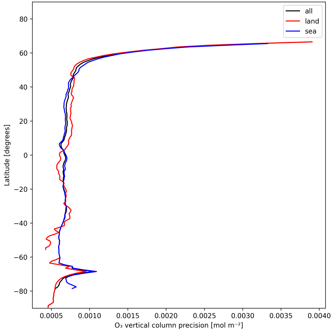
Figure 15: Zonal average of “O 3 vertical column precision” for 2024-12-30 to 2025-01-01.
