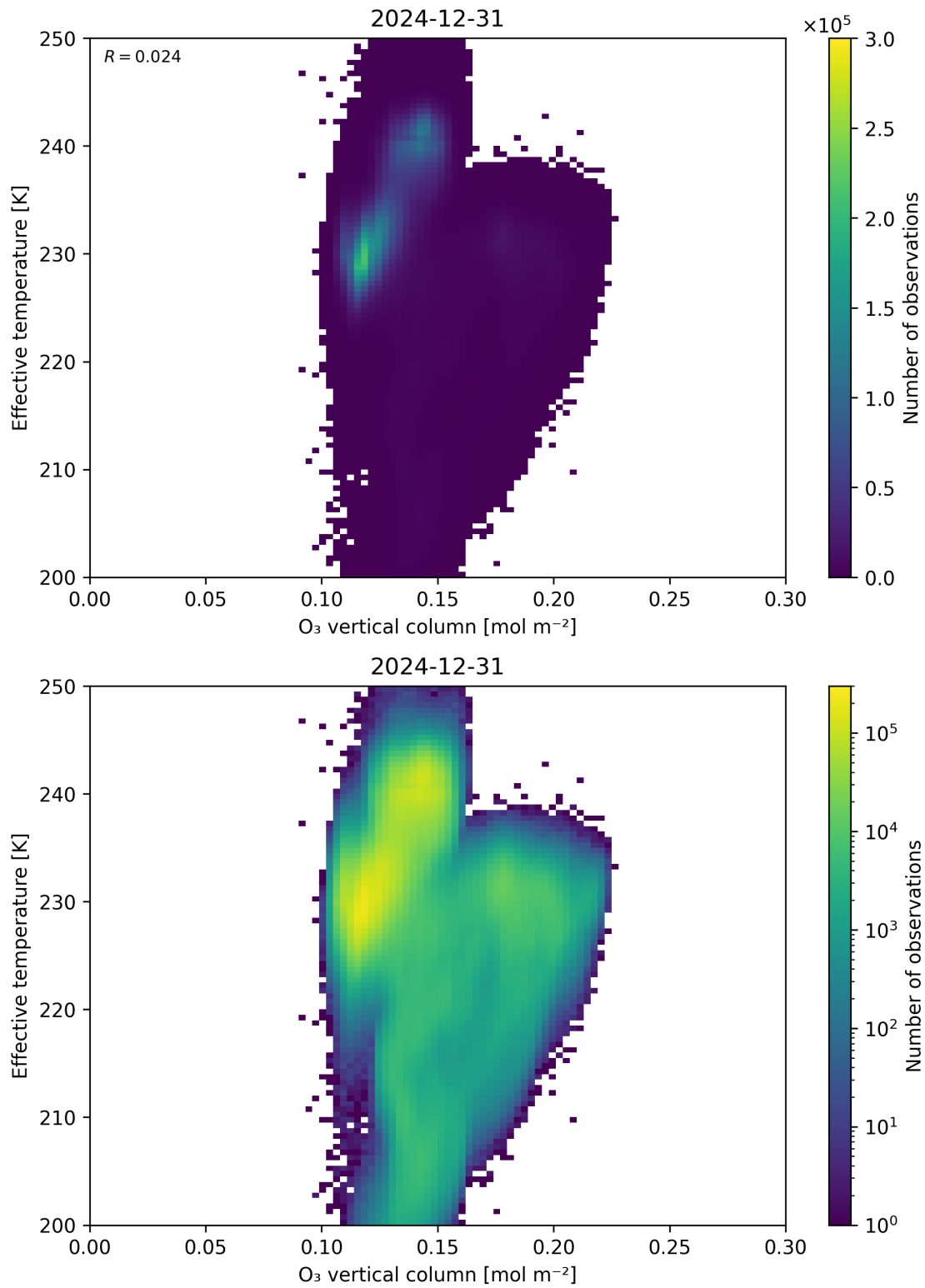
Figure 39: Scatter density plot of “O 3 vertical column” against “Effective temperature” for 2024-12-30 to 2025-01-01.
