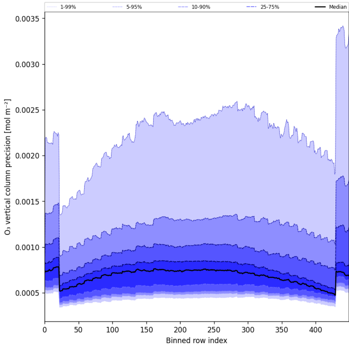
Figure 29: Along track statistics of “O 3 vertical column precision” for 2024-12-30 to 2025-01-01
