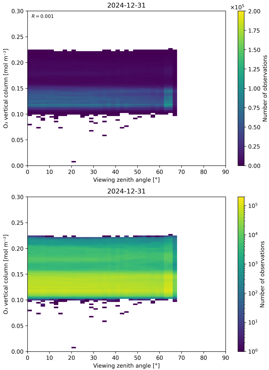
Figure 52: Scatter density plot of “Viewing zenith angle” against “O 3 vertical column” for 2024-12-30 to 2025-01-01.
