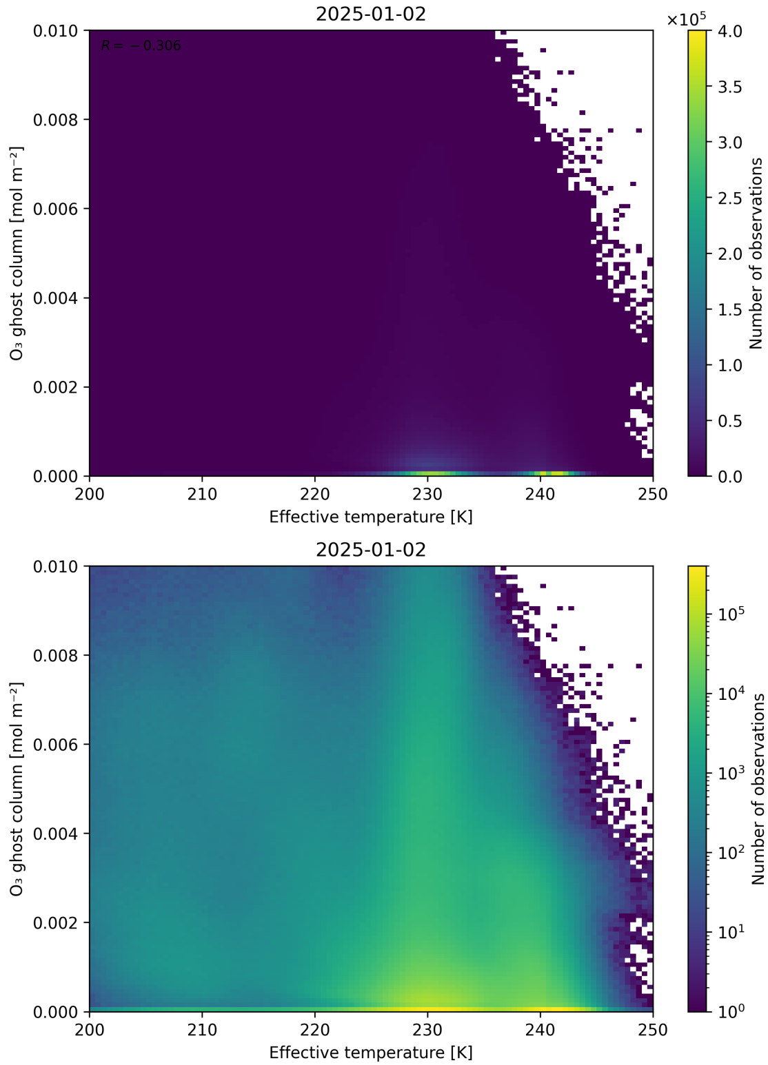
Figure 38: Scatter density plot of “Effective temperature” against “O 3 ghost column” for 2025-01-01 to 2025-01-03.
