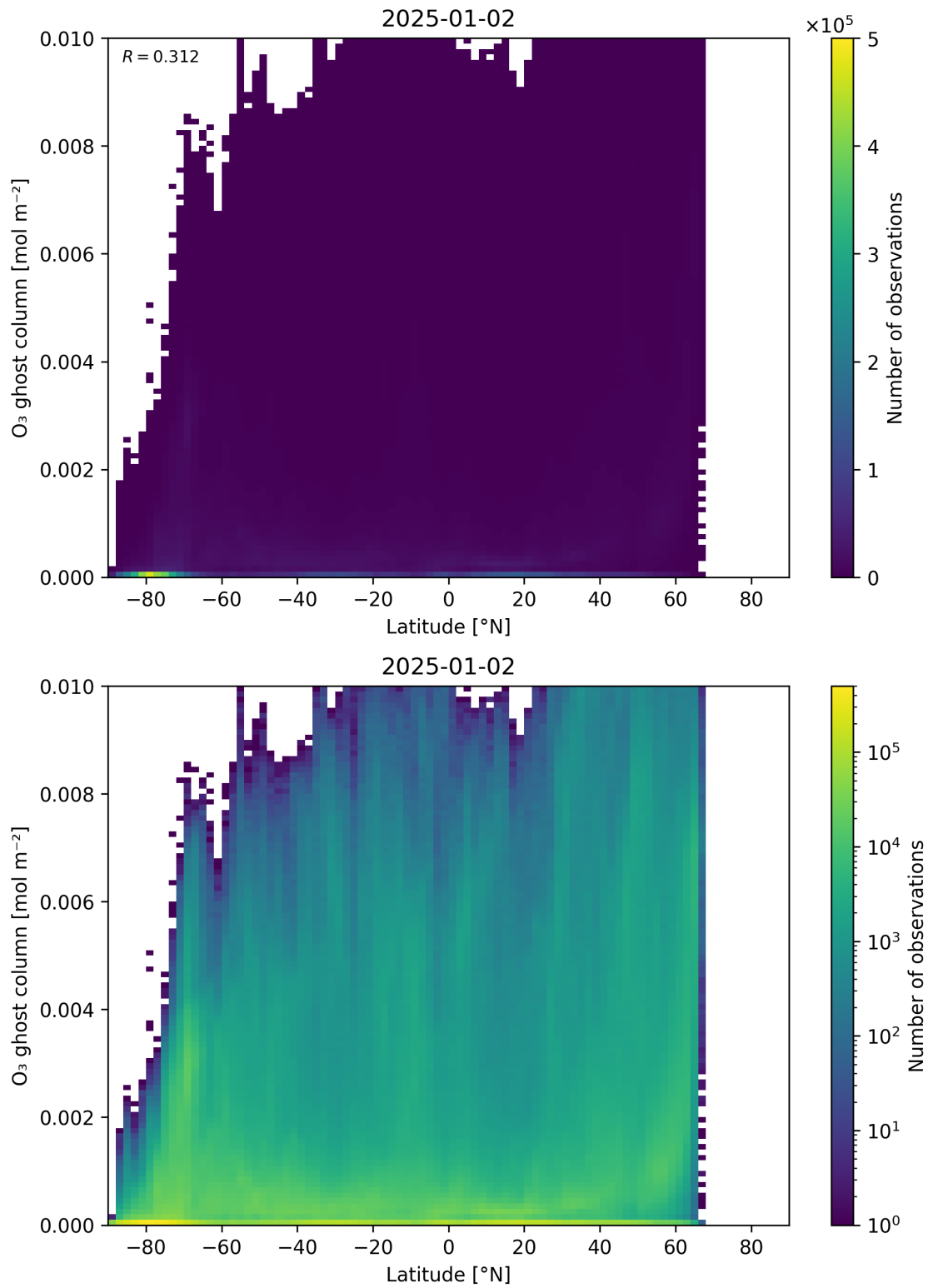
Figure 35: Scatter density plot of “Latitude” against “O 3 ghost column” for 2025-01-01 to 2025-01-03.
