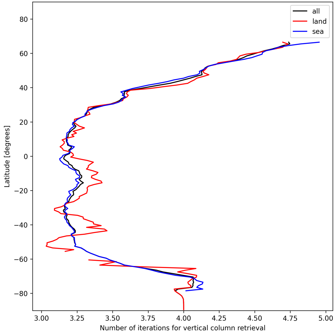
Figure 19: Zonal average of “Number of iterations for vertical column retrieval” for 2025-01-01 to 2025-01-03.
