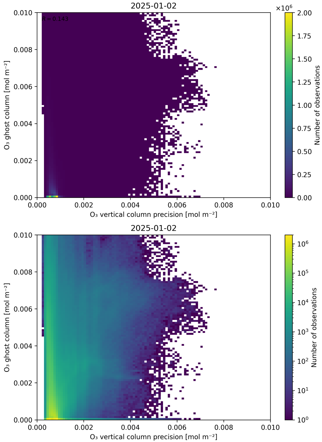
Figure 43: Scatter density plot of “ \text{O}_3 vertical column precision” against “ \text{O}_3 ghost column” for 2025-01-01 to 2025-01-03.
