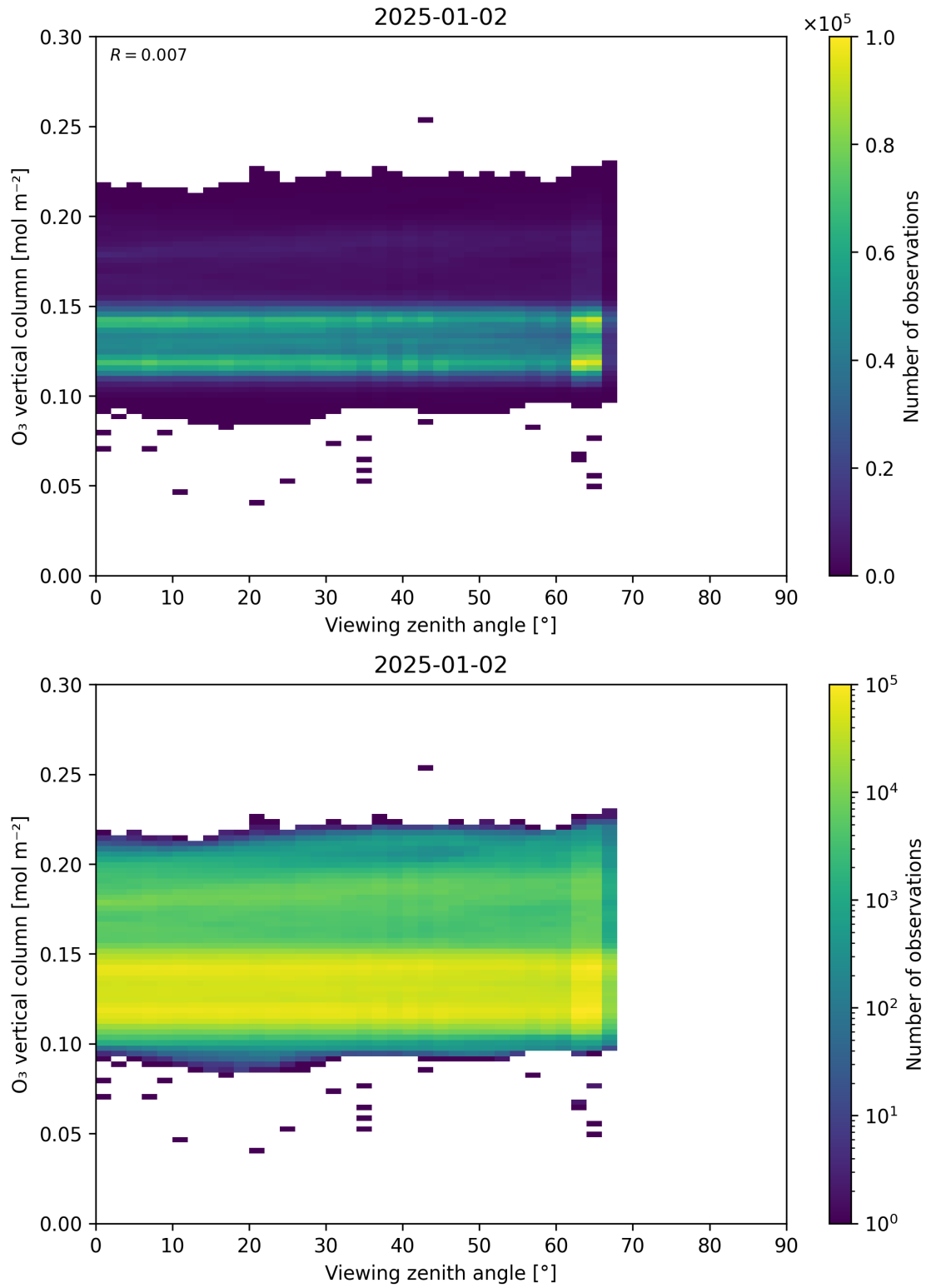
Figure 52: Scatter density plot of “Viewing zenith angle” against “O 3 vertical column” for 2025-01-01 to 2025-01-03.
