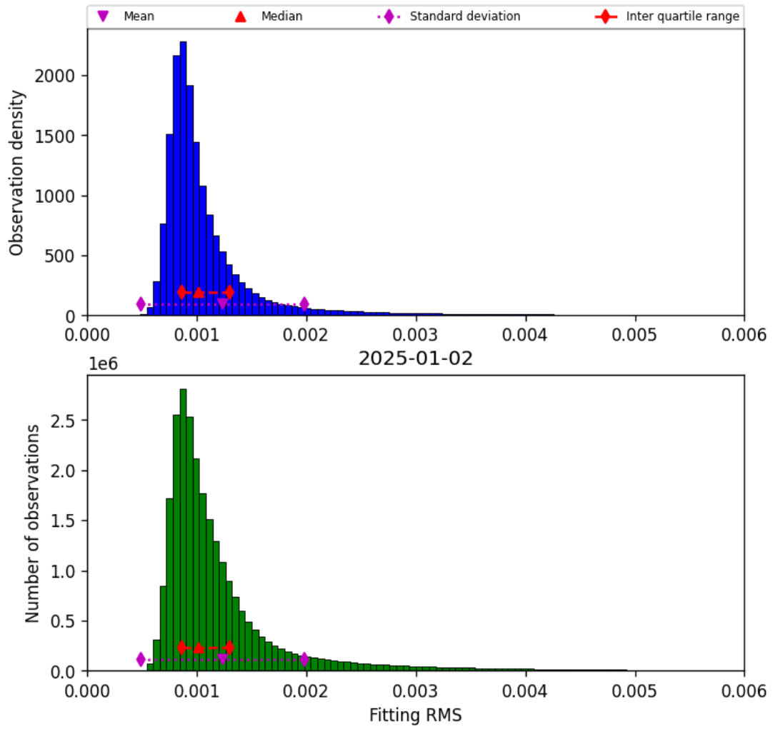
Figure 23: Histogram of “Fitting RMS” for 2025-01-01 to 2025-01-03
