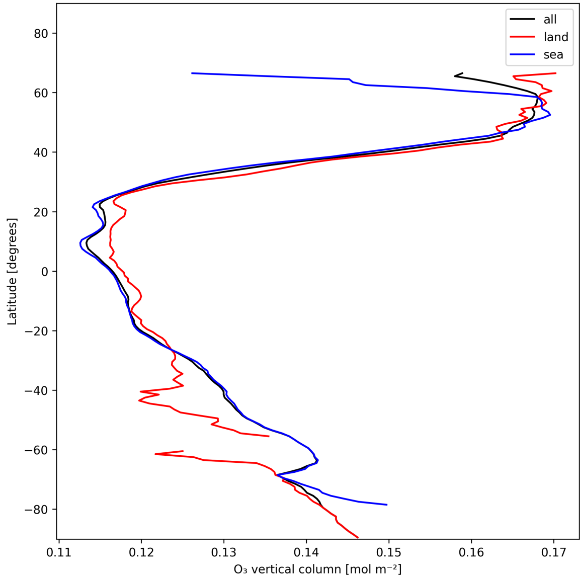
Figure 14: Zonal average of “O 3 vertical column” for 2025-01-01 to 2025-01-03.
