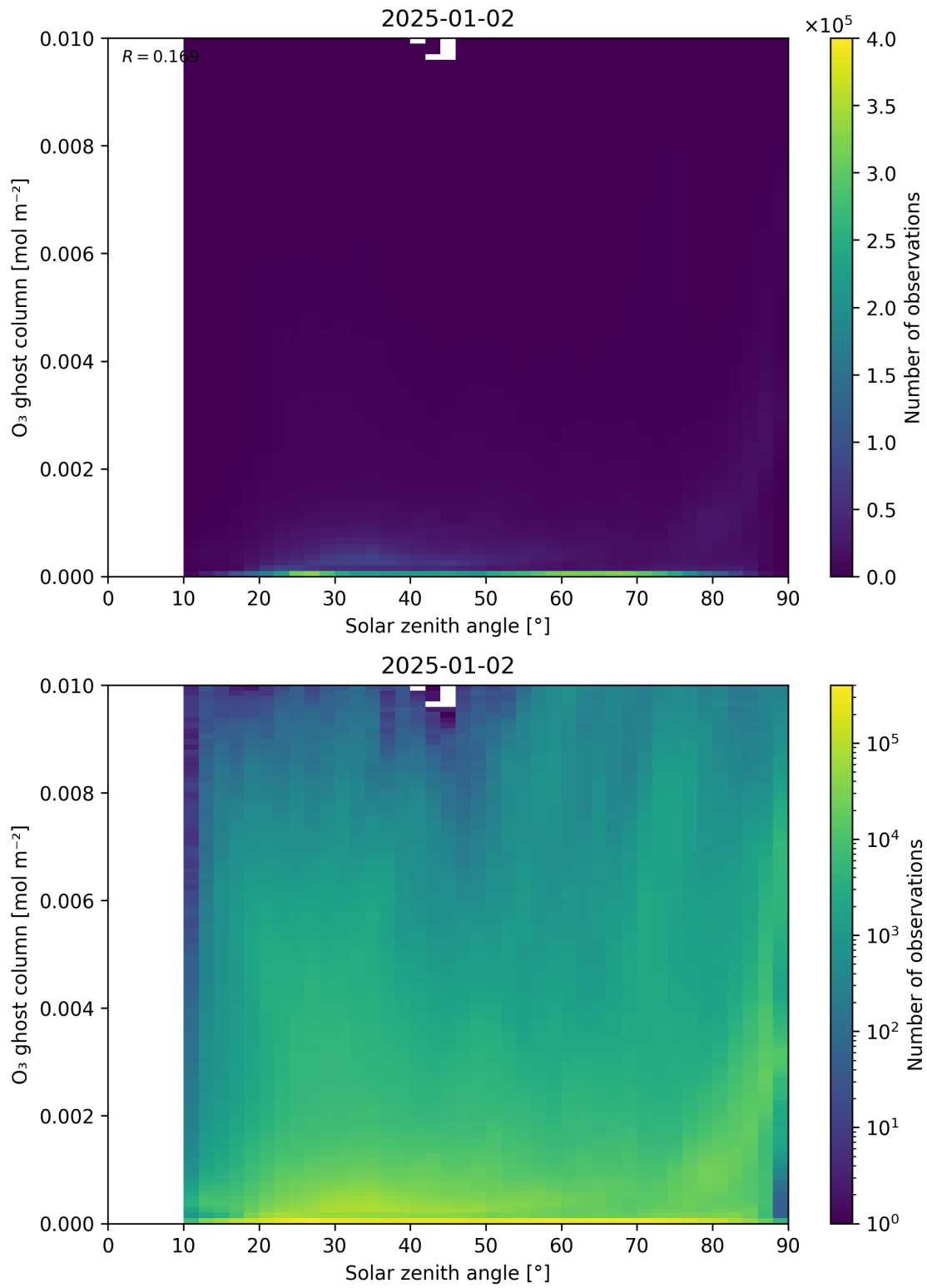
Figure 46: Scatter density plot of “Solar zenith angle” against “O 3 ghost column” for 2025-01-01 to 2025-01-03.
