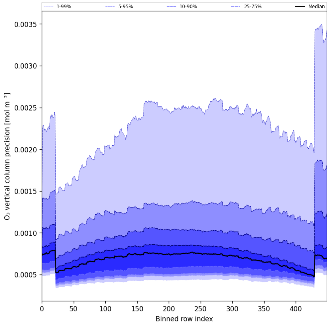
Figure 29: Along track statistics of “O 3 vertical column precision” for 2025-01-01 to 2025-01-03
