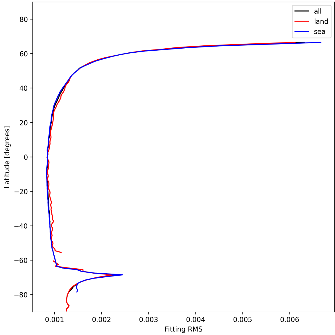
Figure 16: Zonal average of “Fitting RMS” for 2025-01-01 to 2025-01-03.
