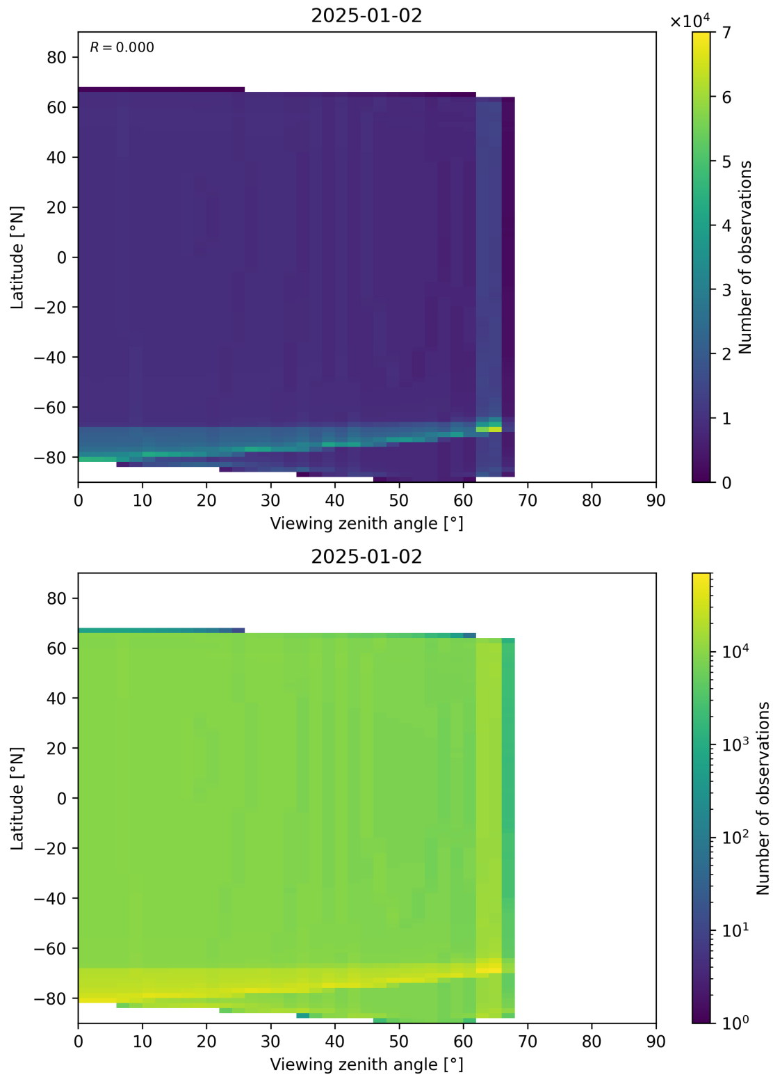
Figure 49: Scatter density plot of “Viewing zenith angle” against “Latitude” for 2025-01-01 to 2025-01-03.
