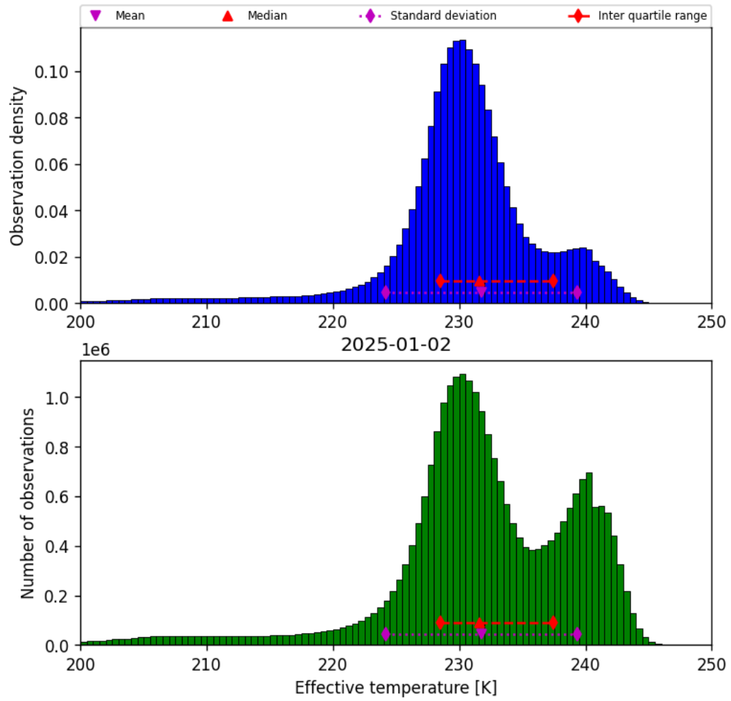
Figure 24: Histogram of “Effective temperature” for 2025-01-01 to 2025-01-03
