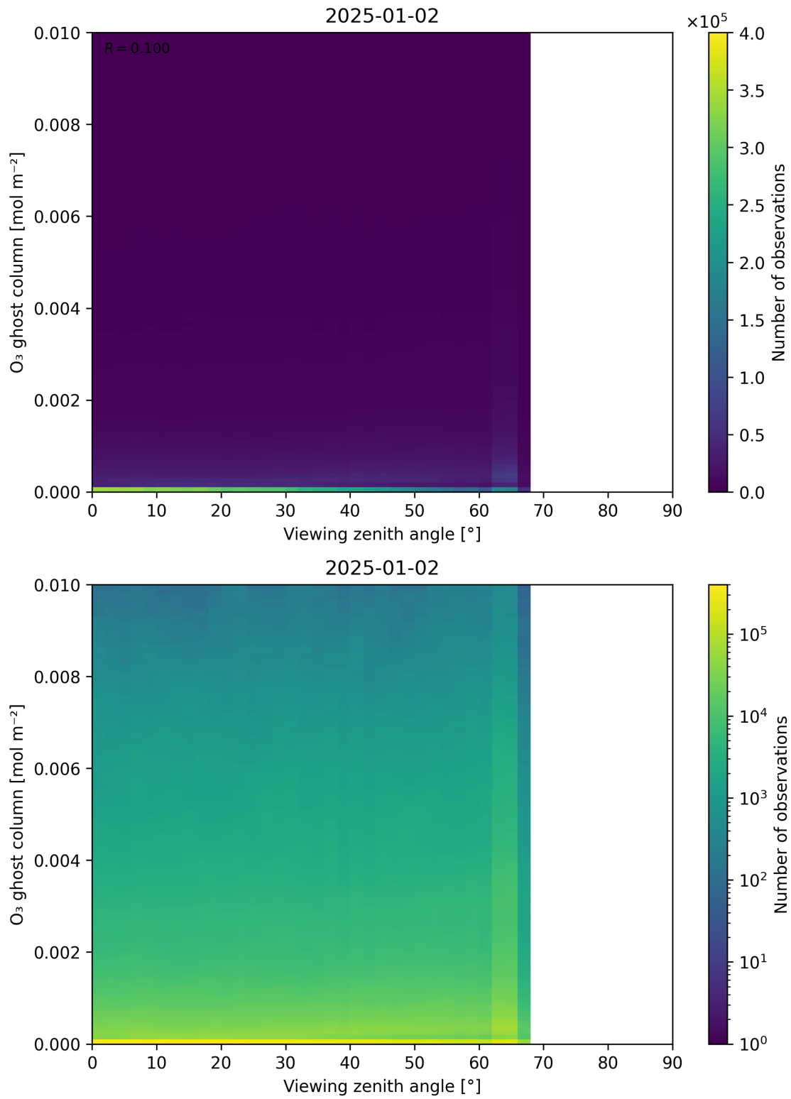
Figure 51: Scatter density plot of “Viewing zenith angle” against “O 3 ghost column” for 2025-01-01 to 2025-01-03.
