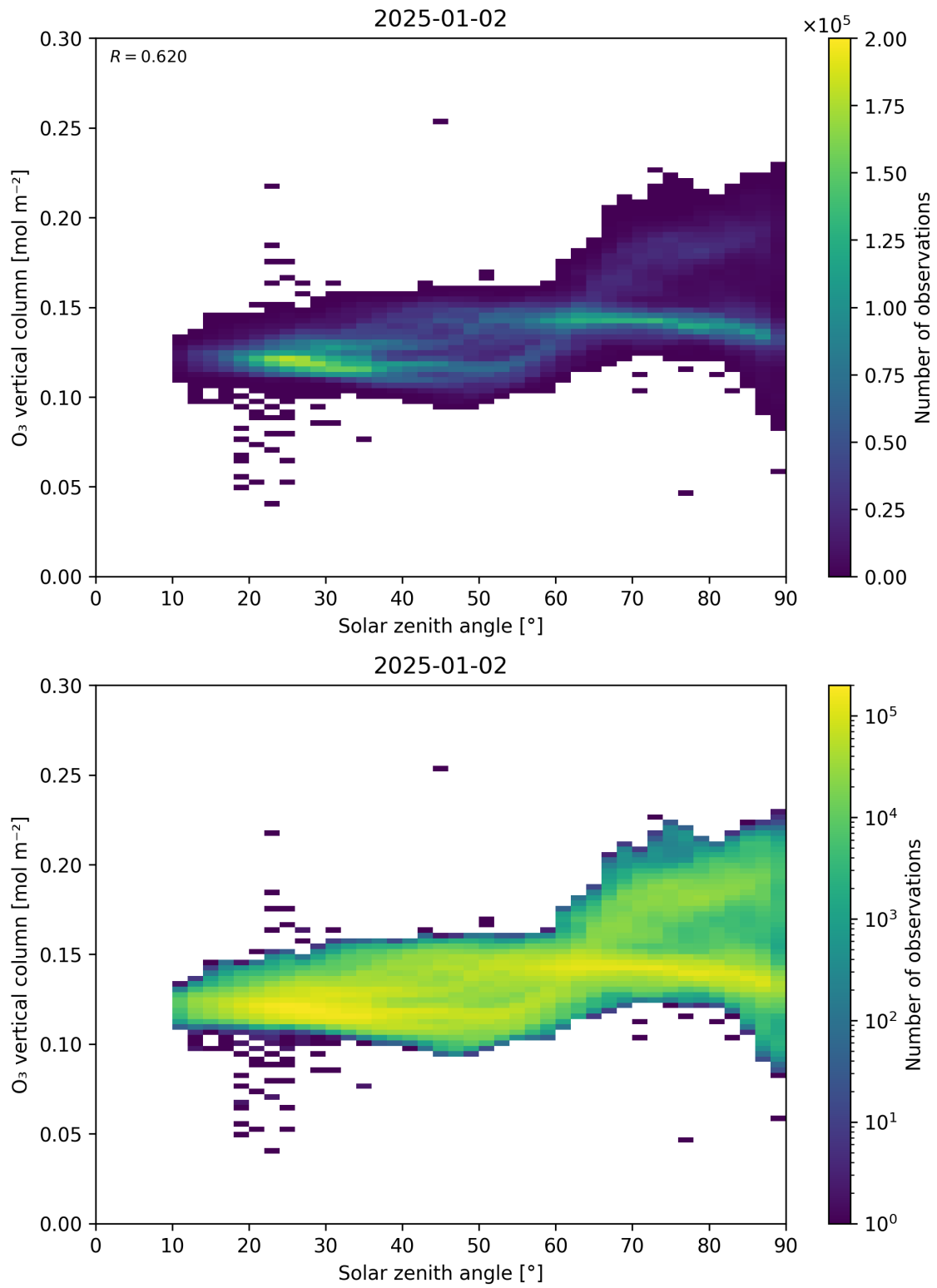
Figure 47: Scatter density plot of “Solar zenith angle” against “O 3 vertical column” for 2025-01-01 to 2025-01-03.
