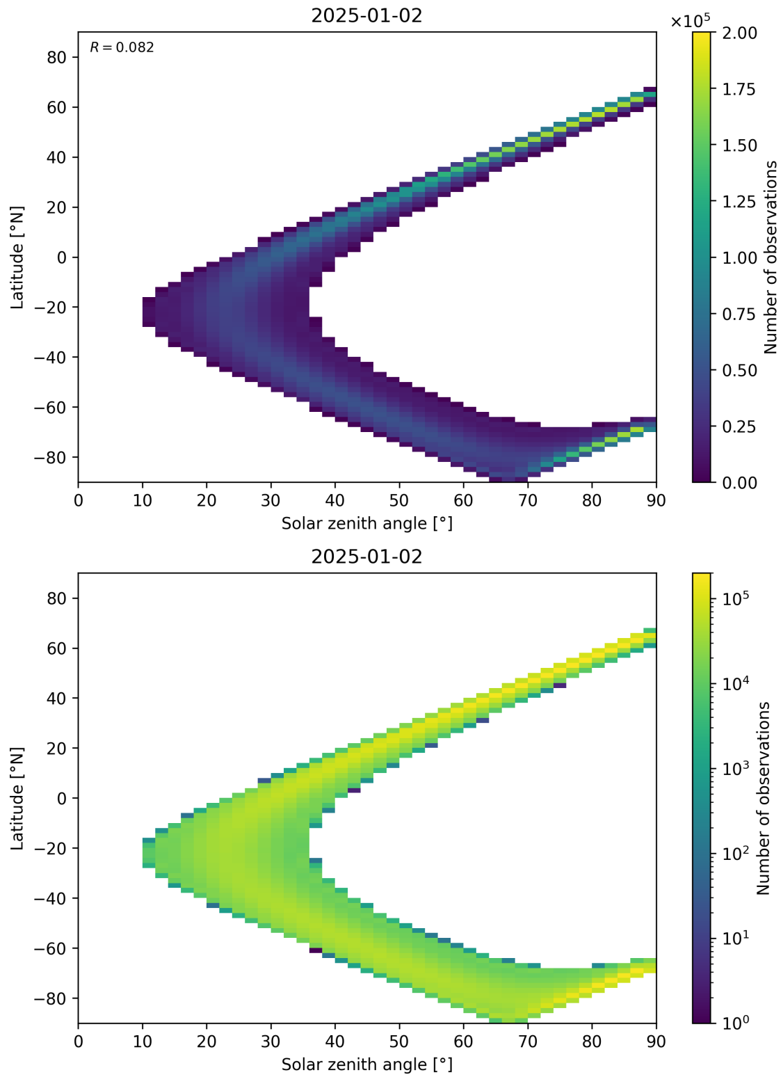
Figure 44: Scatter density plot of “Solar zenith angle” against “Latitude” for 2025-01-01 to 2025-01-03.
