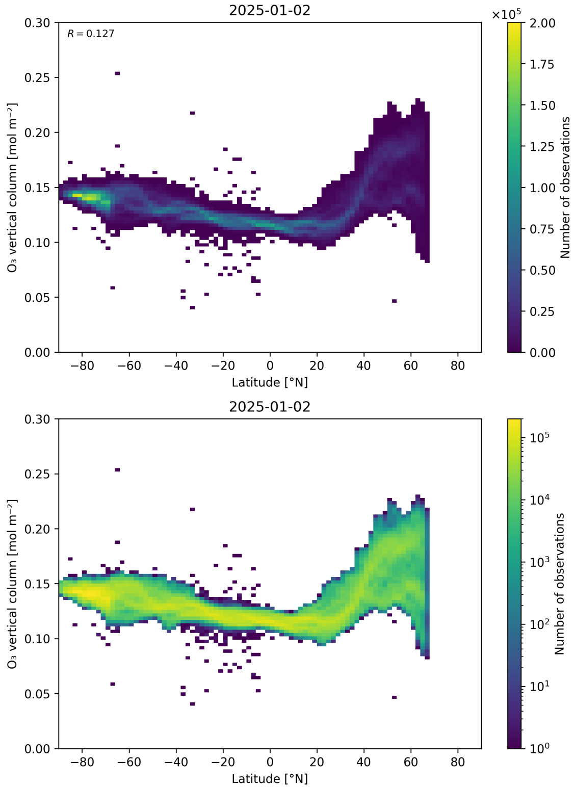
Figure 36: Scatter density plot of “Latitude” against “O 3 vertical column” for 2025-01-01 to 2025-01-03.
