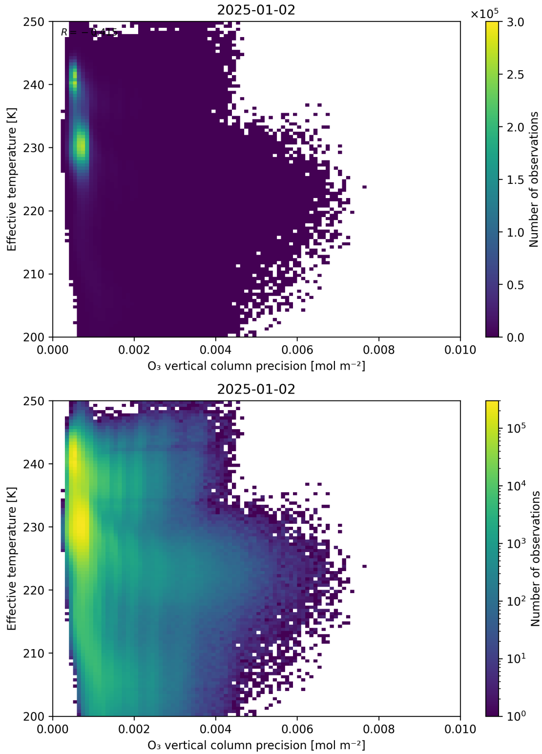
Figure 42: Scatter density plot of “ O_3 vertical column precision” against “Effective temperature” for 2025-01-01 to 2025-01-03.
