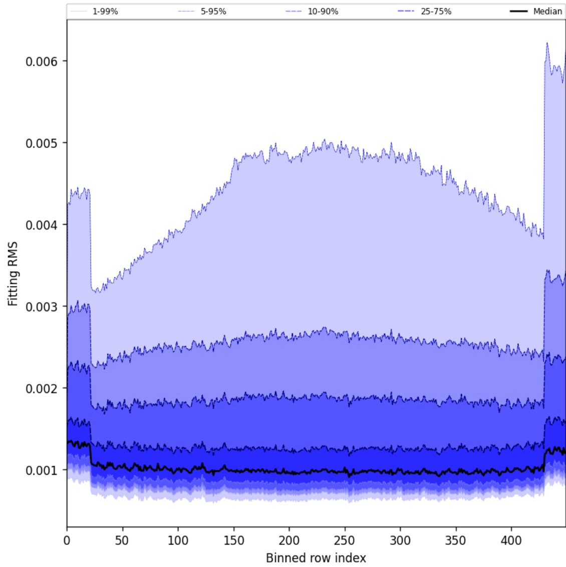
Figure 30: Along track statistics of “Fitting RMS” for 2025-01-01 to 2025-01-03
