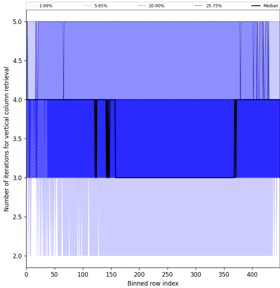
Figure 33: Along track statistics of “Number of iterations for vertical column retrieval” for 2025-01-01 to 2025-01-03
