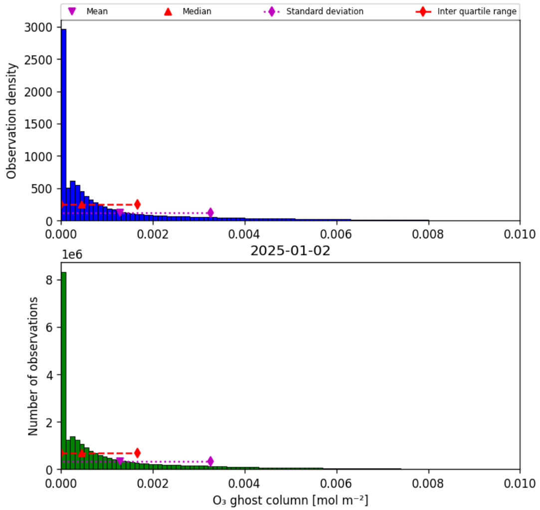
Figure 25: Histogram of “O 3 ghost column” for 2025-01-01 to 2025-01-03
