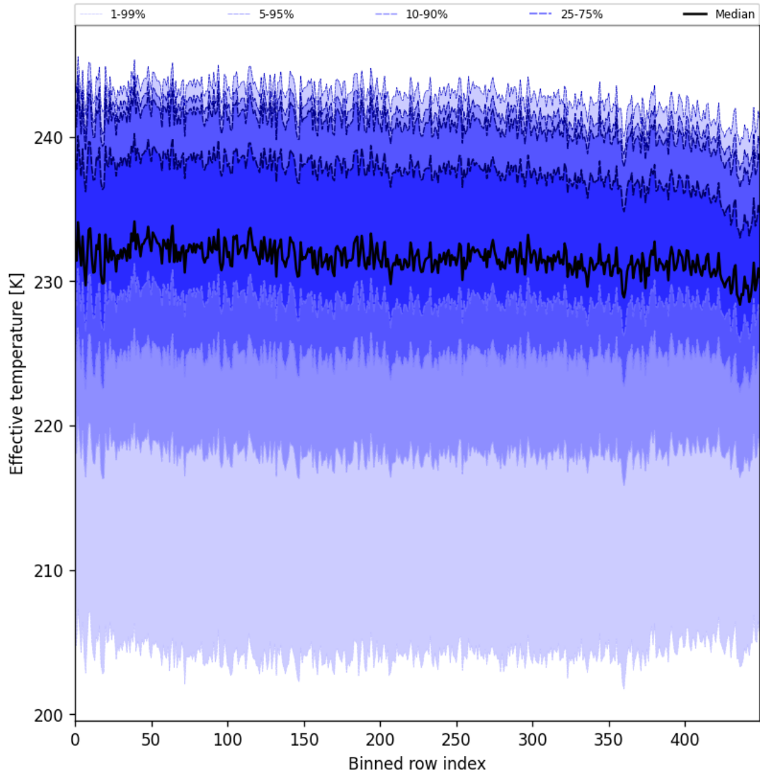
Figure 31: Along track statistics of “Effective temperature” for 2025-01-01 to 2025-01-03
