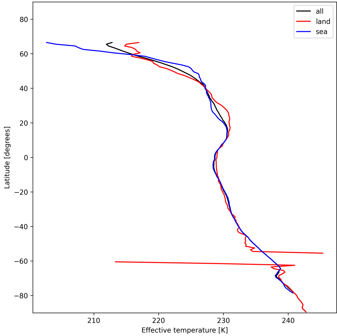
Figure 17: Zonal average of "Effective temperature" for 2025-01-01 to 2025-01-03.
