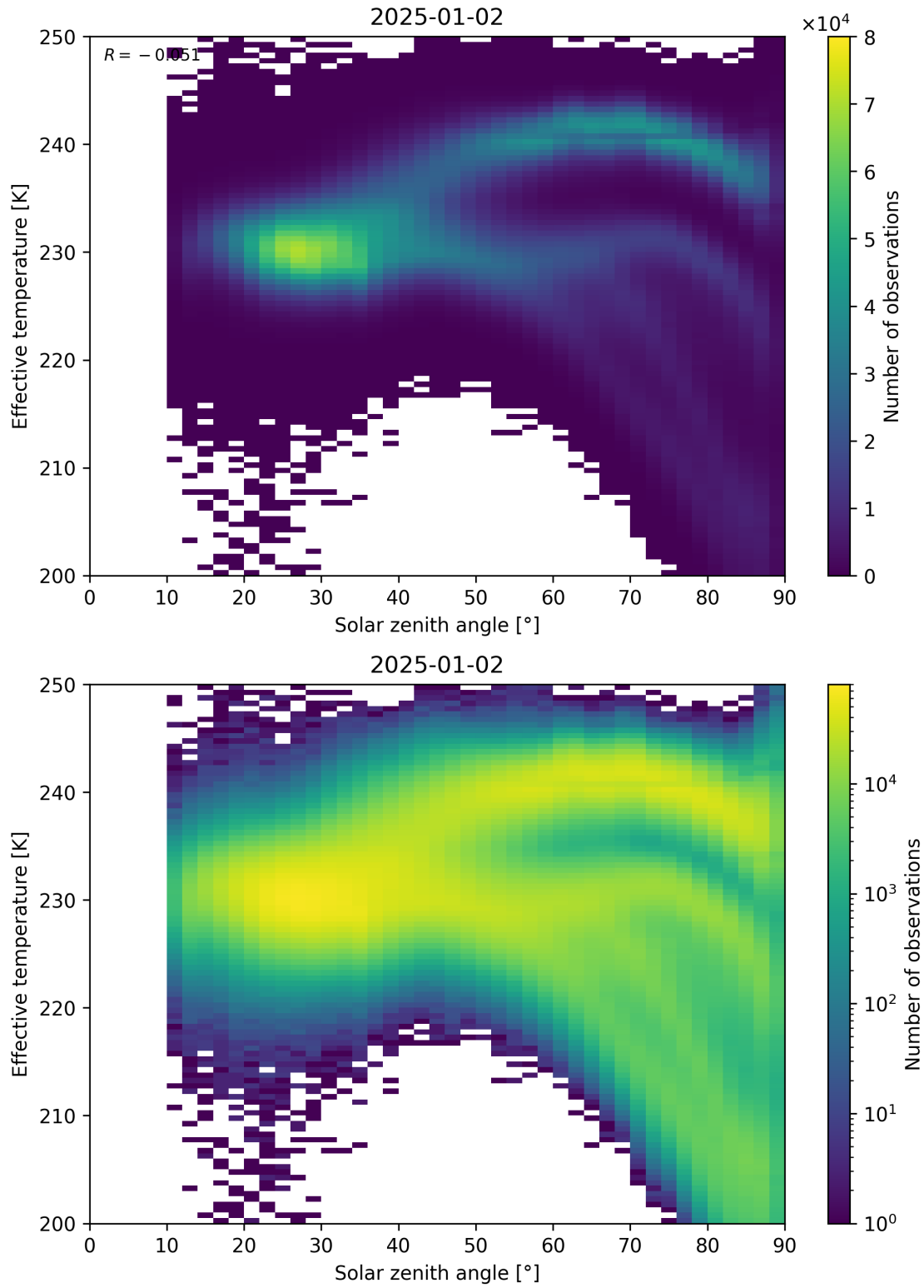
Figure 45: Scatter density plot of “Solar zenith angle” against “Effective temperature” for 2025-01-01 to 2025-01-03.
