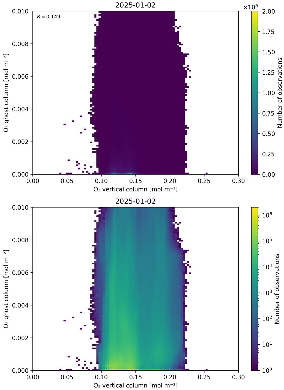
Figure 40: Scatter density plot of “O 3 vertical column” against “O 3 ghost column” for 2025-01-01 to 2025-01-03.
