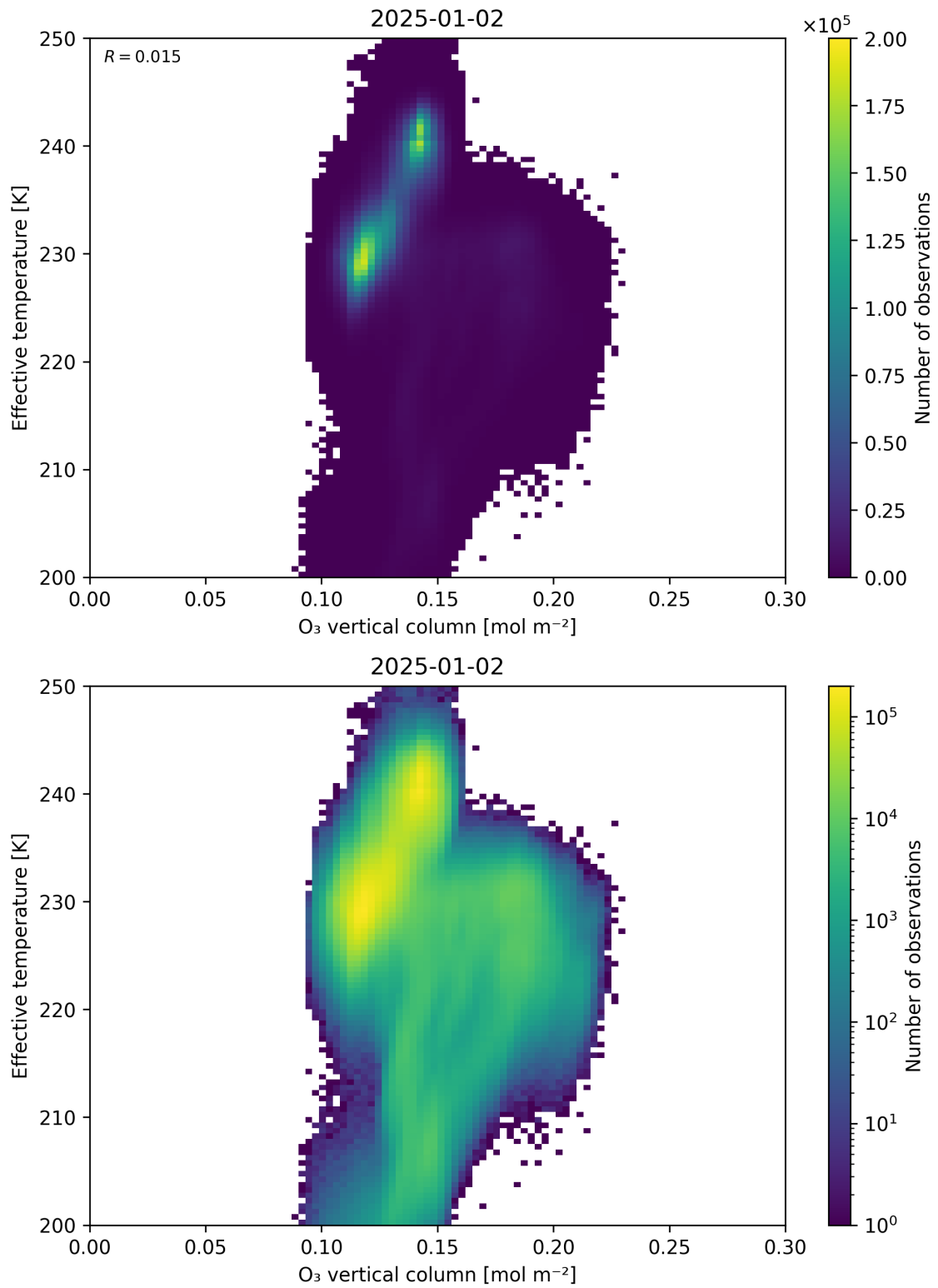
Figure 39: Scatter density plot of “O 3 vertical column” against “Effective temperature” for 2025-01-01 to 2025-01-03.
