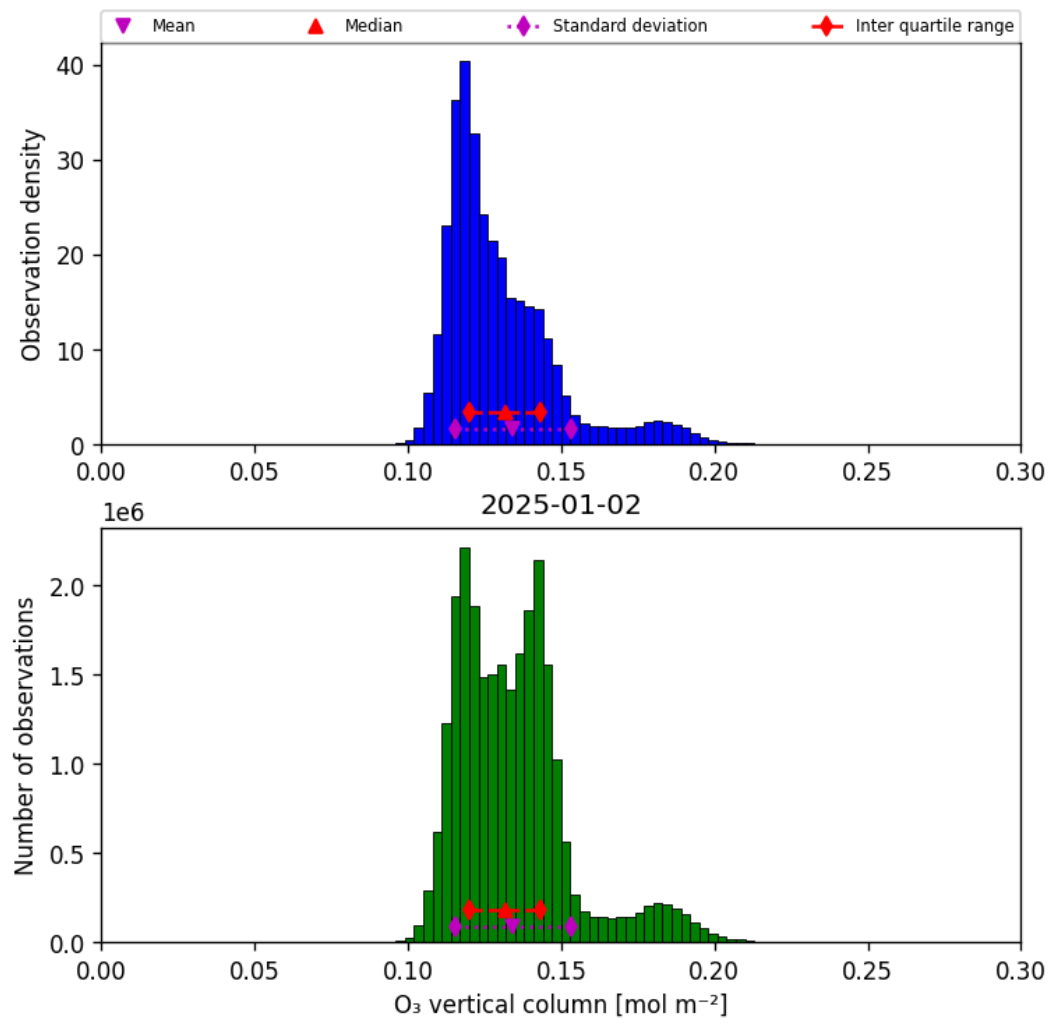
Figure 21: Histogram of “O 3 vertical column” for 2025-01-01 to 2025-01-03
