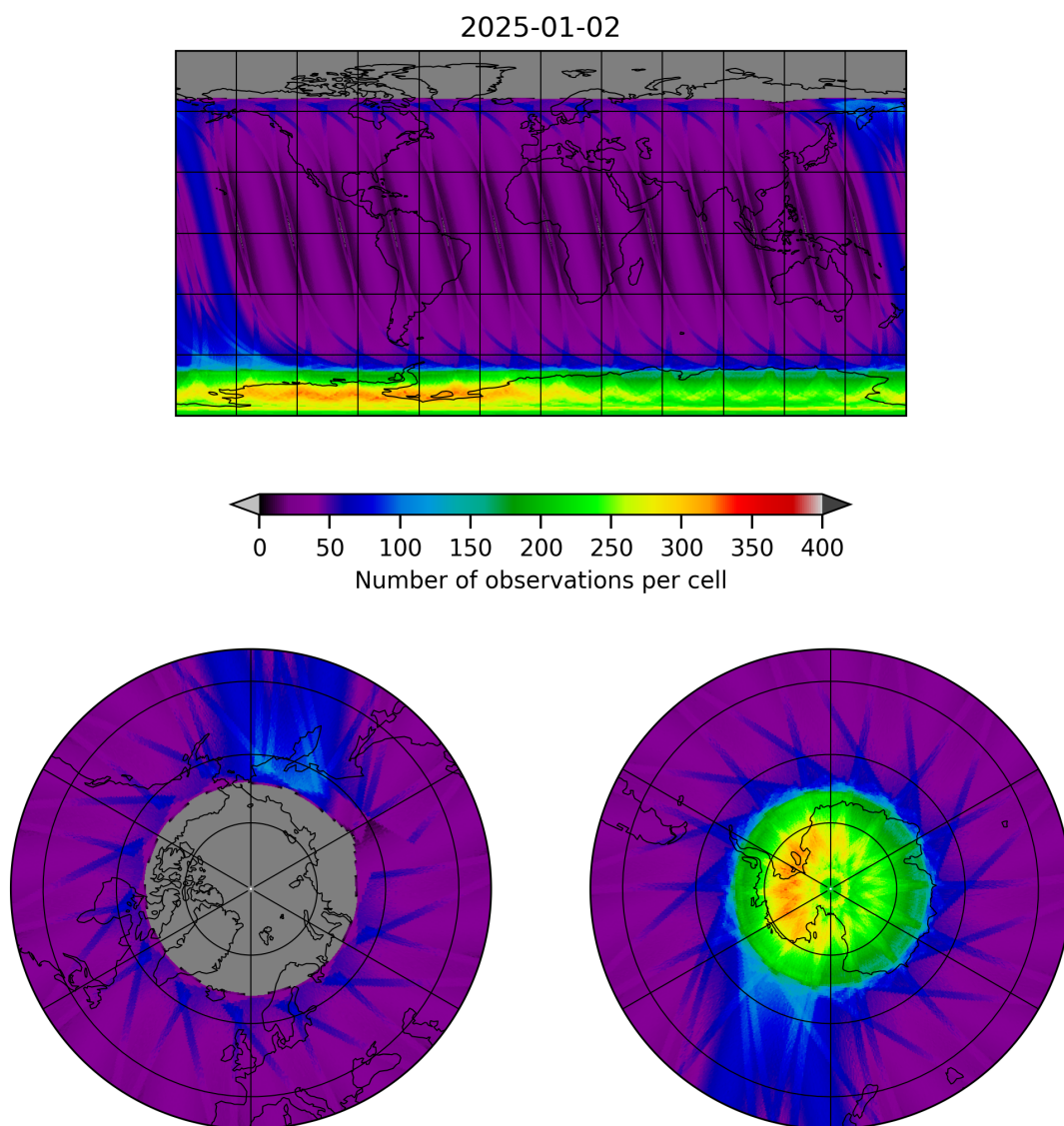
Figure 12: Map of the number of observations for 2025-01-01 to 2025-01-03
