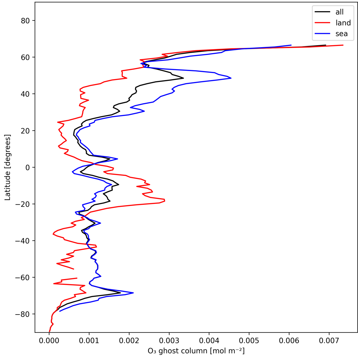
Figure 18: Zonal average of "O 3 ghost column" for 2025-01-01 to 2025-01-03.
