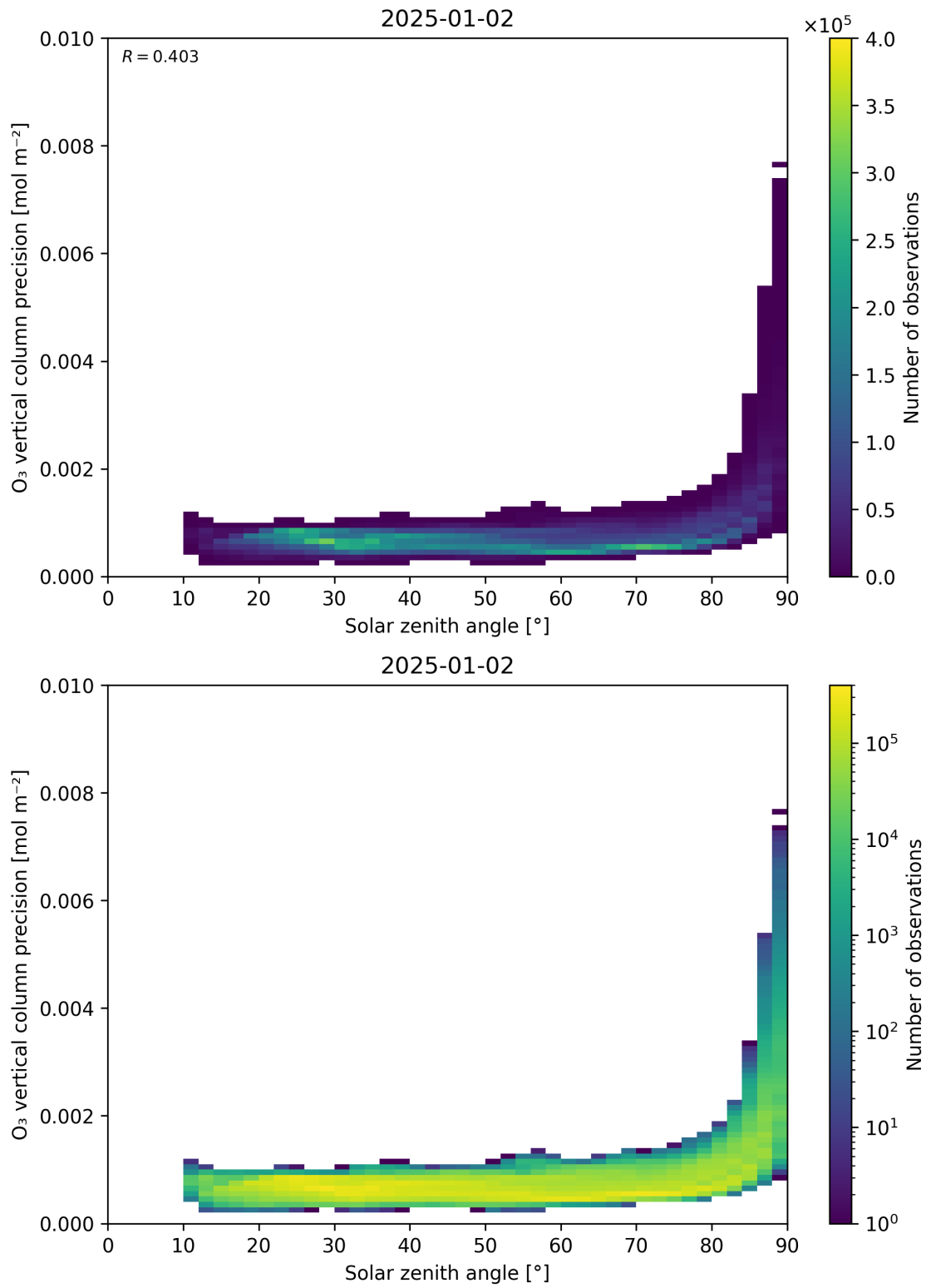
Figure 48: Scatter density plot of “Solar zenith angle” against “O 3 vertical column precision” for 2025-01-01 to 2025-01-03.
