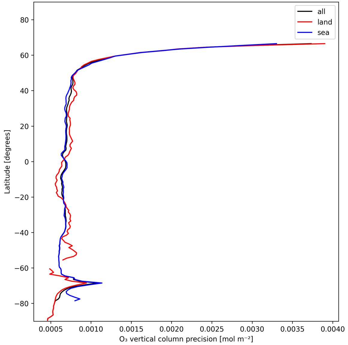
Figure 15: Zonal average of “O 3 vertical column precision” for 2025-01-01 to 2025-01-03.
