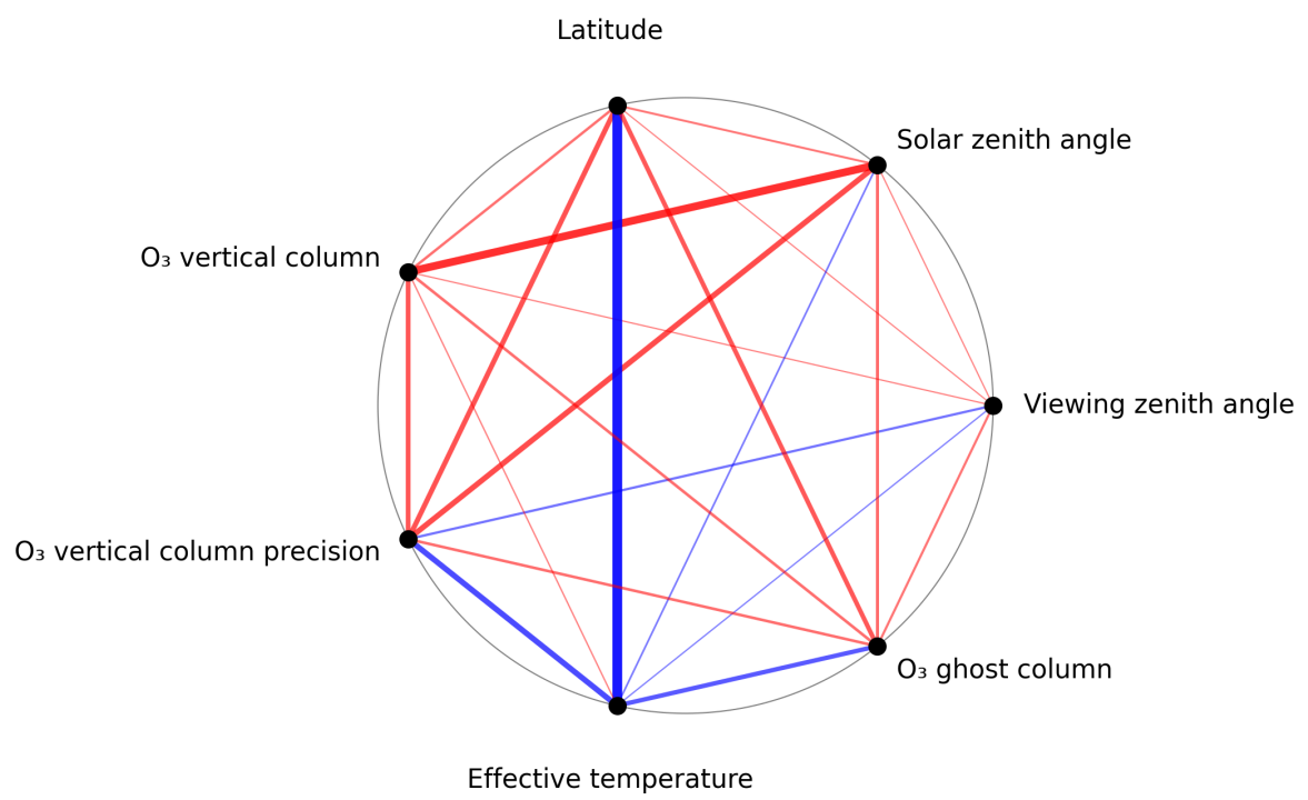
Figure 1: Map of correlation graph for 2025-01-01 to 2025-01-03.
