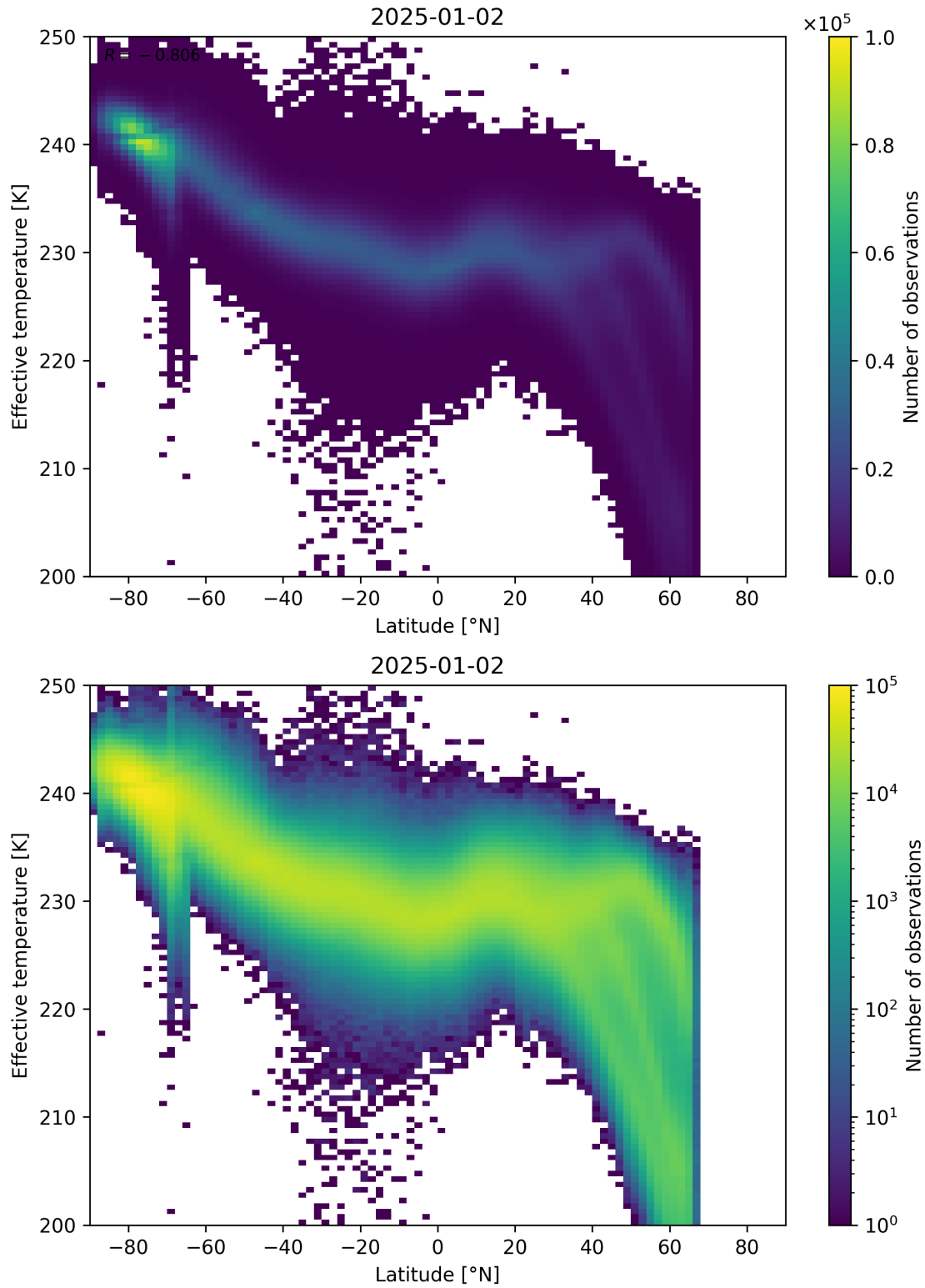
Figure 34: Scatter density plot of “Latitude” against “Effective temperature” for 2025-01-01 to 2025-01-03.
