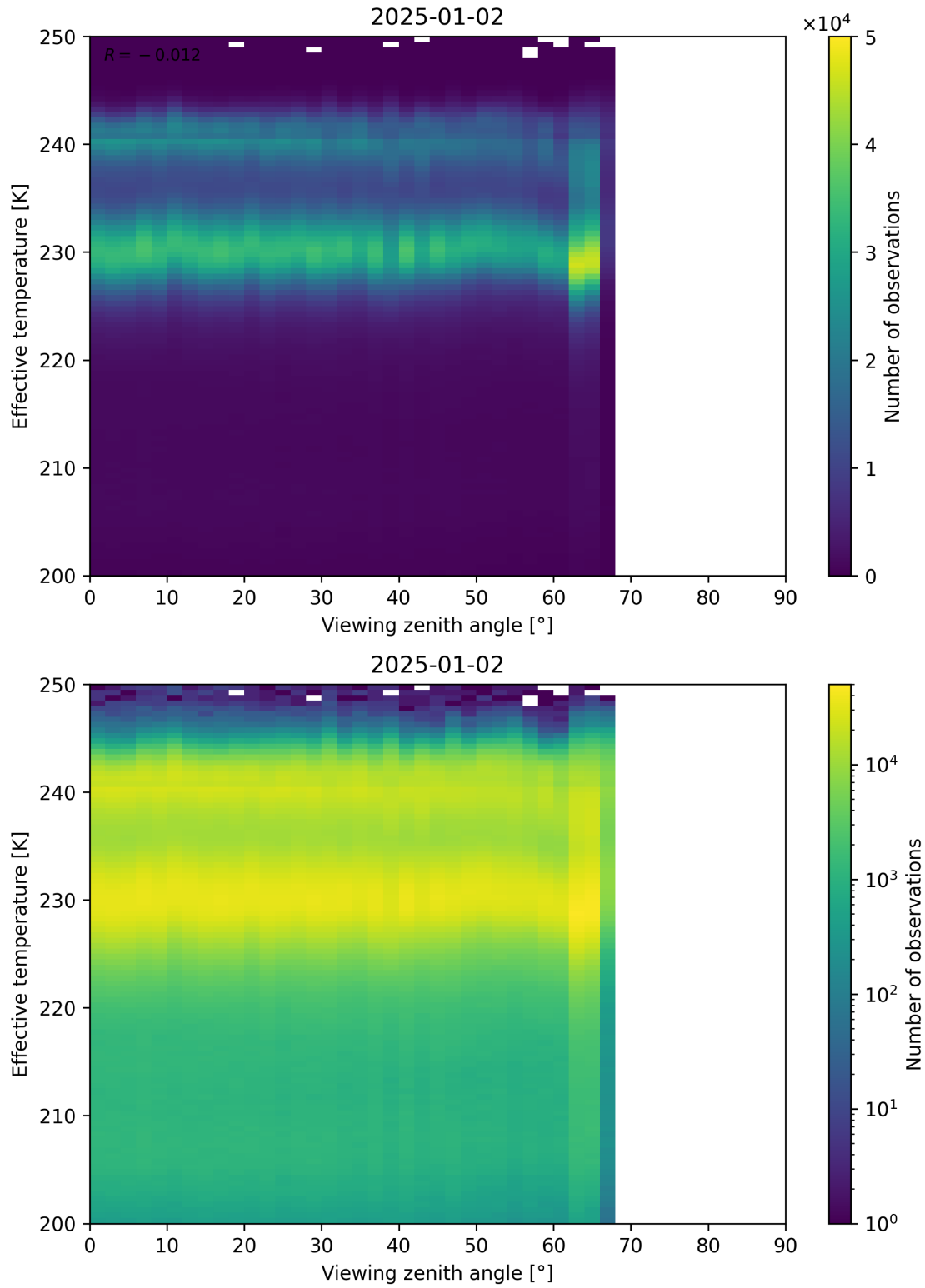
Figure 50: Scatter density plot of “Viewing zenith angle” against “Effective temperature” for 2025-01-01 to 2025-01-03.
