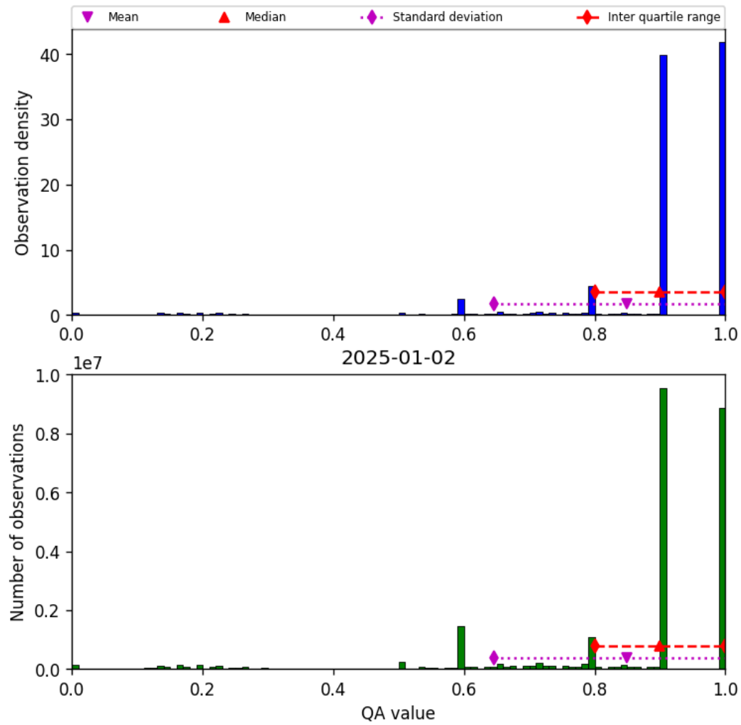
Figure 20: Histogram of “QA value” for 2025-01-01 to 2025-01-03
