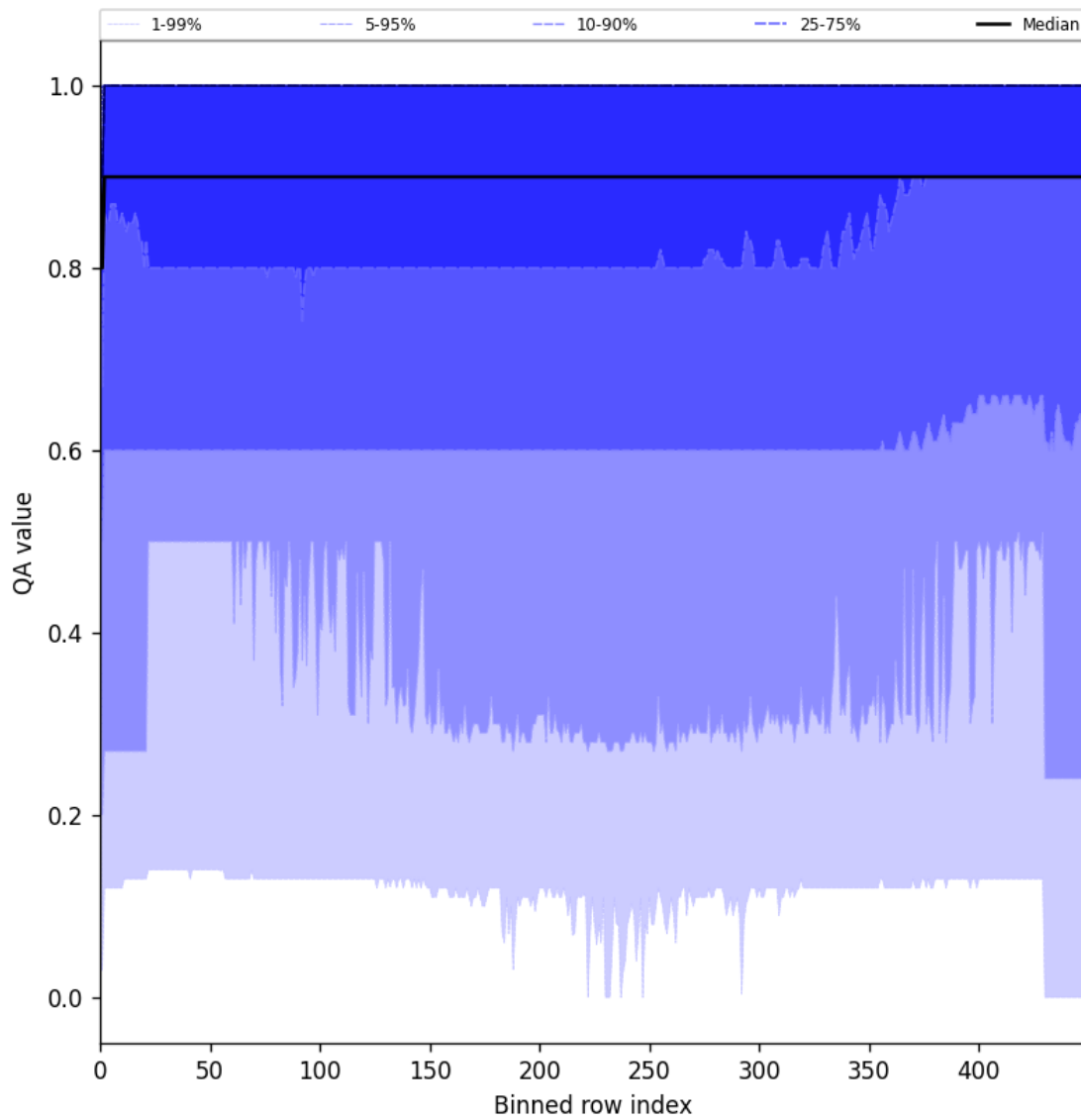
Figure 27: Along track statistics of “QA value” for 2025-01-01 to 2025-01-03
