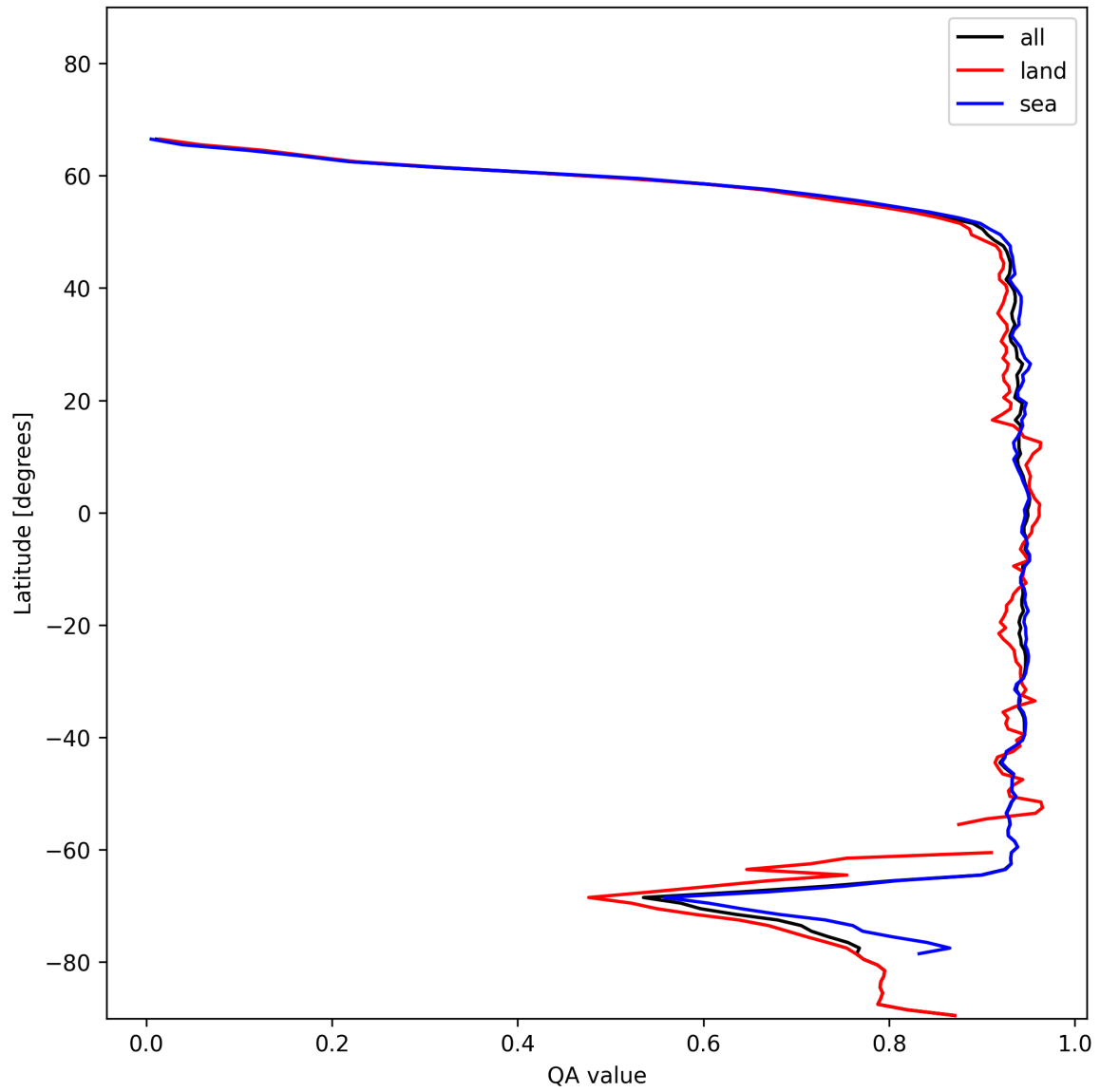
Figure 13: Zonal average of “QA value” for 2025-01-01 to 2025-01-03.
