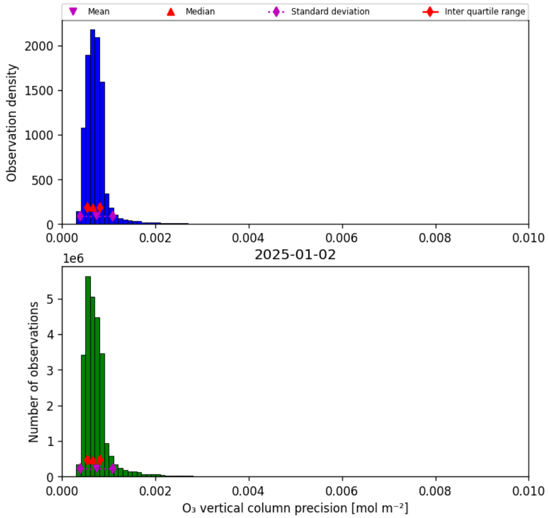
Figure 22: Histogram of “O 3 vertical column precision” for 2025-01-01 to 2025-01-03
