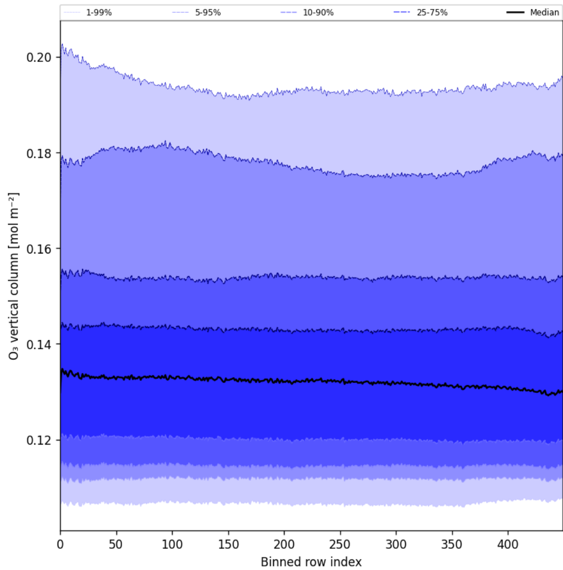
Figure 28: Along track statistics of “O 3 vertical column” for 2025-01-01 to 2025-01-03
