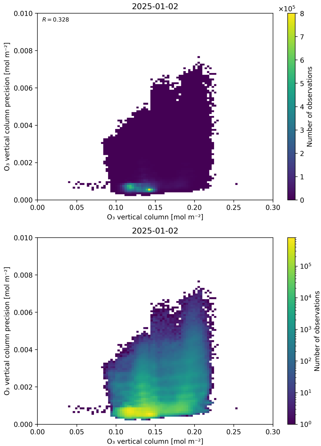
Figure 41: Scatter density plot of “O 3 vertical column” against “O 3 vertical column precision” for 2025-01-01 to 2025-01-03.
