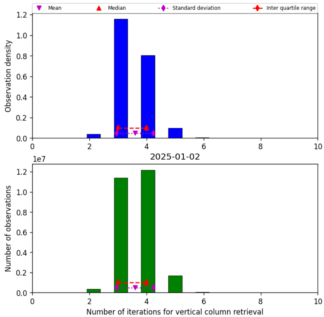
Figure 26: Histogram of “Number of iterations for vertical column retrieval” for 2025-01-01 to 2025-01-03
