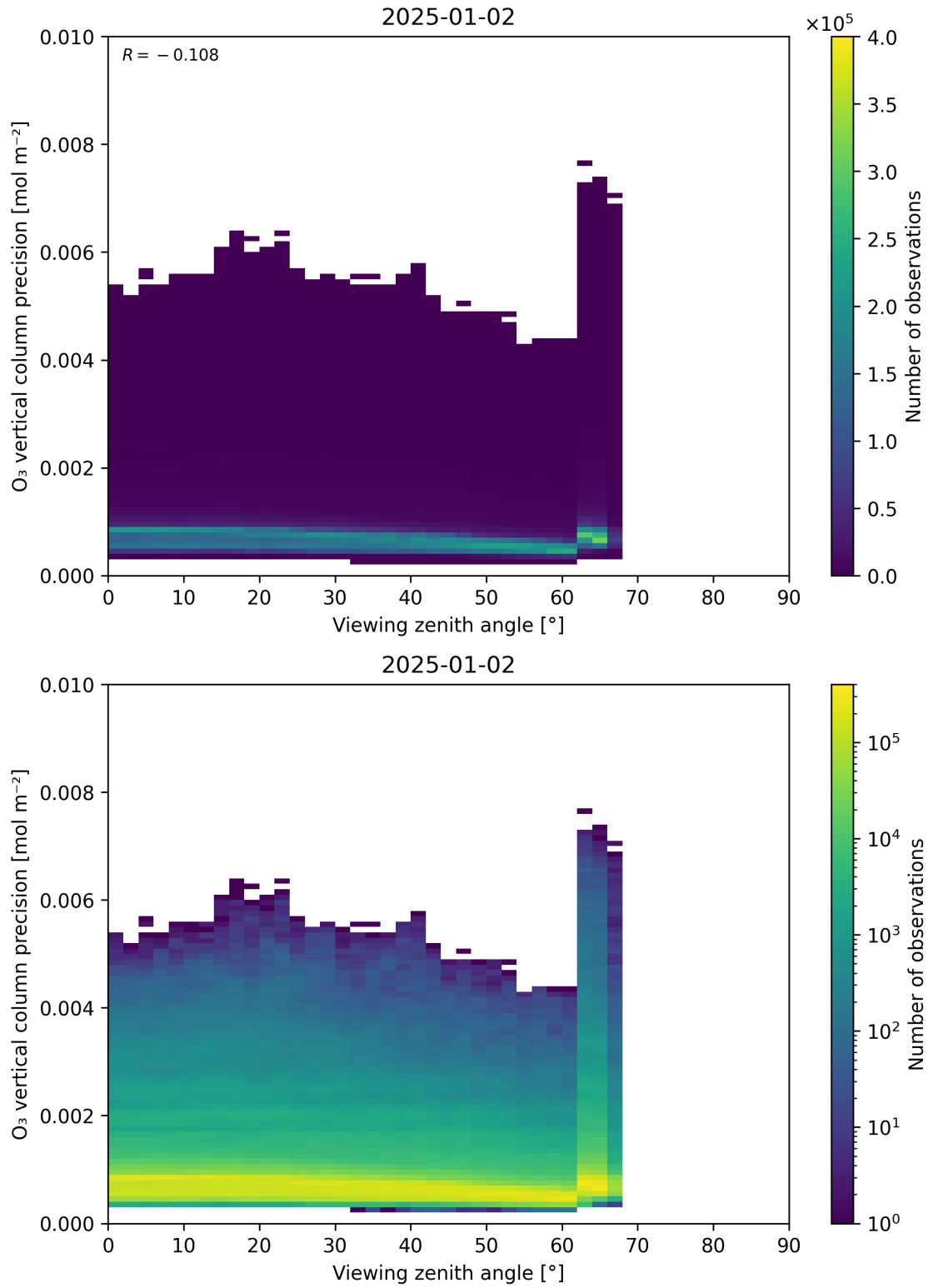
Figure 53: Scatter density plot of “Viewing zenith angle” against “O 3 vertical column precision” for 2025-01-01 to 2025-01-03.
