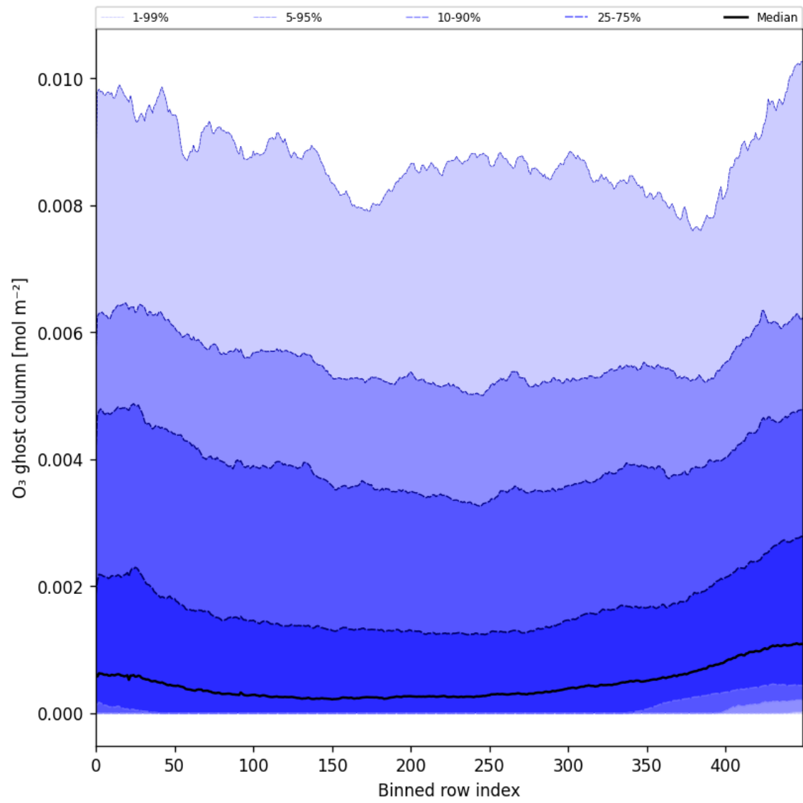
Figure 32: Along track statistics of “O 3 ghost column” for 2025-01-01 to 2025-01-03
