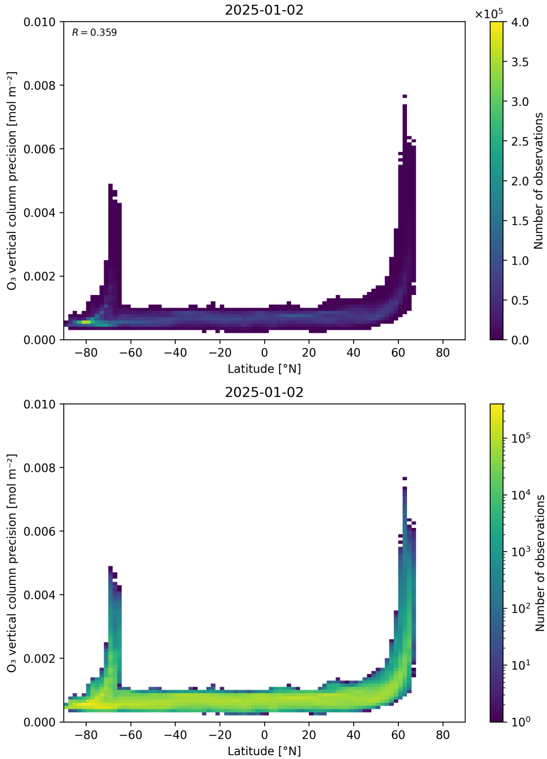
Figure 37: Scatter density plot of “Latitude” against “O 3 vertical column precision” for 2025-01-01 to 2025-01-03.
