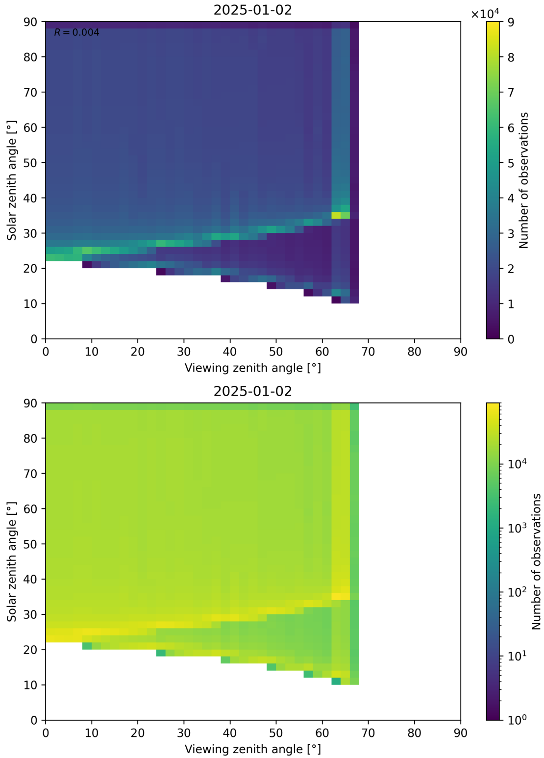
Figure 54: Scatter density plot of “Viewing zenith angle” against “Solar zenith angle” for 2025-01-01 to 2025-01-03.
