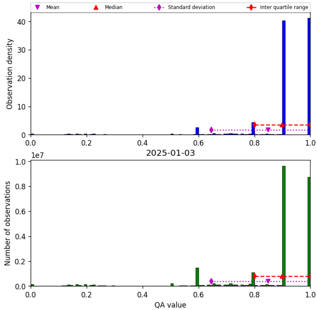
Figure 20: Histogram of “QA value” for 2025-01-02 to 2025-01-04
