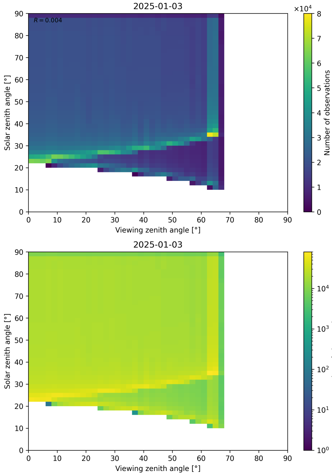
Figure 54: Scatter density plot of “Viewing zenith angle” against “Solar zenith angle” for 2025-01-02 to 2025-01-04.
