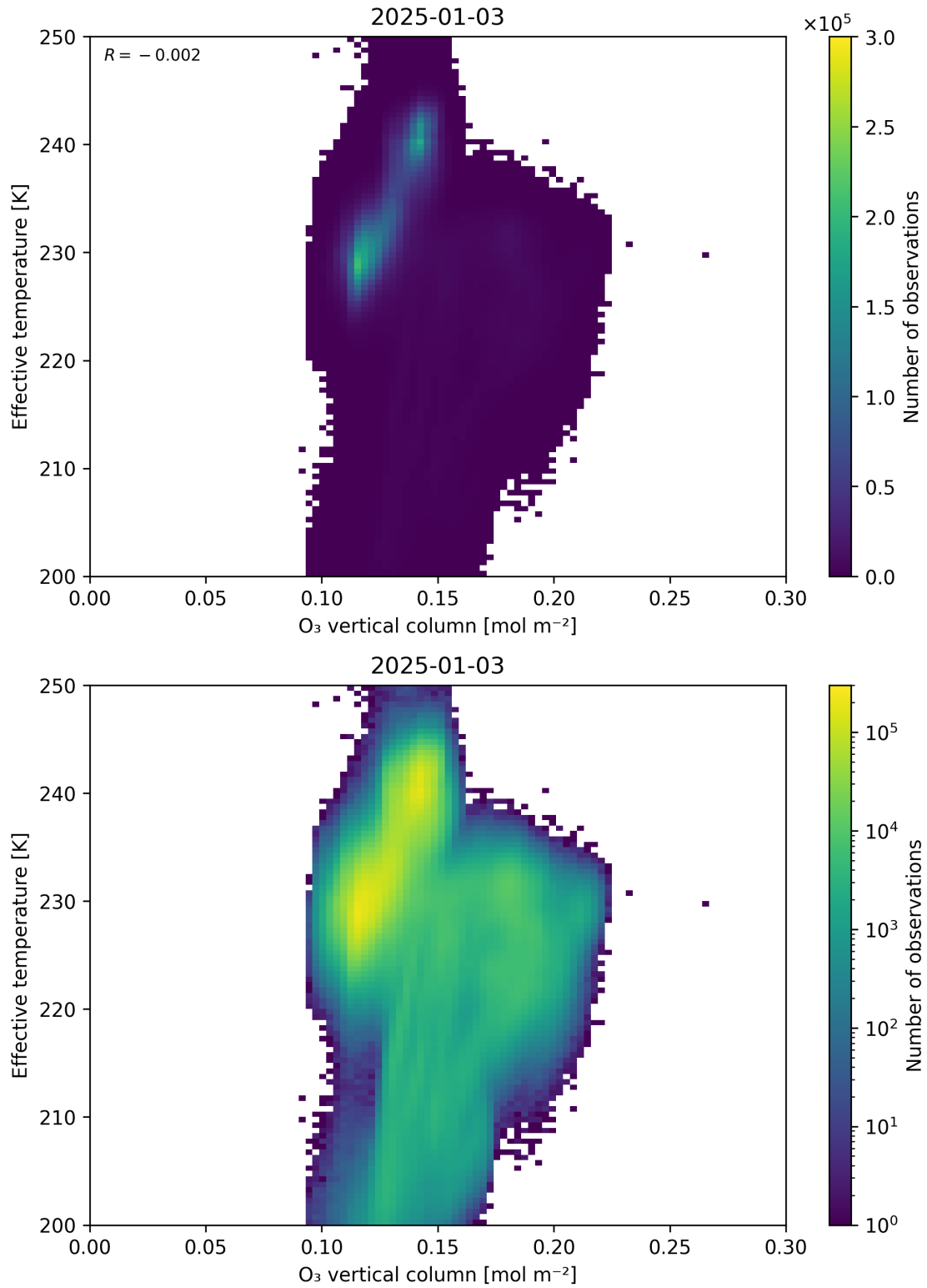
Figure 39: Scatter density plot of “O 3 vertical column” against “Effective temperature” for 2025-01-02 to 2025-01-04.
