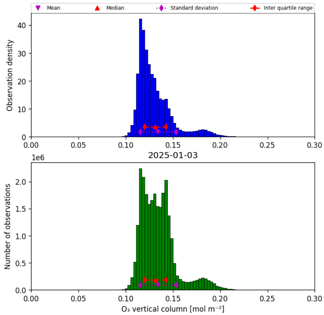
Figure 21: Histogram of “O 3 vertical column” for 2025-01-02 to 2025-01-04
