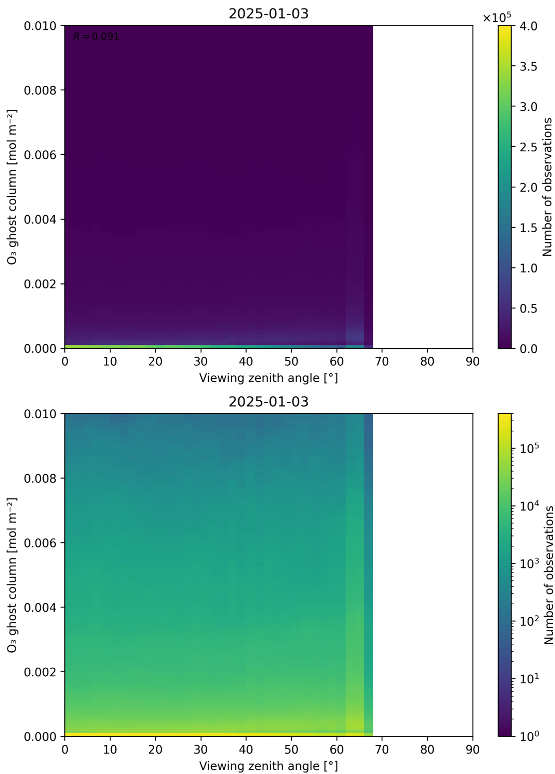
Figure 51: Scatter density plot of “Viewing zenith angle” against “O 3 ghost column” for 2025-01-02 to 2025-01-04.
