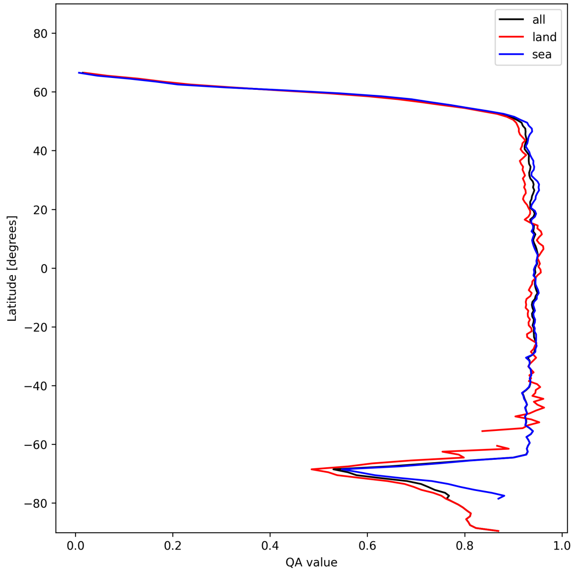
Figure 13: Zonal average of “QA value” for 2025-01-02 to 2025-01-04.
