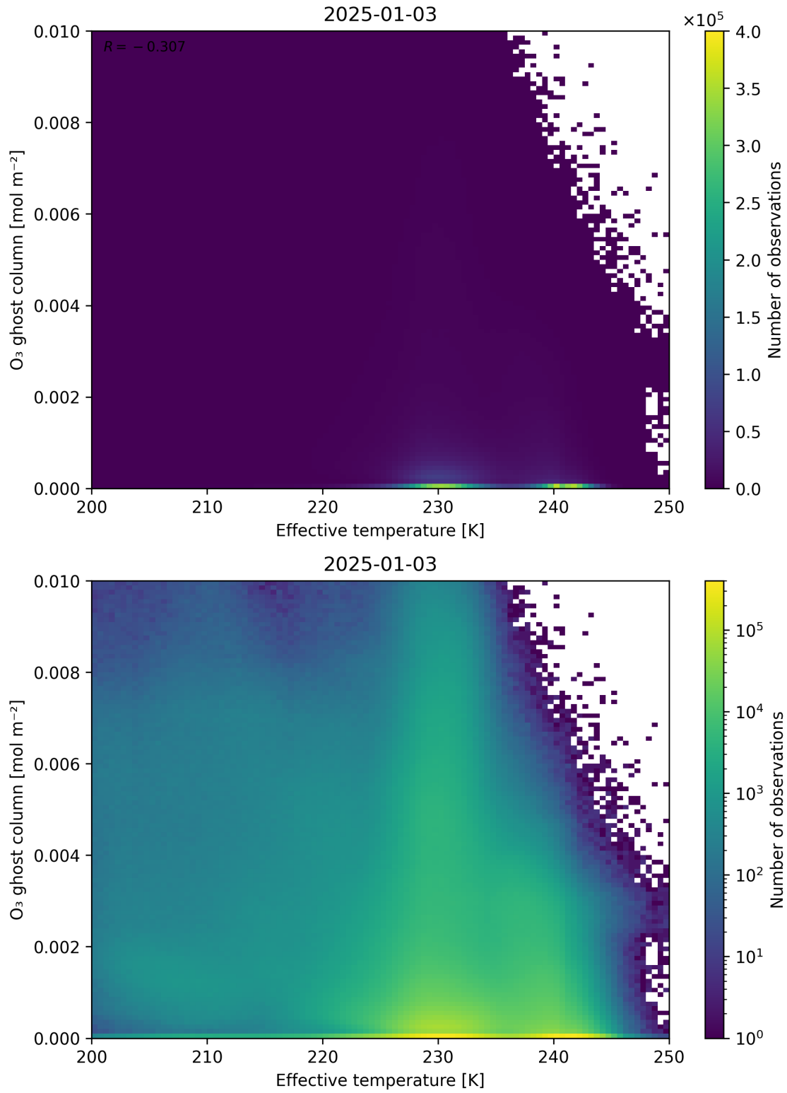
Figure 38: Scatter density plot of “Effective temperature” against “O 3 ghost column” for 2025-01-02 to 2025-01-04.
