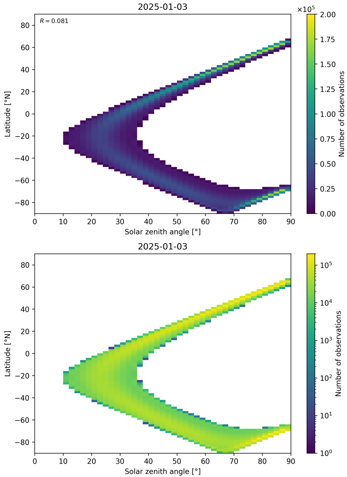
Figure 44: Scatter density plot of “Solar zenith angle” against “Latitude” for 2025-01-02 to 2025-01-04.
