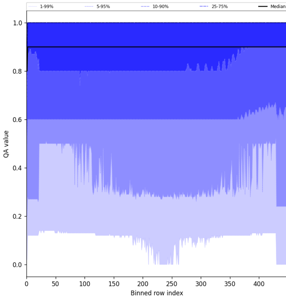
Figure 27: Along track statistics of “QA value” for 2025-01-02 to 2025-01-04
