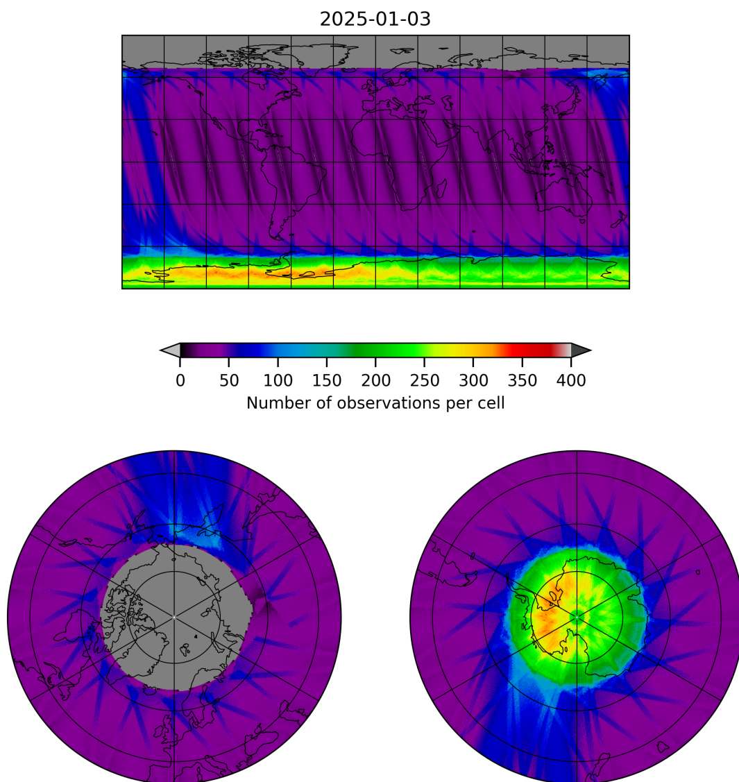
Figure 12: Map of the number of observations for 2025-01-02 to 2025-01-04
