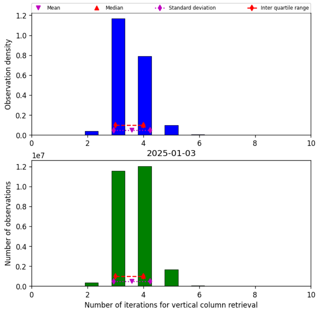
Figure 26: Histogram of “Number of iterations for vertical column retrieval” for 2025-01-02 to 2025-01-04
