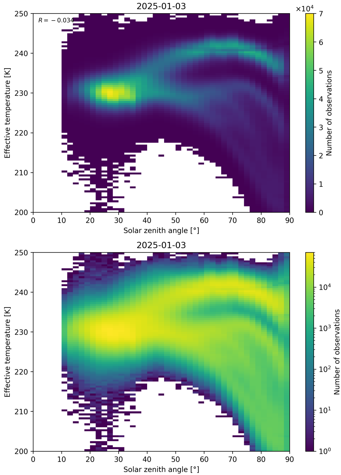
Figure 45: Scatter density plot of “Solar zenith angle” against “Effective temperature” for 2025-01-02 to 2025-01-04.
