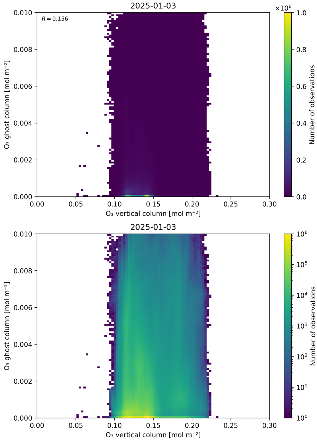
Figure 40: Scatter density plot of “O 3 vertical column” against “O 3 ghost column” for 2025-01-02 to 2025-01-04.
