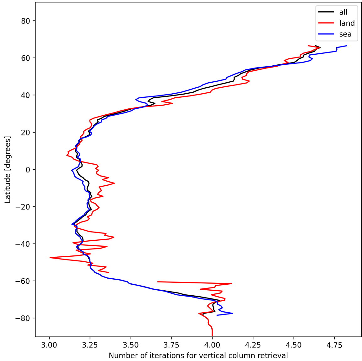
Figure 19: Zonal average of “Number of iterations for vertical column retrieval” for 2025-01-02 to 2025-01-04.
