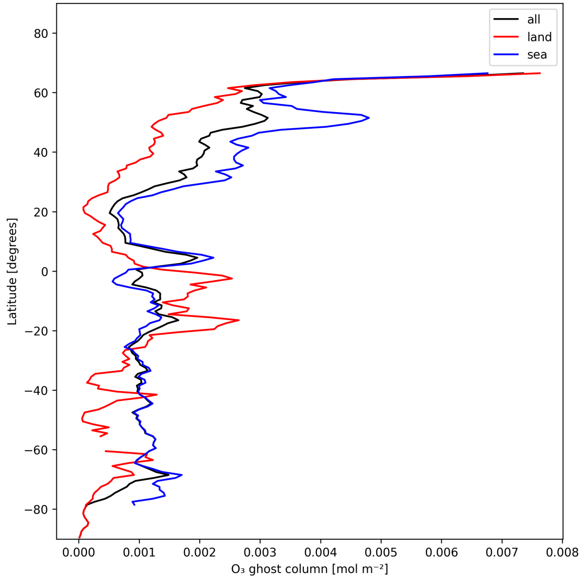
Figure 18: Zonal average of “O 3 ghost column” for 2025-01-02 to 2025-01-04.
