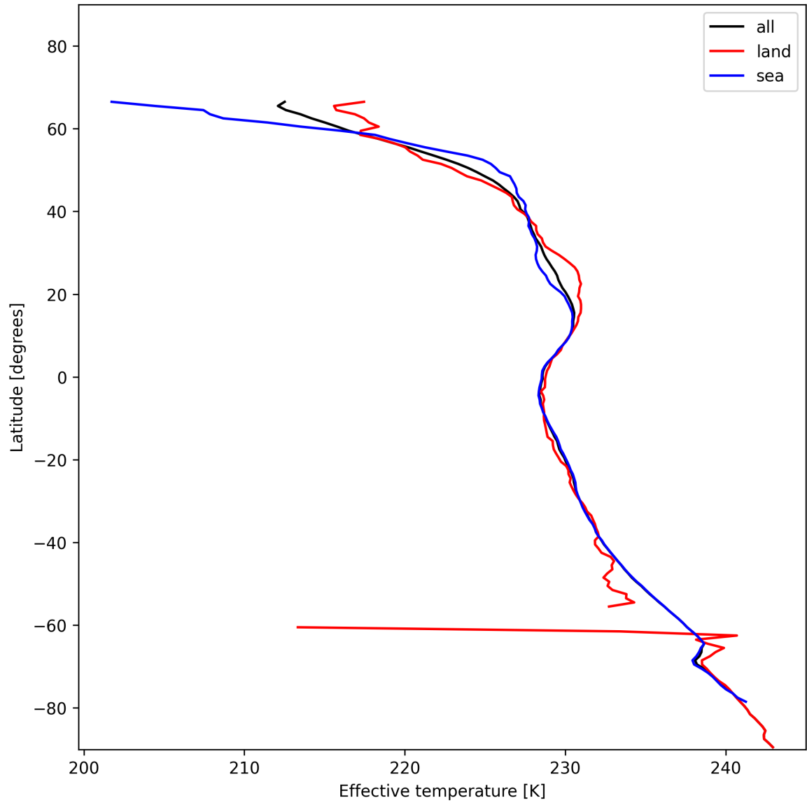
Figure 17: Zonal average of "Effective temperature" for 2025-01-02 to 2025-01-04.
