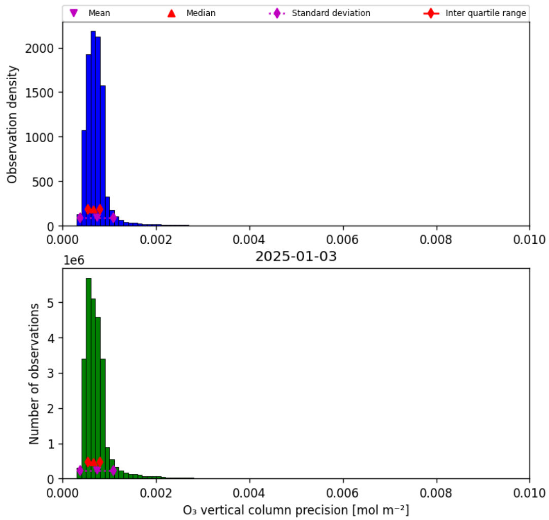
Figure 22: Histogram of “O 3 vertical column precision” for 2025-01-02 to 2025-01-04
