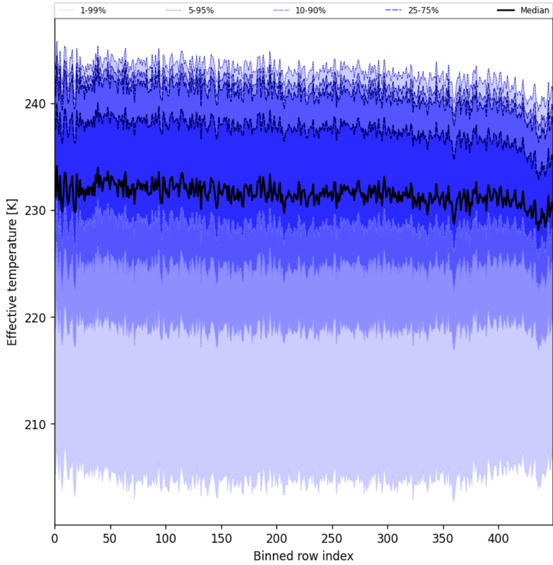
Figure 31: Along track statistics of “Effective temperature” for 2025-01-02 to 2025-01-04
