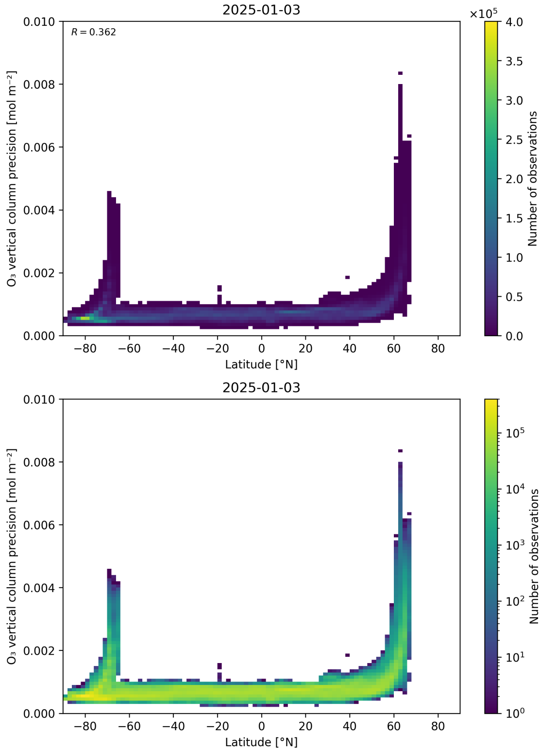
Figure 37: Scatter density plot of “Latitude” against “O 3 vertical column precision” for 2025-01-02 to 2025-01-04.
