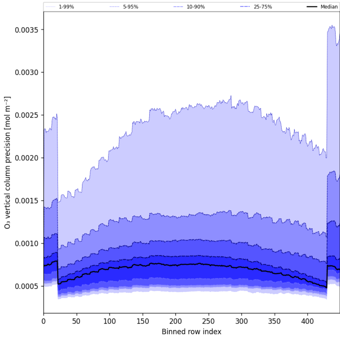
Figure 29: Along track statistics of “O 3 vertical column precision” for 2025-01-02 to 2025-01-04
