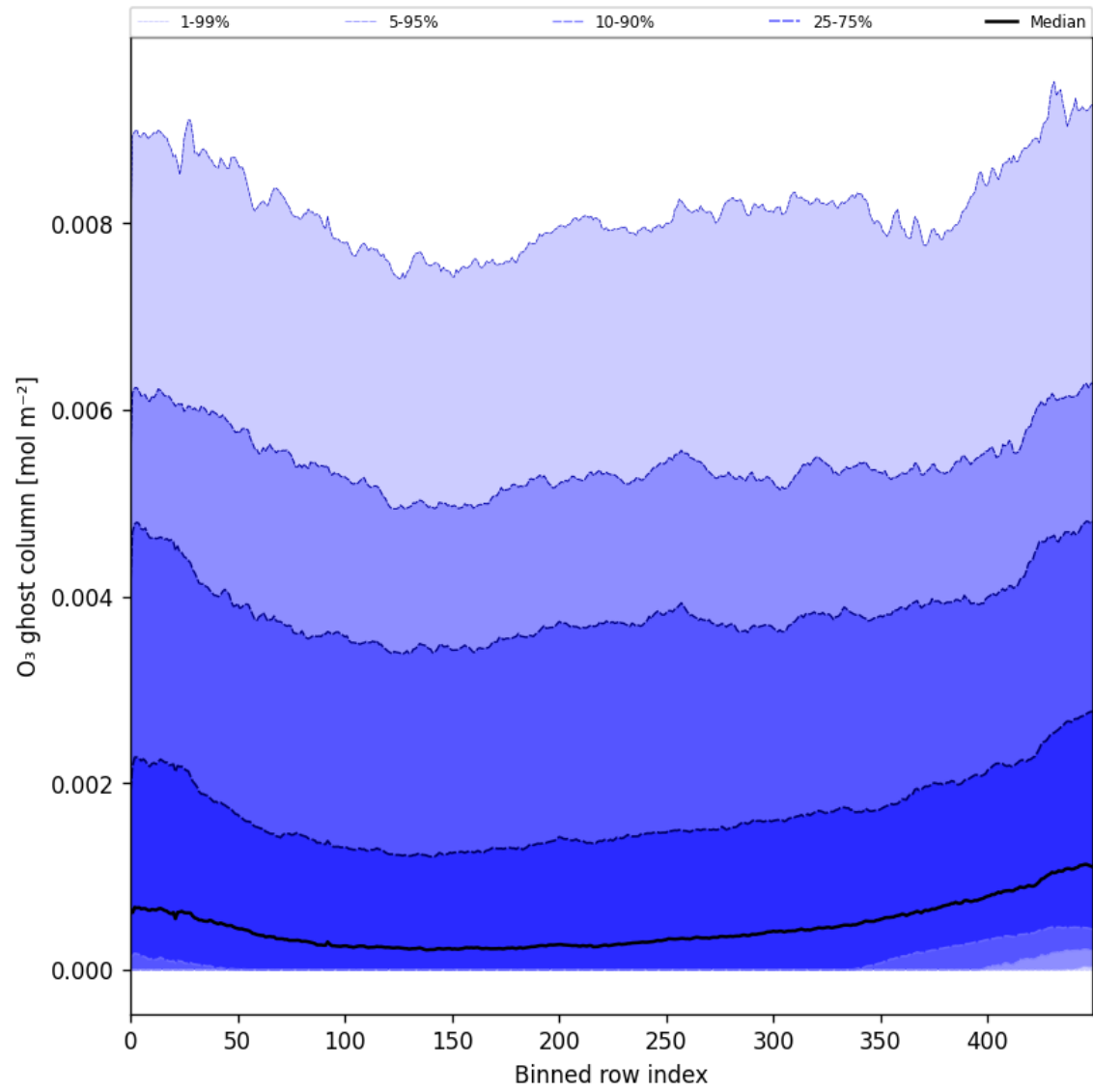
Figure 32: Along track statistics of “O 3 ghost column” for 2025-01-02 to 2025-01-04
