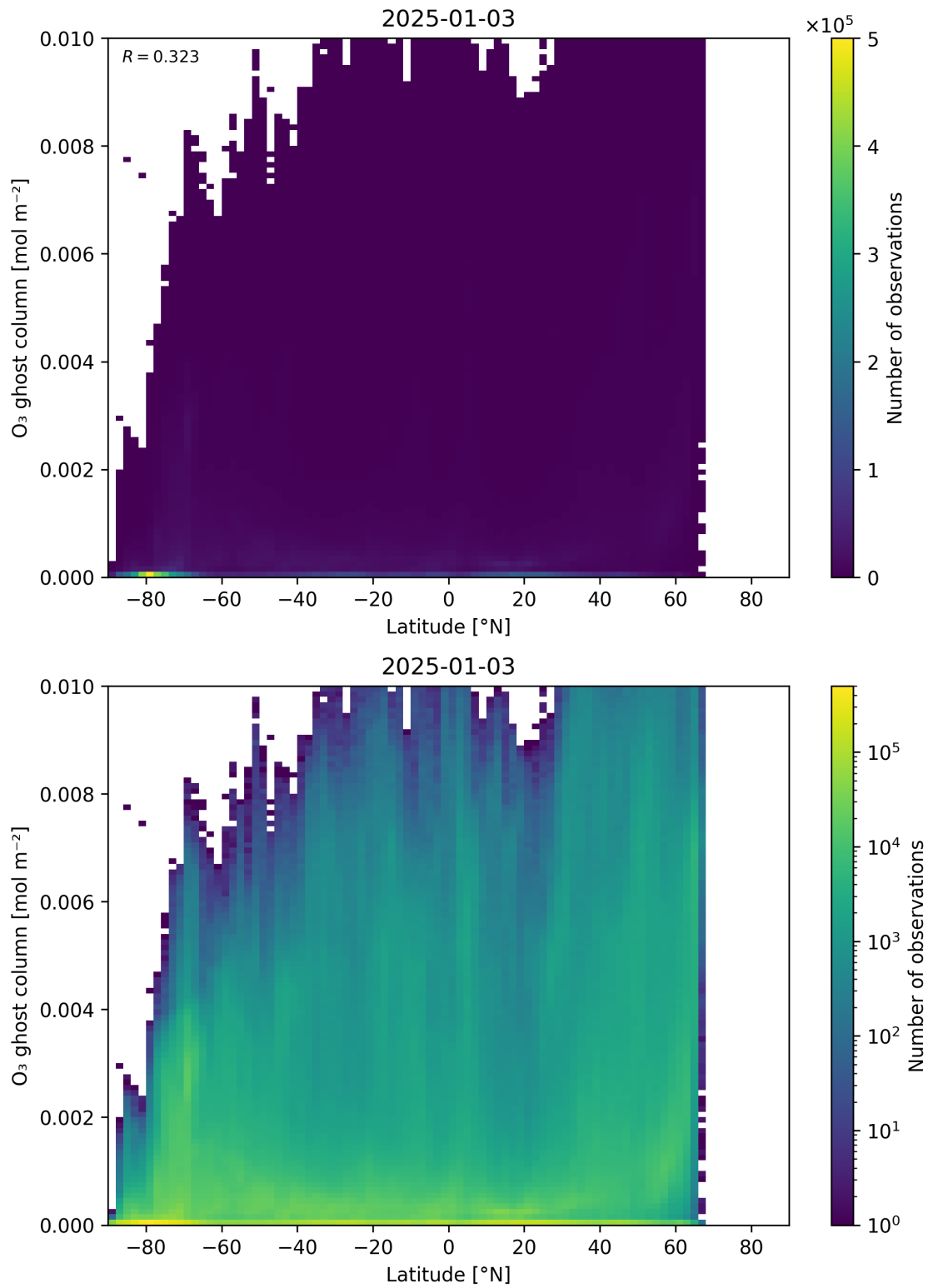
Figure 35: Scatter density plot of “Latitude” against “O 3 ghost column” for 2025-01-02 to 2025-01-04.
