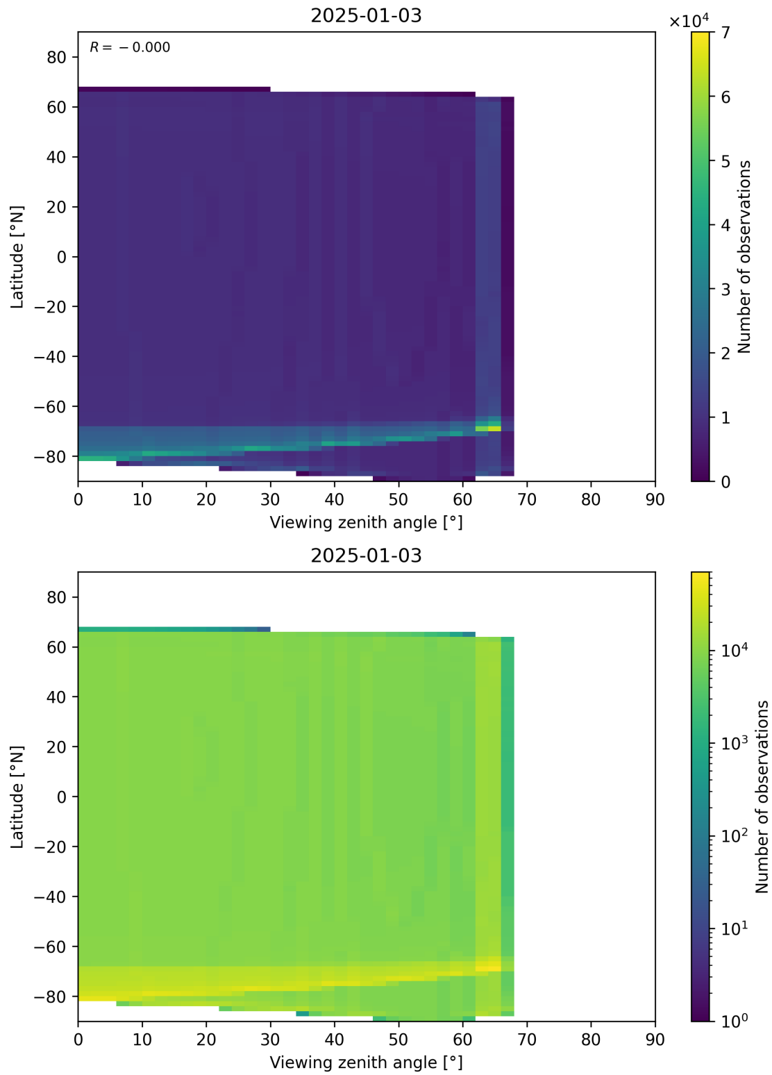
Figure 49: Scatter density plot of “Viewing zenith angle” against “Latitude” for 2025-01-02 to 2025-01-04.
