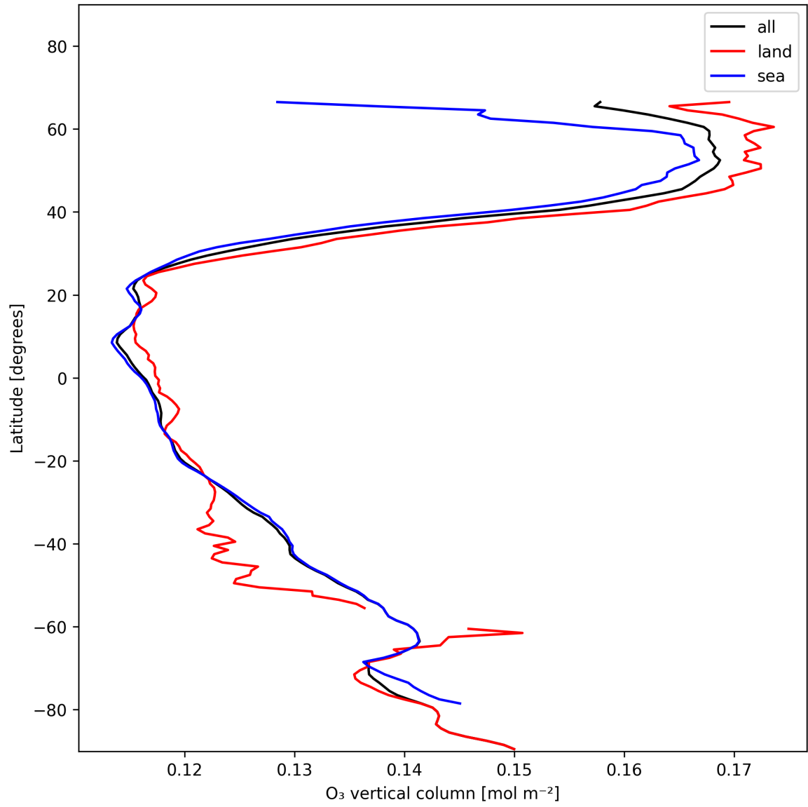
Figure 14: Zonal average of “O 3 vertical column” for 2025-01-02 to 2025-01-04.
