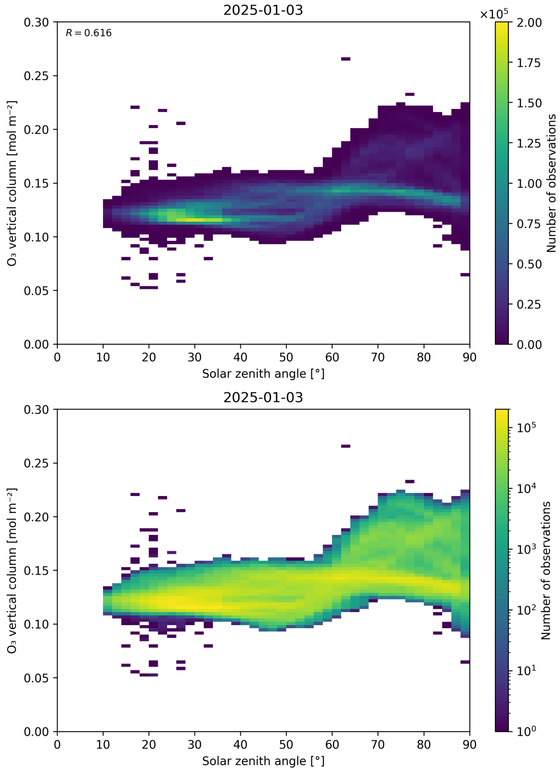
Figure 47: Scatter density plot of “Solar zenith angle” against “O 3 vertical column” for 2025-01-02 to 2025-01-04.
