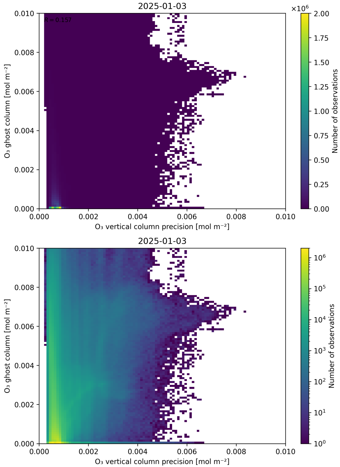
Figure 43: Scatter density plot of “ \text{O}_3 vertical column precision” against “ \text{O}_3 ghost column” for 2025-01-02 to 2025-01-04.
