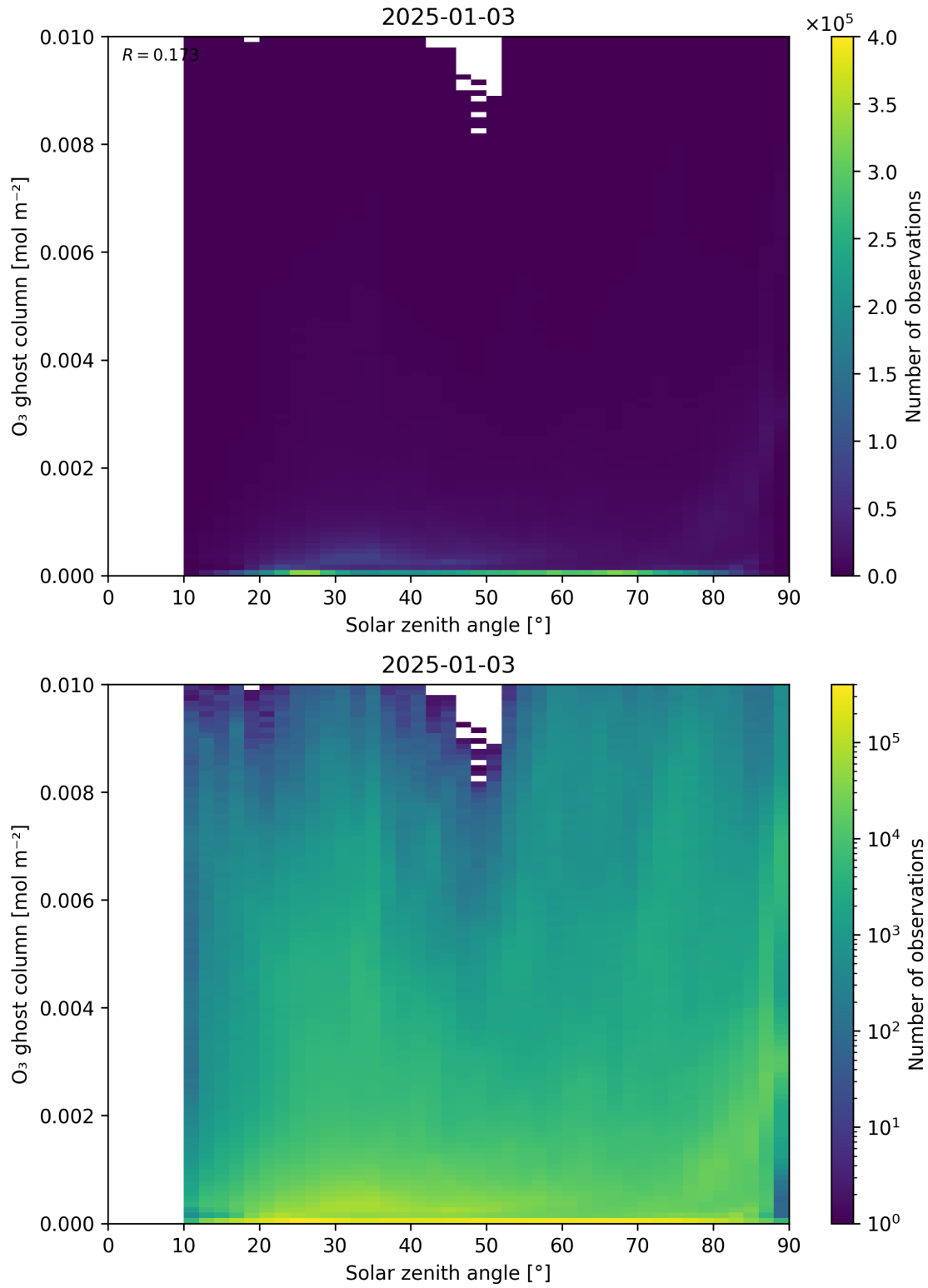
Figure 46: Scatter density plot of “Solar zenith angle” against “O 3 ghost column” for 2025-01-02 to 2025-01-04.
