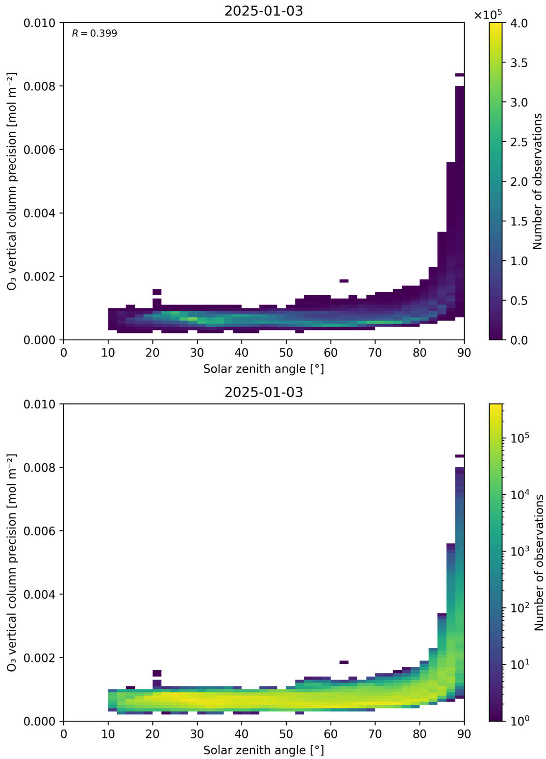
Figure 48: Scatter density plot of “Solar zenith angle” against “O 3 vertical column precision” for 2025-01-02 to 2025-01-04.
