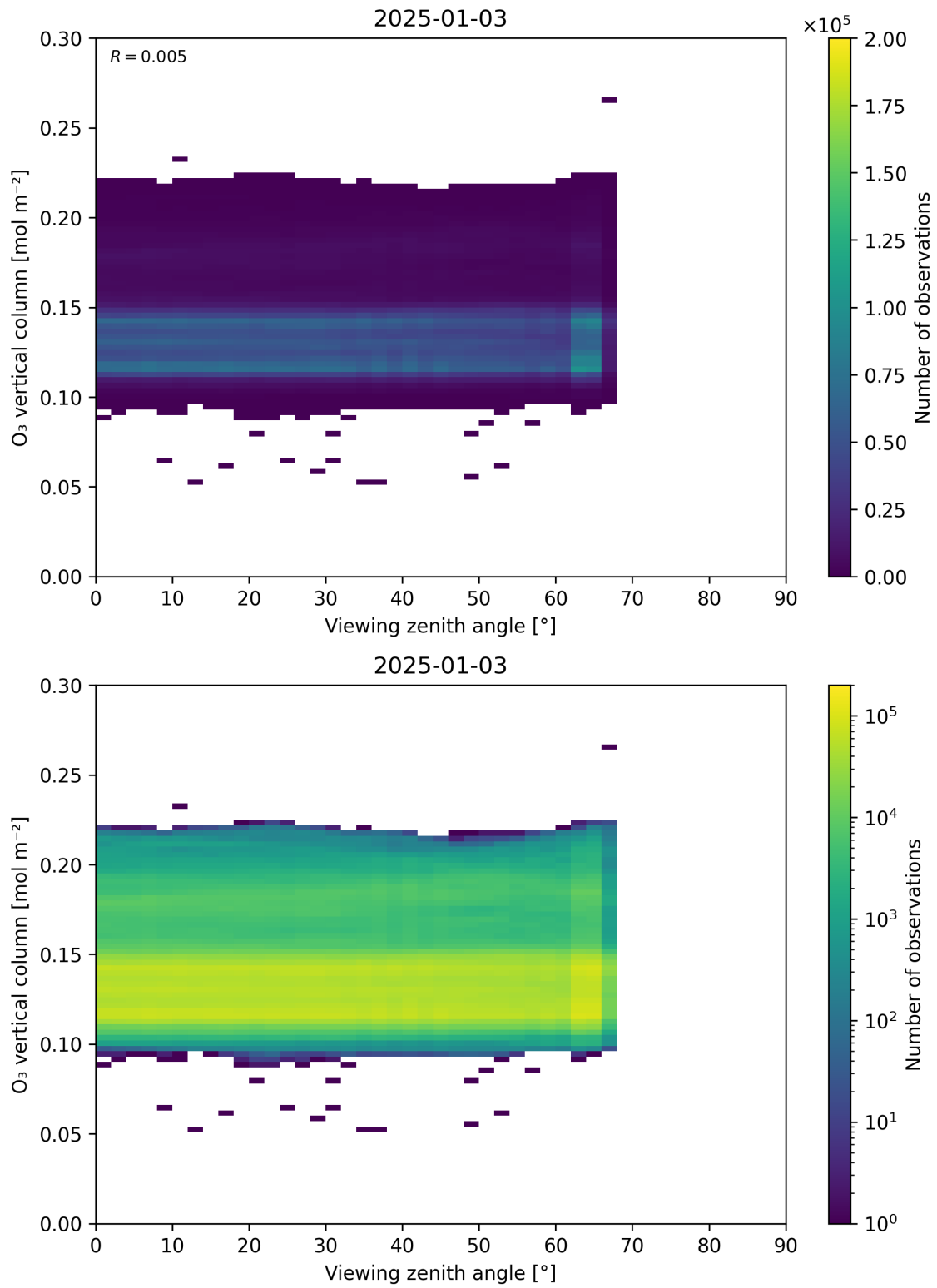
Figure 52: Scatter density plot of “Viewing zenith angle” against “O 3 vertical column” for 2025-01-02 to 2025-01-04.
