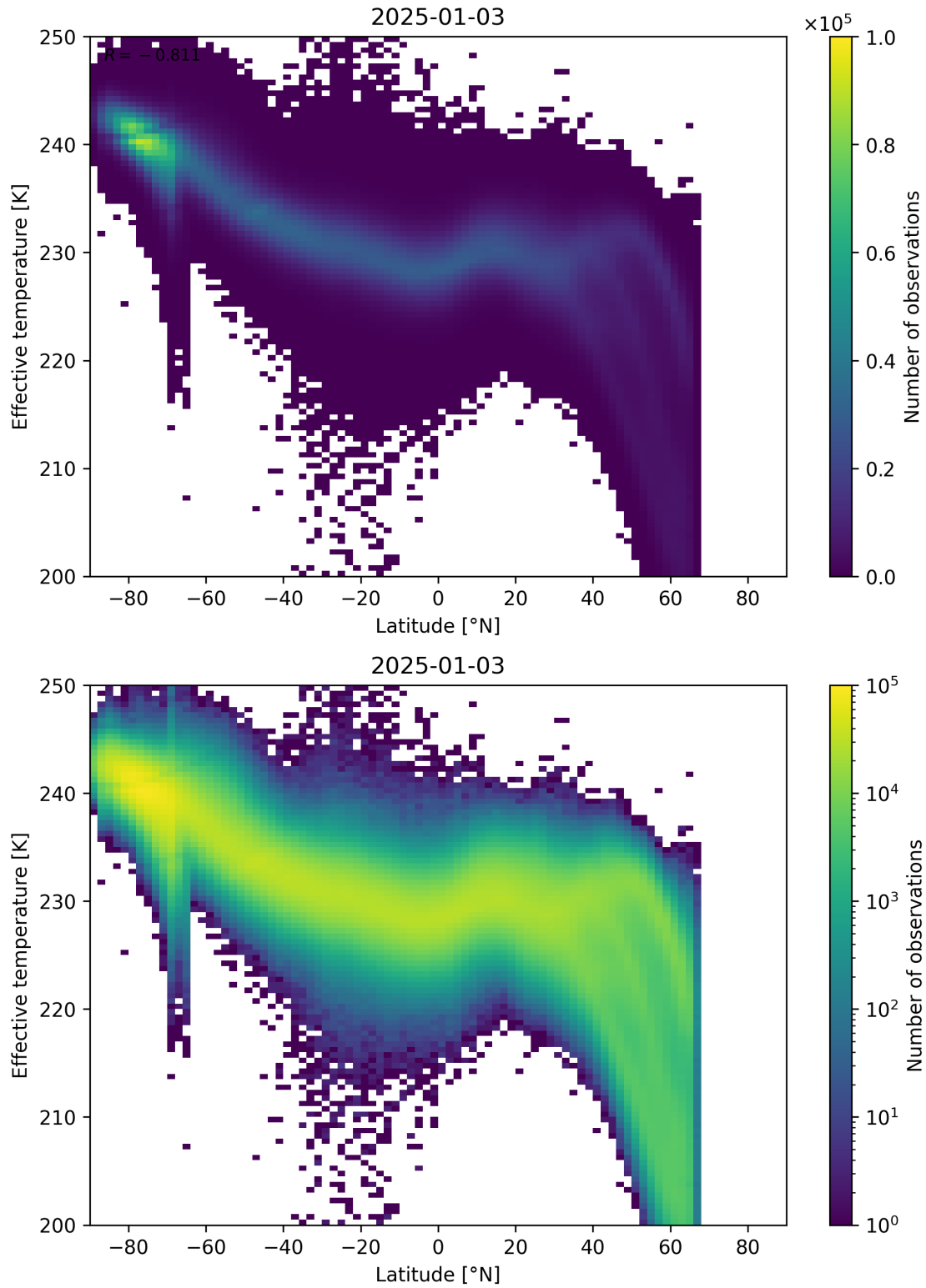
Figure 34: Scatter density plot of “Latitude” against “Effective temperature” for 2025-01-02 to 2025-01-04.
