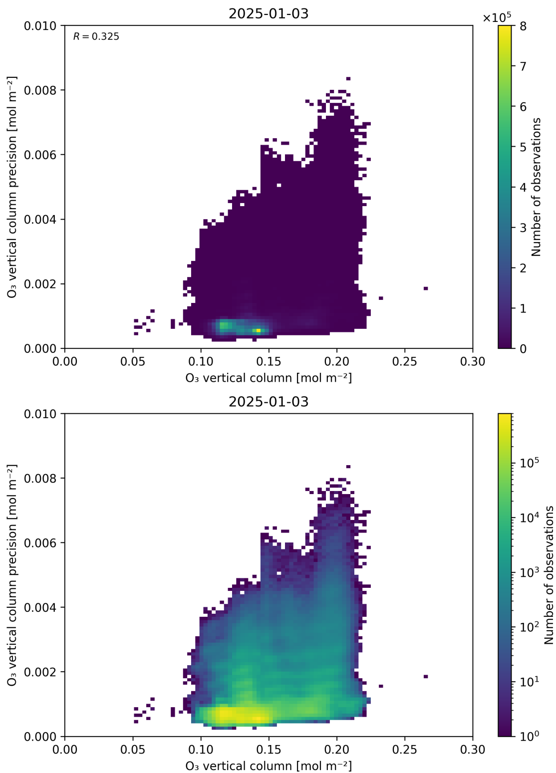
Figure 41: Scatter density plot of “O 3 vertical column” against “O 3 vertical column precision” for 2025-01-02 to 2025-01-04.
