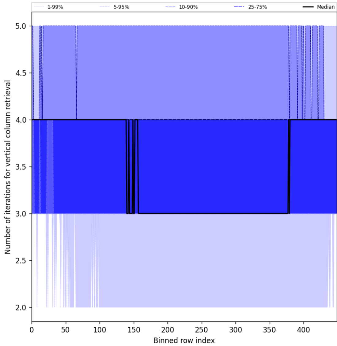
Figure 33: Along track statistics of “Number of iterations for vertical column retrieval” for 2025-01-02 to 2025-01-04
