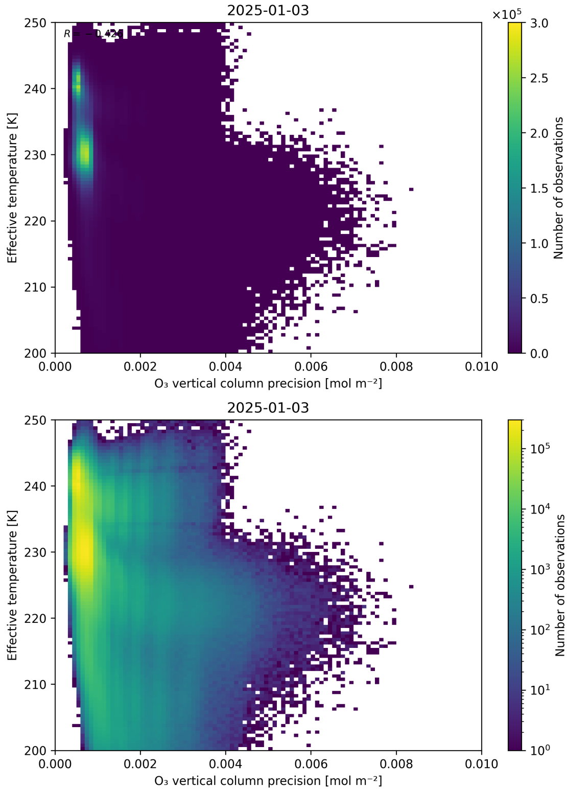
Figure 42: Scatter density plot of “O 3 vertical column precision” against “Effective temperature” for 2025-01-02 to 2025-01-04.
