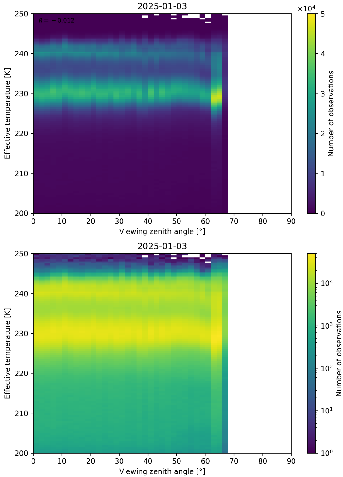
Figure 50: Scatter density plot of “Viewing zenith angle” against “Effective temperature” for 2025-01-02 to 2025-01-04.
