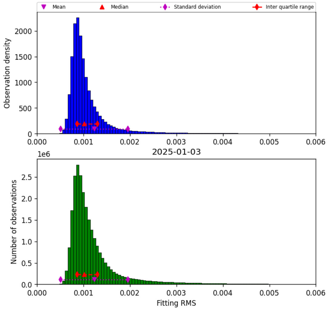
Figure 23: Histogram of “Fitting RMS” for 2025-01-02 to 2025-01-04
