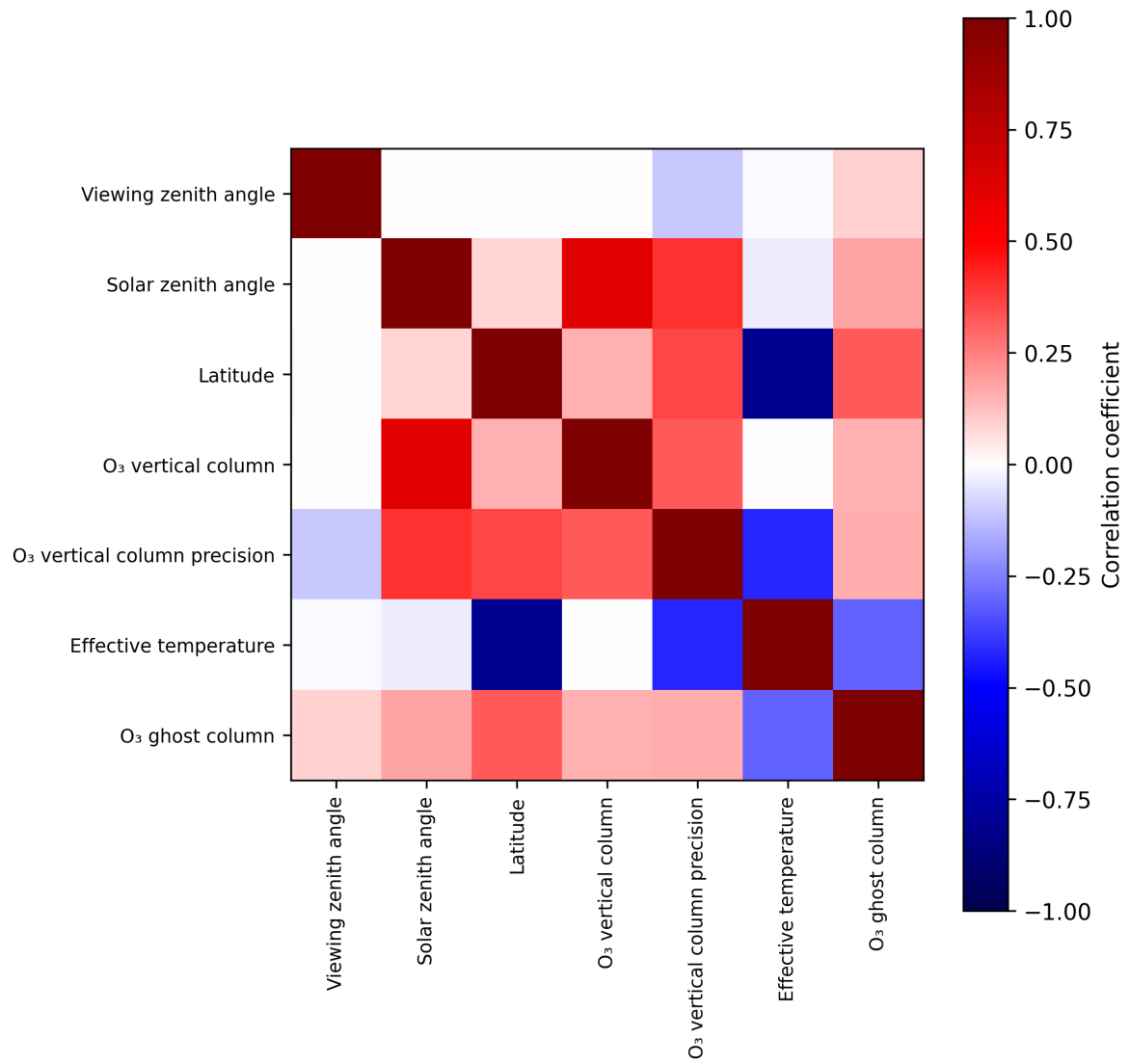
Figure 2: Map of correlation matrix for 2025-01-02 to 2025-01-04.
