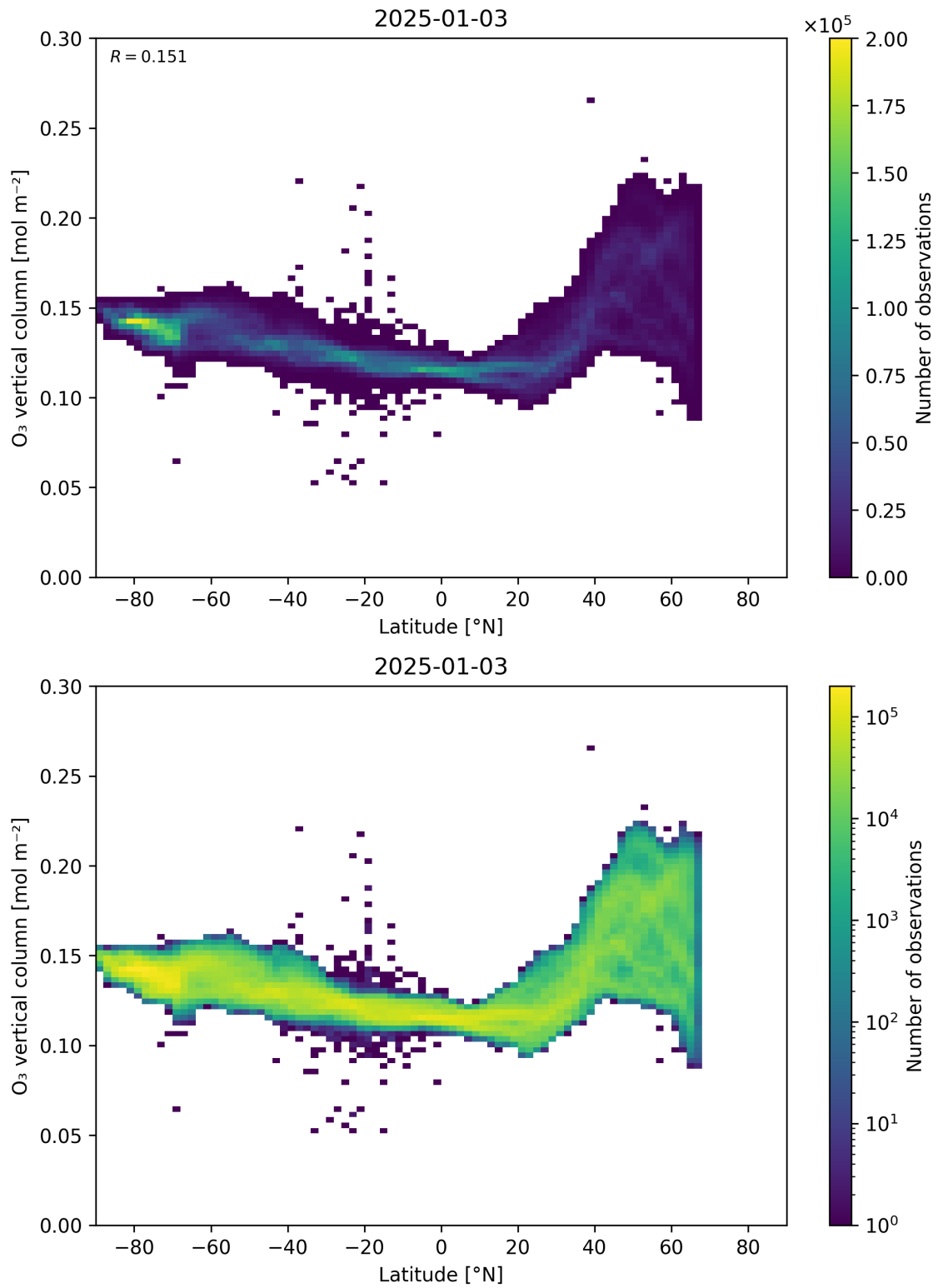
Figure 36: Scatter density plot of “Latitude” against “O 3 vertical column” for 2025-01-02 to 2025-01-04.
