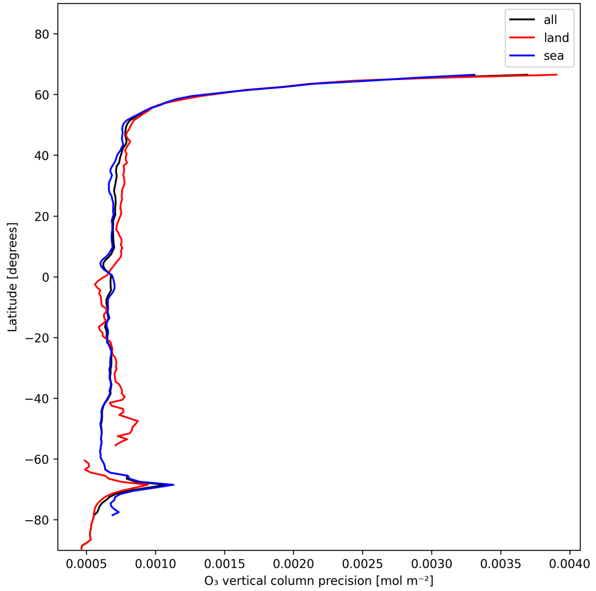
Figure 15: Zonal average of “O 3 vertical column precision” for 2025-01-02 to 2025-01-04.
