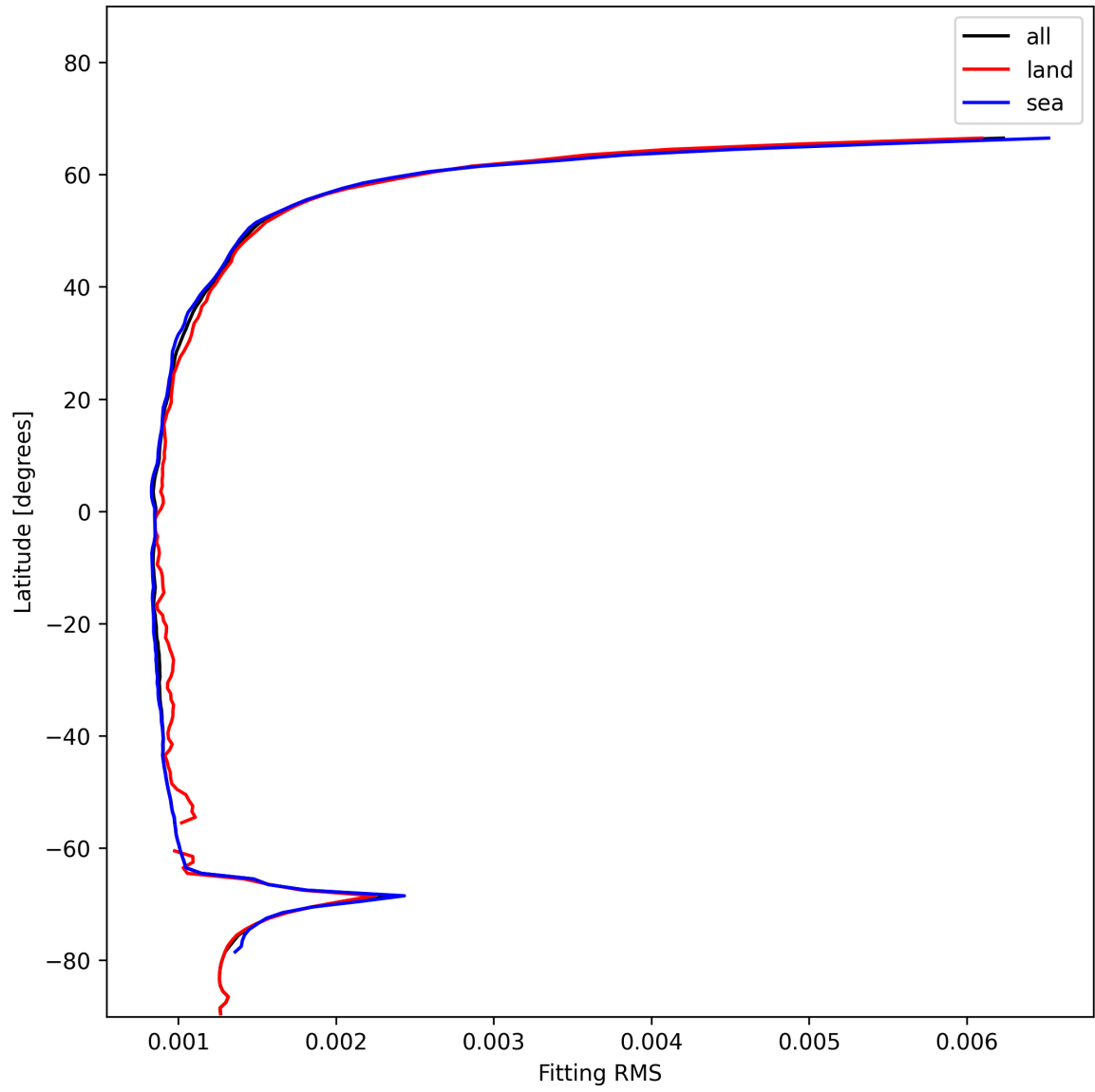
Figure 16: Zonal average of “Fitting RMS” for 2025-01-02 to 2025-01-04.
