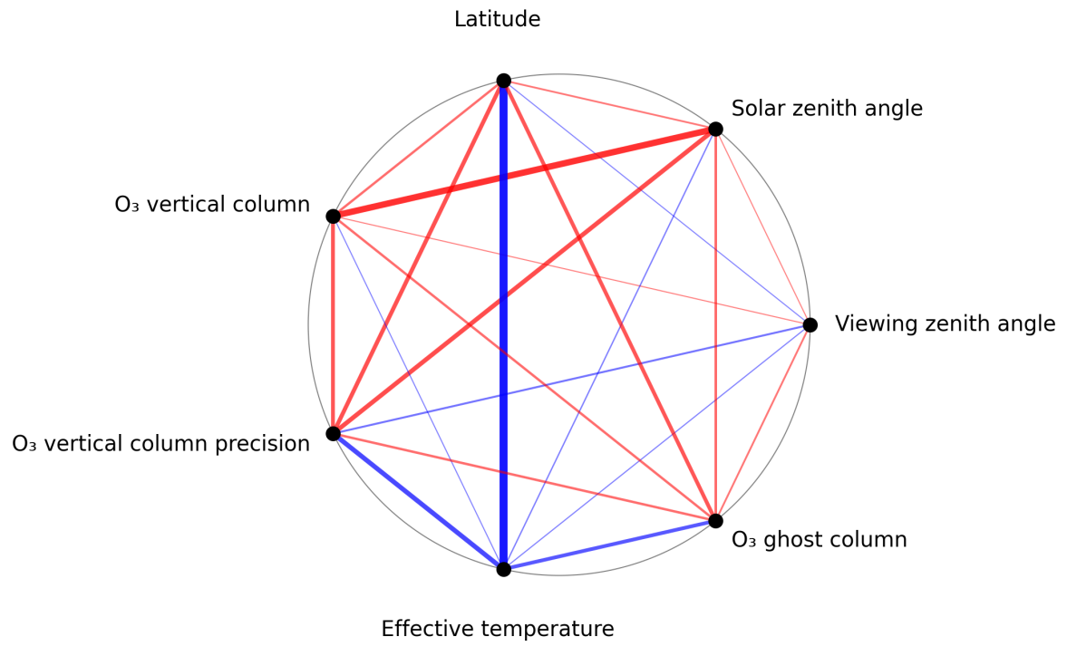
Figure 1: Map of correlation graph for 2025-01-02 to 2025-01-04.
