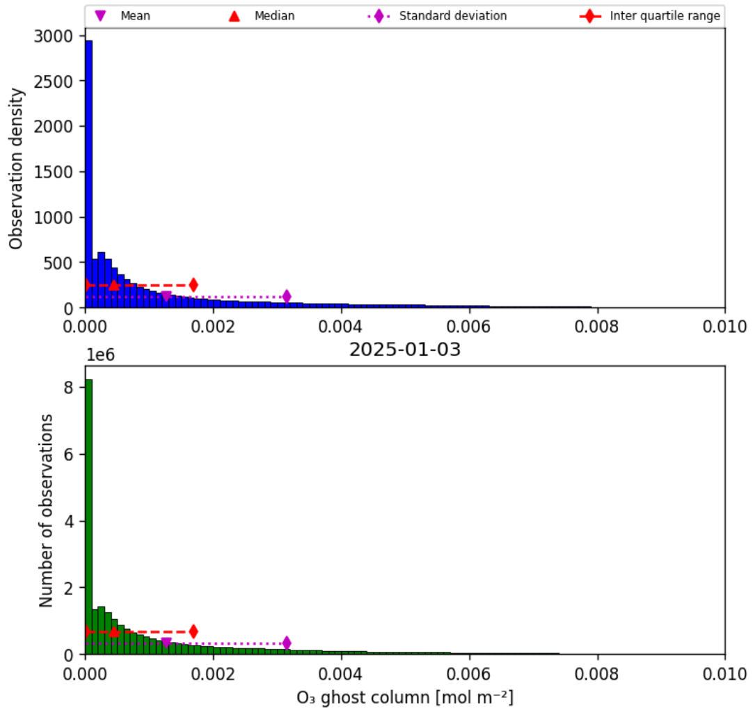
Figure 25: Histogram of “O 3 ghost column” for 2025-01-02 to 2025-01-04
