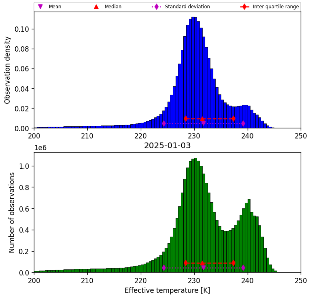
Figure 24: Histogram of “Effective temperature” for 2025-01-02 to 2025-01-04
