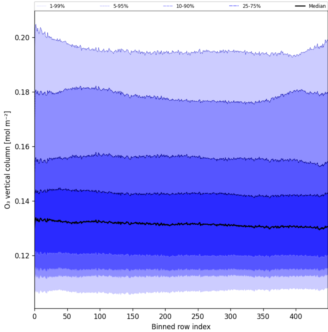
Figure 28: Along track statistics of “O 3 vertical column” for 2025-01-02 to 2025-01-04
