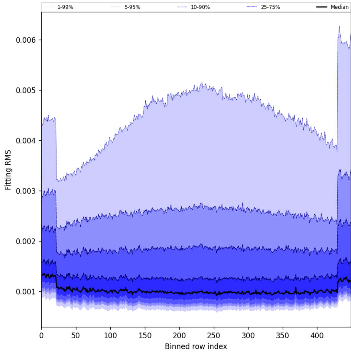
Figure 30: Along track statistics of “Fitting RMS” for 2025-01-02 to 2025-01-04
