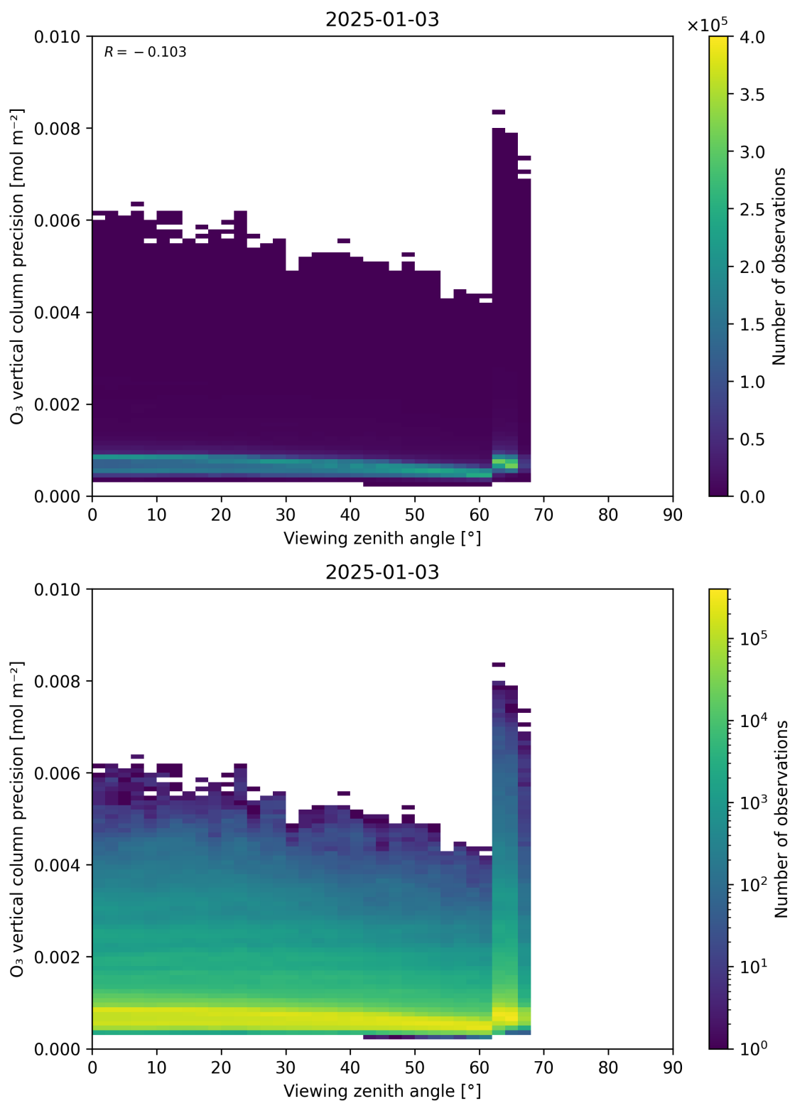
Figure 53: Scatter density plot of “Viewing zenith angle” against “O 3 vertical column precision” for 2025-01-02 to 2025-01-04.
