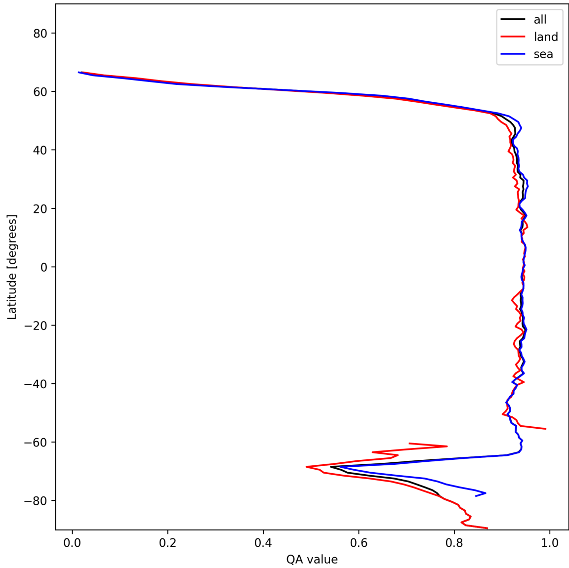
Figure 13: Zonal average of “QA value” for 2025-01-03 to 2025-01-05.
