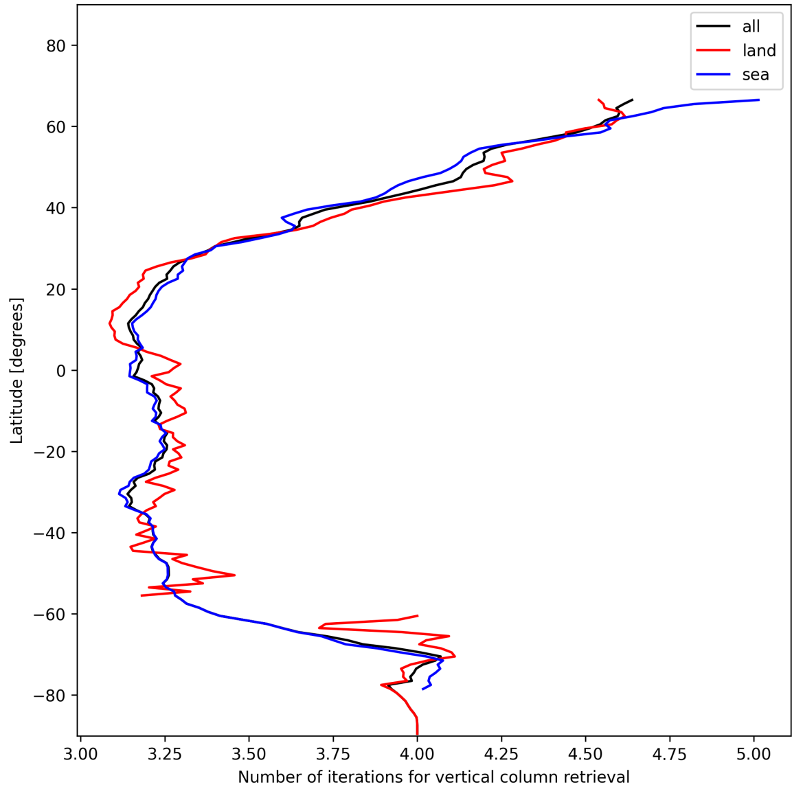
Figure 19: Zonal average of “Number of iterations for vertical column retrieval” for 2025-01-03 to 2025-01-05.
