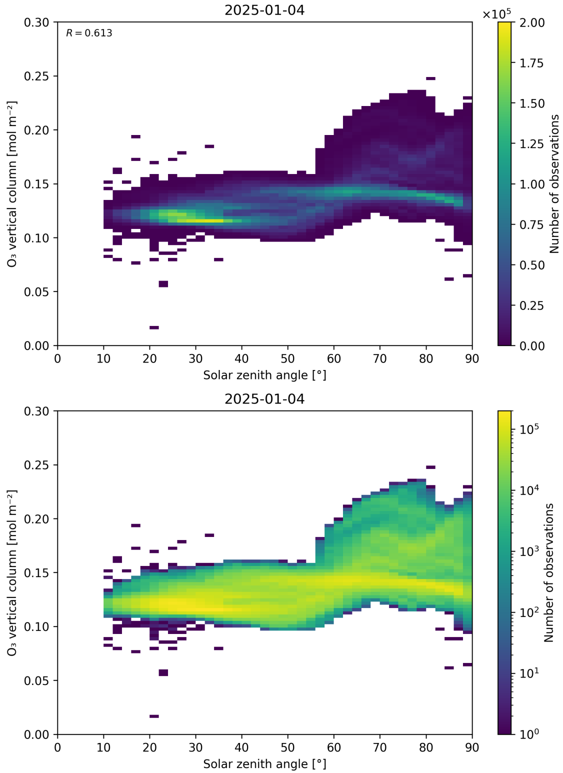
Figure 47: Scatter density plot of “Solar zenith angle” against “O 3 vertical column” for 2025-01-03 to 2025-01-05.
