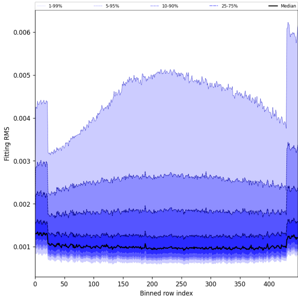
Figure 30: Along track statistics of “Fitting RMS” for 2025-01-03 to 2025-01-05
