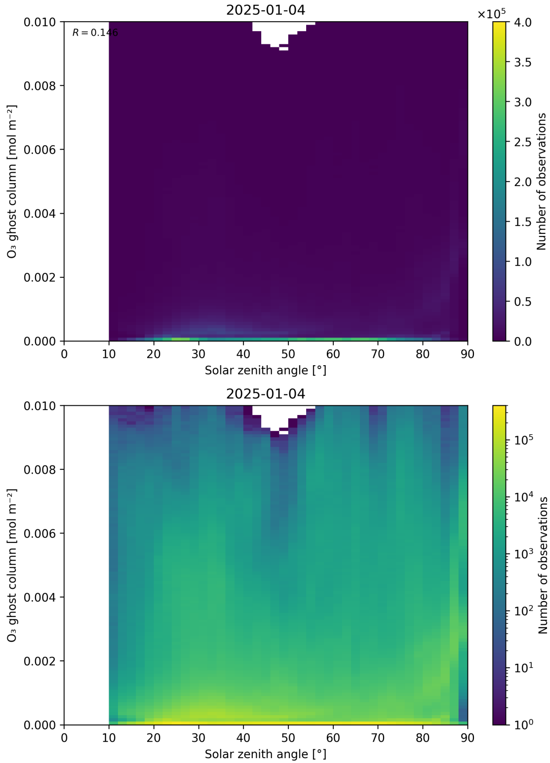
Figure 46: Scatter density plot of “Solar zenith angle” against “O 3 ghost column” for 2025-01-03 to 2025-01-05.
