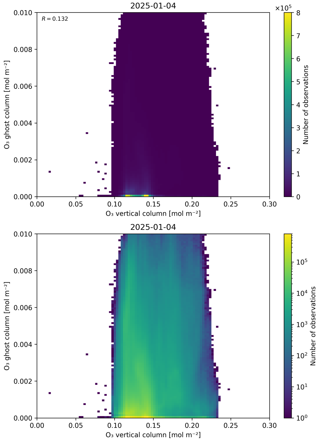
Figure 40: Scatter density plot of “O 3 vertical column” against “O 3 ghost column” for 2025-01-03 to 2025-01-05.
