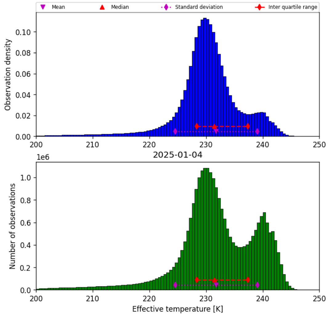
Figure 24: Histogram of “Effective temperature” for 2025-01-03 to 2025-01-05
