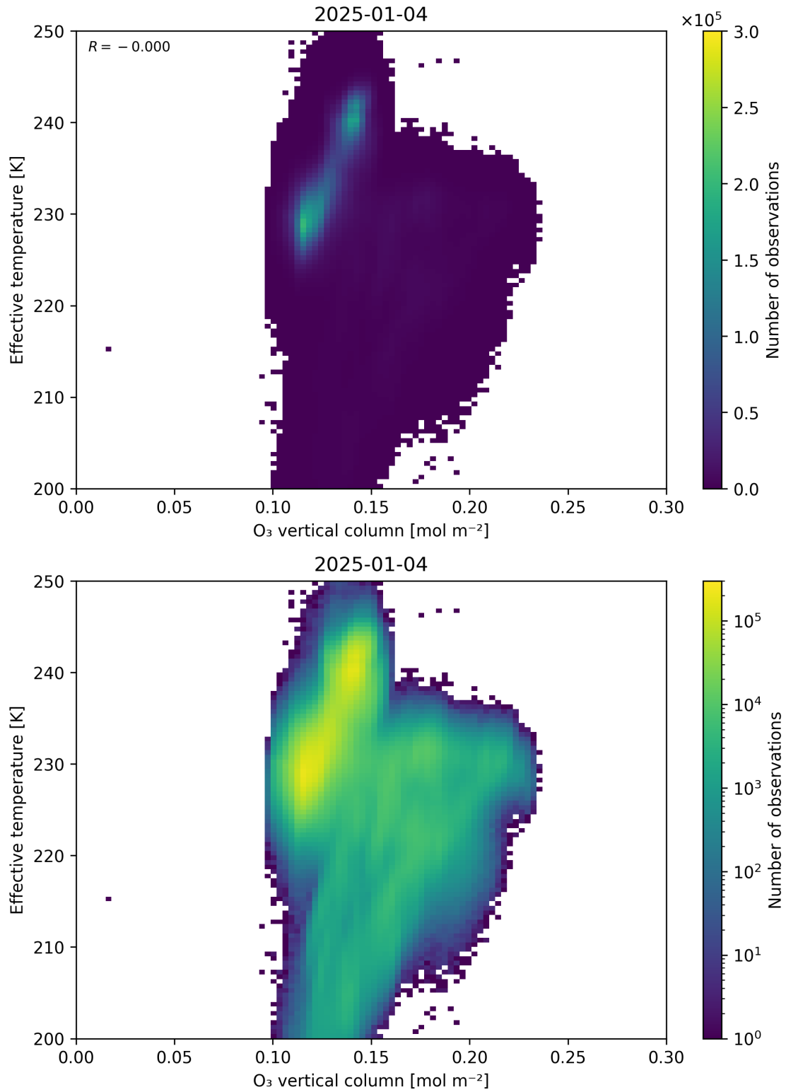
Figure 39: Scatter density plot of “O 3 vertical column” against “Effective temperature” for 2025-01-03 to 2025-01-05.
