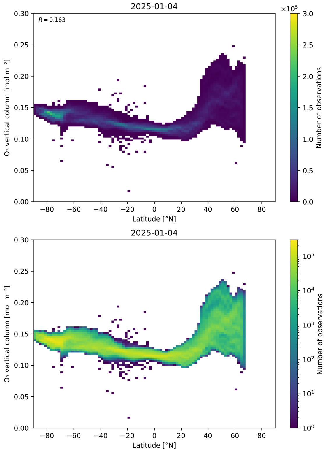
Figure 36: Scatter density plot of “Latitude” against “O 3 vertical column” for 2025-01-03 to 2025-01-05.
