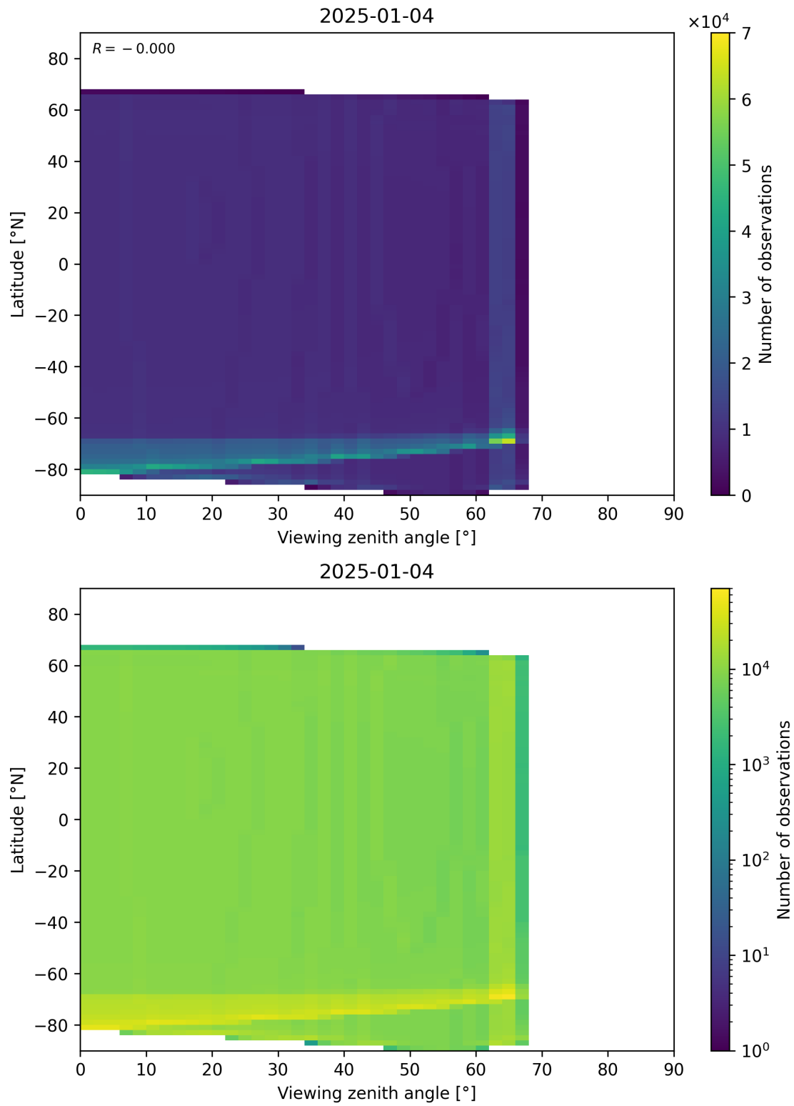
Figure 49: Scatter density plot of “Viewing zenith angle” against “Latitude” for 2025-01-03 to 2025-01-05.
