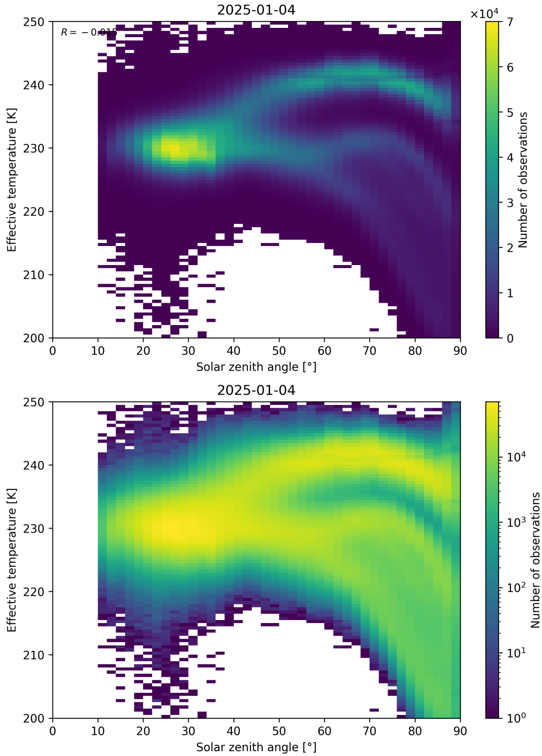
Figure 45: Scatter density plot of “Solar zenith angle” against “Effective temperature” for 2025-01-03 to 2025-01-05.
