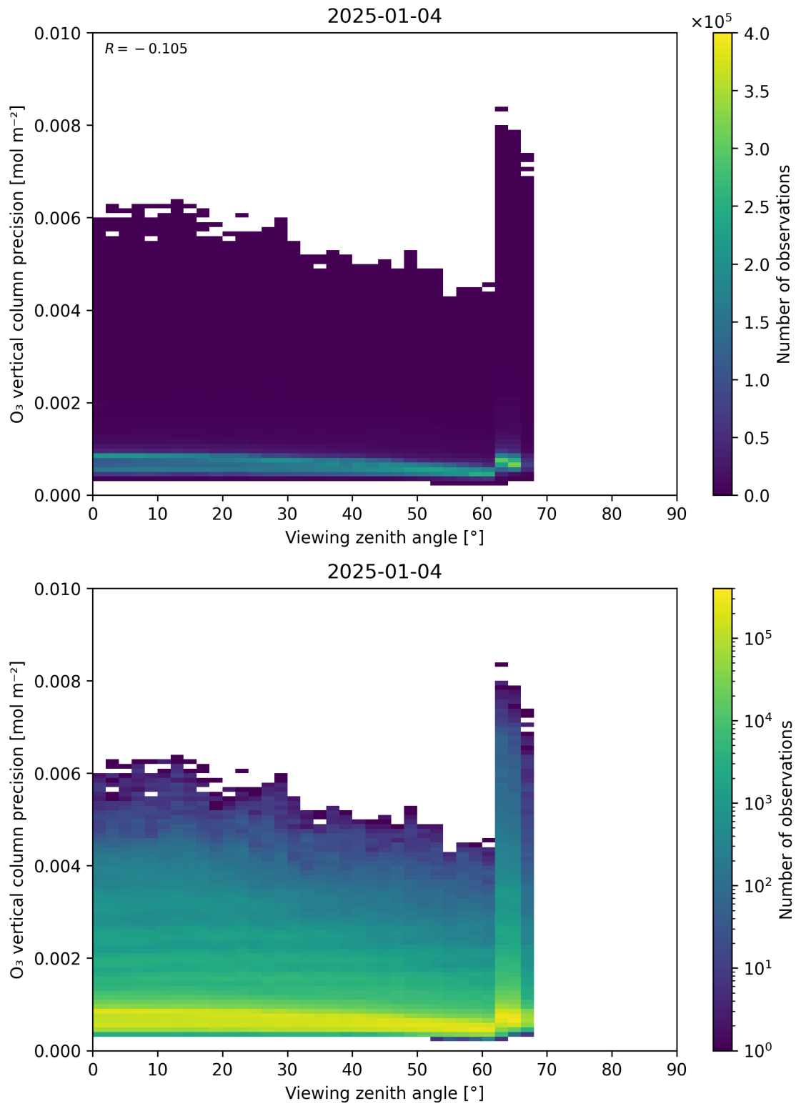
Figure 53: Scatter density plot of “Viewing zenith angle” against “O 3 vertical column precision” for 2025-01-03 to 2025-01-05.
