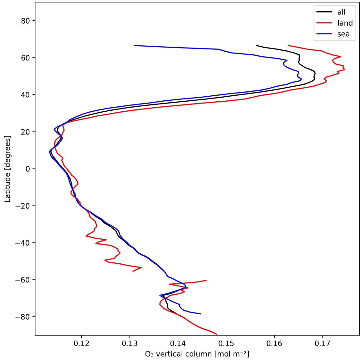
Figure 14: Zonal average of “O 3 vertical column” for 2025-01-03 to 2025-01-05.
