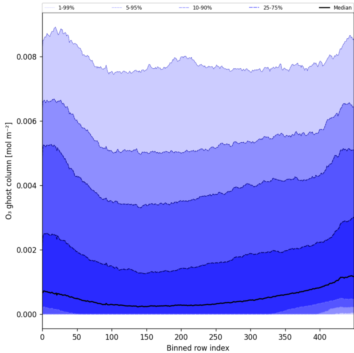
Figure 32: Along track statistics of “O 3 ghost column” for 2025-01-03 to 2025-01-05
