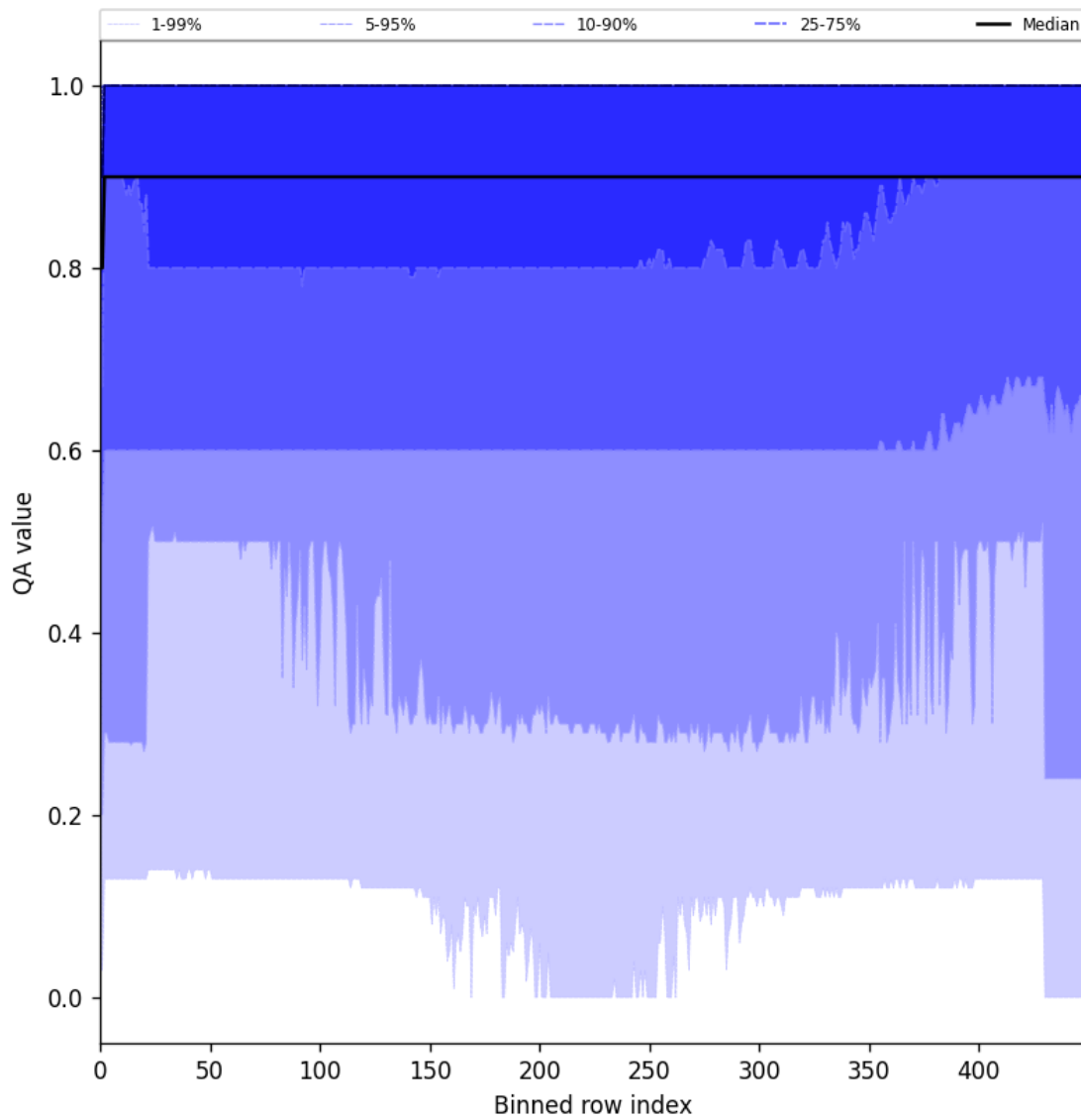
Figure 27: Along track statistics of “QA value” for 2025-01-03 to 2025-01-05
