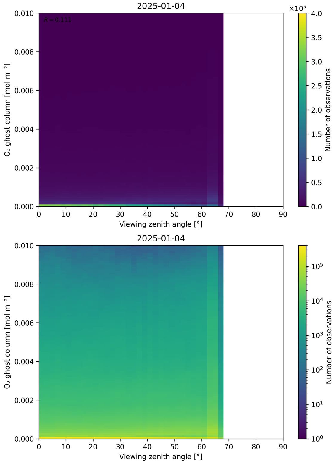
Figure 51: Scatter density plot of “Viewing zenith angle” against “O 3 ghost column” for 2025-01-03 to 2025-01-05.
