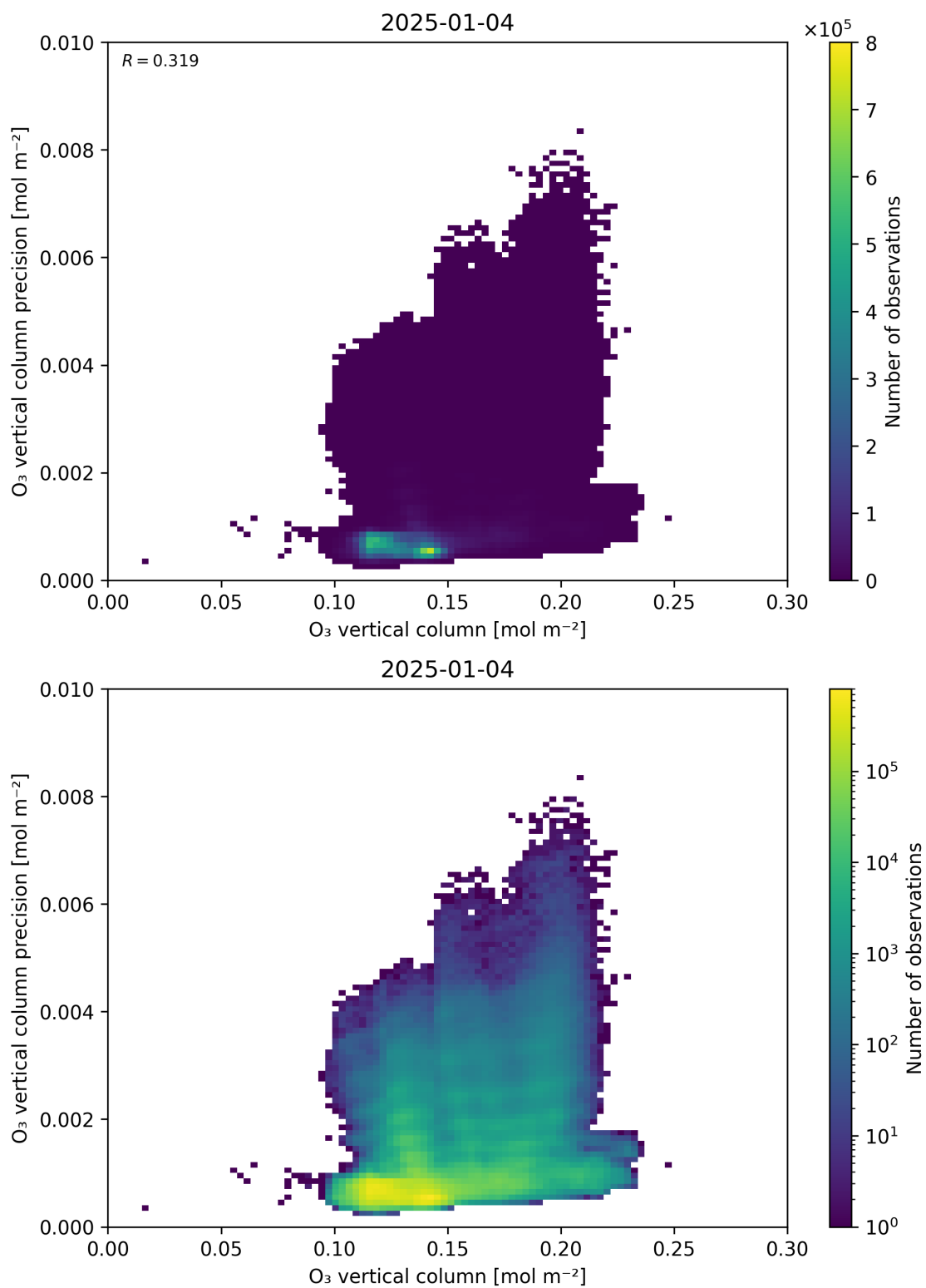
Figure 41: Scatter density plot of “O 3 vertical column” against “O 3 vertical column precision” for 2025-01-03 to 2025-01-05.
