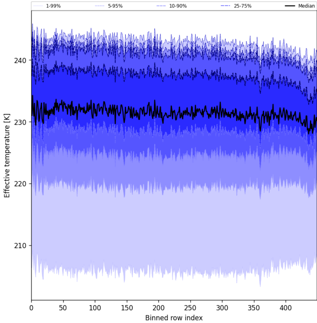
Figure 31: Along track statistics of “Effective temperature” for 2025-01-03 to 2025-01-05
