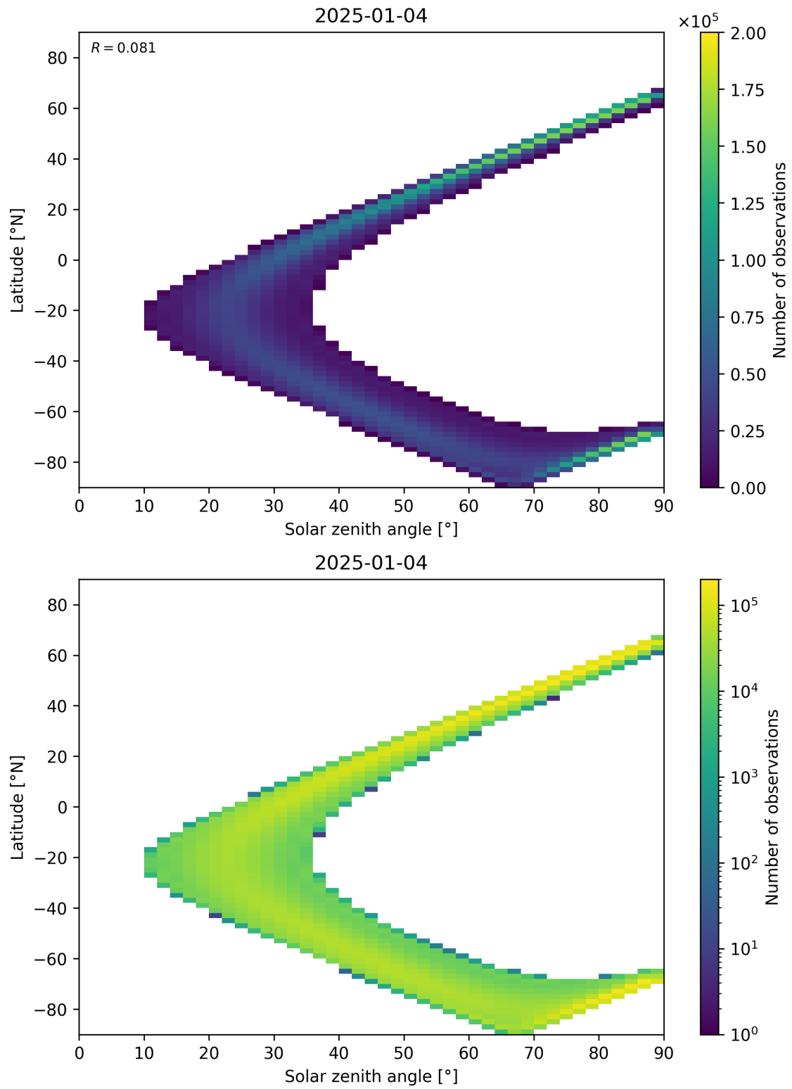
Figure 44: Scatter density plot of “Solar zenith angle” against “Latitude” for 2025-01-03 to 2025-01-05.
