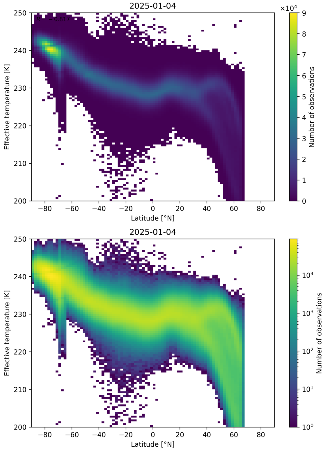
Figure 34: Scatter density plot of “Latitude” against “Effective temperature” for 2025-01-03 to 2025-01-05.
