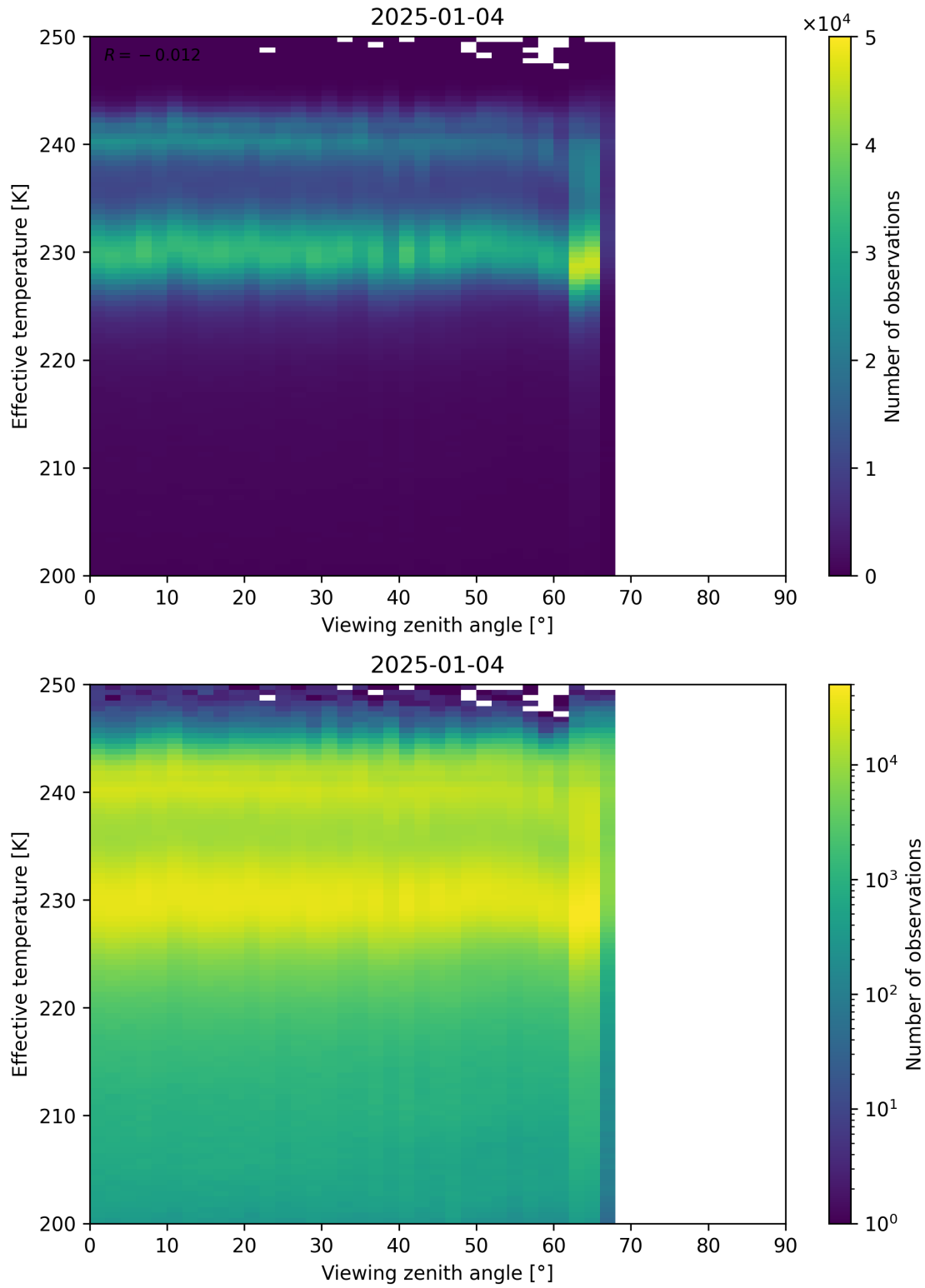
Figure 50: Scatter density plot of “Viewing zenith angle” against “Effective temperature” for 2025-01-03 to 2025-01-05.
