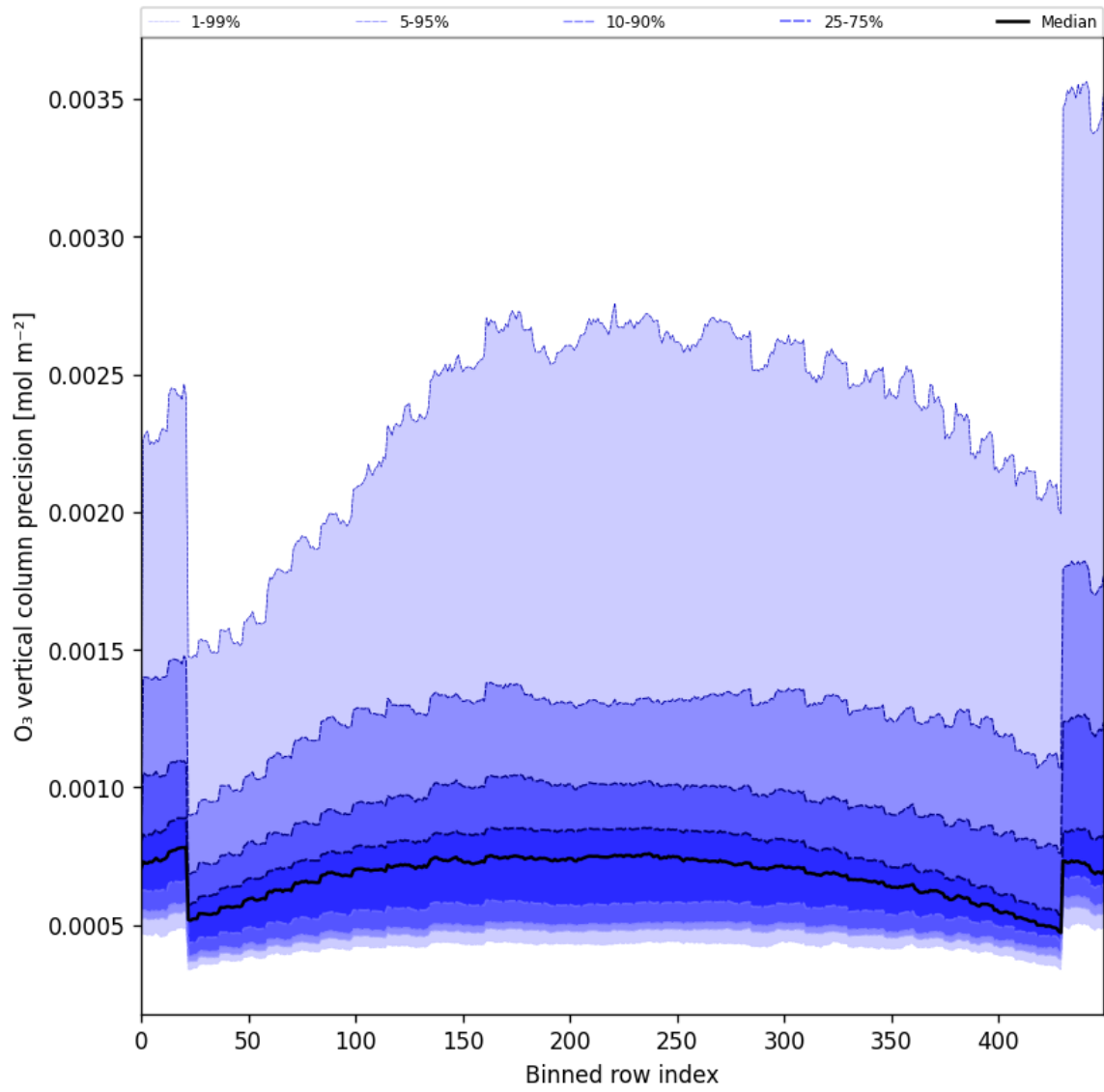
Figure 29: Along track statistics of “O 3 vertical column precision” for 2025-01-03 to 2025-01-05
