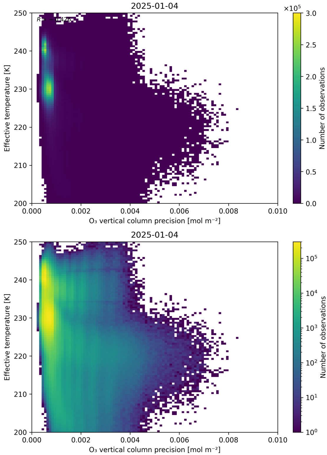
Figure 42: Scatter density plot of “O 3 vertical column precision” against “Effective temperature” for 2025-01-03 to 2025-01-05.
