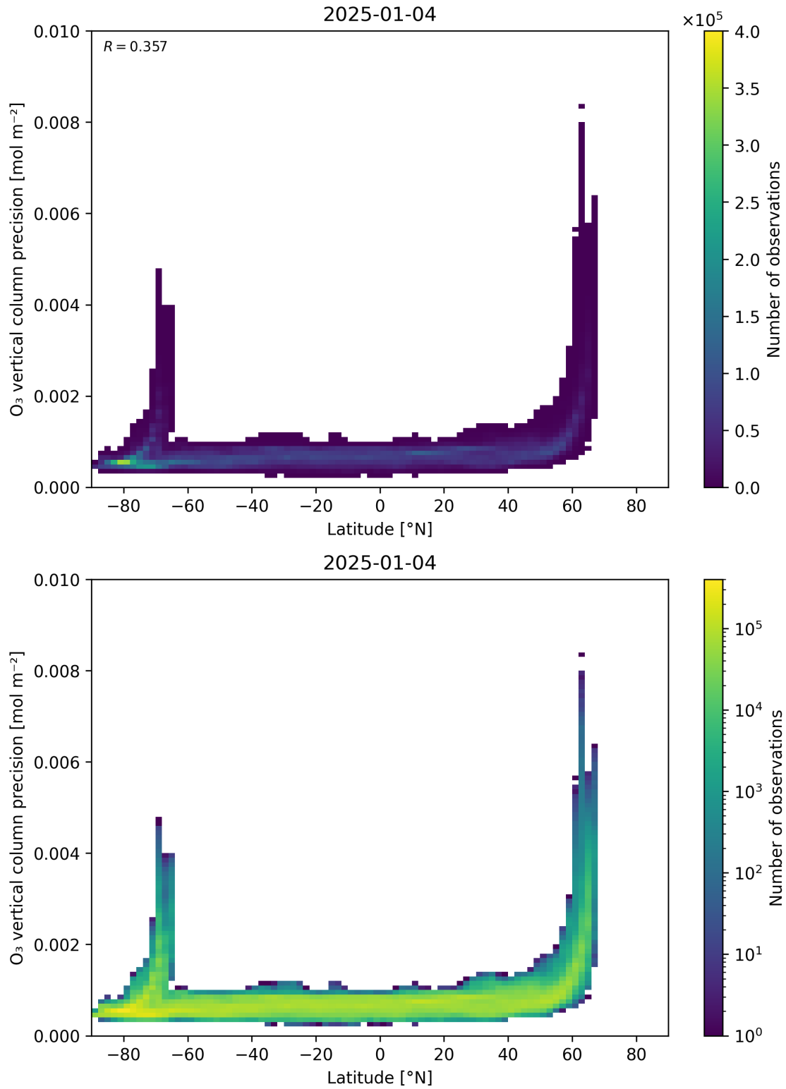
Figure 37: Scatter density plot of “Latitude” against “O 3 vertical column precision” for 2025-01-03 to 2025-01-05.
