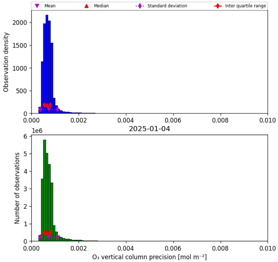
Figure 22: Histogram of “O 3 vertical column precision” for 2025-01-03 to 2025-01-05
