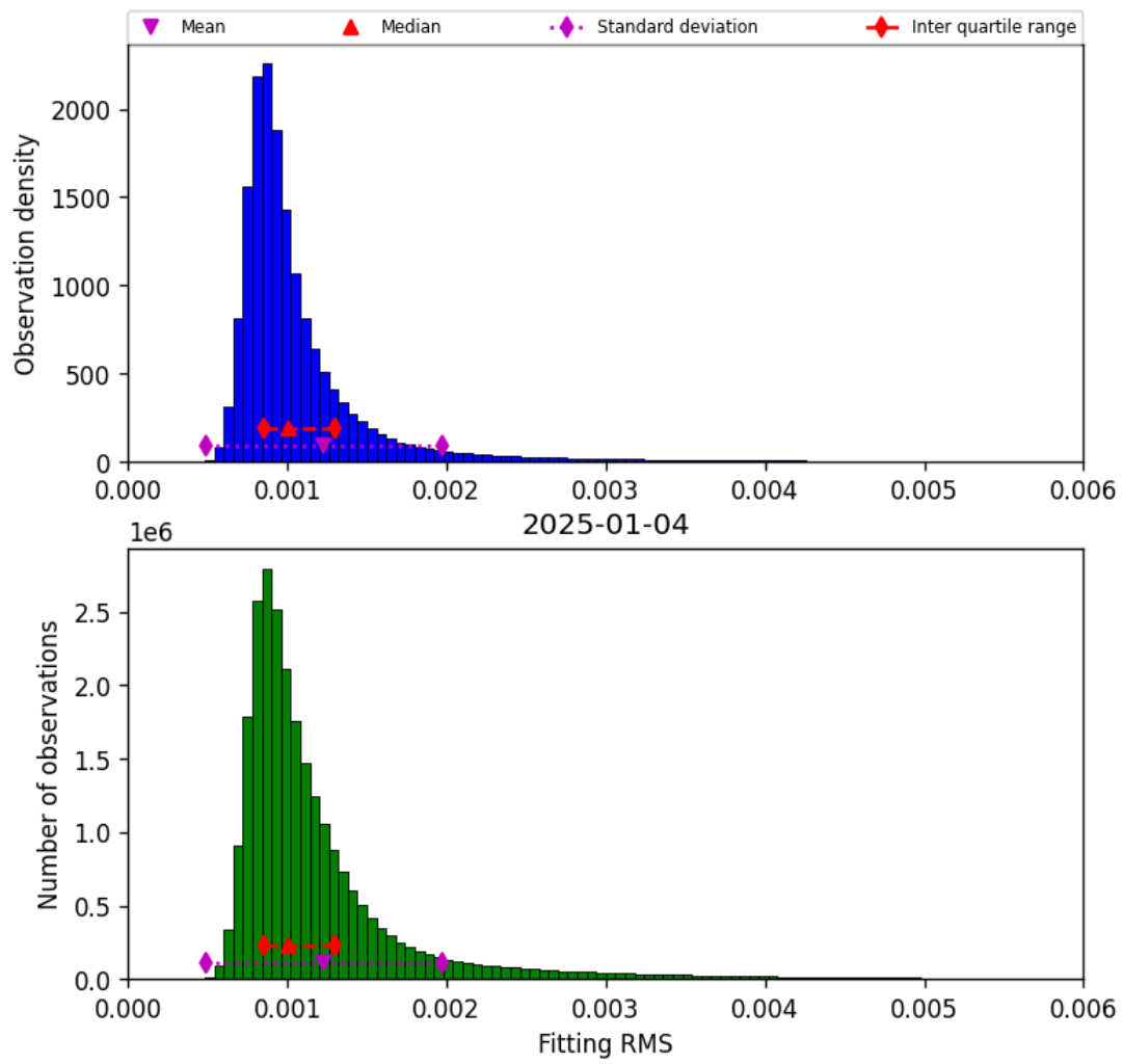
Figure 23: Histogram of “Fitting RMS” for 2025-01-03 to 2025-01-05
