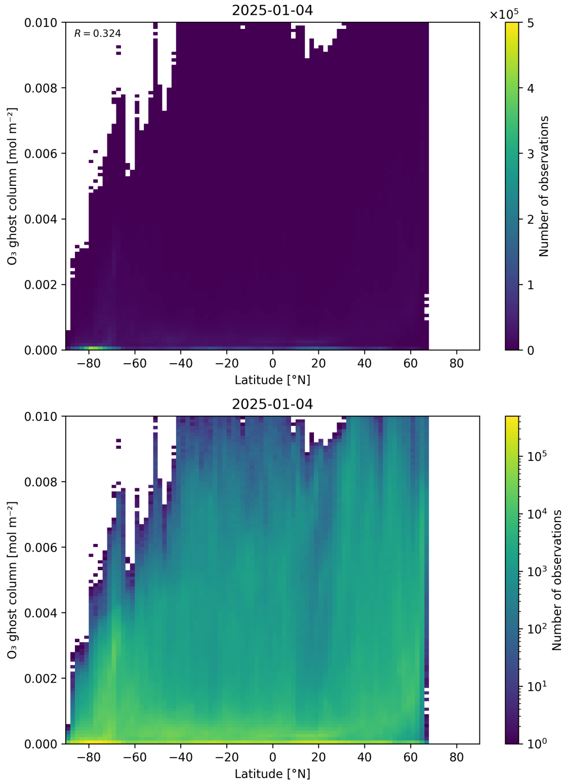
Figure 35: Scatter density plot of “Latitude” against “O 3 ghost column” for 2025-01-03 to 2025-01-05.
