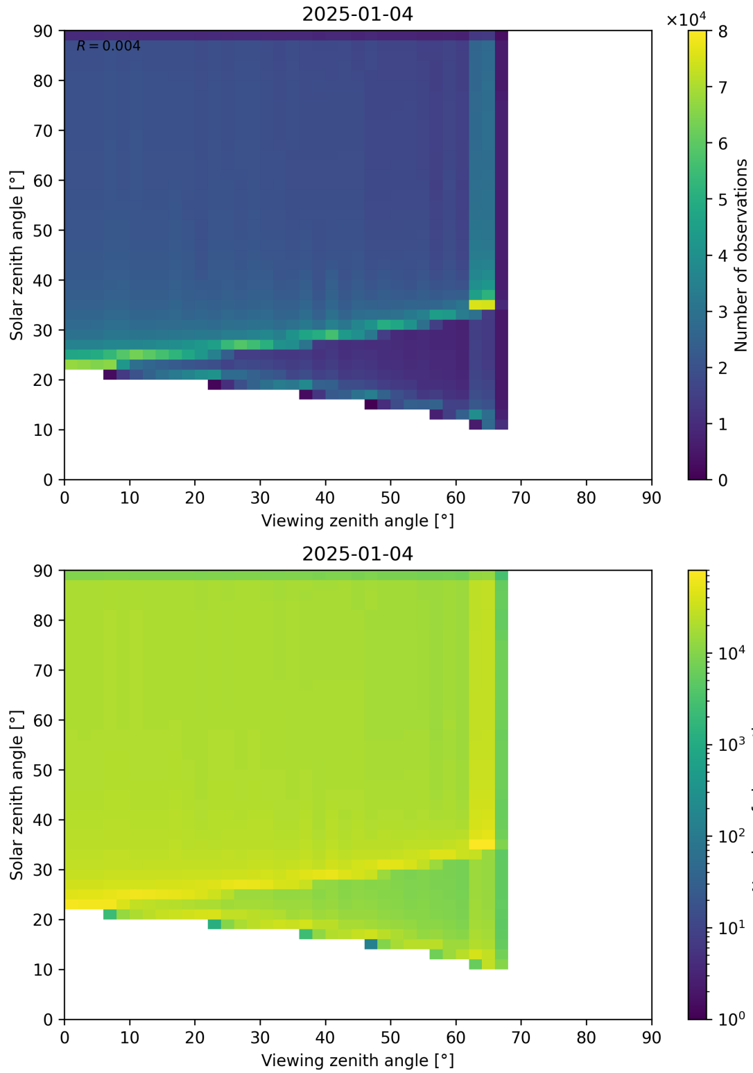
Figure 54: Scatter density plot of “Viewing zenith angle” against “Solar zenith angle” for 2025-01-03 to 2025-01-05.
