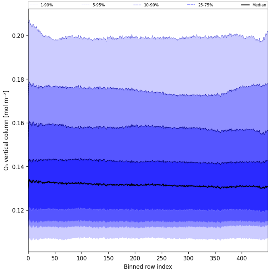
Figure 28: Along track statistics of “O 3 vertical column” for 2025-01-03 to 2025-01-05
