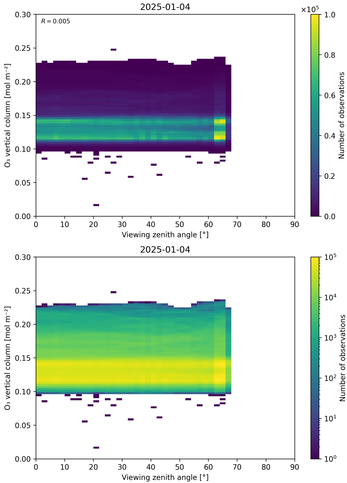
Figure 52: Scatter density plot of “Viewing zenith angle” against “O 3 vertical column” for 2025-01-03 to 2025-01-05.
