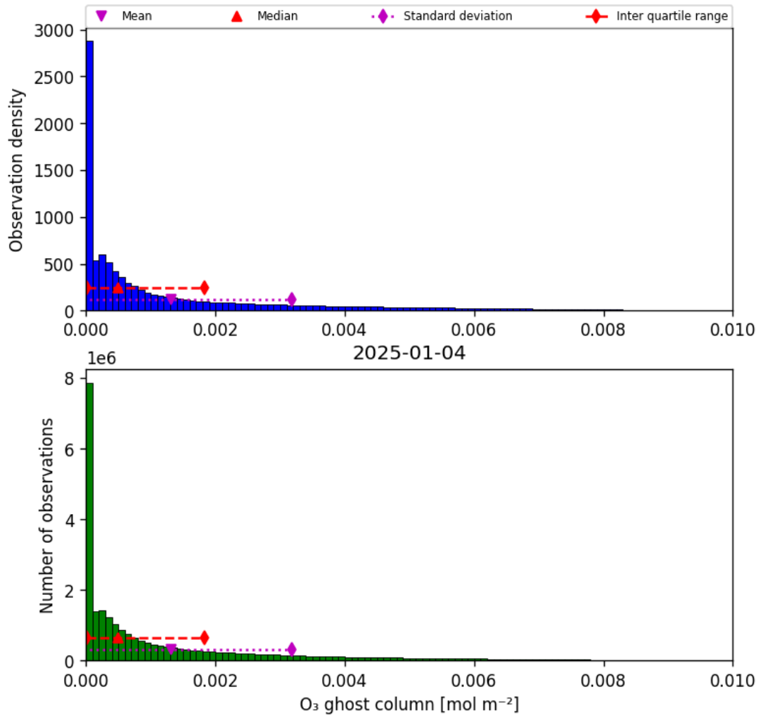
Figure 25: Histogram of “O 3 ghost column” for 2025-01-03 to 2025-01-05
