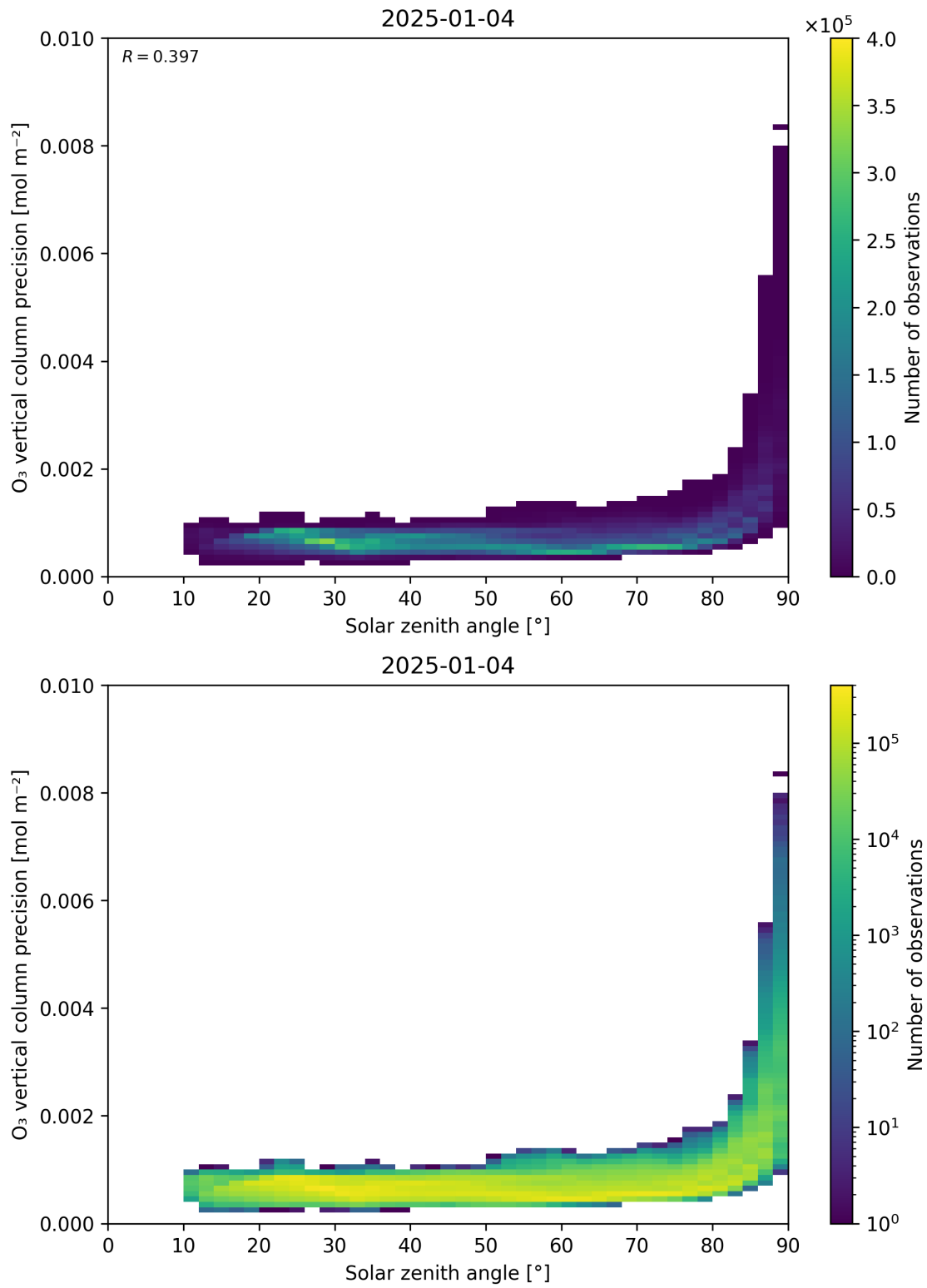
Figure 48: Scatter density plot of “Solar zenith angle” against “O 3 vertical column precision” for 2025-01-03 to 2025-01-05.
