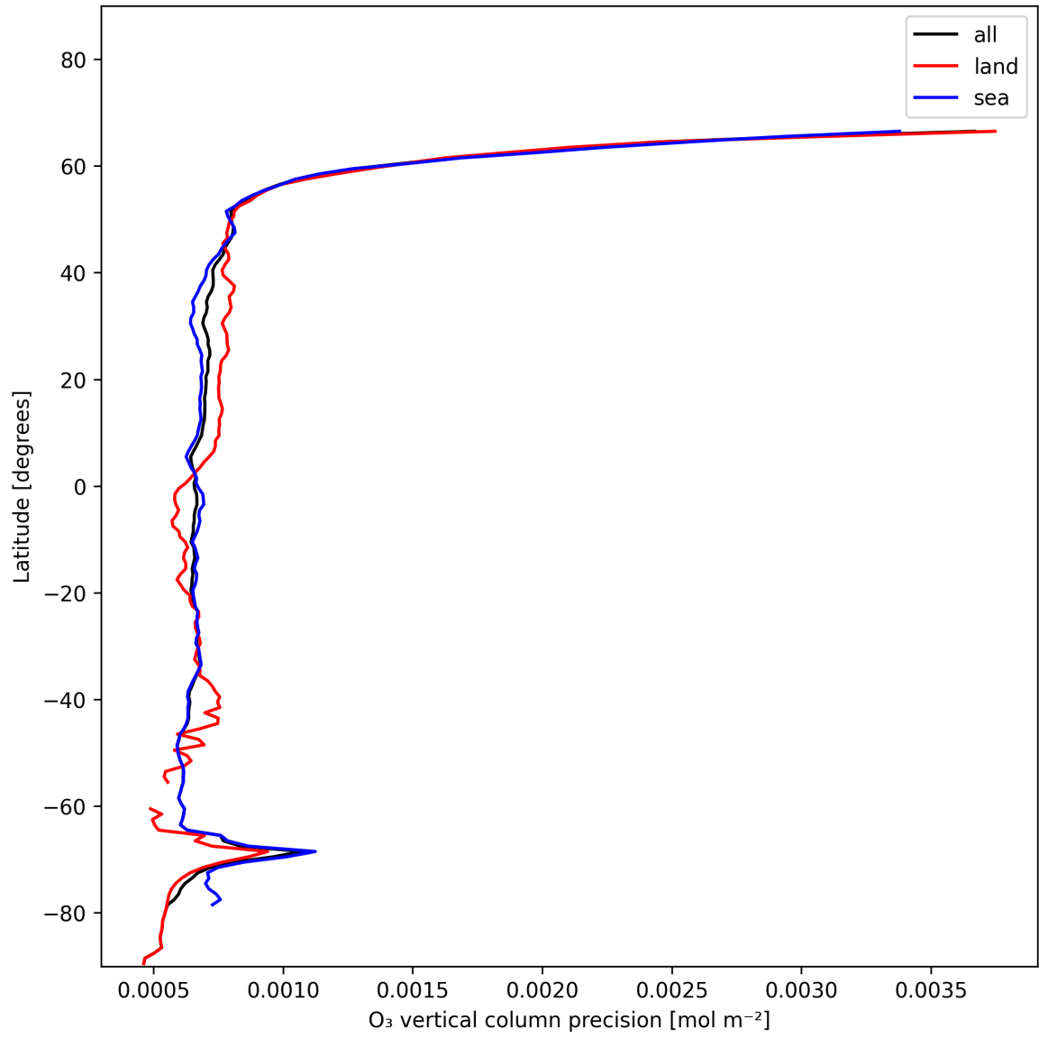
Figure 15: Zonal average of “O 3 vertical column precision” for 2025-01-03 to 2025-01-05.
