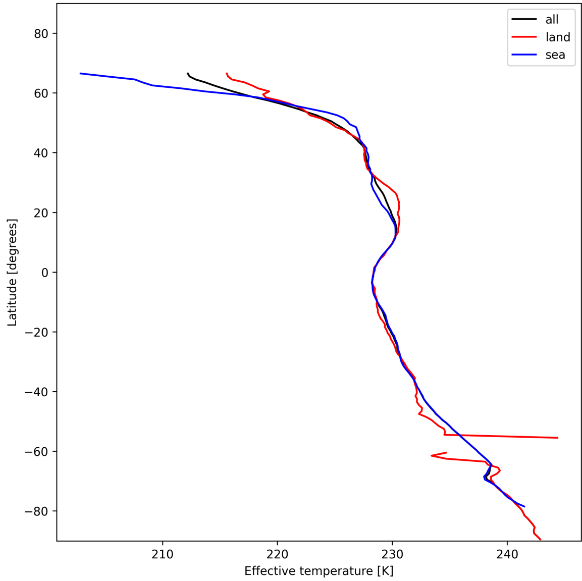
Figure 17: Zonal average of "Effective temperature" for 2025-01-03 to 2025-01-05.
