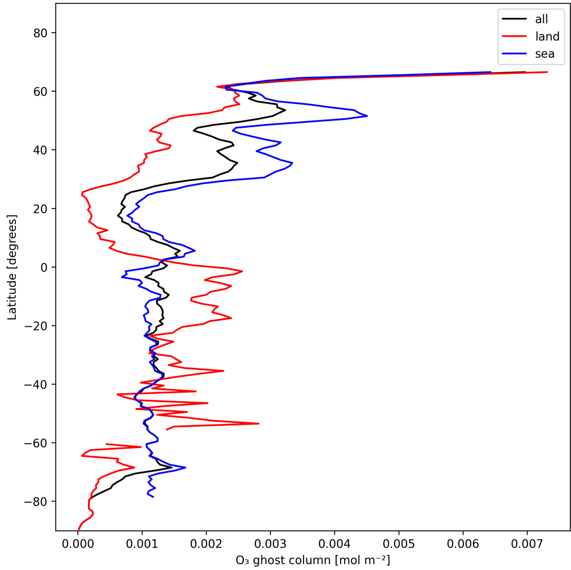
Figure 18: Zonal average of "O 3 ghost column" for 2025-01-03 to 2025-01-05.
