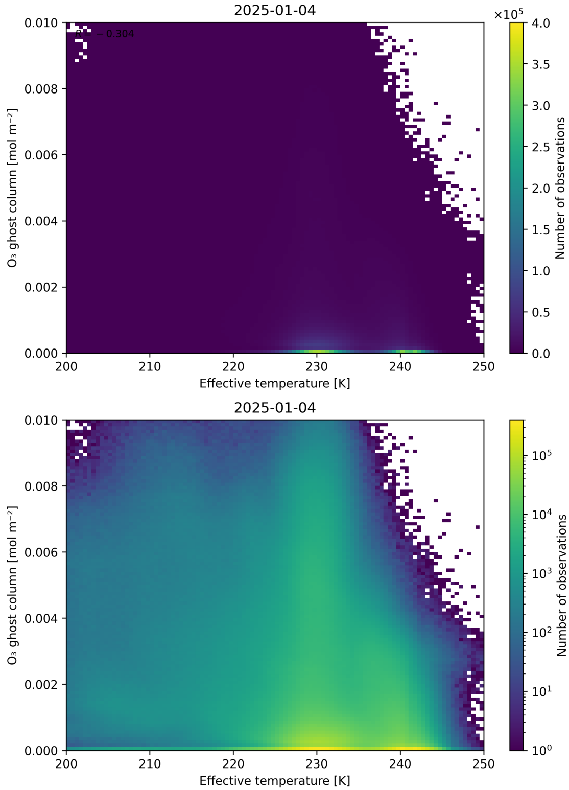
Figure 38: Scatter density plot of “Effective temperature” against “O 3 ghost column” for 2025-01-03 to 2025-01-05.
