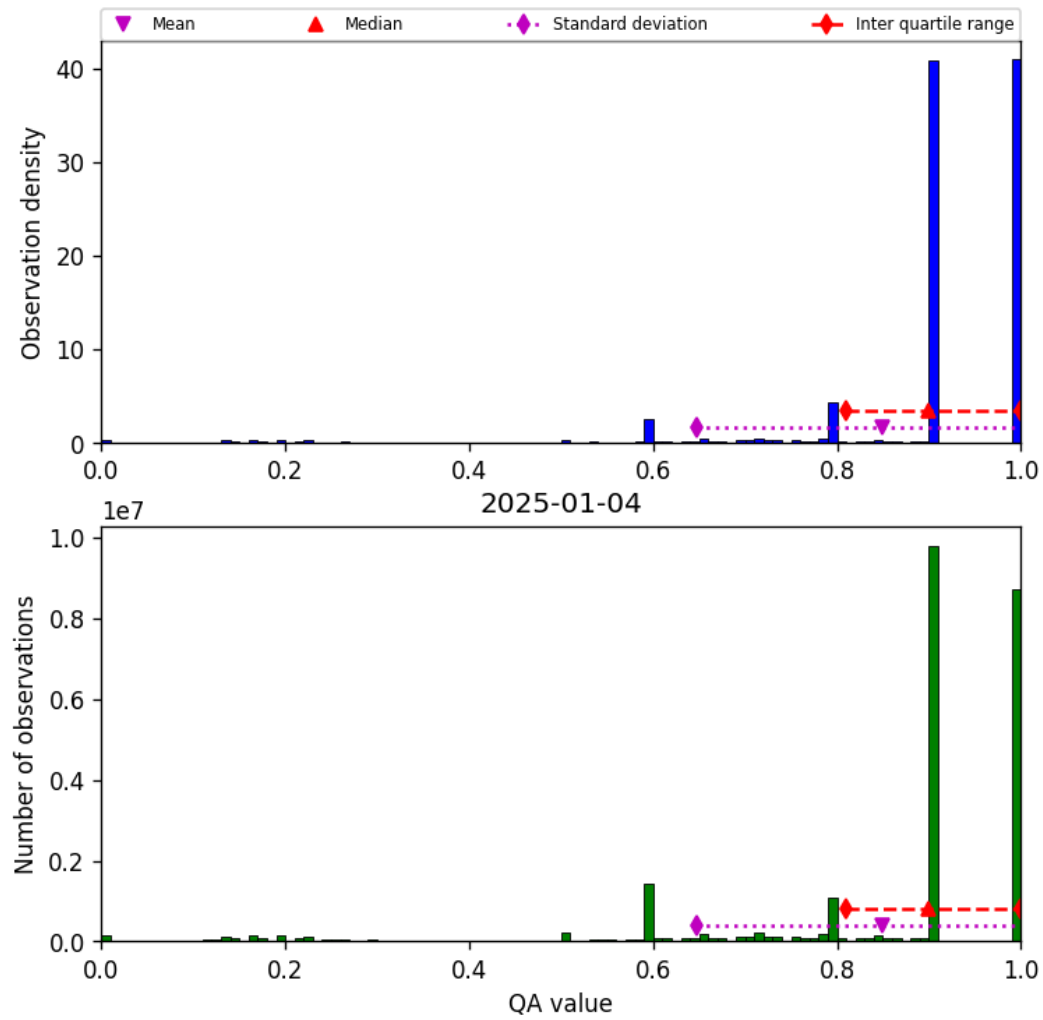
Figure 20: Histogram of “QA value” for 2025-01-03 to 2025-01-05
