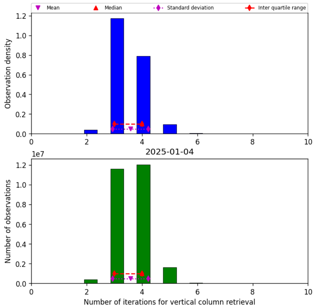
Figure 26: Histogram of “Number of iterations for vertical column retrieval” for 2025-01-03 to 2025-01-05
