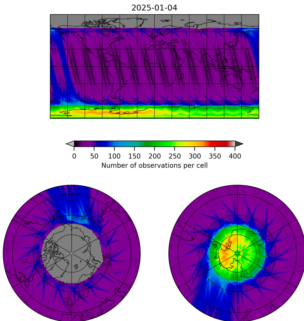
Figure 12: Map of the number of observations for 2025-01-03 to 2025-01-05
