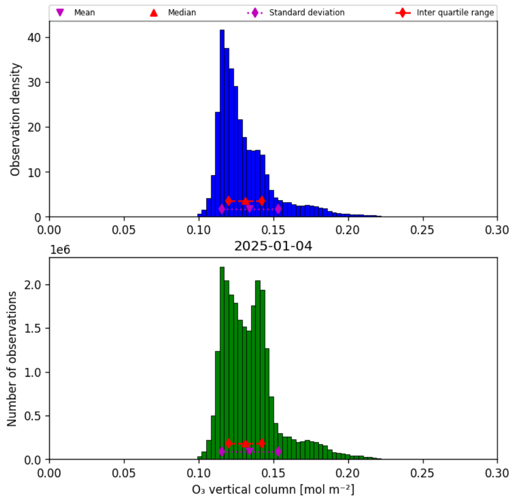
Figure 21: Histogram of “O 3 vertical column” for 2025-01-03 to 2025-01-05
