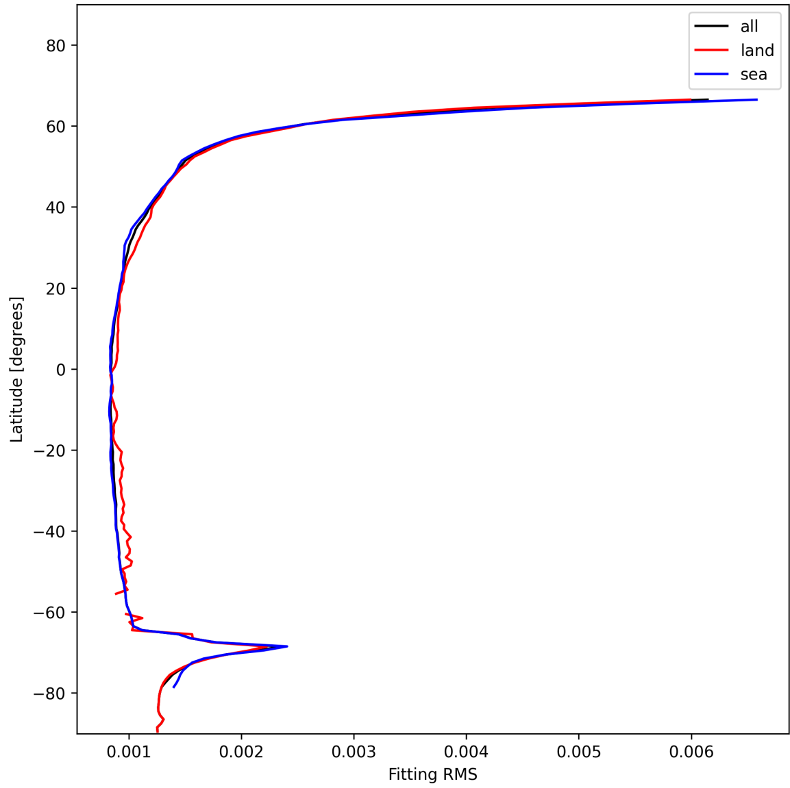
Figure 16: Zonal average of “Fitting RMS” for 2025-01-03 to 2025-01-05.
