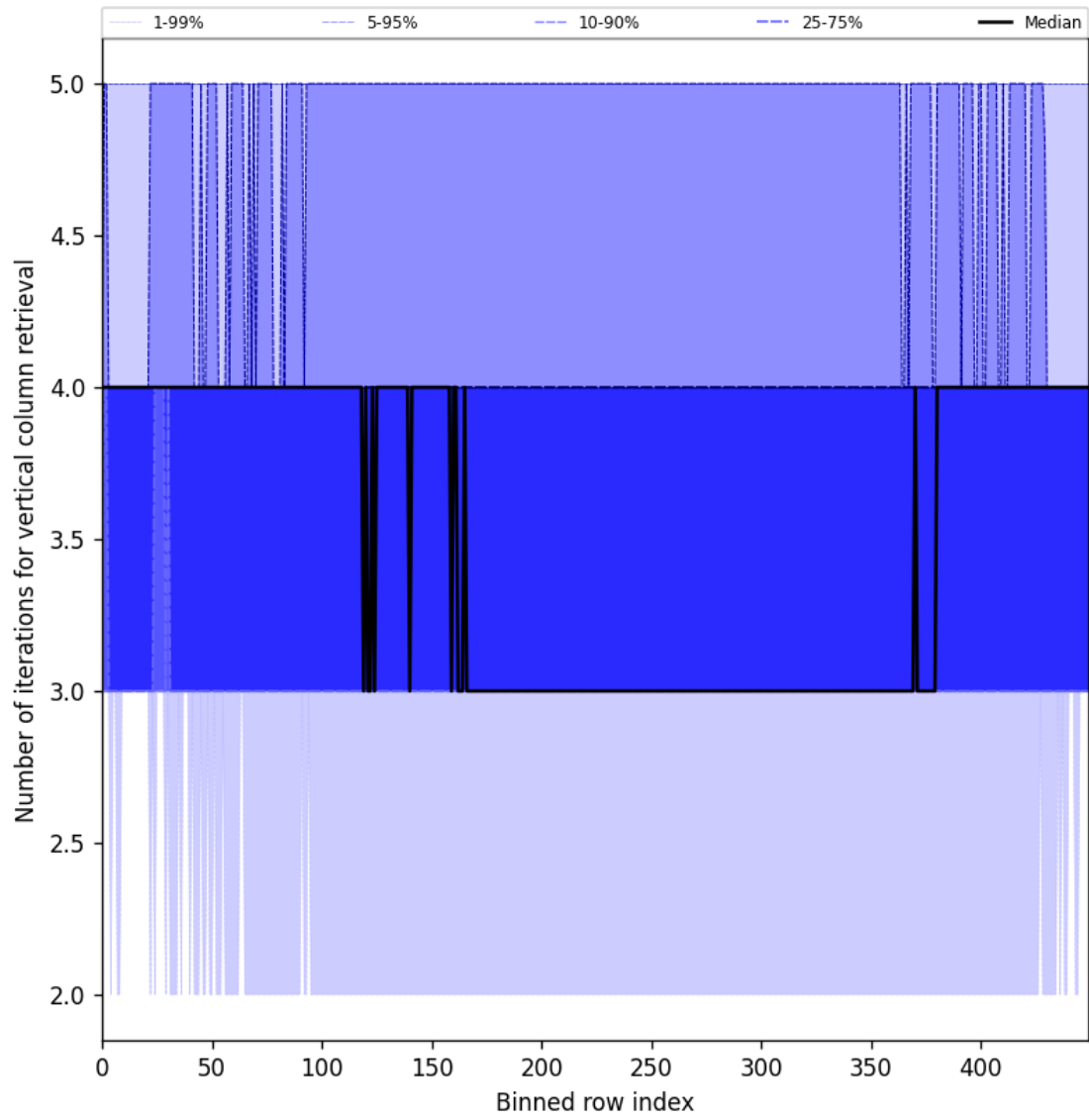
Figure 33: Along track statistics of “Number of iterations for vertical column retrieval” for 2025-01-03 to 2025-01-05
