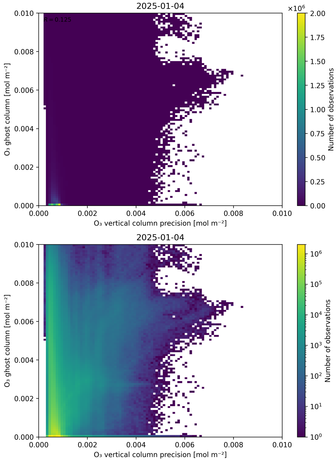
Figure 43: Scatter density plot of “ \text{O}_3 vertical column precision” against “ \text{O}_3 ghost column” for 2025-01-03 to 2025-01-05.
