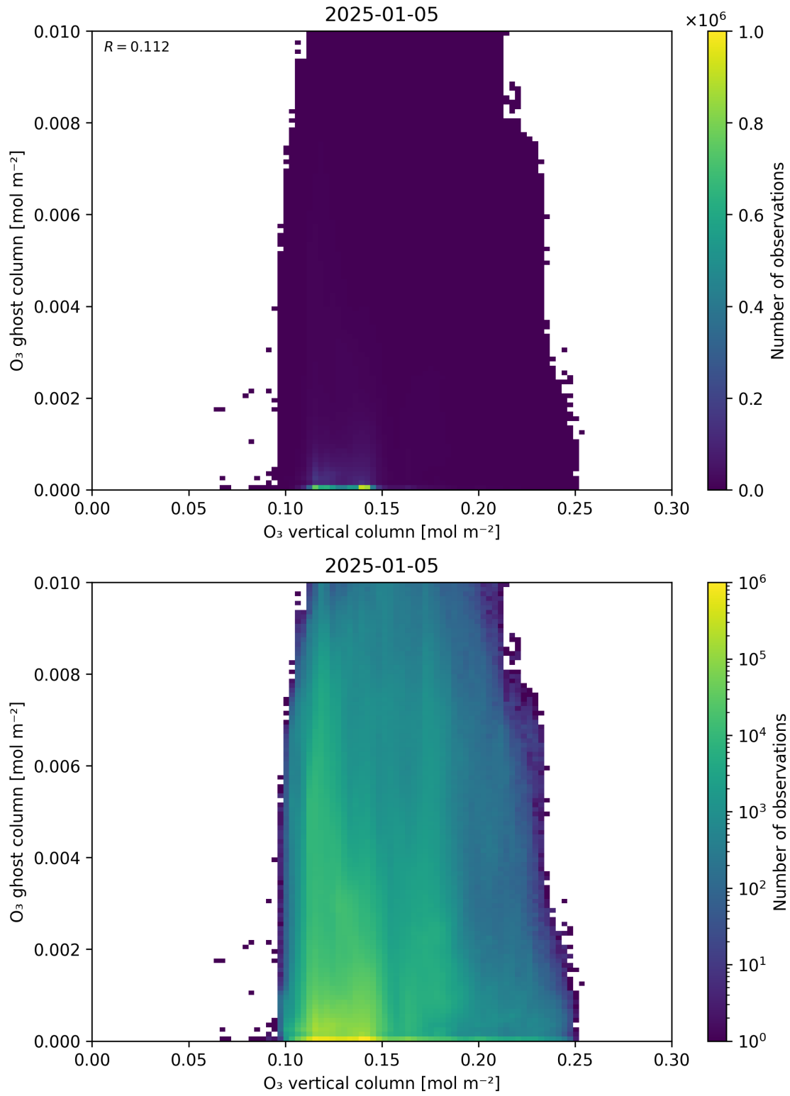
Figure 40: Scatter density plot of “O 3 vertical column” against “O 3 ghost column” for 2025-01-04 to 2025-01-06.
