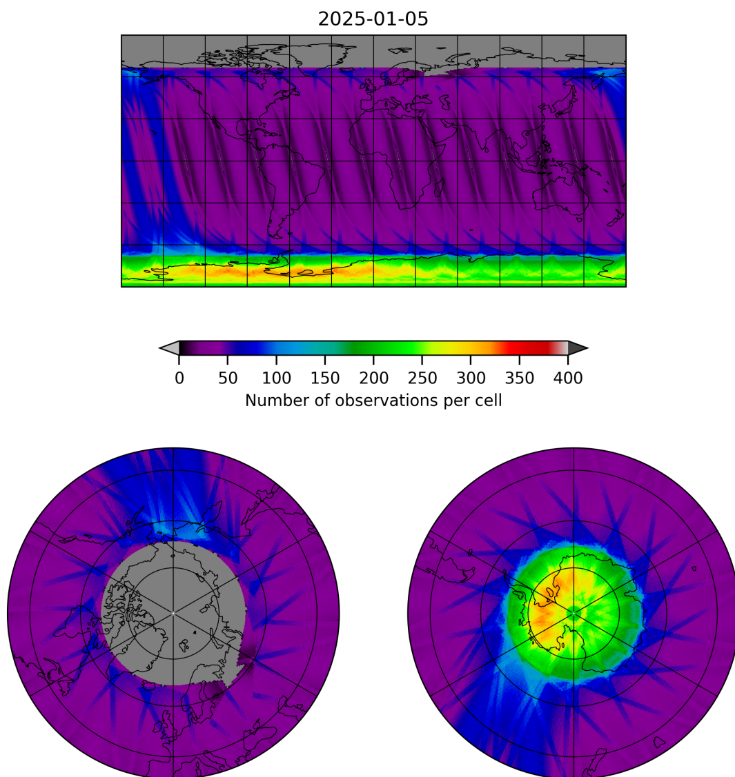
Figure 12: Map of the number of observations for 2025-01-04 to 2025-01-06
