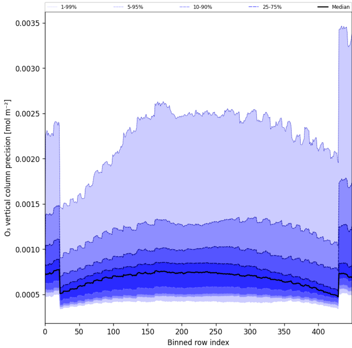
Figure 29: Along track statistics of “O 3 vertical column precision” for 2025-01-04 to 2025-01-06
