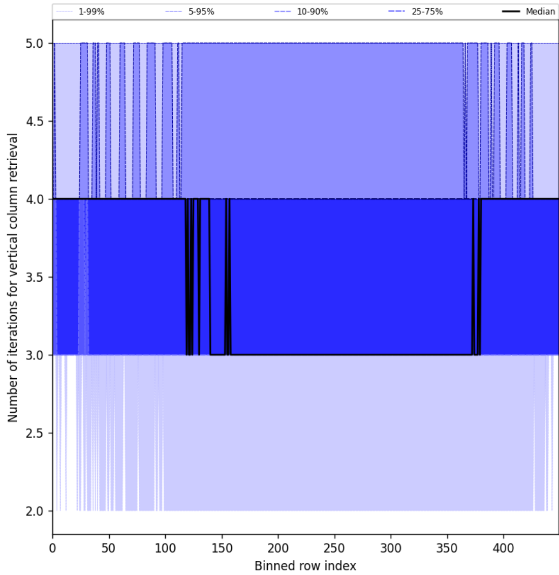
Figure 33: Along track statistics of “Number of iterations for vertical column retrieval” for 2025-01-04 to 2025-01-06
