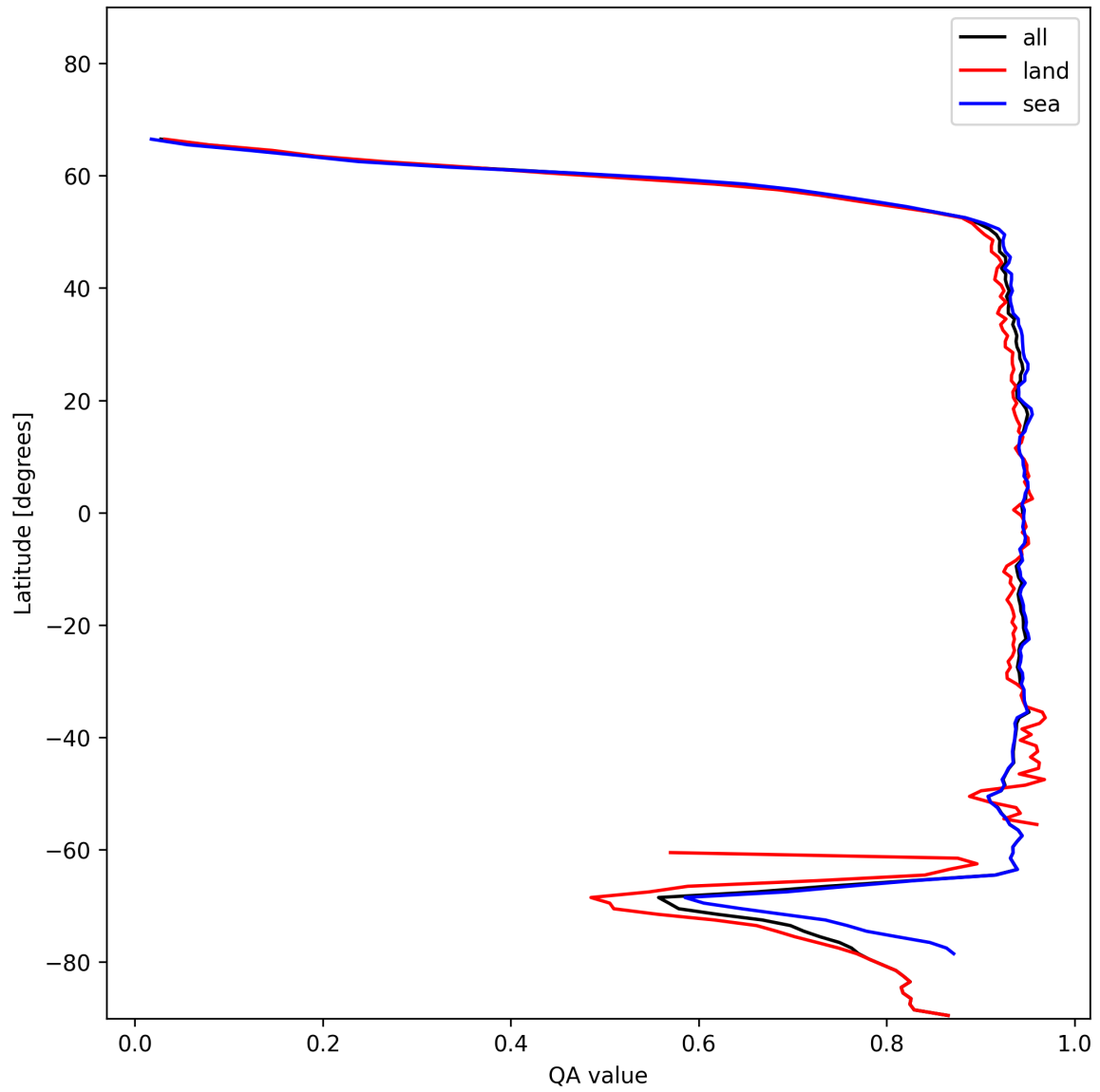
Figure 13: Zonal average of “QA value” for 2025-01-04 to 2025-01-06.
