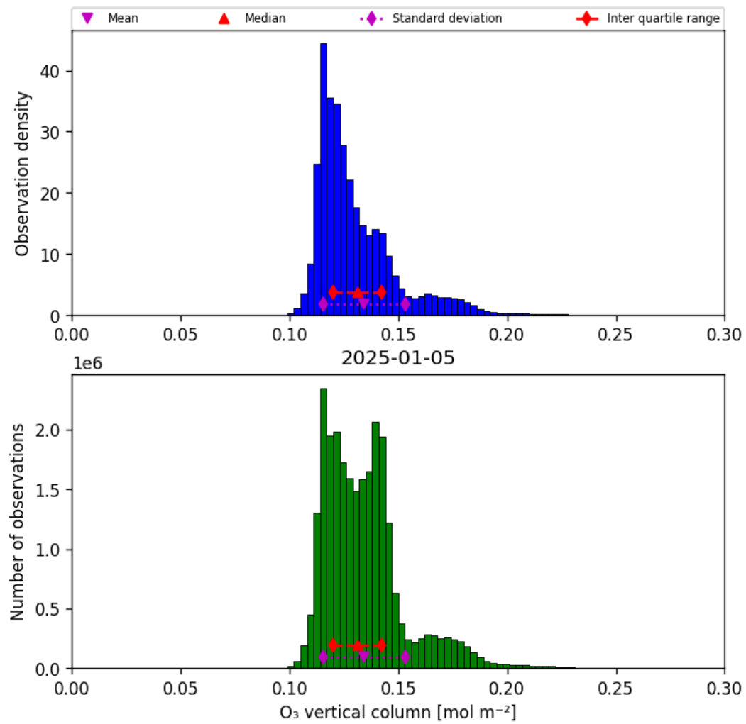
Figure 21: Histogram of “O 3 vertical column” for 2025-01-04 to 2025-01-06
