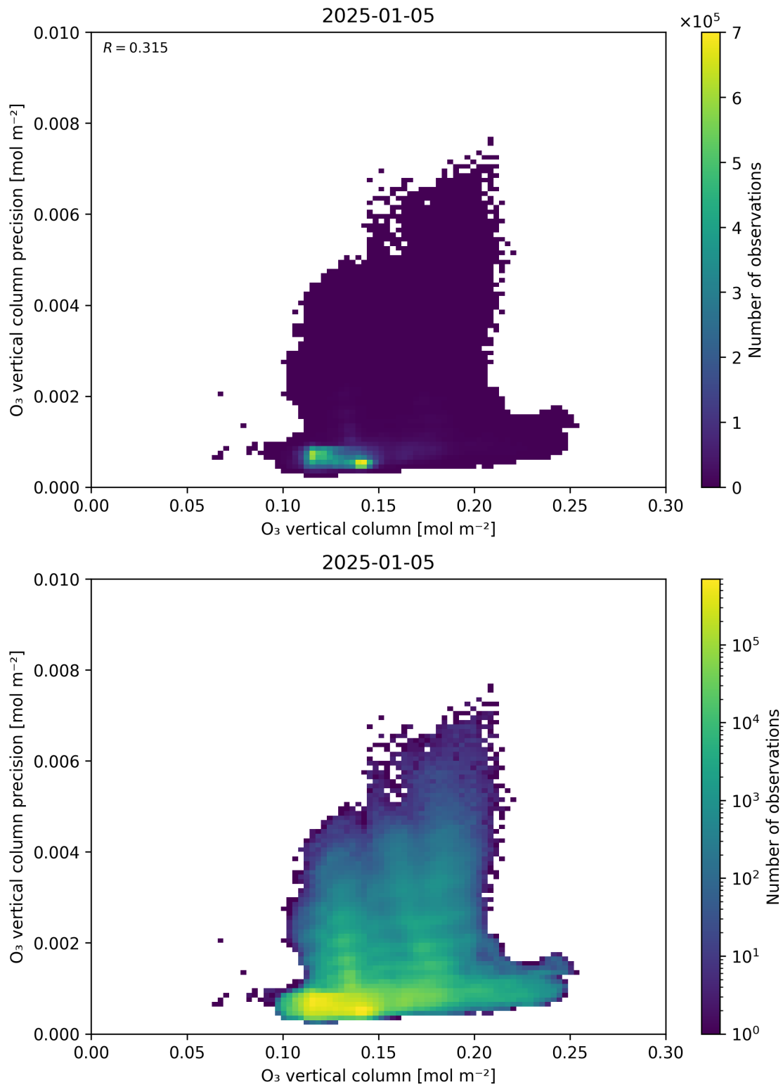
Figure 41: Scatter density plot of “O 3 vertical column” against “O 3 vertical column precision” for 2025-01-04 to 2025-01-06.
