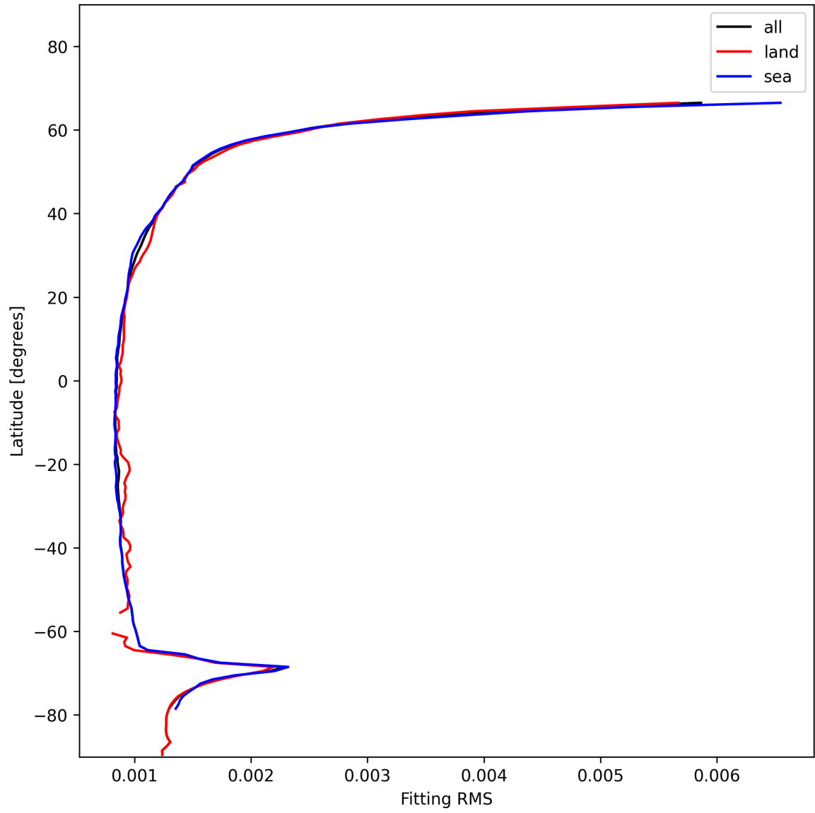
Figure 16: Zonal average of “Fitting RMS” for 2025-01-04 to 2025-01-06.
