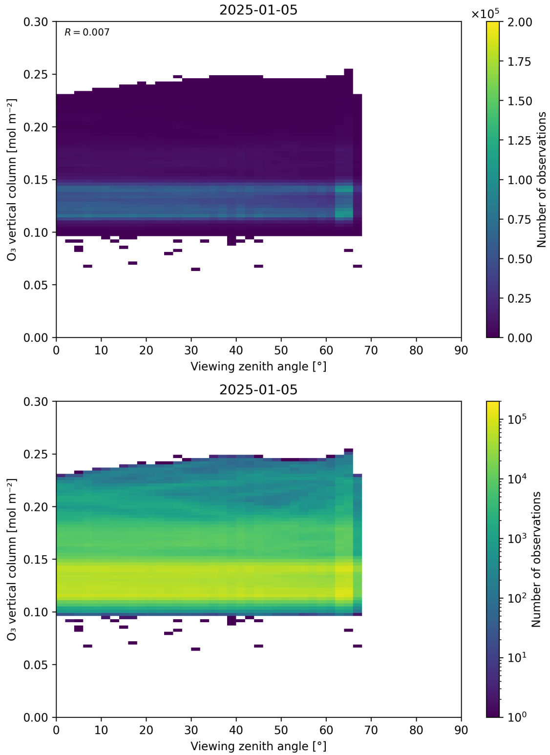
Figure 52: Scatter density plot of “Viewing zenith angle” against “O 3 vertical column” for 2025-01-04 to 2025-01-06.
