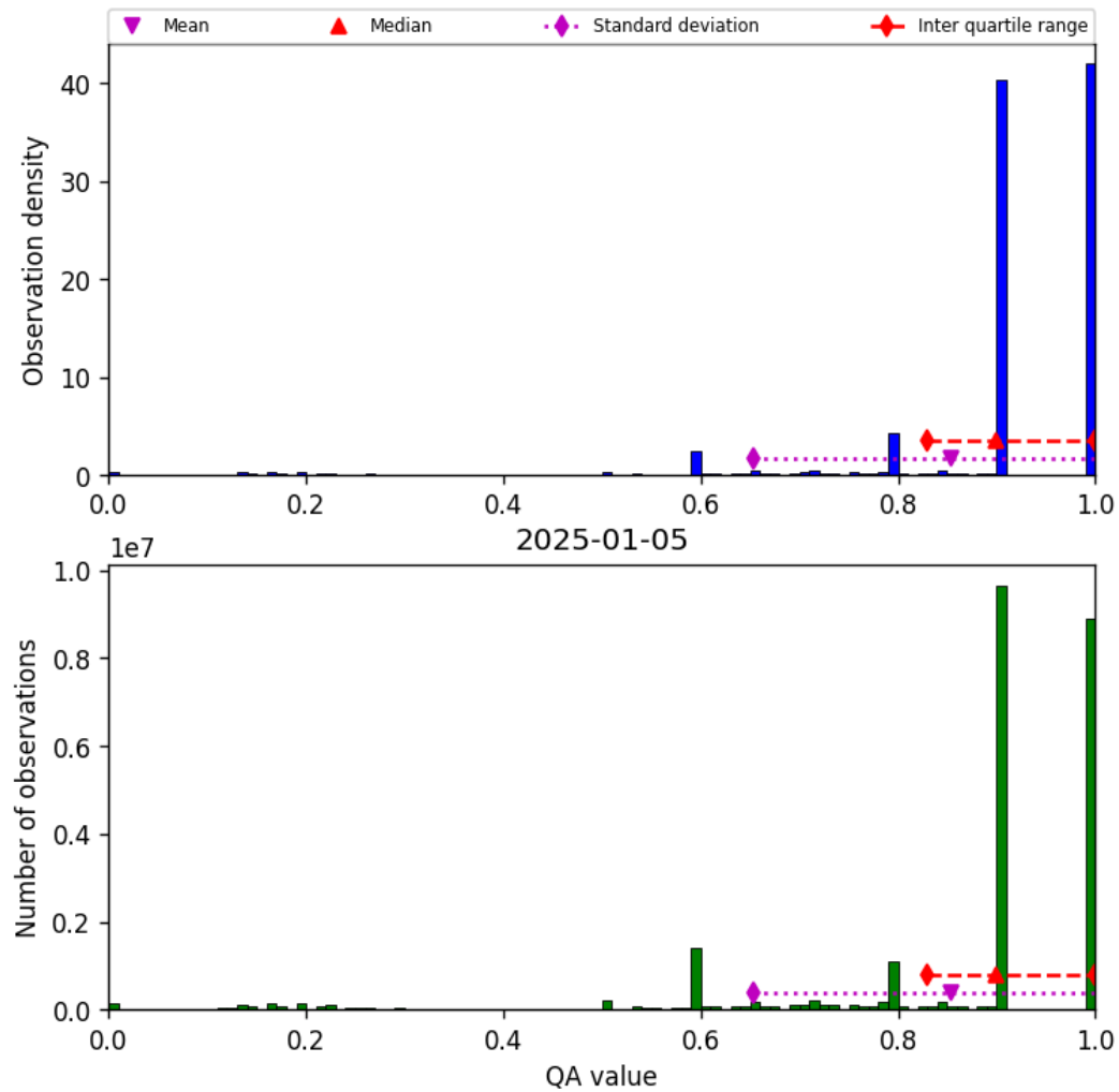
Figure 20: Histogram of “QA value” for 2025-01-04 to 2025-01-06
