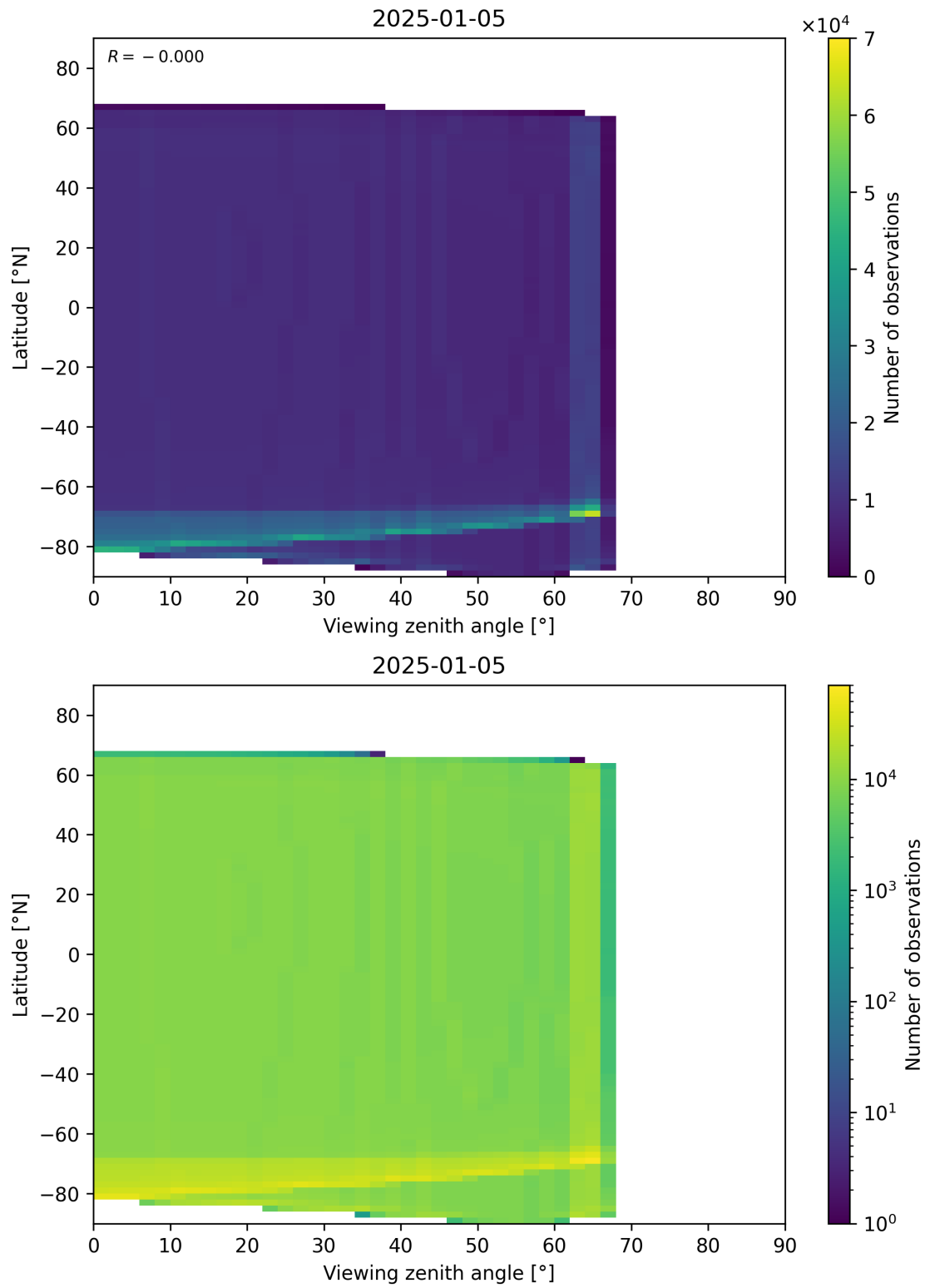
Figure 49: Scatter density plot of “Viewing zenith angle” against “Latitude” for 2025-01-04 to 2025-01-06.
