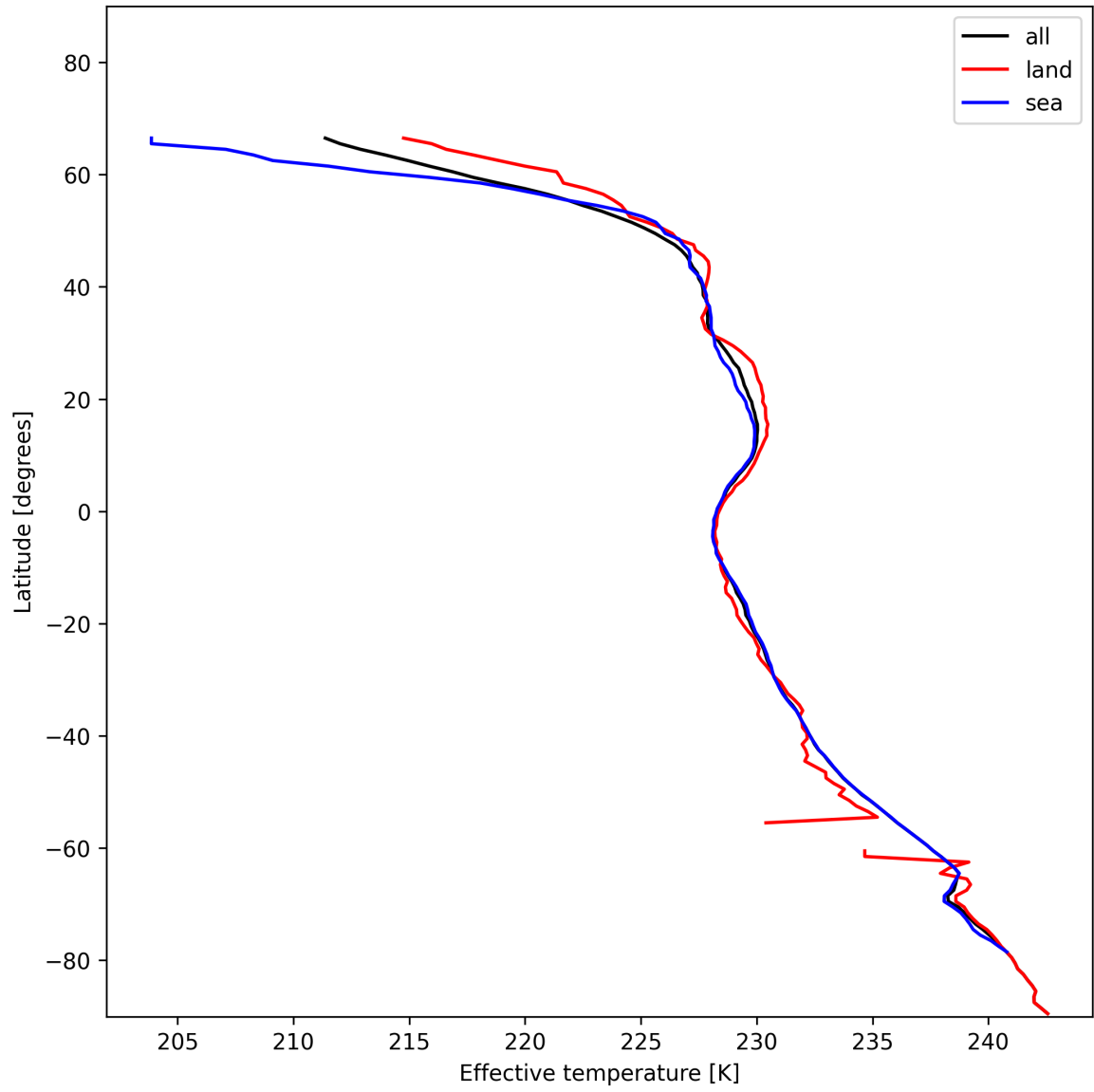
Figure 17: Zonal average of "Effective temperature" for 2025-01-04 to 2025-01-06.
