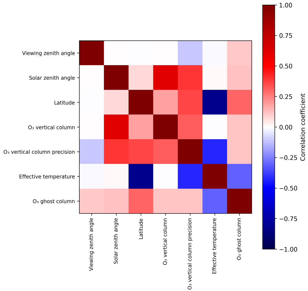
Figure 2: Map of correlation matrix for 2025-01-04 to 2025-01-06.
