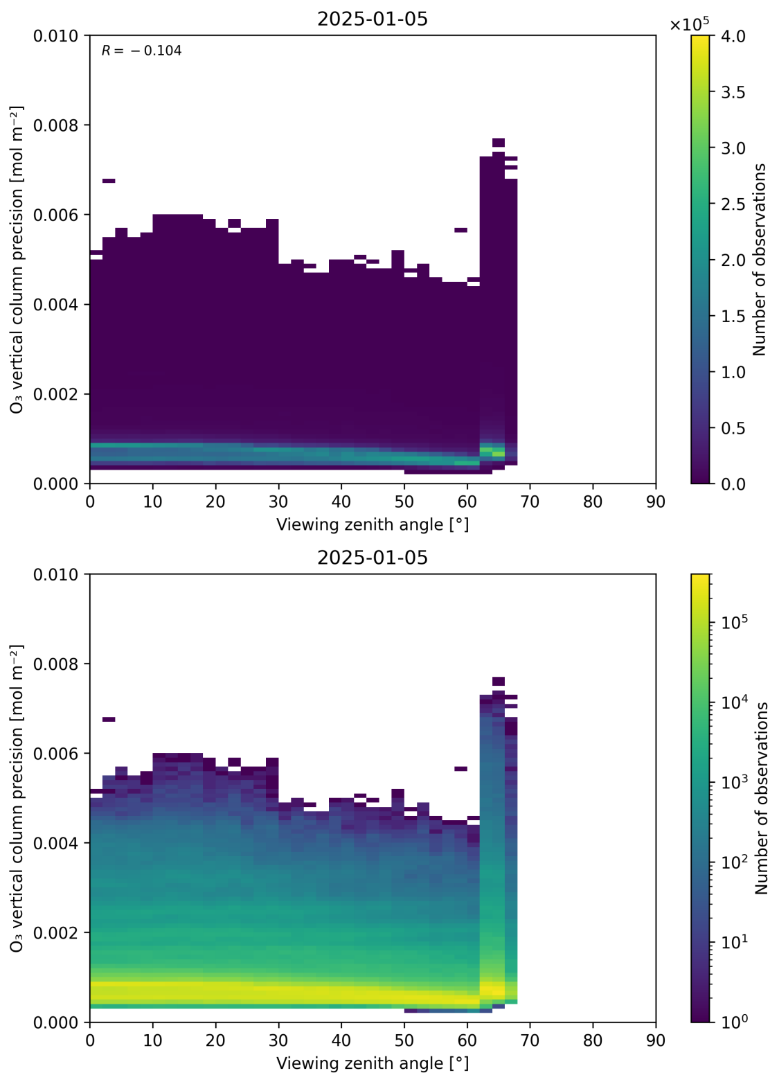
Figure 53: Scatter density plot of “Viewing zenith angle” against “O 3 vertical column precision” for 2025-01-04 to 2025-01-06.
