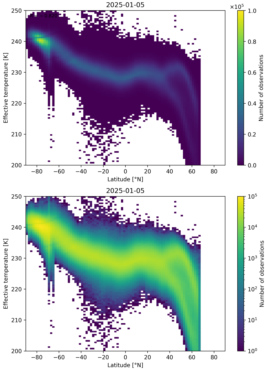
Figure 34: Scatter density plot of “Latitude” against “Effective temperature” for 2025-01-04 to 2025-01-06.
