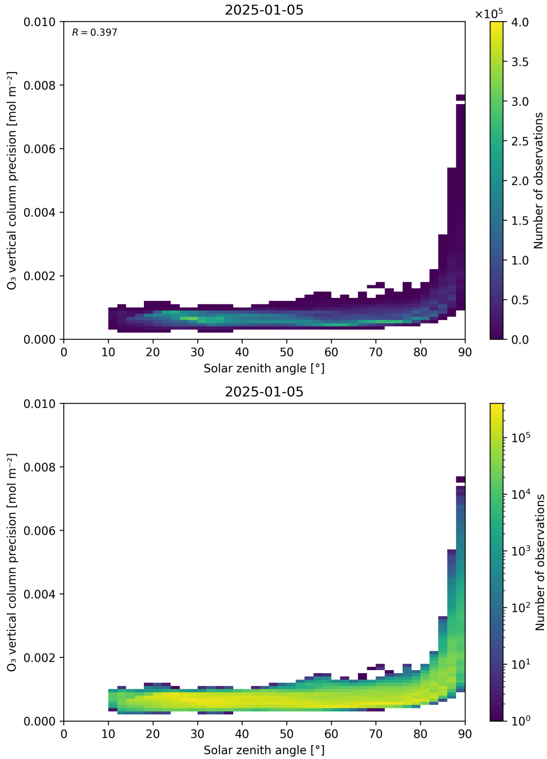
Figure 48: Scatter density plot of “Solar zenith angle” against “O 3 vertical column precision” for 2025-01-04 to 2025-01-06.
