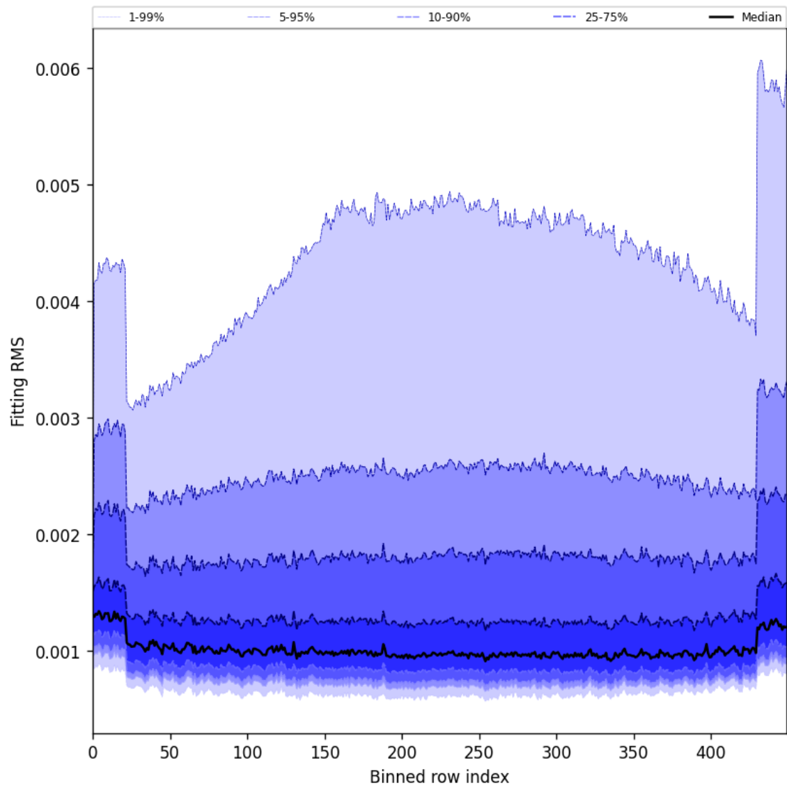
Figure 30: Along track statistics of “Fitting RMS” for 2025-01-04 to 2025-01-06
