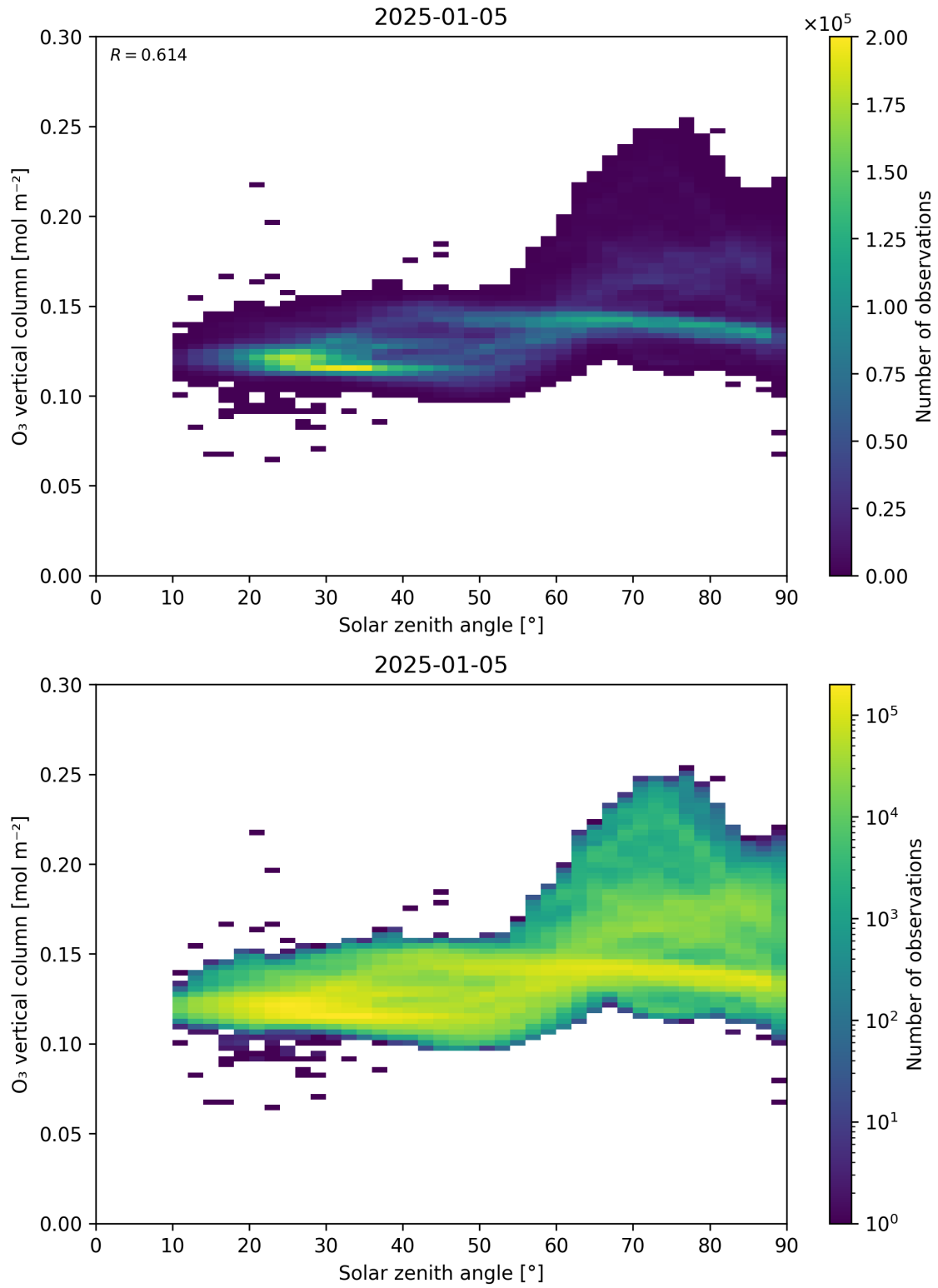
Figure 47: Scatter density plot of “Solar zenith angle” against “O 3 vertical column” for 2025-01-04 to 2025-01-06.
