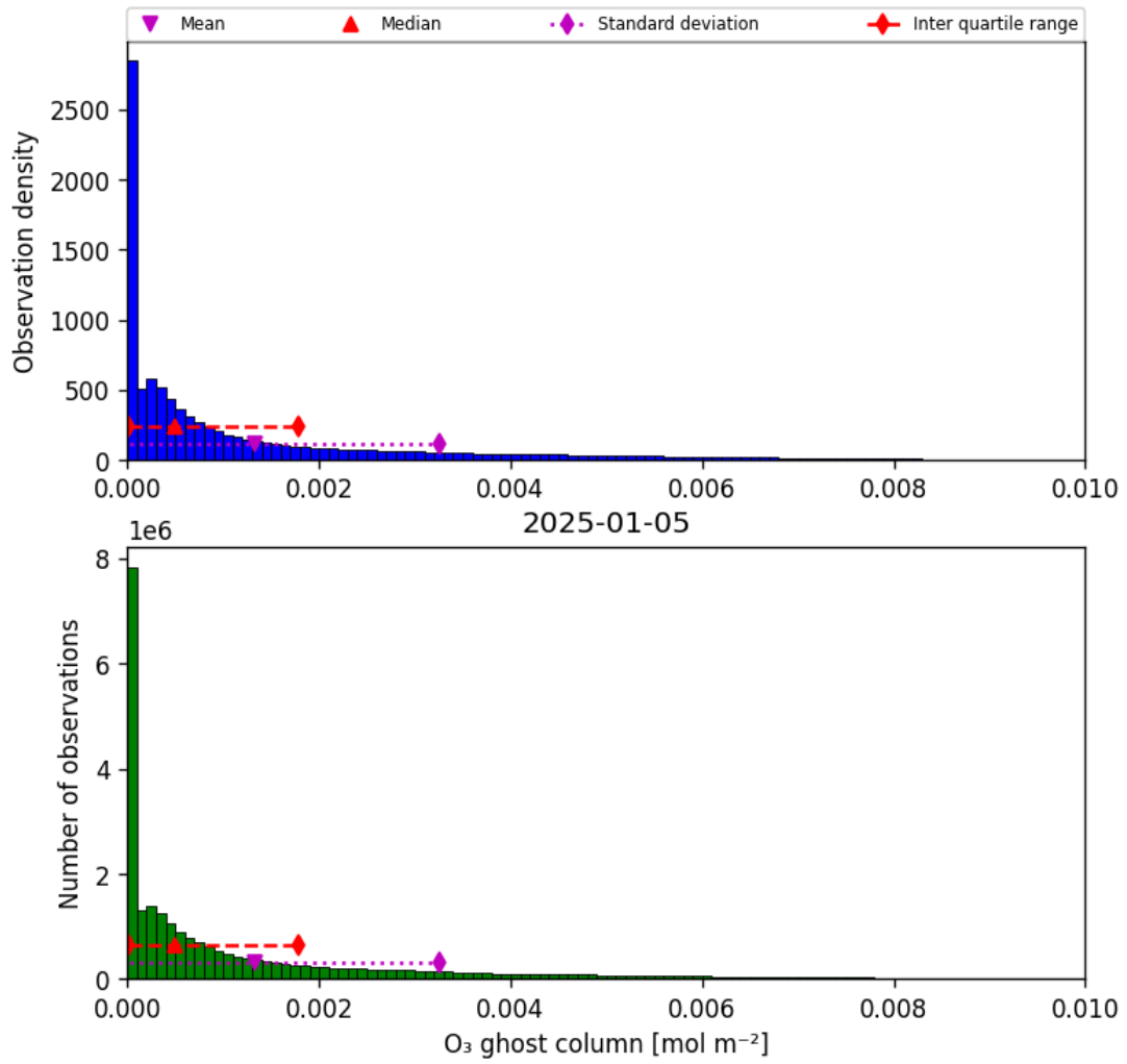
Figure 25: Histogram of “O 3 ghost column” for 2025-01-04 to 2025-01-06
