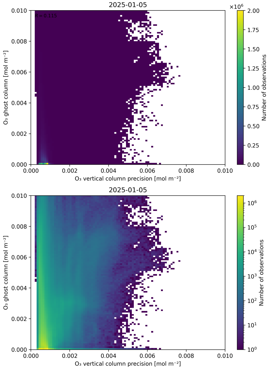
Figure 43: Scatter density plot of “ \text{O}_3 vertical column precision” against “ \text{O}_3 ghost column” for 2025-01-04 to 2025-01-06.
