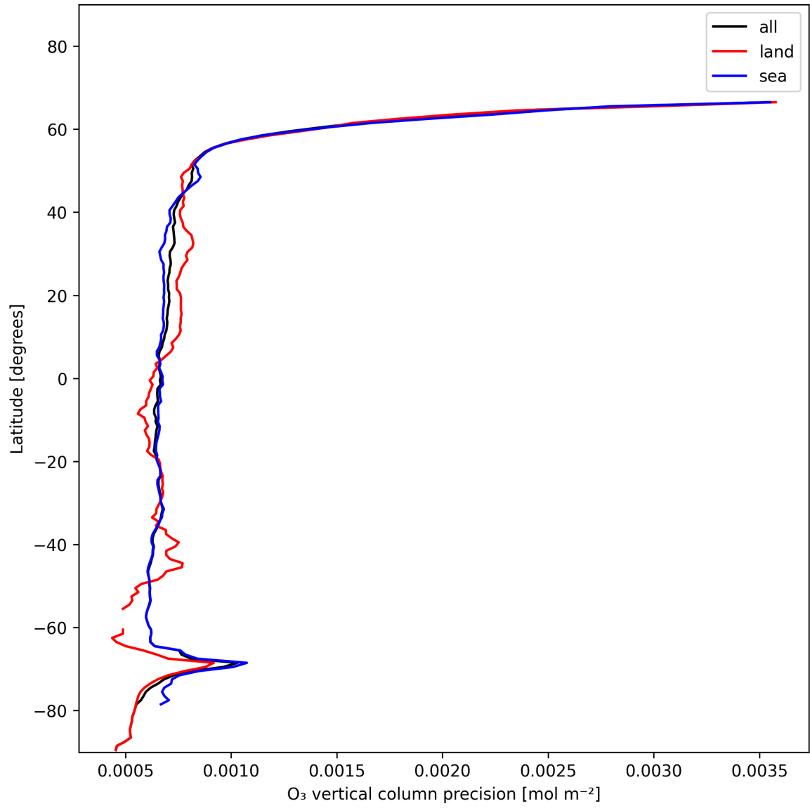
Figure 15: Zonal average of “O 3 vertical column precision” for 2025-01-04 to 2025-01-06.
