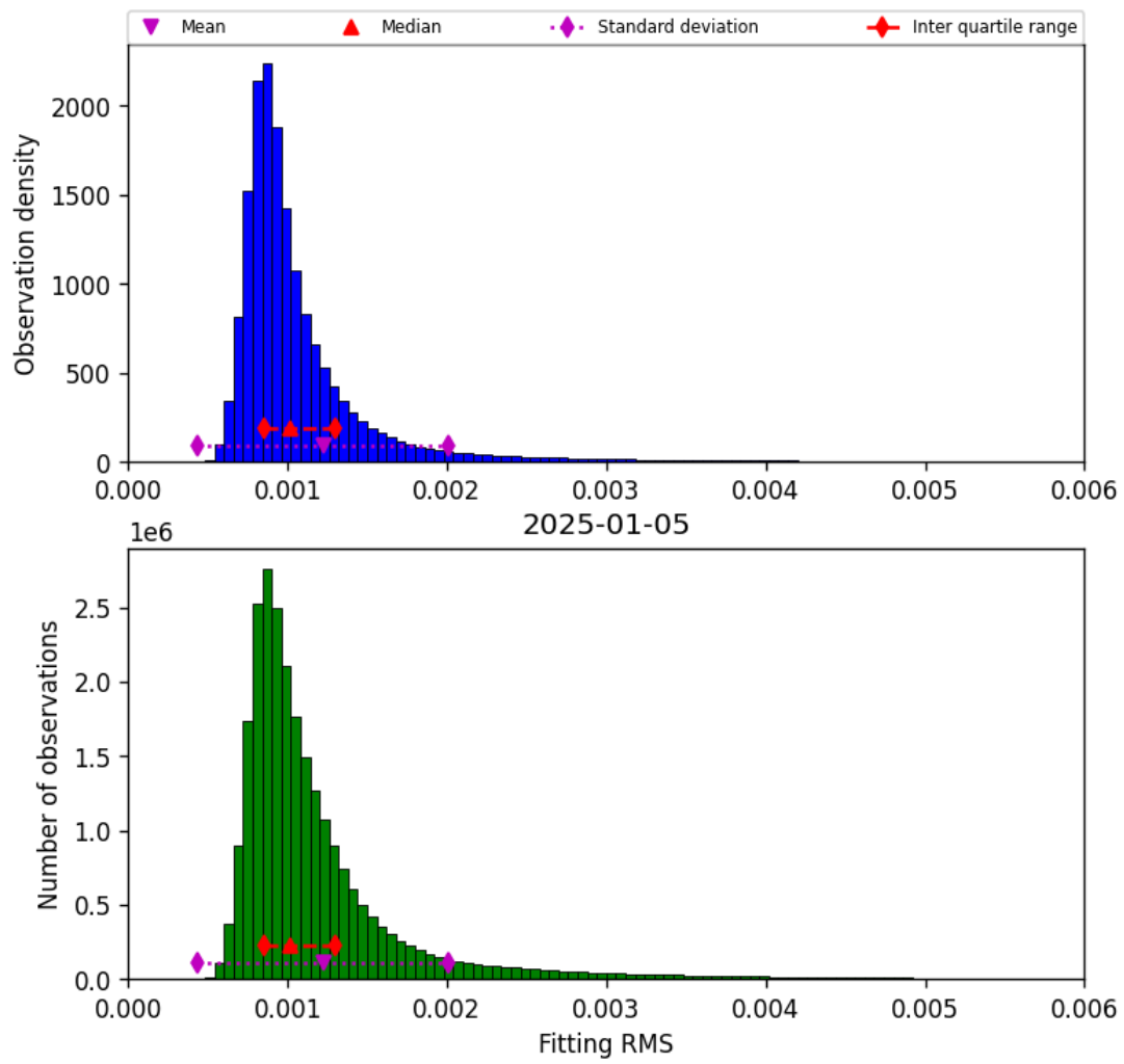
Figure 23: Histogram of “Fitting RMS” for 2025-01-04 to 2025-01-06
