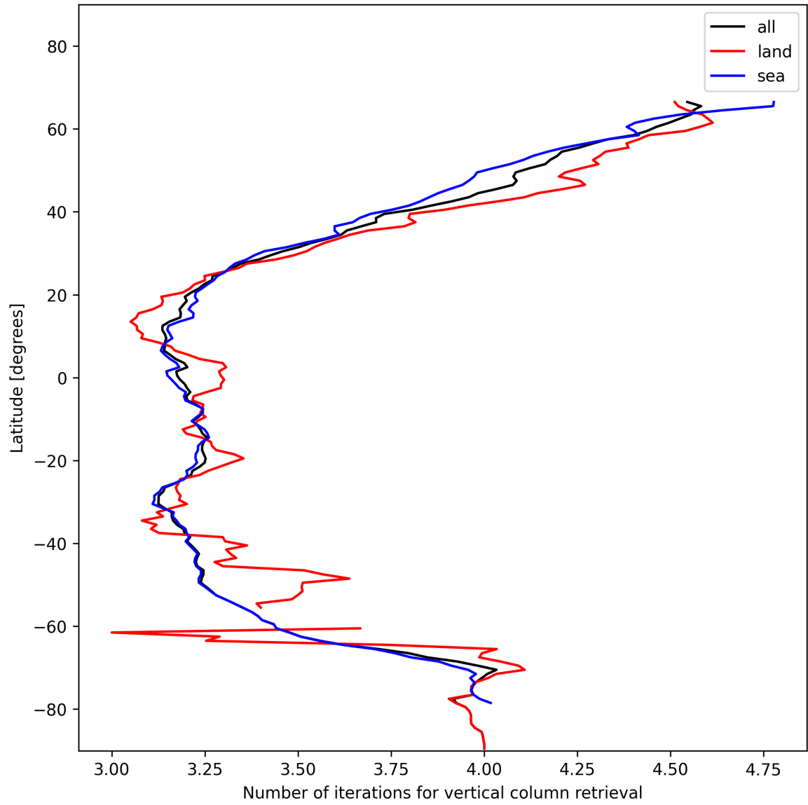
Figure 19: Zonal average of “Number of iterations for vertical column retrieval” for 2025-01-04 to 2025-01-06.
