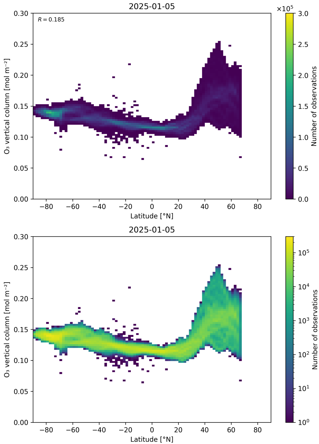
Figure 36: Scatter density plot of “Latitude” against “O 3 vertical column” for 2025-01-04 to 2025-01-06.
