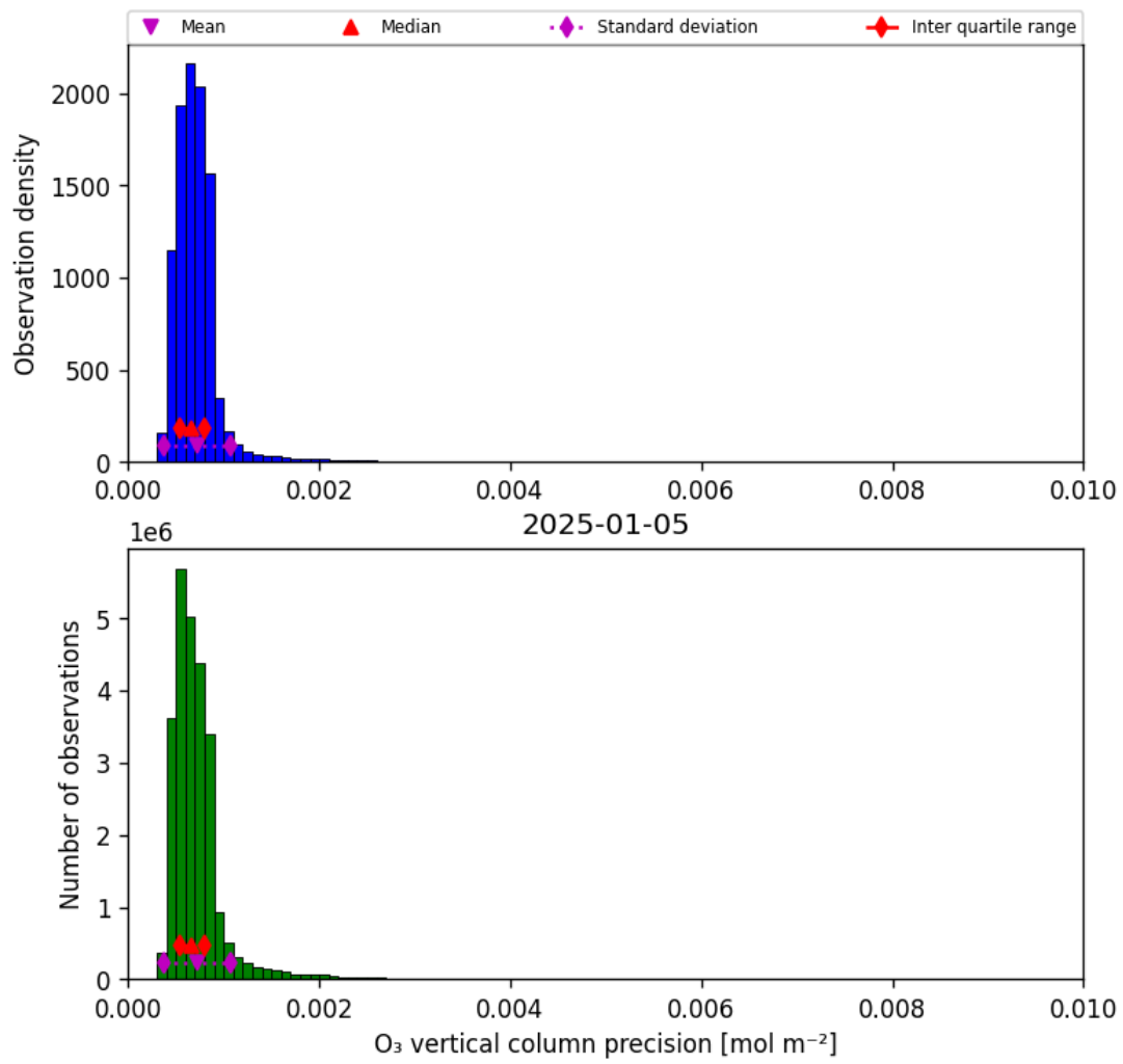
Figure 22: Histogram of “O 3 vertical column precision” for 2025-01-04 to 2025-01-06
