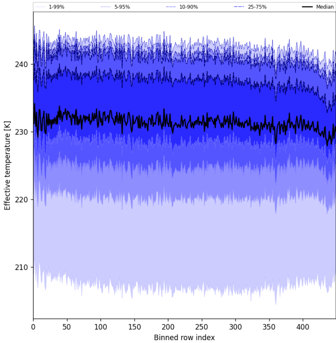
Figure 31: Along track statistics of “Effective temperature” for 2025-01-04 to 2025-01-06
