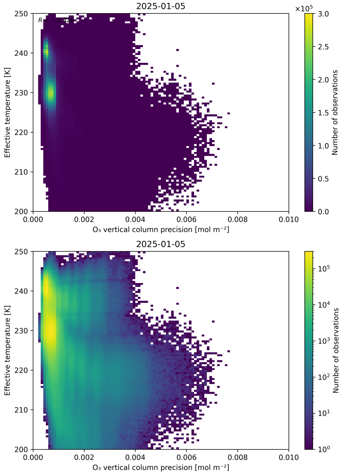
Figure 42: Scatter density plot of “O 3 vertical column precision” against “Effective temperature” for 2025-01-04 to 2025-01-06.
