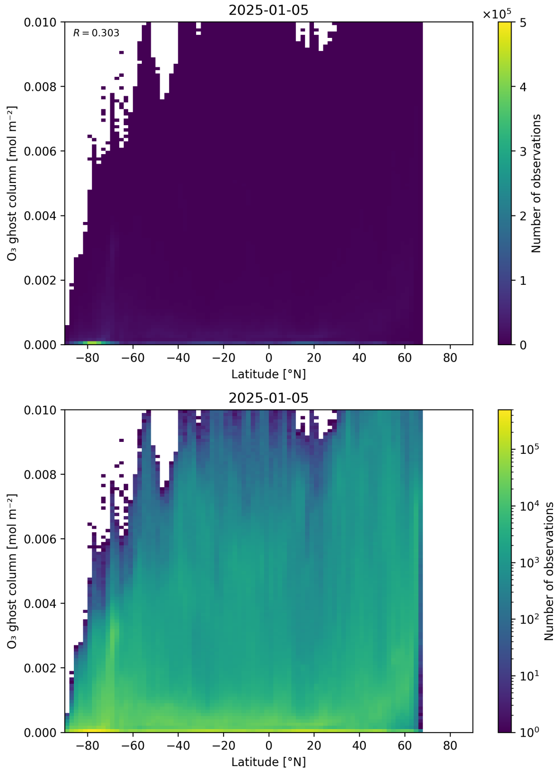
Figure 35: Scatter density plot of “Latitude” against “O 3 ghost column” for 2025-01-04 to 2025-01-06.
