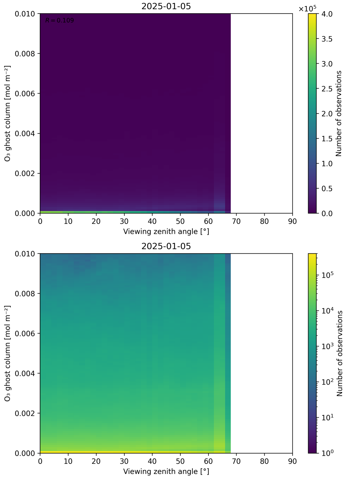
Figure 51: Scatter density plot of “Viewing zenith angle” against “O 3 ghost column” for 2025-01-04 to 2025-01-06.
