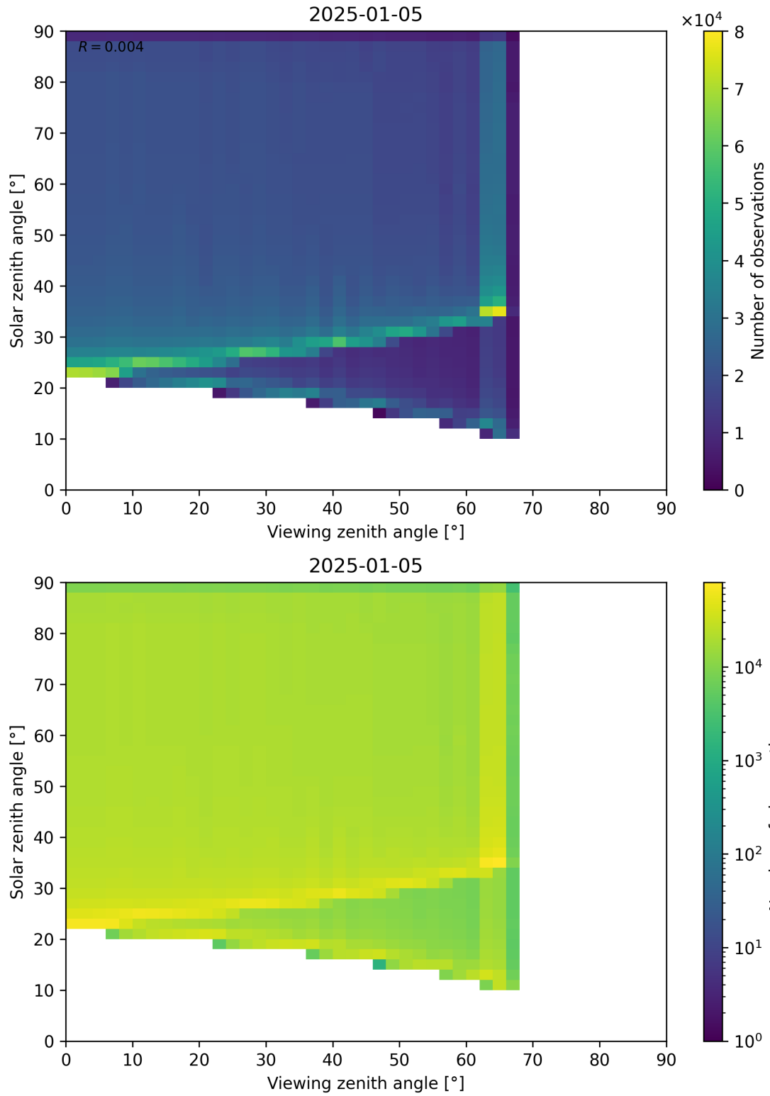
Figure 54: Scatter density plot of “Viewing zenith angle” against “Solar zenith angle” for 2025-01-04 to 2025-01-06.
