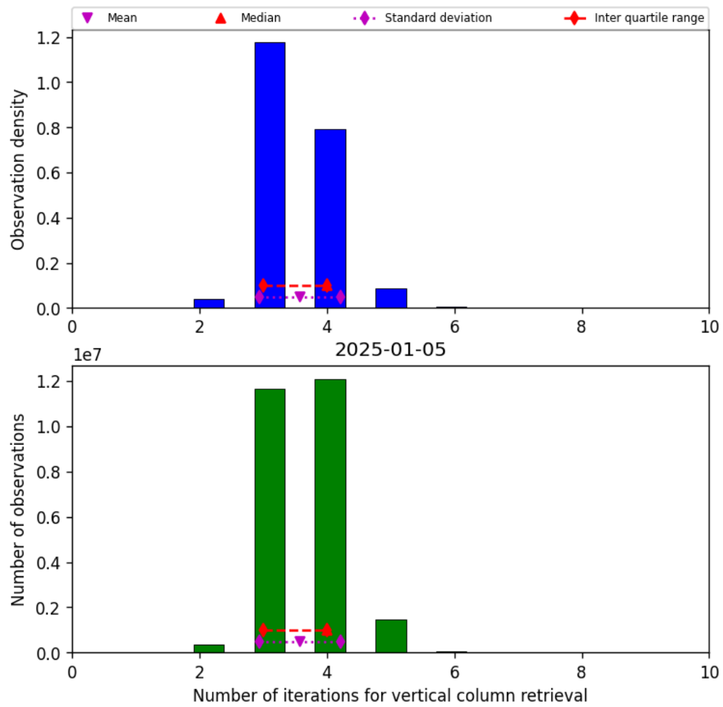
Figure 26: Histogram of “Number of iterations for vertical column retrieval” for 2025-01-04 to 2025-01-06
