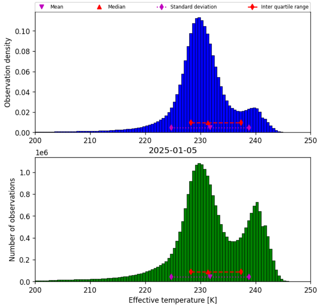
Figure 24: Histogram of “Effective temperature” for 2025-01-04 to 2025-01-06
