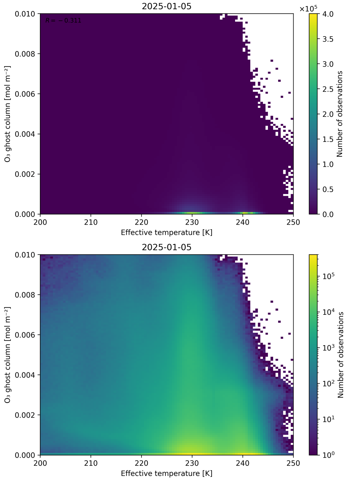
Figure 38: Scatter density plot of “Effective temperature” against “O 3 ghost column” for 2025-01-04 to 2025-01-06.
