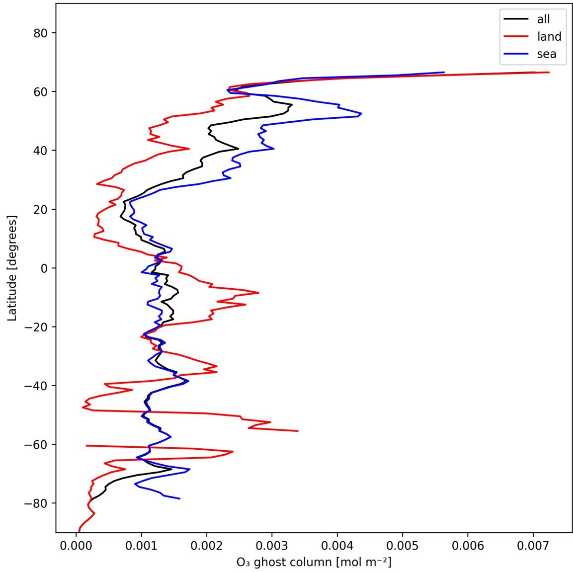
Figure 18: Zonal average of "O 3 ghost column" for 2025-01-04 to 2025-01-06.
