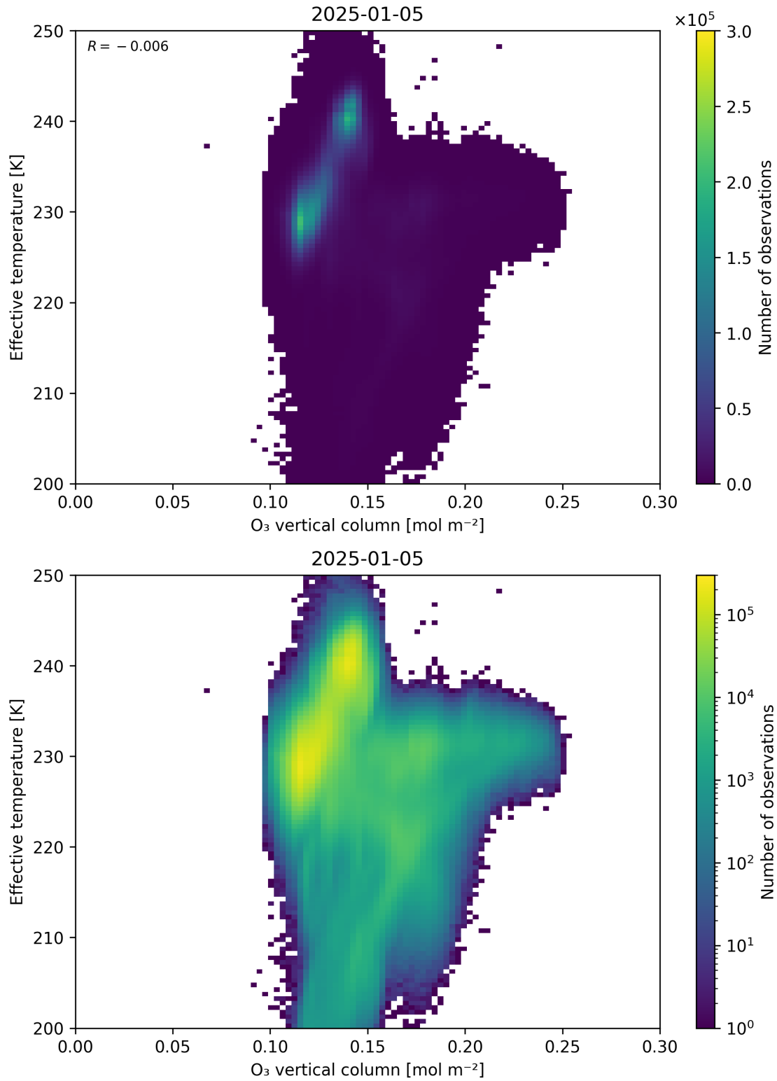
Figure 39: Scatter density plot of “O 3 vertical column” against “Effective temperature” for 2025-01-04 to 2025-01-06.
