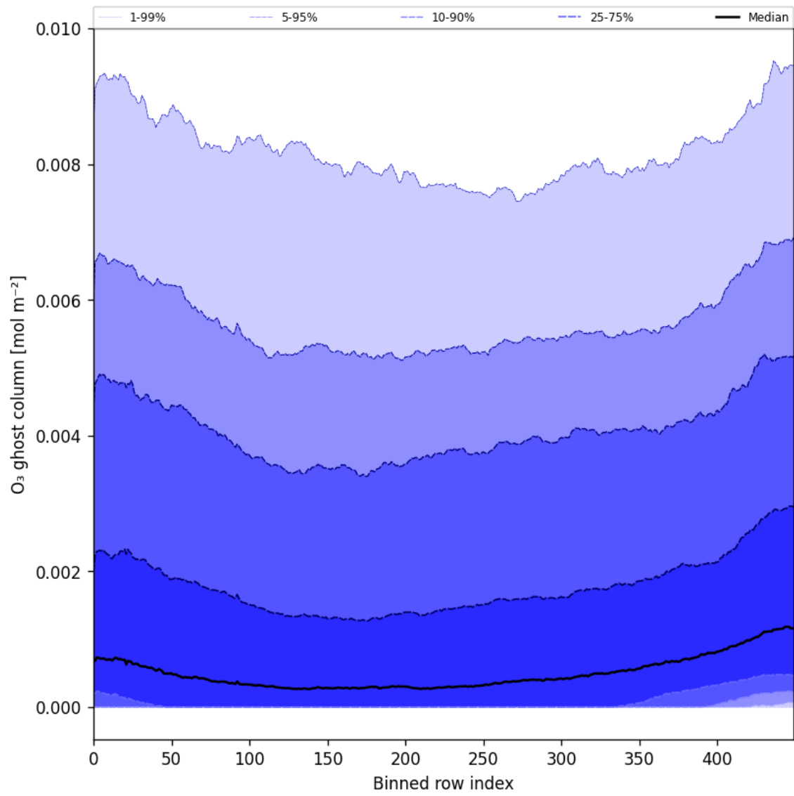
Figure 32: Along track statistics of “O 3 ghost column” for 2025-01-04 to 2025-01-06
