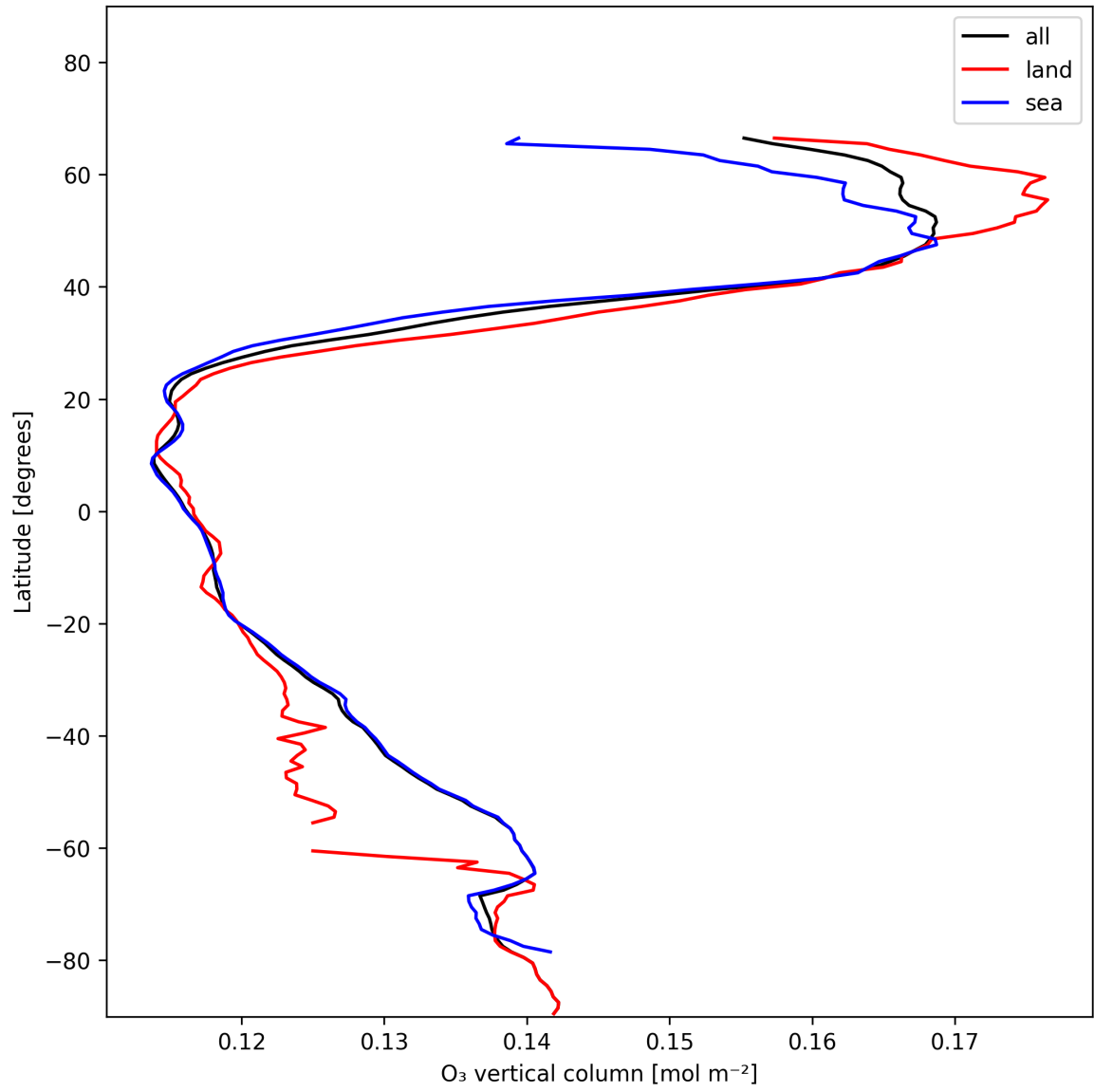
Figure 14: Zonal average of “O 3 vertical column” for 2025-01-04 to 2025-01-06.
