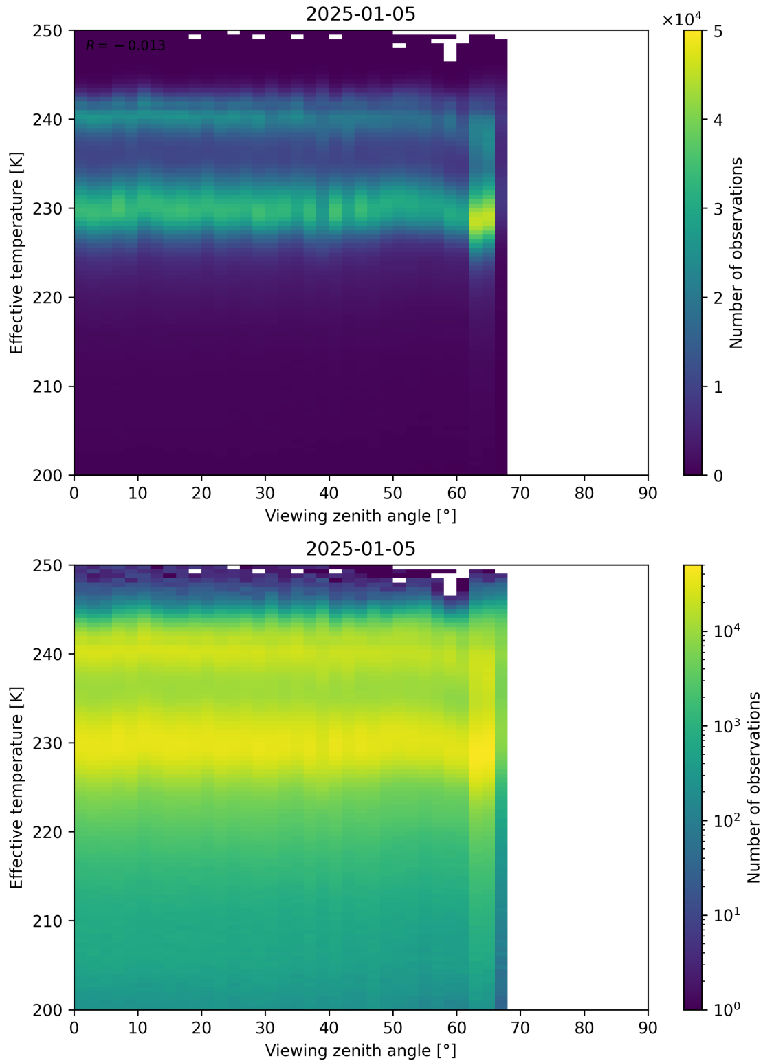
Figure 50: Scatter density plot of “Viewing zenith angle” against “Effective temperature” for 2025-01-04 to 2025-01-06.
