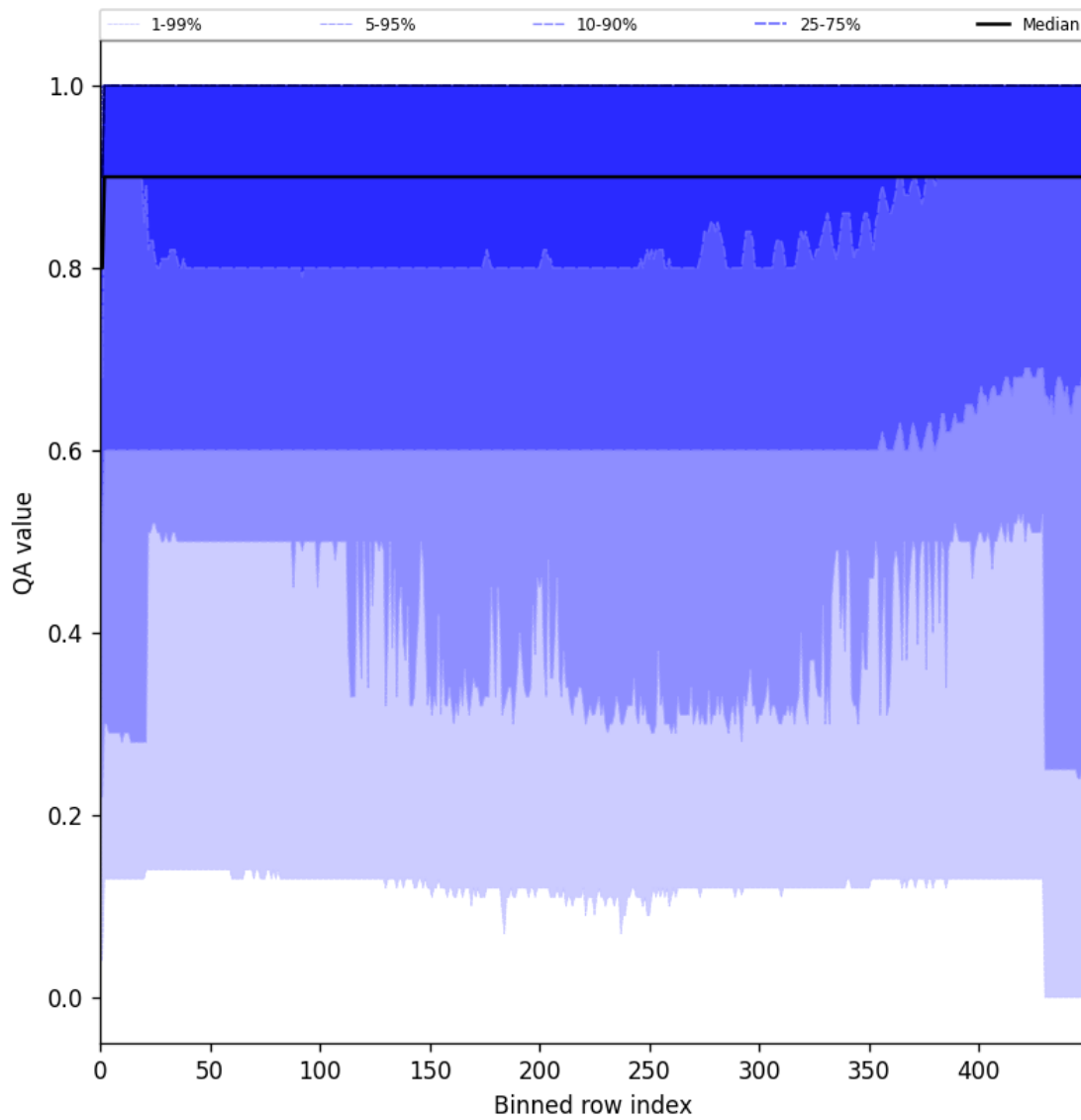
Figure 27: Along track statistics of “QA value” for 2025-01-04 to 2025-01-06
