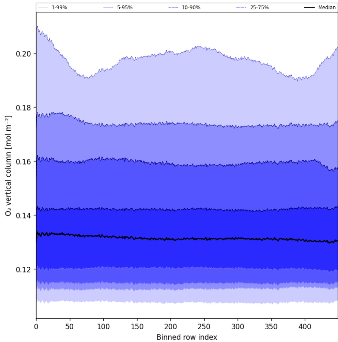
Figure 28: Along track statistics of “O 3 vertical column” for 2025-01-04 to 2025-01-06
