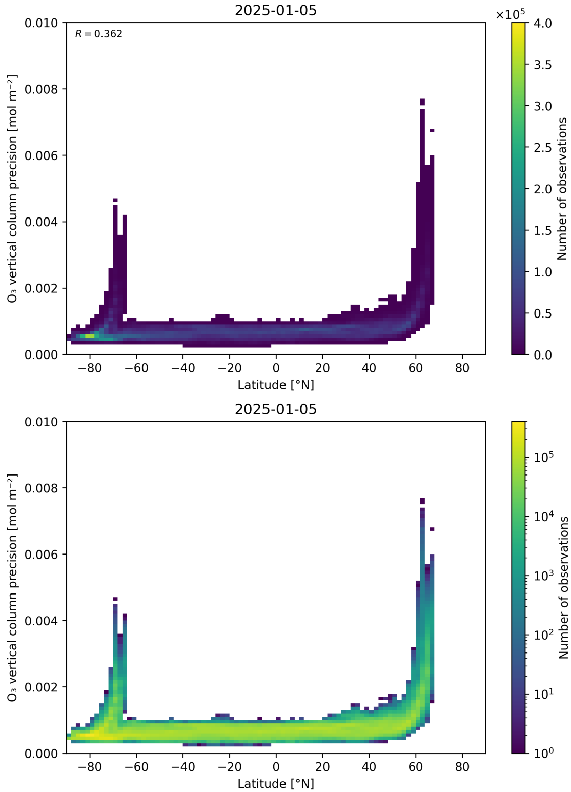
Figure 37: Scatter density plot of “Latitude” against “O 3 vertical column precision” for 2025-01-04 to 2025-01-06.
