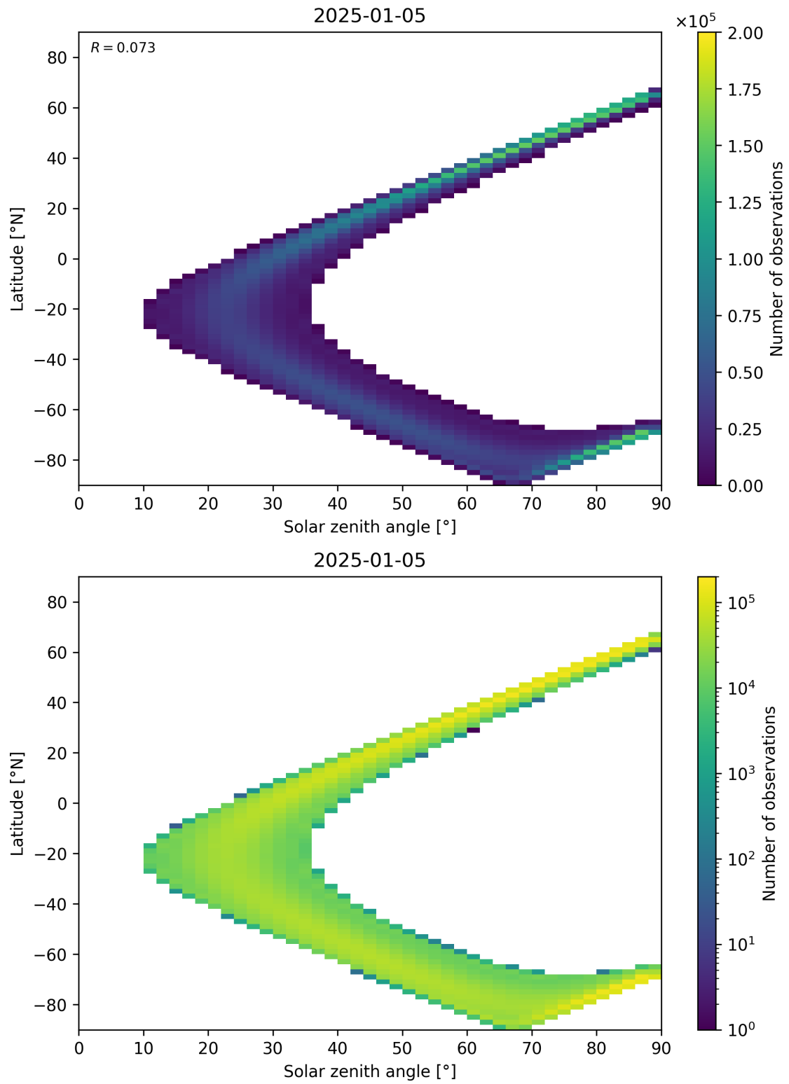
Figure 44: Scatter density plot of “Solar zenith angle” against “Latitude” for 2025-01-04 to 2025-01-06.
