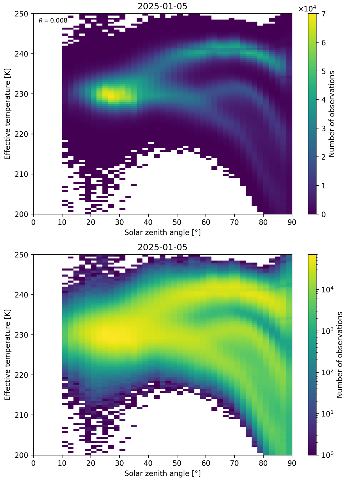
Figure 45: Scatter density plot of “Solar zenith angle” against “Effective temperature” for 2025-01-04 to 2025-01-06.
