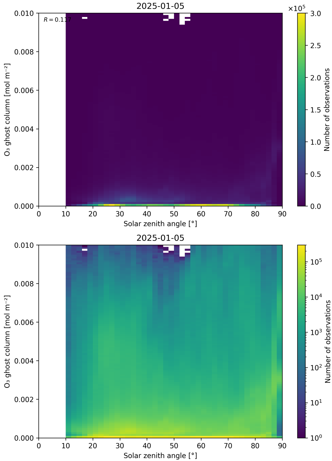
Figure 46: Scatter density plot of “Solar zenith angle” against “O 3 ghost column” for 2025-01-04 to 2025-01-06.
