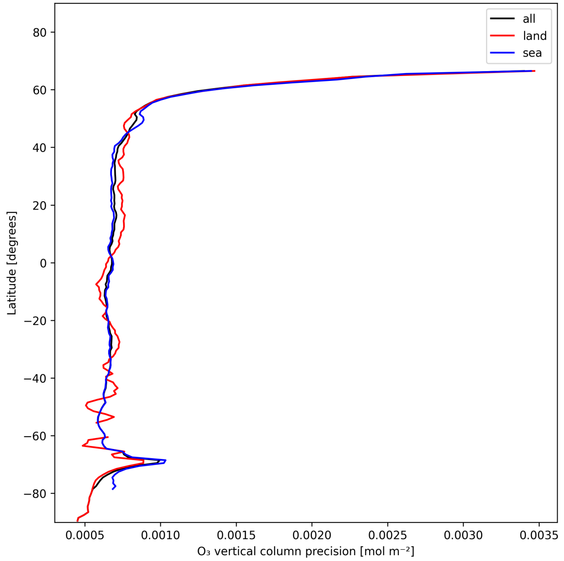
Figure 15: Zonal average of “O 3 vertical column precision” for 2025-01-05 to 2025-01-07.
