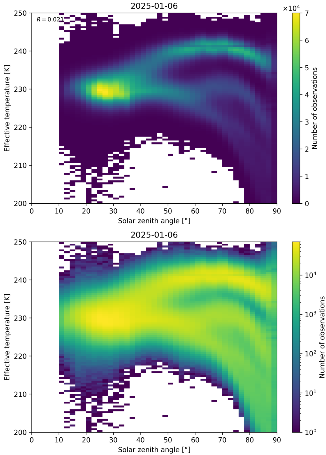
Figure 45: Scatter density plot of “Solar zenith angle” against “Effective temperature” for 2025-01-05 to 2025-01-07.
