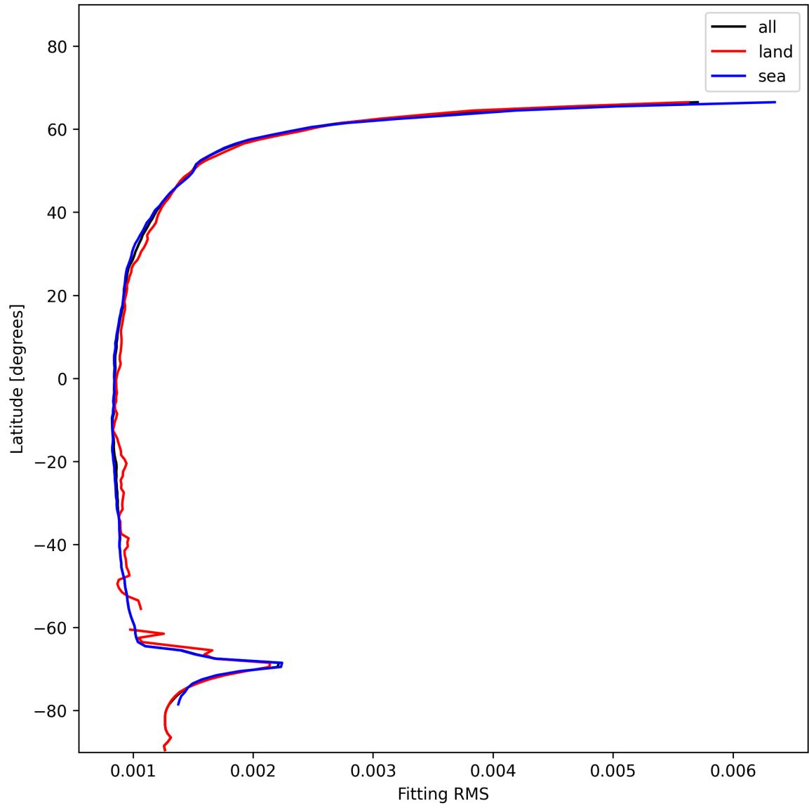
Figure 16: Zonal average of “Fitting RMS” for 2025-01-05 to 2025-01-07.
