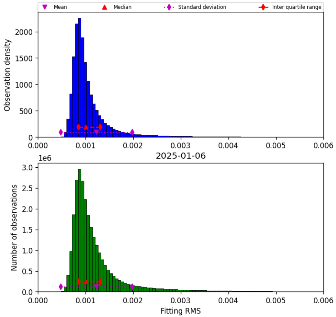
Figure 23: Histogram of “Fitting RMS” for 2025-01-05 to 2025-01-07
