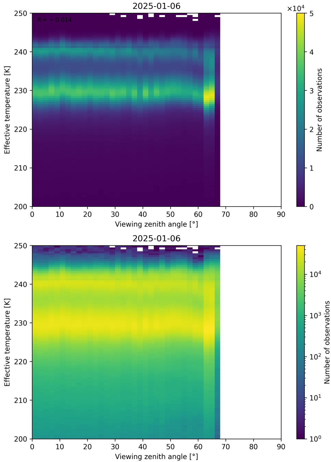
Figure 50: Scatter density plot of “Viewing zenith angle” against “Effective temperature” for 2025-01-05 to 2025-01-07.
