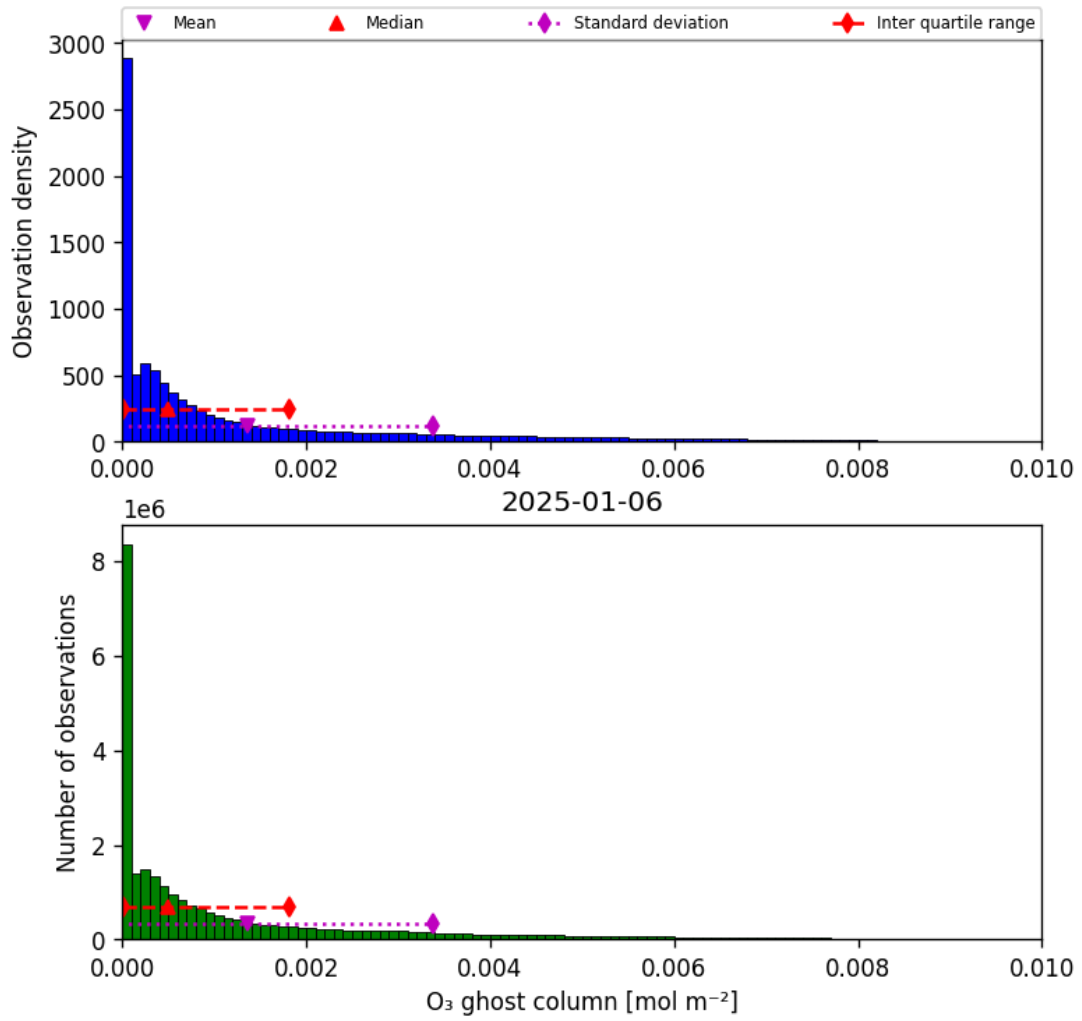
Figure 25: Histogram of “O 3 ghost column” for 2025-01-05 to 2025-01-07
