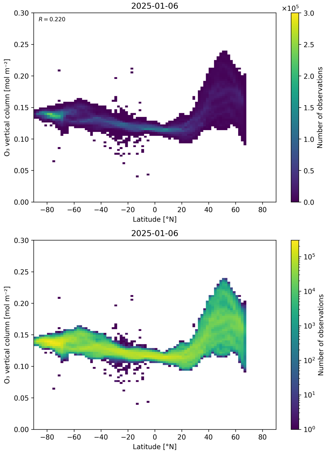
Figure 36: Scatter density plot of “Latitude” against “O 3 vertical column” for 2025-01-05 to 2025-01-07.
