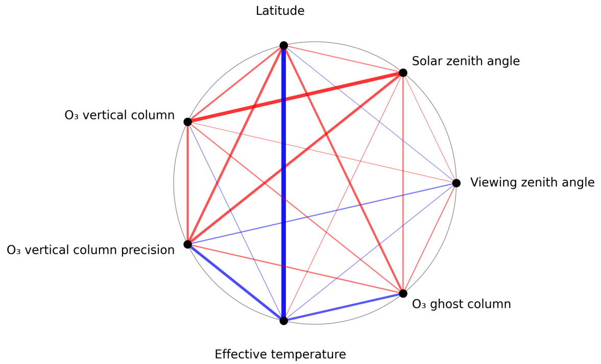
Figure 1: Map of correlation graph for 2025-01-05 to 2025-01-07.
