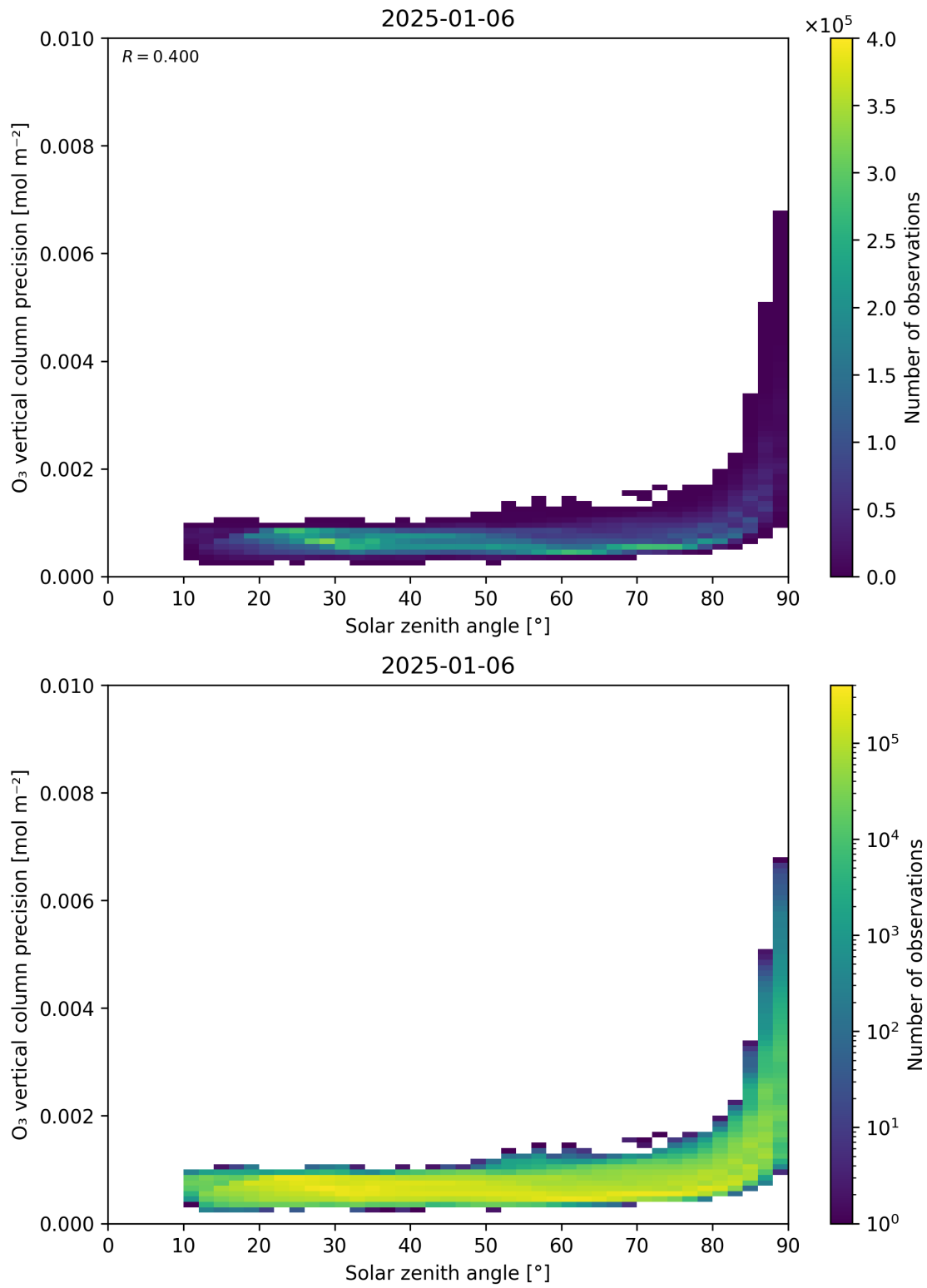
Figure 48: Scatter density plot of “Solar zenith angle” against “O 3 vertical column precision” for 2025-01-05 to 2025-01-07.
