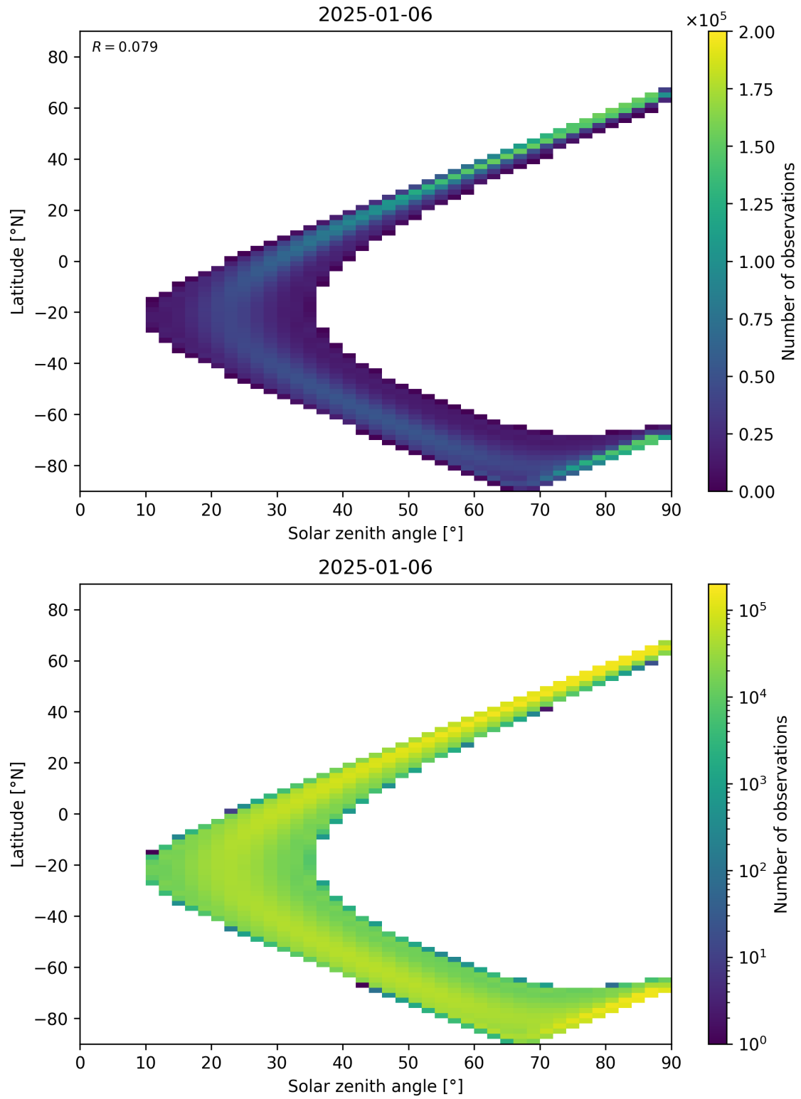
Figure 44: Scatter density plot of “Solar zenith angle” against “Latitude” for 2025-01-05 to 2025-01-07.
