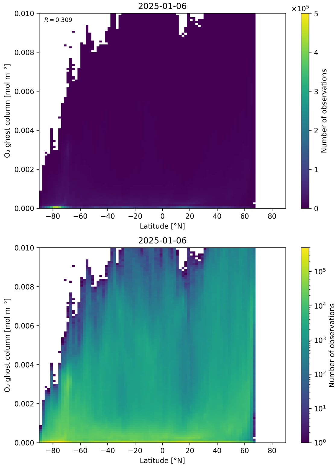
Figure 35: Scatter density plot of “Latitude” against “O 3 ghost column” for 2025-01-05 to 2025-01-07.
