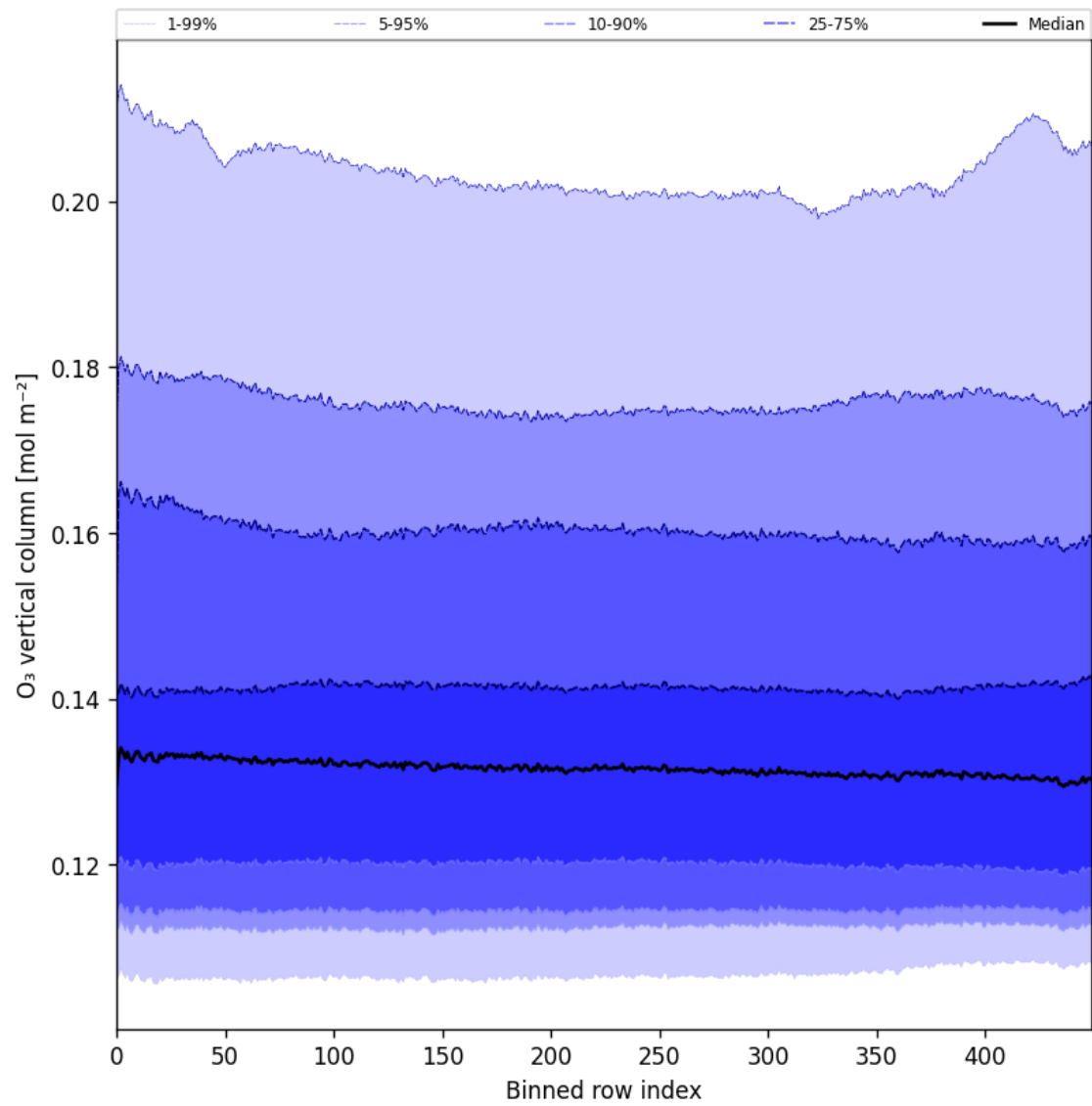
Figure 28: Along track statistics of “O 3 vertical column” for 2025-01-05 to 2025-01-07
