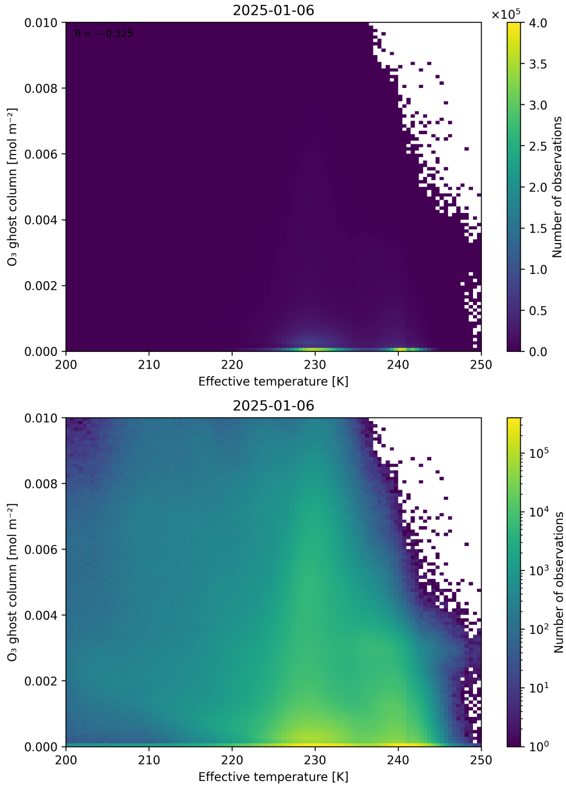
Figure 38: Scatter density plot of “Effective temperature” against “O 3 ghost column” for 2025-01-05 to 2025-01-07.
