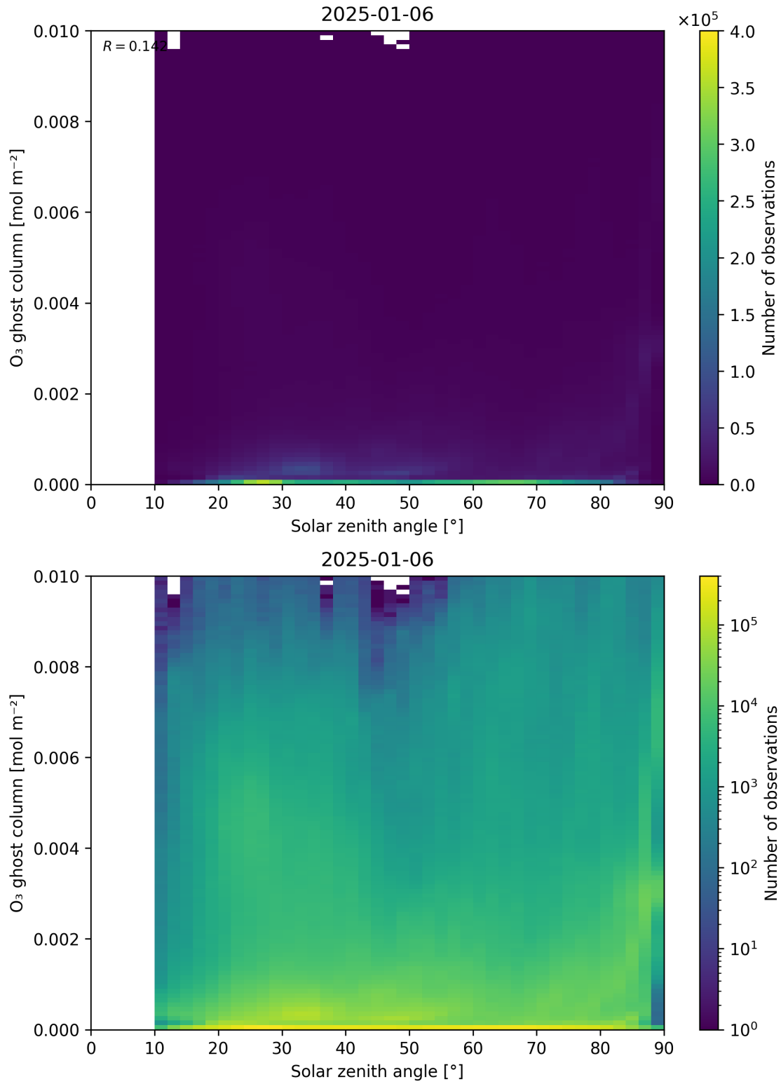
Figure 46: Scatter density plot of “Solar zenith angle” against “O 3 ghost column” for 2025-01-05 to 2025-01-07.
