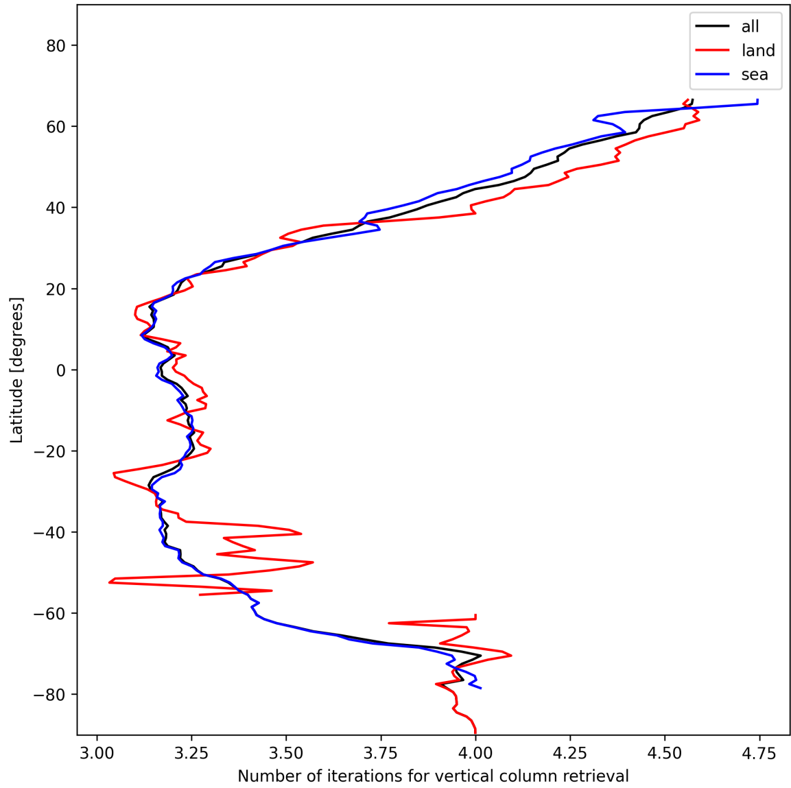
Figure 19: Zonal average of “Number of iterations for vertical column retrieval” for 2025-01-05 to 2025-01-07.
