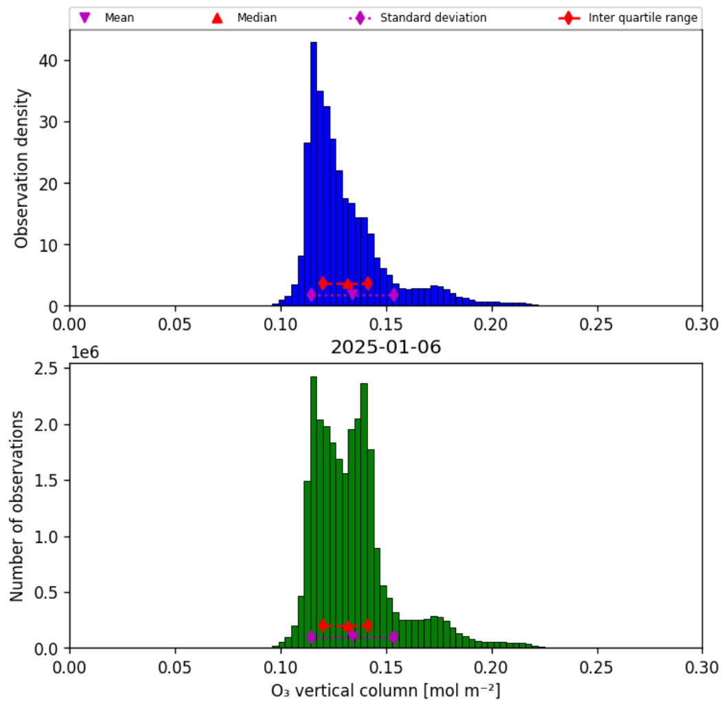
Figure 21: Histogram of “O 3 vertical column” for 2025-01-05 to 2025-01-07
