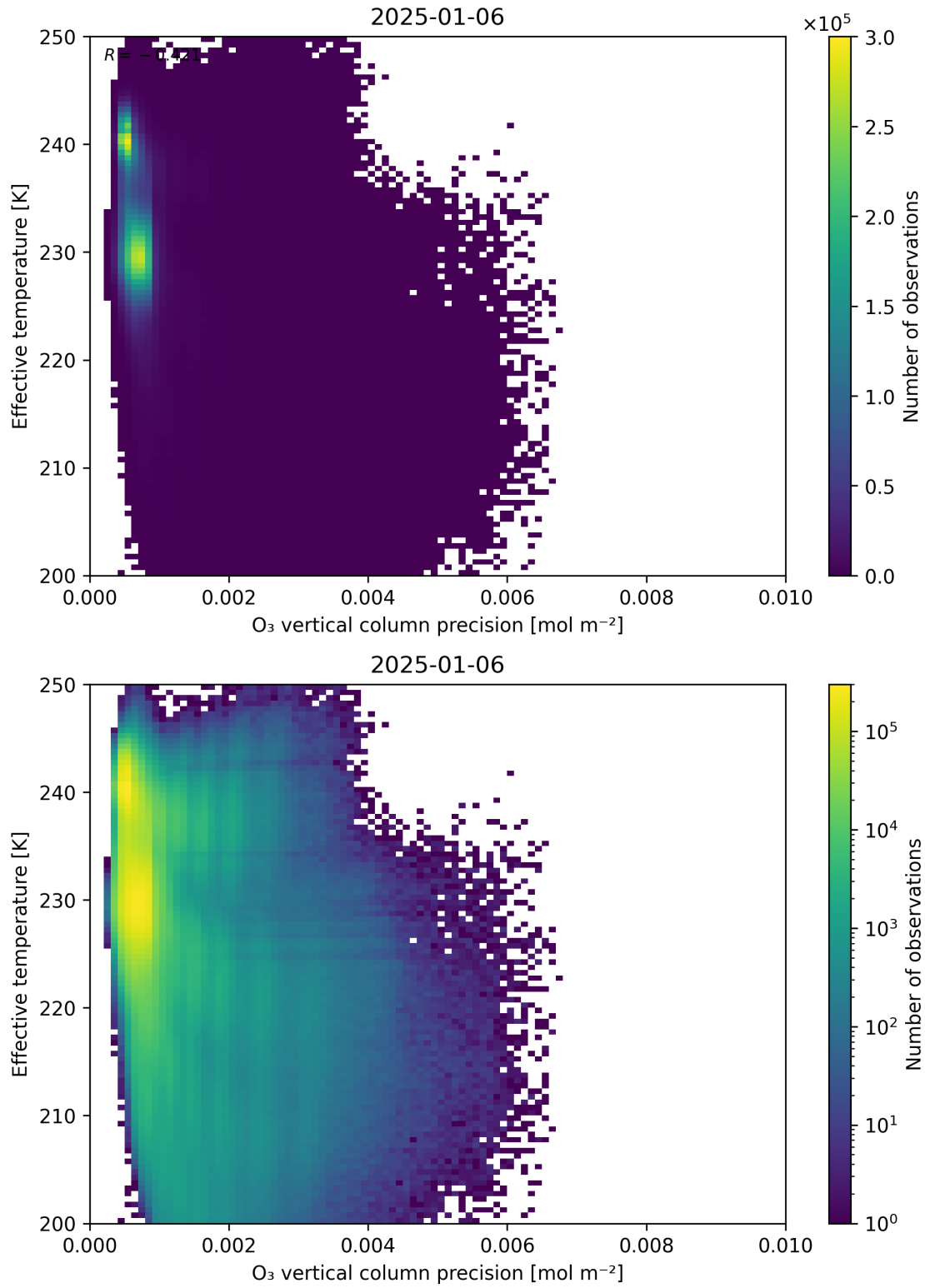
Figure 42: Scatter density plot of “O 3 vertical column precision” against “Effective temperature” for 2025-01-05 to 2025-01-07.
