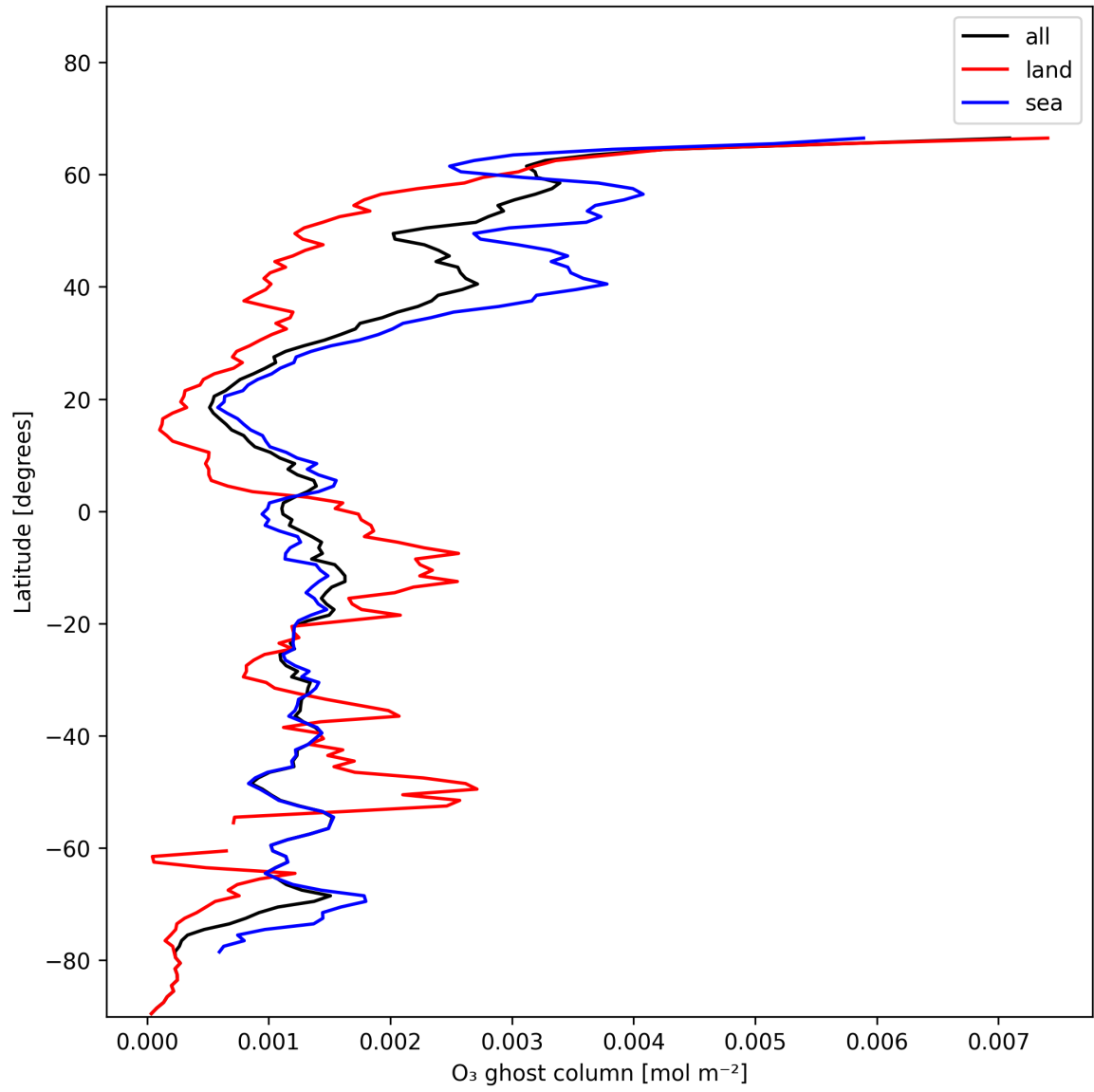
Figure 18: Zonal average of “O 3 ghost column” for 2025-01-05 to 2025-01-07.
