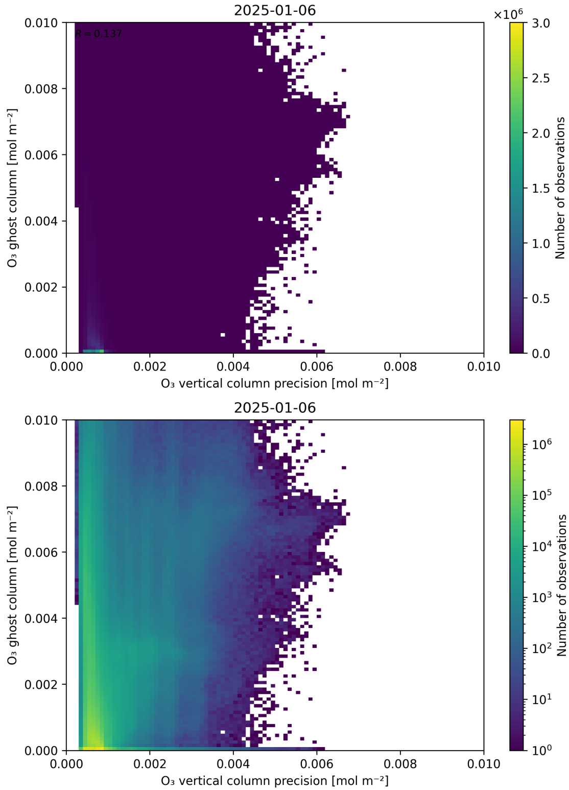
Figure 43: Scatter density plot of “O 3 vertical column precision” against “O 3 ghost column” for 2025-01-05 to 2025-01-07.
