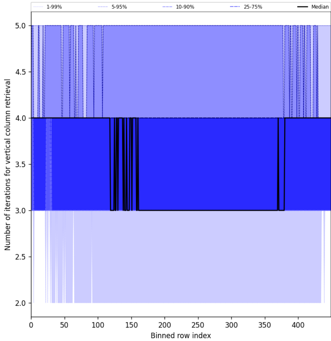
Figure 33: Along track statistics of “Number of iterations for vertical column retrieval” for 2025-01-05 to 2025-01-07
