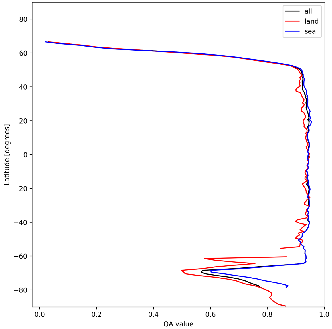
Figure 13: Zonal average of “QA value” for 2025-01-05 to 2025-01-07.
