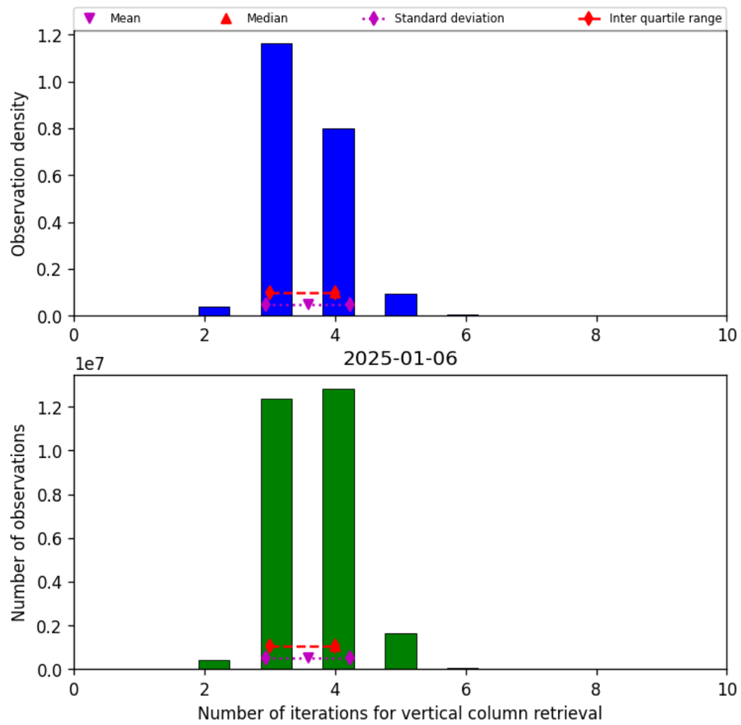
Figure 26: Histogram of “Number of iterations for vertical column retrieval” for 2025-01-05 to 2025-01-07
