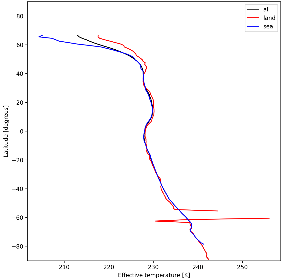
Figure 17: Zonal average of “Effective temperature” for 2025-01-05 to 2025-01-07.
