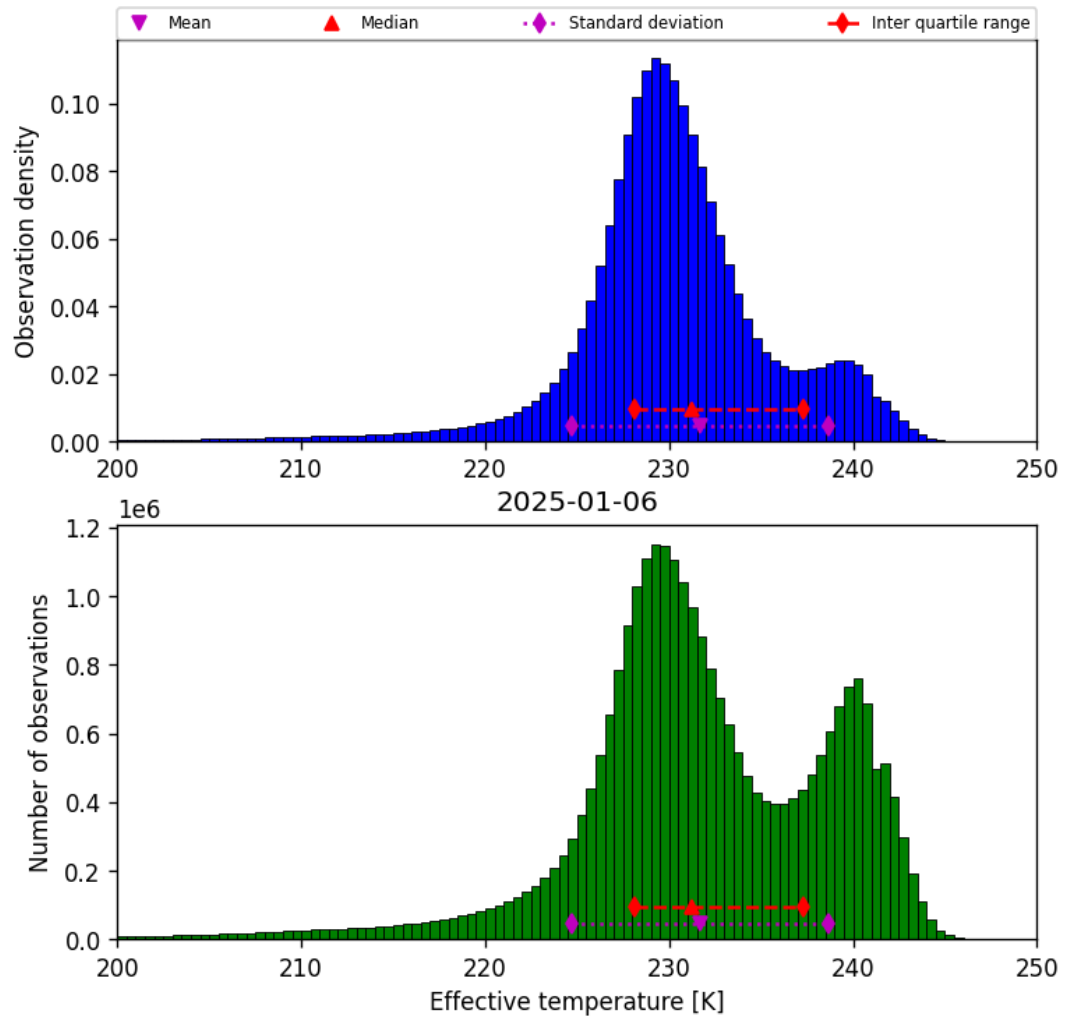
Figure 24: Histogram of “Effective temperature” for 2025-01-05 to 2025-01-07
