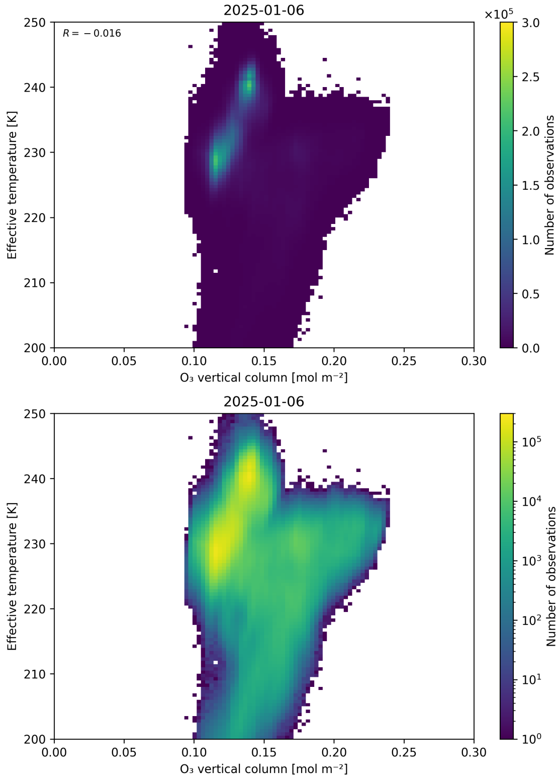
Figure 39: Scatter density plot of “O 3 vertical column” against “Effective temperature” for 2025-01-05 to 2025-01-07.
