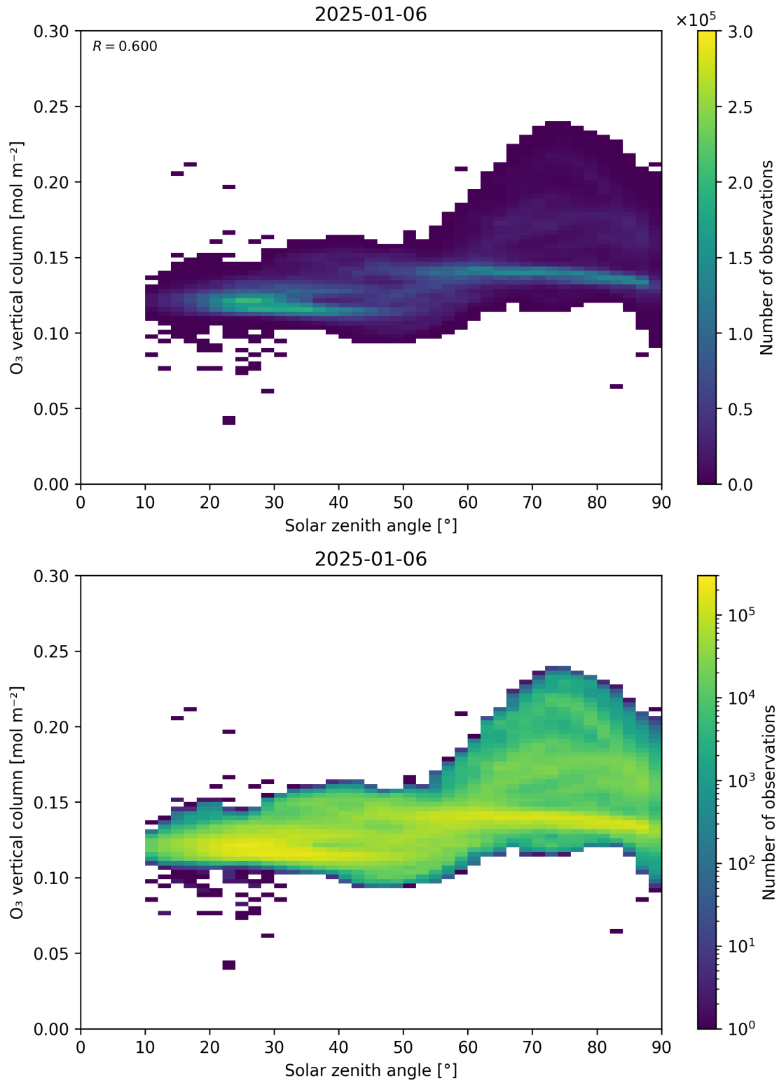
Figure 47: Scatter density plot of “Solar zenith angle” against “O 3 vertical column” for 2025-01-05 to 2025-01-07.
