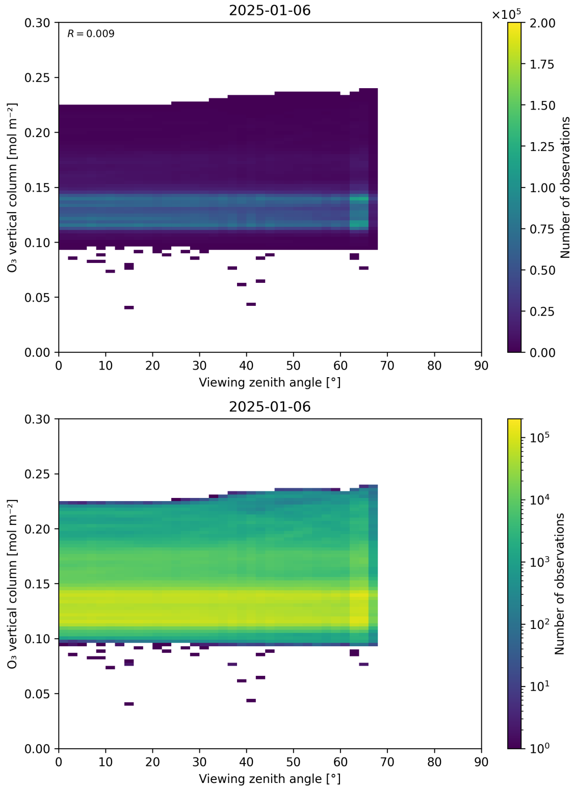
Figure 52: Scatter density plot of “Viewing zenith angle” against “O 3 vertical column” for 2025-01-05 to 2025-01-07.
