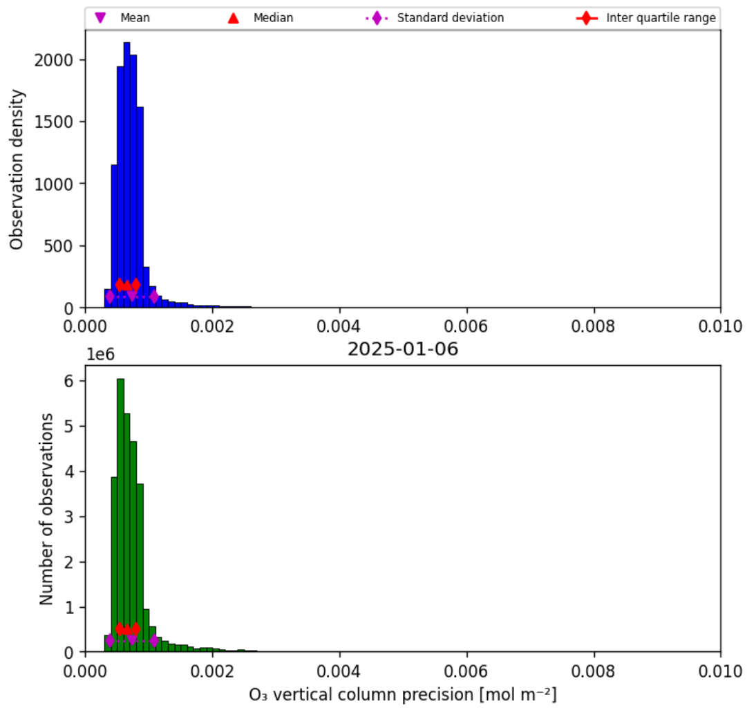
Figure 22: Histogram of “O 3 vertical column precision” for 2025-01-05 to 2025-01-07
