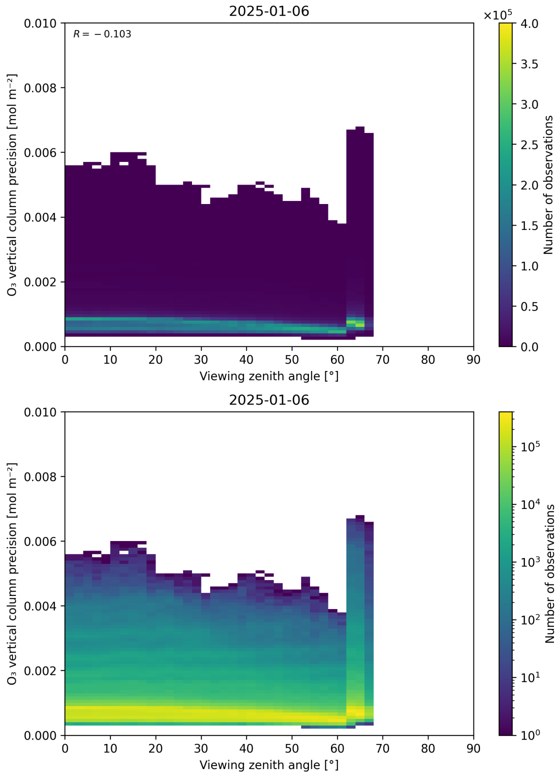
Figure 53: Scatter density plot of “Viewing zenith angle” against “O 3 vertical column precision” for 2025-01-05 to 2025-01-07.
