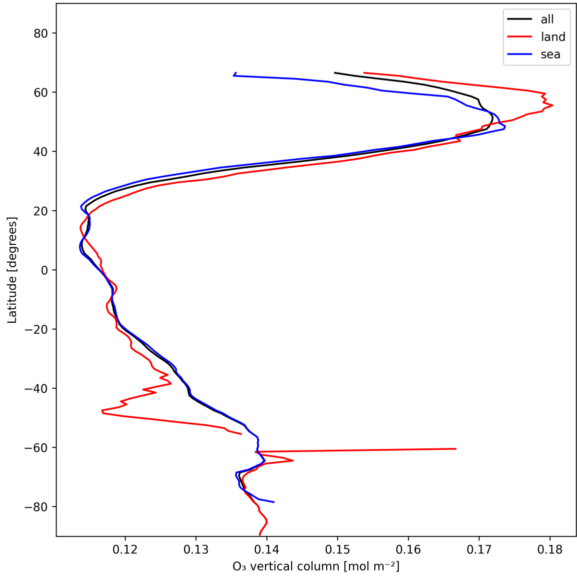
Figure 14: Zonal average of “O 3 vertical column” for 2025-01-05 to 2025-01-07.
