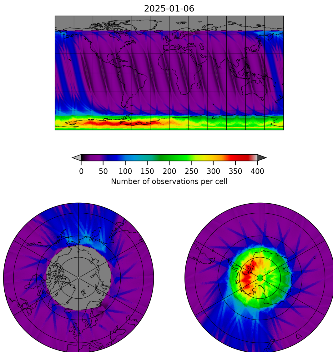
Figure 12: Map of the number of observations for 2025-01-05 to 2025-01-07
