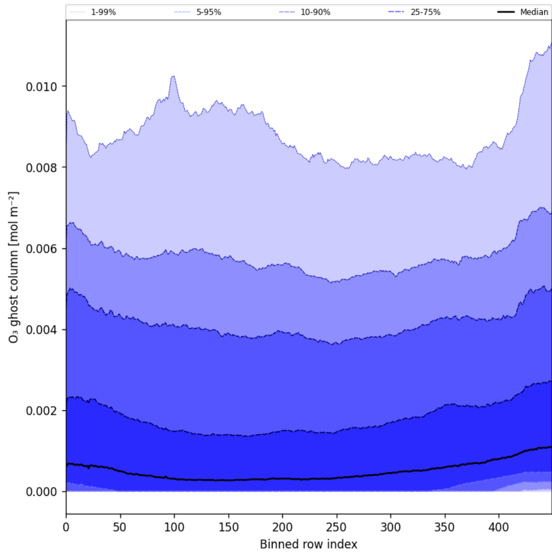
Figure 32: Along track statistics of “O 3 ghost column” for 2025-01-05 to 2025-01-07
