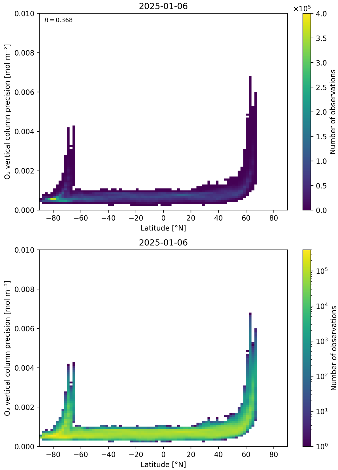
Figure 37: Scatter density plot of “Latitude” against “O 3 vertical column precision” for 2025-01-05 to 2025-01-07.
