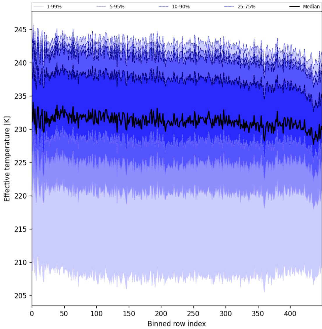
Figure 31: Along track statistics of “Effective temperature” for 2025-01-05 to 2025-01-07
