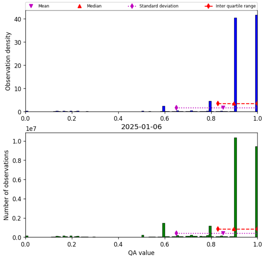
Figure 20: Histogram of “QA value” for 2025-01-05 to 2025-01-07
