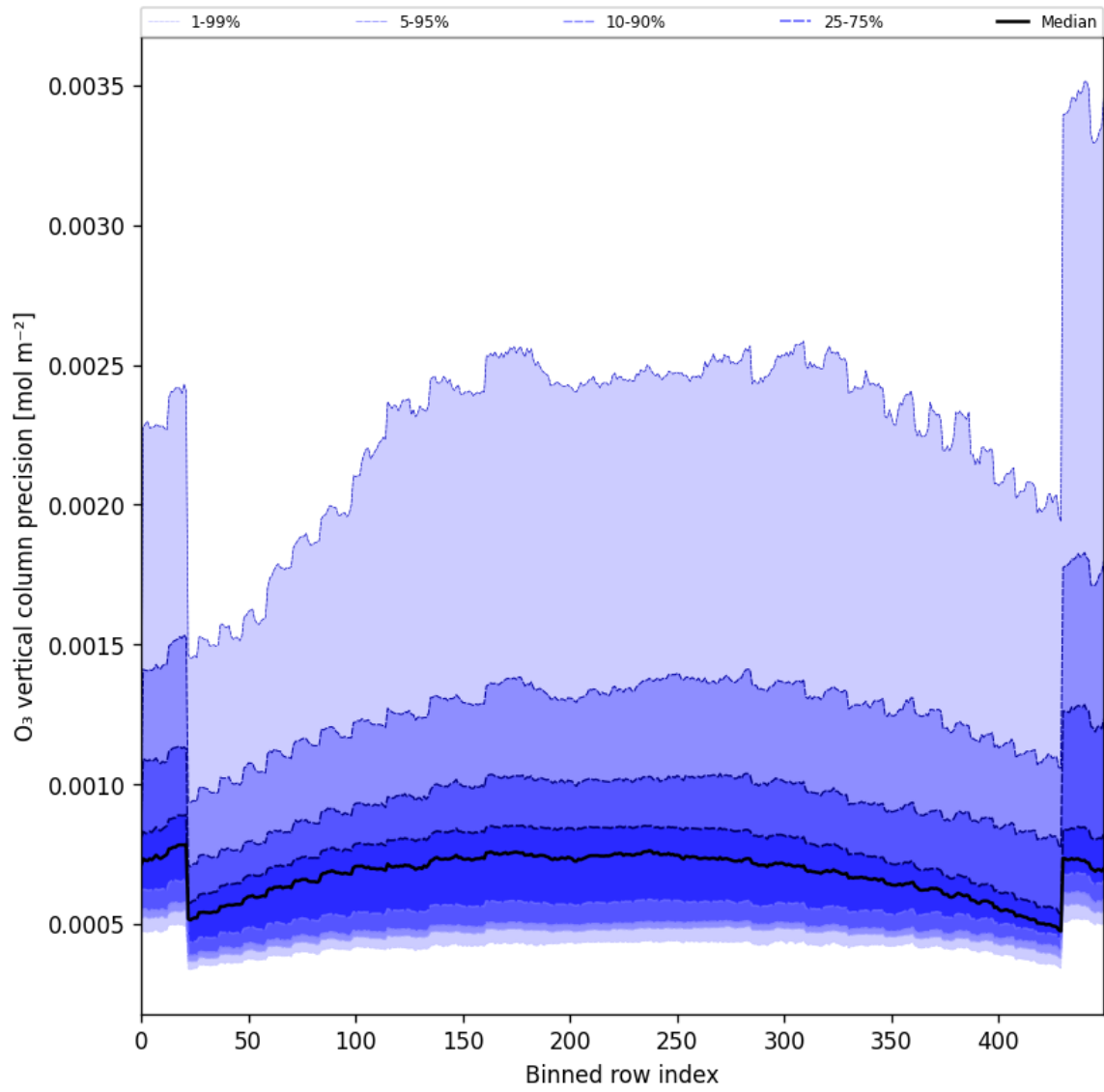
Figure 29: Along track statistics of “O 3 vertical column precision” for 2025-01-05 to 2025-01-07
