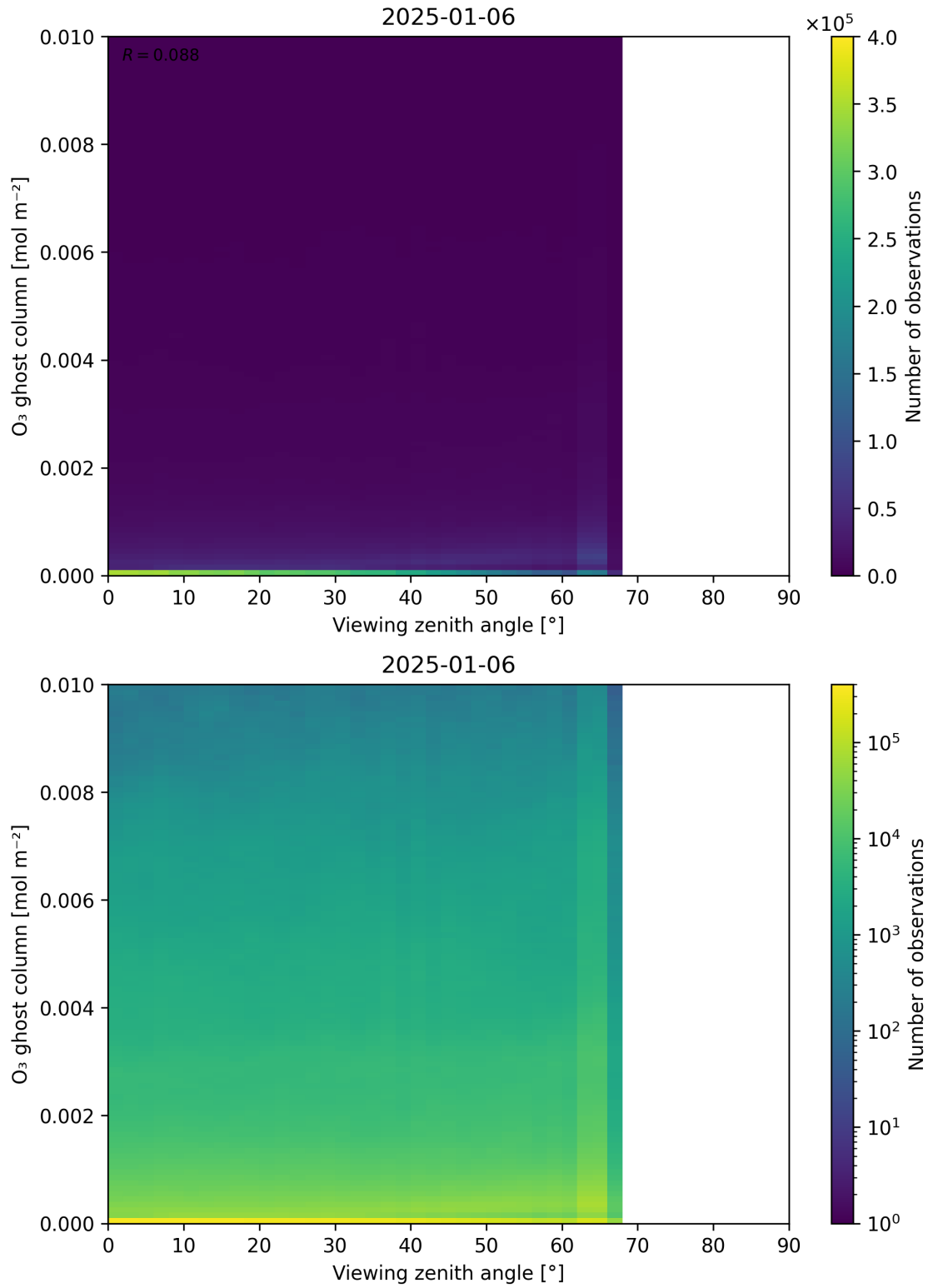
Figure 51: Scatter density plot of “Viewing zenith angle” against “O 3 ghost column” for 2025-01-05 to 2025-01-07.
