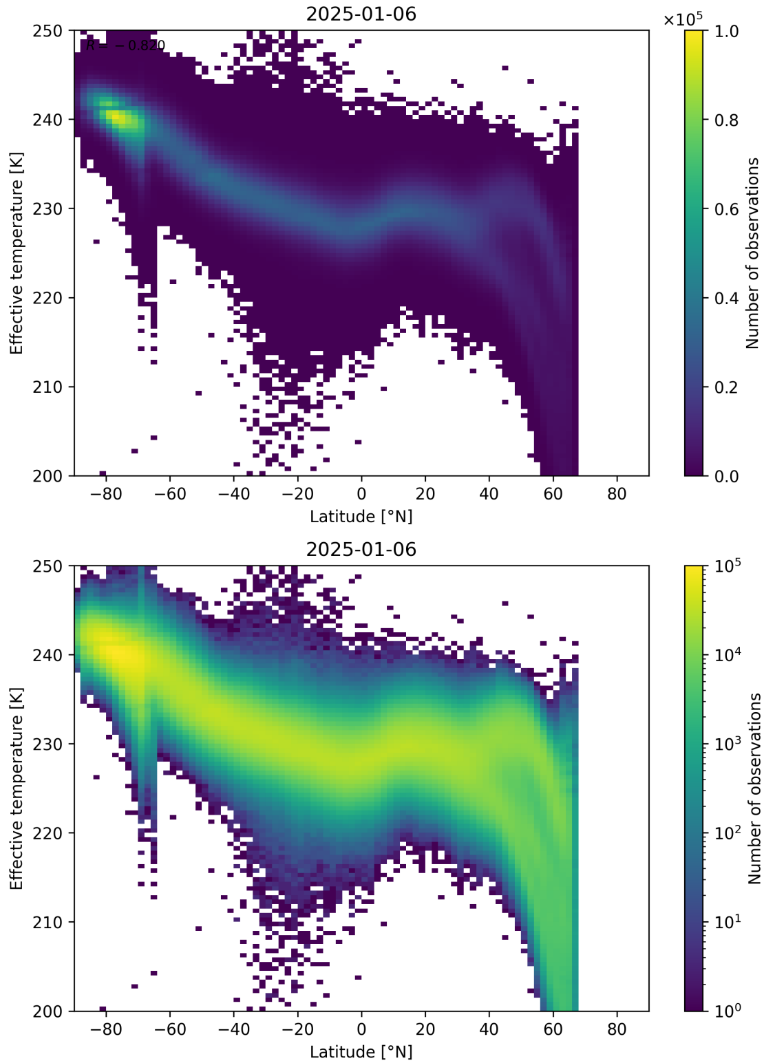
Figure 34: Scatter density plot of “Latitude” against “Effective temperature” for 2025-01-05 to 2025-01-07.
