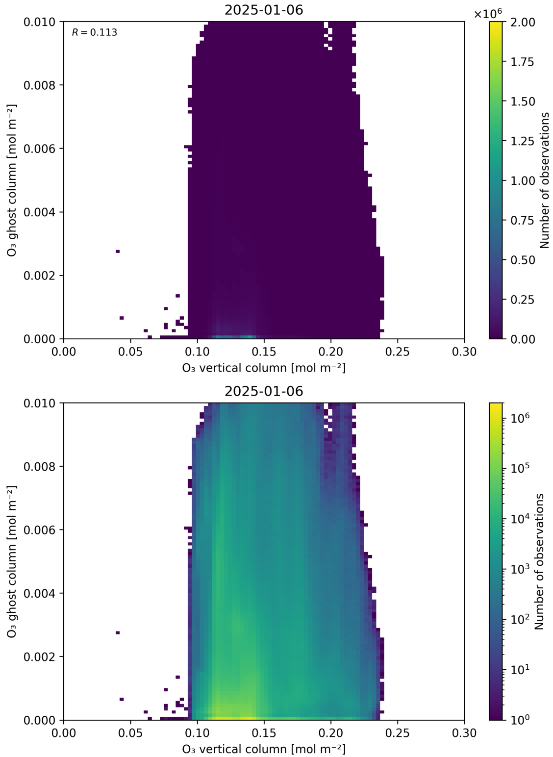
Figure 40: Scatter density plot of “O 3 vertical column” against “O 3 ghost column” for 2025-01-05 to 2025-01-07.
