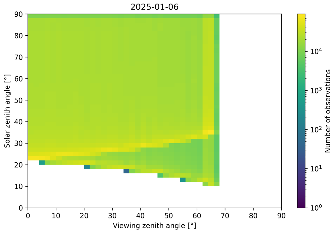
Figure 54: Scatter density plot of “Viewing zenith angle” against “Solar zenith angle” for 2025-01-05 to 2025-01-07.
