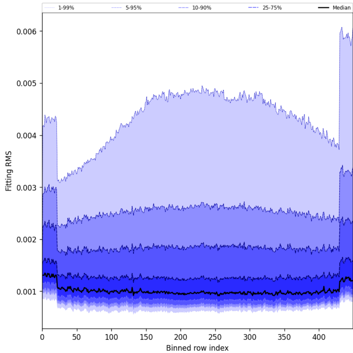
Figure 30: Along track statistics of “Fitting RMS” for 2025-01-05 to 2025-01-07
