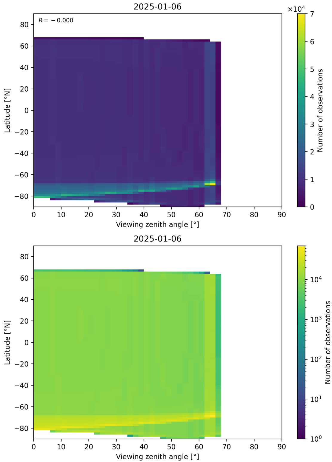
Figure 49: Scatter density plot of “Viewing zenith angle” against “Latitude” for 2025-01-05 to 2025-01-07.
