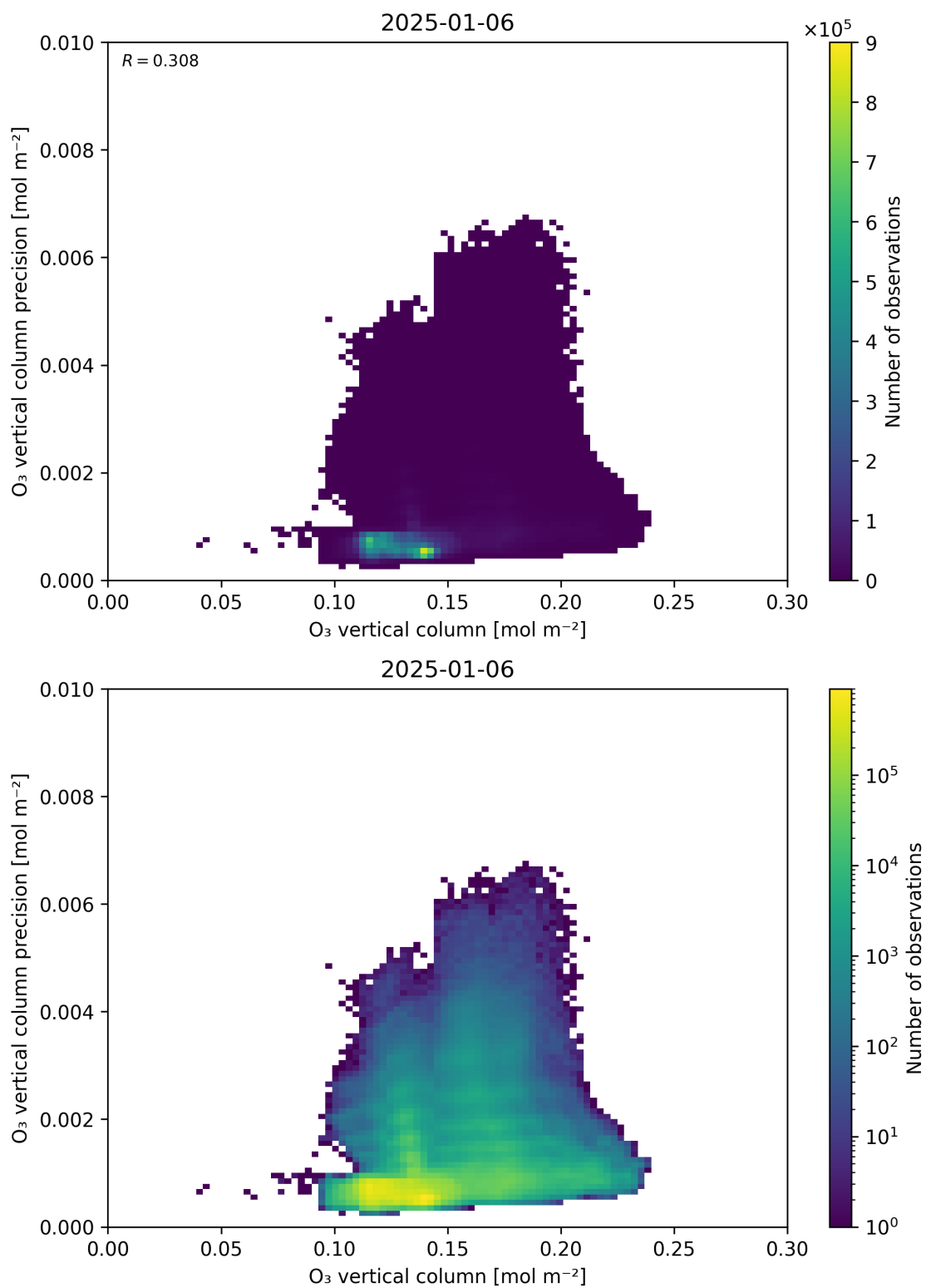
Figure 41: Scatter density plot of “O 3 vertical column” against “O 3 vertical column precision” for 2025-01-05 to 2025-01-07.
