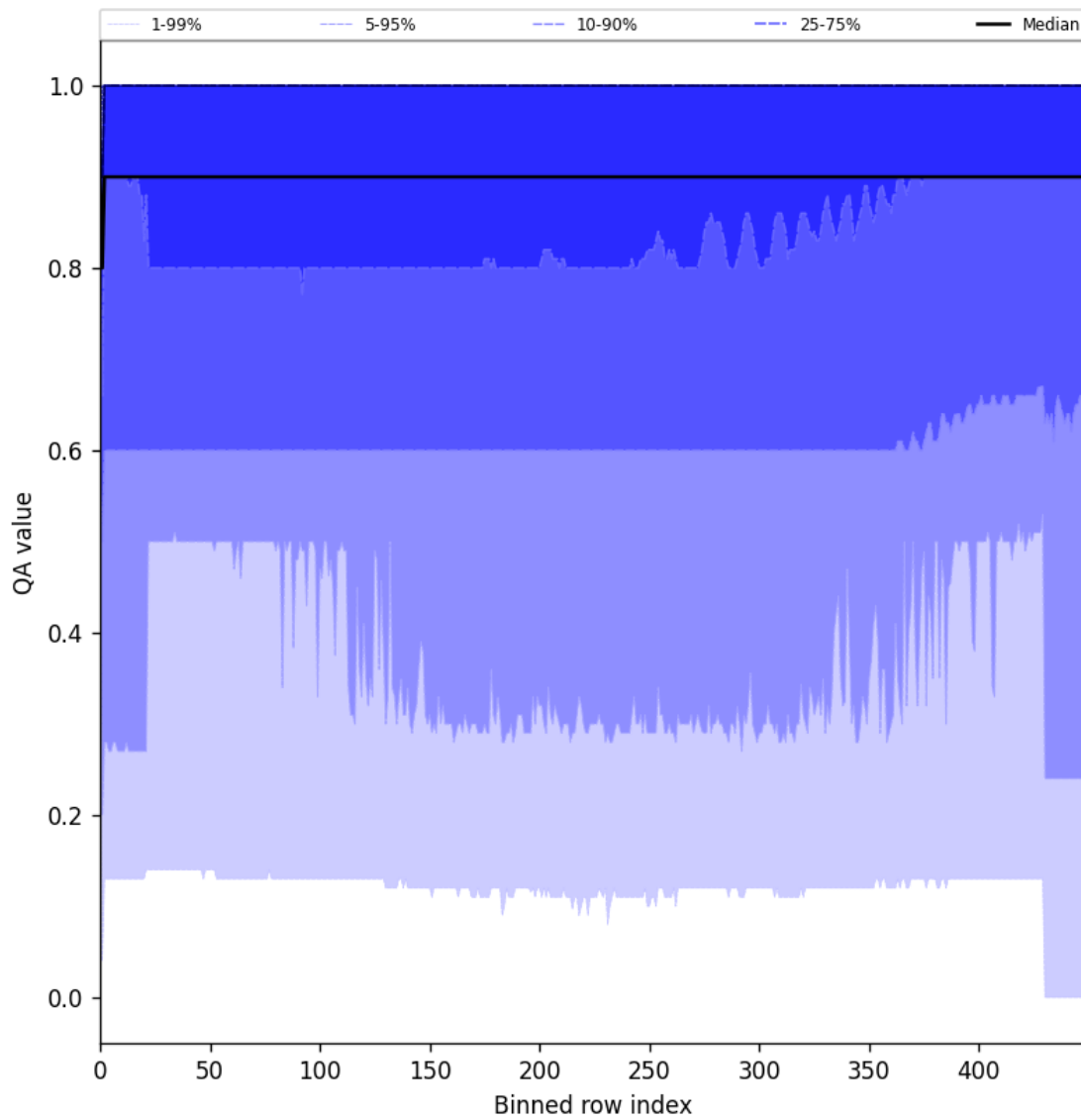
Figure 27: Along track statistics of “QA value” for 2025-01-05 to 2025-01-07
