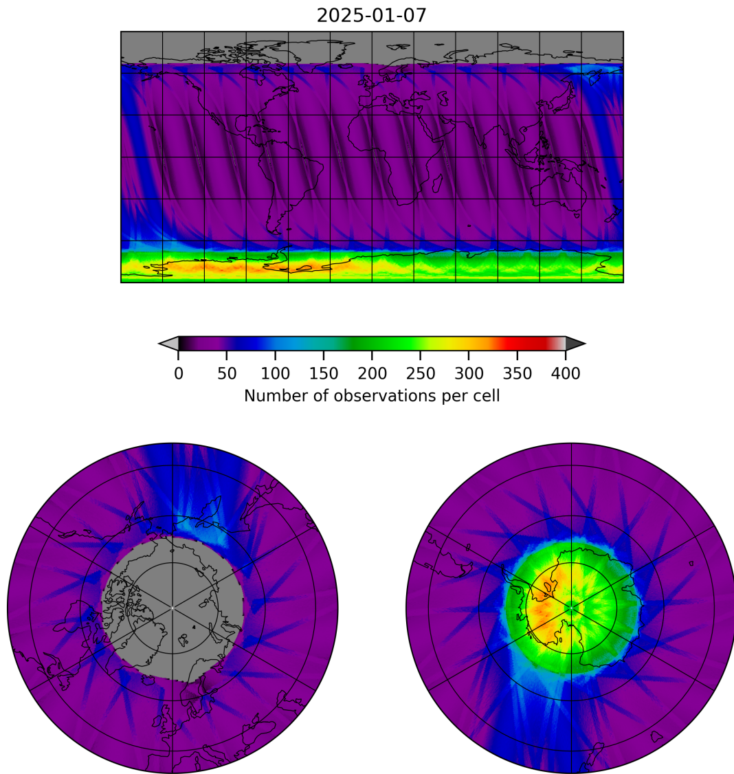
Figure 12: Map of the number of observations for 2025-01-07 to 2025-01-08
