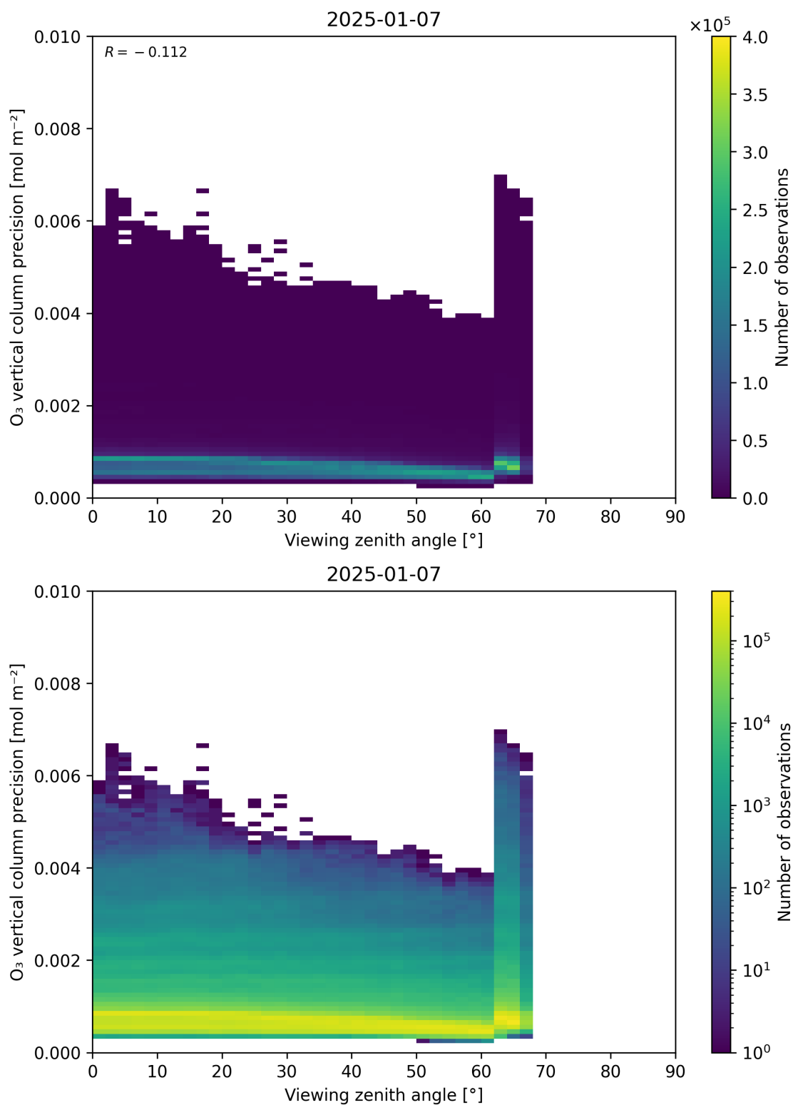
Figure 53: Scatter density plot of “Viewing zenith angle” against “O 3 vertical column precision” for 2025-01-07 to 2025-01-08.
