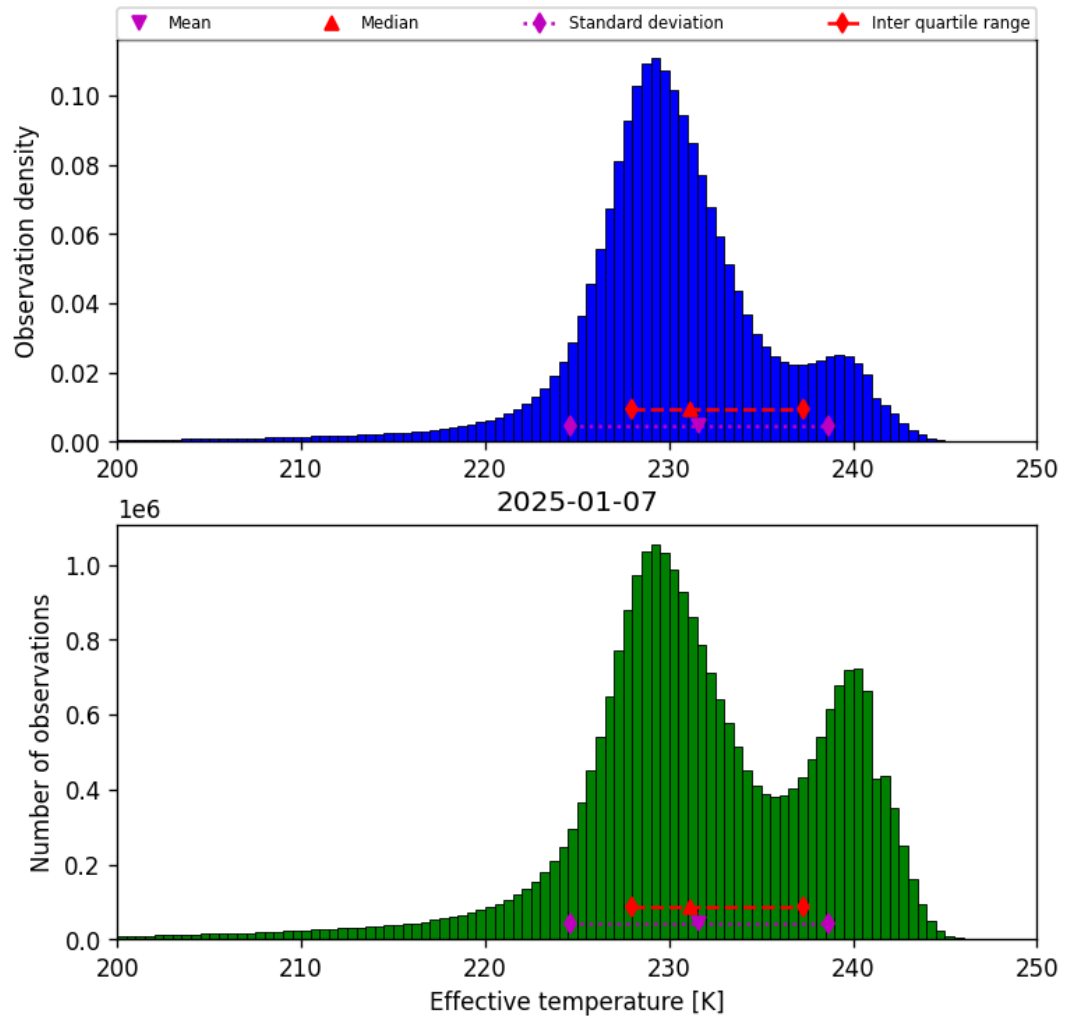
Figure 24: Histogram of “Effective temperature” for 2025-01-07 to 2025-01-08
