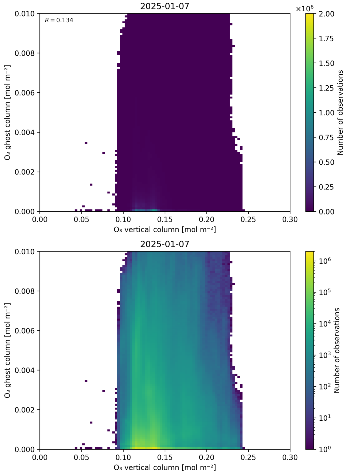
Figure 40: Scatter density plot of “O 3 vertical column” against “O 3 ghost column” for 2025-01-07 to 2025-01-08.
