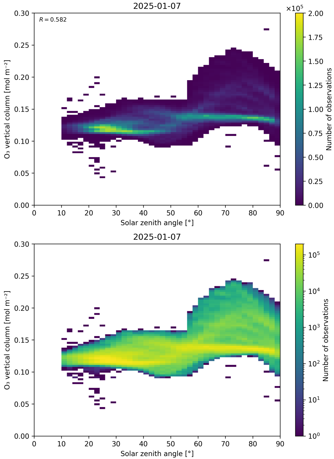
Figure 47: Scatter density plot of “Solar zenith angle” against “O 3 vertical column” for 2025-01-07 to 2025-01-08.
