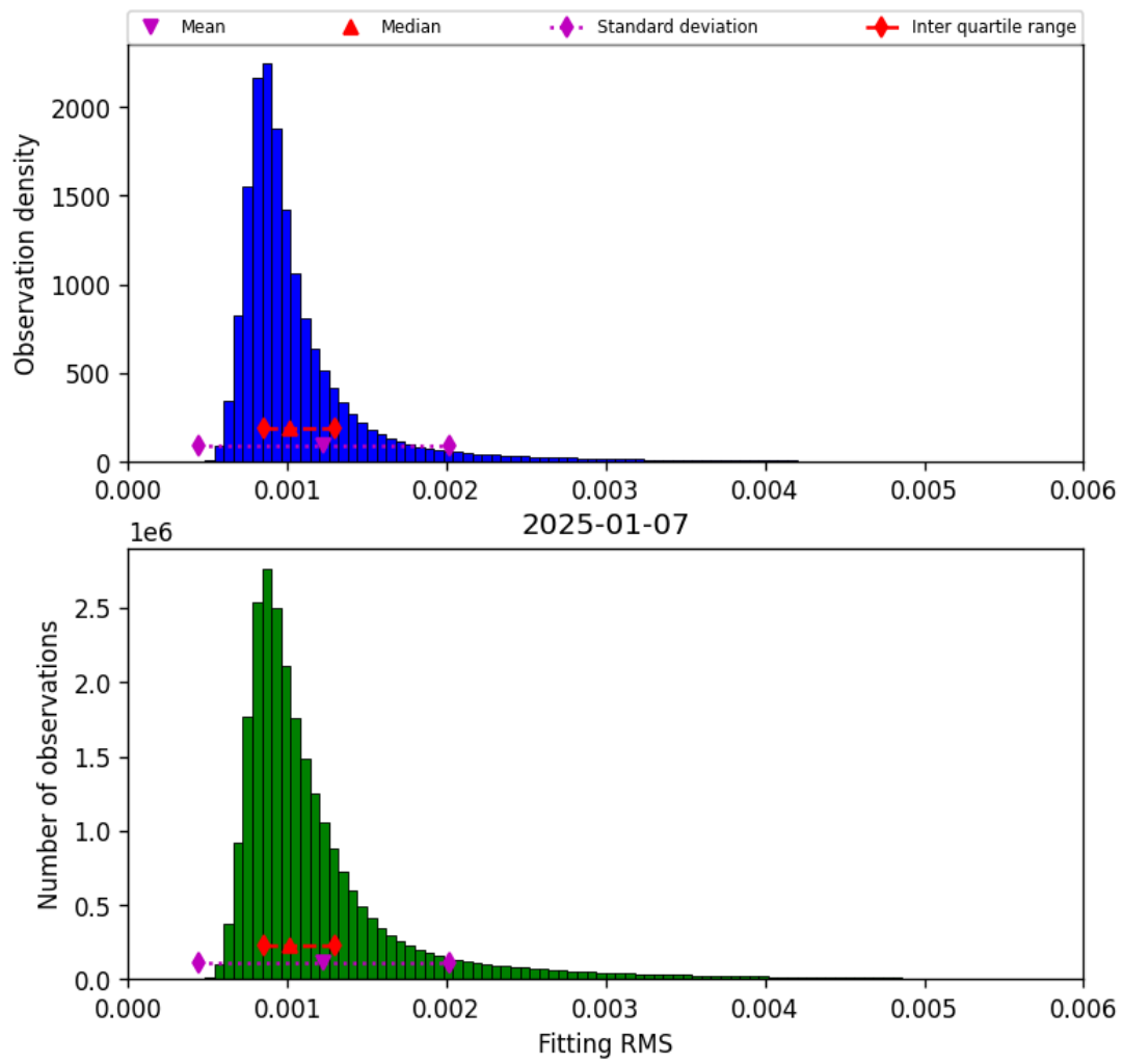
Figure 23: Histogram of “Fitting RMS” for 2025-01-07 to 2025-01-08
