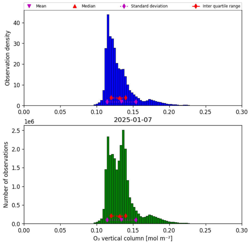
Figure 21: Histogram of “O 3 vertical column” for 2025-01-07 to 2025-01-08
