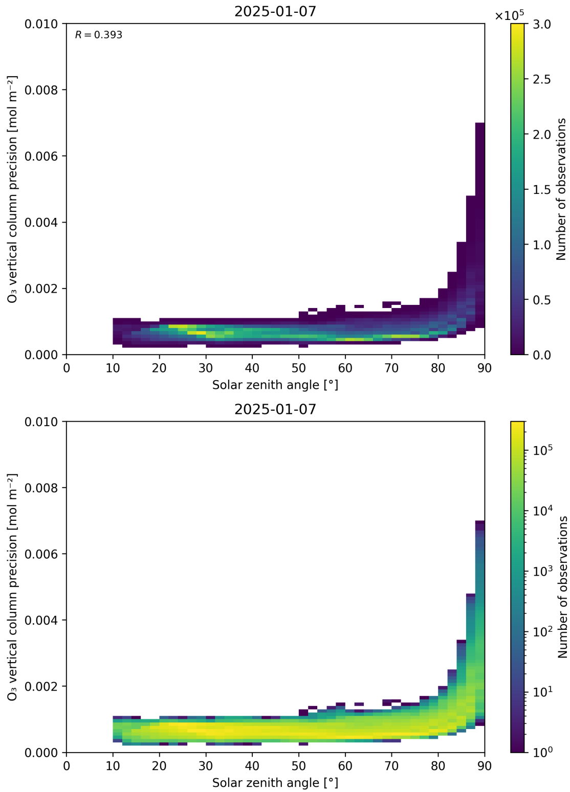
Figure 48: Scatter density plot of “Solar zenith angle” against “O 3 vertical column precision” for 2025-01-07 to 2025-01-08.
