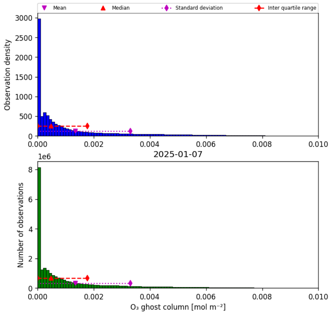
Figure 25: Histogram of “O 3 ghost column” for 2025-01-07 to 2025-01-08
