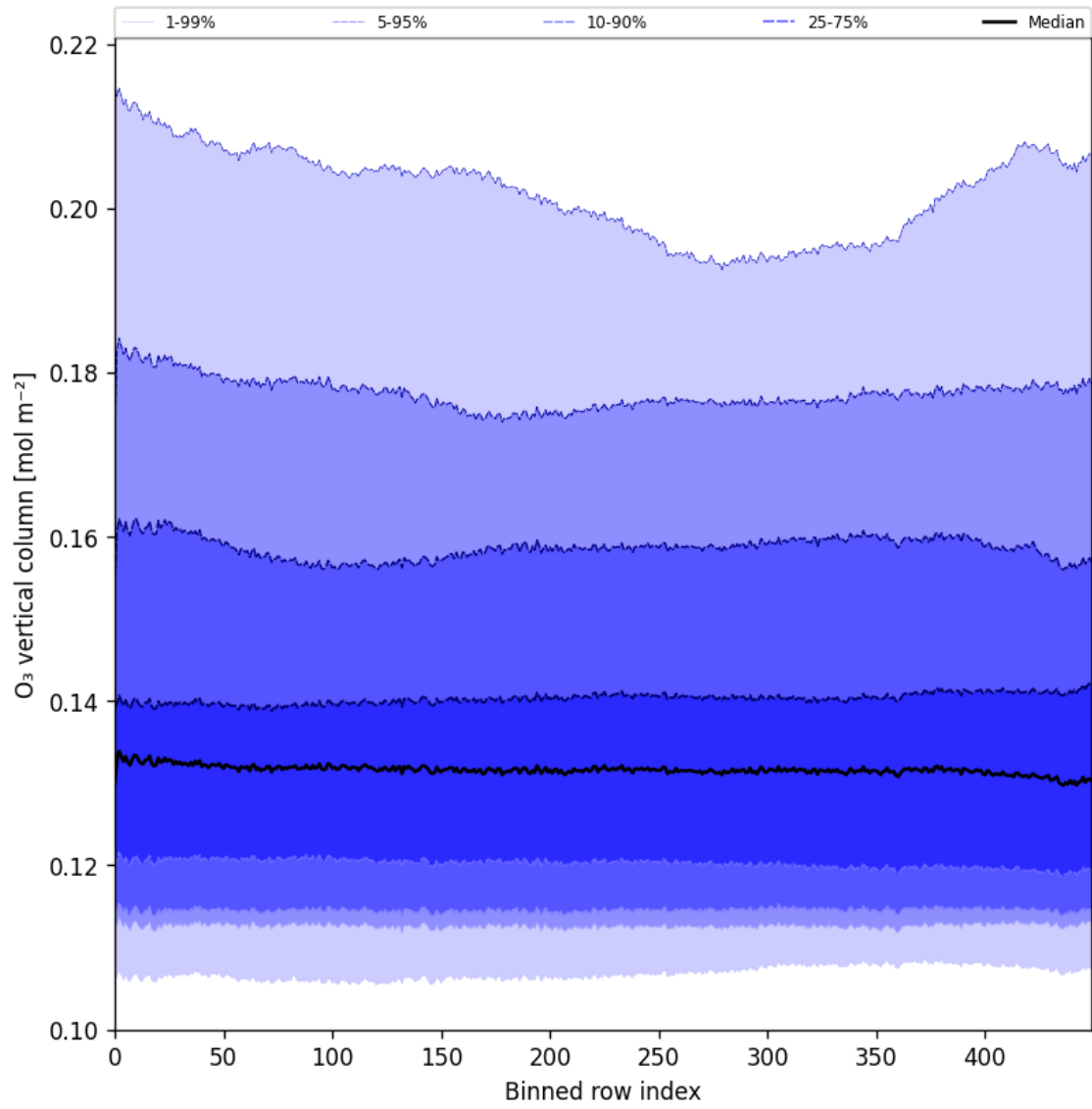
Figure 28: Along track statistics of “O 3 vertical column” for 2025-01-07 to 2025-01-08
