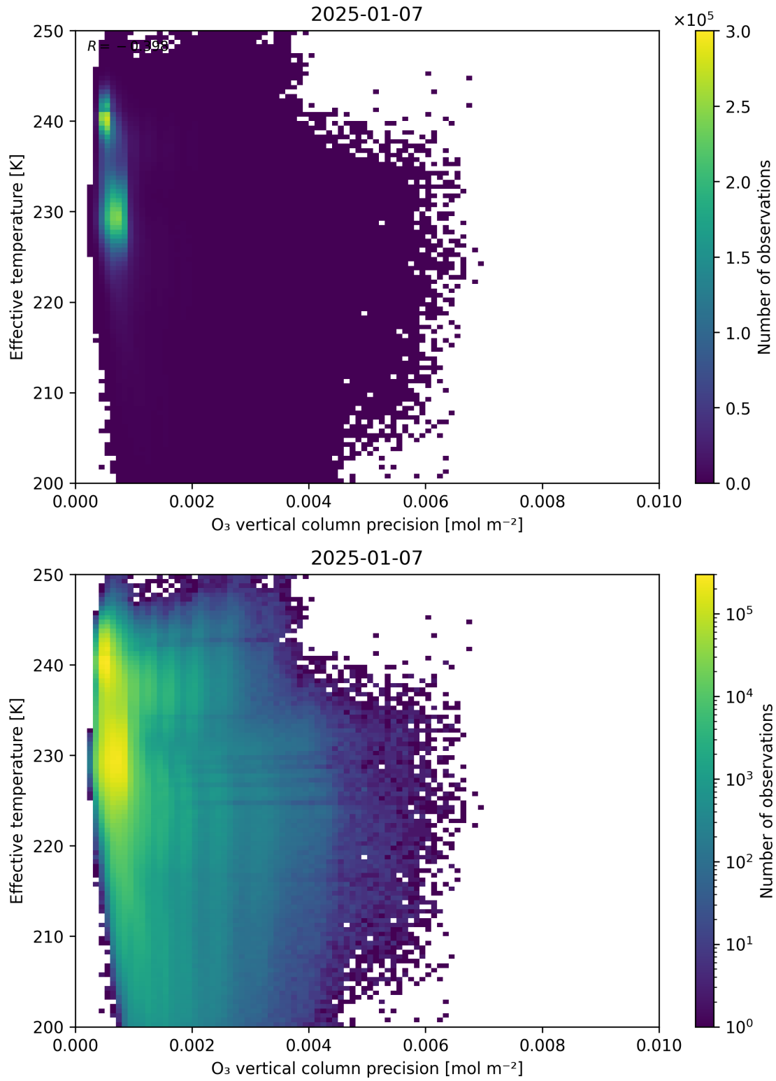
Figure 42: Scatter density plot of “O 3 vertical column precision” against “Effective temperature” for 2025-01-07 to 2025-01-08.
