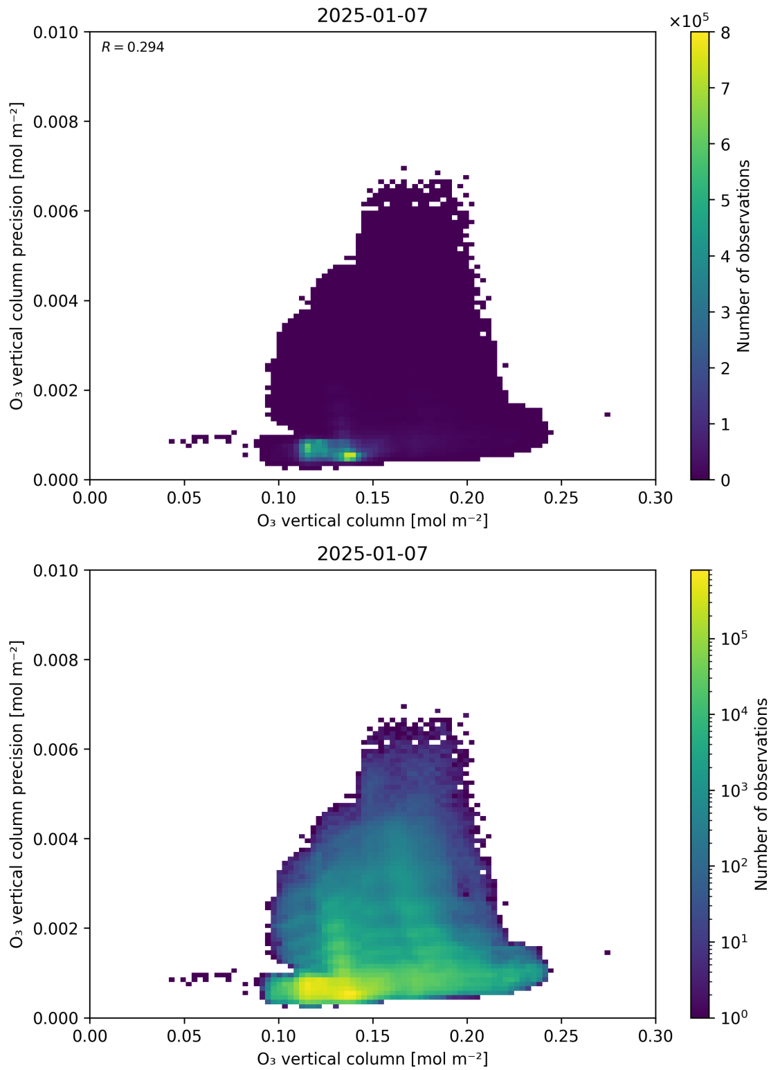
Figure 41: Scatter density plot of “O 3 vertical column” against “O 3 vertical column precision” for 2025-01-07 to 2025-01-08.
