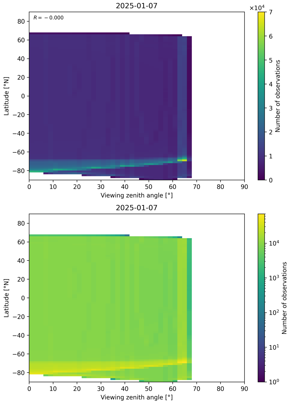
Figure 49: Scatter density plot of “Viewing zenith angle” against “Latitude” for 2025-01-07 to 2025-01-08.
