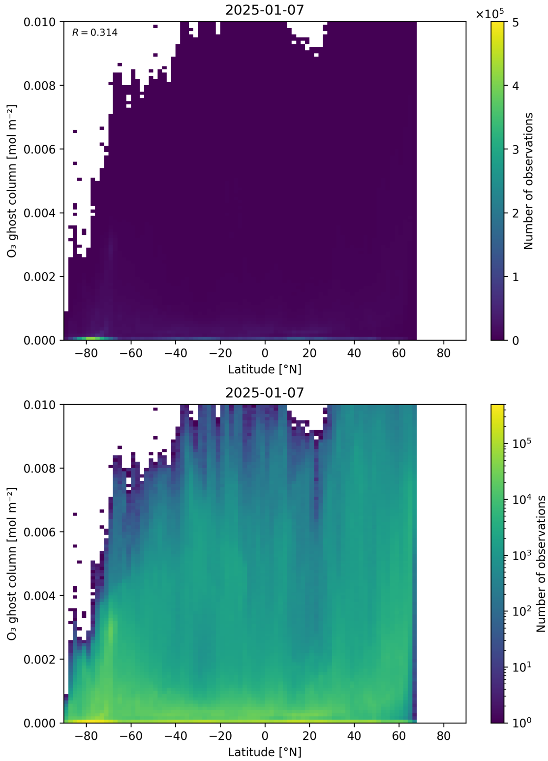
Figure 35: Scatter density plot of “Latitude” against “O 3 ghost column” for 2025-01-07 to 2025-01-08.
