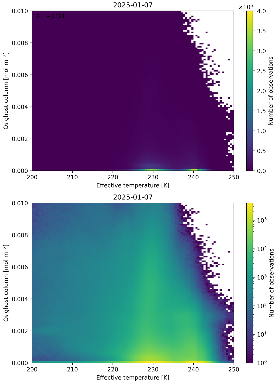
Figure 38: Scatter density plot of “Effective temperature” against “O 3 ghost column” for 2025-01-07 to 2025-01-08.
