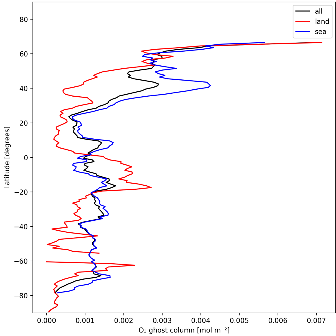
Figure 18: Zonal average of “O 3 ghost column” for 2025-01-07 to 2025-01-08.
