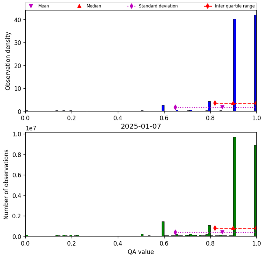
Figure 20: Histogram of “QA value” for 2025-01-07 to 2025-01-08
