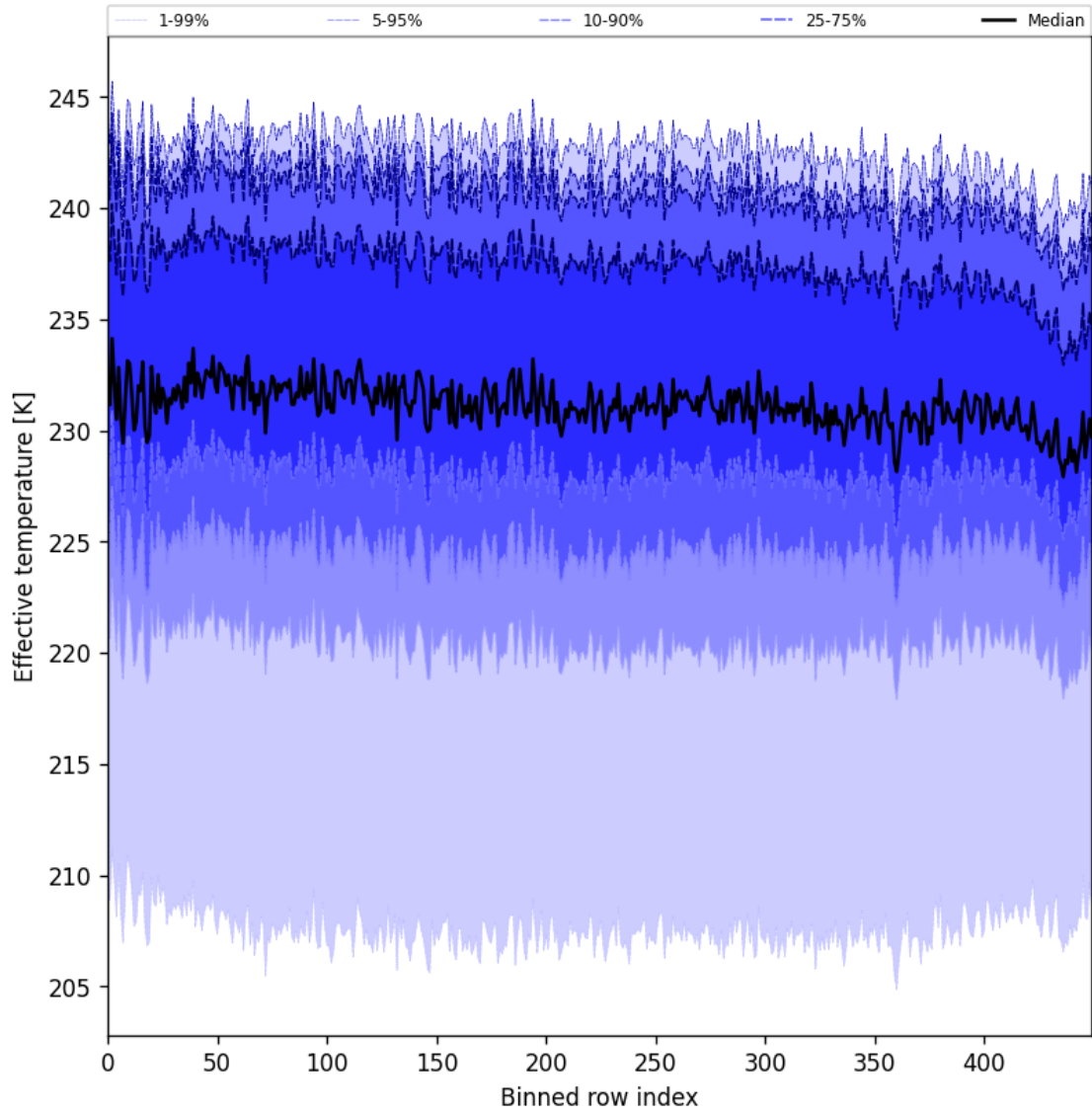
Figure 31: Along track statistics of “Effective temperature” for 2025-01-07 to 2025-01-08
