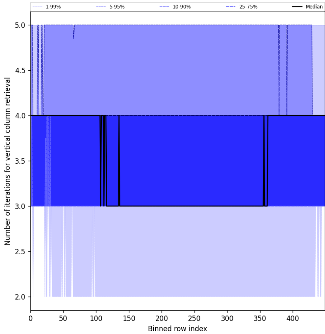
Figure 33: Along track statistics of “Number of iterations for vertical column retrieval” for 2025-01-07 to 2025-01-08
