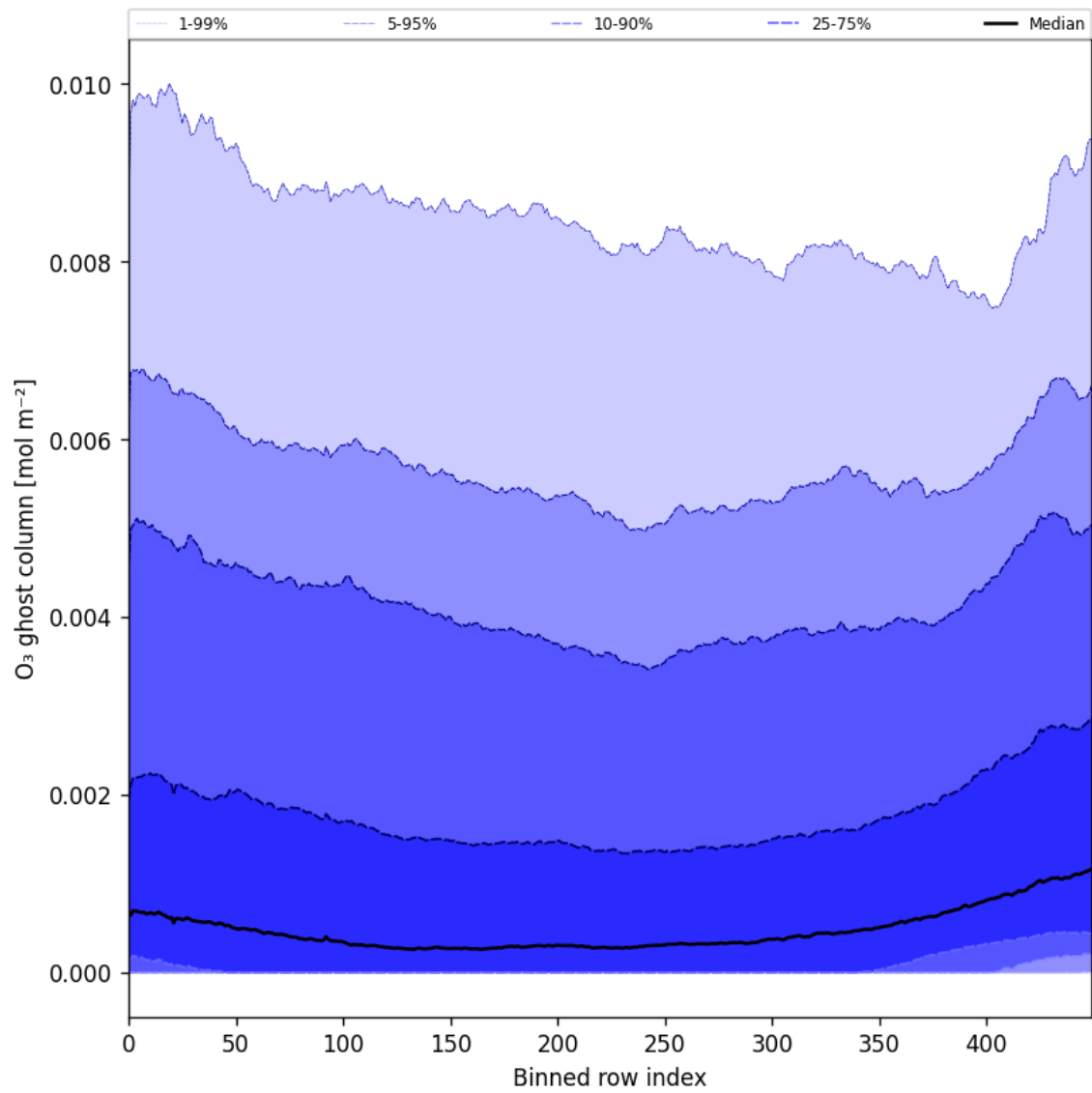
Figure 32: Along track statistics of “O 3 ghost column” for 2025-01-07 to 2025-01-08
