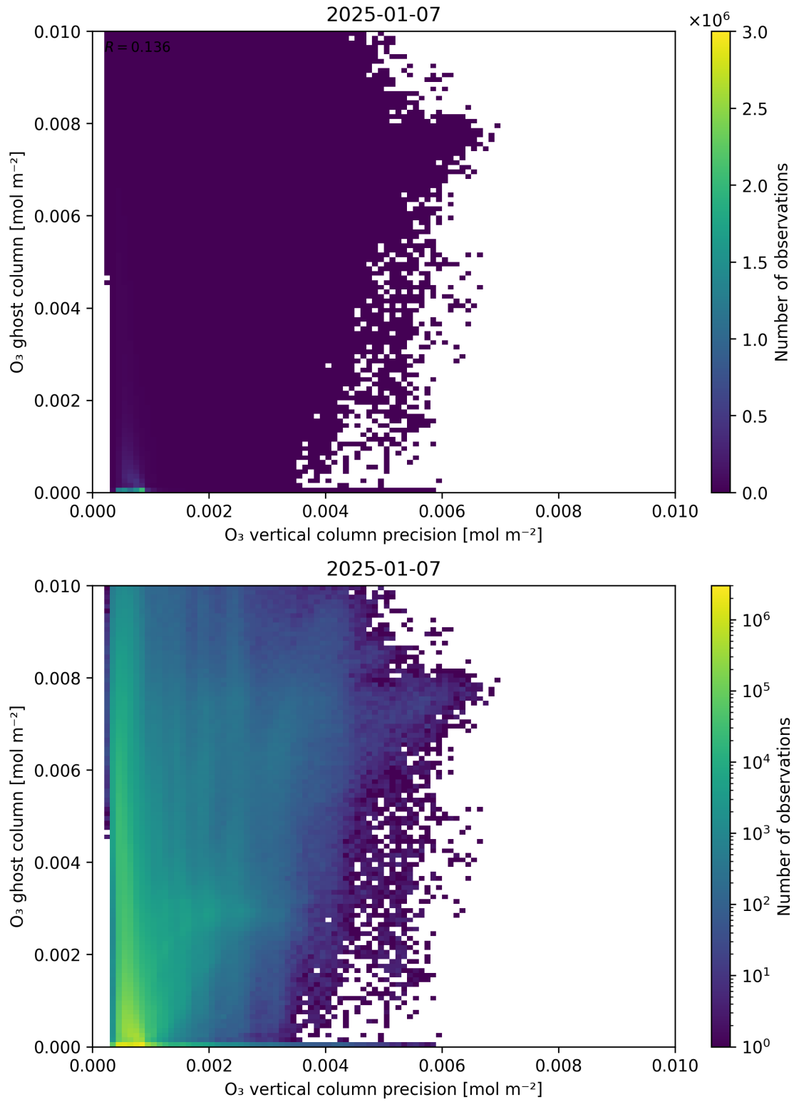
Figure 43: Scatter density plot of “O 3 vertical column precision” against “O 3 ghost column” for 2025-01-07 to 2025-01-08.
