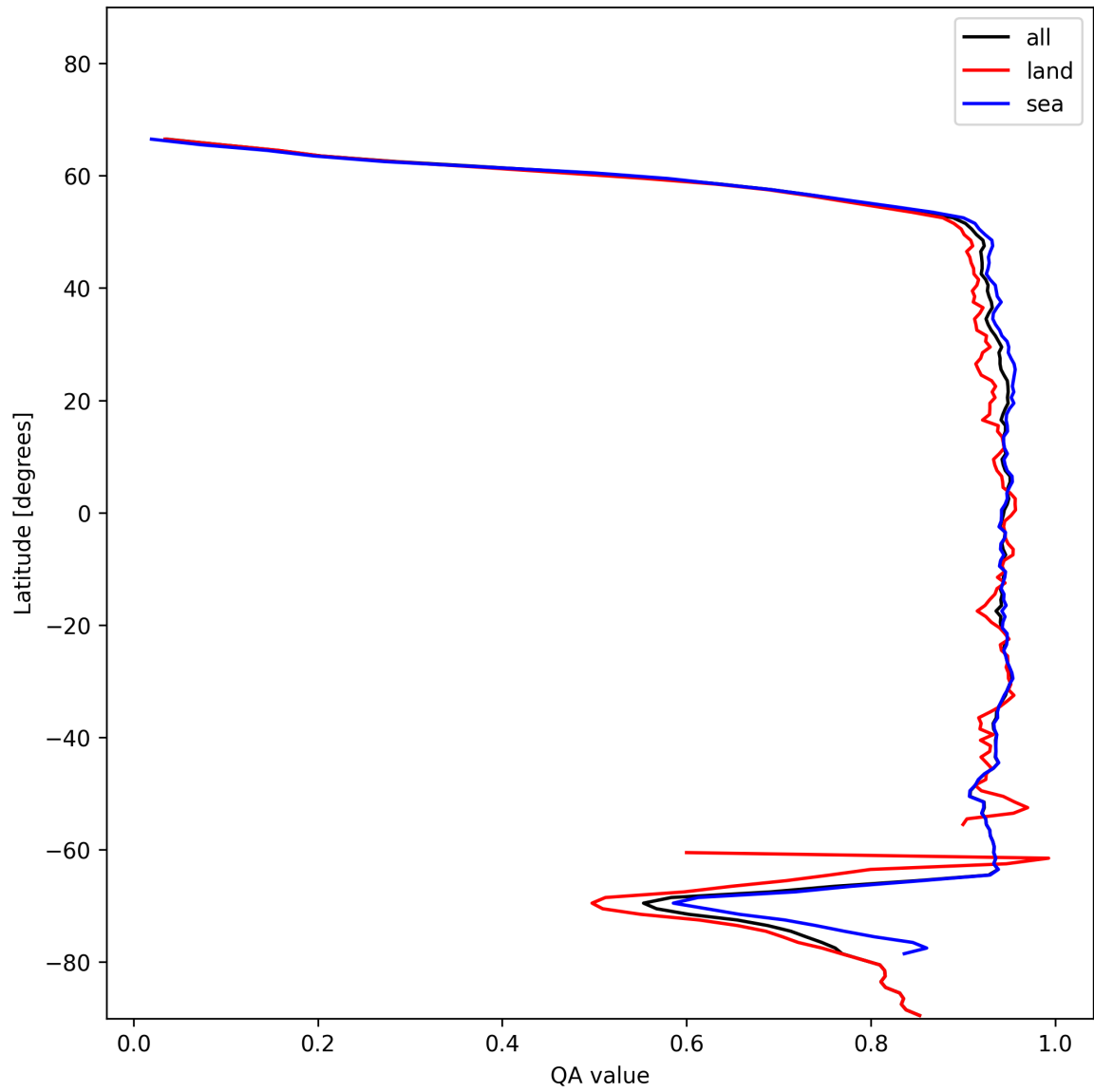
Figure 13: Zonal average of “QA value” for 2025-01-07 to 2025-01-08.
