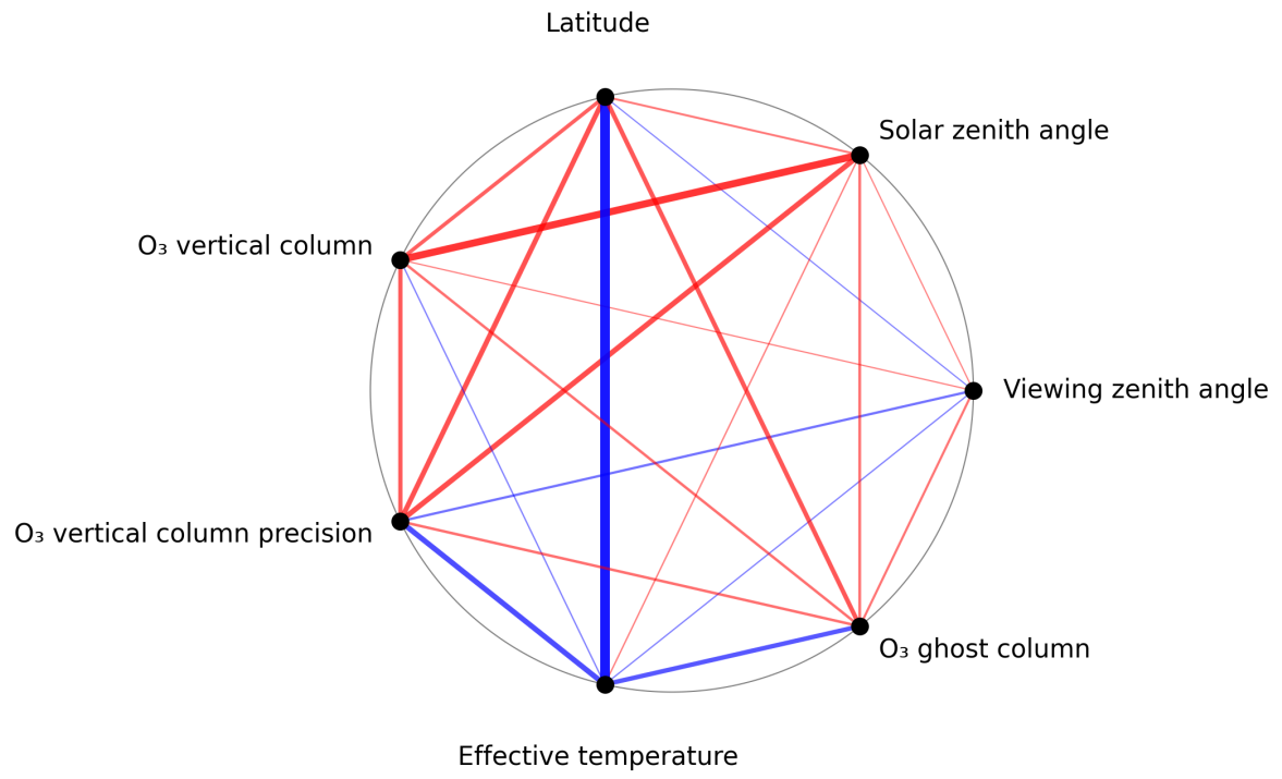
Figure 1: Map of correlation graph for 2025-01-07 to 2025-01-08.
