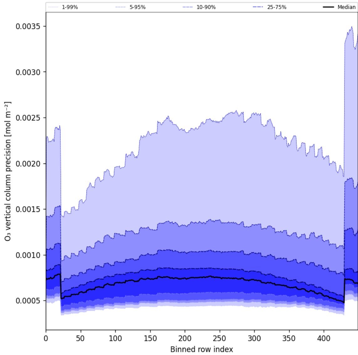
Figure 29: Along track statistics of “O 3 vertical column precision” for 2025-01-07 to 2025-01-08
