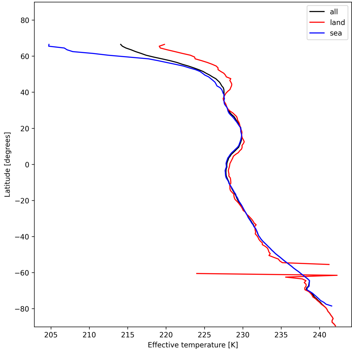
Figure 17: Zonal average of "Effective temperature" for 2025-01-07 to 2025-01-08.
