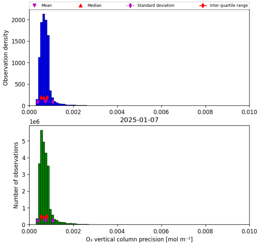
Figure 22: Histogram of “O 3 vertical column precision” for 2025-01-07 to 2025-01-08
