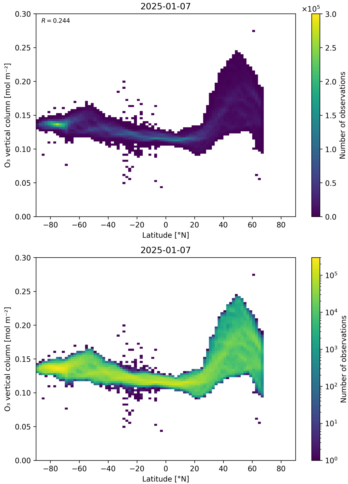
Figure 36: Scatter density plot of “Latitude” against “O 3 vertical column” for 2025-01-07 to 2025-01-08.
