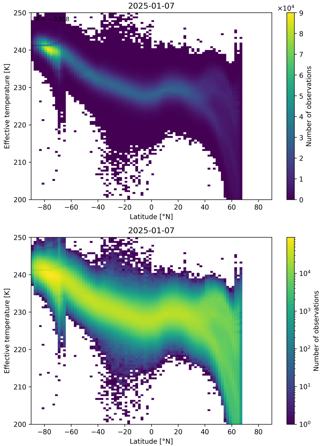
Figure 34: Scatter density plot of “Latitude” against “Effective temperature” for 2025-01-07 to 2025-01-08.
