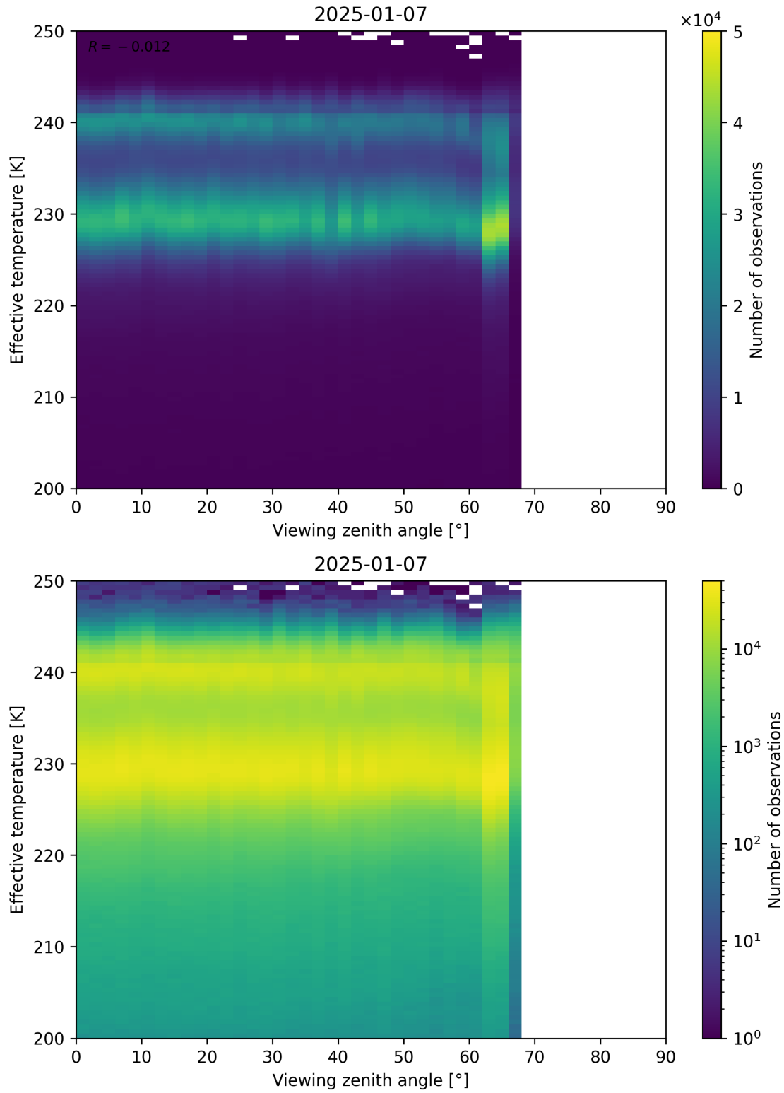
Figure 50: Scatter density plot of “Viewing zenith angle” against “Effective temperature” for 2025-01-07 to 2025-01-08.
