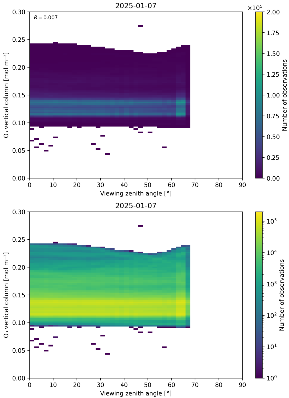
Figure 52: Scatter density plot of “Viewing zenith angle” against “O 3 vertical column” for 2025-01-07 to 2025-01-08.
