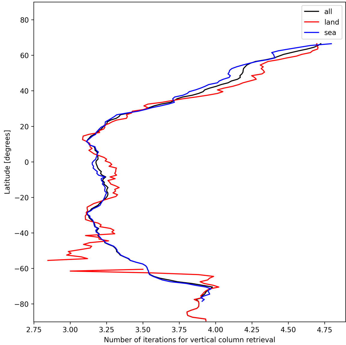
Figure 19: Zonal average of “Number of iterations for vertical column retrieval” for 2025-01-07 to 2025-01-08.
