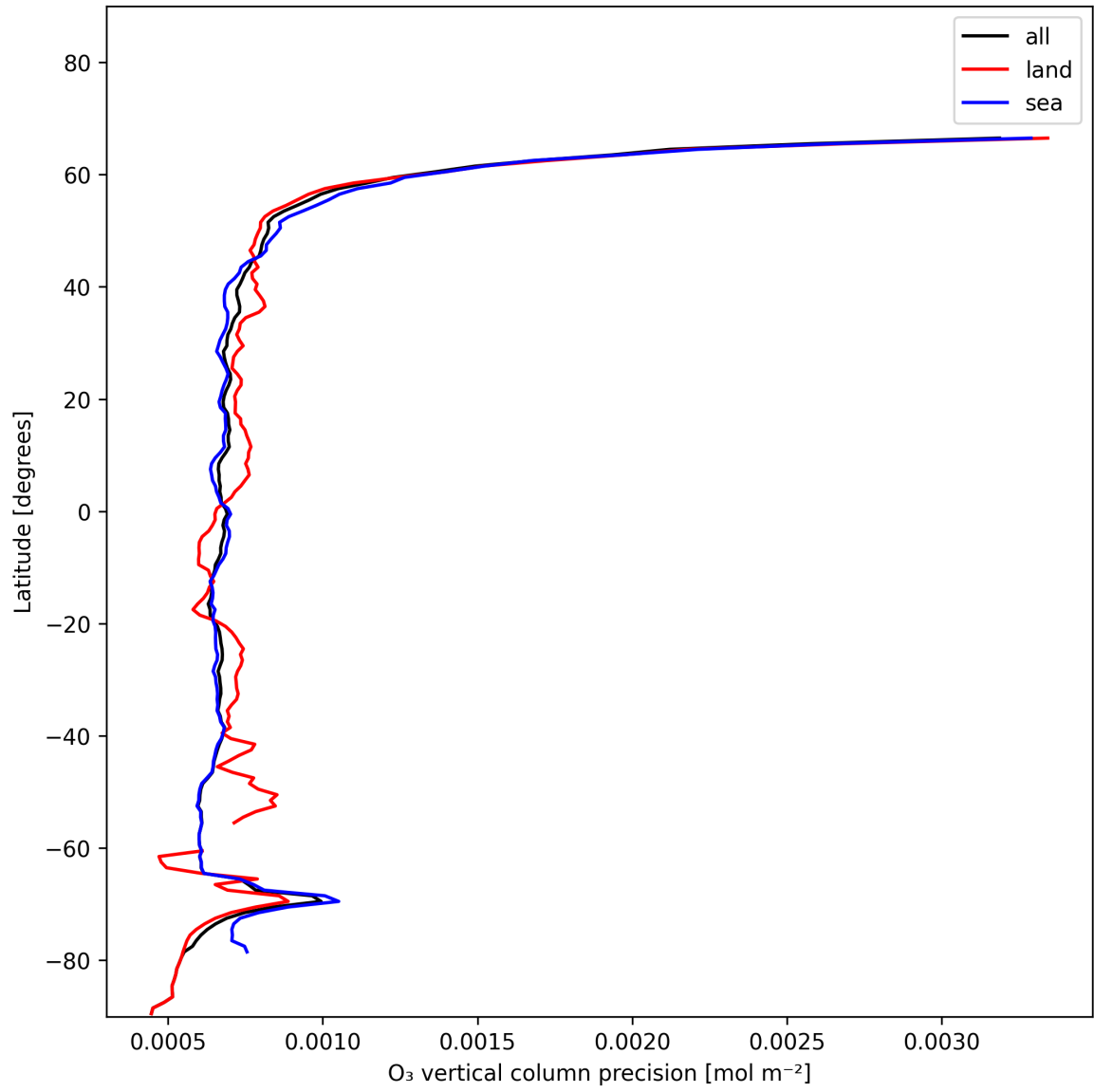
Figure 15: Zonal average of “O 3 vertical column precision” for 2025-01-07 to 2025-01-08.
