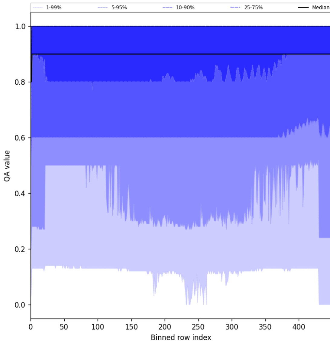
Figure 27: Along track statistics of “QA value” for 2025-01-07 to 2025-01-08
