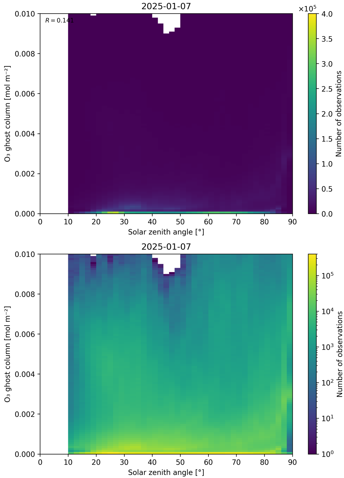
Figure 46: Scatter density plot of “Solar zenith angle” against “O 3 ghost column” for 2025-01-07 to 2025-01-08.
