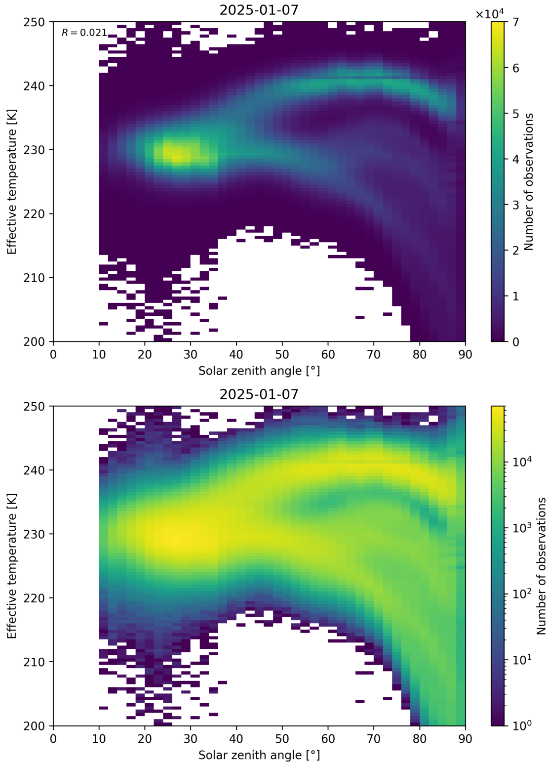
Figure 45: Scatter density plot of “Solar zenith angle” against “Effective temperature” for 2025-01-07 to 2025-01-08.
