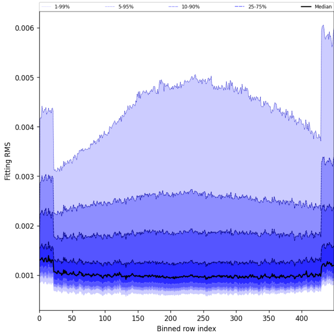
Figure 30: Along track statistics of “Fitting RMS” for 2025-01-07 to 2025-01-08
