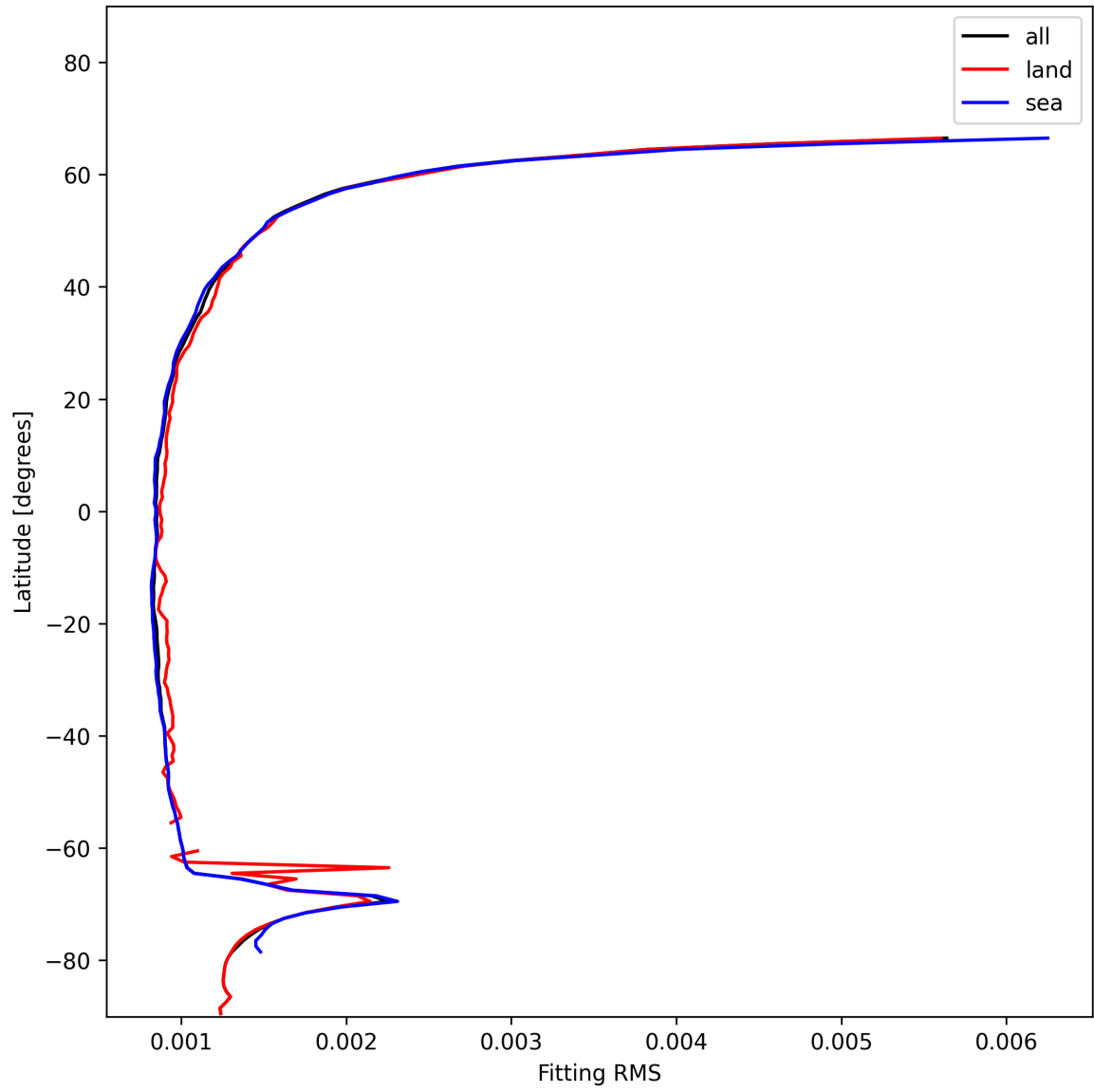
Figure 16: Zonal average of “Fitting RMS” for 2025-01-07 to 2025-01-08.
