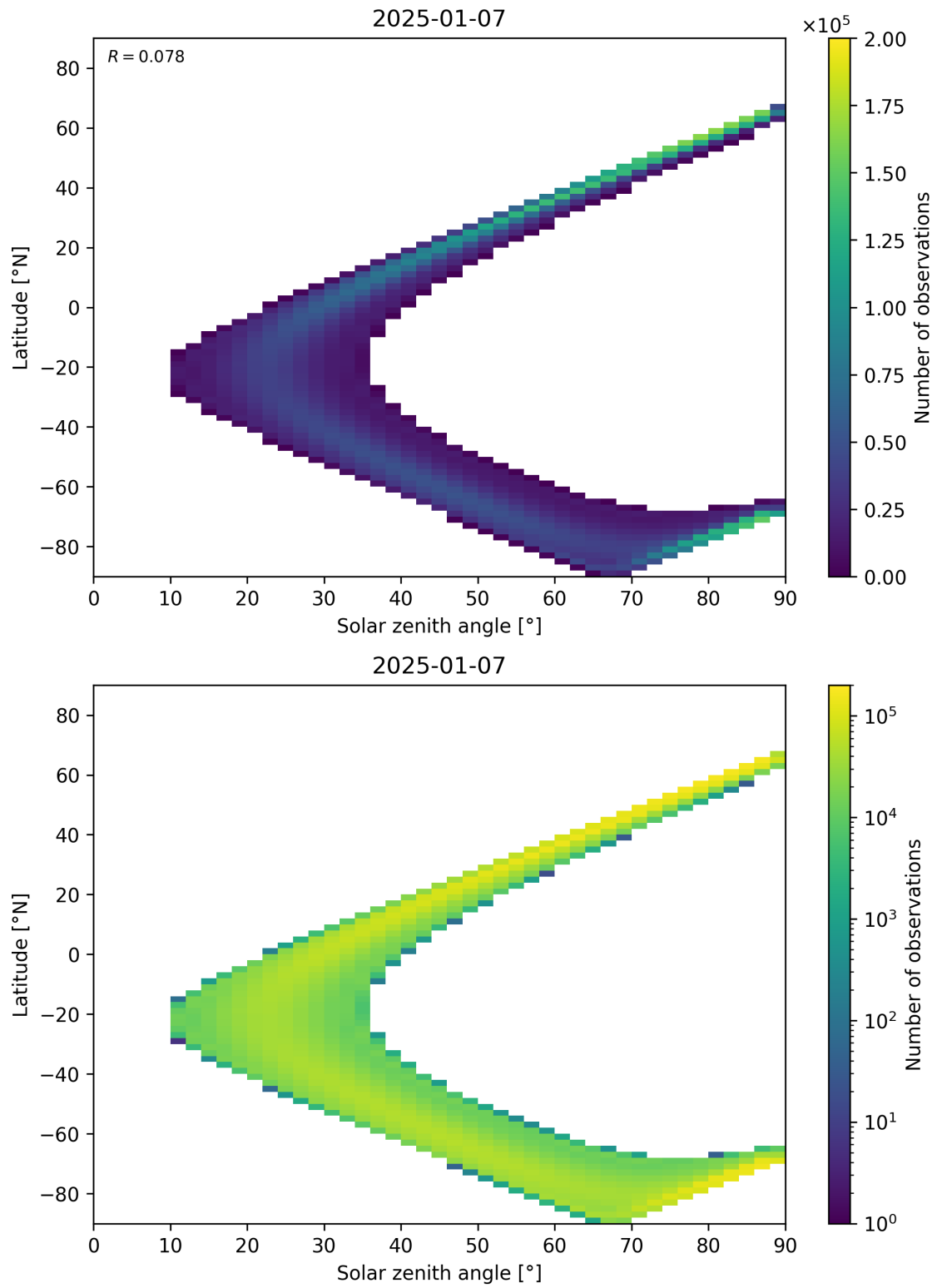
Figure 44: Scatter density plot of “Solar zenith angle” against “Latitude” for 2025-01-07 to 2025-01-08.
