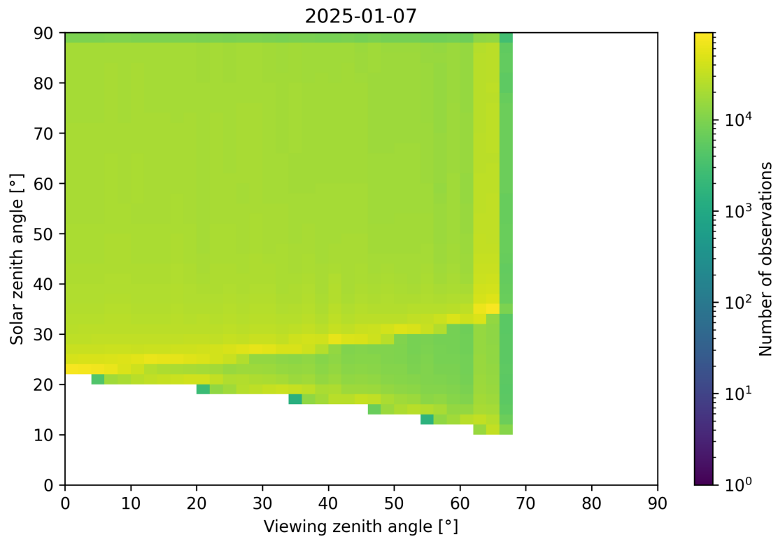
Figure 54: Scatter density plot of “Viewing zenith angle” against “Solar zenith angle” for 2025-01-07 to 2025-01-08.
