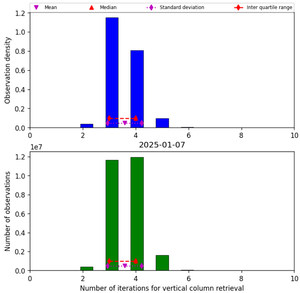
Figure 26: Histogram of “Number of iterations for vertical column retrieval” for 2025-01-07 to 2025-01-08
