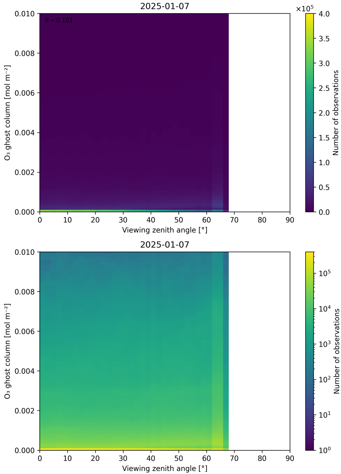
Figure 51: Scatter density plot of “Viewing zenith angle” against “O 3 ghost column” for 2025-01-07 to 2025-01-08.
