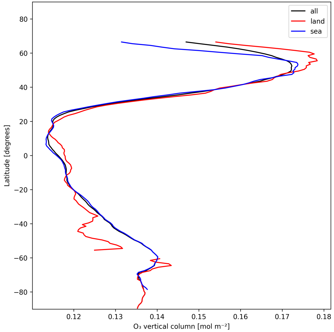
Figure 14: Zonal average of “O 3 vertical column” for 2025-01-07 to 2025-01-08.
