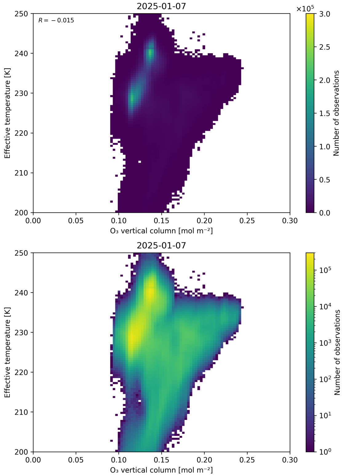
Figure 39: Scatter density plot of “O 3 vertical column” against “Effective temperature” for 2025-01-07 to 2025-01-08.
