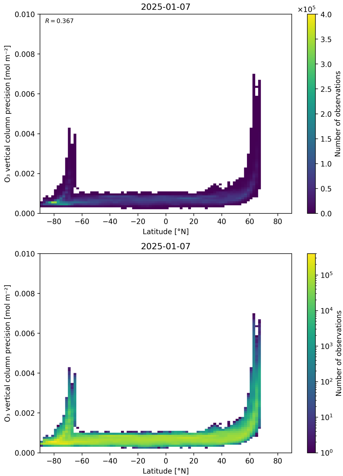
Figure 37: Scatter density plot of “Latitude” against “O 3 vertical column precision” for 2025-01-07 to 2025-01-08.
