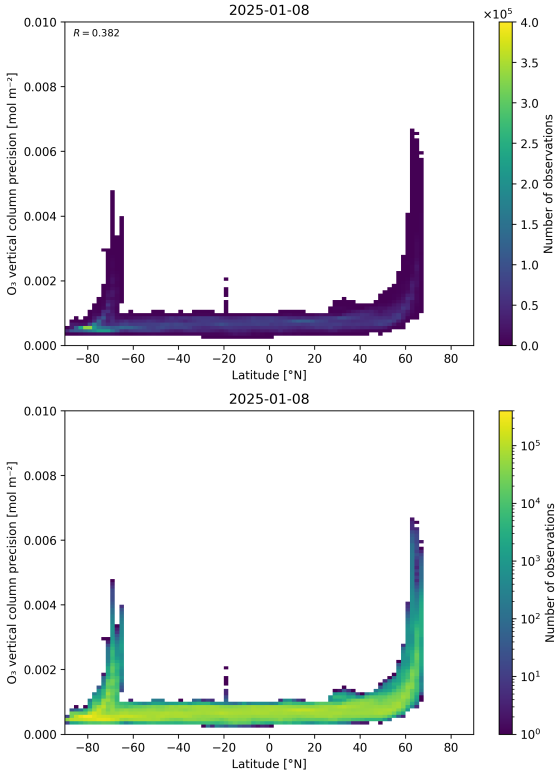
Figure 37: Scatter density plot of “Latitude” against “O 3 vertical column precision” for 2025-01-07 to 2025-01-09.
