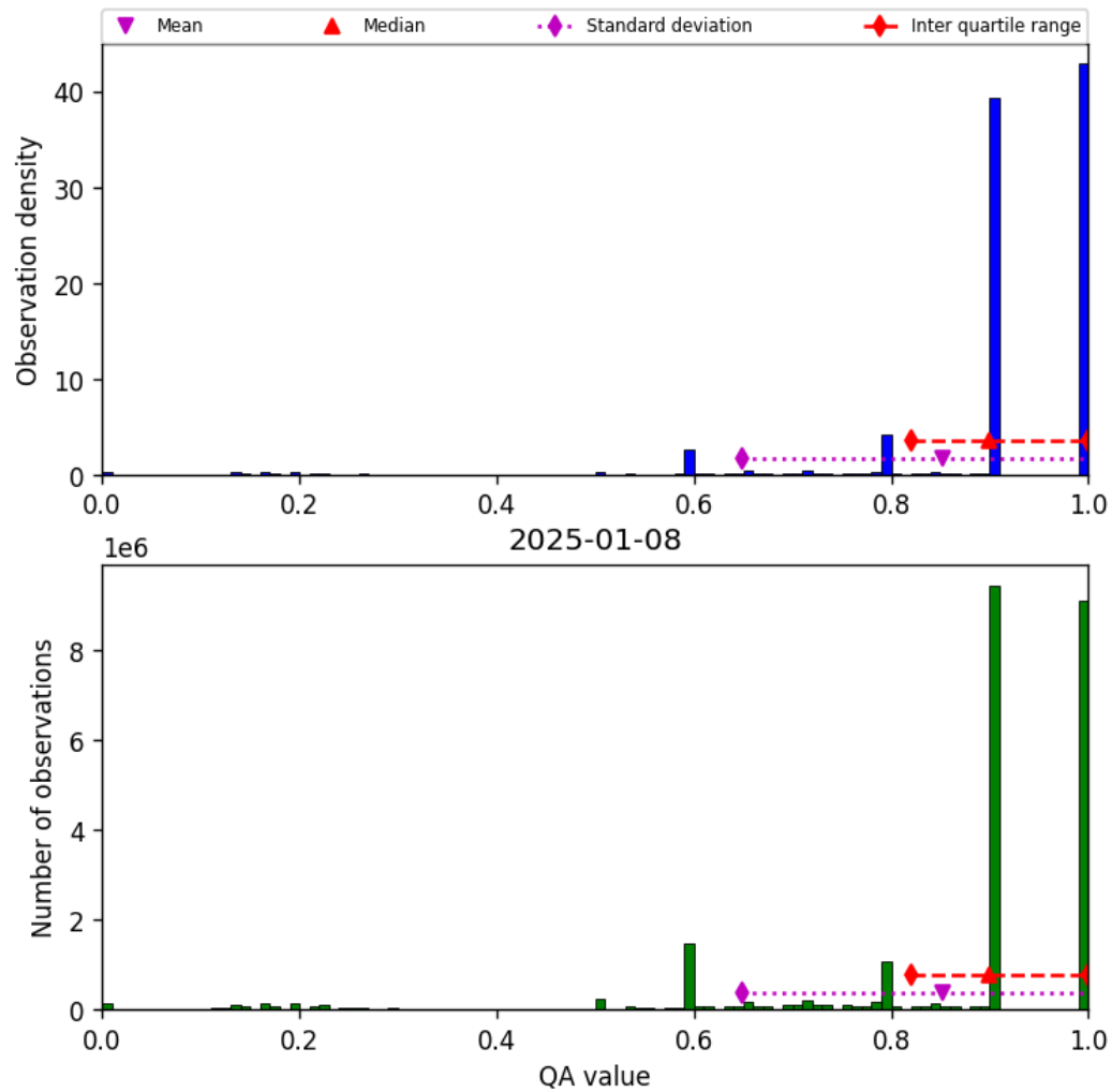
Figure 20: Histogram of “QA value” for 2025-01-07 to 2025-01-09
