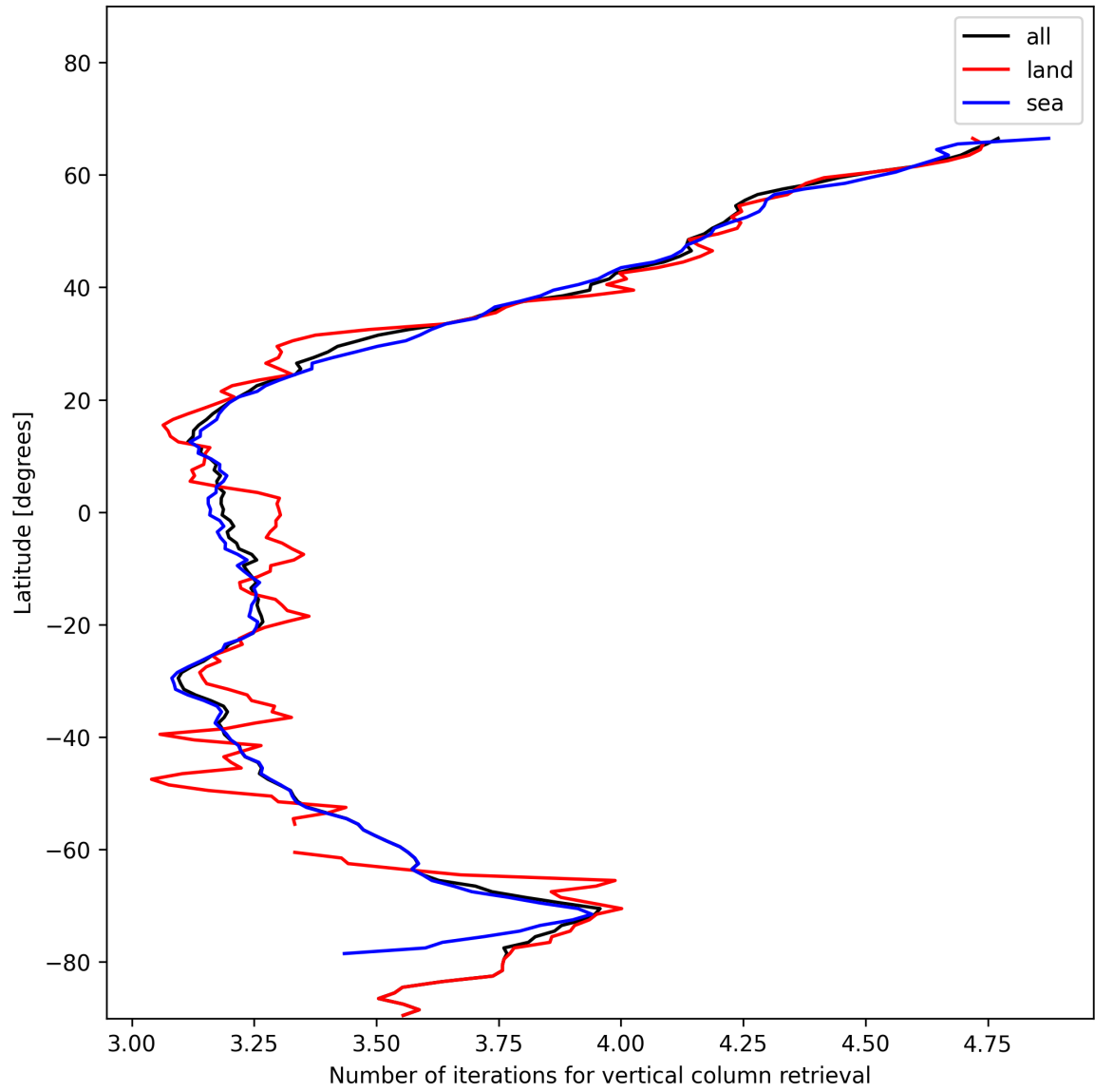
Figure 19: Zonal average of “Number of iterations for vertical column retrieval” for 2025-01-07 to 2025-01-09.
