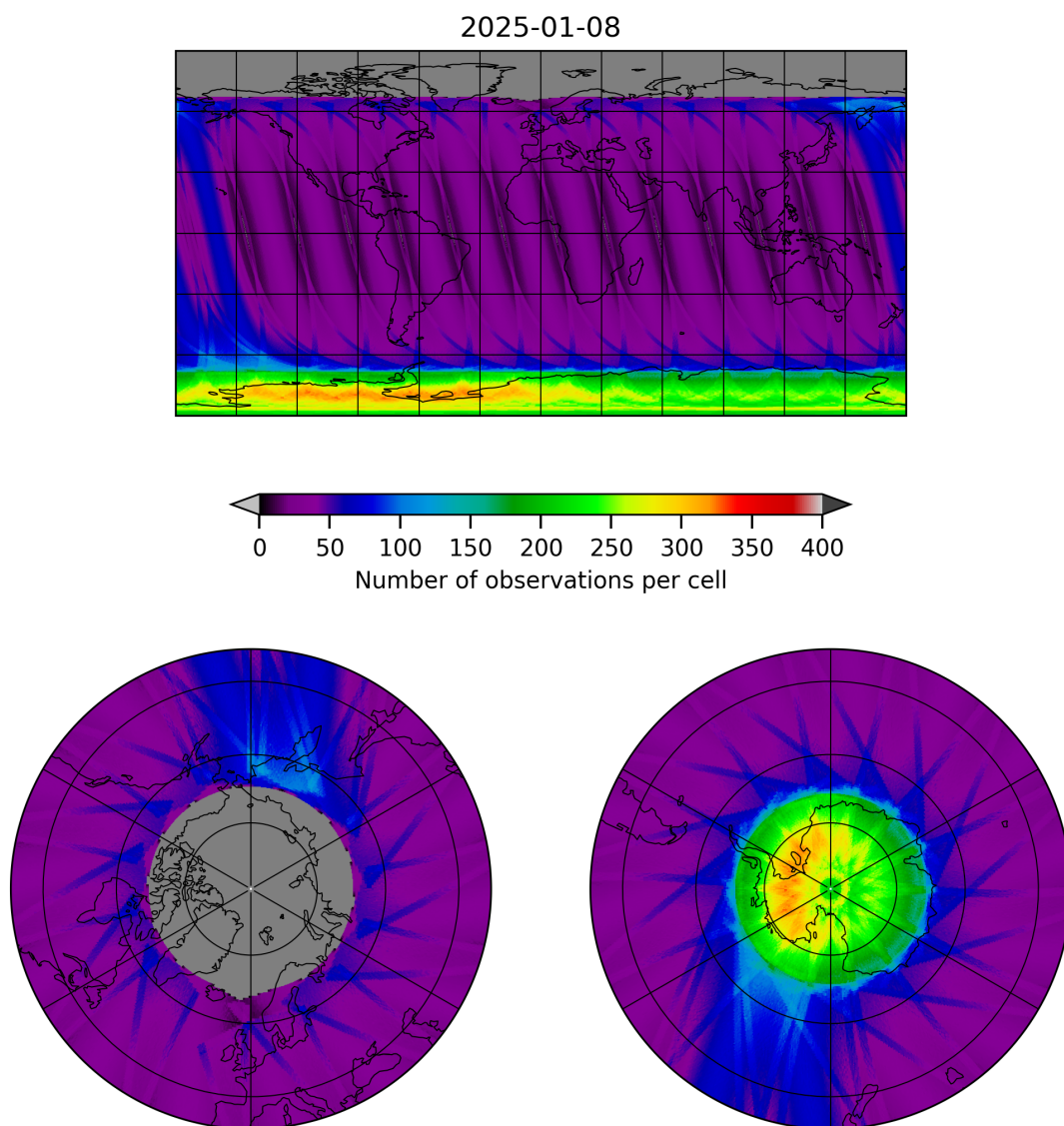
Figure 12: Map of the number of observations for 2025-01-07 to 2025-01-09
