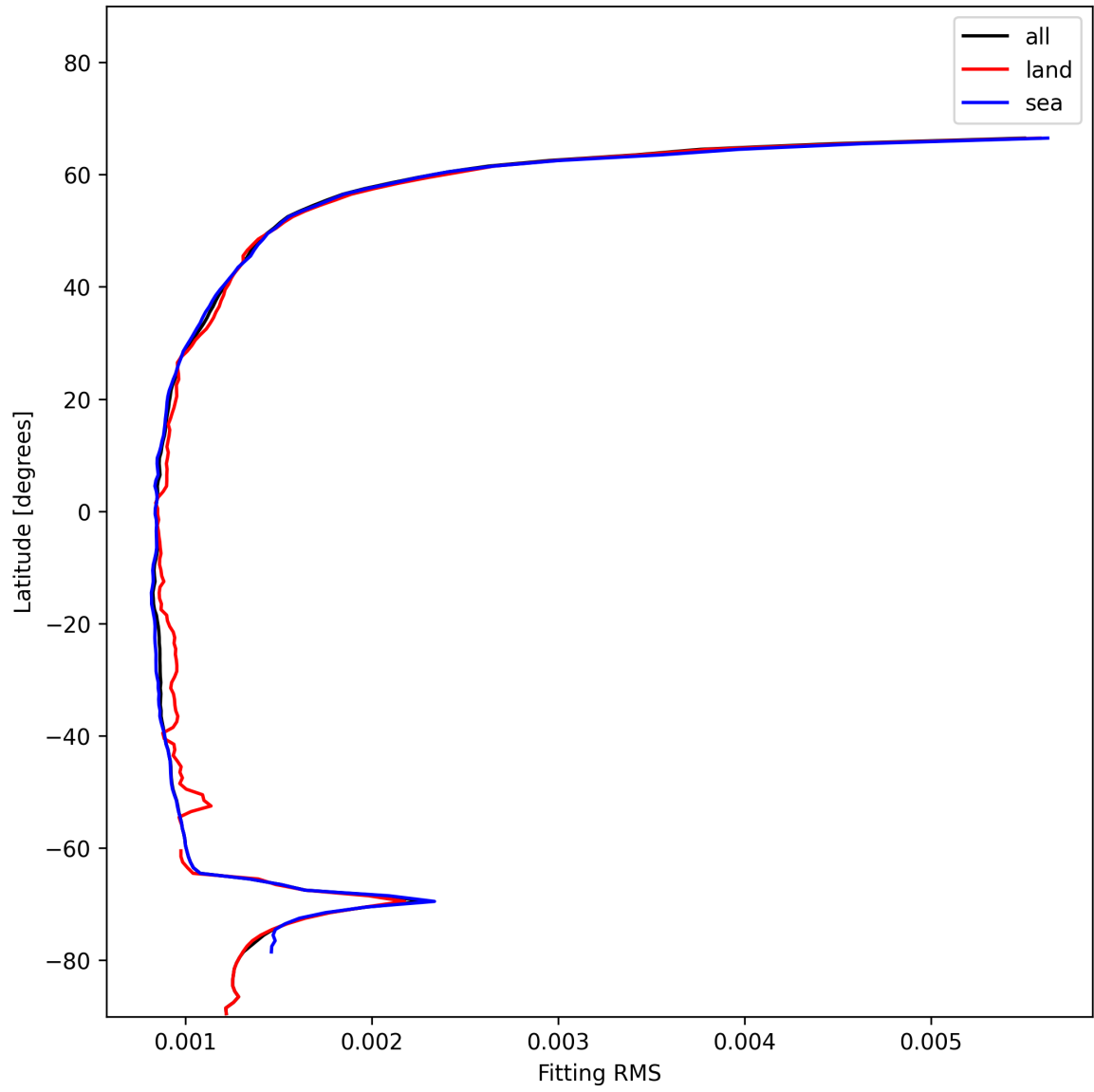
Figure 16: Zonal average of “Fitting RMS” for 2025-01-07 to 2025-01-09.
