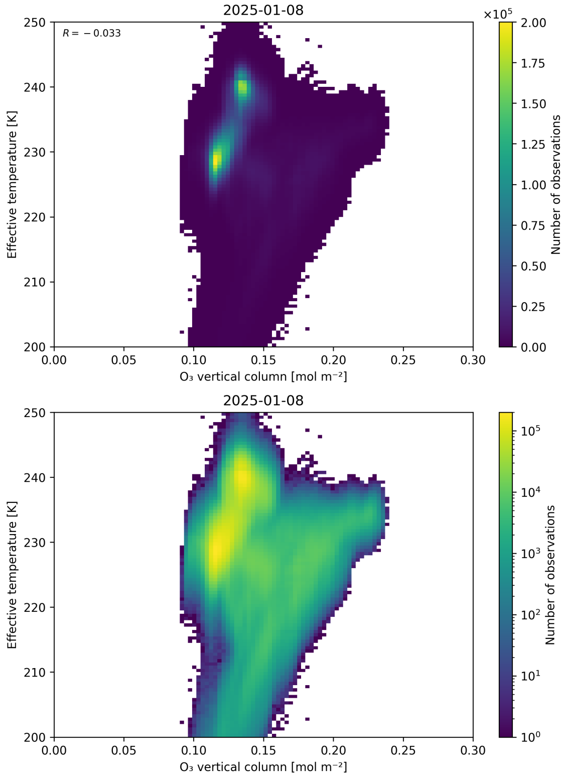
Figure 39: Scatter density plot of “O 3 vertical column” against “Effective temperature” for 2025-01-07 to 2025-01-09.
