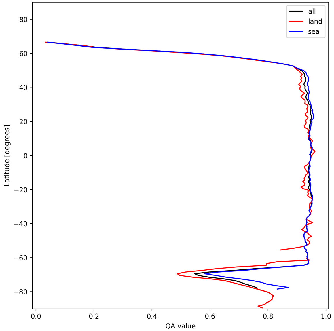
Figure 13: Zonal average of “QA value” for 2025-01-07 to 2025-01-09.
