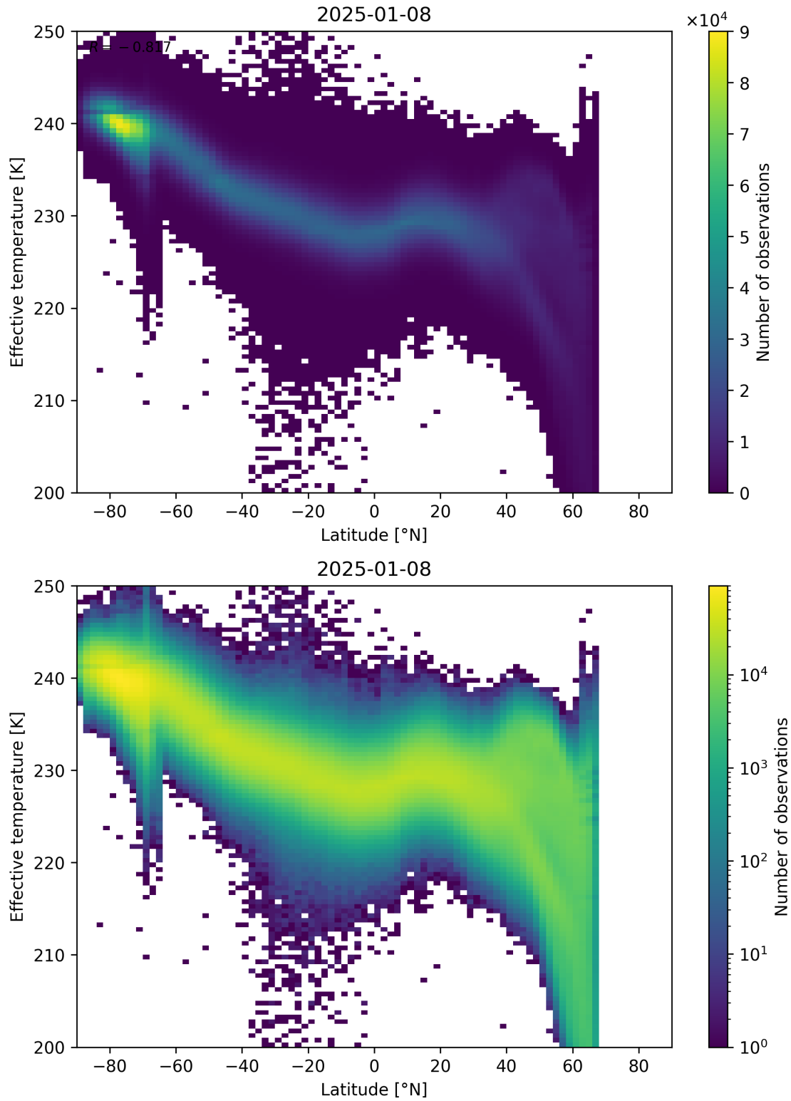
Figure 34: Scatter density plot of “Latitude” against “Effective temperature” for 2025-01-07 to 2025-01-09.
