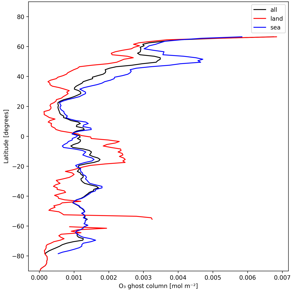
Figure 18: Zonal average of “O 3 ghost column” for 2025-01-07 to 2025-01-09.
