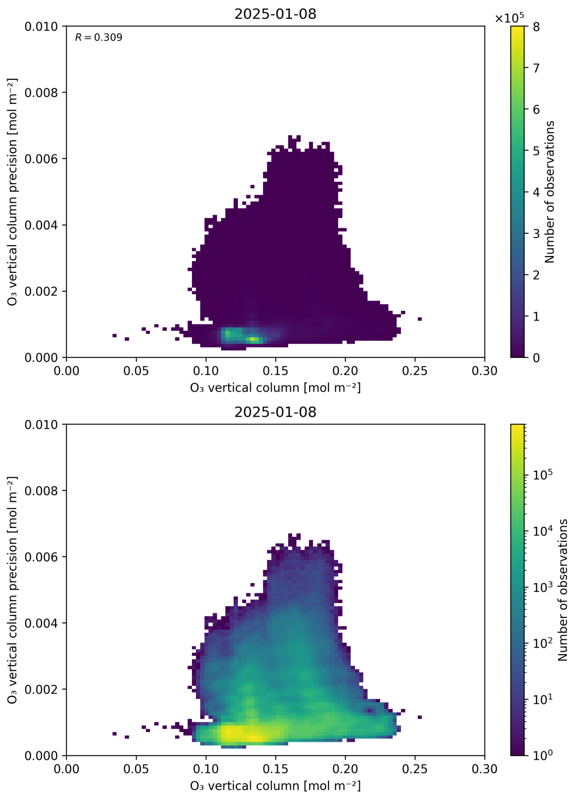
Figure 41: Scatter density plot of “O 3 vertical column” against “O 3 vertical column precision” for 2025-01-07 to 2025-01-09.
