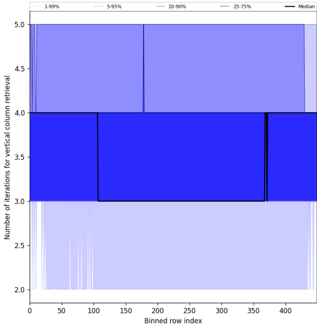
Figure 33: Along track statistics of “Number of iterations for vertical column retrieval” for 2025-01-07 to 2025-01-09
