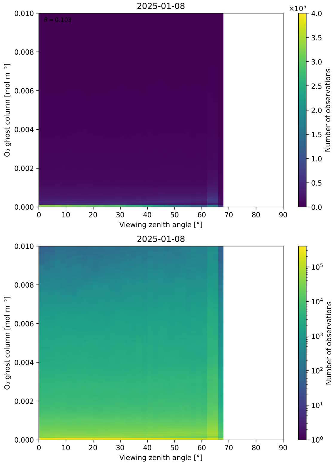
Figure 51: Scatter density plot of “Viewing zenith angle” against “O 3 ghost column” for 2025-01-07 to 2025-01-09.
