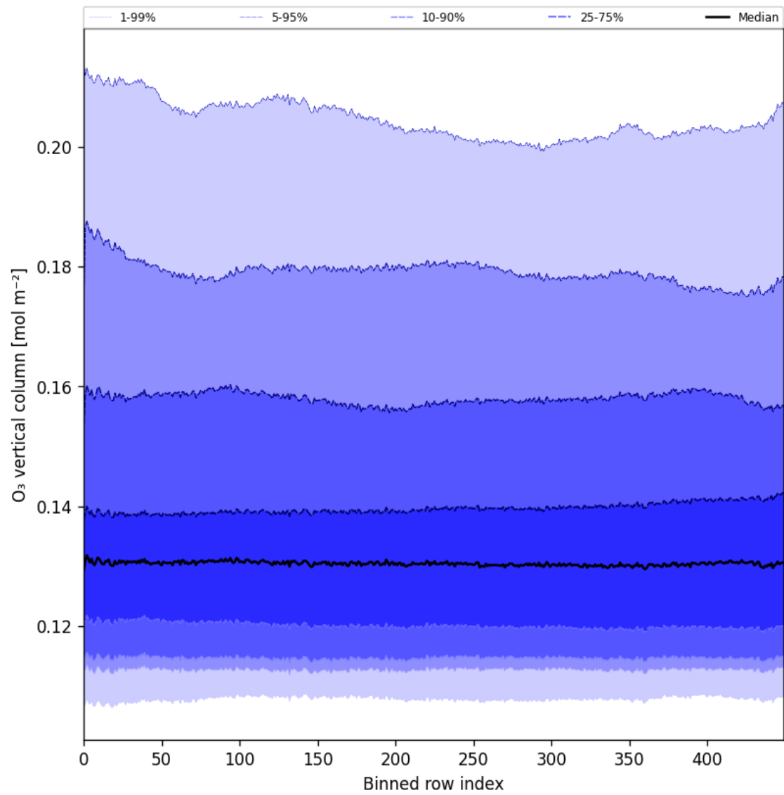
Figure 28: Along track statistics of “O 3 vertical column” for 2025-01-07 to 2025-01-09
