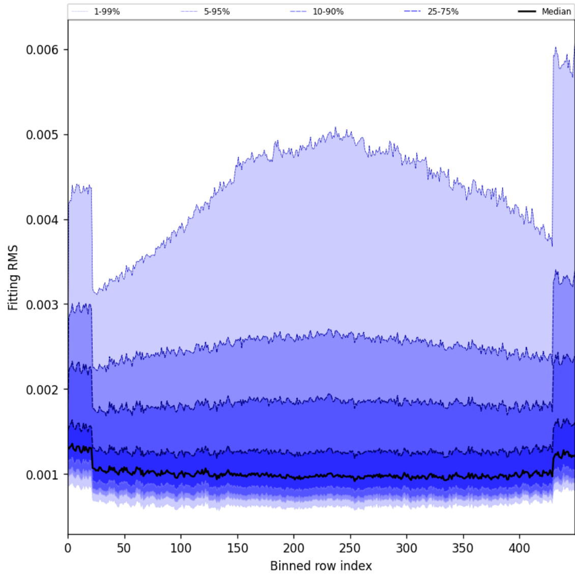
Figure 30: Along track statistics of “Fitting RMS” for 2025-01-07 to 2025-01-09
