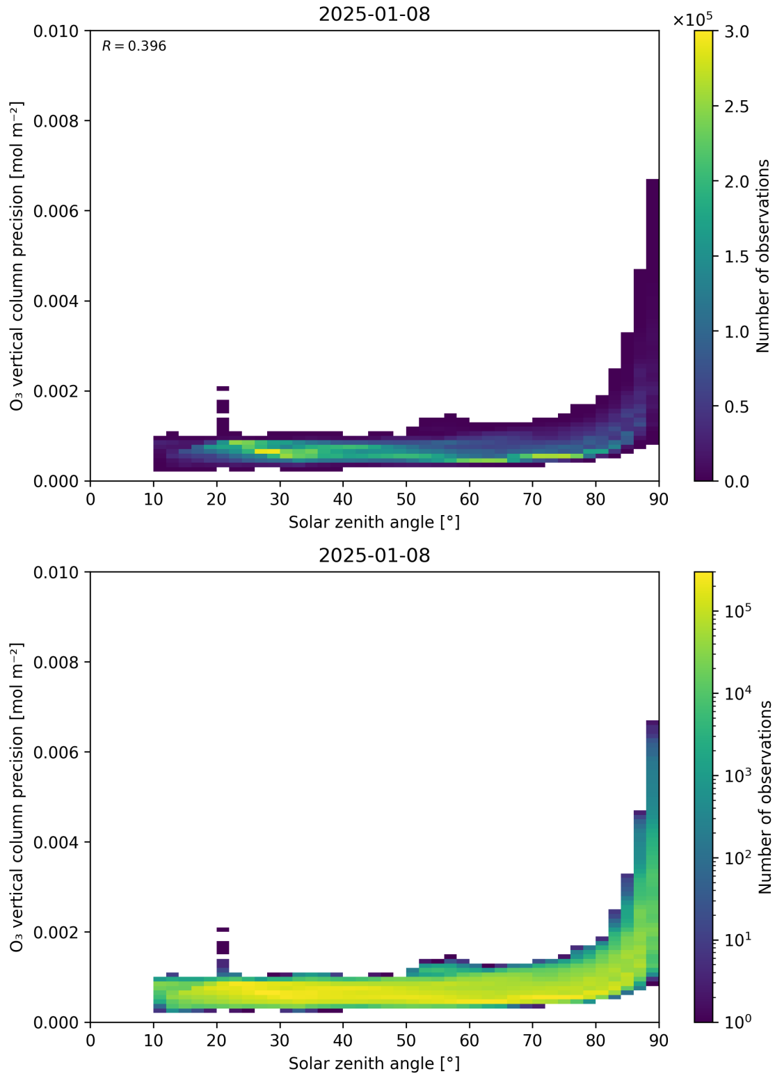
Figure 48: Scatter density plot of “Solar zenith angle” against “O 3 vertical column precision” for 2025-01-07 to 2025-01-09.
