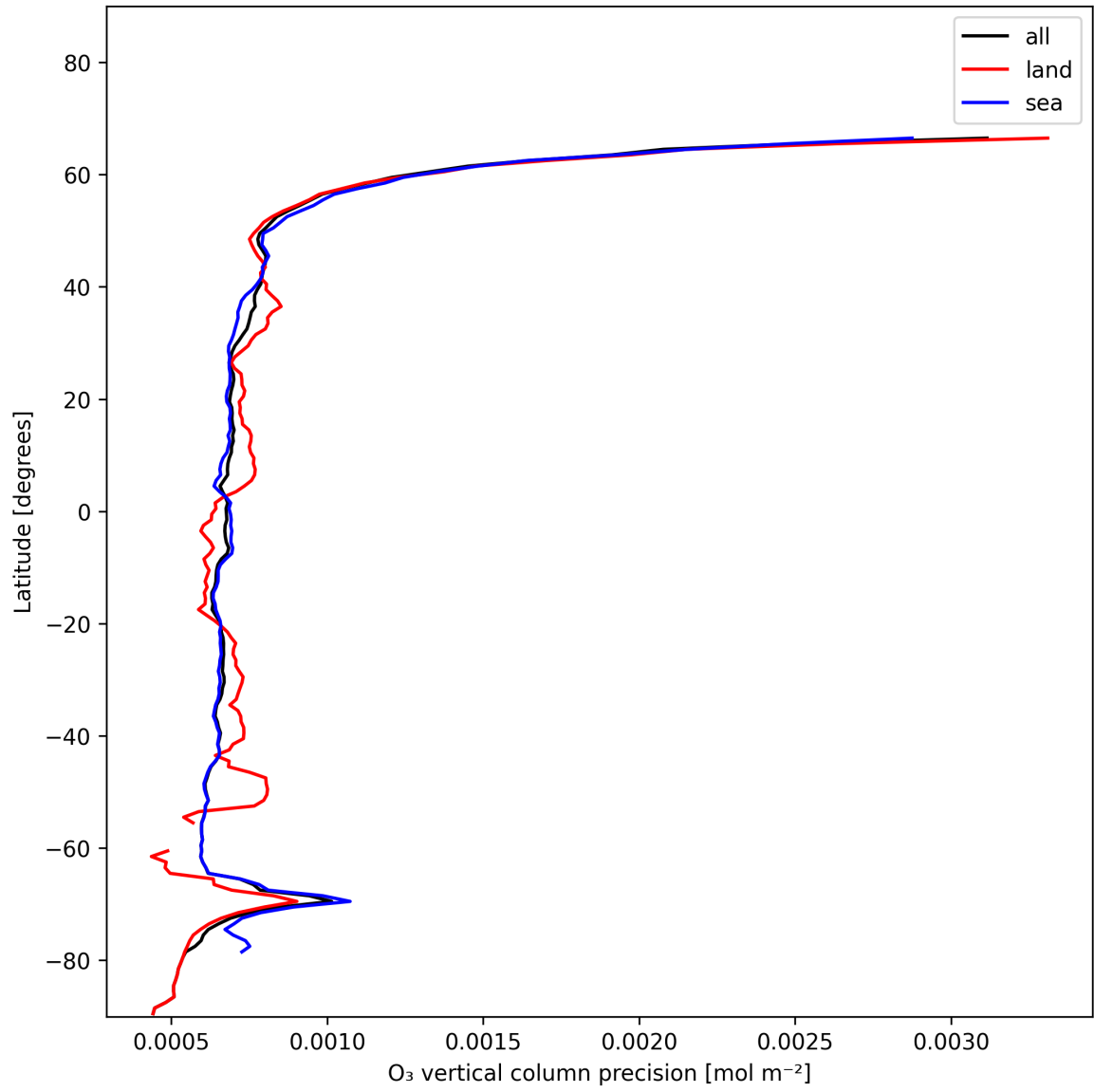
Figure 15: Zonal average of “O 3 vertical column precision” for 2025-01-07 to 2025-01-09.
