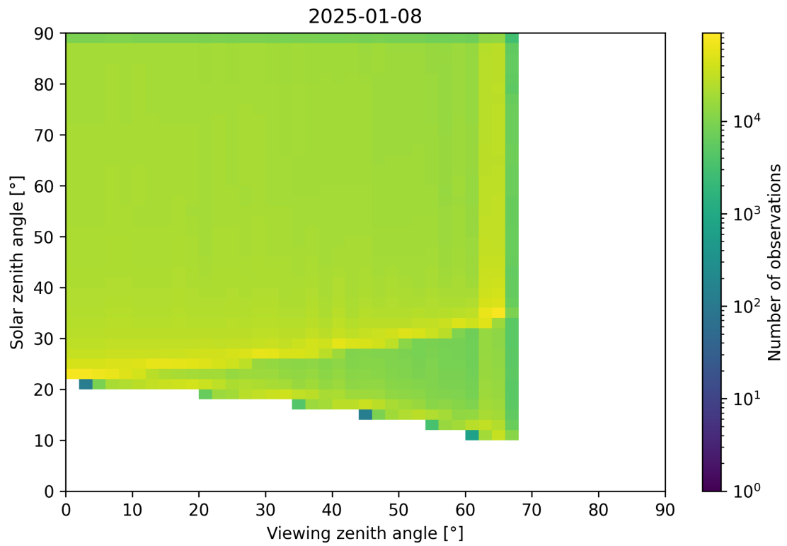
Figure 54: Scatter density plot of “Viewing zenith angle” against “Solar zenith angle” for 2025-01-07 to 2025-01-09.
