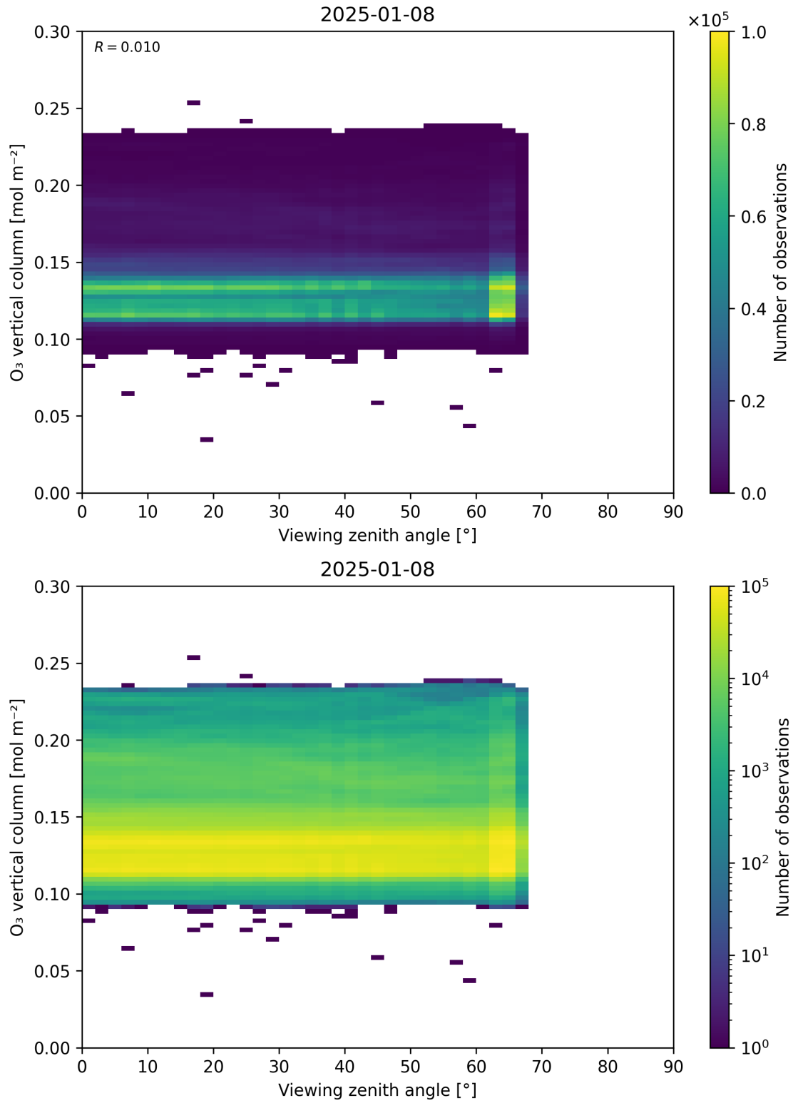
Figure 52: Scatter density plot of “Viewing zenith angle” against “O 3 vertical column” for 2025-01-07 to 2025-01-09.
