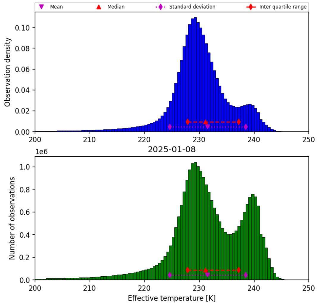
Figure 24: Histogram of “Effective temperature” for 2025-01-07 to 2025-01-09
