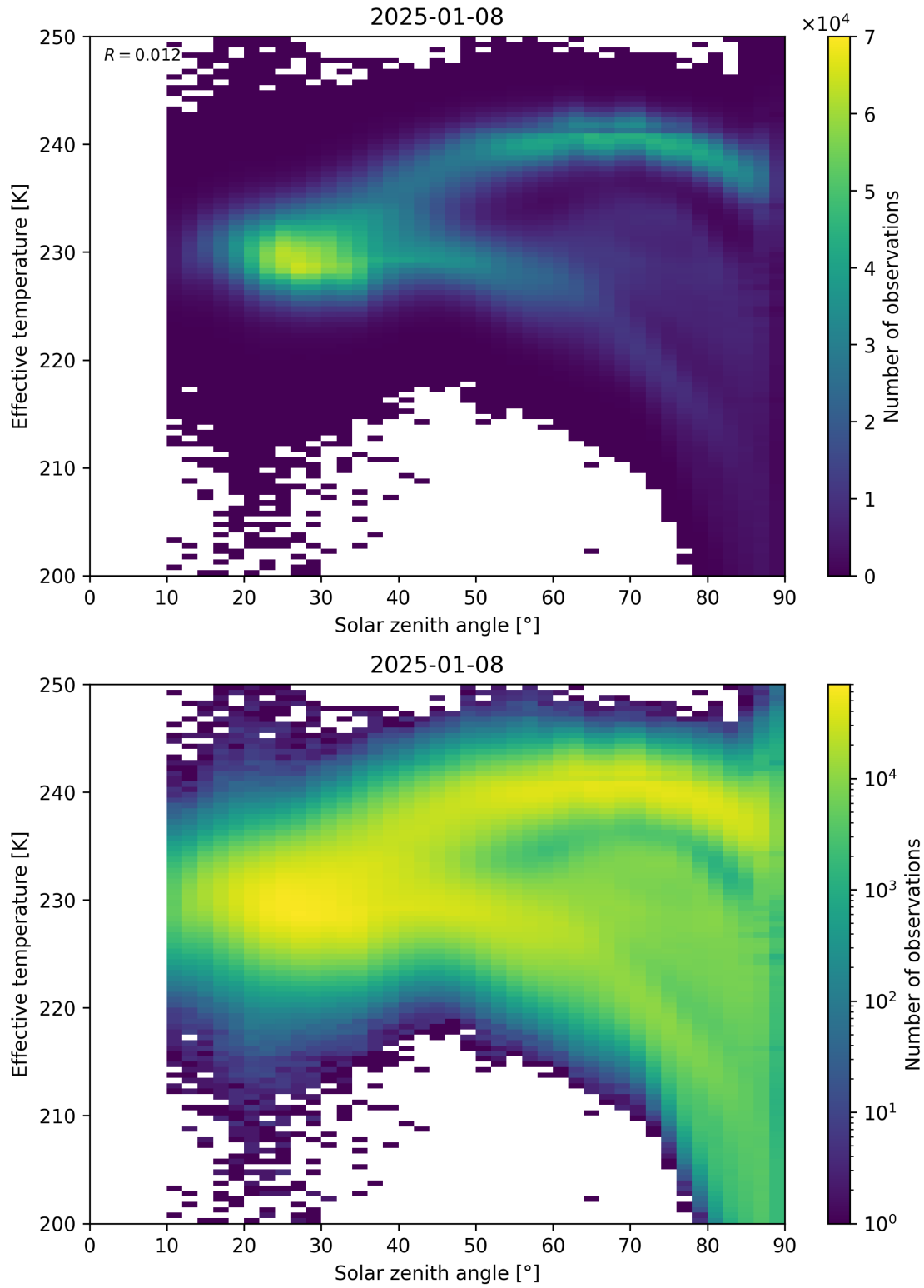
Figure 45: Scatter density plot of “Solar zenith angle” against “Effective temperature” for 2025-01-07 to 2025-01-09.
