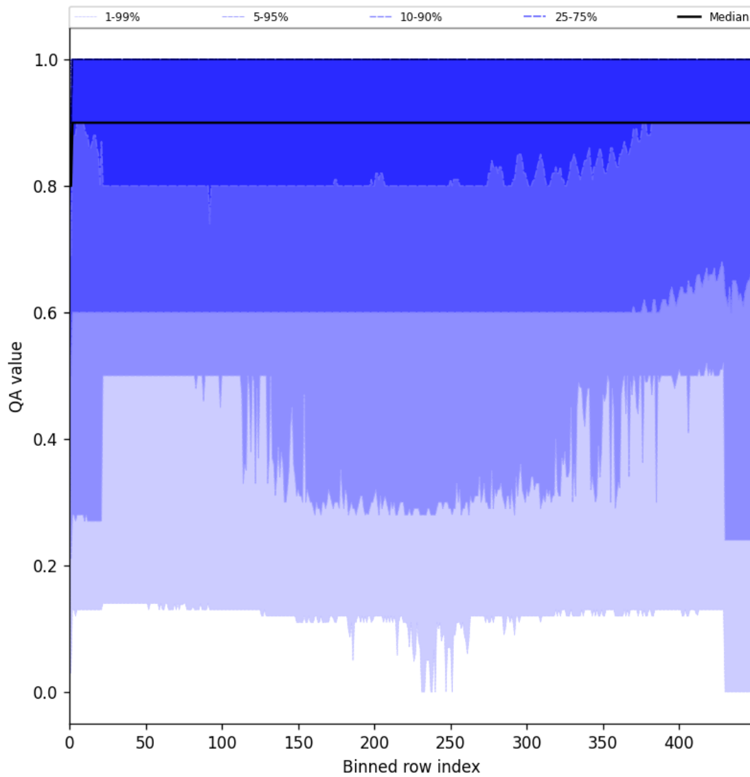
Figure 27: Along track statistics of “QA value” for 2025-01-07 to 2025-01-09
