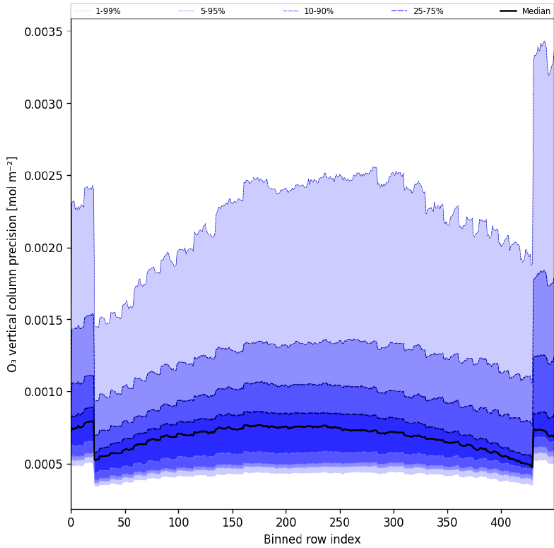
Figure 29: Along track statistics of “O 3 vertical column precision” for 2025-01-07 to 2025-01-09
