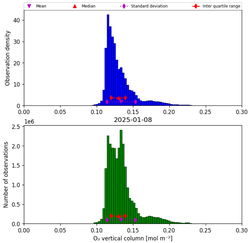
Figure 21: Histogram of “O 3 vertical column” for 2025-01-07 to 2025-01-09
