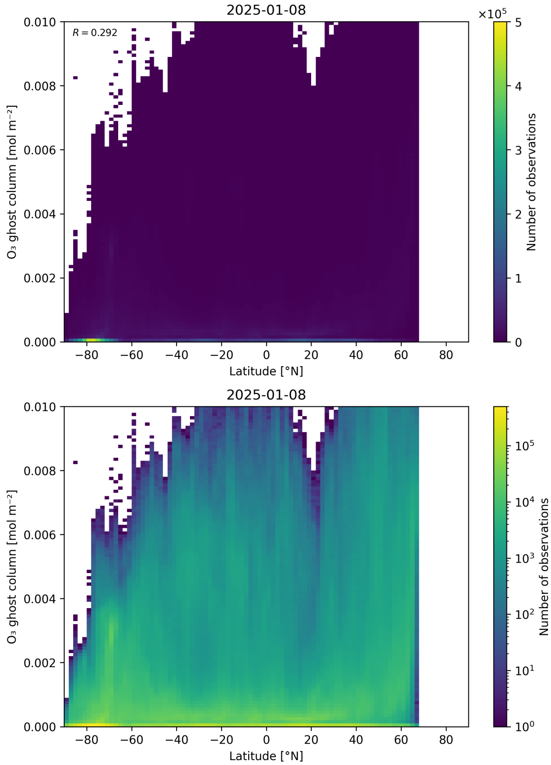
Figure 35: Scatter density plot of “Latitude” against “O 3 ghost column” for 2025-01-07 to 2025-01-09.
