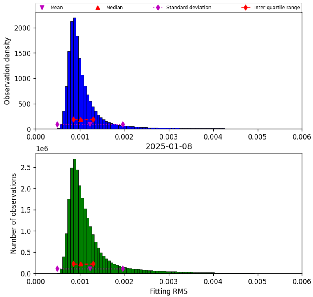
Figure 23: Histogram of “Fitting RMS” for 2025-01-07 to 2025-01-09
