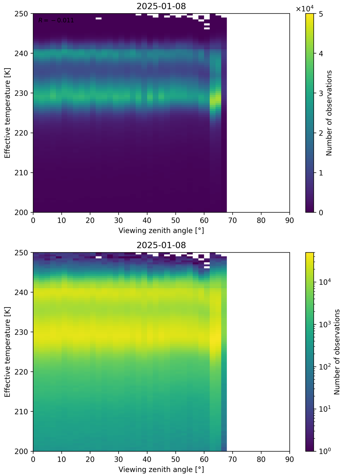
Figure 50: Scatter density plot of “Viewing zenith angle” against “Effective temperature” for 2025-01-07 to 2025-01-09.
