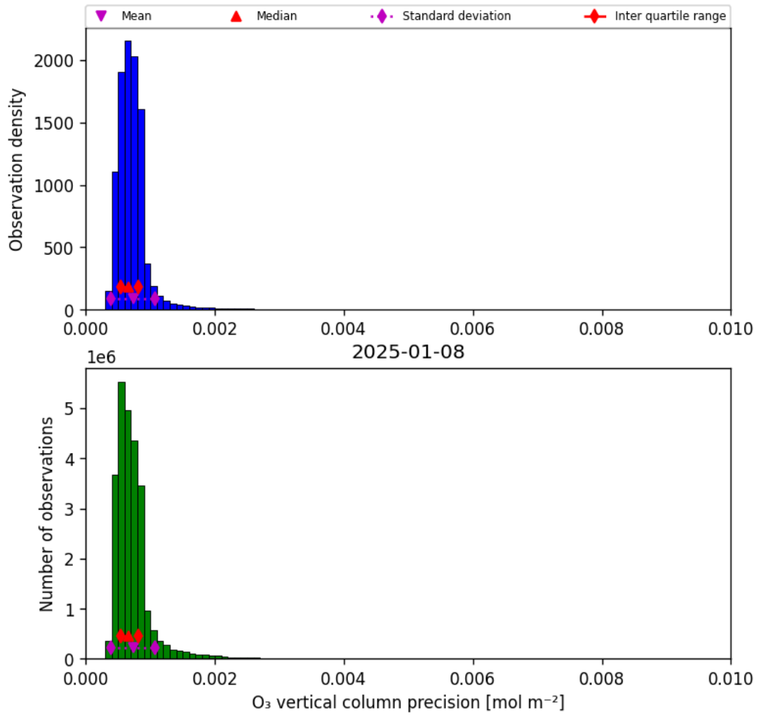
Figure 22: Histogram of “O 3 vertical column precision” for 2025-01-07 to 2025-01-09
