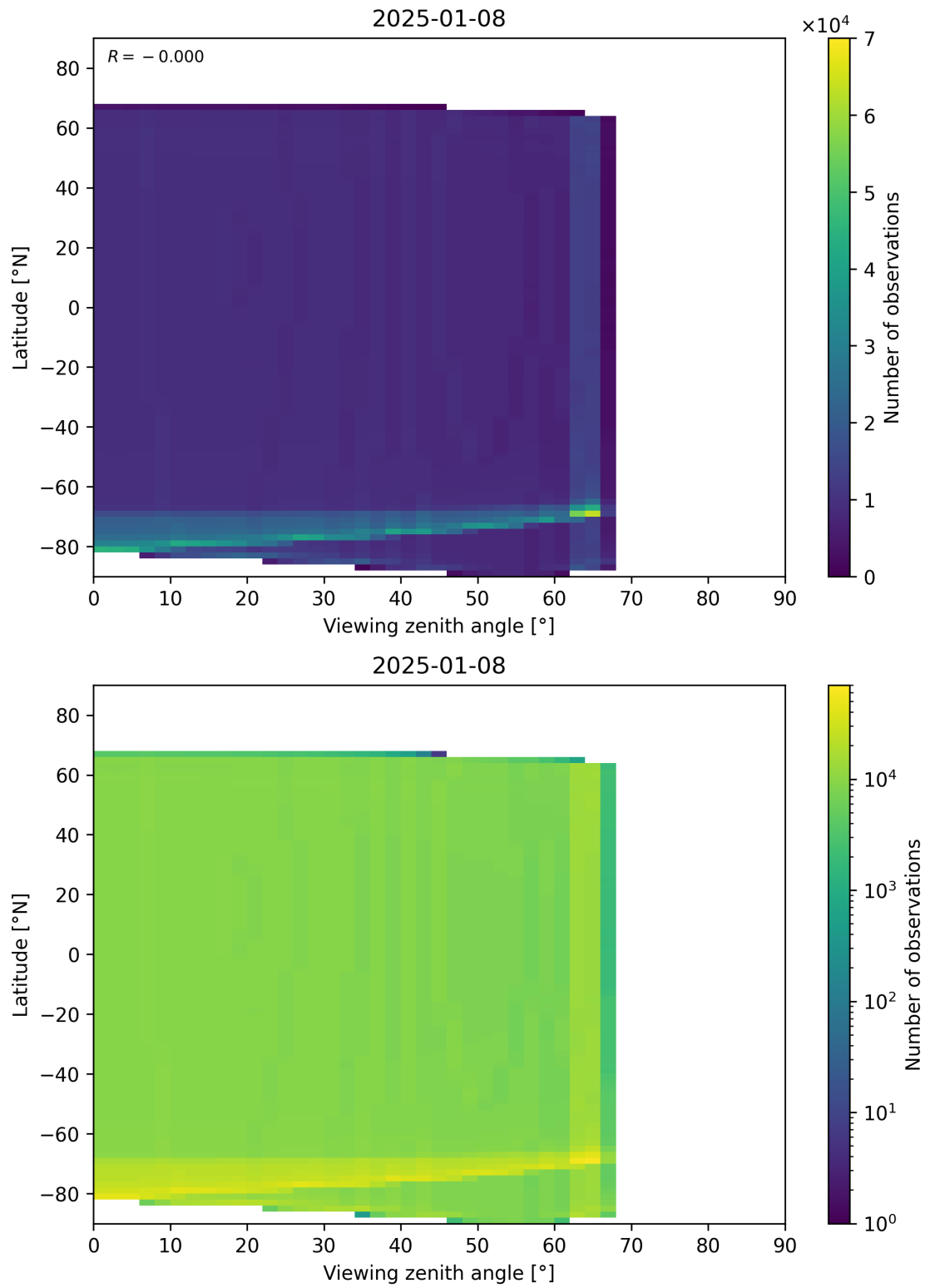
Figure 49: Scatter density plot of “Viewing zenith angle” against “Latitude” for 2025-01-07 to 2025-01-09.
