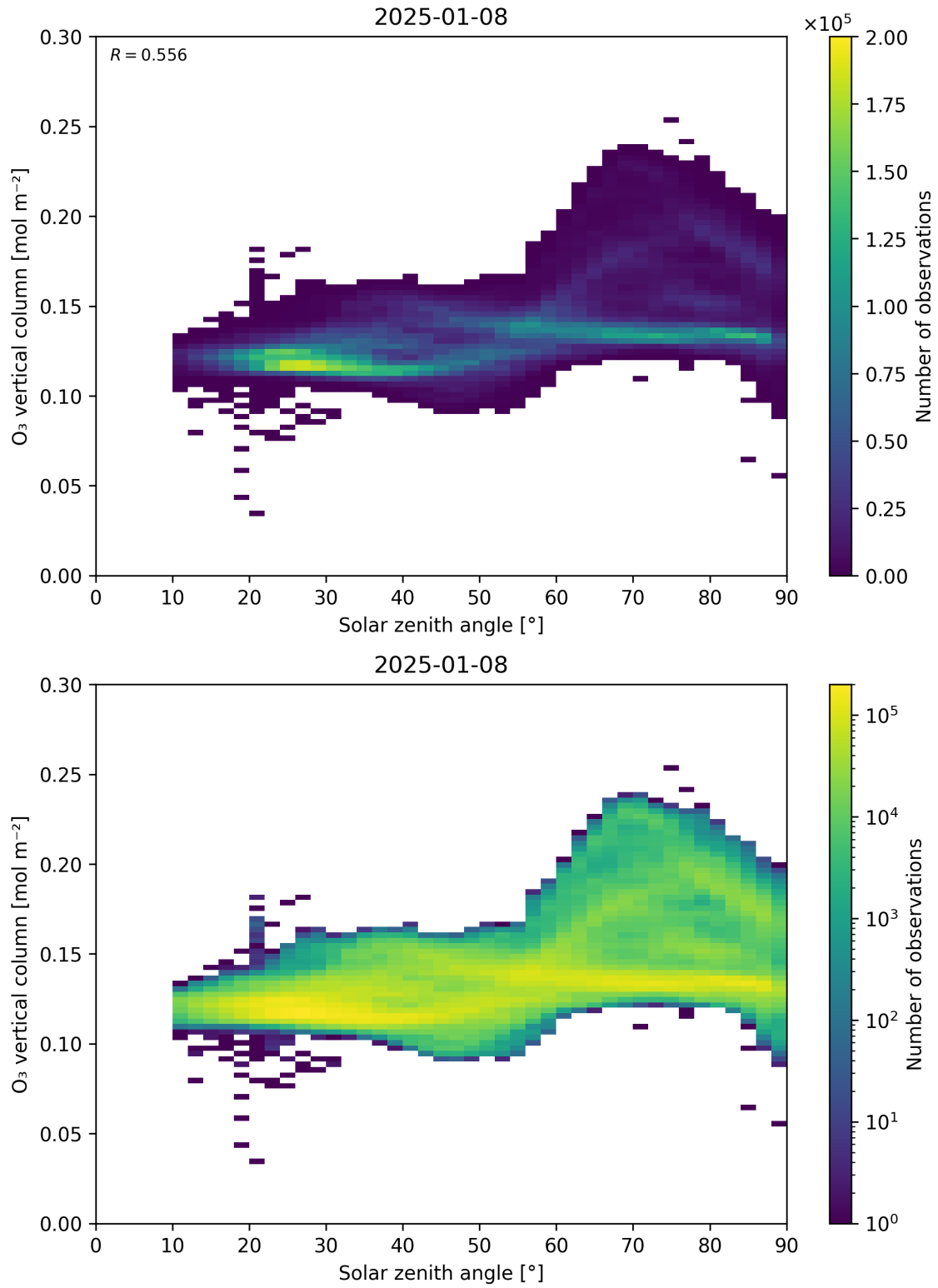
Figure 47: Scatter density plot of “Solar zenith angle” against “O 3 vertical column” for 2025-01-07 to 2025-01-09.
