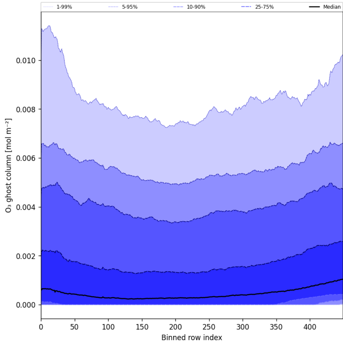
Figure 32: Along track statistics of “O 3 ghost column” for 2025-01-07 to 2025-01-09
