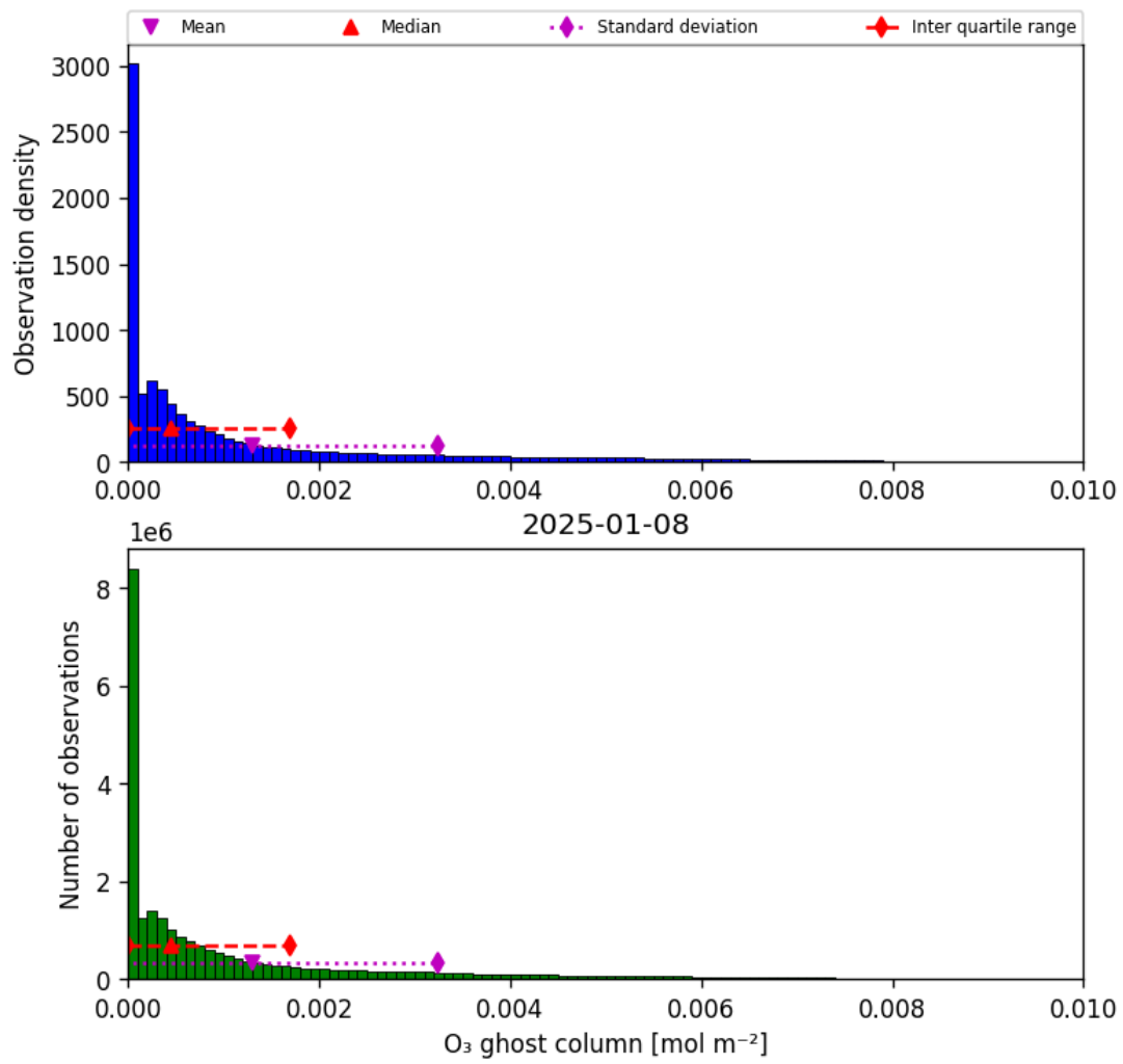
Figure 25: Histogram of “O 3 ghost column” for 2025-01-07 to 2025-01-09
