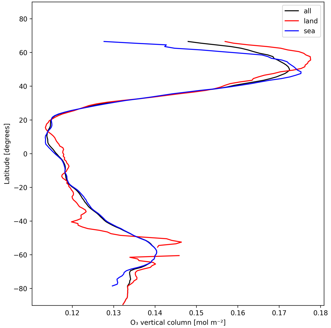
Figure 14: Zonal average of “O 3 vertical column” for 2025-01-07 to 2025-01-09.
