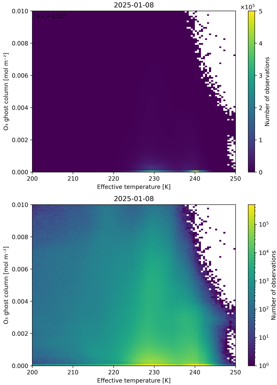
Figure 38: Scatter density plot of “Effective temperature” against “O 3 ghost column” for 2025-01-07 to 2025-01-09.
