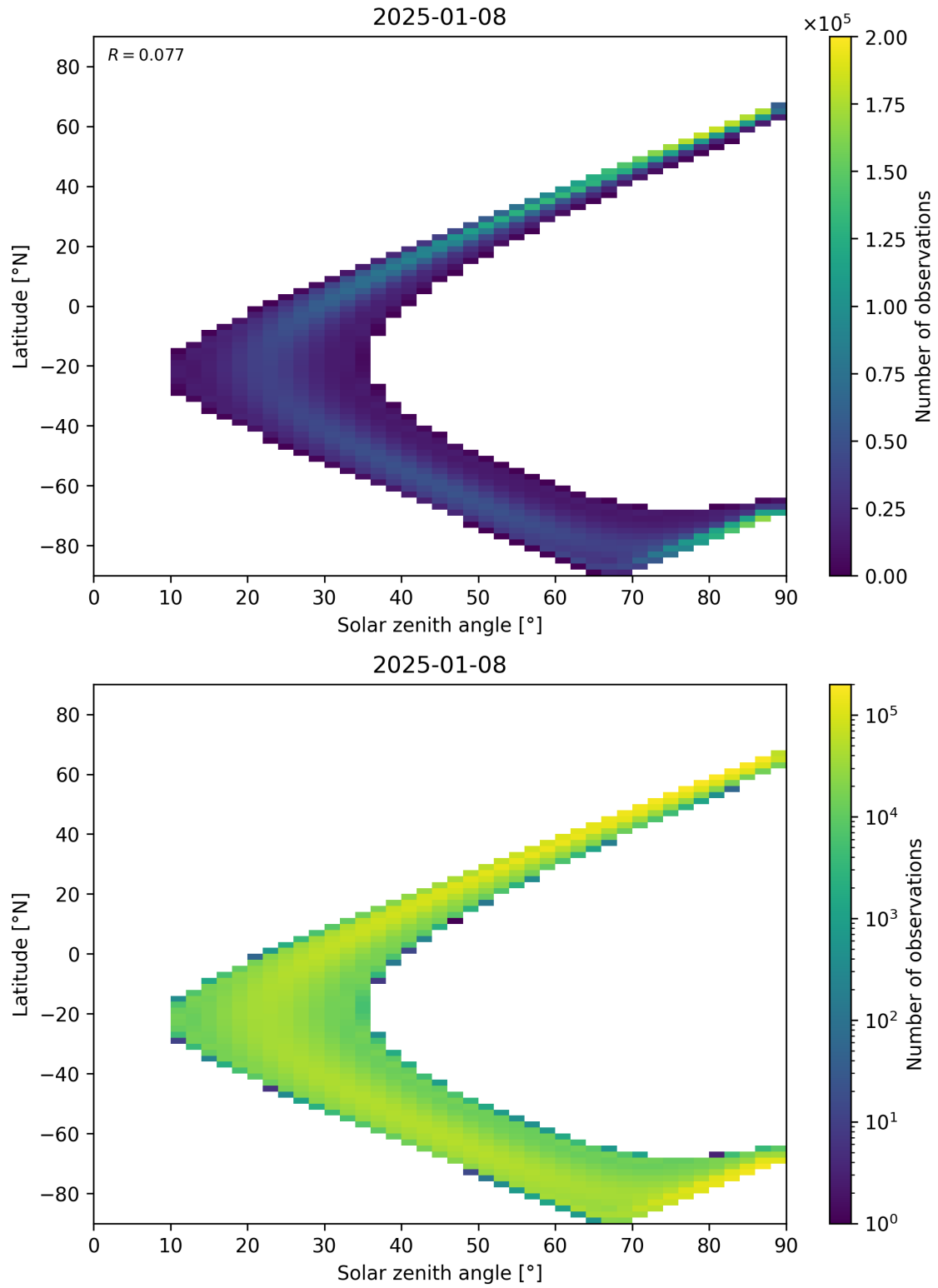
Figure 44: Scatter density plot of “Solar zenith angle” against “Latitude” for 2025-01-07 to 2025-01-09.
