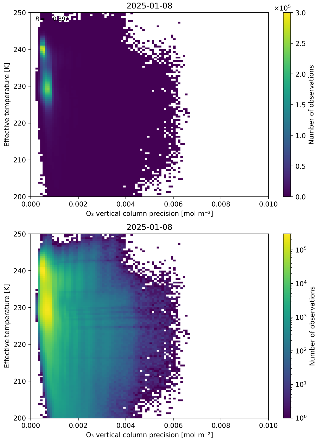
Figure 42: Scatter density plot of “O 3 vertical column precision” against “Effective temperature” for 2025-01-07 to 2025-01-09.
