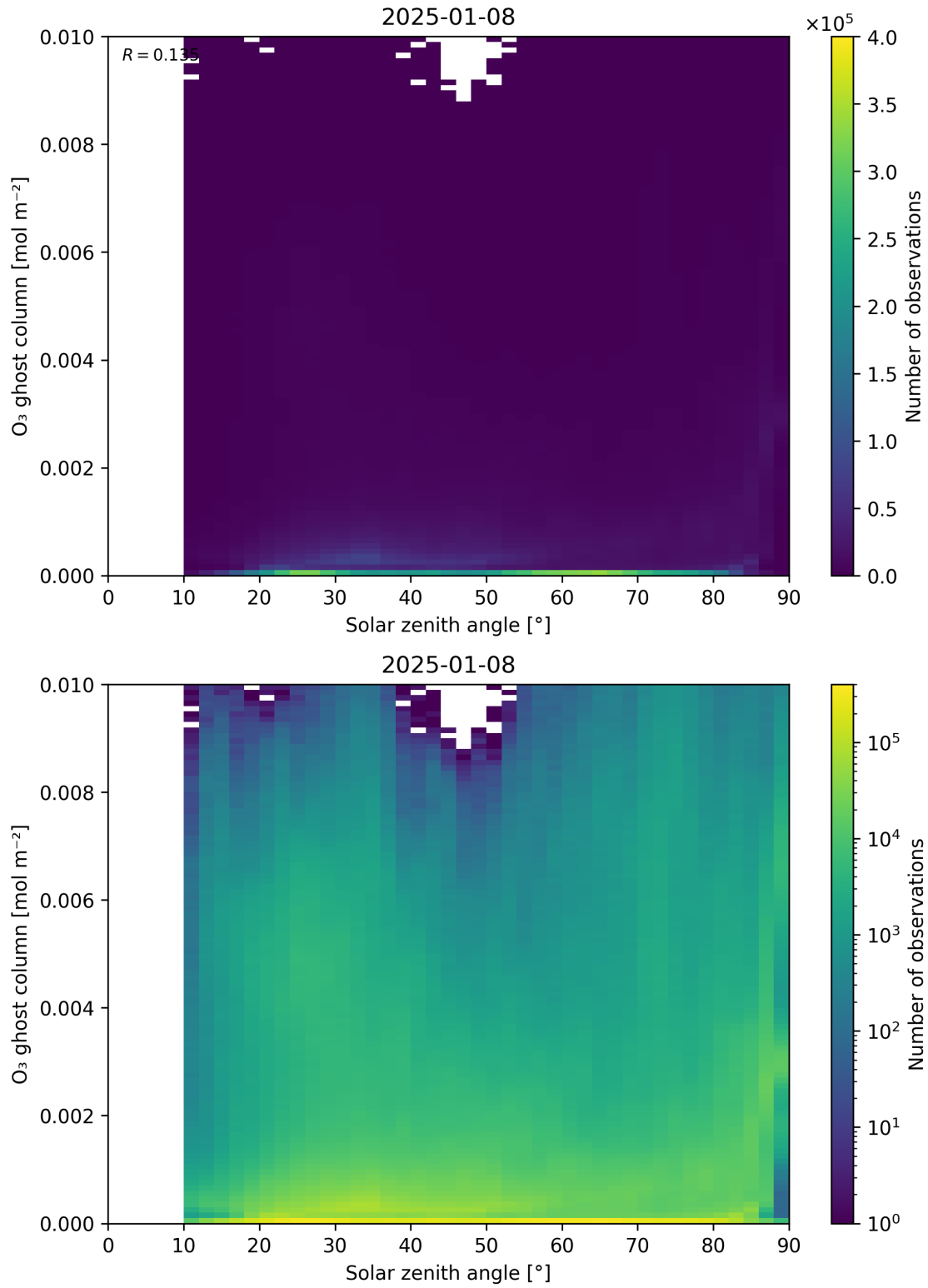
Figure 46: Scatter density plot of “Solar zenith angle” against “O 3 ghost column” for 2025-01-07 to 2025-01-09.
