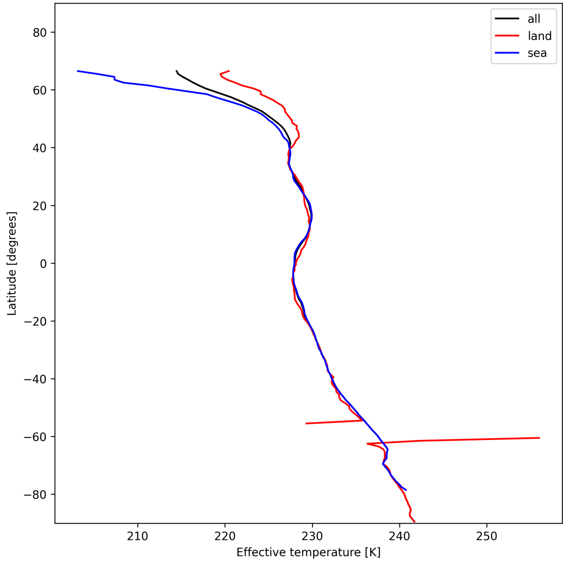
Figure 17: Zonal average of "Effective temperature" for 2025-01-07 to 2025-01-09.
