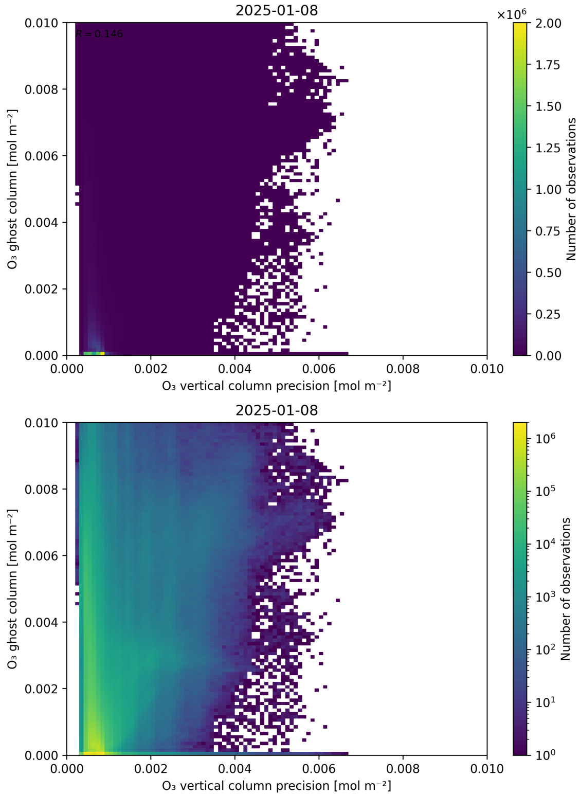
Figure 43: Scatter density plot of “ \text{O}_3 vertical column precision” against “ \text{O}_3 ghost column” for 2025-01-07 to 2025-01-09.
