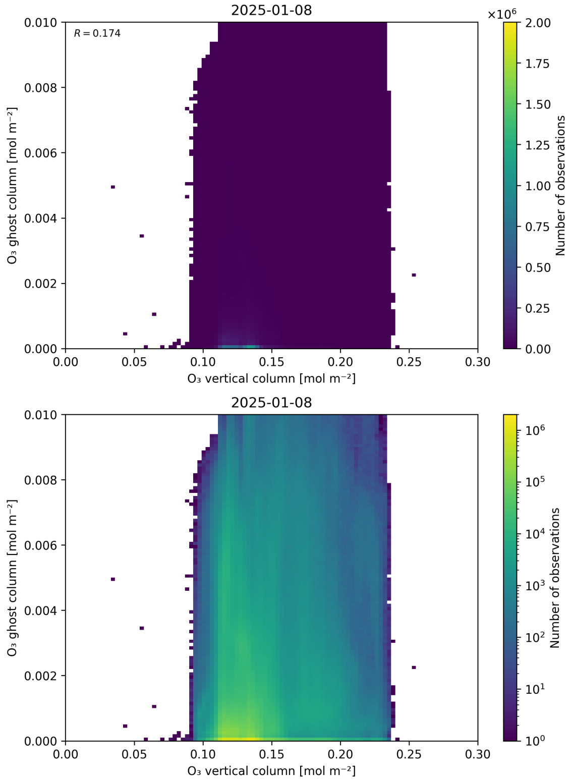
Figure 40: Scatter density plot of “O 3 vertical column” against “O 3 ghost column” for 2025-01-07 to 2025-01-09.
