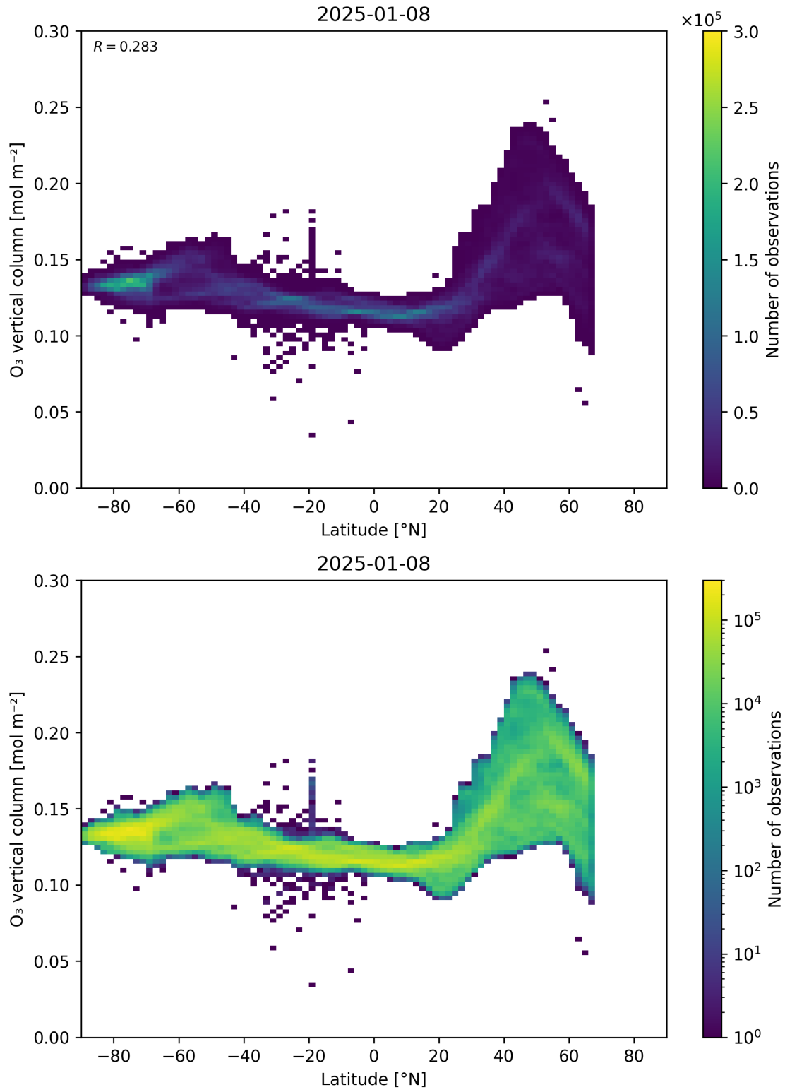
Figure 36: Scatter density plot of “Latitude” against “O 3 vertical column” for 2025-01-07 to 2025-01-09.
