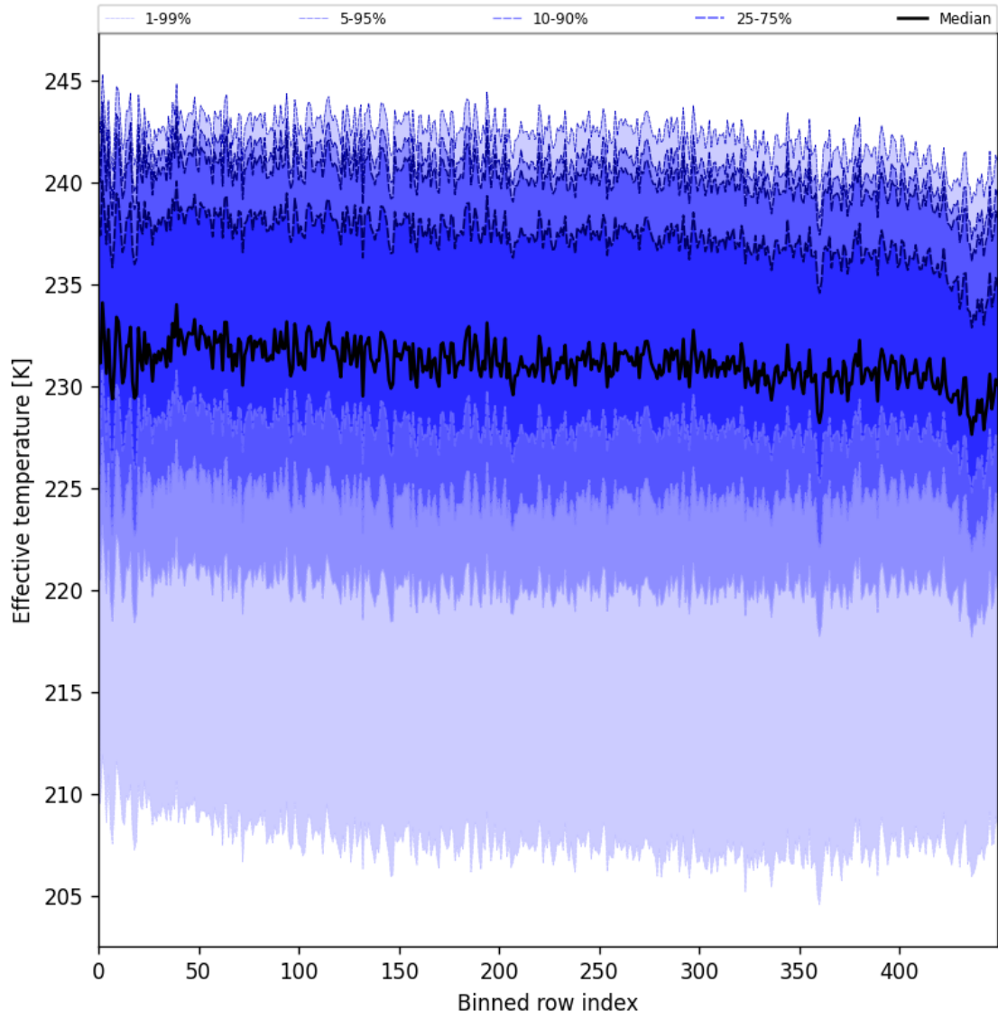
Figure 31: Along track statistics of “Effective temperature” for 2025-01-07 to 2025-01-09
