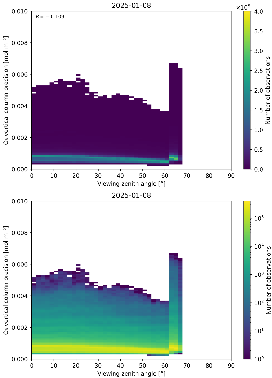
Figure 53: Scatter density plot of “Viewing zenith angle” against “O 3 vertical column precision” for 2025-01-07 to 2025-01-09.
