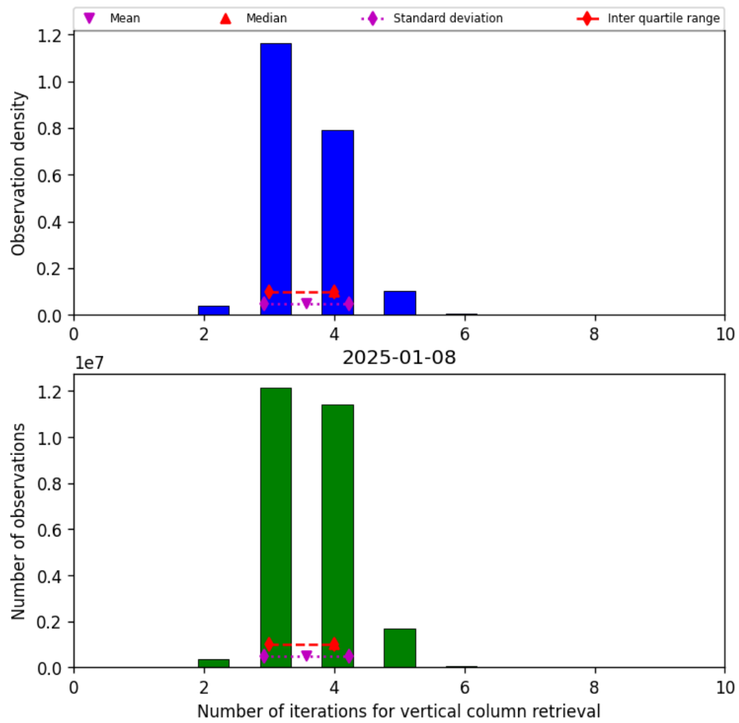
Figure 26: Histogram of “Number of iterations for vertical column retrieval” for 2025-01-07 to 2025-01-09
