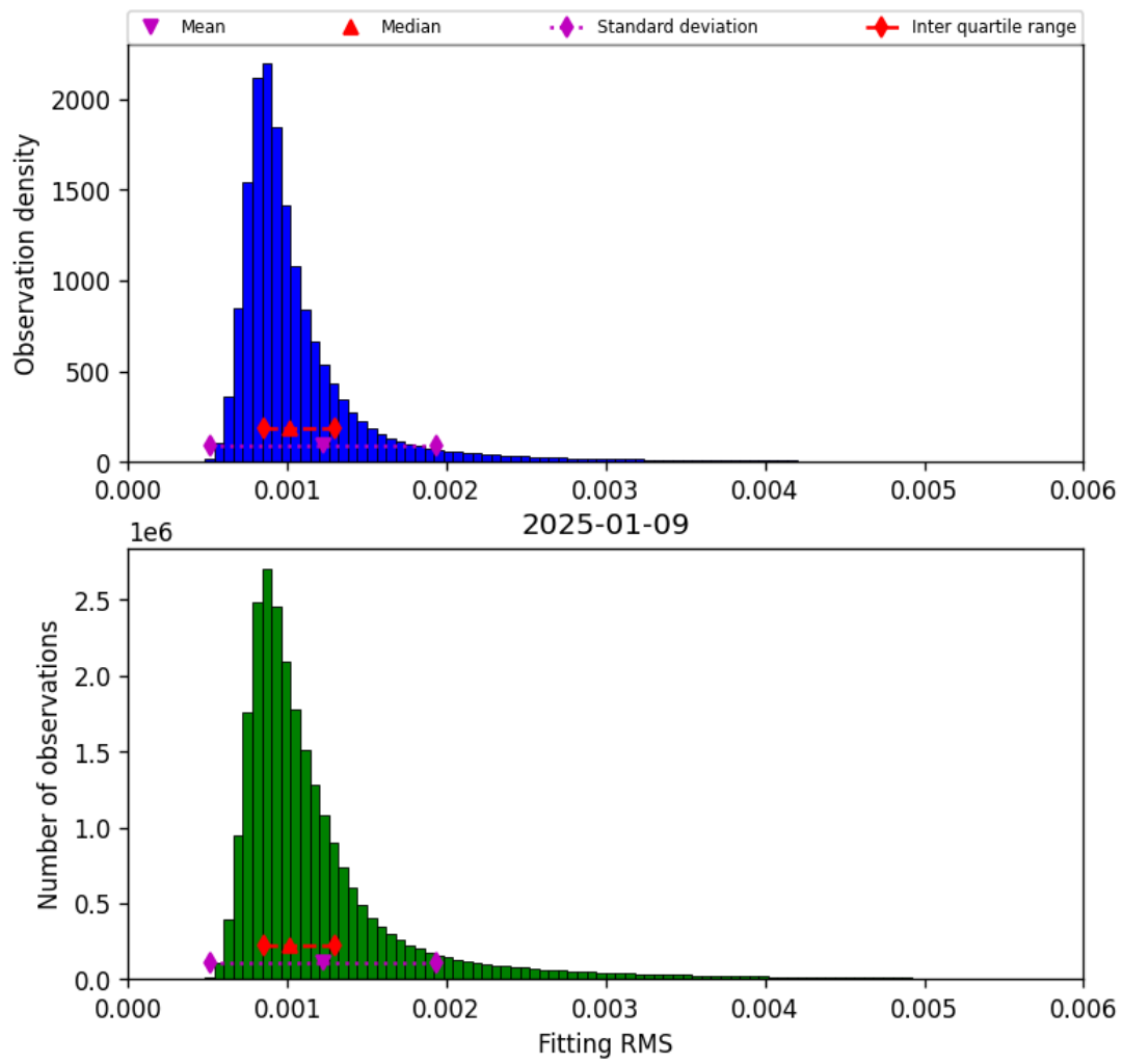
Figure 23: Histogram of “Fitting RMS” for 2025-01-08 to 2025-01-10
