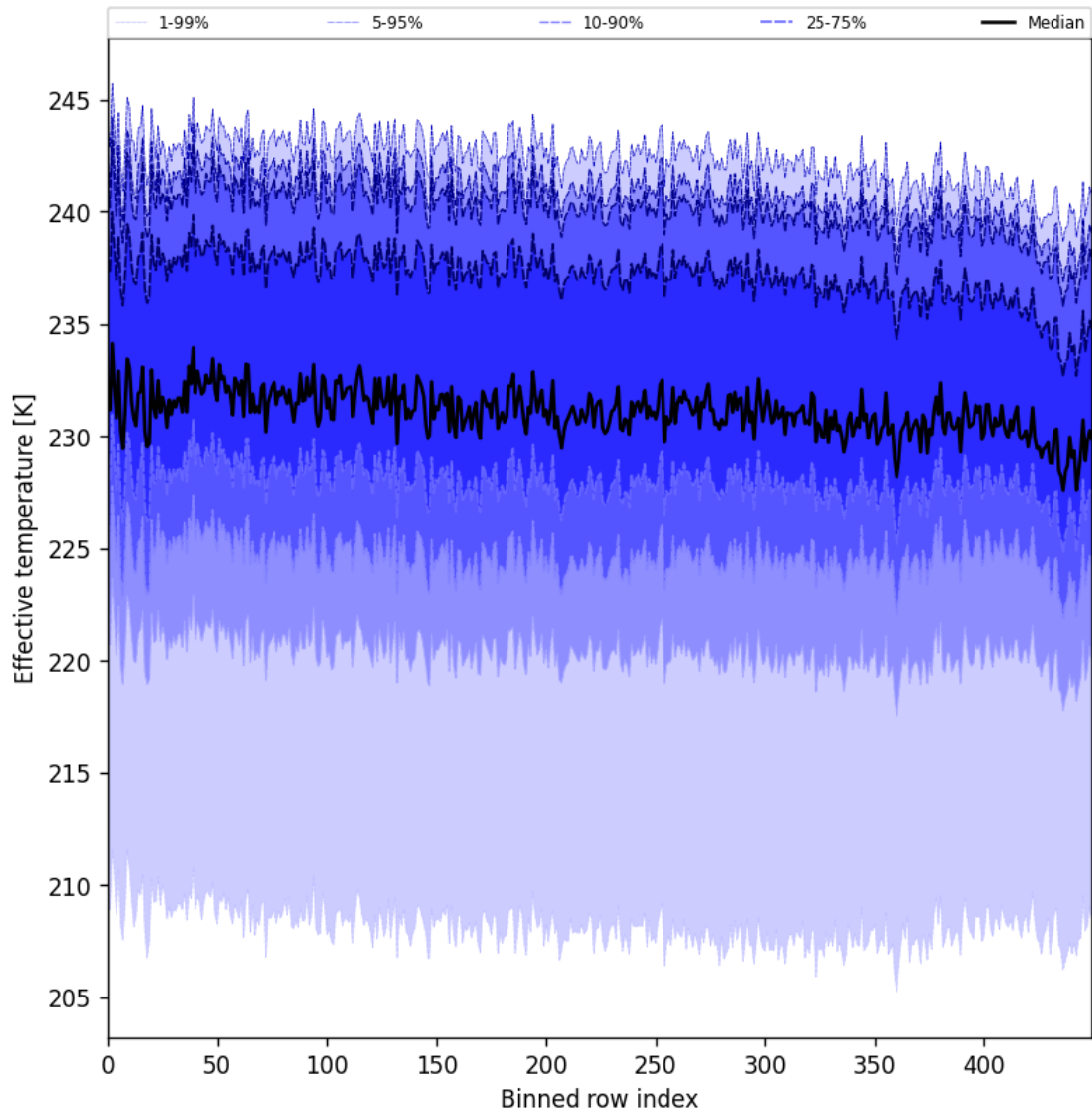
Figure 31: Along track statistics of “Effective temperature” for 2025-01-08 to 2025-01-10
