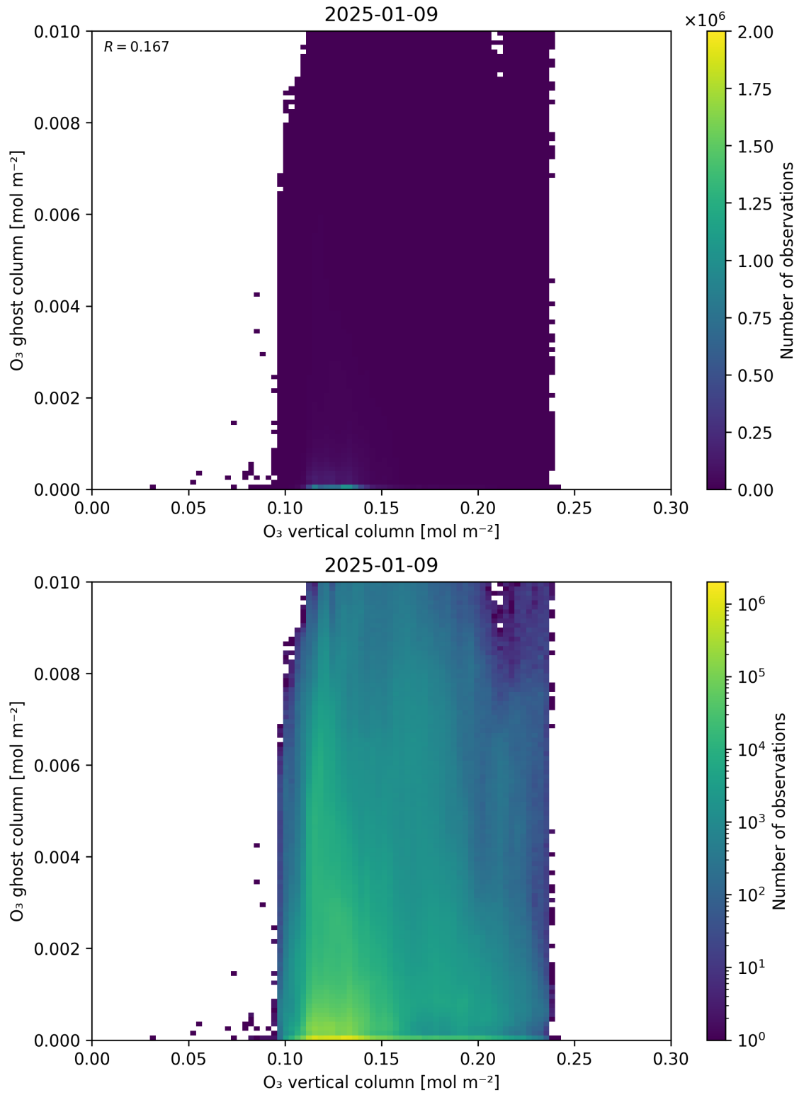
Figure 40: Scatter density plot of “O 3 vertical column” against “O 3 ghost column” for 2025-01-08 to 2025-01-10.
