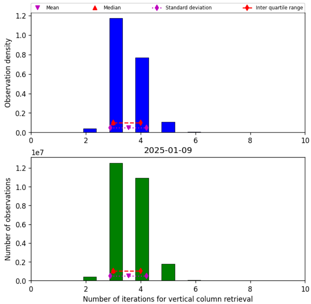
Figure 26: Histogram of “Number of iterations for vertical column retrieval” for 2025-01-08 to 2025-01-10
