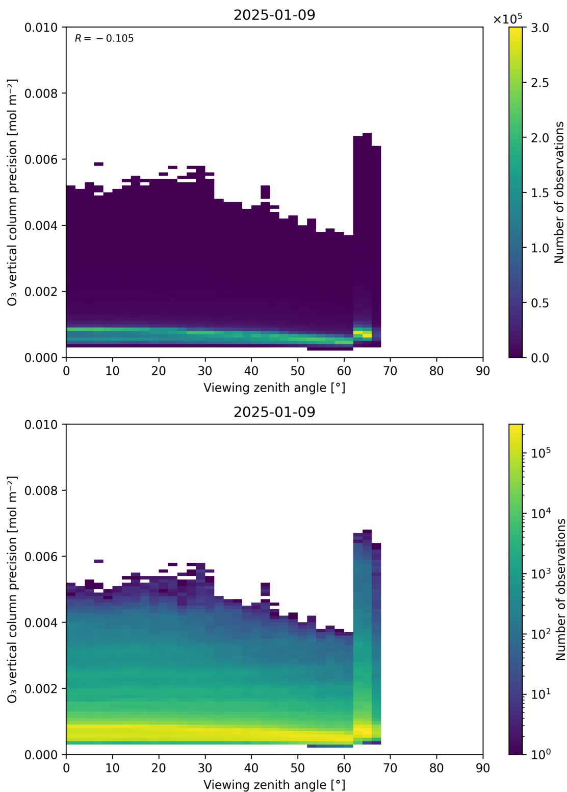
Figure 53: Scatter density plot of “Viewing zenith angle” against “O 3 vertical column precision” for 2025-01-08 to 2025-01-10.
