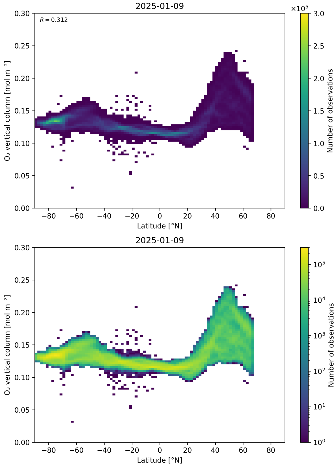
Figure 36: Scatter density plot of “Latitude” against “O 3 vertical column” for 2025-01-08 to 2025-01-10.
