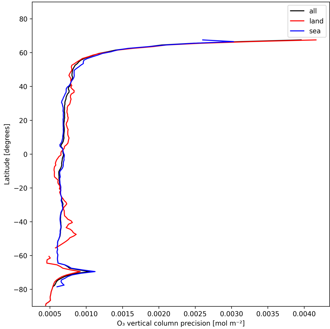
Figure 15: Zonal average of “O 3 vertical column precision” for 2025-01-08 to 2025-01-10.
