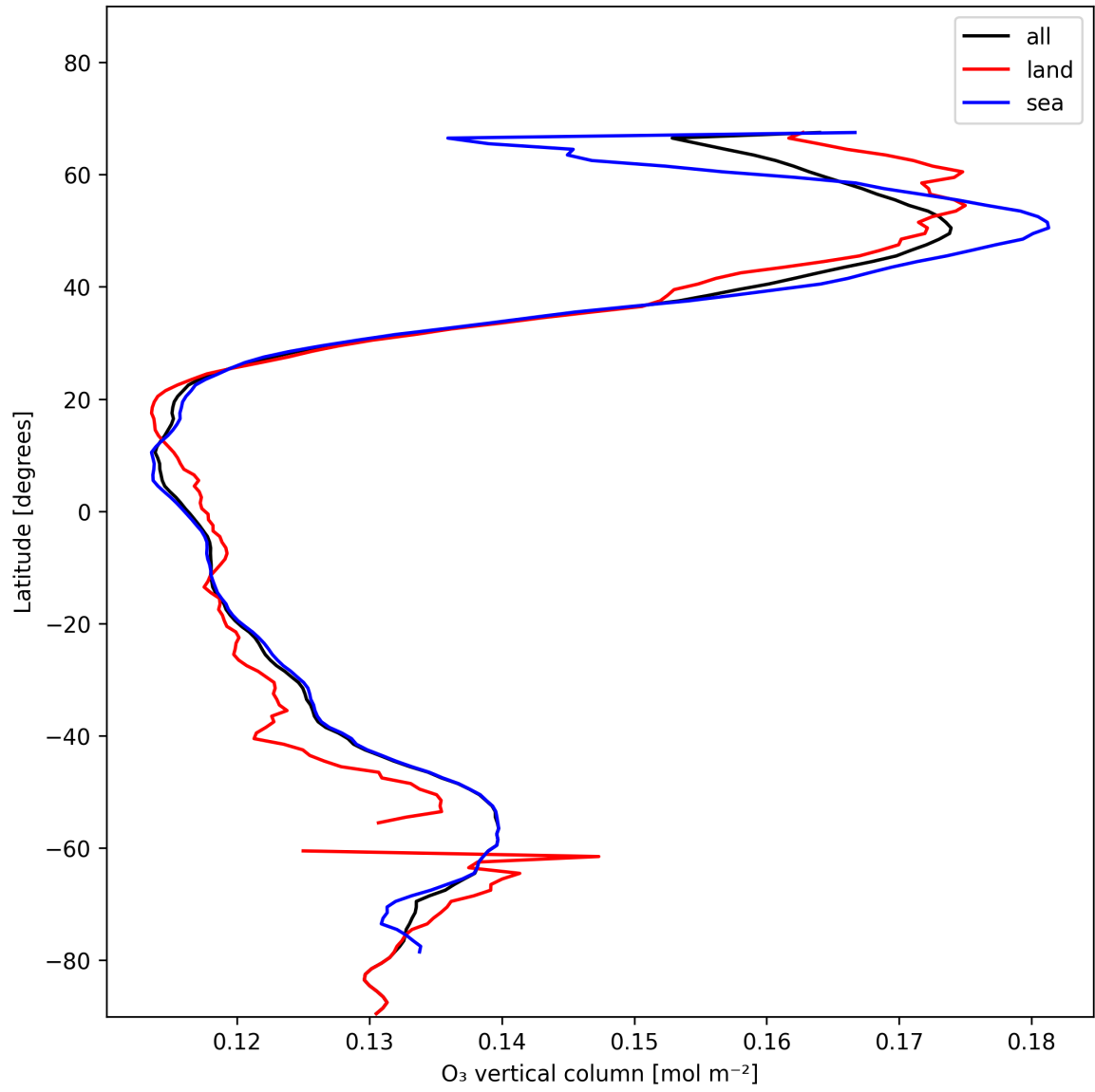
Figure 14: Zonal average of “O 3 vertical column” for 2025-01-08 to 2025-01-10.
