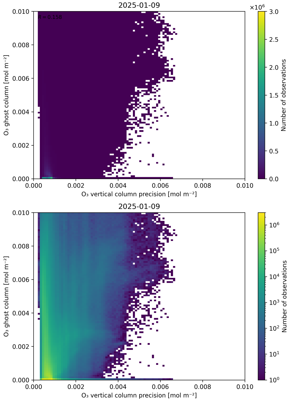
Figure 43: Scatter density plot of “ \text{O}_3 vertical column precision” against “ \text{O}_3 ghost column” for 2025-01-08 to 2025-01-10.
