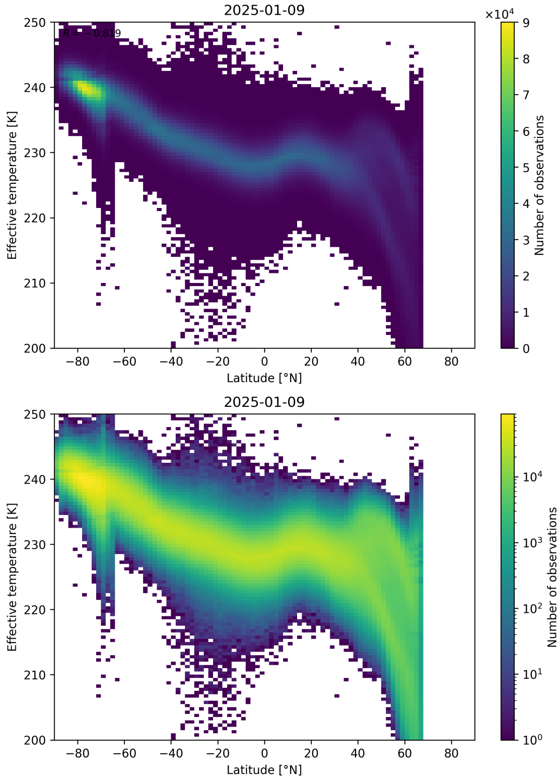
Figure 34: Scatter density plot of “Latitude” against “Effective temperature” for 2025-01-08 to 2025-01-10.
