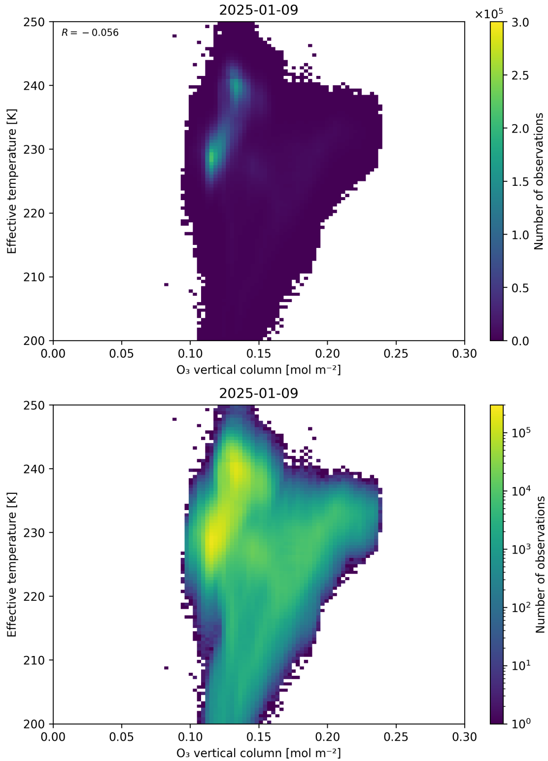
Figure 39: Scatter density plot of “O 3 vertical column” against “Effective temperature” for 2025-01-08 to 2025-01-10.
