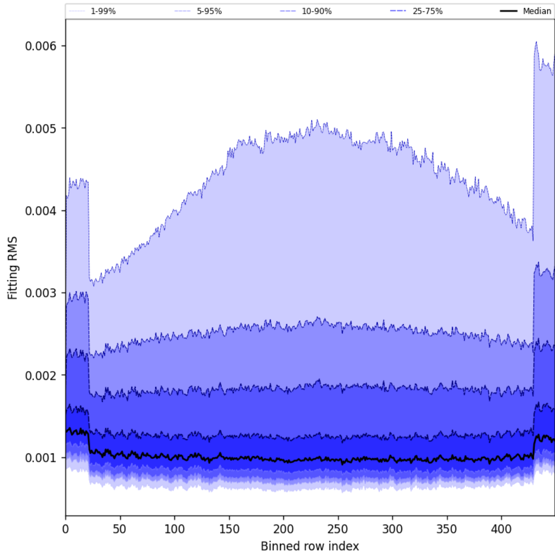
Figure 30: Along track statistics of “Fitting RMS” for 2025-01-08 to 2025-01-10
