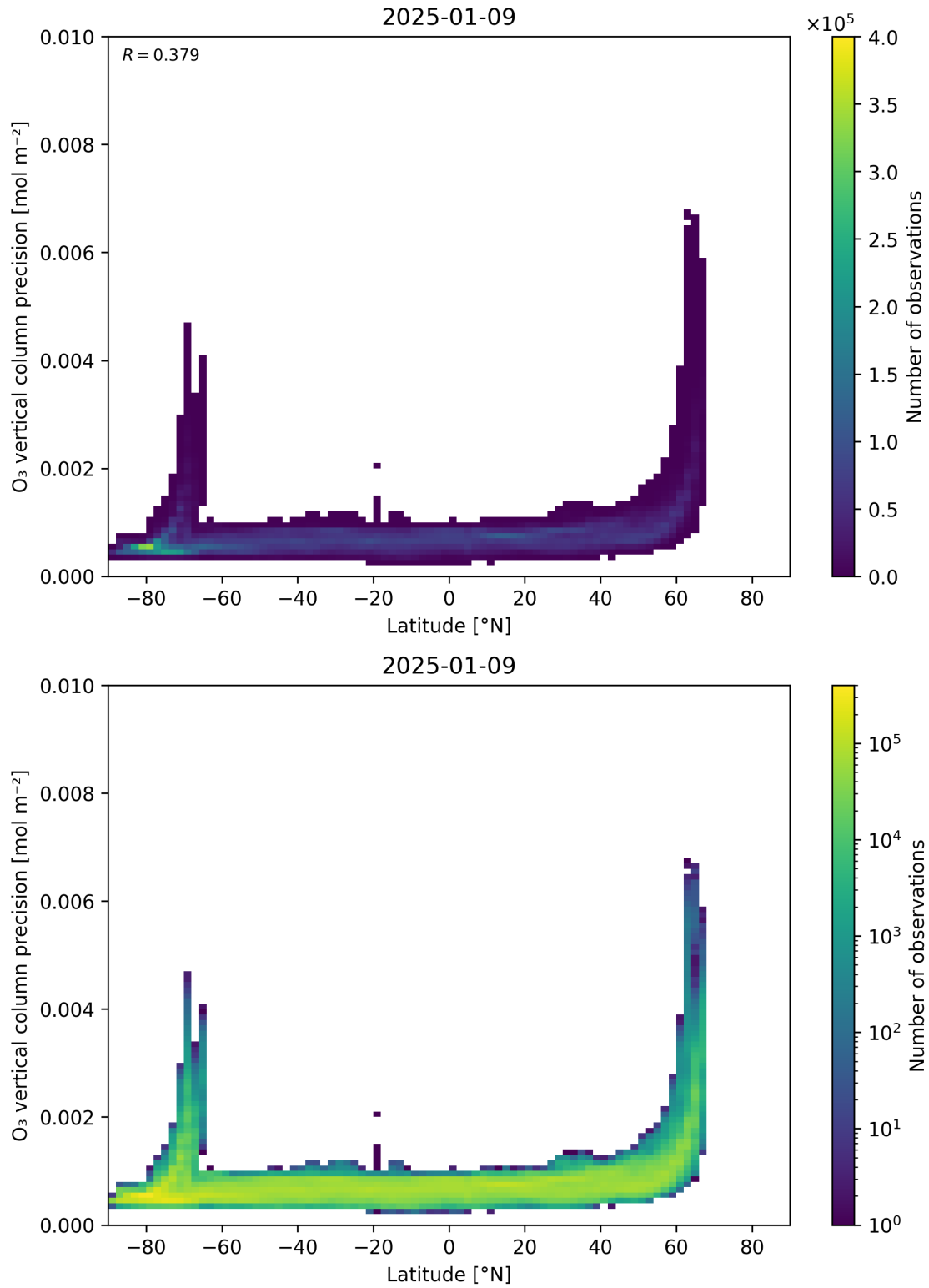
Figure 37: Scatter density plot of “Latitude” against “O 3 vertical column precision” for 2025-01-08 to 2025-01-10.
