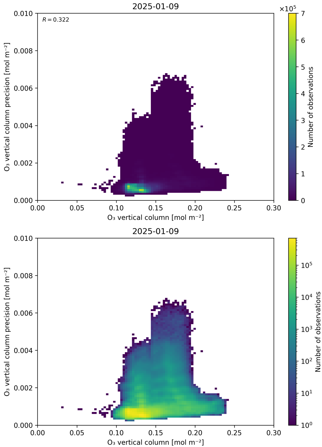
Figure 41: Scatter density plot of “O 3 vertical column” against “O 3 vertical column precision” for 2025-01-08 to 2025-01-10.
