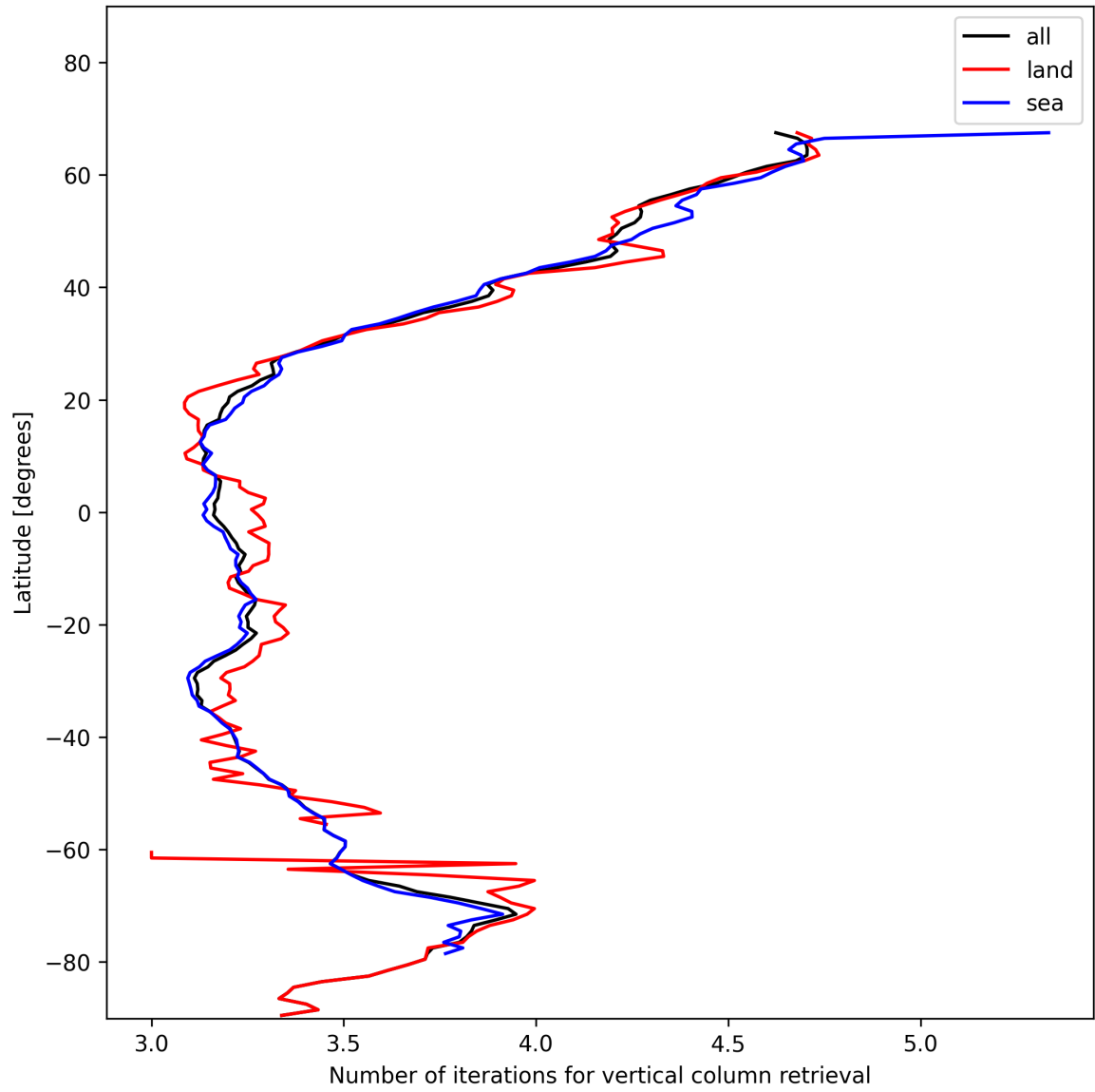
Figure 19: Zonal average of “Number of iterations for vertical column retrieval” for 2025-01-08 to 2025-01-10.
