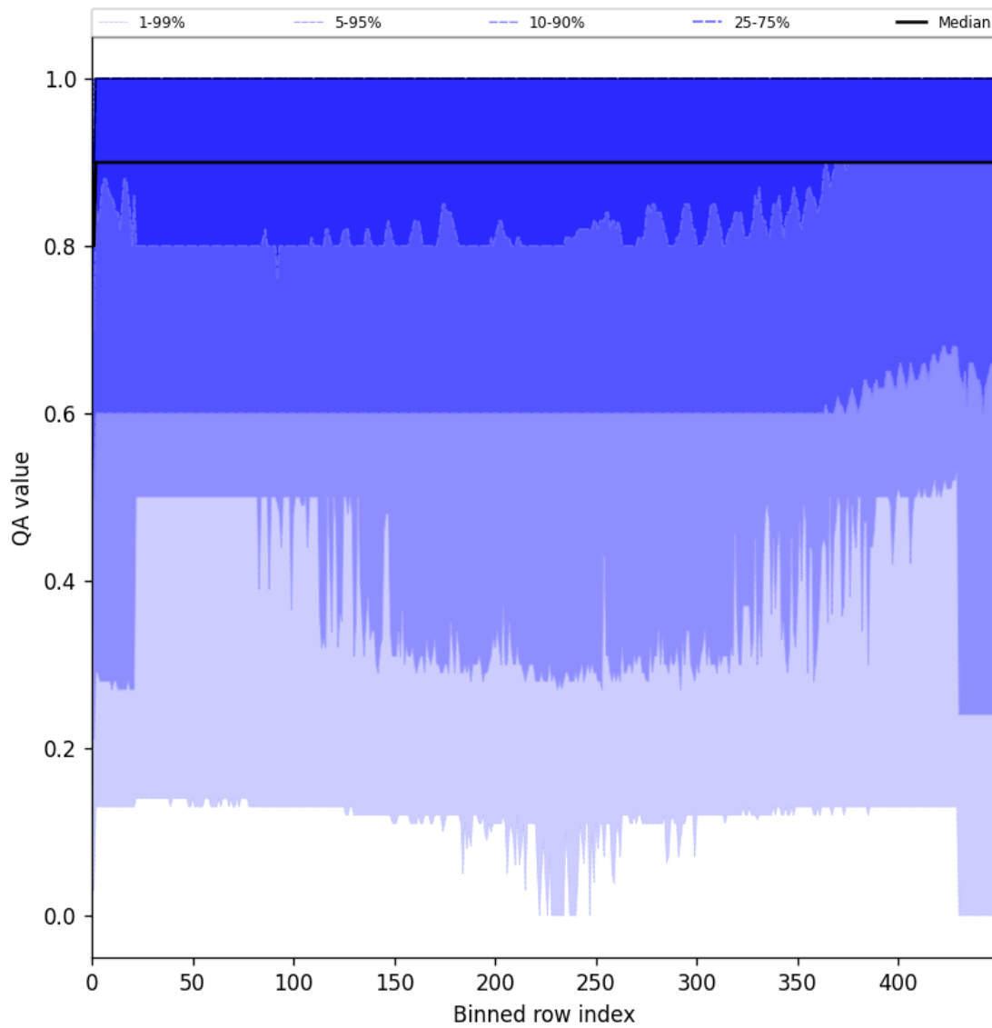
Figure 27: Along track statistics of “QA value” for 2025-01-08 to 2025-01-10
