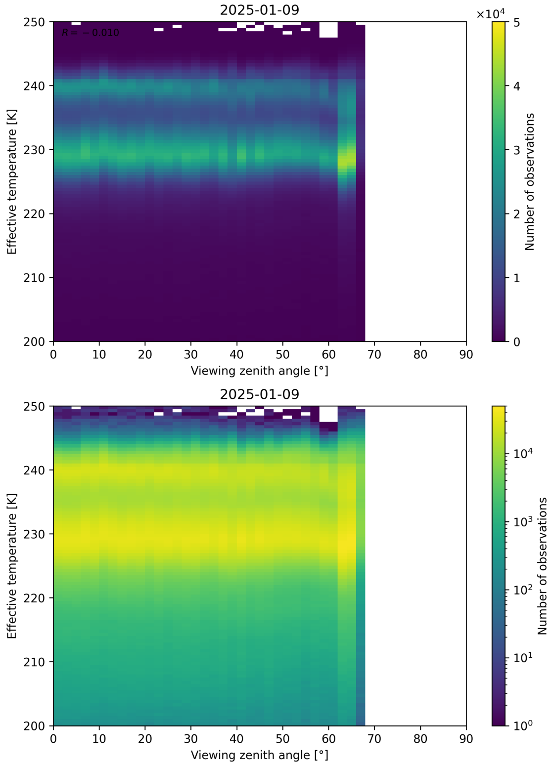
Figure 50: Scatter density plot of “Viewing zenith angle” against “Effective temperature” for 2025-01-08 to 2025-01-10.
