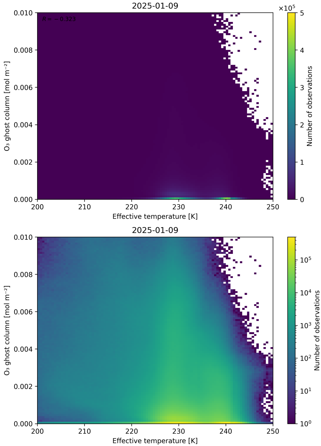
Figure 38: Scatter density plot of “Effective temperature” against “O 3 ghost column” for 2025-01-08 to 2025-01-10.
