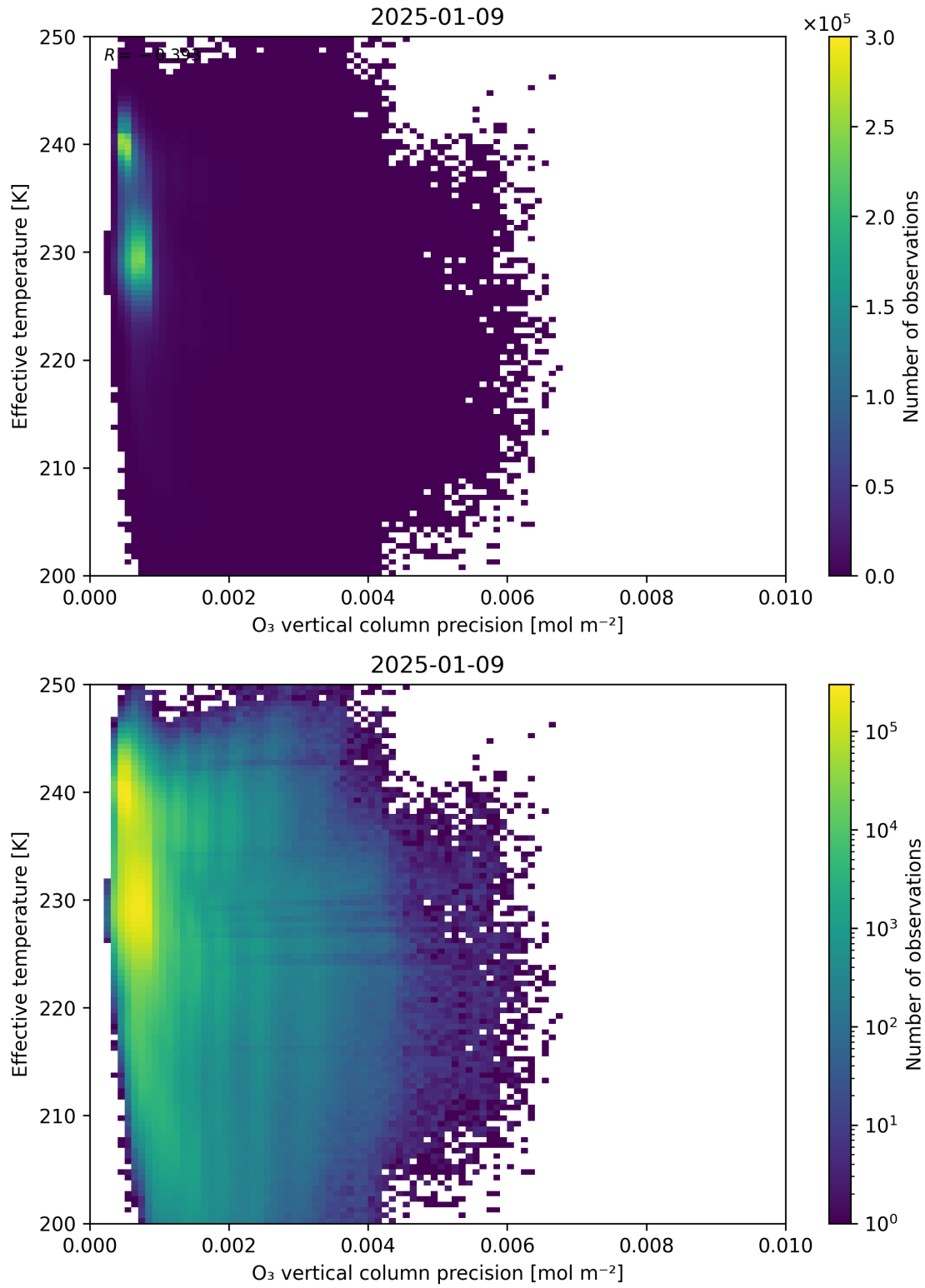
Figure 42: Scatter density plot of “O 3 vertical column precision” against “Effective temperature” for 2025-01-08 to 2025-01-10.
