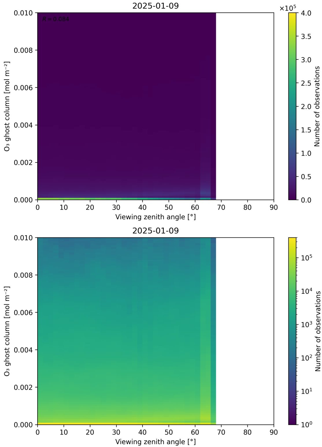
Figure 51: Scatter density plot of “Viewing zenith angle” against “O 3 ghost column” for 2025-01-08 to 2025-01-10.
