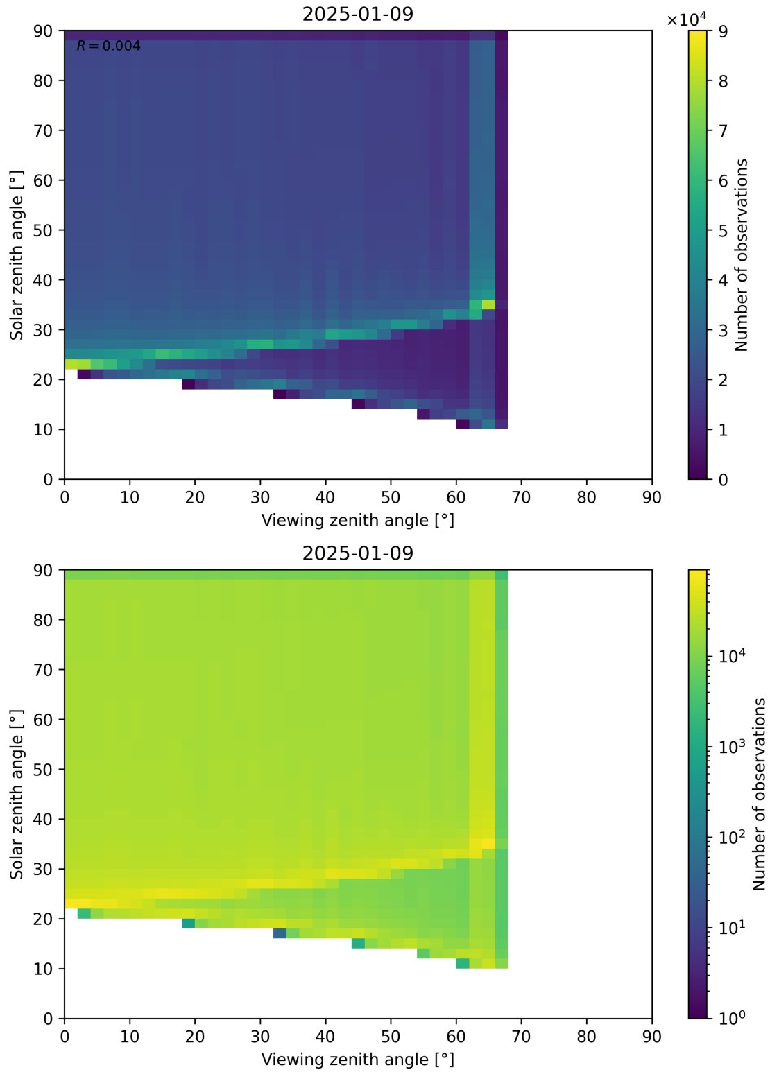
Figure 54: Scatter density plot of “Viewing zenith angle” against “Solar zenith angle” for 2025-01-08 to 2025-01-10.
