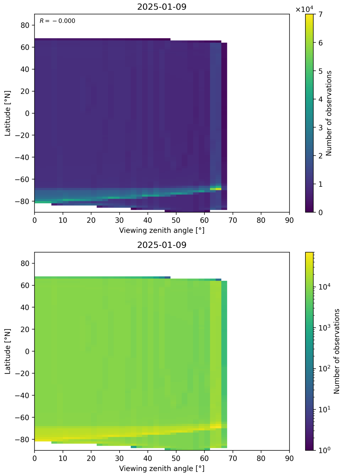
Figure 49: Scatter density plot of “Viewing zenith angle” against “Latitude” for 2025-01-08 to 2025-01-10.
