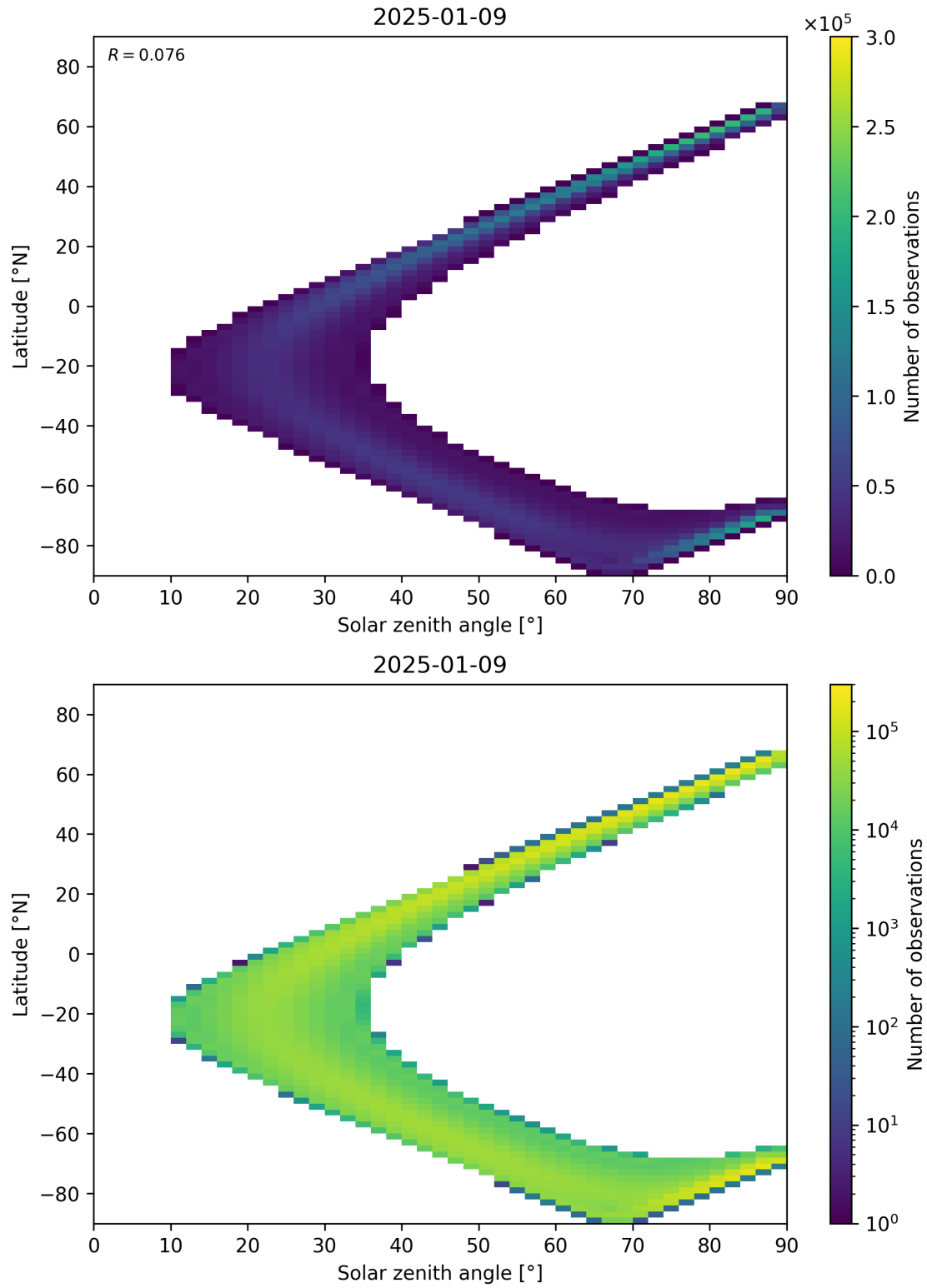
Figure 44: Scatter density plot of “Solar zenith angle” against “Latitude” for 2025-01-08 to 2025-01-10.
