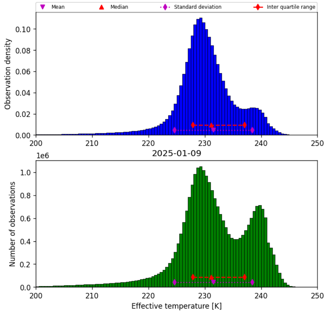
Figure 24: Histogram of “Effective temperature” for 2025-01-08 to 2025-01-10
