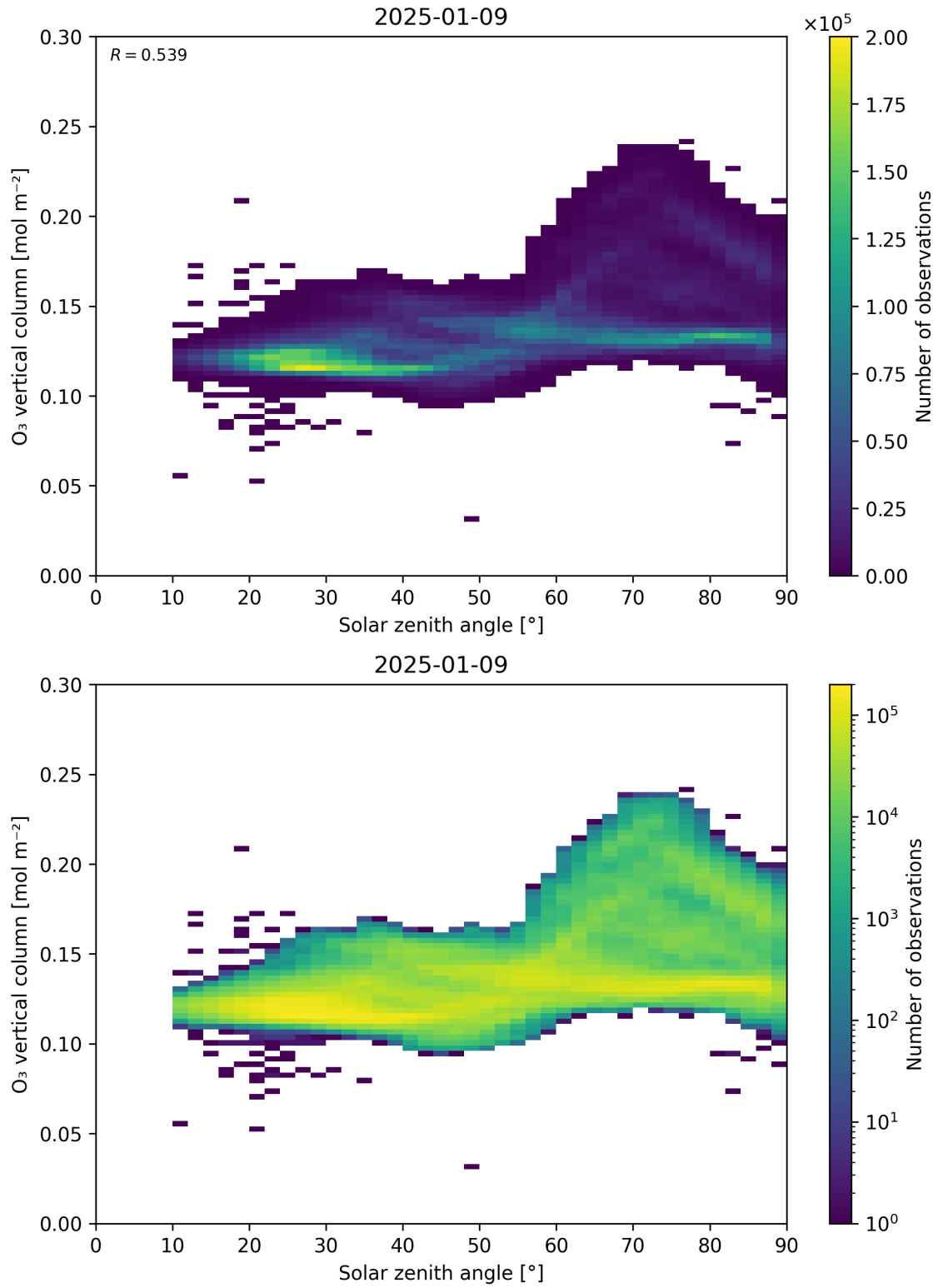
Figure 47: Scatter density plot of “Solar zenith angle” against “O 3 vertical column” for 2025-01-08 to 2025-01-10.
