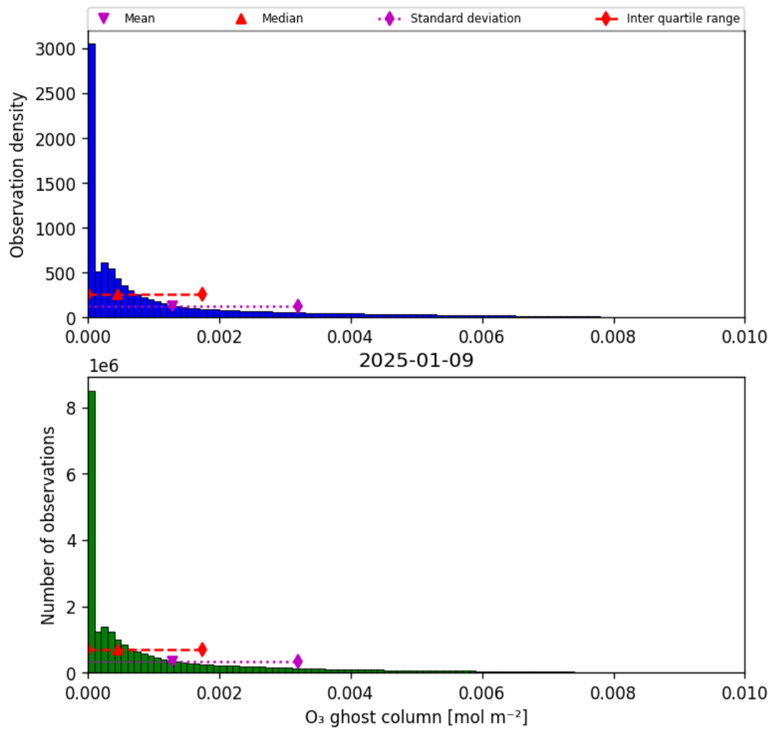
Figure 25: Histogram of “O 3 ghost column” for 2025-01-08 to 2025-01-10
