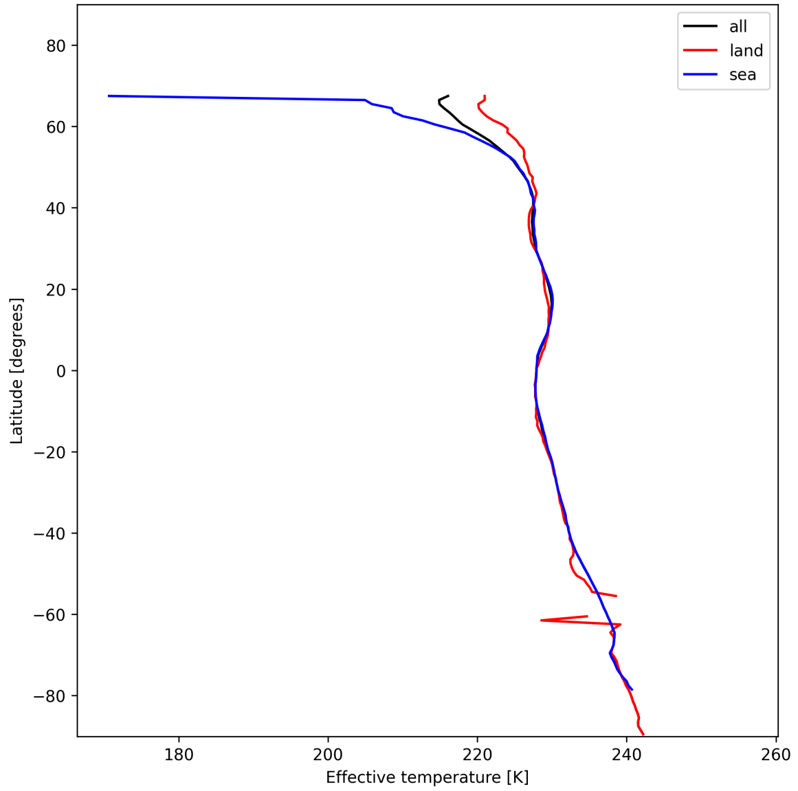
Figure 17: Zonal average of "Effective temperature" for 2025-01-08 to 2025-01-10.
