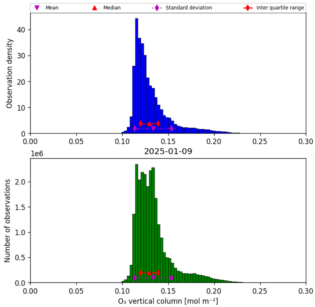
Figure 21: Histogram of “O 3 vertical column” for 2025-01-08 to 2025-01-10
