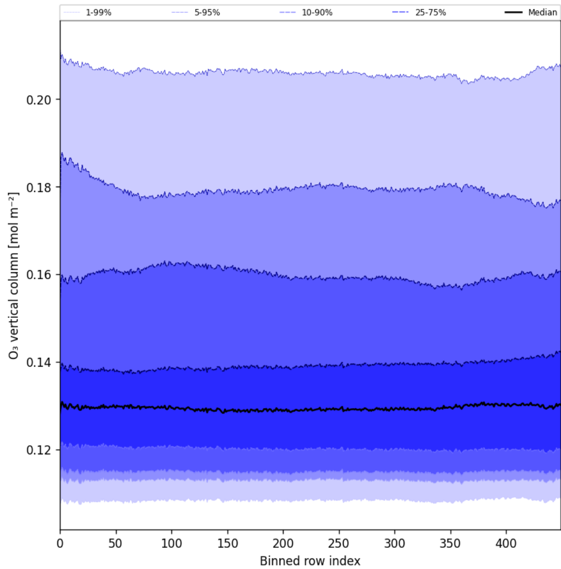
Figure 28: Along track statistics of “O 3 vertical column” for 2025-01-08 to 2025-01-10
