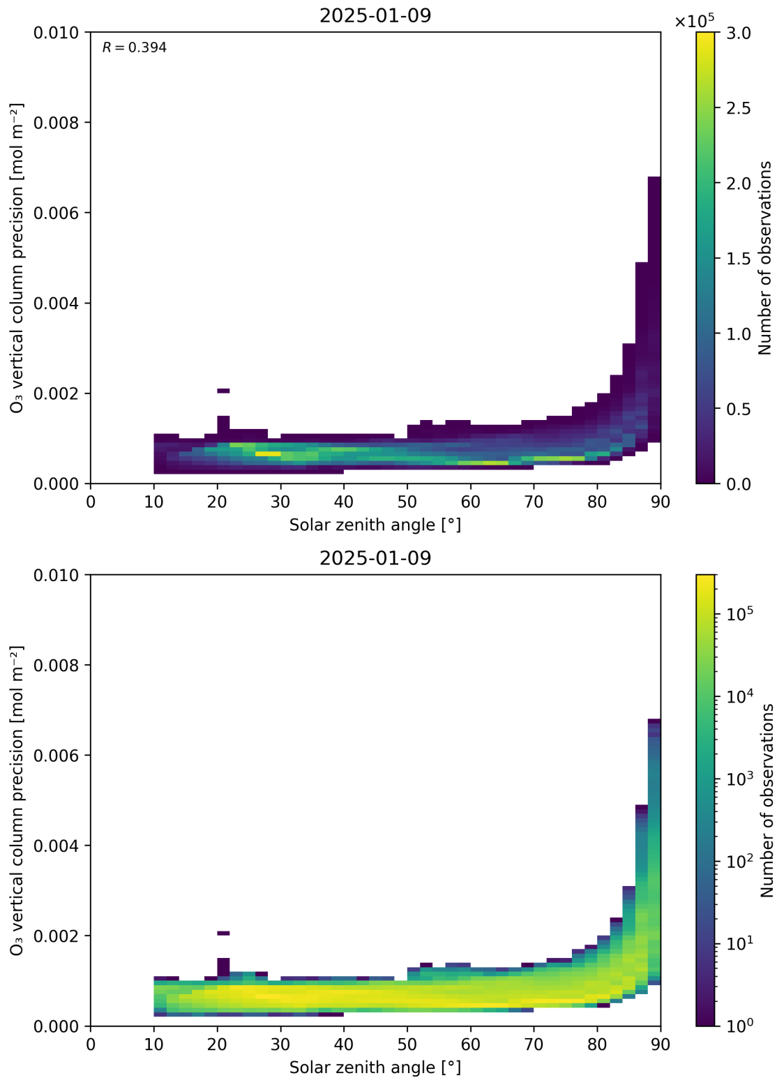
Figure 48: Scatter density plot of “Solar zenith angle” against “O 3 vertical column precision” for 2025-01-08 to 2025-01-10.
