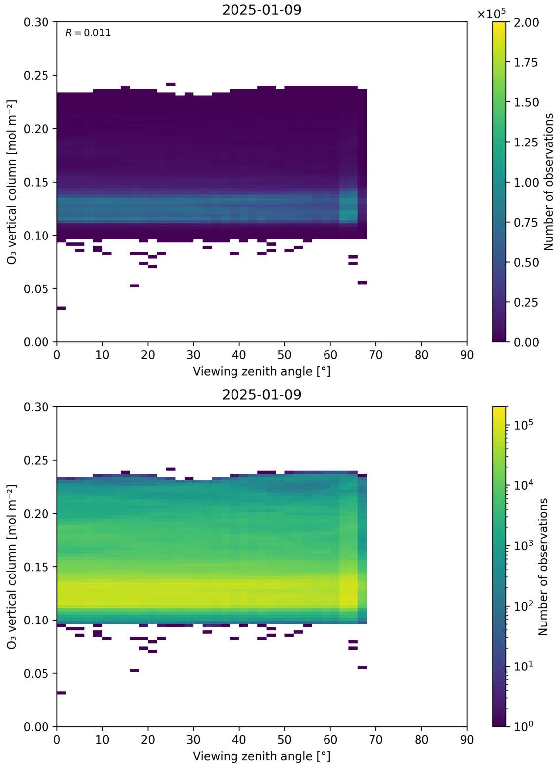
Figure 52: Scatter density plot of “Viewing zenith angle” against “O 3 vertical column” for 2025-01-08 to 2025-01-10.
