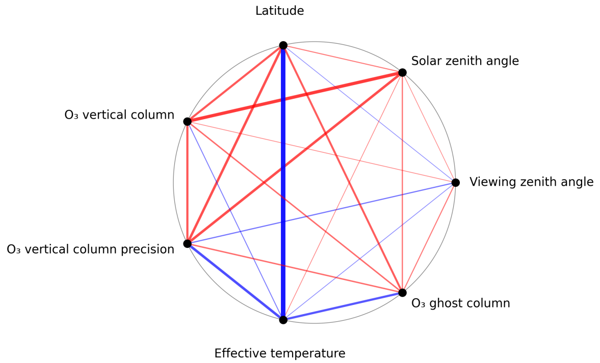
Figure 1: Map of correlation graph for 2025-01-08 to 2025-01-10.
