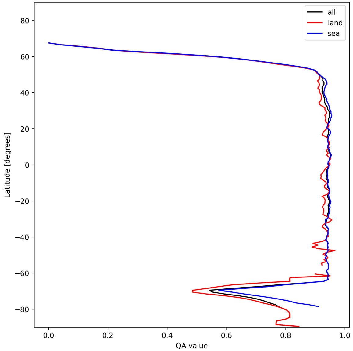
Figure 13: Zonal average of “QA value” for 2025-01-08 to 2025-01-10.
