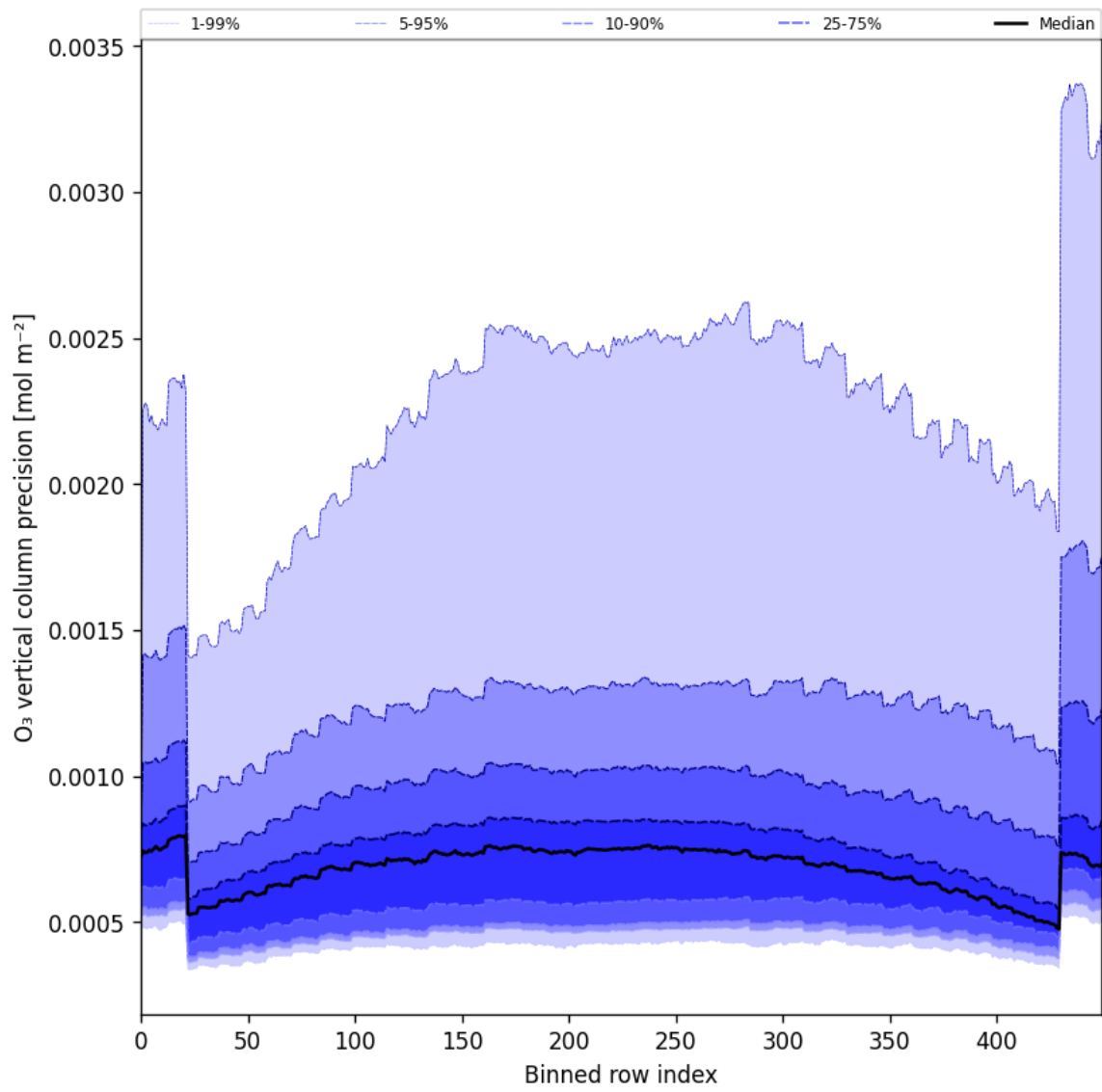
Figure 29: Along track statistics of “O 3 vertical column precision” for 2025-01-08 to 2025-01-10
