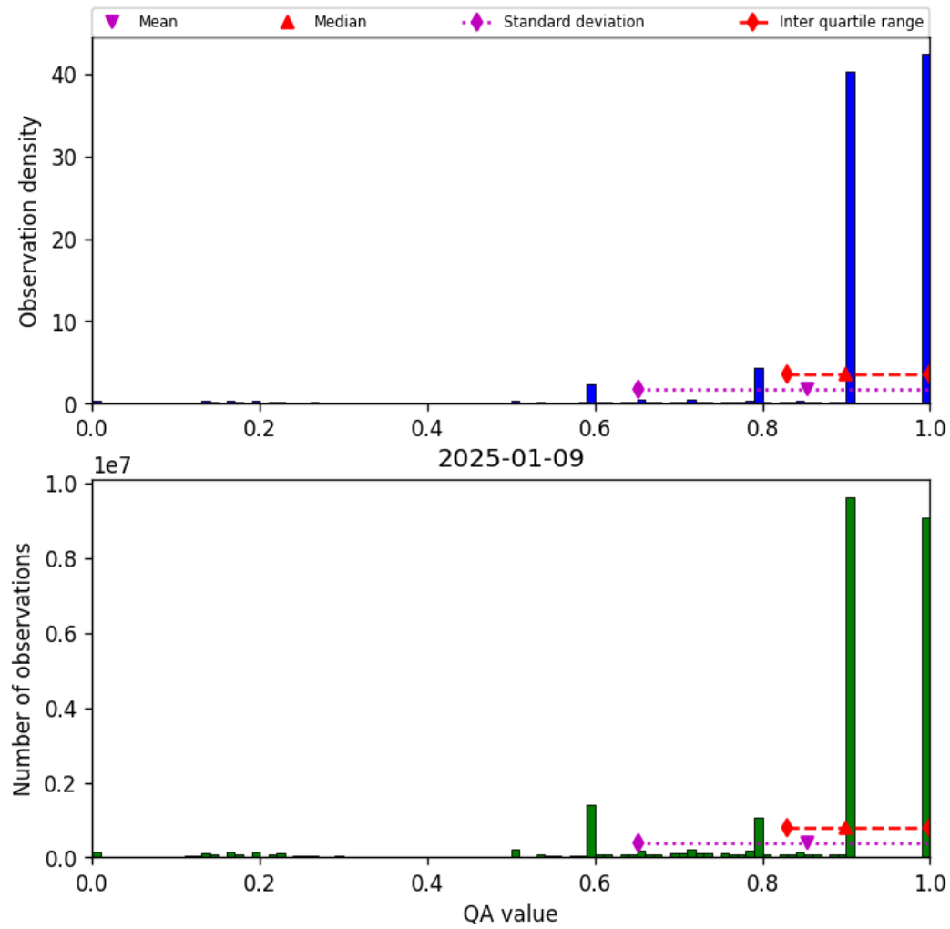
Figure 20: Histogram of “QA value” for 2025-01-08 to 2025-01-10
