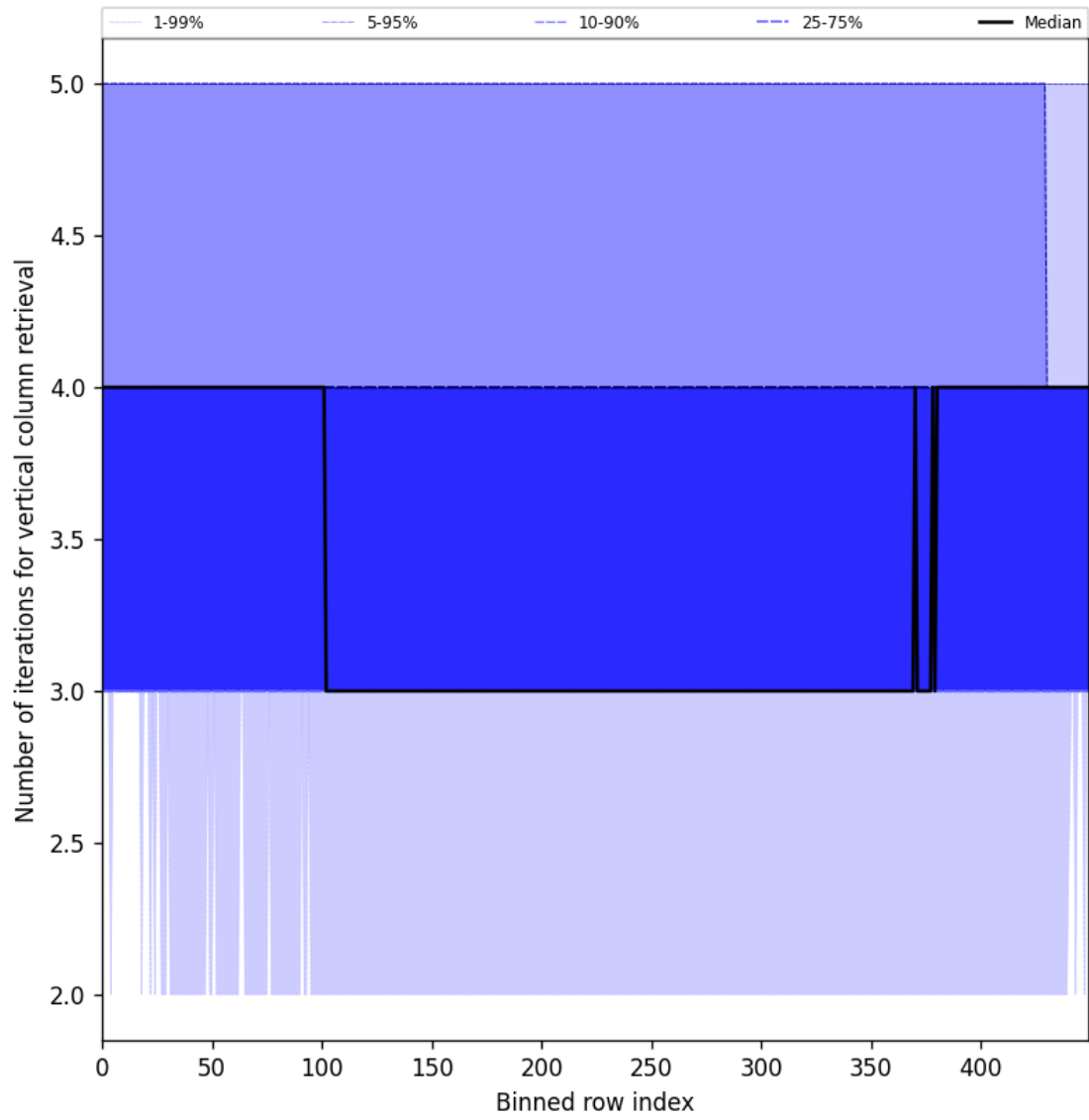
Figure 33: Along track statistics of “Number of iterations for vertical column retrieval” for 2025-01-08 to 2025-01-10
