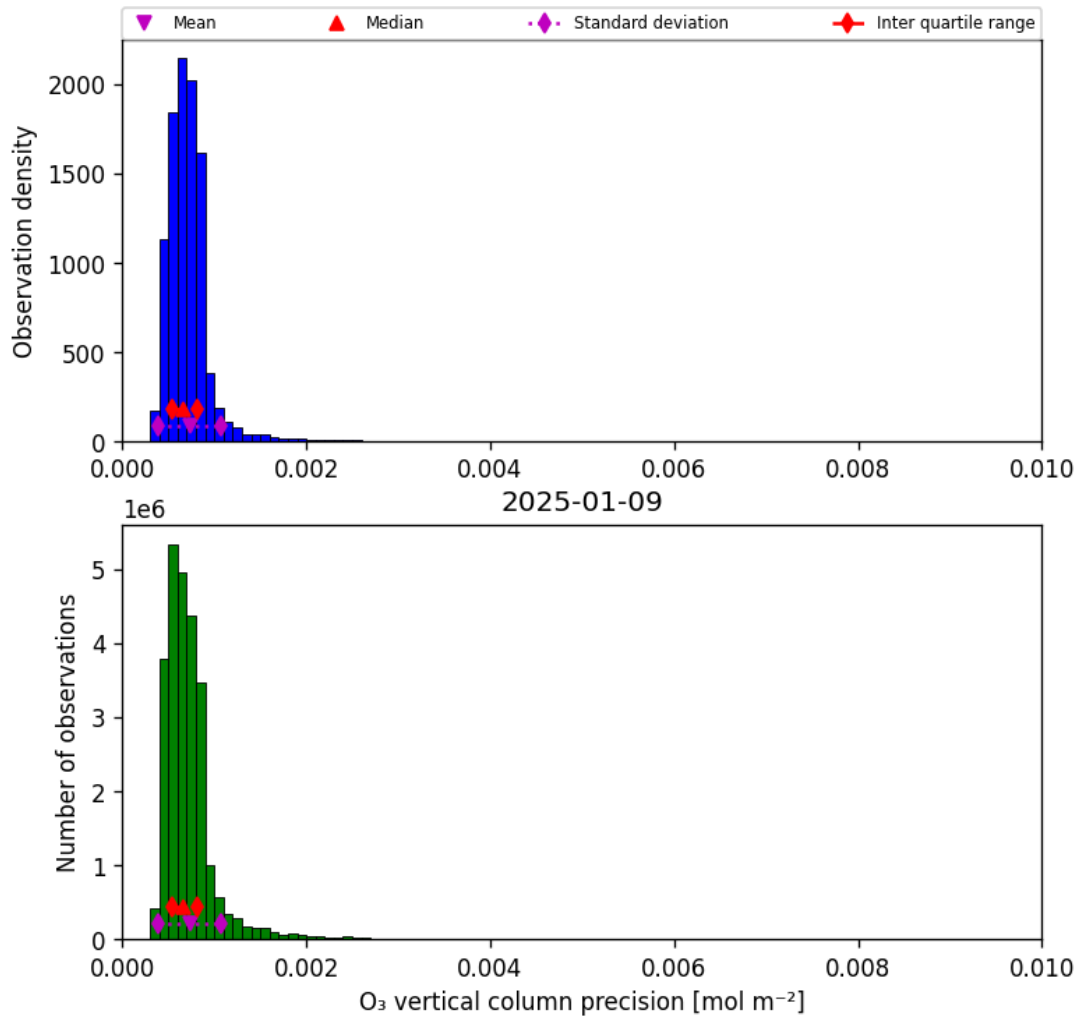
Figure 22: Histogram of “O 3 vertical column precision” for 2025-01-08 to 2025-01-10
