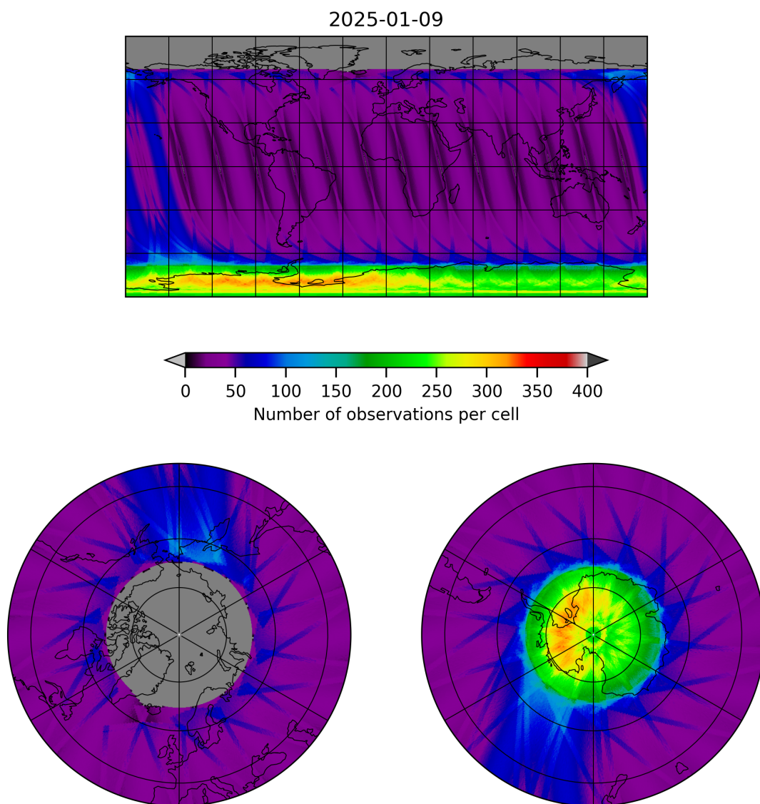
Figure 12: Map of the number of observations for 2025-01-08 to 2025-01-10
