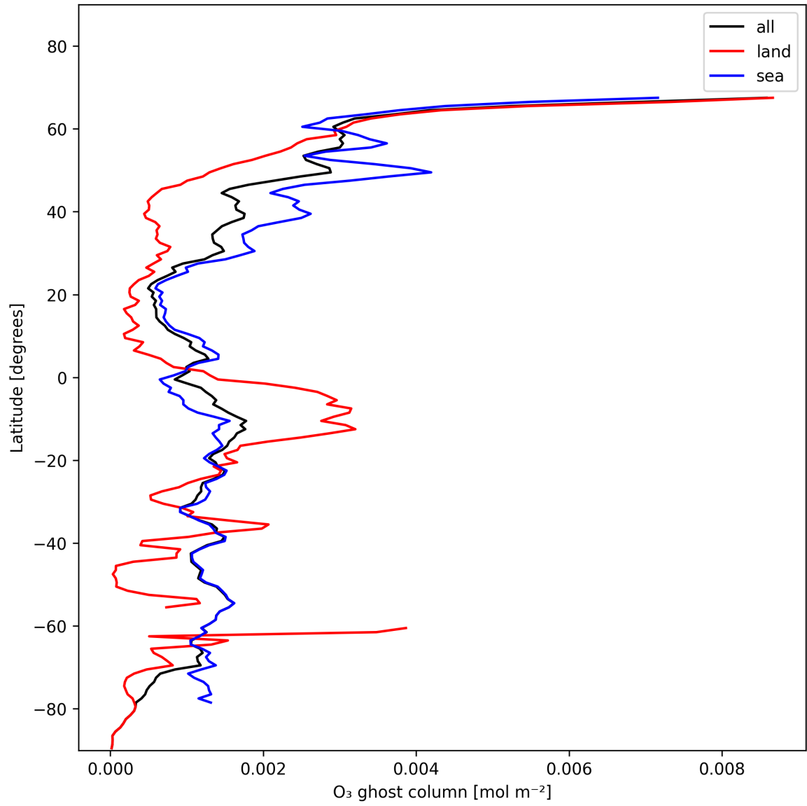
Figure 18: Zonal average of “O 3 ghost column” for 2025-01-08 to 2025-01-10.
