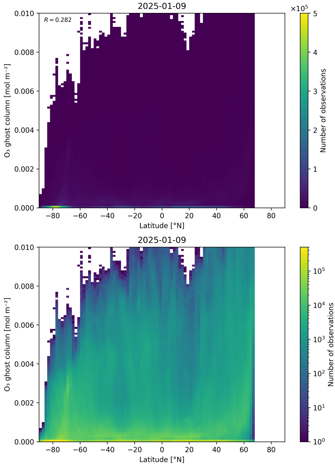
Figure 35: Scatter density plot of “Latitude” against “O 3 ghost column” for 2025-01-08 to 2025-01-10.
