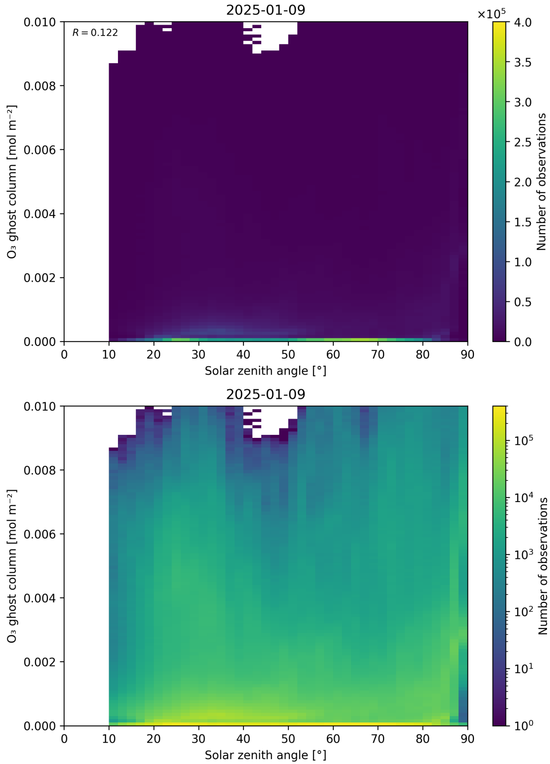
Figure 46: Scatter density plot of “Solar zenith angle” against “O 3 ghost column” for 2025-01-08 to 2025-01-10.
