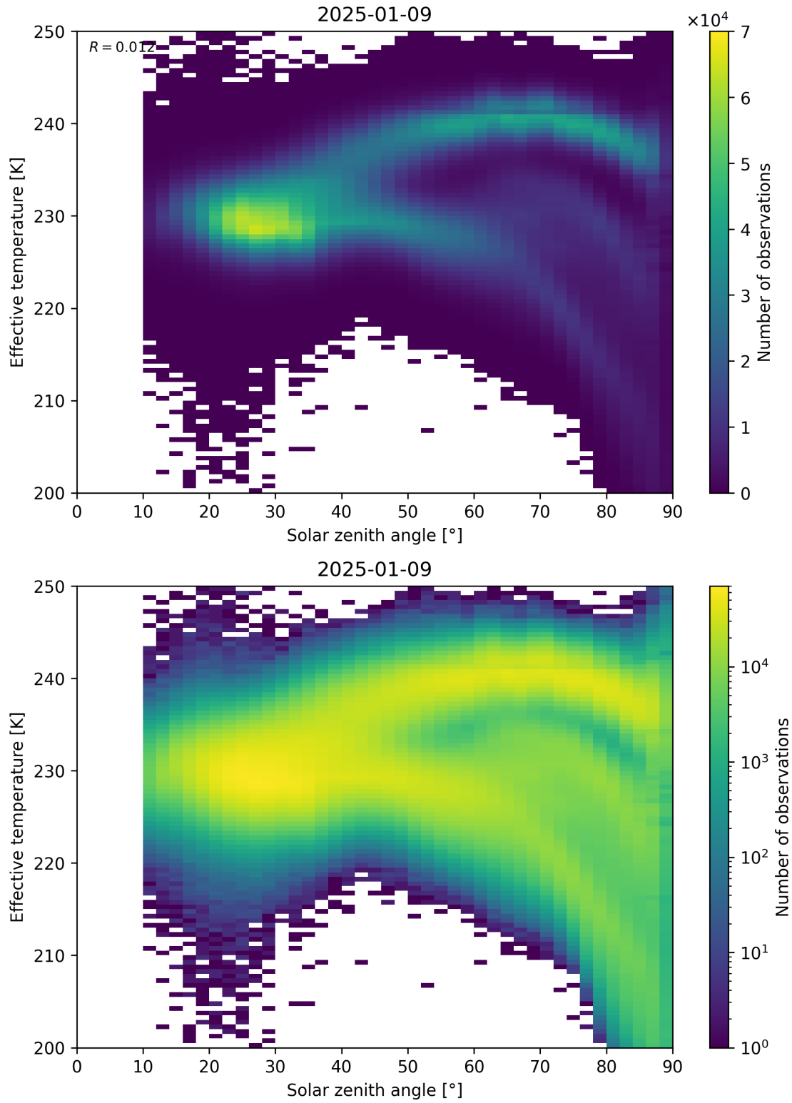
Figure 45: Scatter density plot of “Solar zenith angle” against “Effective temperature” for 2025-01-08 to 2025-01-10.
