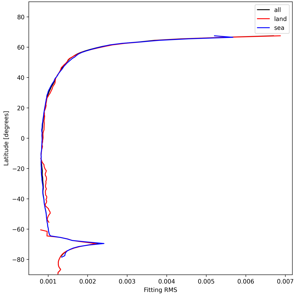
Figure 16: Zonal average of “Fitting RMS” for 2025-01-08 to 2025-01-10.
