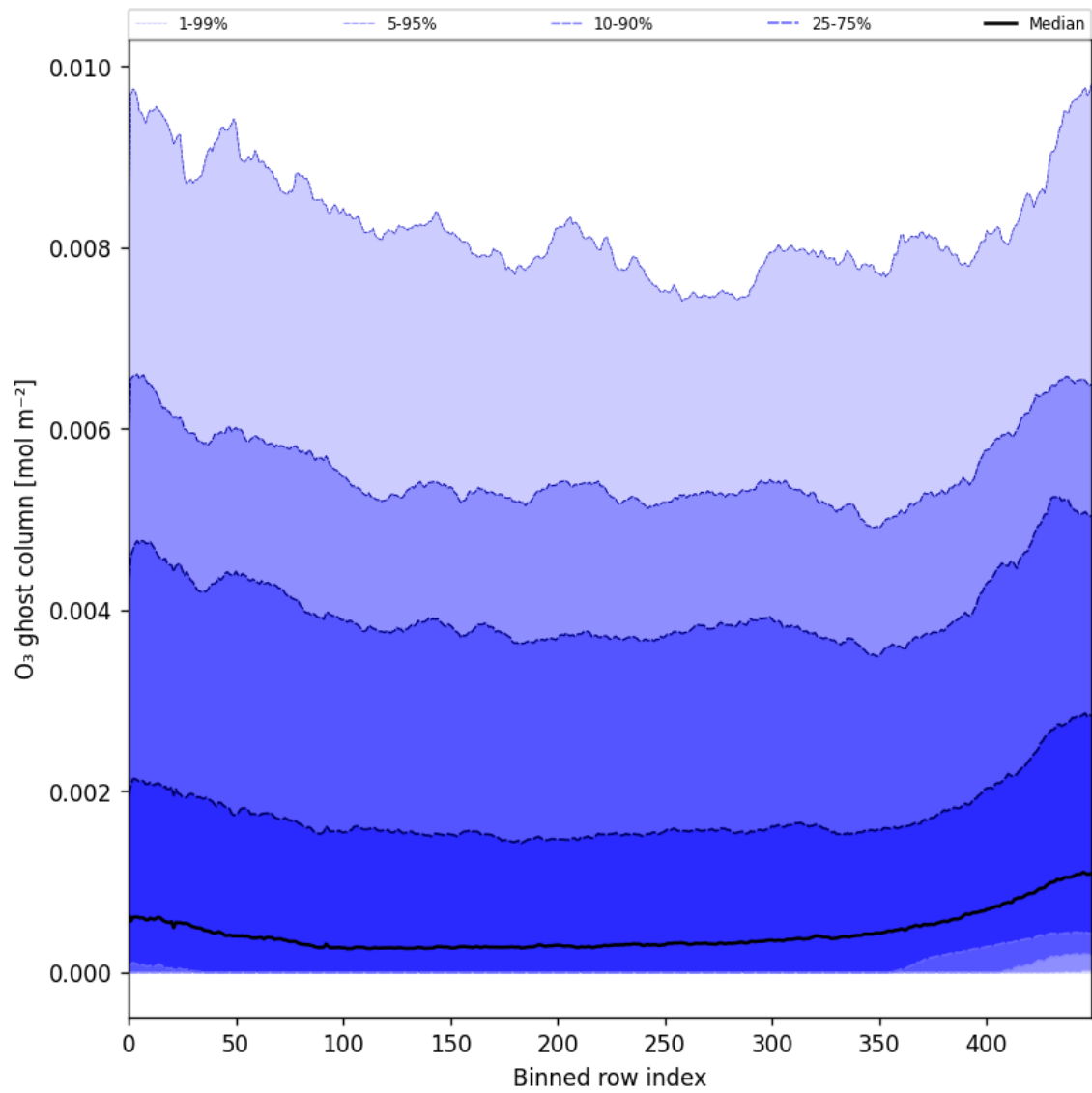
Figure 32: Along track statistics of “O 3 ghost column” for 2025-01-08 to 2025-01-10
