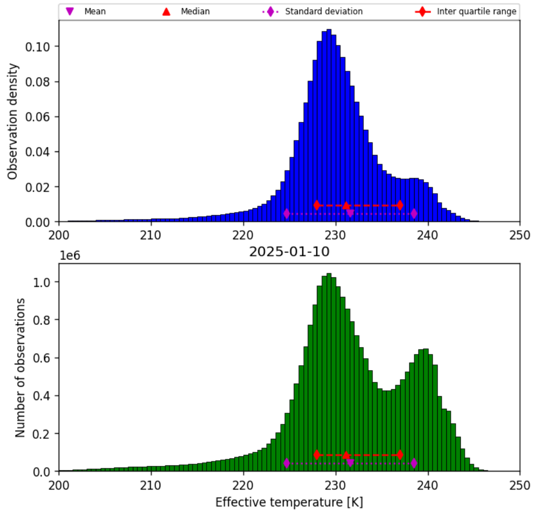
Figure 24: Histogram of “Effective temperature” for 2025-01-09 to 2025-01-11
