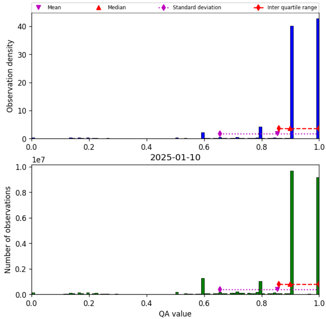
Figure 20: Histogram of “QA value” for 2025-01-09 to 2025-01-11
