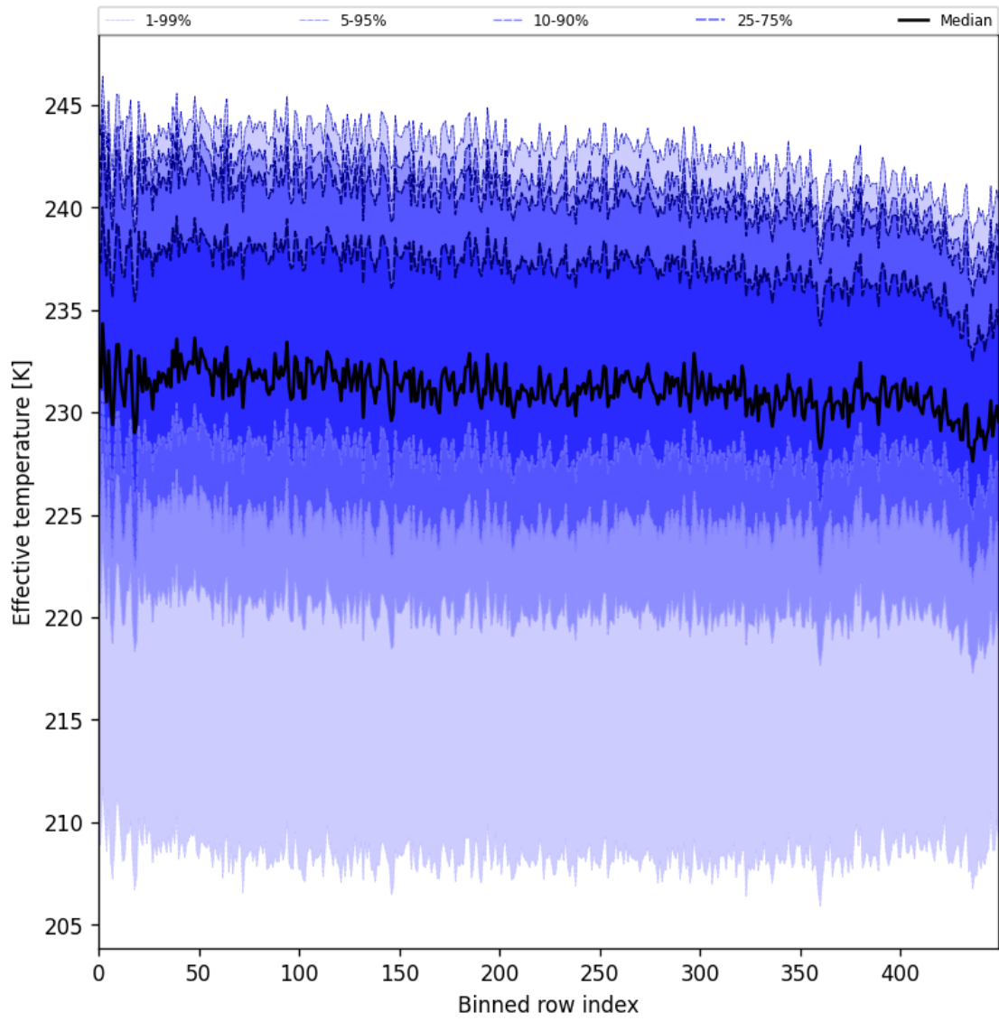
Figure 31: Along track statistics of “Effective temperature” for 2025-01-09 to 2025-01-11
