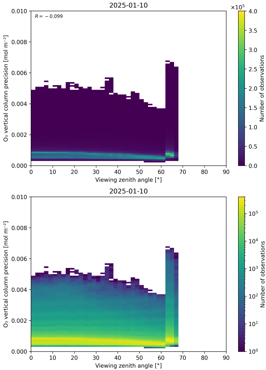
Figure 53: Scatter density plot of “Viewing zenith angle” against “O 3 vertical column precision” for 2025-01-09 to 2025-01-11.
