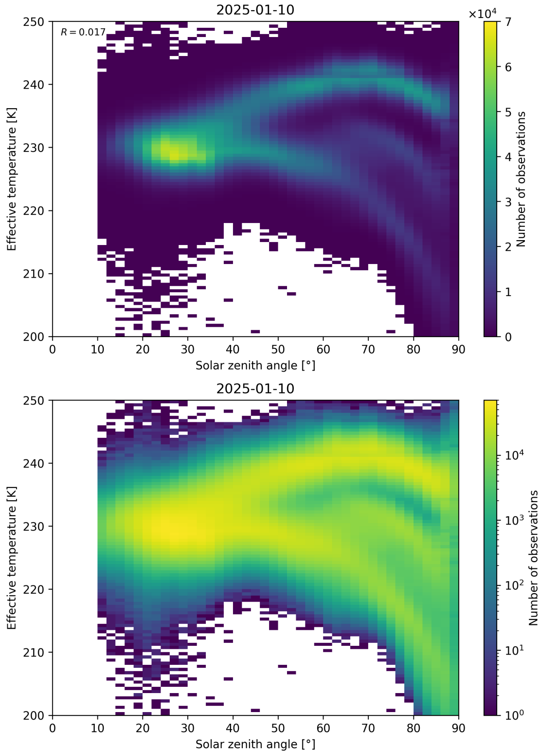
Figure 45: Scatter density plot of “Solar zenith angle” against “Effective temperature” for 2025-01-09 to 2025-01-11.
