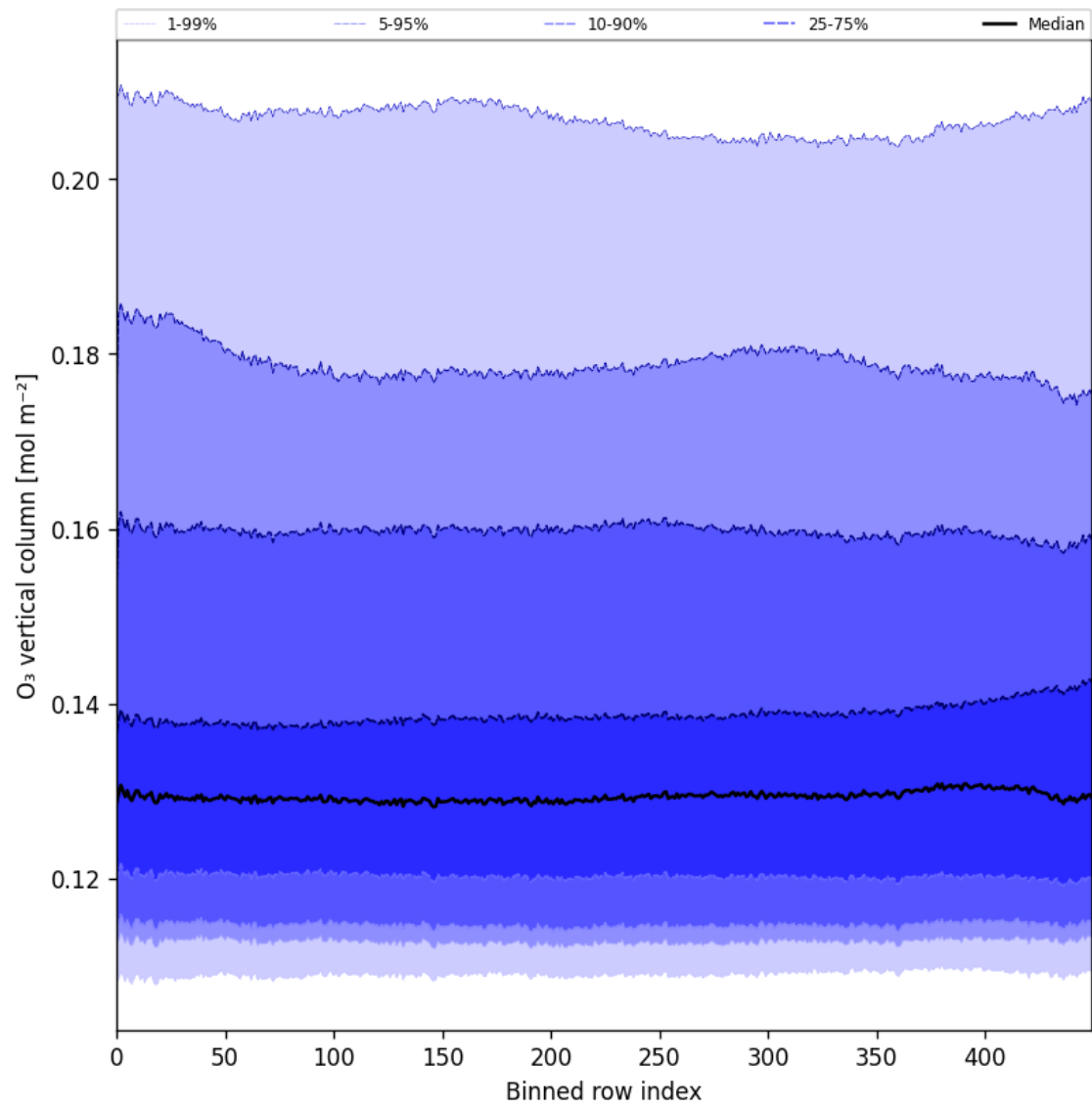
Figure 28: Along track statistics of “O 3 vertical column” for 2025-01-09 to 2025-01-11
