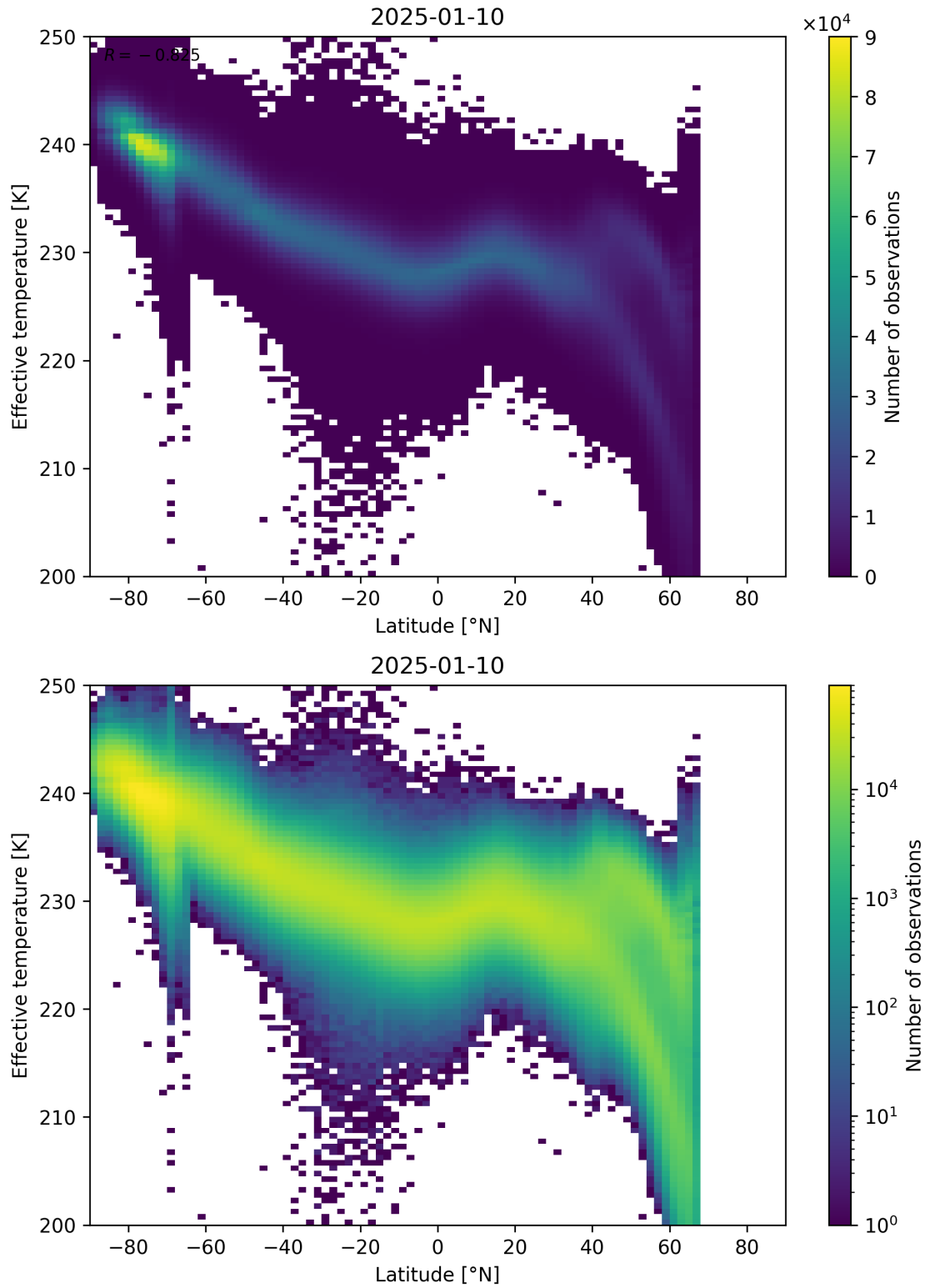
Figure 34: Scatter density plot of “Latitude” against “Effective temperature” for 2025-01-09 to 2025-01-11.
