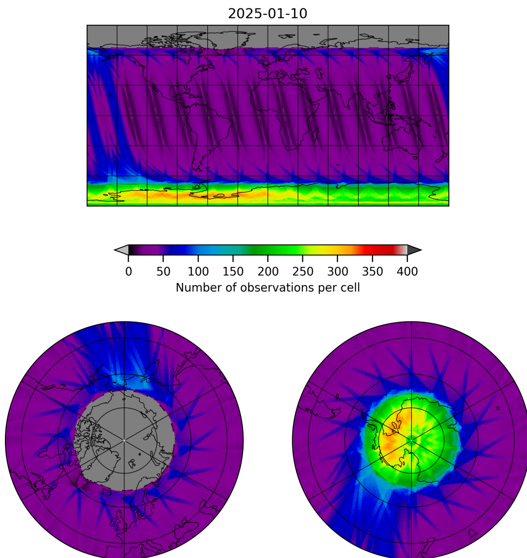
Figure 12: Map of the number of observations for 2025-01-09 to 2025-01-11
