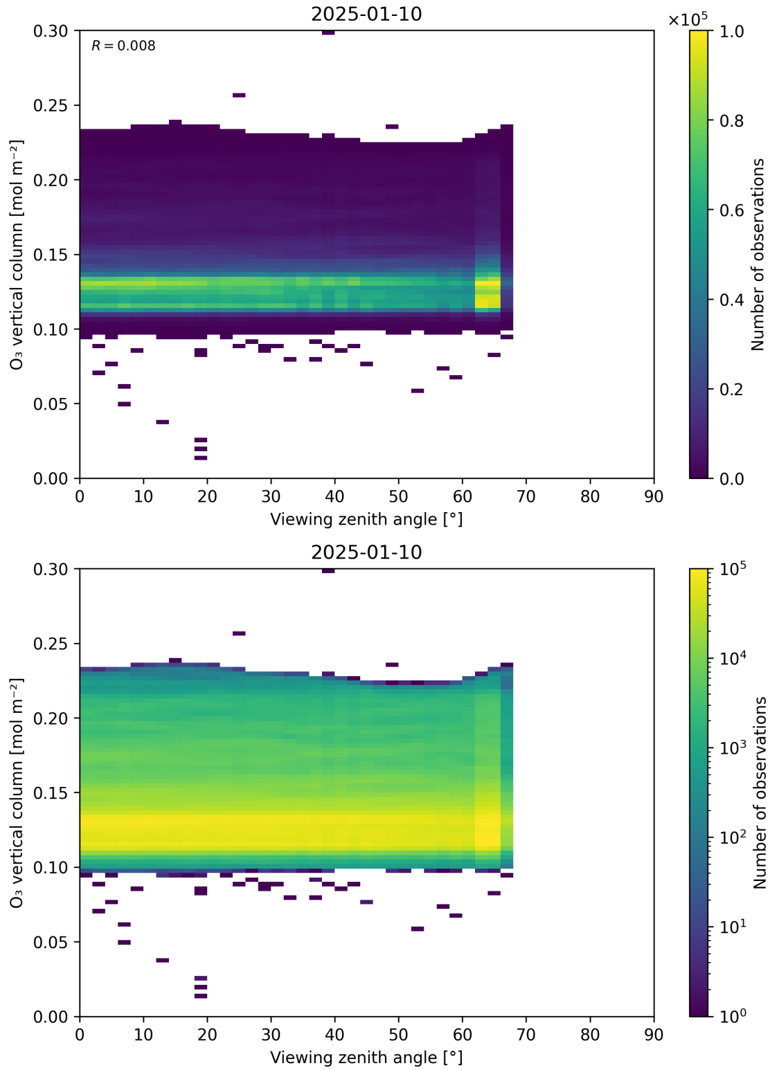
Figure 52: Scatter density plot of “Viewing zenith angle” against “O 3 vertical column” for 2025-01-09 to 2025-01-11.
