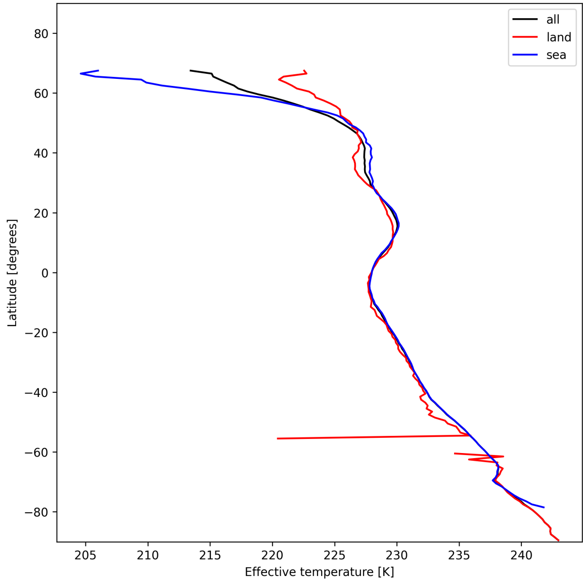
Figure 17: Zonal average of “Effective temperature” for 2025-01-09 to 2025-01-11.
