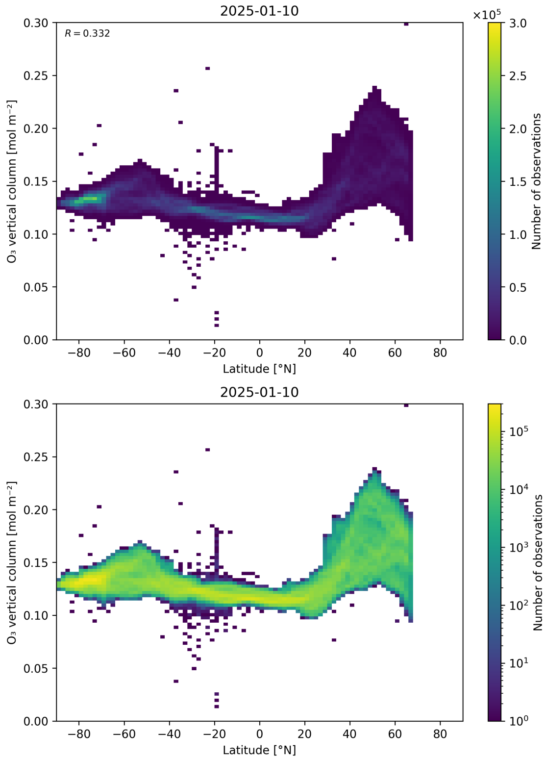
Figure 36: Scatter density plot of “Latitude” against “O 3 vertical column” for 2025-01-09 to 2025-01-11.
