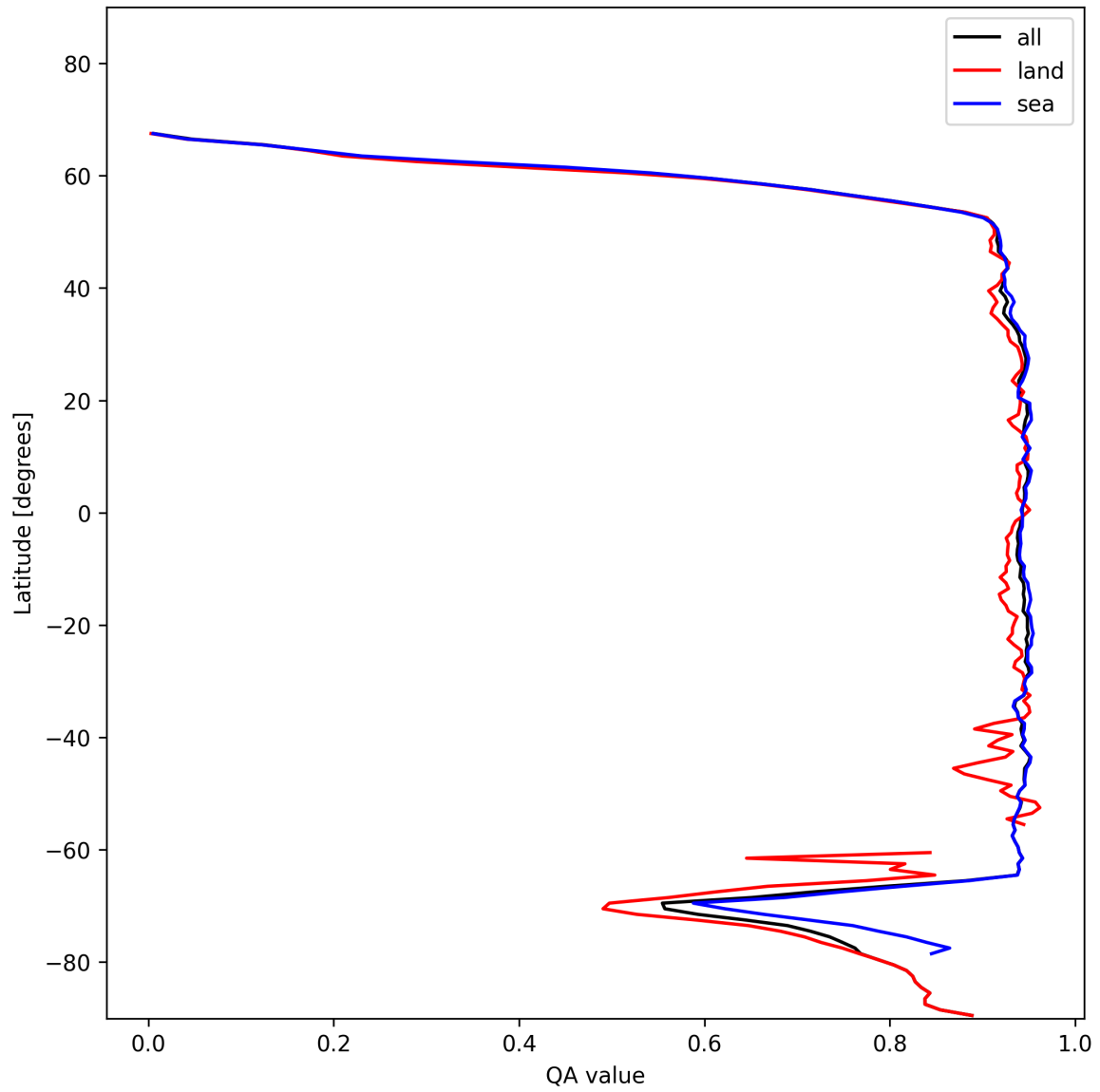
Figure 13: Zonal average of "QA value" for 2025-01-09 to 2025-01-11.
