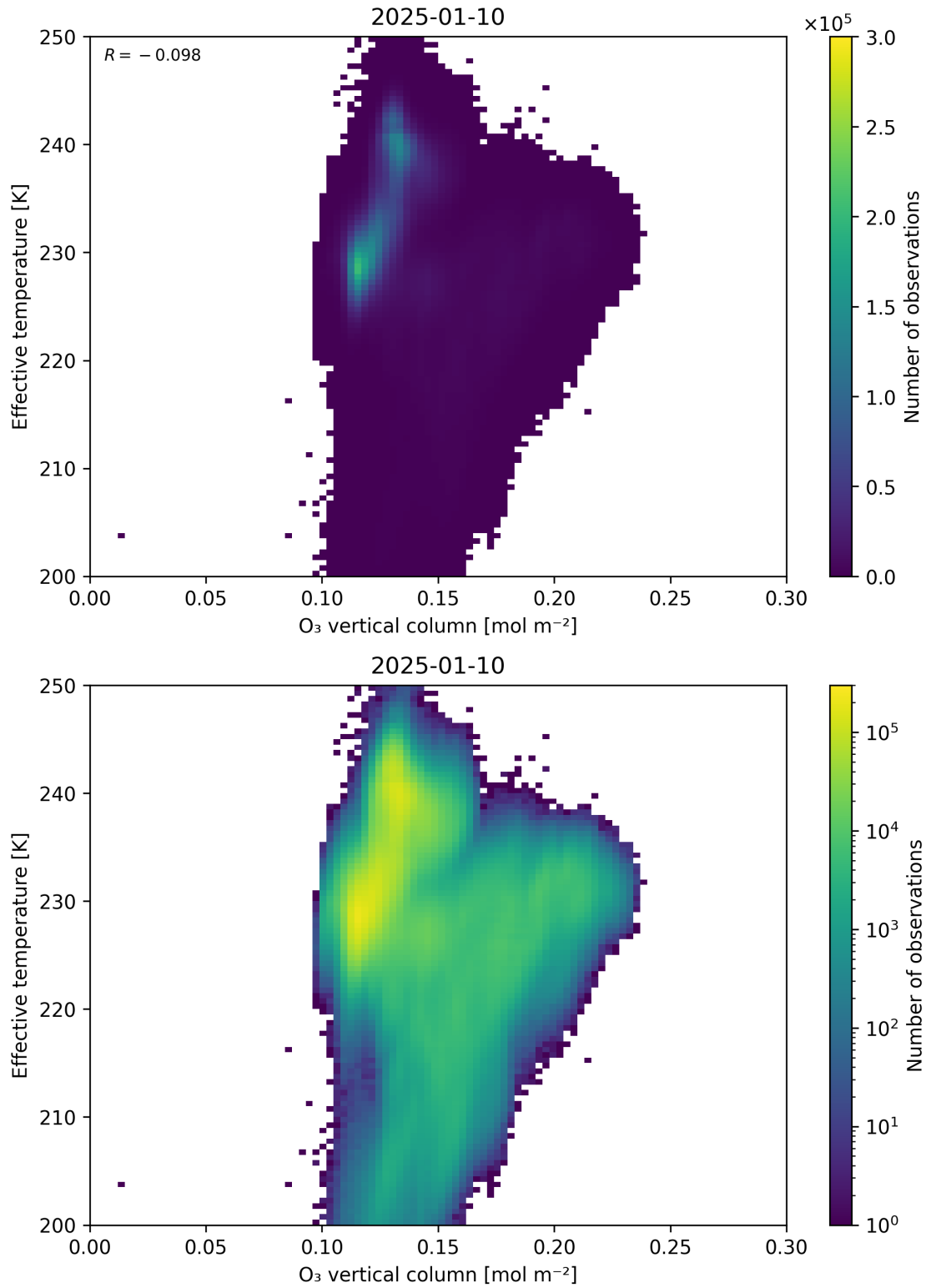
Figure 39: Scatter density plot of “O 3 vertical column” against “Effective temperature” for 2025-01-09 to 2025-01-11.
