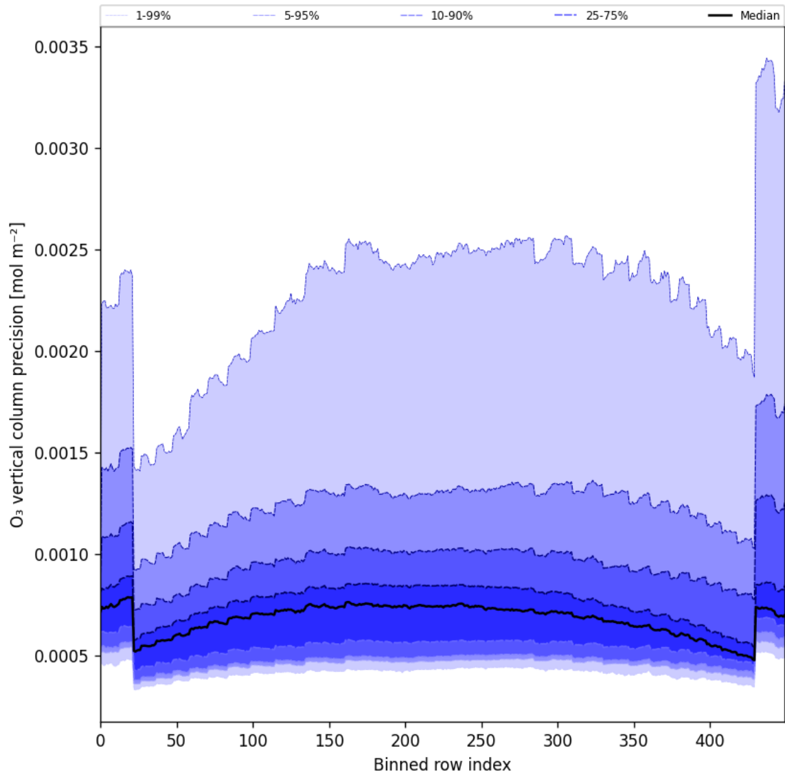
Figure 29: Along track statistics of “O 3 vertical column precision” for 2025-01-09 to 2025-01-11
