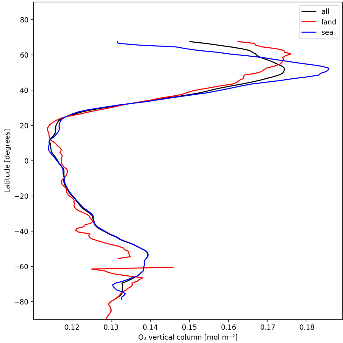
Figure 14: Zonal average of “O 3 vertical column” for 2025-01-09 to 2025-01-11.
