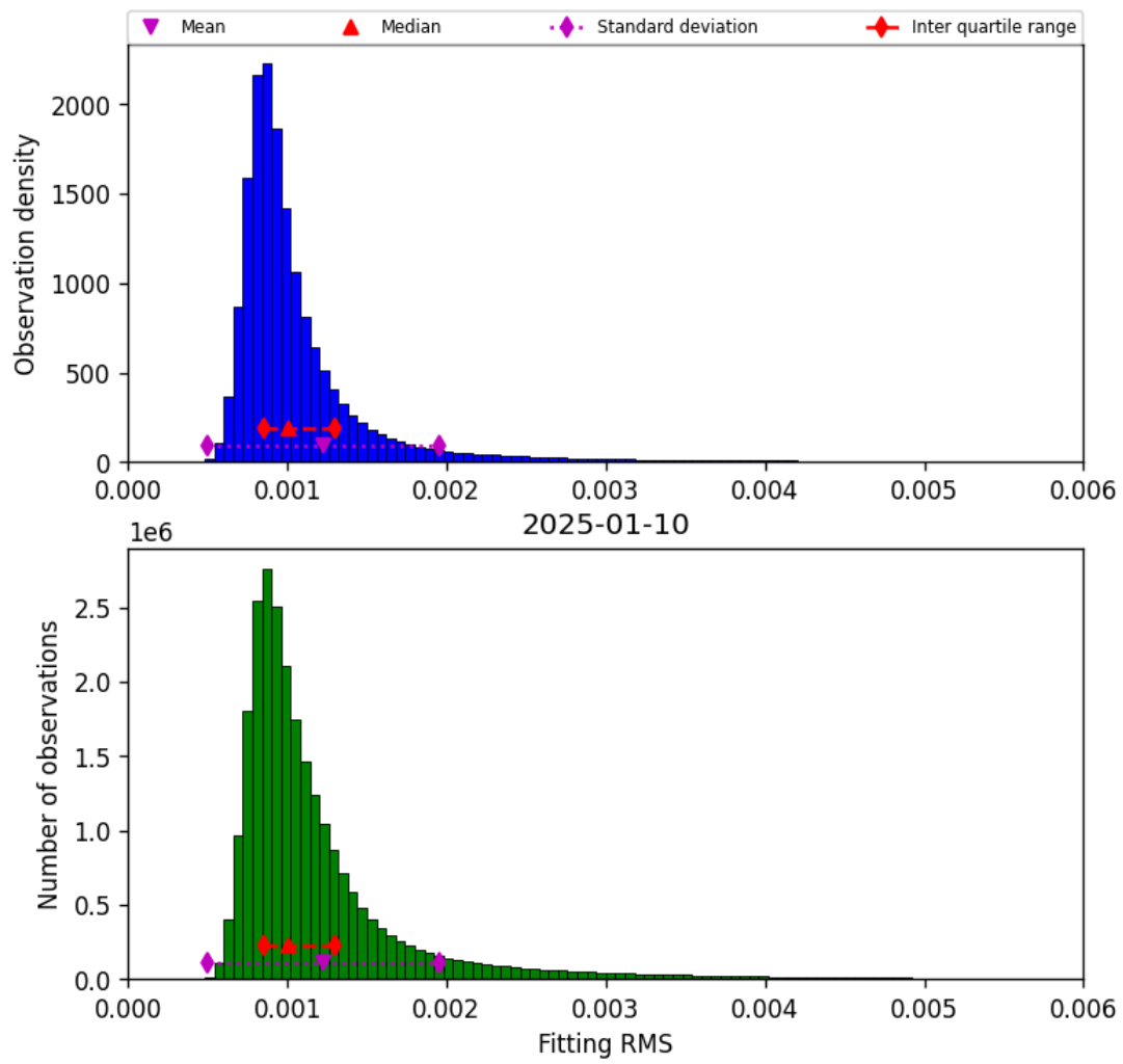
Figure 23: Histogram of “Fitting RMS” for 2025-01-09 to 2025-01-11
