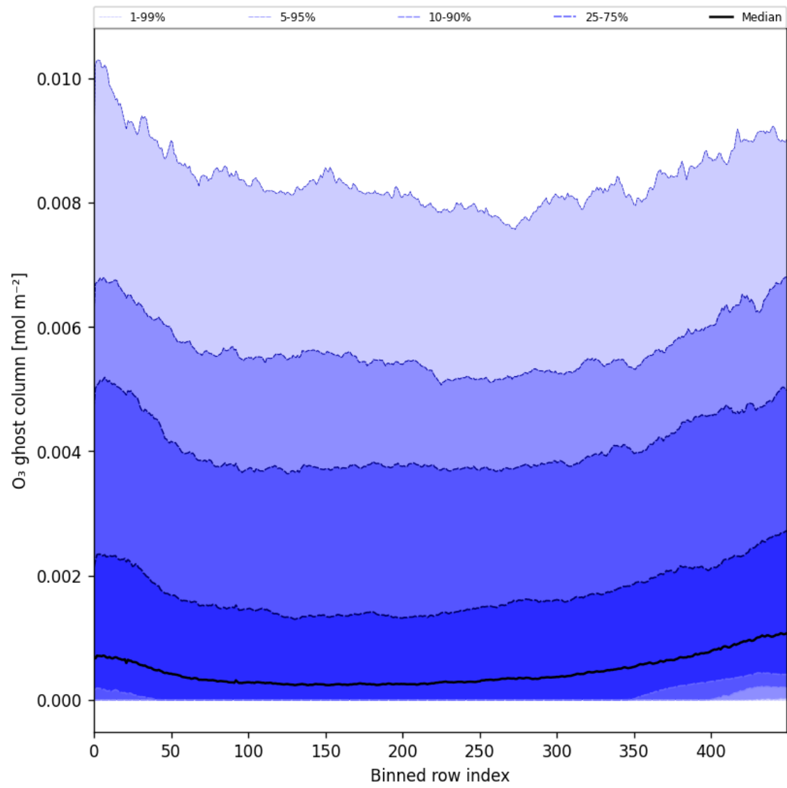
Figure 32: Along track statistics of “O 3 ghost column” for 2025-01-09 to 2025-01-11
