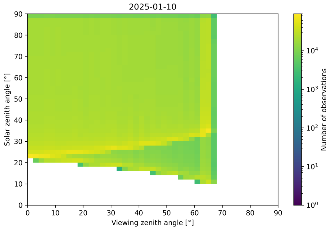
Figure 54: Scatter density plot of “Viewing zenith angle” against “Solar zenith angle” for 2025-01-09 to 2025-01-11.
