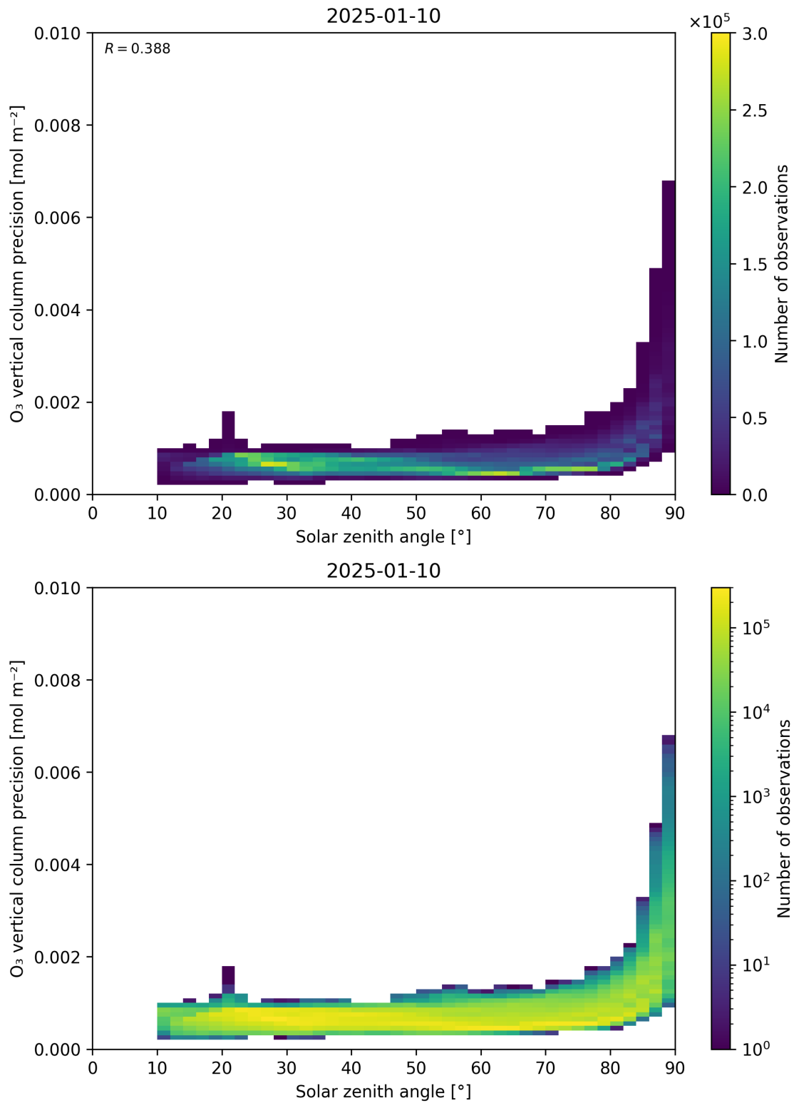
Figure 48: Scatter density plot of “Solar zenith angle” against “O 3 vertical column precision” for 2025-01-09 to 2025-01-11.
