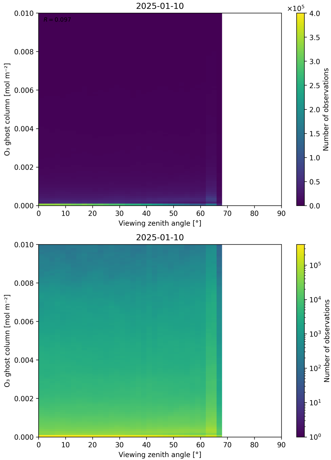
Figure 51: Scatter density plot of “Viewing zenith angle” against “O 3 ghost column” for 2025-01-09 to 2025-01-11.
