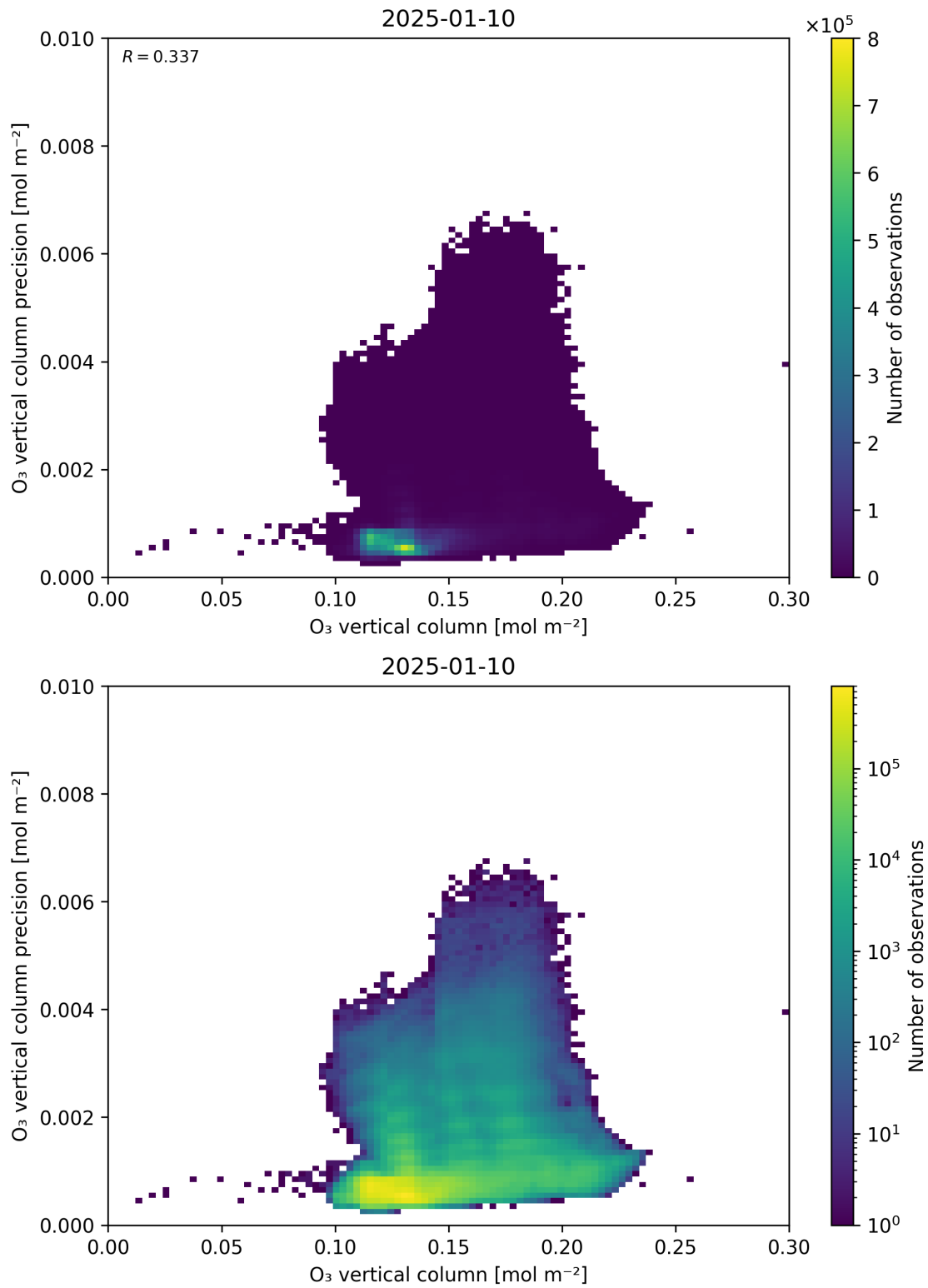
Figure 41: Scatter density plot of “O 3 vertical column” against “O 3 vertical column precision” for 2025-01-09 to 2025-01-11.
