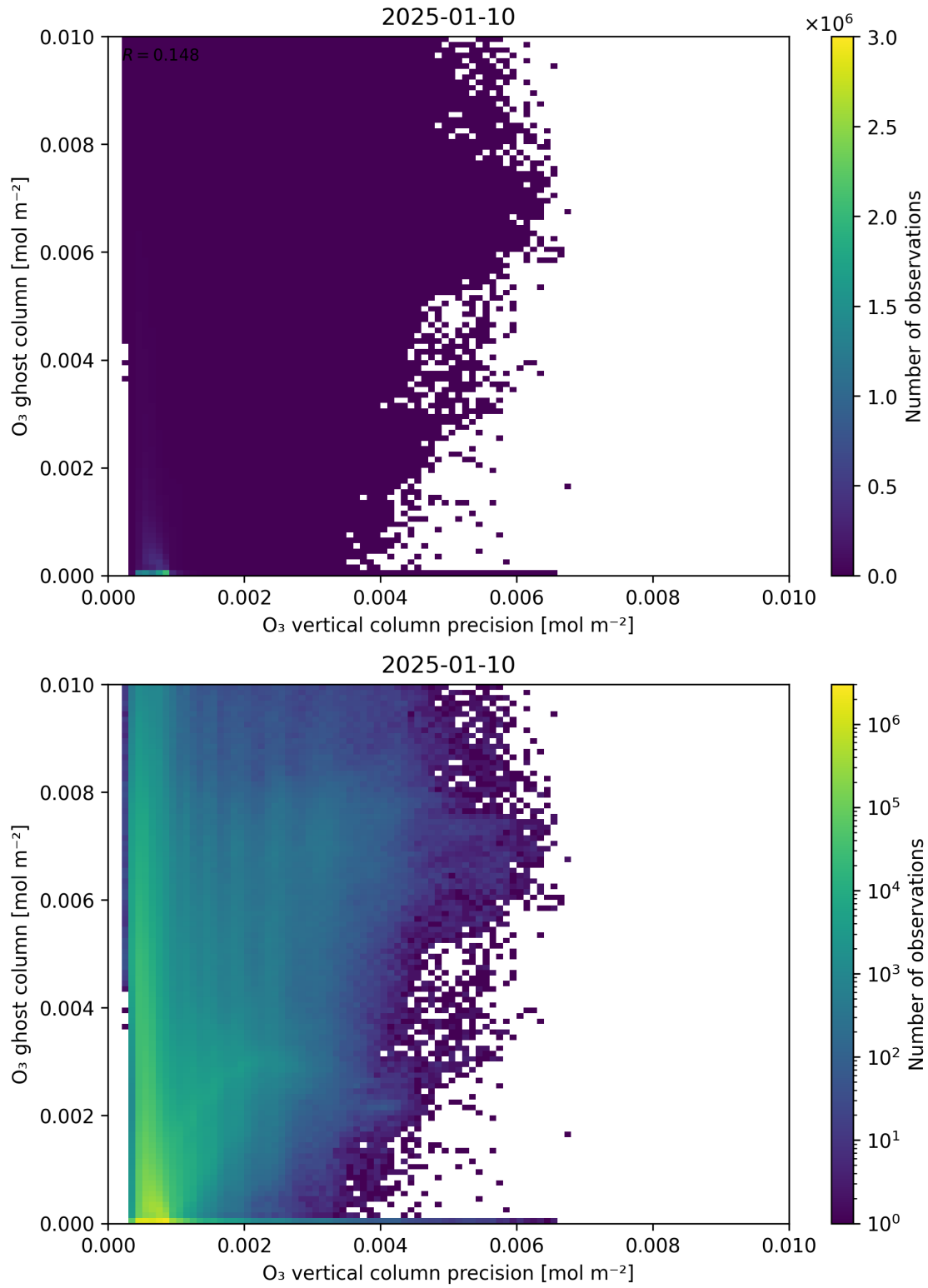
Figure 43: Scatter density plot of “O 3 vertical column precision” against “O 3 ghost column” for 2025-01-09 to 2025-01-11.
