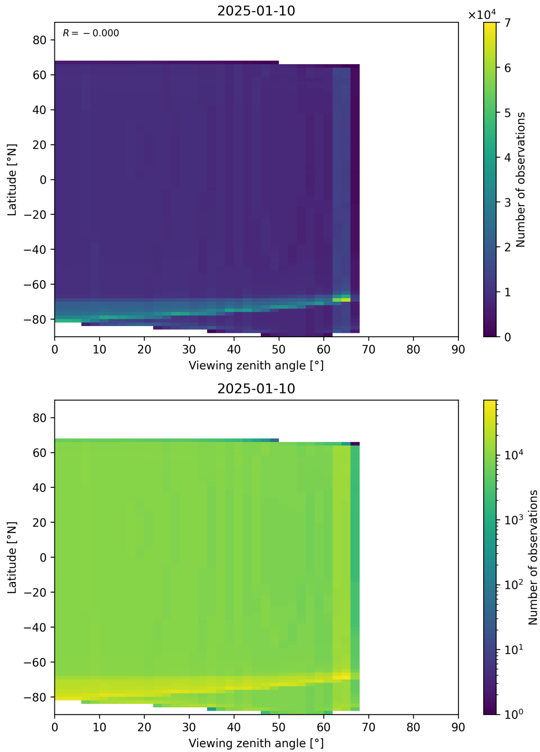
Figure 49: Scatter density plot of “Viewing zenith angle” against “Latitude” for 2025-01-09 to 2025-01-11.
