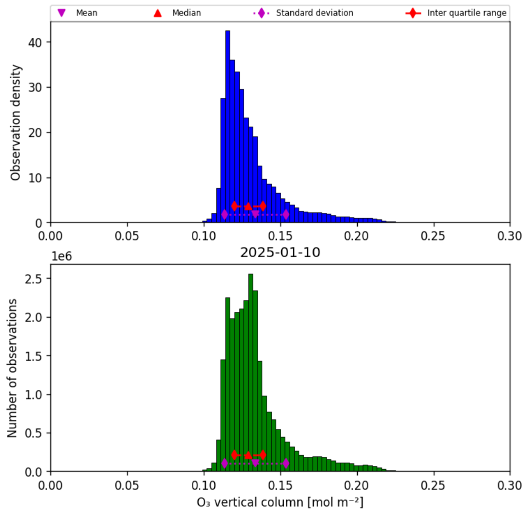
Figure 21: Histogram of “O 3 vertical column” for 2025-01-09 to 2025-01-11
