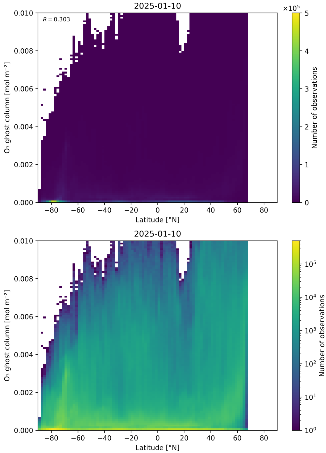
Figure 35: Scatter density plot of “Latitude” against “O 3 ghost column” for 2025-01-09 to 2025-01-11.
