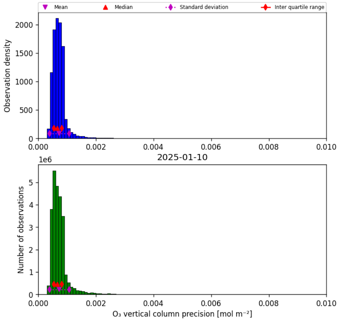
Figure 22: Histogram of “O 3 vertical column precision” for 2025-01-09 to 2025-01-11
