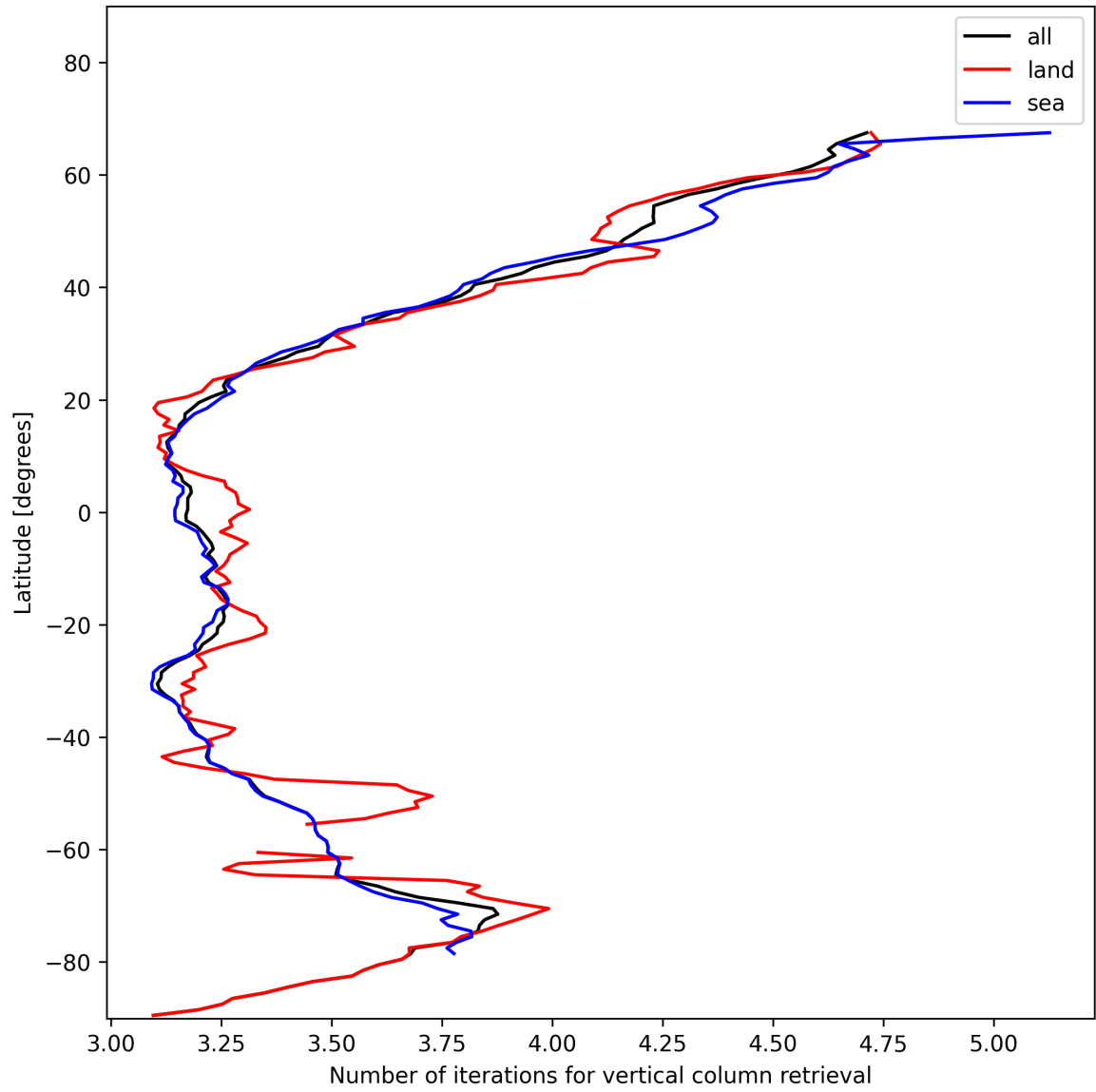
Figure 19: Zonal average of “Number of iterations for vertical column retrieval” for 2025-01-09 to 2025-01-11.
