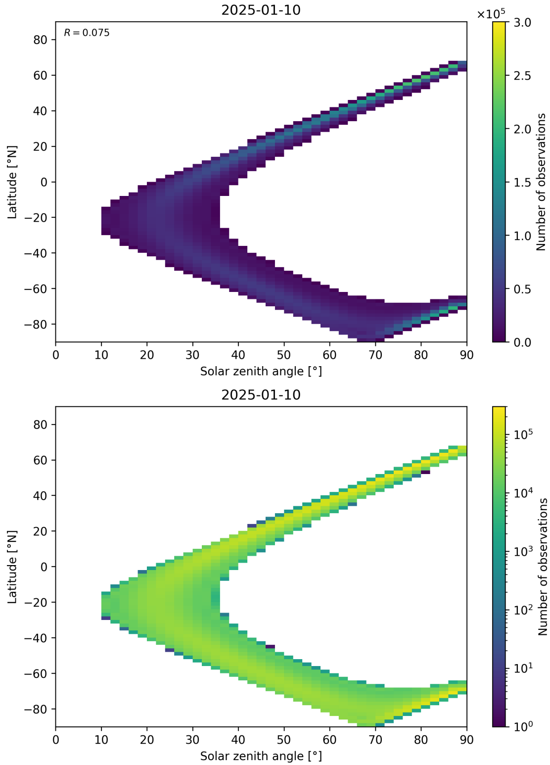
Figure 44: Scatter density plot of “Solar zenith angle” against “Latitude” for 2025-01-09 to 2025-01-11.
