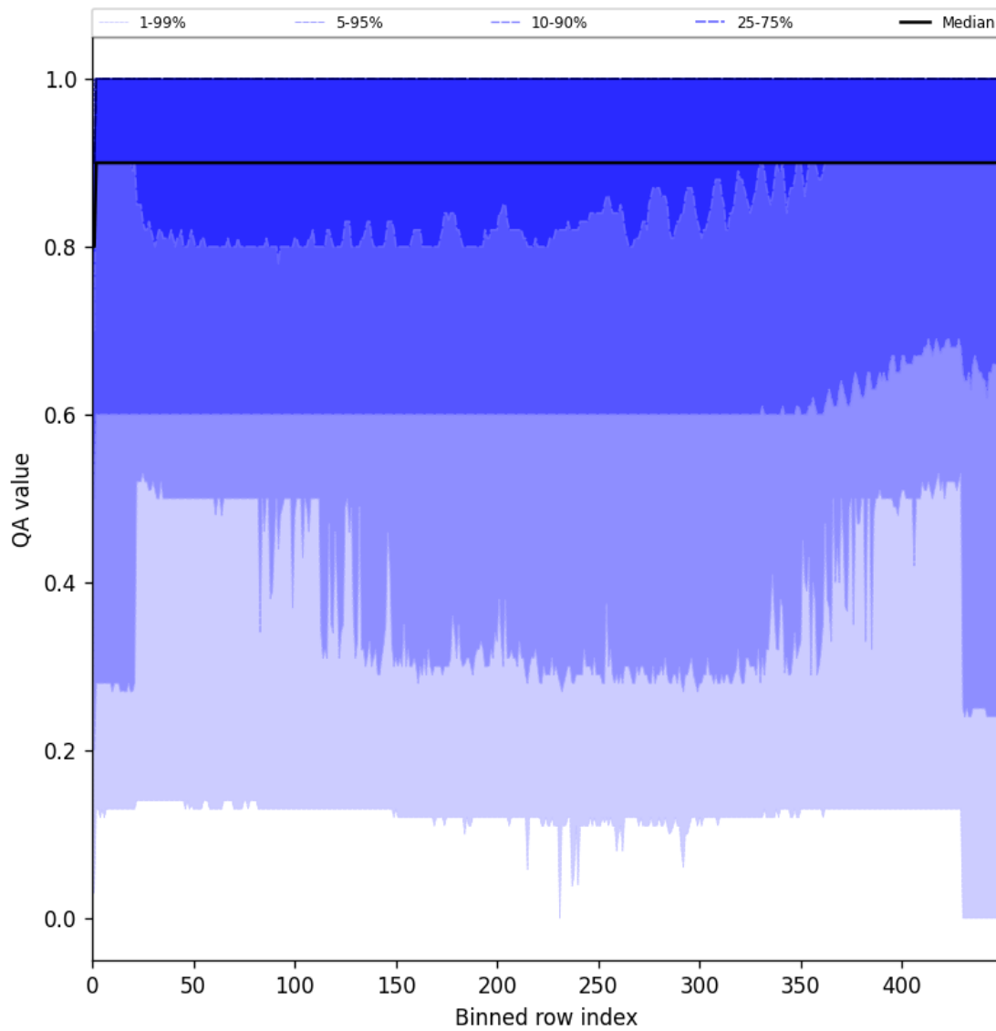
Figure 27: Along track statistics of “QA value” for 2025-01-09 to 2025-01-11
