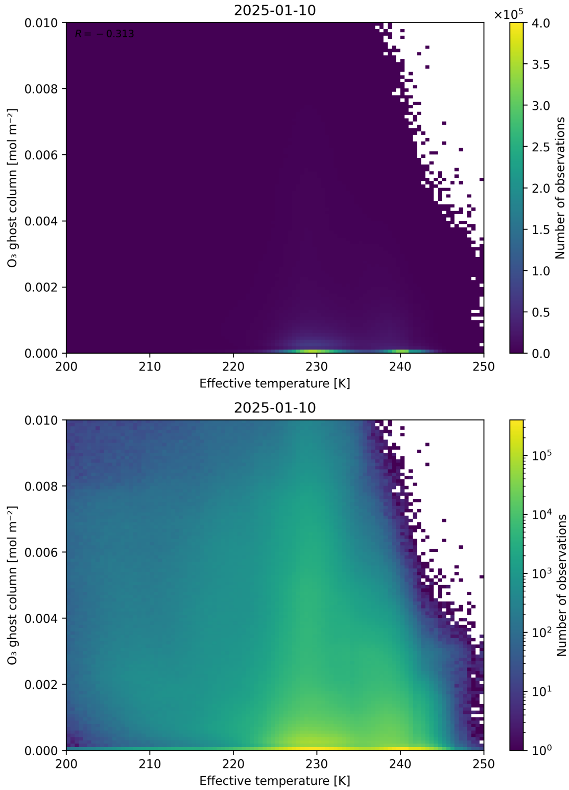
Figure 38: Scatter density plot of “Effective temperature” against “O 3 ghost column” for 2025-01-09 to 2025-01-11.
