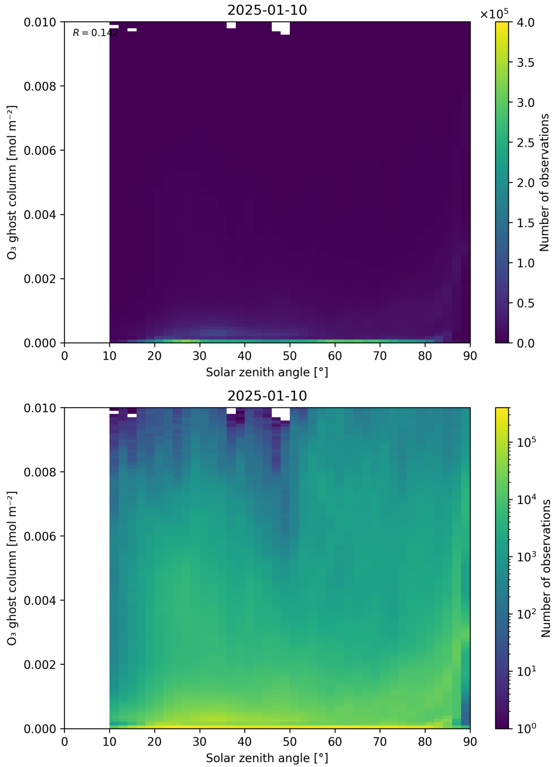
Figure 46: Scatter density plot of “Solar zenith angle” against “O 3 ghost column” for 2025-01-09 to 2025-01-11.
