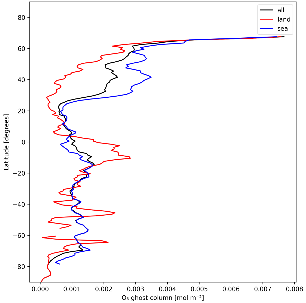
Figure 18: Zonal average of "O 3 ghost column" for 2025-01-09 to 2025-01-11.
