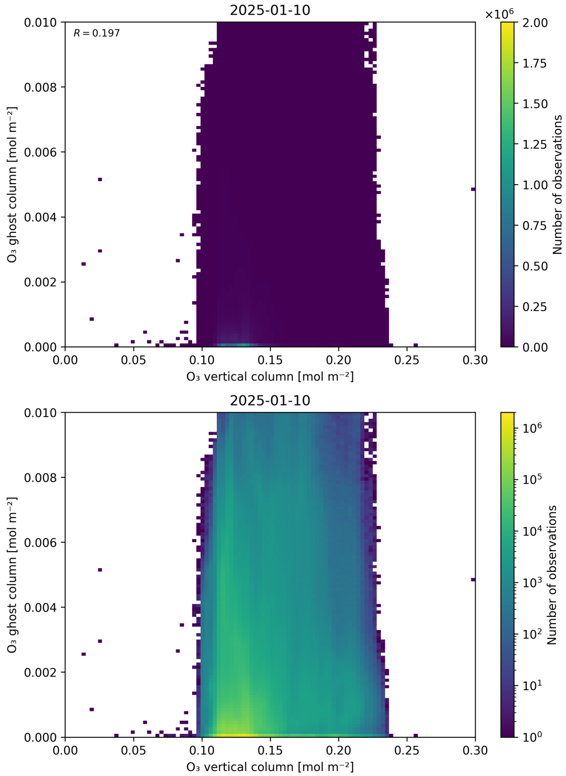
Figure 40: Scatter density plot of “O 3 vertical column” against “O 3 ghost column” for 2025-01-09 to 2025-01-11.
