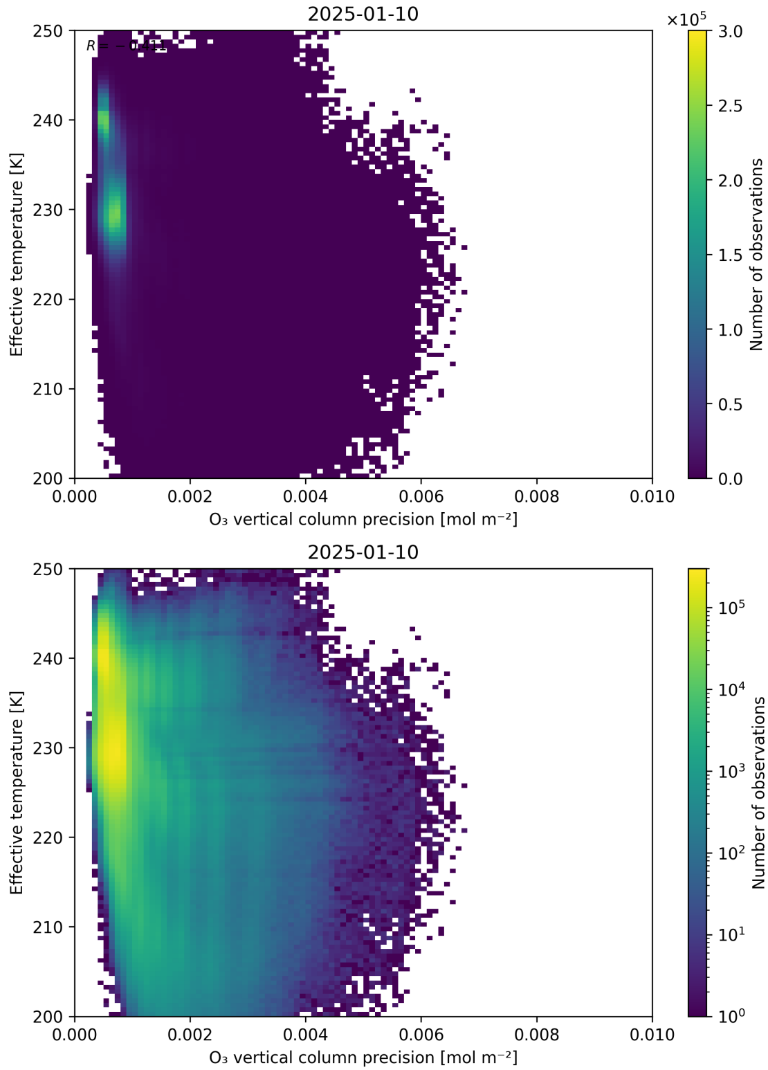
Figure 42: Scatter density plot of “O 3 vertical column precision” against “Effective temperature” for 2025-01-09 to 2025-01-11.
