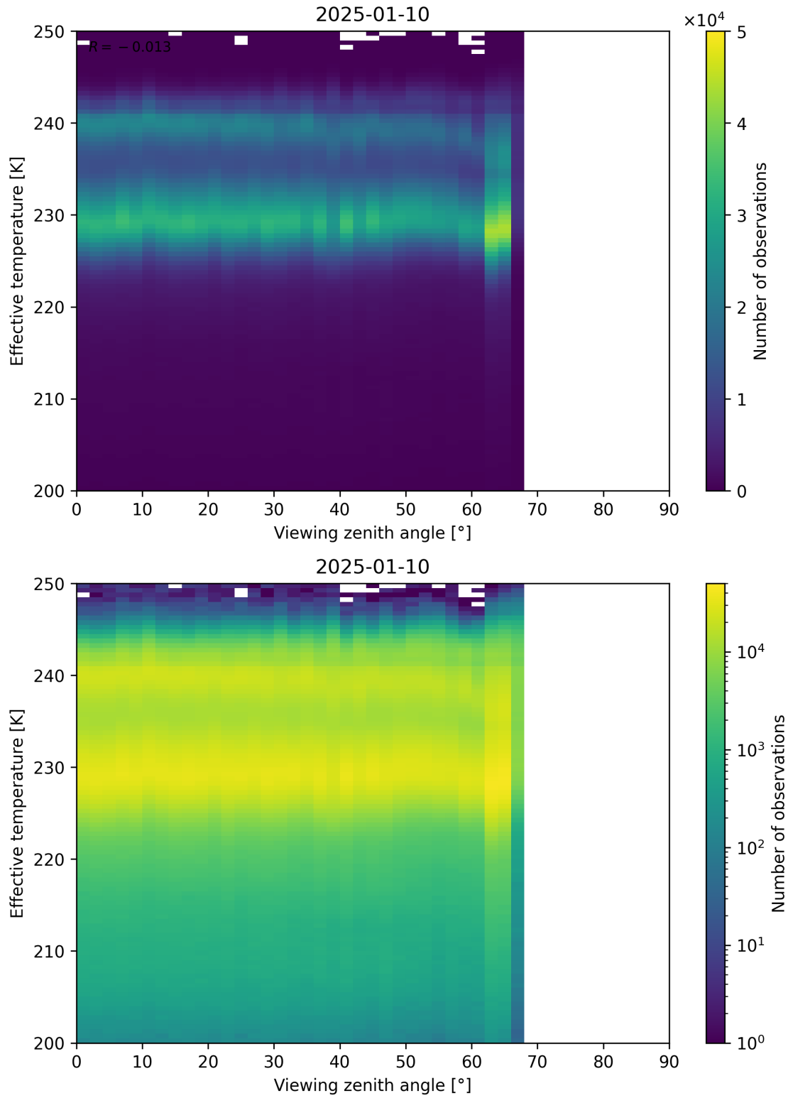
Figure 50: Scatter density plot of “Viewing zenith angle” against “Effective temperature” for 2025-01-09 to 2025-01-11.
