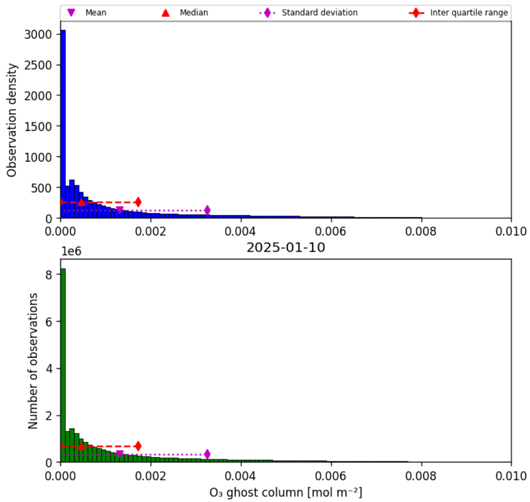
Figure 25: Histogram of “O 3 ghost column” for 2025-01-09 to 2025-01-11
