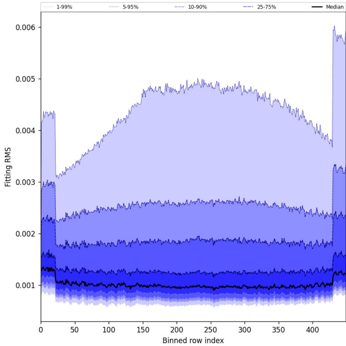
Figure 30: Along track statistics of “Fitting RMS” for 2025-01-09 to 2025-01-11
