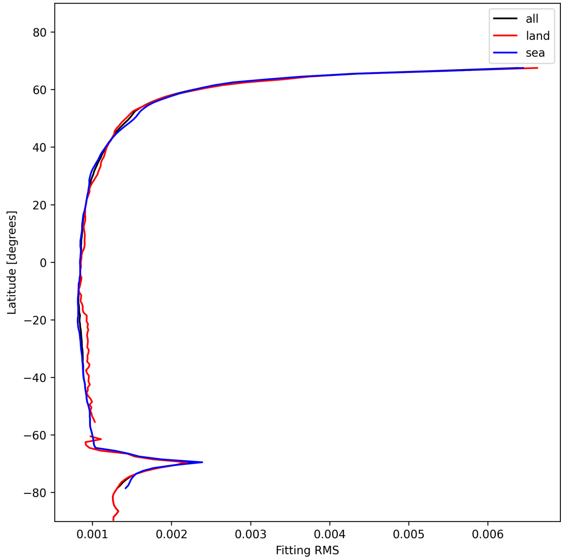
Figure 16: Zonal average of “Fitting RMS” for 2025-01-09 to 2025-01-11.
