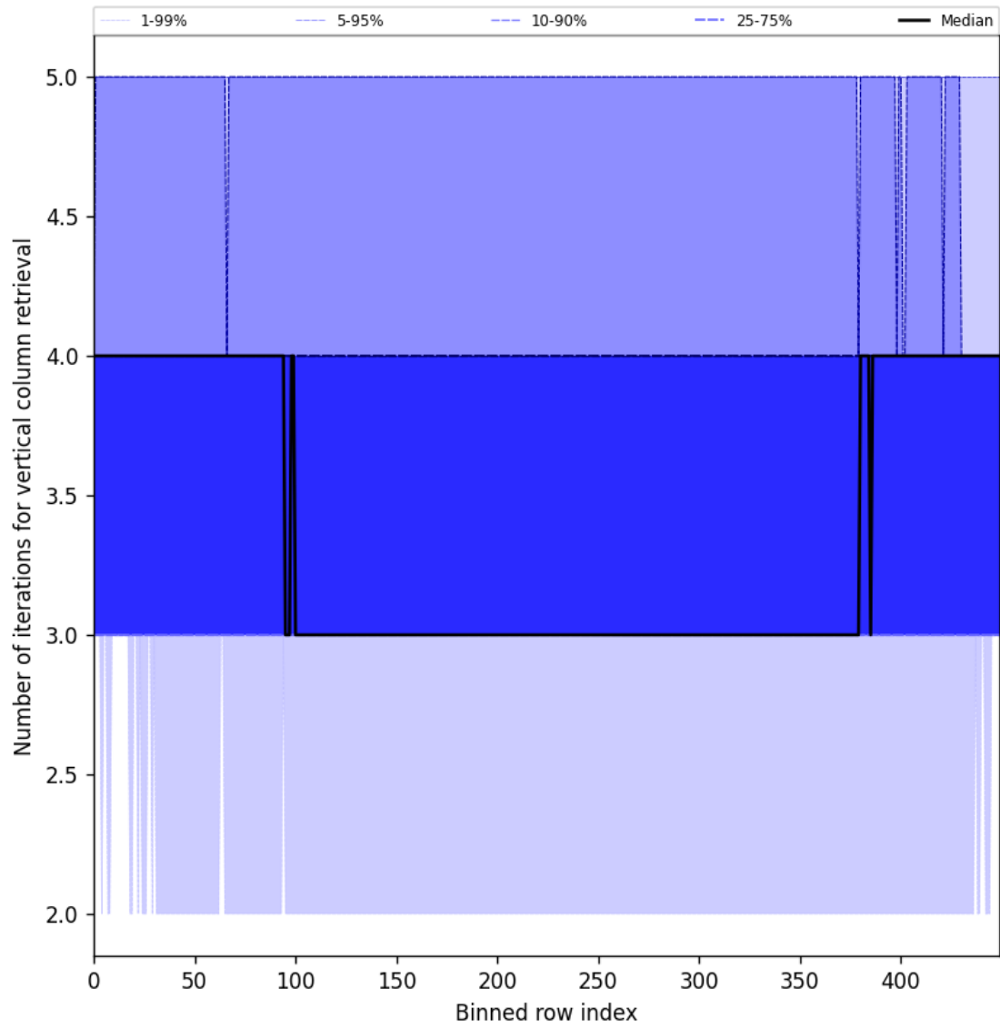
Figure 33: Along track statistics of “Number of iterations for vertical column retrieval” for 2025-01-09 to 2025-01-11
