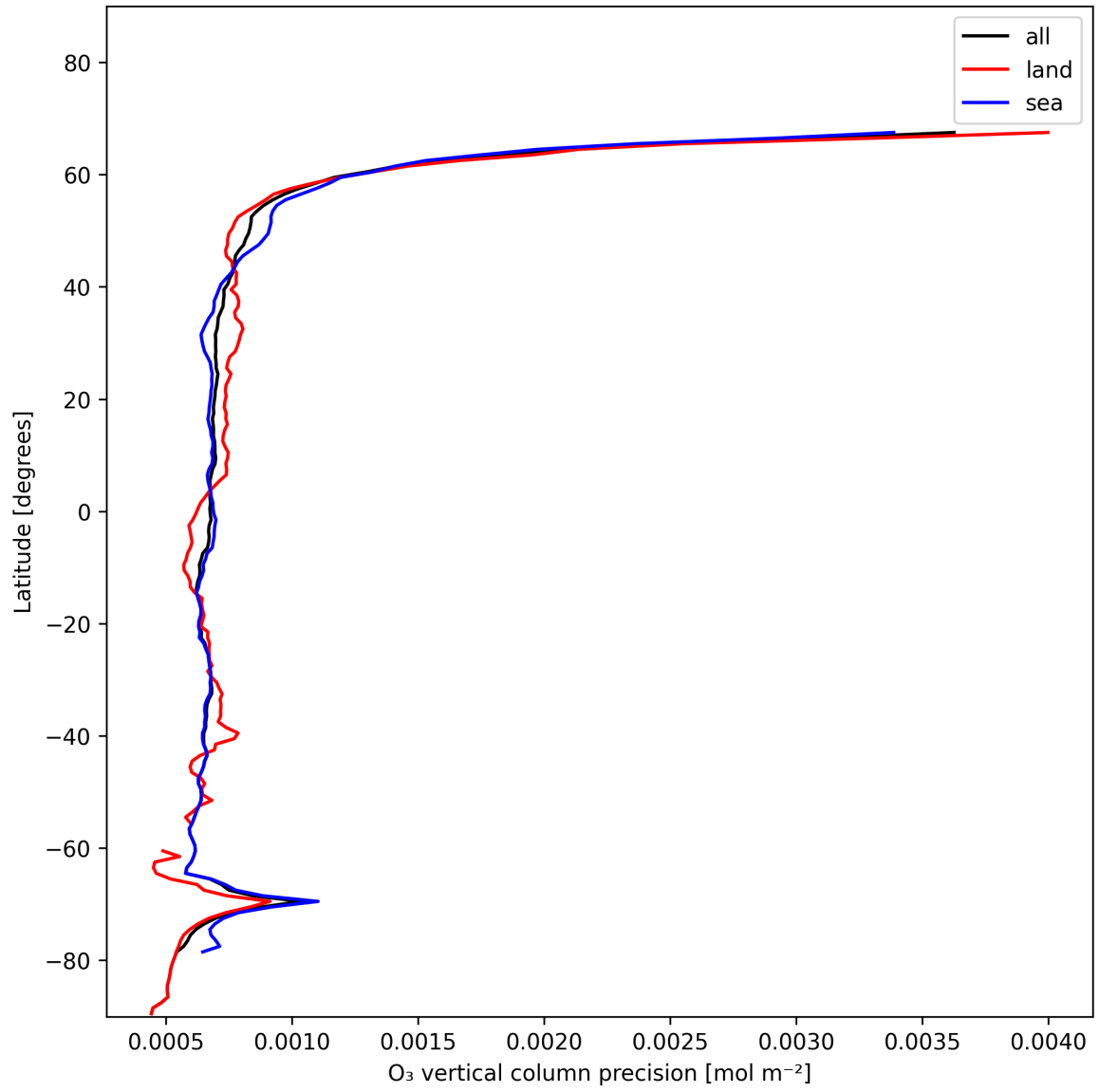
Figure 15: Zonal average of “O 3 vertical column precision” for 2025-01-09 to 2025-01-11.
