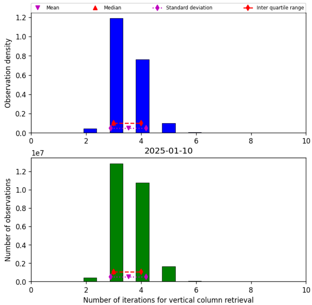
Figure 26: Histogram of “Number of iterations for vertical column retrieval” for 2025-01-09 to 2025-01-11
