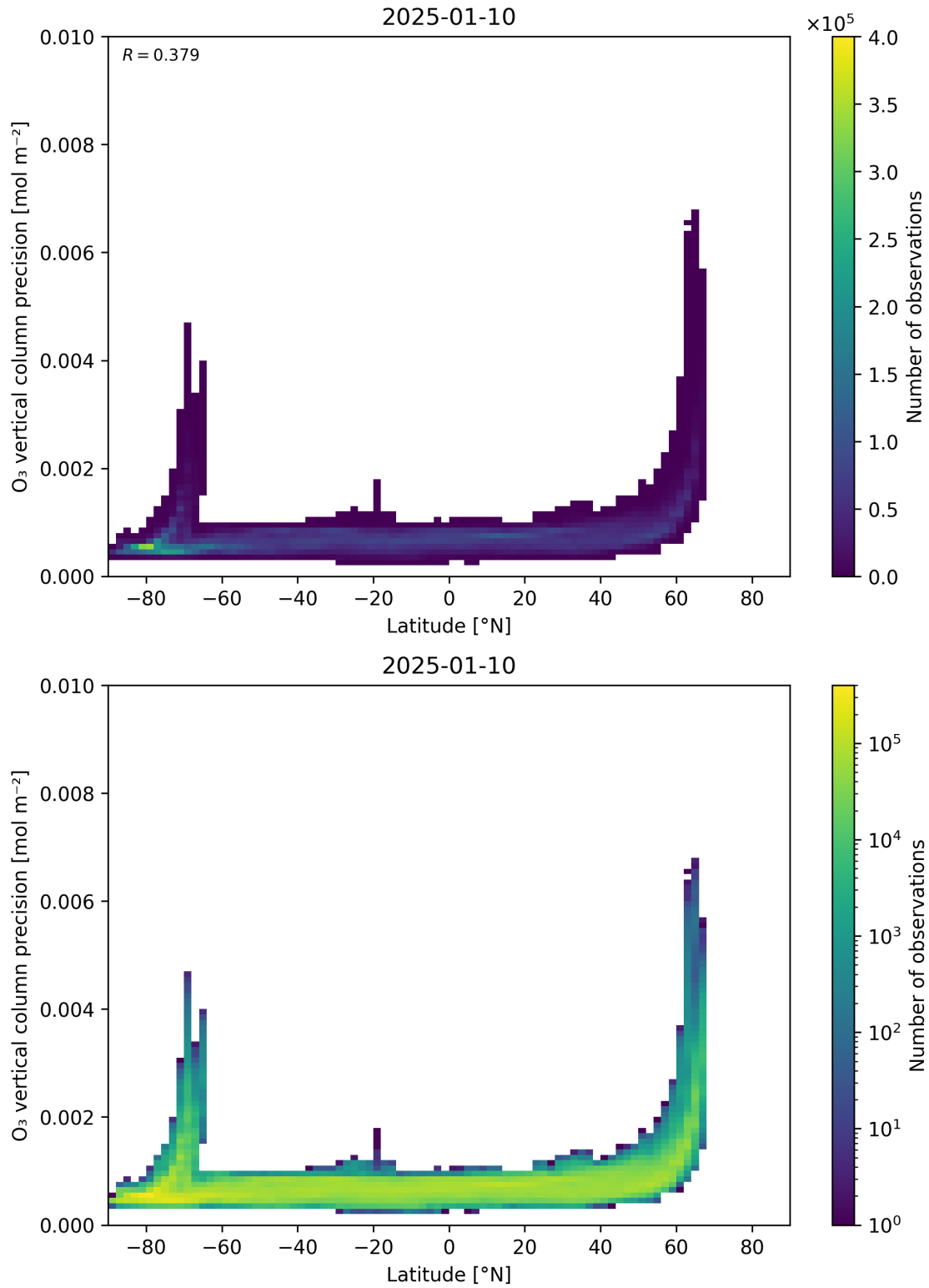
Figure 37: Scatter density plot of “Latitude” against “O 3 vertical column precision” for 2025-01-09 to 2025-01-11.
