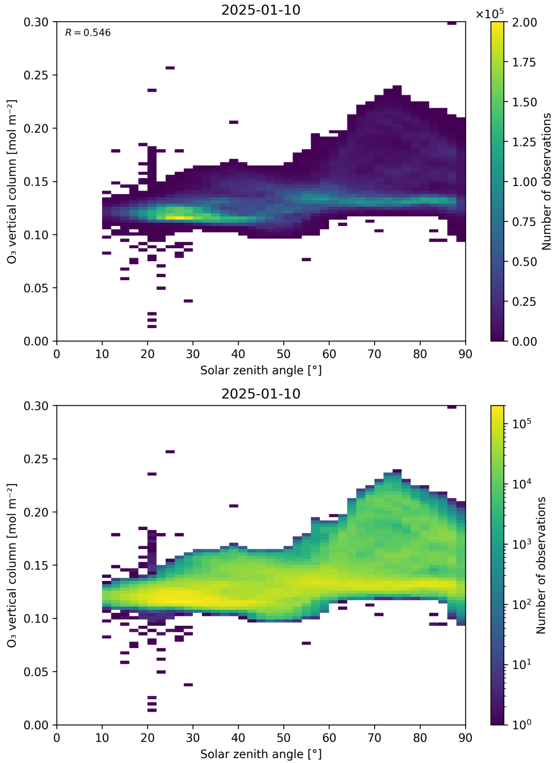
Figure 47: Scatter density plot of “Solar zenith angle” against “O 3 vertical column” for 2025-01-09 to 2025-01-11.
