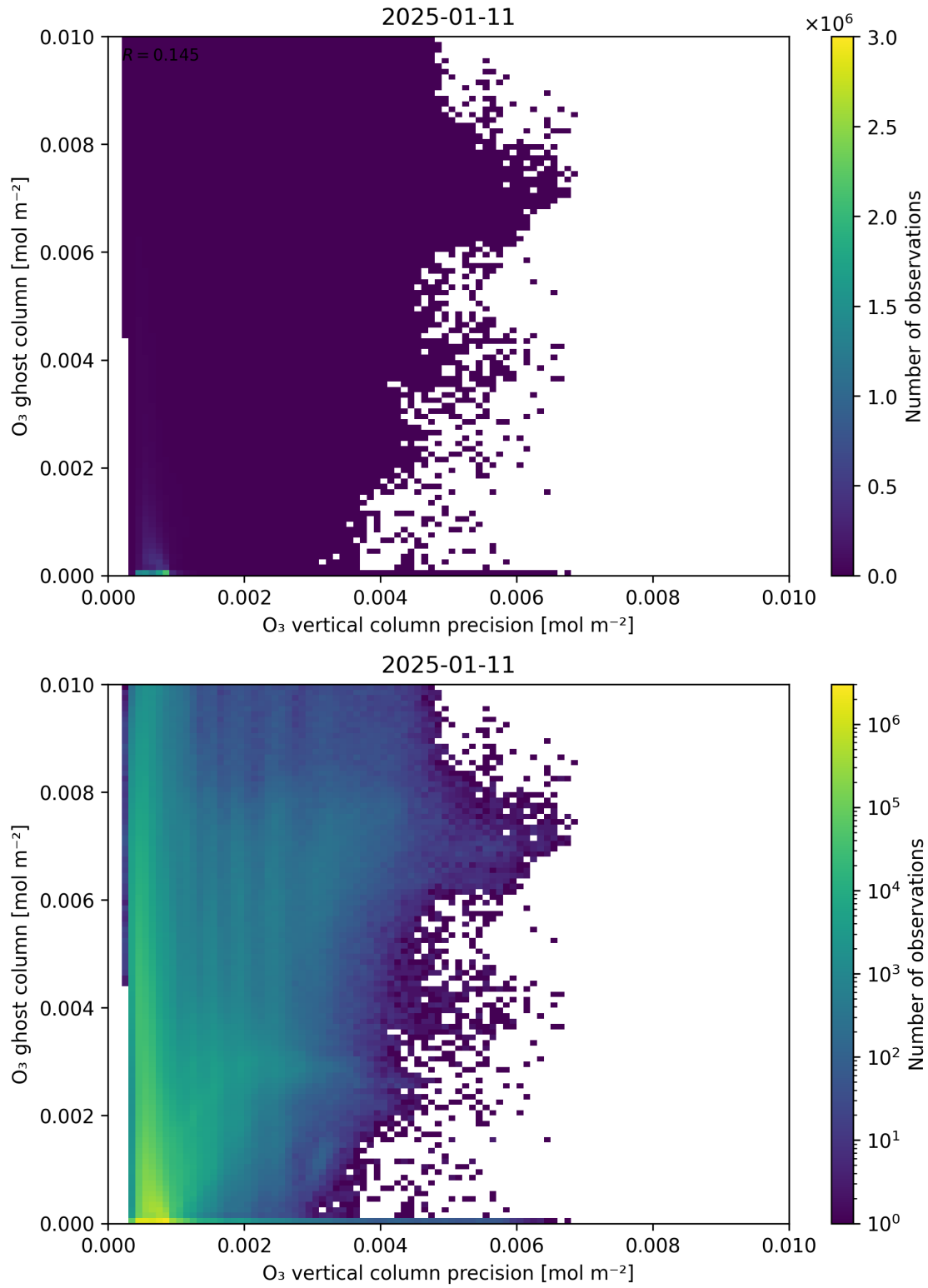
Figure 43: Scatter density plot of “O 3 vertical column precision” against “O 3 ghost column” for 2025-01-10 to 2025-01-12.
