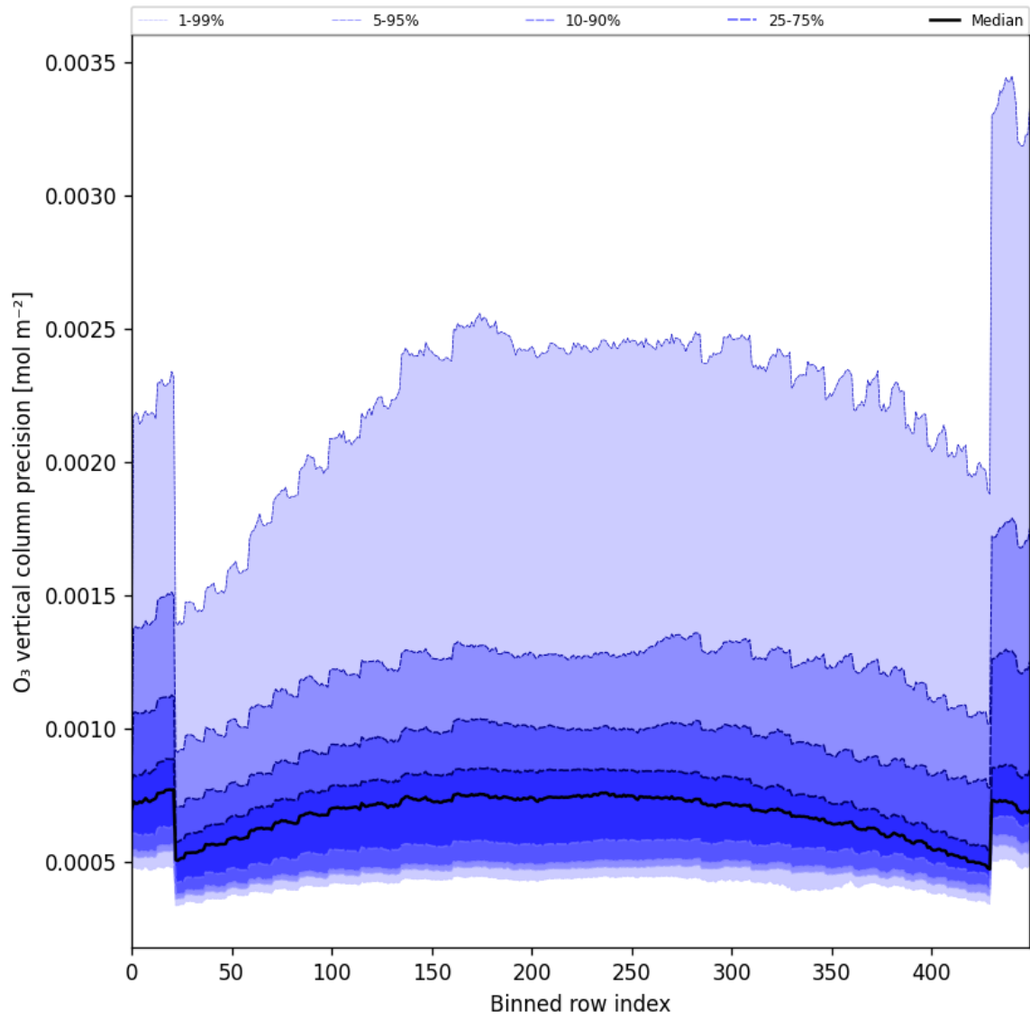
Figure 29: Along track statistics of “O 3 vertical column precision” for 2025-01-10 to 2025-01-12
