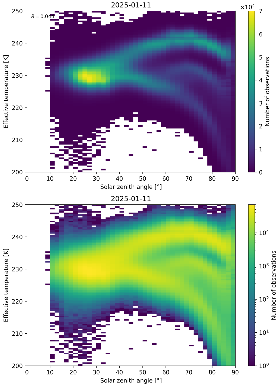
Figure 45: Scatter density plot of “Solar zenith angle” against “Effective temperature” for 2025-01-10 to 2025-01-12.
