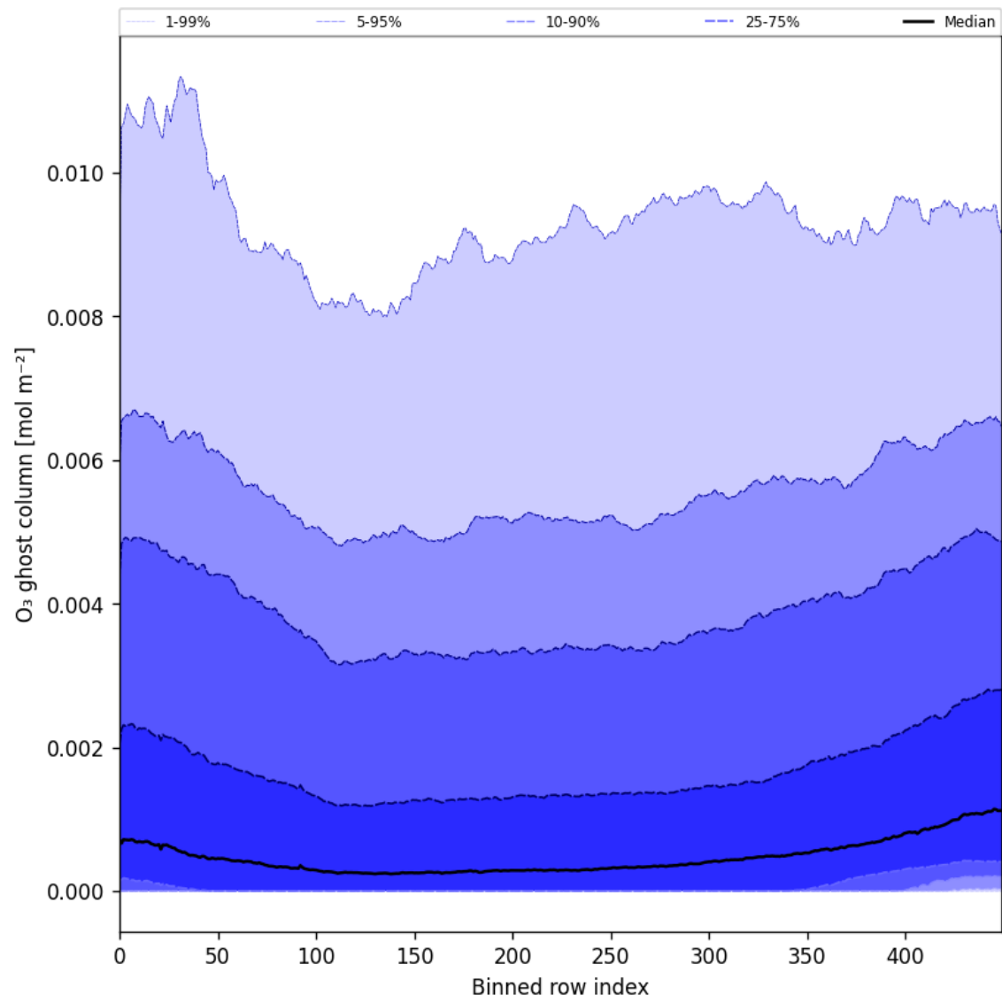
Figure 32: Along track statistics of “O 3 ghost column” for 2025-01-10 to 2025-01-12
