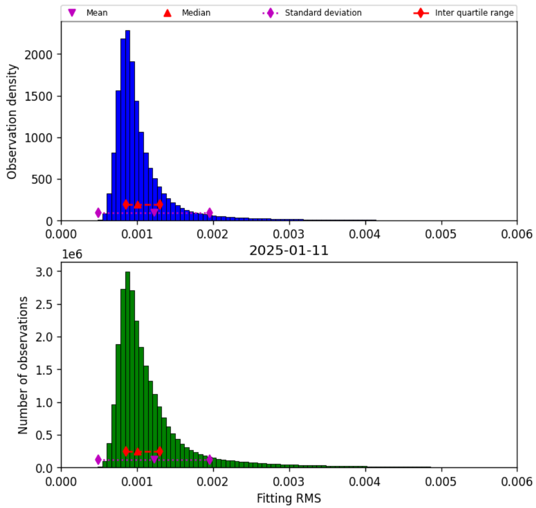
Figure 23: Histogram of “Fitting RMS” for 2025-01-10 to 2025-01-12
