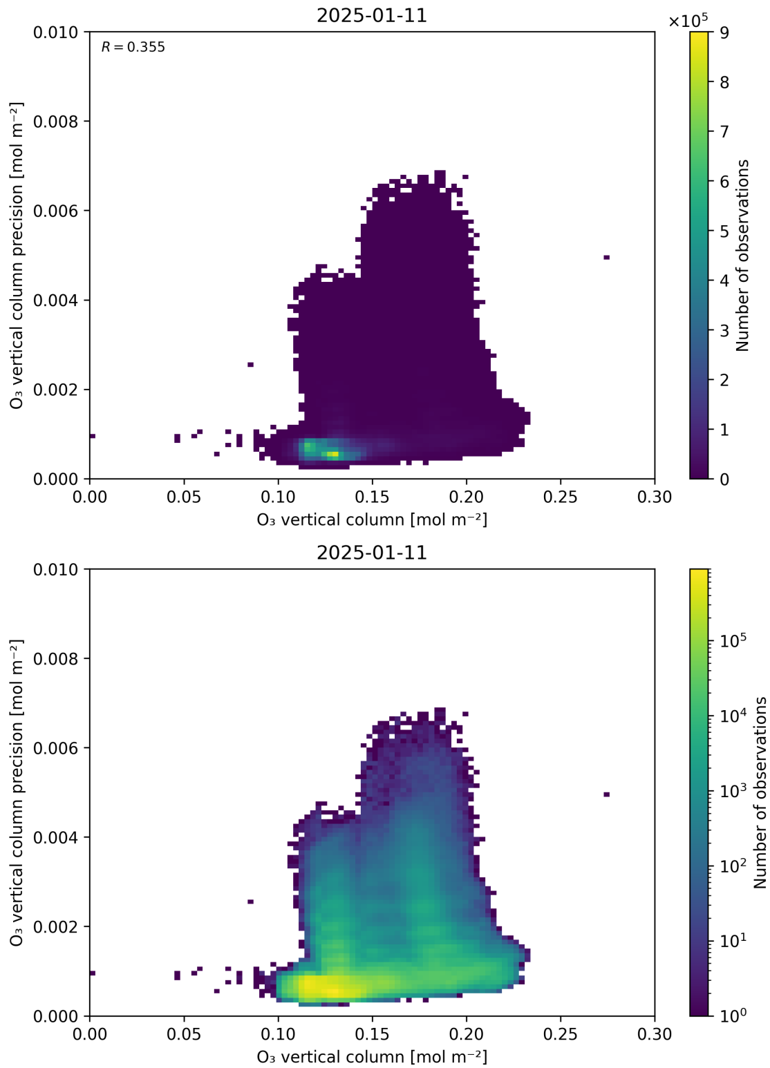
Figure 41: Scatter density plot of “O 3 vertical column” against “O 3 vertical column precision” for 2025-01-10 to 2025-01-12.
