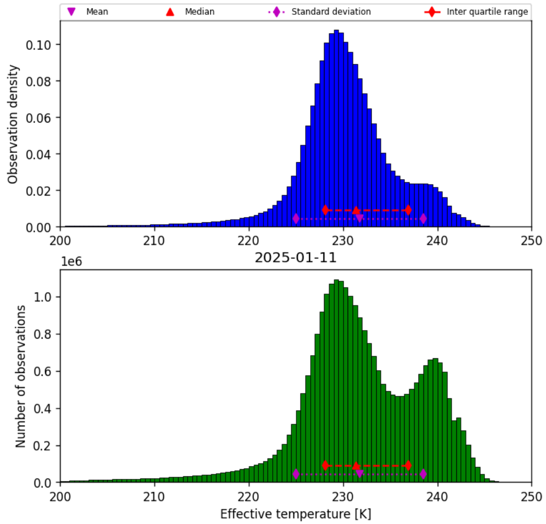
Figure 24: Histogram of “Effective temperature” for 2025-01-10 to 2025-01-12
