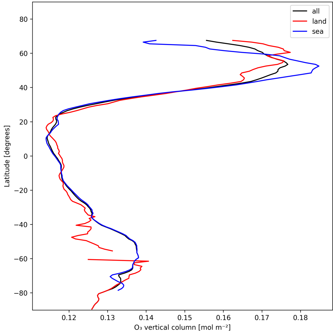
Figure 14: Zonal average of “O 3 vertical column” for 2025-01-10 to 2025-01-12.
