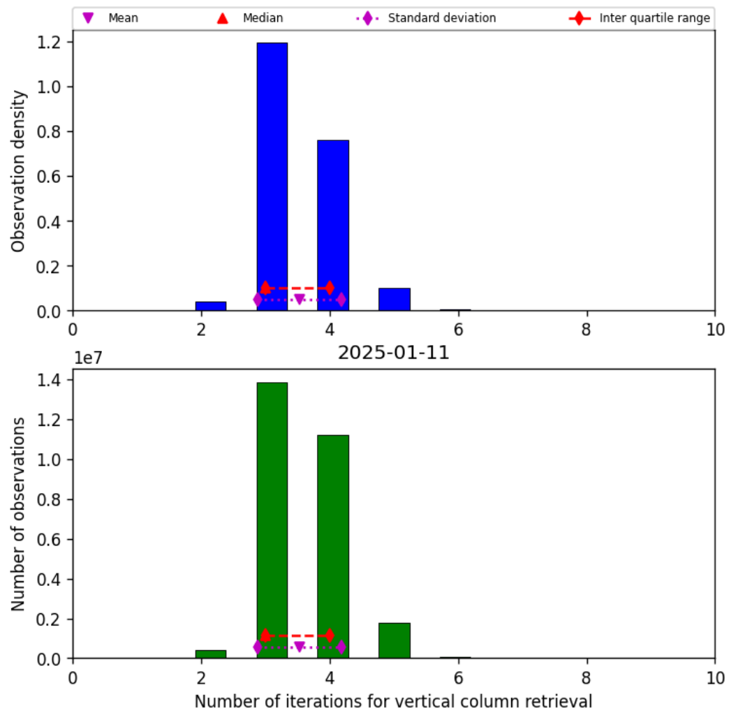
Figure 26: Histogram of “Number of iterations for vertical column retrieval” for 2025-01-10 to 2025-01-12
