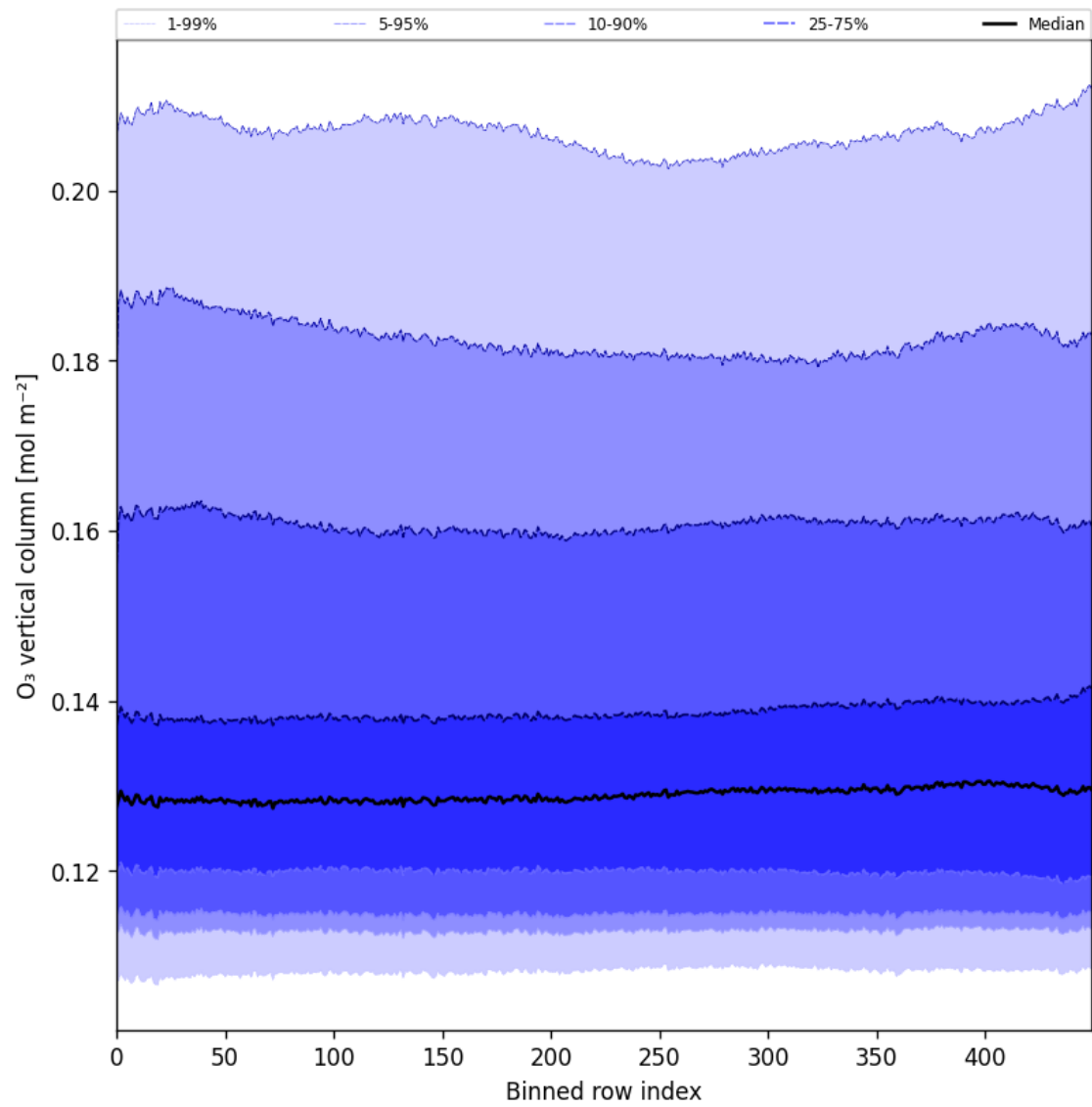
Figure 28: Along track statistics of “O 3 vertical column” for 2025-01-10 to 2025-01-12
