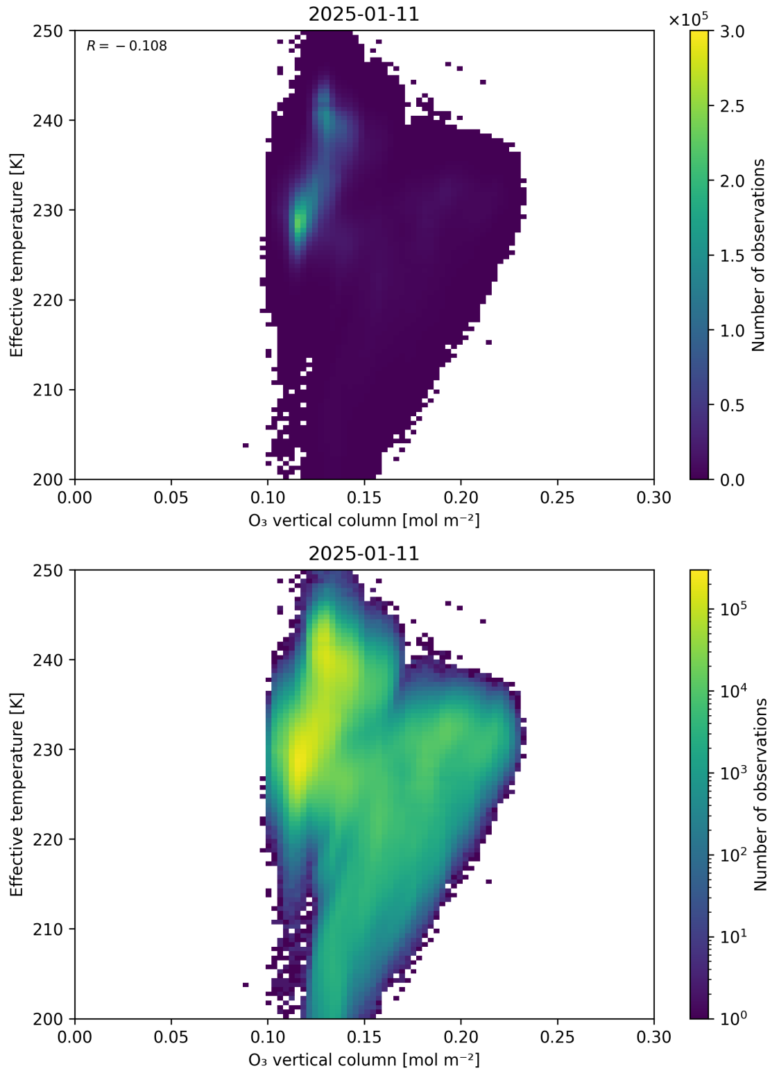
Figure 39: Scatter density plot of “O 3 vertical column” against “Effective temperature” for 2025-01-10 to 2025-01-12.
