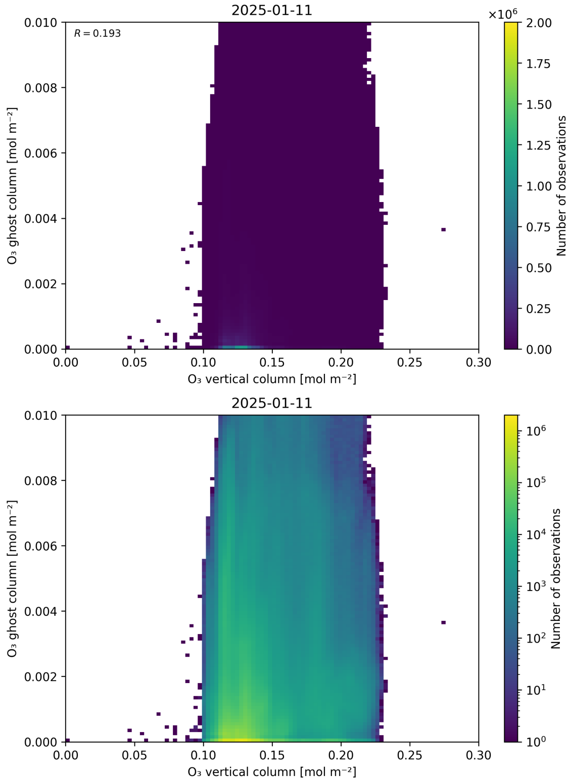
Figure 40: Scatter density plot of “O 3 vertical column” against “O 3 ghost column” for 2025-01-10 to 2025-01-12.
