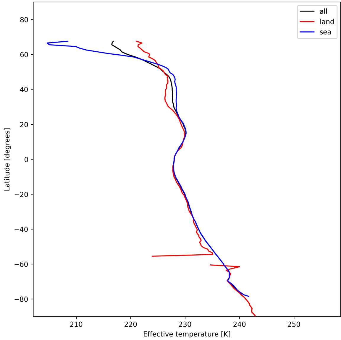
Figure 17: Zonal average of "Effective temperature" for 2025-01-10 to 2025-01-12.
