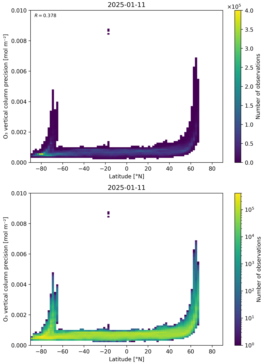
Figure 37: Scatter density plot of “Latitude” against “O 3 vertical column precision” for 2025-01-10 to 2025-01-12.
