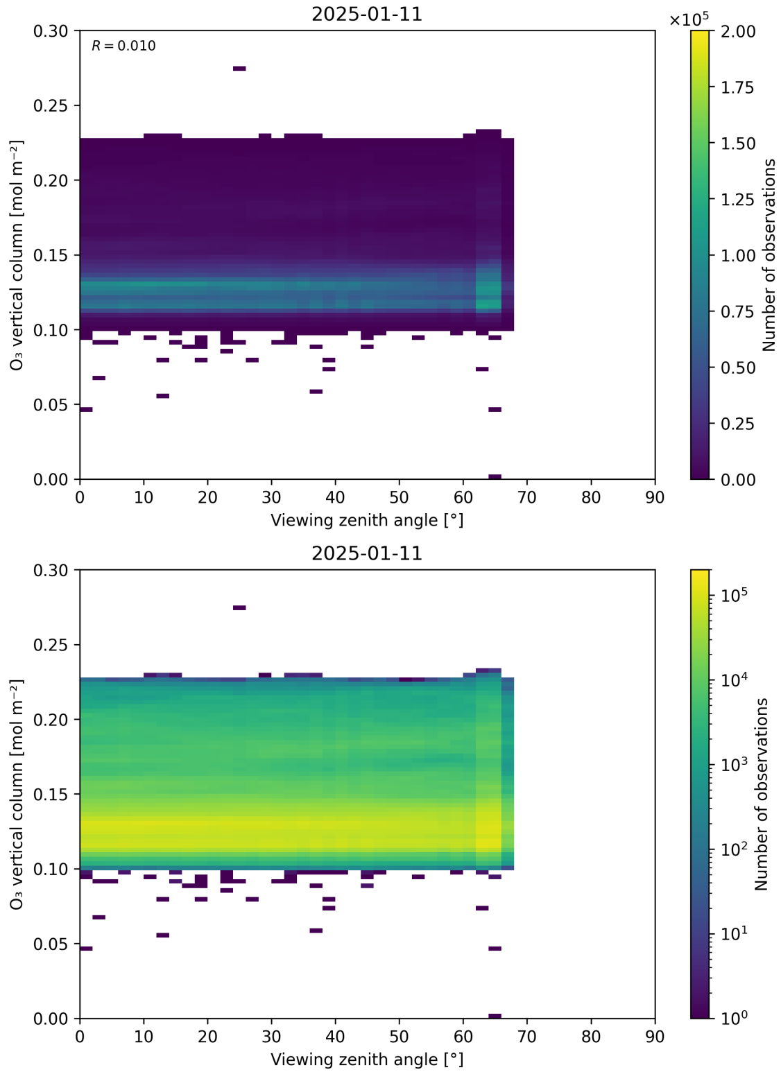
Figure 52: Scatter density plot of “Viewing zenith angle” against “O 3 vertical column” for 2025-01-10 to 2025-01-12.
