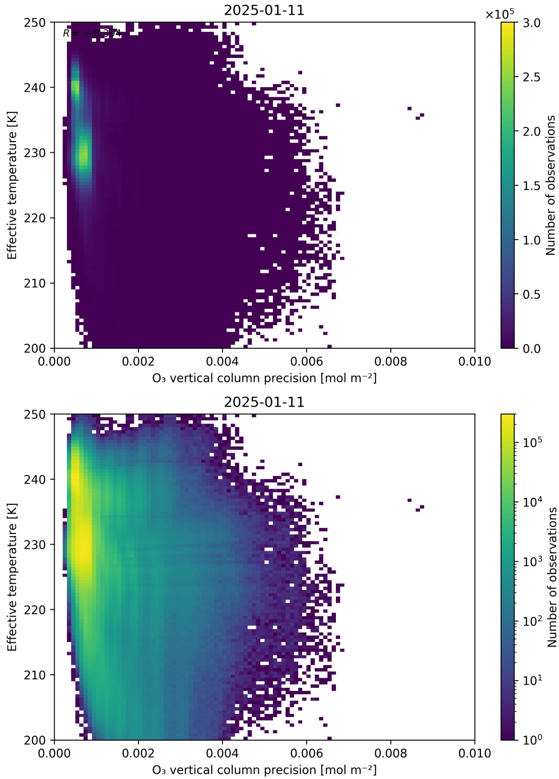
Figure 42: Scatter density plot of “O 3 vertical column precision” against “Effective temperature” for 2025-01-10 to 2025-01-12.
