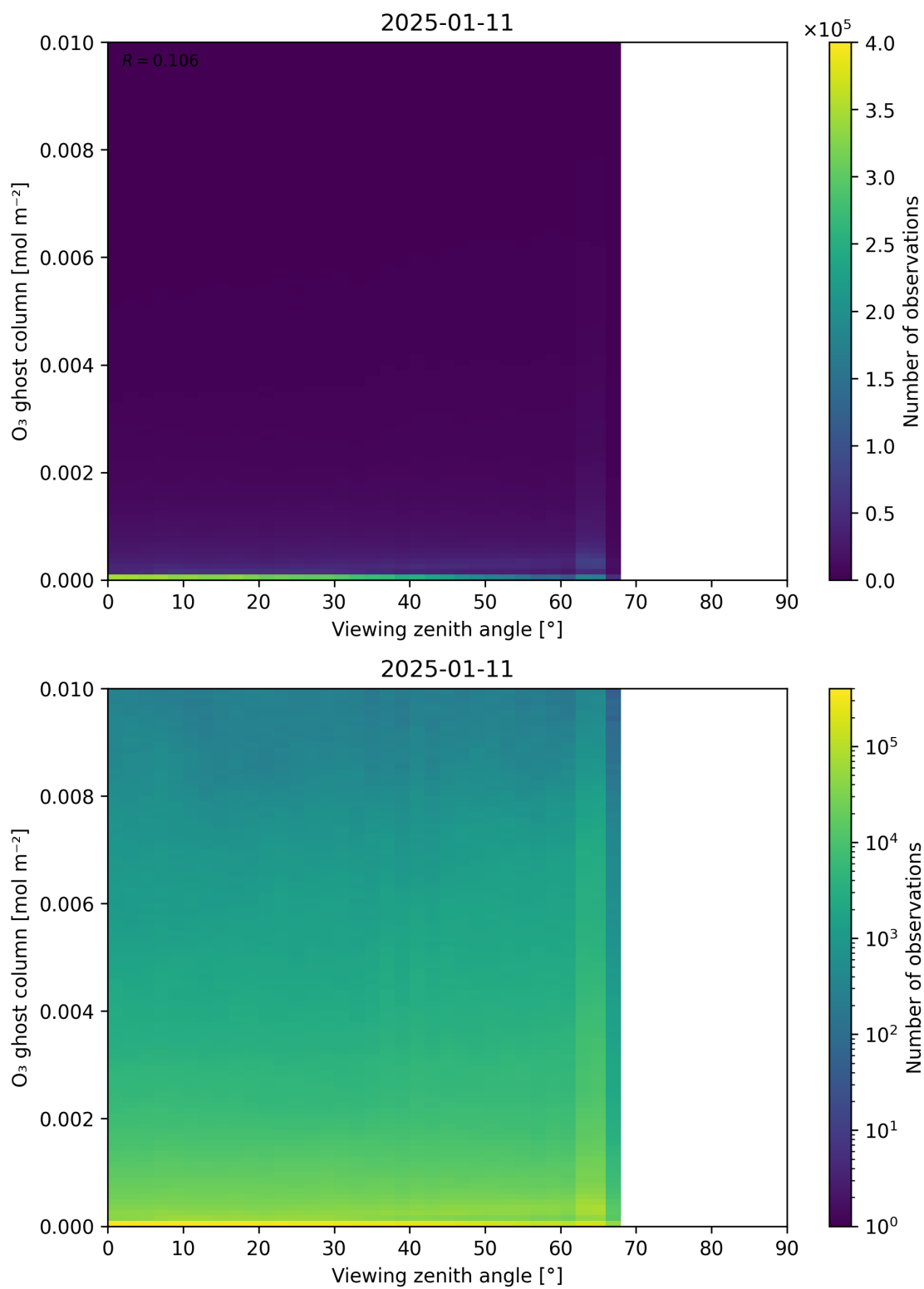
Figure 51: Scatter density plot of “Viewing zenith angle” against “O 3 ghost column” for 2025-01-10 to 2025-01-12.
