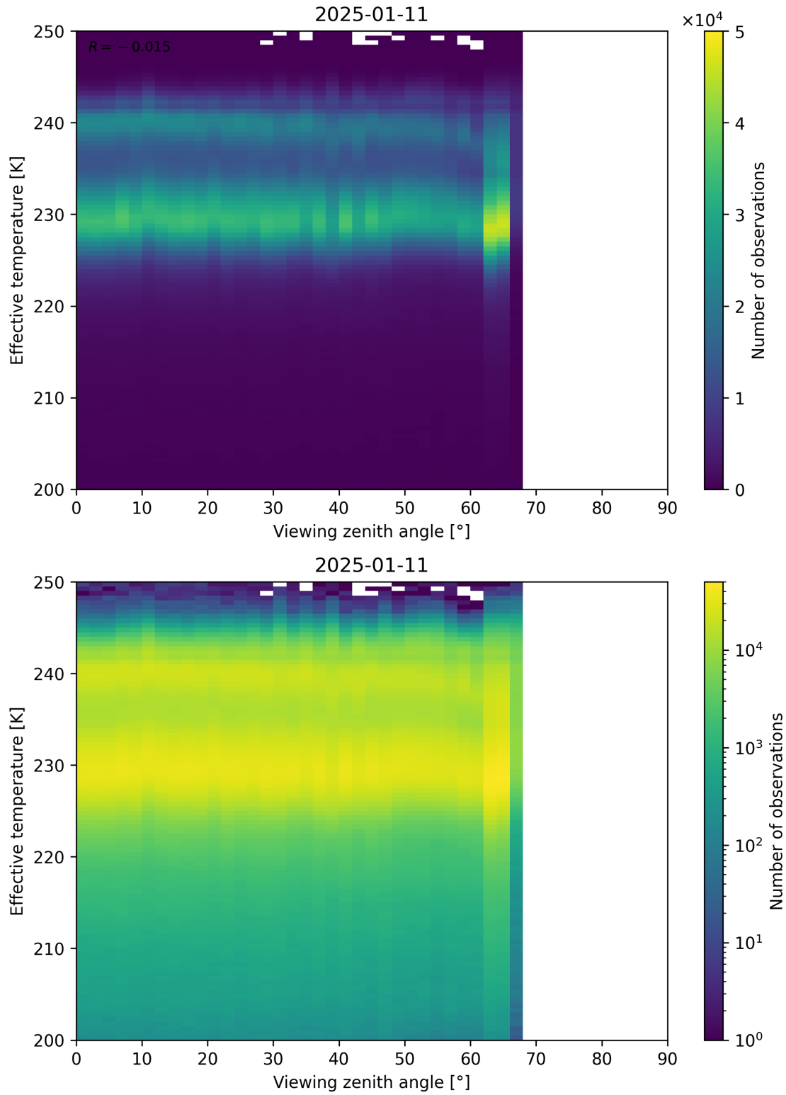
Figure 50: Scatter density plot of “Viewing zenith angle” against “Effective temperature” for 2025-01-10 to 2025-01-12.
