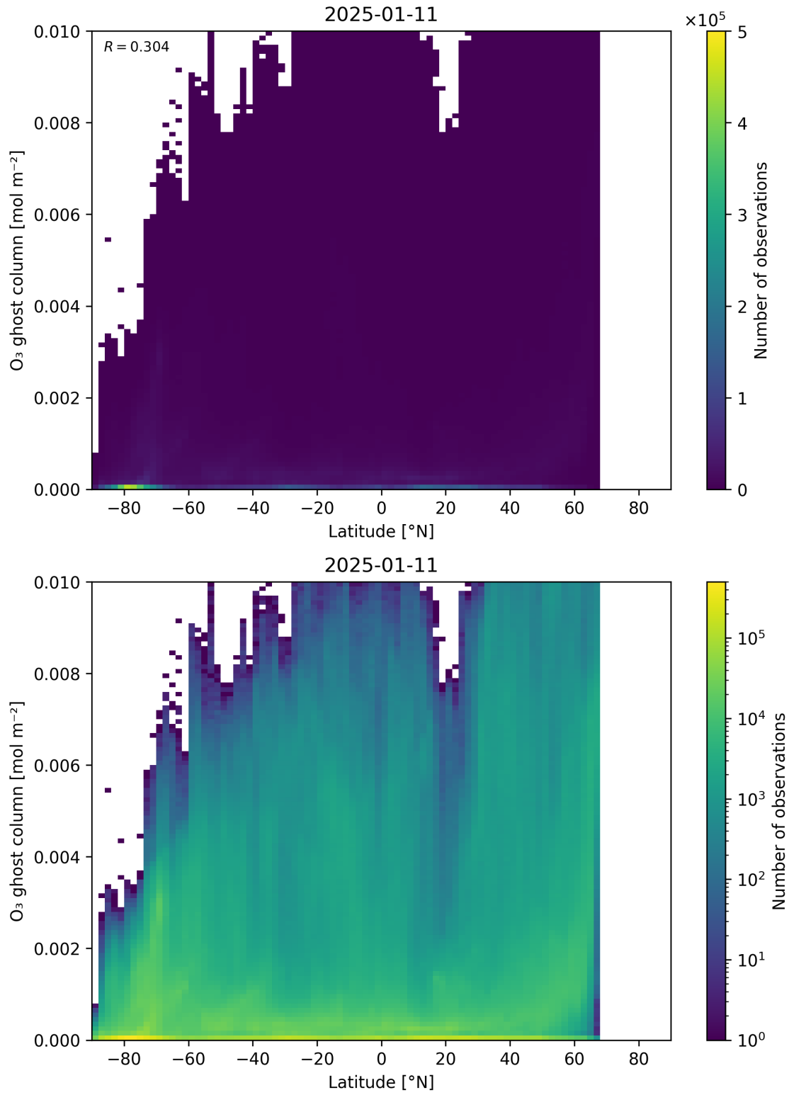
Figure 35: Scatter density plot of “Latitude” against “O 3 ghost column” for 2025-01-10 to 2025-01-12.
