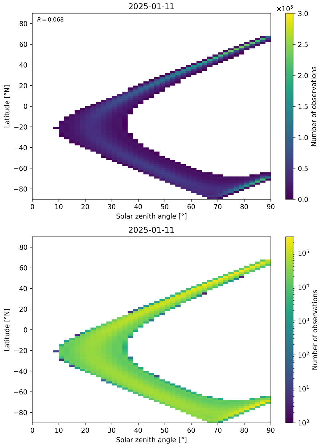
Figure 44: Scatter density plot of “Solar zenith angle” against “Latitude” for 2025-01-10 to 2025-01-12.
