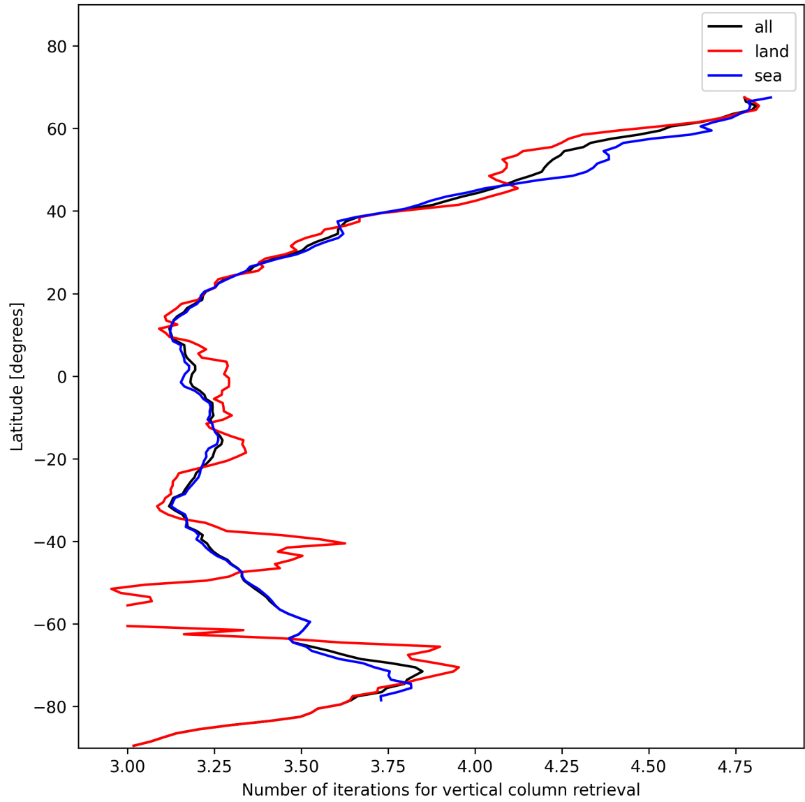
Figure 19: Zonal average of “Number of iterations for vertical column retrieval” for 2025-01-10 to 2025-01-12.
