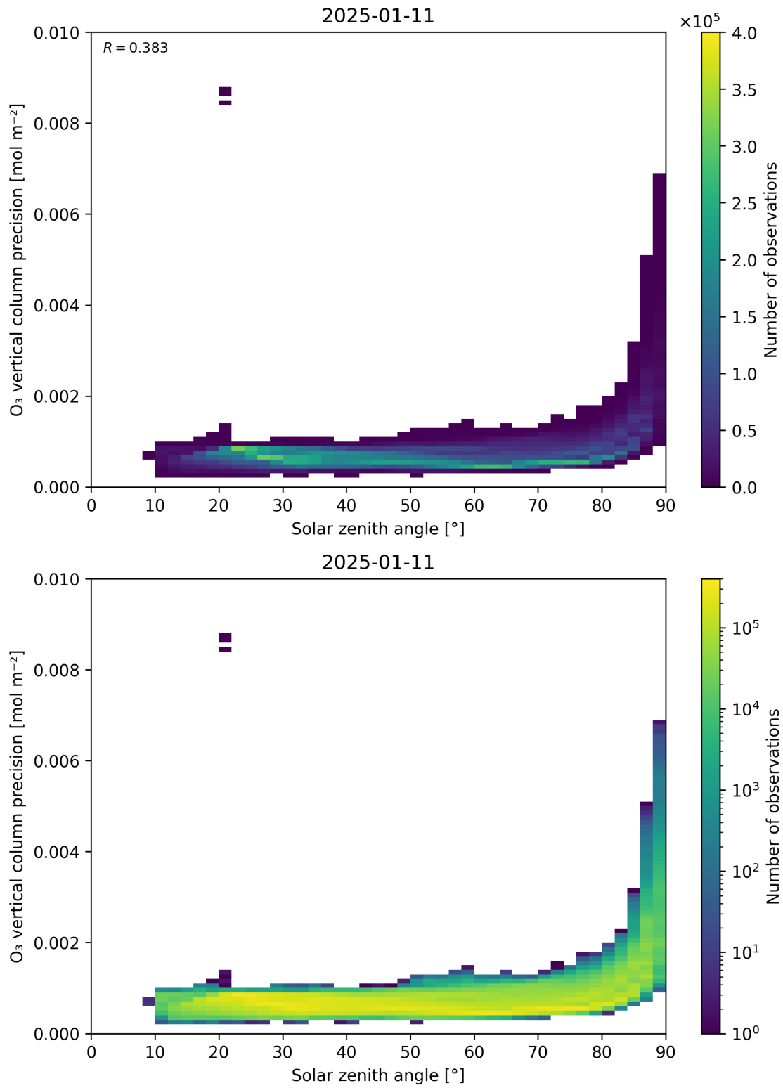
Figure 48: Scatter density plot of “Solar zenith angle” against “O 3 vertical column precision” for 2025-01-10 to 2025-01-12.
