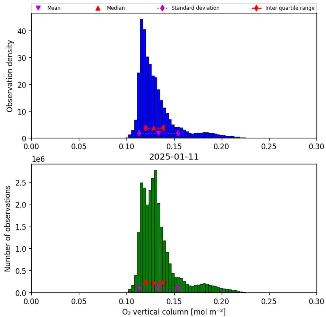
Figure 21: Histogram of “O 3 vertical column” for 2025-01-10 to 2025-01-12
