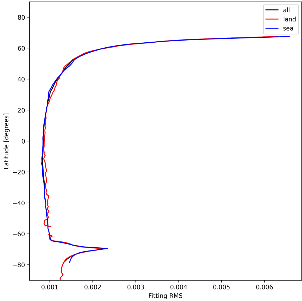
Figure 16: Zonal average of “Fitting RMS” for 2025-01-10 to 2025-01-12.
