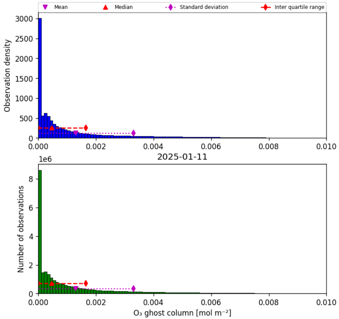
Figure 25: Histogram of “O 3 ghost column” for 2025-01-10 to 2025-01-12
