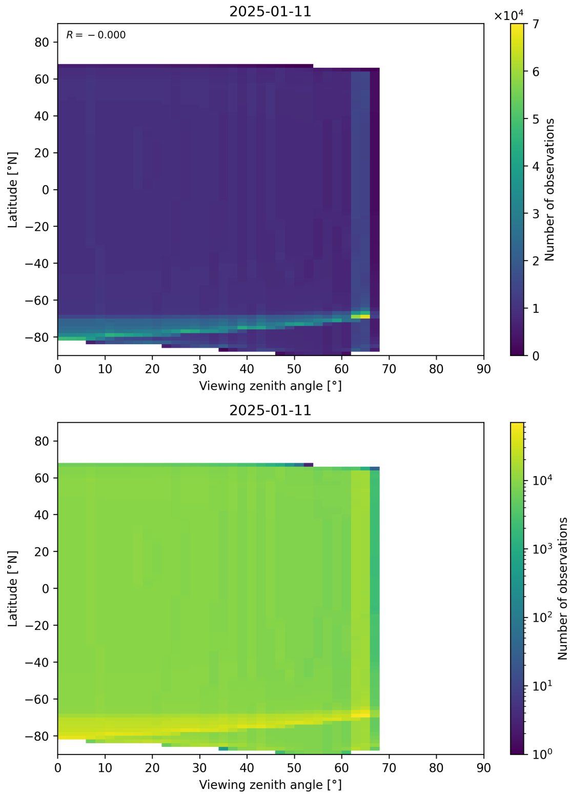
Figure 49: Scatter density plot of “Viewing zenith angle” against “Latitude” for 2025-01-10 to 2025-01-12.
