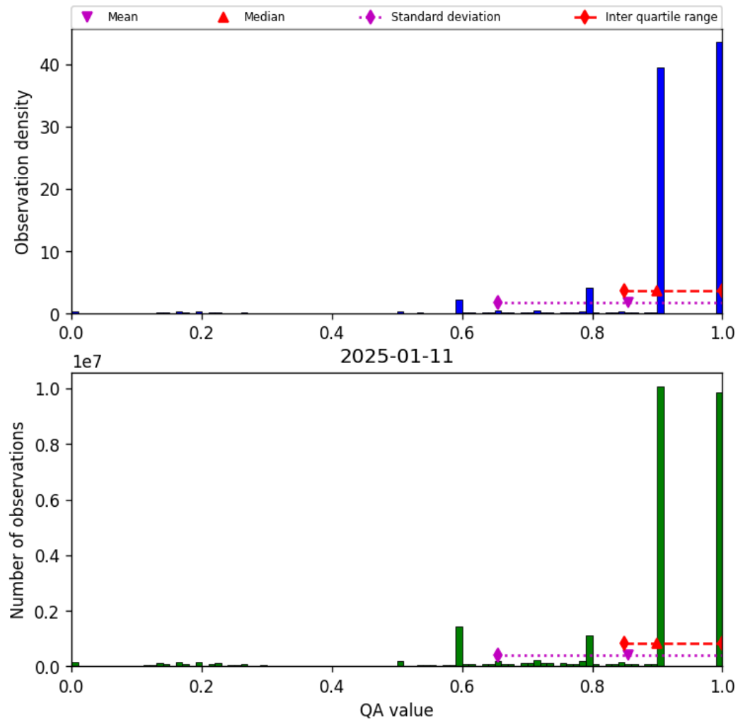
Figure 20: Histogram of “QA value” for 2025-01-10 to 2025-01-12
