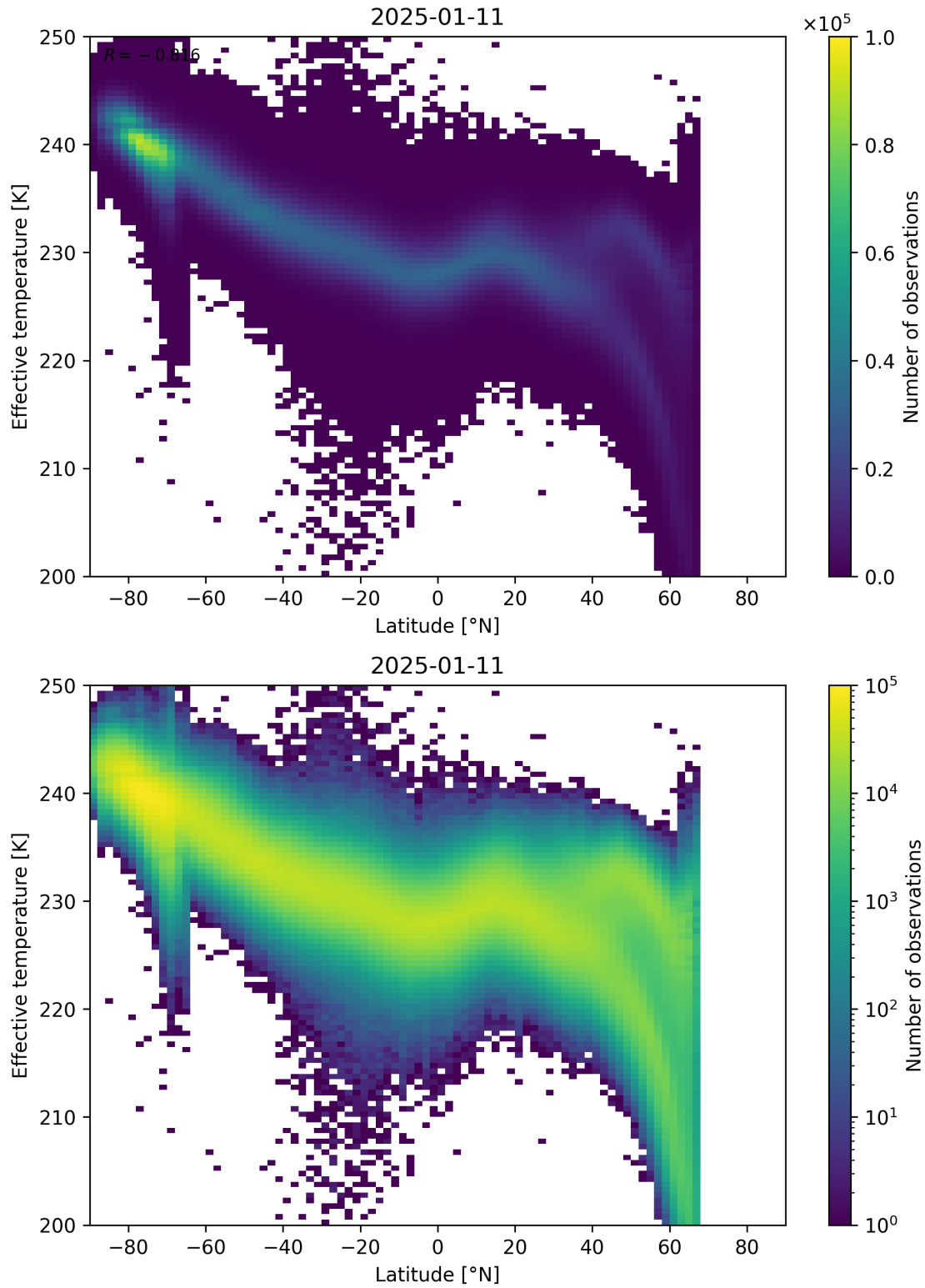
Figure 34: Scatter density plot of “Latitude” against “Effective temperature” for 2025-01-10 to 2025-01-12.
