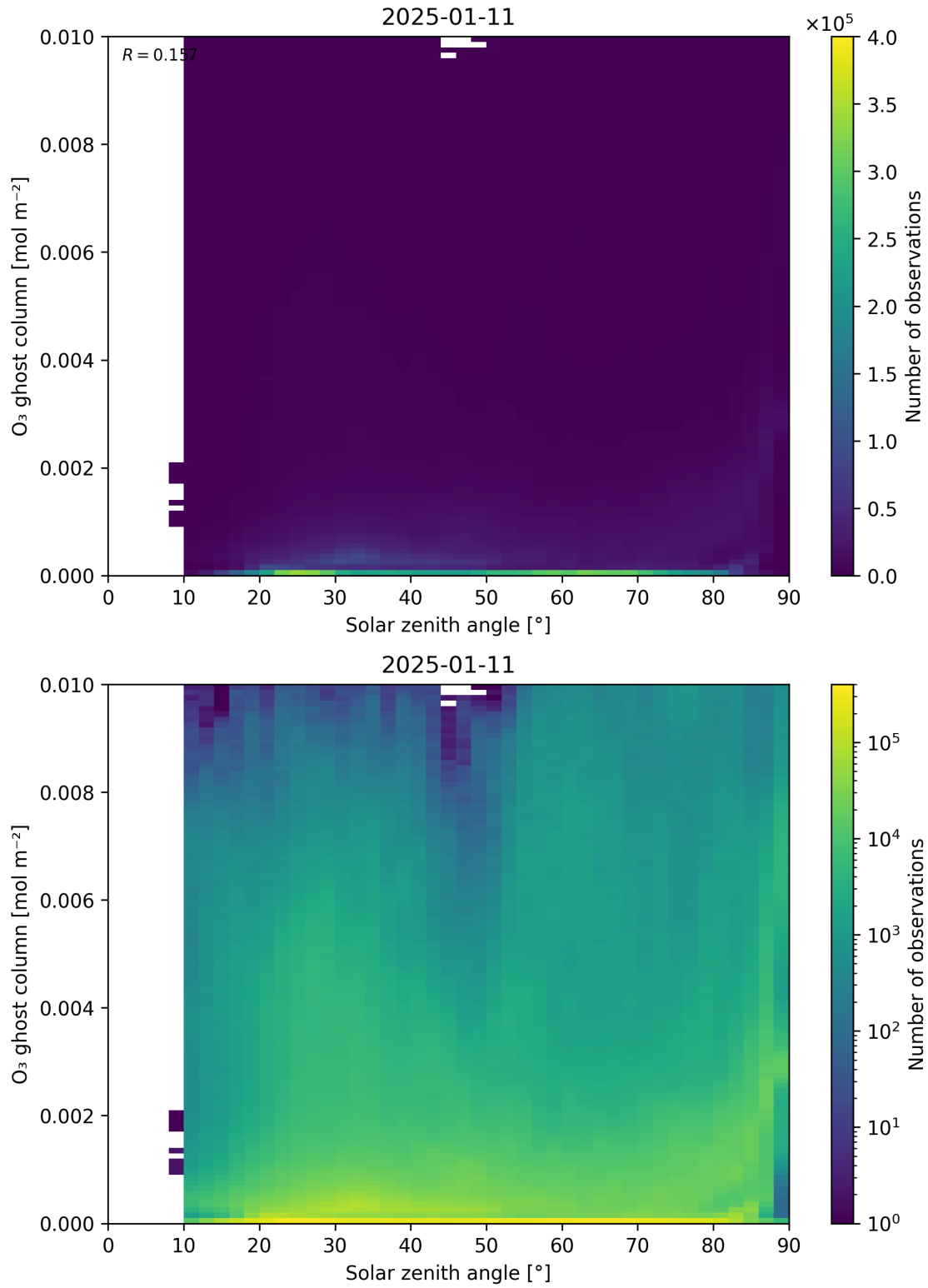
Figure 46: Scatter density plot of “Solar zenith angle” against “O 3 ghost column” for 2025-01-10 to 2025-01-12.
