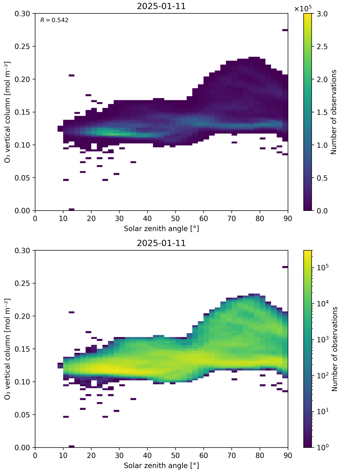
Figure 47: Scatter density plot of “Solar zenith angle” against “O 3 vertical column” for 2025-01-10 to 2025-01-12.
