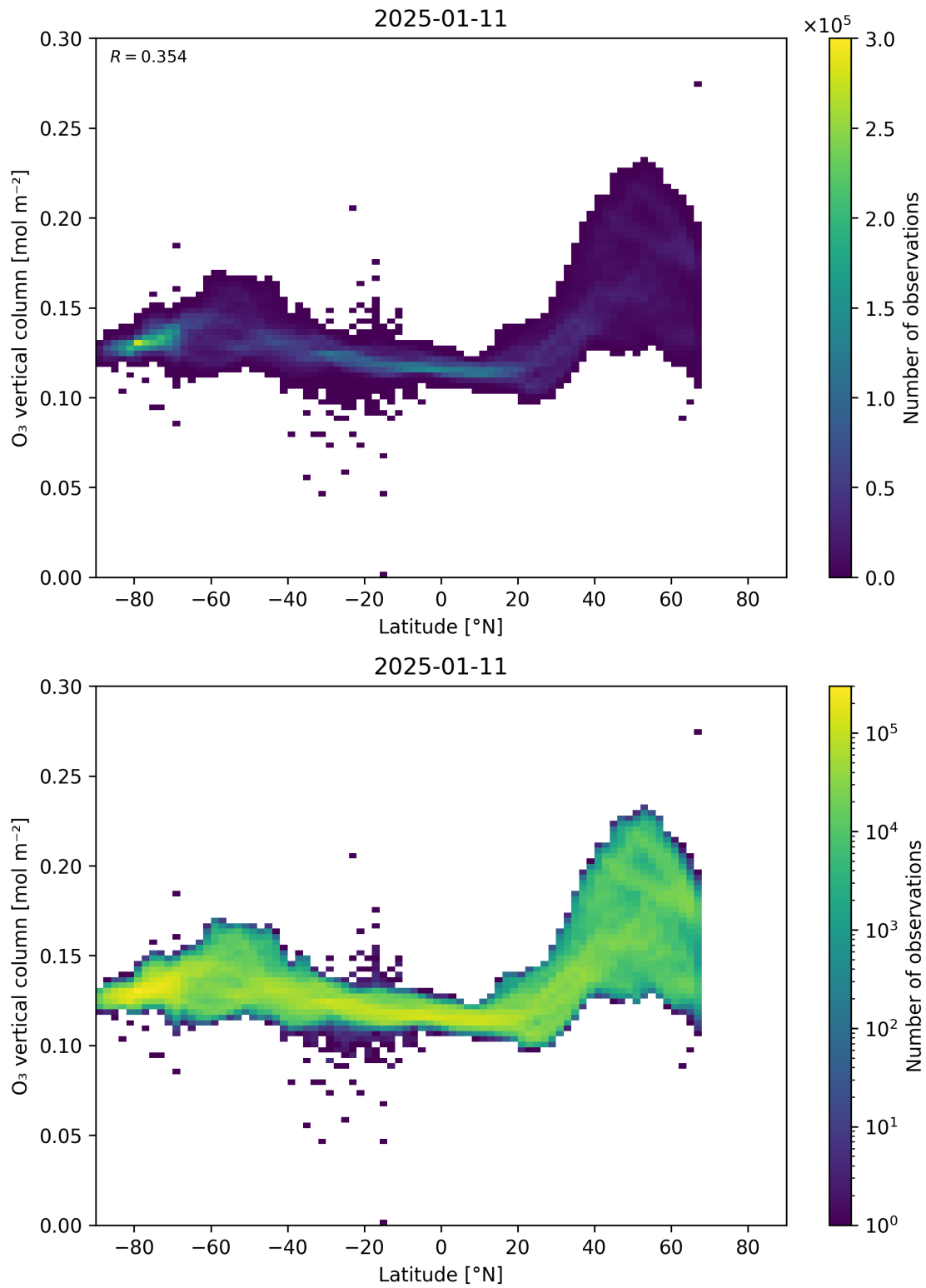
Figure 36: Scatter density plot of “Latitude” against “O 3 vertical column” for 2025-01-10 to 2025-01-12.
