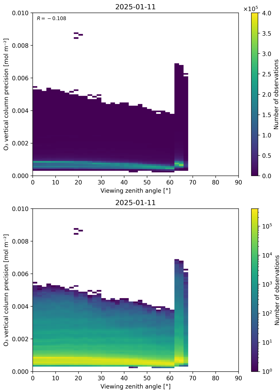
Figure 53: Scatter density plot of “Viewing zenith angle” against “O 3 vertical column precision” for 2025-01-10 to 2025-01-12.
