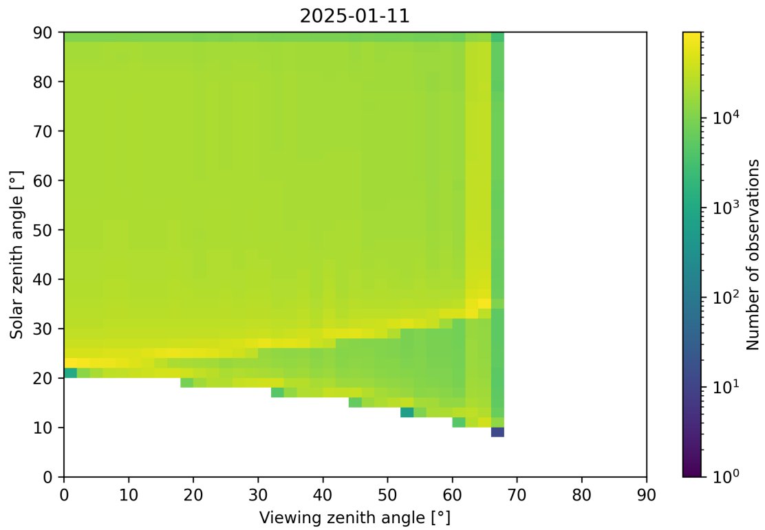
Figure 54: Scatter density plot of “Viewing zenith angle” against “Solar zenith angle” for 2025-01-10 to 2025-01-12.
