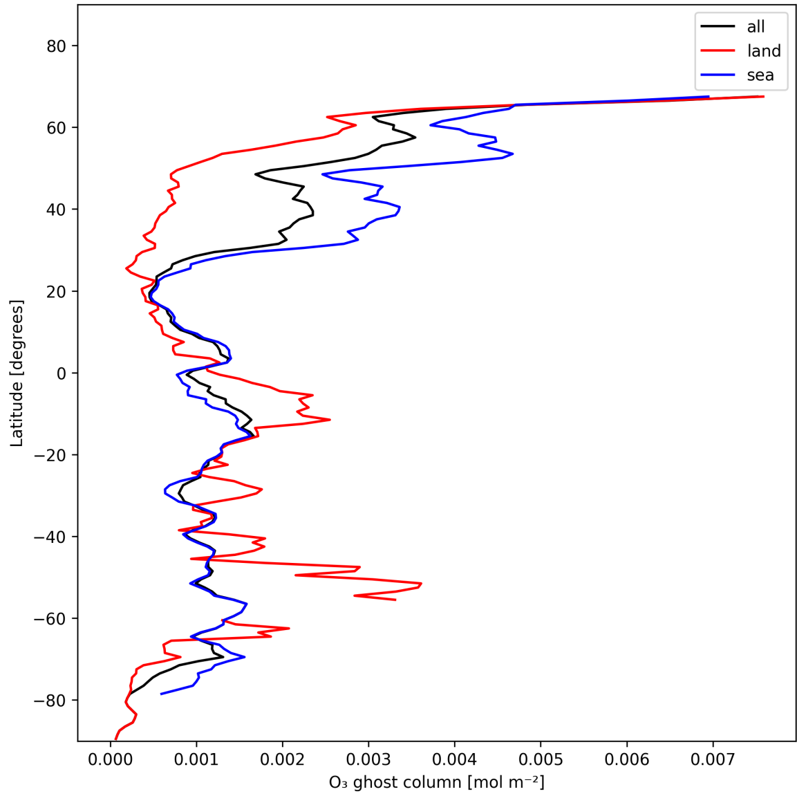
Figure 18: Zonal average of “O 3 ghost column” for 2025-01-10 to 2025-01-12.
