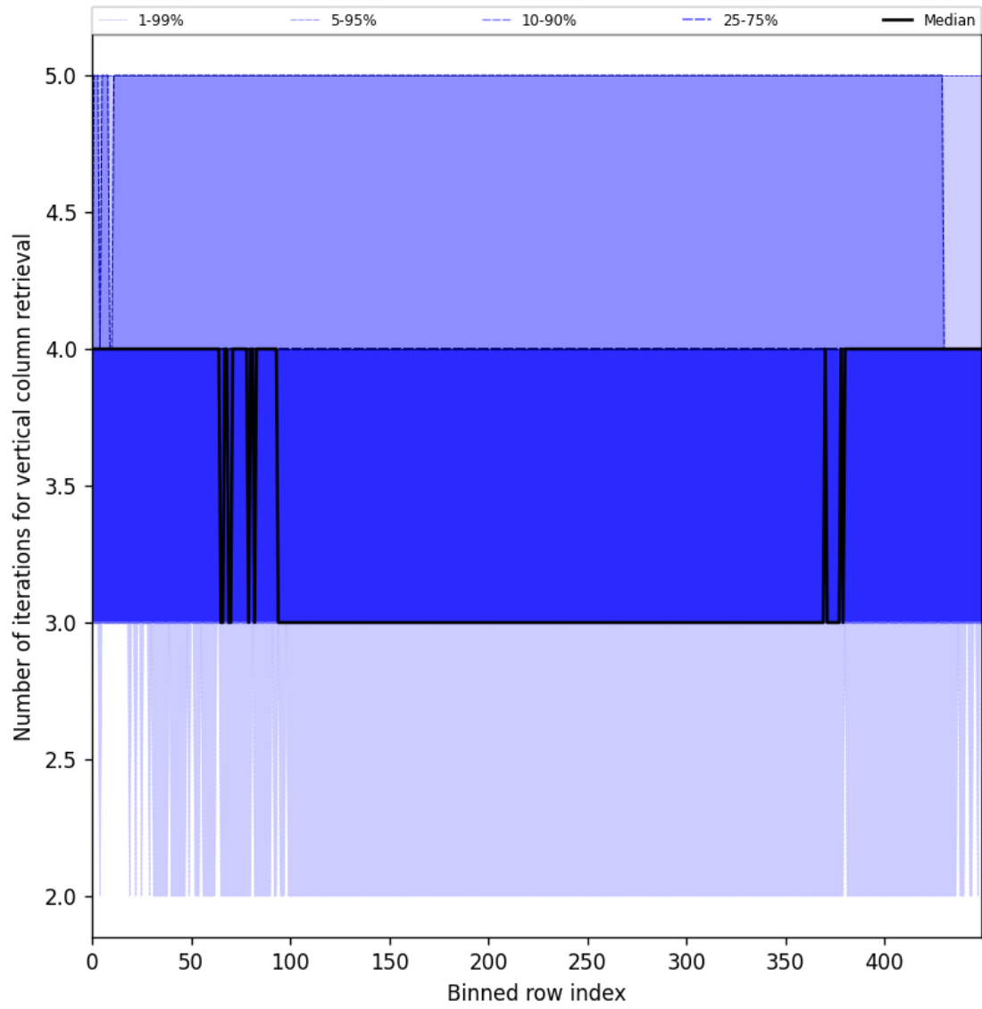
Figure 33: Along track statistics of “Number of iterations for vertical column retrieval” for 2025-01-10 to 2025-01-12
