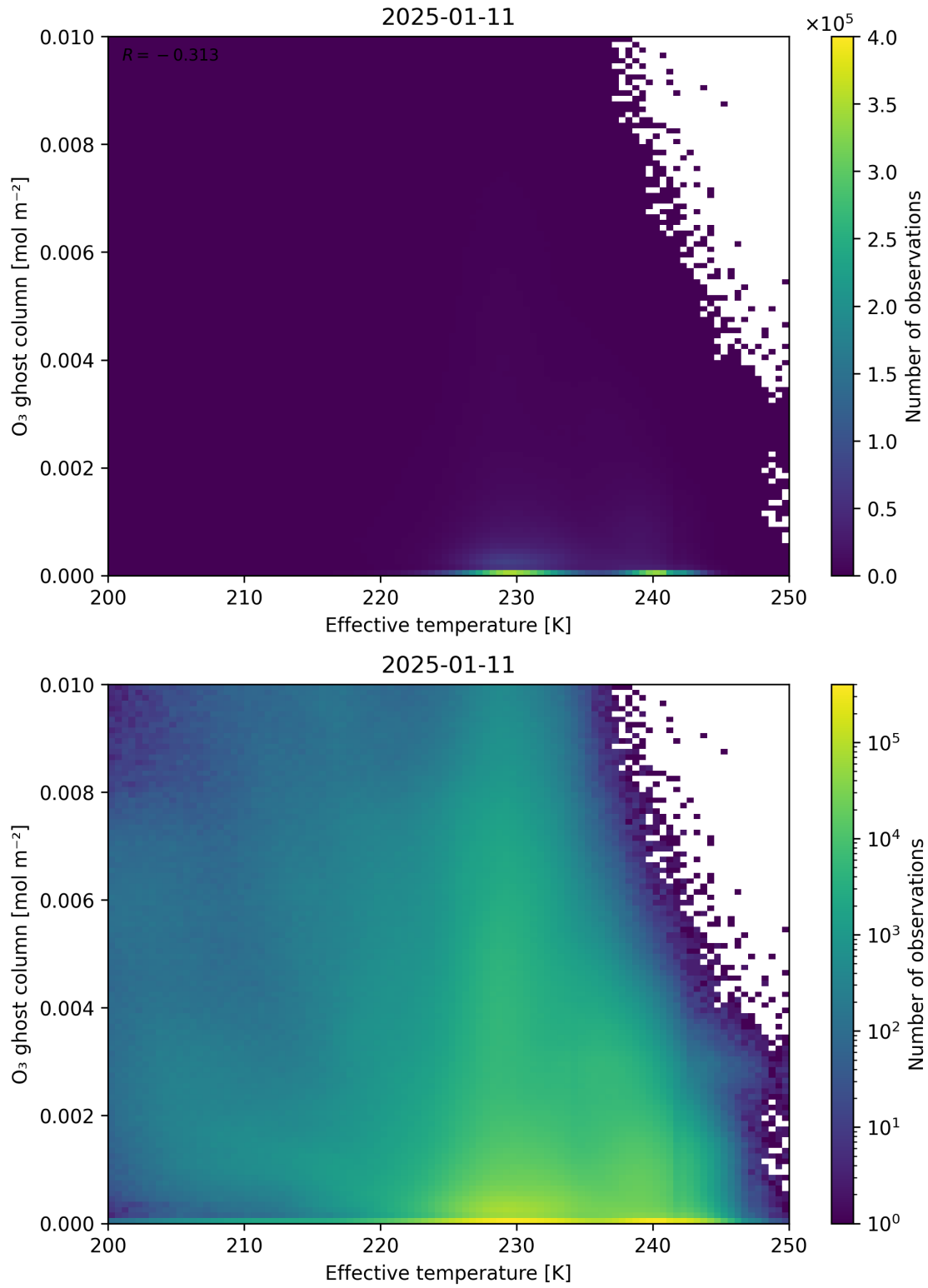
Figure 38: Scatter density plot of “Effective temperature” against “O 3 ghost column” for 2025-01-10 to 2025-01-12.
