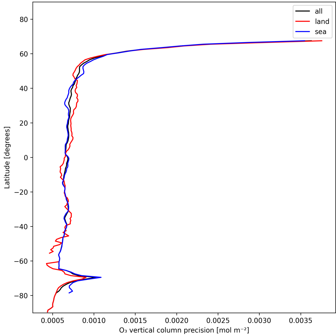
Figure 15: Zonal average of “O 3 vertical column precision” for 2025-01-10 to 2025-01-12.
