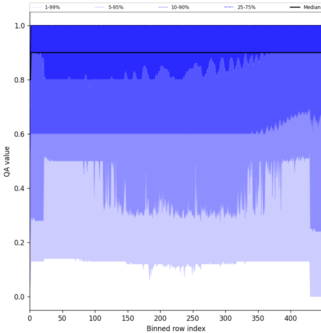
Figure 27: Along track statistics of “QA value” for 2025-01-10 to 2025-01-12
