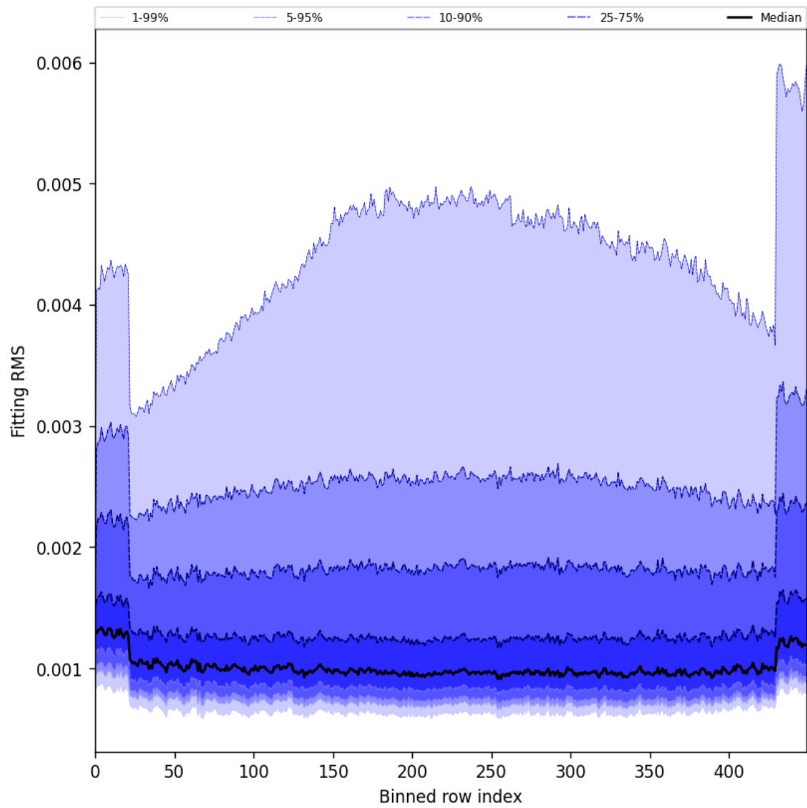
Figure 30: Along track statistics of “Fitting RMS” for 2025-01-10 to 2025-01-12
