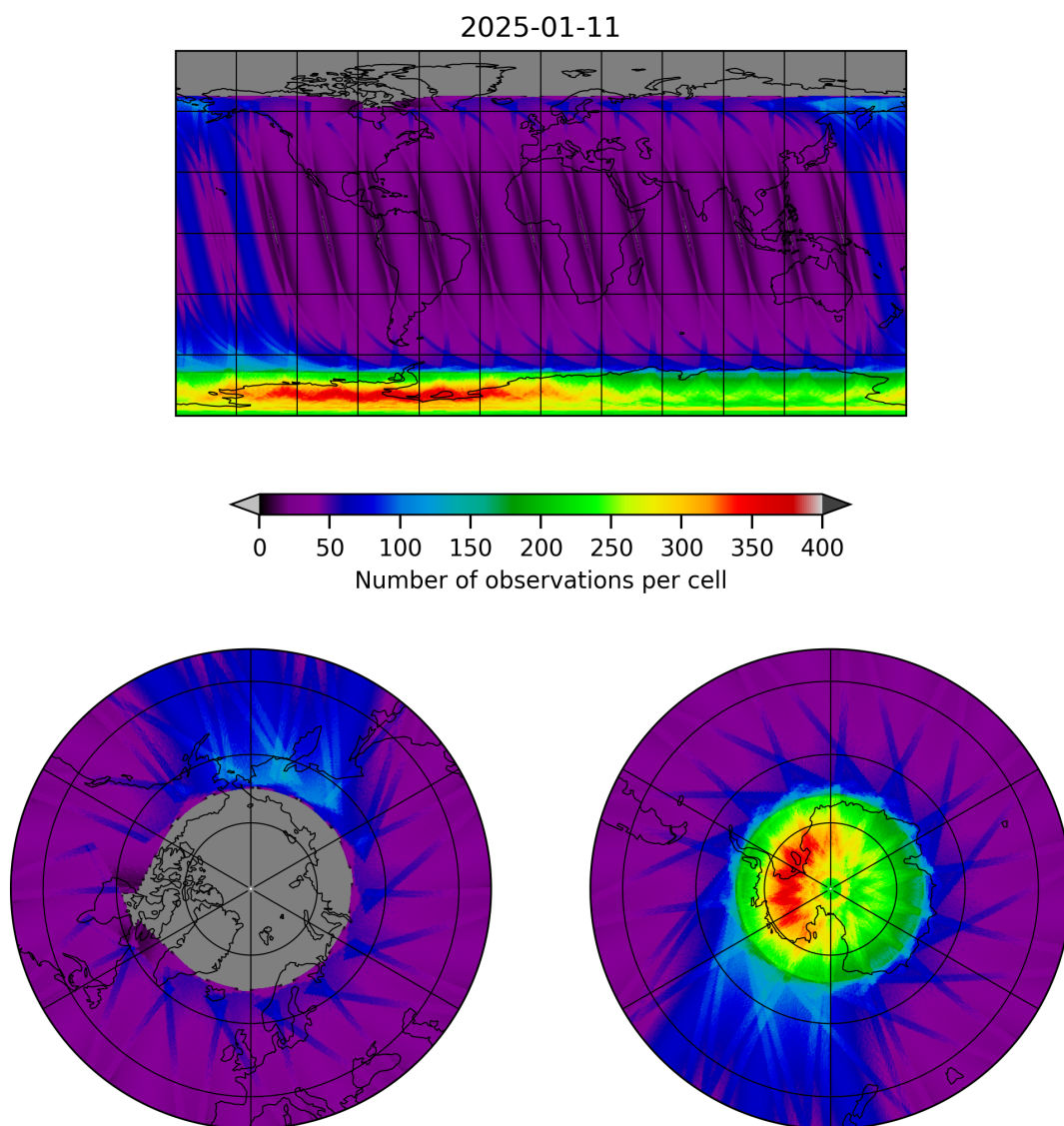
Figure 12: Map of the number of observations for 2025-01-10 to 2025-01-12
