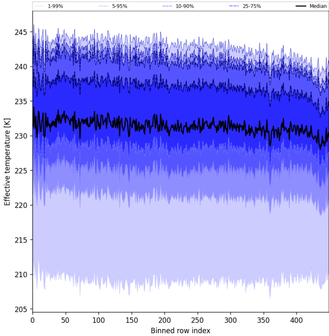
Figure 31: Along track statistics of “Effective temperature” for 2025-01-10 to 2025-01-12
