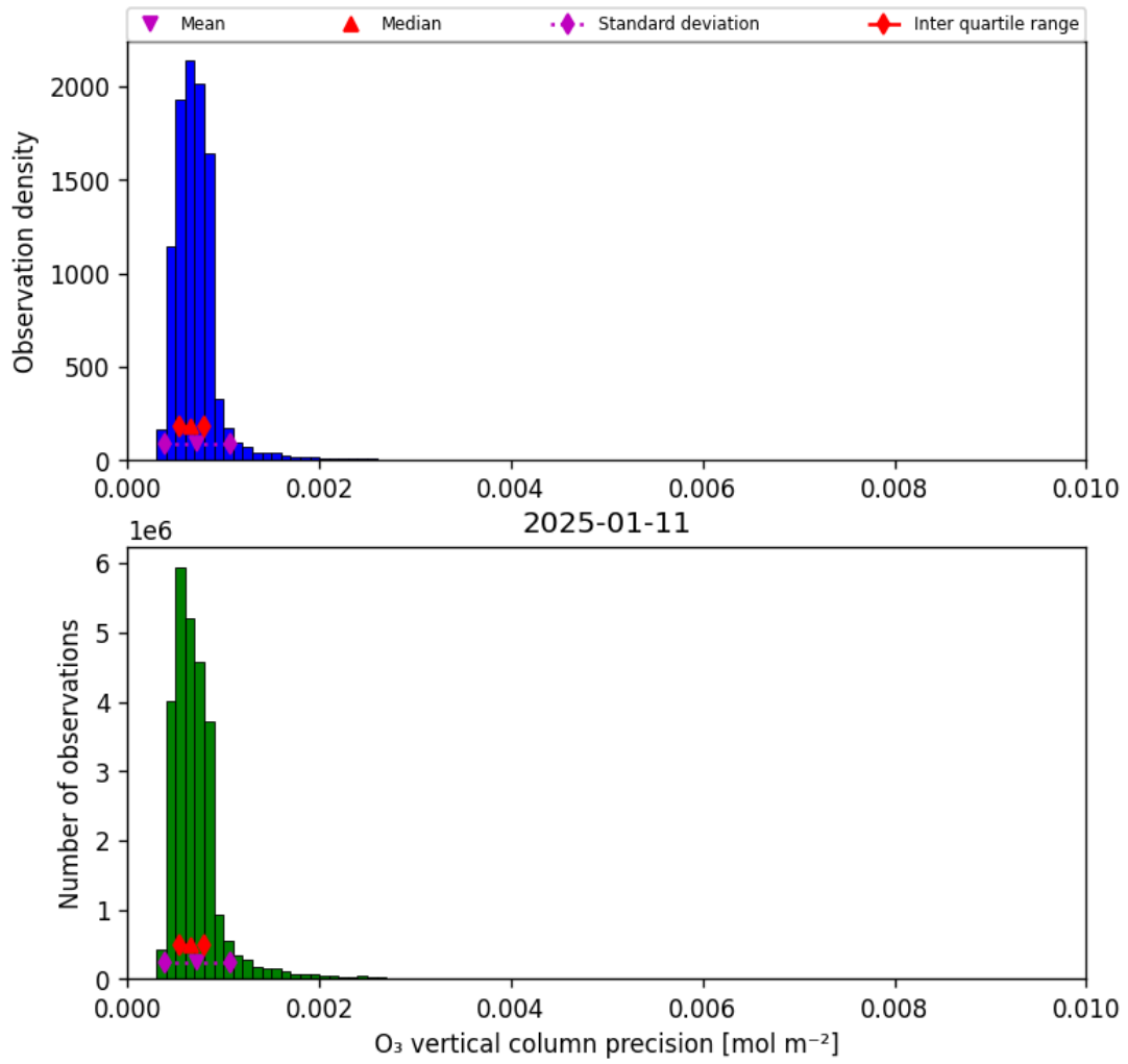
Figure 22: Histogram of “O 3 vertical column precision” for 2025-01-10 to 2025-01-12
