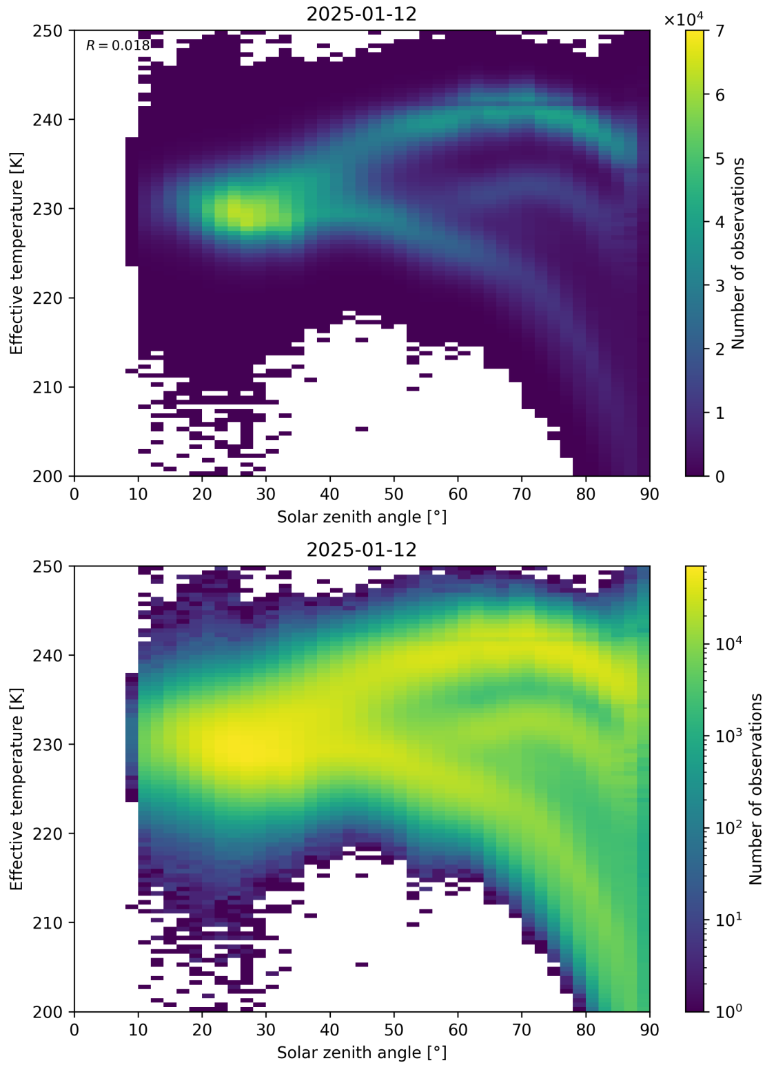
Figure 45: Scatter density plot of “Solar zenith angle” against “Effective temperature” for 2025-01-12 to 2025-01-13.
