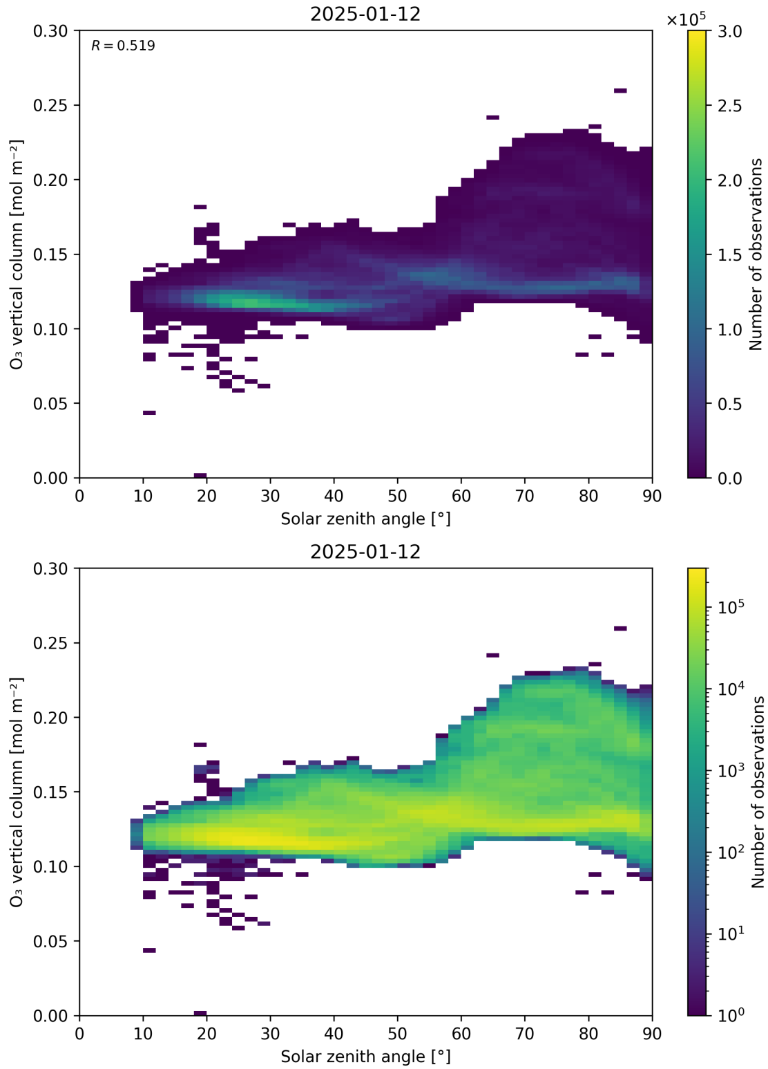
Figure 47: Scatter density plot of “Solar zenith angle” against “O 3 vertical column” for 2025-01-12 to 2025-01-13.
