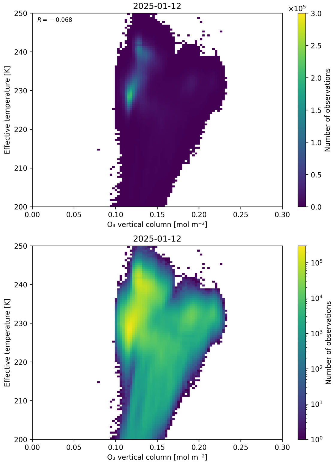
Figure 39: Scatter density plot of “O 3 vertical column” against “Effective temperature” for 2025-01-12 to 2025-01-13.
