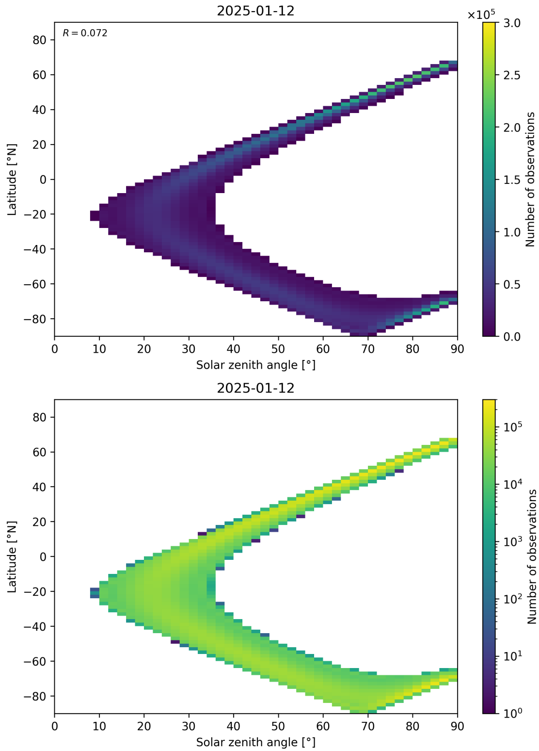
Figure 44: Scatter density plot of “Solar zenith angle” against “Latitude” for 2025-01-12 to 2025-01-13.
