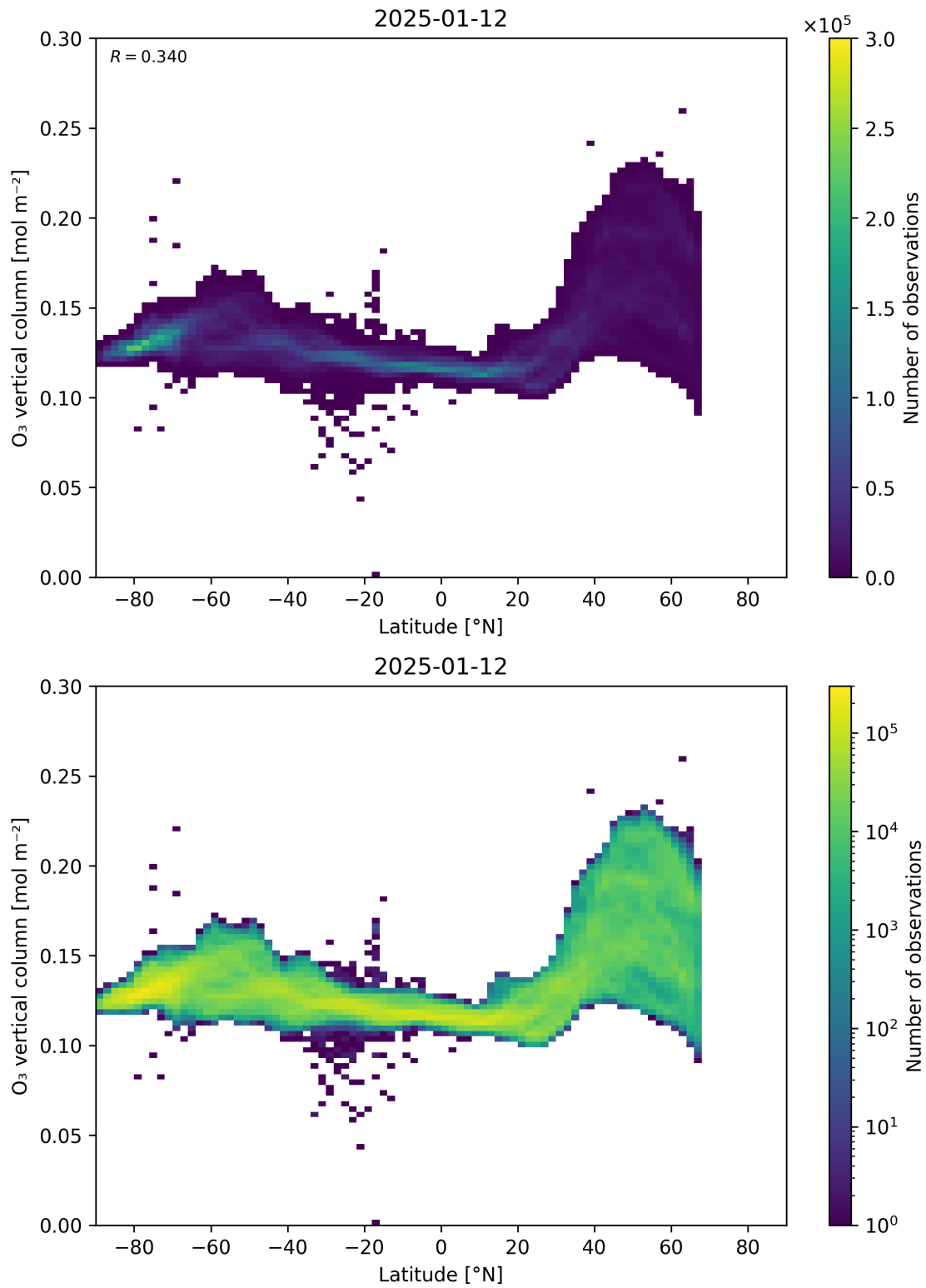
Figure 36: Scatter density plot of “Latitude” against “O 3 vertical column” for 2025-01-12 to 2025-01-13.
