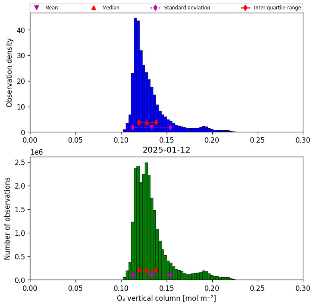
Figure 21: Histogram of “O 3 vertical column” for 2025-01-12 to 2025-01-13
