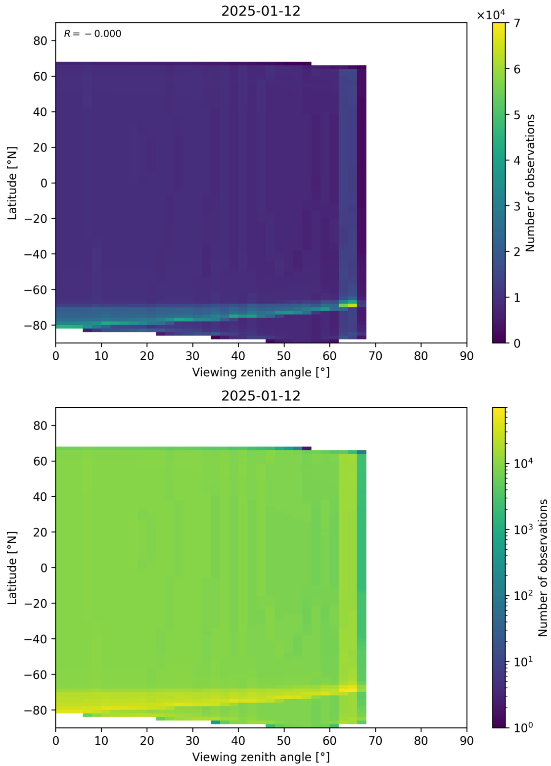
Figure 49: Scatter density plot of “Viewing zenith angle” against “Latitude” for 2025-01-12 to 2025-01-13.
