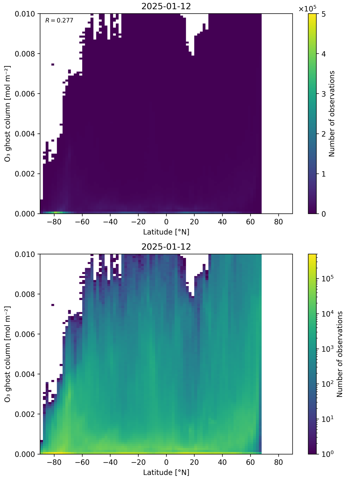
Figure 35: Scatter density plot of “Latitude” against “O 3 ghost column” for 2025-01-12 to 2025-01-13.
