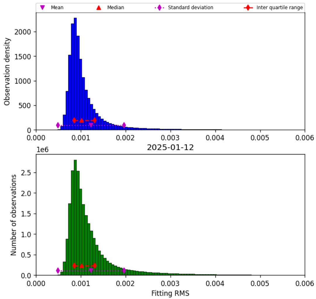
Figure 23: Histogram of “Fitting RMS” for 2025-01-12 to 2025-01-13
