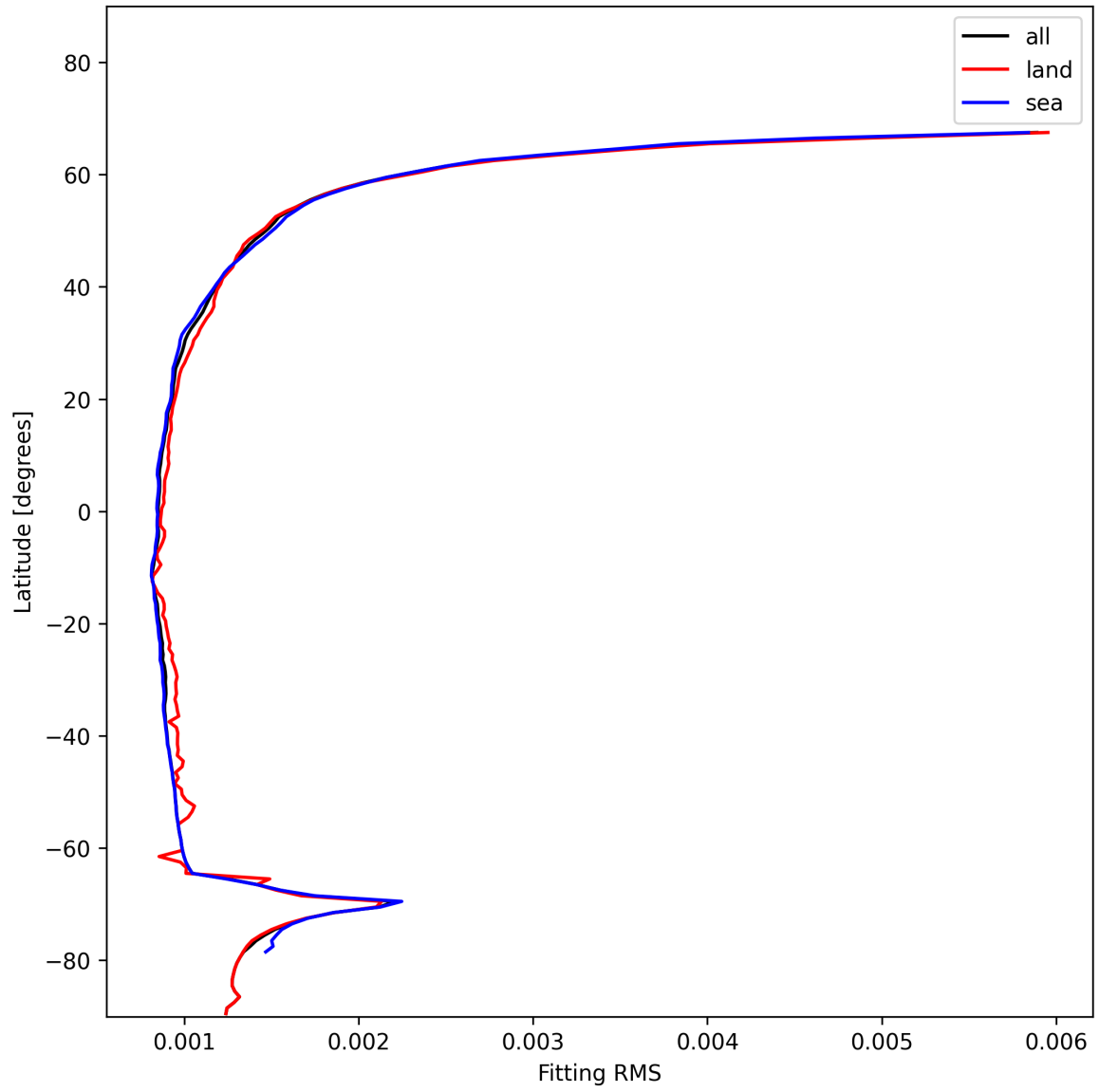
Figure 16: Zonal average of “Fitting RMS” for 2025-01-12 to 2025-01-13.
