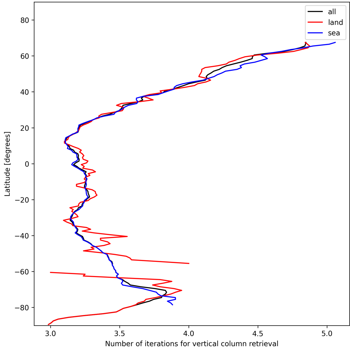
Figure 19: Zonal average of “Number of iterations for vertical column retrieval” for 2025-01-12 to 2025-01-13.
