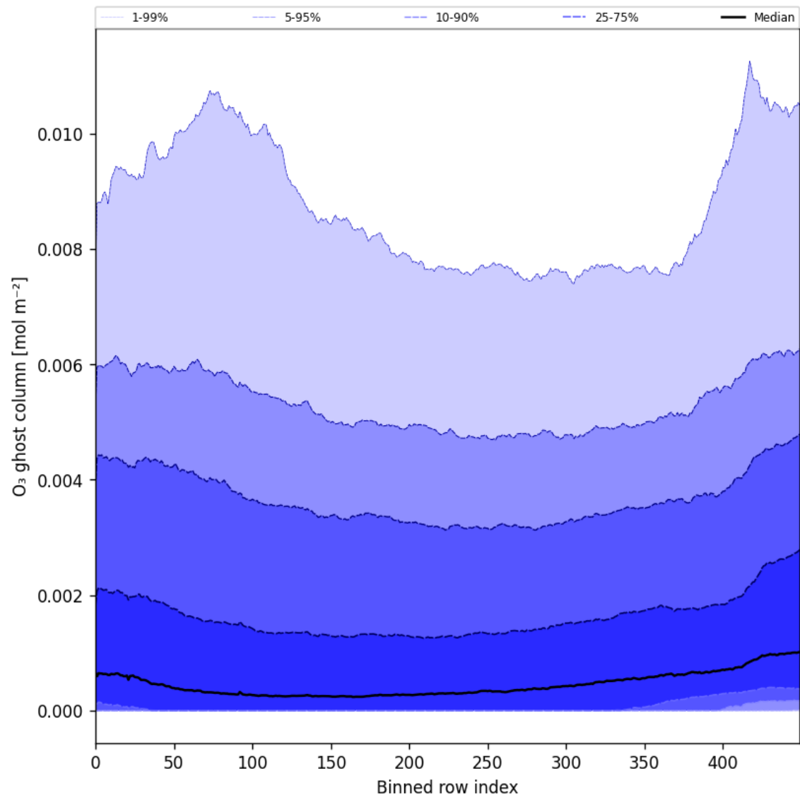
Figure 32: Along track statistics of “O 3 ghost column” for 2025-01-12 to 2025-01-13
