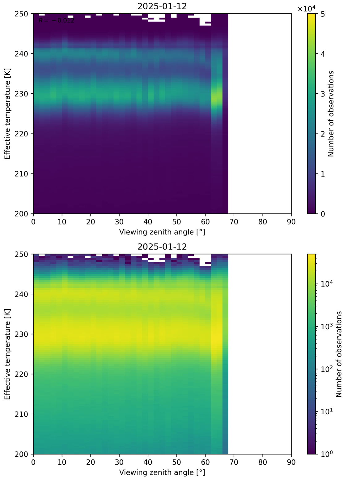
Figure 50: Scatter density plot of “Viewing zenith angle” against “Effective temperature” for 2025-01-12 to 2025-01-13.
