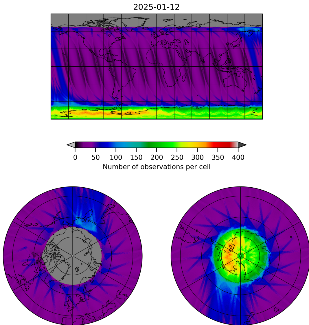
Figure 12: Map of the number of observations for 2025-01-12 to 2025-01-13
