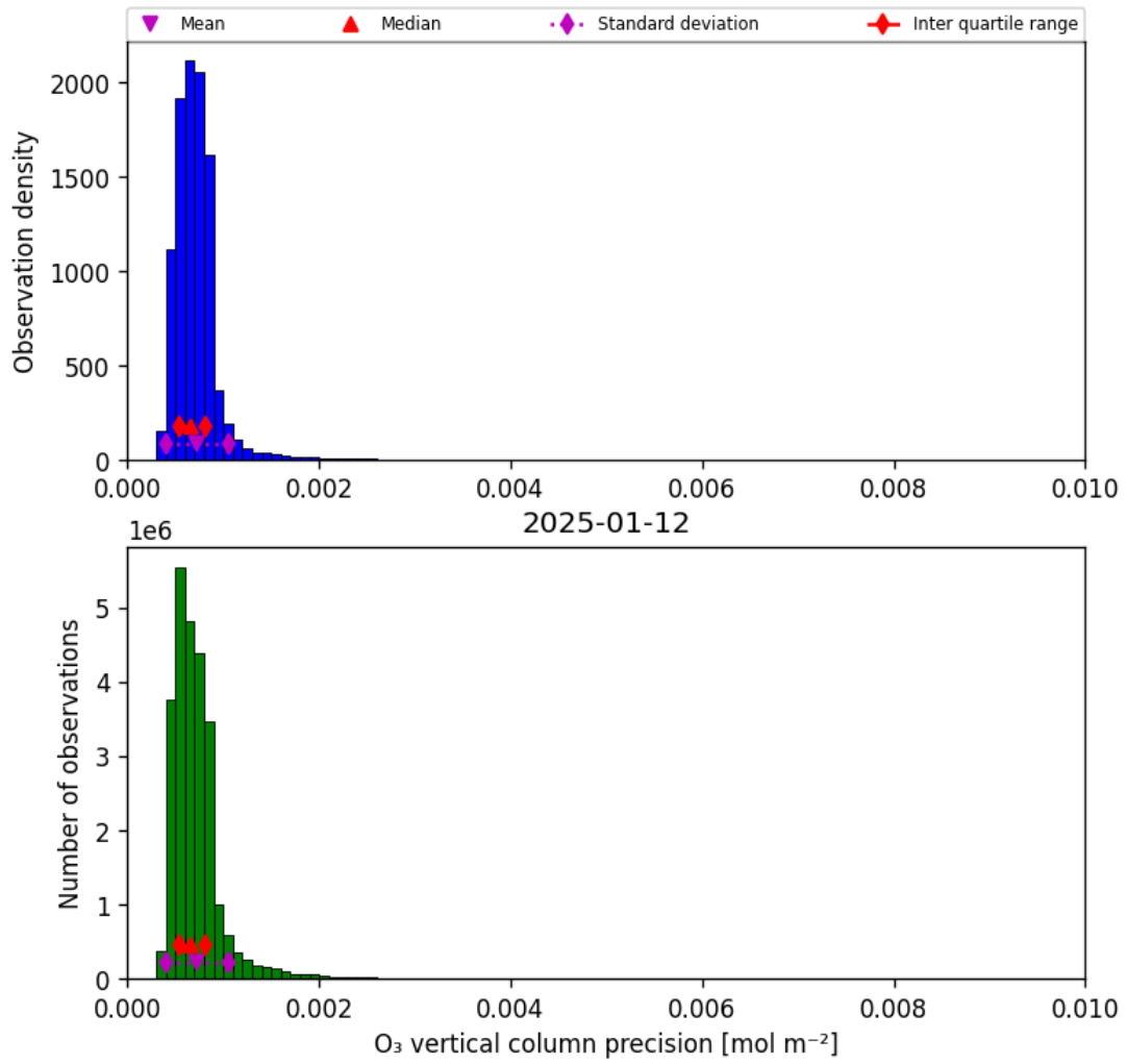
Figure 22: Histogram of “O 3 vertical column precision” for 2025-01-12 to 2025-01-13
