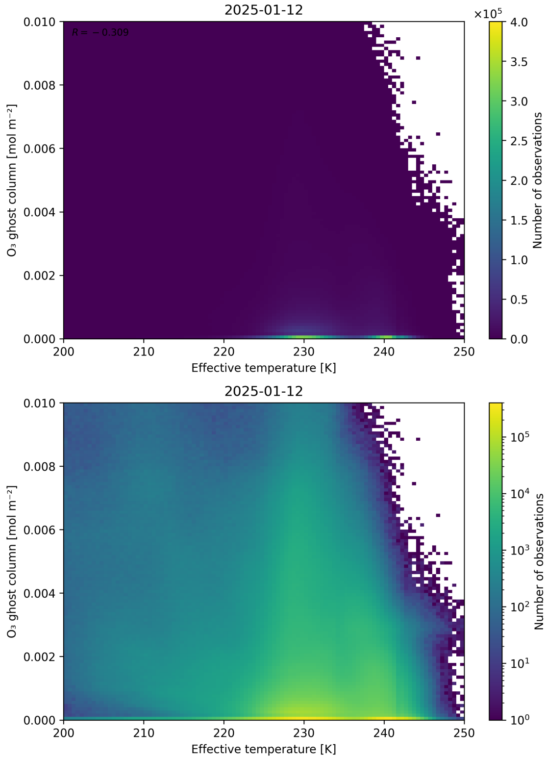
Figure 38: Scatter density plot of “Effective temperature” against “O 3 ghost column” for 2025-01-12 to 2025-01-13.
