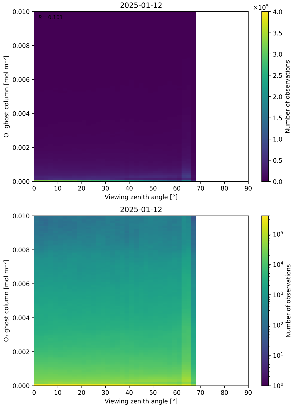
Figure 51: Scatter density plot of “Viewing zenith angle” against “O 3 ghost column” for 2025-01-12 to 2025-01-13.
