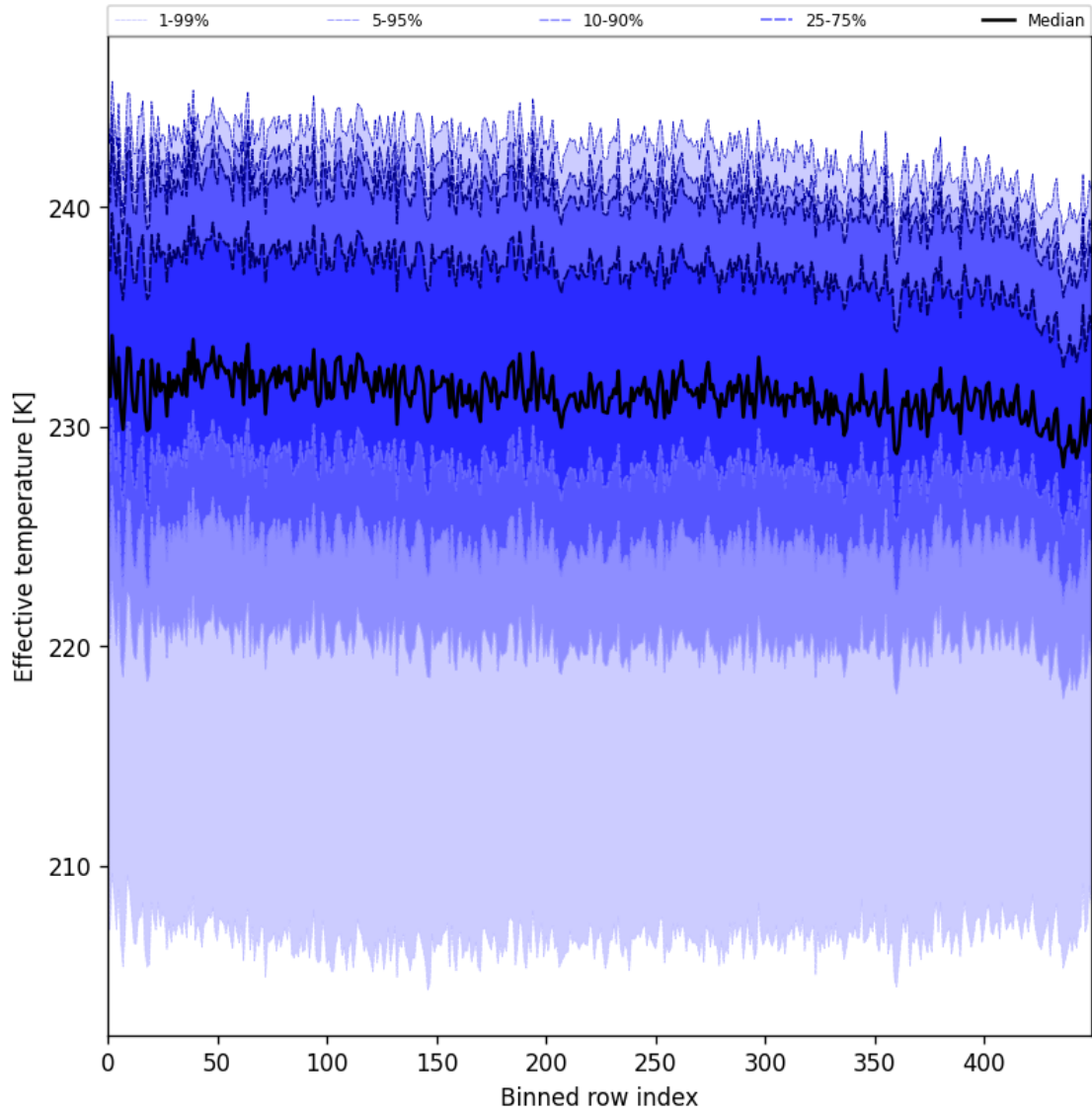
Figure 31: Along track statistics of “Effective temperature” for 2025-01-12 to 2025-01-13
