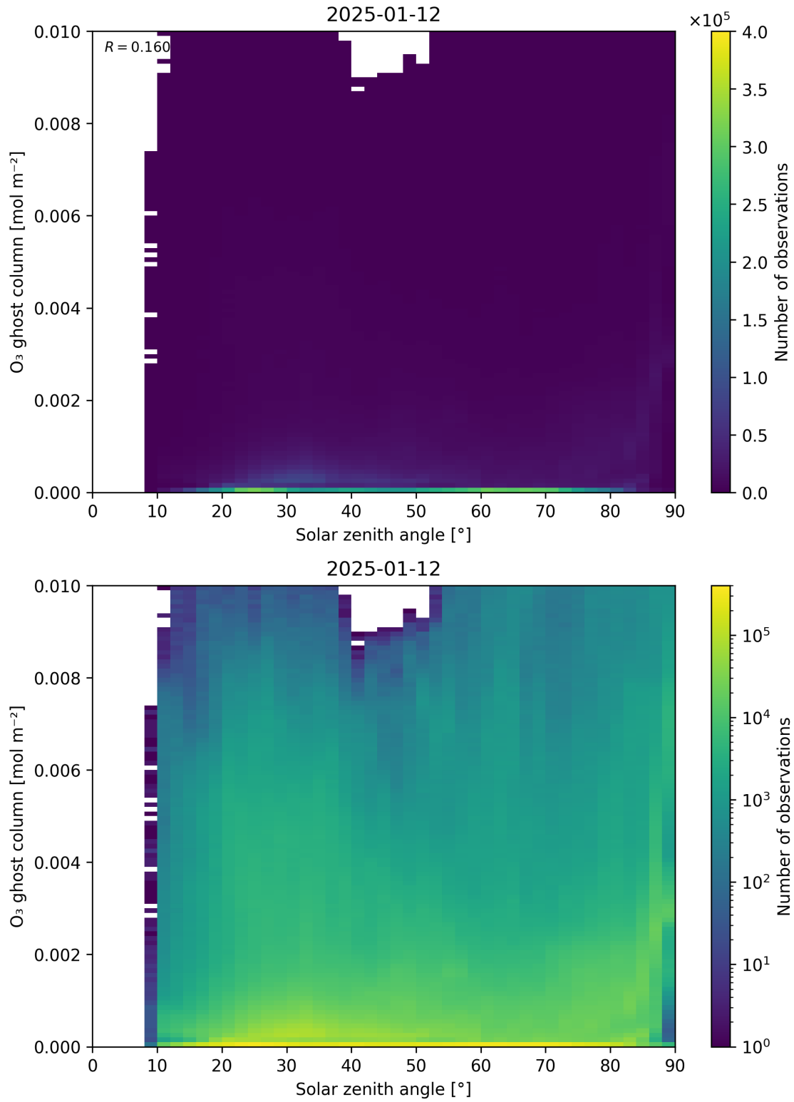
Figure 46: Scatter density plot of “Solar zenith angle” against “O 3 ghost column” for 2025-01-12 to 2025-01-13.
