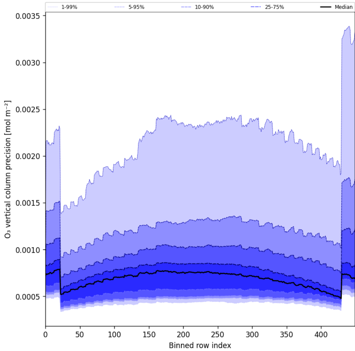
Figure 29: Along track statistics of “O 3 vertical column precision” for 2025-01-12 to 2025-01-13
