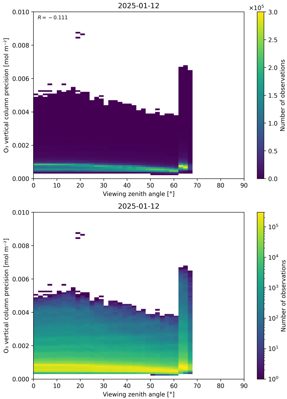
Figure 53: Scatter density plot of “Viewing zenith angle” against “O 3 vertical column precision” for 2025-01-12 to 2025-01-13.
