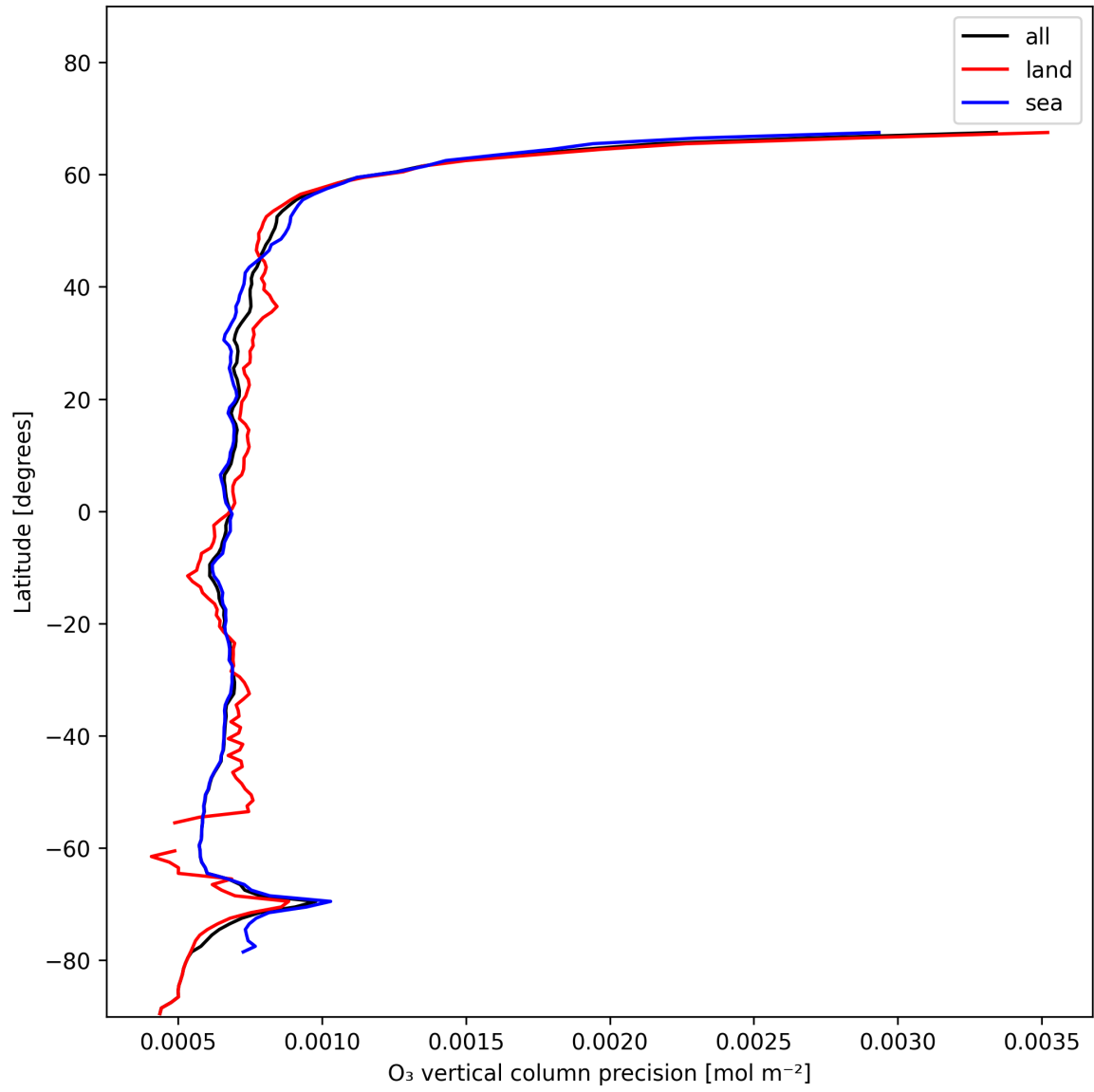
Figure 15: Zonal average of “O 3 vertical column precision” for 2025-01-12 to 2025-01-13.
