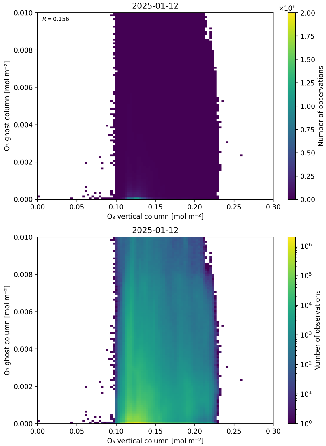
Figure 40: Scatter density plot of “O 3 vertical column” against “O 3 ghost column” for 2025-01-12 to 2025-01-13.
