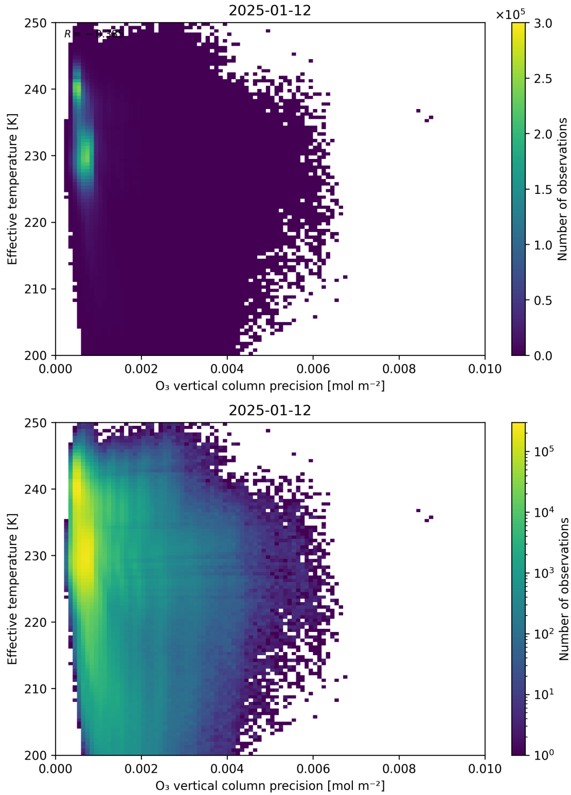
Figure 42: Scatter density plot of “O 3 vertical column precision” against “Effective temperature” for 2025-01-12 to 2025-01-13.
