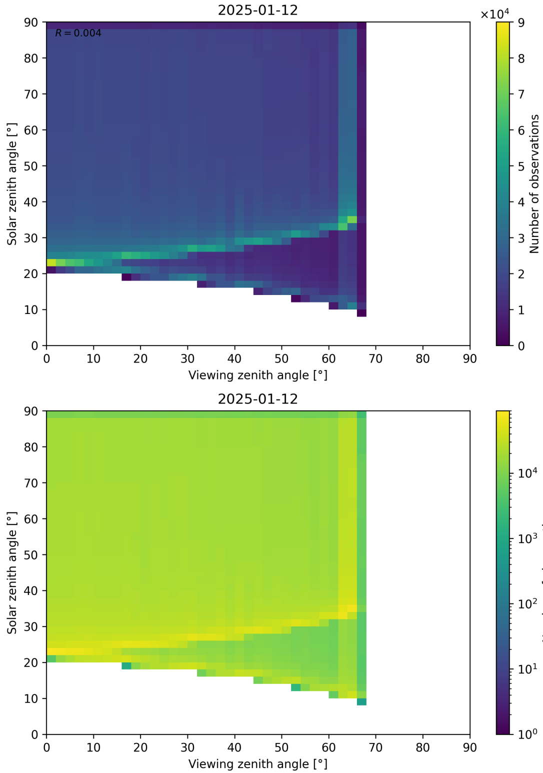
Figure 54: Scatter density plot of “Viewing zenith angle” against “Solar zenith angle” for 2025-01-12 to 2025-01-13.
