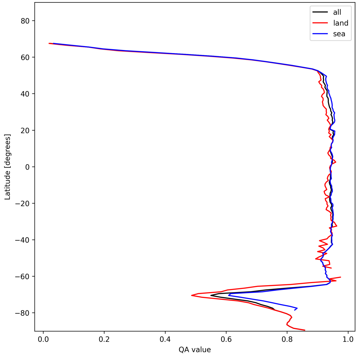
Figure 13: Zonal average of “QA value” for 2025-01-12 to 2025-01-13.
