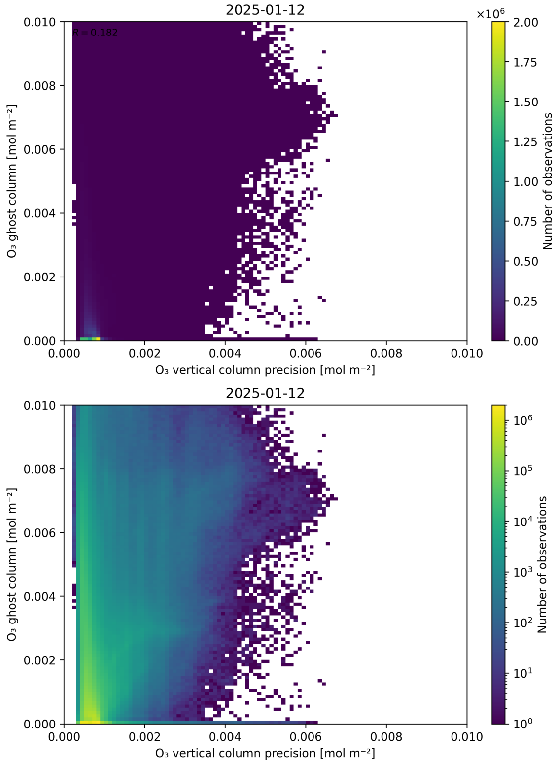
Figure 43: Scatter density plot of “ \text{O}_3 vertical column precision” against “ \text{O}_3 ghost column” for 2025-01-12 to 2025-01-13.
