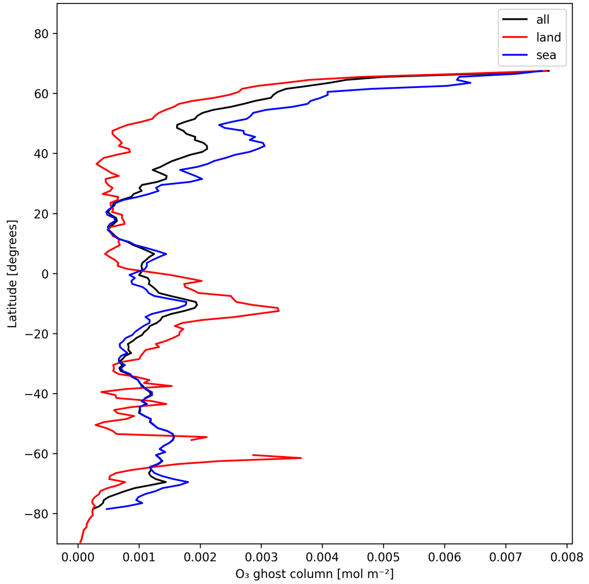
Figure 18: Zonal average of "O 3 ghost column" for 2025-01-12 to 2025-01-13.
