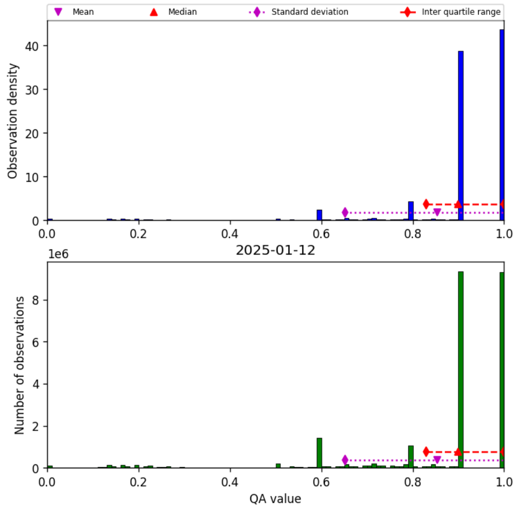
Figure 20: Histogram of “QA value” for 2025-01-12 to 2025-01-13
