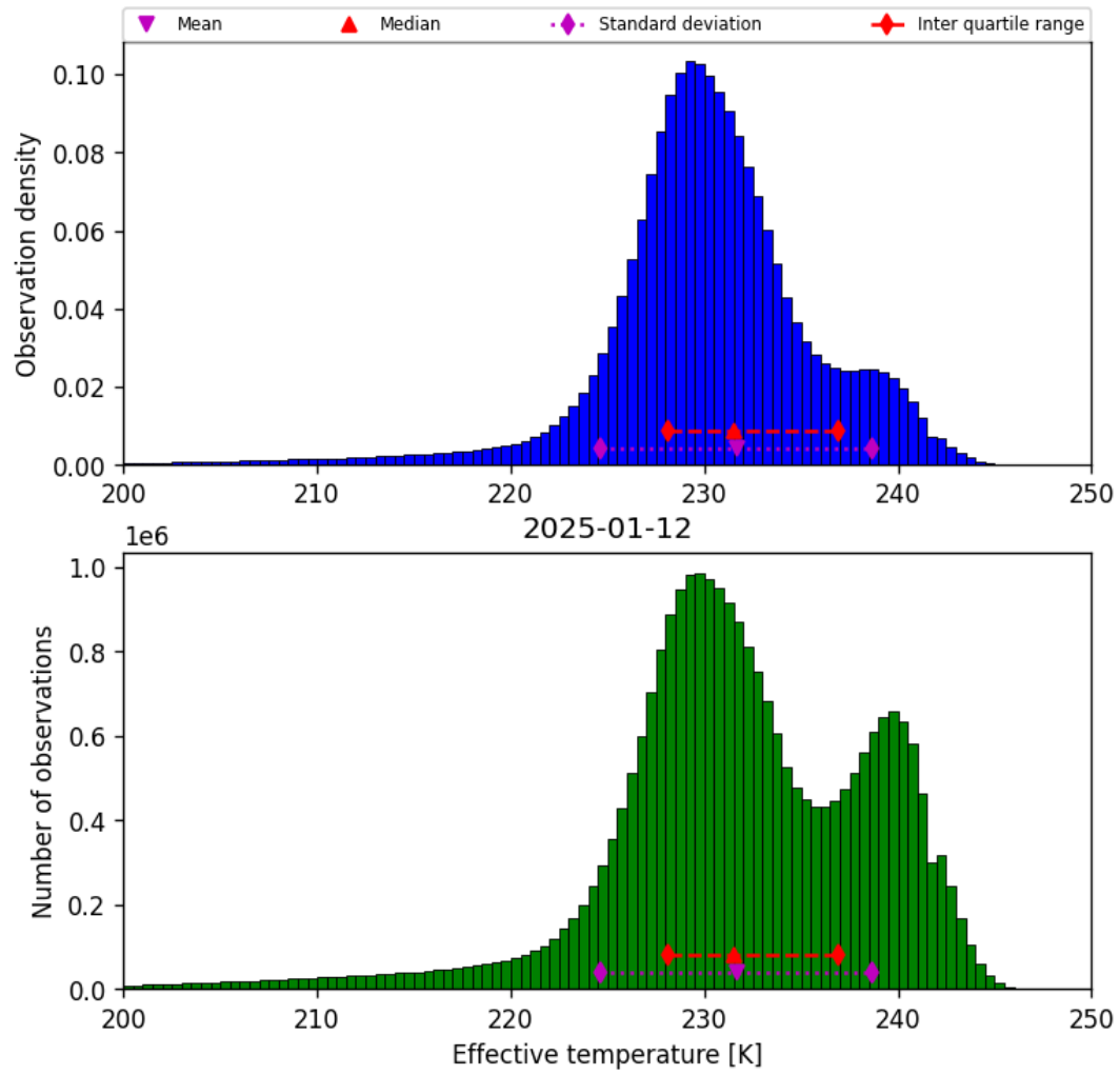
Figure 24: Histogram of “Effective temperature” for 2025-01-12 to 2025-01-13
