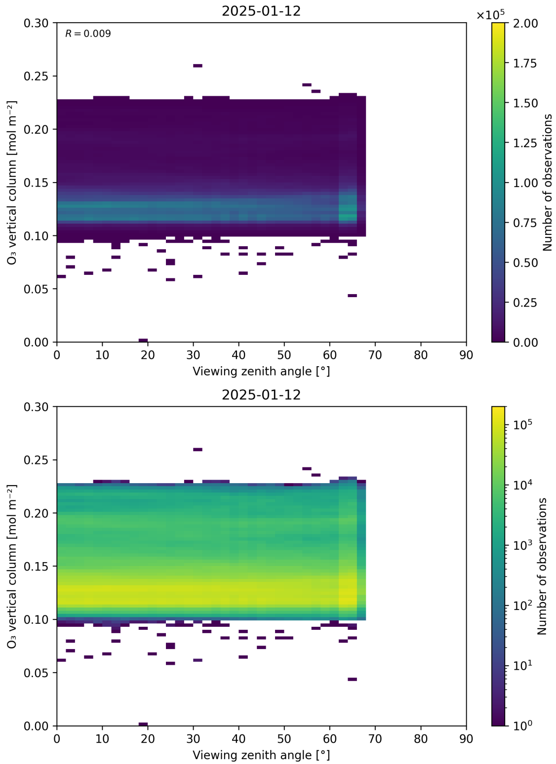
Figure 52: Scatter density plot of “Viewing zenith angle” against “O 3 vertical column” for 2025-01-12 to 2025-01-13.
