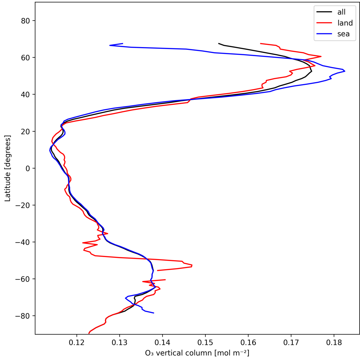
Figure 14: Zonal average of “O 3 vertical column” for 2025-01-12 to 2025-01-13.
