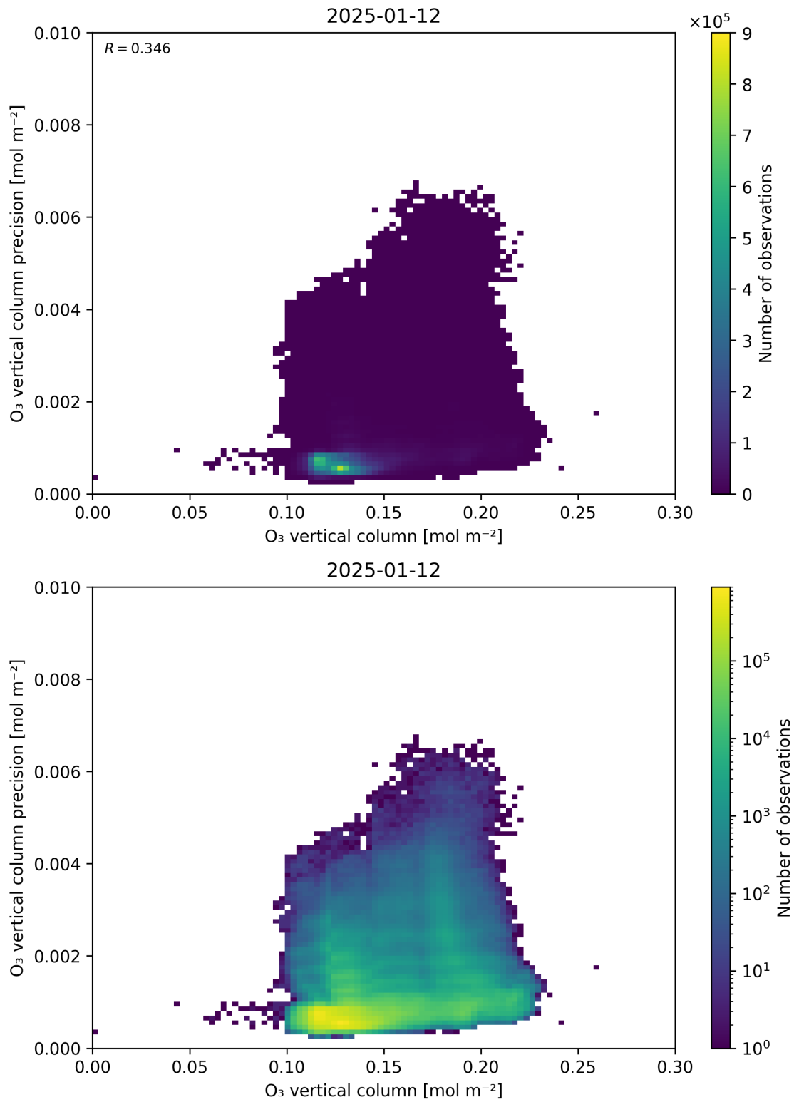
Figure 41: Scatter density plot of “O 3 vertical column” against “O 3 vertical column precision” for 2025-01-12 to 2025-01-13.
