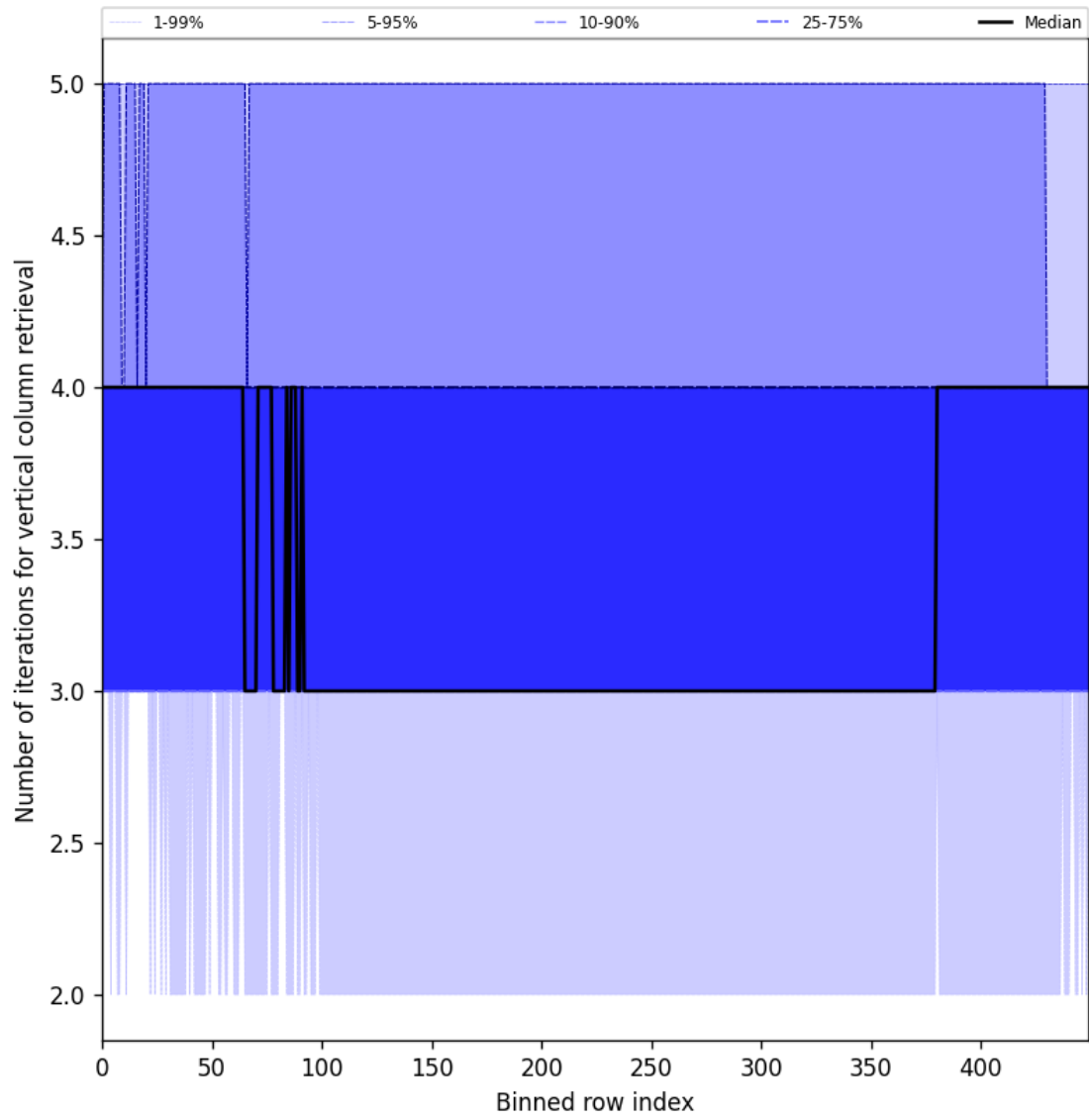
Figure 33: Along track statistics of “Number of iterations for vertical column retrieval” for 2025-01-12 to 2025-01-13
