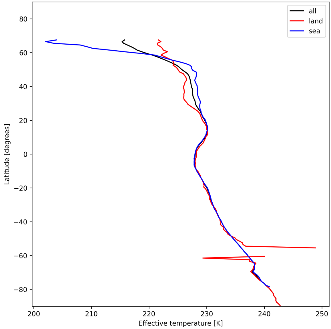
Figure 17: Zonal average of “Effective temperature” for 2025-01-12 to 2025-01-13.
