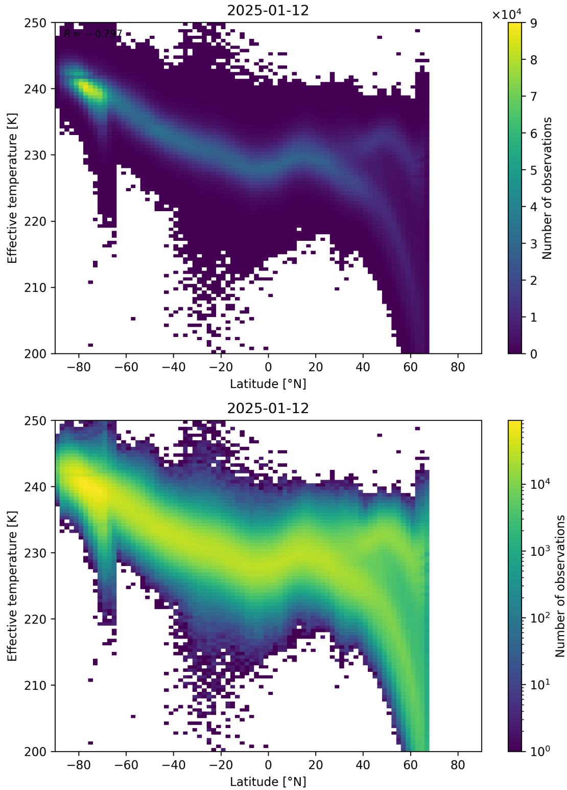
Figure 34: Scatter density plot of “Latitude” against “Effective temperature” for 2025-01-12 to 2025-01-13.
