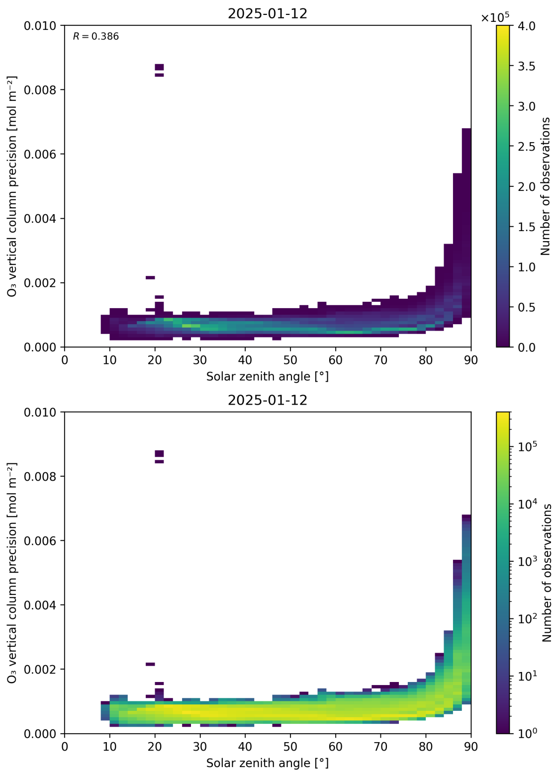
Figure 48: Scatter density plot of “Solar zenith angle” against “O 3 vertical column precision” for 2025-01-12 to 2025-01-13.
