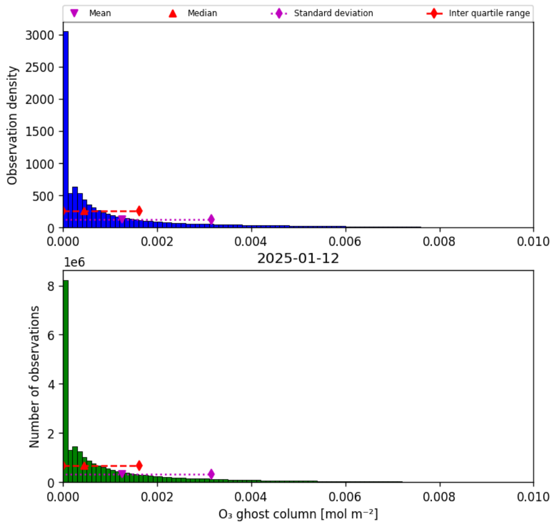
Figure 25: Histogram of “O 3 ghost column” for 2025-01-12 to 2025-01-13
