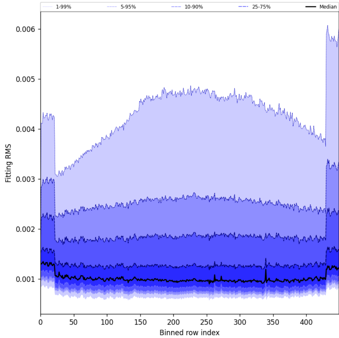
Figure 30: Along track statistics of “Fitting RMS” for 2025-01-12 to 2025-01-13
