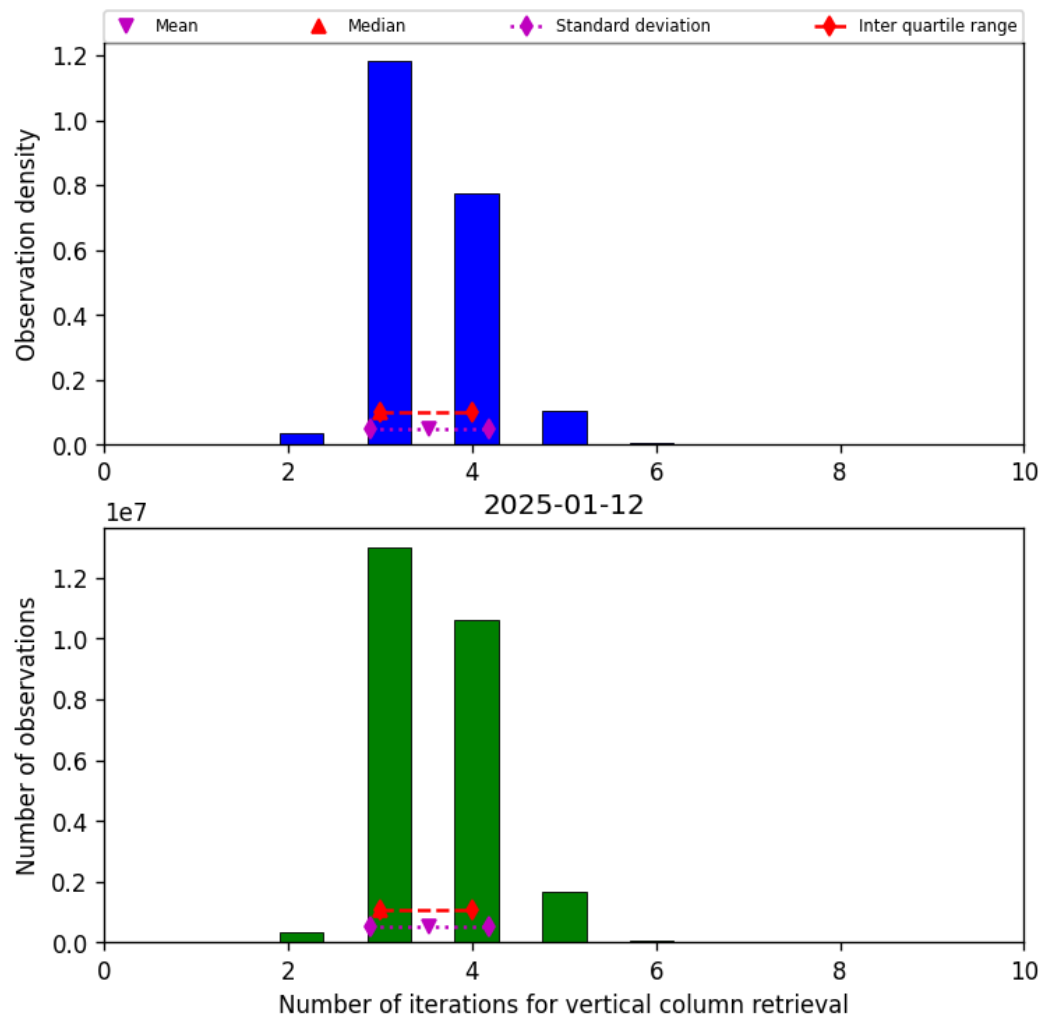
Figure 26: Histogram of “Number of iterations for vertical column retrieval” for 2025-01-12 to 2025-01-13
