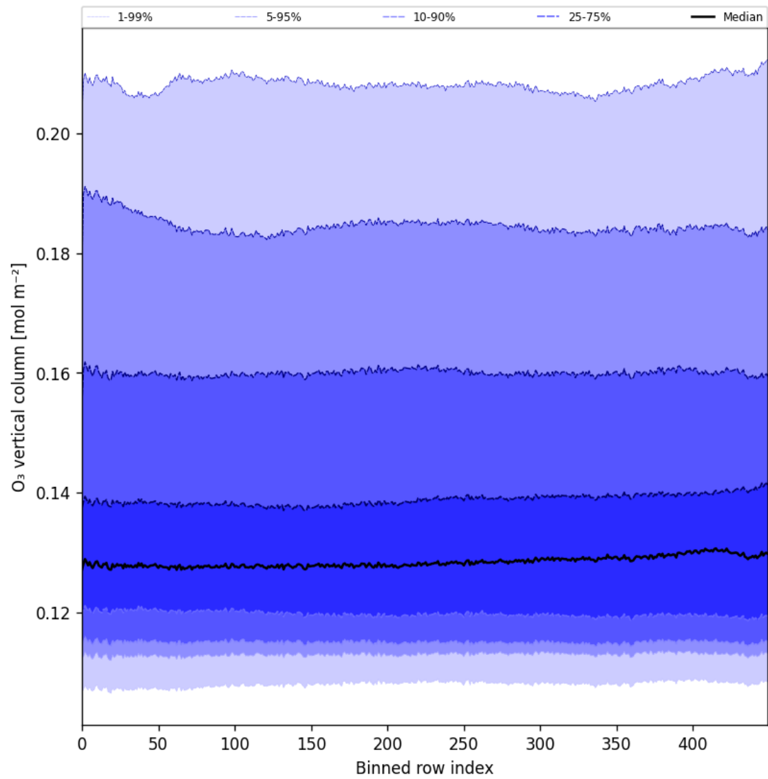
Figure 28: Along track statistics of “O 3 vertical column” for 2025-01-12 to 2025-01-13
