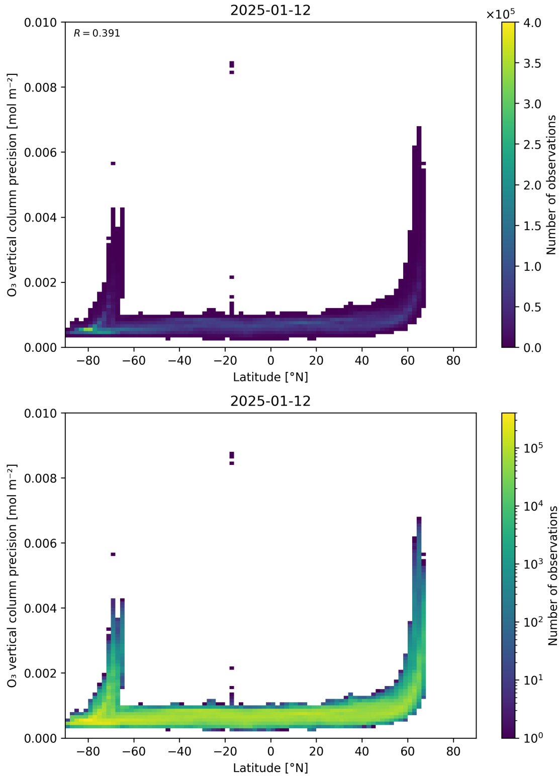
Figure 37: Scatter density plot of “Latitude” against “O 3 vertical column precision” for 2025-01-12 to 2025-01-13.
