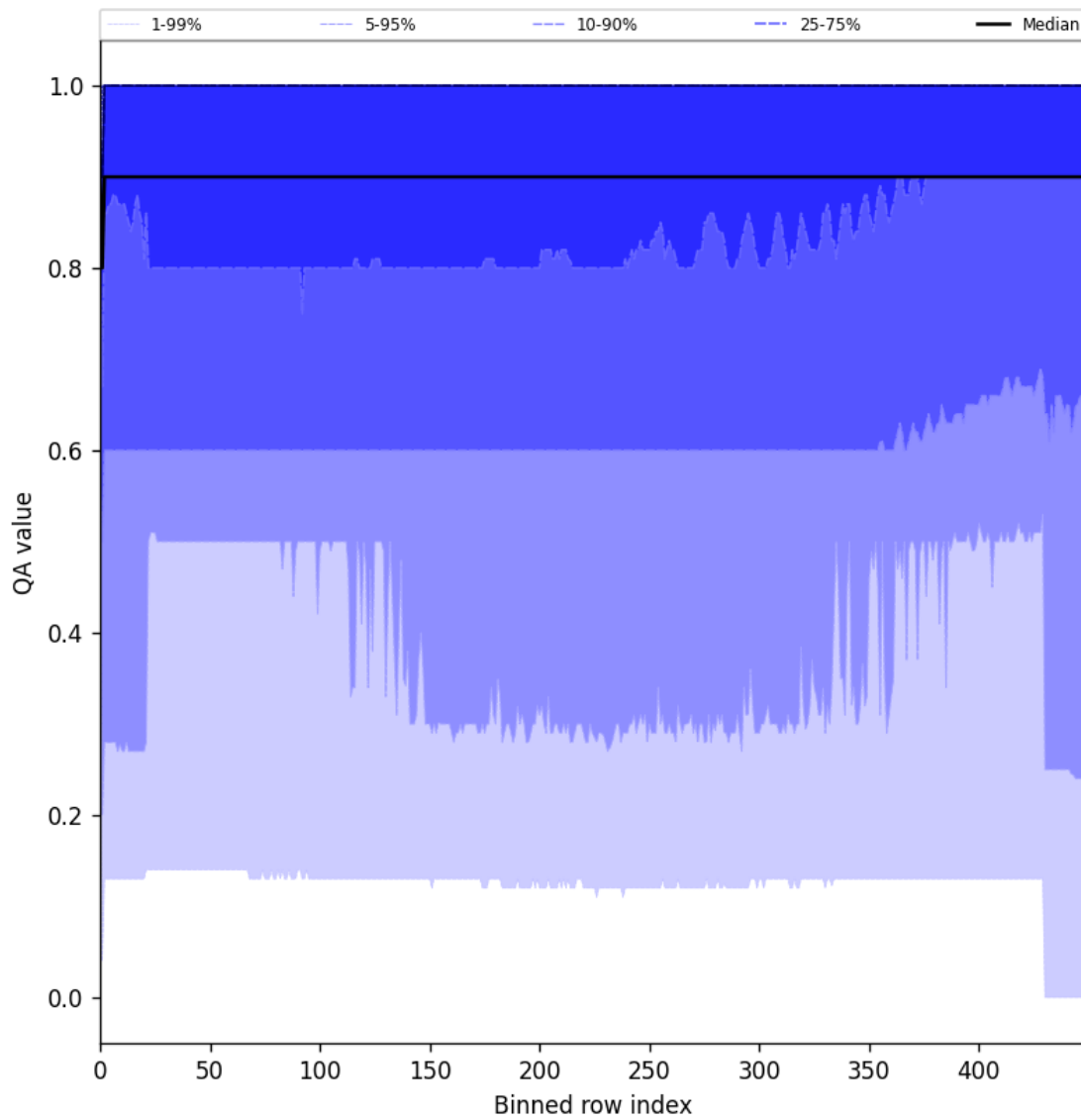
Figure 27: Along track statistics of “QA value” for 2025-01-12 to 2025-01-13
