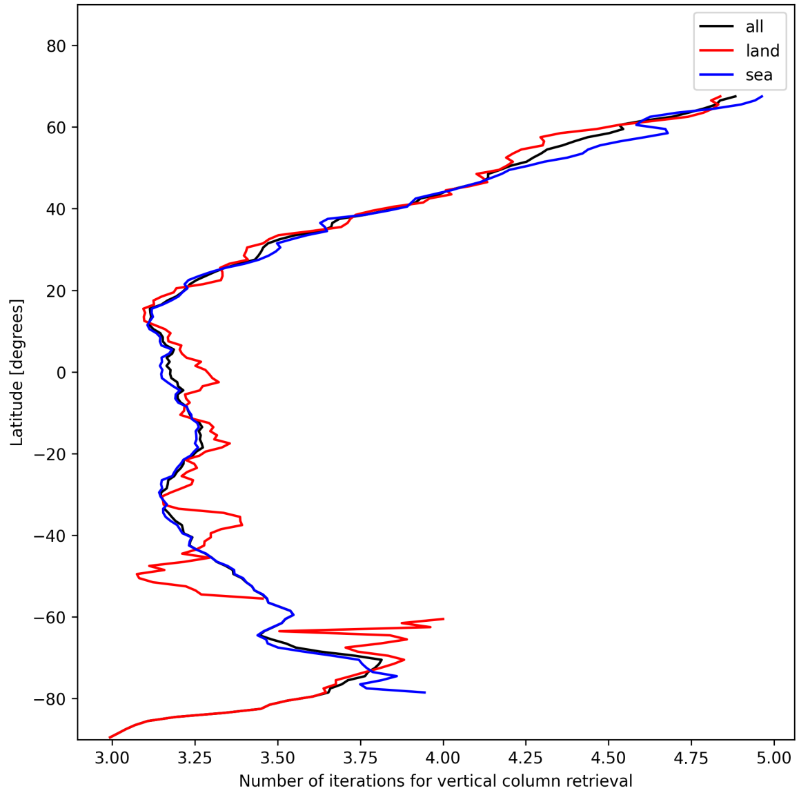
Figure 19: Zonal average of “Number of iterations for vertical column retrieval” for 2025-01-12 to 2025-01-14.
