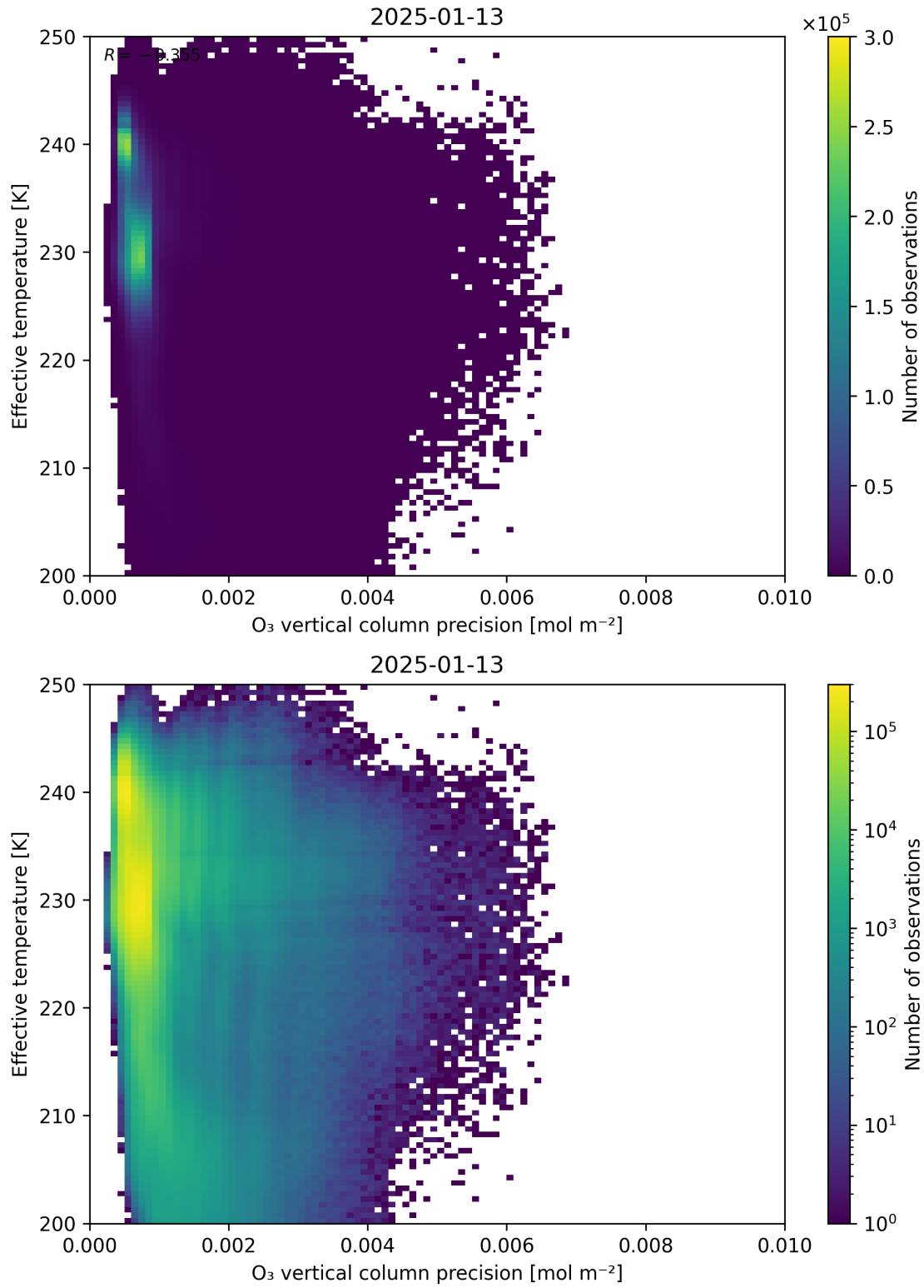
Figure 42: Scatter density plot of “O 3 vertical column precision” against “Effective temperature” for 2025-01-12 to 2025-01-14.
