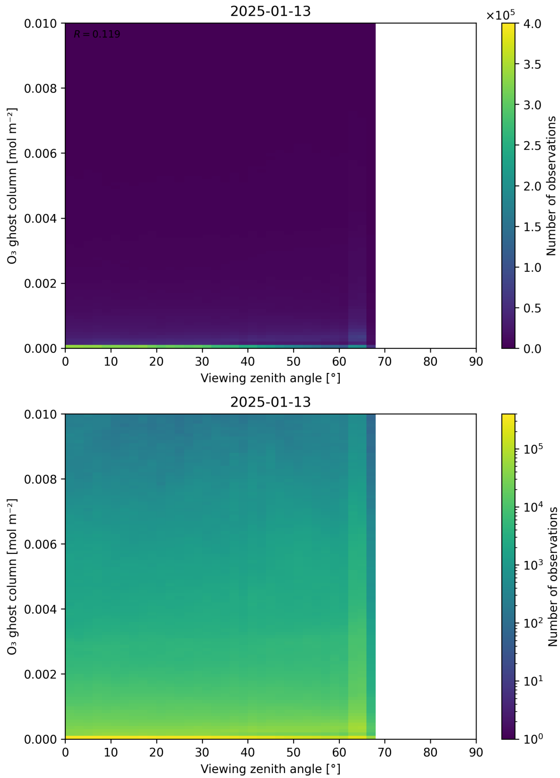
Figure 51: Scatter density plot of “Viewing zenith angle” against “O 3 ghost column” for 2025-01-12 to 2025-01-14.
