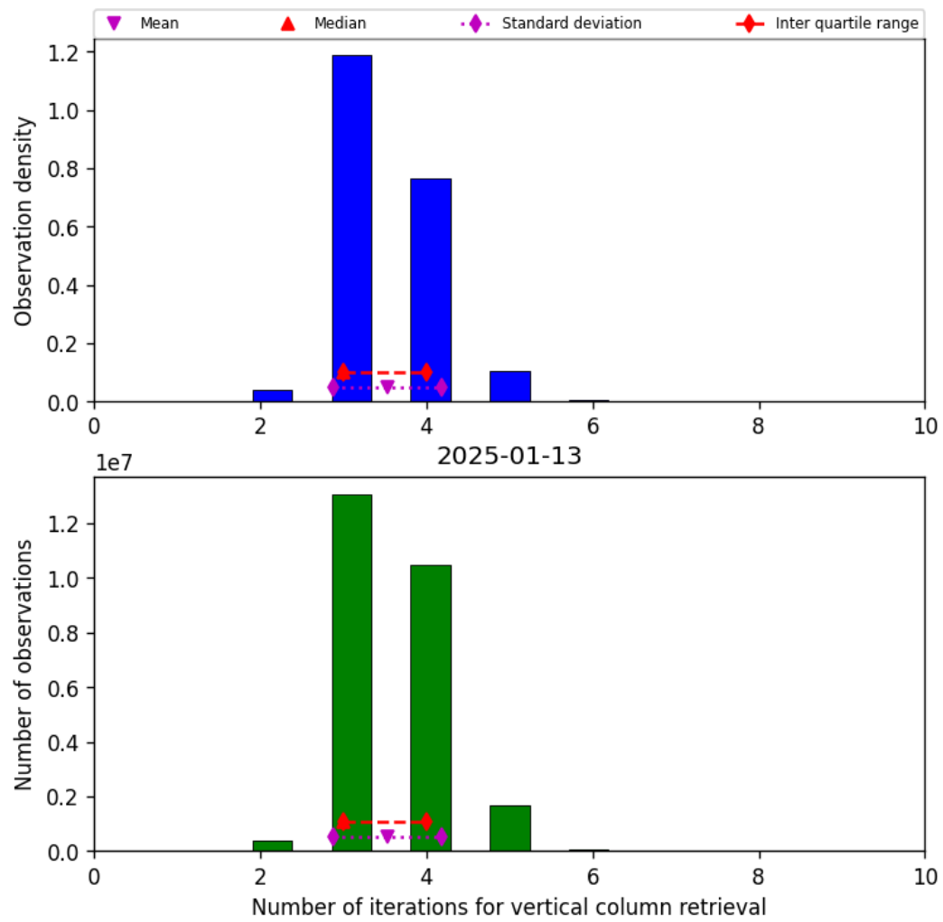
Figure 26: Histogram of “Number of iterations for vertical column retrieval” for 2025-01-12 to 2025-01-14
