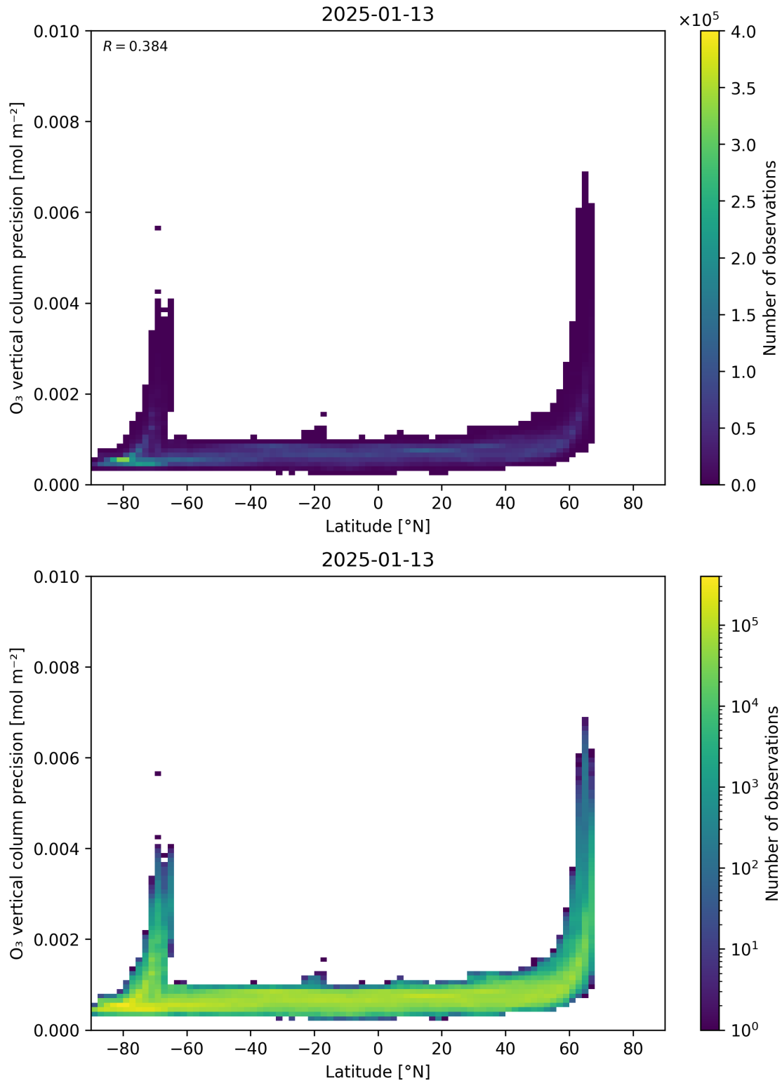
Figure 37: Scatter density plot of “Latitude” against “O 3 vertical column precision” for 2025-01-12 to 2025-01-14.
