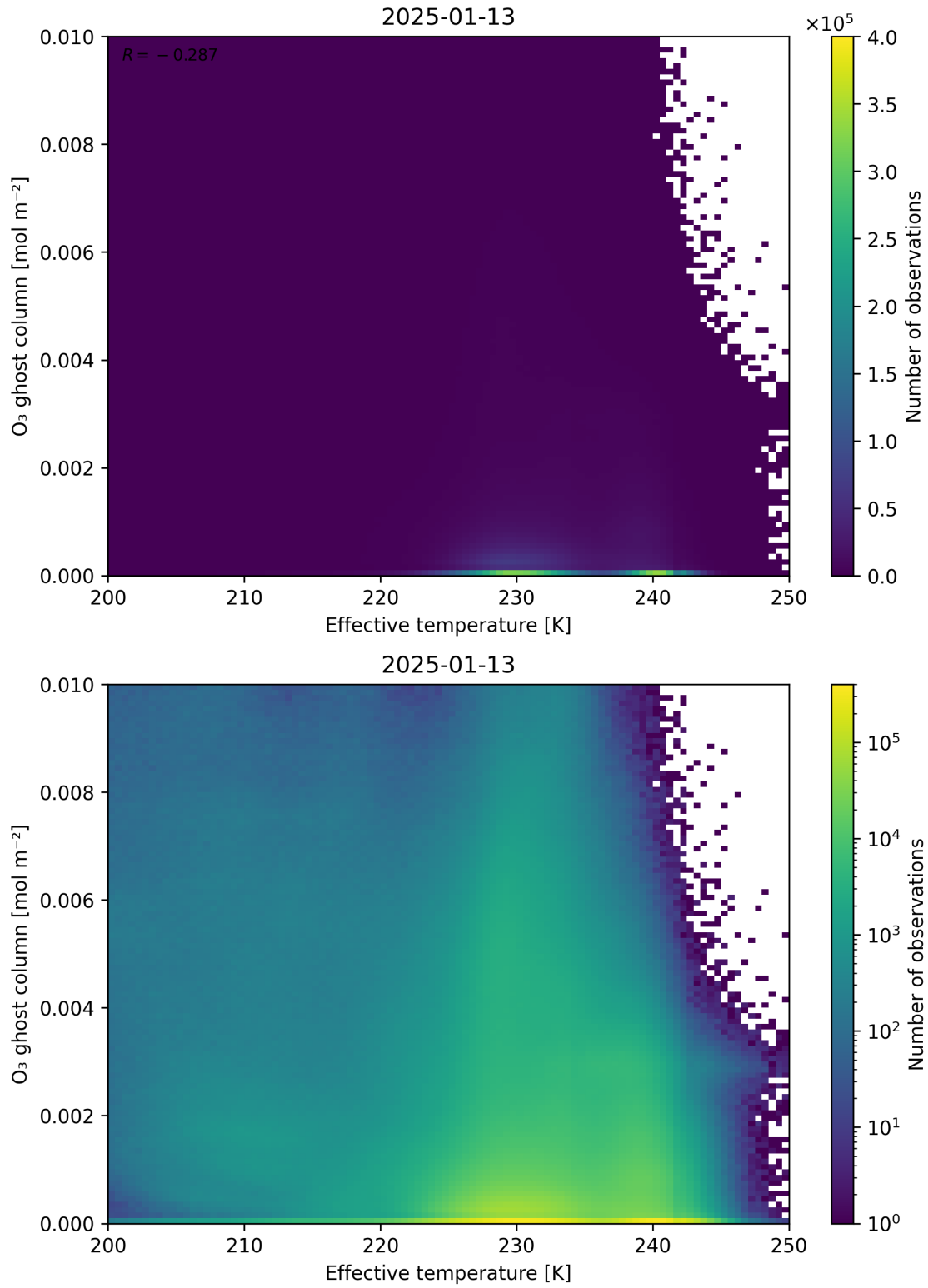
Figure 38: Scatter density plot of “Effective temperature” against “O 3 ghost column” for 2025-01-12 to 2025-01-14.
