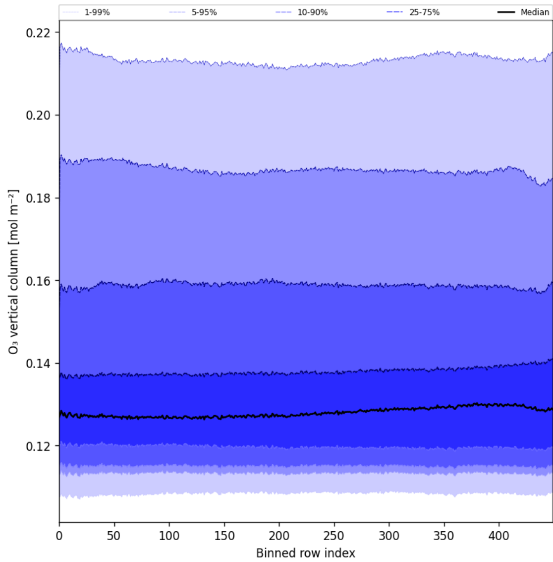
Figure 28: Along track statistics of “O 3 vertical column” for 2025-01-12 to 2025-01-14
