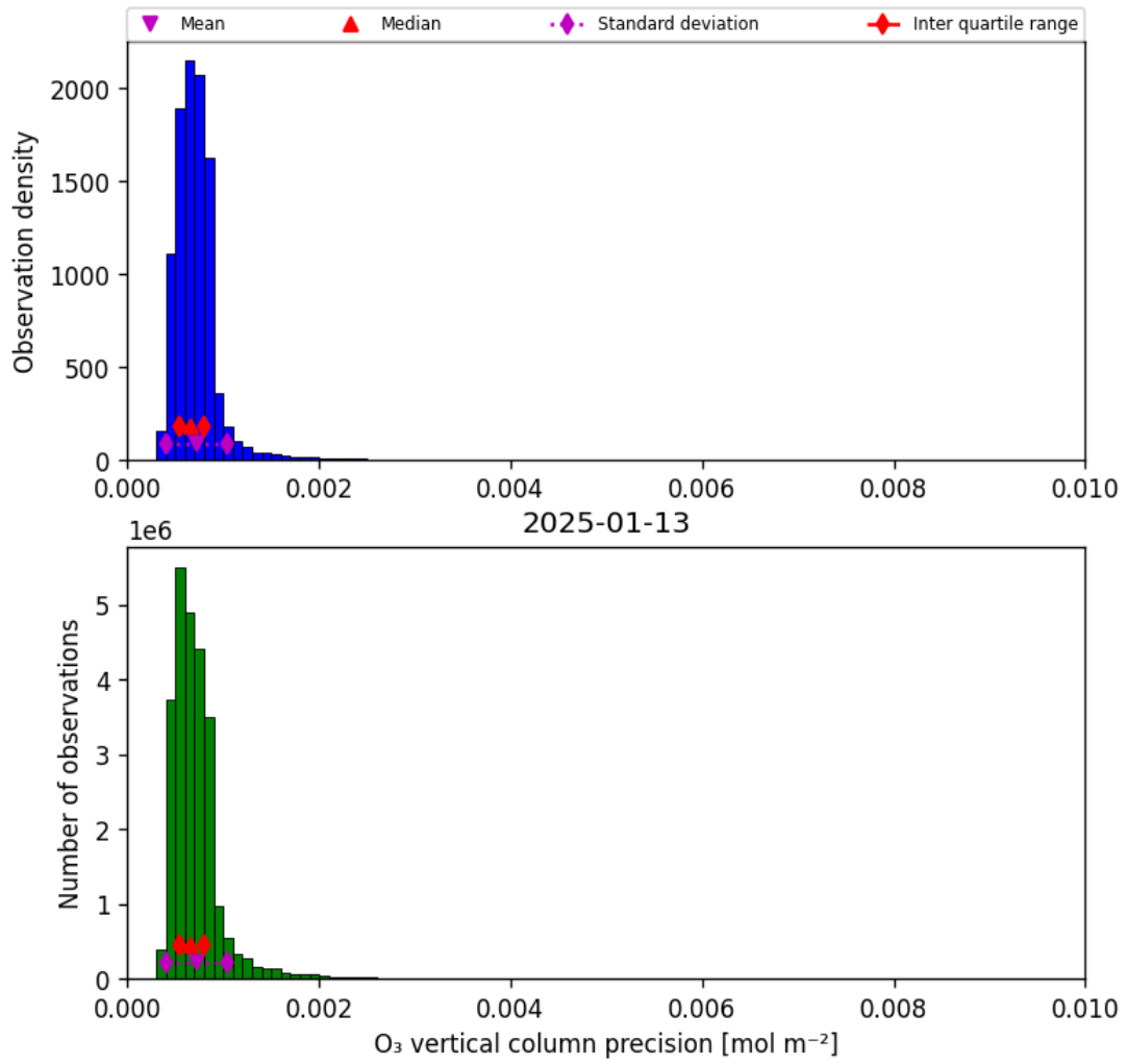
Figure 22: Histogram of “O 3 vertical column precision” for 2025-01-12 to 2025-01-14
