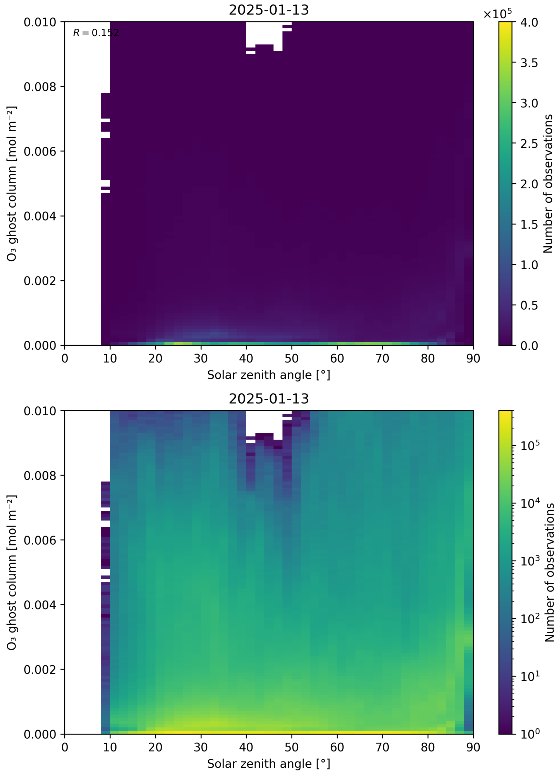
Figure 46: Scatter density plot of “Solar zenith angle” against “O 3 ghost column” for 2025-01-12 to 2025-01-14.
