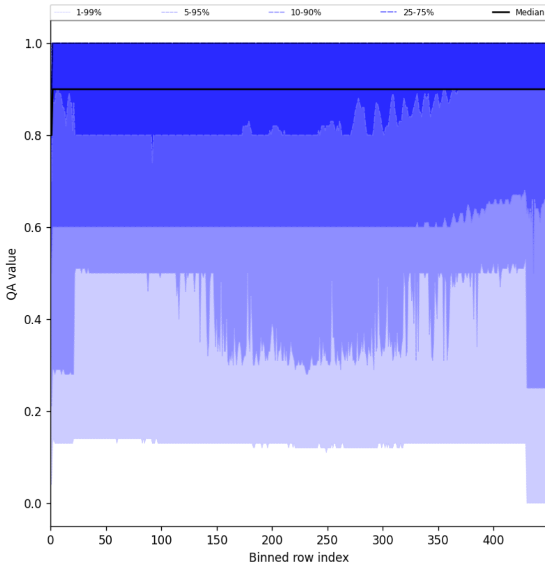
Figure 27: Along track statistics of “QA value” for 2025-01-12 to 2025-01-14
