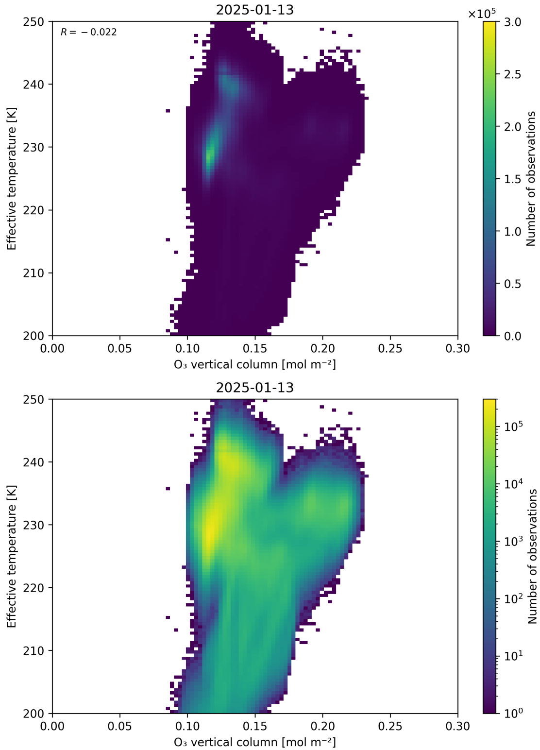
Figure 39: Scatter density plot of “O 3 vertical column” against “Effective temperature” for 2025-01-12 to 2025-01-14.
