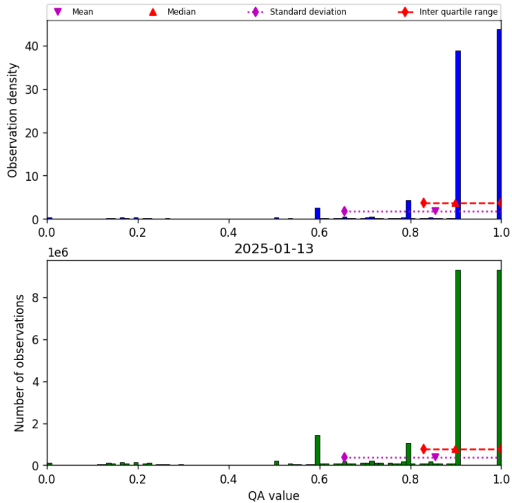
Figure 20: Histogram of “QA value” for 2025-01-12 to 2025-01-14
