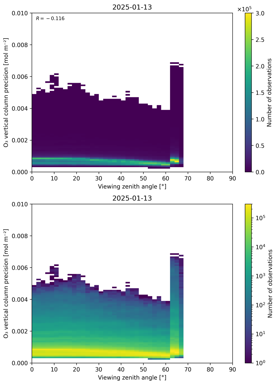
Figure 53: Scatter density plot of “Viewing zenith angle” against “O 3 vertical column precision” for 2025-01-12 to 2025-01-14.
