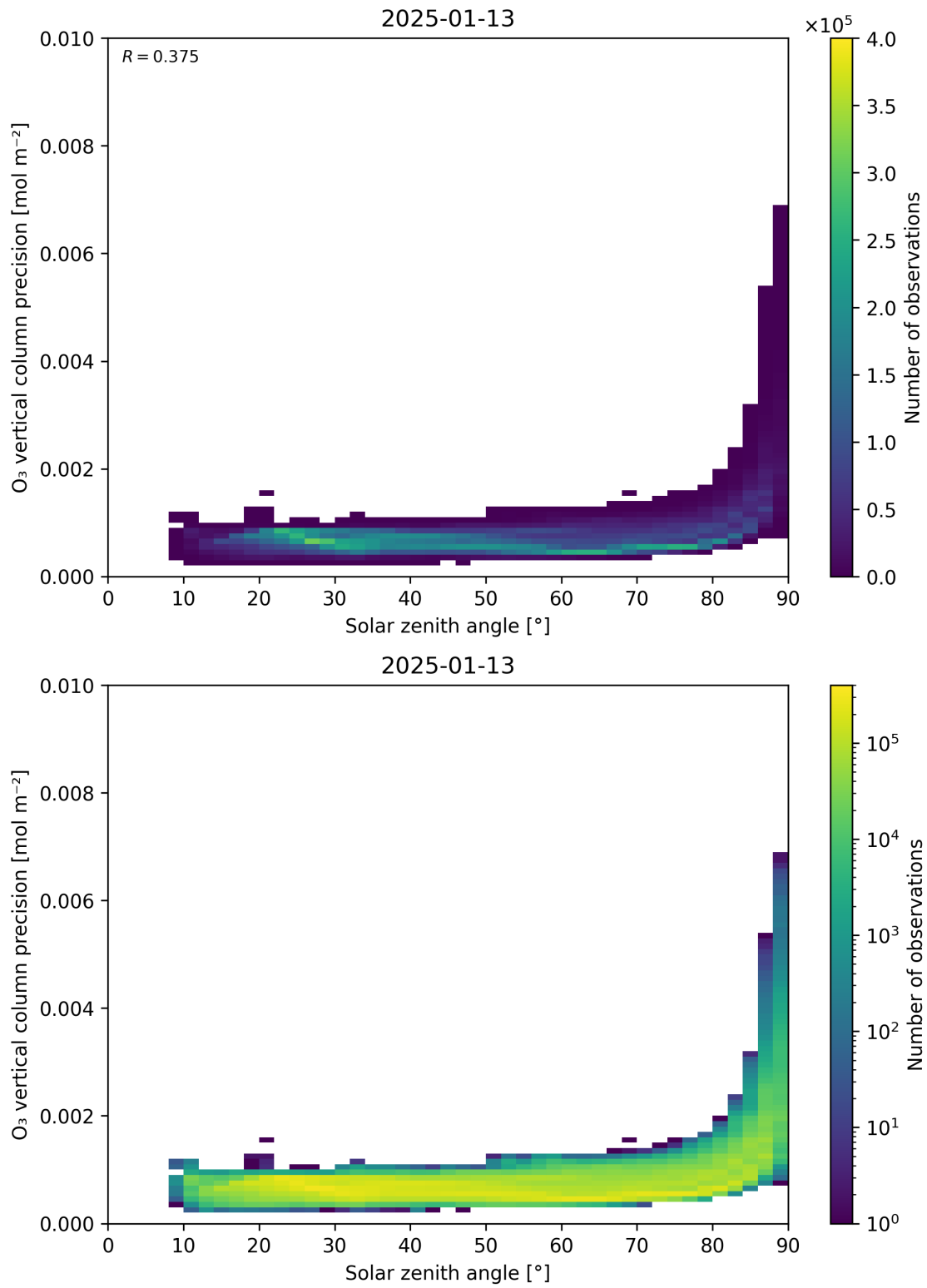
Figure 48: Scatter density plot of “Solar zenith angle” against “O 3 vertical column precision” for 2025-01-12 to 2025-01-14.
