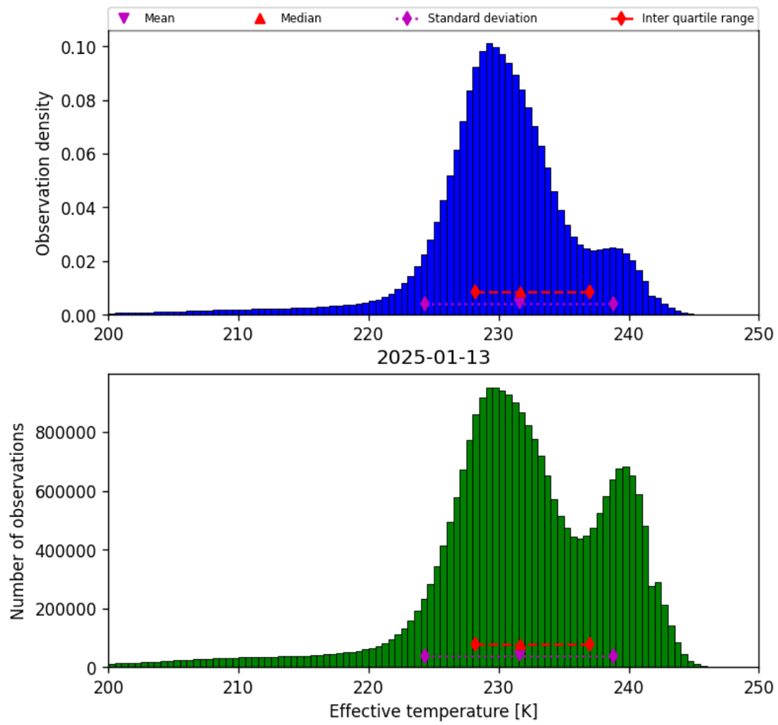
Figure 24: Histogram of “Effective temperature” for 2025-01-12 to 2025-01-14
