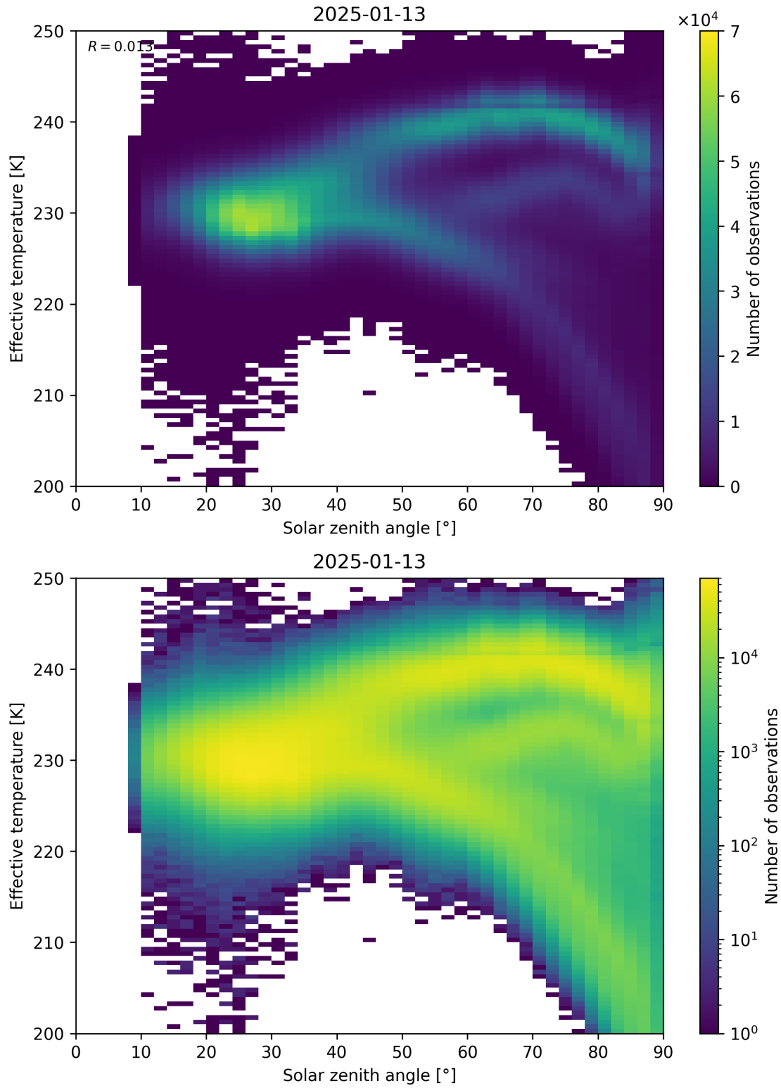
Figure 45: Scatter density plot of “Solar zenith angle” against “Effective temperature” for 2025-01-12 to 2025-01-14.
