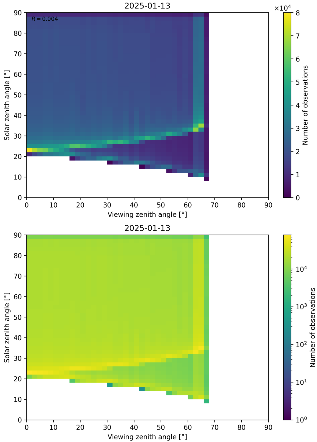
Figure 54: Scatter density plot of “Viewing zenith angle” against “Solar zenith angle” for 2025-01-12 to 2025-01-14.
