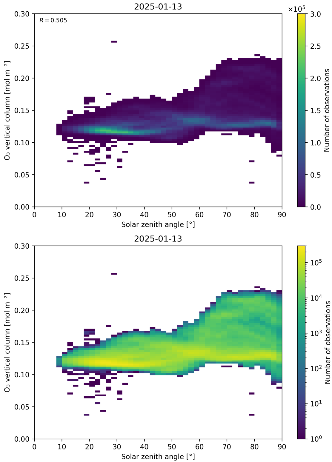
Figure 47: Scatter density plot of “Solar zenith angle” against “O 3 vertical column” for 2025-01-12 to 2025-01-14.
