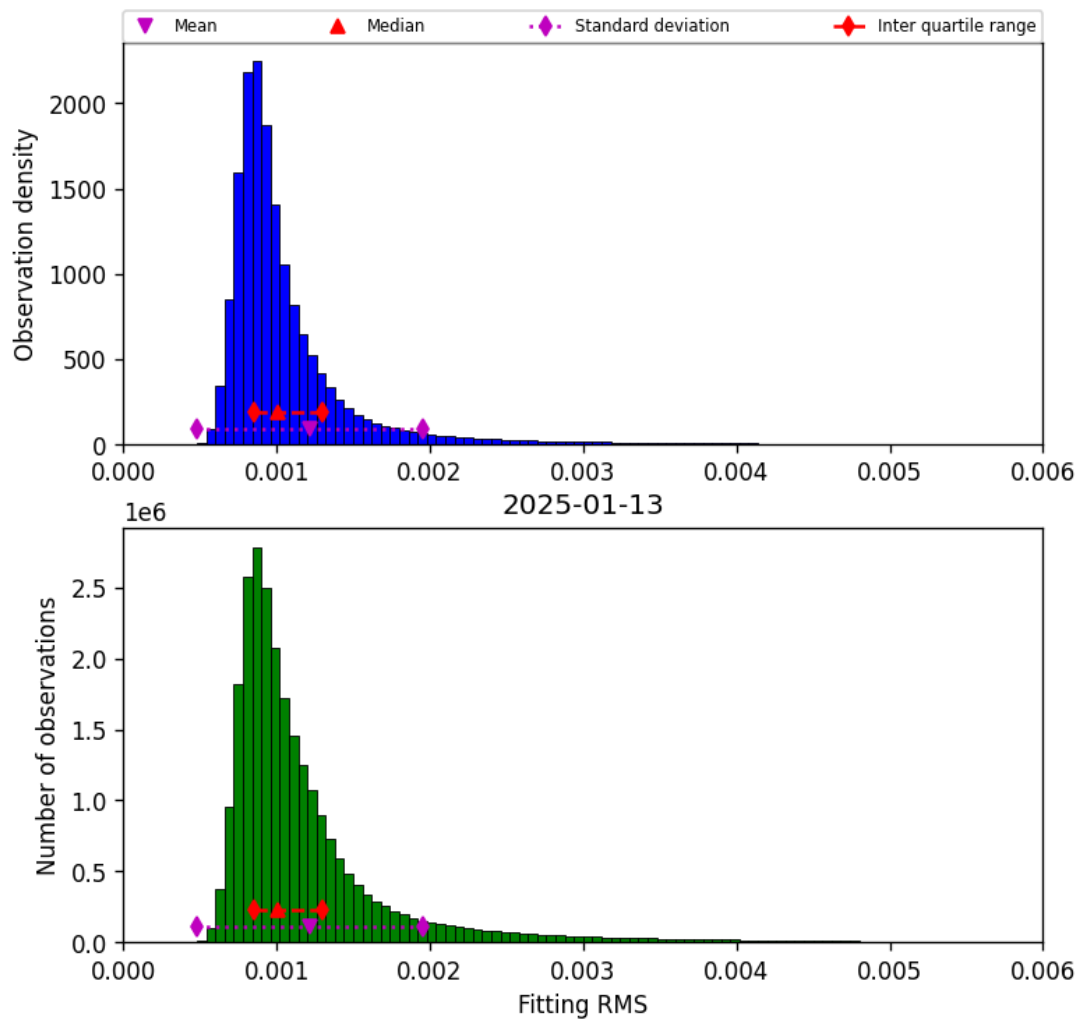
Figure 23: Histogram of “Fitting RMS” for 2025-01-12 to 2025-01-14
