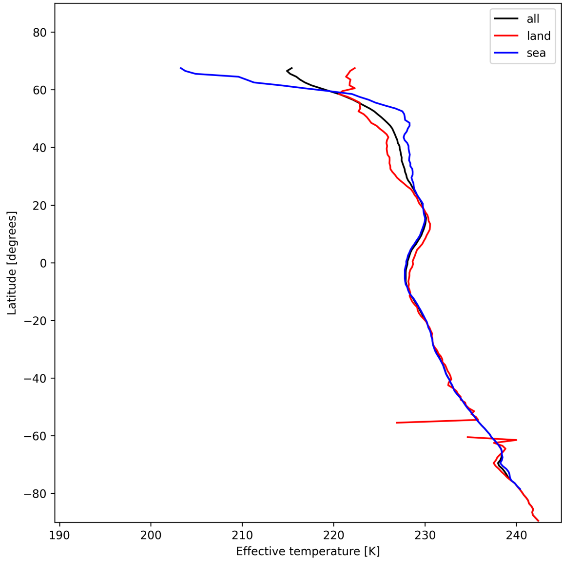
Figure 17: Zonal average of "Effective temperature" for 2025-01-12 to 2025-01-14.
