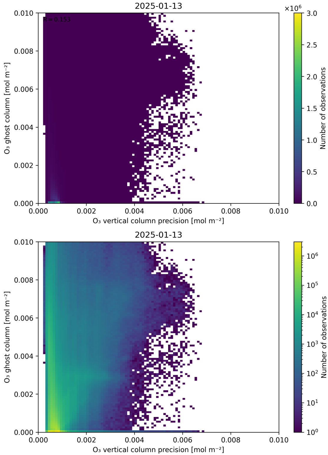
Figure 43: Scatter density plot of “ \text{O}_3 vertical column precision” against “ \text{O}_3 ghost column” for 2025-01-12 to 2025-01-14.
