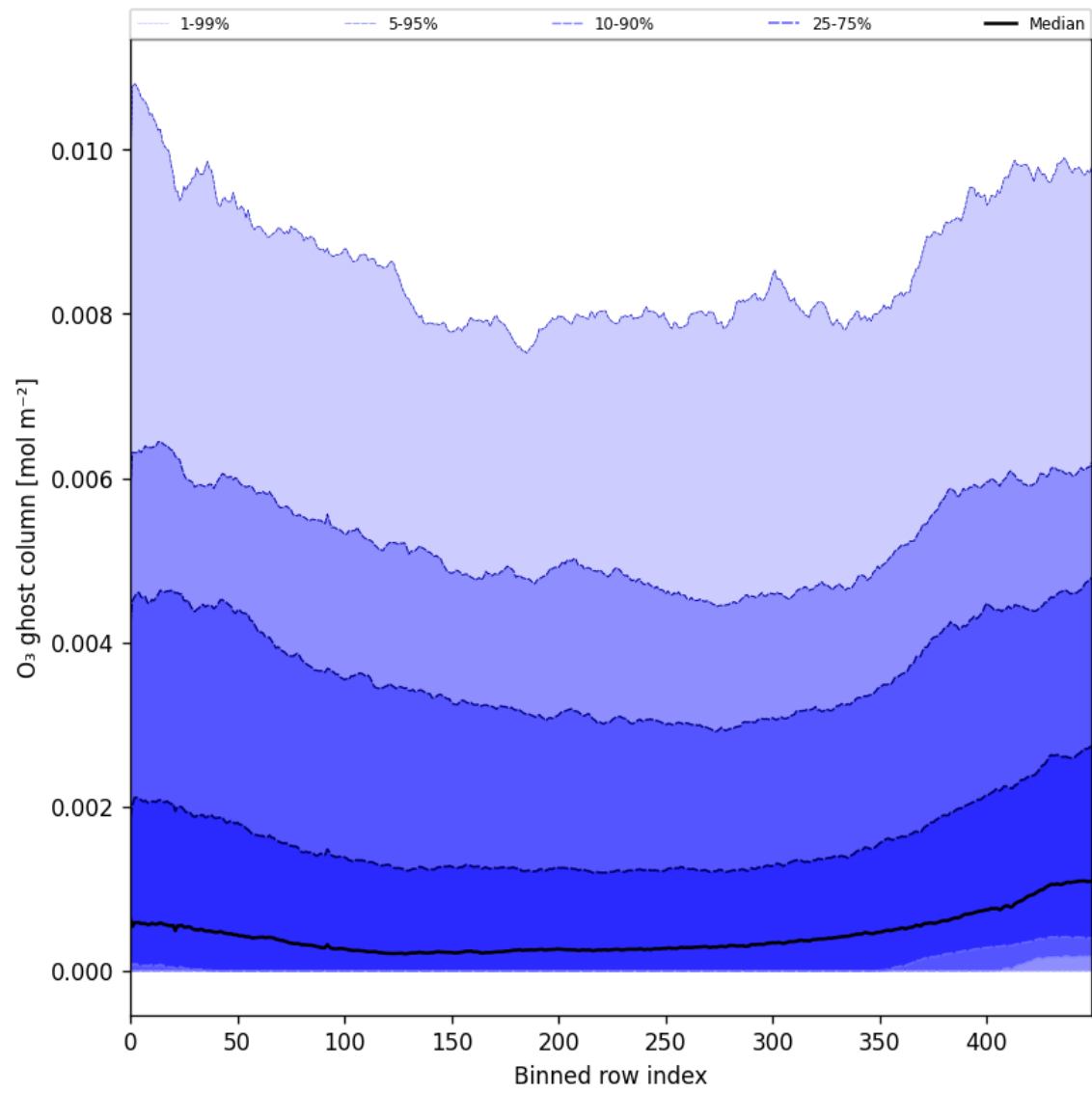
Figure 32: Along track statistics of “O 3 ghost column” for 2025-01-12 to 2025-01-14
