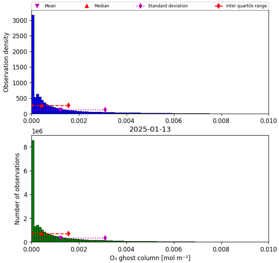
Figure 25: Histogram of “O 3 ghost column” for 2025-01-12 to 2025-01-14
