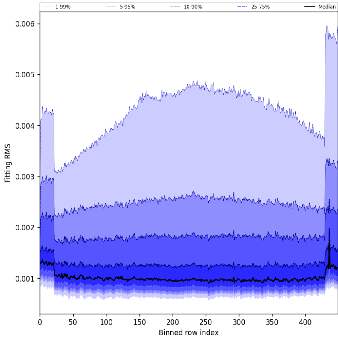
Figure 30: Along track statistics of “Fitting RMS” for 2025-01-12 to 2025-01-14
