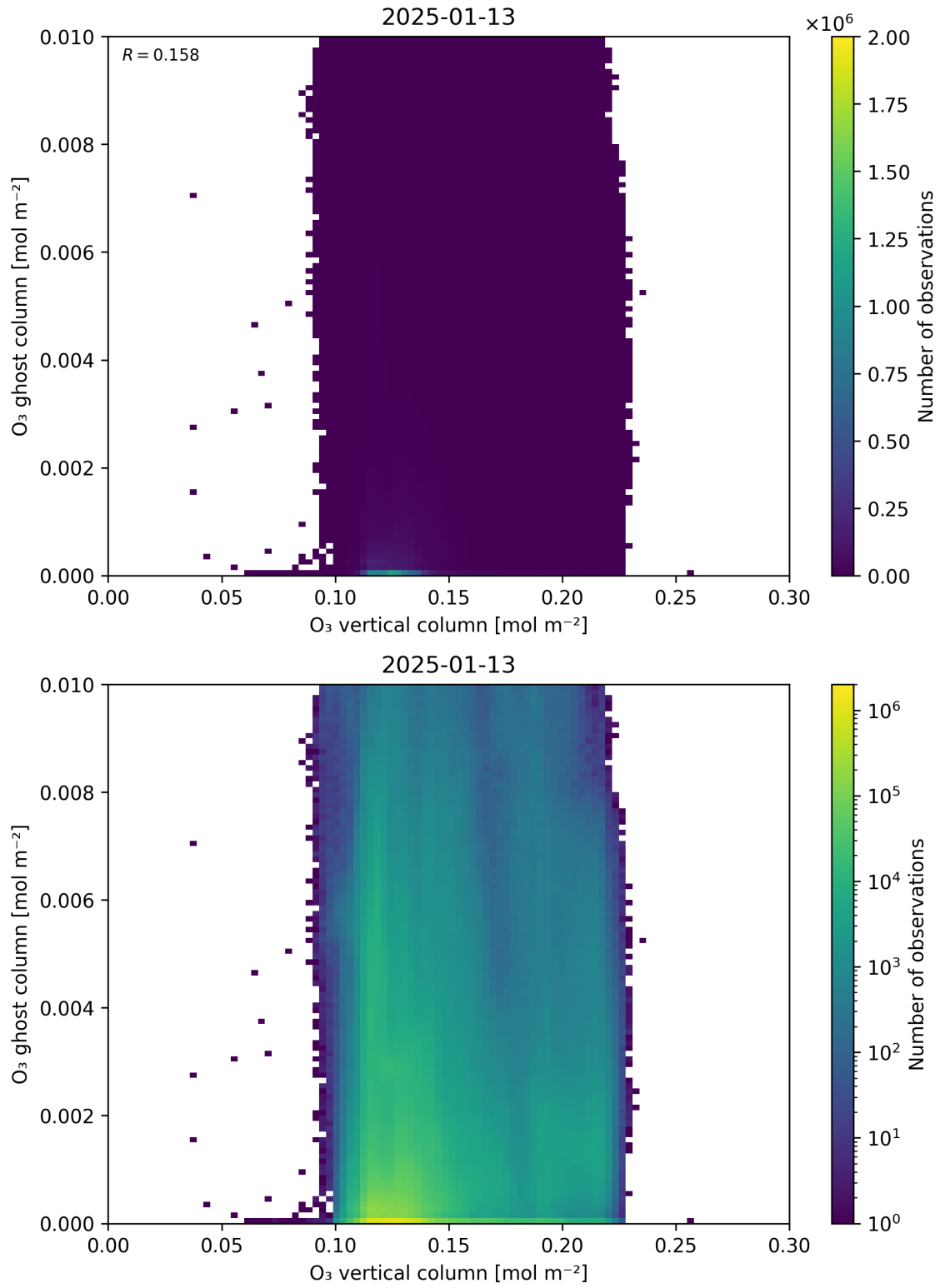
Figure 40: Scatter density plot of “O 3 vertical column” against “O 3 ghost column” for 2025-01-12 to 2025-01-14.
