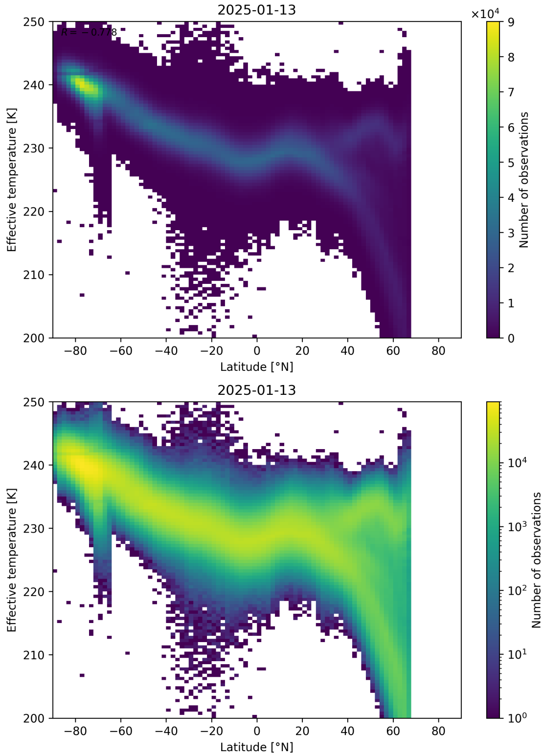
Figure 34: Scatter density plot of “Latitude” against “Effective temperature” for 2025-01-12 to 2025-01-14.
