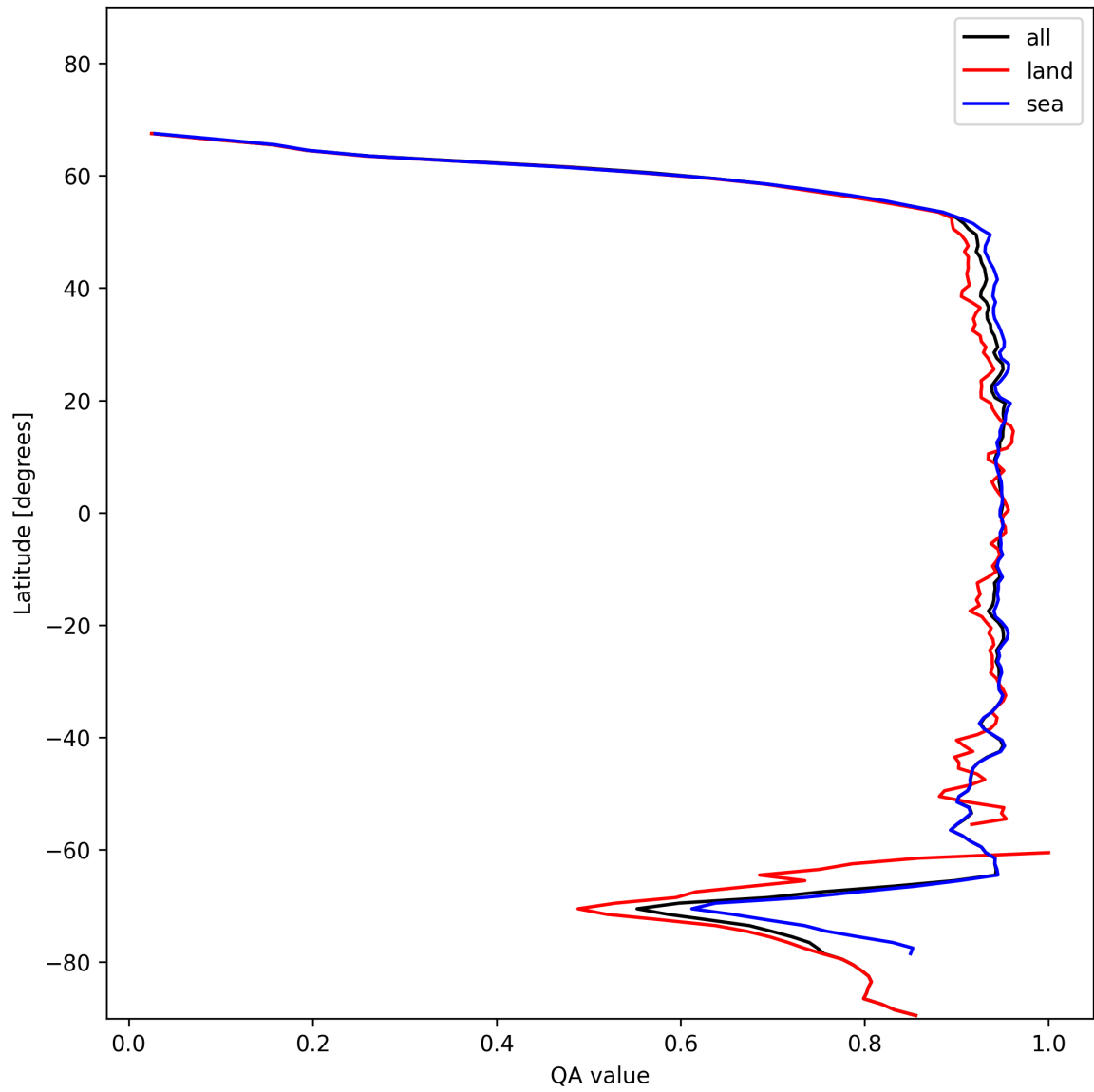
Figure 13: Zonal average of “QA value” for 2025-01-12 to 2025-01-14.
