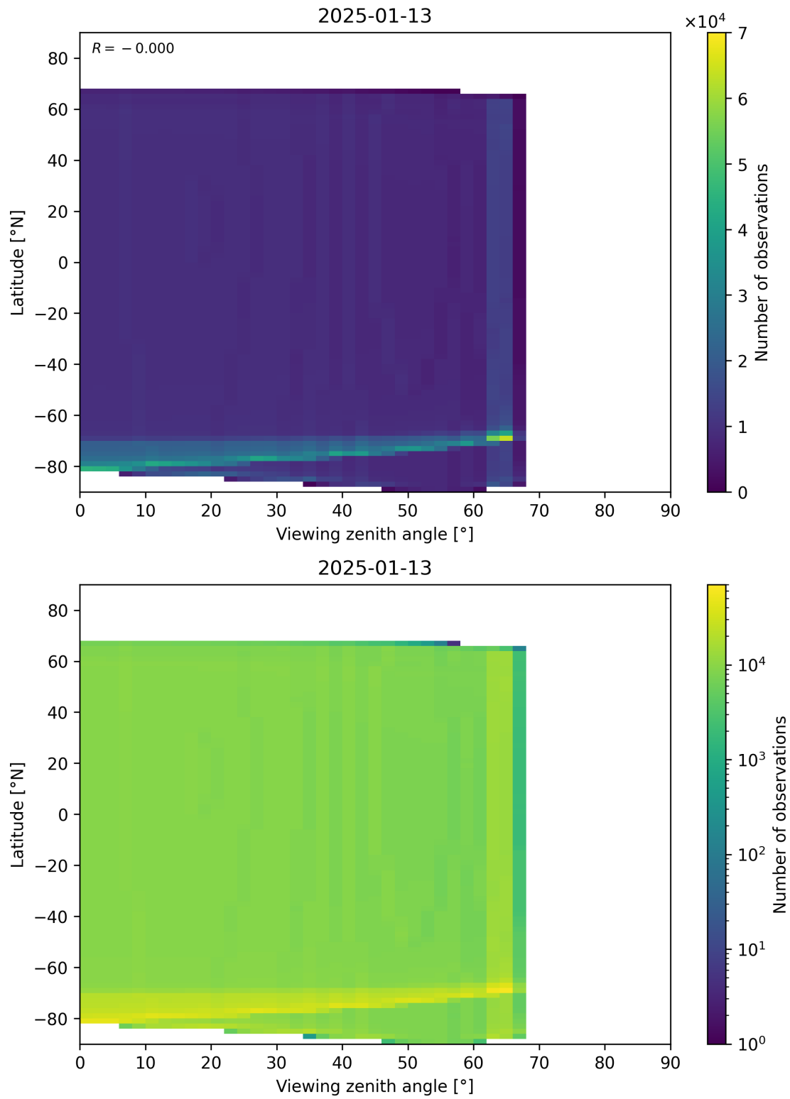
Figure 49: Scatter density plot of “Viewing zenith angle” against “Latitude” for 2025-01-12 to 2025-01-14.
