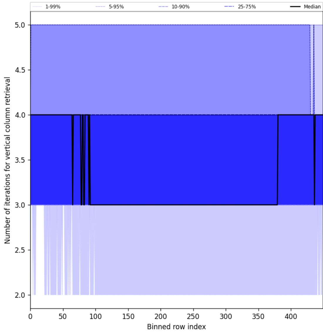
Figure 33: Along track statistics of “Number of iterations for vertical column retrieval” for 2025-01-12 to 2025-01-14
