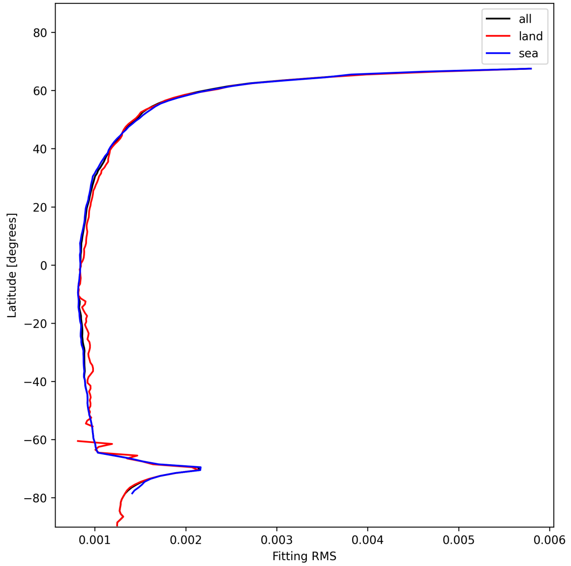
Figure 16: Zonal average of “Fitting RMS” for 2025-01-12 to 2025-01-14.
