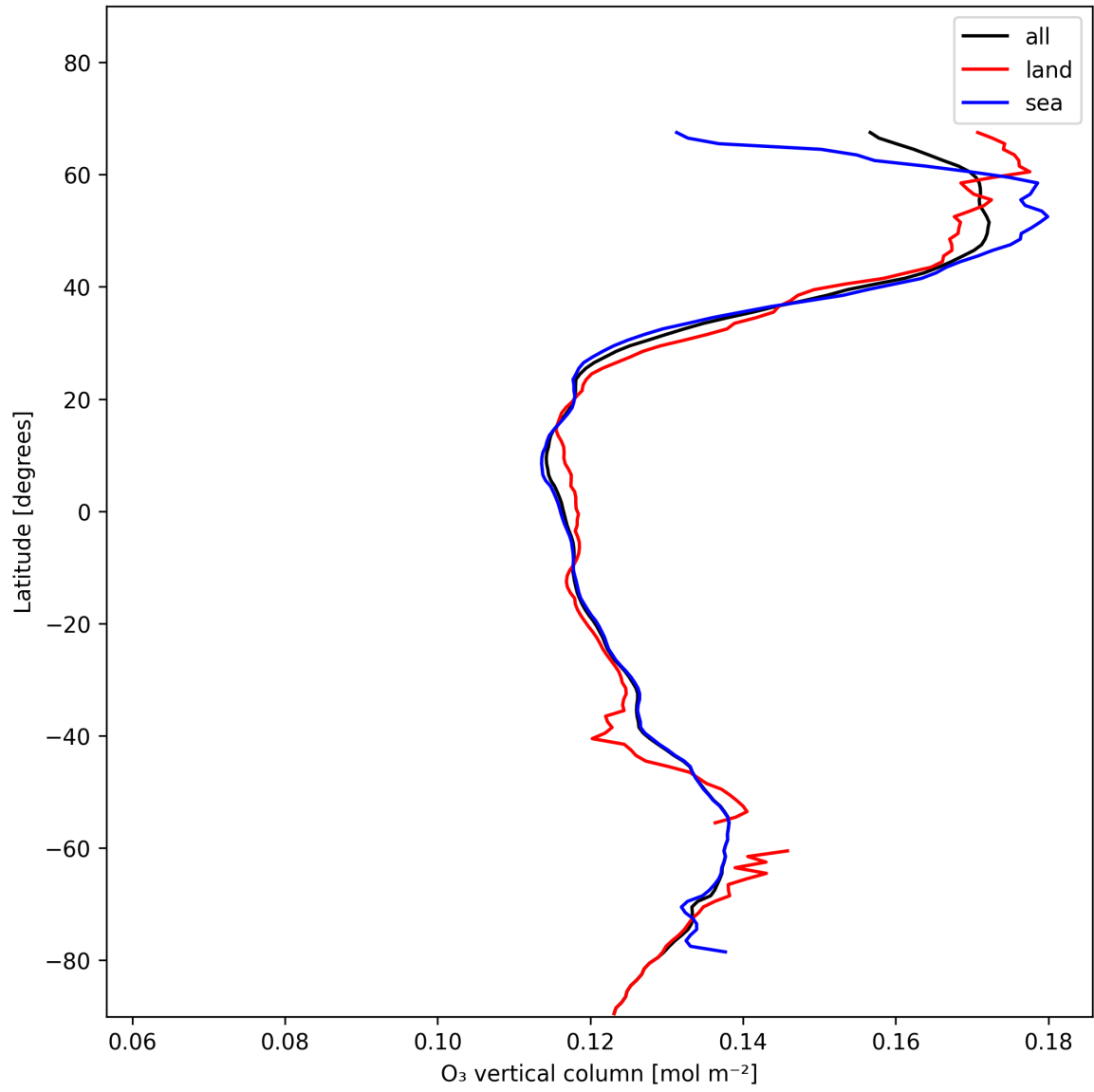
Figure 14: Zonal average of “O 3 vertical column” for 2025-01-12 to 2025-01-14.
