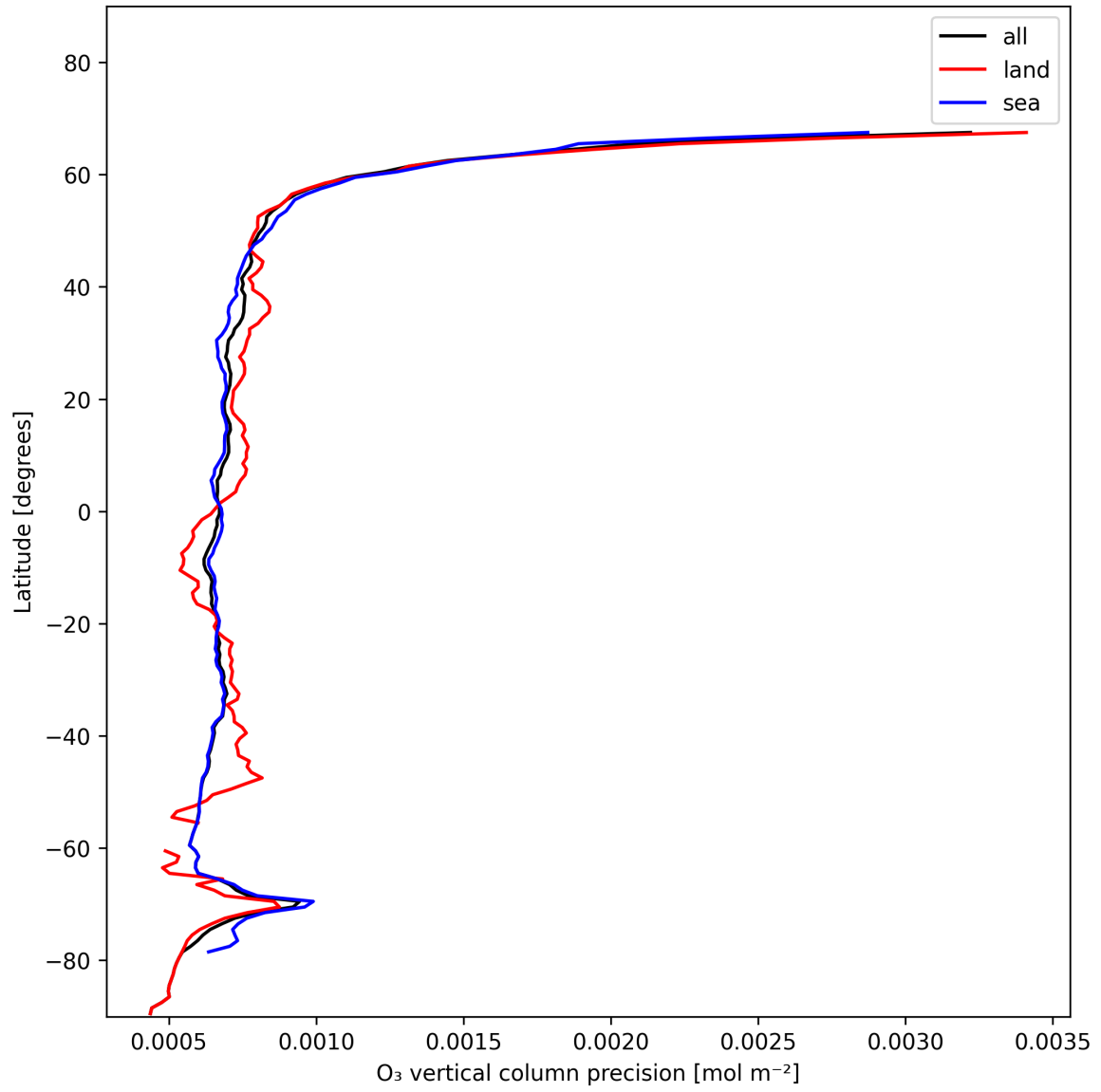
Figure 15: Zonal average of “O 3 vertical column precision” for 2025-01-12 to 2025-01-14.
