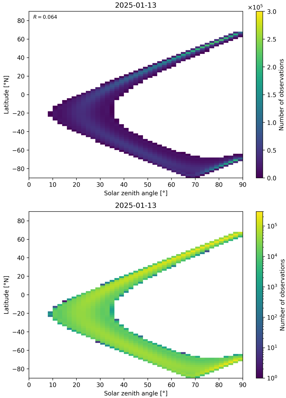
Figure 44: Scatter density plot of “Solar zenith angle” against “Latitude” for 2025-01-12 to 2025-01-14.
