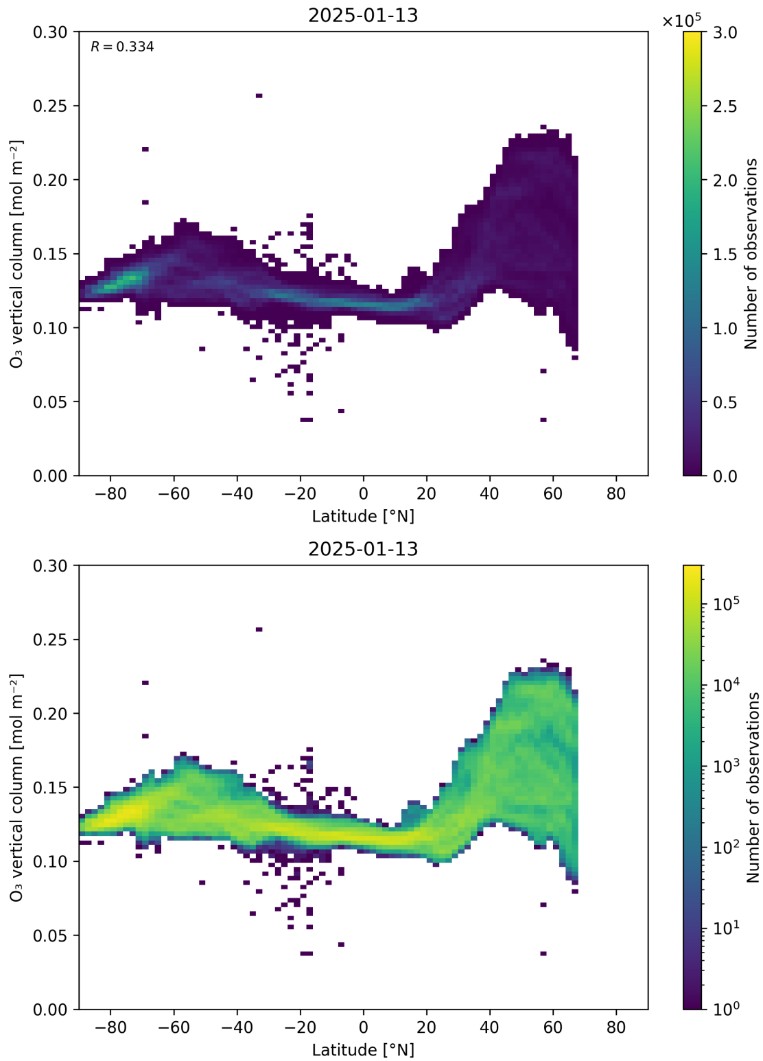
Figure 36: Scatter density plot of “Latitude” against “O 3 vertical column” for 2025-01-12 to 2025-01-14.
