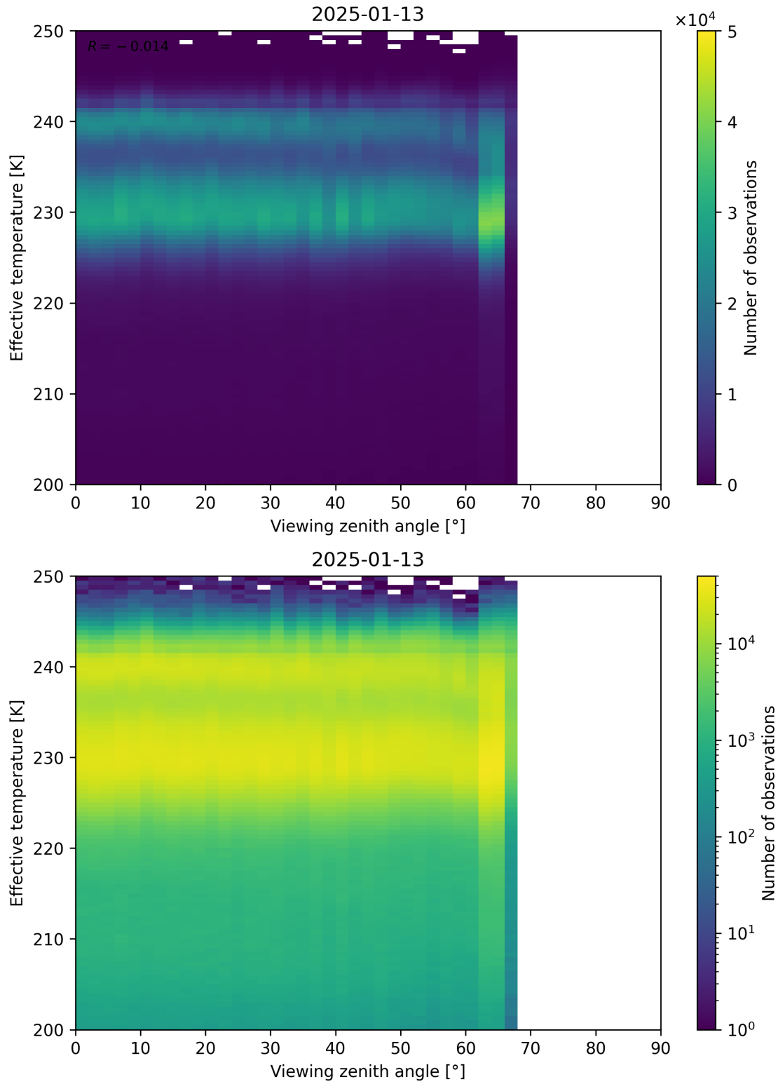
Figure 50: Scatter density plot of “Viewing zenith angle” against “Effective temperature” for 2025-01-12 to 2025-01-14.
