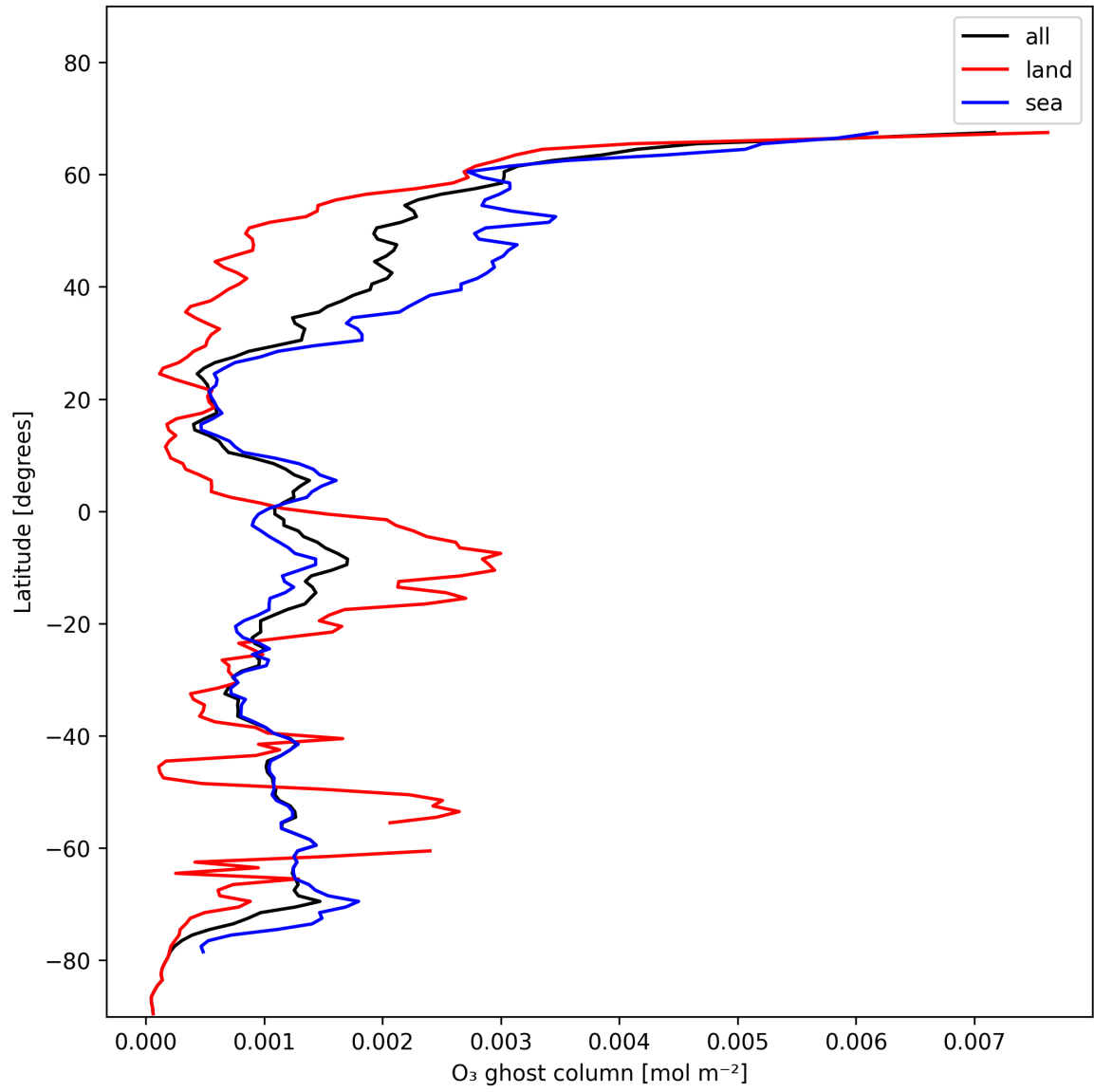
Figure 18: Zonal average of “O 3 ghost column” for 2025-01-12 to 2025-01-14.
