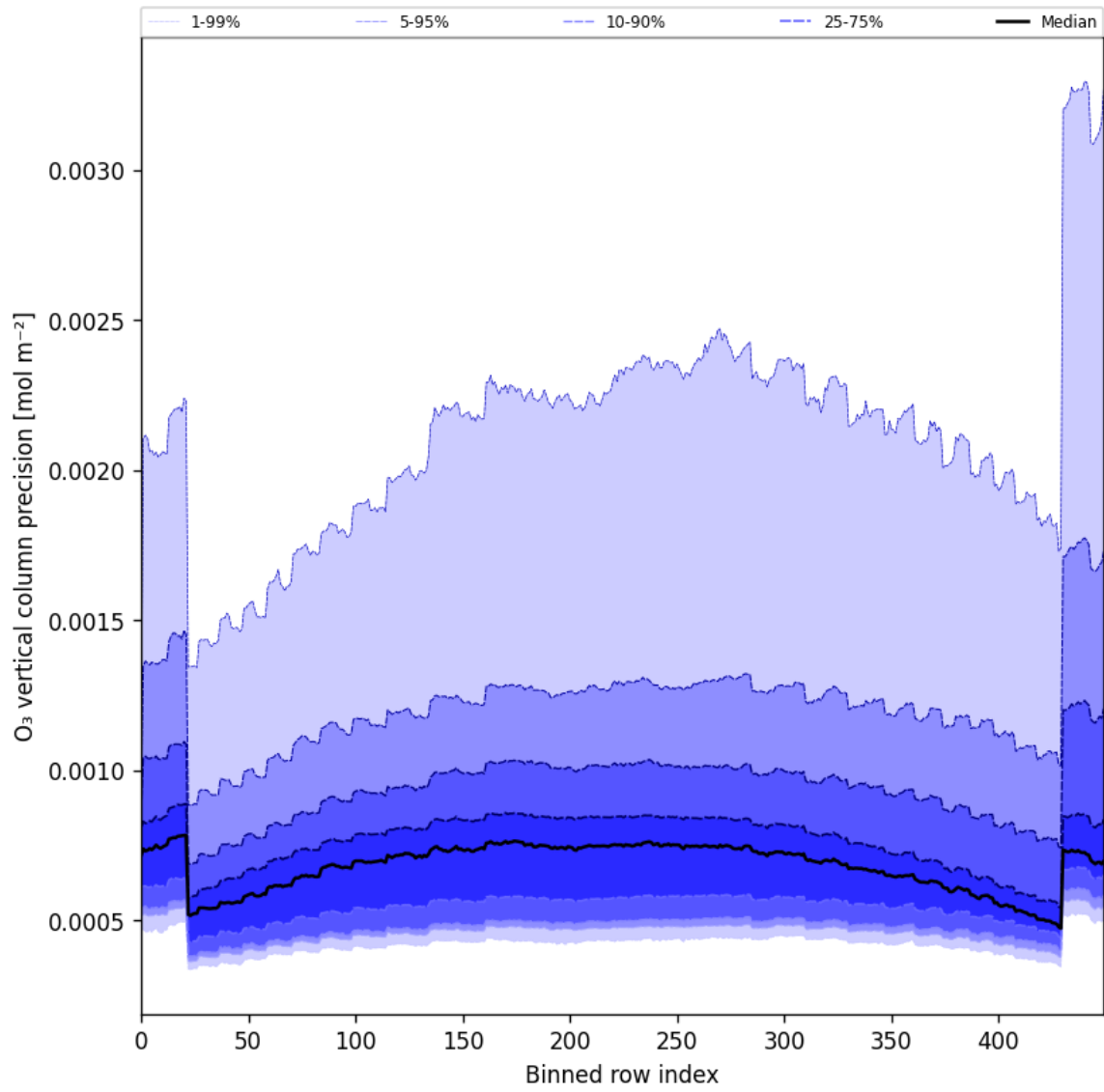
Figure 29: Along track statistics of “O 3 vertical column precision” for 2025-01-12 to 2025-01-14
