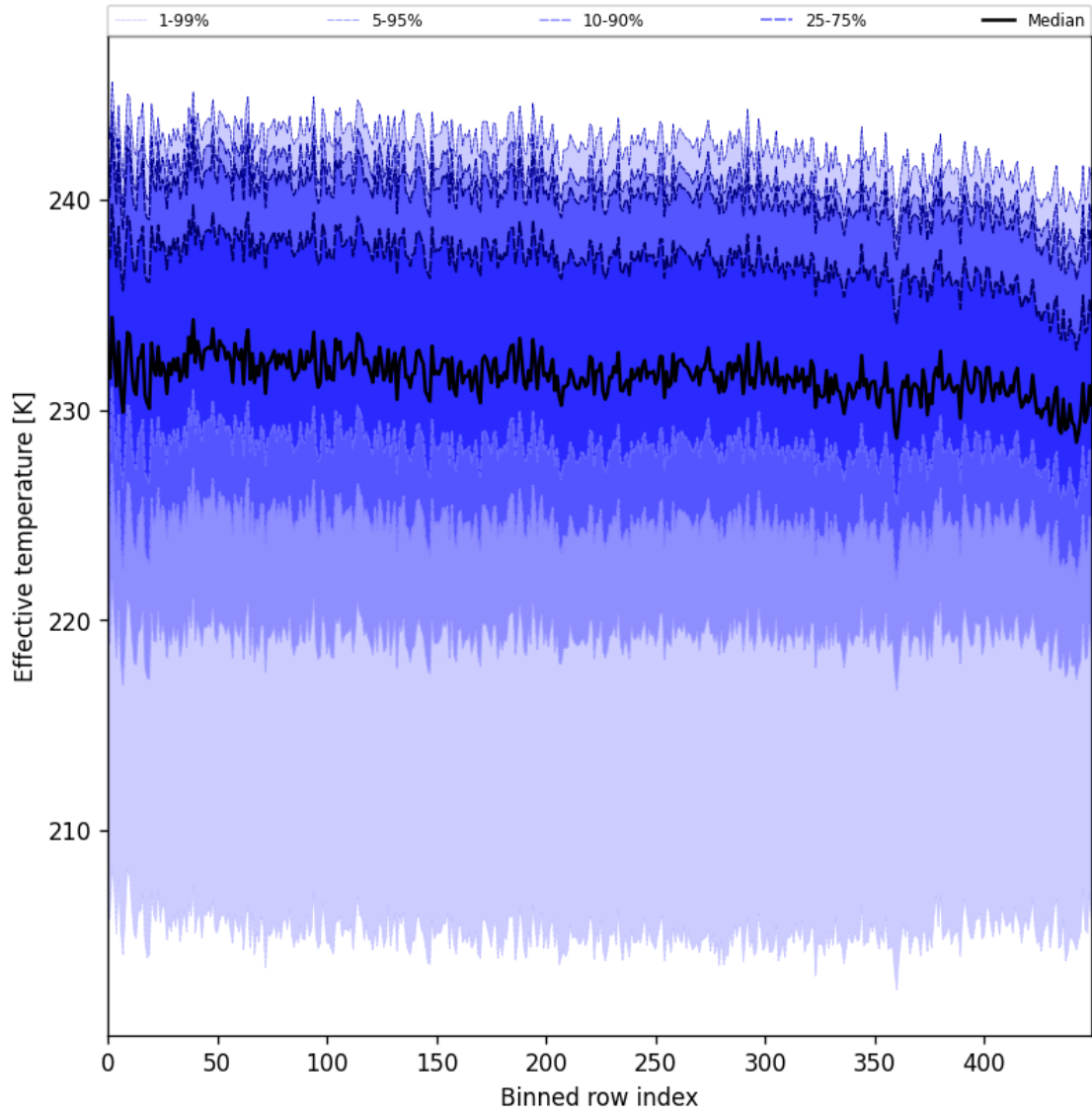
Figure 31: Along track statistics of “Effective temperature” for 2025-01-12 to 2025-01-14
