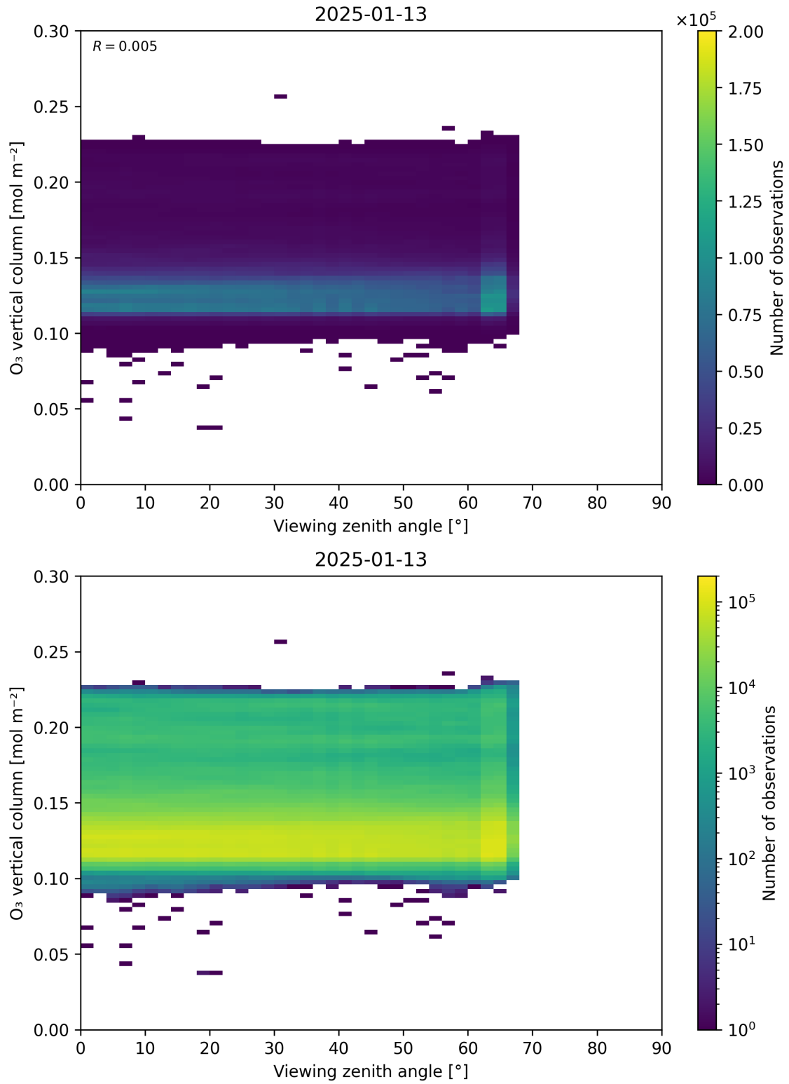
Figure 52: Scatter density plot of “Viewing zenith angle” against “O 3 vertical column” for 2025-01-12 to 2025-01-14.
