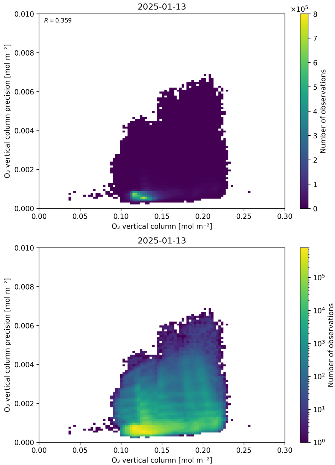
Figure 41: Scatter density plot of “O 3 vertical column” against “O 3 vertical column precision” for 2025-01-12 to 2025-01-14.
