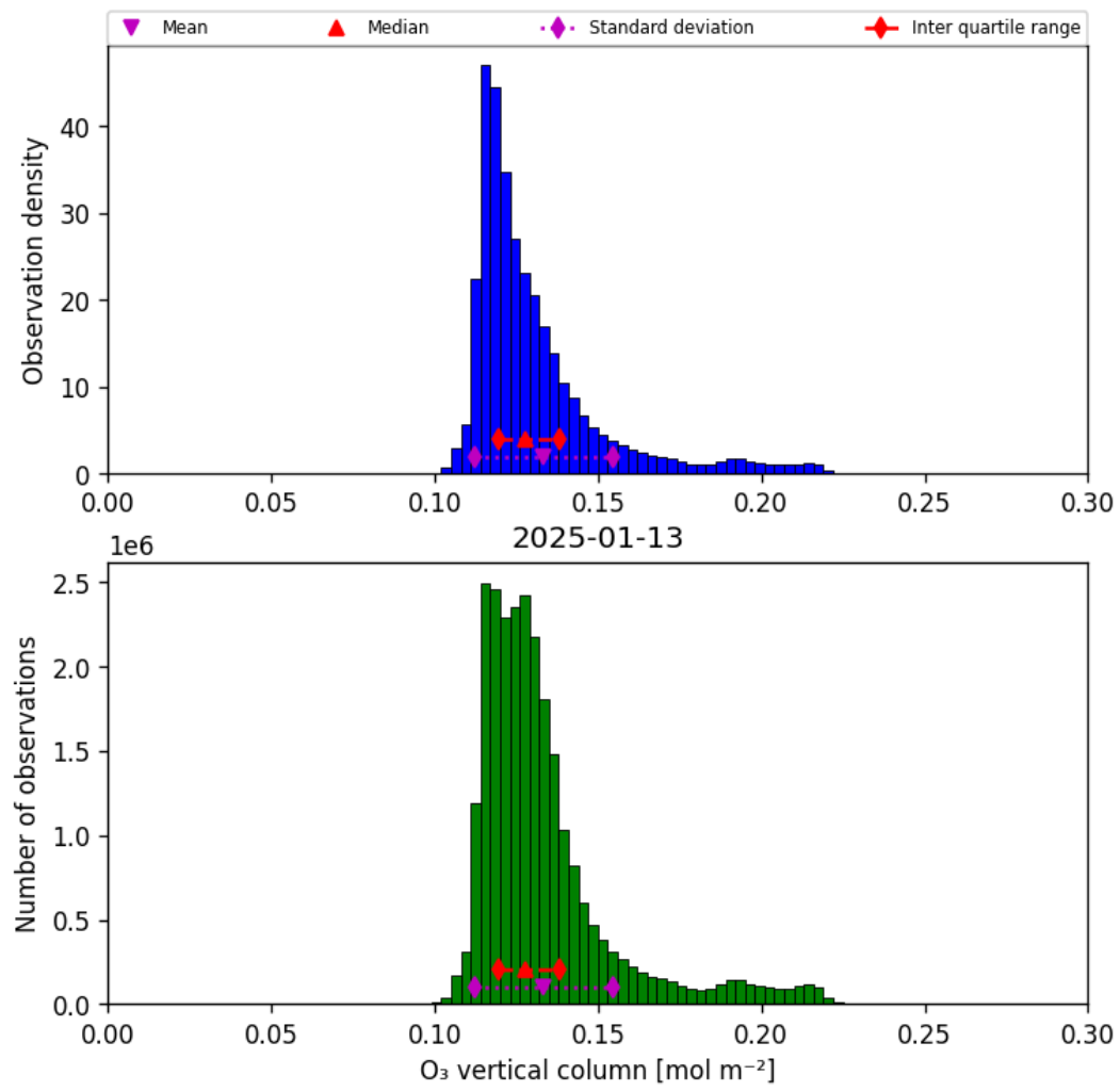
Figure 21: Histogram of “O 3 vertical column” for 2025-01-12 to 2025-01-14
