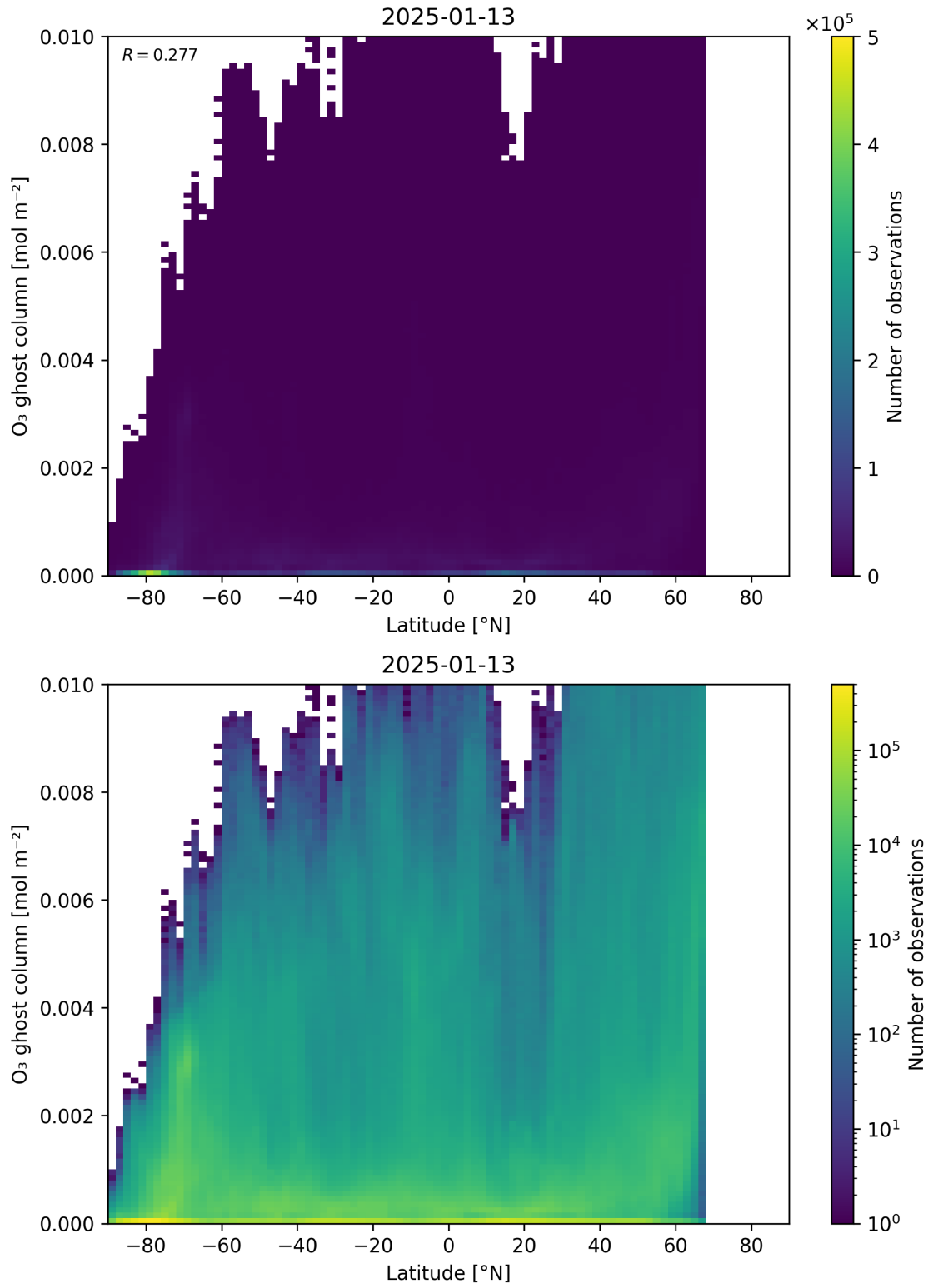
Figure 35: Scatter density plot of “Latitude” against “O 3 ghost column” for 2025-01-12 to 2025-01-14.
