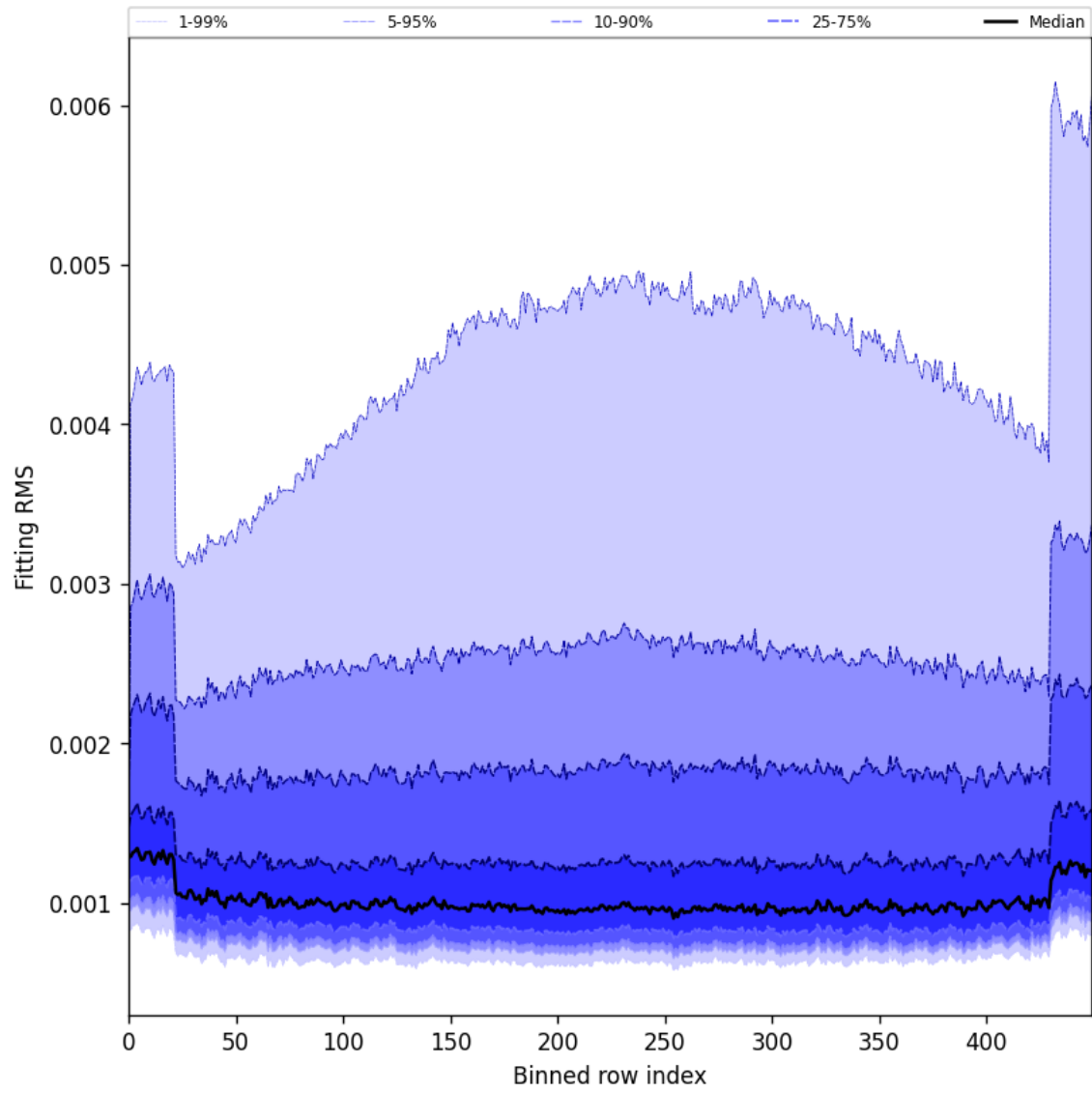
Figure 30: Along track statistics of “Fitting RMS” for 2025-01-13 to 2025-01-15
