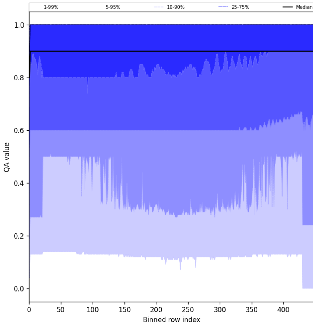
Figure 27: Along track statistics of “QA value” for 2025-01-13 to 2025-01-15
