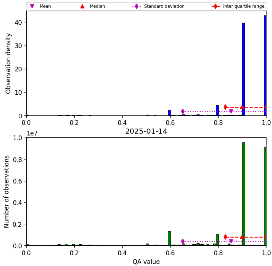
Figure 20: Histogram of “QA value” for 2025-01-13 to 2025-01-15
