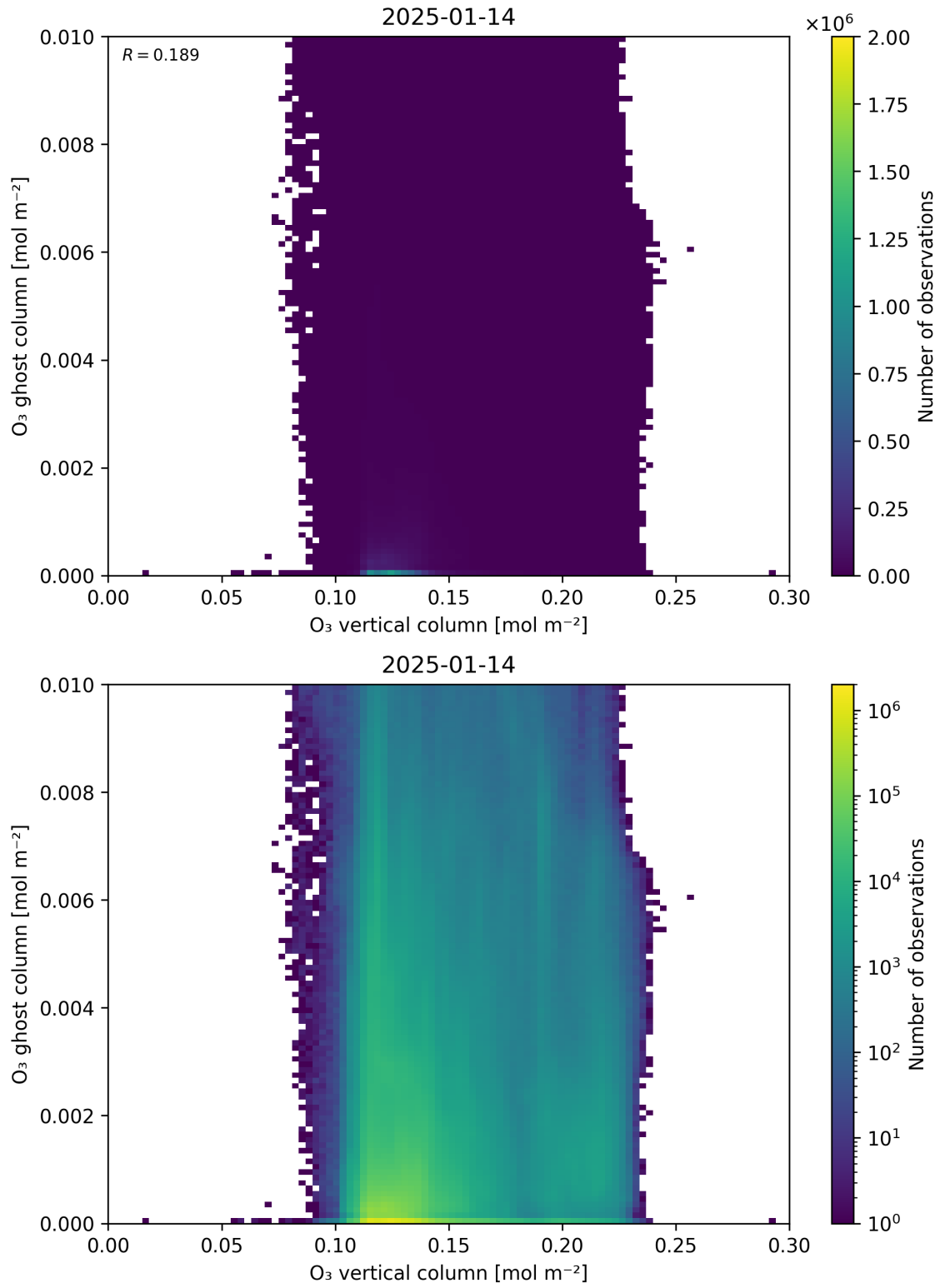
Figure 40: Scatter density plot of “ \text{O}_3 vertical column” against “ \text{O}_3 ghost column” for 2025-01-13 to 2025-01-15.
