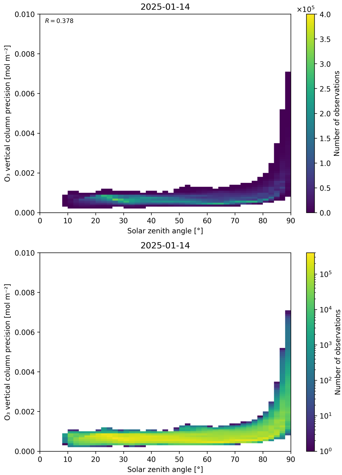
Figure 48: Scatter density plot of “Solar zenith angle” against “O 3 vertical column precision” for 2025-01-13 to 2025-01-15.
