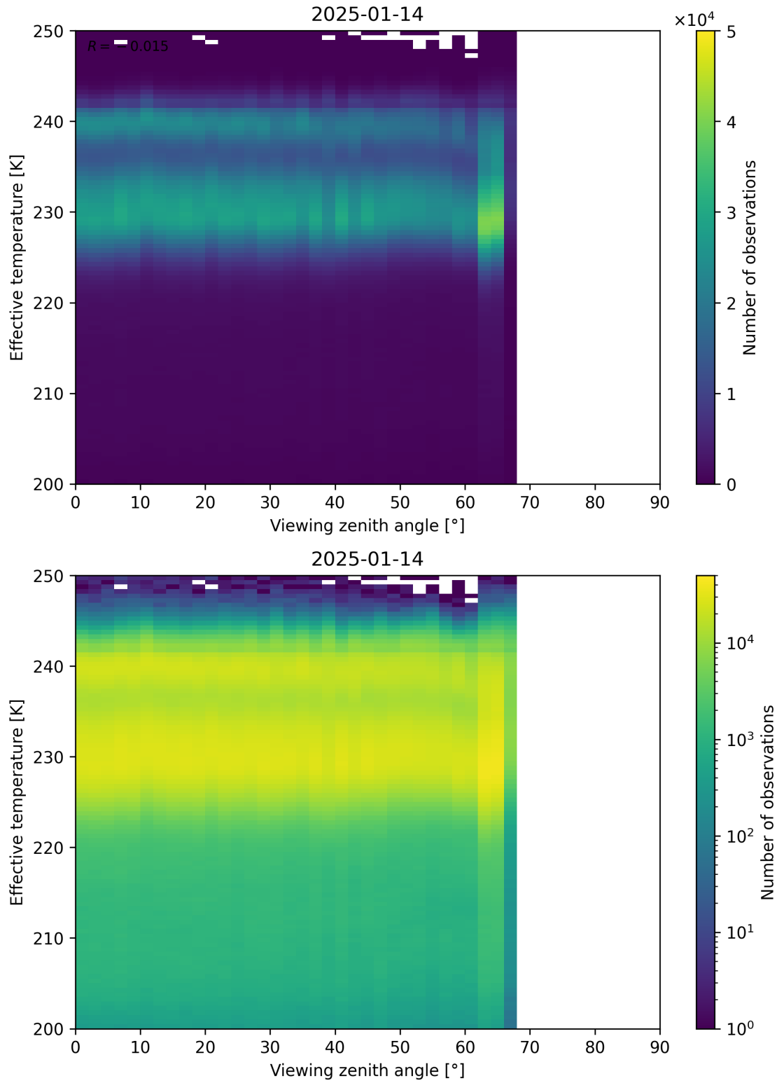
Figure 50: Scatter density plot of “Viewing zenith angle” against “Effective temperature” for 2025-01-13 to 2025-01-15.
