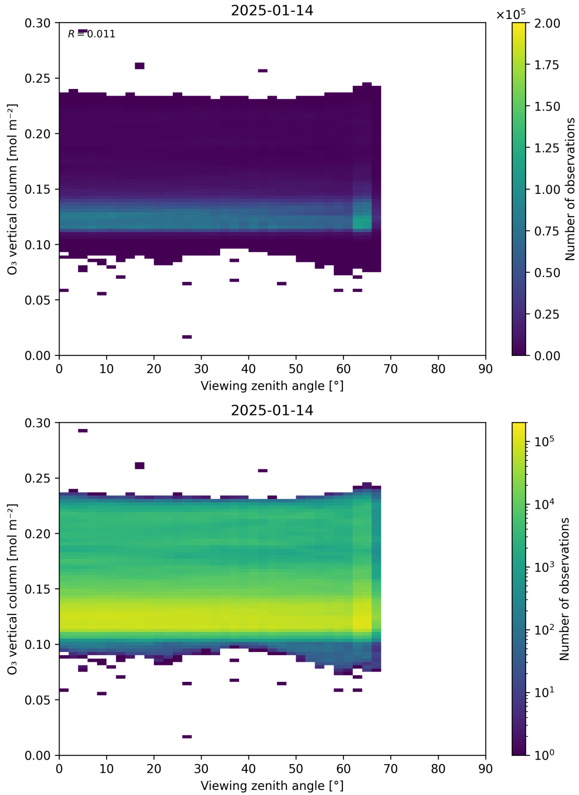
Figure 52: Scatter density plot of “Viewing zenith angle” against “O 3 vertical column” for 2025-01-13 to 2025-01-15.
