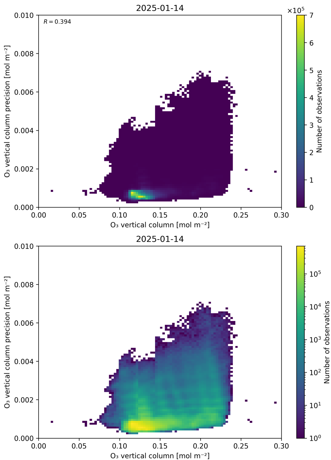
Figure 41: Scatter density plot of “O 3 vertical column” against “O 3 vertical column precision” for 2025-01-13 to 2025-01-15.
