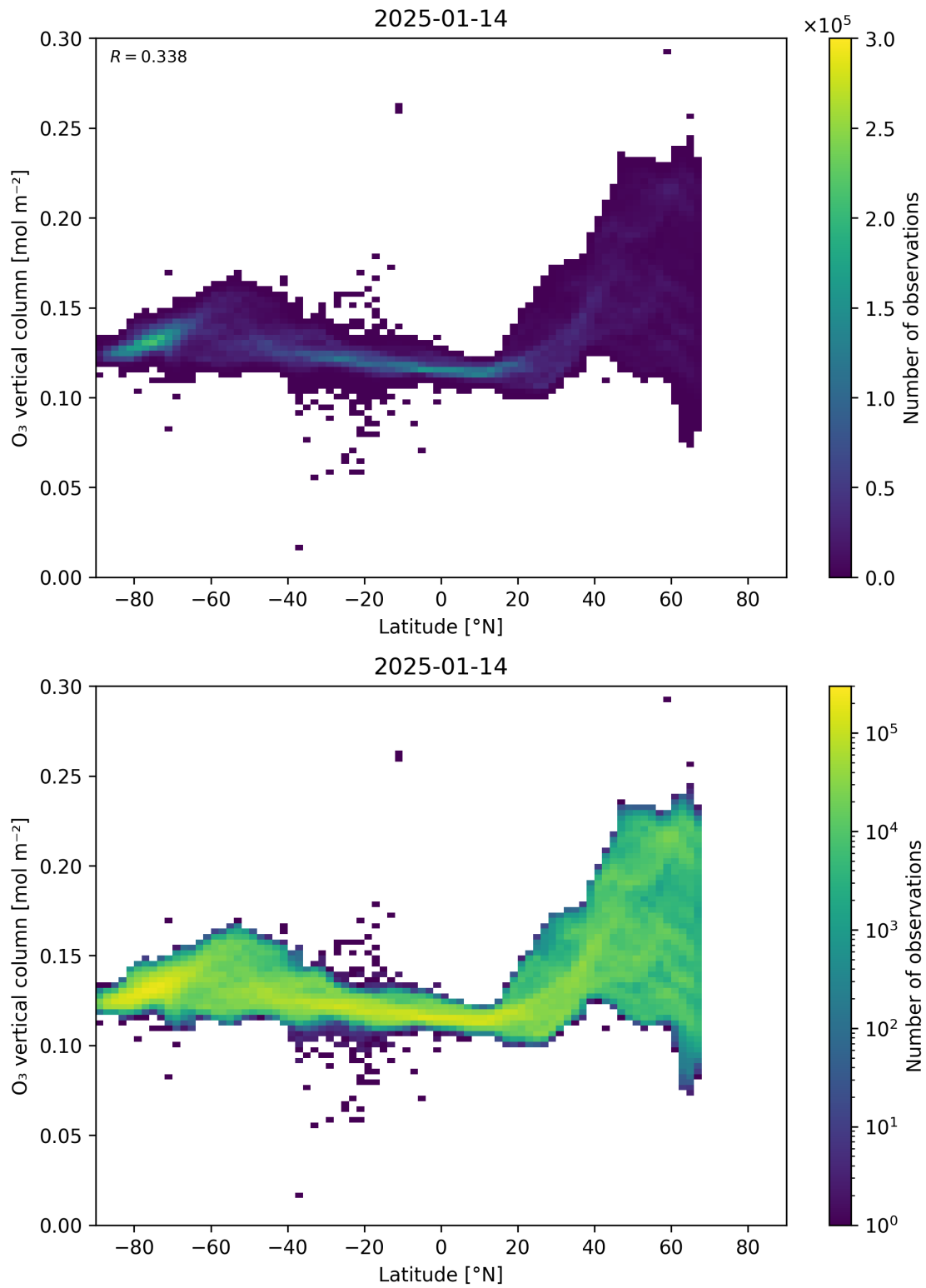
Figure 36: Scatter density plot of “Latitude” against “O 3 vertical column” for 2025-01-13 to 2025-01-15.
