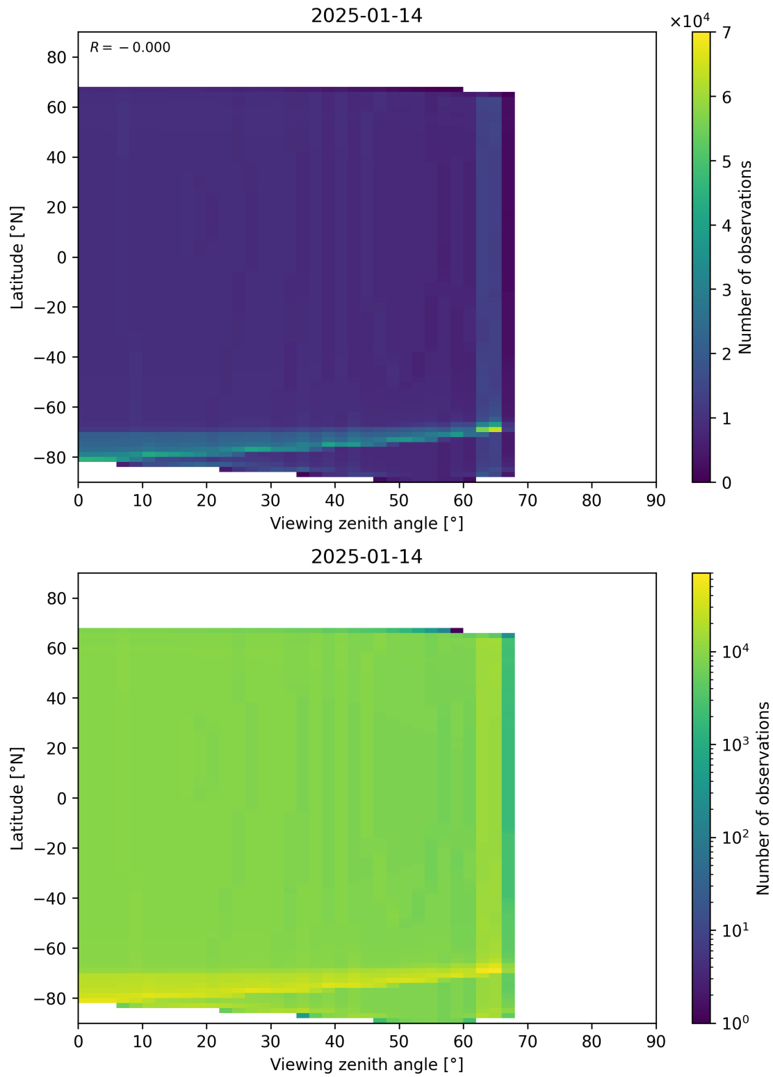
Figure 49: Scatter density plot of “Viewing zenith angle” against “Latitude” for 2025-01-13 to 2025-01-15.
