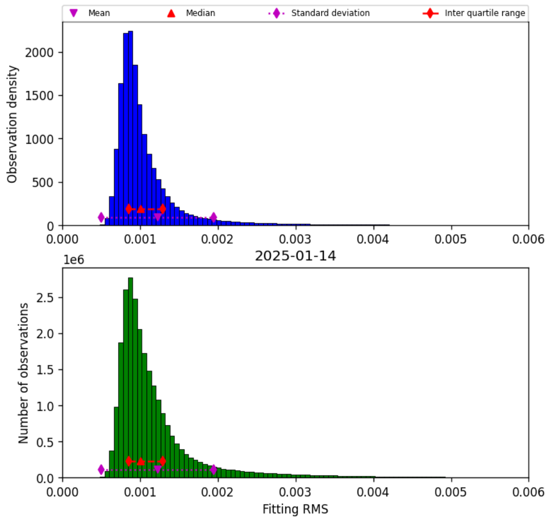
Figure 23: Histogram of “Fitting RMS” for 2025-01-13 to 2025-01-15
