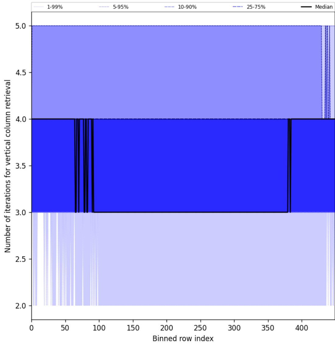
Figure 33: Along track statistics of “Number of iterations for vertical column retrieval” for 2025-01-13 to 2025-01-15
