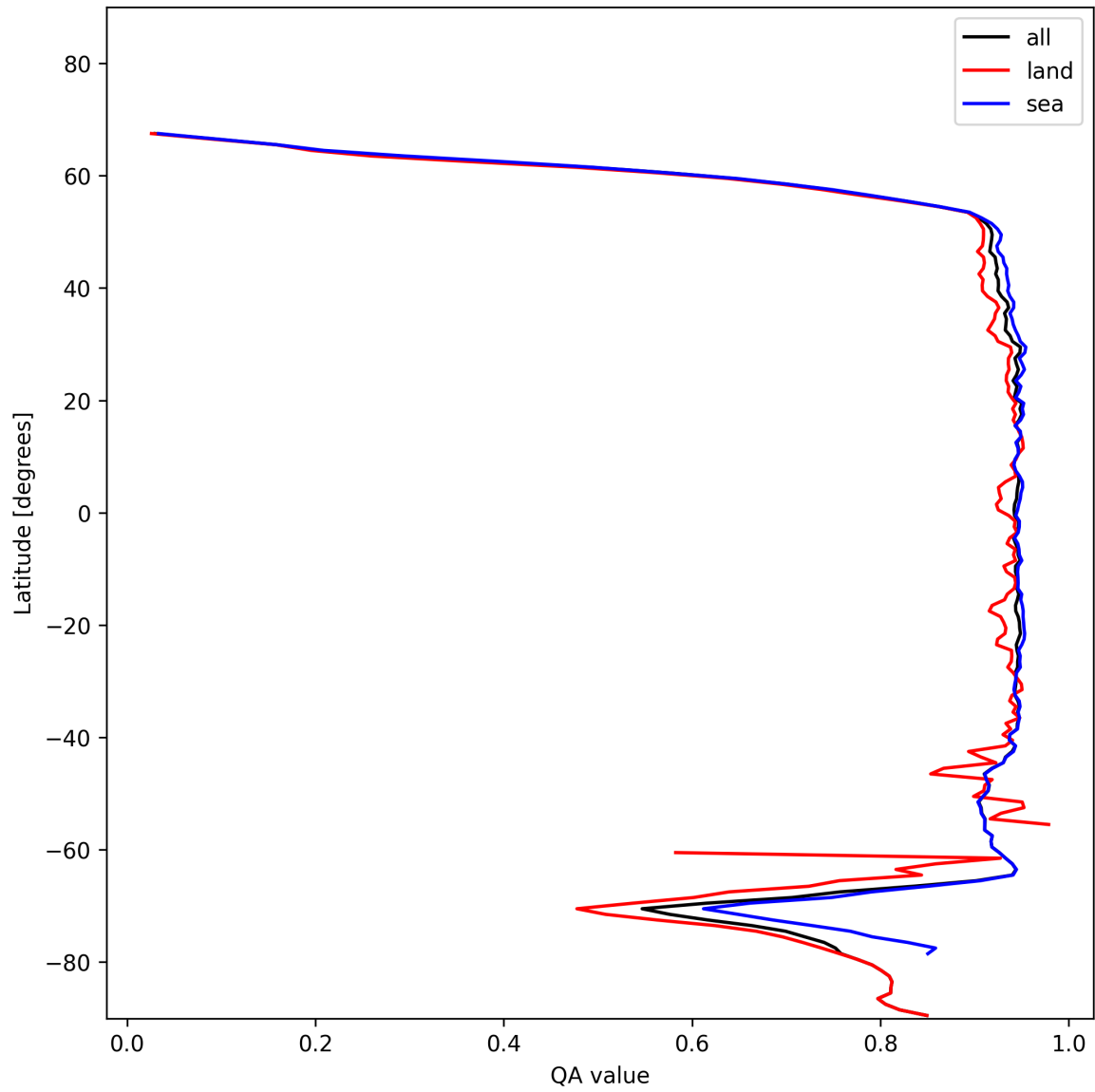
Figure 13: Zonal average of “QA value” for 2025-01-13 to 2025-01-15.
