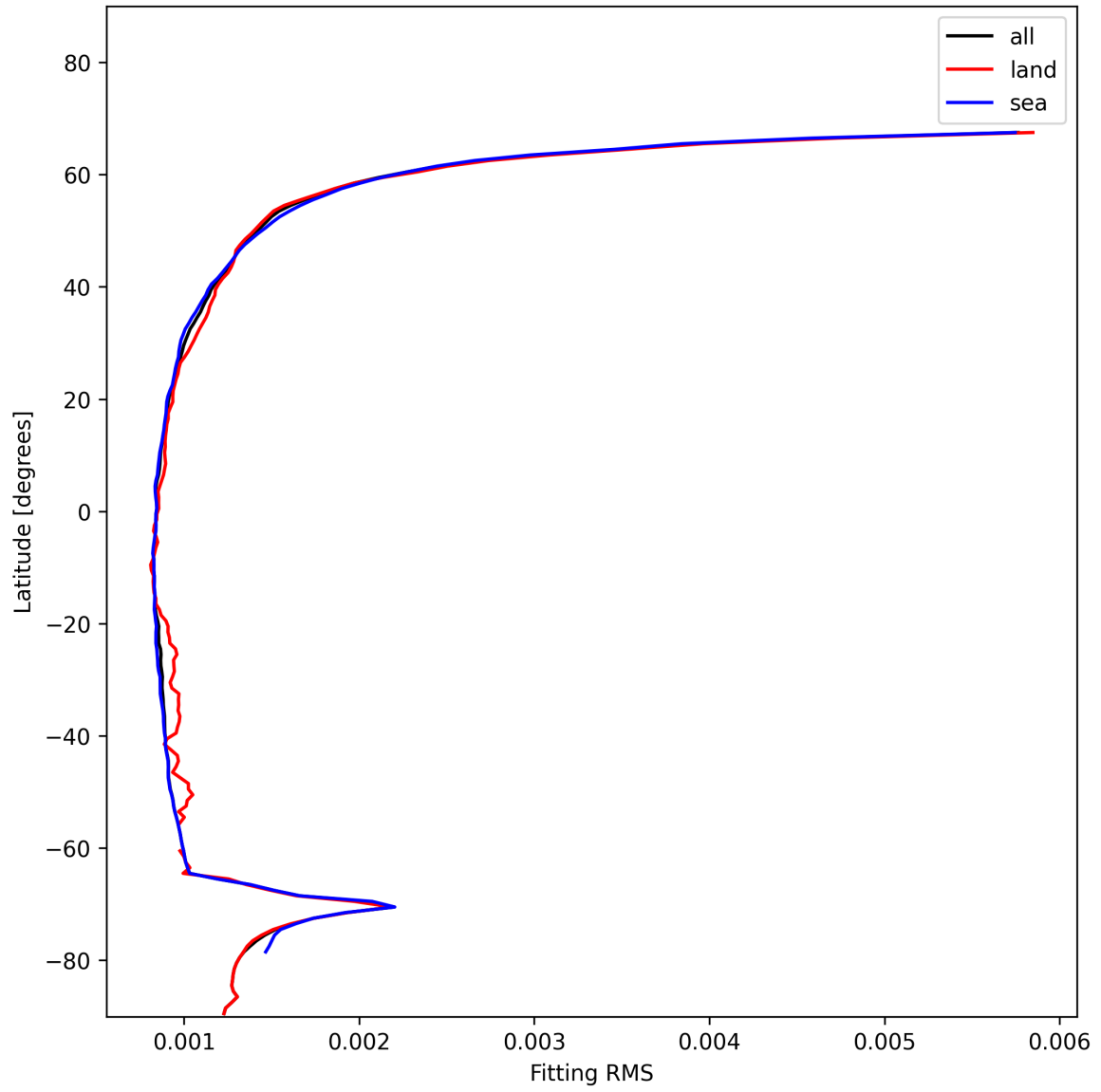
Figure 16: Zonal average of “Fitting RMS” for 2025-01-13 to 2025-01-15.
