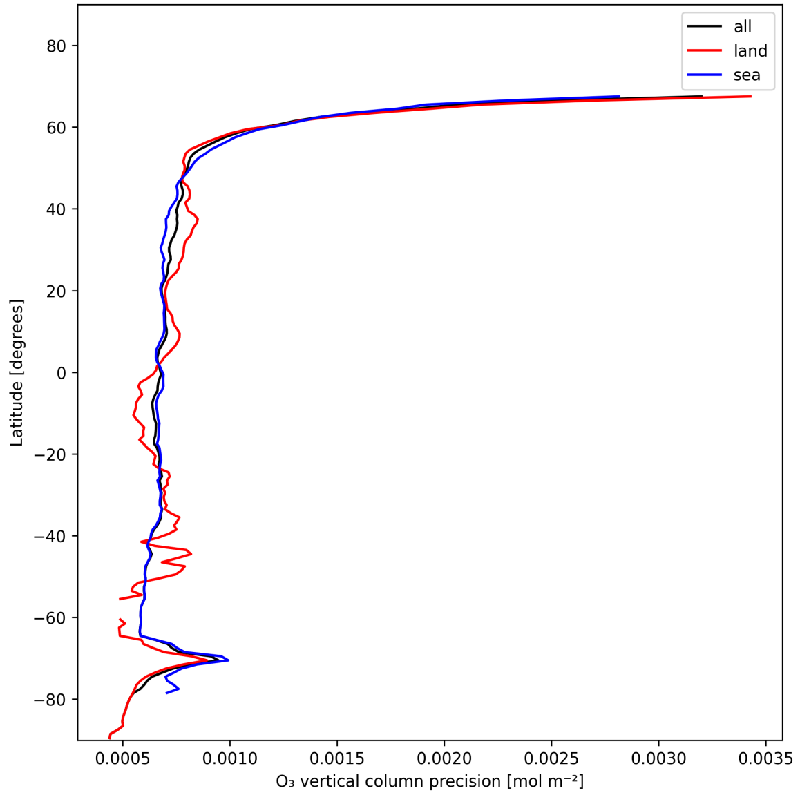
Figure 15: Zonal average of “O 3 vertical column precision” for 2025-01-13 to 2025-01-15.
