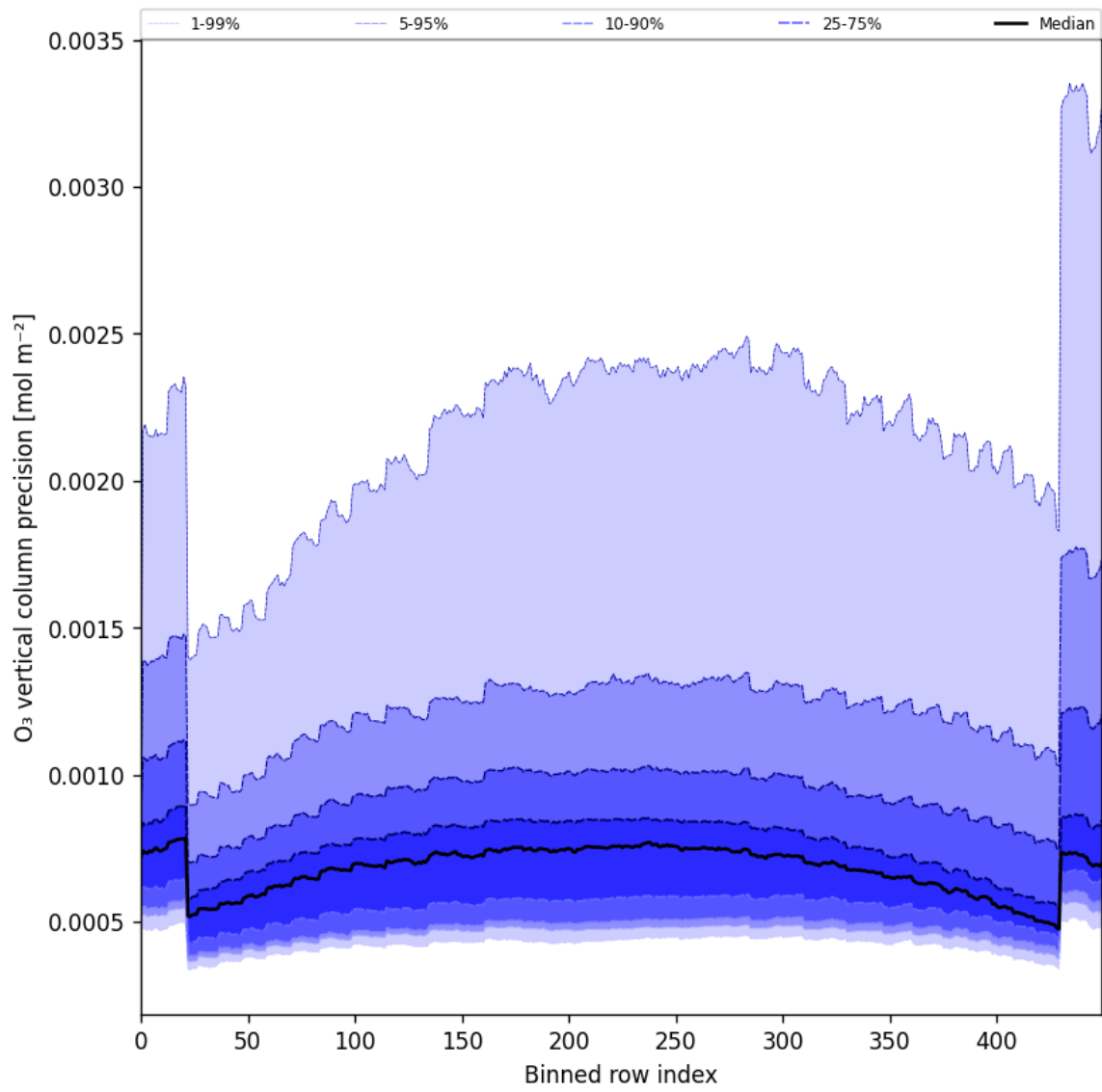
Figure 29: Along track statistics of “O 3 vertical column precision” for 2025-01-13 to 2025-01-15
