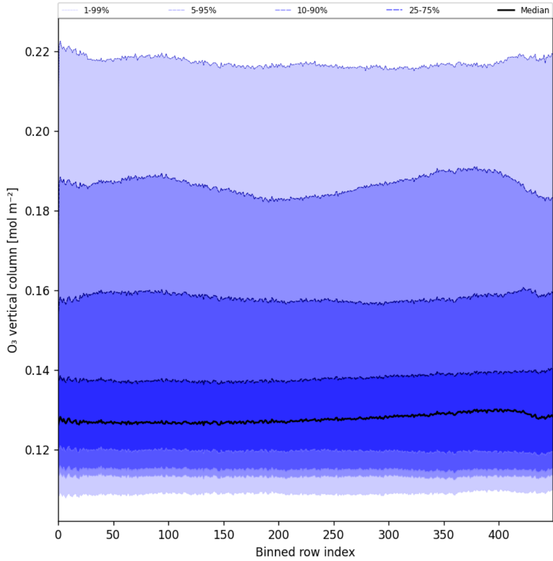
Figure 28: Along track statistics of “O 3 vertical column” for 2025-01-13 to 2025-01-15
