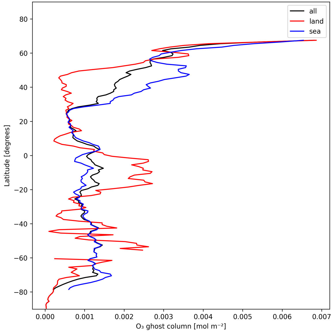
Figure 18: Zonal average of “O 3 ghost column” for 2025-01-13 to 2025-01-15.
