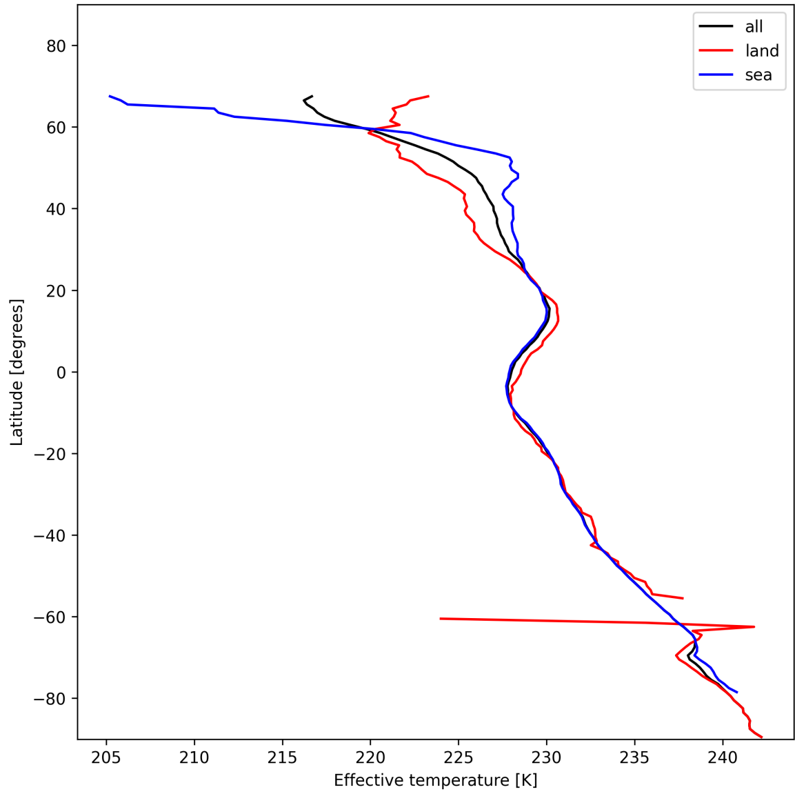
Figure 17: Zonal average of "Effective temperature" for 2025-01-13 to 2025-01-15.
