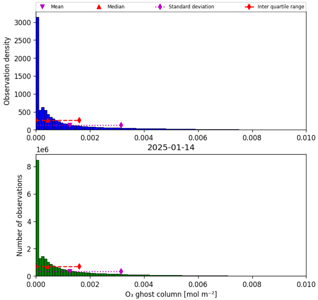
Figure 25: Histogram of "O 3 ghost column" for 2025-01-13 to 2025-01-15
