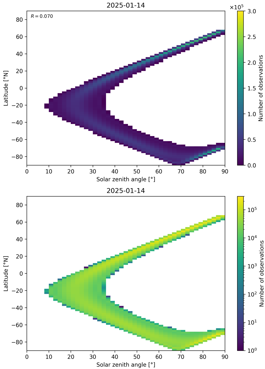
Figure 44: Scatter density plot of “Solar zenith angle” against “Latitude” for 2025-01-13 to 2025-01-15.
