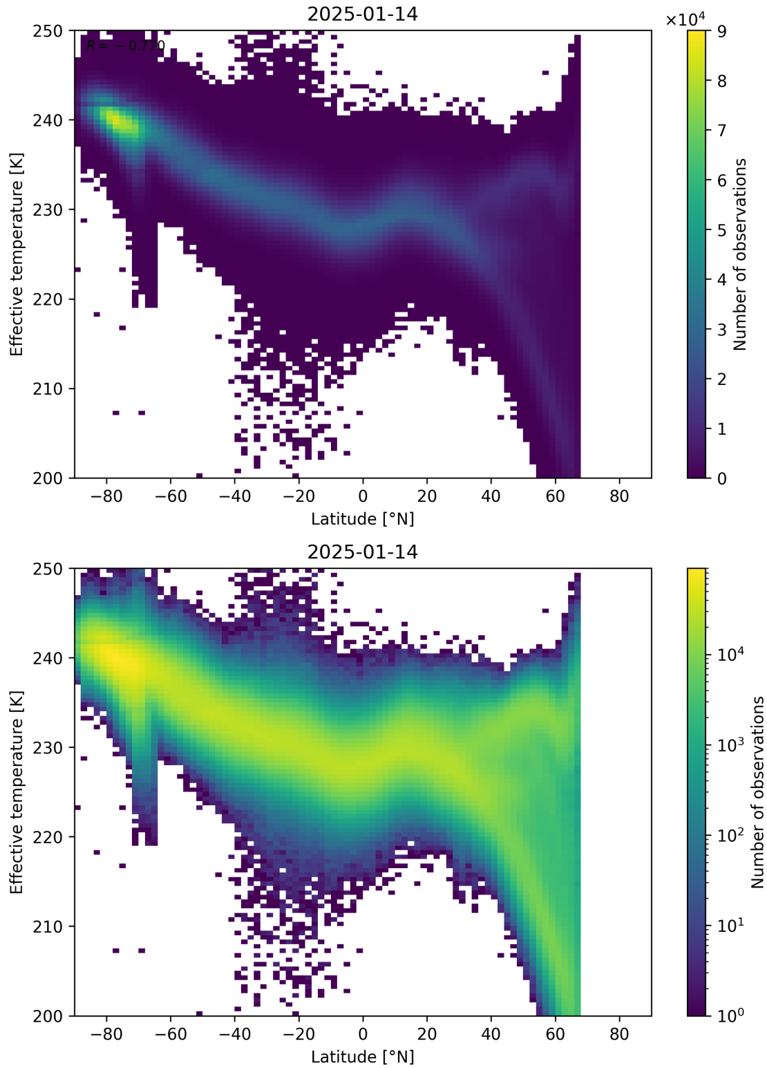
Figure 34: Scatter density plot of “Latitude” against “Effective temperature” for 2025-01-13 to 2025-01-15.
