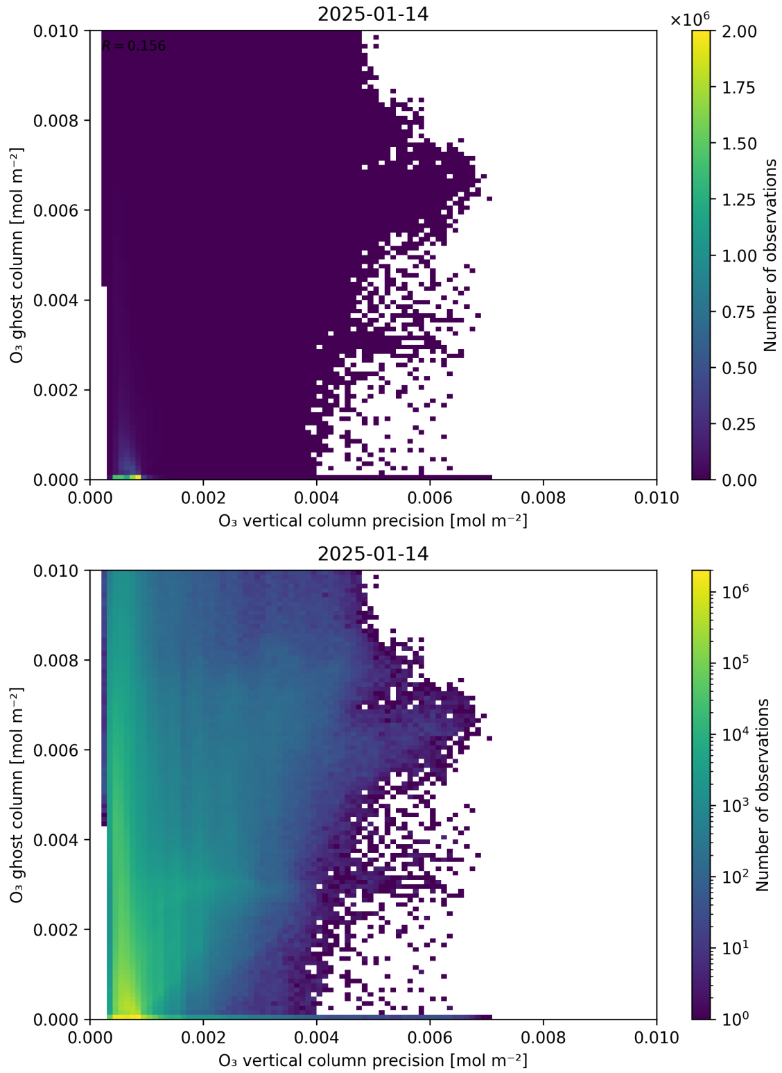
Figure 43: Scatter density plot of “ \text{O}_3 vertical column precision” against “ \text{O}_3 ghost column” for 2025-01-13 to 2025-01-15.
