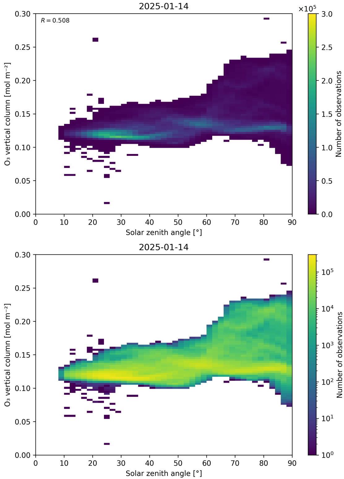
Figure 47: Scatter density plot of “Solar zenith angle” against “O 3 vertical column” for 2025-01-13 to 2025-01-15.
