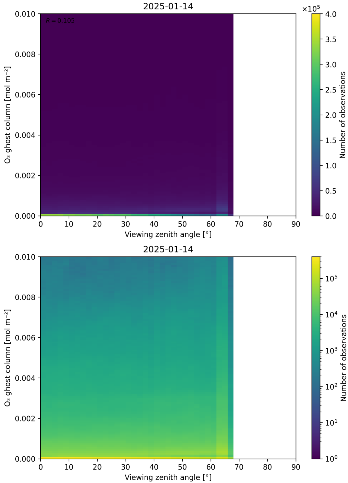
Figure 51: Scatter density plot of “Viewing zenith angle” against “O 3 ghost column” for 2025-01-13 to 2025-01-15.
