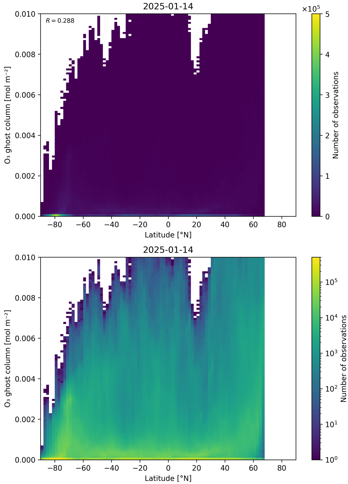
Figure 35: Scatter density plot of “Latitude” against “O 3 ghost column” for 2025-01-13 to 2025-01-15.
