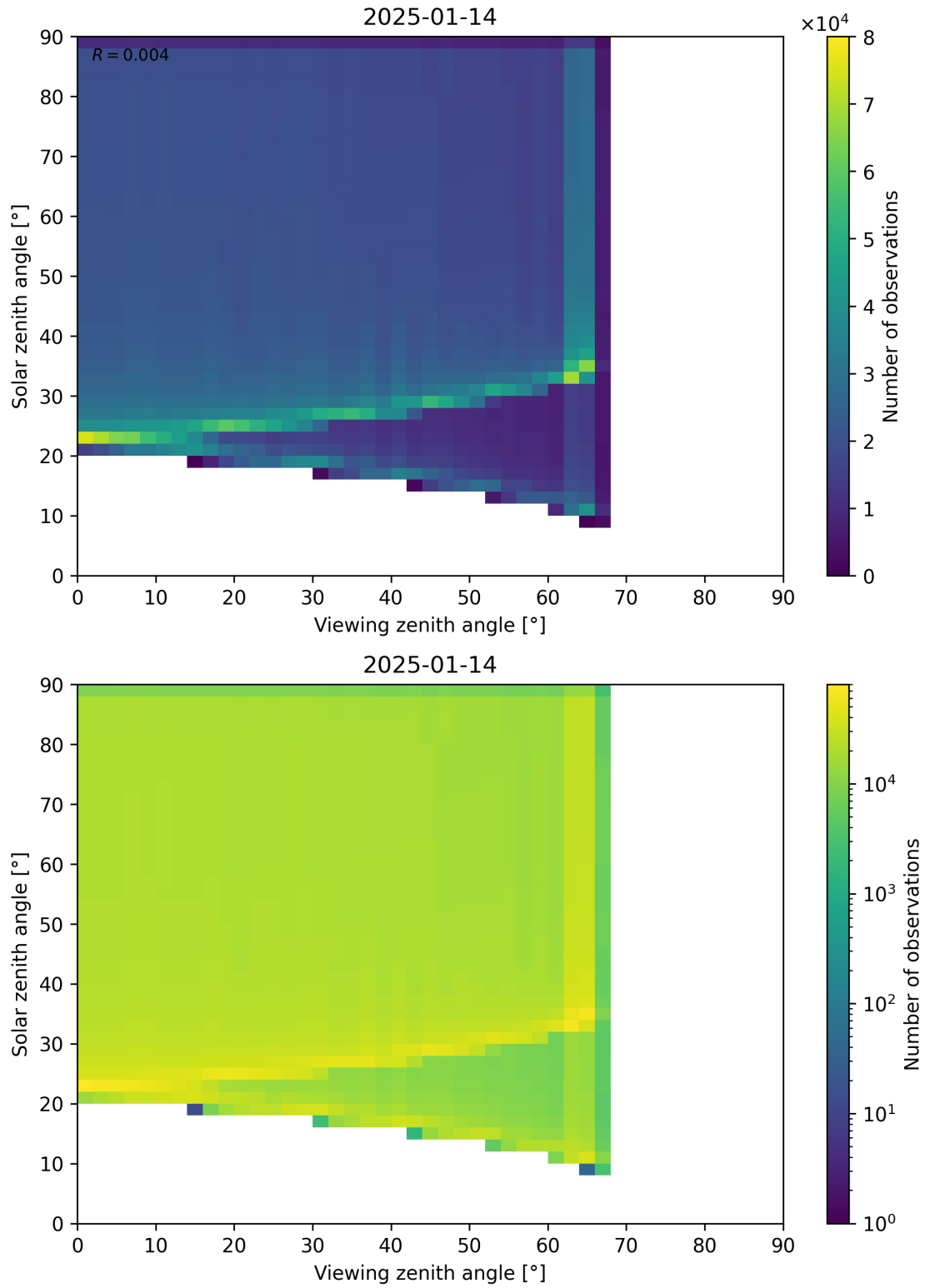
Figure 54: Scatter density plot of “Viewing zenith angle” against “Solar zenith angle” for 2025-01-13 to 2025-01-15.
