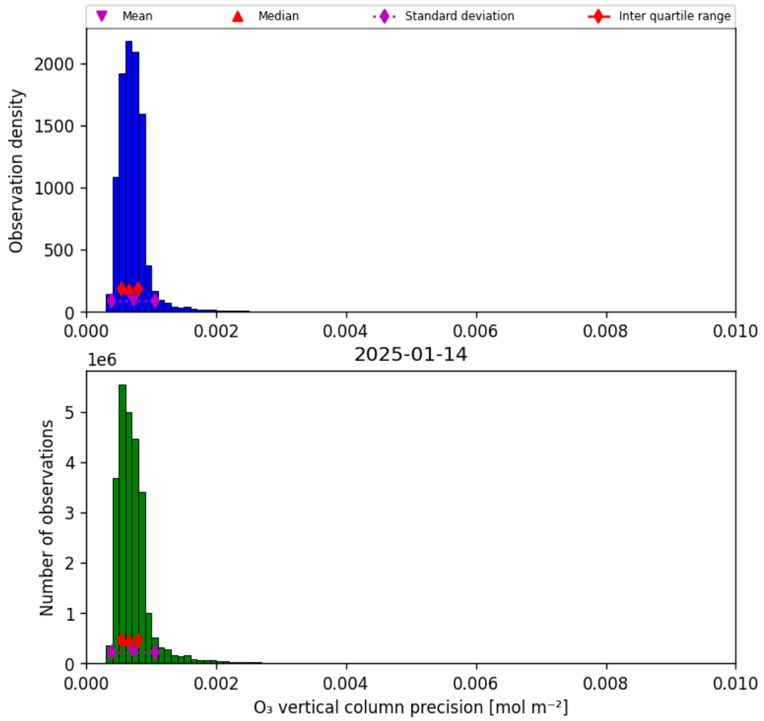
Figure 22: Histogram of “O 3 vertical column precision” for 2025-01-13 to 2025-01-15
