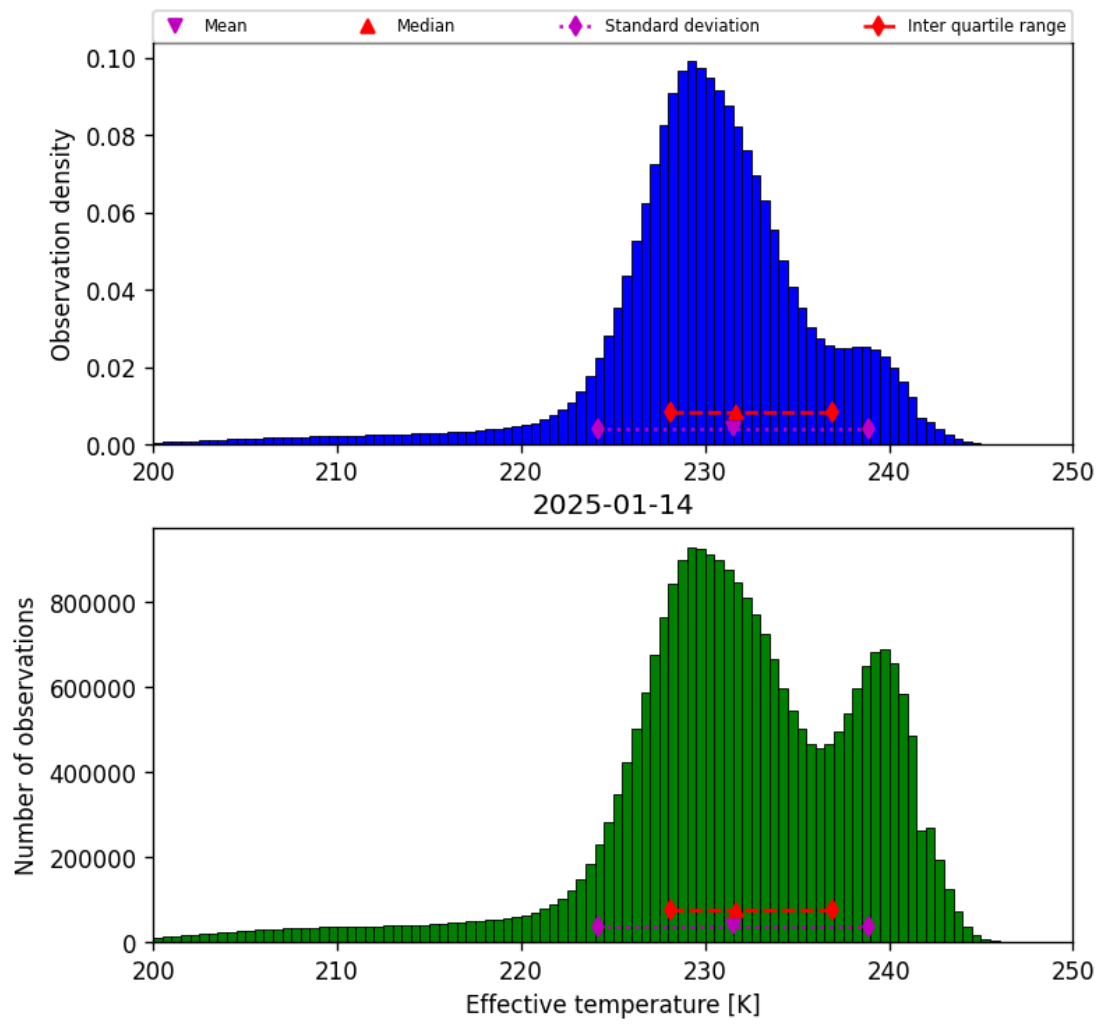
Figure 24: Histogram of “Effective temperature” for 2025-01-13 to 2025-01-15
