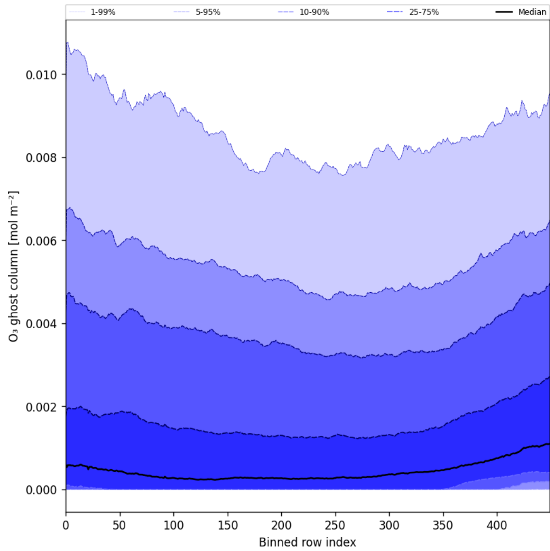
Figure 32: Along track statistics of “O 3 ghost column” for 2025-01-13 to 2025-01-15
