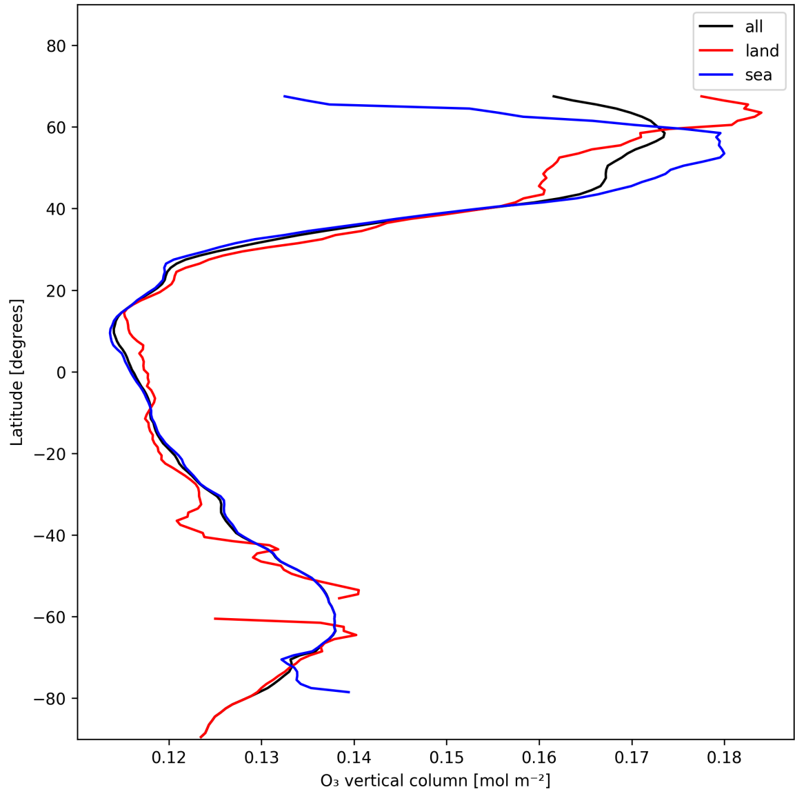
Figure 14: Zonal average of “O 3 vertical column” for 2025-01-13 to 2025-01-15.
