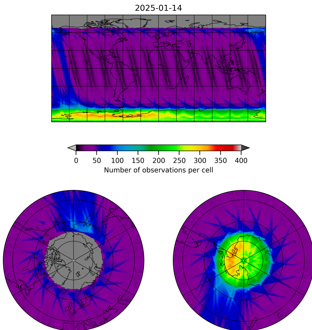
Figure 12: Map of the number of observations for 2025-01-13 to 2025-01-15
