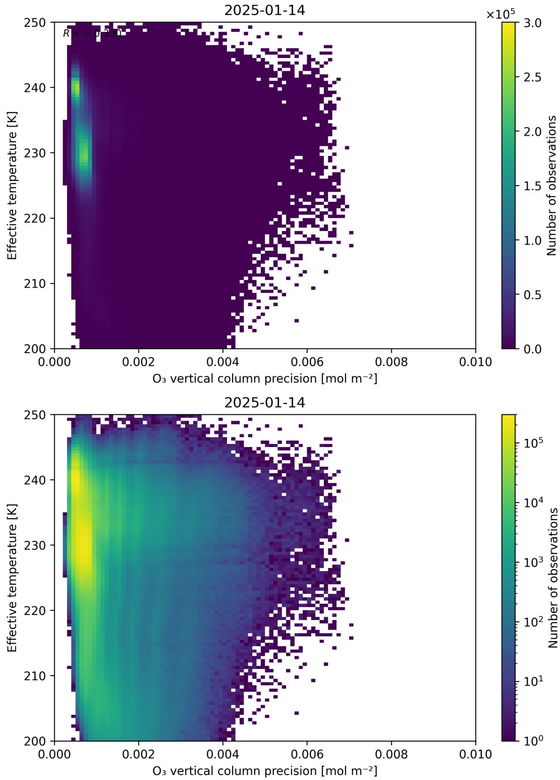
Figure 42: Scatter density plot of “O 3 vertical column precision” against “Effective temperature” for 2025-01-13 to 2025-01-15.
