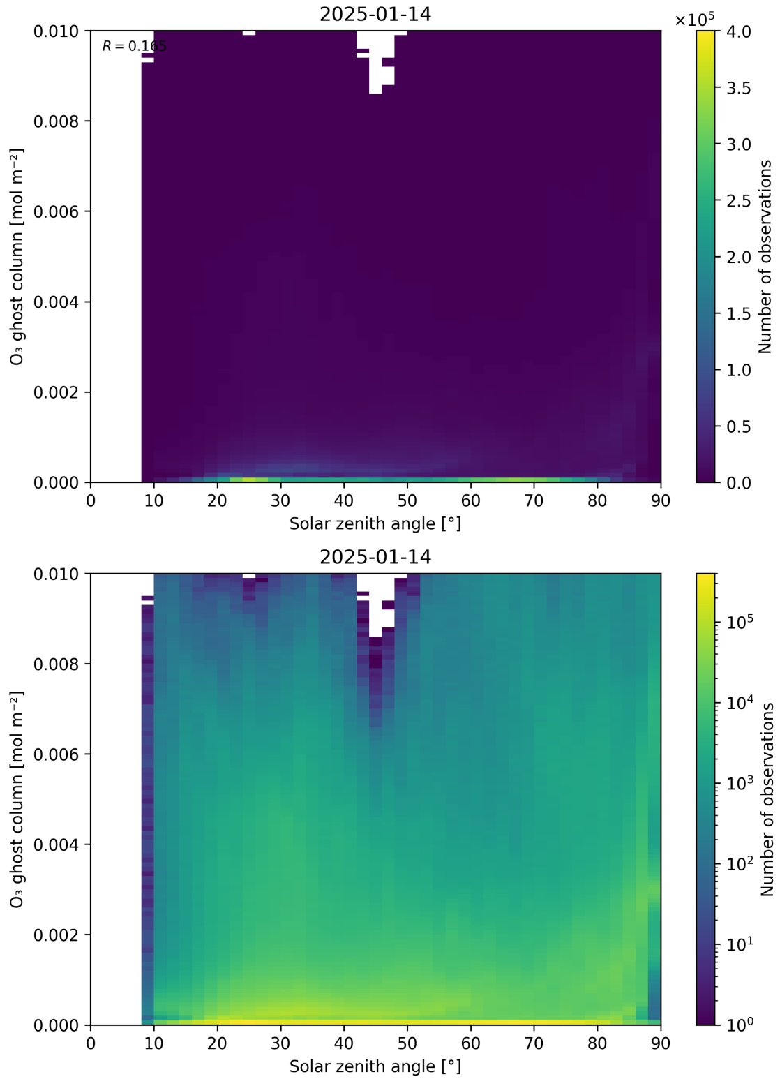
Figure 46: Scatter density plot of “Solar zenith angle” against “O 3 ghost column” for 2025-01-13 to 2025-01-15.
