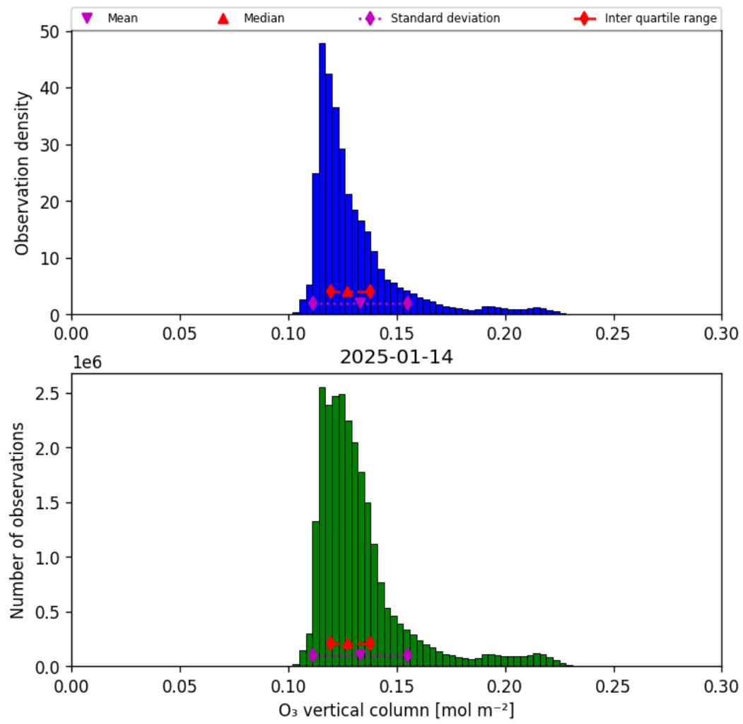
Figure 21: Histogram of “O 3 vertical column” for 2025-01-13 to 2025-01-15
