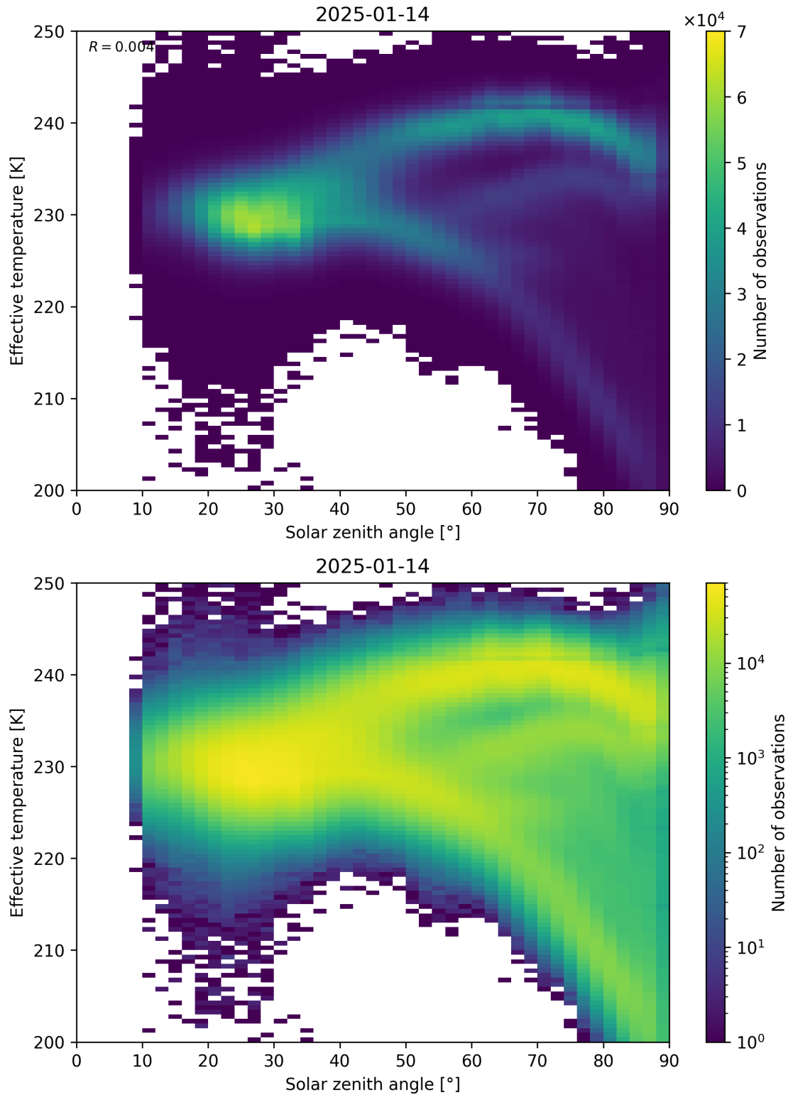
Figure 45: Scatter density plot of “Solar zenith angle” against “Effective temperature” for 2025-01-13 to 2025-01-15.
