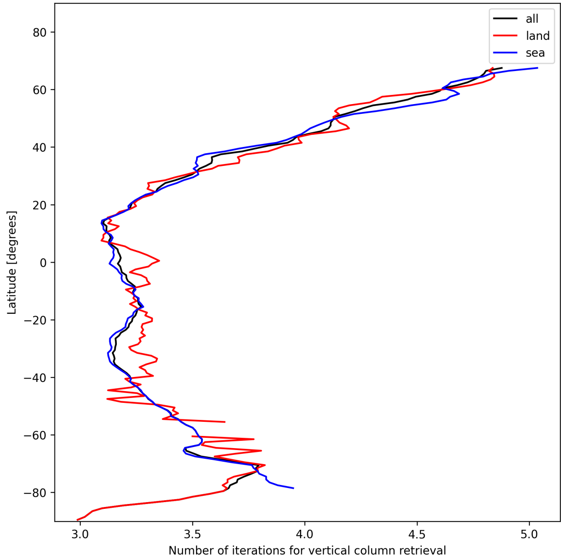
Figure 19: Zonal average of “Number of iterations for vertical column retrieval” for 2025-01-13 to 2025-01-15.
