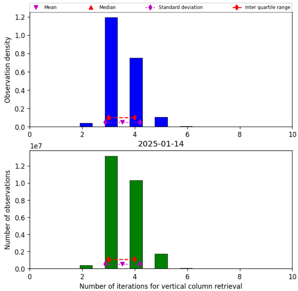
Figure 26: Histogram of “Number of iterations for vertical column retrieval” for 2025-01-13 to 2025-01-15
