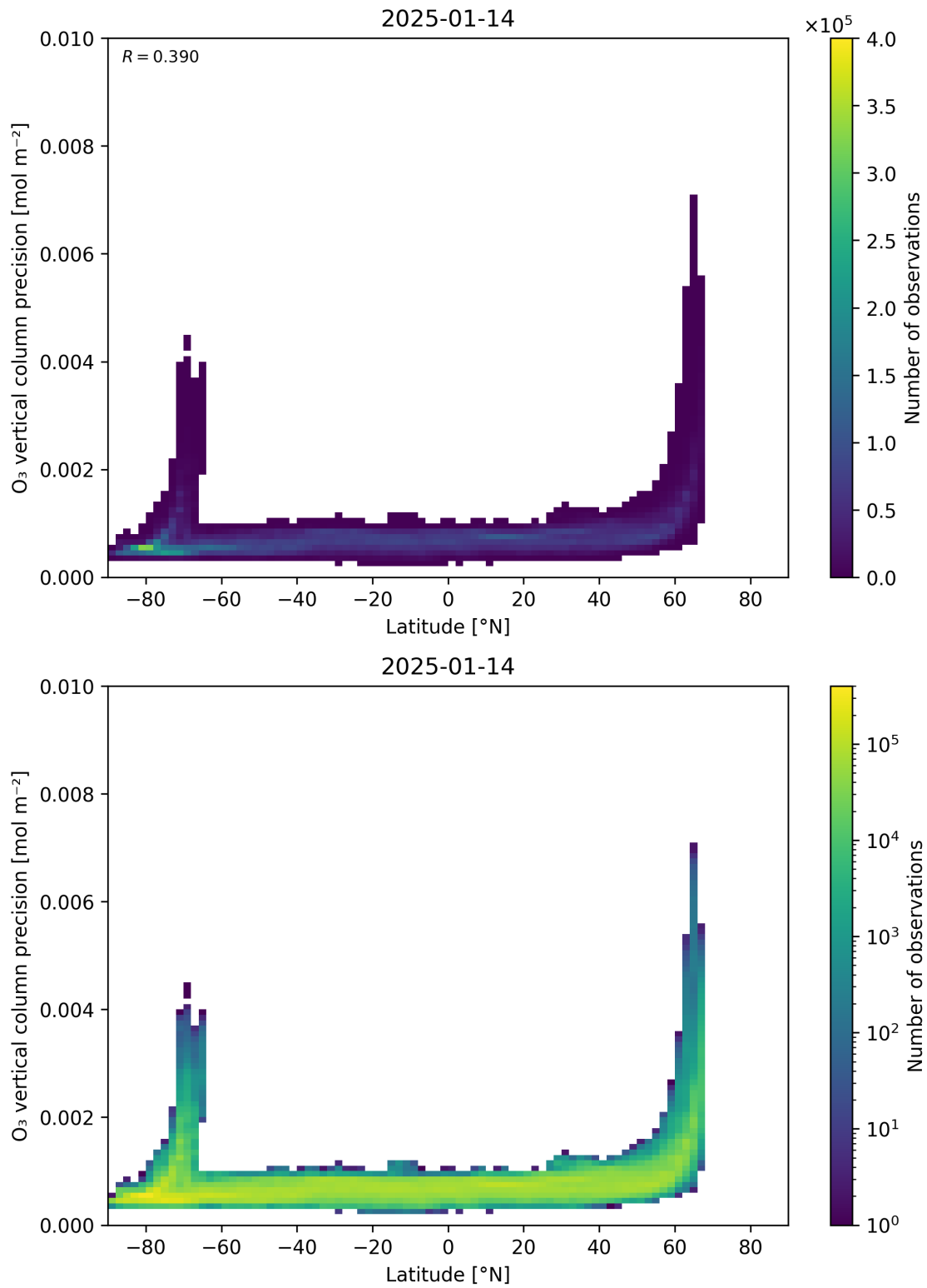
Figure 37: Scatter density plot of “Latitude” against “O 3 vertical column precision” for 2025-01-13 to 2025-01-15.
