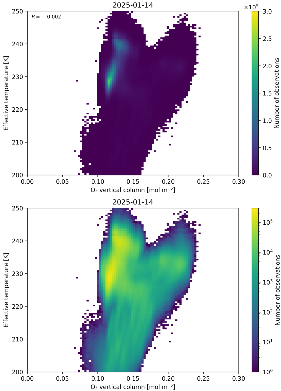
Figure 39: Scatter density plot of “O 3 vertical column” against “Effective temperature” for 2025-01-13 to 2025-01-15.
