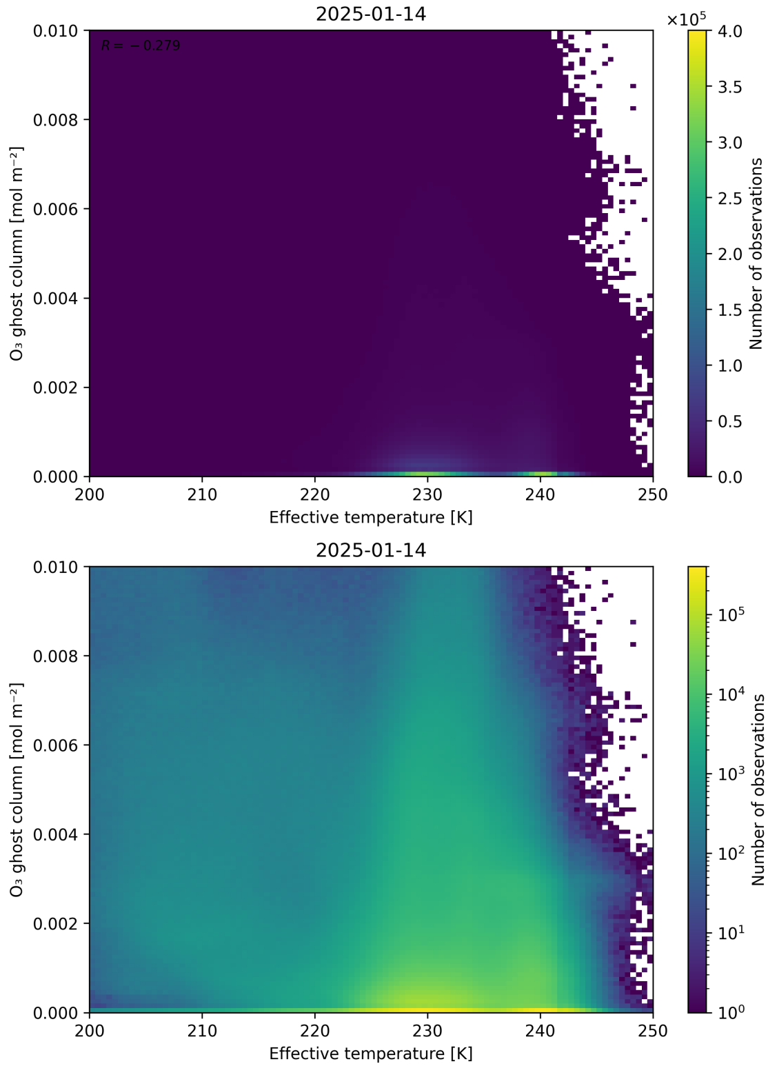
Figure 38: Scatter density plot of “Effective temperature” against “O 3 ghost column” for 2025-01-13 to 2025-01-15.
