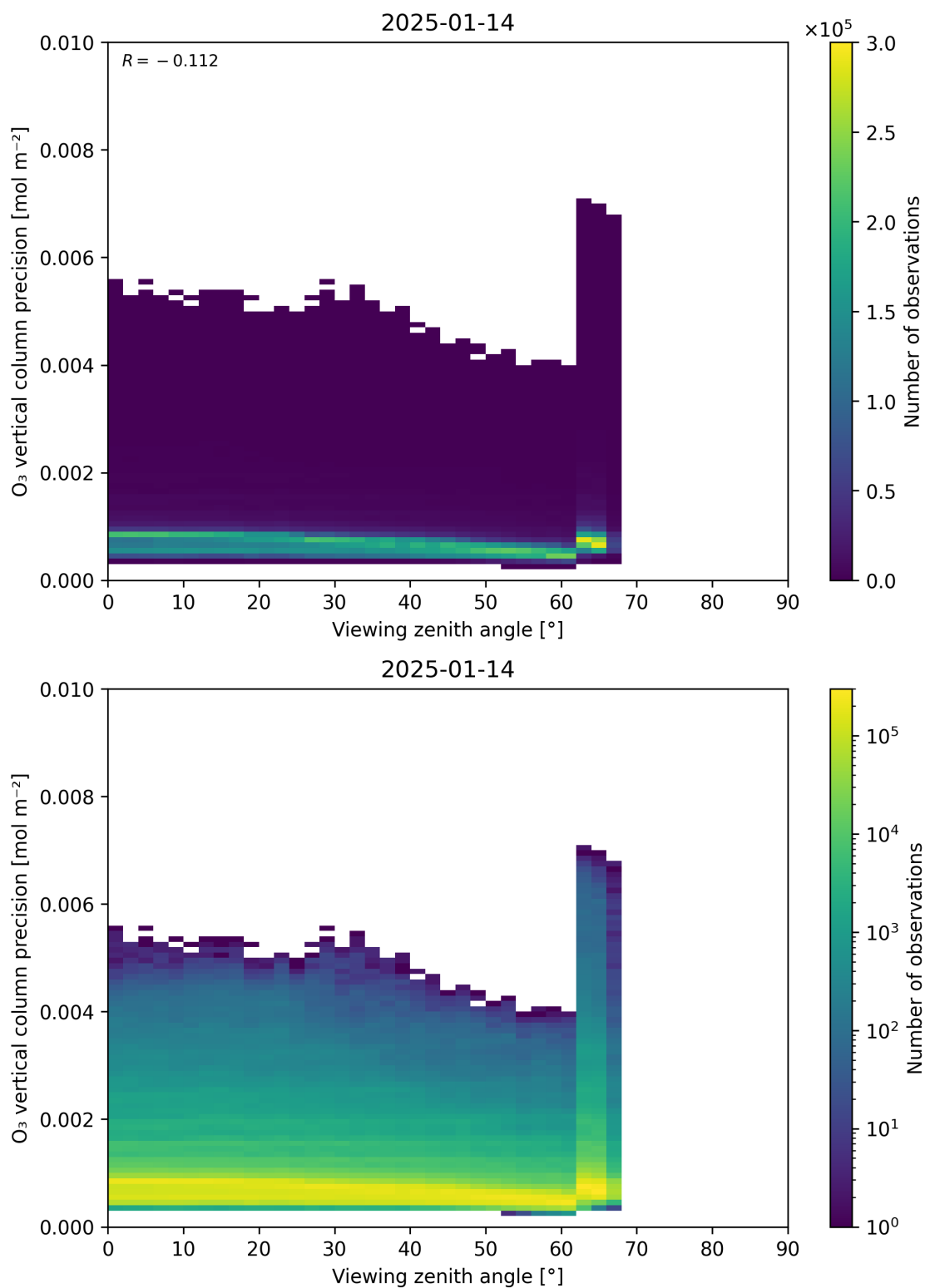
Figure 53: Scatter density plot of “Viewing zenith angle” against “O 3 vertical column precision” for 2025-01-13 to 2025-01-15.
