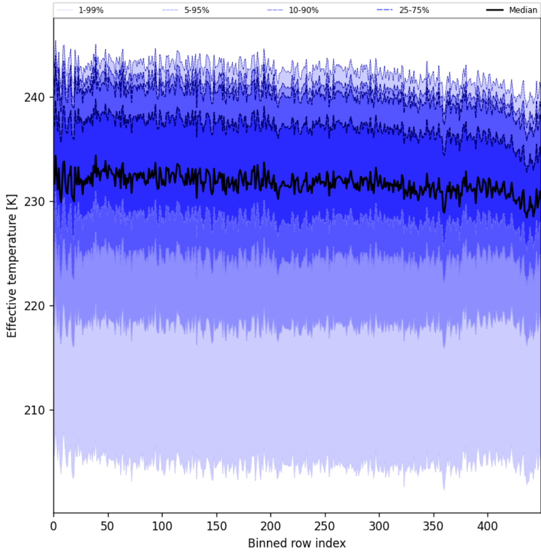
Figure 31: Along track statistics of “Effective temperature” for 2025-01-13 to 2025-01-15
