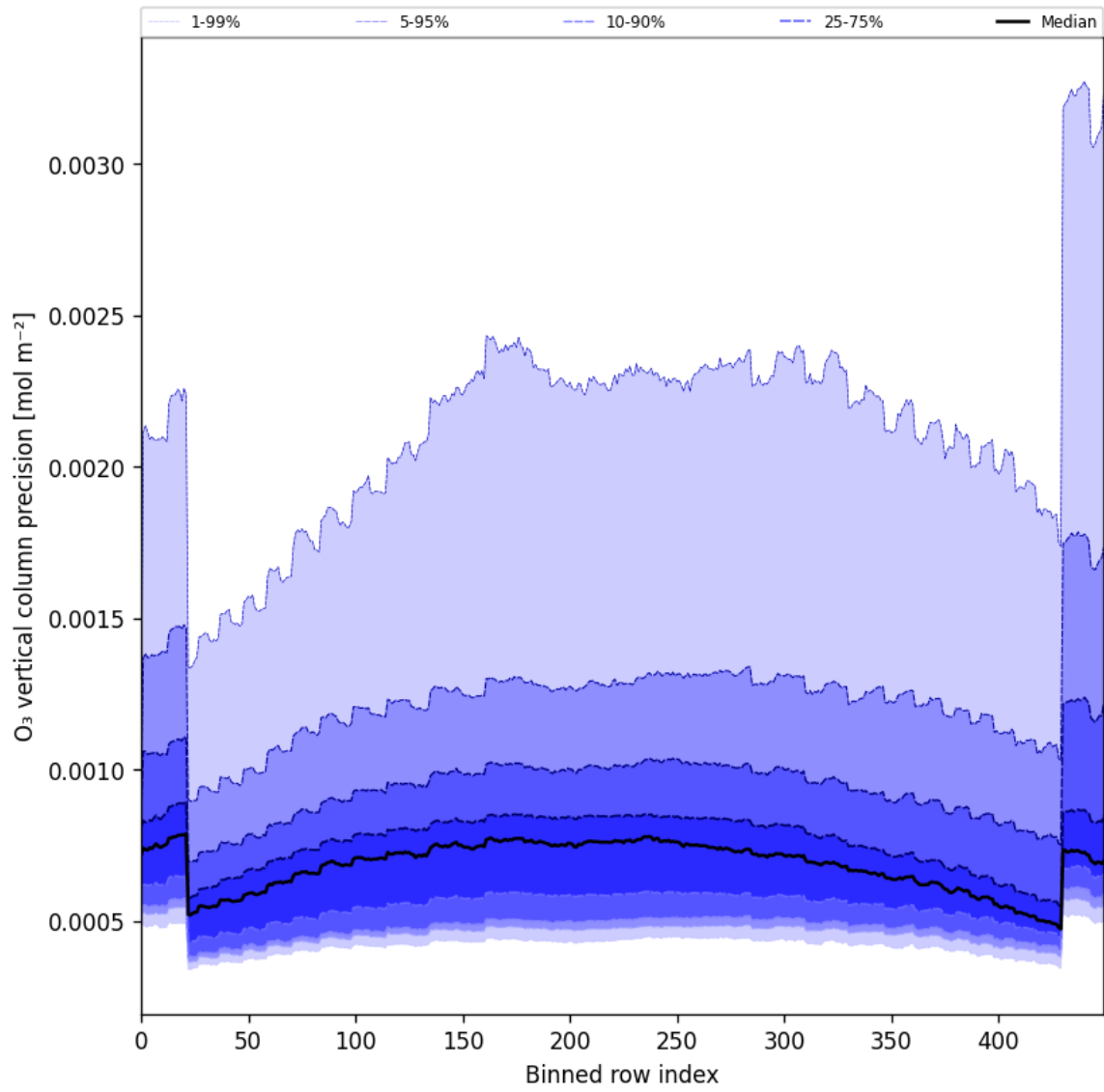
Figure 29: Along track statistics of “O 3 vertical column precision” for 2025-01-14 to 2025-01-16
