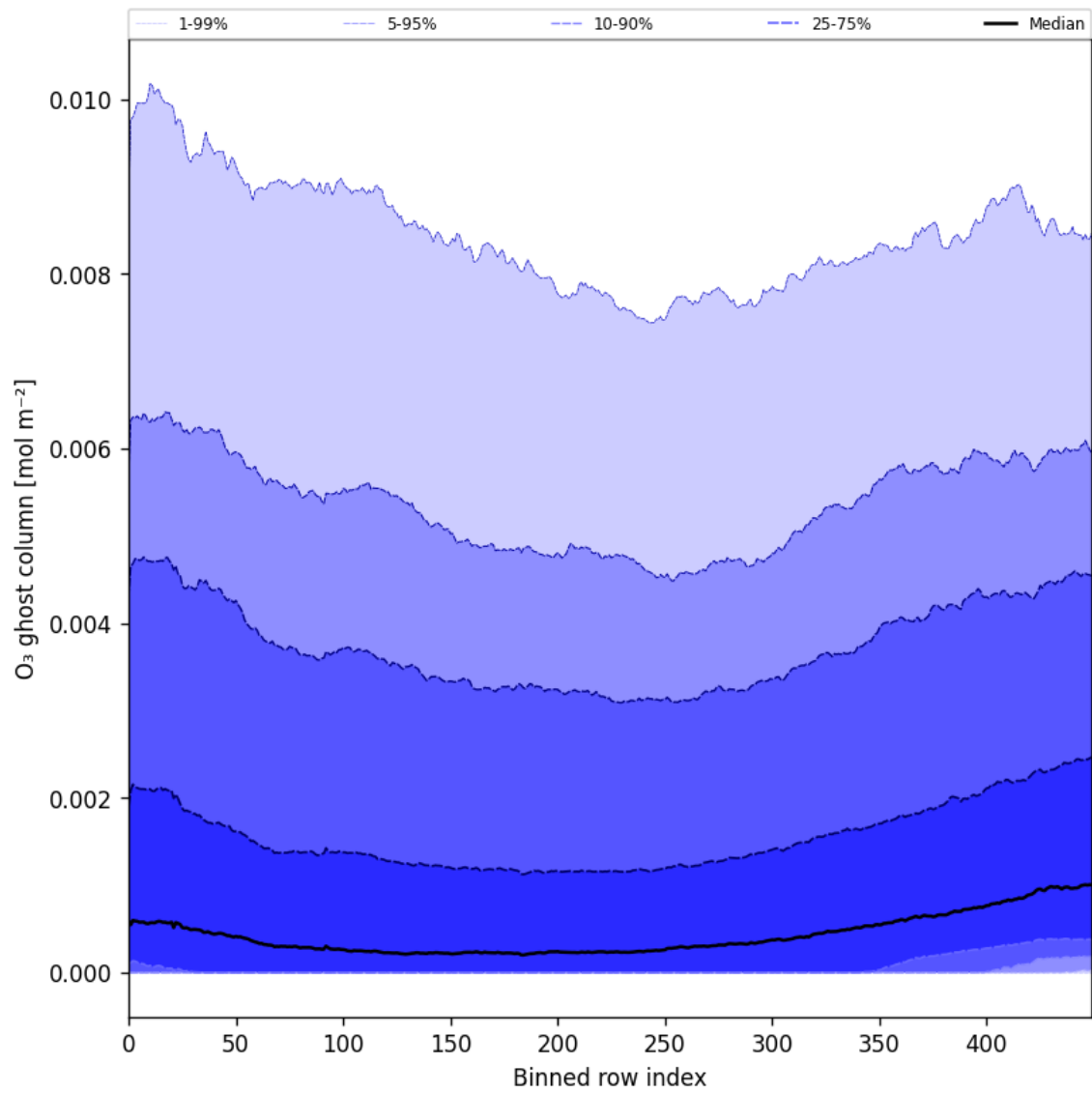
Figure 32: Along track statistics of “O 3 ghost column” for 2025-01-14 to 2025-01-16
