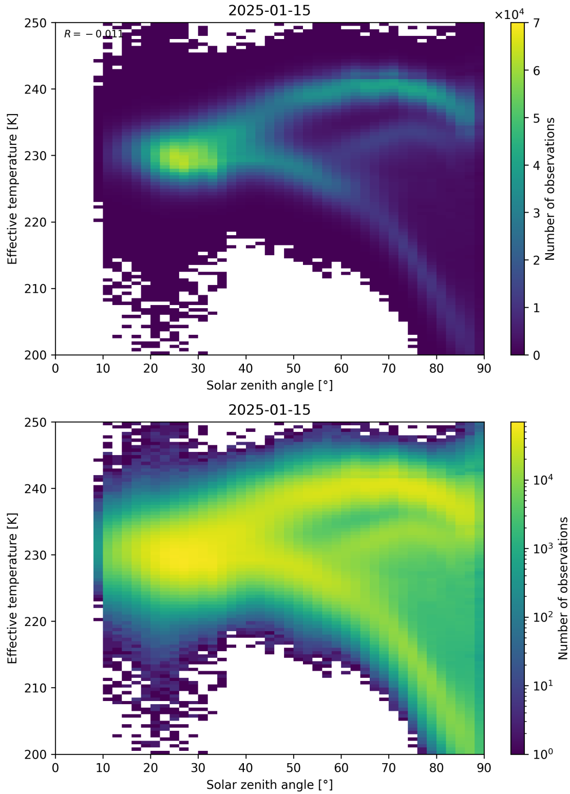
Figure 45: Scatter density plot of “Solar zenith angle” against “Effective temperature” for 2025-01-14 to 2025-01-16.
