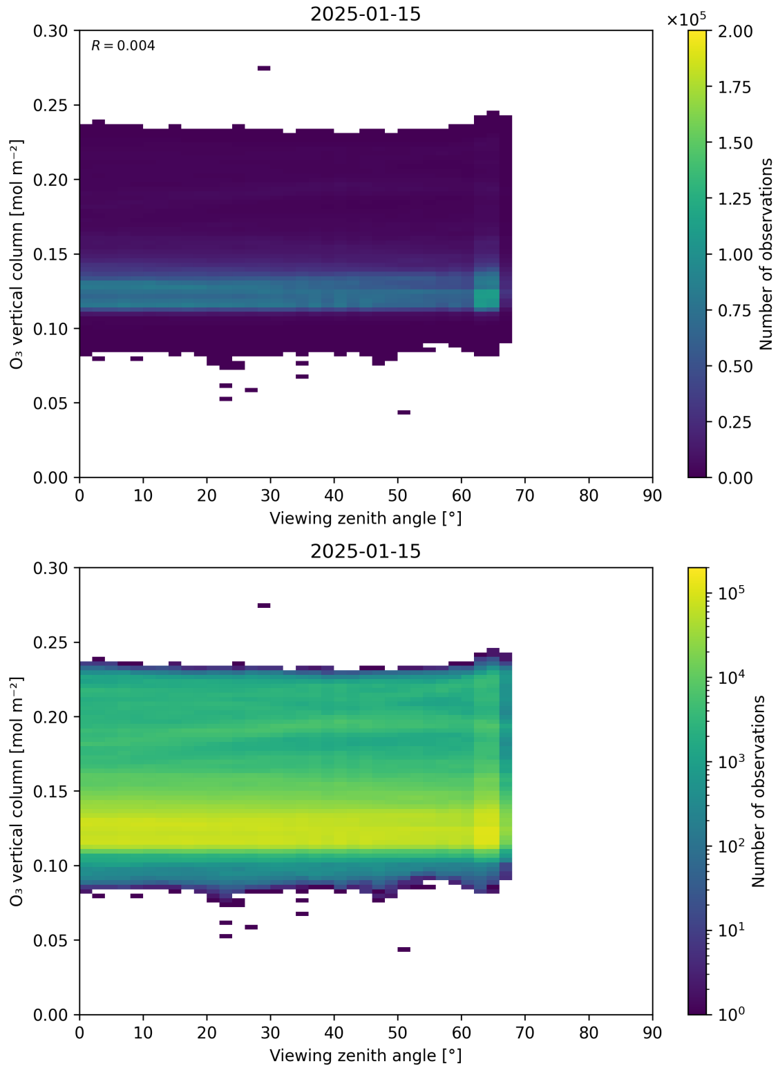
Figure 52: Scatter density plot of “Viewing zenith angle” against “O 3 vertical column” for 2025-01-14 to 2025-01-16.
