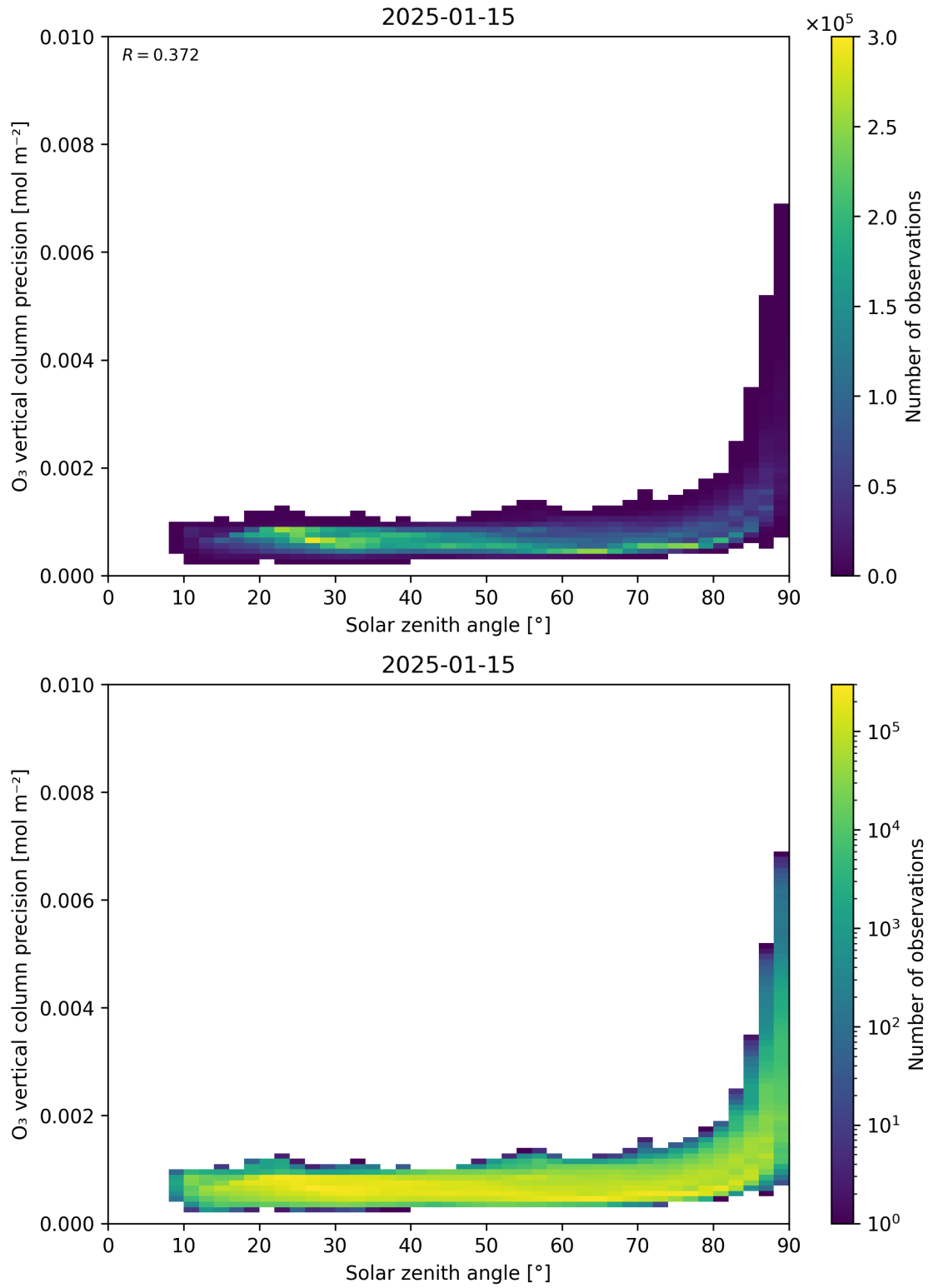
Figure 48: Scatter density plot of “Solar zenith angle” against “O 3 vertical column precision” for 2025-01-14 to 2025-01-16.
