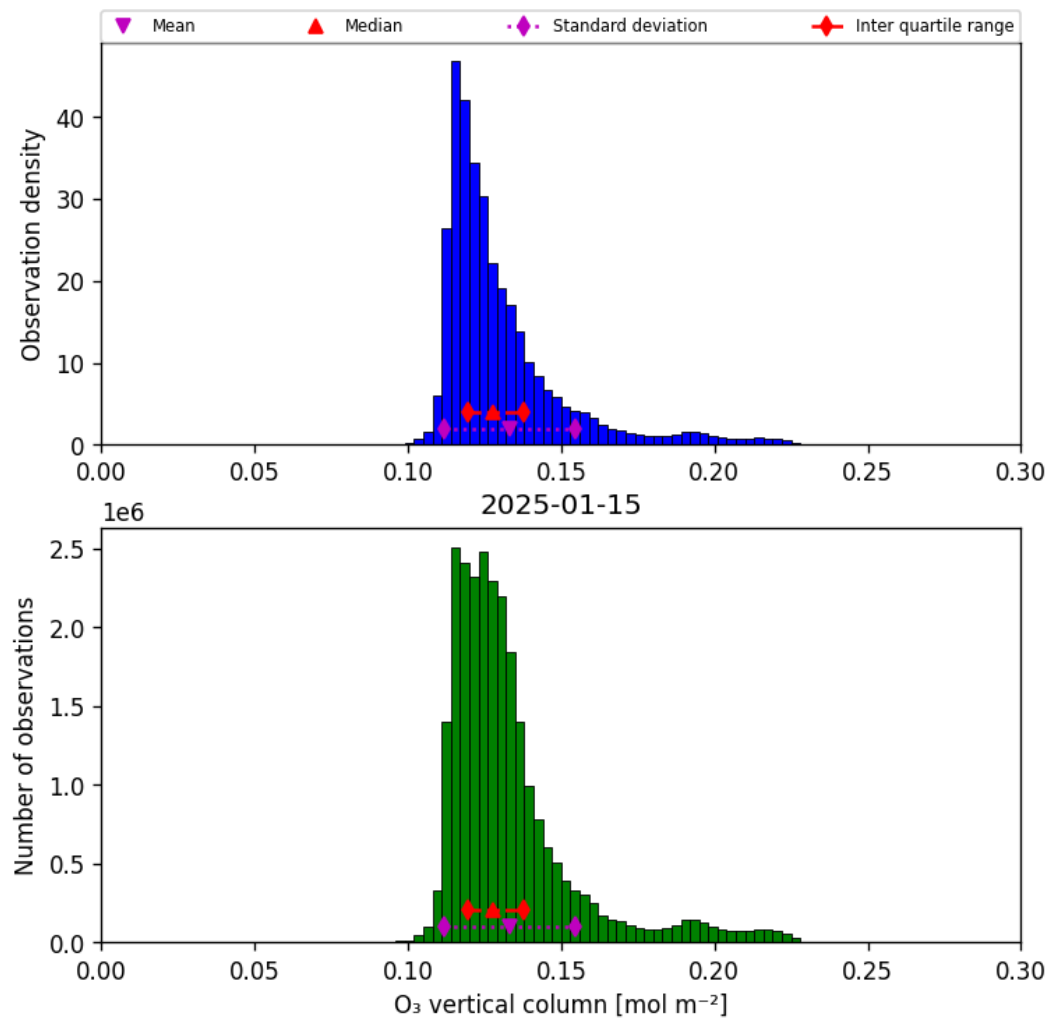
Figure 21: Histogram of “O 3 vertical column” for 2025-01-14 to 2025-01-16
