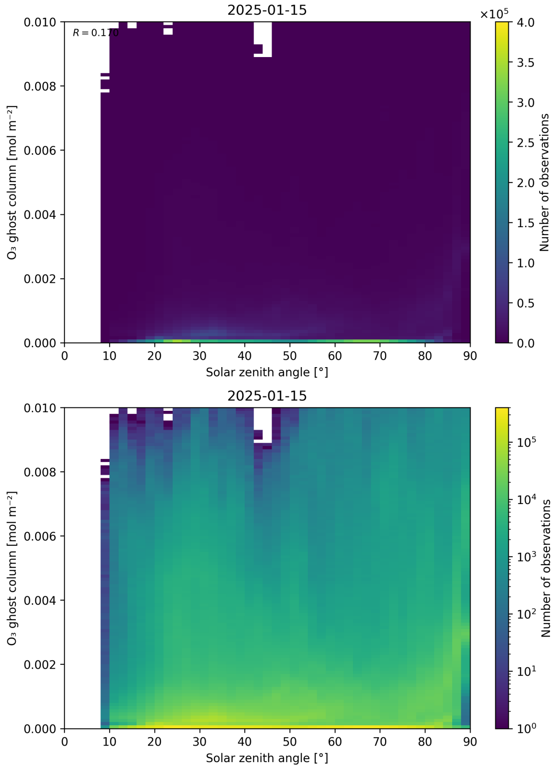
Figure 46: Scatter density plot of “Solar zenith angle” against “O 3 ghost column” for 2025-01-14 to 2025-01-16.
