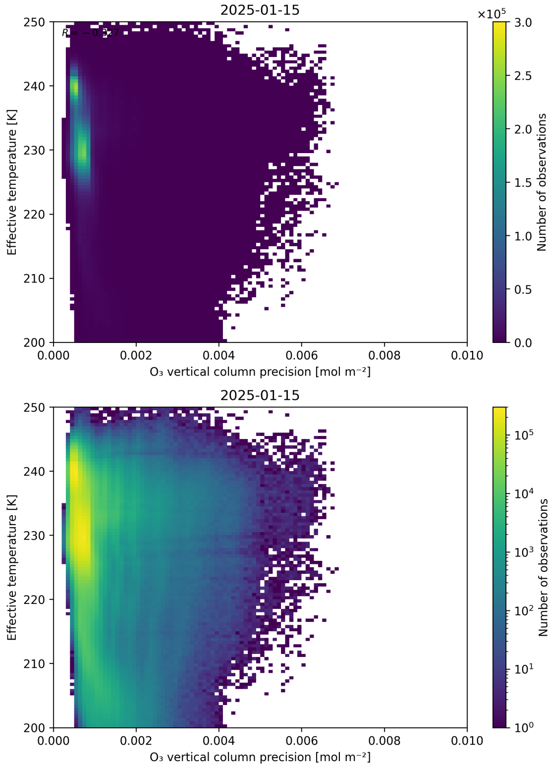
Figure 42: Scatter density plot of “O 3 vertical column precision” against “Effective temperature” for 2025-01-14 to 2025-01-16.
