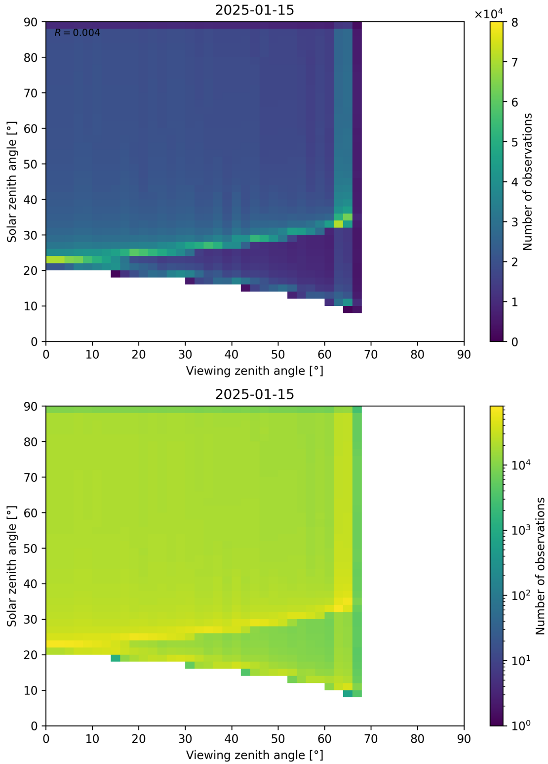
Figure 54: Scatter density plot of “Viewing zenith angle” against “Solar zenith angle” for 2025-01-14 to 2025-01-16.
