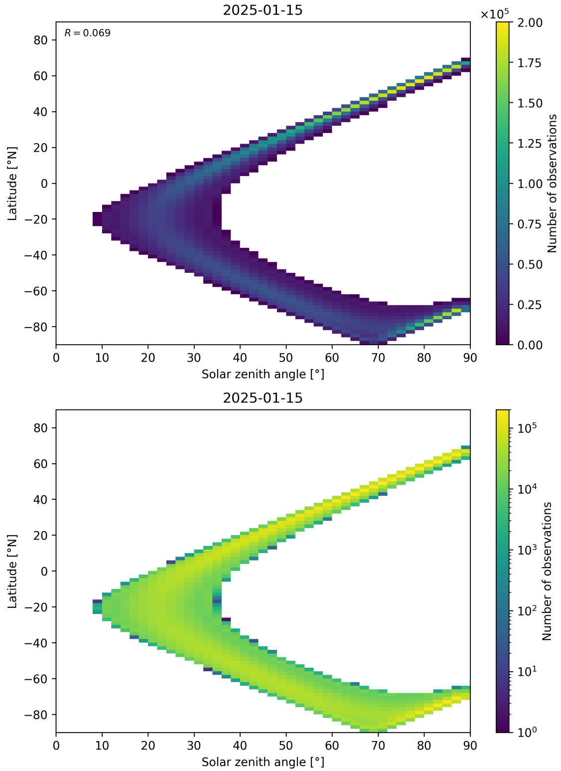
Figure 44: Scatter density plot of “Solar zenith angle” against “Latitude” for 2025-01-14 to 2025-01-16.
