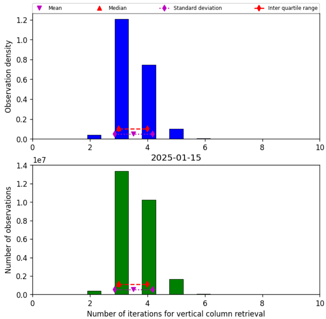
Figure 26: Histogram of “Number of iterations for vertical column retrieval” for 2025-01-14 to 2025-01-16
