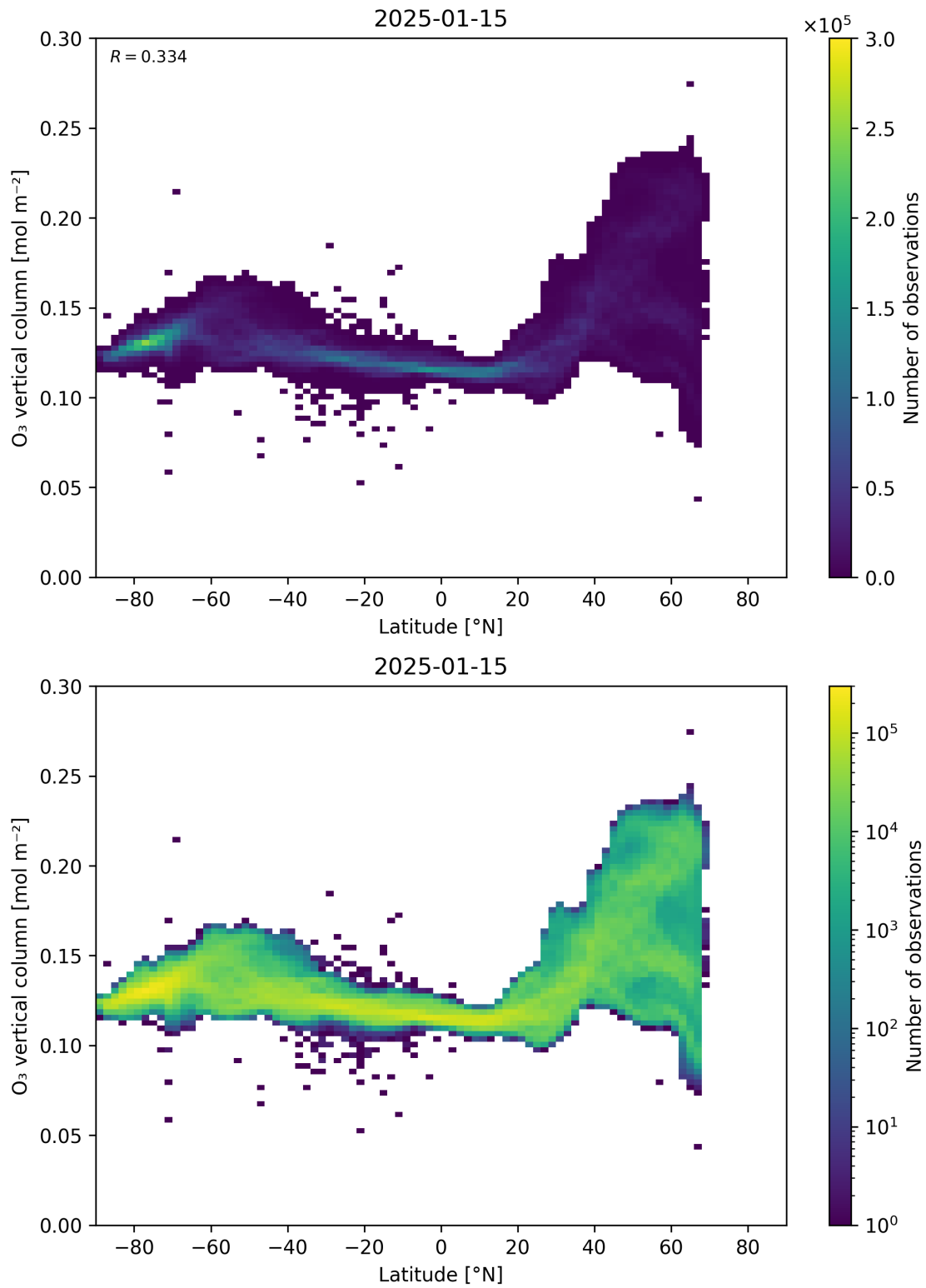
Figure 36: Scatter density plot of “Latitude” against “O 3 vertical column” for 2025-01-14 to 2025-01-16.
