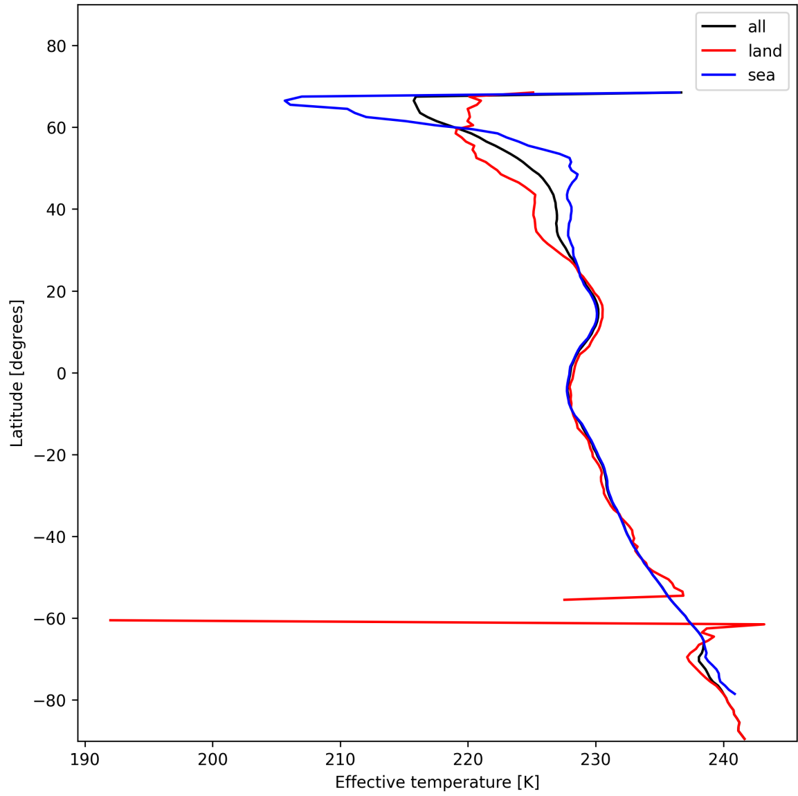
Figure 17: Zonal average of “Effective temperature” for 2025-01-14 to 2025-01-16.
