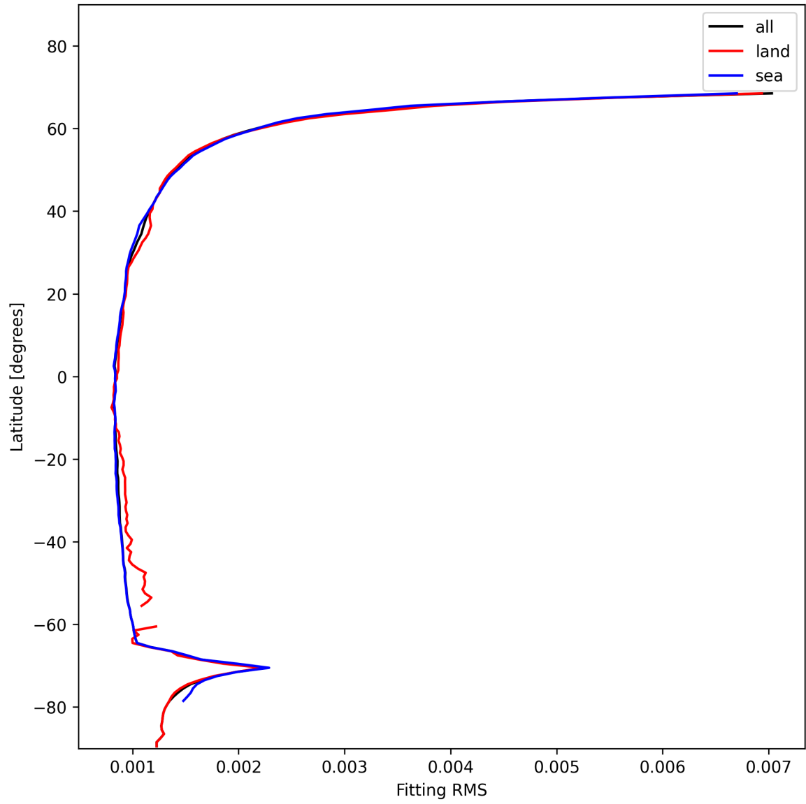
Figure 16: Zonal average of “Fitting RMS” for 2025-01-14 to 2025-01-16.
