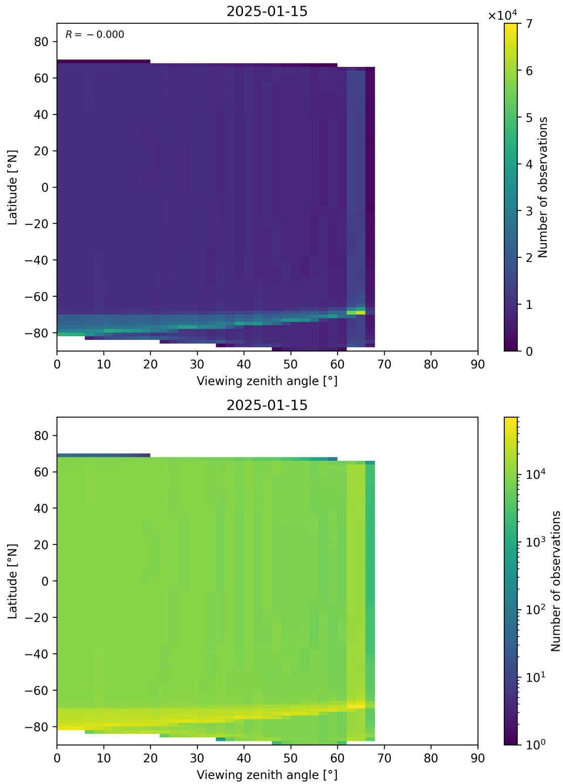
Figure 49: Scatter density plot of “Viewing zenith angle” against “Latitude” for 2025-01-14 to 2025-01-16.
