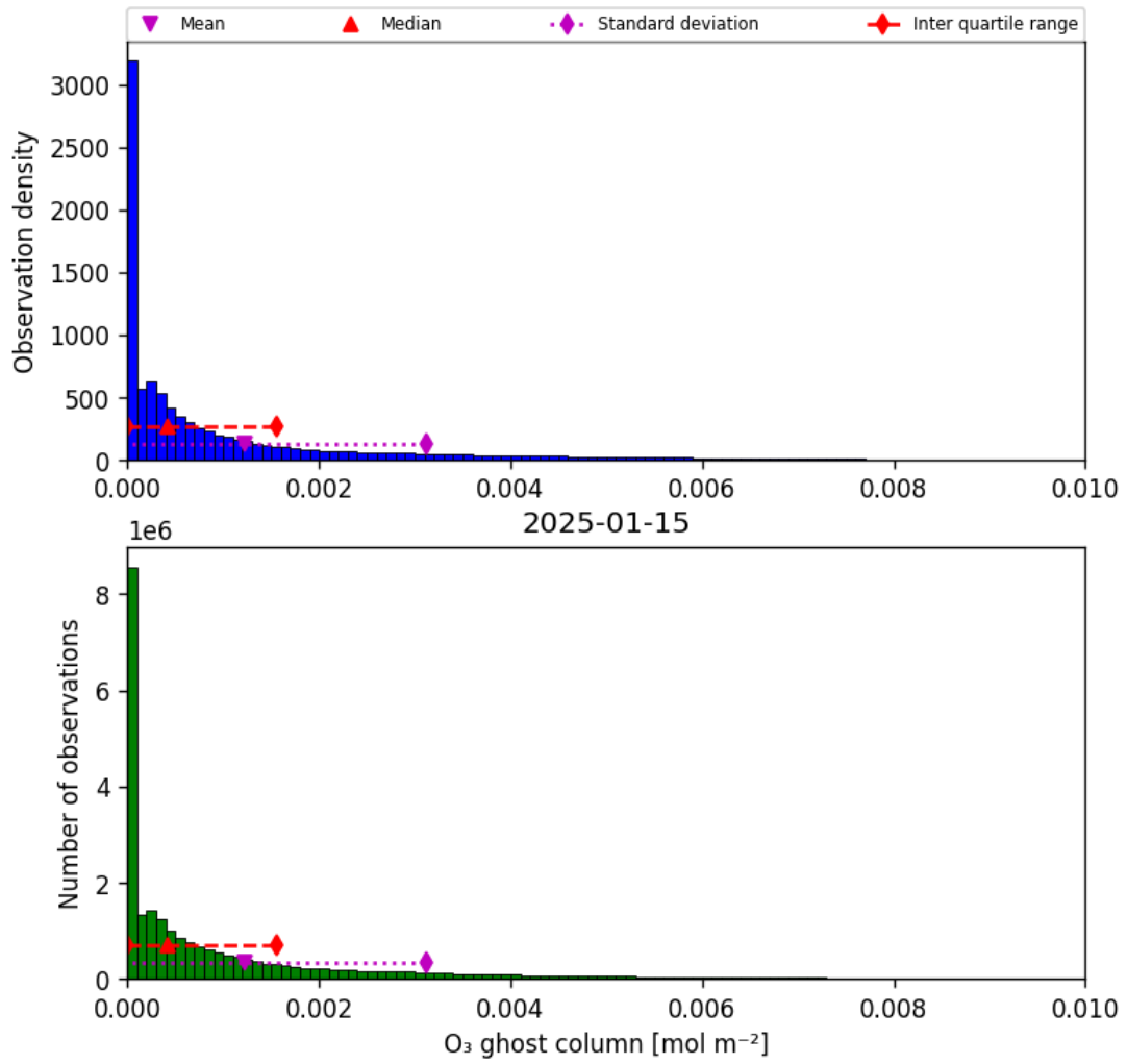
Figure 25: Histogram of “O 3 ghost column” for 2025-01-14 to 2025-01-16
