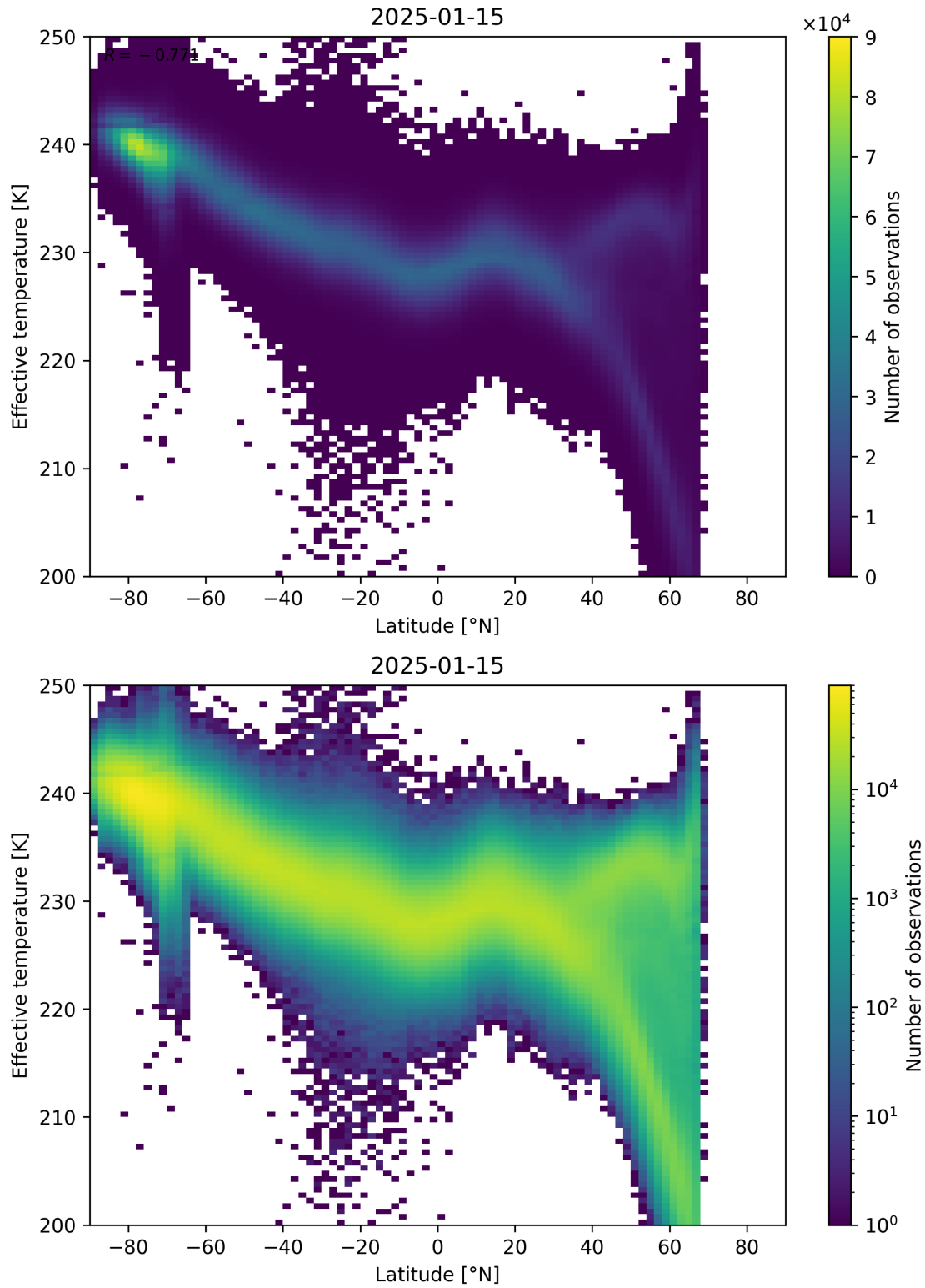
Figure 34: Scatter density plot of “Latitude” against “Effective temperature” for 2025-01-14 to 2025-01-16.
