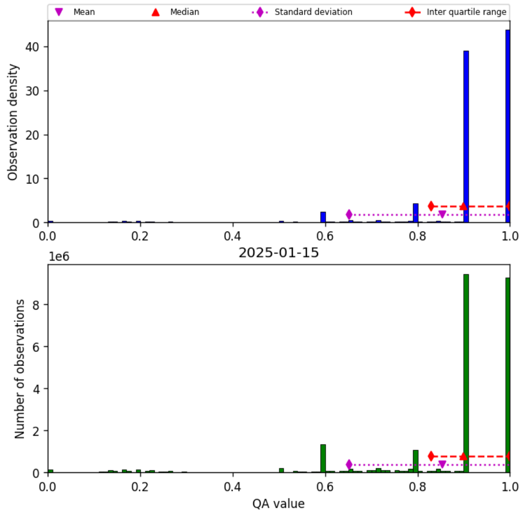
Figure 20: Histogram of “QA value” for 2025-01-14 to 2025-01-16
