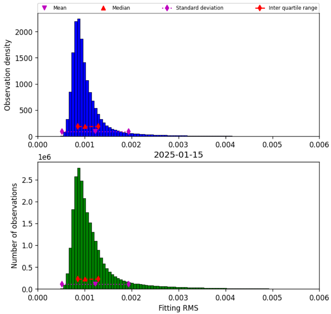
Figure 23: Histogram of “Fitting RMS” for 2025-01-14 to 2025-01-16
