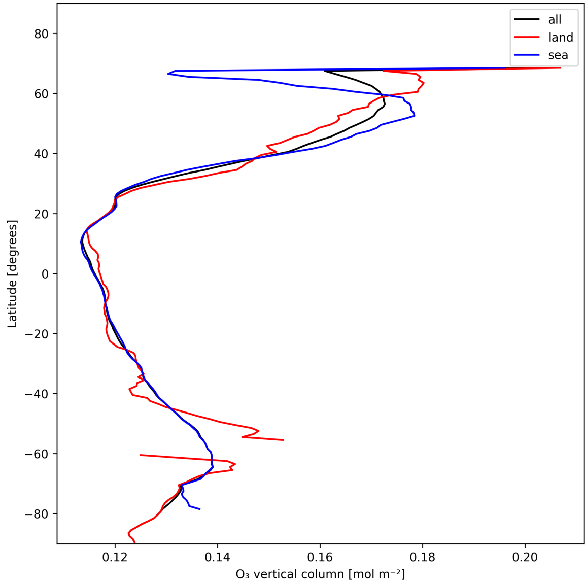
Figure 14: Zonal average of “O 3 vertical column” for 2025-01-14 to 2025-01-16.
