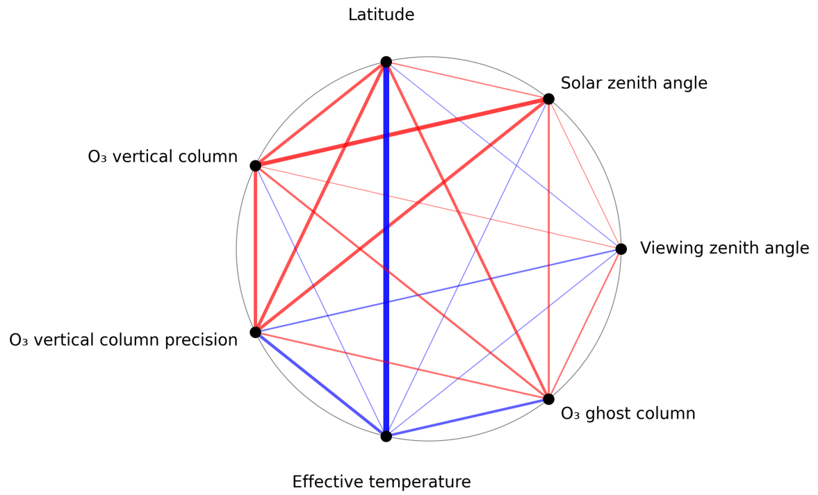
Figure 1: Map of correlation graph for 2025-01-14 to 2025-01-16.
