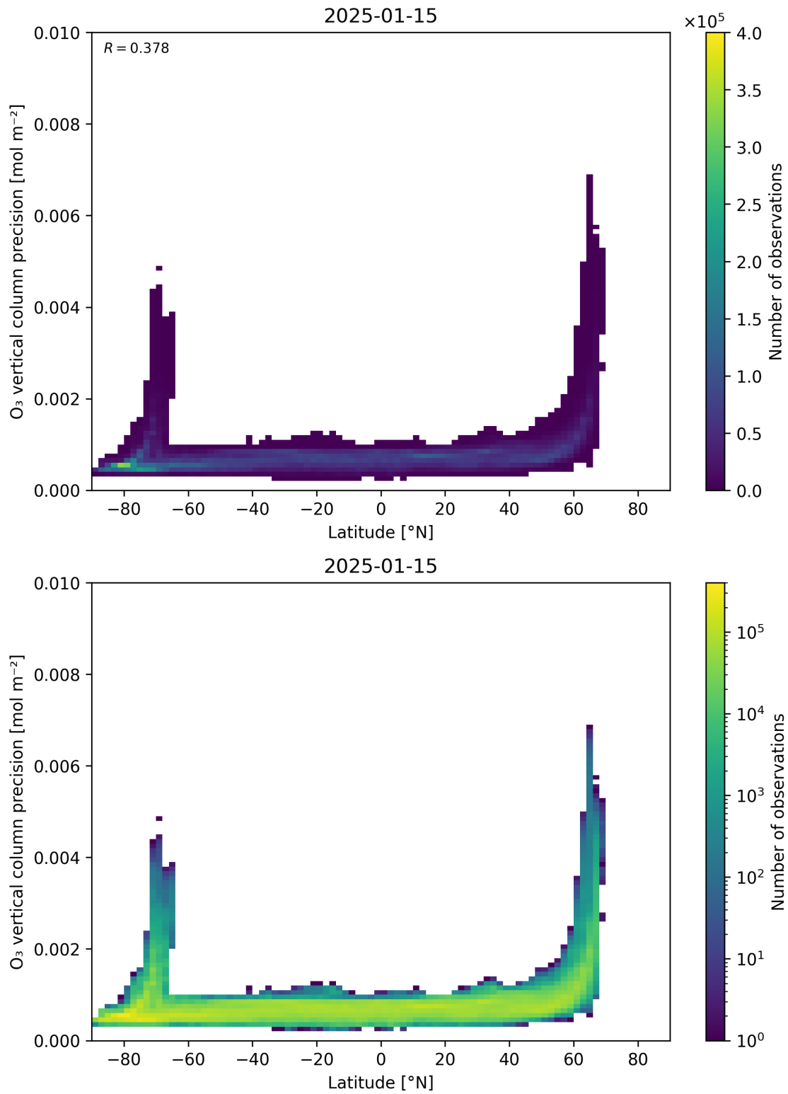
Figure 37: Scatter density plot of “Latitude” against “O 3 vertical column precision” for 2025-01-14 to 2025-01-16.
