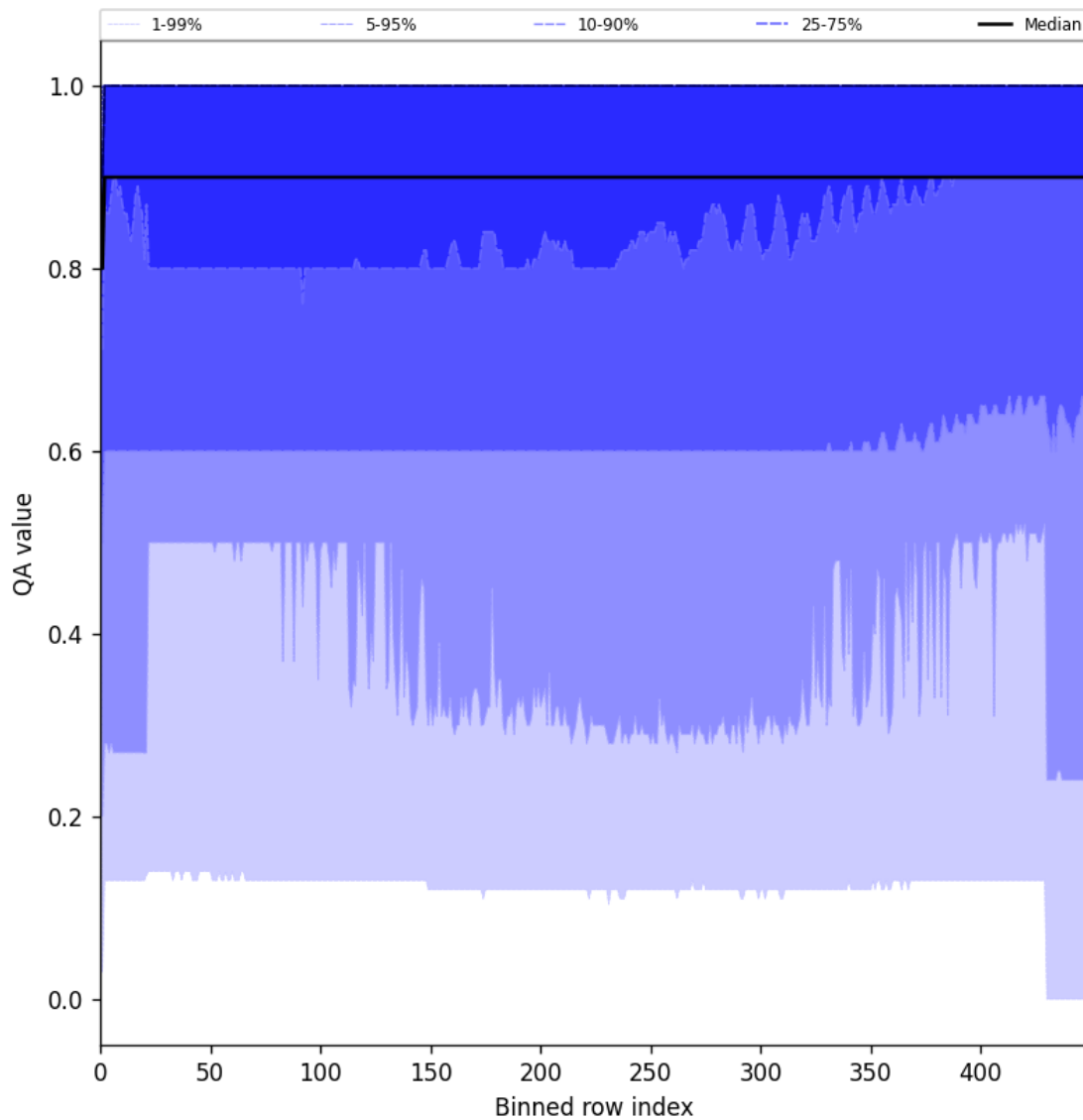
Figure 27: Along track statistics of “QA value” for 2025-01-14 to 2025-01-16
