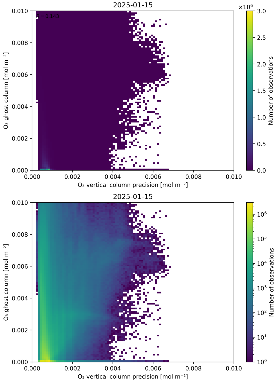
Figure 43: Scatter density plot of “O 3 vertical column precision” against “O 3 ghost column” for 2025-01-14 to 2025-01-16.
