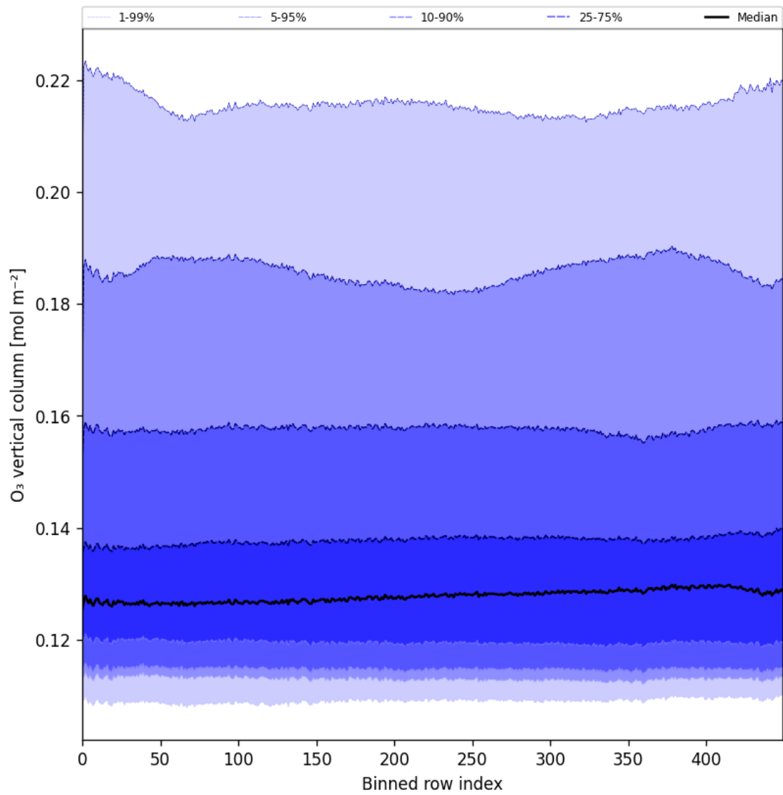
Figure 28: Along track statistics of “O 3 vertical column” for 2025-01-14 to 2025-01-16
