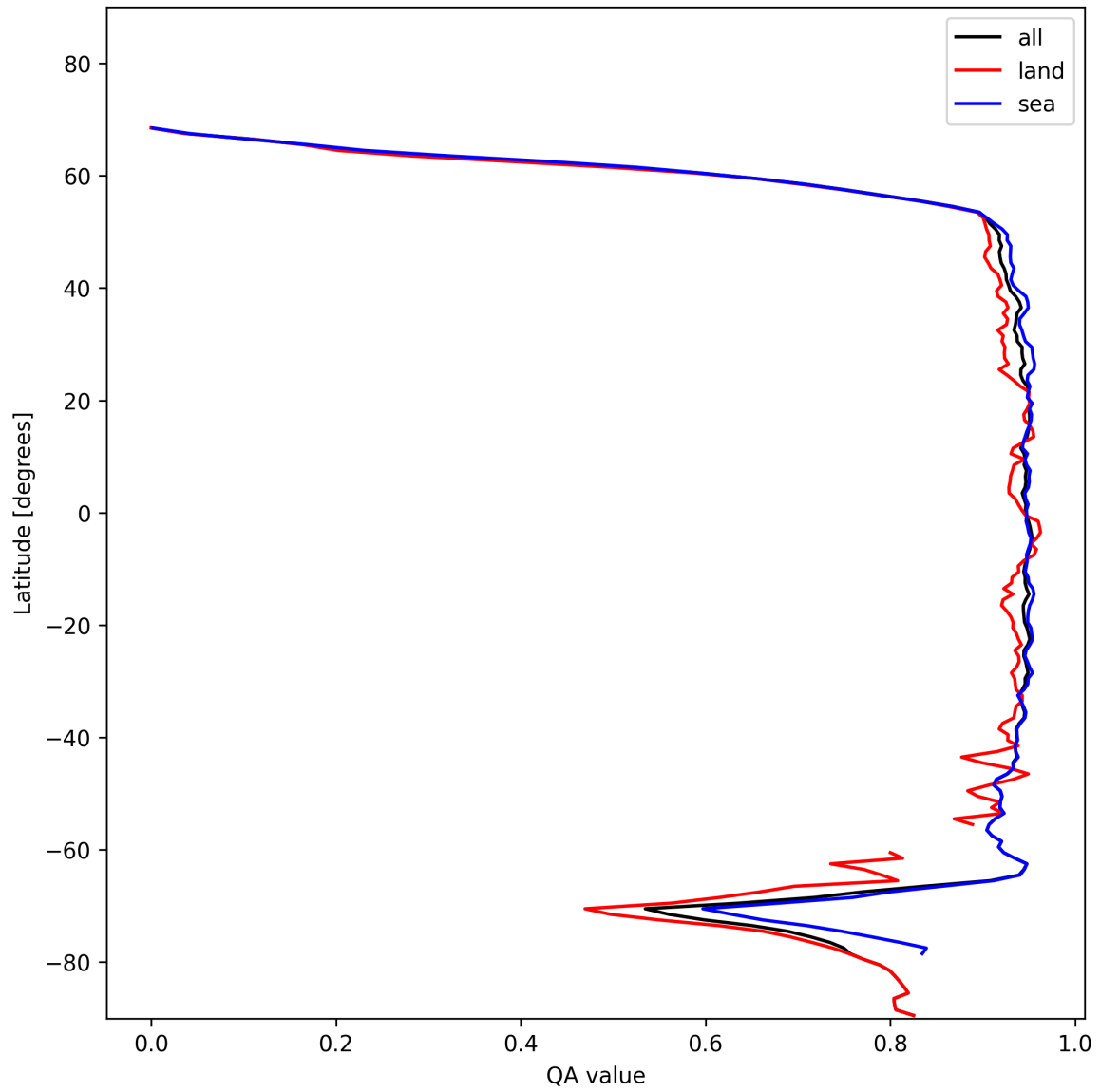
Figure 13: Zonal average of “QA value” for 2025-01-14 to 2025-01-16.
