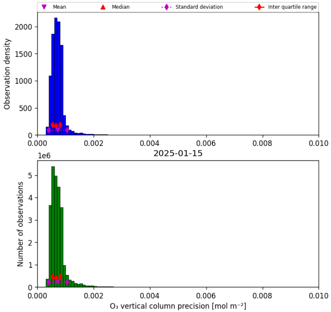
Figure 22: Histogram of “O 3 vertical column precision” for 2025-01-14 to 2025-01-16
