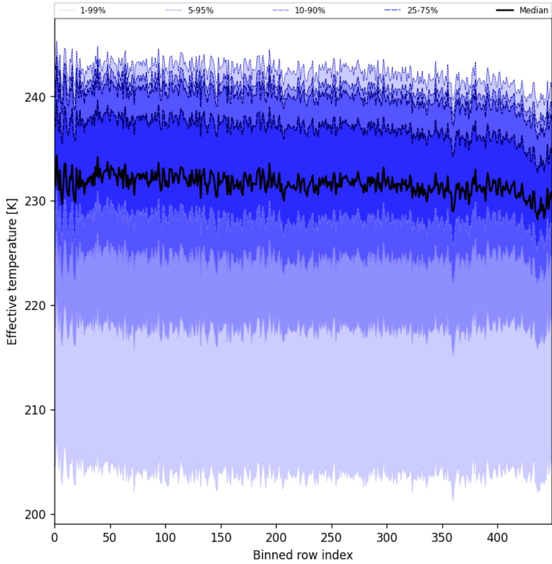
Figure 31: Along track statistics of “Effective temperature” for 2025-01-14 to 2025-01-16
