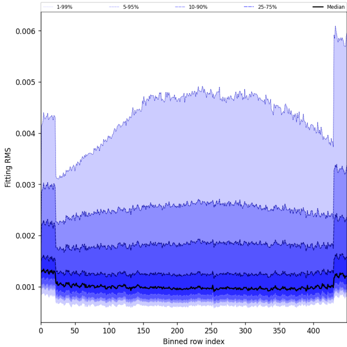
Figure 30: Along track statistics of “Fitting RMS” for 2025-01-14 to 2025-01-16
