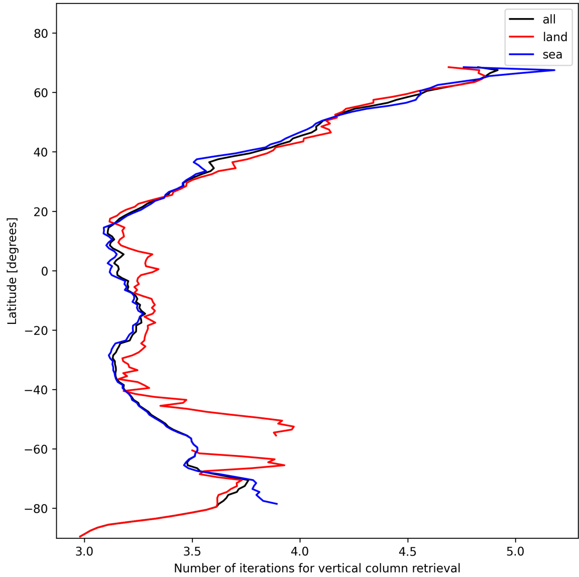
Figure 19: Zonal average of “Number of iterations for vertical column retrieval” for 2025-01-14 to 2025-01-16.
