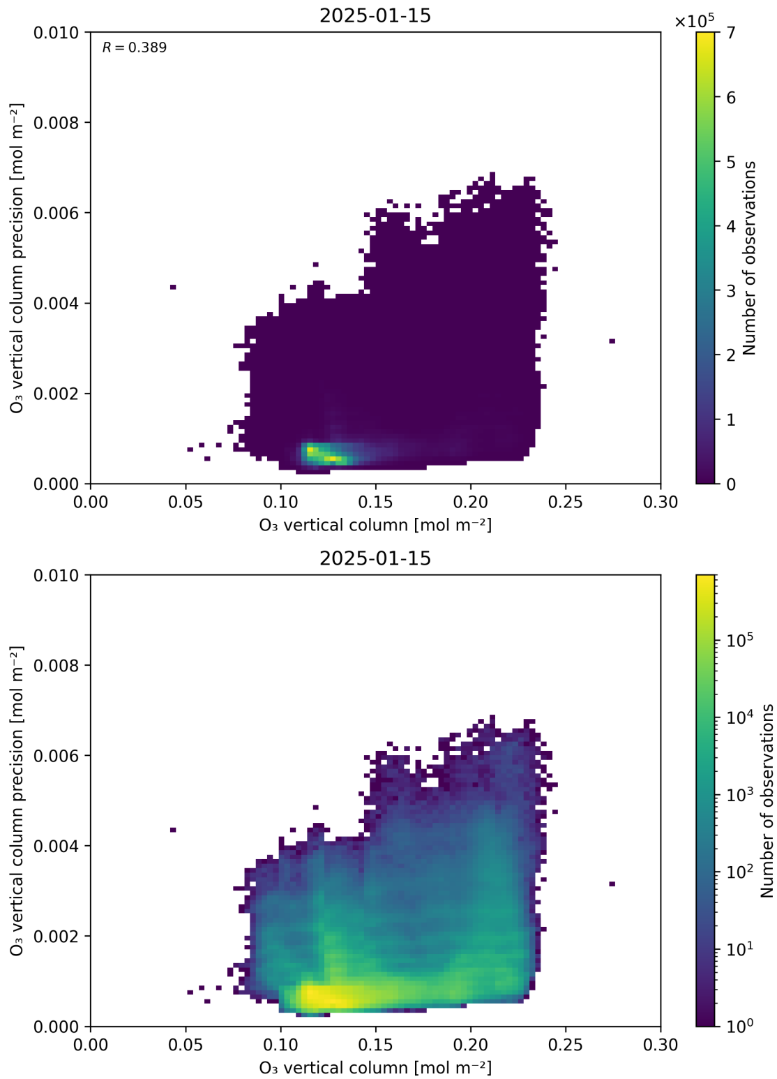
Figure 41: Scatter density plot of “O 3 vertical column” against “O 3 vertical column precision” for 2025-01-14 to 2025-01-16.
