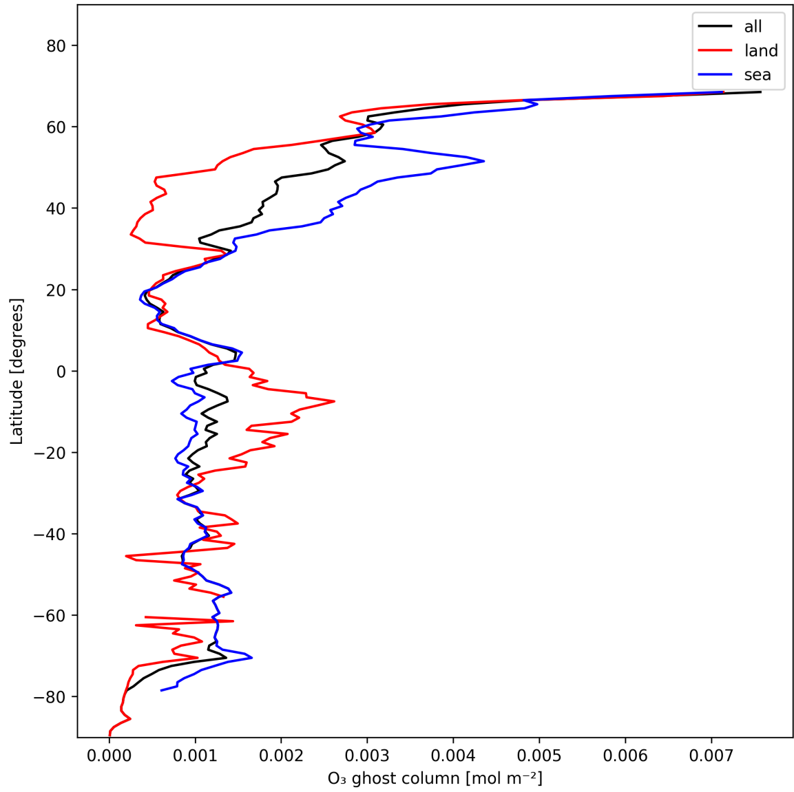
Figure 18: Zonal average of “O 3 ghost column” for 2025-01-14 to 2025-01-16.
