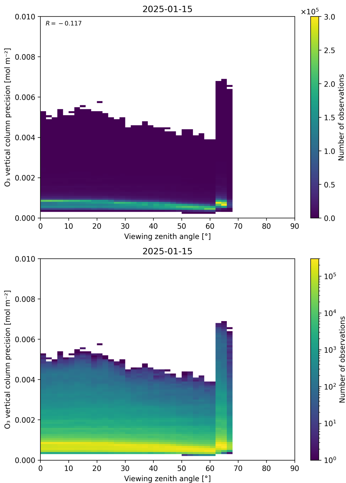
Figure 53: Scatter density plot of “Viewing zenith angle” against “O 3 vertical column precision” for 2025-01-14 to 2025-01-16.
