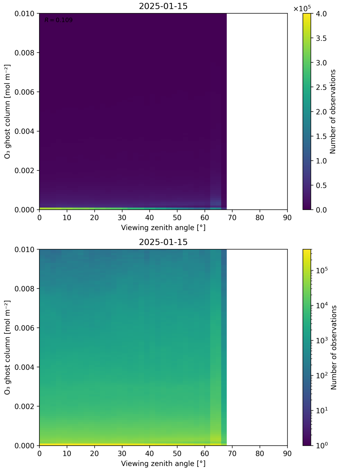
Figure 51: Scatter density plot of “Viewing zenith angle” against “O 3 ghost column” for 2025-01-14 to 2025-01-16.
