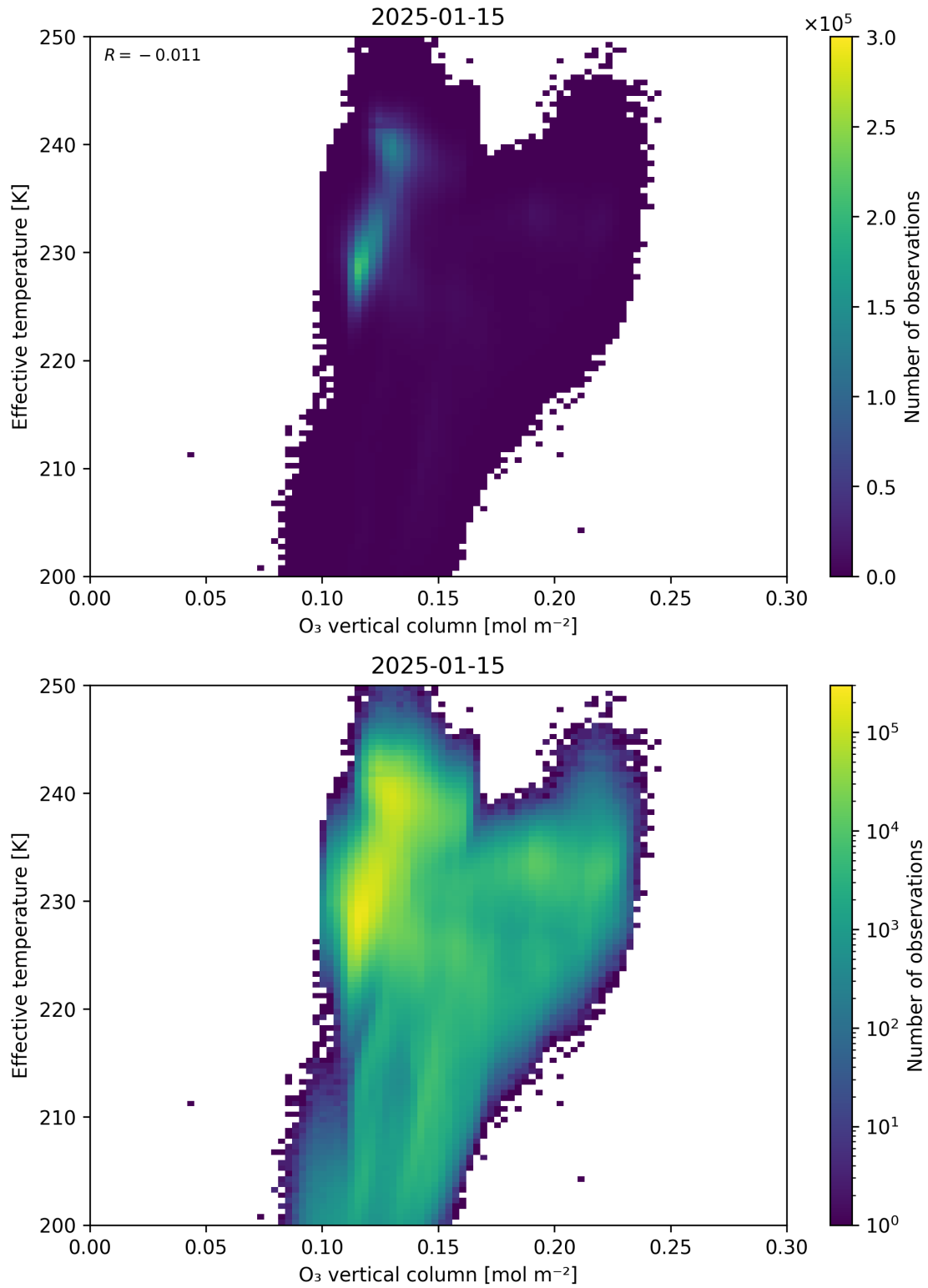
Figure 39: Scatter density plot of “O 3 vertical column” against “Effective temperature” for 2025-01-14 to 2025-01-16.
