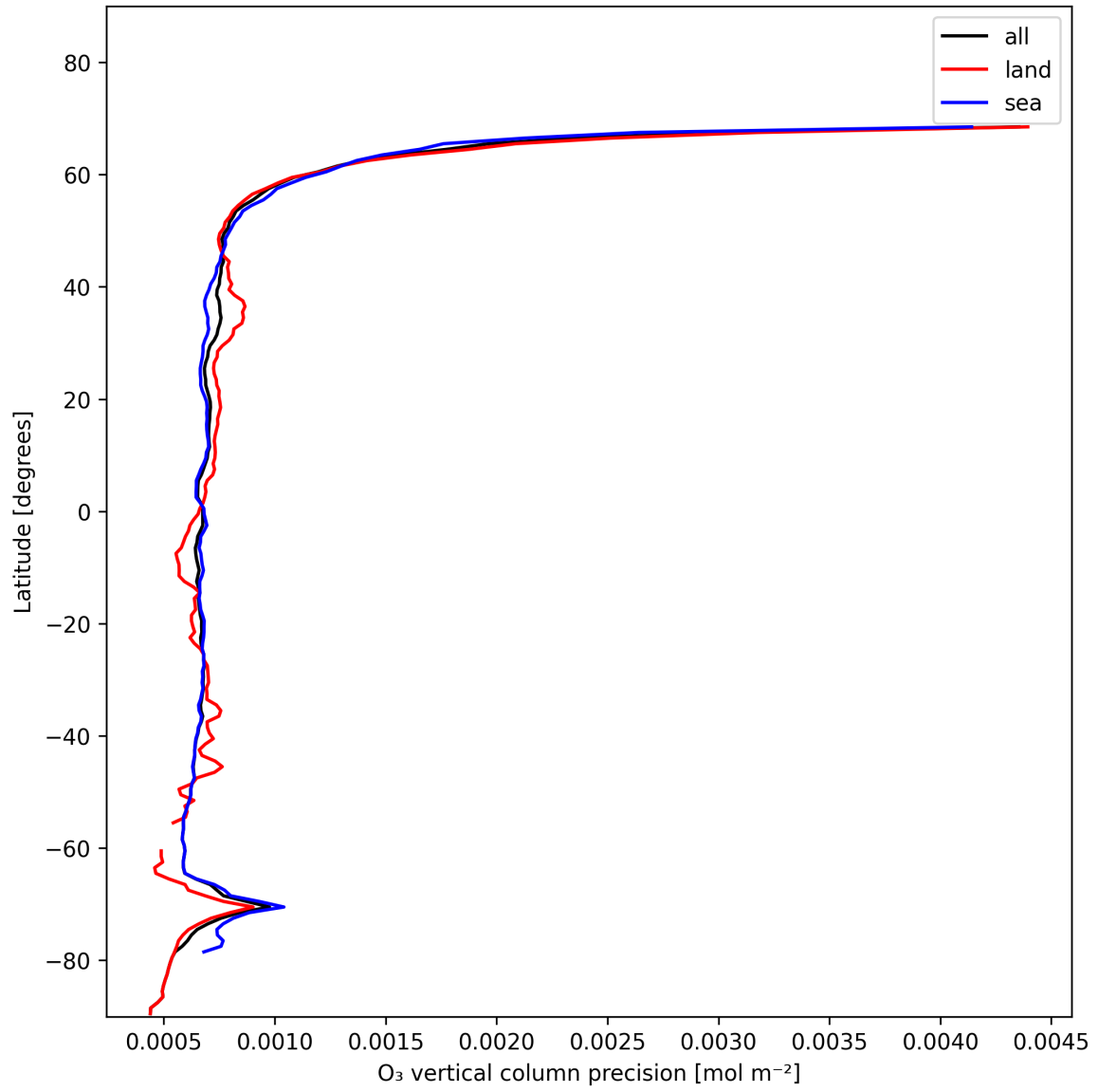
Figure 15: Zonal average of “O 3 vertical column precision” for 2025-01-14 to 2025-01-16.
