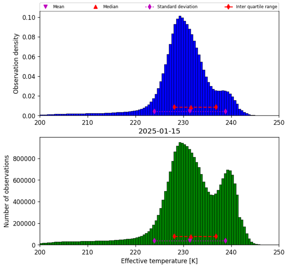
Figure 24: Histogram of “Effective temperature” for 2025-01-14 to 2025-01-16
