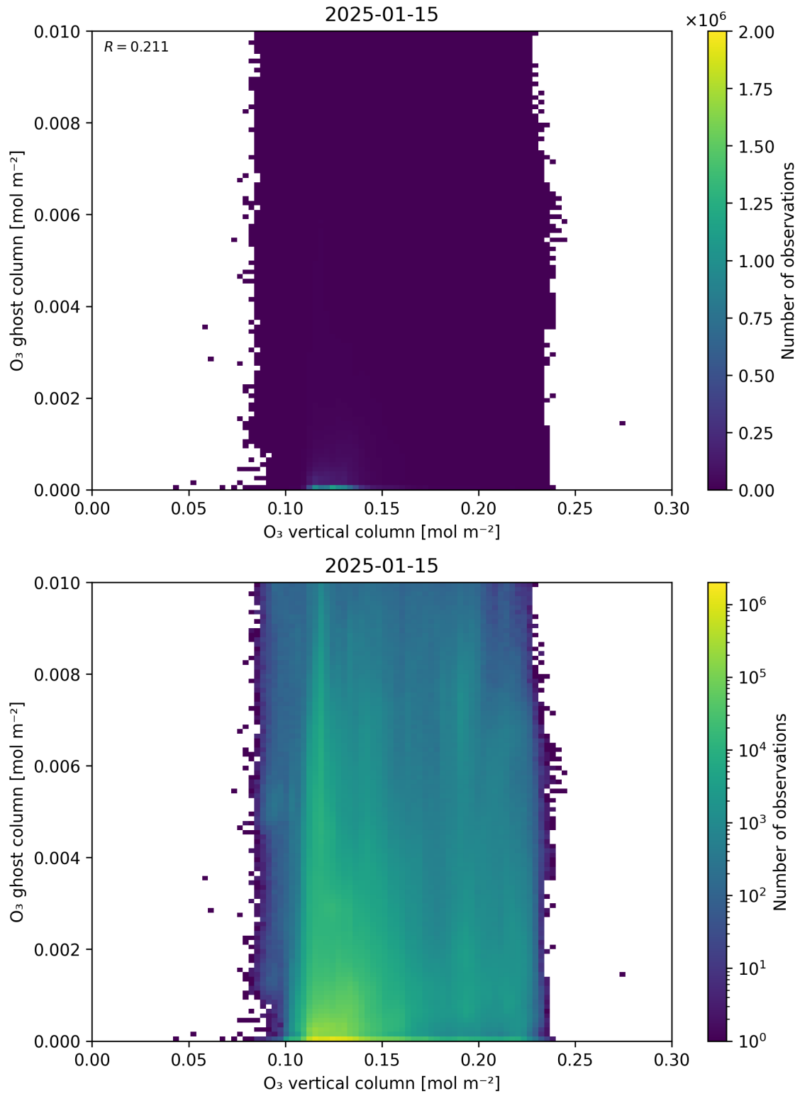
Figure 40: Scatter density plot of “O 3 vertical column” against “O 3 ghost column” for 2025-01-14 to 2025-01-16.
