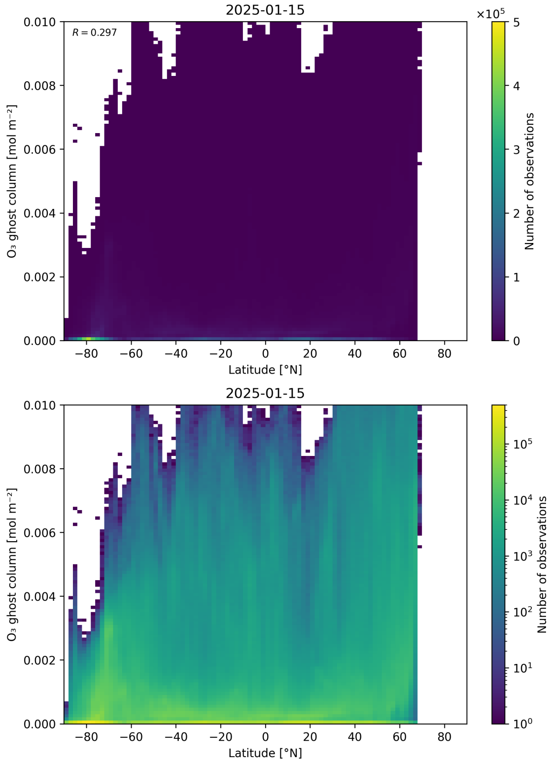
Figure 35: Scatter density plot of “Latitude” against “O 3 ghost column” for 2025-01-14 to 2025-01-16.
