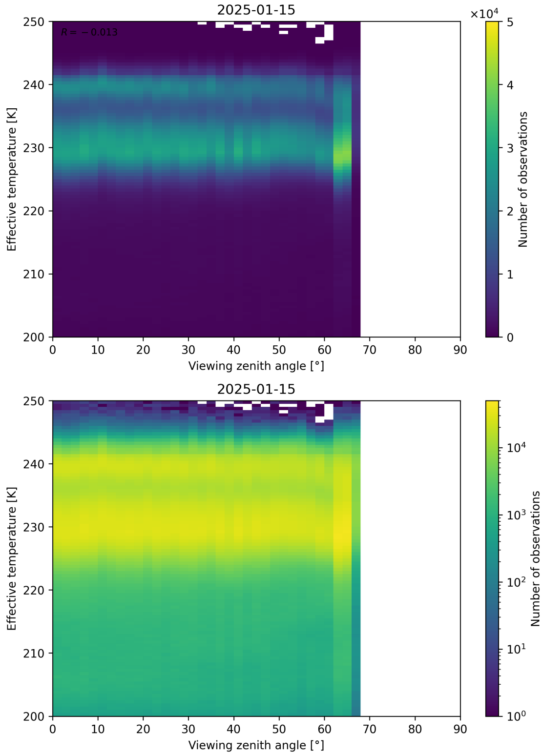
Figure 50: Scatter density plot of “Viewing zenith angle” against “Effective temperature” for 2025-01-14 to 2025-01-16.
