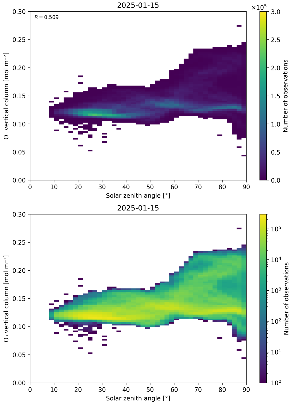
Figure 47: Scatter density plot of “Solar zenith angle” against “O 3 vertical column” for 2025-01-14 to 2025-01-16.
