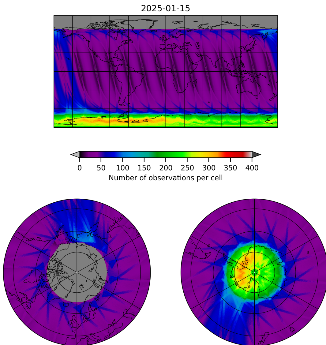
Figure 12: Map of the number of observations for 2025-01-14 to 2025-01-16
