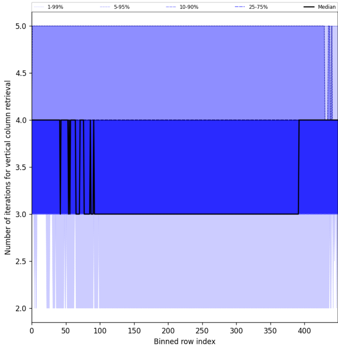
Figure 33: Along track statistics of “Number of iterations for vertical column retrieval” for 2025-01-14 to 2025-01-16
