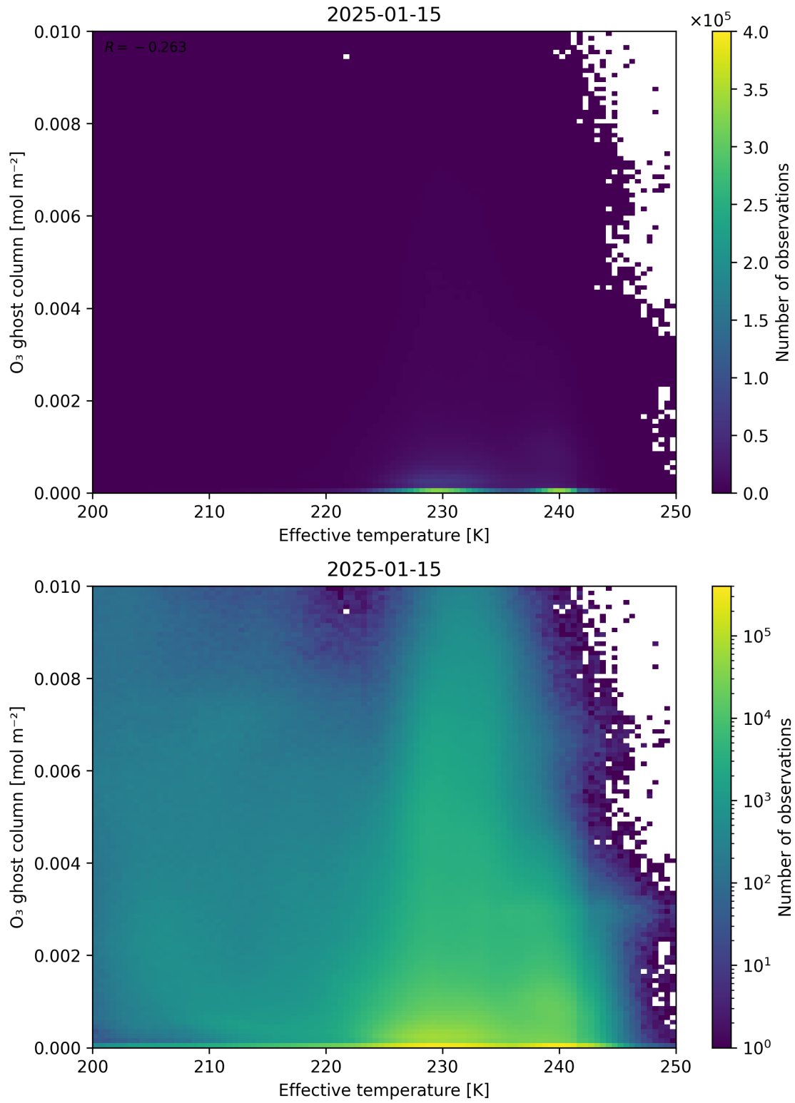
Figure 38: Scatter density plot of “Effective temperature” against “O 3 ghost column” for 2025-01-14 to 2025-01-16.
