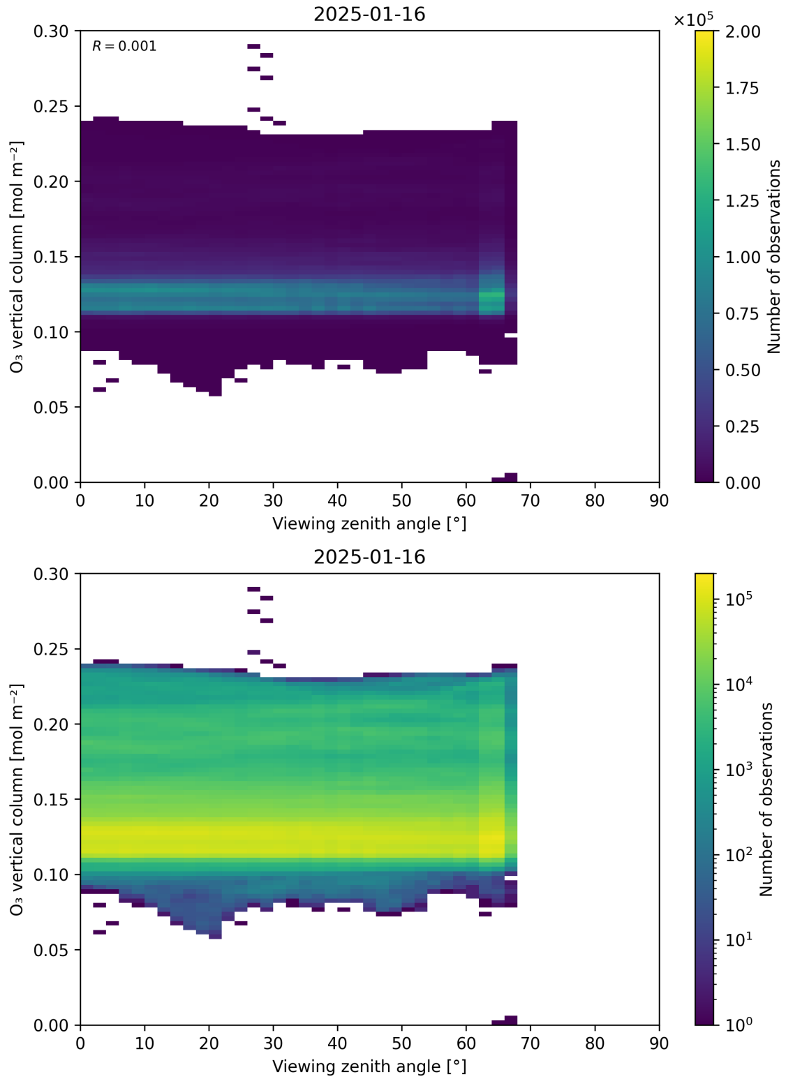
Figure 52: Scatter density plot of “Viewing zenith angle” against “O 3 vertical column” for 2025-01-15 to 2025-01-17.
