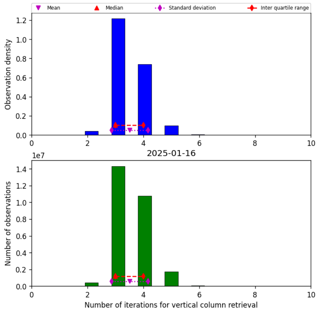
Figure 26: Histogram of “Number of iterations for vertical column retrieval” for 2025-01-15 to 2025-01-17
