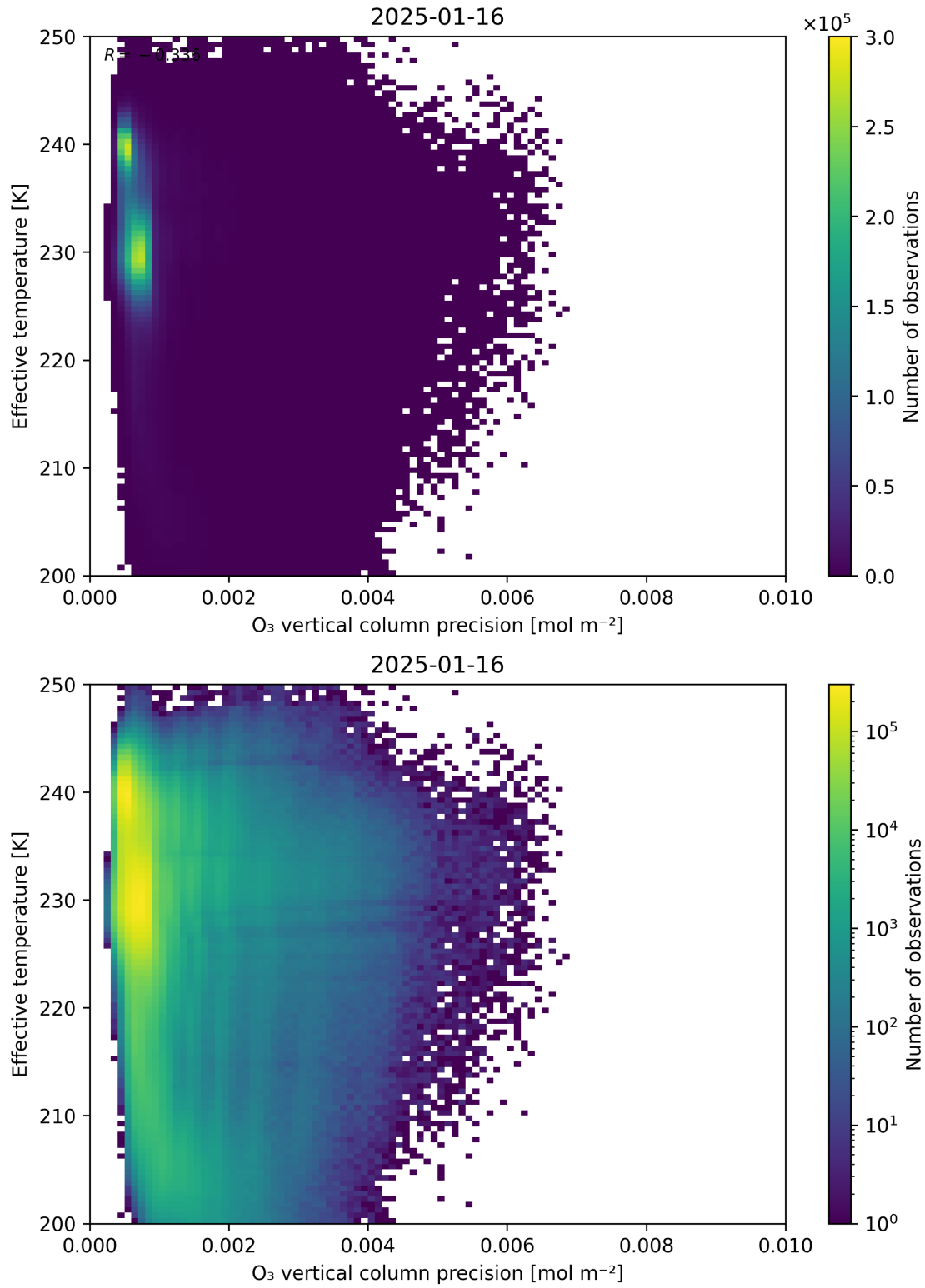
Figure 42: Scatter density plot of “ O_3 vertical column precision” against “Effective temperature” for 2025-01-15 to 2025-01-17.
