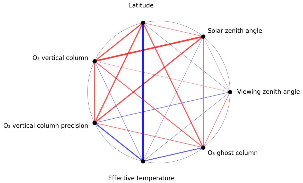
Figure 1: Map of correlation graph for 2025-01-15 to 2025-01-17.
