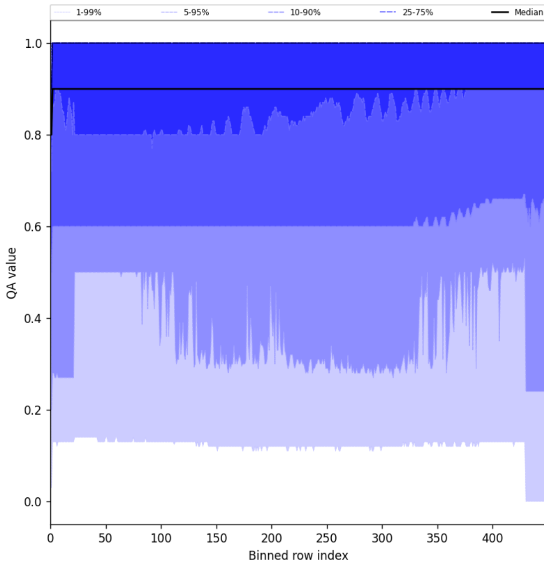
Figure 27: Along track statistics of “QA value” for 2025-01-15 to 2025-01-17
