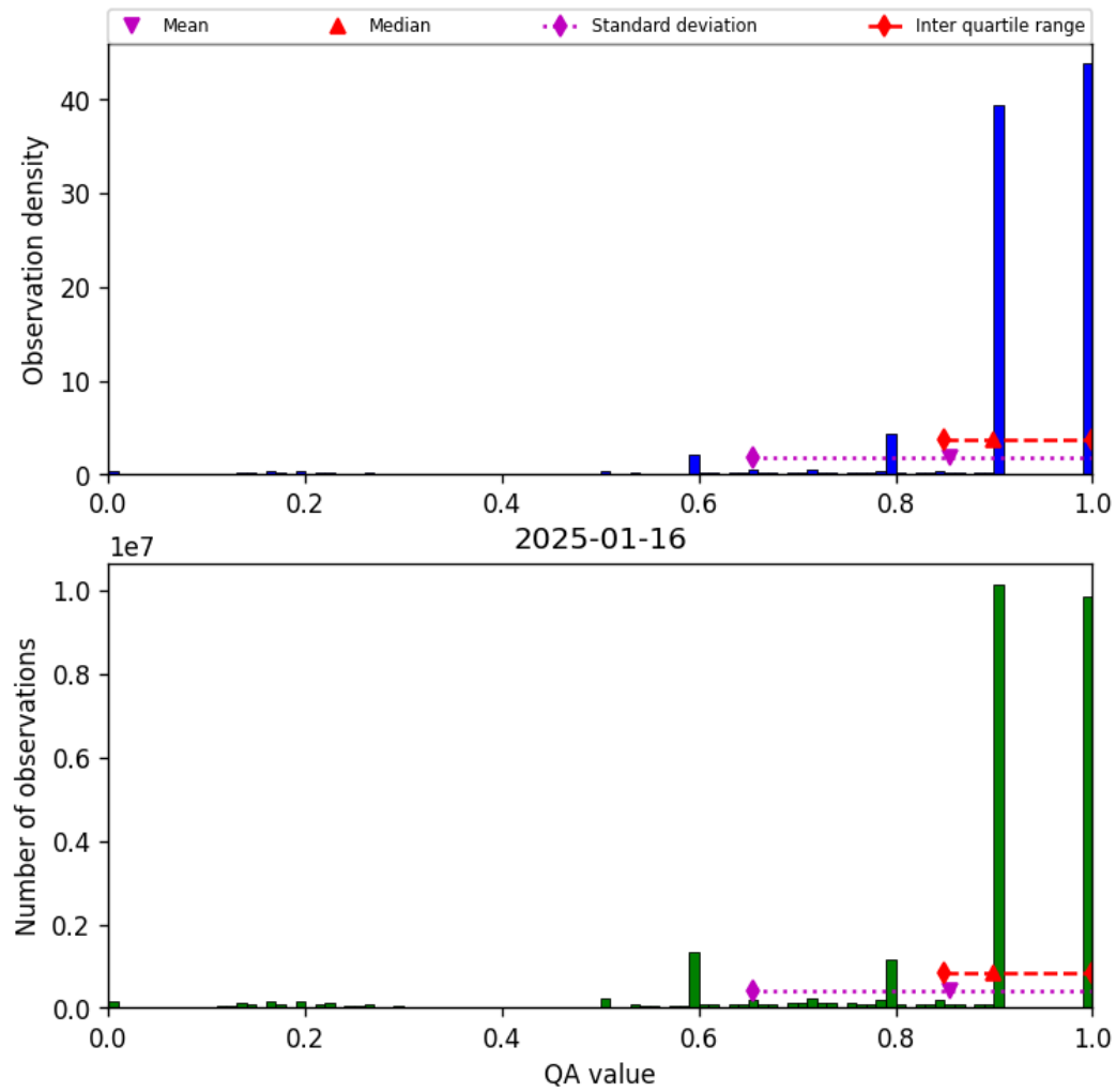
Figure 20: Histogram of “QA value” for 2025-01-15 to 2025-01-17
