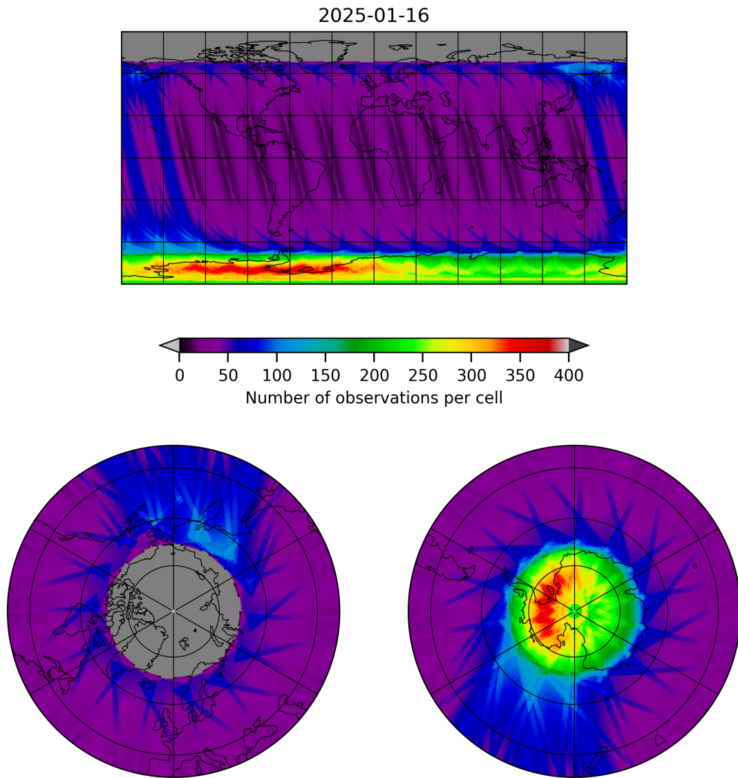
Figure 12: Map of the number of observations for 2025-01-15 to 2025-01-17
