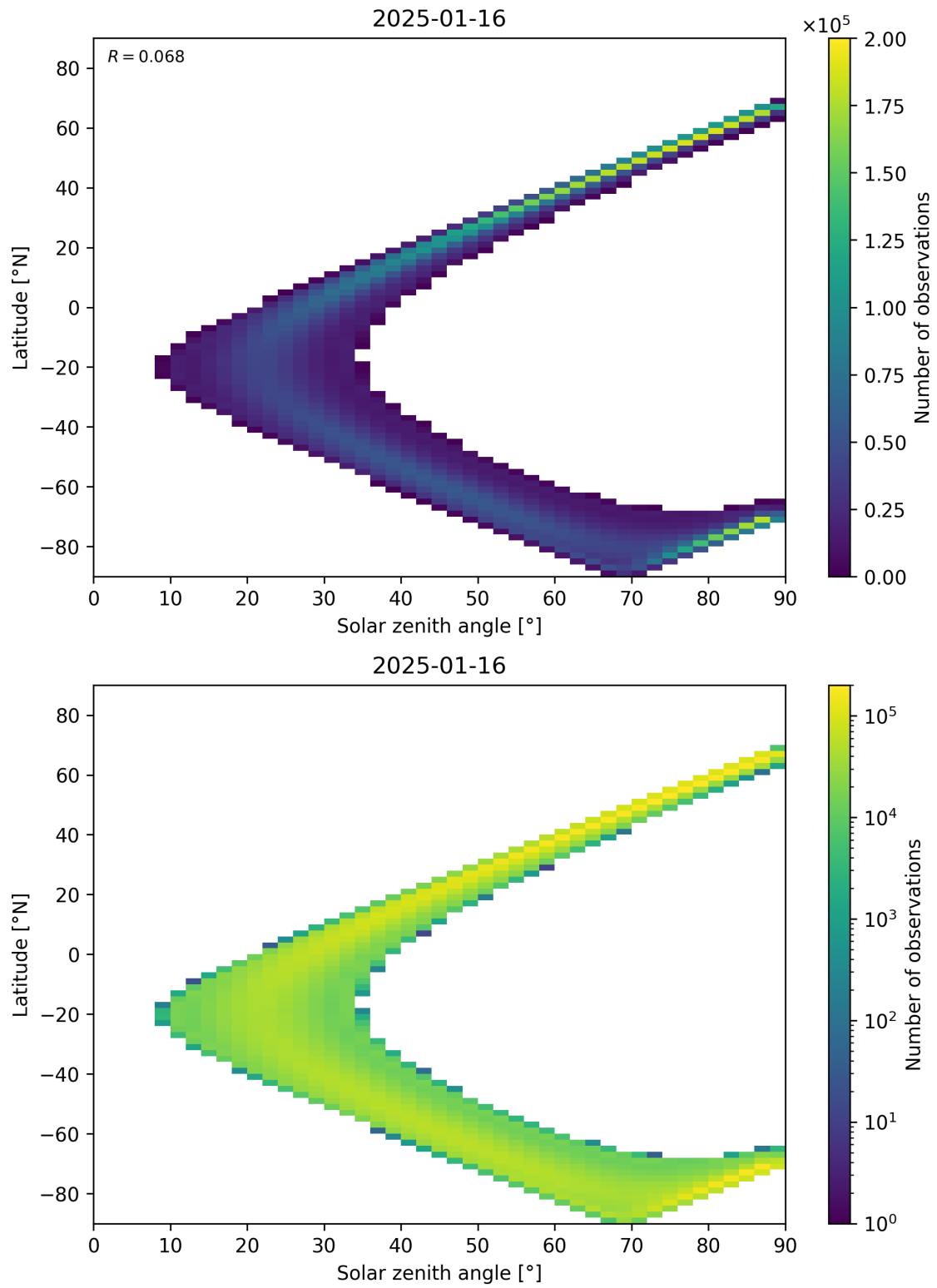
Figure 44: Scatter density plot of “Solar zenith angle” against “Latitude” for 2025-01-15 to 2025-01-17.
