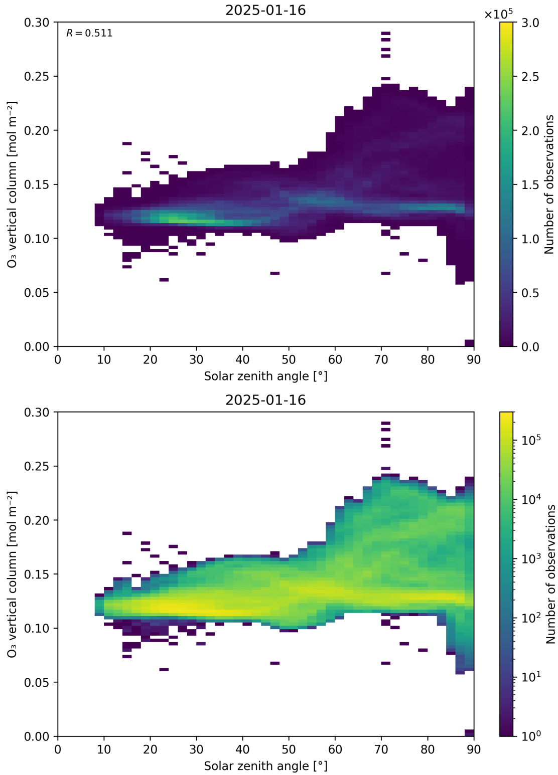
Figure 47: Scatter density plot of “Solar zenith angle” against “O 3 vertical column” for 2025-01-15 to 2025-01-17.
