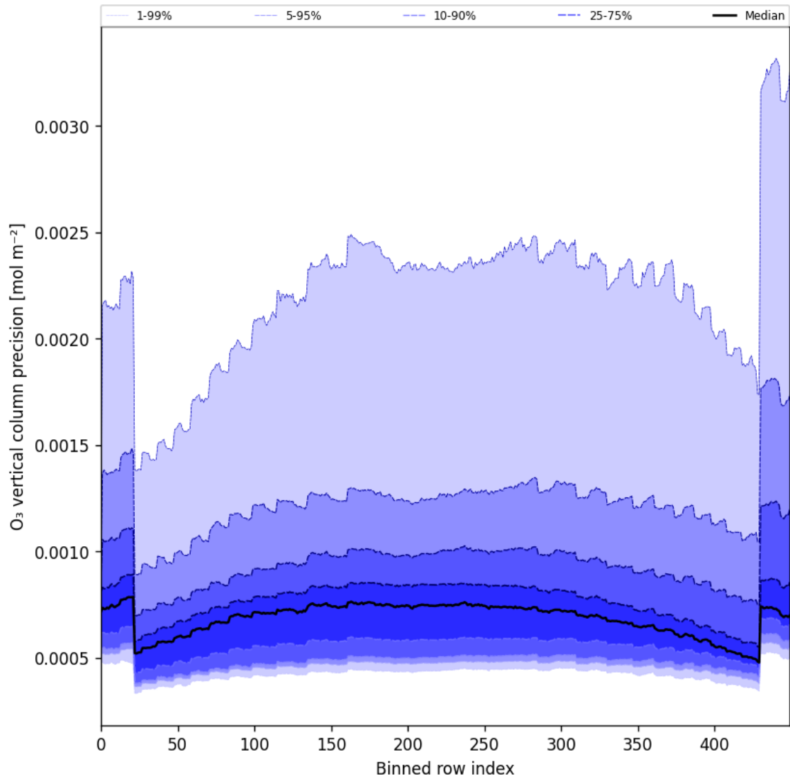
Figure 29: Along track statistics of “O 3 vertical column precision” for 2025-01-15 to 2025-01-17
