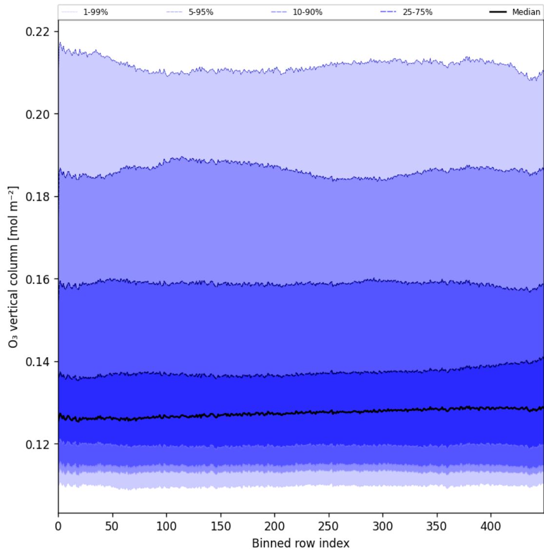
Figure 28: Along track statistics of “O 3 vertical column” for 2025-01-15 to 2025-01-17
