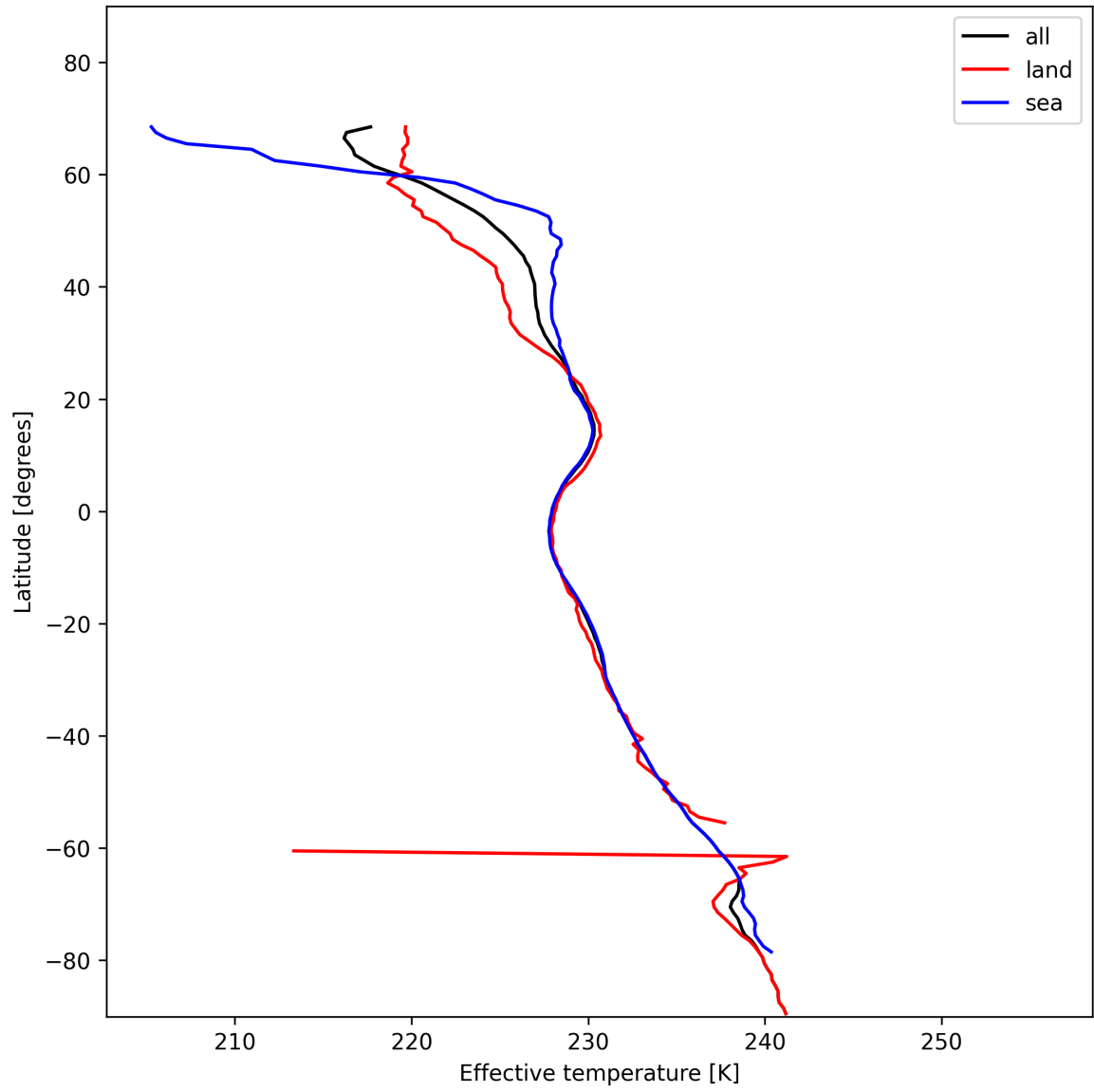
Figure 17: Zonal average of “Effective temperature” for 2025-01-15 to 2025-01-17.
