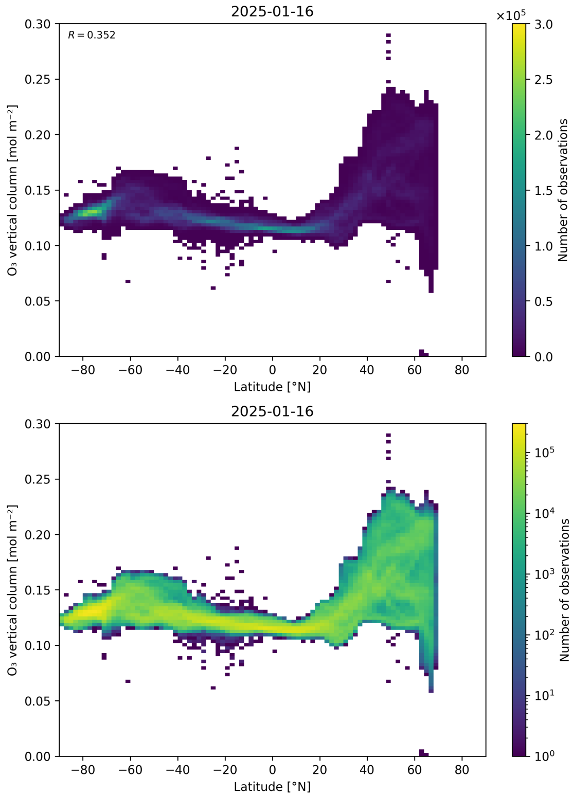
Figure 36: Scatter density plot of “Latitude” against “O 3 vertical column” for 2025-01-15 to 2025-01-17.
