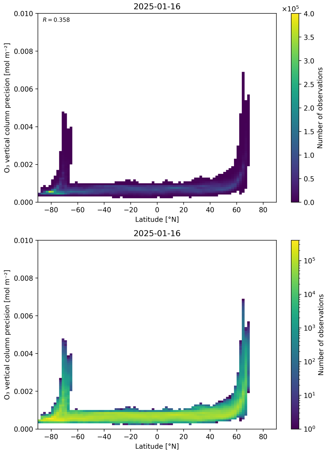
Figure 37: Scatter density plot of “Latitude” against “O 3 vertical column precision” for 2025-01-15 to 2025-01-17.
