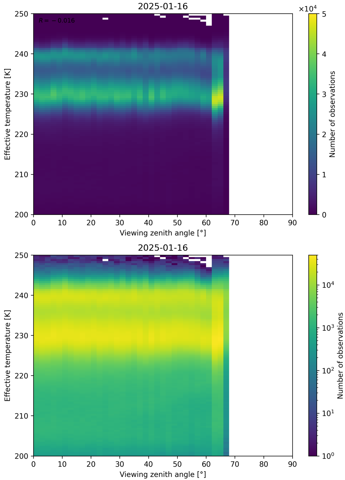
Figure 50: Scatter density plot of “Viewing zenith angle” against “Effective temperature” for 2025-01-15 to 2025-01-17.
