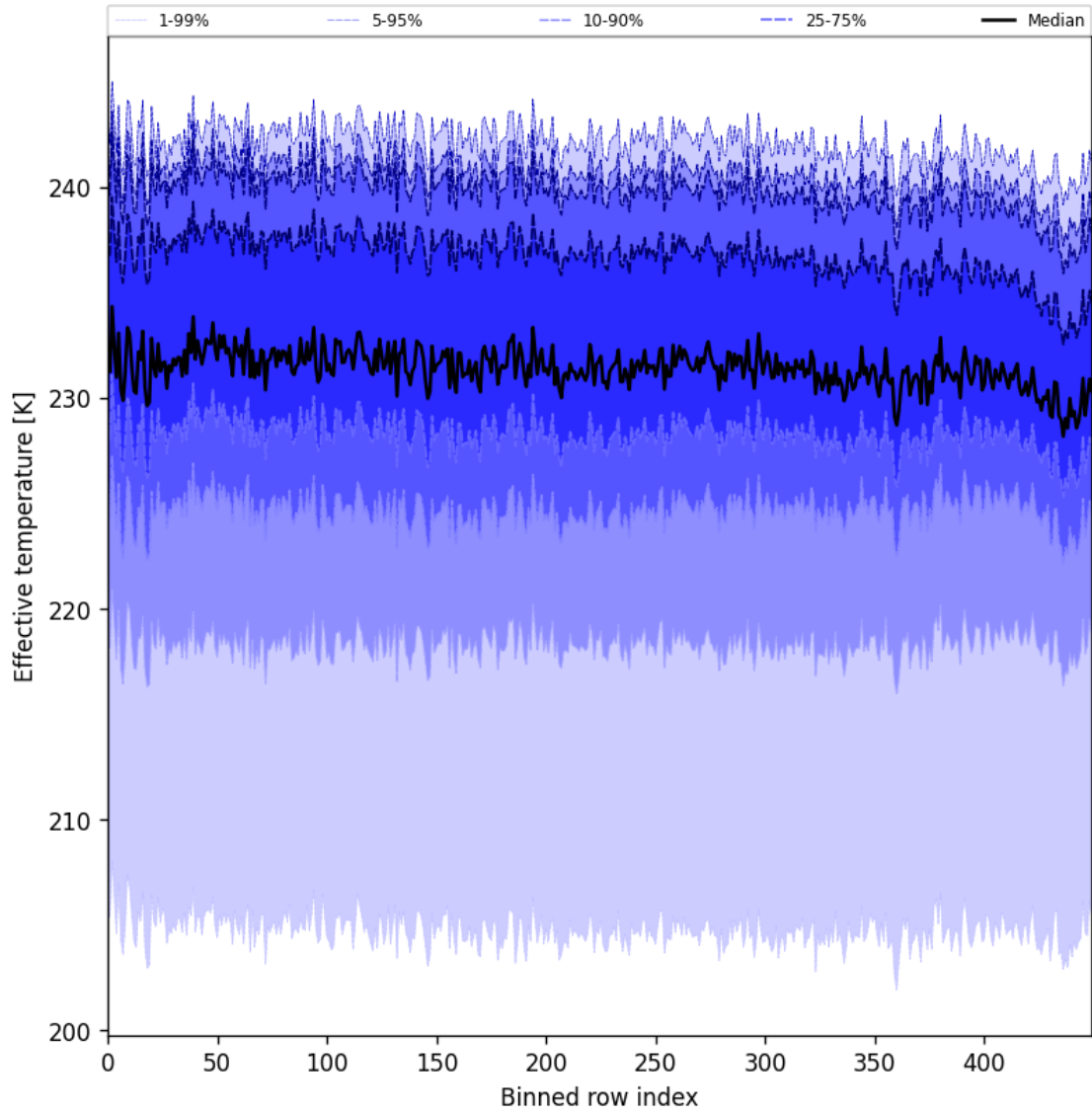
Figure 31: Along track statistics of “Effective temperature” for 2025-01-15 to 2025-01-17
