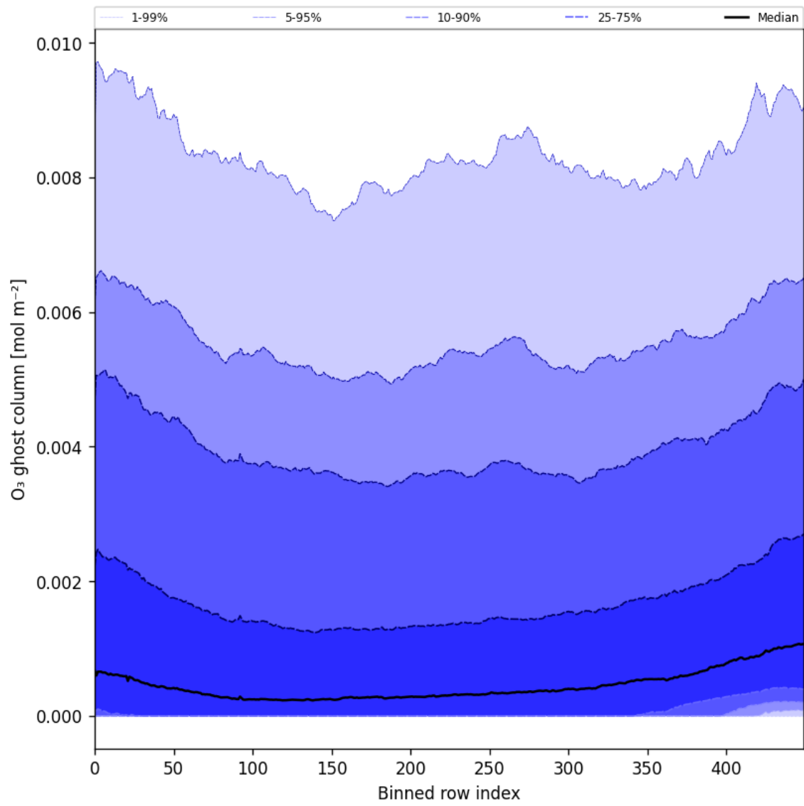
Figure 32: Along track statistics of “O 3 ghost column” for 2025-01-15 to 2025-01-17
