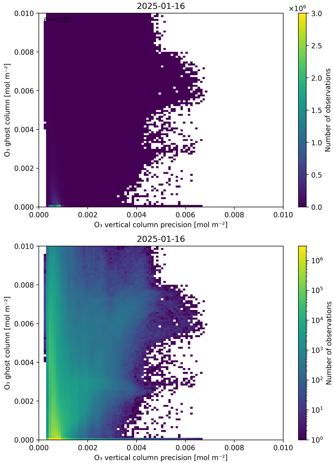
Figure 43: Scatter density plot of “ \text{O}_3 vertical column precision” against “ \text{O}_3 ghost column” for 2025-01-15 to 2025-01-17.
