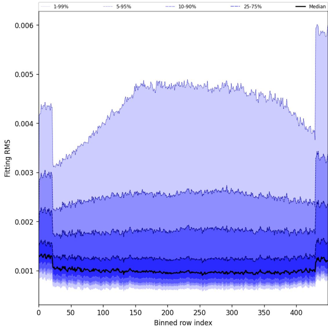
Figure 30: Along track statistics of “Fitting RMS” for 2025-01-15 to 2025-01-17
