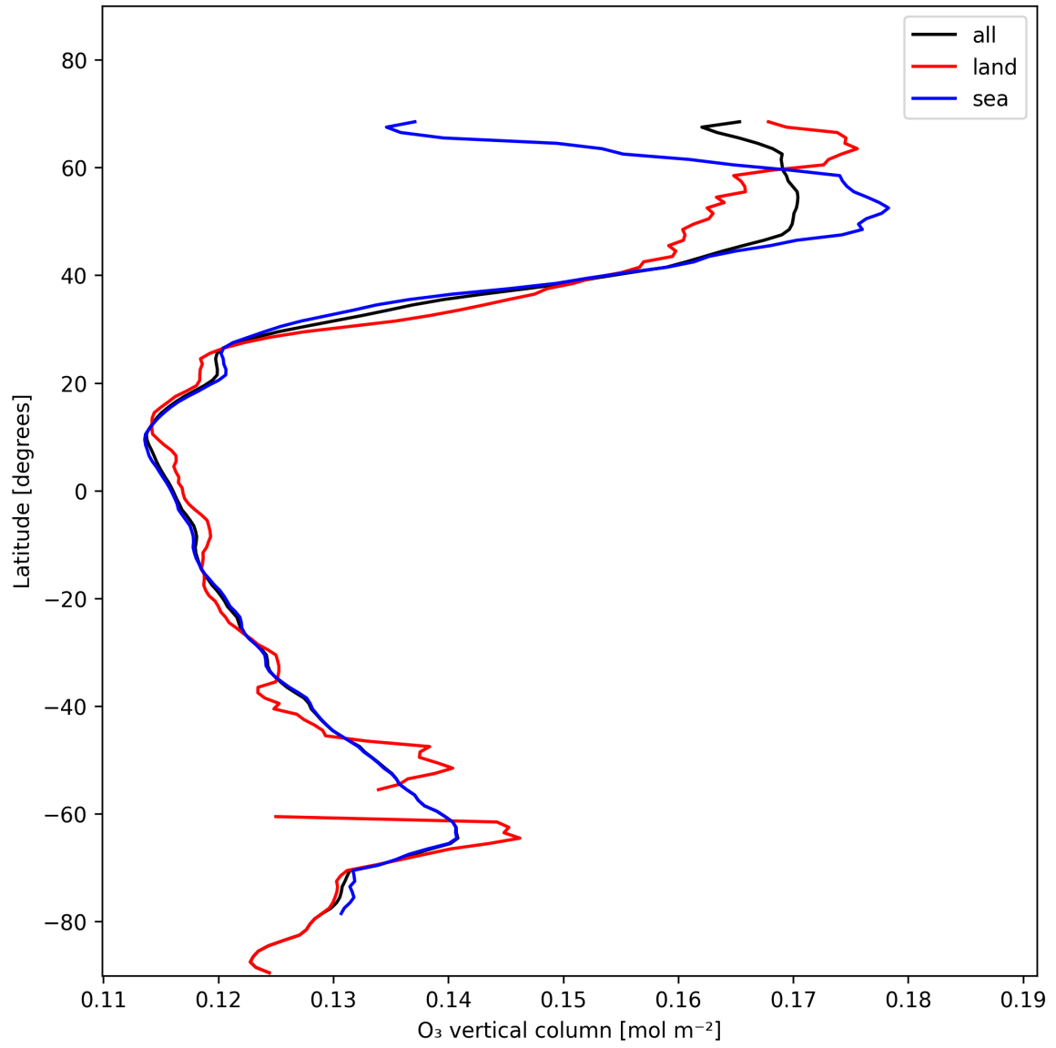
Figure 14: Zonal average of “O 3 vertical column” for 2025-01-15 to 2025-01-17.
