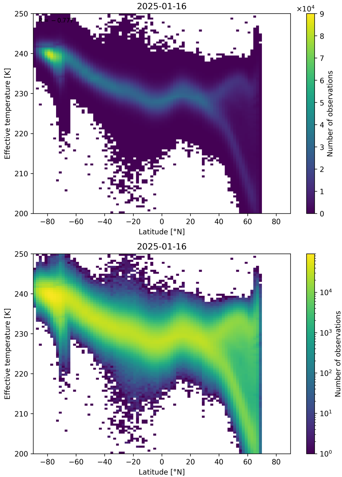
Figure 34: Scatter density plot of “Latitude” against “Effective temperature” for 2025-01-15 to 2025-01-17.
