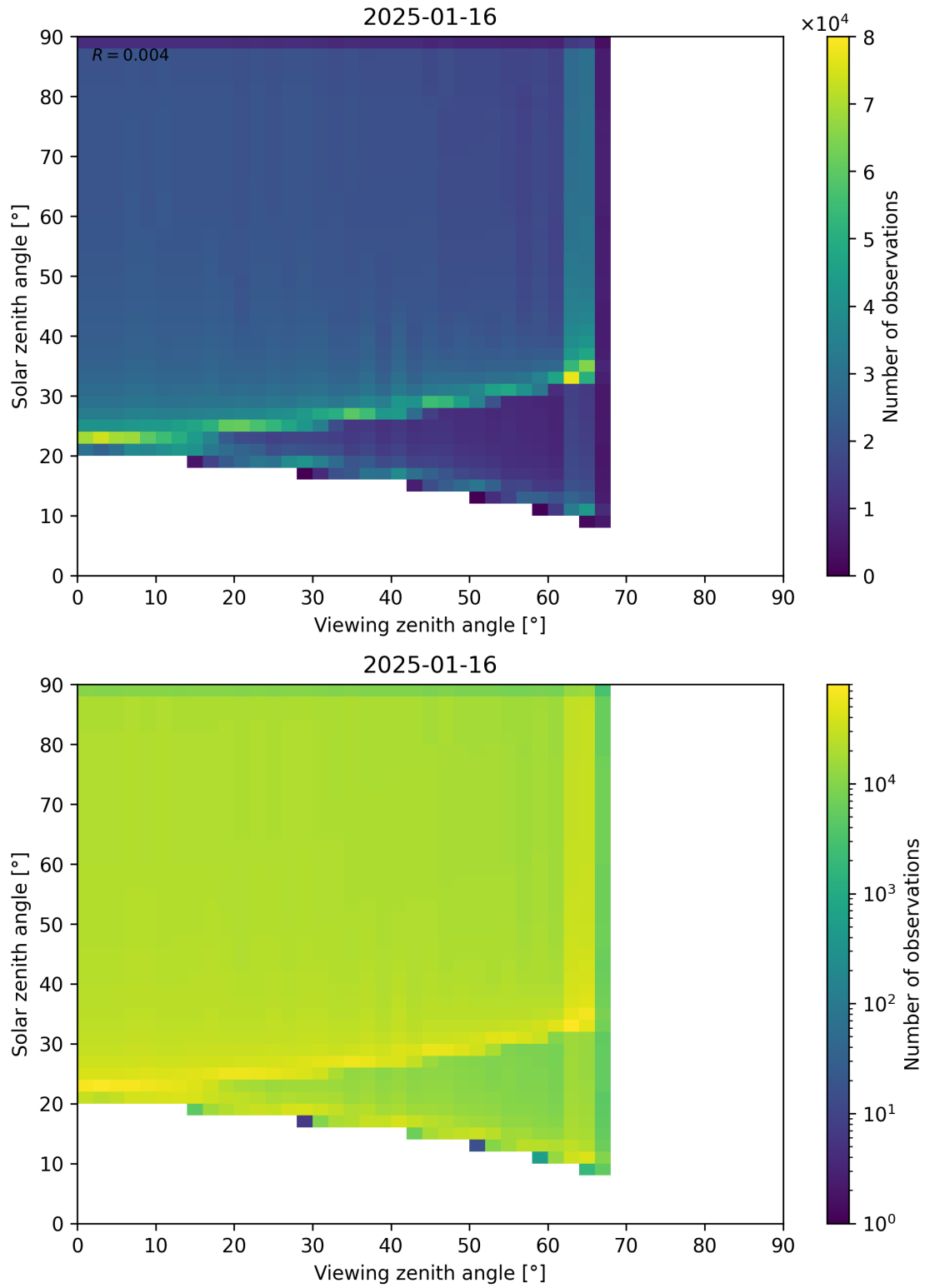
Figure 54: Scatter density plot of “Viewing zenith angle” against “Solar zenith angle” for 2025-01-15 to 2025-01-17.
