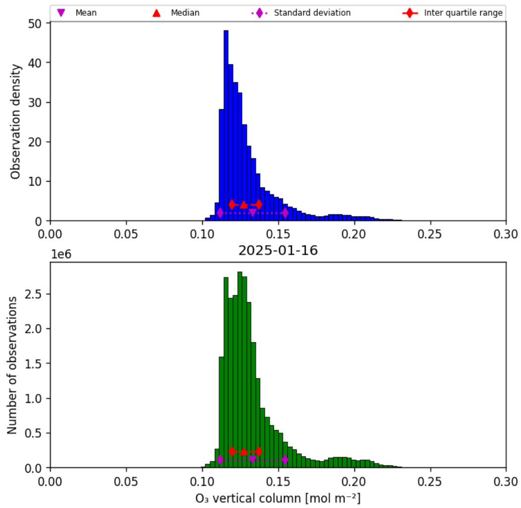
Figure 21: Histogram of “O 3 vertical column” for 2025-01-15 to 2025-01-17
