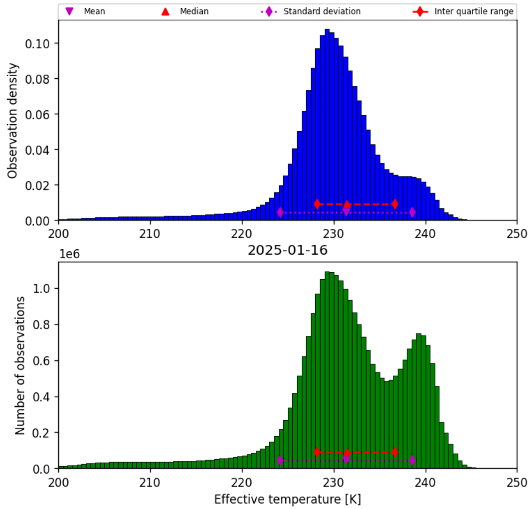
Figure 24: Histogram of “Effective temperature” for 2025-01-15 to 2025-01-17
