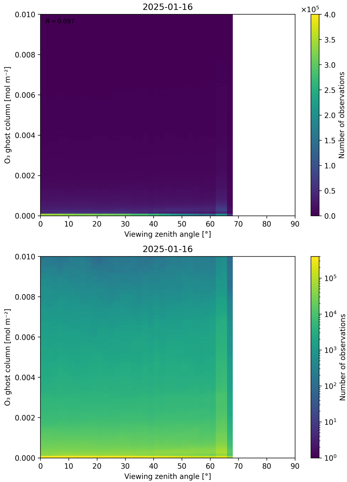
Figure 51: Scatter density plot of “Viewing zenith angle” against “O 3 ghost column” for 2025-01-15 to 2025-01-17.
