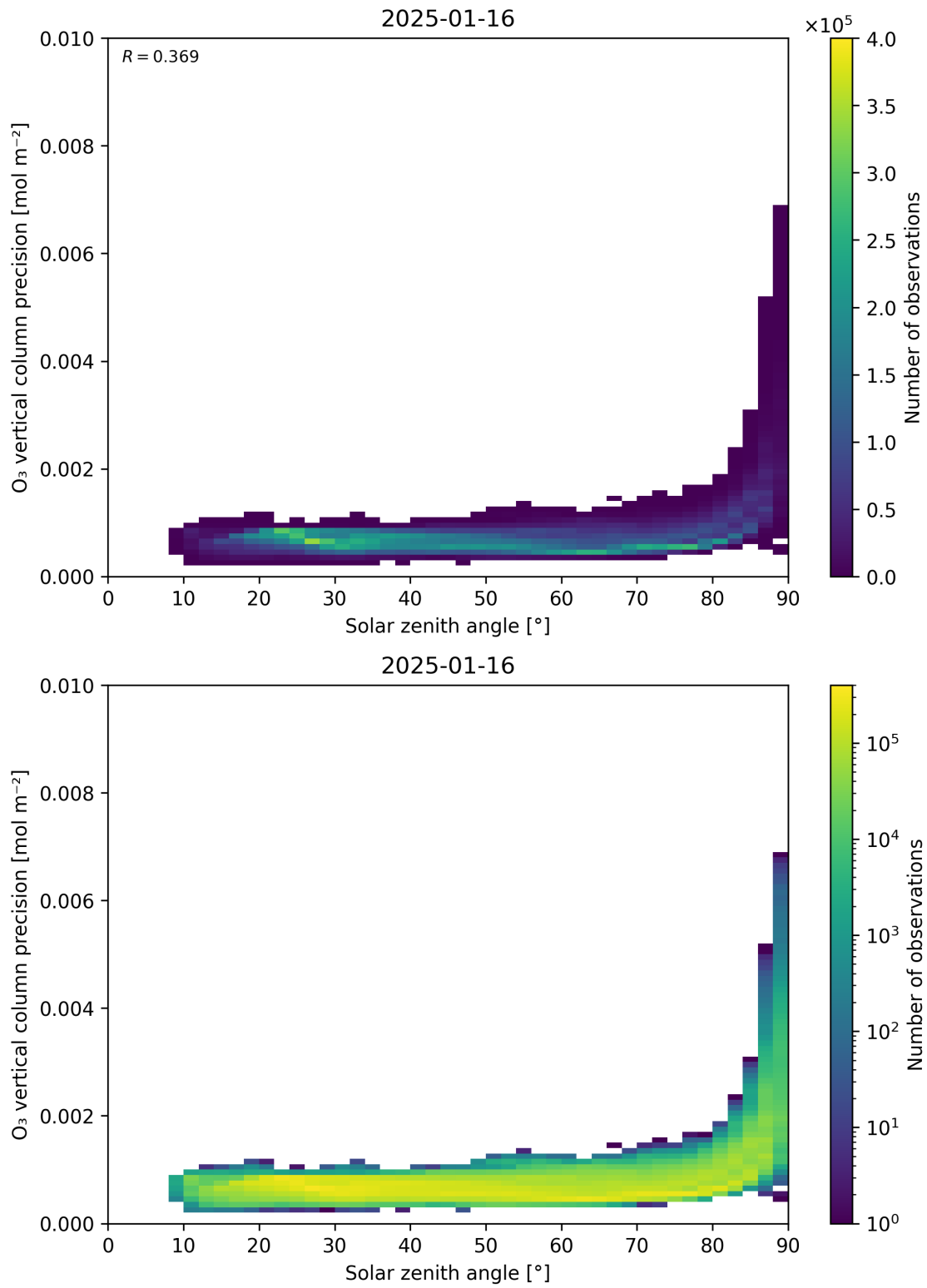
Figure 48: Scatter density plot of “Solar zenith angle” against “O 3 vertical column precision” for 2025-01-15 to 2025-01-17.
