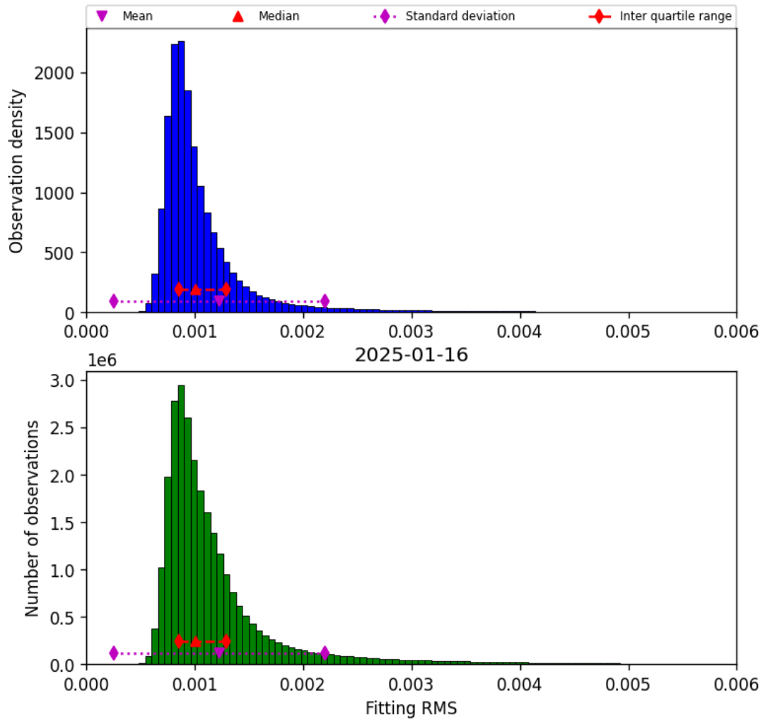
Figure 23: Histogram of “Fitting RMS” for 2025-01-15 to 2025-01-17
