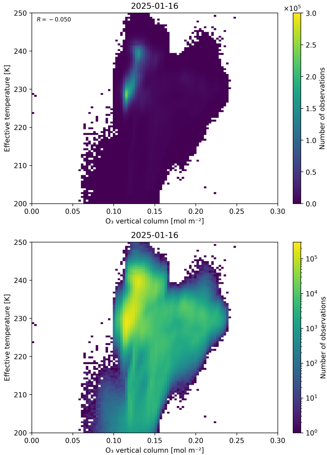
Figure 39: Scatter density plot of “O 3 vertical column” against “Effective temperature” for 2025-01-15 to 2025-01-17.
