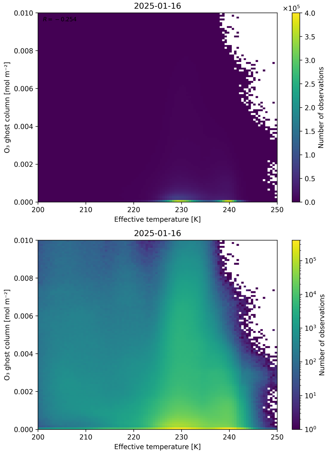
Figure 38: Scatter density plot of “Effective temperature” against “O 3 ghost column” for 2025-01-15 to 2025-01-17.
