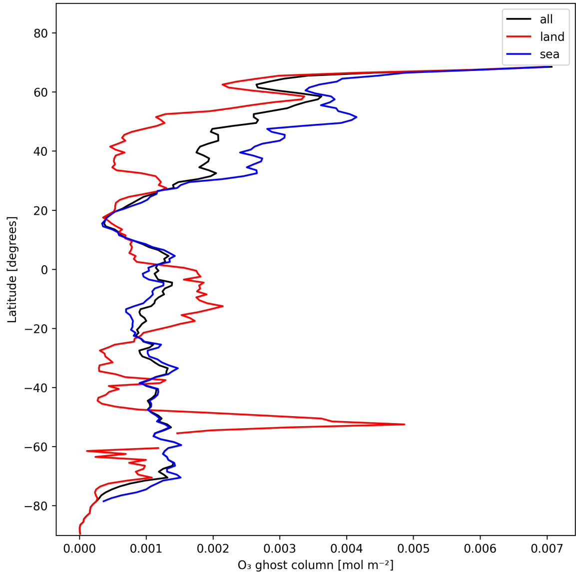
Figure 18: Zonal average of “O 3 ghost column” for 2025-01-15 to 2025-01-17.
