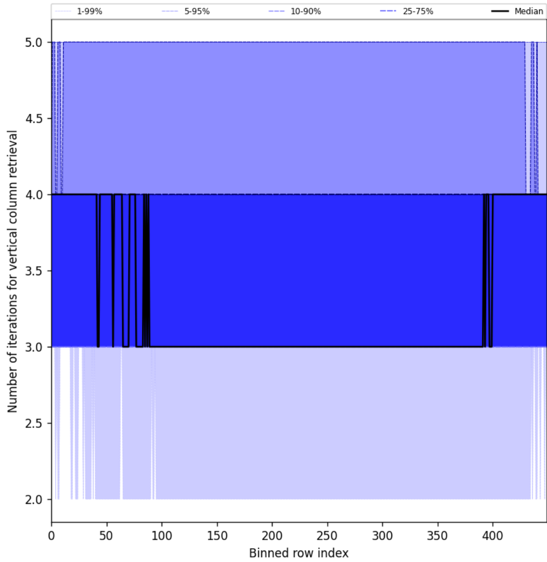
Figure 33: Along track statistics of “Number of iterations for vertical column retrieval” for 2025-01-15 to 2025-01-17
