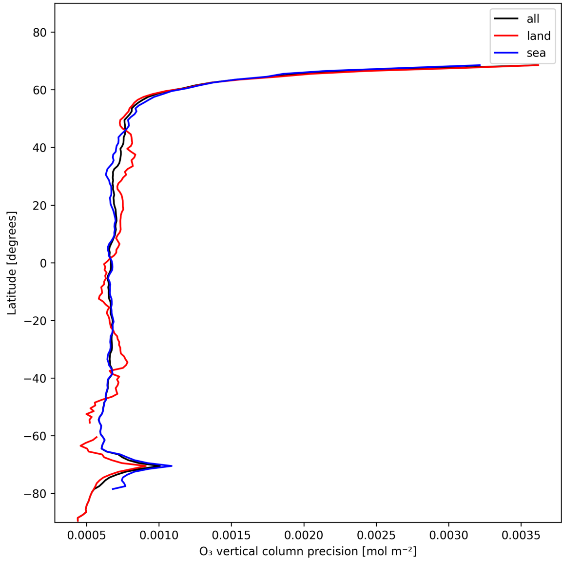
Figure 15: Zonal average of “O 3 vertical column precision” for 2025-01-15 to 2025-01-17.
