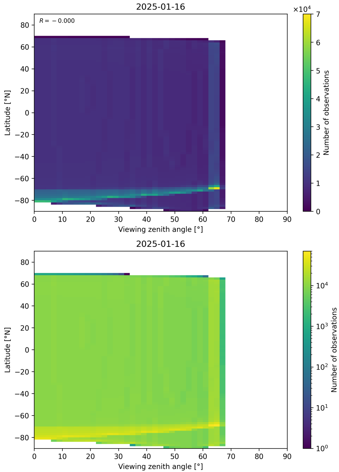
Figure 49: Scatter density plot of “Viewing zenith angle” against “Latitude” for 2025-01-15 to 2025-01-17.
