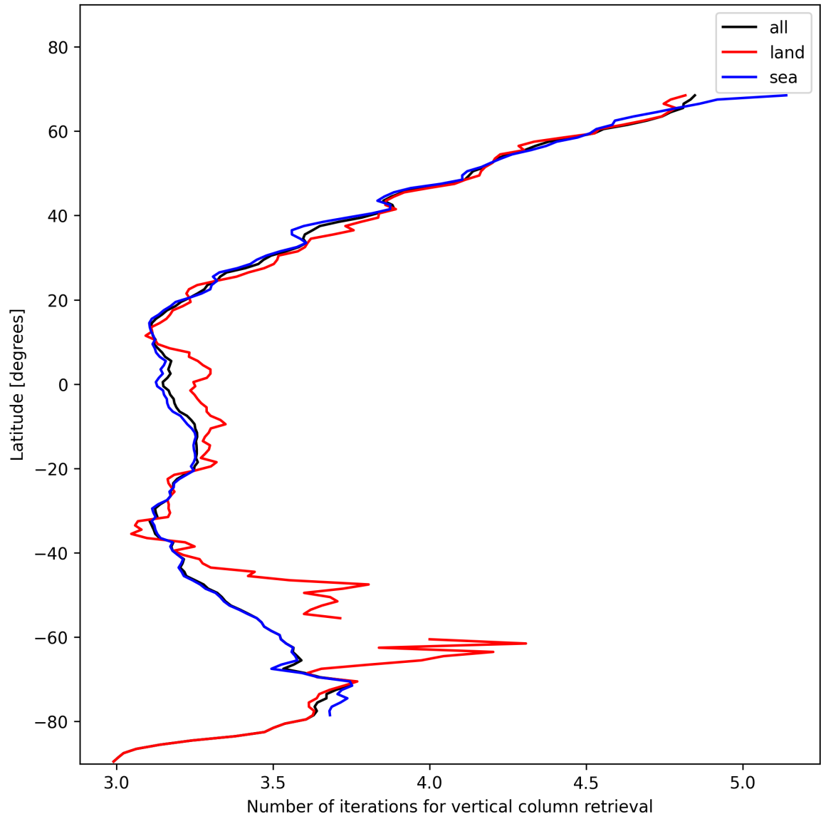
Figure 19: Zonal average of “Number of iterations for vertical column retrieval” for 2025-01-15 to 2025-01-17.
