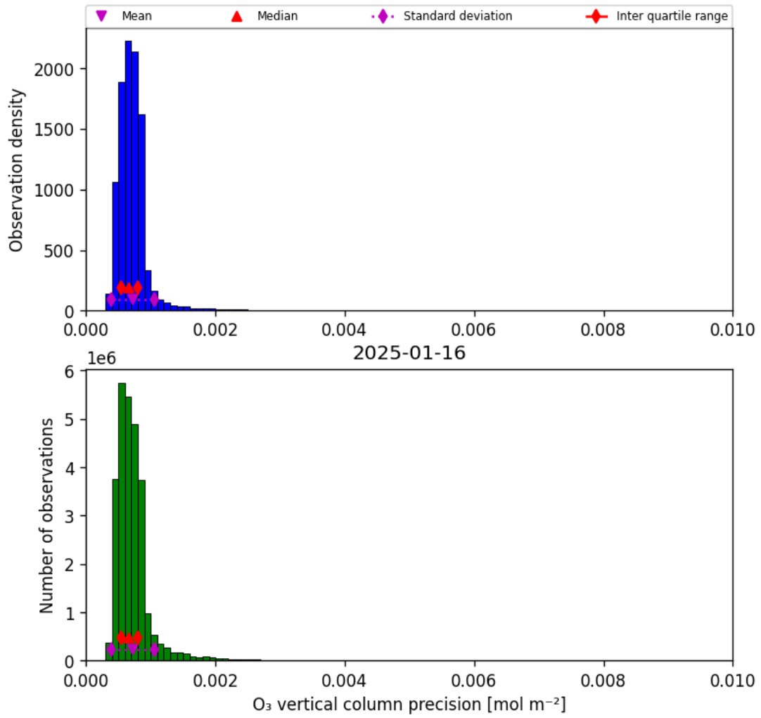
Figure 22: Histogram of "O 3 vertical column precision" for 2025-01-15 to 2025-01-17
