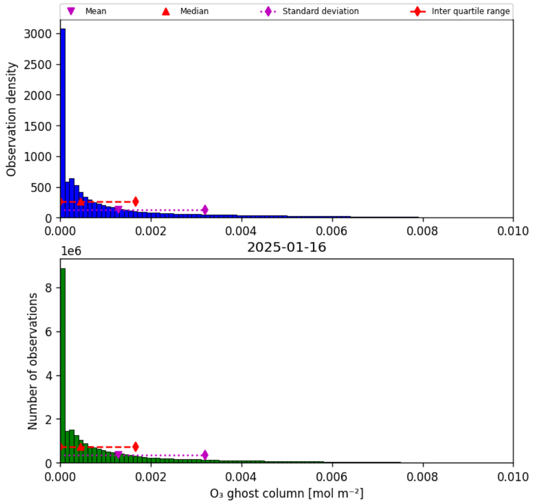
Figure 25: Histogram of “O 3 ghost column” for 2025-01-15 to 2025-01-17
