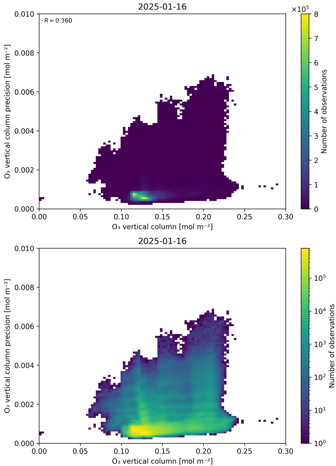
Figure 41: Scatter density plot of “O 3 vertical column” against “O 3 vertical column precision” for 2025-01-15 to 2025-01-17.
