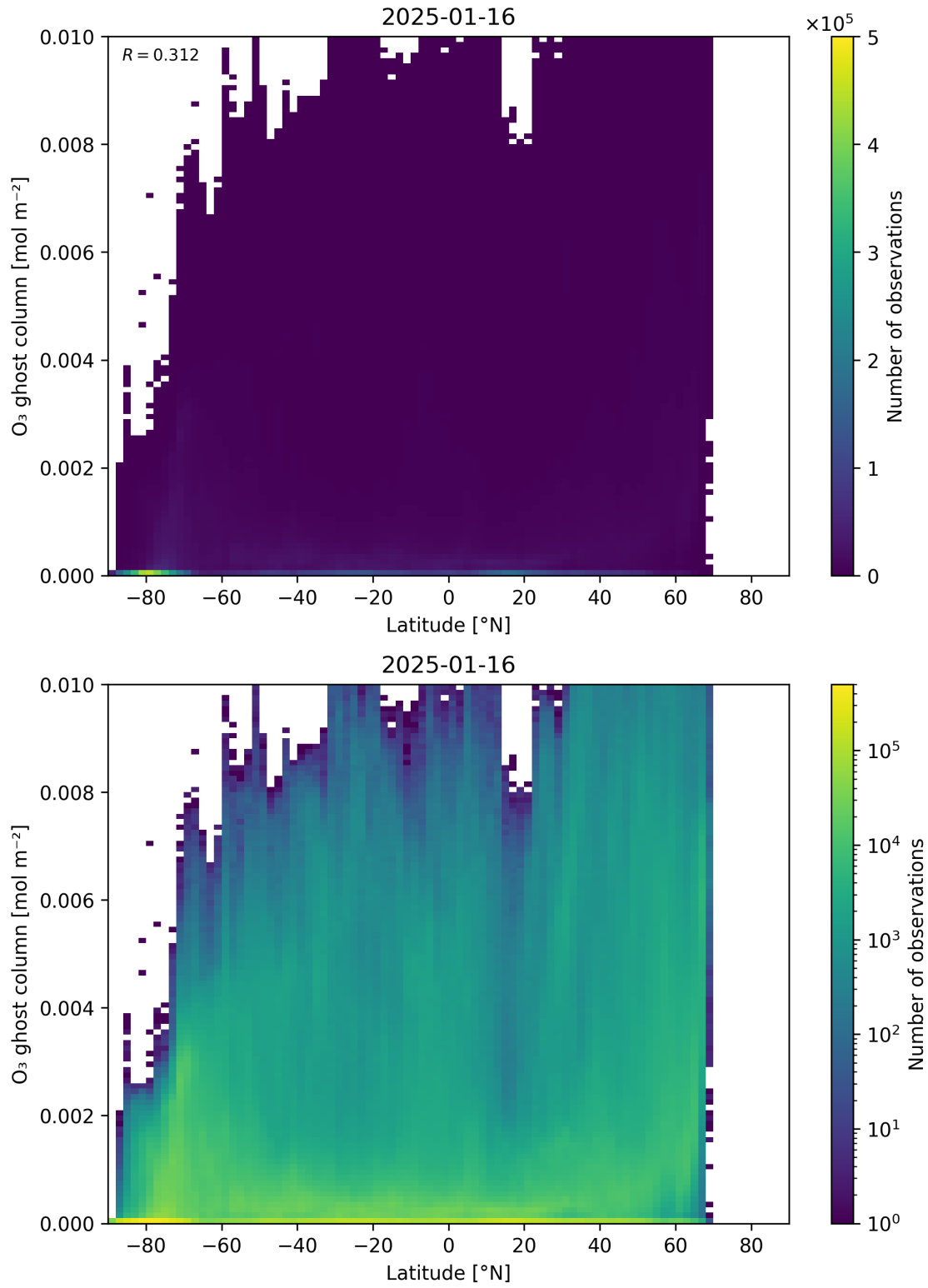
Figure 35: Scatter density plot of “Latitude” against “O 3 ghost column” for 2025-01-15 to 2025-01-17.
