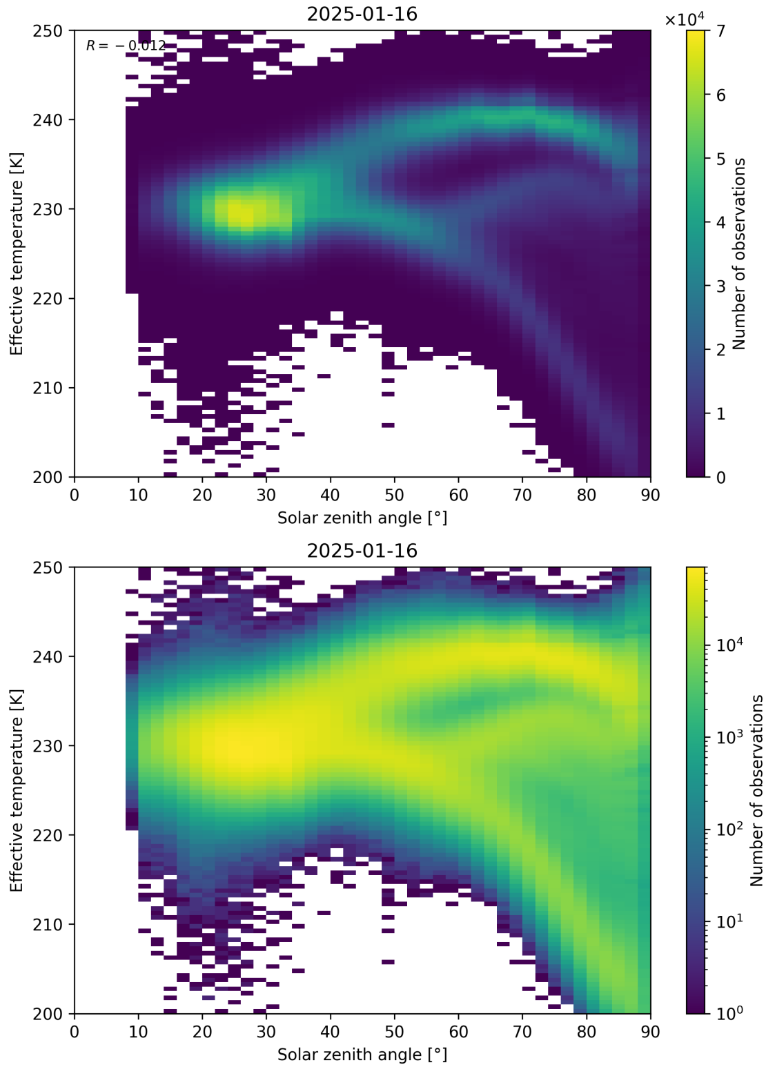
Figure 45: Scatter density plot of “Solar zenith angle” against “Effective temperature” for 2025-01-15 to 2025-01-17.
