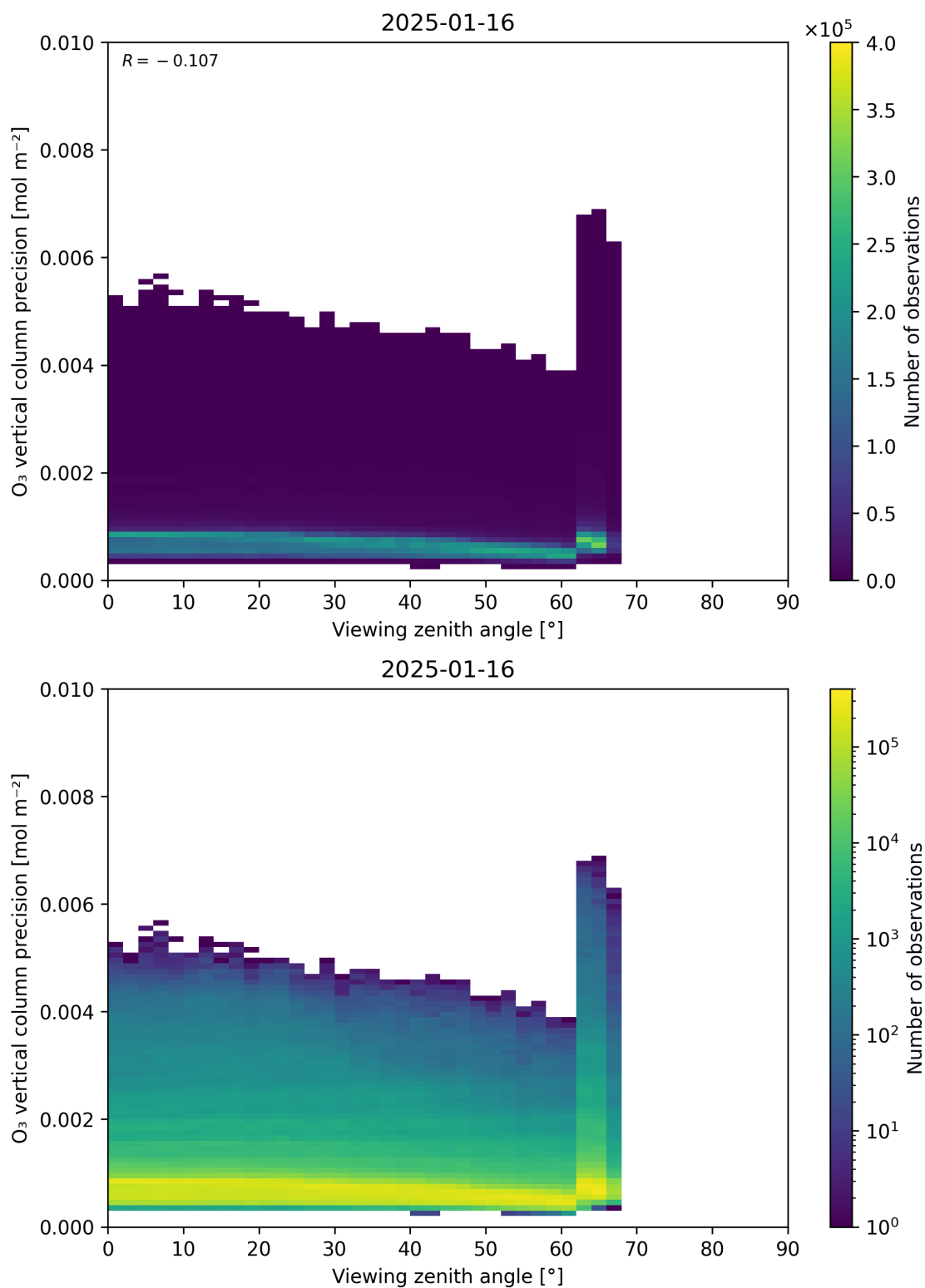
Figure 53: Scatter density plot of “Viewing zenith angle” against “O 3 vertical column precision” for 2025-01-15 to 2025-01-17.
