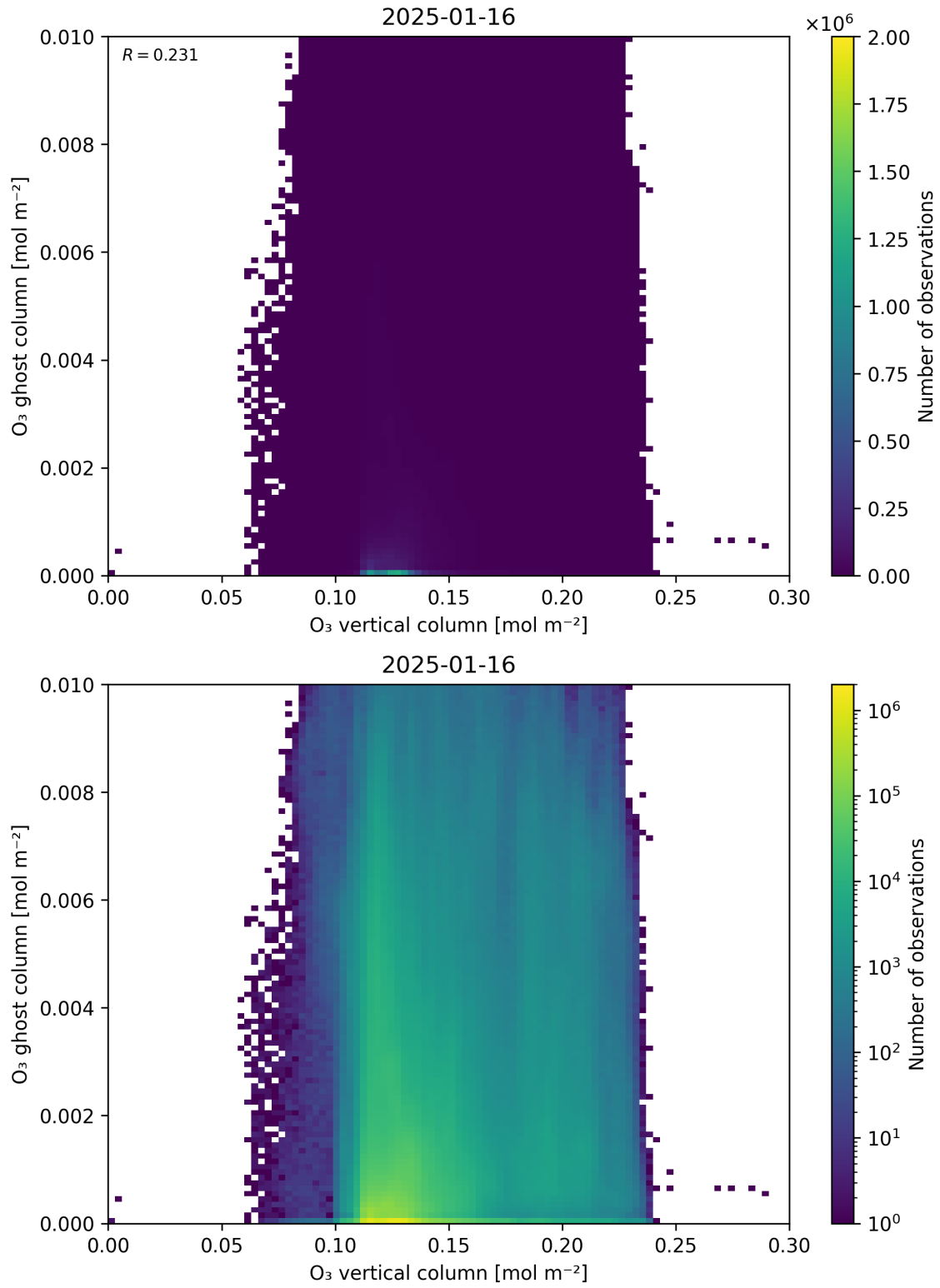
Figure 40: Scatter density plot of “O 3 vertical column” against “O 3 ghost column” for 2025-01-15 to 2025-01-17.
