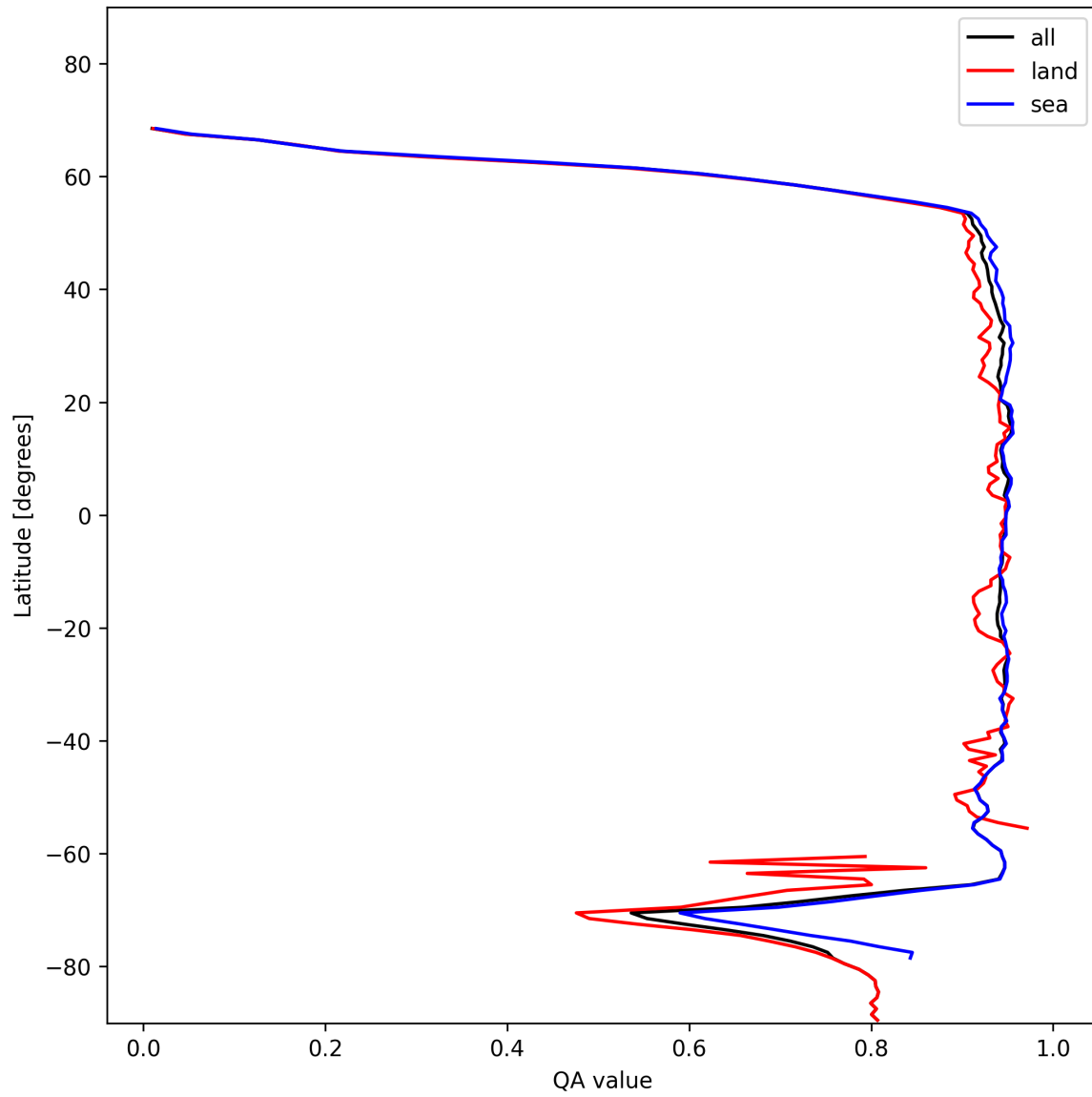
Figure 13: Zonal average of “QA value” for 2025-01-15 to 2025-01-17.
