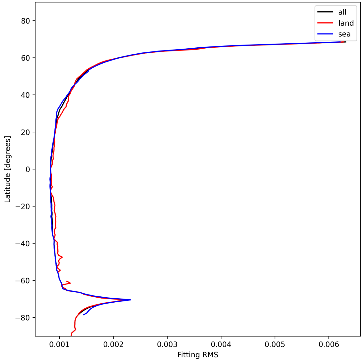
Figure 16: Zonal average of “Fitting RMS” for 2025-01-15 to 2025-01-17.
