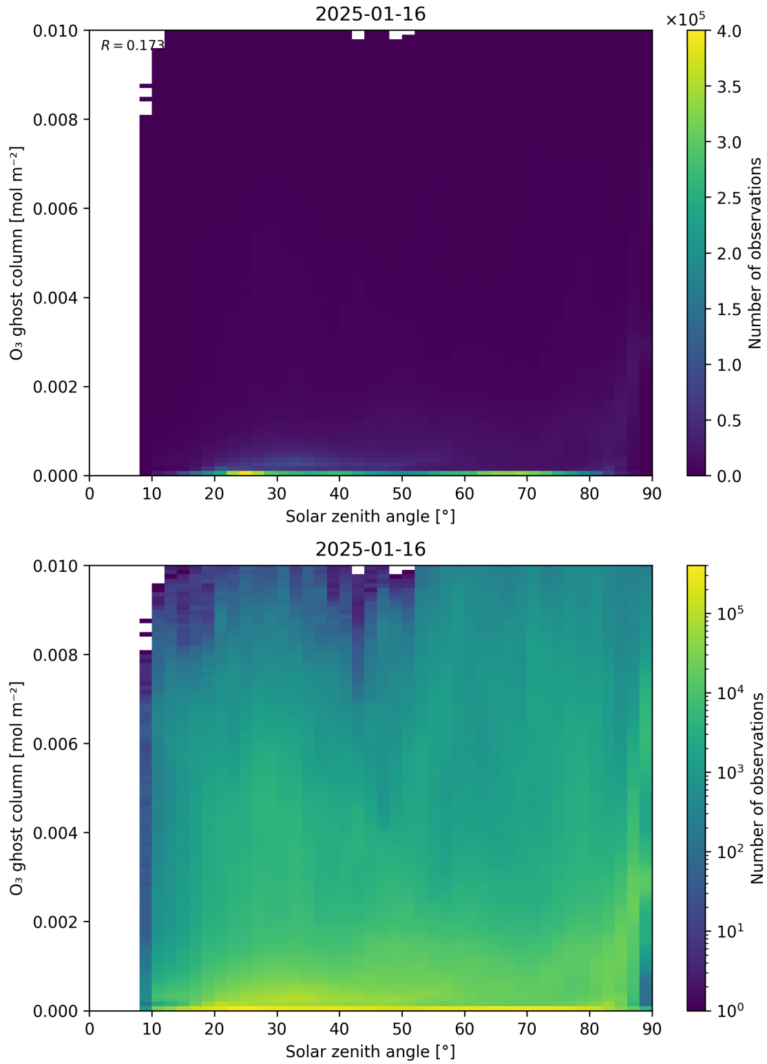
Figure 46: Scatter density plot of “Solar zenith angle” against “O 3 ghost column” for 2025-01-15 to 2025-01-17.
