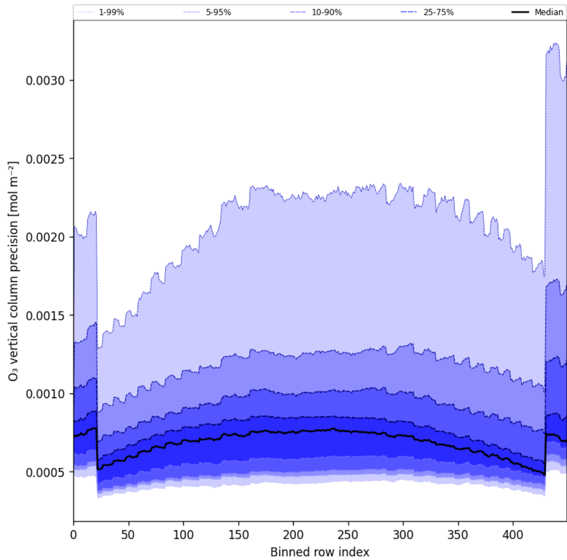
Figure 29: Along track statistics of “O 3 vertical column precision” for 2025-01-17 to 2025-01-18
