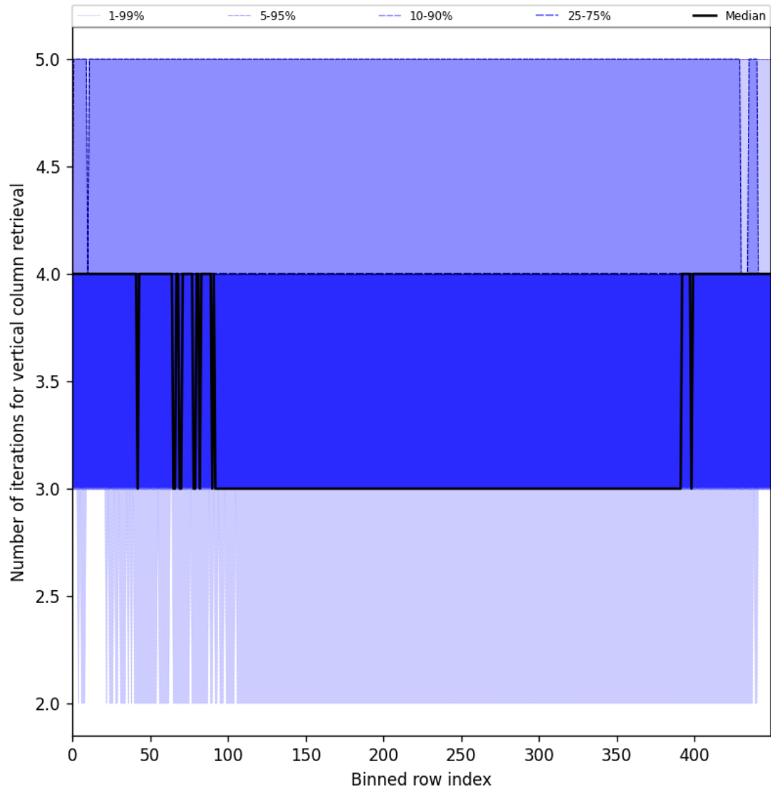
Figure 33: Along track statistics of “Number of iterations for vertical column retrieval” for 2025-01-17 to 2025-01-18
