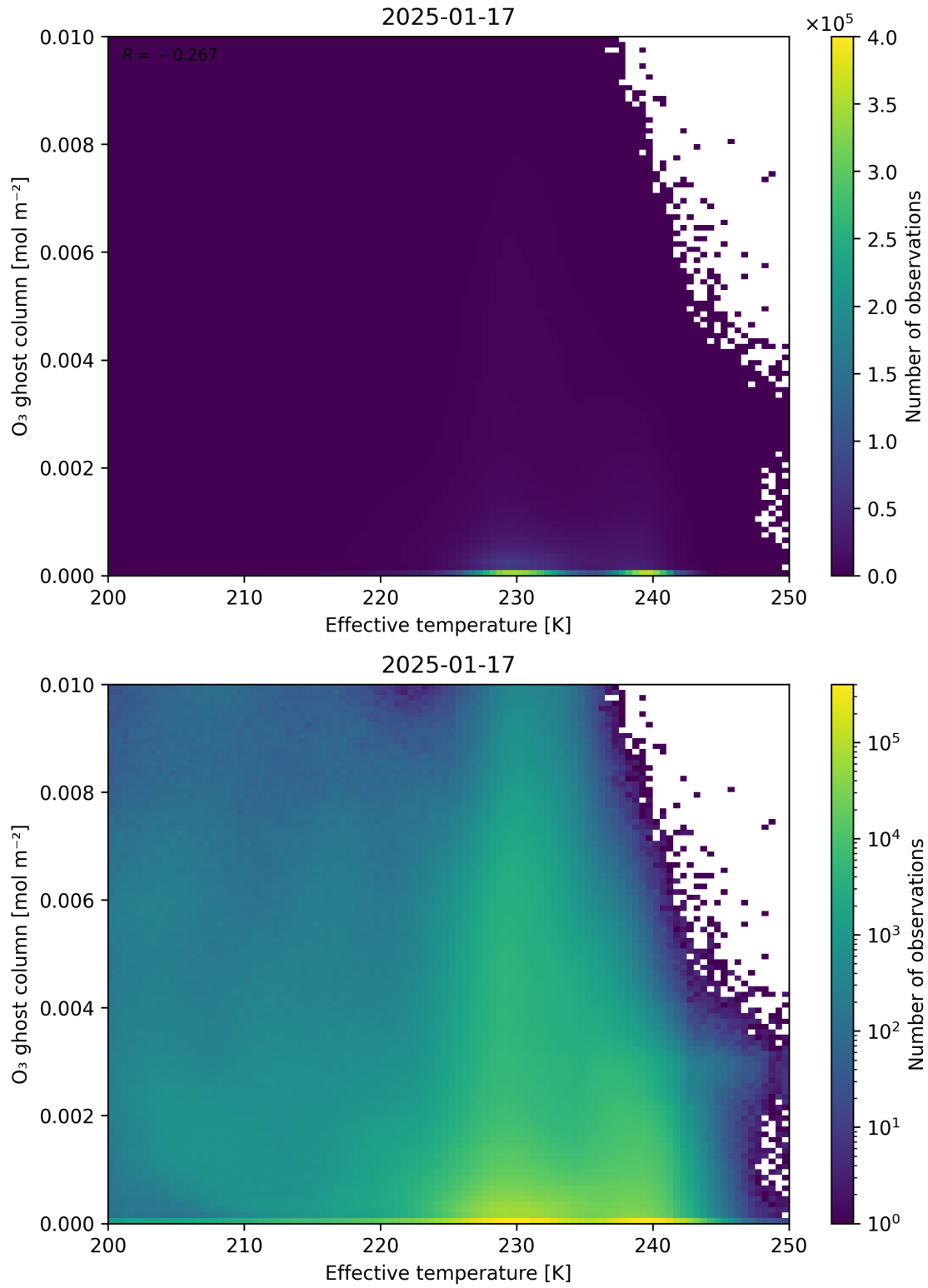
Figure 38: Scatter density plot of “Effective temperature” against “O 3 ghost column” for 2025-01-17 to 2025-01-18.
