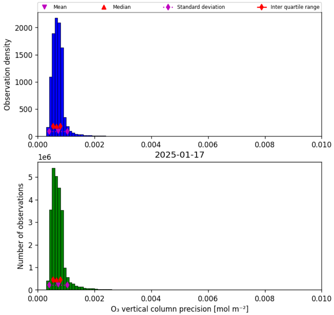
Figure 22: Histogram of “O 3 vertical column precision” for 2025-01-17 to 2025-01-18
