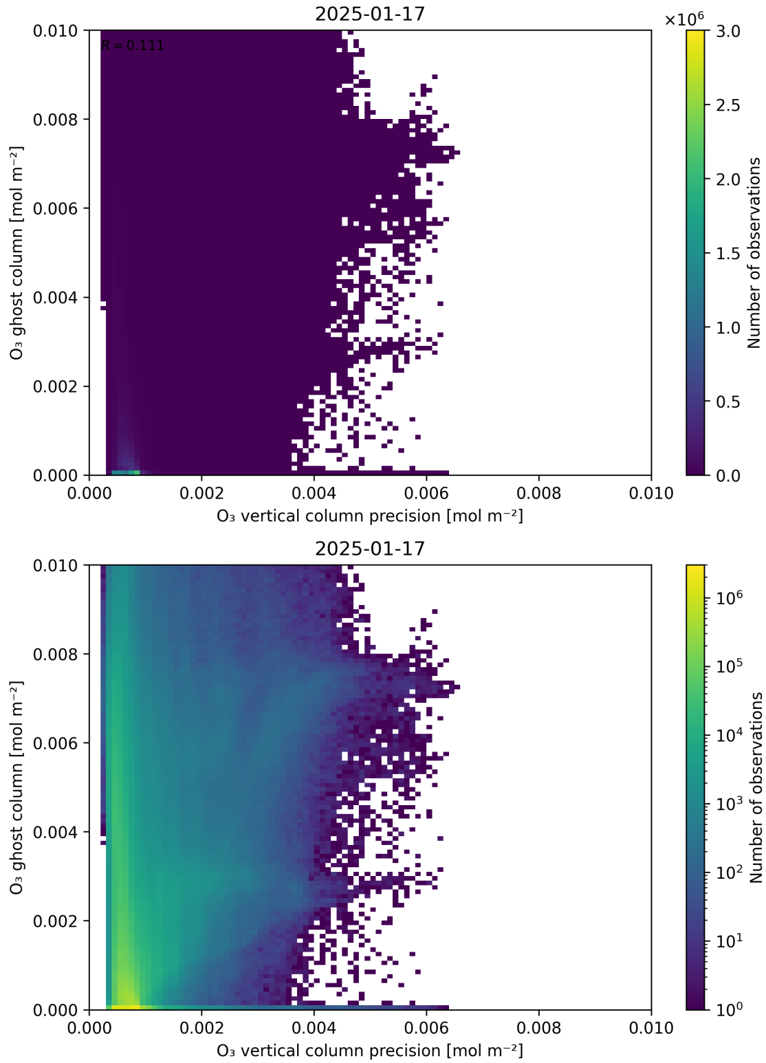
Figure 43: Scatter density plot of “O 3 vertical column precision” against “O 3 ghost column” for 2025-01-17 to 2025-01-18.
