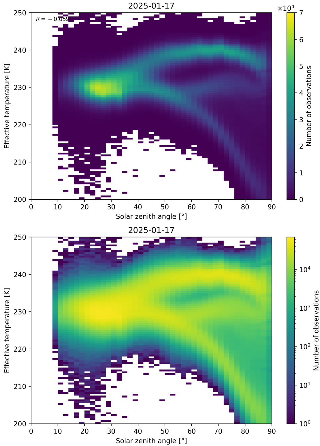
Figure 45: Scatter density plot of “Solar zenith angle” against “Effective temperature” for 2025-01-17 to 2025-01-18.
