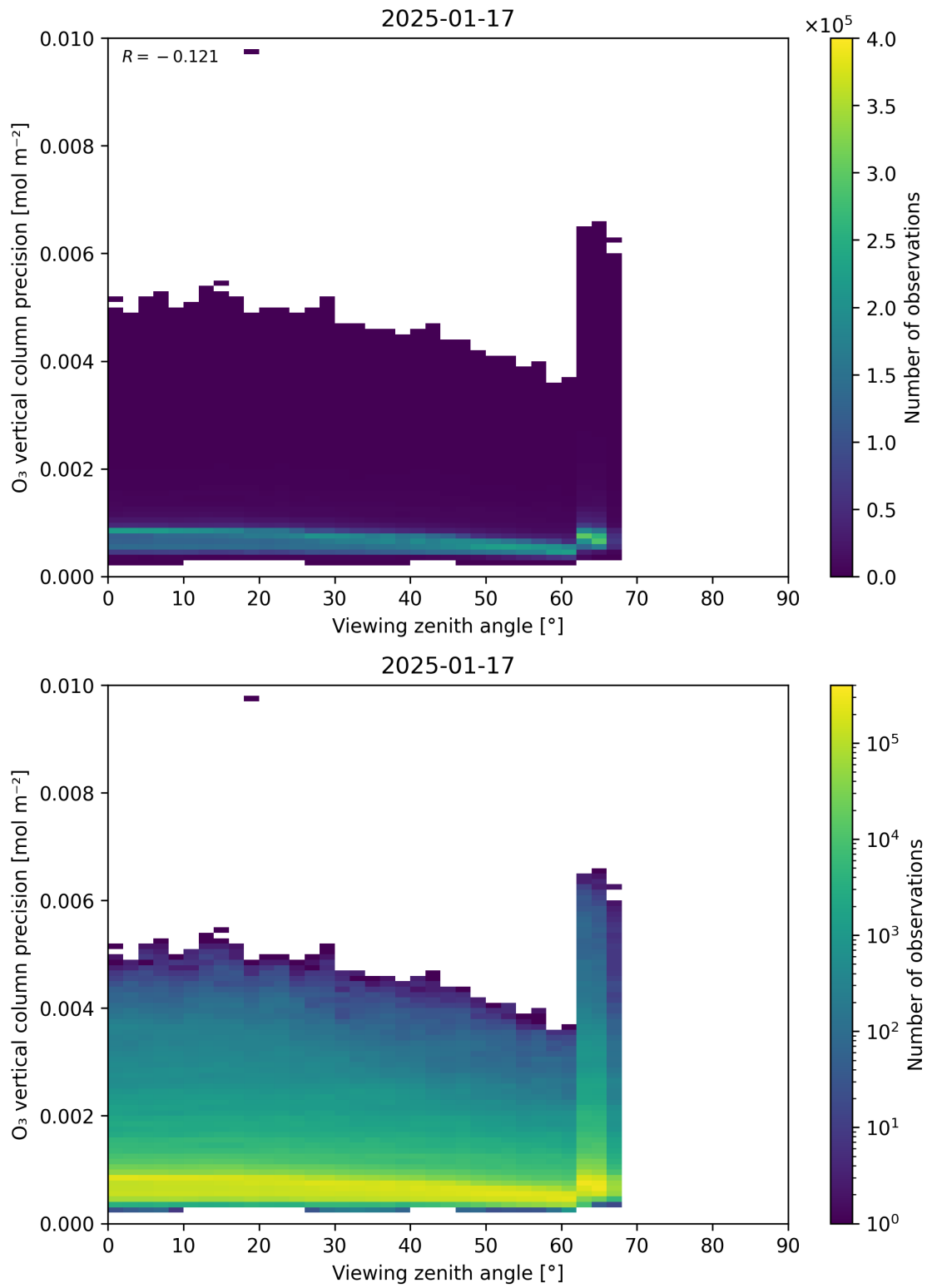
Figure 53: Scatter density plot of “Viewing zenith angle” against “O 3 vertical column precision” for 2025-01-17 to 2025-01-18.
