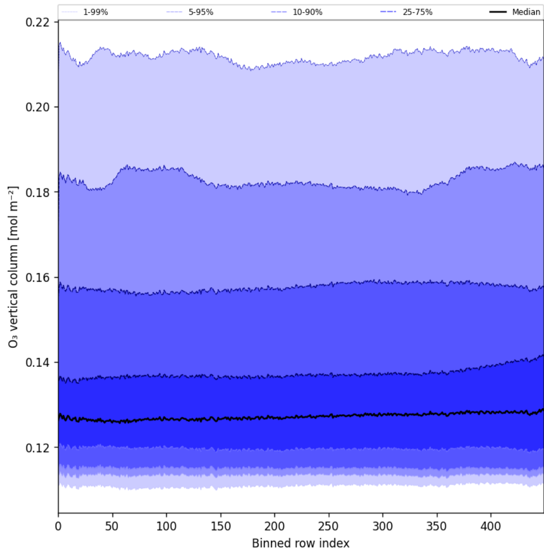
Figure 28: Along track statistics of “O 3 vertical column” for 2025-01-17 to 2025-01-18
