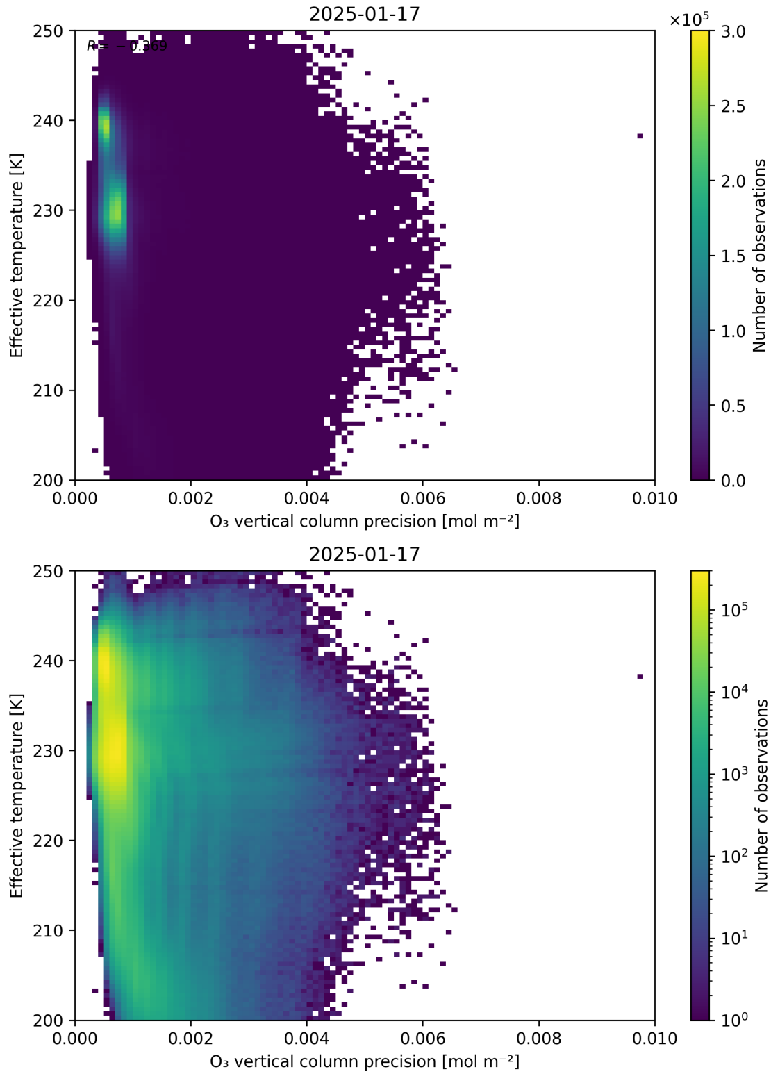
Figure 42: Scatter density plot of “O 3 vertical column precision” against “Effective temperature” for 2025-01-17 to 2025-01-18.
