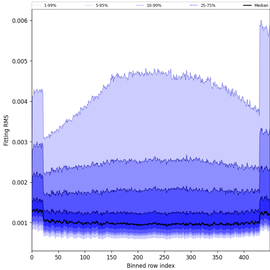
Figure 30: Along track statistics of “Fitting RMS” for 2025-01-17 to 2025-01-18
