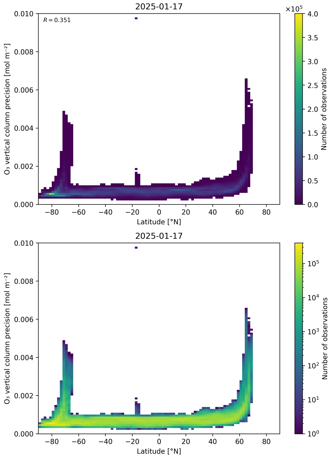
Figure 37: Scatter density plot of “Latitude” against “O 3 vertical column precision” for 2025-01-17 to 2025-01-18.
