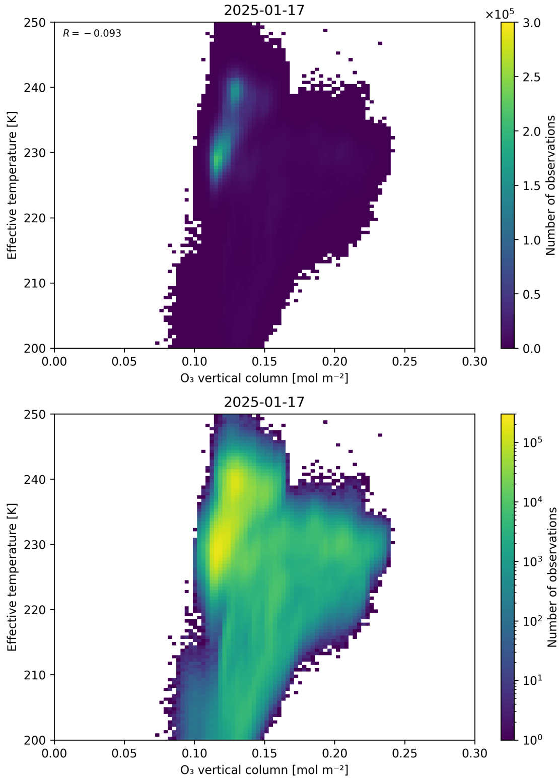
Figure 39: Scatter density plot of “O 3 vertical column” against “Effective temperature” for 2025-01-17 to 2025-01-18.
