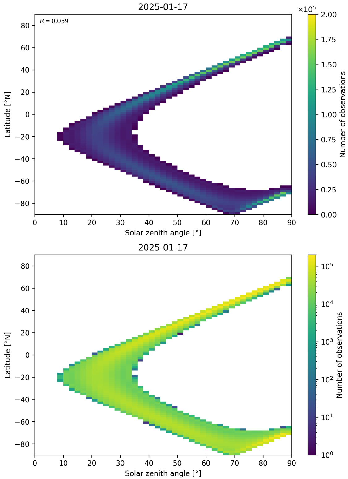
Figure 44: Scatter density plot of “Solar zenith angle” against “Latitude” for 2025-01-17 to 2025-01-18.
