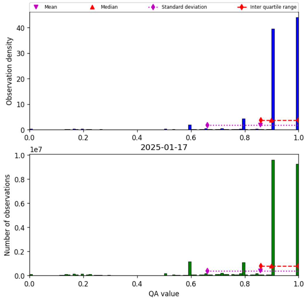
Figure 20: Histogram of “QA value” for 2025-01-17 to 2025-01-18
