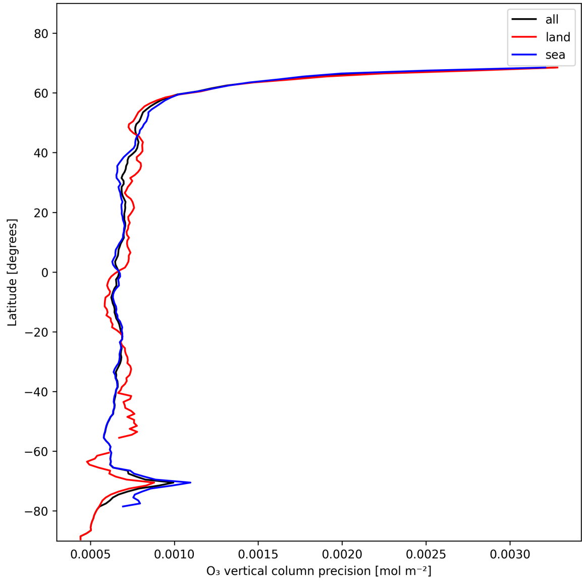
Figure 15: Zonal average of “O 3 vertical column precision” for 2025-01-17 to 2025-01-18.
