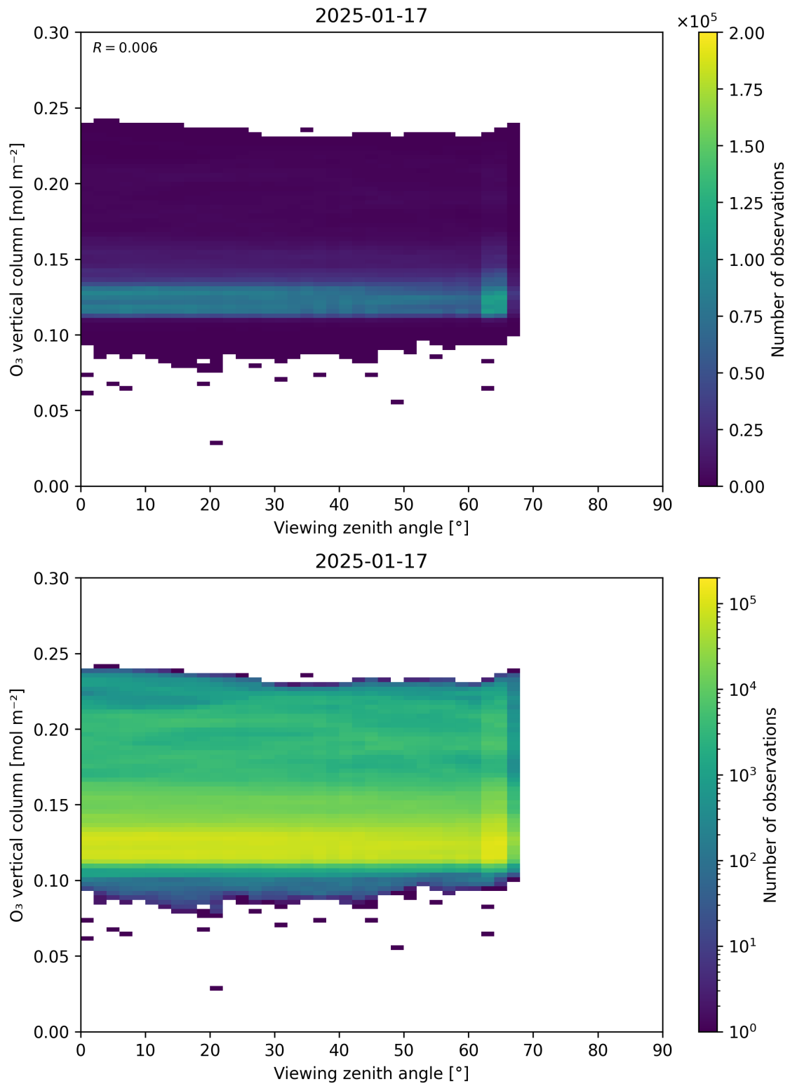
Figure 52: Scatter density plot of “Viewing zenith angle” against “O 3 vertical column” for 2025-01-17 to 2025-01-18.
