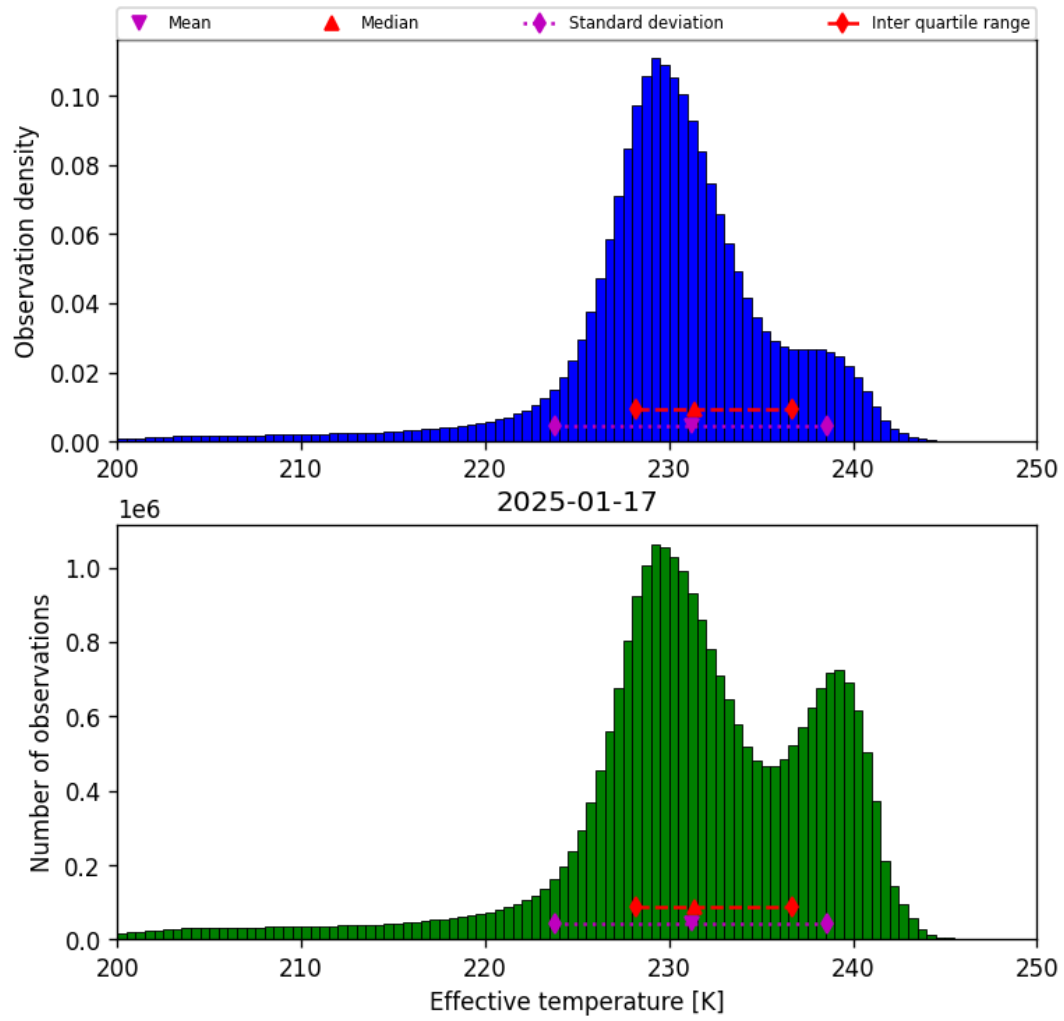
Figure 24: Histogram of “Effective temperature” for 2025-01-17 to 2025-01-18
