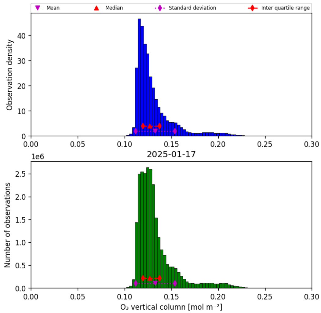
Figure 21: Histogram of “O 3 vertical column” for 2025-01-17 to 2025-01-18
