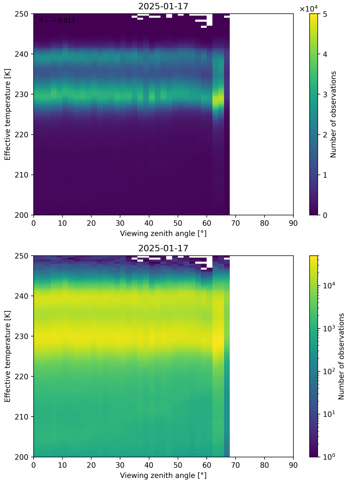
Figure 50: Scatter density plot of “Viewing zenith angle” against “Effective temperature” for 2025-01-17 to 2025-01-18.
