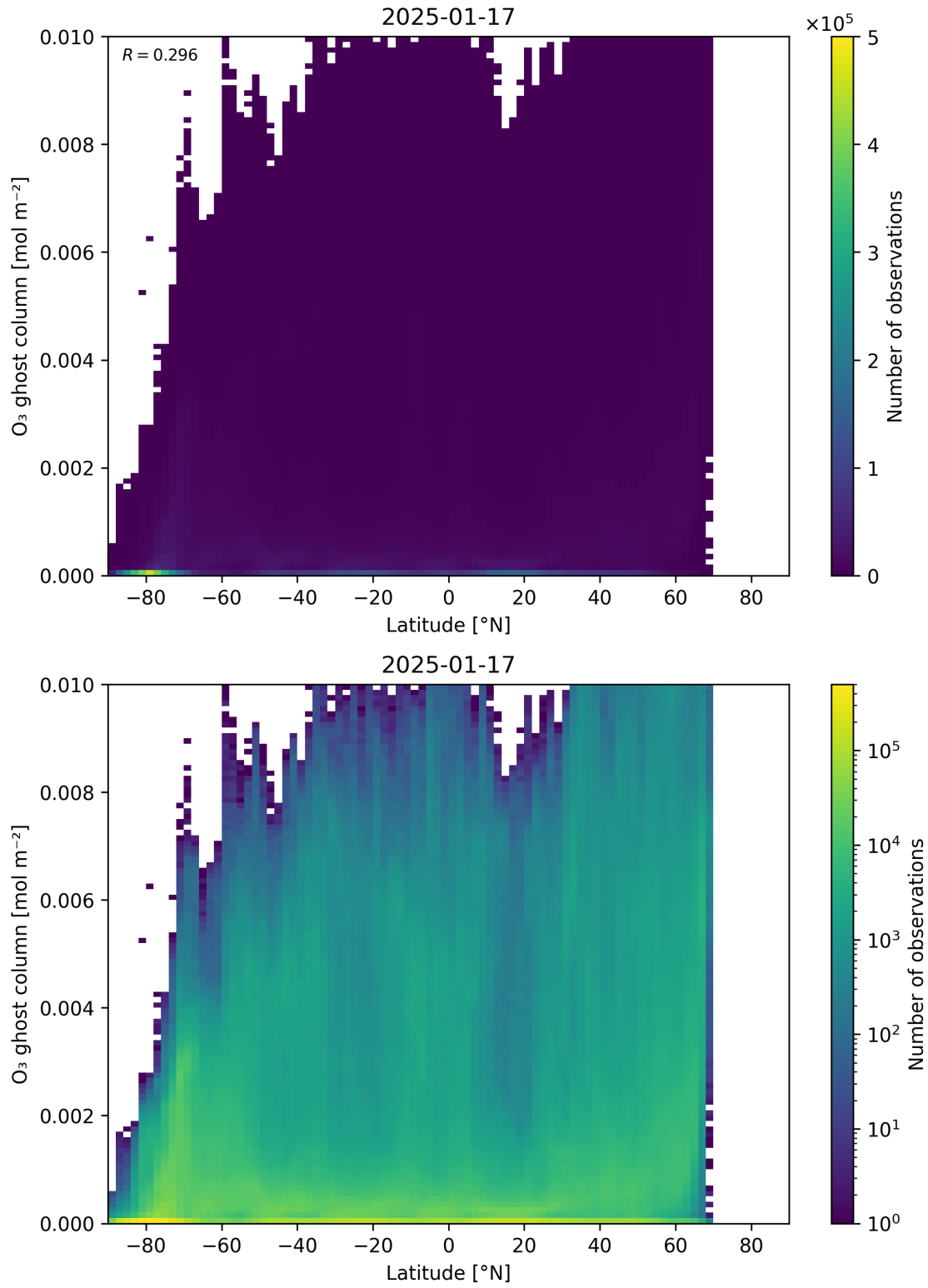
Figure 35: Scatter density plot of “Latitude” against “O 3 ghost column” for 2025-01-17 to 2025-01-18.
