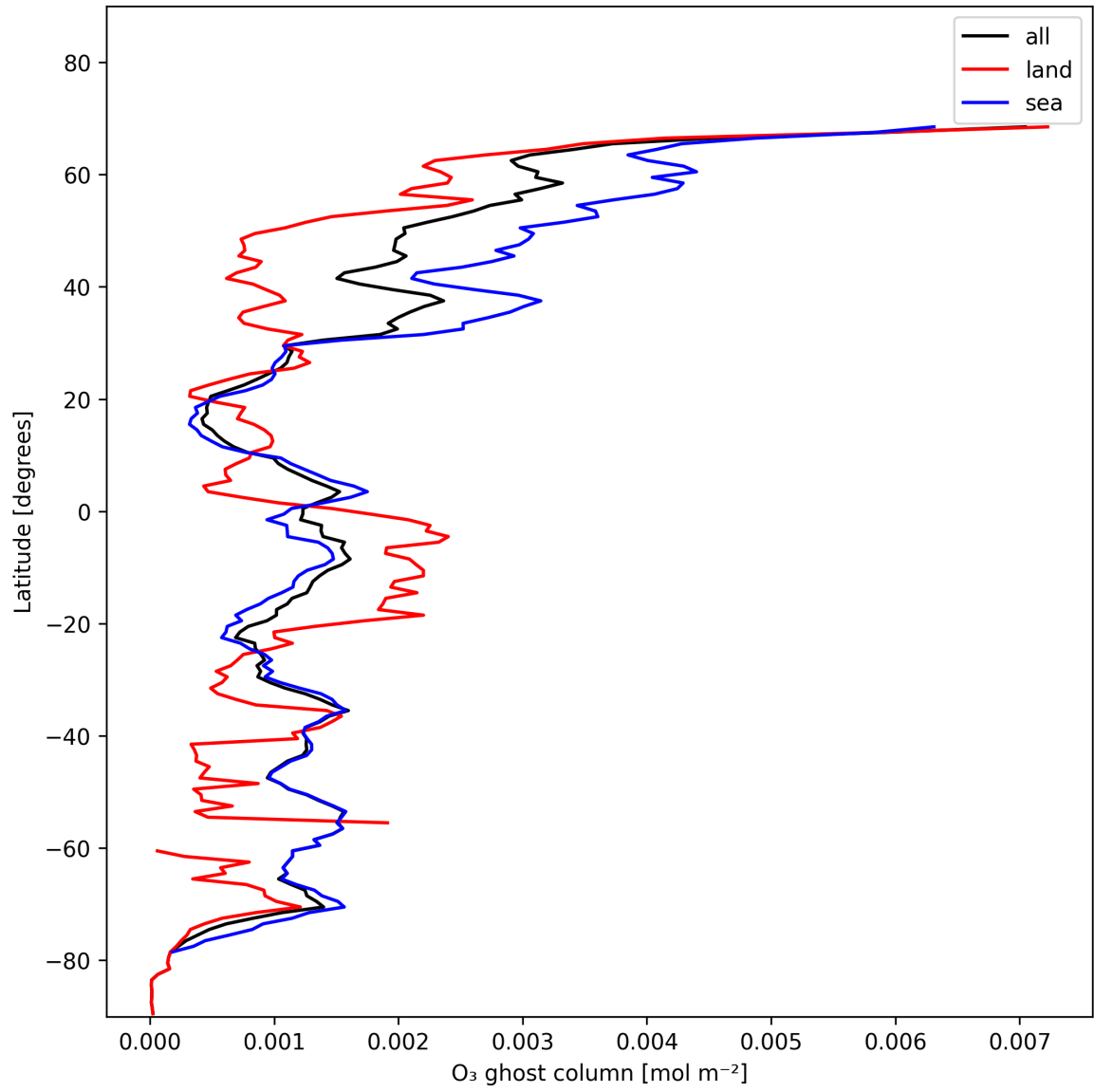
Figure 18: Zonal average of "O 3 ghost column" for 2025-01-17 to 2025-01-18.
