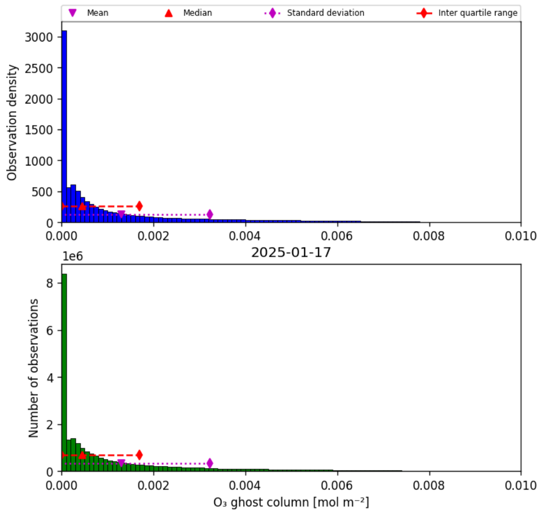
Figure 25: Histogram of “O 3 ghost column” for 2025-01-17 to 2025-01-18
