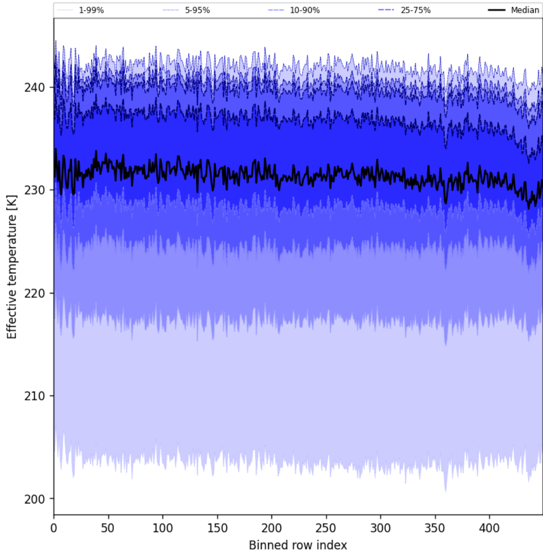
Figure 31: Along track statistics of “Effective temperature” for 2025-01-17 to 2025-01-18
