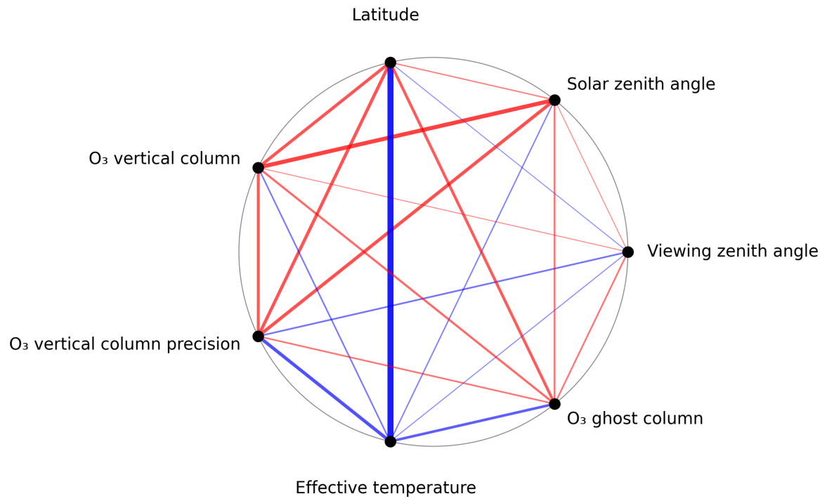
Figure 1: Map of correlation graph for 2025-01-17 to 2025-01-18.
