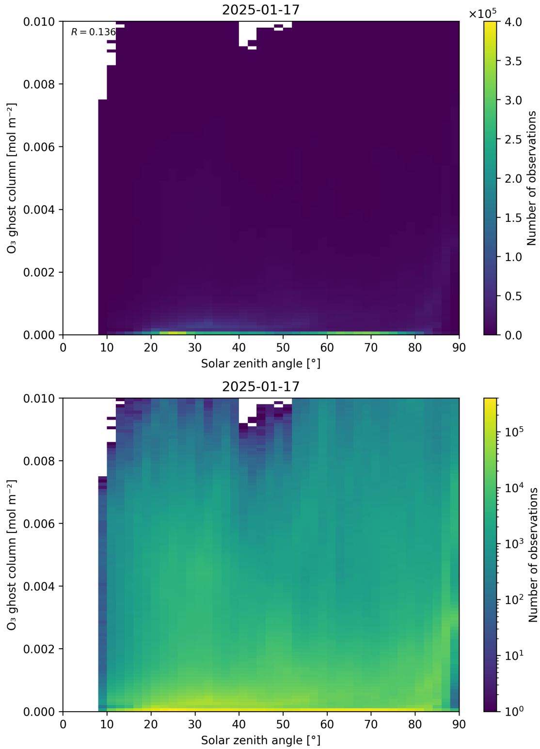
Figure 46: Scatter density plot of “Solar zenith angle” against “O 3 ghost column” for 2025-01-17 to 2025-01-18.
