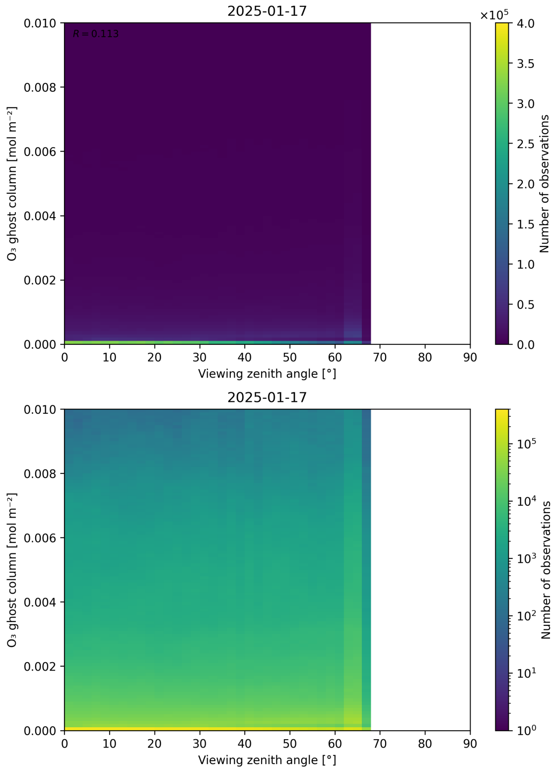
Figure 51: Scatter density plot of “Viewing zenith angle” against “O 3 ghost column” for 2025-01-17 to 2025-01-18.
