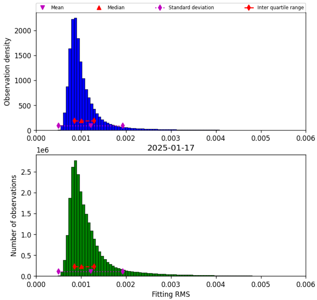
Figure 23: Histogram of “Fitting RMS” for 2025-01-17 to 2025-01-18
