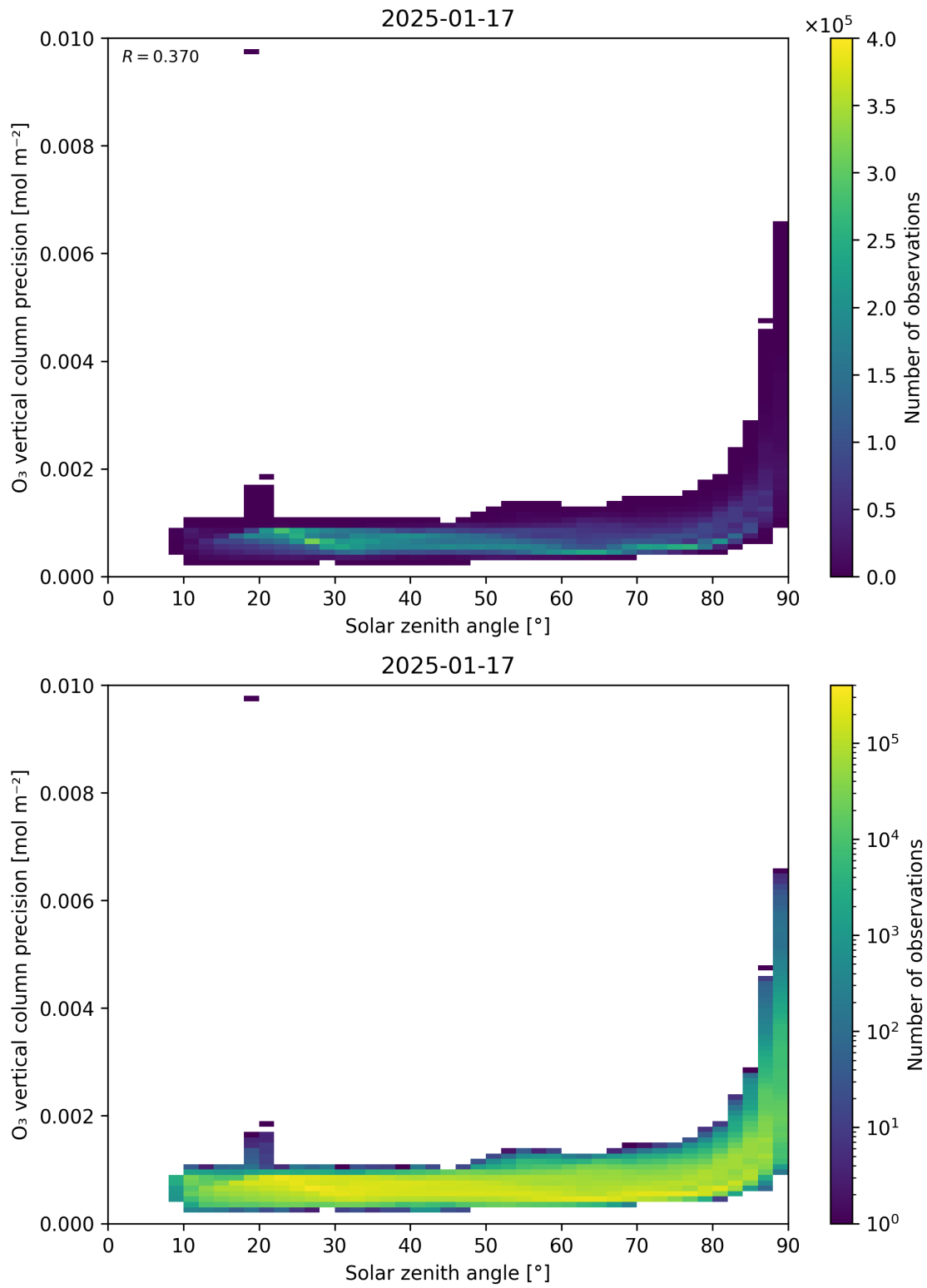
Figure 48: Scatter density plot of “Solar zenith angle” against “O 3 vertical column precision” for 2025-01-17 to 2025-01-18.
