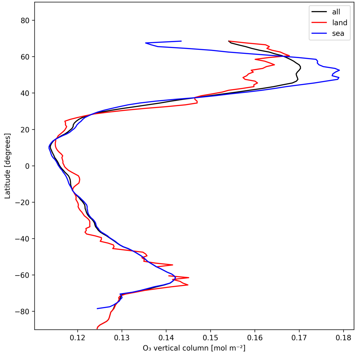
Figure 14: Zonal average of “O 3 vertical column” for 2025-01-17 to 2025-01-18.
