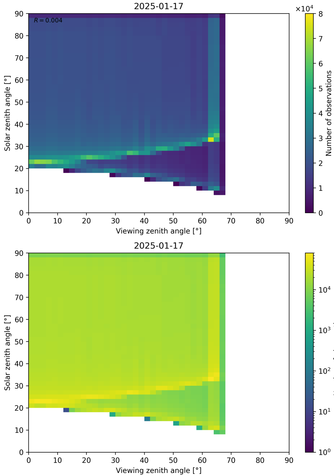
Figure 54: Scatter density plot of “Viewing zenith angle” against “Solar zenith angle” for 2025-01-17 to 2025-01-18.
