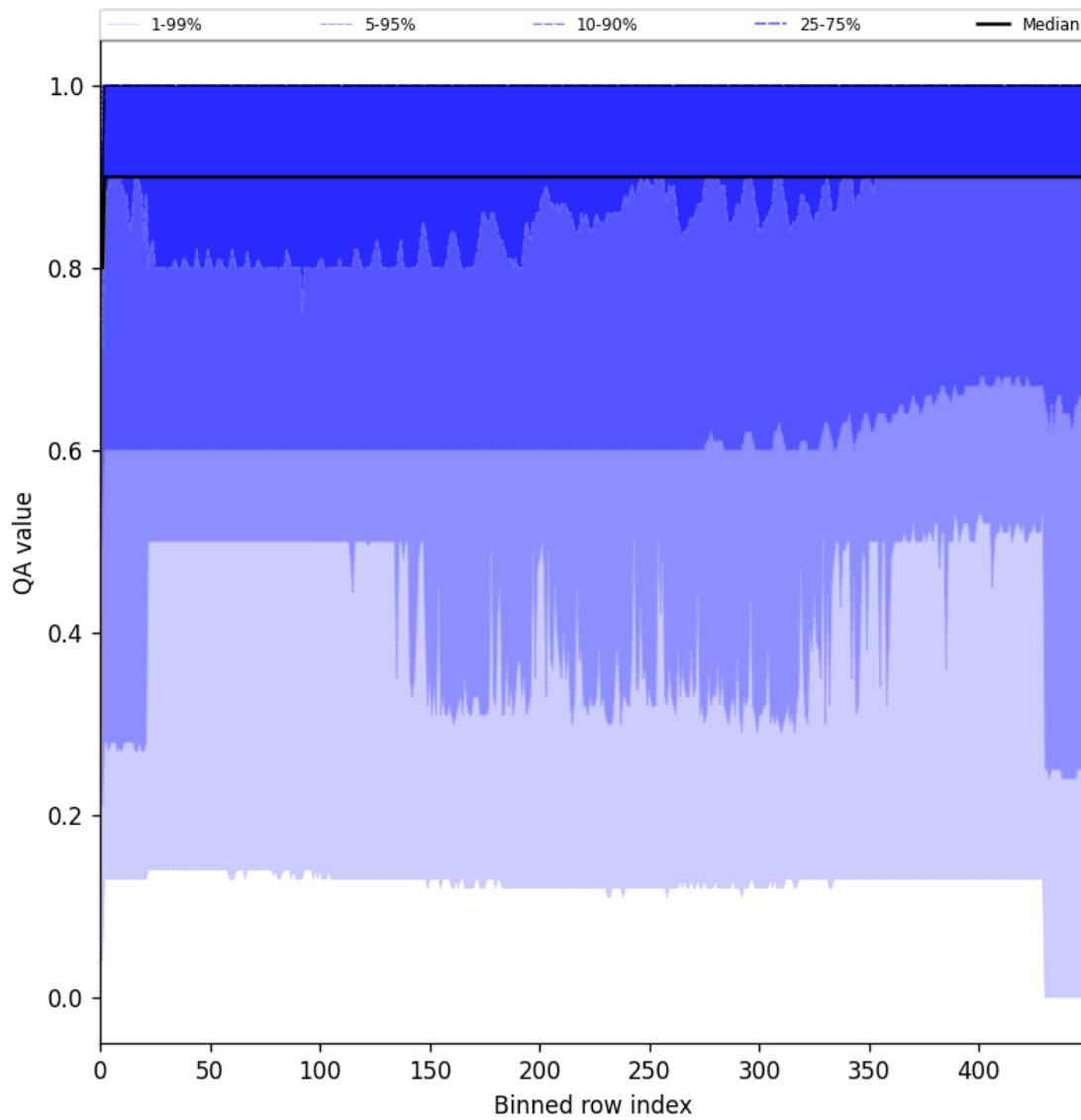
Figure 27: Along track statistics of “QA value” for 2025-01-17 to 2025-01-18
