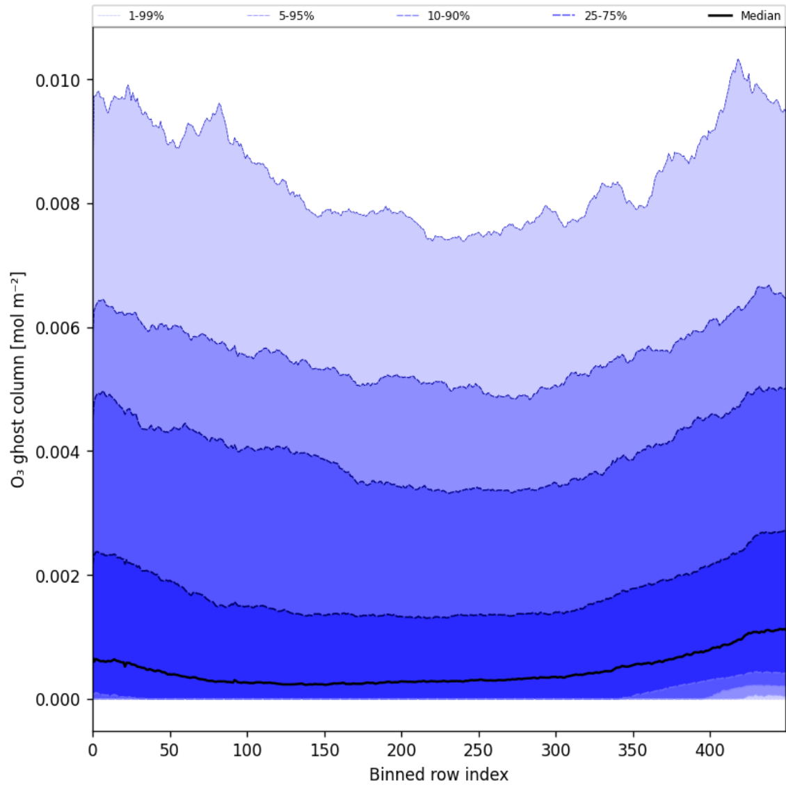
Figure 32: Along track statistics of “O 3 ghost column” for 2025-01-17 to 2025-01-18
