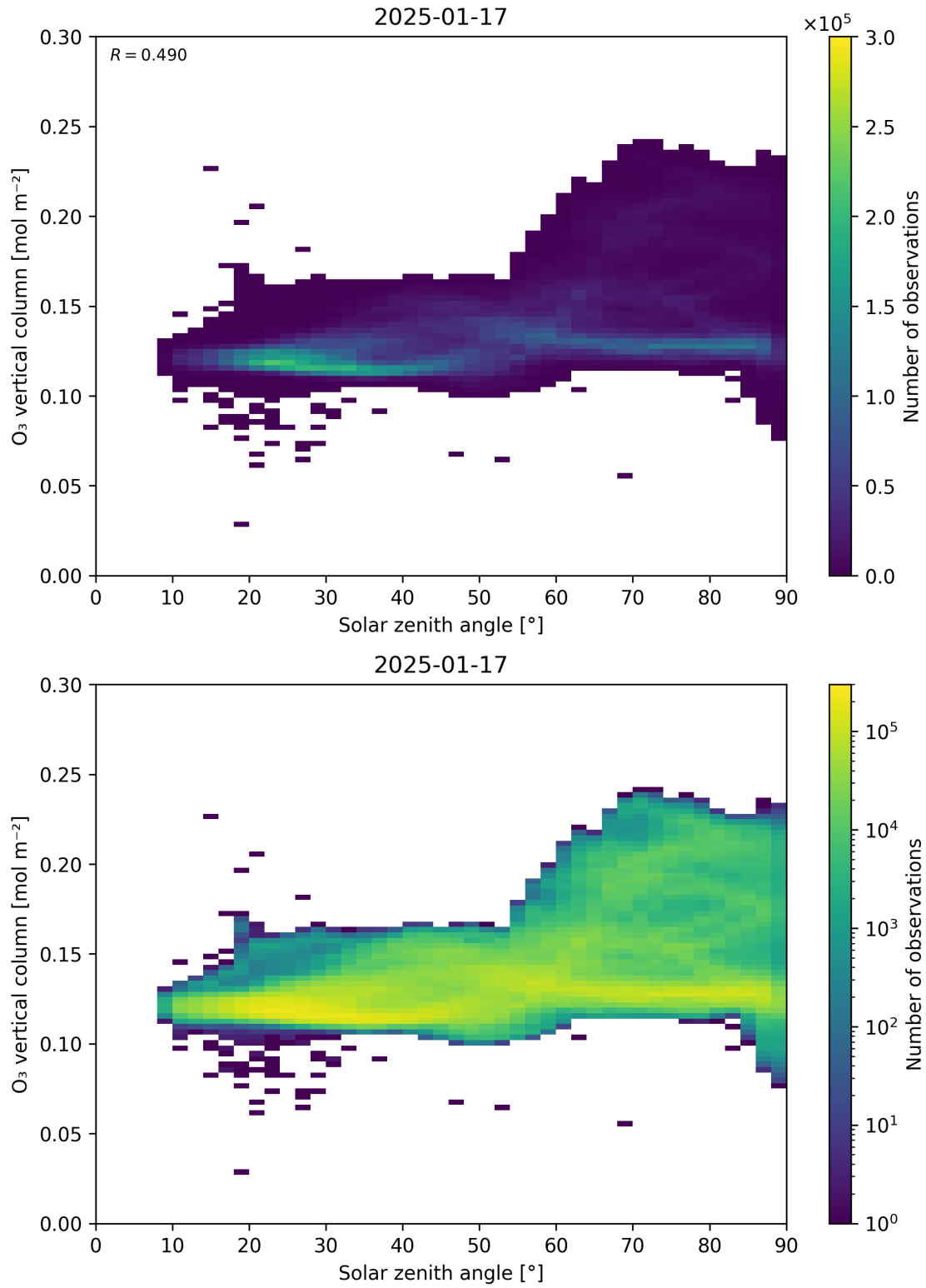
Figure 47: Scatter density plot of “Solar zenith angle” against “O 3 vertical column” for 2025-01-17 to 2025-01-18.
