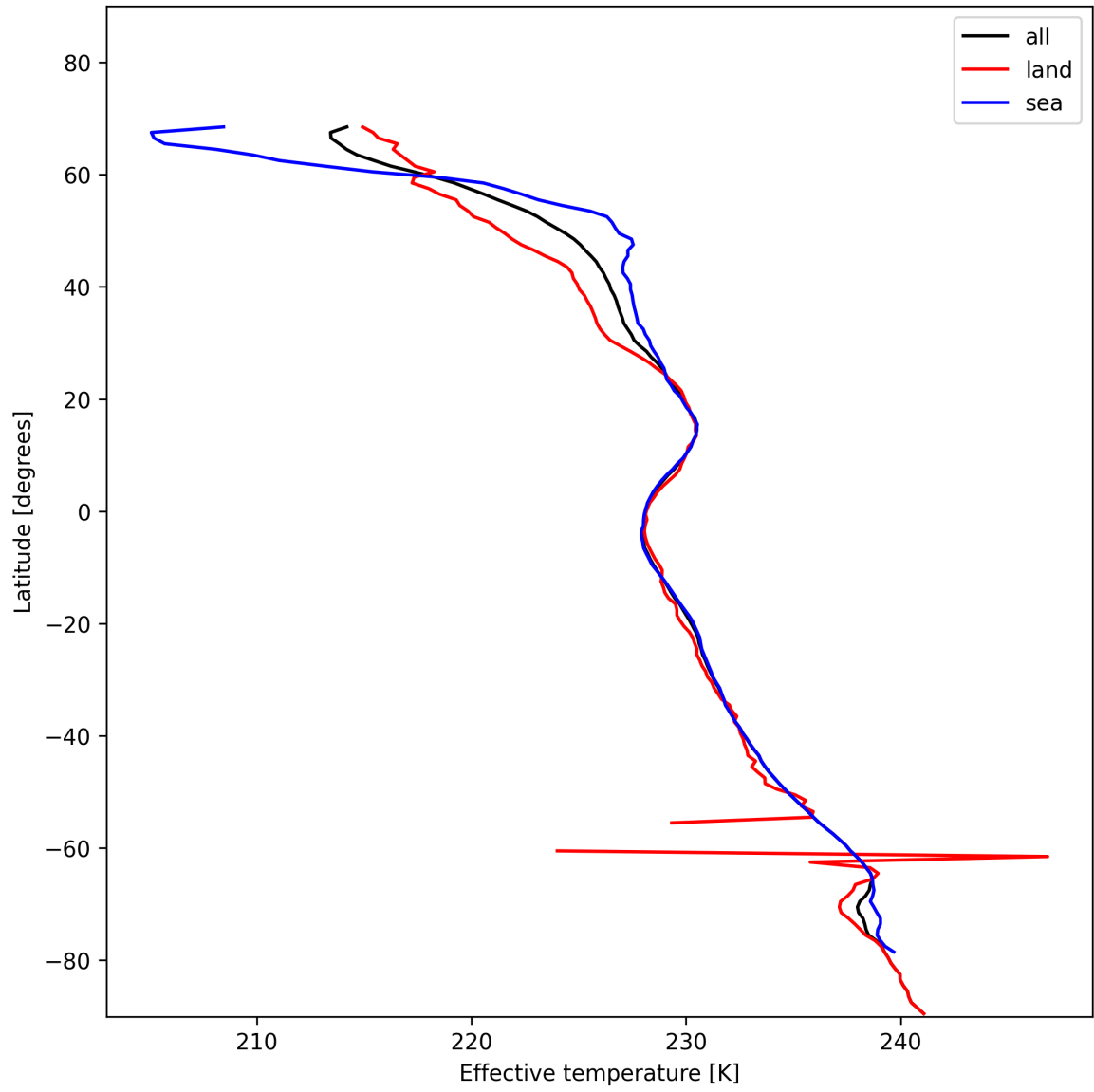
Figure 17: Zonal average of “Effective temperature” for 2025-01-17 to 2025-01-18.
