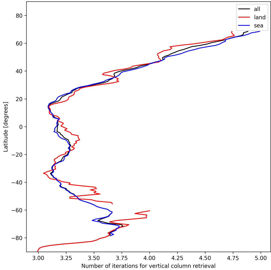
Figure 19: Zonal average of “Number of iterations for vertical column retrieval” for 2025-01-17 to 2025-01-18.
