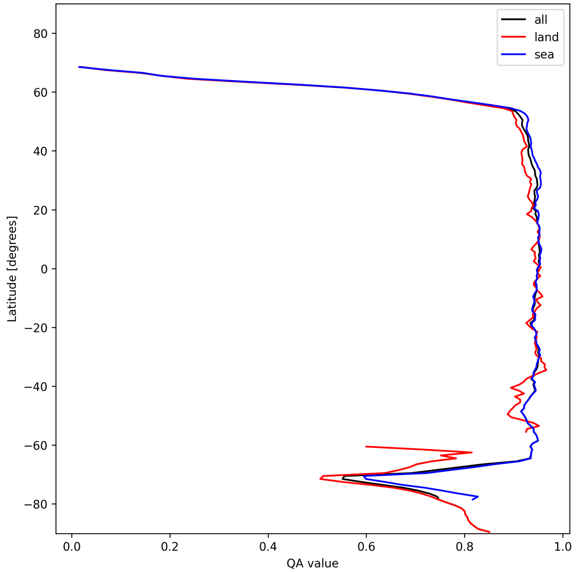
Figure 13: Zonal average of “QA value” for 2025-01-17 to 2025-01-18.
