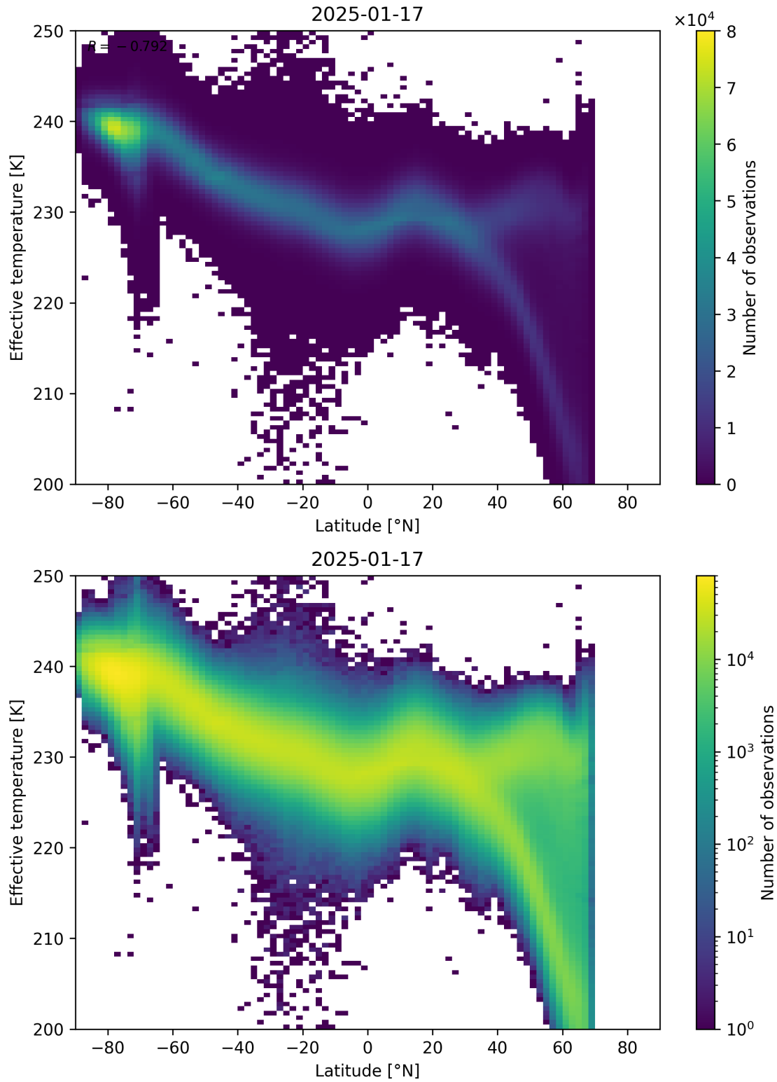
Figure 34: Scatter density plot of “Latitude” against “Effective temperature” for 2025-01-17 to 2025-01-18.
