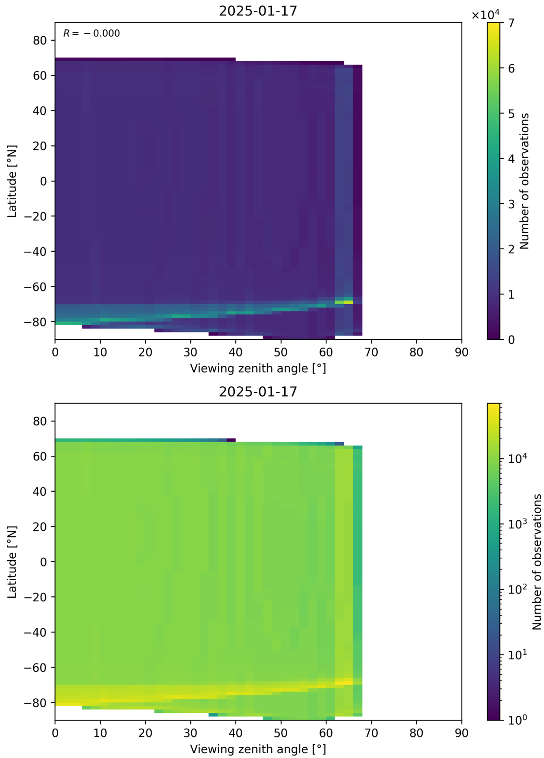
Figure 49: Scatter density plot of “Viewing zenith angle” against “Latitude” for 2025-01-17 to 2025-01-18.
