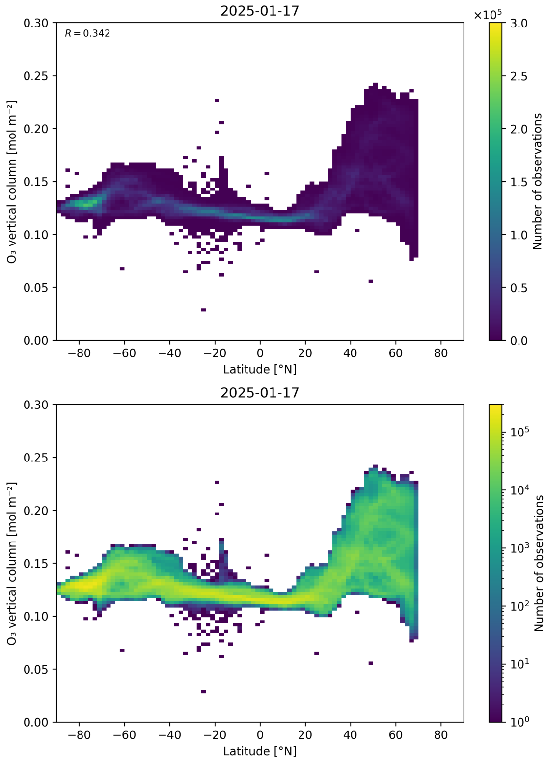
Figure 36: Scatter density plot of “Latitude” against “O 3 vertical column” for 2025-01-17 to 2025-01-18.
