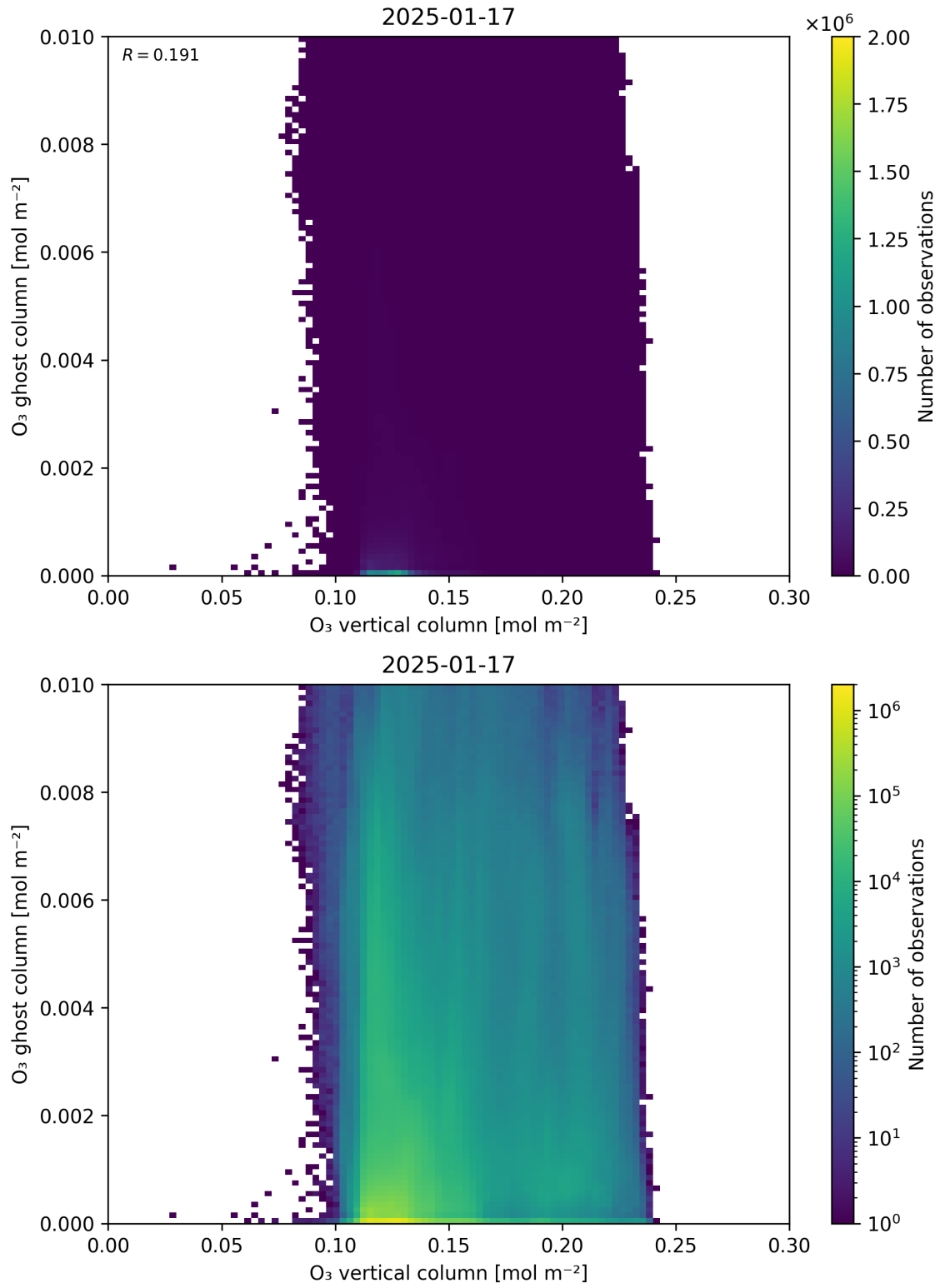
Figure 40: Scatter density plot of “O 3 vertical column” against “O 3 ghost column” for 2025-01-17 to 2025-01-18.
