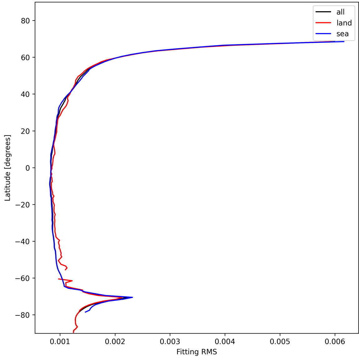
Figure 16: Zonal average of “Fitting RMS” for 2025-01-17 to 2025-01-18.
