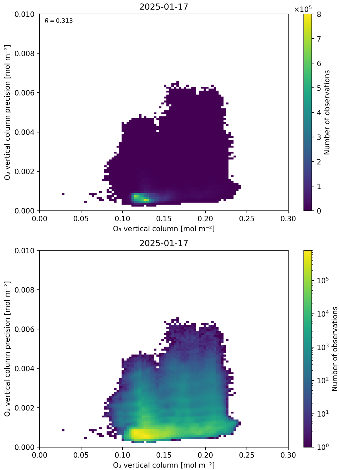
Figure 41: Scatter density plot of “O 3 vertical column” against “O 3 vertical column precision” for 2025-01-17 to 2025-01-18.
