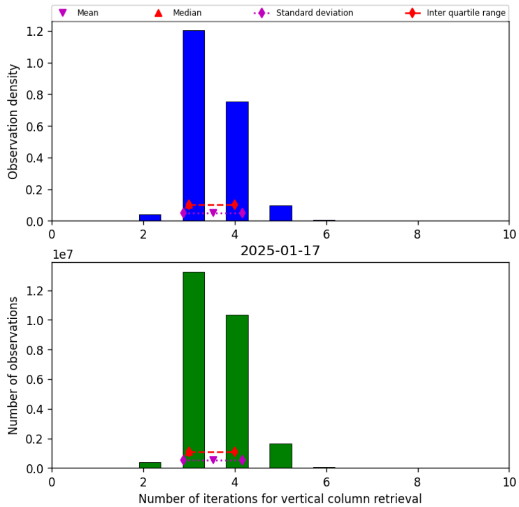
Figure 26: Histogram of “Number of iterations for vertical column retrieval” for 2025-01-17 to 2025-01-18
