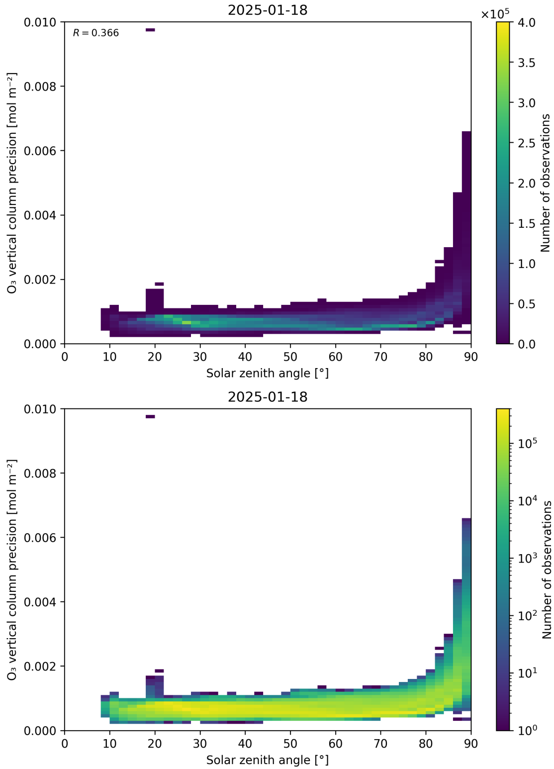
Figure 48: Scatter density plot of “Solar zenith angle” against “O 3 vertical column precision” for 2025-01-17 to 2025-01-19.
