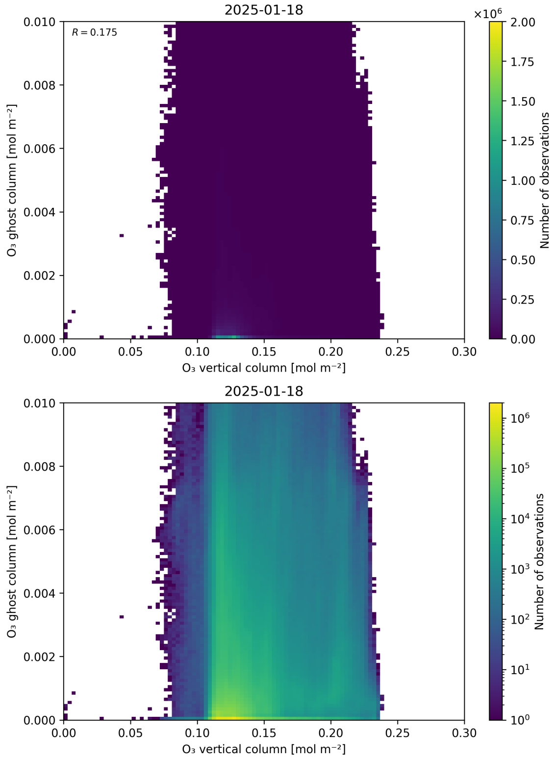
Figure 40: Scatter density plot of “O 3 vertical column” against “O 3 ghost column” for 2025-01-17 to 2025-01-19.
