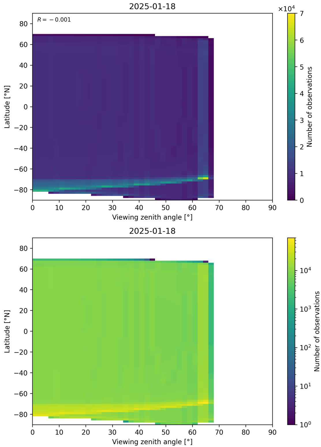
Figure 49: Scatter density plot of “Viewing zenith angle” against “Latitude” for 2025-01-17 to 2025-01-19.
