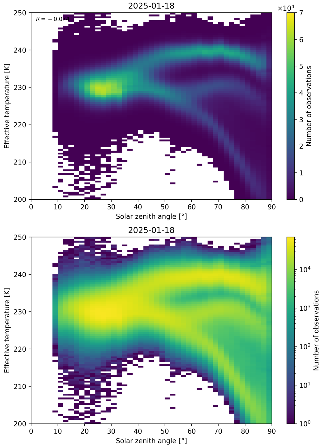
Figure 45: Scatter density plot of “Solar zenith angle” against “Effective temperature” for 2025-01-17 to 2025-01-19.
