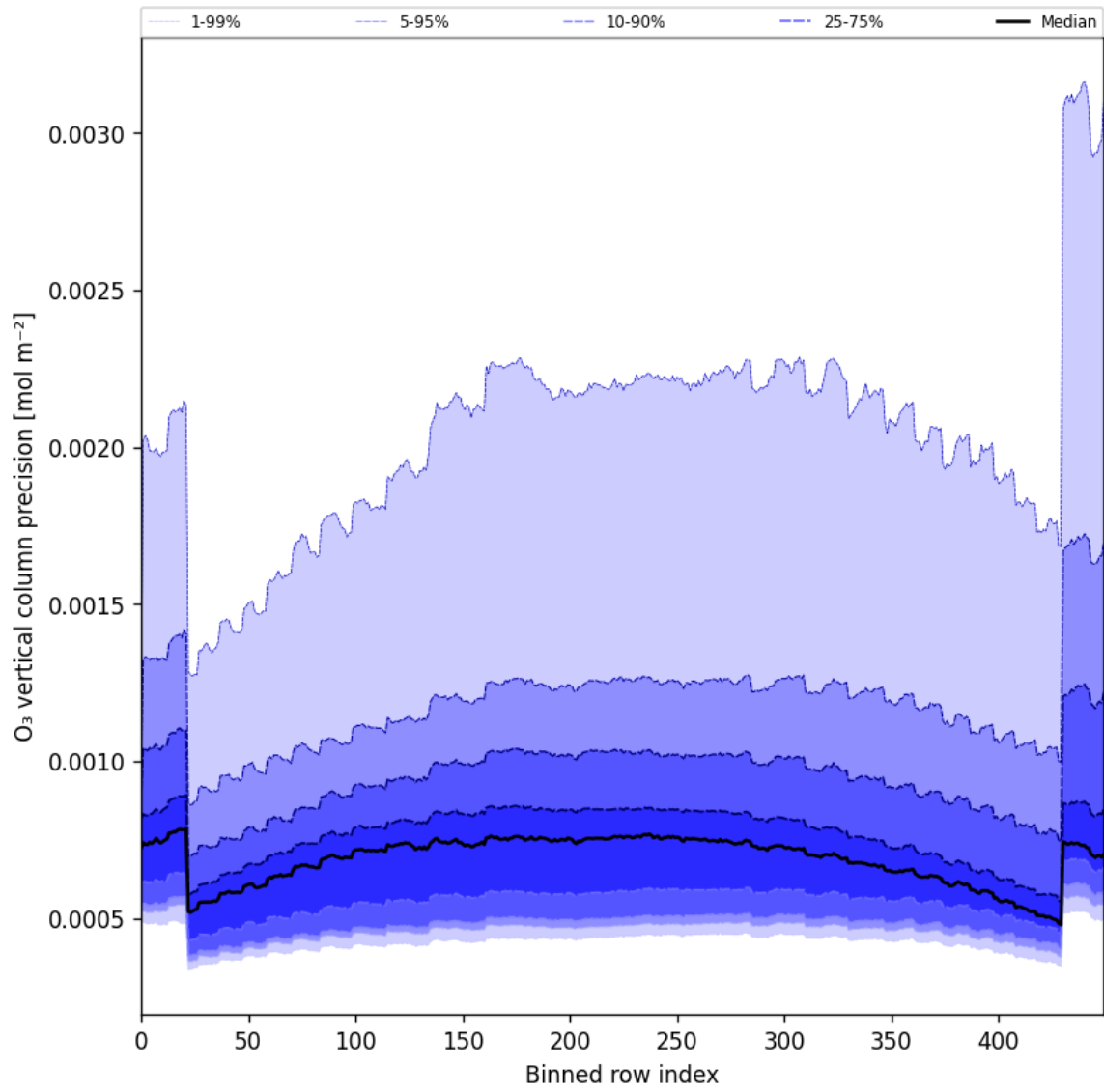
Figure 29: Along track statistics of “O 3 vertical column precision” for 2025-01-17 to 2025-01-19
