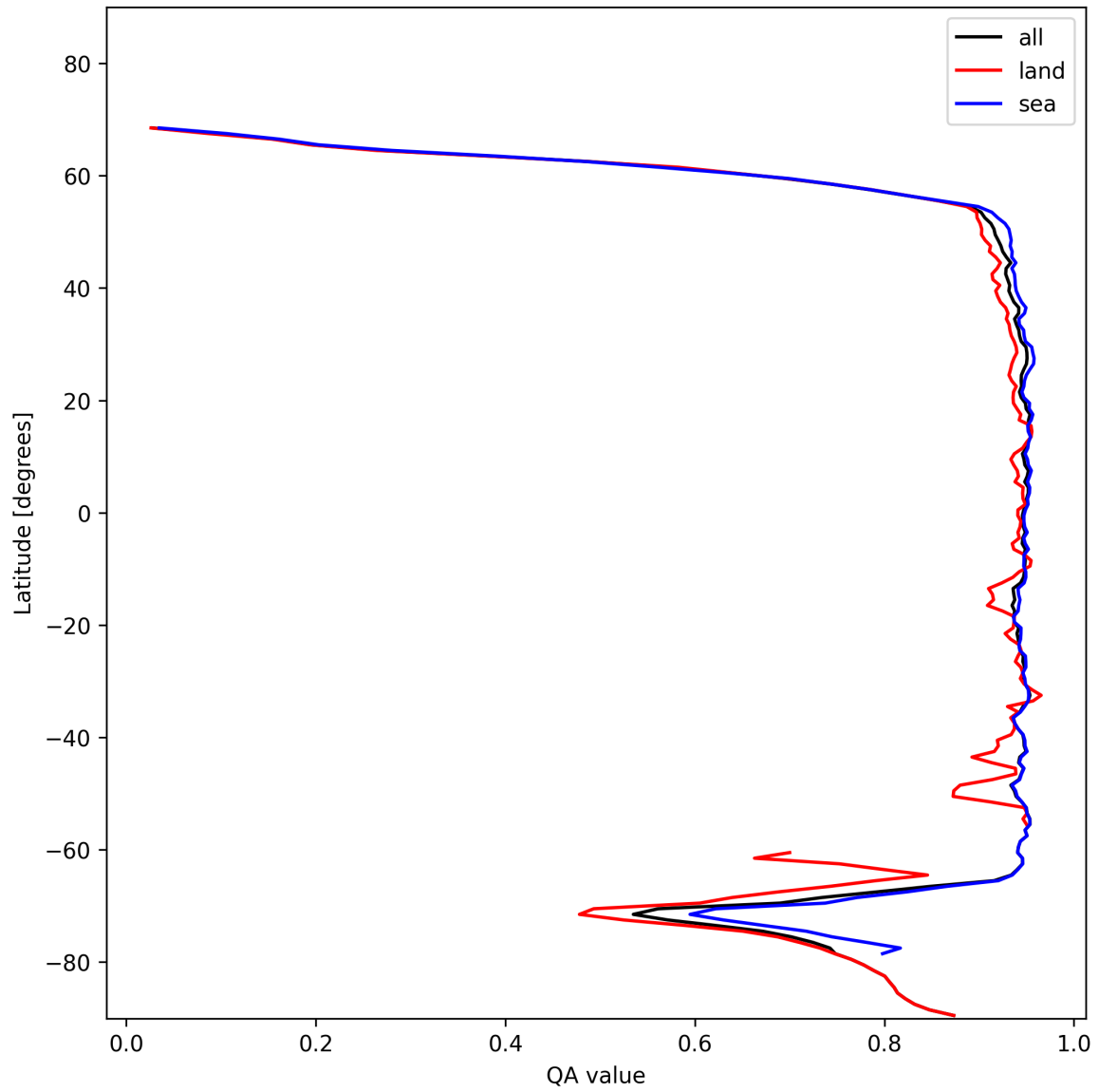
Figure 13: Zonal average of “QA value” for 2025-01-17 to 2025-01-19.
