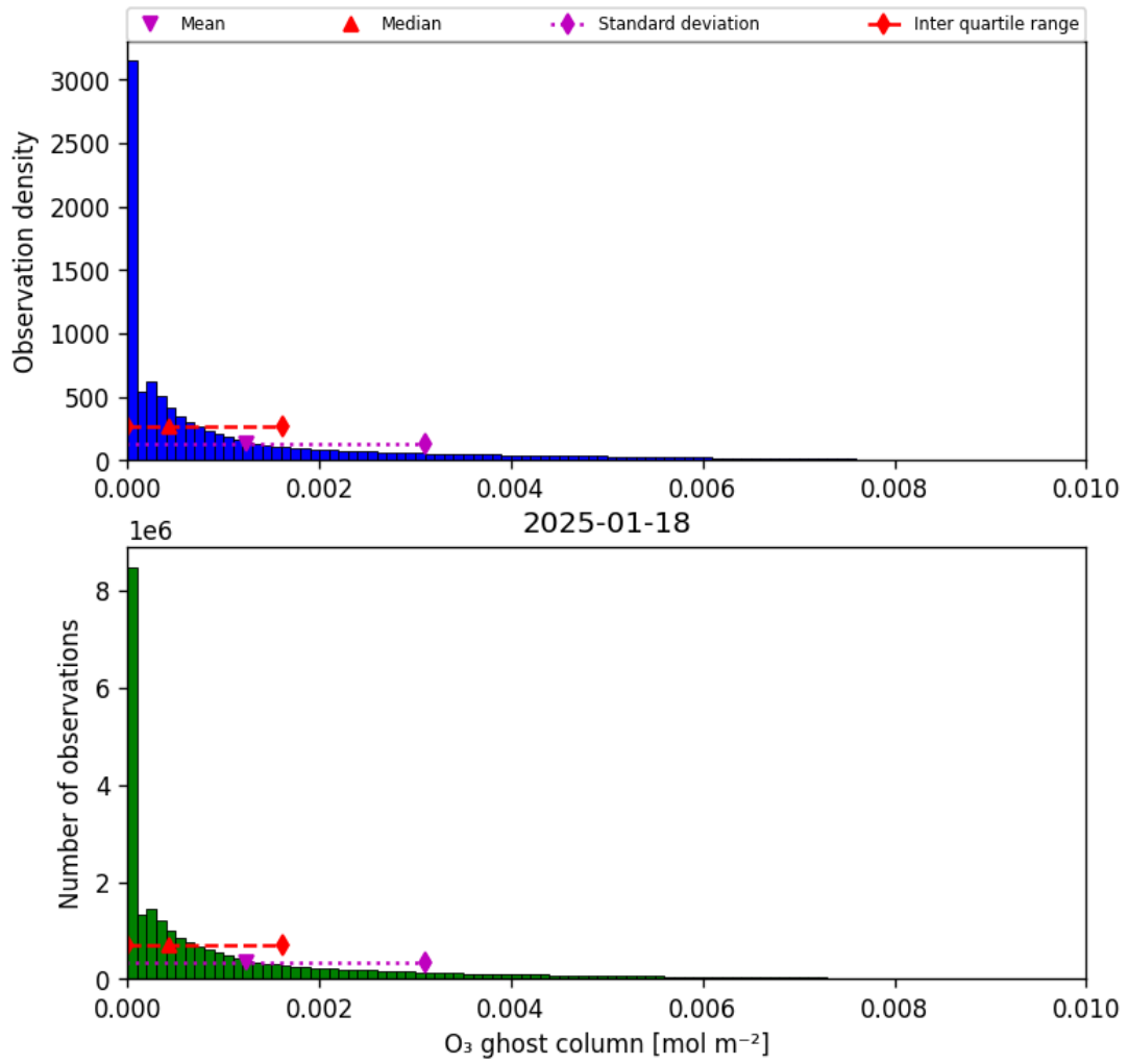
Figure 25: Histogram of "O 3 ghost column" for 2025-01-17 to 2025-01-19
