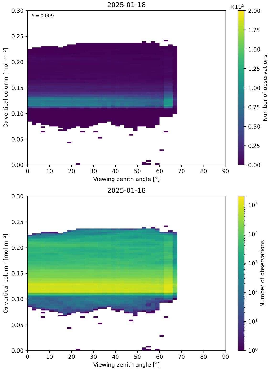
Figure 52: Scatter density plot of “Viewing zenith angle” against “O 3 vertical column” for 2025-01-17 to 2025-01-19.
