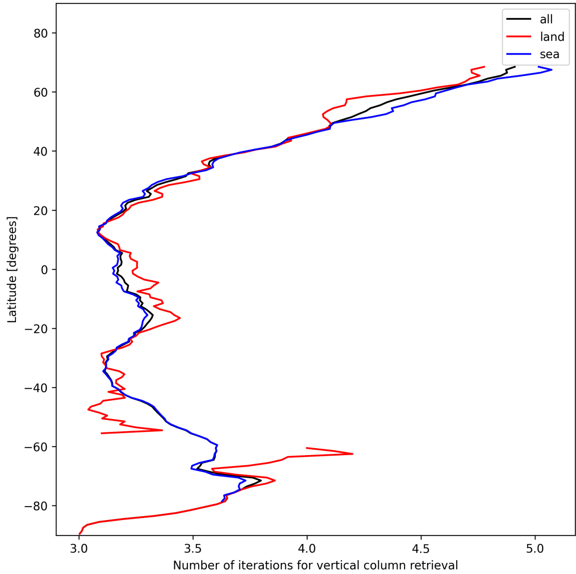
Figure 19: Zonal average of “Number of iterations for vertical column retrieval” for 2025-01-17 to 2025-01-19.
