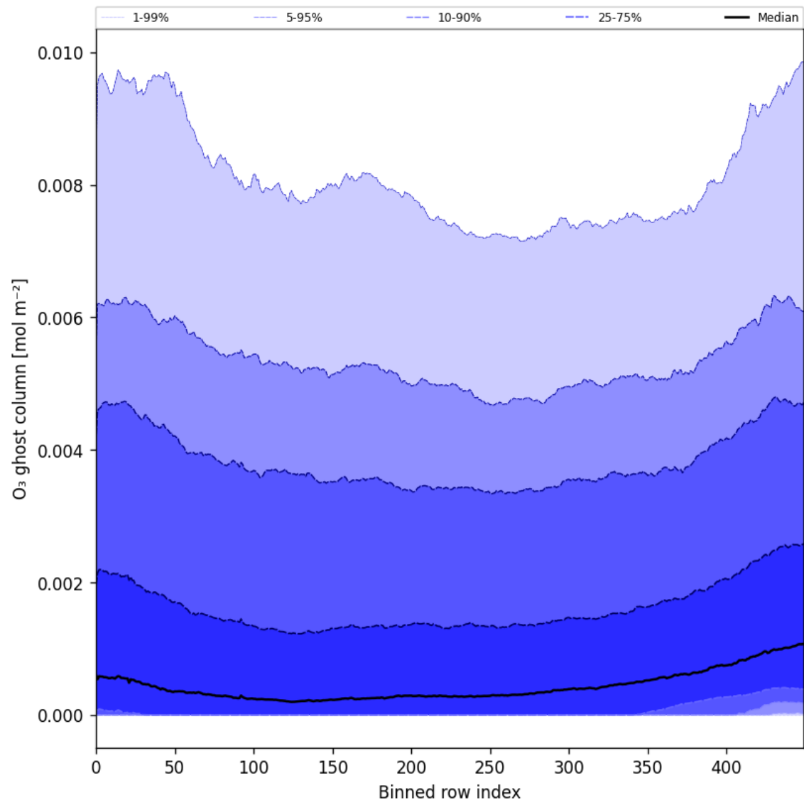
Figure 32: Along track statistics of “O 3 ghost column” for 2025-01-17 to 2025-01-19
