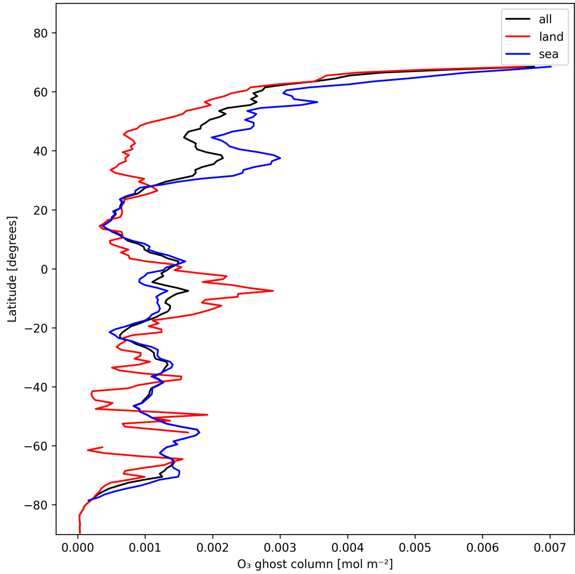
Figure 18: Zonal average of “O 3 ghost column” for 2025-01-17 to 2025-01-19.
