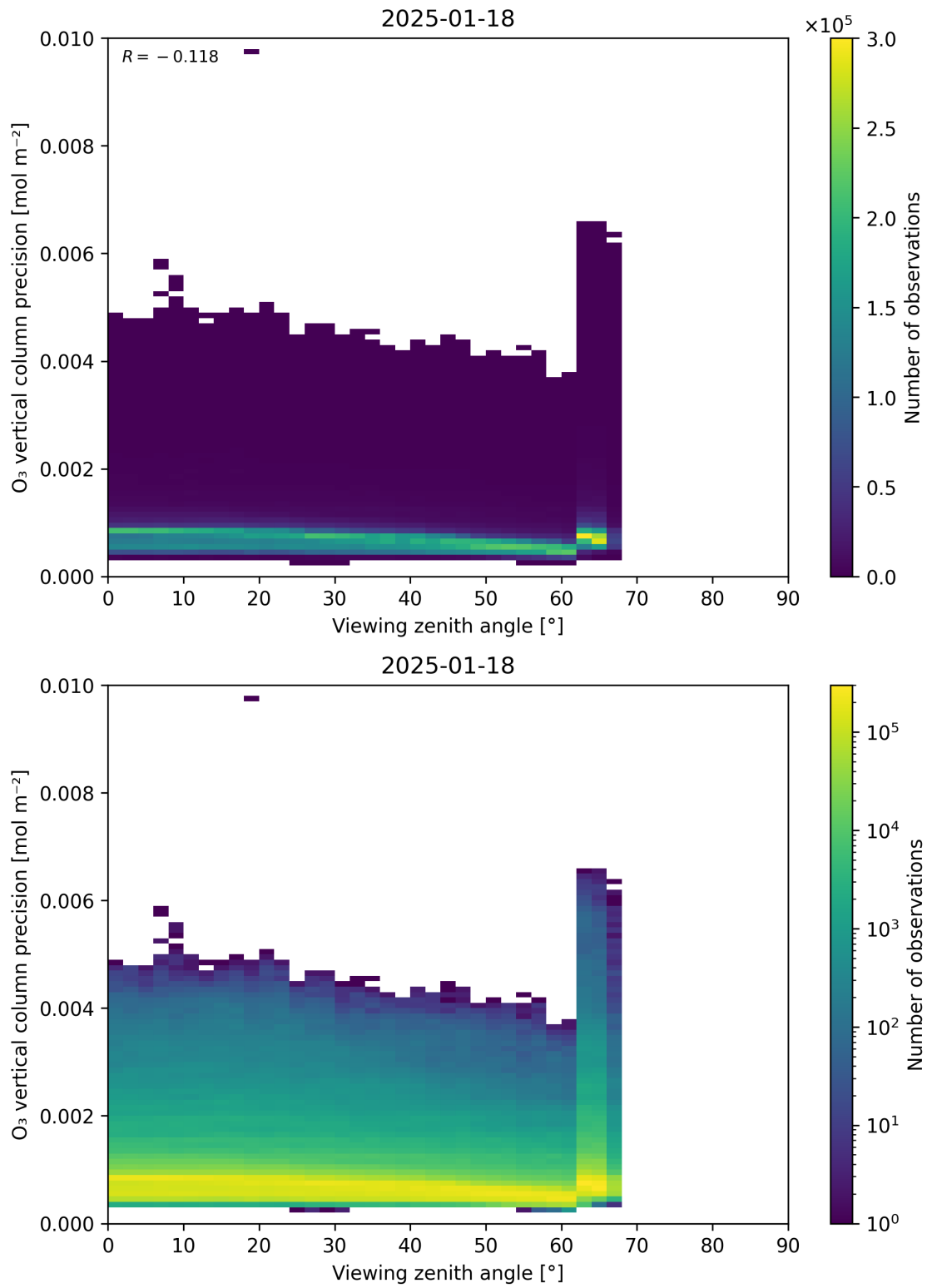
Figure 53: Scatter density plot of “Viewing zenith angle” against “O 3 vertical column precision” for 2025-01-17 to 2025-01-19.
