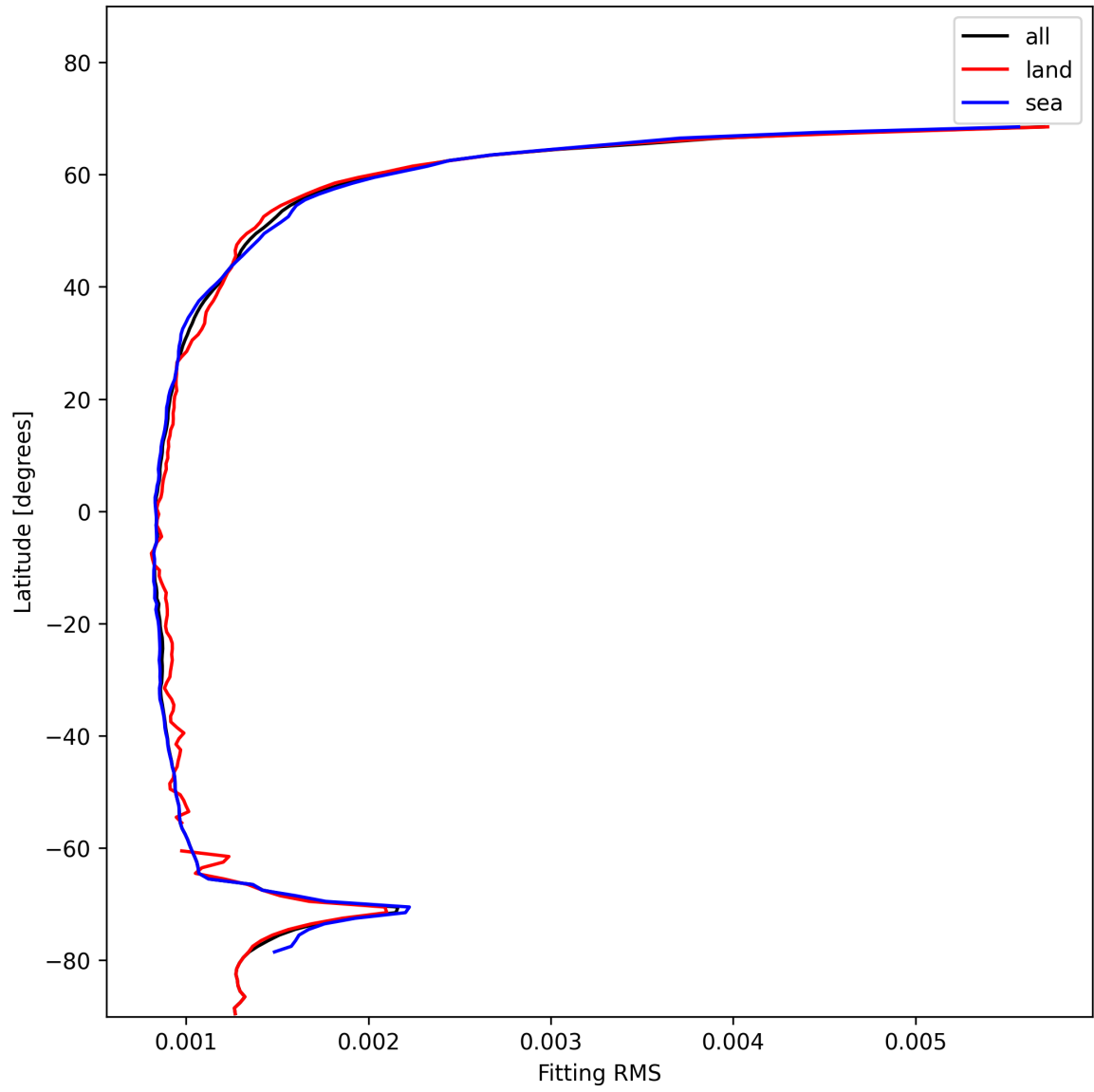
Figure 16: Zonal average of “Fitting RMS” for 2025-01-17 to 2025-01-19.
