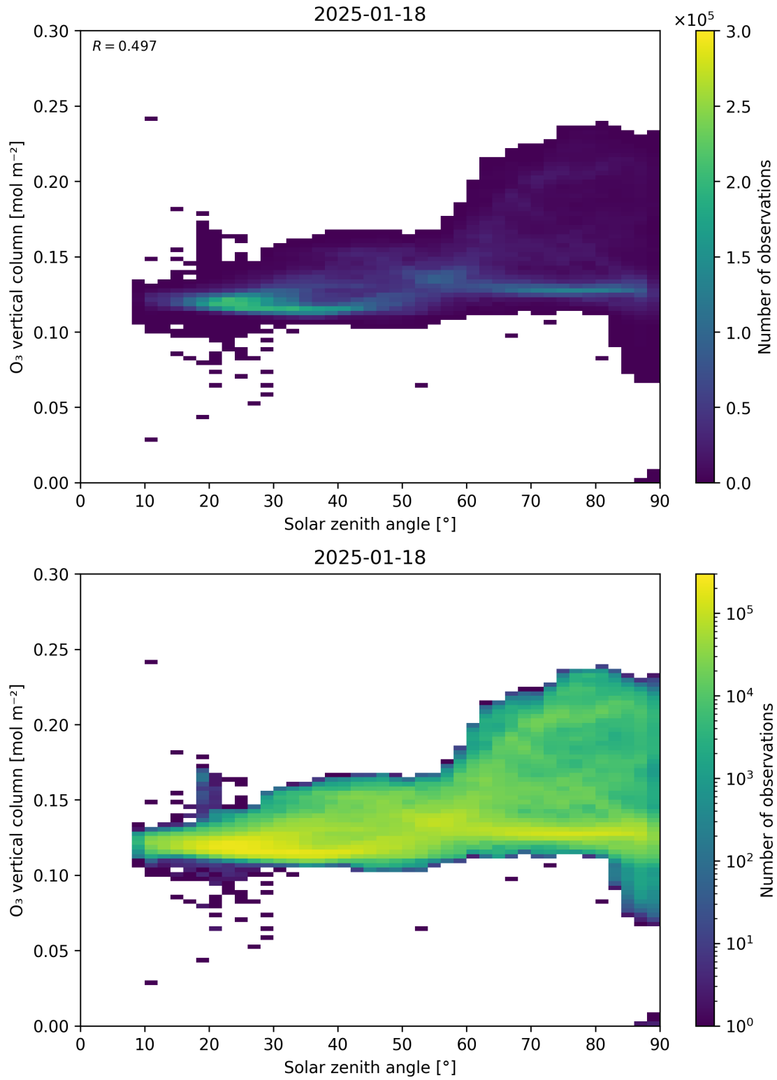
Figure 47: Scatter density plot of “Solar zenith angle” against “O 3 vertical column” for 2025-01-17 to 2025-01-19.
