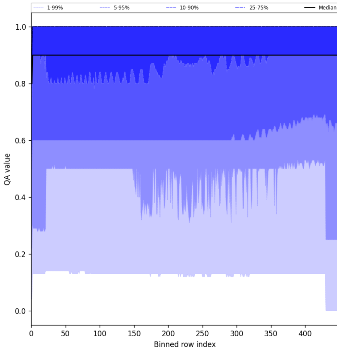
Figure 27: Along track statistics of “QA value” for 2025-01-17 to 2025-01-19
