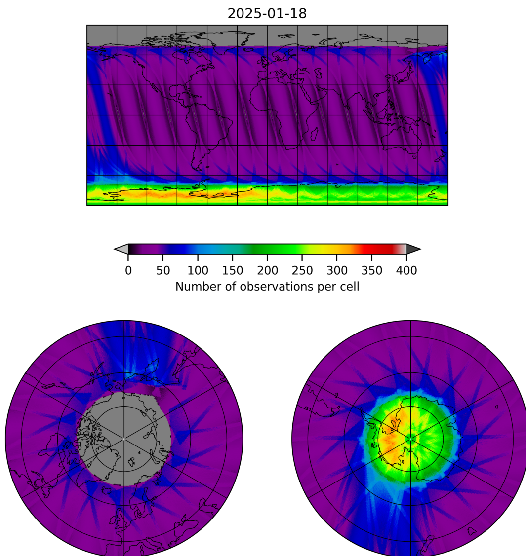
Figure 12: Map of the number of observations for 2025-01-17 to 2025-01-19
