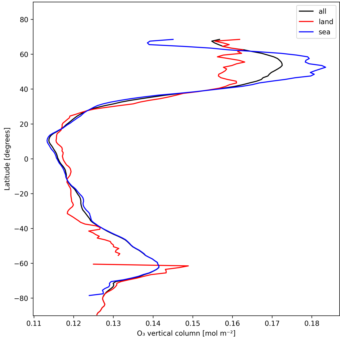
Figure 14: Zonal average of “O 3 vertical column” for 2025-01-17 to 2025-01-19.
