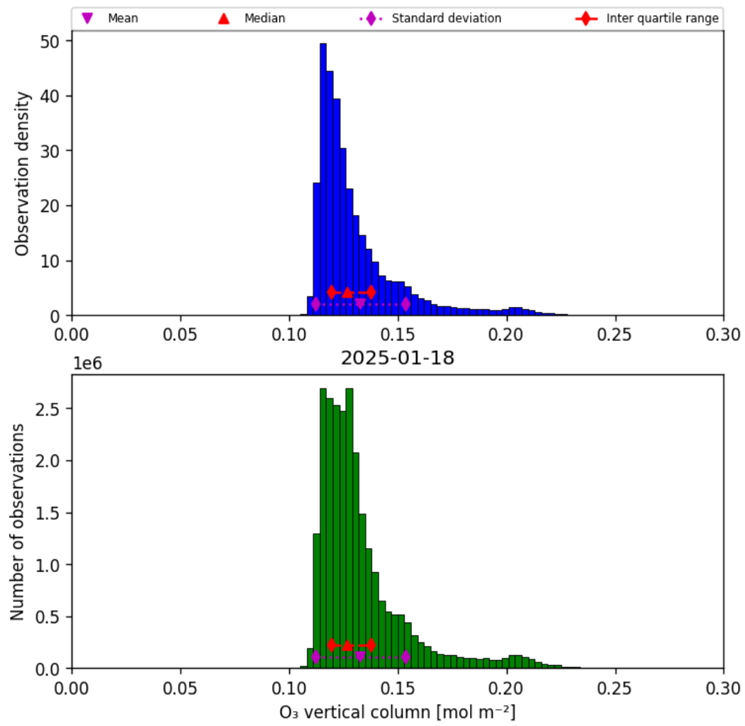
Figure 21: Histogram of “O 3 vertical column” for 2025-01-17 to 2025-01-19
