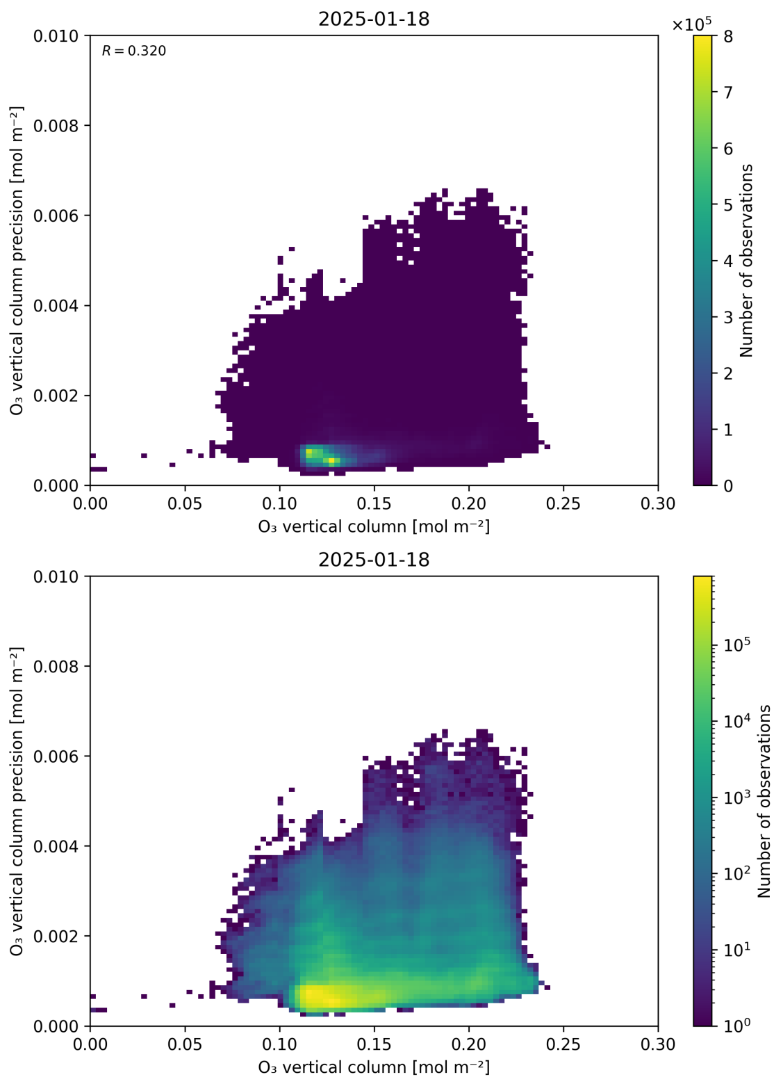
Figure 41: Scatter density plot of “O 3 vertical column” against “O 3 vertical column precision” for 2025-01-17 to 2025-01-19.
