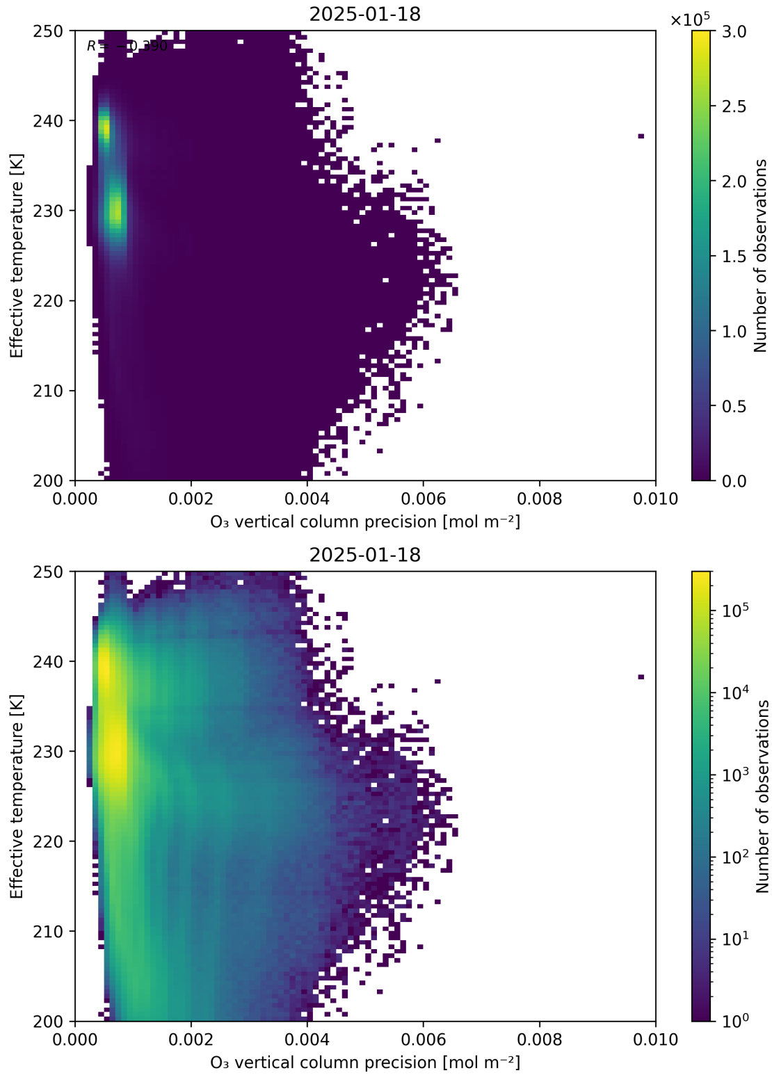
Figure 42: Scatter density plot of “O 3 vertical column precision” against “Effective temperature” for 2025-01-17 to 2025-01-19.
