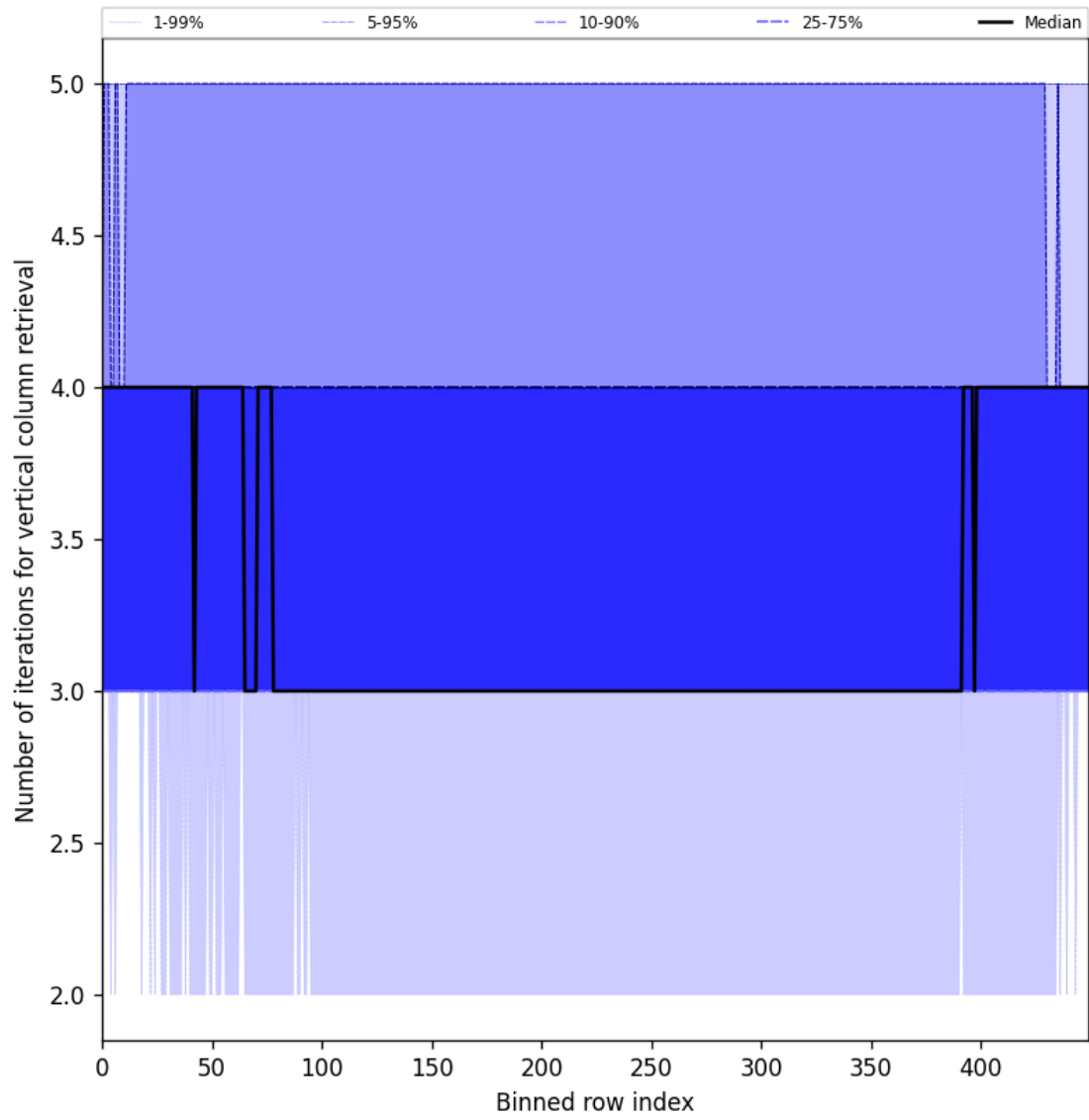
Figure 33: Along track statistics of “Number of iterations for vertical column retrieval” for 2025-01-17 to 2025-01-19
