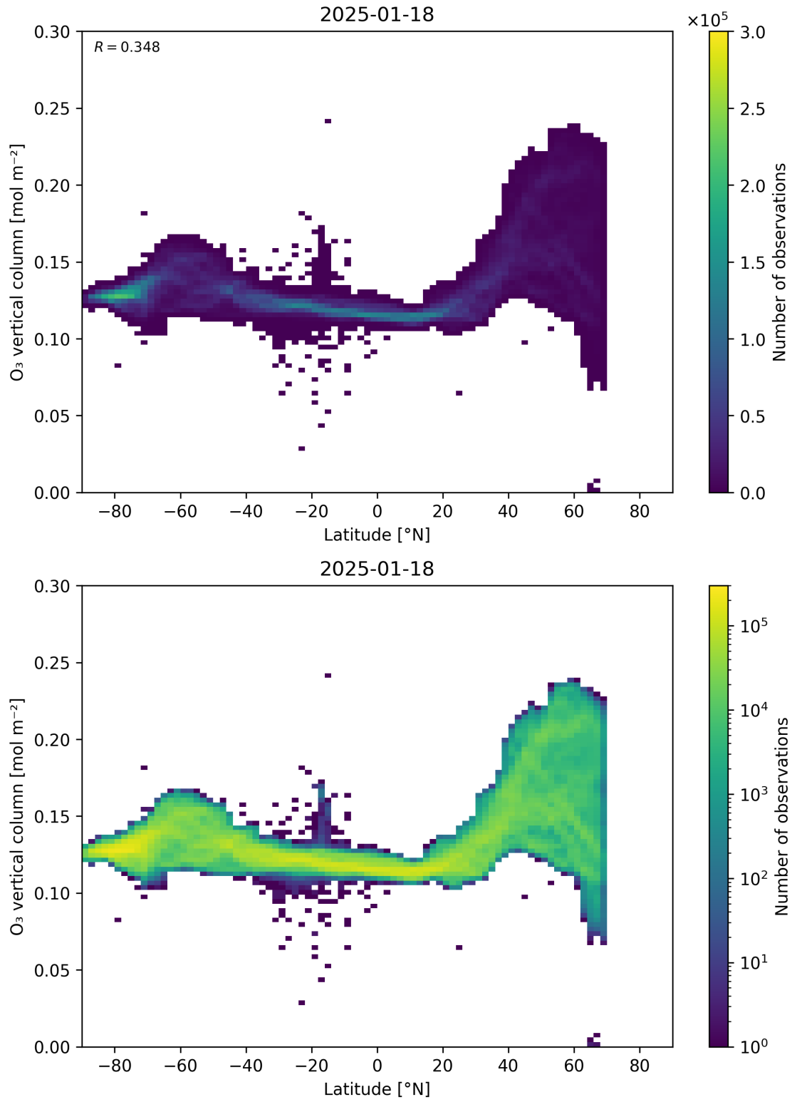
Figure 36: Scatter density plot of “Latitude” against “O 3 vertical column” for 2025-01-17 to 2025-01-19.
