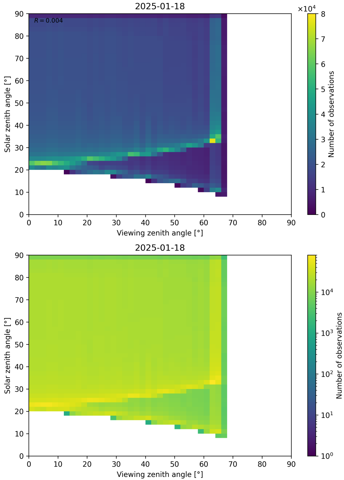
Figure 54: Scatter density plot of “Viewing zenith angle” against “Solar zenith angle” for 2025-01-17 to 2025-01-19.
