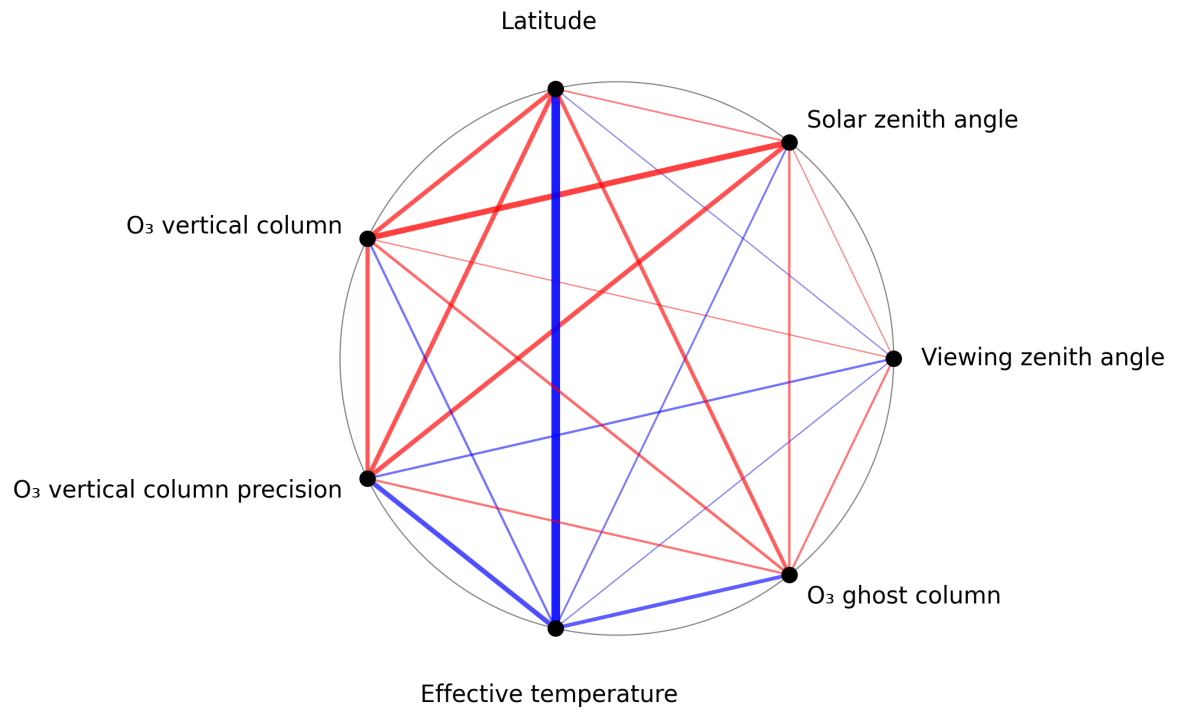
Figure 1: Map of correlation graph for 2025-01-17 to 2025-01-19.
