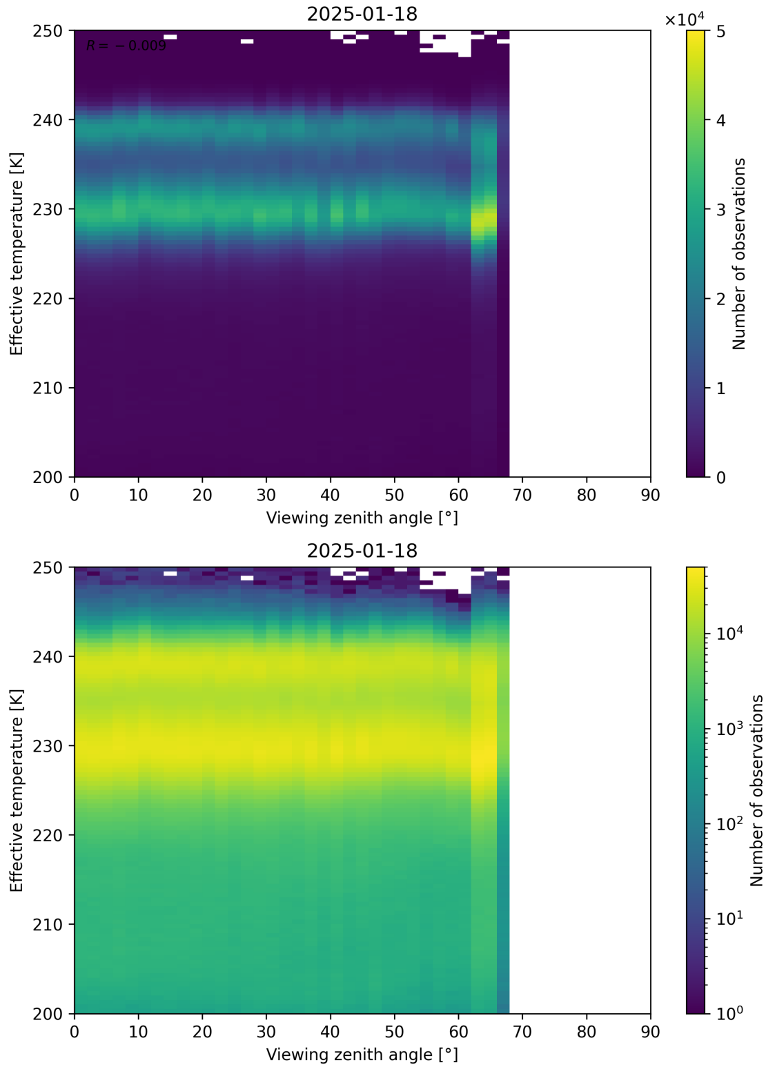
Figure 50: Scatter density plot of “Viewing zenith angle” against “Effective temperature” for 2025-01-17 to 2025-01-19.
