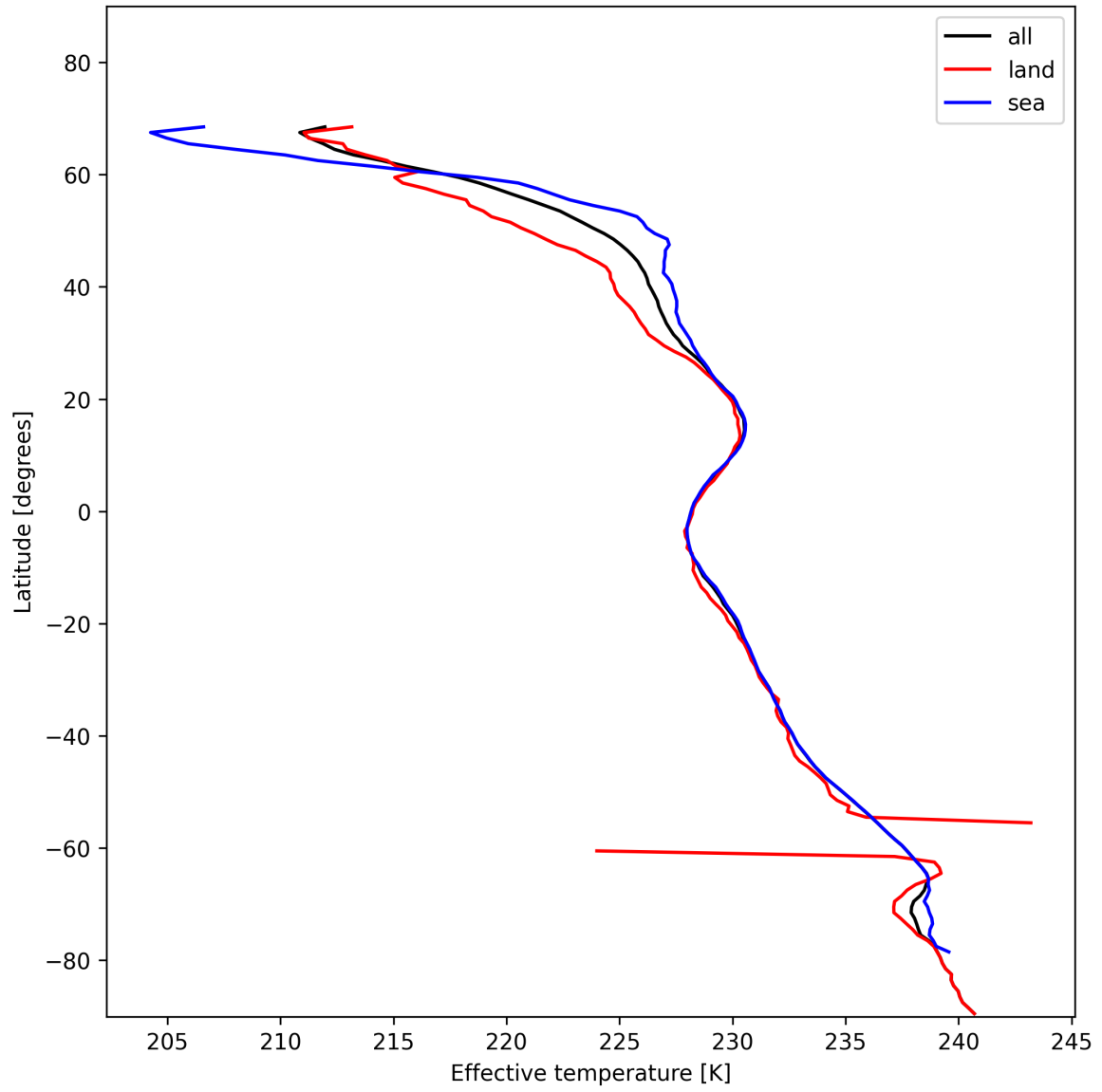
Figure 17: Zonal average of “Effective temperature” for 2025-01-17 to 2025-01-19.
