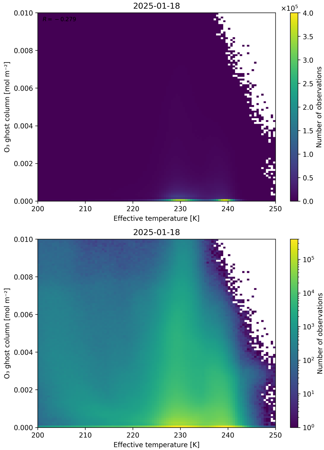
Figure 38: Scatter density plot of “Effective temperature” against “O 3 ghost column” for 2025-01-17 to 2025-01-19.
