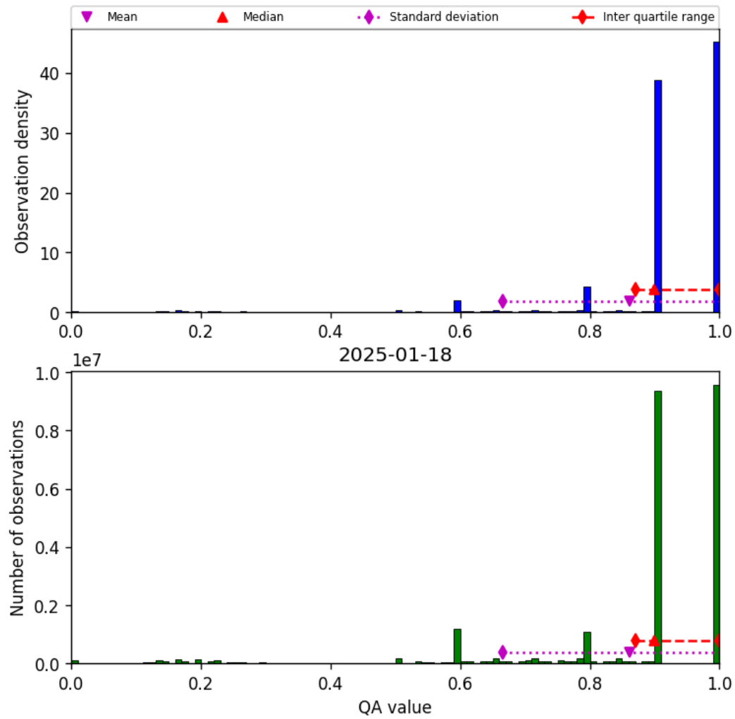
Figure 20: Histogram of “QA value” for 2025-01-17 to 2025-01-19
