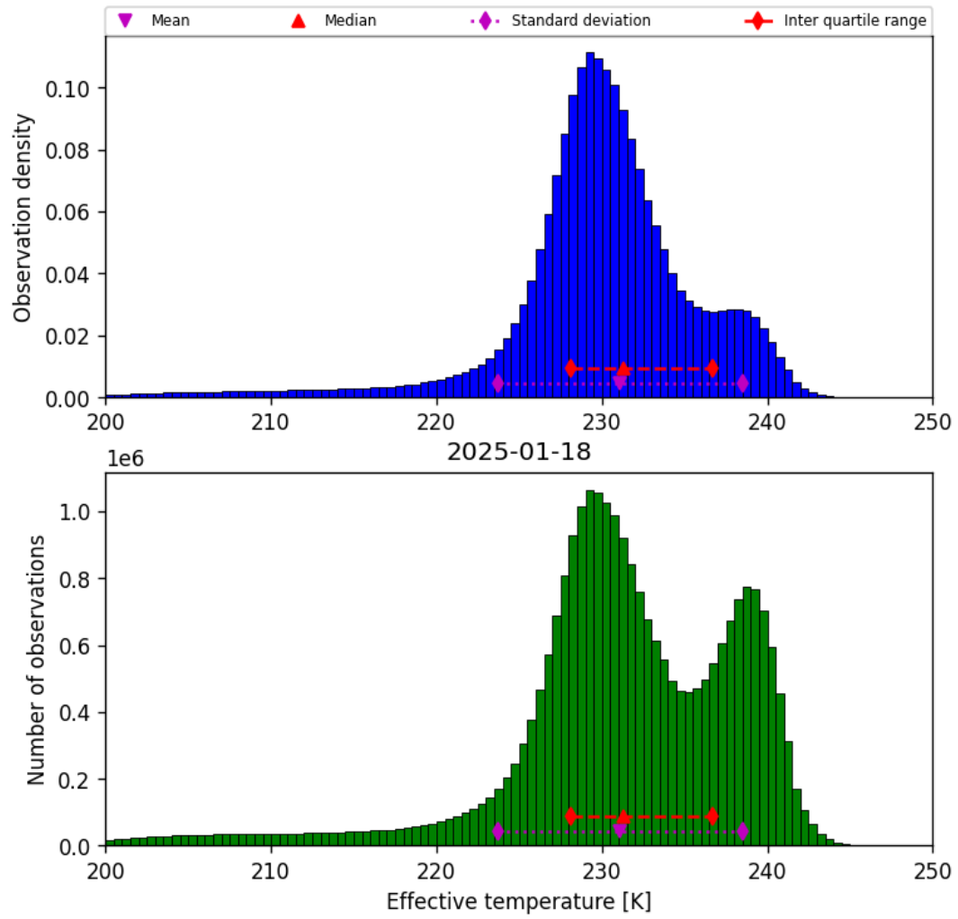
Figure 24: Histogram of “Effective temperature” for 2025-01-17 to 2025-01-19
