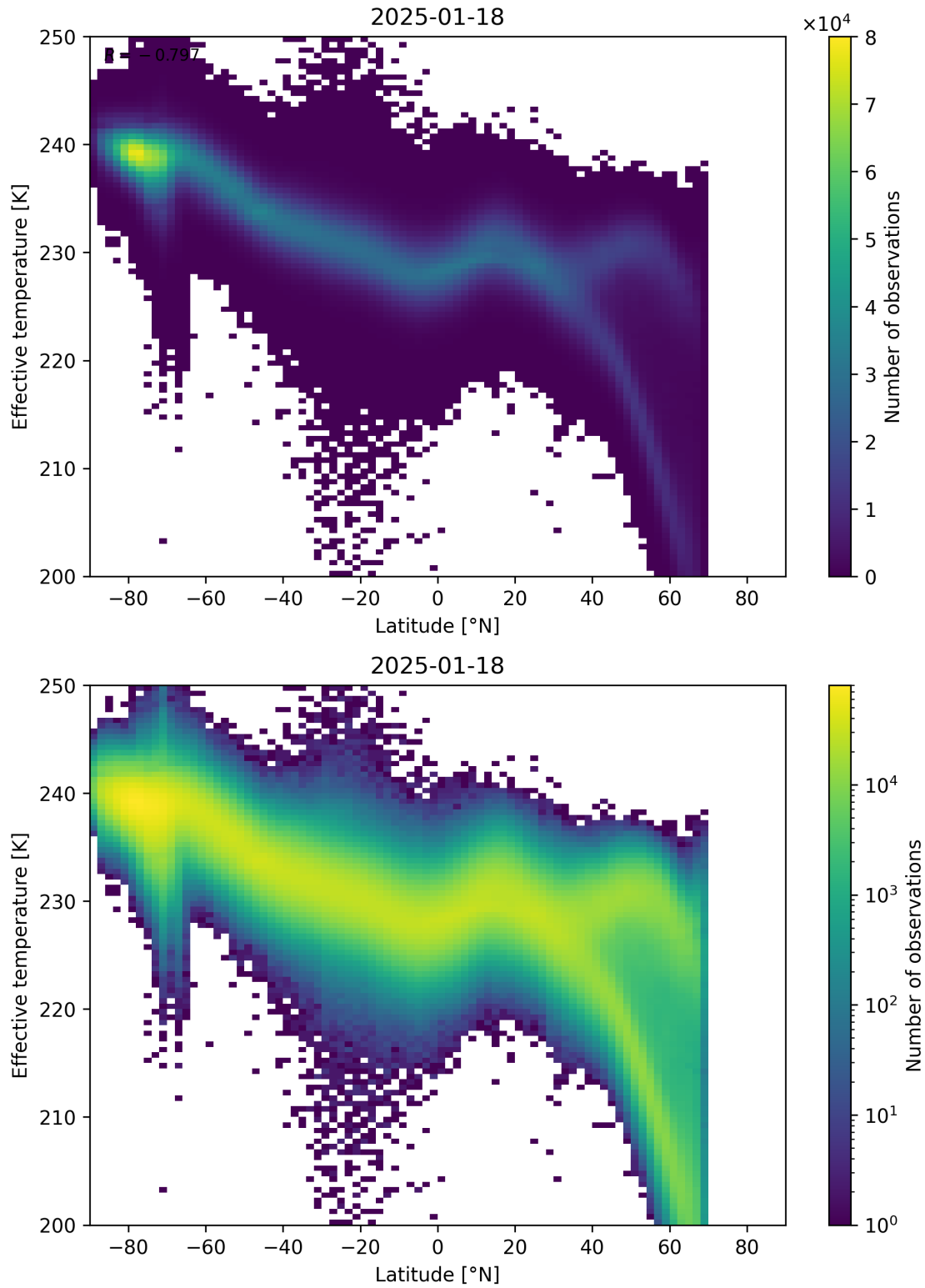
Figure 34: Scatter density plot of “Latitude” against “Effective temperature” for 2025-01-17 to 2025-01-19.
