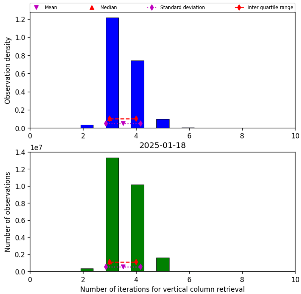
Figure 26: Histogram of “Number of iterations for vertical column retrieval” for 2025-01-17 to 2025-01-19
