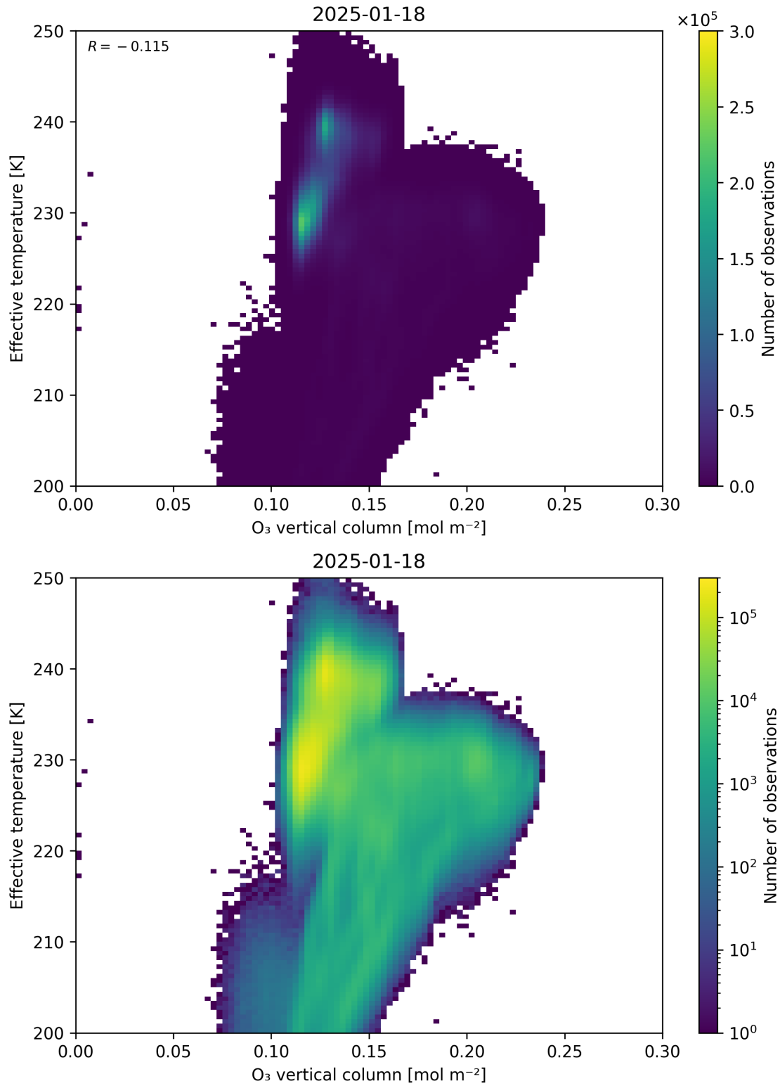
Figure 39: Scatter density plot of “O 3 vertical column” against “Effective temperature” for 2025-01-17 to 2025-01-19.
