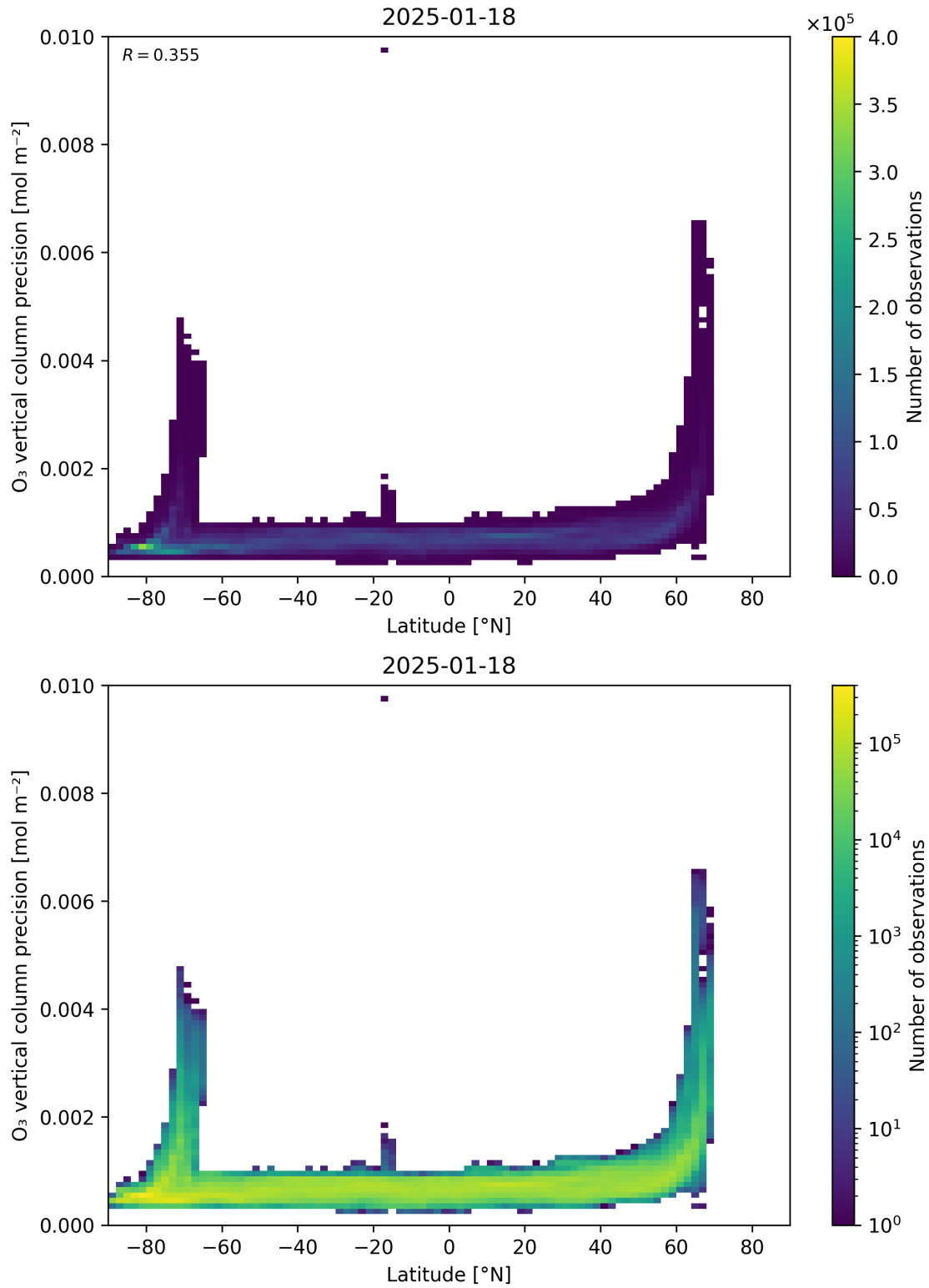
Figure 37: Scatter density plot of “Latitude” against “O 3 vertical column precision” for 2025-01-17 to 2025-01-19.
