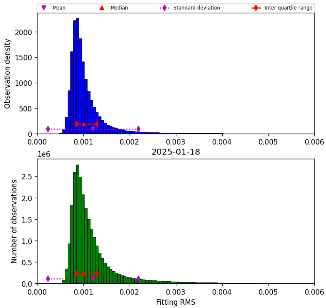
Figure 23: Histogram of “Fitting RMS” for 2025-01-17 to 2025-01-19
