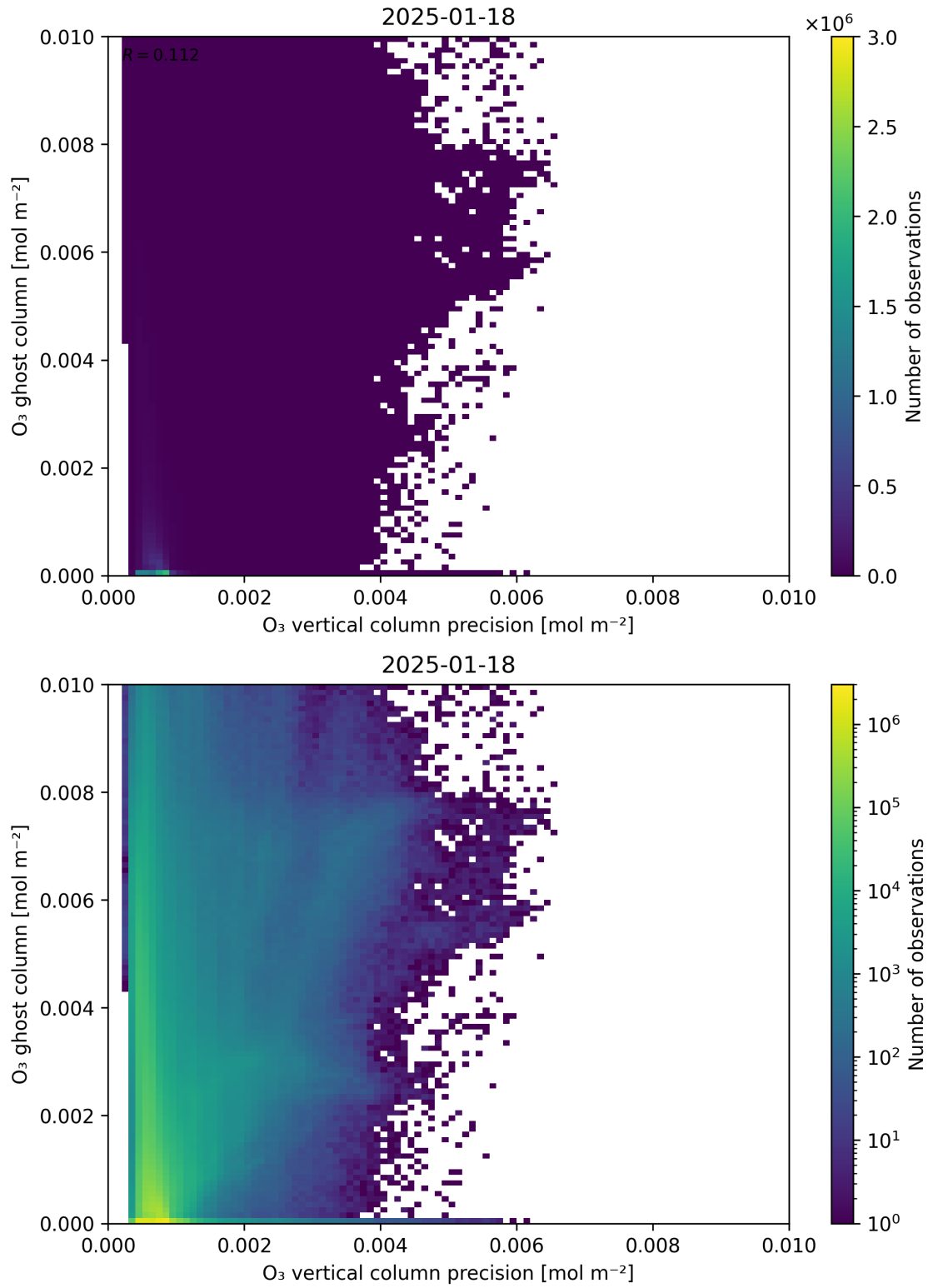
Figure 43: Scatter density plot of “ \text{O}_3 vertical column precision” against “ \text{O}_3 ghost column” for 2025-01-17 to 2025-01-19.
