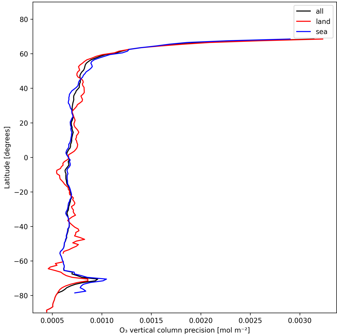
Figure 15: Zonal average of “O 3 vertical column precision” for 2025-01-17 to 2025-01-19.
