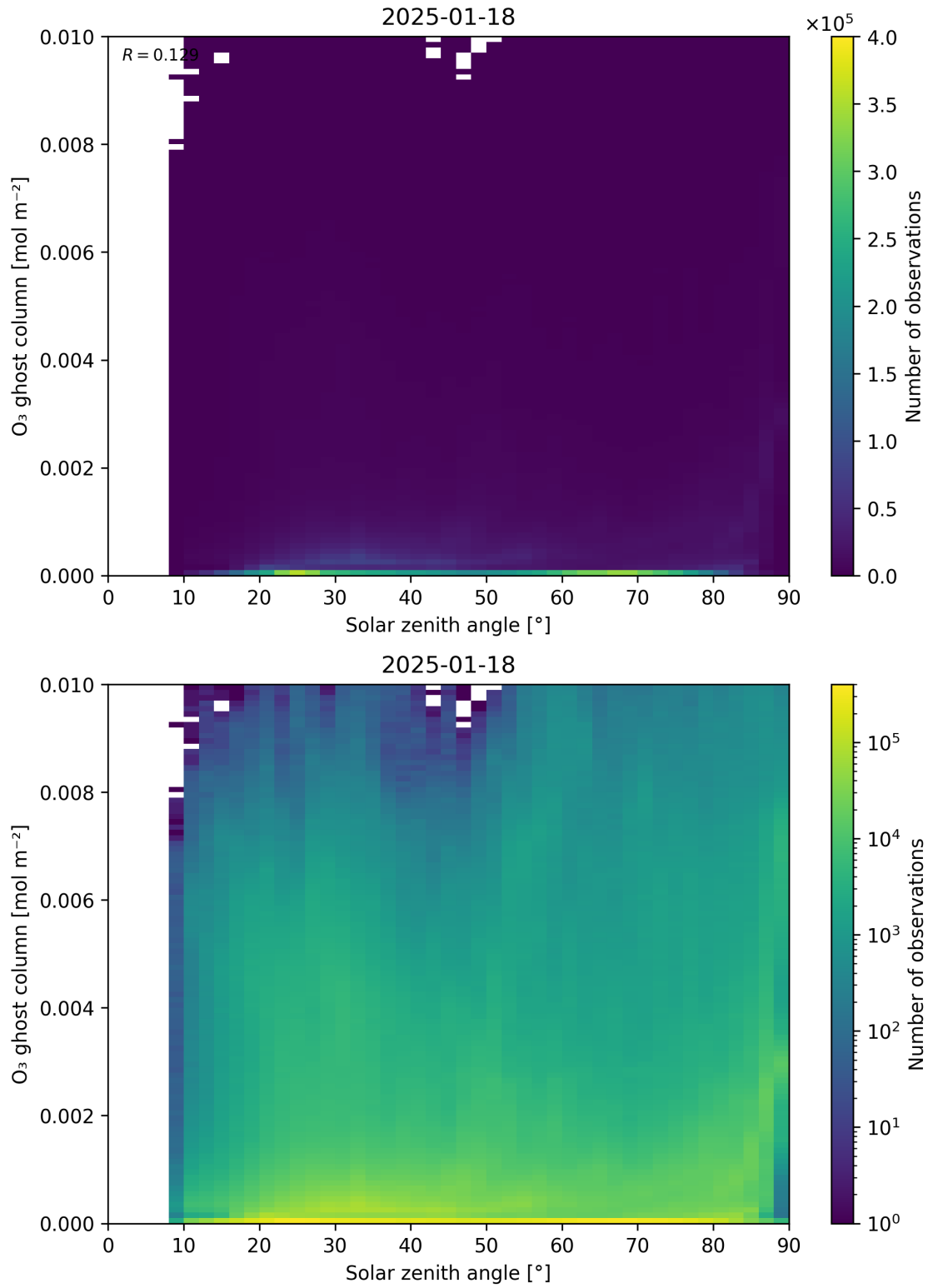
Figure 46: Scatter density plot of “Solar zenith angle” against “O 3 ghost column” for 2025-01-17 to 2025-01-19.
