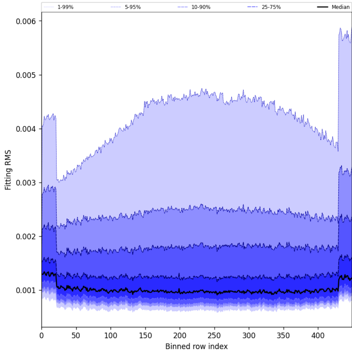
Figure 30: Along track statistics of “Fitting RMS” for 2025-01-17 to 2025-01-19
