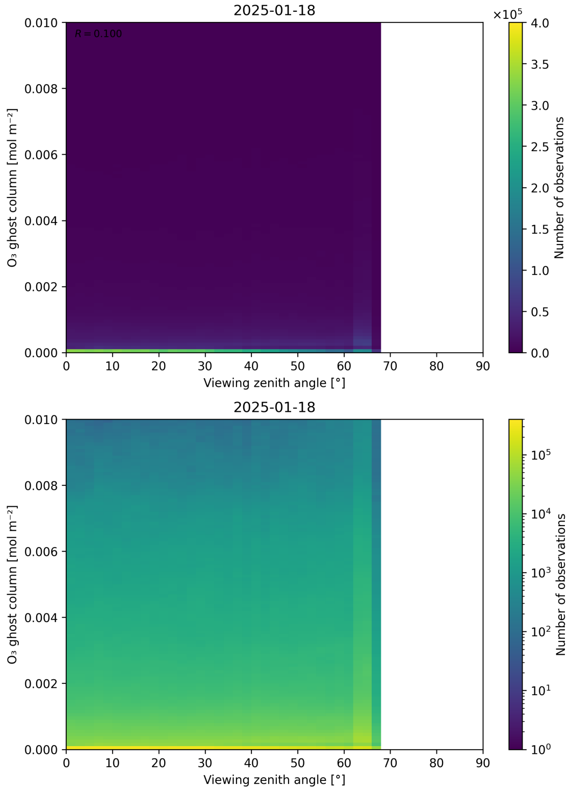
Figure 51: Scatter density plot of “Viewing zenith angle” against “O 3 ghost column” for 2025-01-17 to 2025-01-19.
