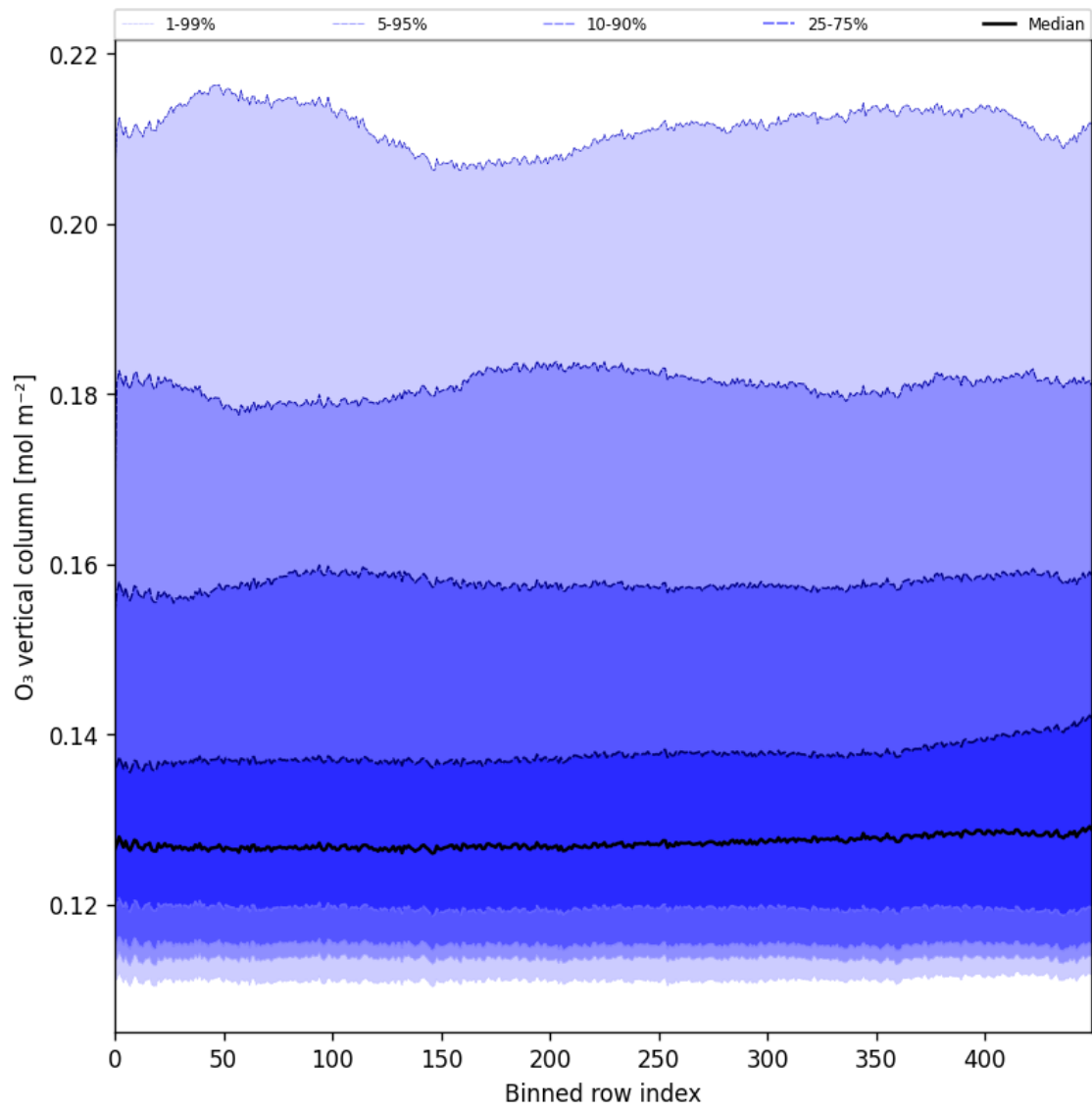
Figure 28: Along track statistics of “O 3 vertical column” for 2025-01-17 to 2025-01-19
