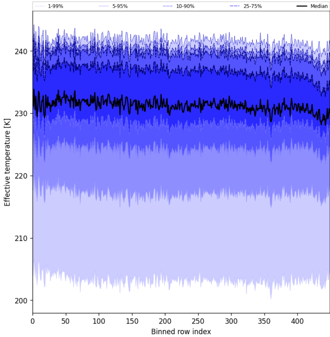
Figure 31: Along track statistics of “Effective temperature” for 2025-01-17 to 2025-01-19
