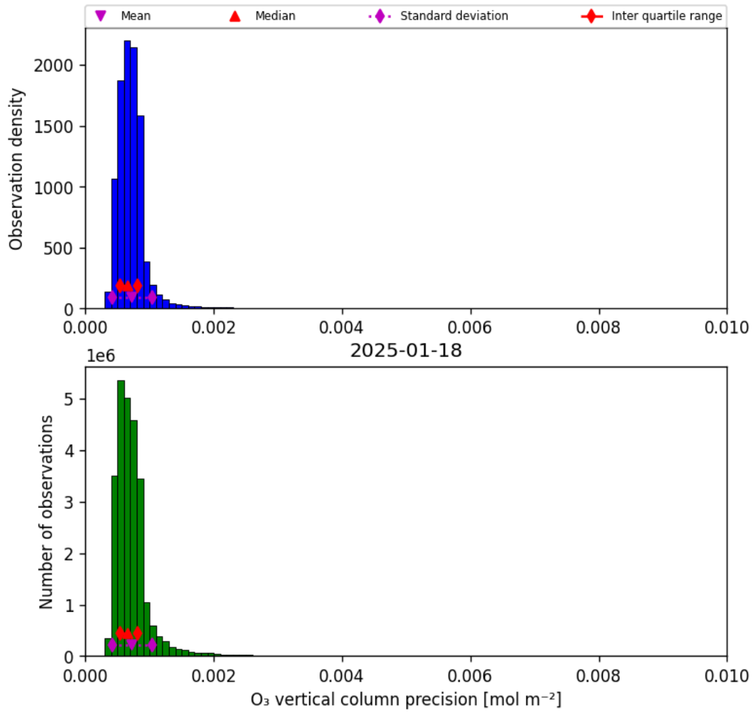
Figure 22: Histogram of “O 3 vertical column precision” for 2025-01-17 to 2025-01-19
