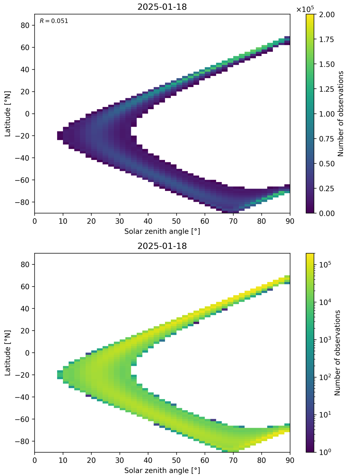
Figure 44: Scatter density plot of “Solar zenith angle” against “Latitude” for 2025-01-17 to 2025-01-19.
