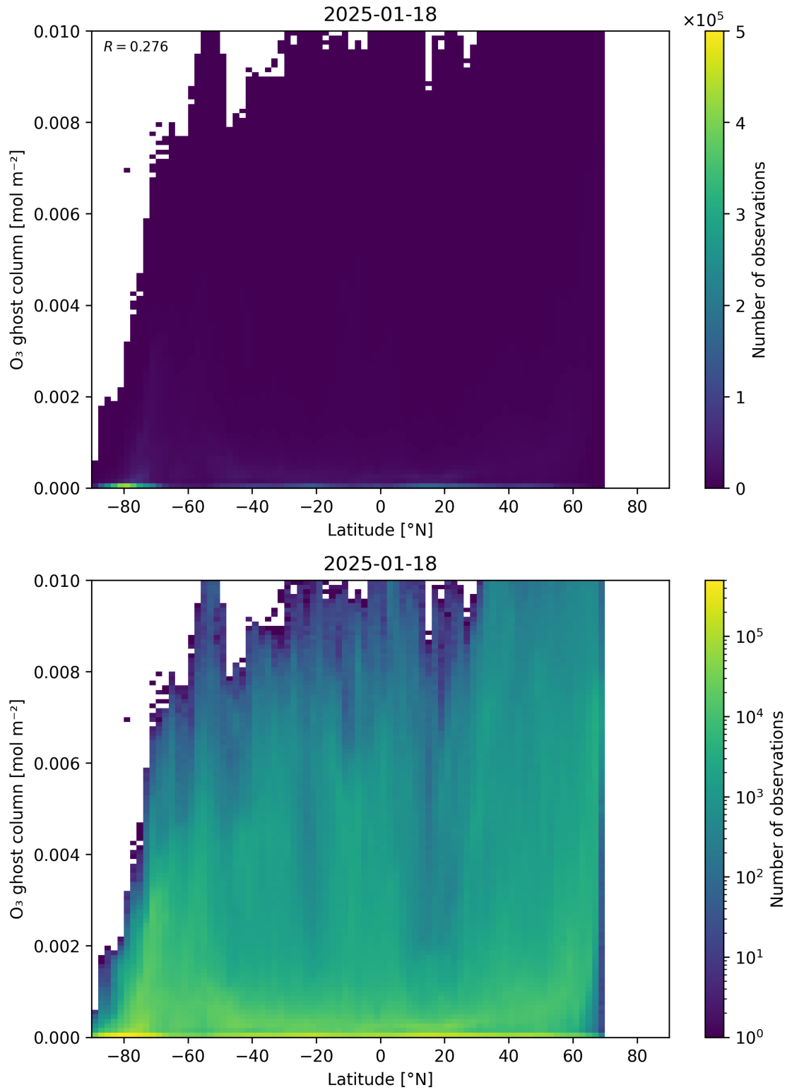
Figure 35: Scatter density plot of “Latitude” against “O 3 ghost column” for 2025-01-17 to 2025-01-19.
