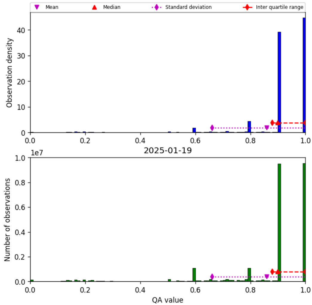
Figure 20: Histogram of “QA value” for 2025-01-18 to 2025-01-20
