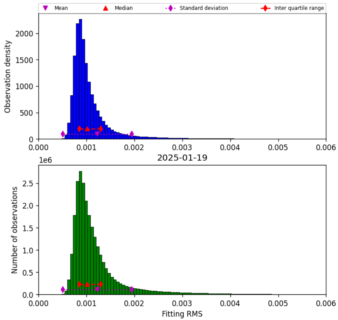
Figure 23: Histogram of “Fitting RMS” for 2025-01-18 to 2025-01-20
