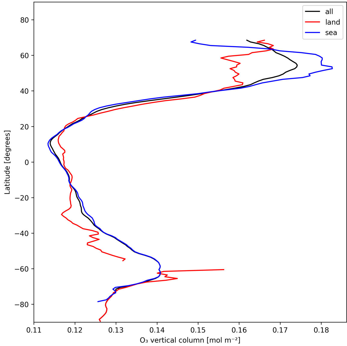
Figure 14: Zonal average of “O 3 vertical column” for 2025-01-18 to 2025-01-20.
