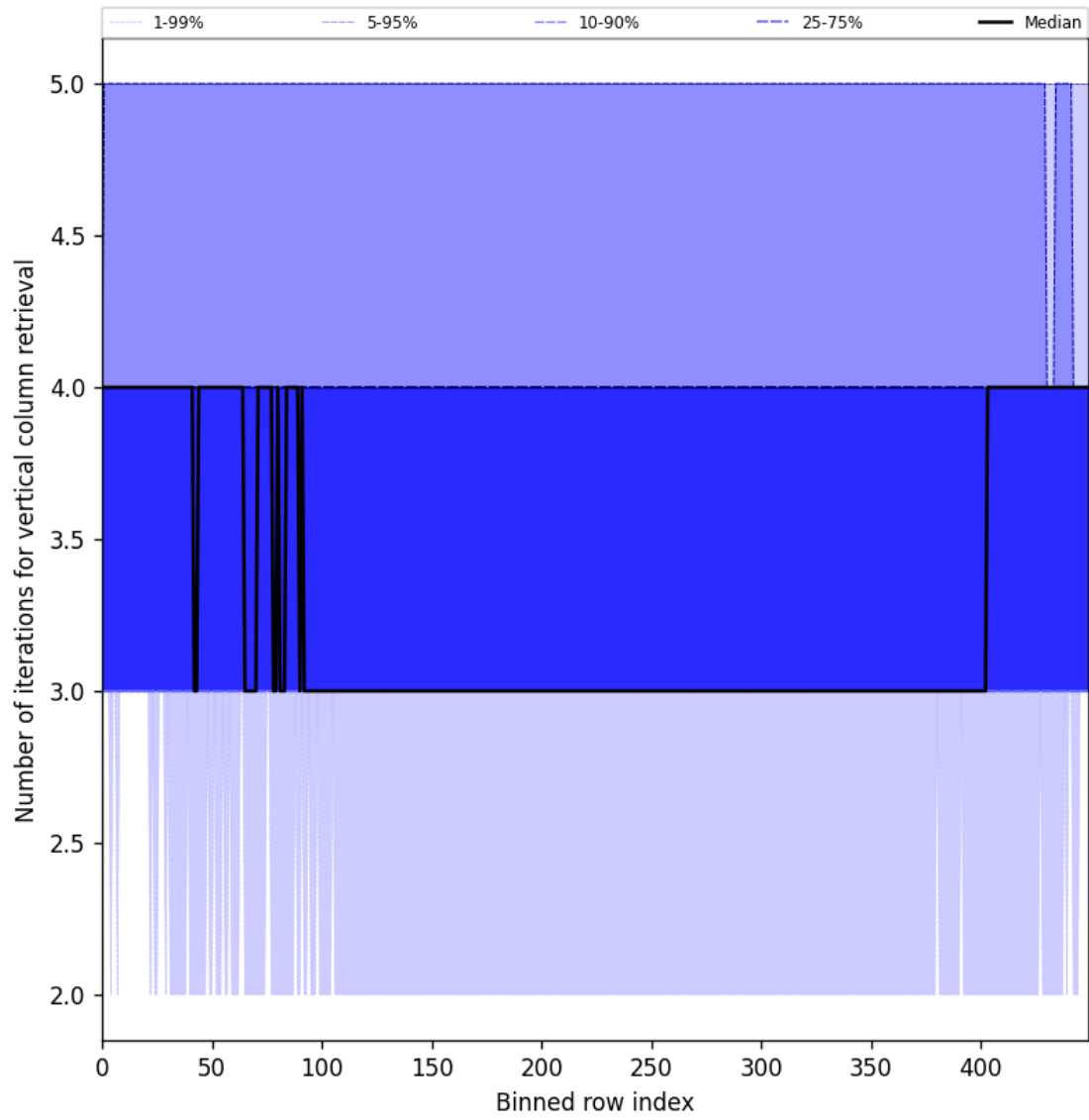
Figure 33: Along track statistics of “Number of iterations for vertical column retrieval” for 2025-01-18 to 2025-01-20
