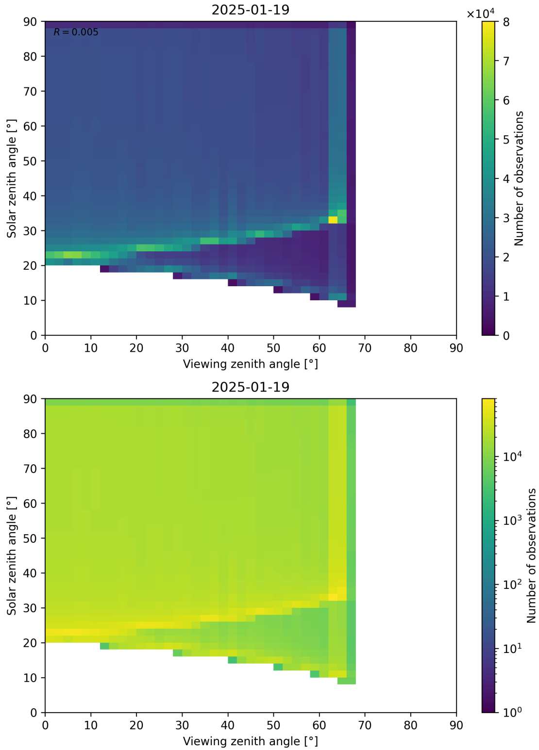
Figure 54: Scatter density plot of “Viewing zenith angle” against “Solar zenith angle” for 2025-01-18 to 2025-01-20.
