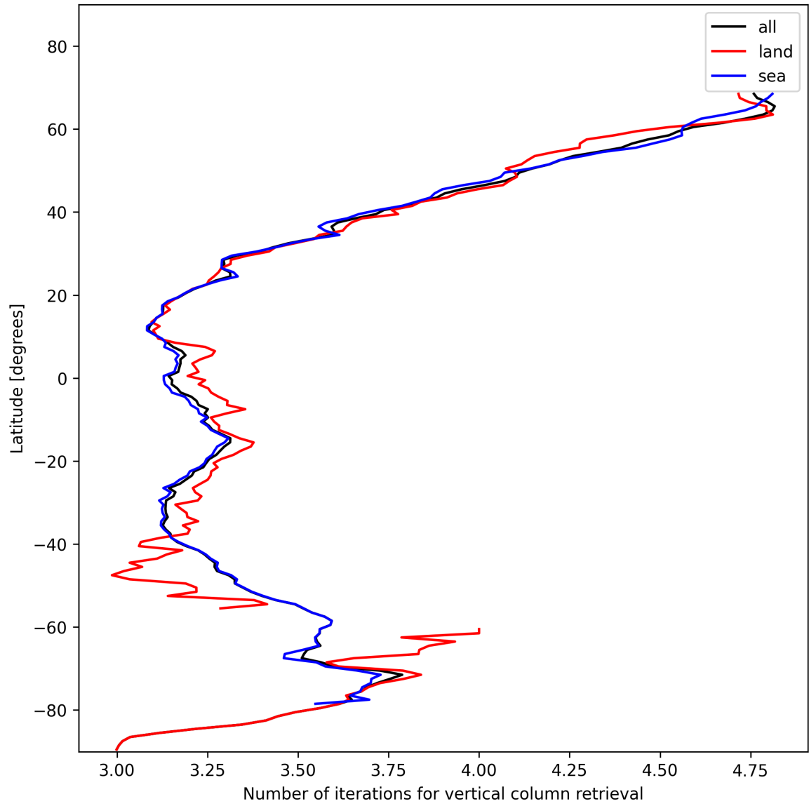
Figure 19: Zonal average of “Number of iterations for vertical column retrieval” for 2025-01-18 to 2025-01-20.
