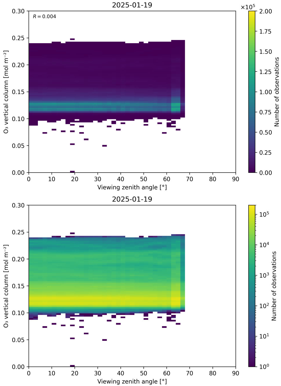
Figure 52: Scatter density plot of “Viewing zenith angle” against “O 3 vertical column” for 2025-01-18 to 2025-01-20.
