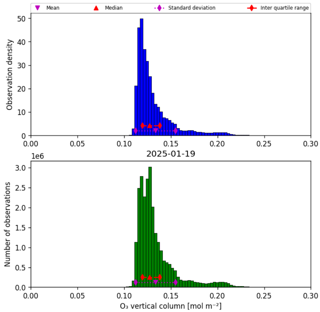
Figure 21: Histogram of “O 3 vertical column” for 2025-01-18 to 2025-01-20
