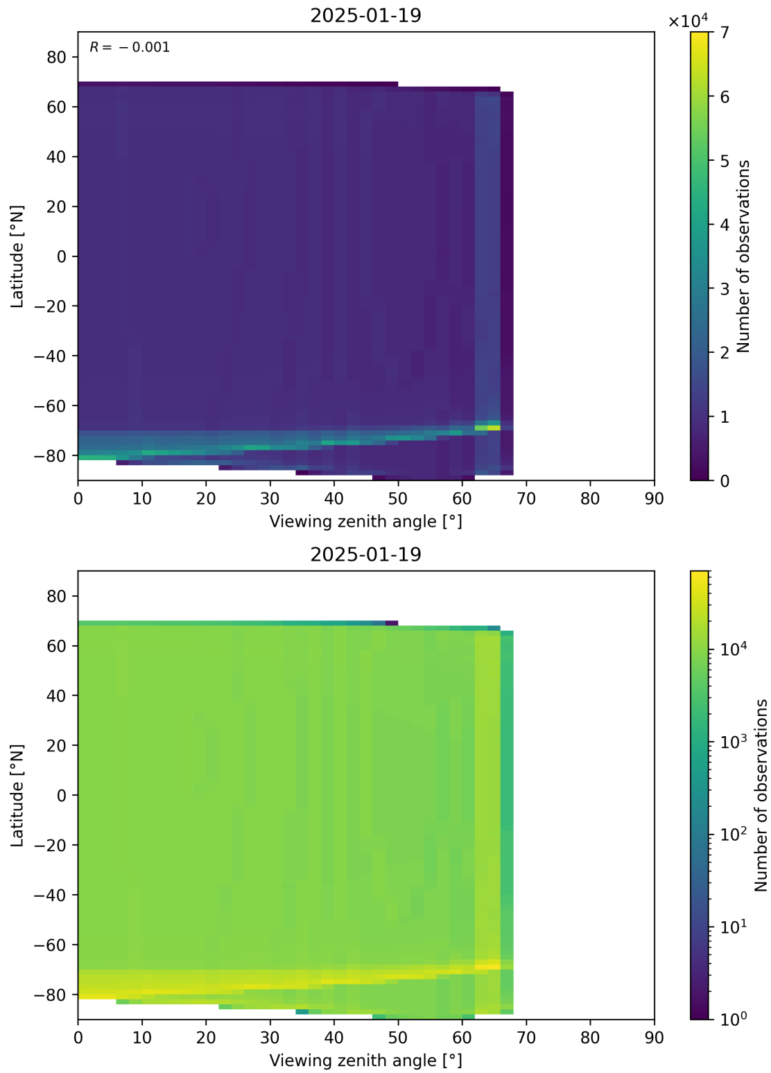
Figure 49: Scatter density plot of “Viewing zenith angle” against “Latitude” for 2025-01-18 to 2025-01-20.
