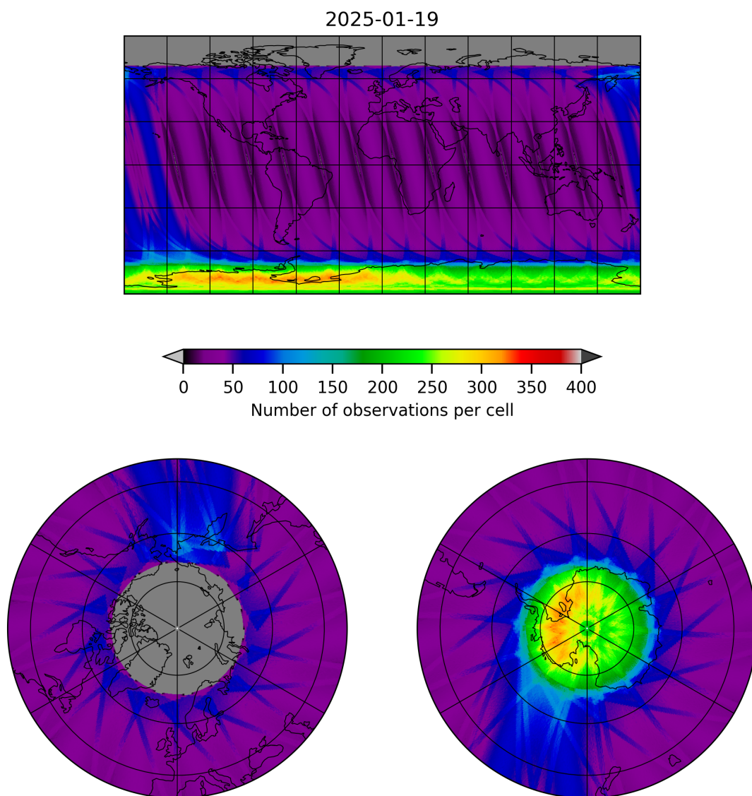
Figure 12: Map of the number of observations for 2025-01-18 to 2025-01-20
