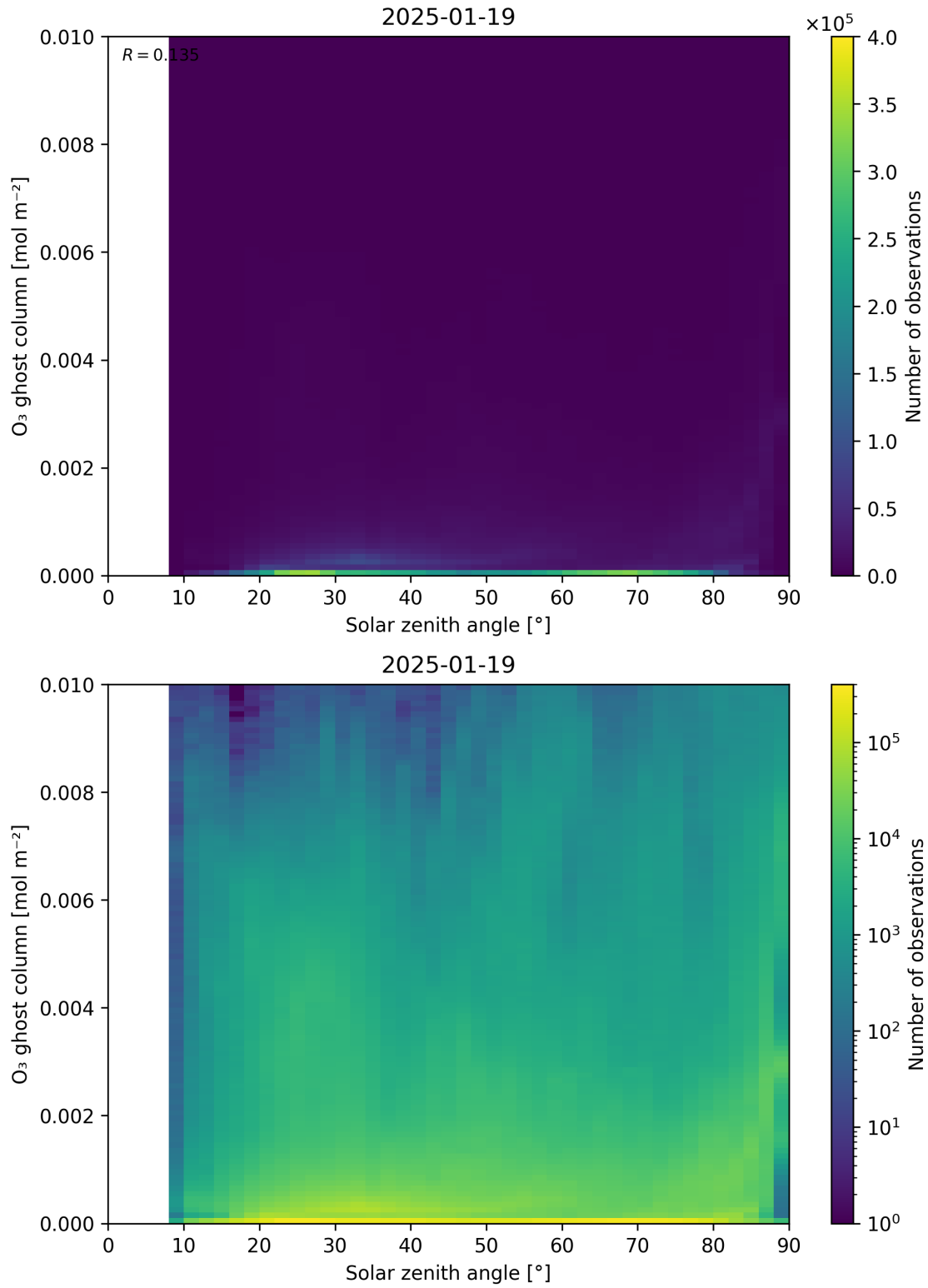
Figure 46: Scatter density plot of “Solar zenith angle” against “O 3 ghost column” for 2025-01-18 to 2025-01-20.
