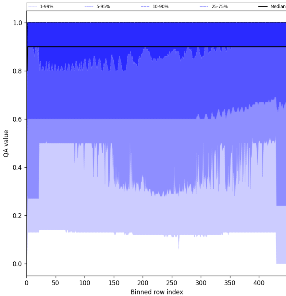
Figure 27: Along track statistics of “QA value” for 2025-01-18 to 2025-01-20
