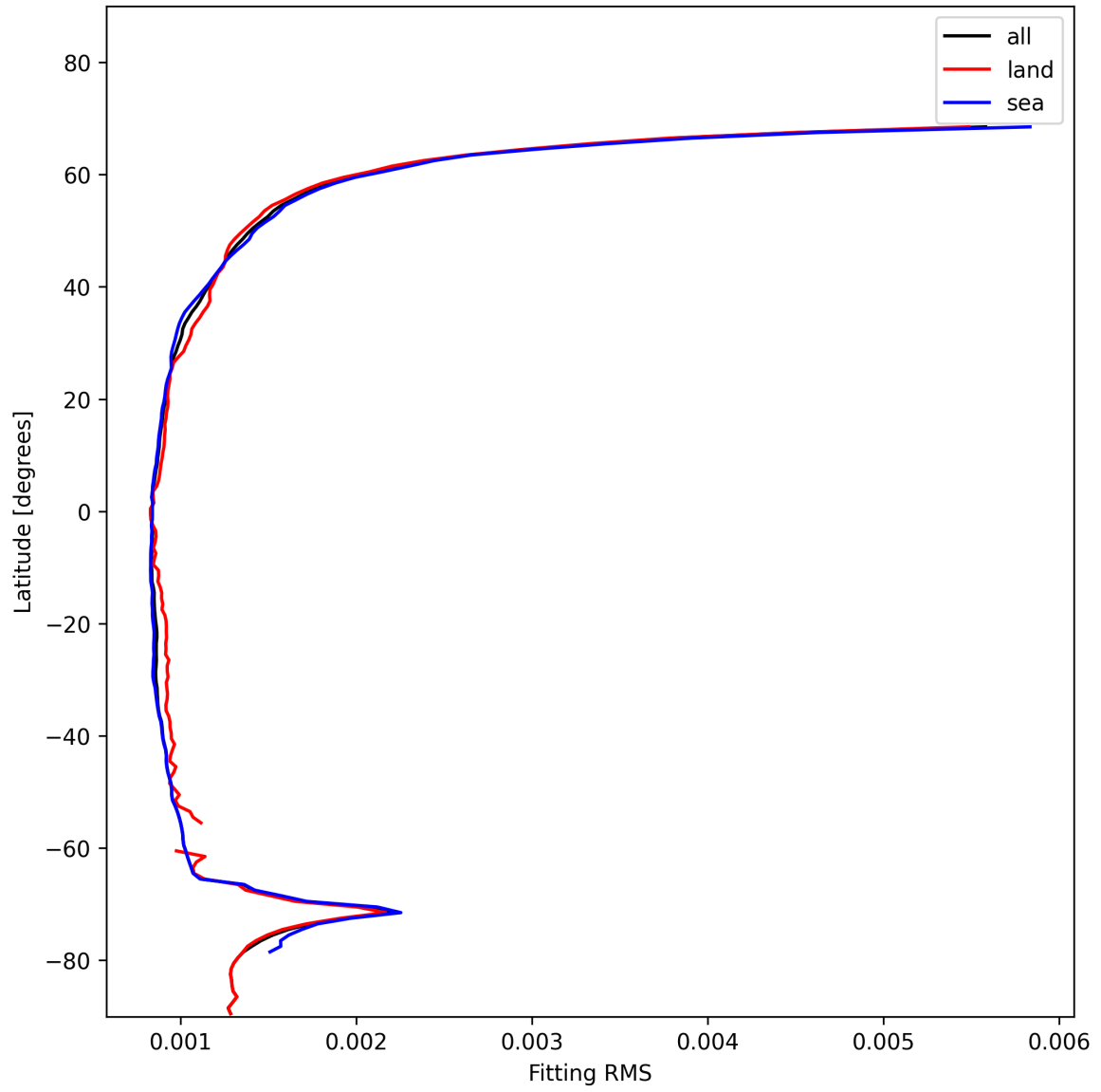
Figure 16: Zonal average of “Fitting RMS” for 2025-01-18 to 2025-01-20.
