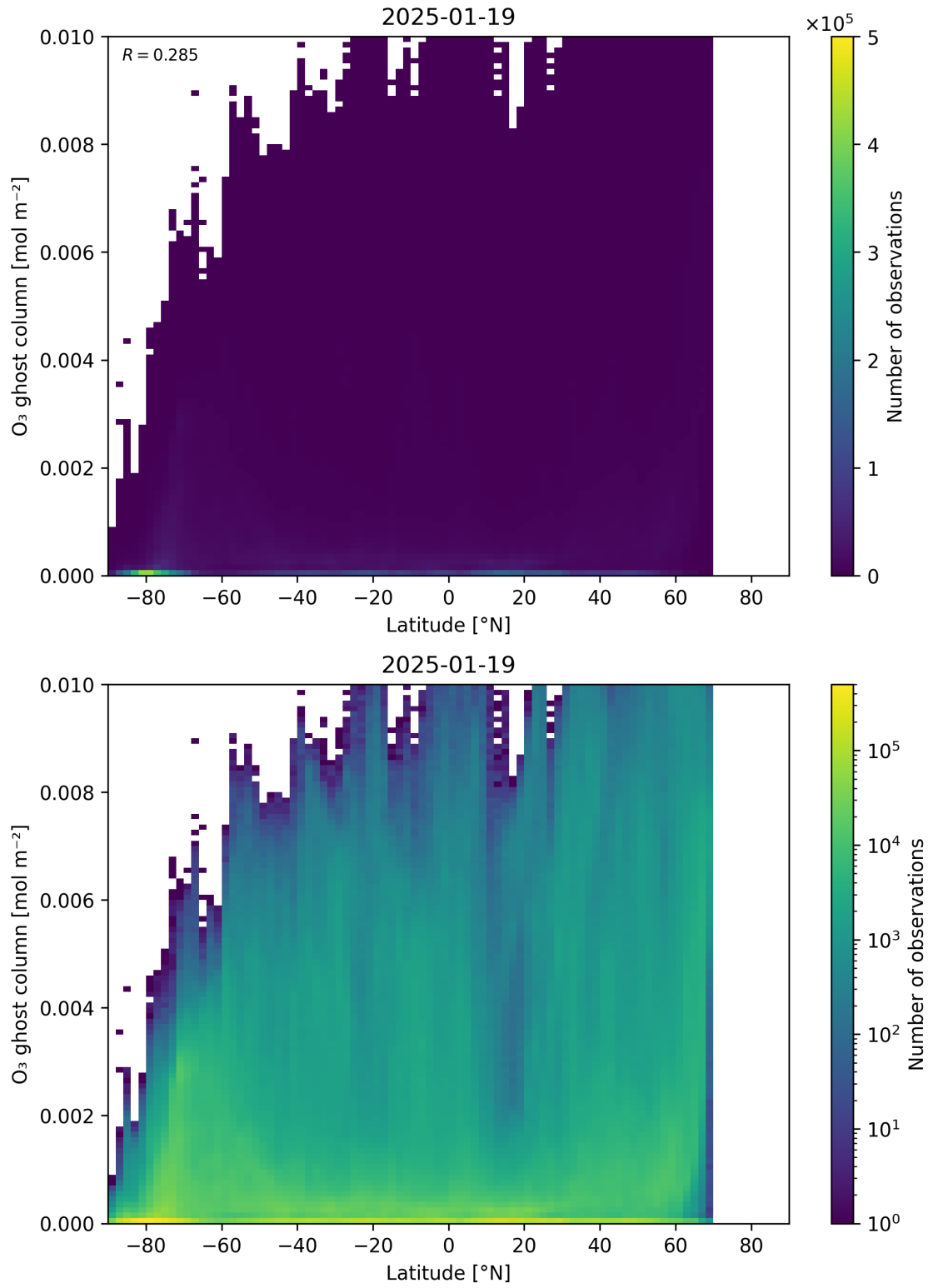
Figure 35: Scatter density plot of “Latitude” against “O 3 ghost column” for 2025-01-18 to 2025-01-20.
