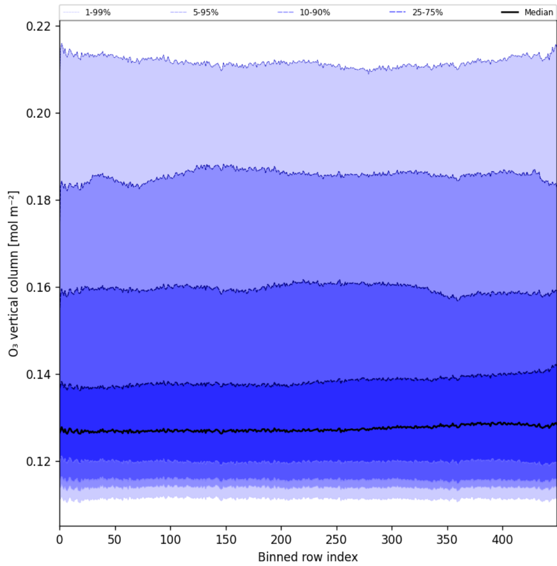
Figure 28: Along track statistics of “O 3 vertical column” for 2025-01-18 to 2025-01-20
