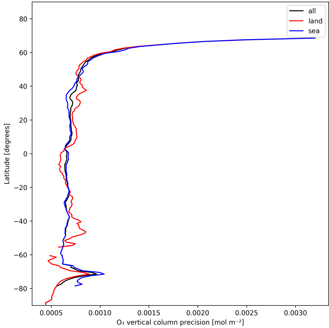
Figure 15: Zonal average of “O 3 vertical column precision” for 2025-01-18 to 2025-01-20.
