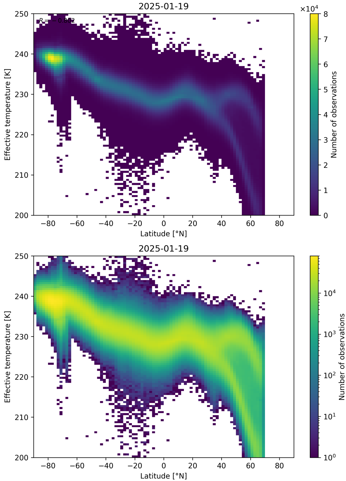
Figure 34: Scatter density plot of “Latitude” against “Effective temperature” for 2025-01-18 to 2025-01-20.
