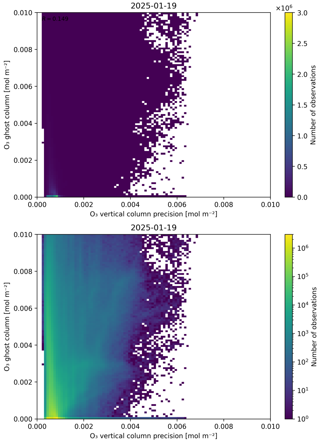
Figure 43: Scatter density plot of “O 3 vertical column precision” against “O 3 ghost column” for 2025-01-18 to 2025-01-20.
