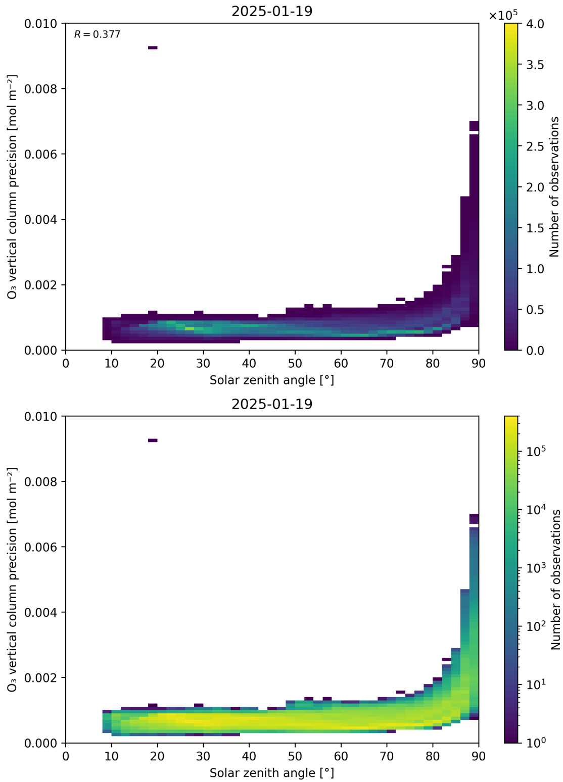
Figure 48: Scatter density plot of “Solar zenith angle” against “O 3 vertical column precision” for 2025-01-18 to 2025-01-20.
