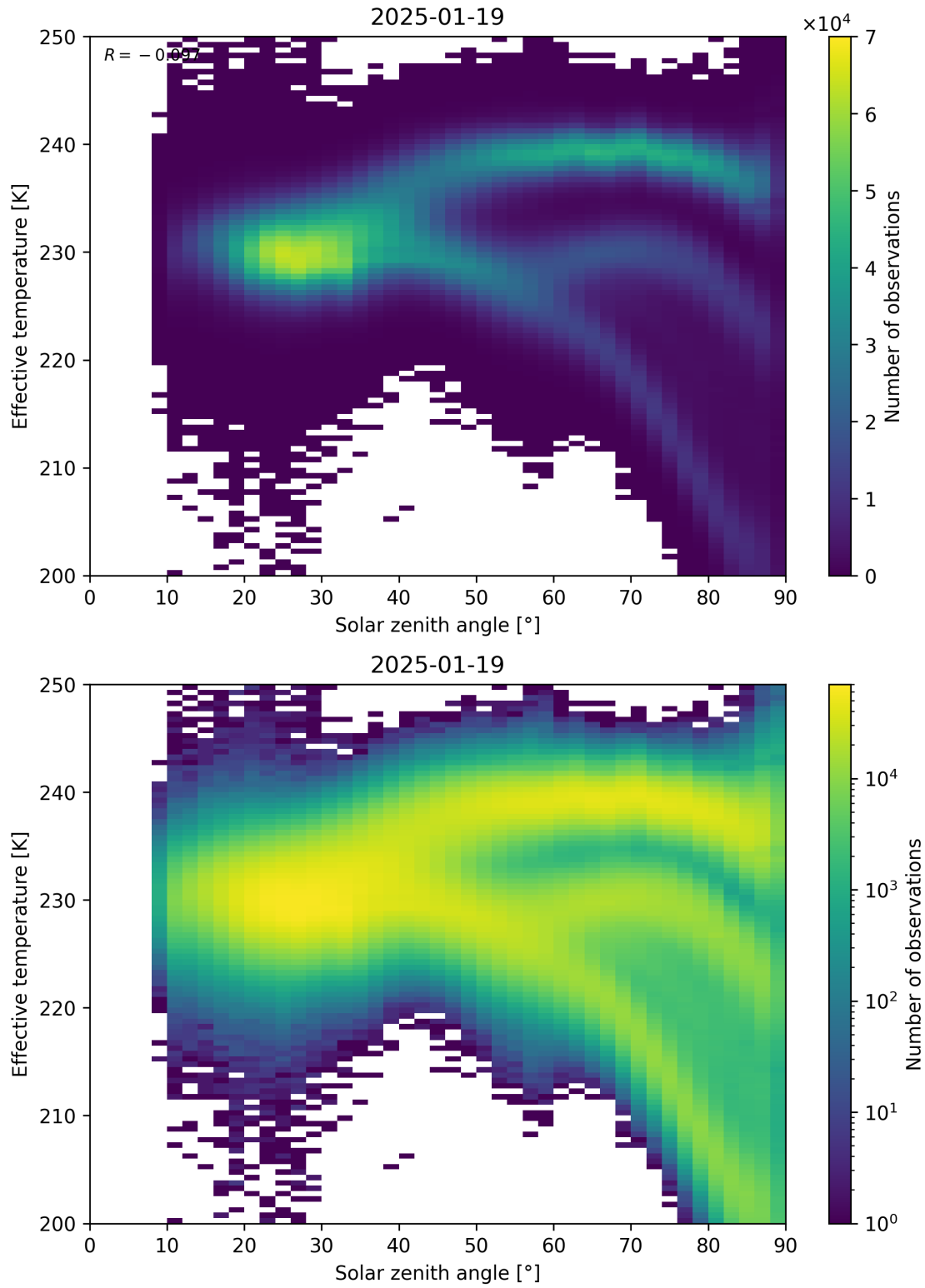
Figure 45: Scatter density plot of “Solar zenith angle” against “Effective temperature” for 2025-01-18 to 2025-01-20.
