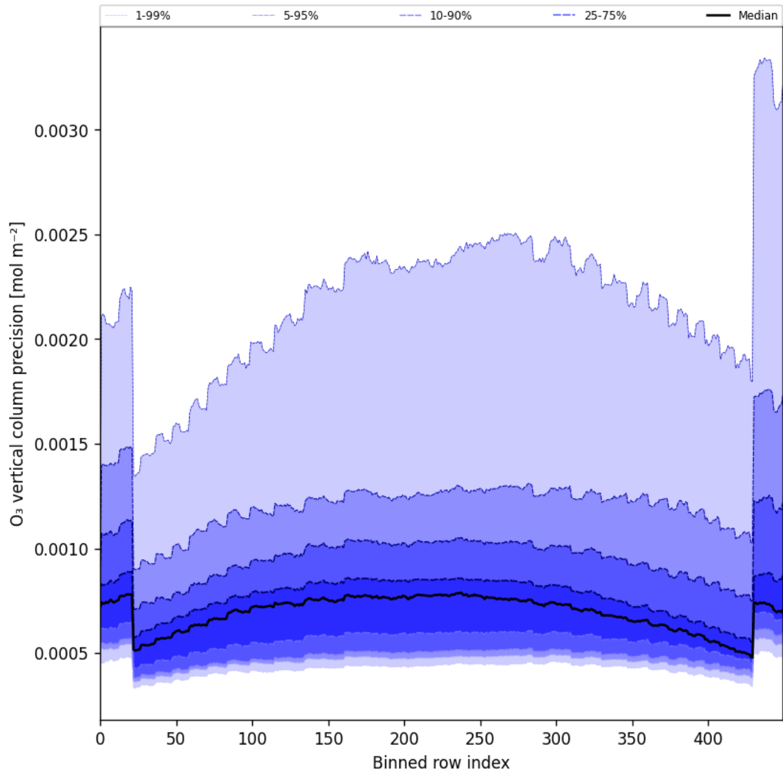
Figure 29: Along track statistics of “O 3 vertical column precision” for 2025-01-18 to 2025-01-20
