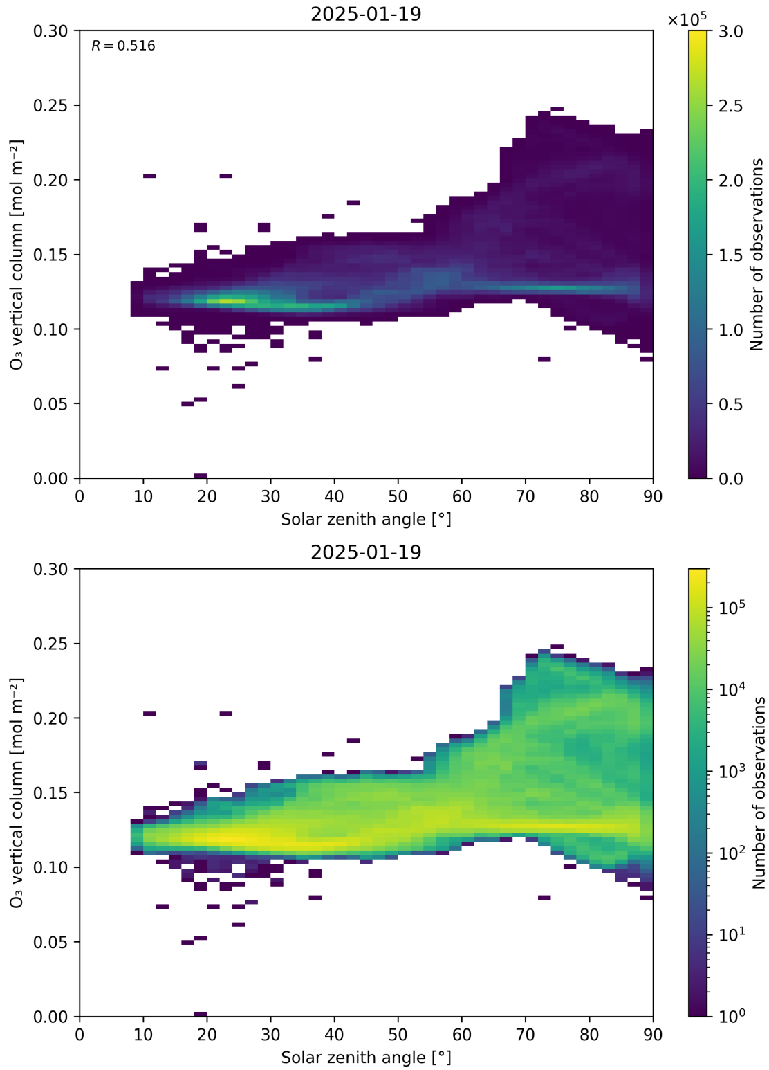
Figure 47: Scatter density plot of “Solar zenith angle” against “O 3 vertical column” for 2025-01-18 to 2025-01-20.
