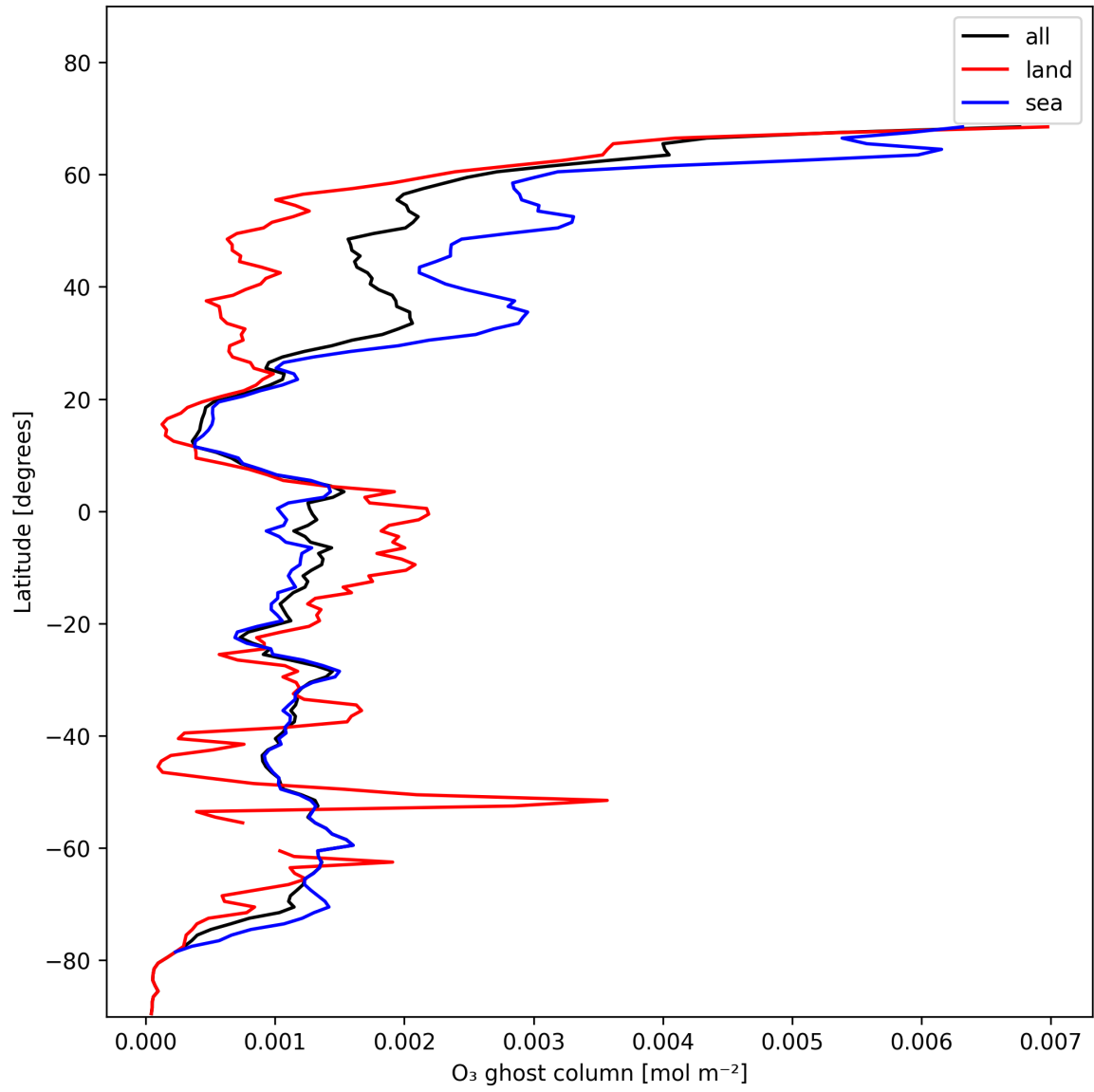
Figure 18: Zonal average of “O 3 ghost column” for 2025-01-18 to 2025-01-20.
