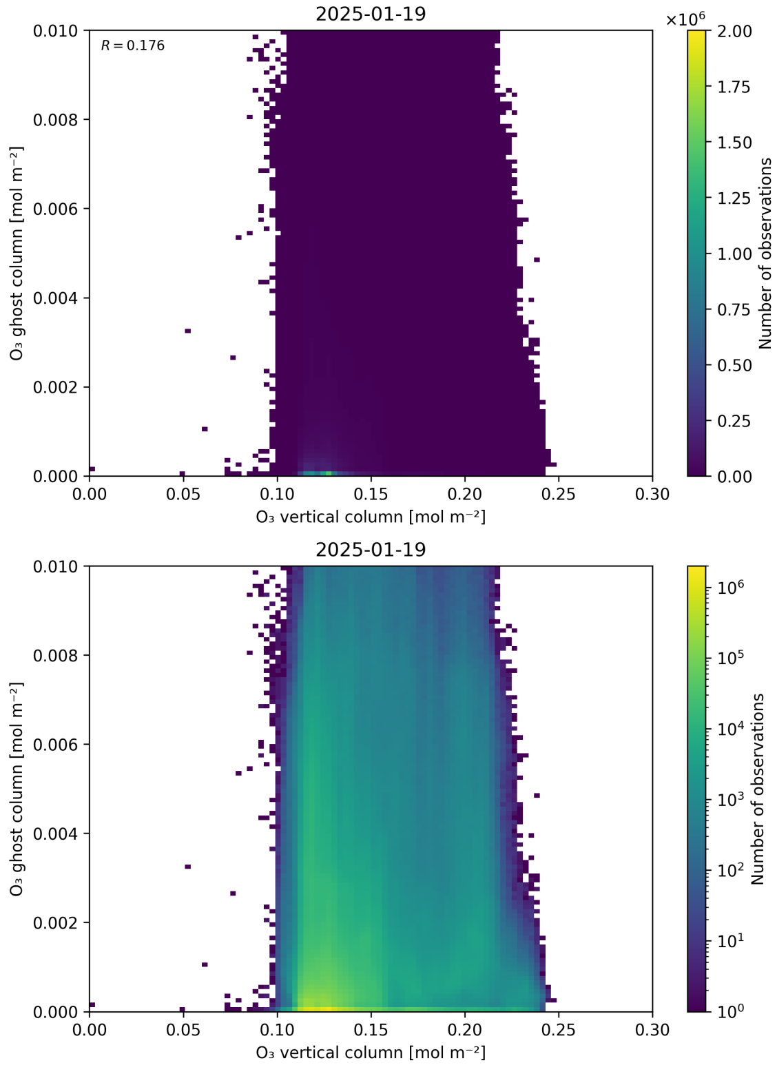
Figure 40: Scatter density plot of “O 3 vertical column” against “O 3 ghost column” for 2025-01-18 to 2025-01-20.
