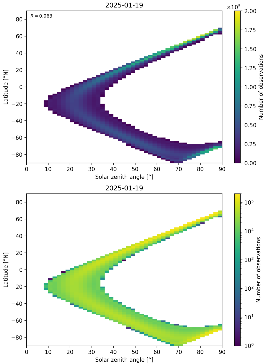
Figure 44: Scatter density plot of “Solar zenith angle” against “Latitude” for 2025-01-18 to 2025-01-20.
