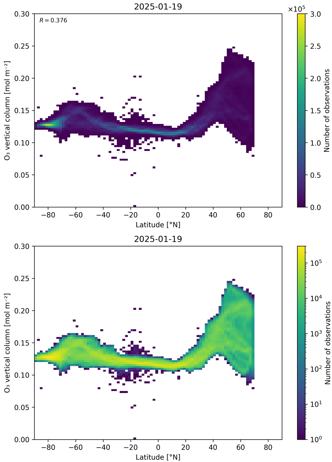
Figure 36: Scatter density plot of “Latitude” against “O 3 vertical column” for 2025-01-18 to 2025-01-20.
