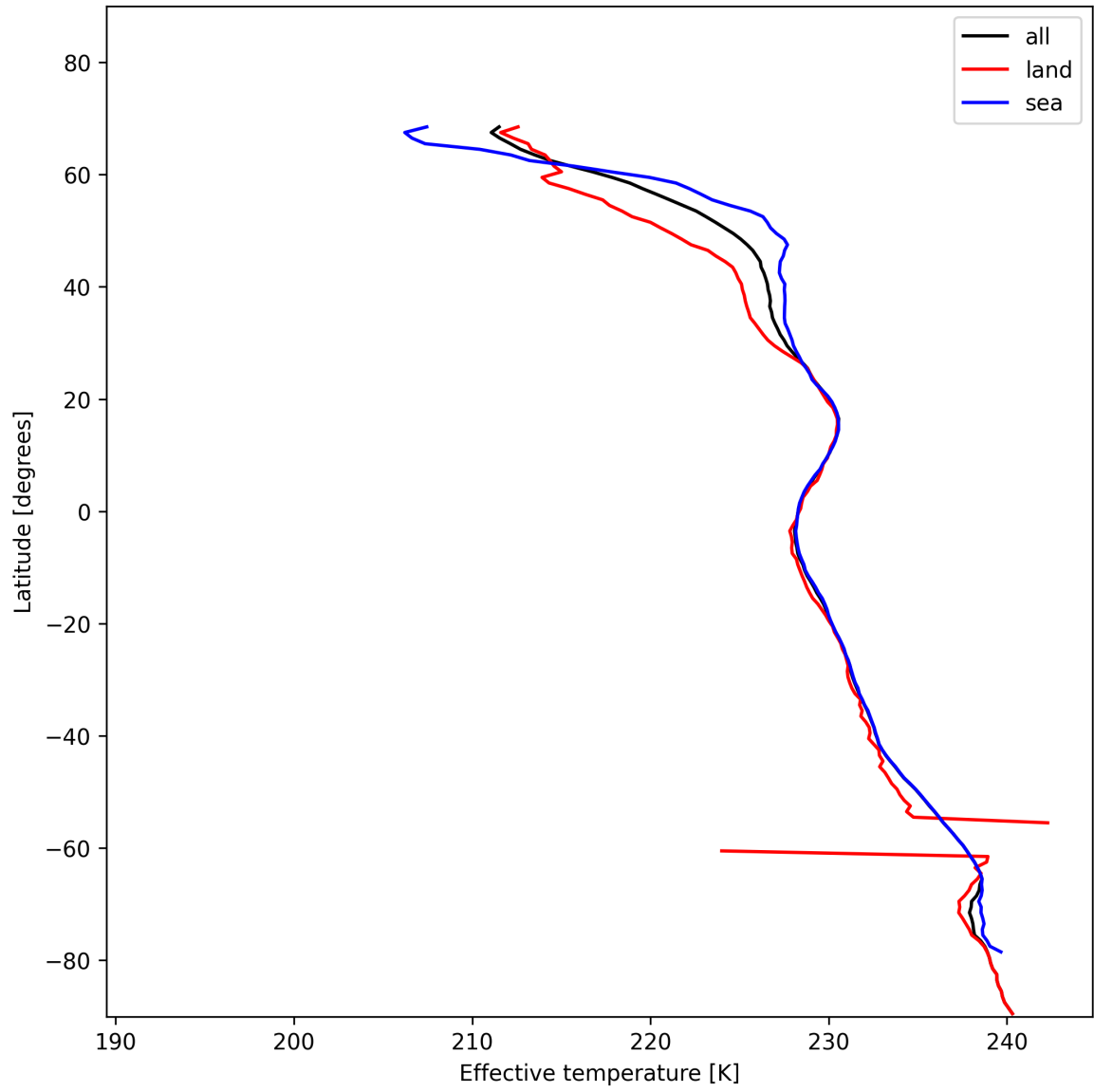
Figure 17: Zonal average of "Effective temperature" for 2025-01-18 to 2025-01-20.
