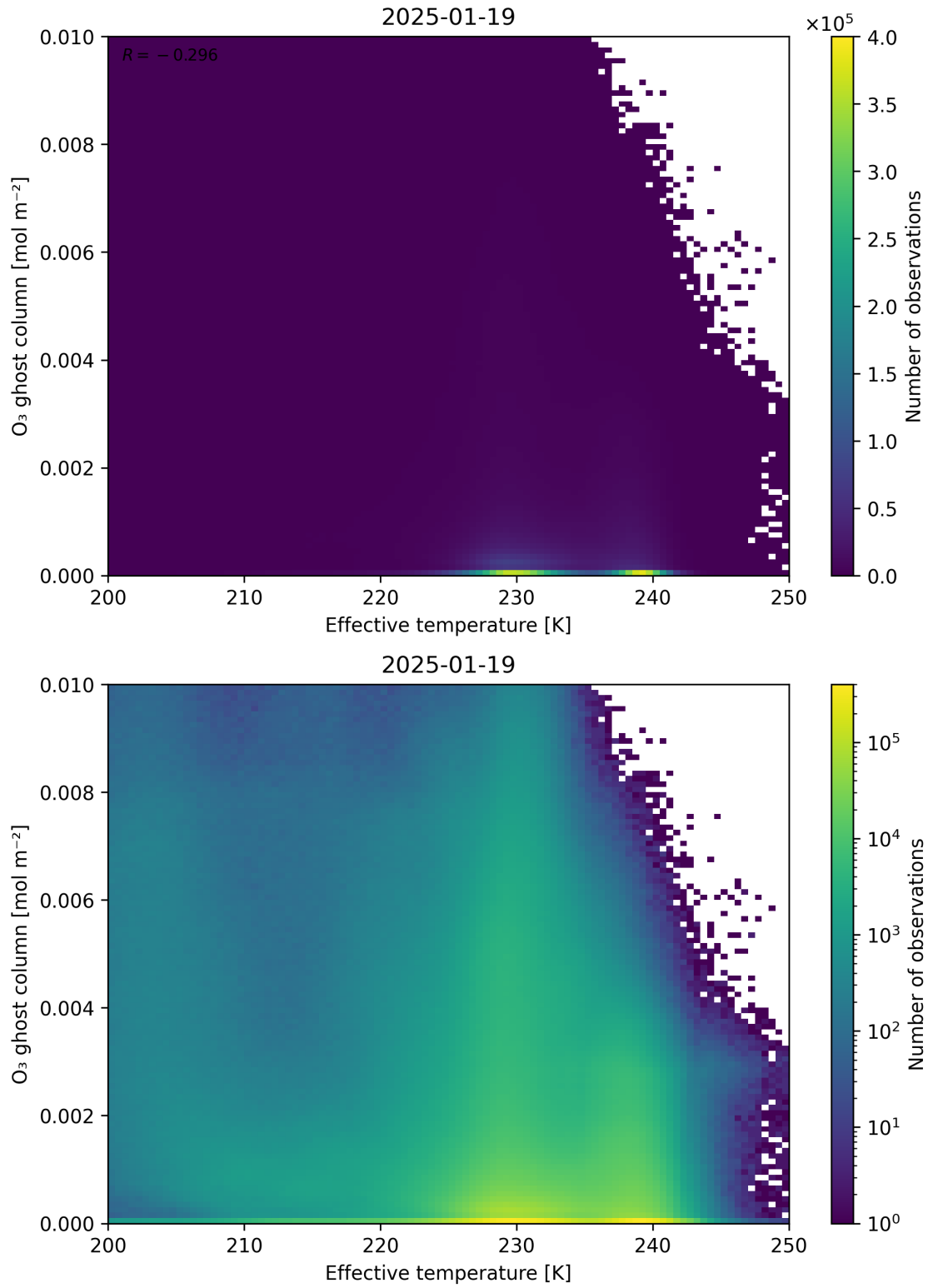
Figure 38: Scatter density plot of “Effective temperature” against “O 3 ghost column” for 2025-01-18 to 2025-01-20.
