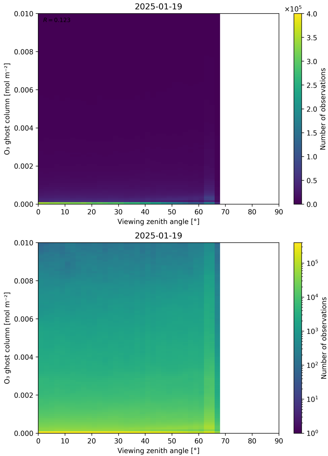
Figure 51: Scatter density plot of “Viewing zenith angle” against “O 3 ghost column” for 2025-01-18 to 2025-01-20.
