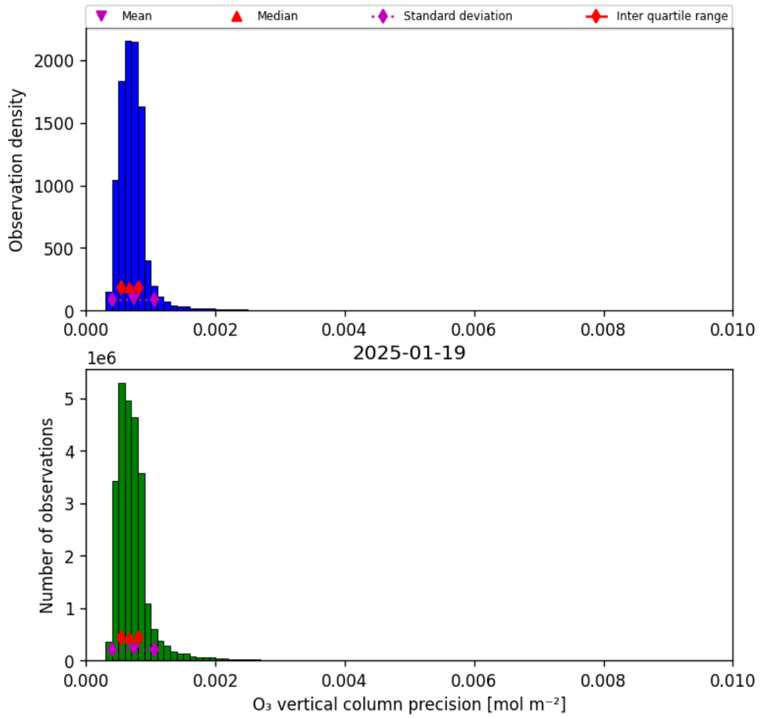
Figure 22: Histogram of “O 3 vertical column precision” for 2025-01-18 to 2025-01-20
