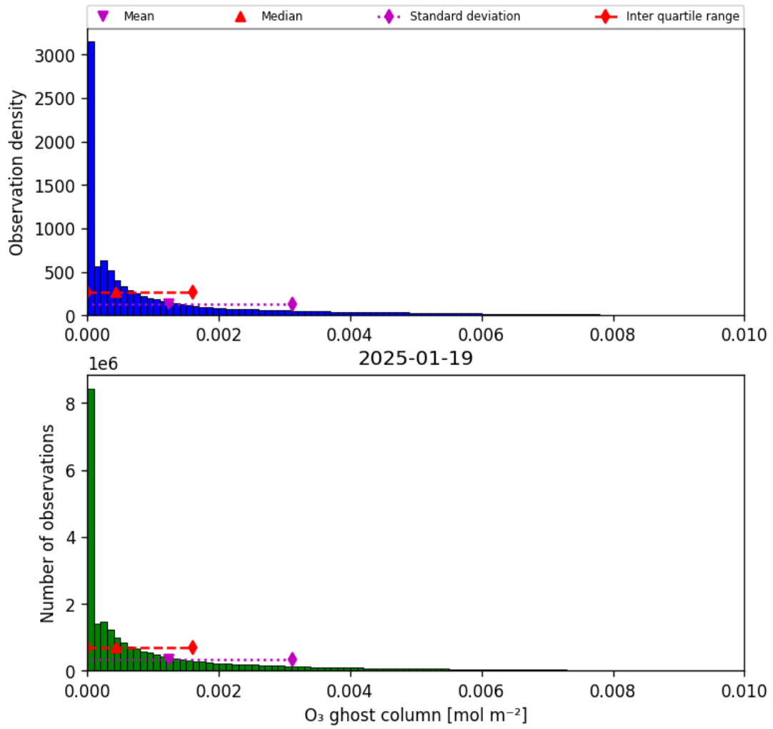
Figure 25: Histogram of "O 3 ghost column" for 2025-01-18 to 2025-01-20
