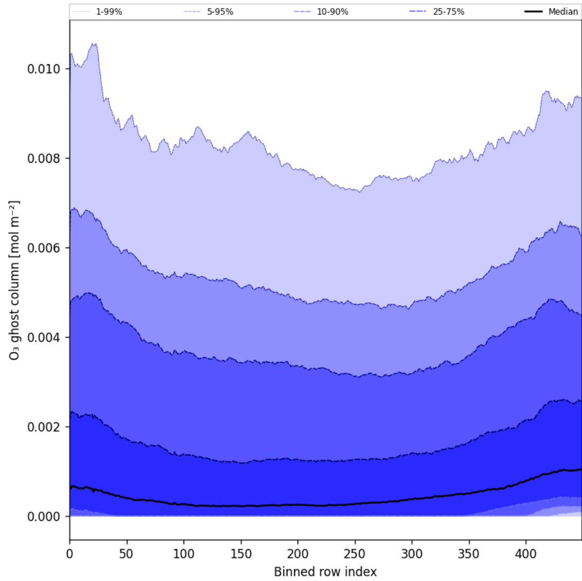
Figure 32: Along track statistics of “O 3 ghost column” for 2025-01-18 to 2025-01-20
