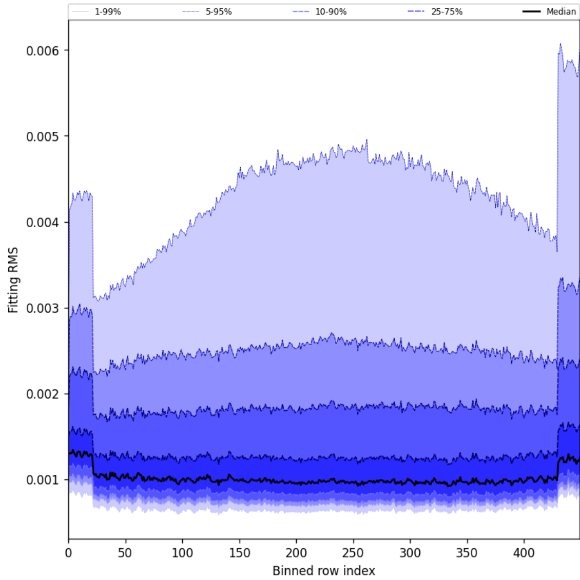
Figure 30: Along track statistics of “Fitting RMS” for 2025-01-18 to 2025-01-20
