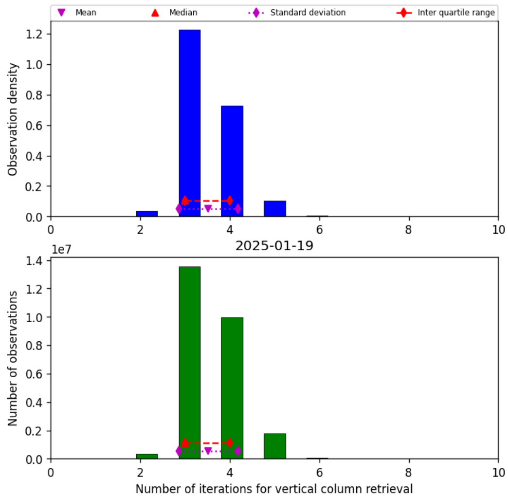
Figure 26: Histogram of “Number of iterations for vertical column retrieval” for 2025-01-18 to 2025-01-20
