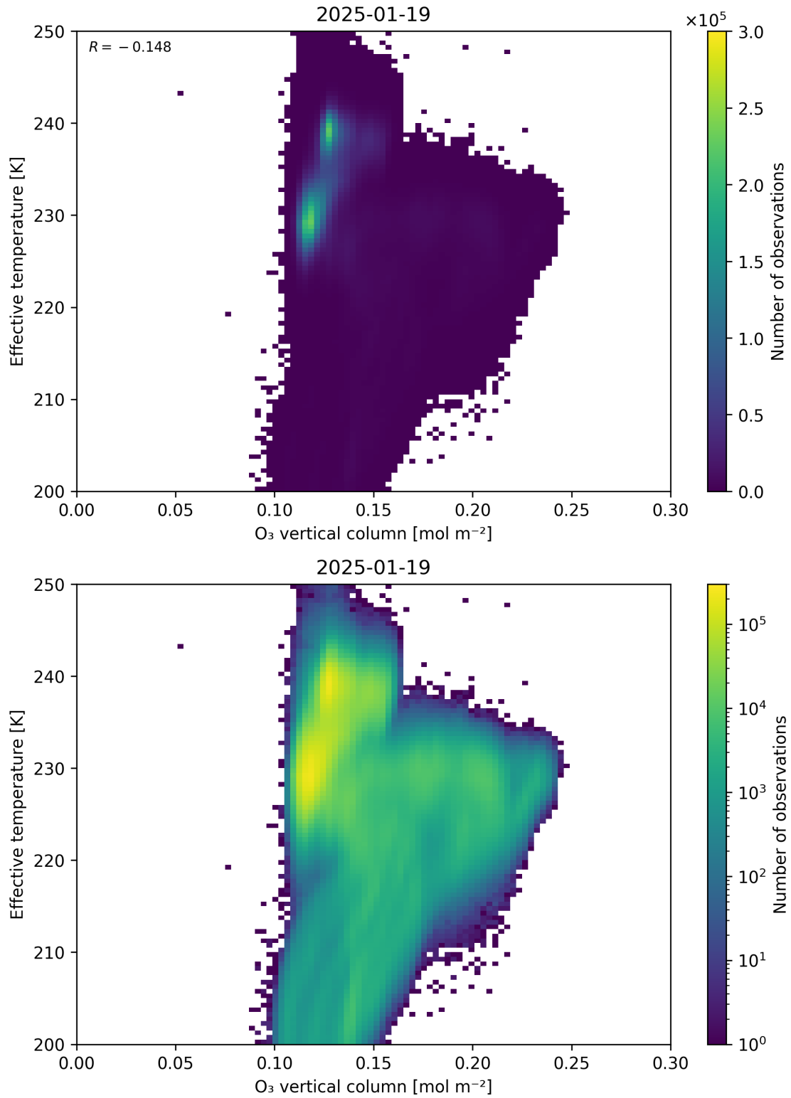
Figure 39: Scatter density plot of “O 3 vertical column” against “Effective temperature” for 2025-01-18 to 2025-01-20.
