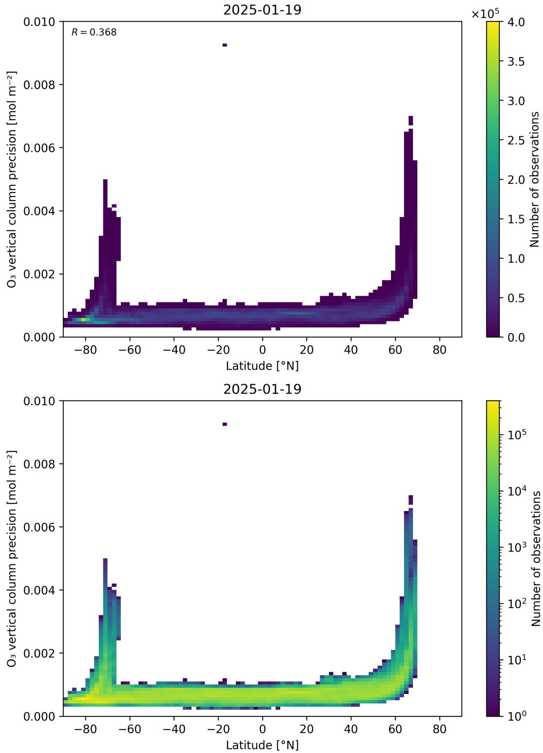
Figure 37: Scatter density plot of “Latitude” against “O 3 vertical column precision” for 2025-01-18 to 2025-01-20.
