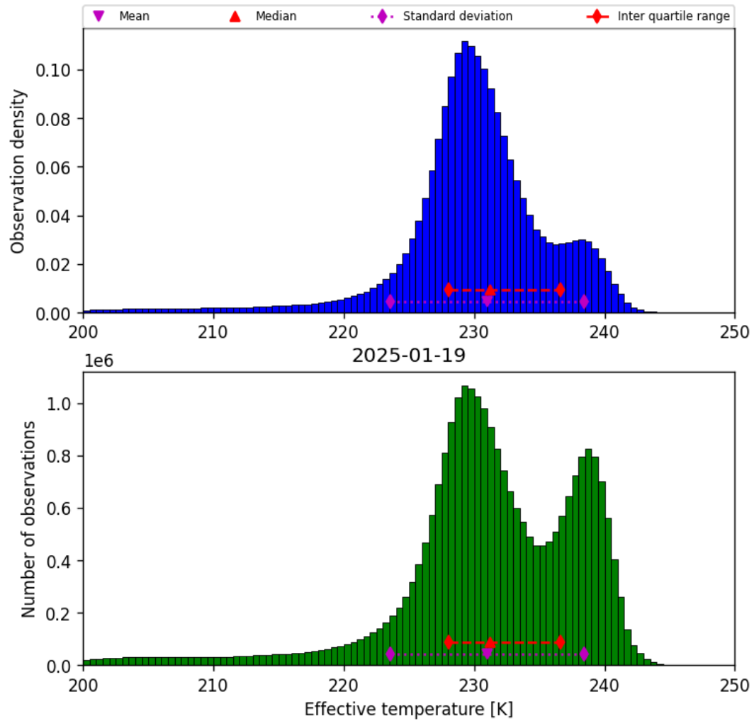
Figure 24: Histogram of “Effective temperature” for 2025-01-18 to 2025-01-20
