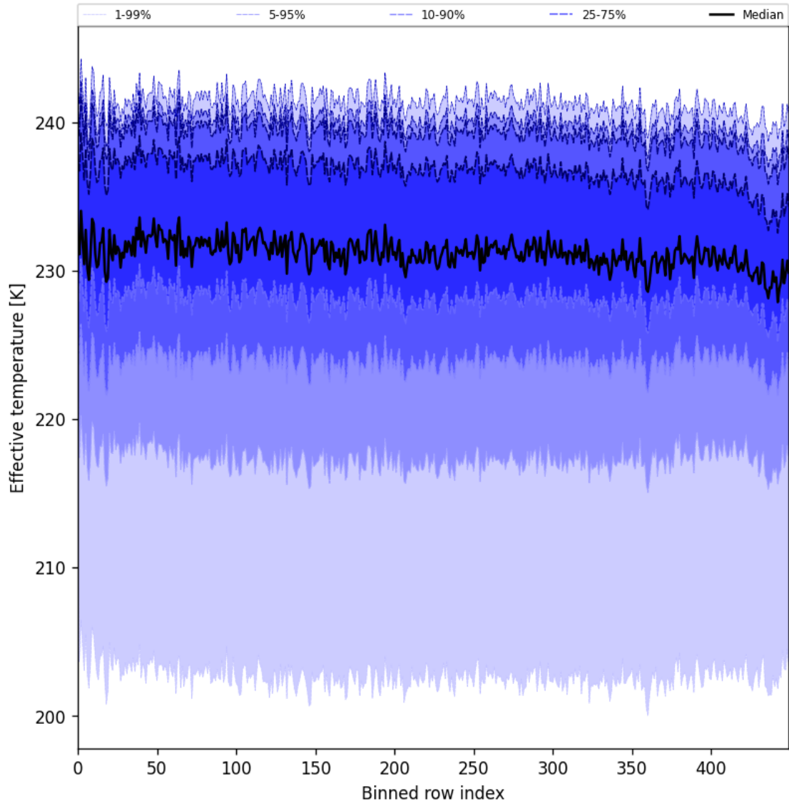
Figure 31: Along track statistics of “Effective temperature” for 2025-01-18 to 2025-01-20
