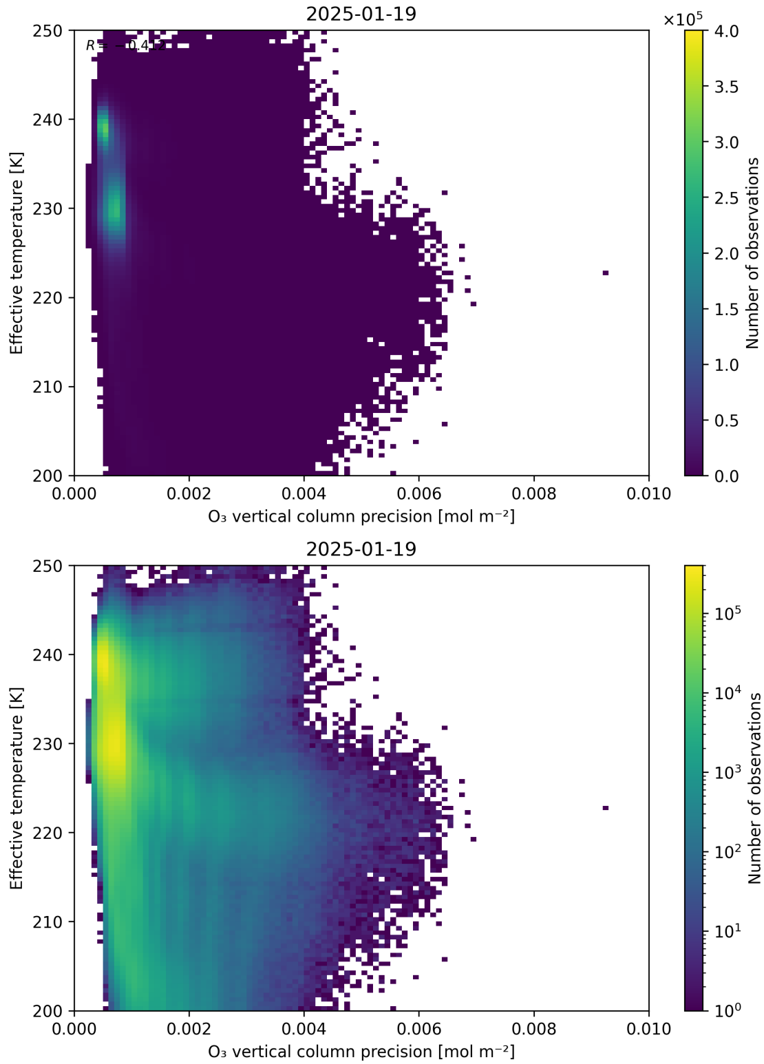
Figure 42: Scatter density plot of “O 3 vertical column precision” against “Effective temperature” for 2025-01-18 to 2025-01-20.
