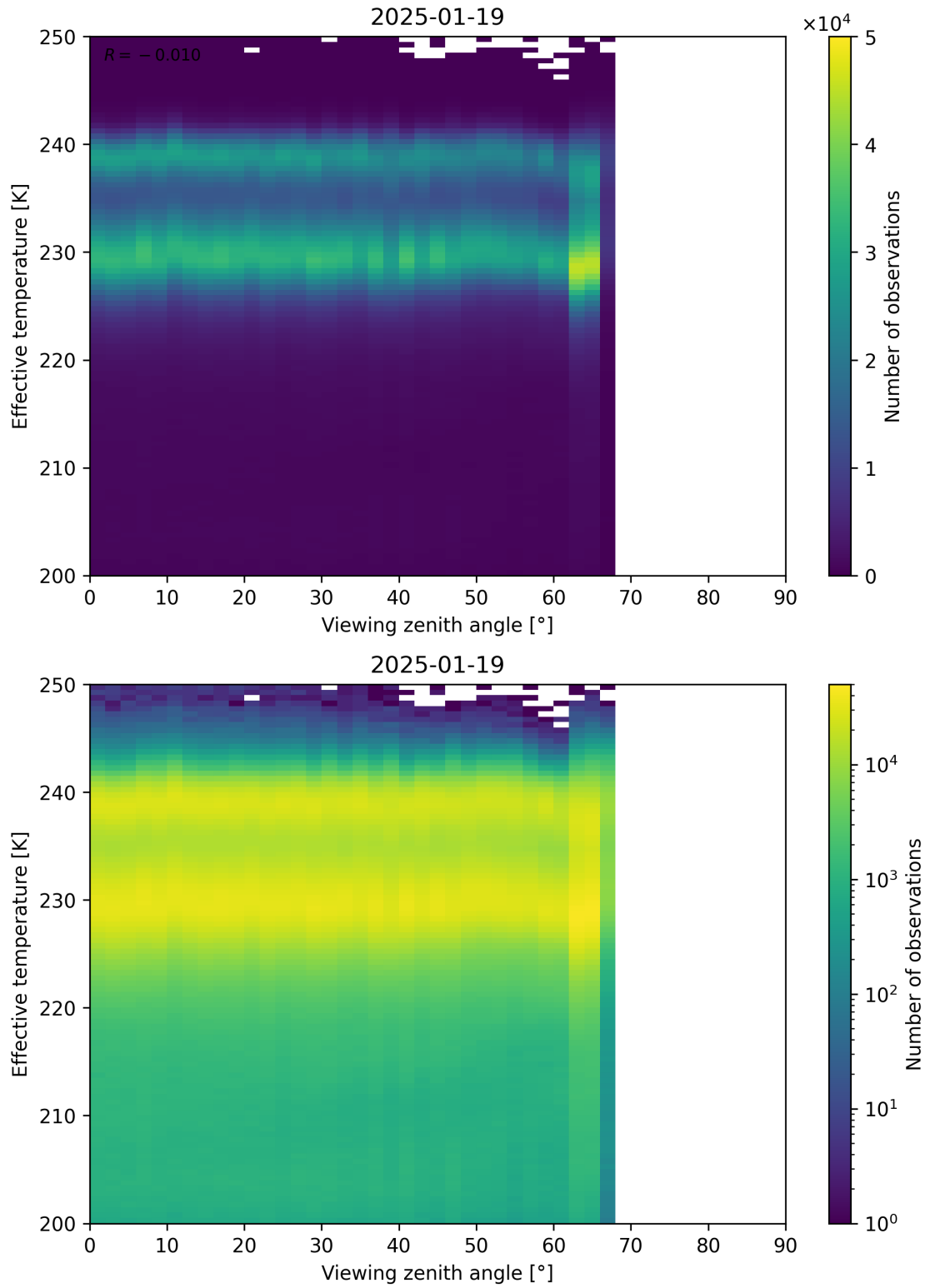
Figure 50: Scatter density plot of “Viewing zenith angle” against “Effective temperature” for 2025-01-18 to 2025-01-20.
