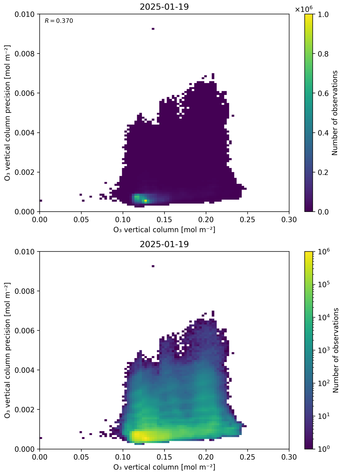
Figure 41: Scatter density plot of “O 3 vertical column” against “O 3 vertical column precision” for 2025-01-18 to 2025-01-20.
