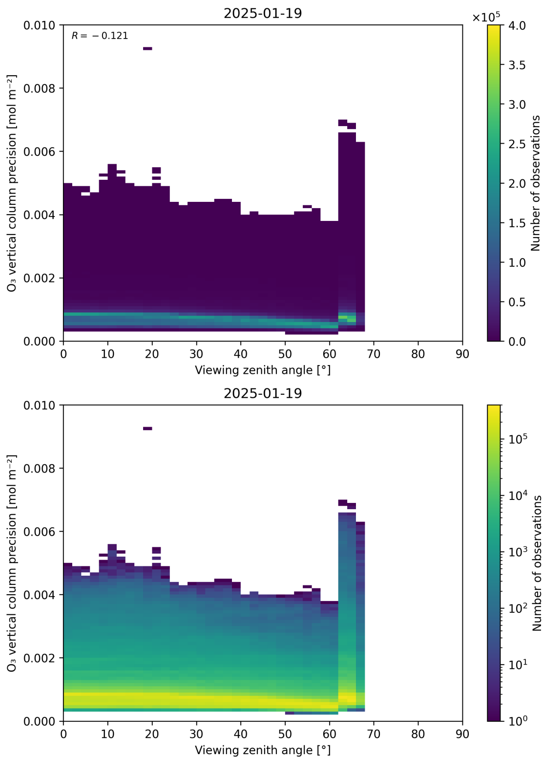
Figure 53: Scatter density plot of “Viewing zenith angle” against “O 3 vertical column precision” for 2025-01-18 to 2025-01-20.
