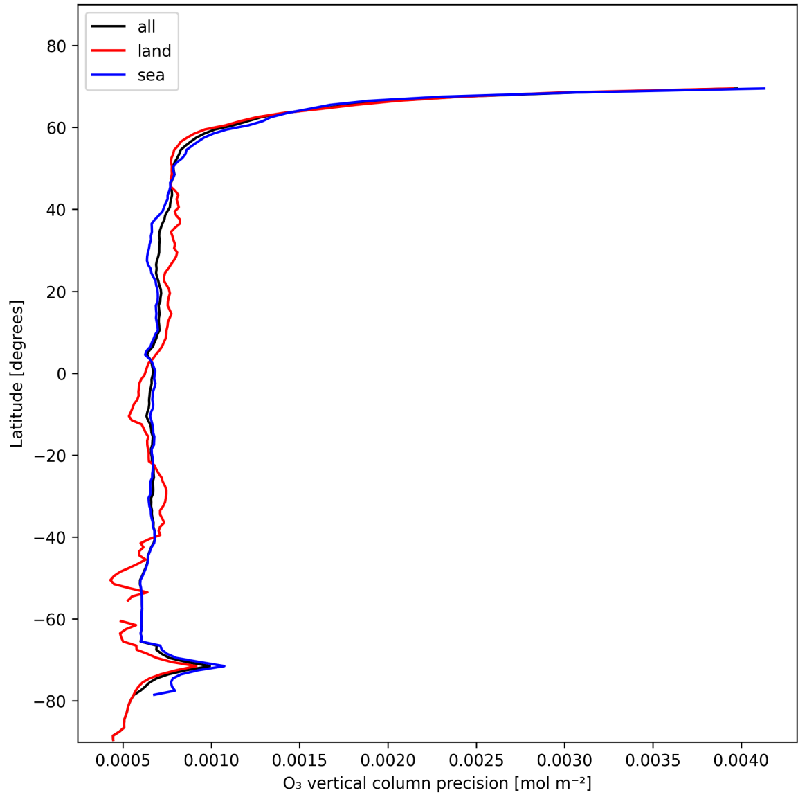
Figure 15: Zonal average of “O 3 vertical column precision” for 2025-01-19 to 2025-01-21.
