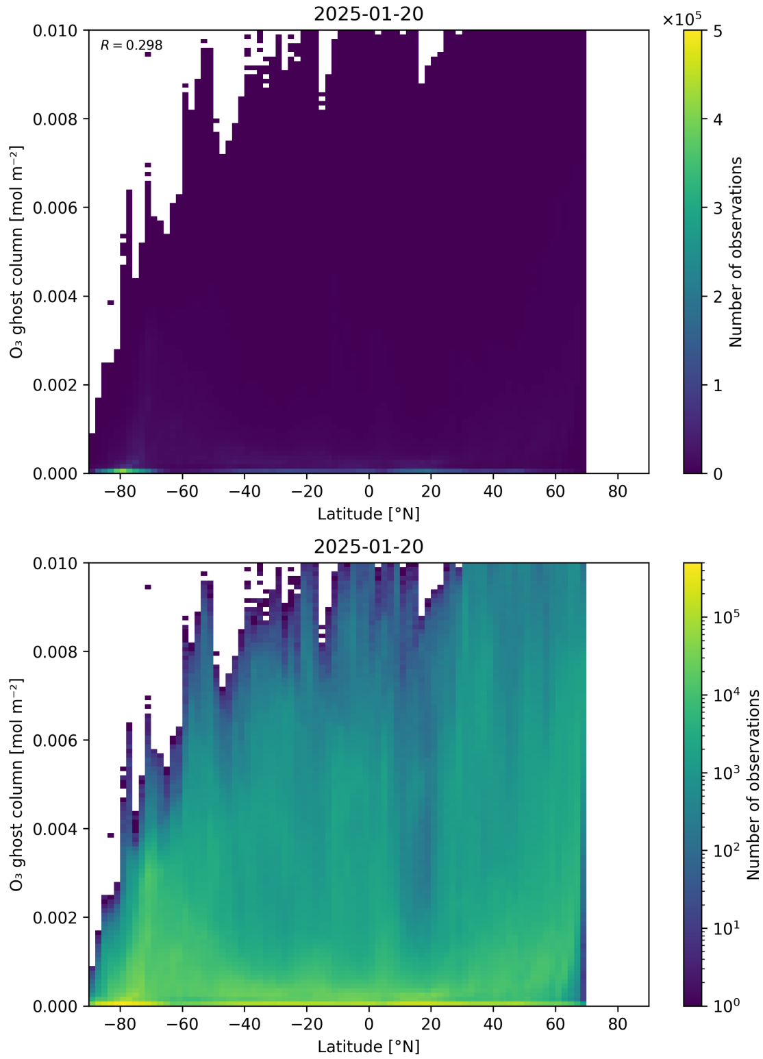
Figure 35: Scatter density plot of “Latitude” against “O 3 ghost column” for 2025-01-19 to 2025-01-21.
