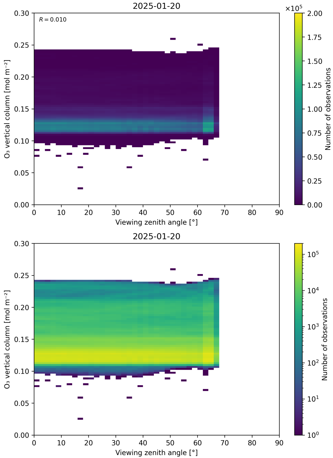
Figure 52: Scatter density plot of “Viewing zenith angle” against “O 3 vertical column” for 2025-01-19 to 2025-01-21.
