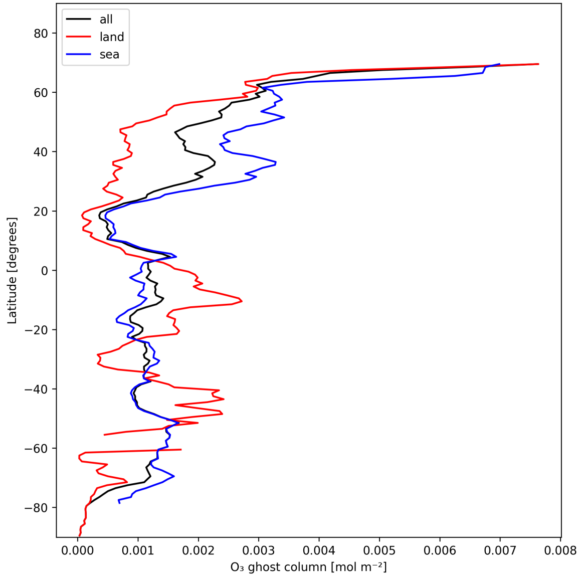
Figure 18: Zonal average of “O 3 ghost column” for 2025-01-19 to 2025-01-21.
