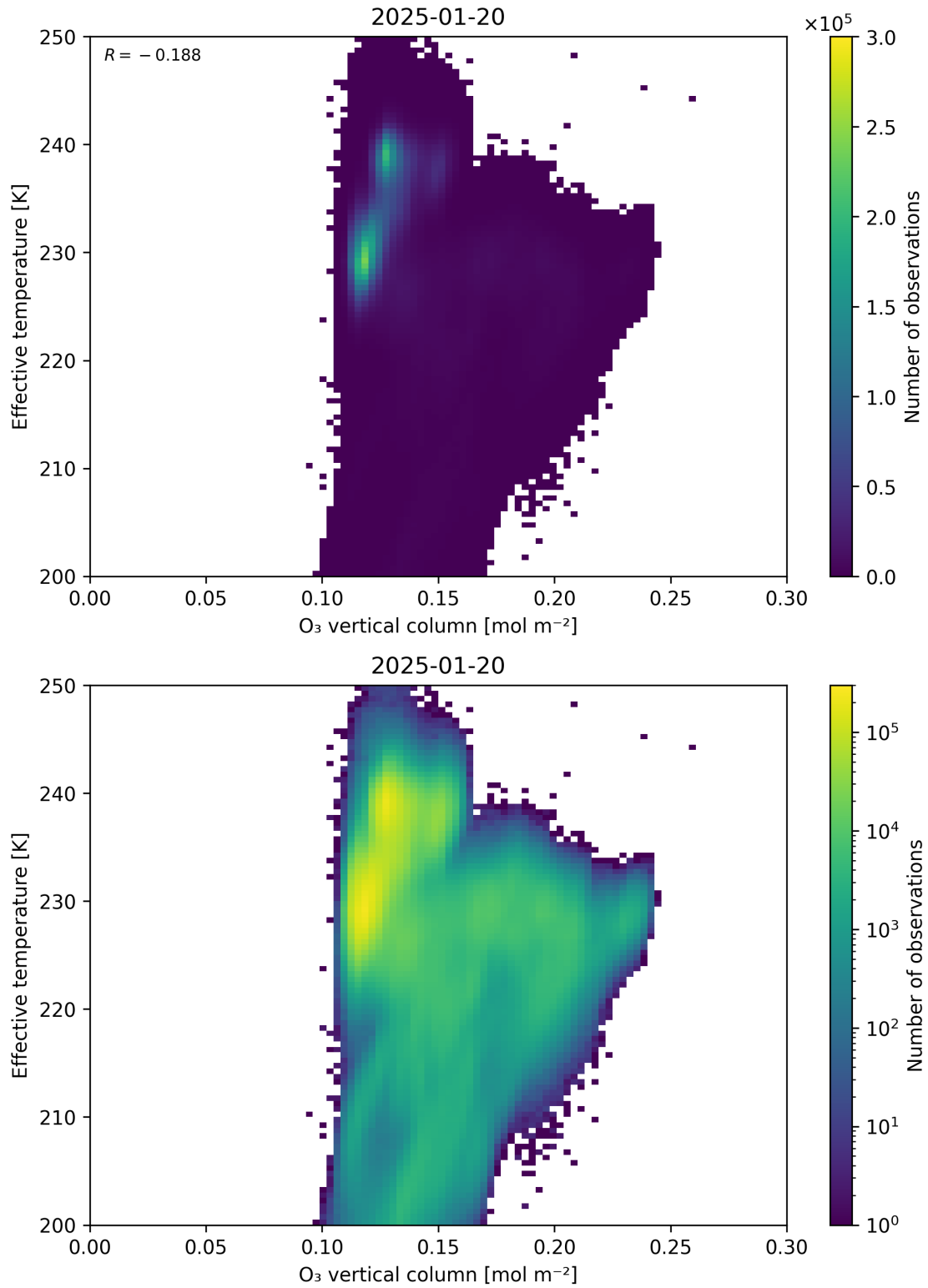
Figure 39: Scatter density plot of “O 3 vertical column” against “Effective temperature” for 2025-01-19 to 2025-01-21.
