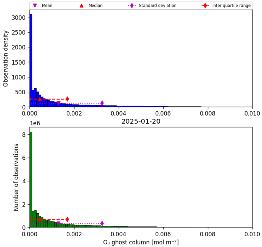
Figure 25: Histogram of “O 3 ghost column” for 2025-01-19 to 2025-01-21
