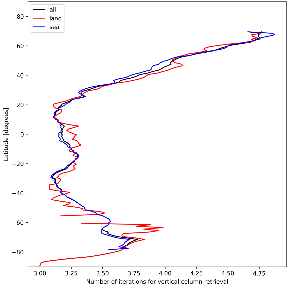
Figure 19: Zonal average of “Number of iterations for vertical column retrieval” for 2025-01-19 to 2025-01-21.
