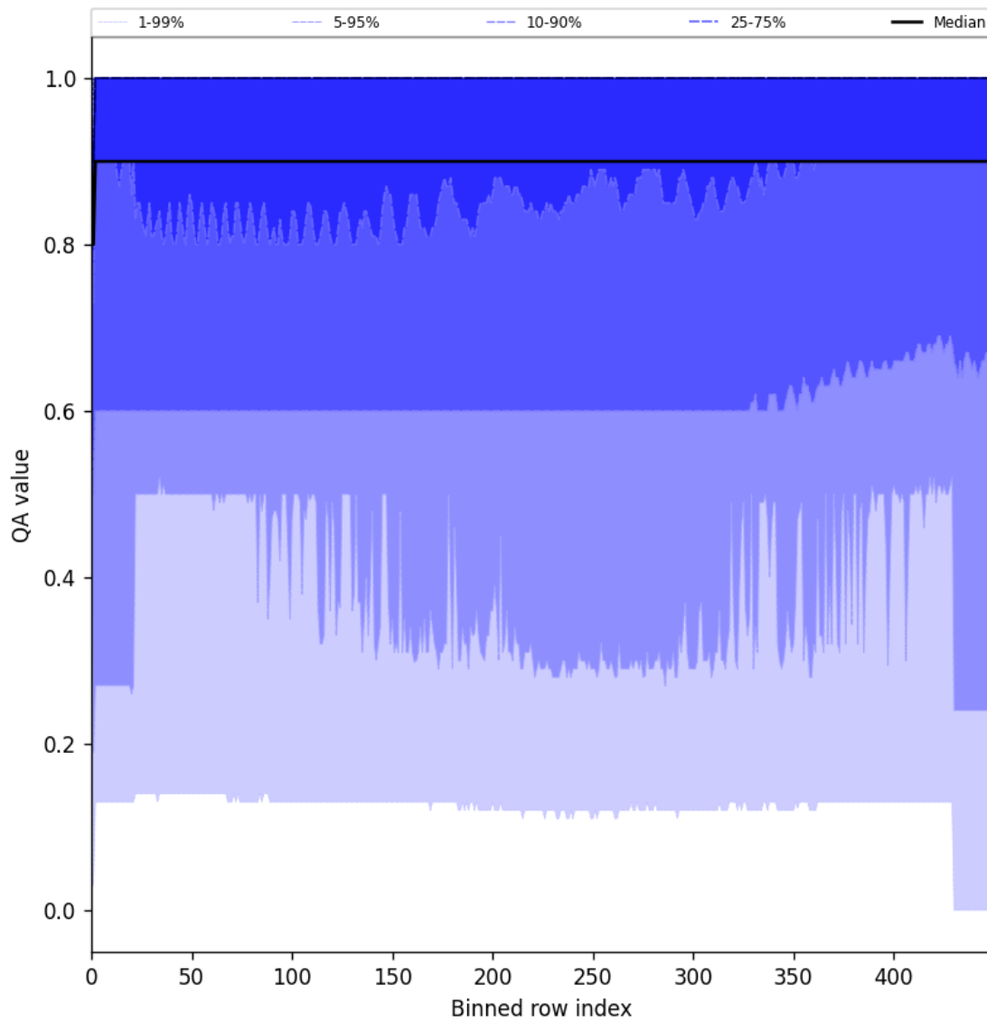
Figure 27: Along track statistics of “QA value” for 2025-01-19 to 2025-01-21
