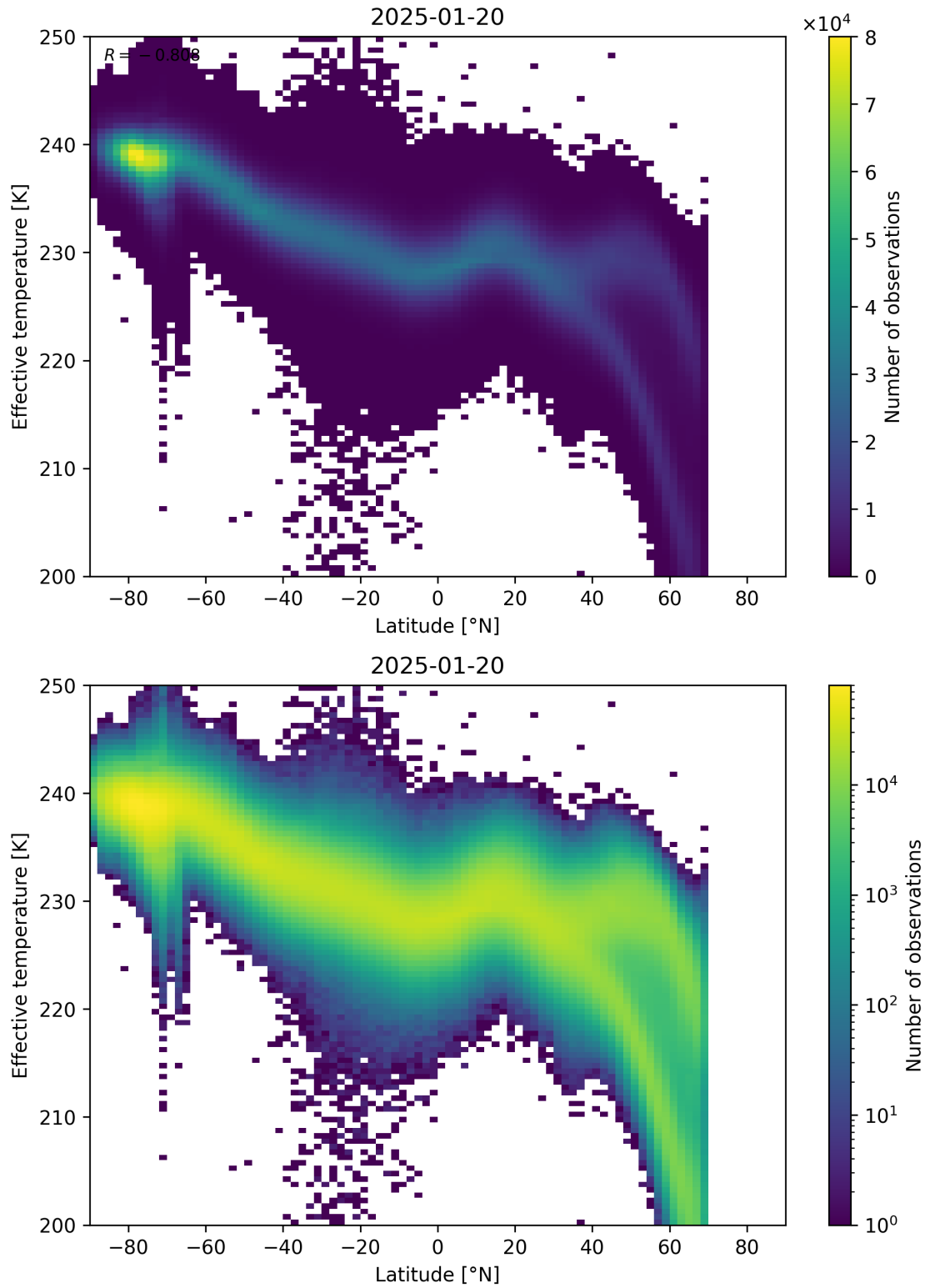
Figure 34: Scatter density plot of “Latitude” against “Effective temperature” for 2025-01-19 to 2025-01-21.
