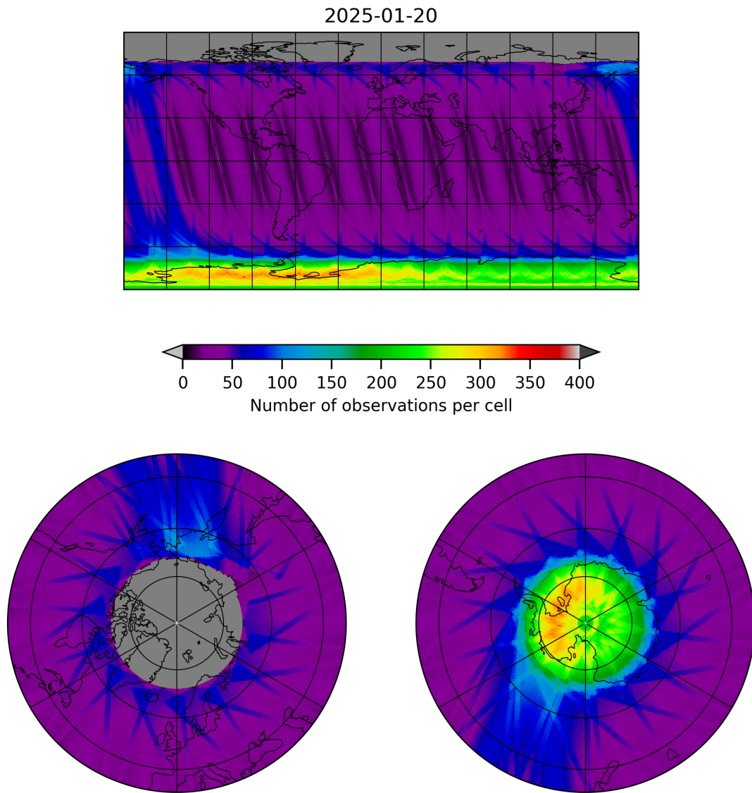
Figure 12: Map of the number of observations for 2025-01-19 to 2025-01-21
