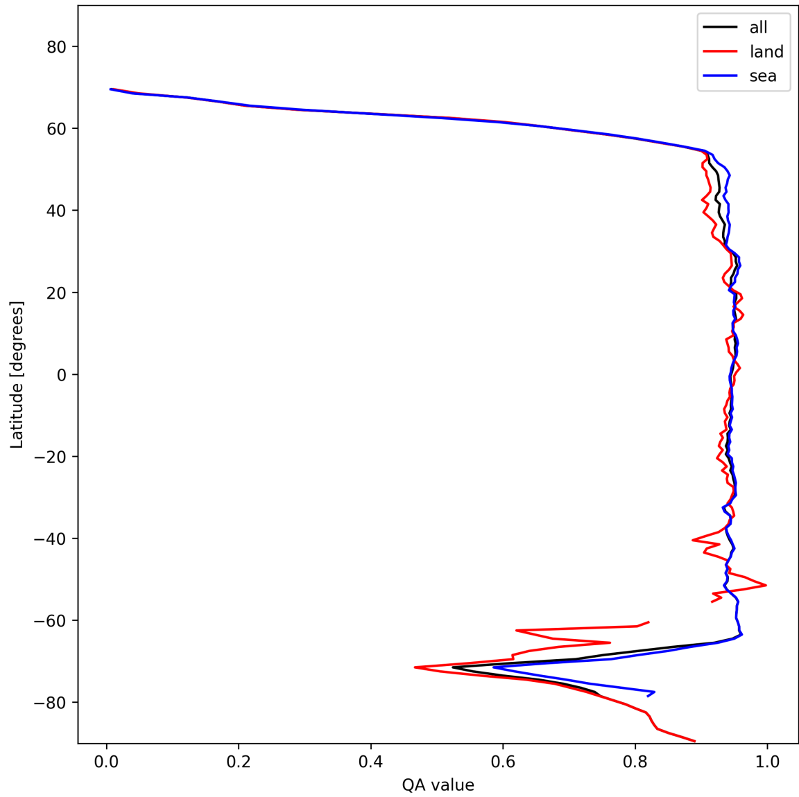
Figure 13: Zonal average of “QA value” for 2025-01-19 to 2025-01-21.
