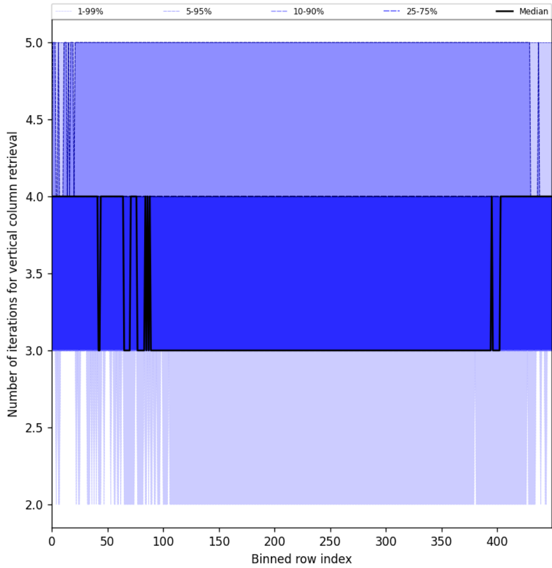
Figure 33: Along track statistics of “Number of iterations for vertical column retrieval” for 2025-01-19 to 2025-01-21
