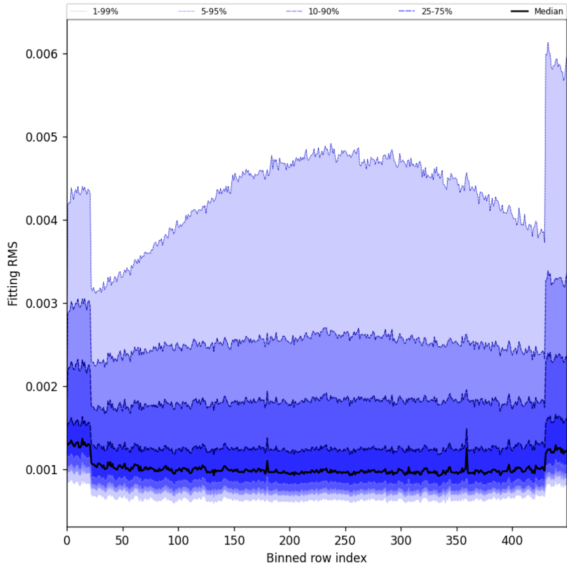
Figure 30: Along track statistics of “Fitting RMS” for 2025-01-19 to 2025-01-21
