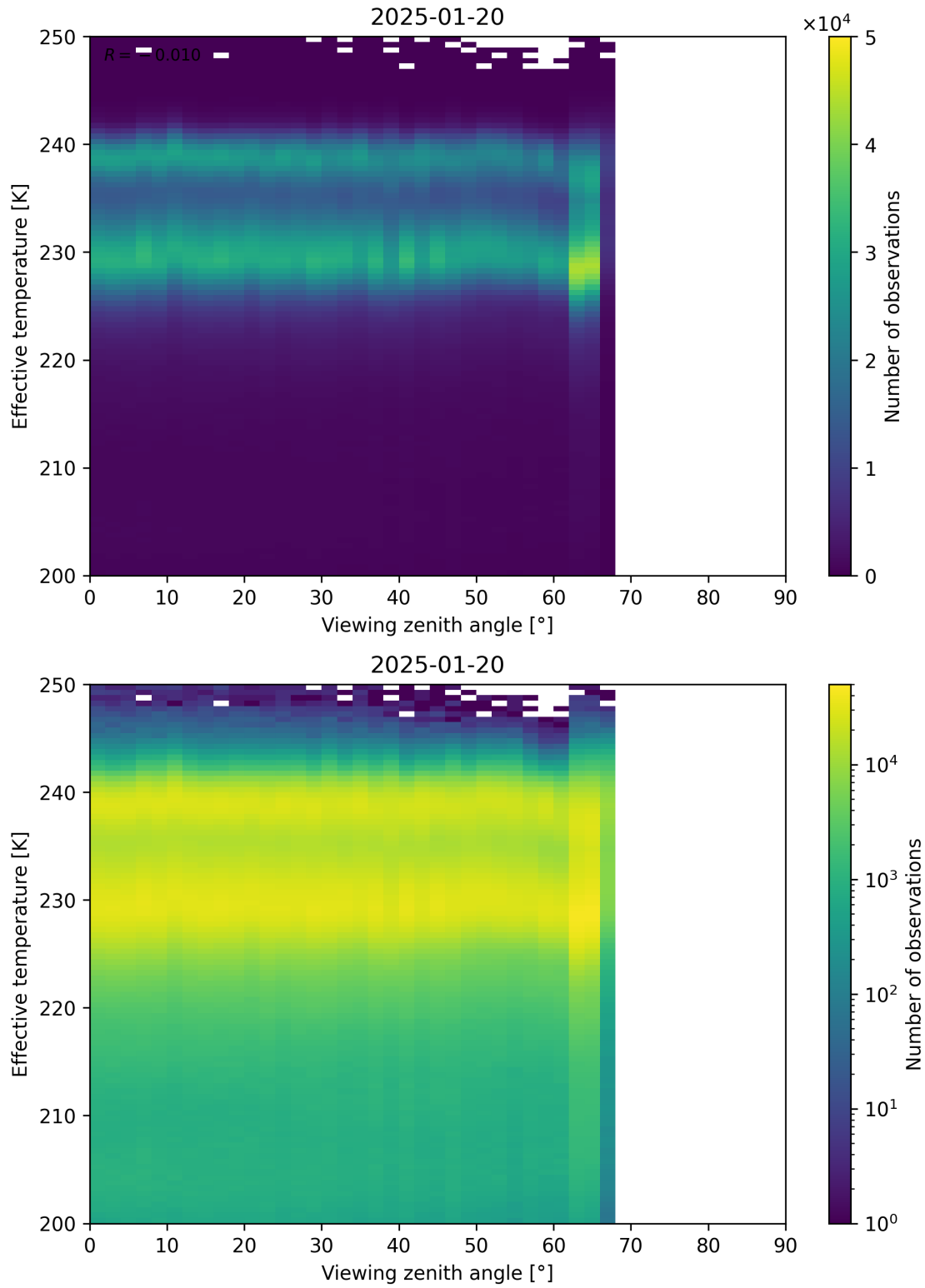
Figure 50: Scatter density plot of “Viewing zenith angle” against “Effective temperature” for 2025-01-19 to 2025-01-21.
