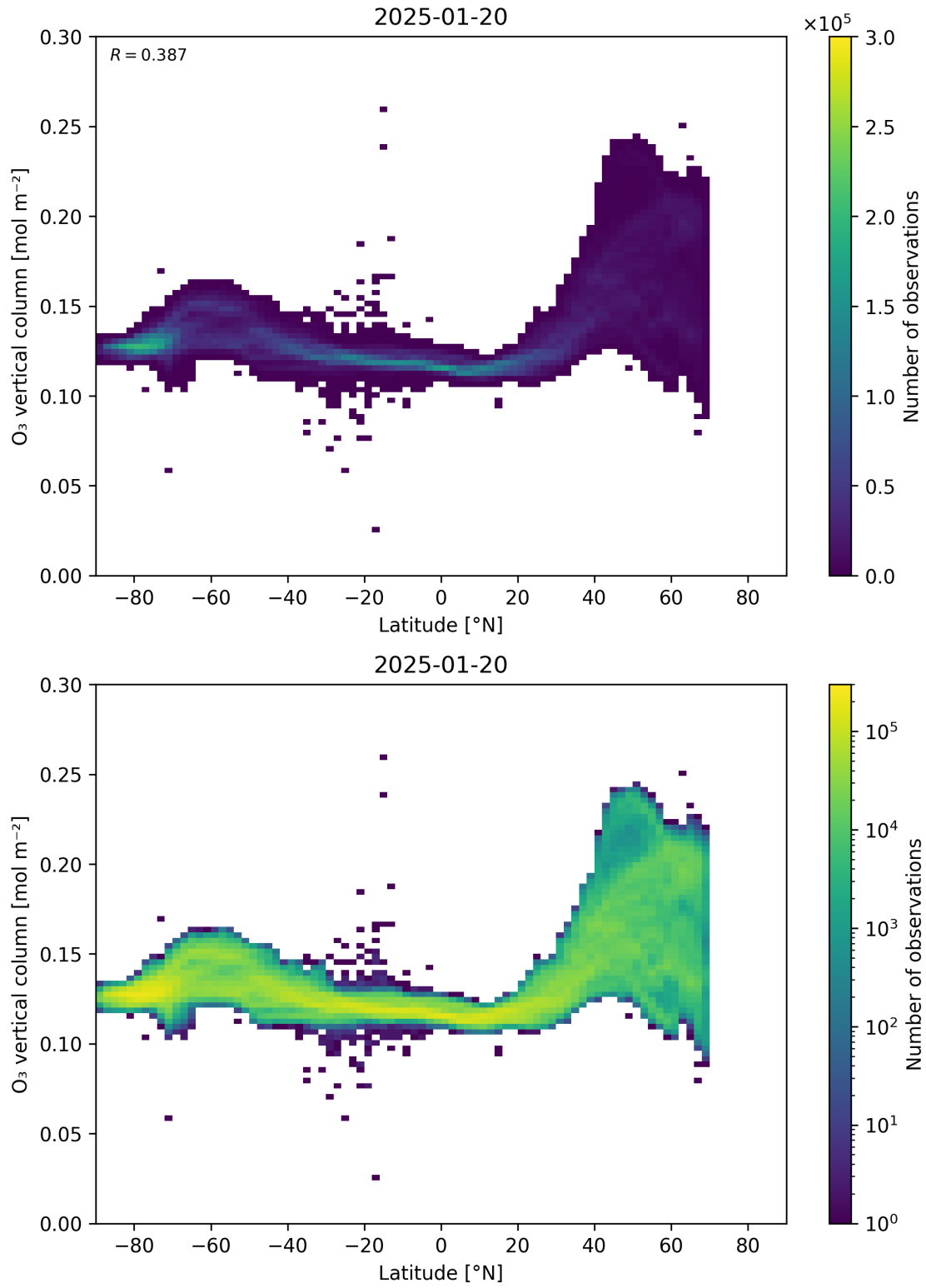
Figure 36: Scatter density plot of “Latitude” against “O 3 vertical column” for 2025-01-19 to 2025-01-21.
