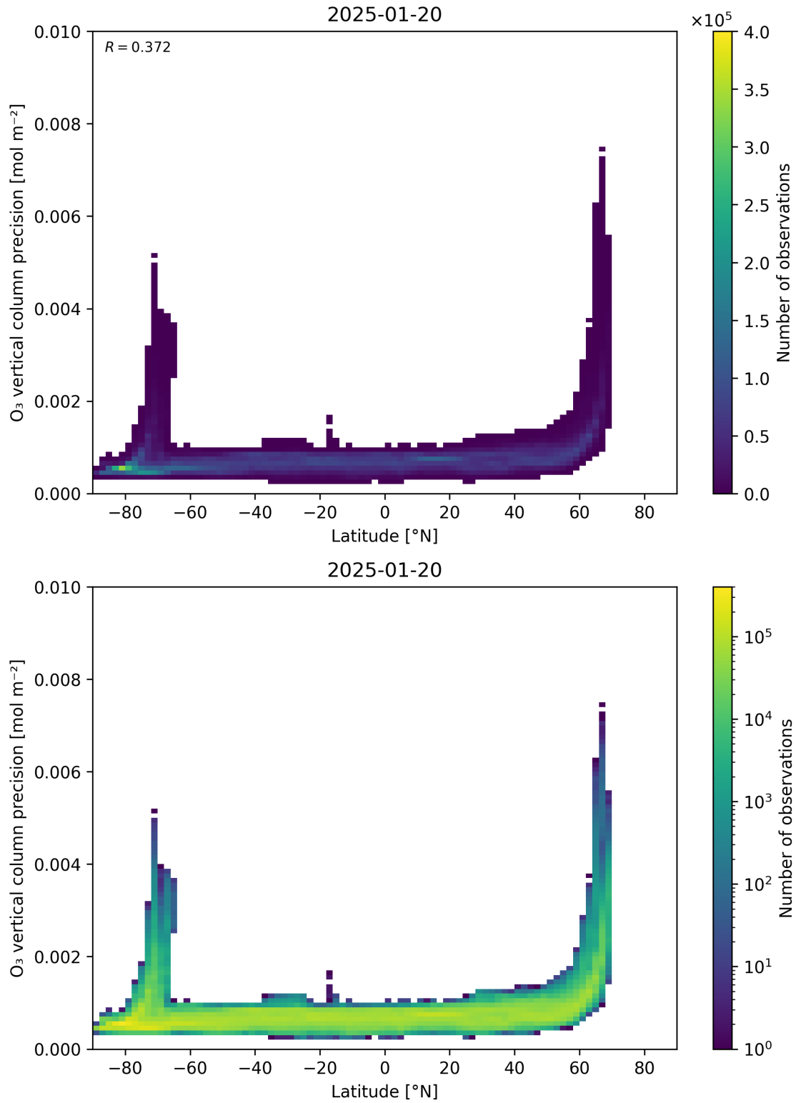
Figure 37: Scatter density plot of “Latitude” against “O 3 vertical column precision” for 2025-01-19 to 2025-01-21.
