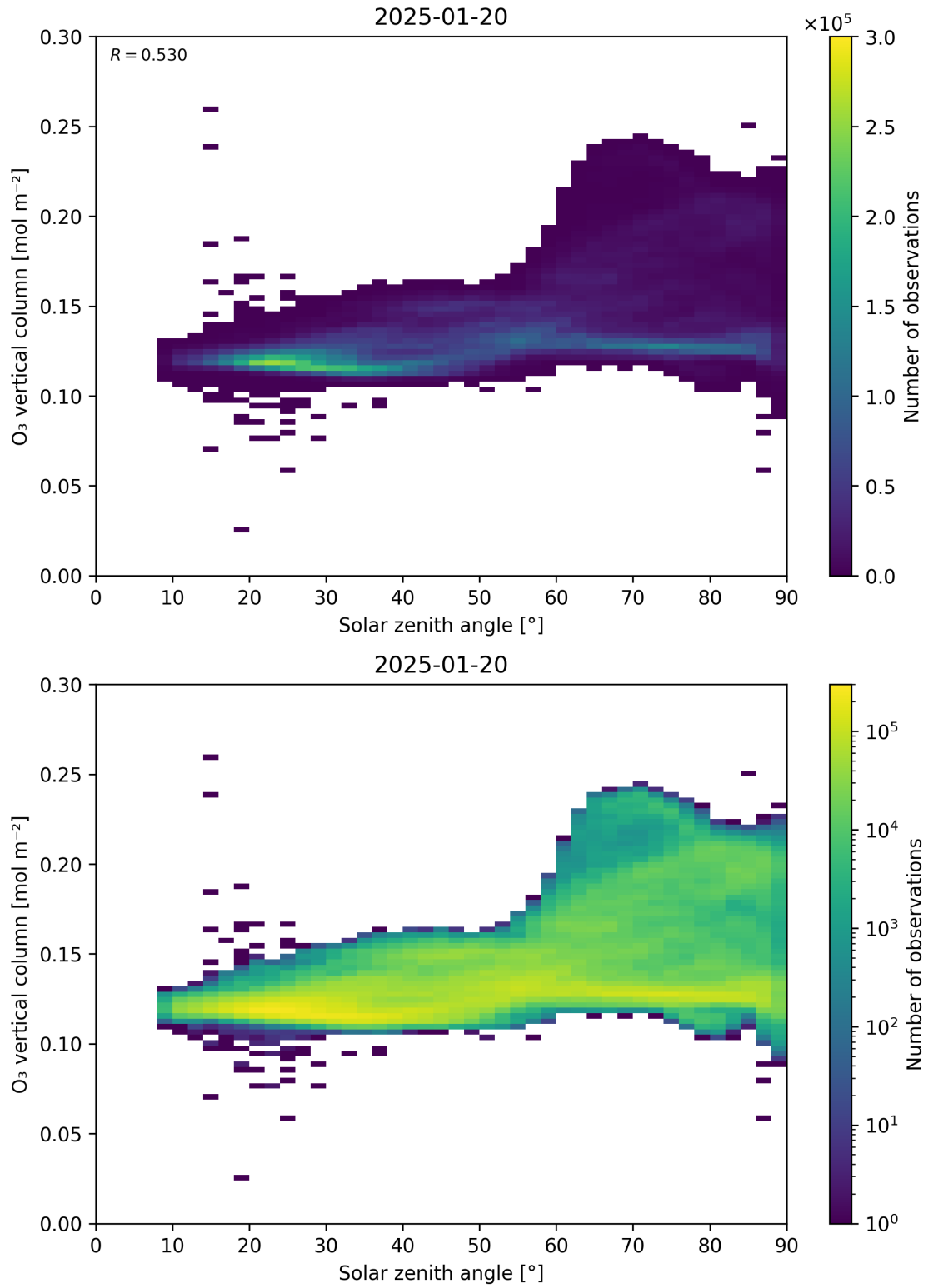
Figure 47: Scatter density plot of “Solar zenith angle” against “O 3 vertical column” for 2025-01-19 to 2025-01-21.
