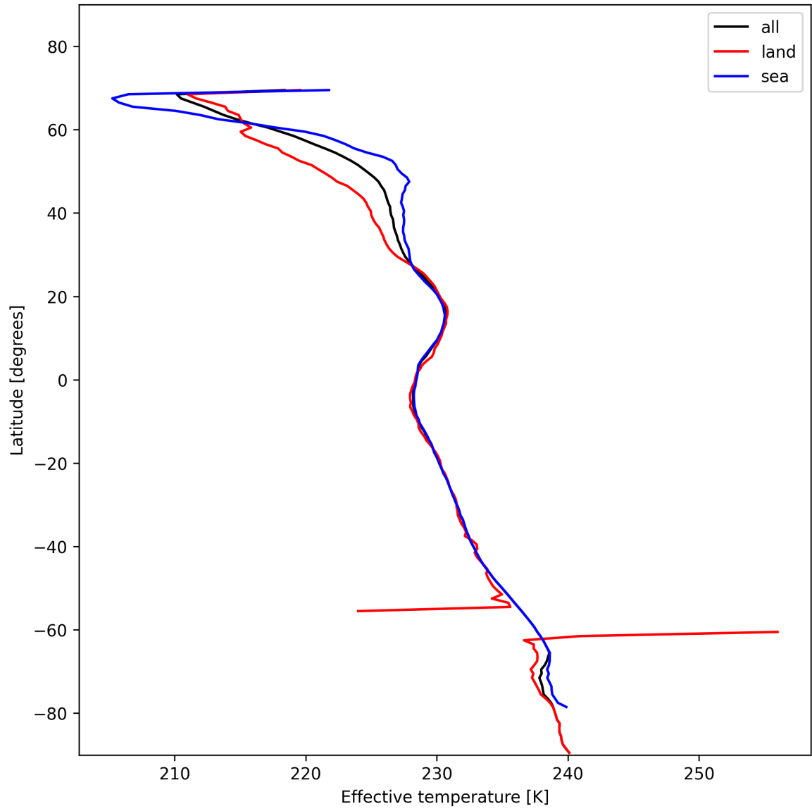
Figure 17: Zonal average of “Effective temperature” for 2025-01-19 to 2025-01-21.
