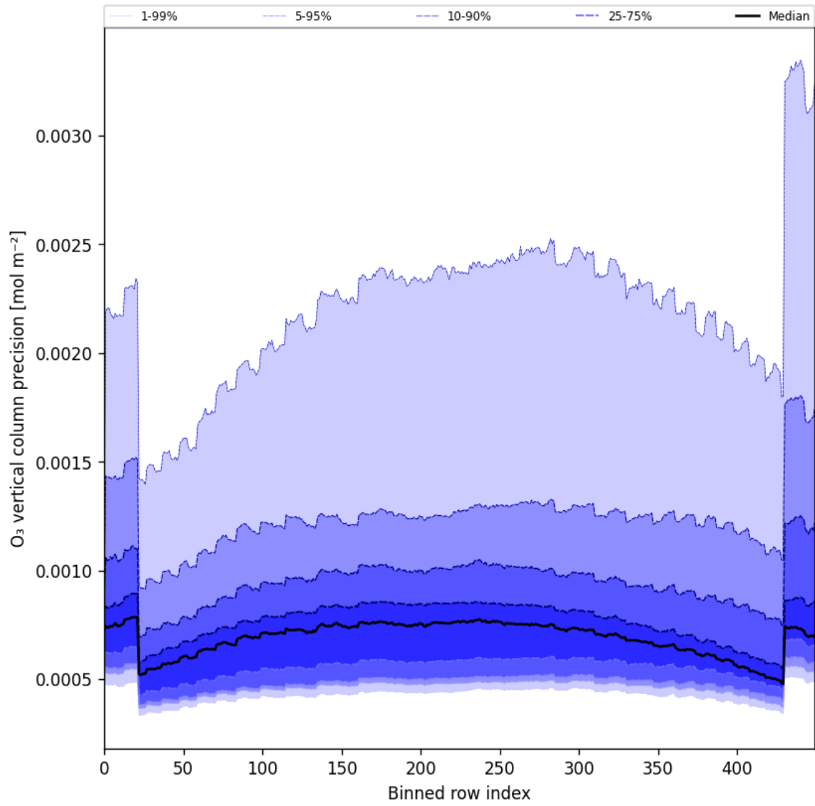
Figure 29: Along track statistics of “O 3 vertical column precision” for 2025-01-19 to 2025-01-21
