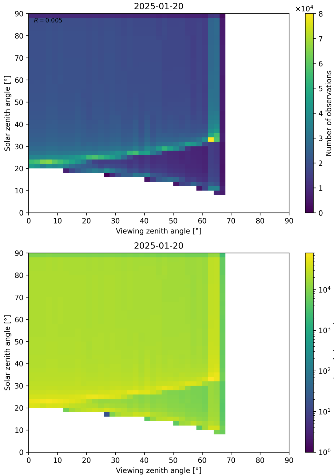
Figure 54: Scatter density plot of “Viewing zenith angle” against “Solar zenith angle” for 2025-01-19 to 2025-01-21.
