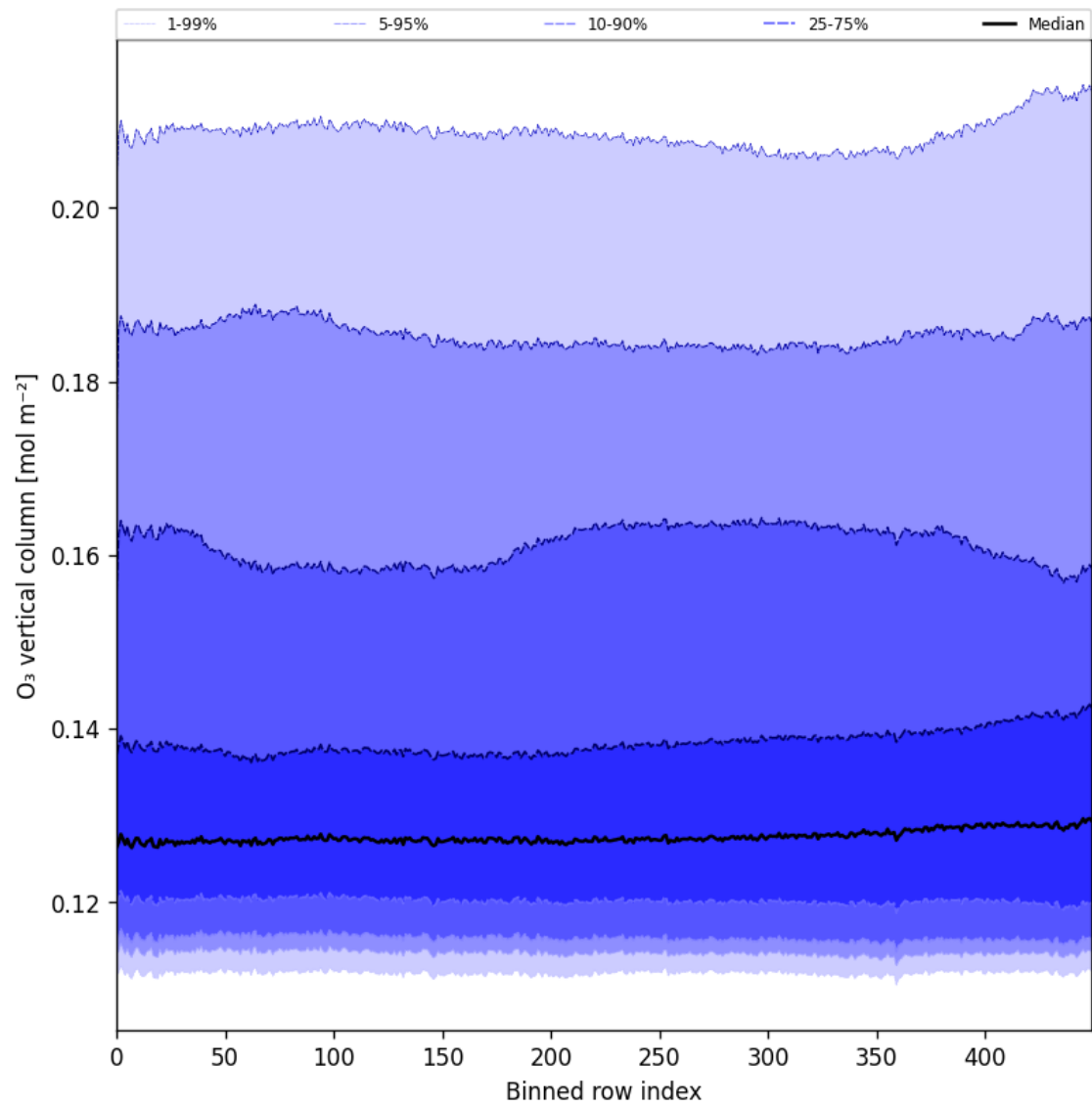
Figure 28: Along track statistics of “O 3 vertical column” for 2025-01-19 to 2025-01-21
