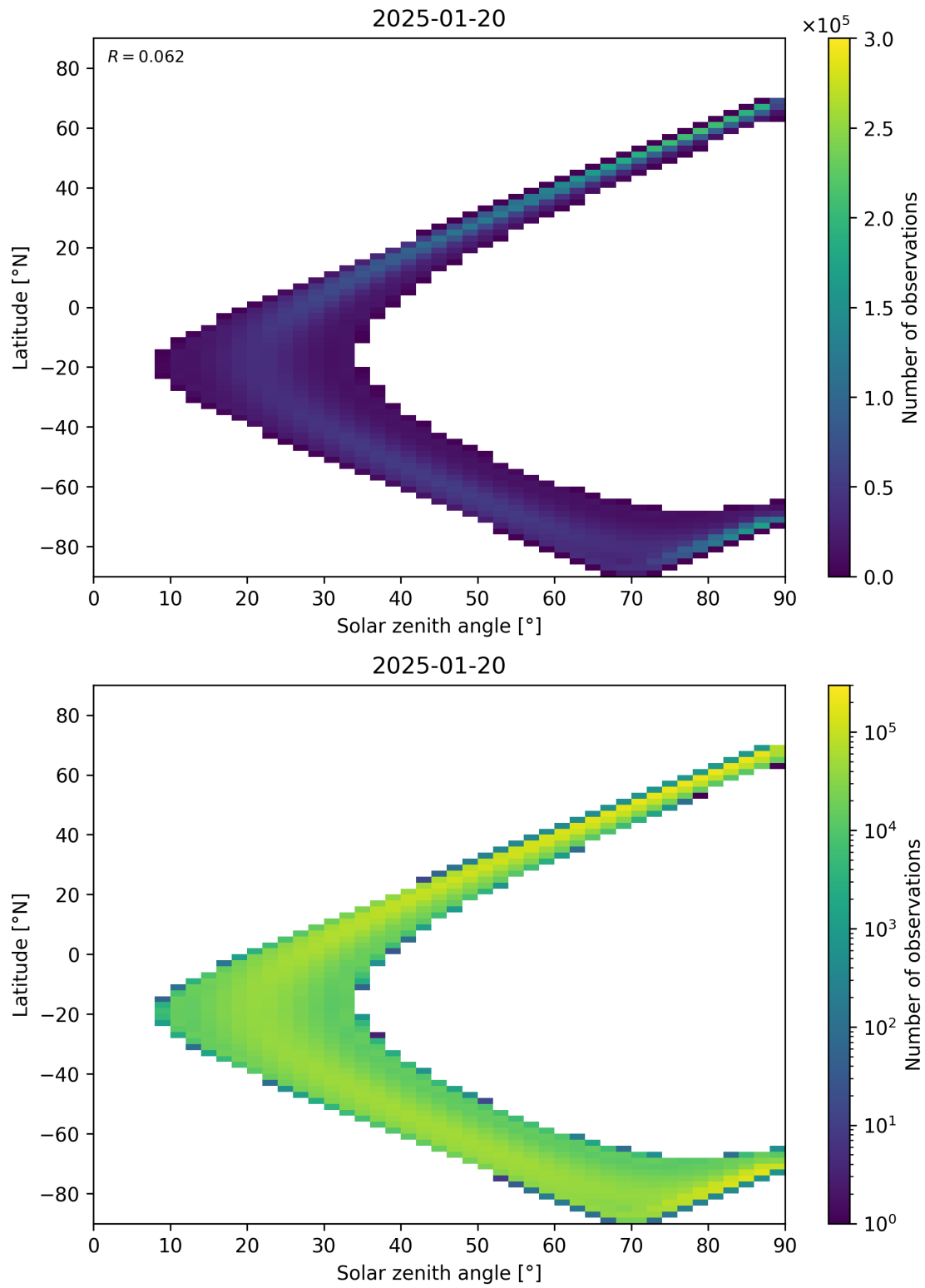
Figure 44: Scatter density plot of “Solar zenith angle” against “Latitude” for 2025-01-19 to 2025-01-21.
