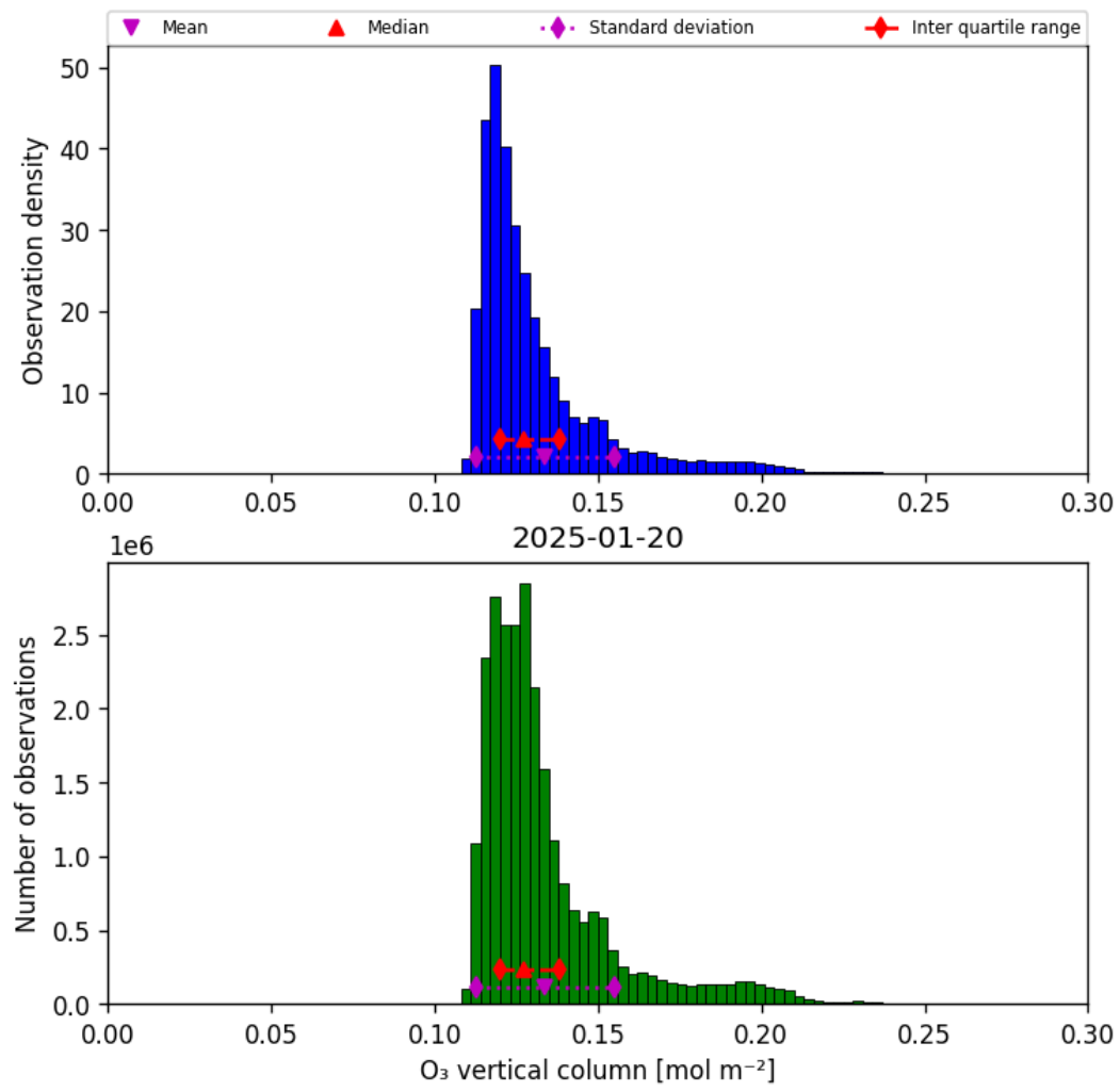
Figure 21: Histogram of “O 3 vertical column” for 2025-01-19 to 2025-01-21
