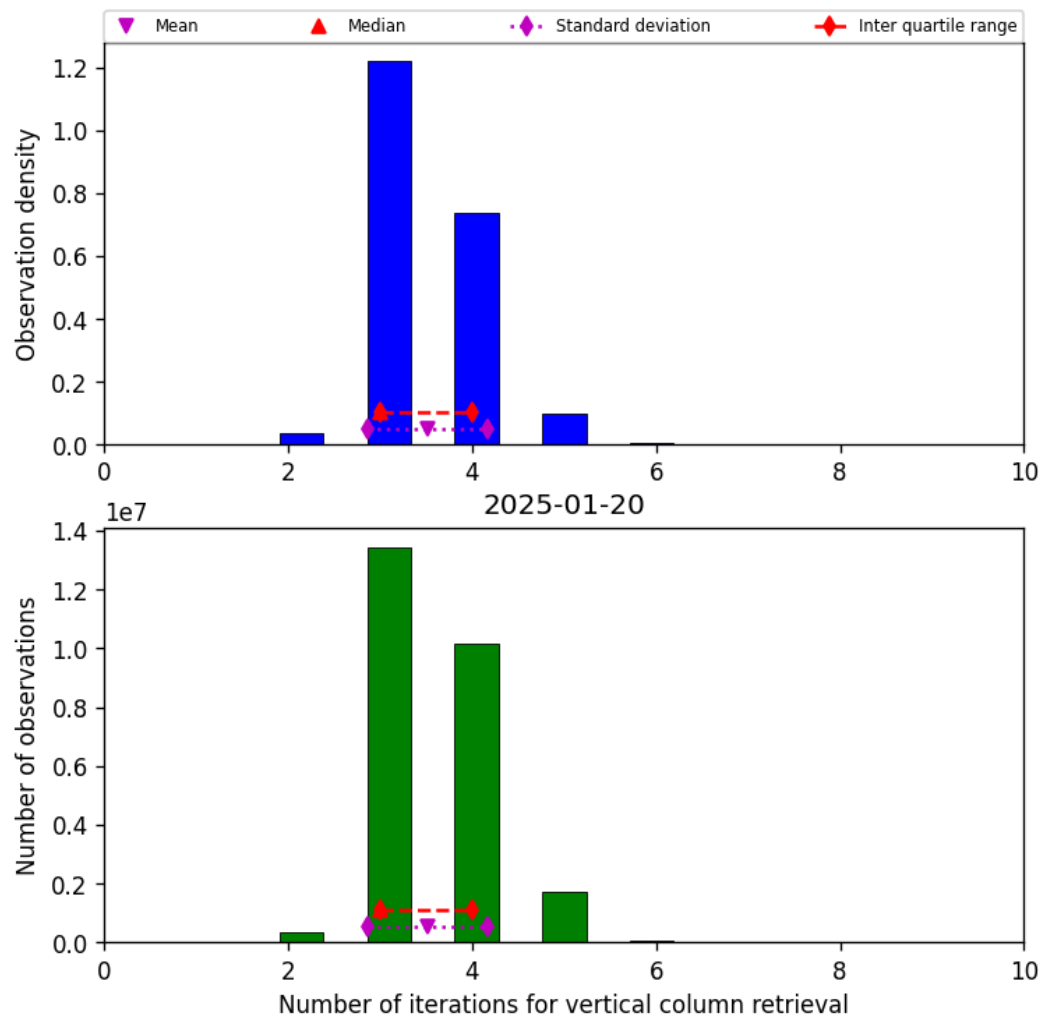
Figure 26: Histogram of “Number of iterations for vertical column retrieval” for 2025-01-19 to 2025-01-21
