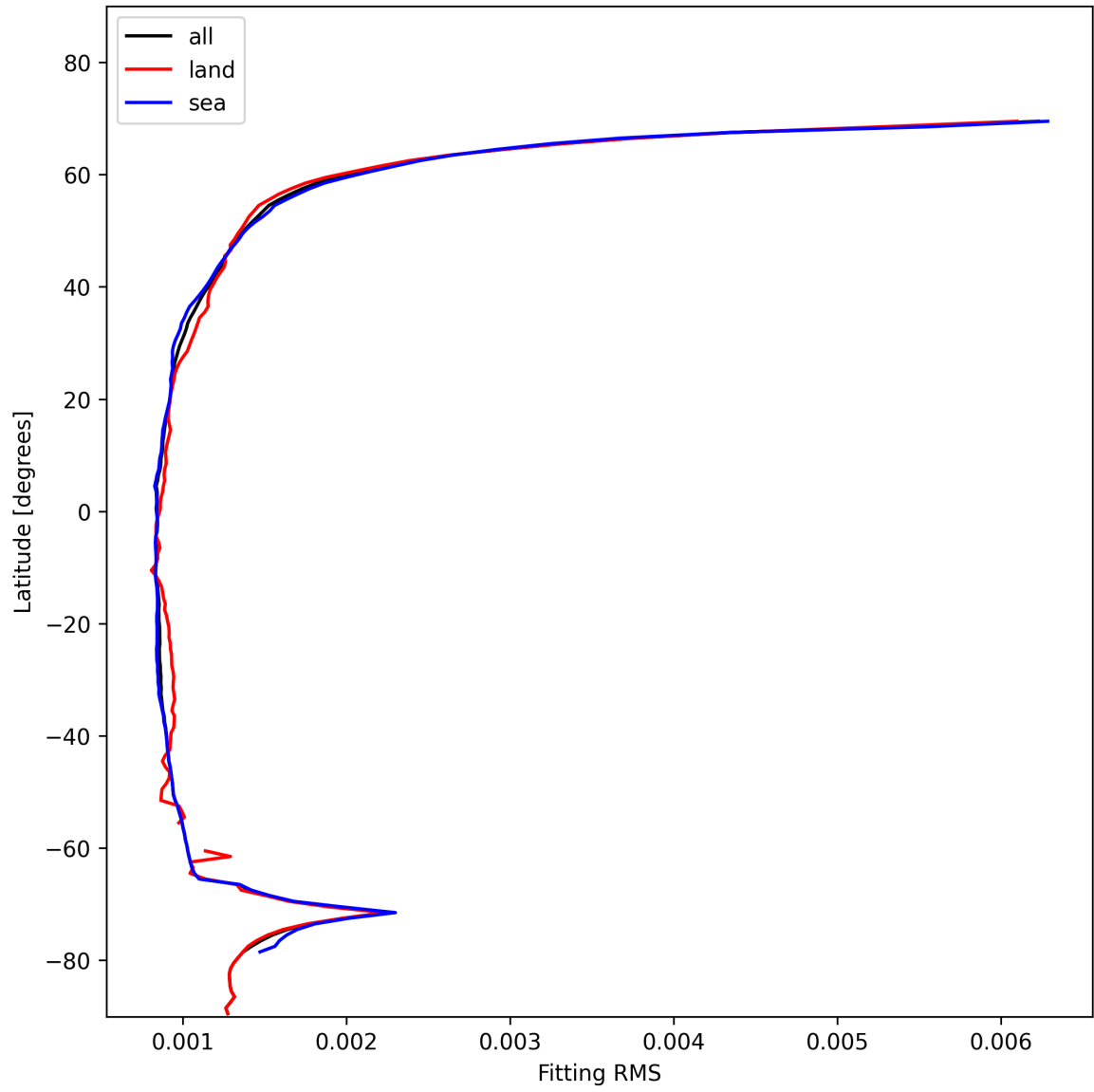
Figure 16: Zonal average of “Fitting RMS” for 2025-01-19 to 2025-01-21.
