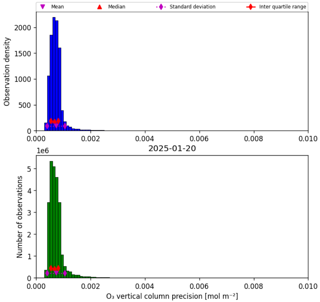
Figure 22: Histogram of “O 3 vertical column precision” for 2025-01-19 to 2025-01-21
