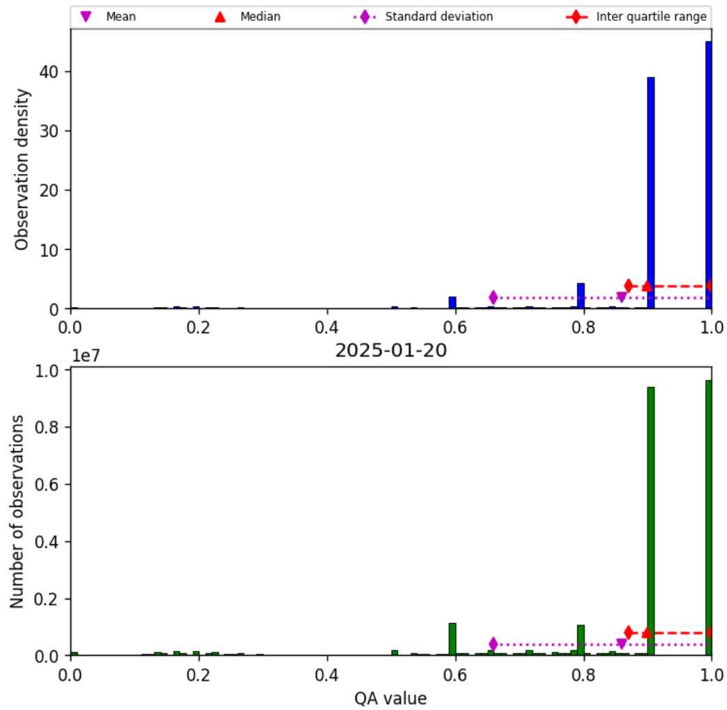
Figure 20: Histogram of “QA value” for 2025-01-19 to 2025-01-21
