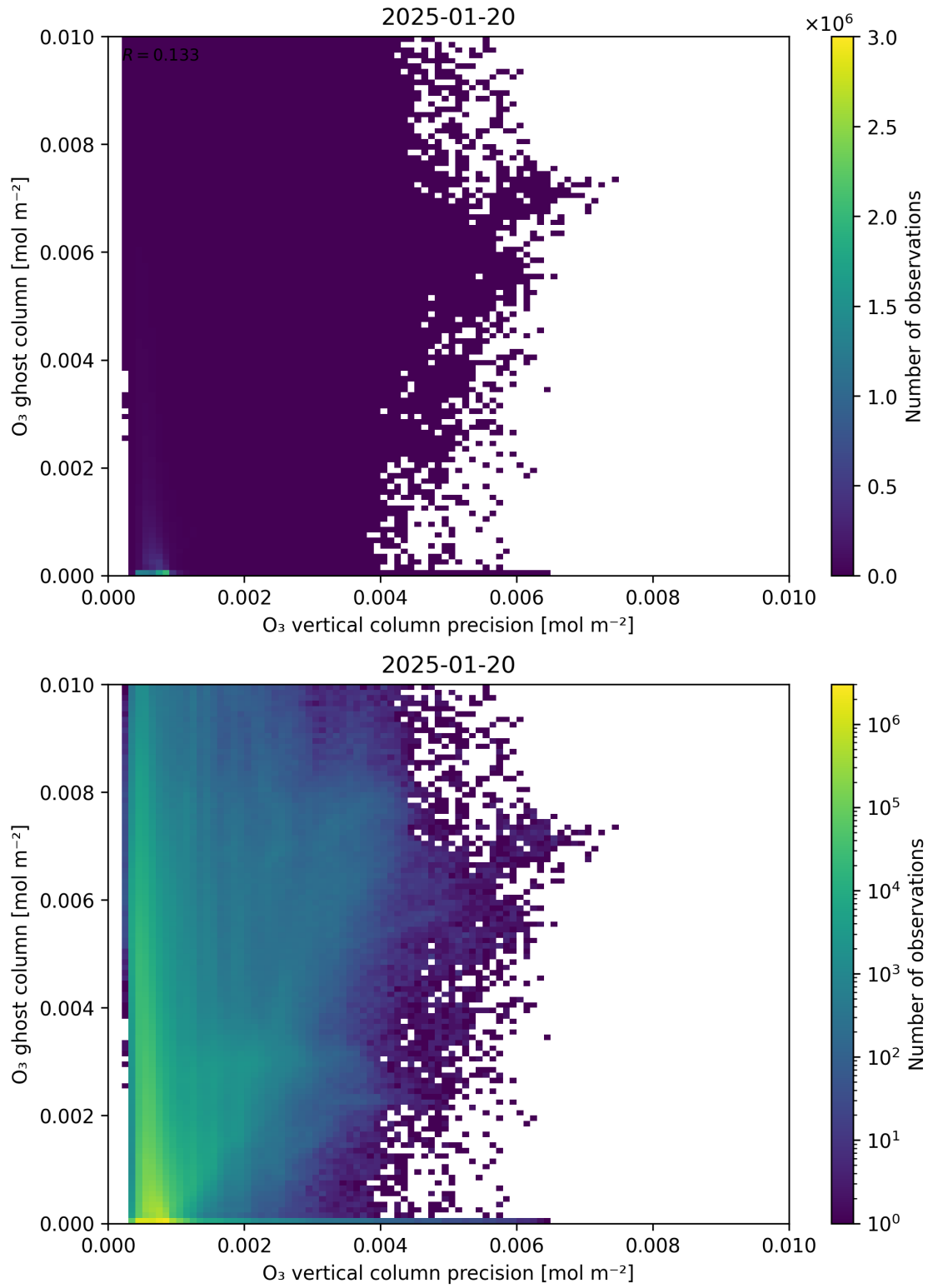
Figure 43: Scatter density plot of “O 3 vertical column precision” against “O 3 ghost column” for 2025-01-19 to 2025-01-21.
