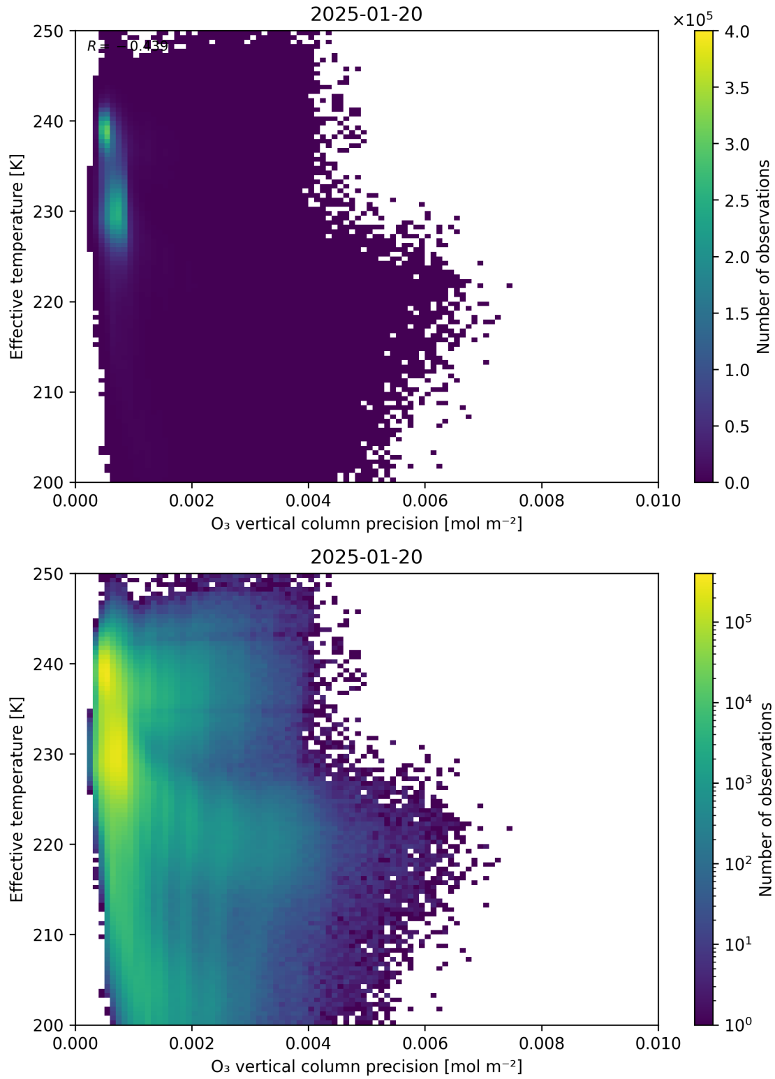
Figure 42: Scatter density plot of “O 3 vertical column precision” against “Effective temperature” for 2025-01-19 to 2025-01-21.
