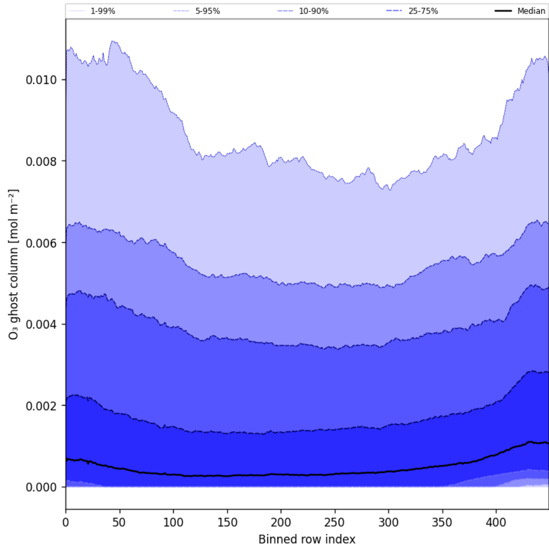
Figure 32: Along track statistics of “O 3 ghost column” for 2025-01-19 to 2025-01-21
