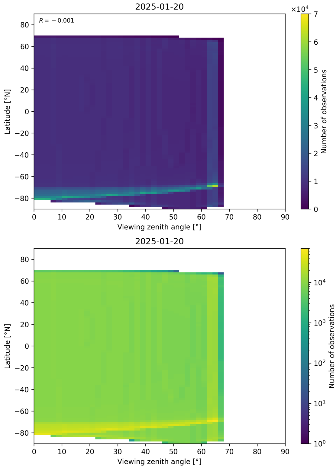
Figure 49: Scatter density plot of “Viewing zenith angle” against “Latitude” for 2025-01-19 to 2025-01-21.
