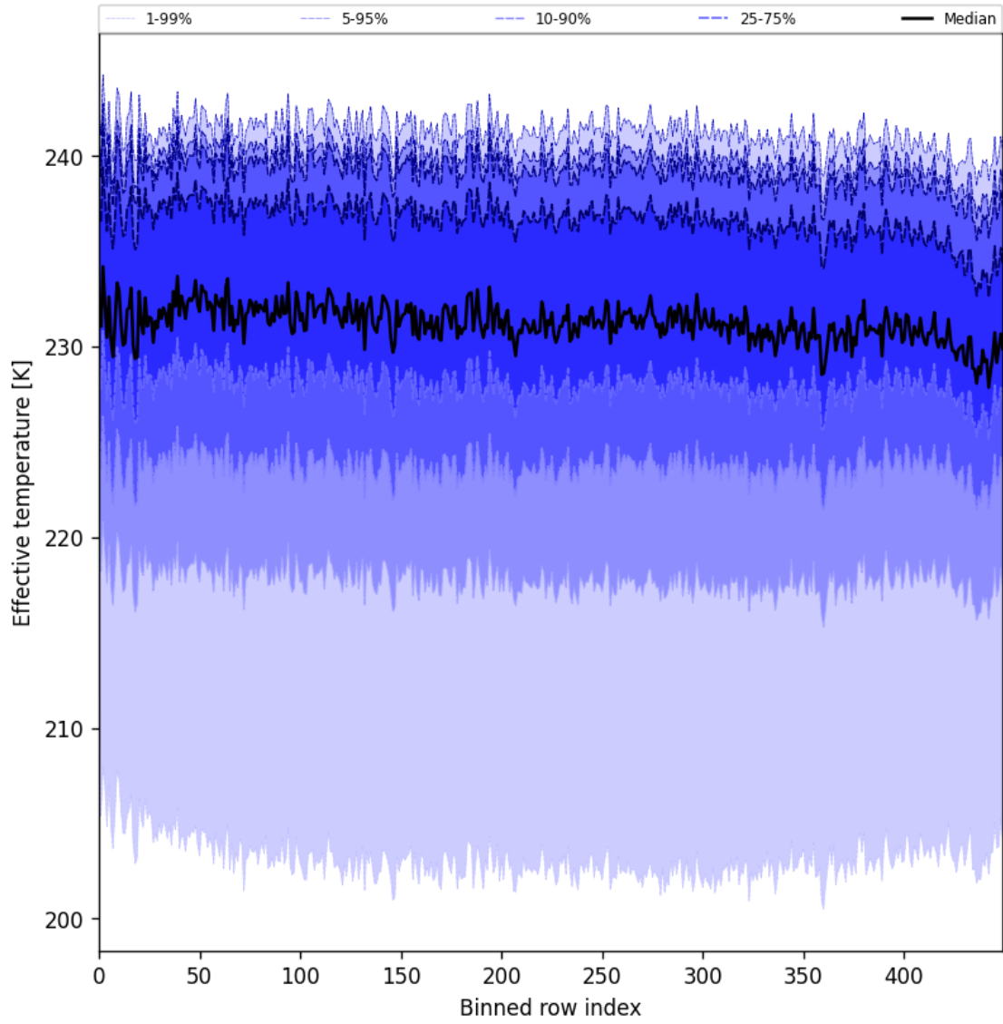
Figure 31: Along track statistics of "Effective temperature" for 2025-01-19 to 2025-01-21
