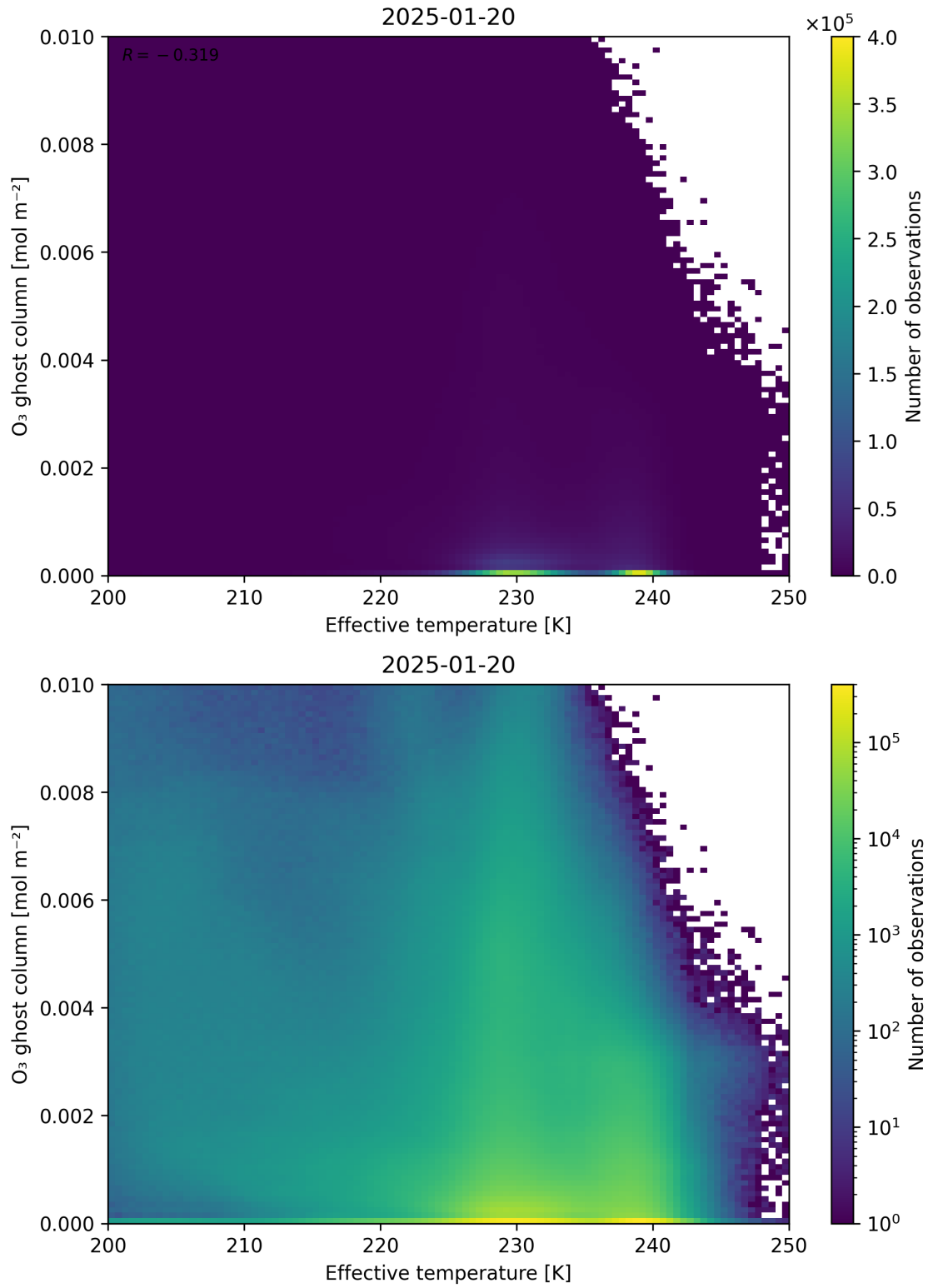
Figure 38: Scatter density plot of “Effective temperature” against “O 3 ghost column” for 2025-01-19 to 2025-01-21.
