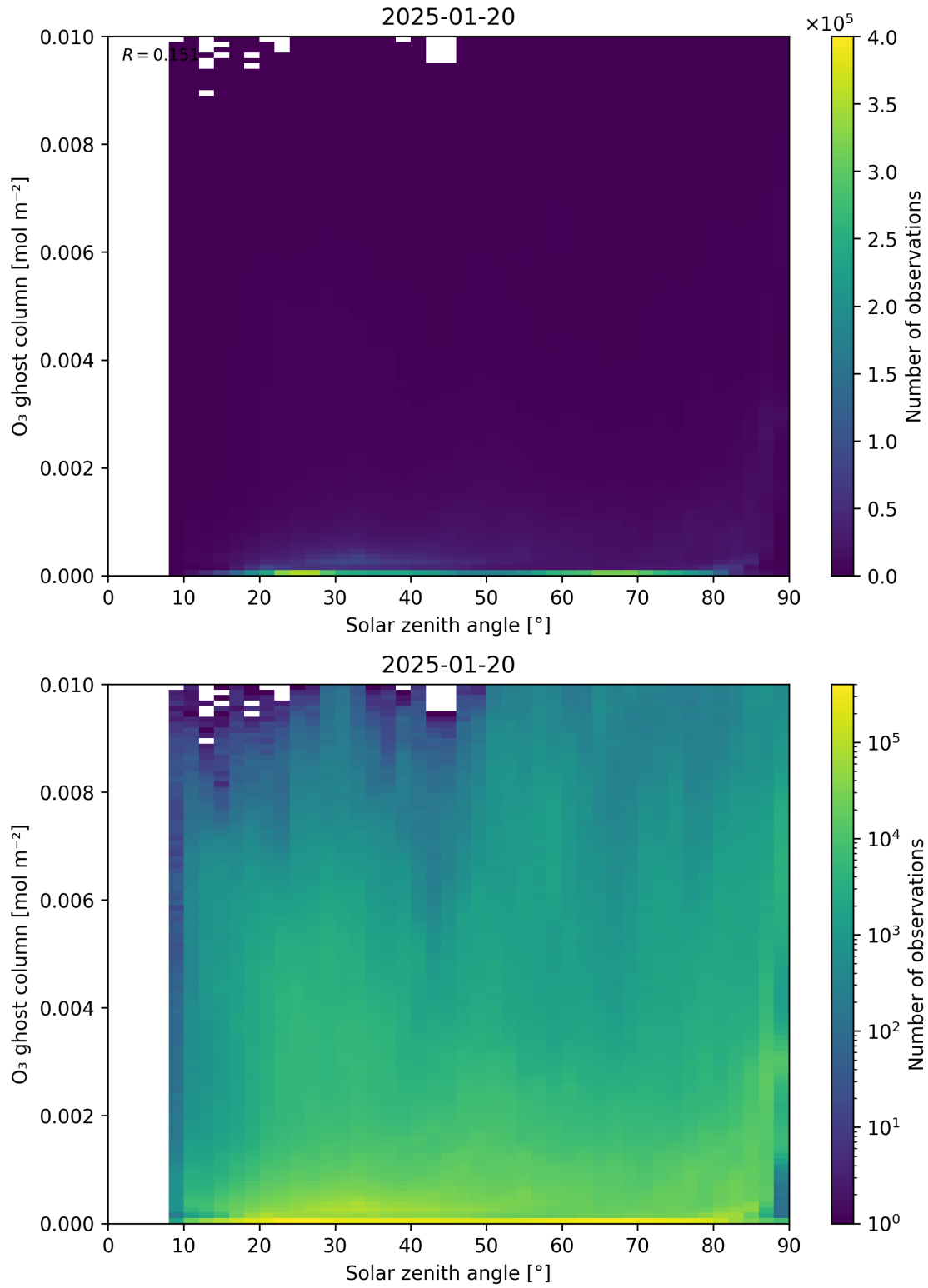
Figure 46: Scatter density plot of “Solar zenith angle” against “O 3 ghost column” for 2025-01-19 to 2025-01-21.
