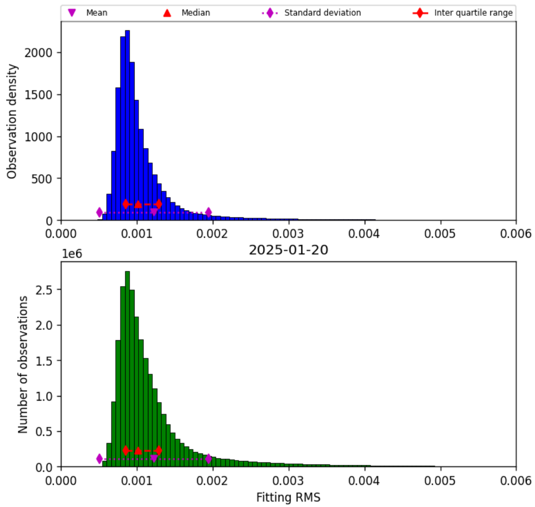
Figure 23: Histogram of “Fitting RMS” for 2025-01-19 to 2025-01-21
