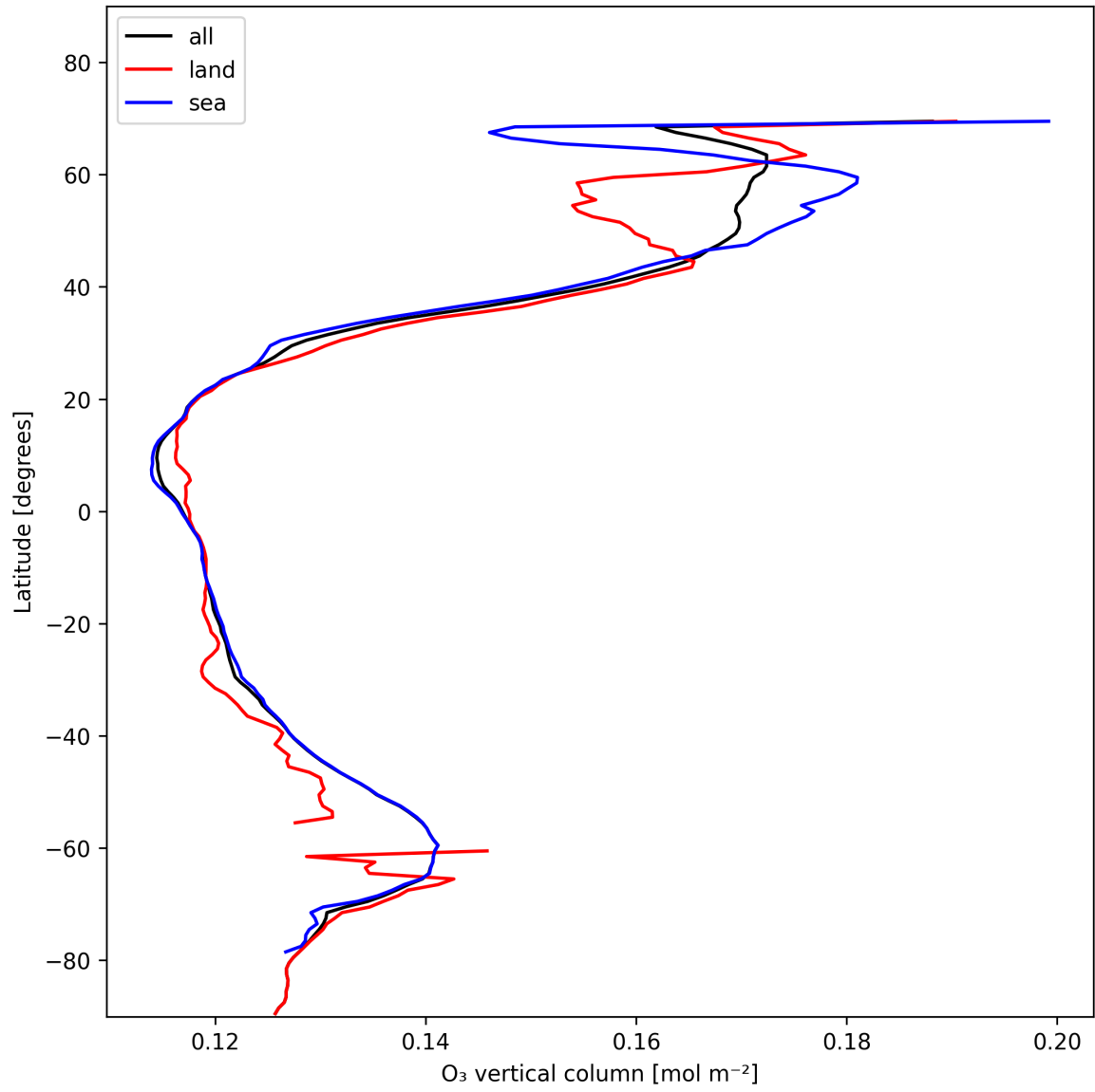
Figure 14: Zonal average of “O 3 vertical column” for 2025-01-19 to 2025-01-21.
