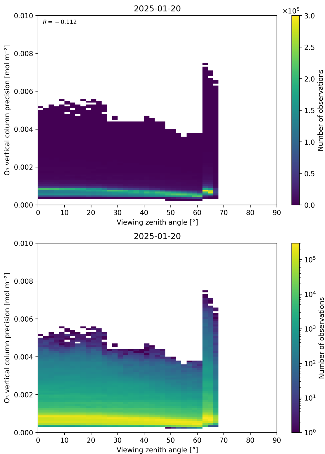
Figure 53: Scatter density plot of “Viewing zenith angle” against “O 3 vertical column precision” for 2025-01-19 to 2025-01-21.
