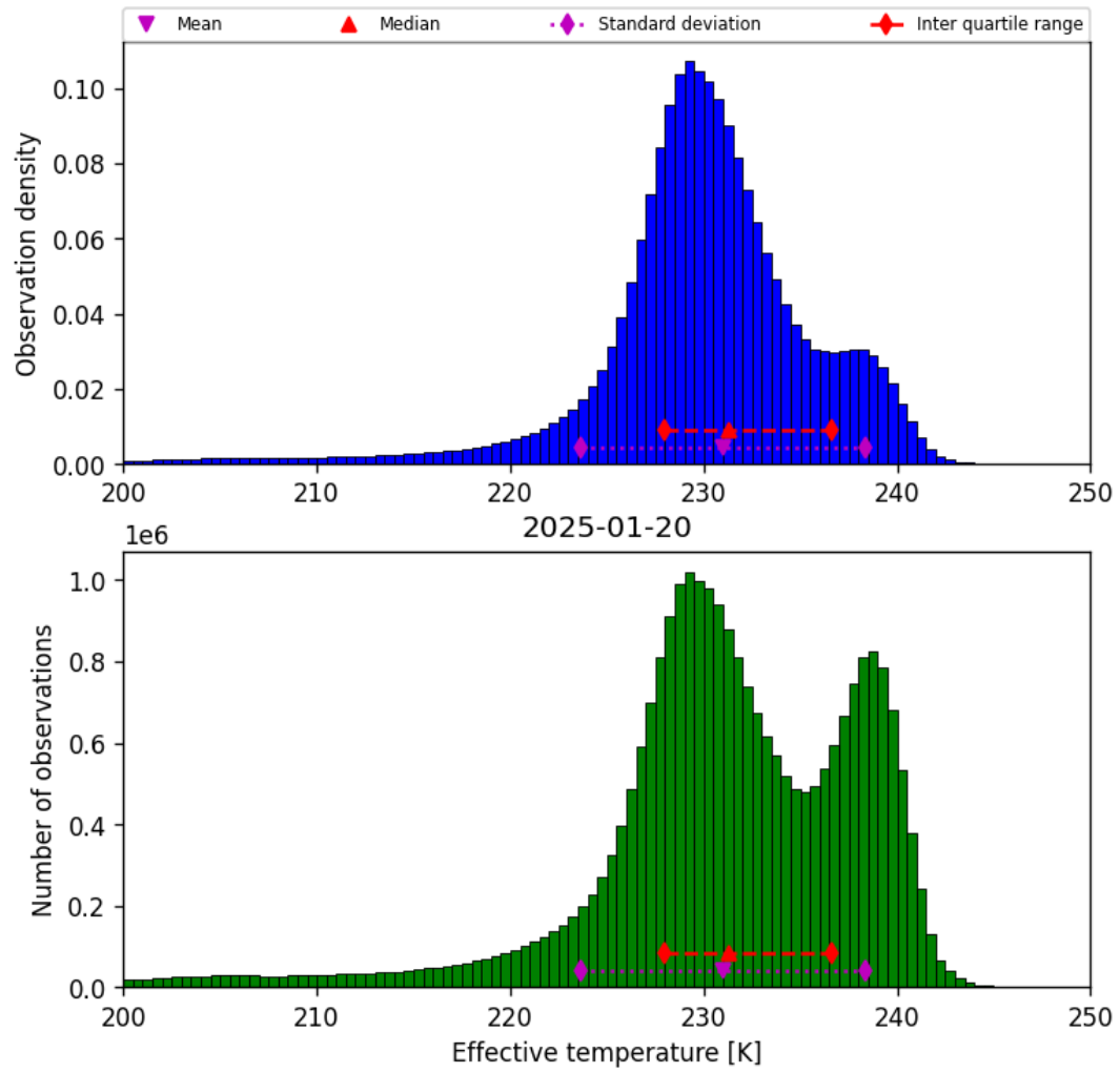
Figure 24: Histogram of “Effective temperature” for 2025-01-19 to 2025-01-21
