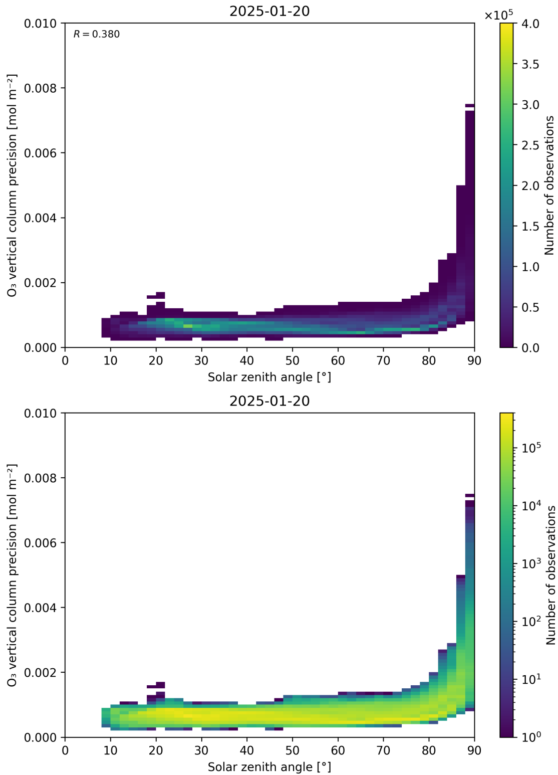
Figure 48: Scatter density plot of “Solar zenith angle” against “O 3 vertical column precision” for 2025-01-19 to 2025-01-21.
