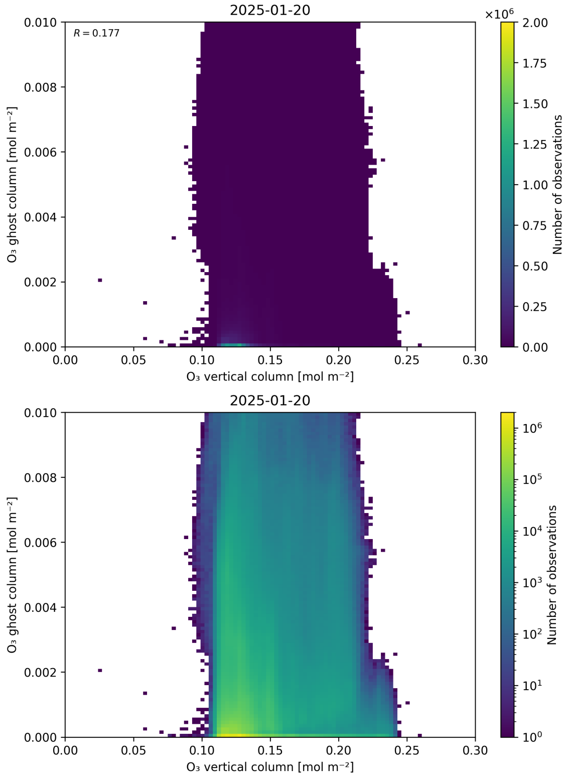
Figure 40: Scatter density plot of “O 3 vertical column” against “O 3 ghost column” for 2025-01-19 to 2025-01-21.
