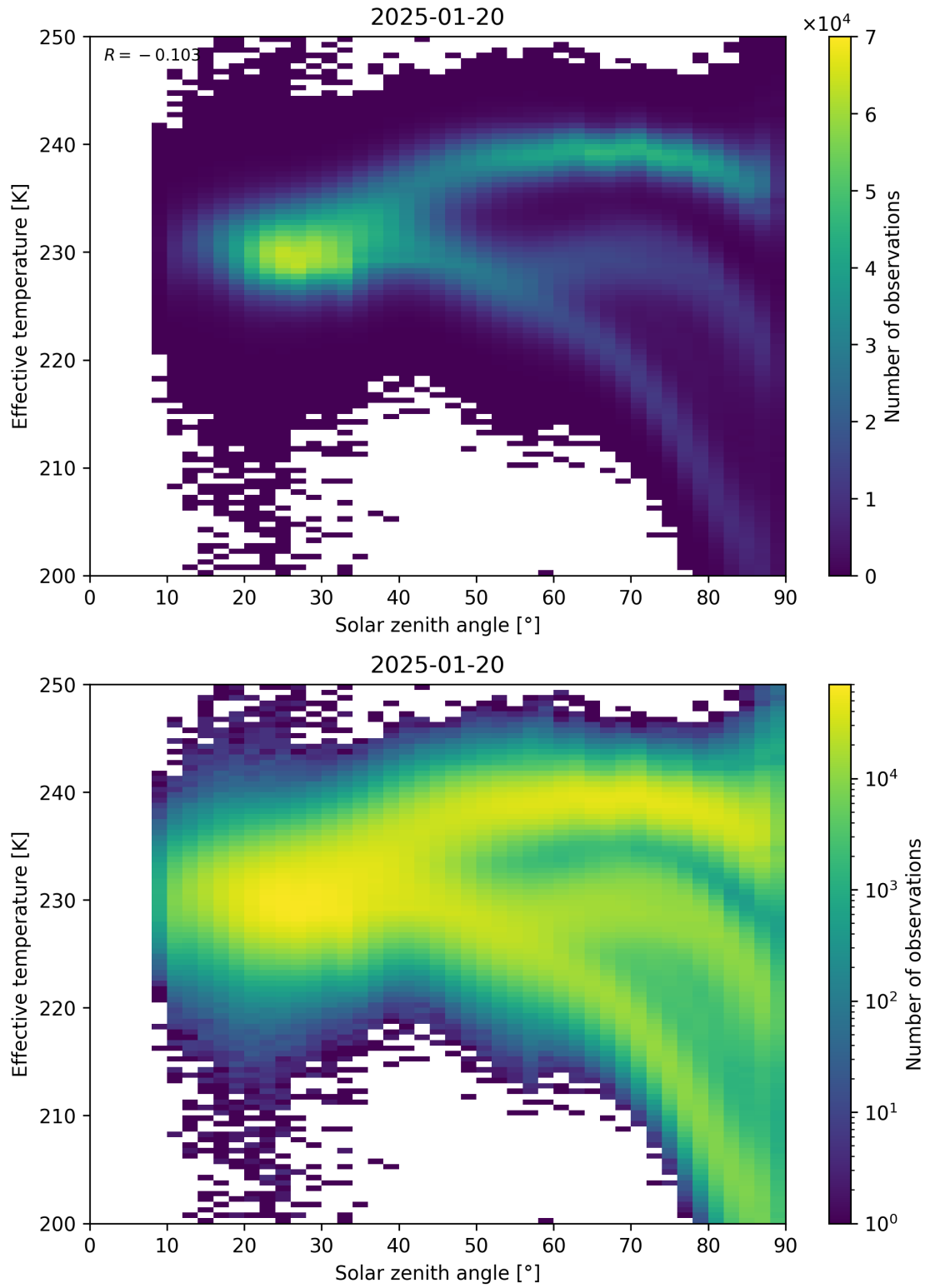
Figure 45: Scatter density plot of “Solar zenith angle” against “Effective temperature” for 2025-01-19 to 2025-01-21.
