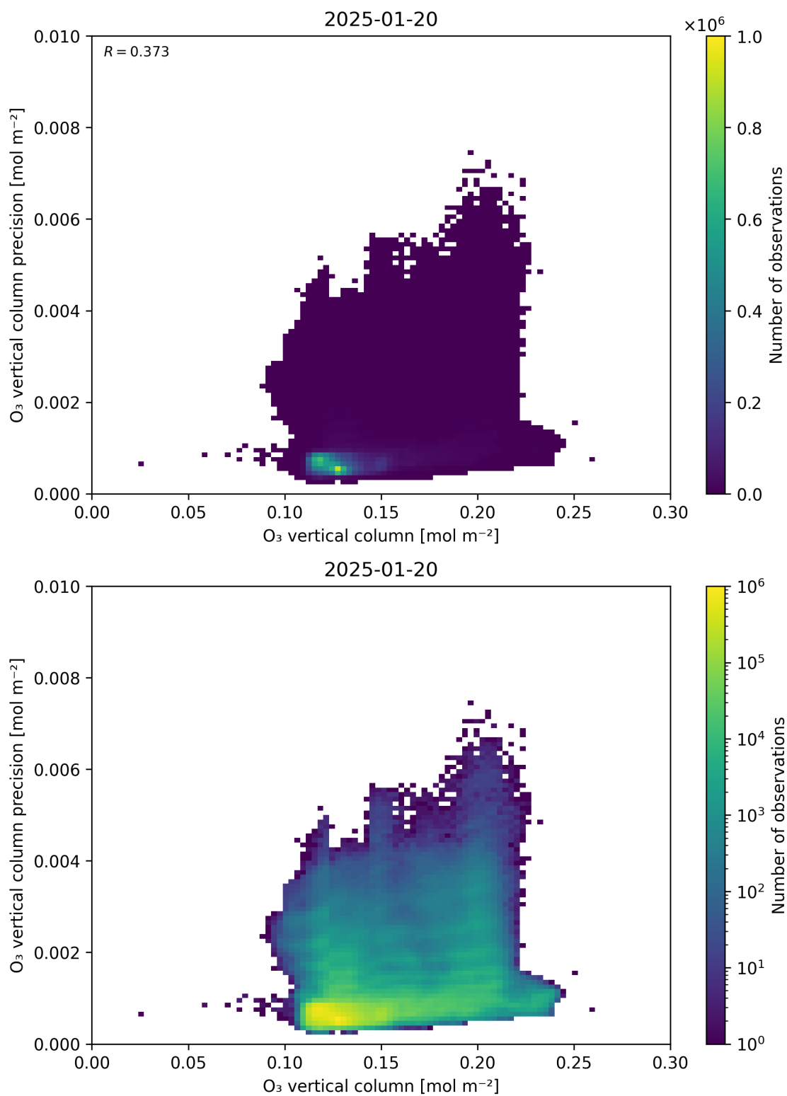
Figure 41: Scatter density plot of “O 3 vertical column” against “O 3 vertical column precision” for 2025-01-19 to 2025-01-21.
