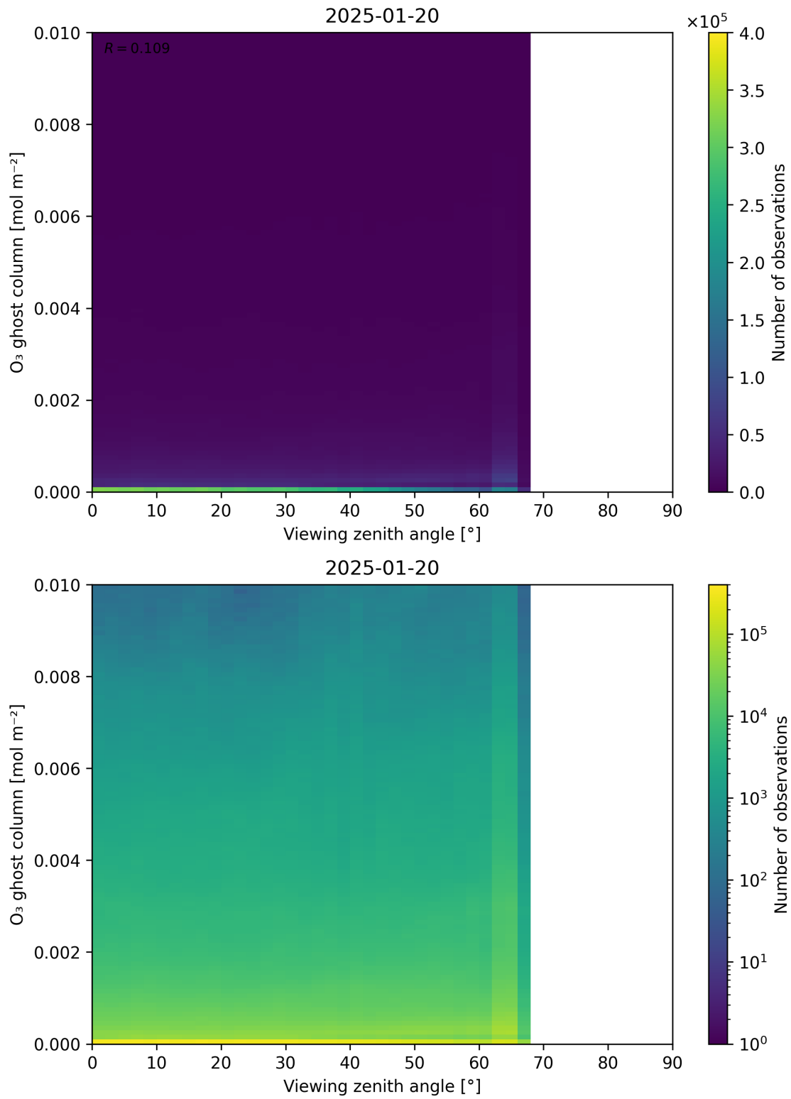
Figure 51: Scatter density plot of “Viewing zenith angle” against “O 3 ghost column” for 2025-01-19 to 2025-01-21.
