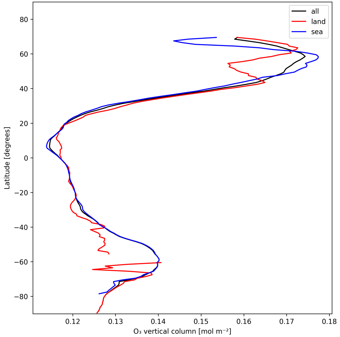
Figure 14: Zonal average of “O 3 vertical column” for 2025-01-20 to 2025-01-22.
