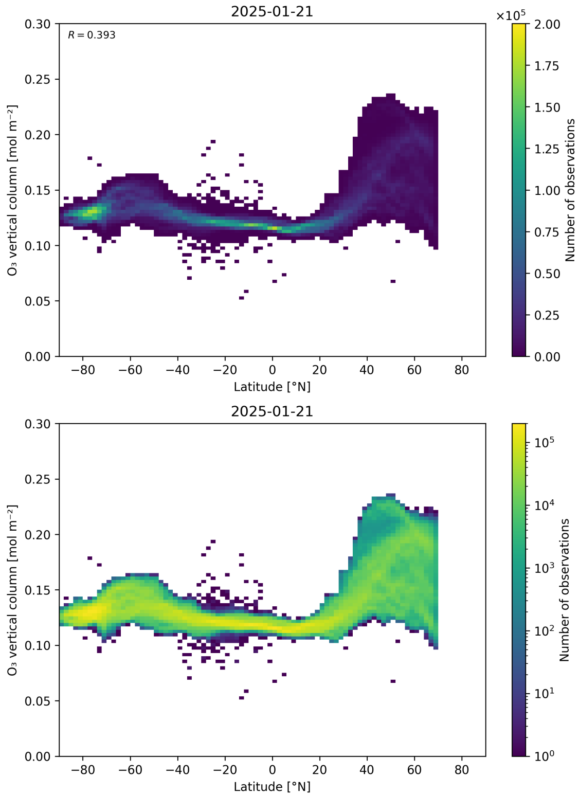
Figure 36: Scatter density plot of “Latitude” against “O 3 vertical column” for 2025-01-20 to 2025-01-22.
