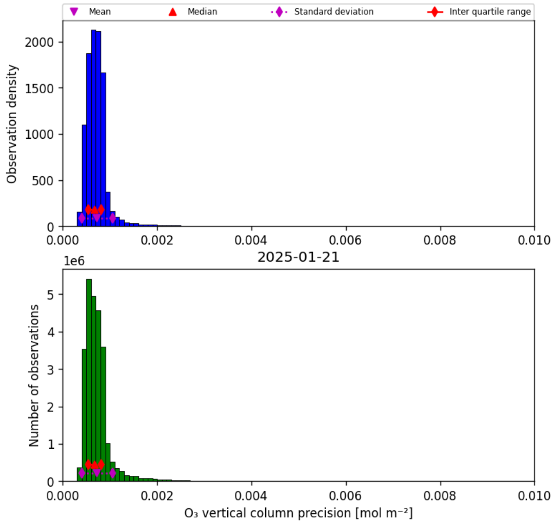
Figure 22: Histogram of “O 3 vertical column precision” for 2025-01-20 to 2025-01-22
