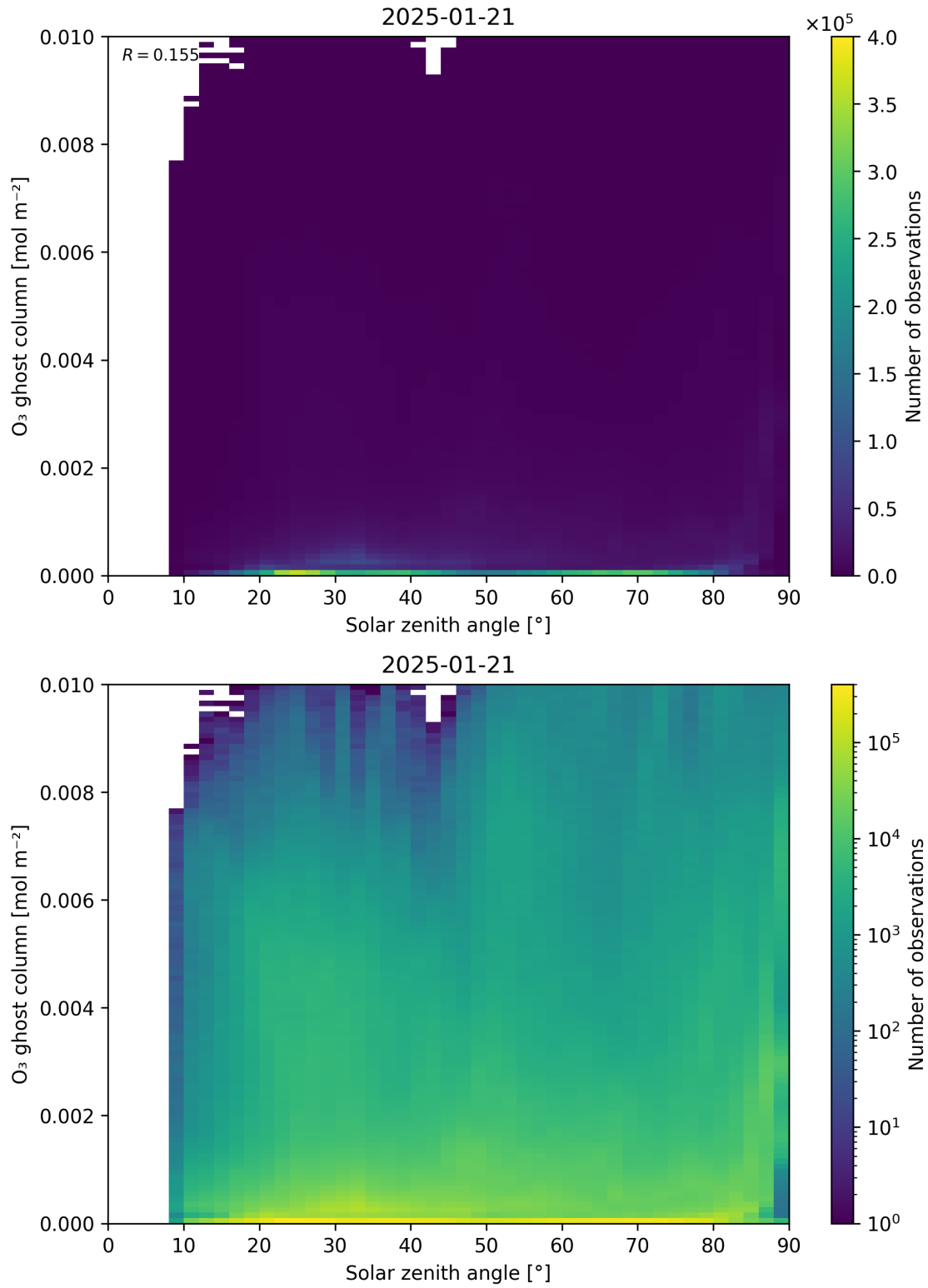
Figure 46: Scatter density plot of “Solar zenith angle” against “O 3 ghost column” for 2025-01-20 to 2025-01-22.
