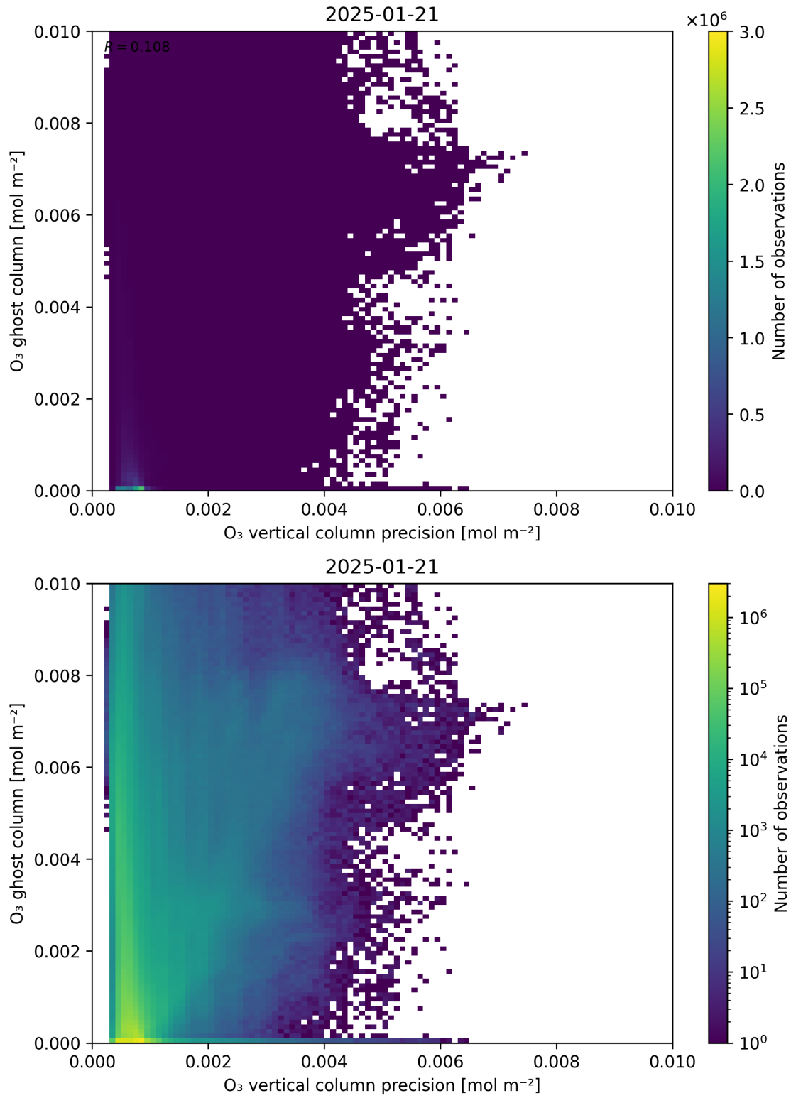
Figure 43: Scatter density plot of “ O_3 vertical column precision” against “ O_3 ghost column” for 2025-01-20 to 2025-01-22.
