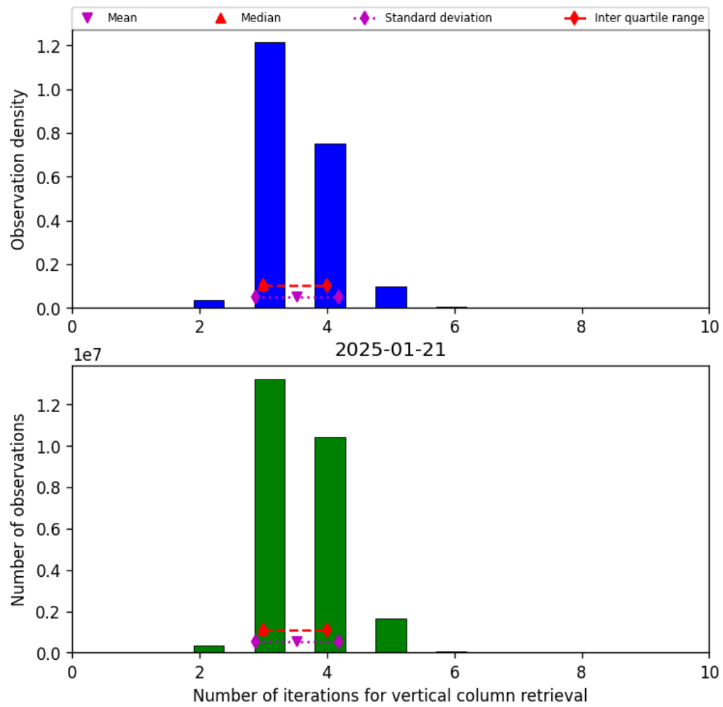
Figure 26: Histogram of “Number of iterations for vertical column retrieval” for 2025-01-20 to 2025-01-22
