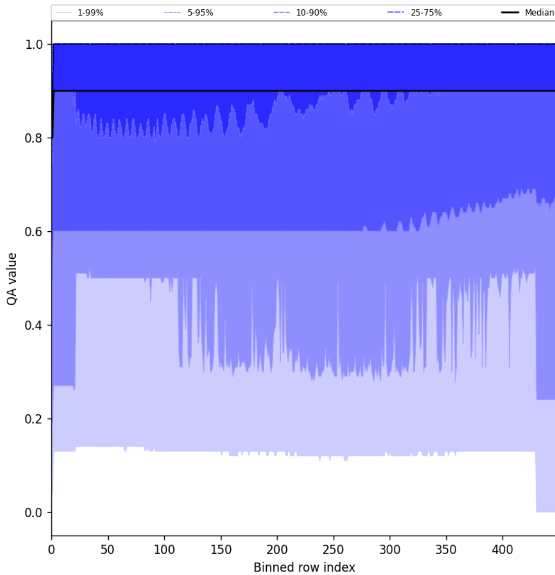
Figure 27: Along track statistics of “QA value” for 2025-01-20 to 2025-01-22
