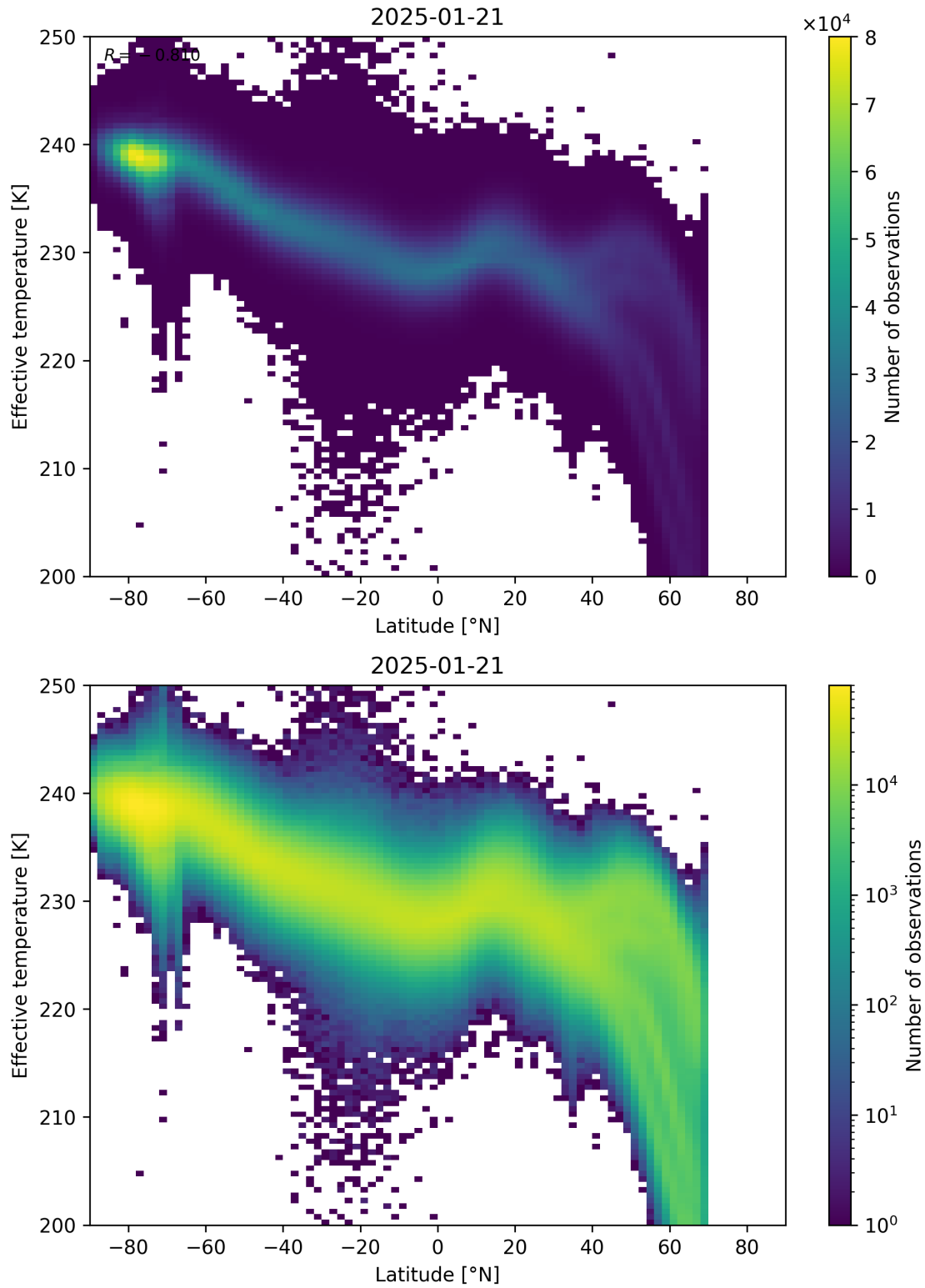
Figure 34: Scatter density plot of “Latitude” against “Effective temperature” for 2025-01-20 to 2025-01-22.
