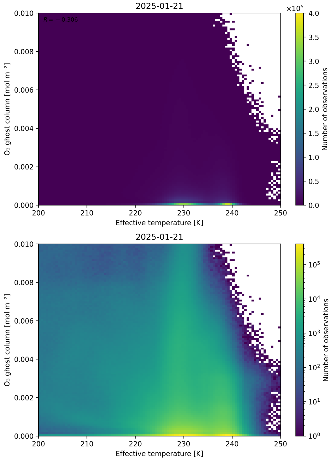
Figure 38: Scatter density plot of “Effective temperature” against “O 3 ghost column” for 2025-01-20 to 2025-01-22.
