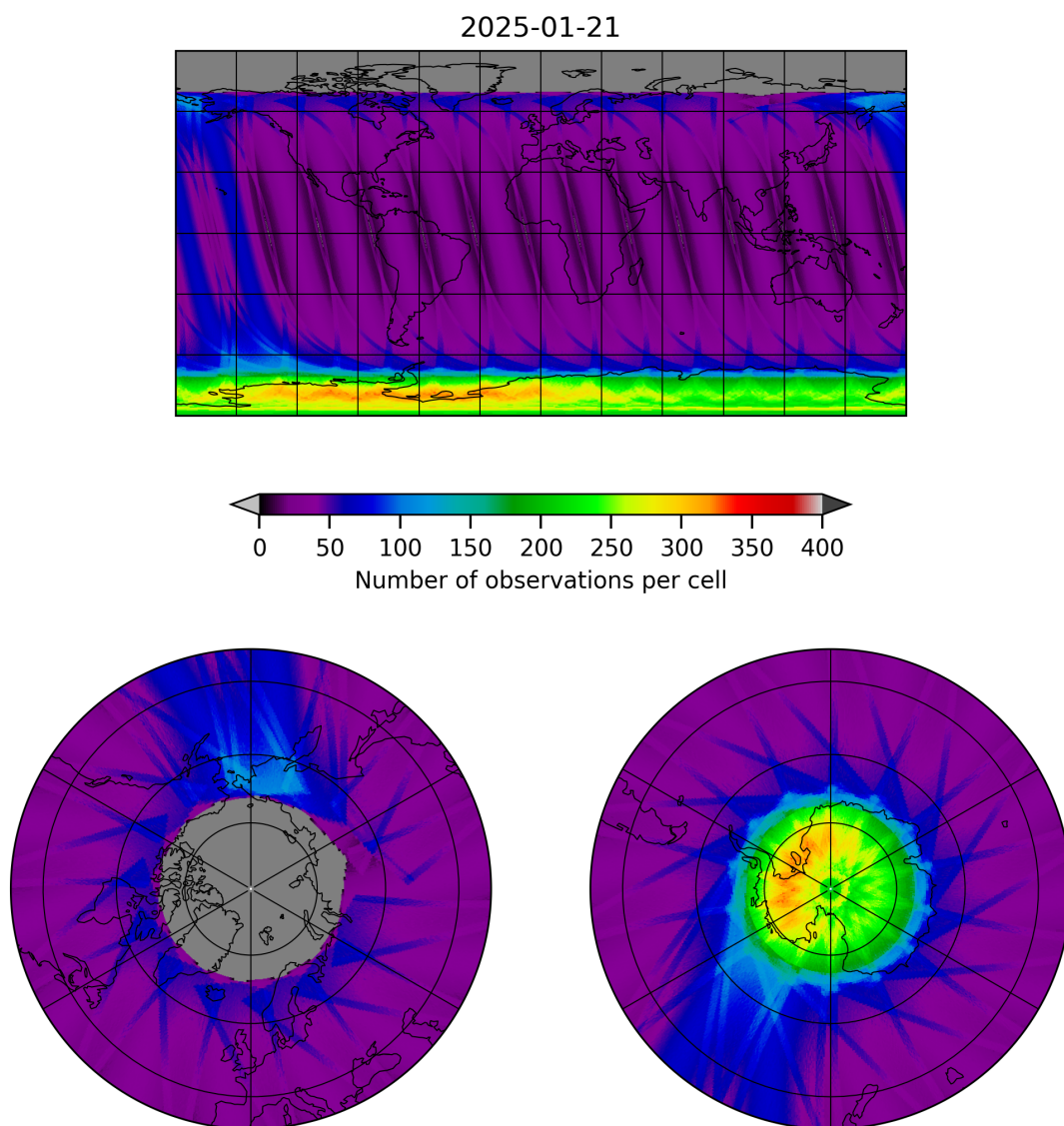
Figure 12: Map of the number of observations for 2025-01-20 to 2025-01-22
