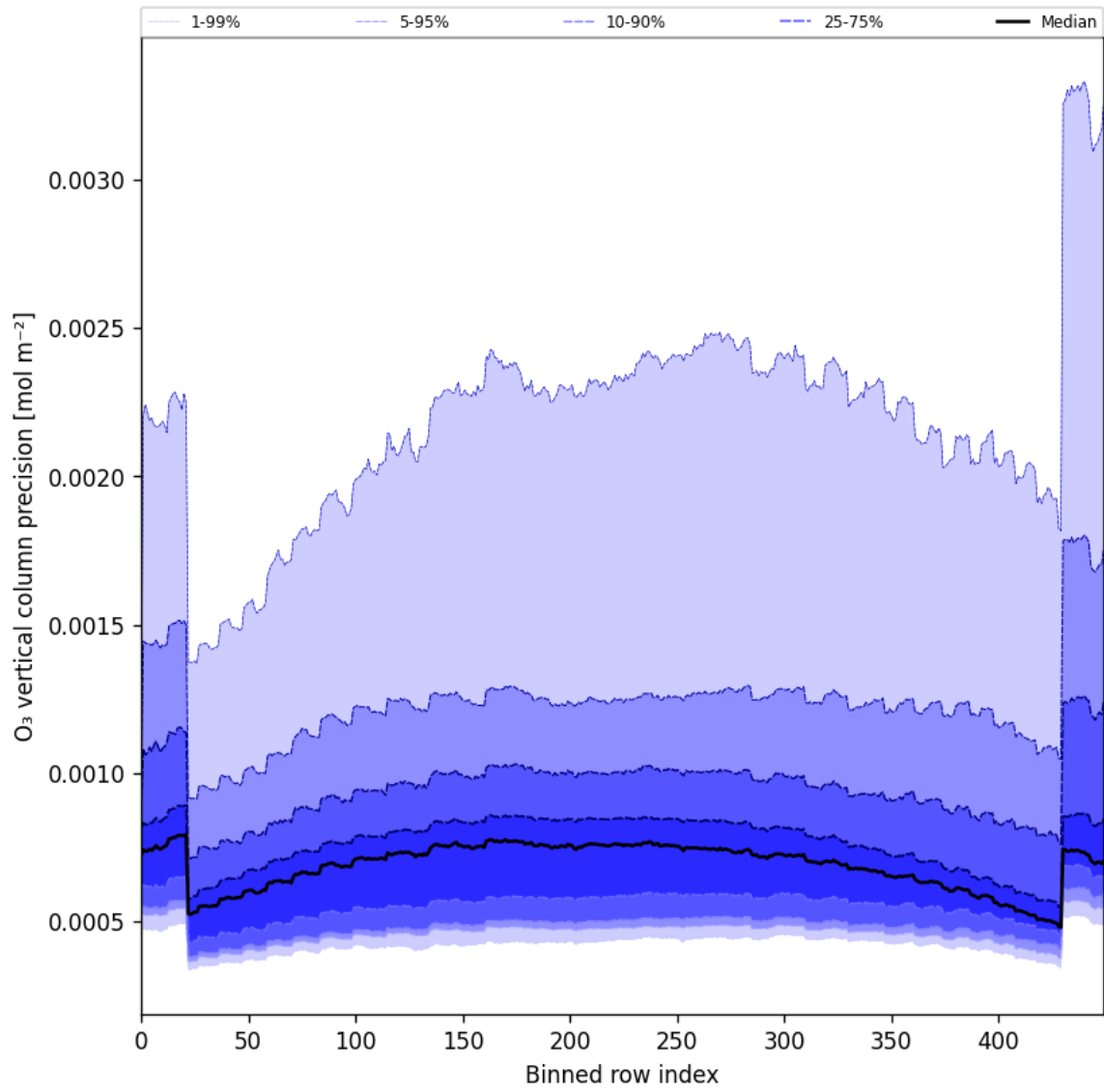
Figure 29: Along track statistics of “O 3 vertical column precision” for 2025-01-20 to 2025-01-22
