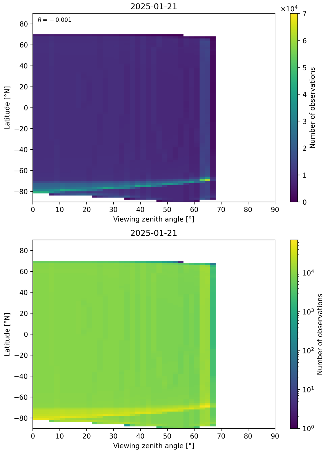
Figure 49: Scatter density plot of “Viewing zenith angle” against “Latitude” for 2025-01-20 to 2025-01-22.
