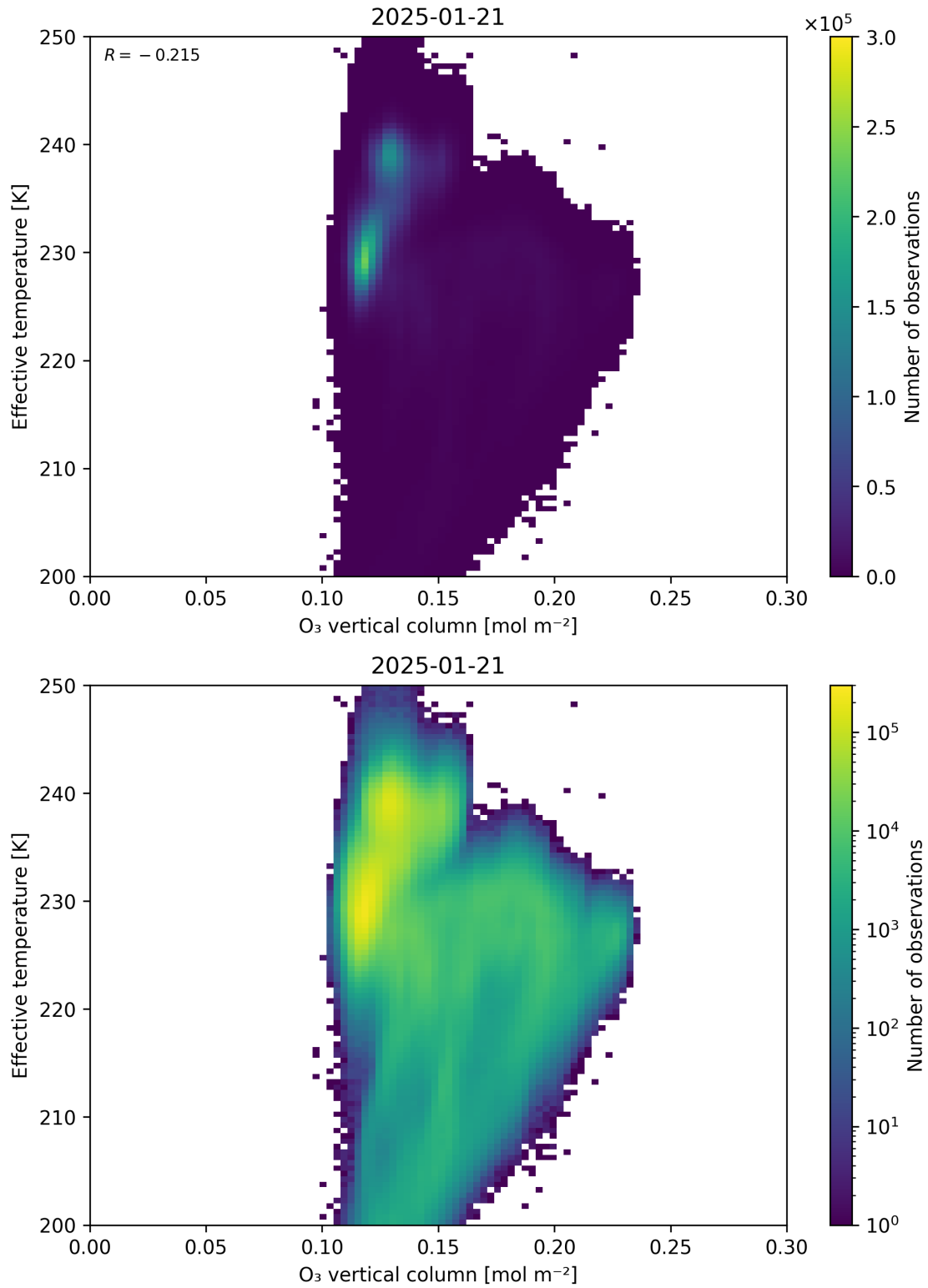
Figure 39: Scatter density plot of “O 3 vertical column” against “Effective temperature” for 2025-01-20 to 2025-01-22.
