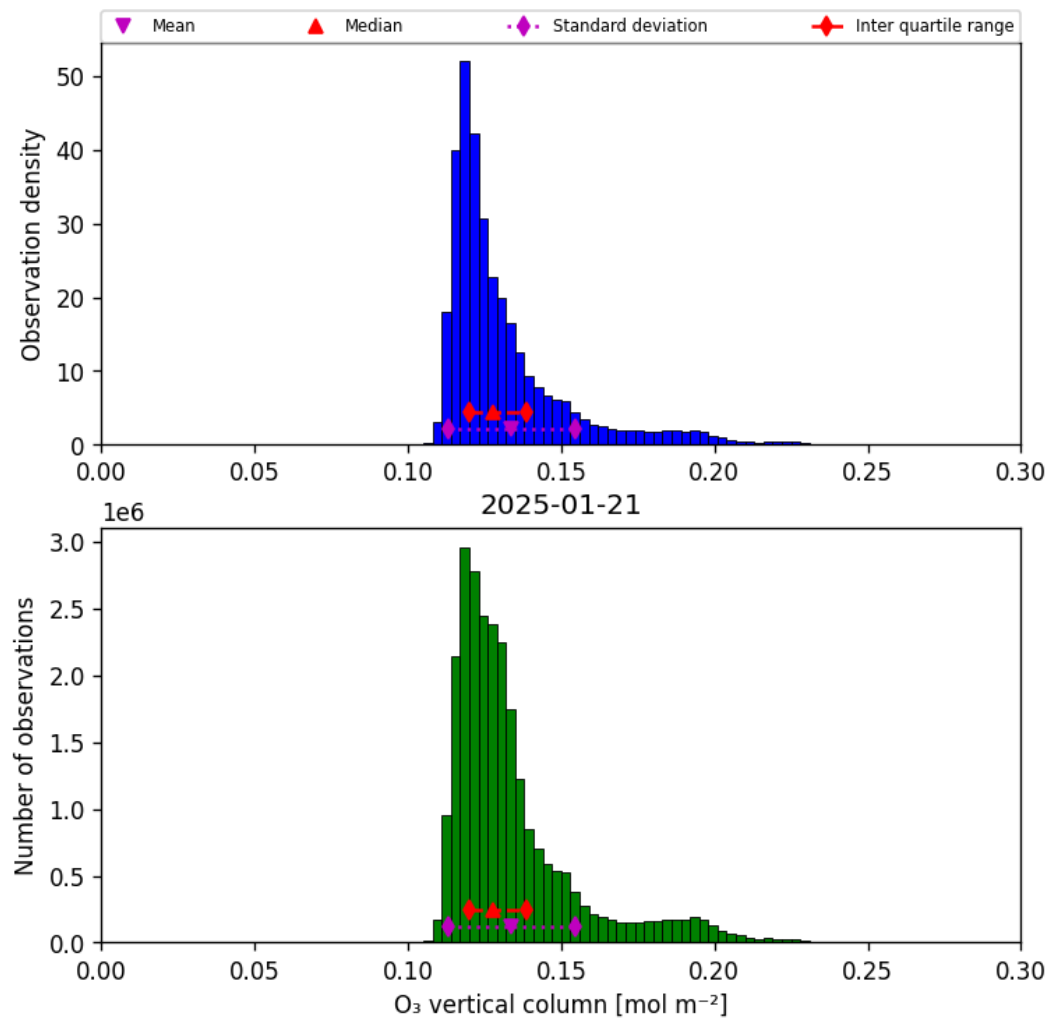
Figure 21: Histogram of “O 3 vertical column” for 2025-01-20 to 2025-01-22
