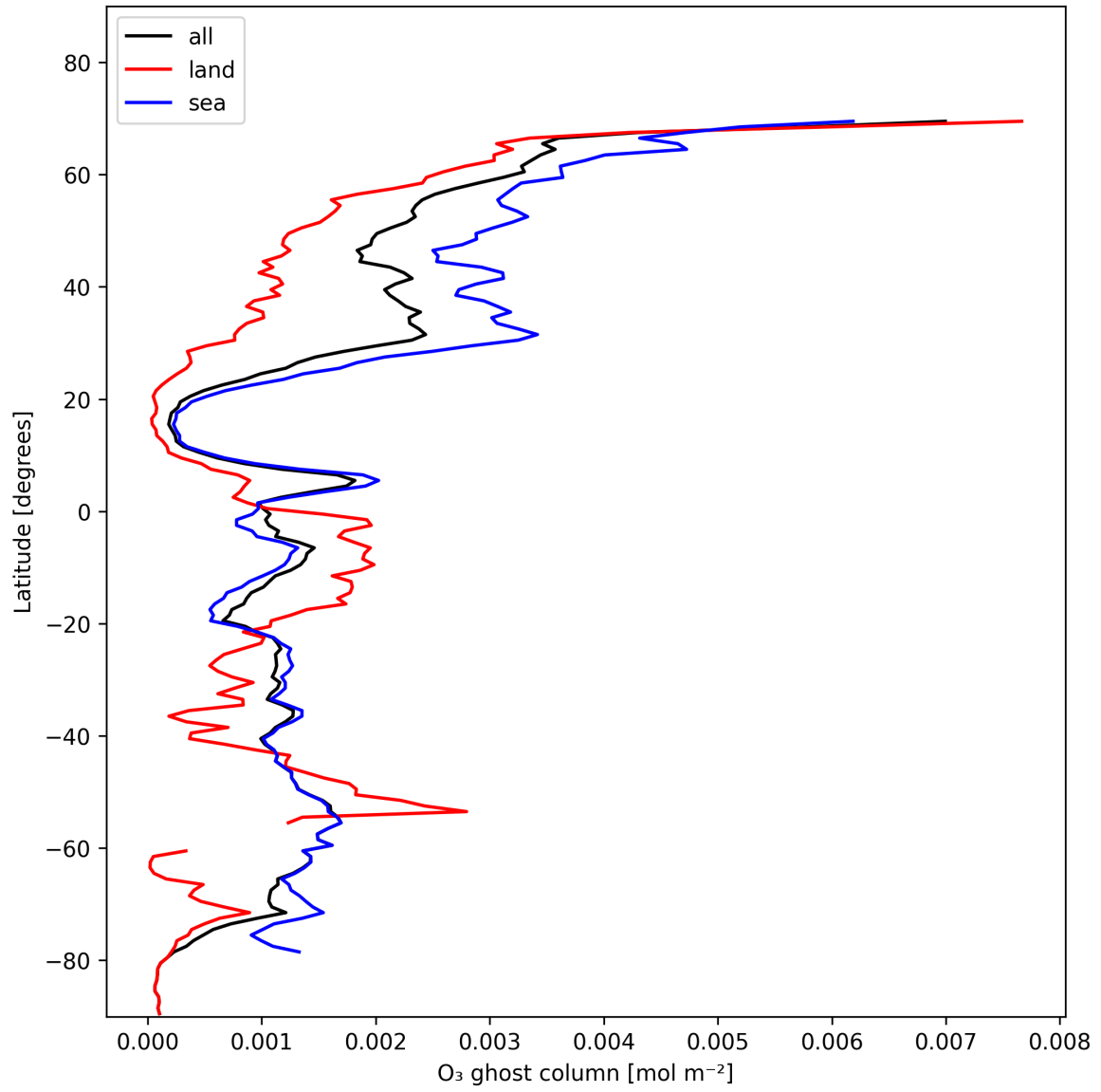
Figure 18: Zonal average of "O 3 ghost column" for 2025-01-20 to 2025-01-22.
