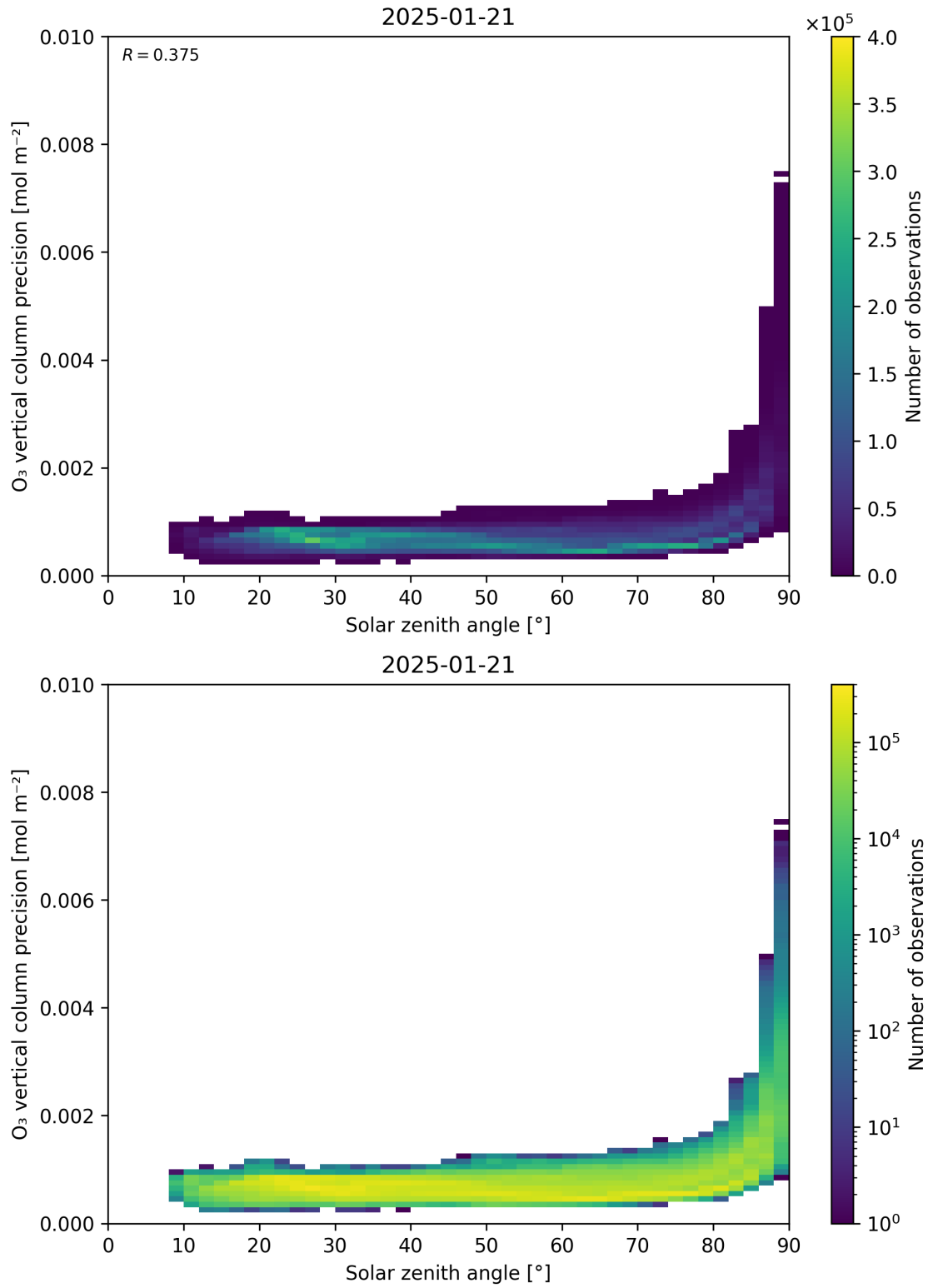
Figure 48: Scatter density plot of “Solar zenith angle” against “O 3 vertical column precision” for 2025-01-20 to 2025-01-22.
