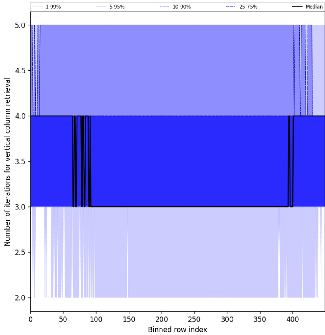
Figure 33: Along track statistics of “Number of iterations for vertical column retrieval” for 2025-01-20 to 2025-01-22
