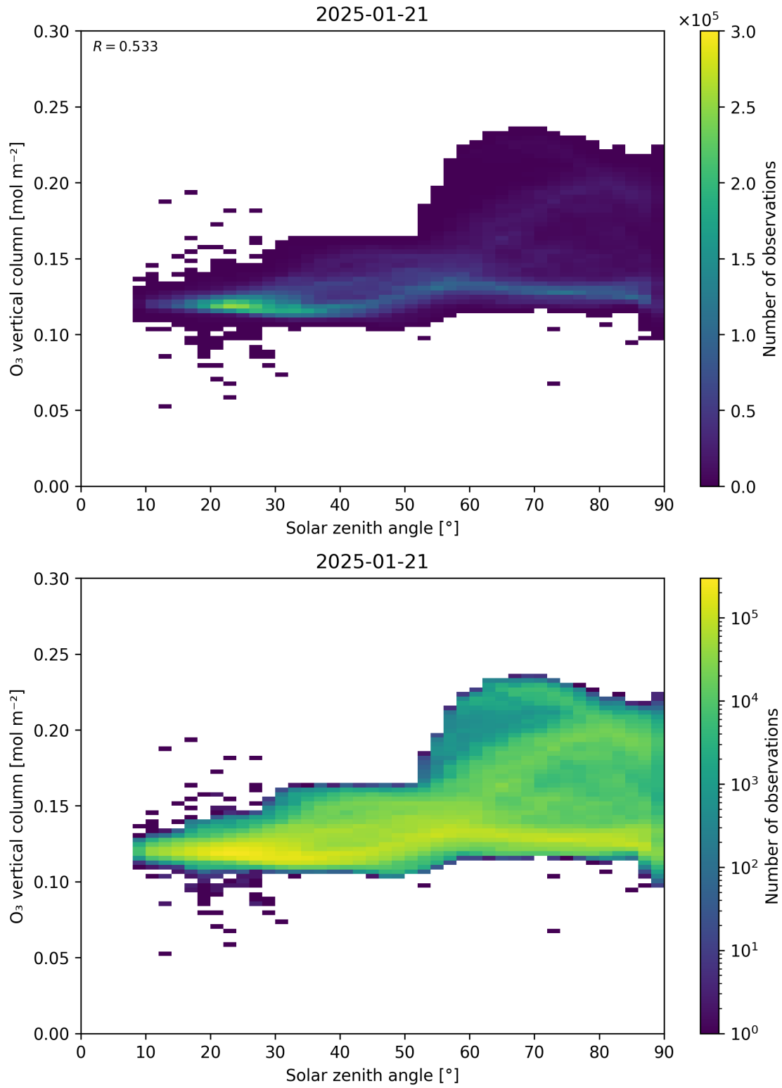
Figure 47: Scatter density plot of “Solar zenith angle” against “O 3 vertical column” for 2025-01-20 to 2025-01-22.
