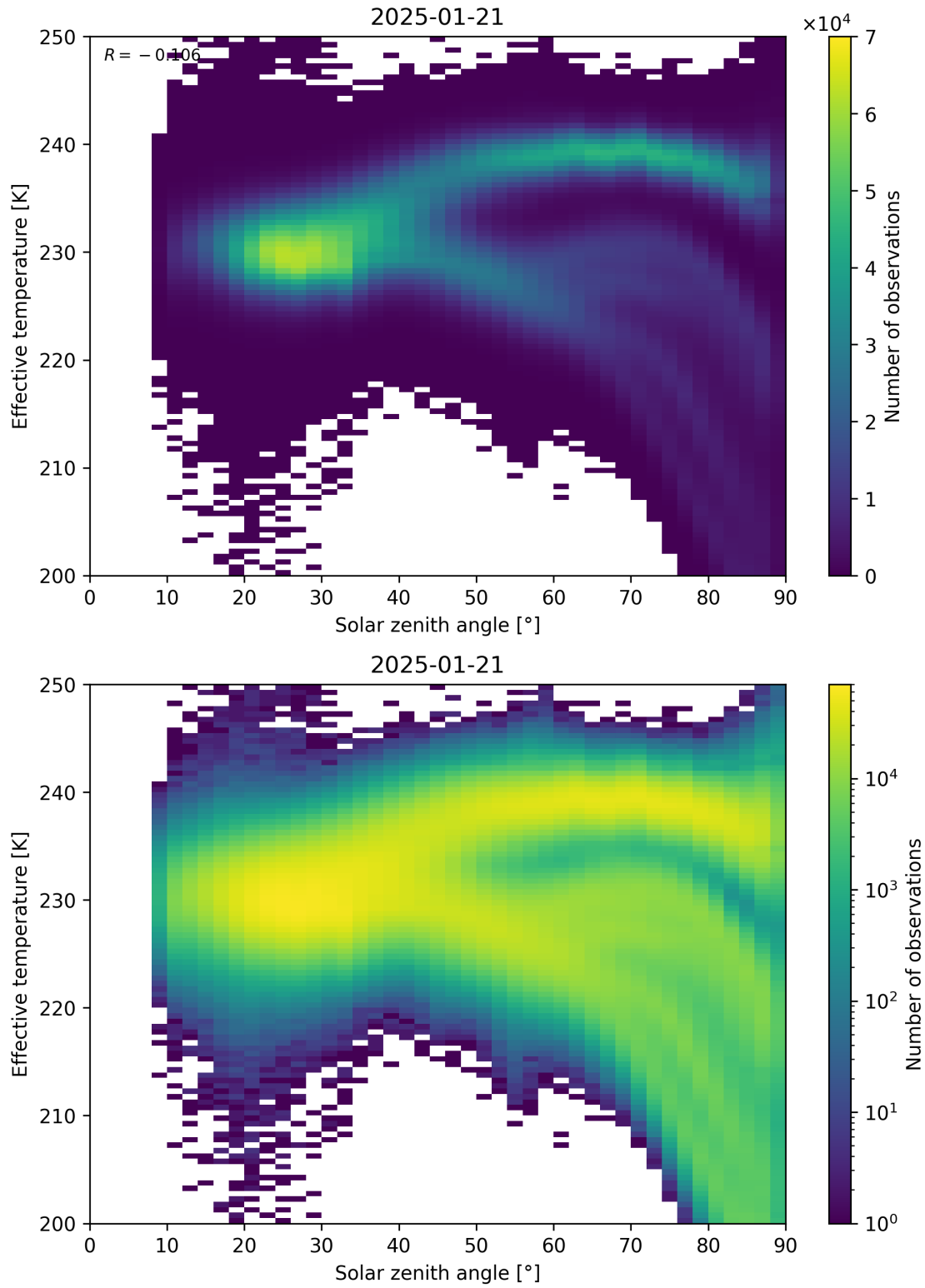
Figure 45: Scatter density plot of “Solar zenith angle” against “Effective temperature” for 2025-01-20 to 2025-01-22.
