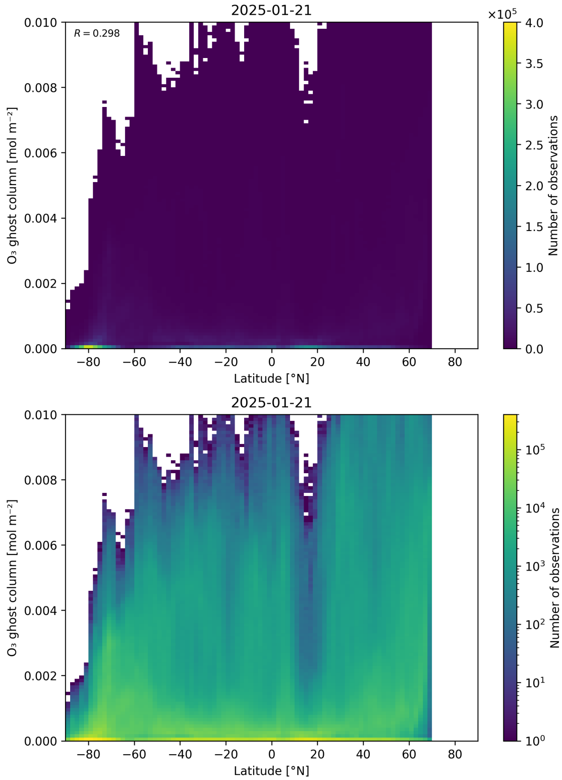
Figure 35: Scatter density plot of “Latitude” against “O 3 ghost column” for 2025-01-20 to 2025-01-22.
