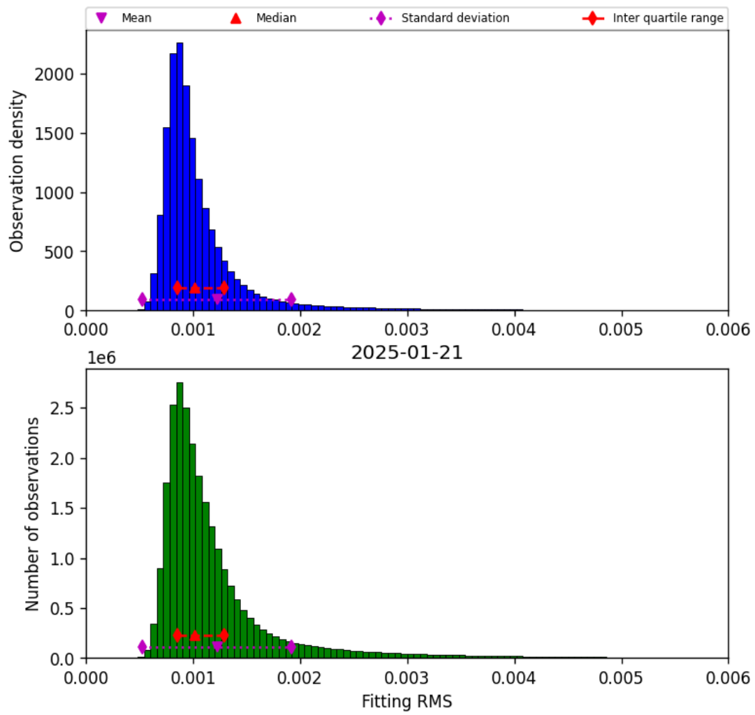
Figure 23: Histogram of “Fitting RMS” for 2025-01-20 to 2025-01-22
