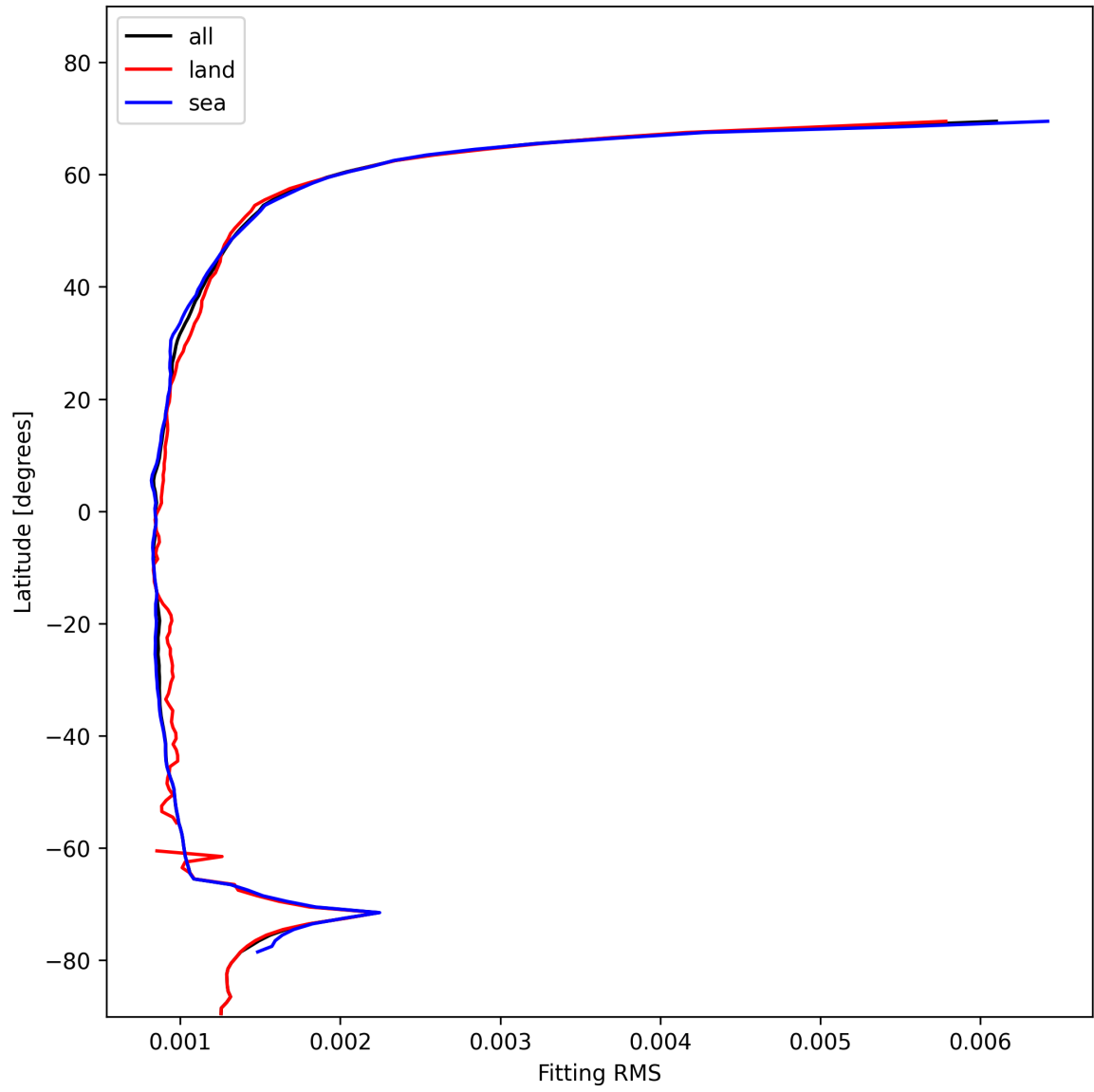
Figure 16: Zonal average of “Fitting RMS” for 2025-01-20 to 2025-01-22.
