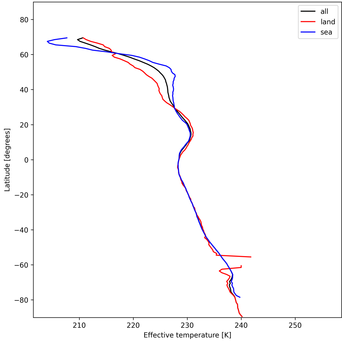
Figure 17: Zonal average of "Effective temperature" for 2025-01-20 to 2025-01-22.
