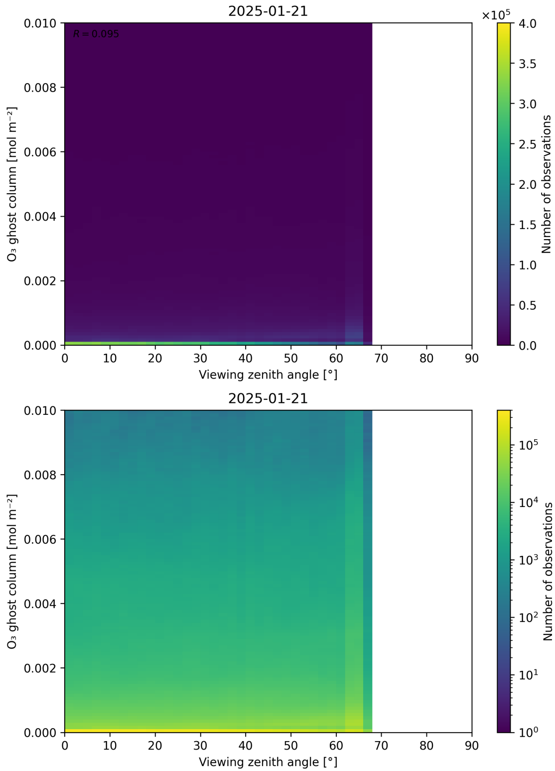
Figure 51: Scatter density plot of “Viewing zenith angle” against “O 3 ghost column” for 2025-01-20 to 2025-01-22.
