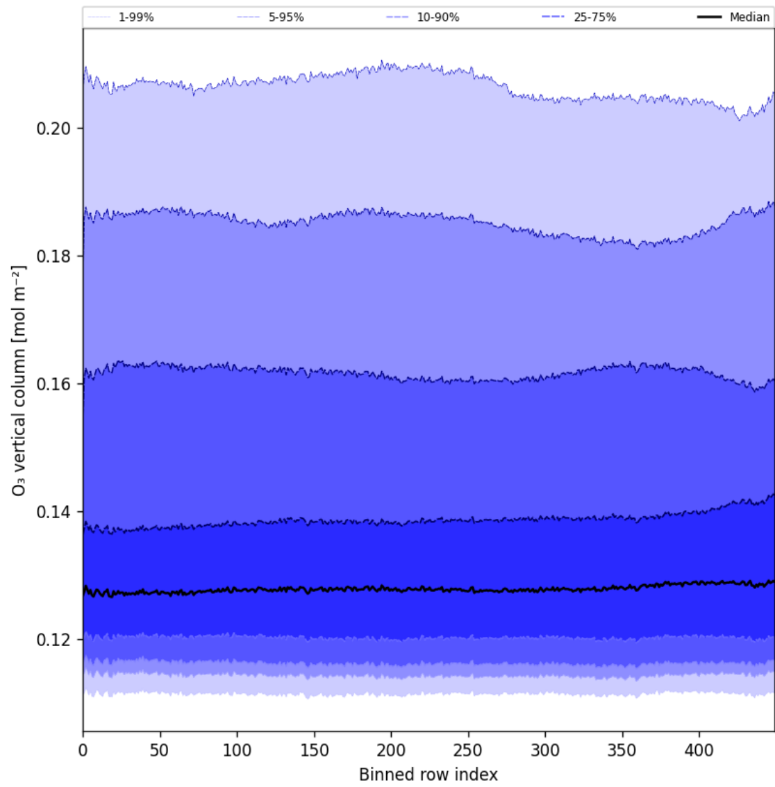
Figure 28: Along track statistics of “ \text{O}_3 vertical column” for 2025-01-20 to 2025-01-22
