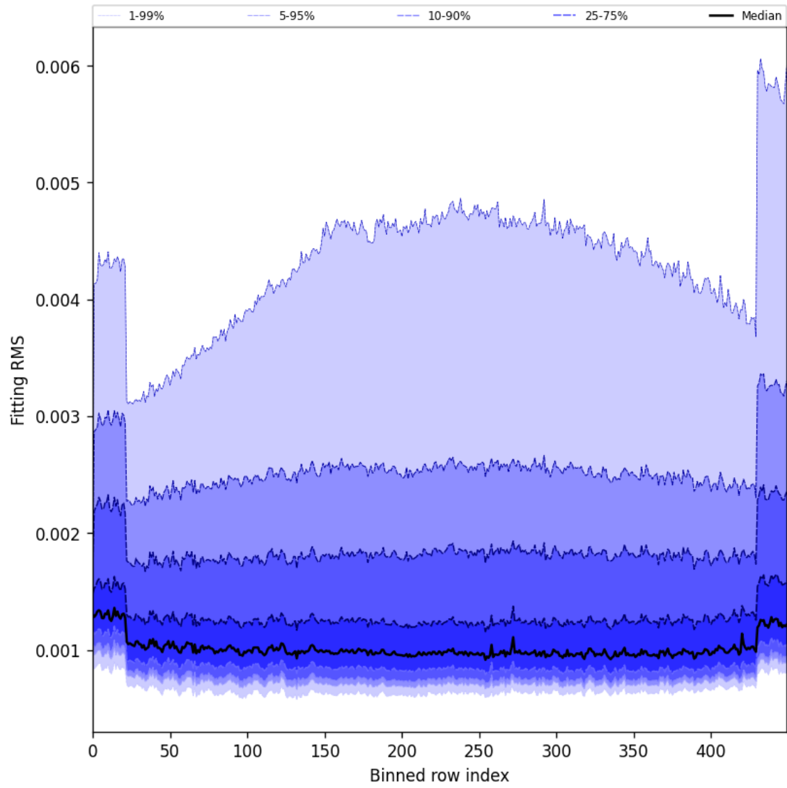
Figure 30: Along track statistics of “Fitting RMS” for 2025-01-20 to 2025-01-22
