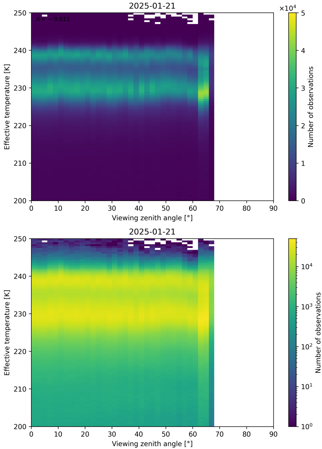
Figure 50: Scatter density plot of “Viewing zenith angle” against “Effective temperature” for 2025-01-20 to 2025-01-22.
