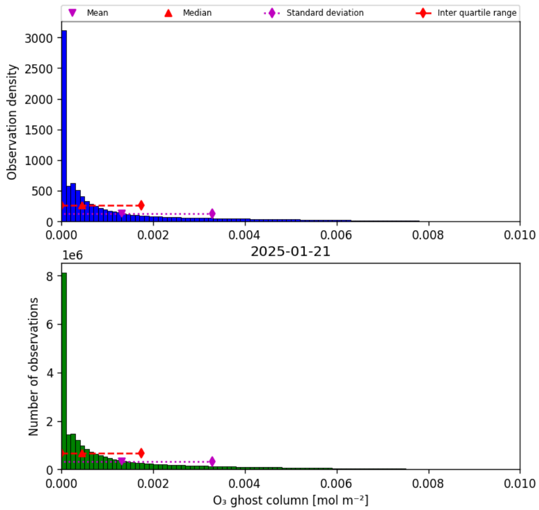
Figure 25: Histogram of “O 3 ghost column” for 2025-01-20 to 2025-01-22
