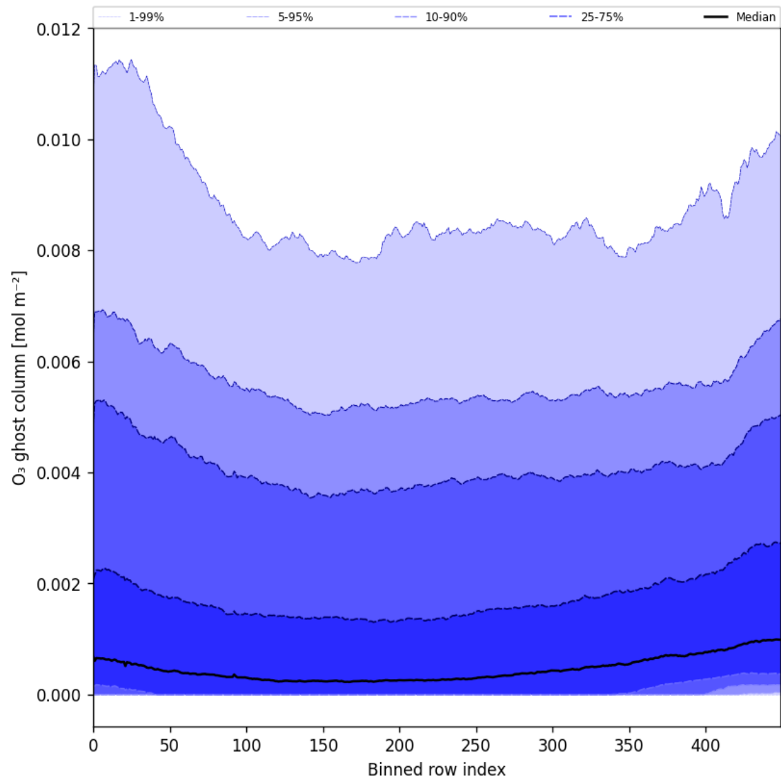
Figure 32: Along track statistics of “O 3 ghost column” for 2025-01-20 to 2025-01-22
