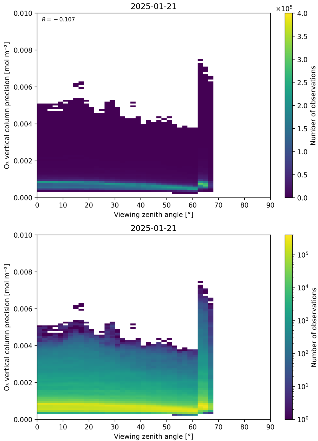
Figure 53: Scatter density plot of “Viewing zenith angle” against “O 3 vertical column precision” for 2025-01-20 to 2025-01-22.
