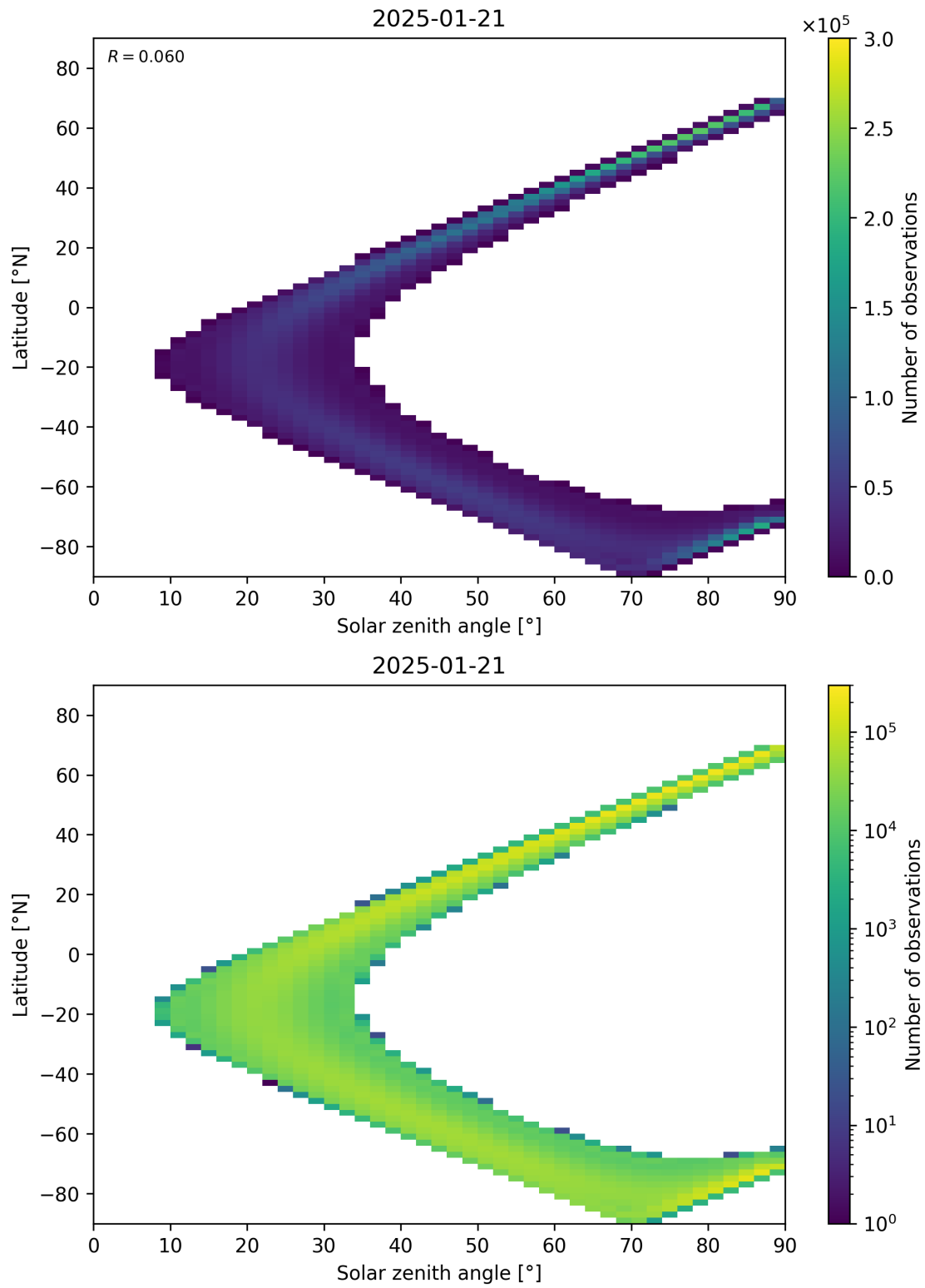
Figure 44: Scatter density plot of “Solar zenith angle” against “Latitude” for 2025-01-20 to 2025-01-22.
