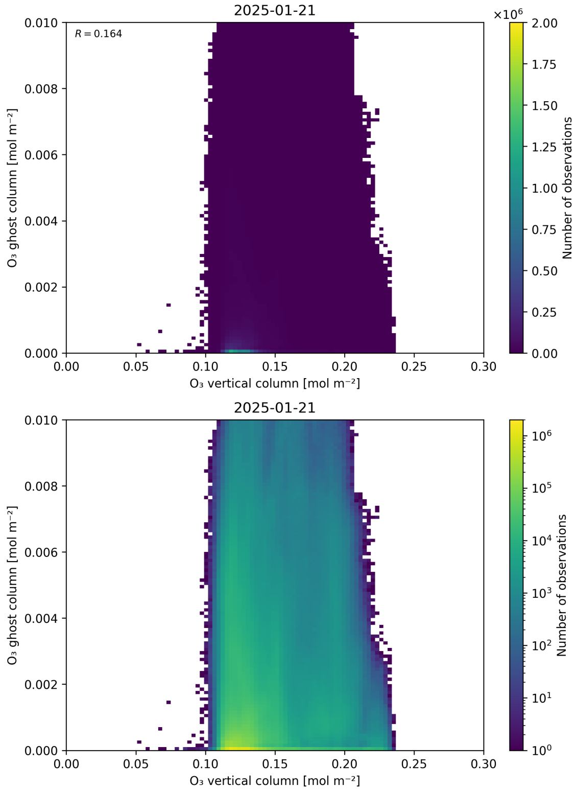
Figure 40: Scatter density plot of “O 3 vertical column” against “O 3 ghost column” for 2025-01-20 to 2025-01-22.
