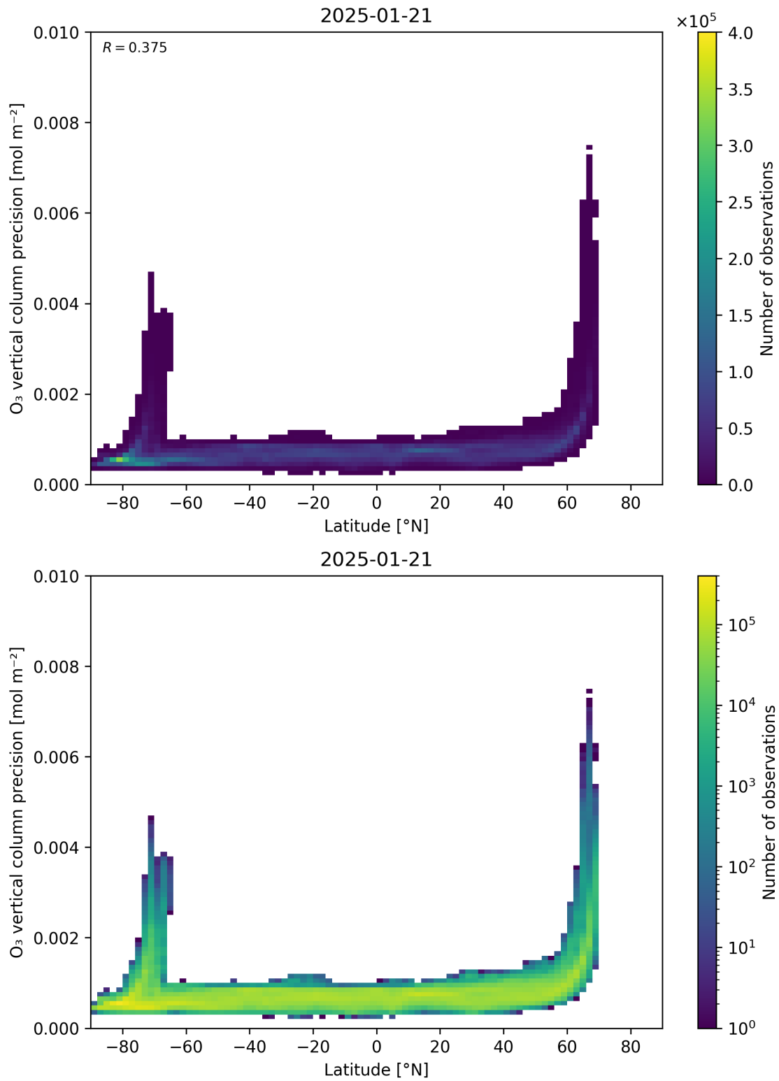
Figure 37: Scatter density plot of “Latitude” against “O 3 vertical column precision” for 2025-01-20 to 2025-01-22.
