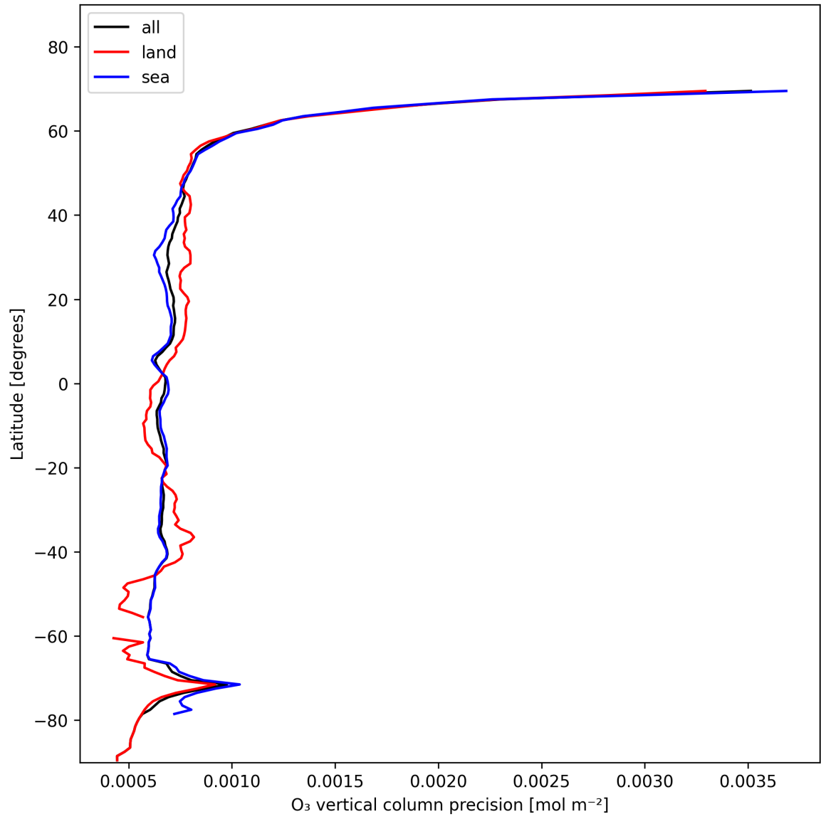
Figure 15: Zonal average of “O 3 vertical column precision” for 2025-01-20 to 2025-01-22.
