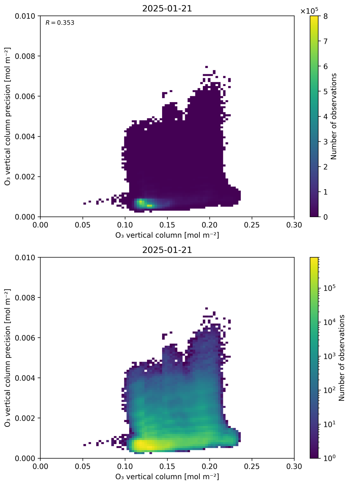
Figure 41: Scatter density plot of “O 3 vertical column” against “O 3 vertical column precision” for 2025-01-20 to 2025-01-22.
