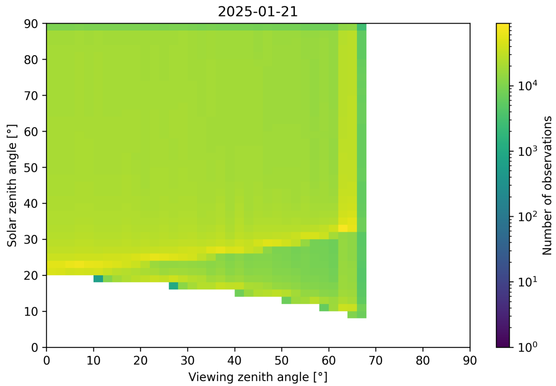
Figure 54: Scatter density plot of “Viewing zenith angle” against “Solar zenith angle” for 2025-01-20 to 2025-01-22.
