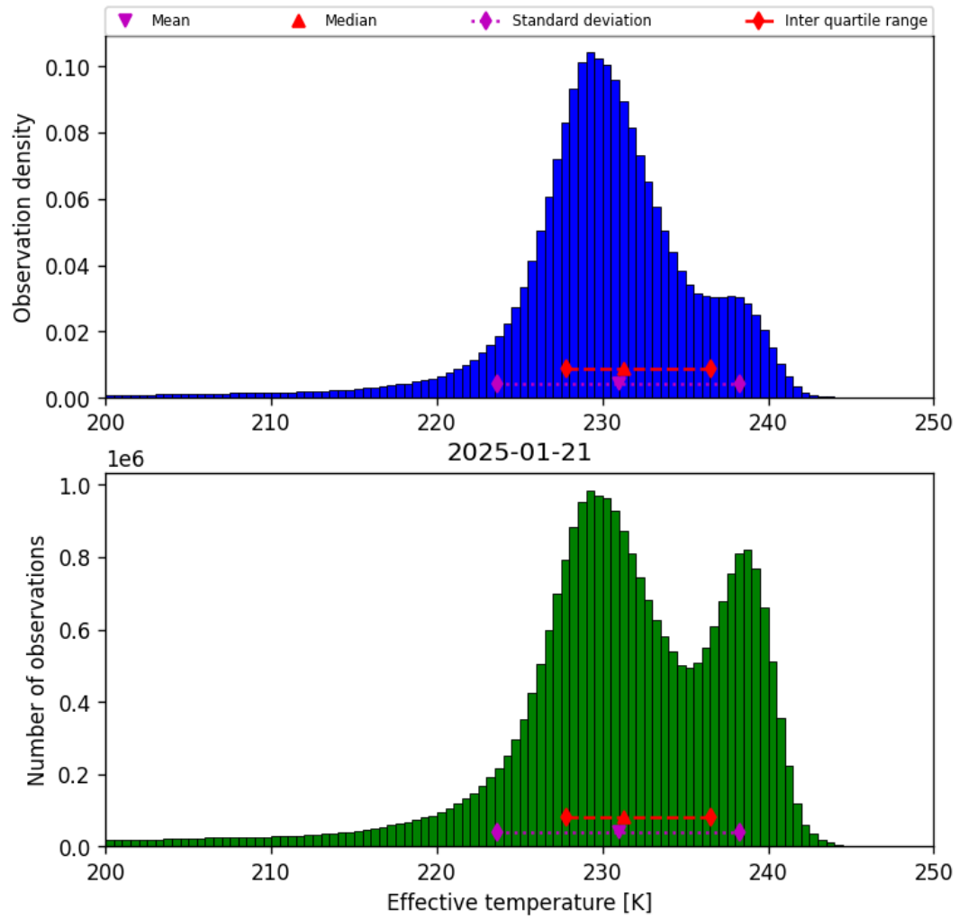
Figure 24: Histogram of “Effective temperature” for 2025-01-20 to 2025-01-22
