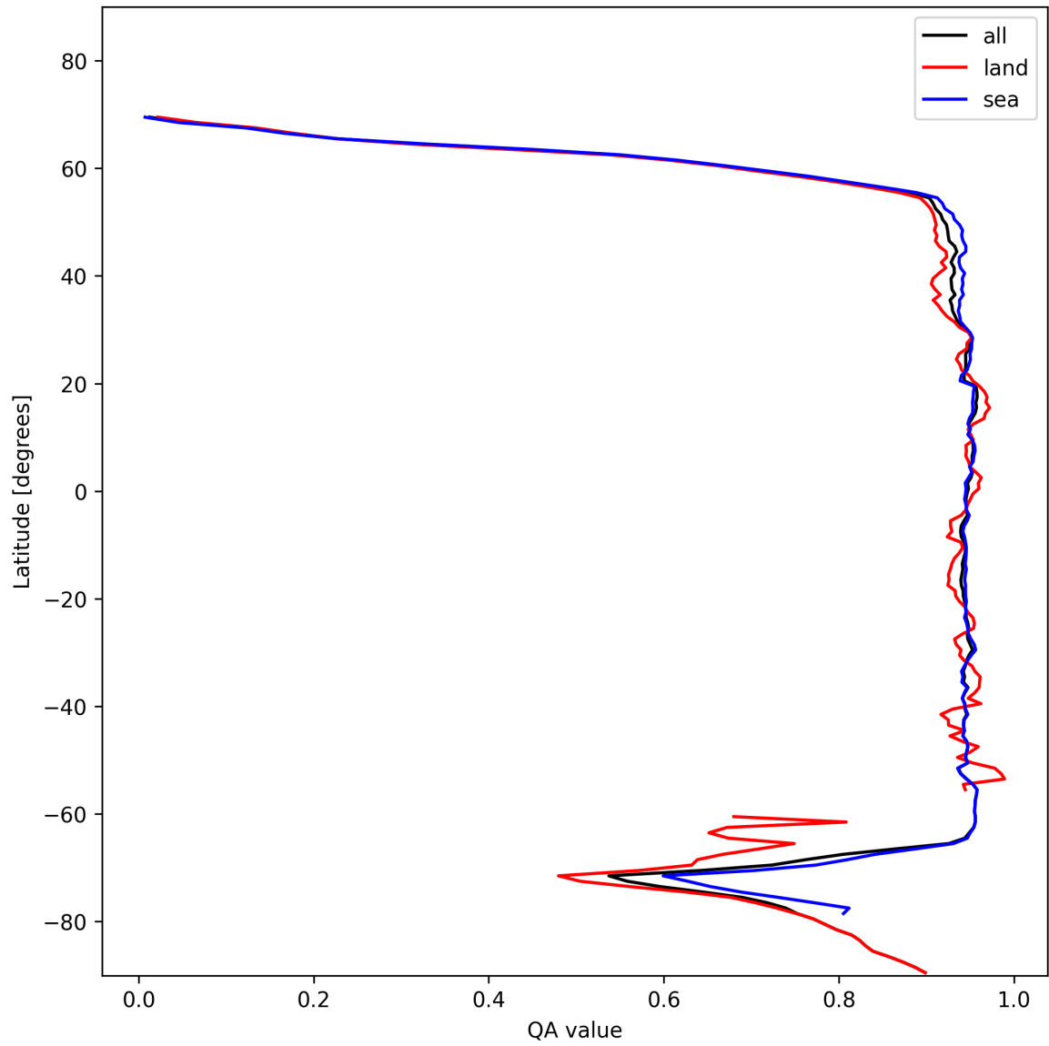
Figure 13: Zonal average of “QA value” for 2025-01-20 to 2025-01-22.
