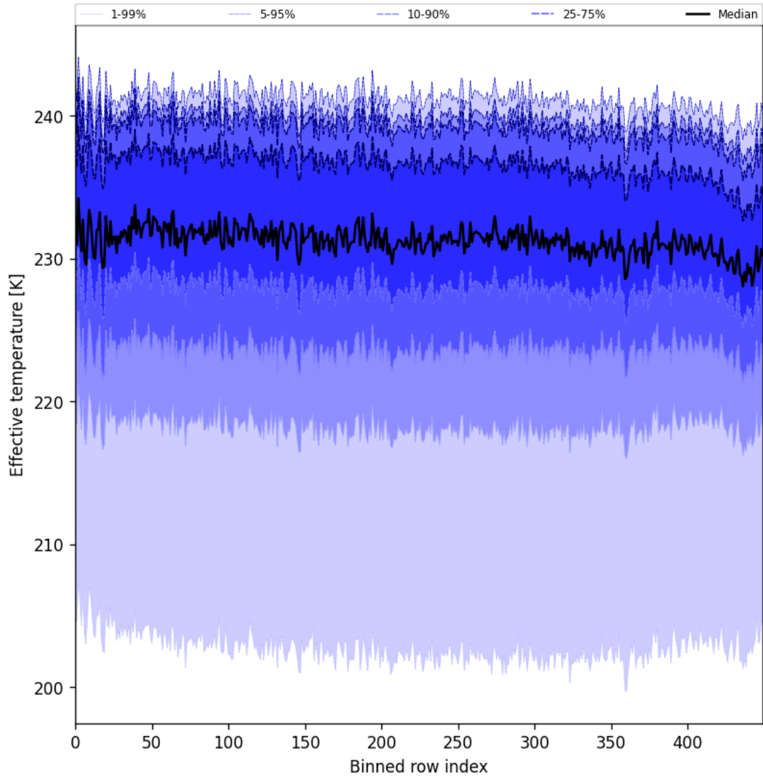
Figure 31: Along track statistics of “Effective temperature” for 2025-01-20 to 2025-01-22
