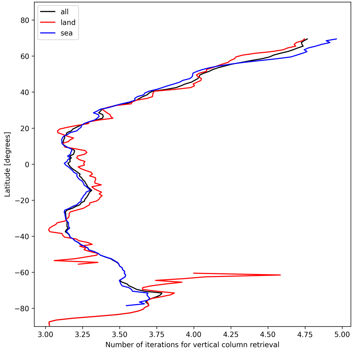
Figure 19: Zonal average of “Number of iterations for vertical column retrieval” for 2025-01-20 to 2025-01-22.
