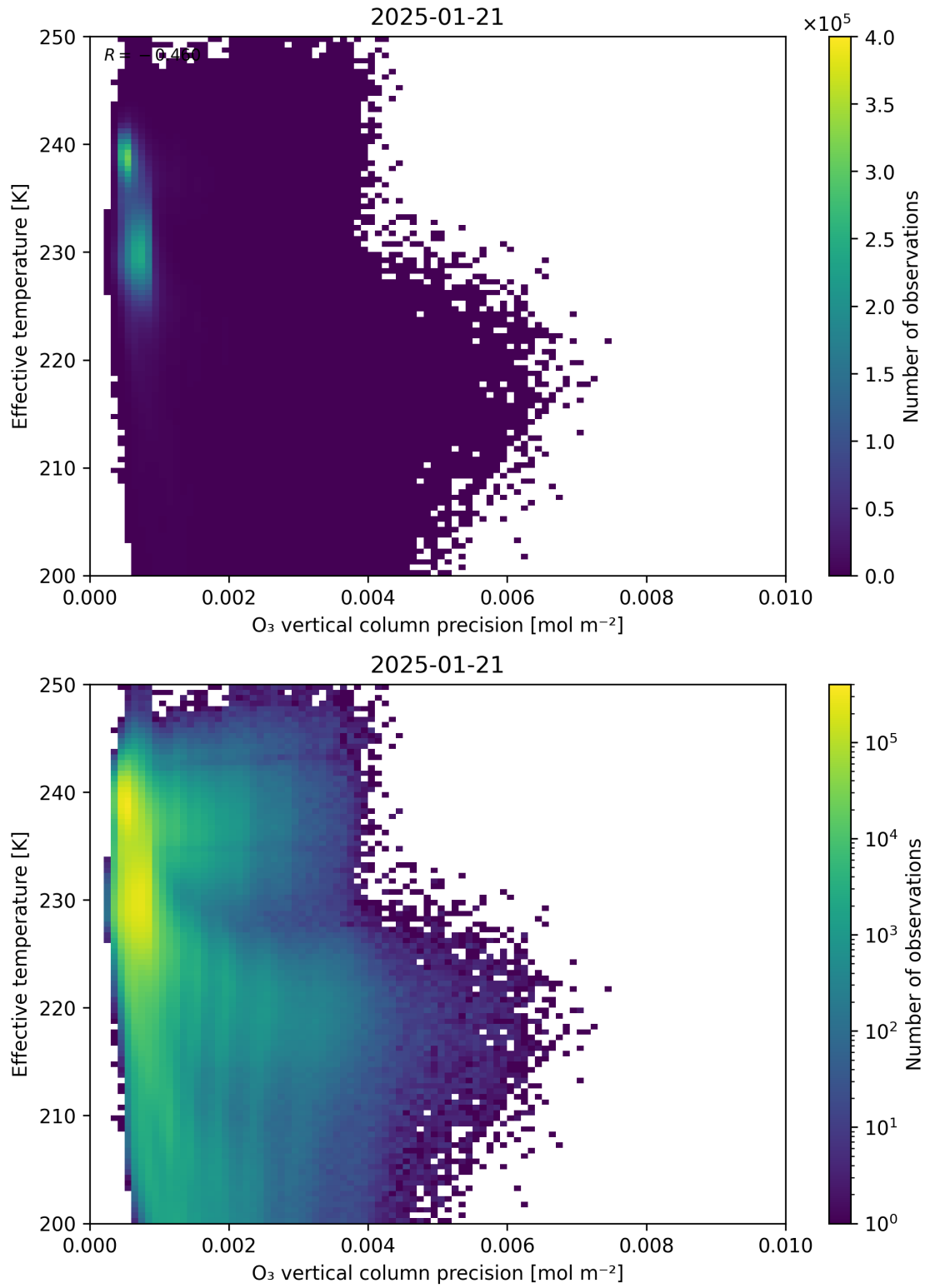
Figure 42: Scatter density plot of “O 3 vertical column precision” against “Effective temperature” for 2025-01-20 to 2025-01-22.
