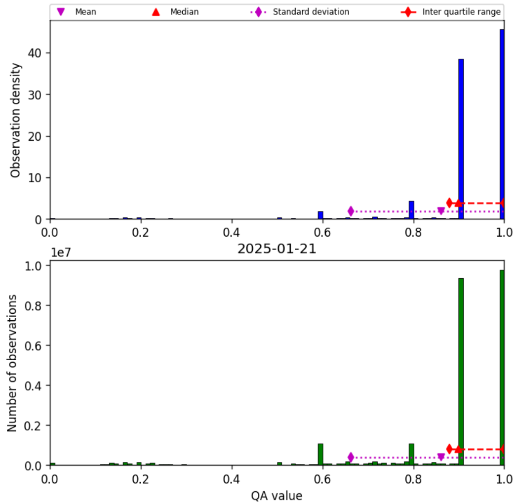
Figure 20: Histogram of “QA value” for 2025-01-20 to 2025-01-22
