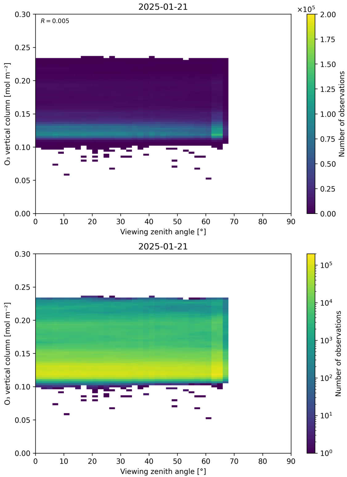
Figure 52: Scatter density plot of “Viewing zenith angle” against “O 3 vertical column” for 2025-01-20 to 2025-01-22.
