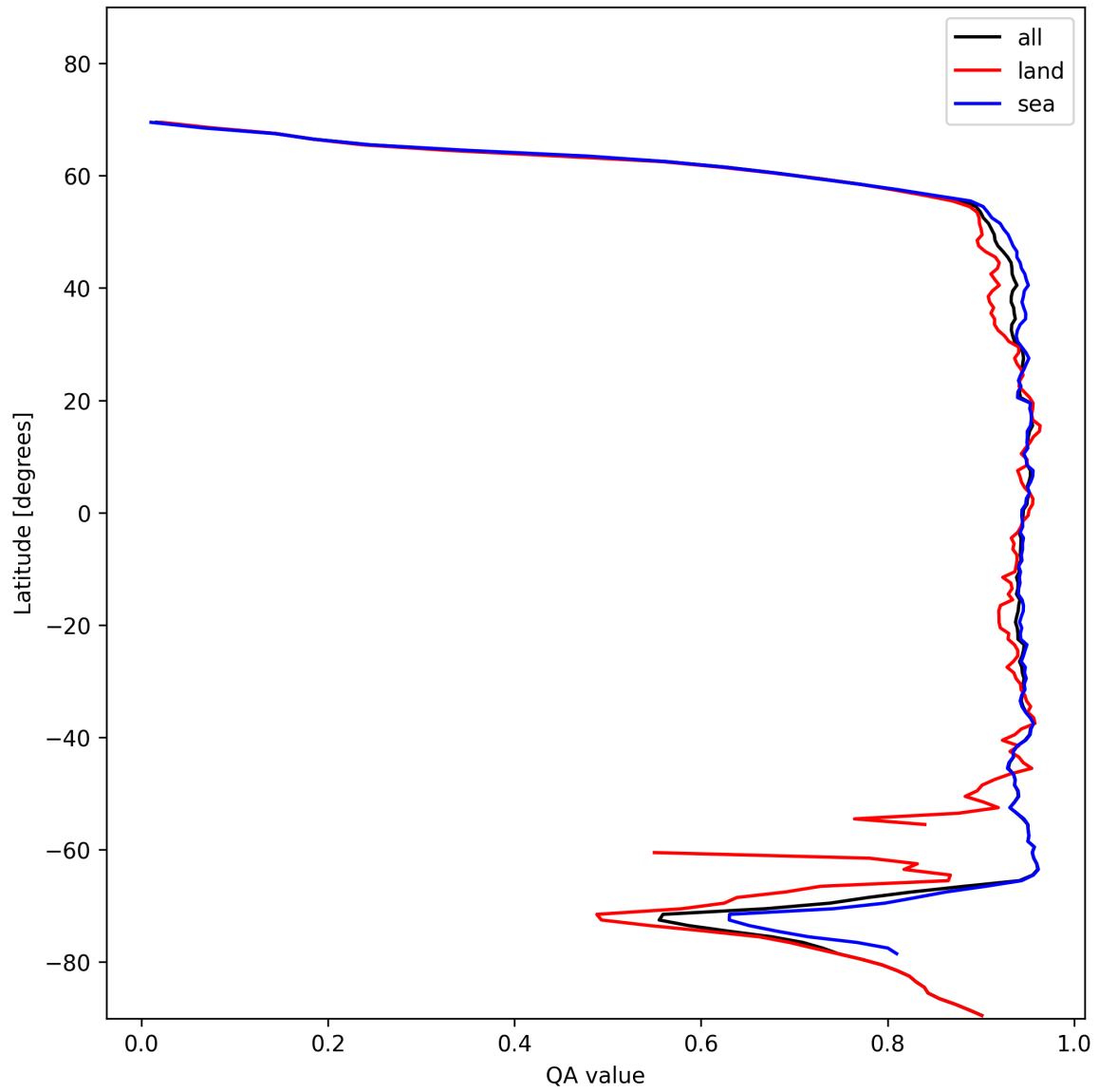
Figure 13: Zonal average of “QA value” for 2025-01-21 to 2025-01-23.
