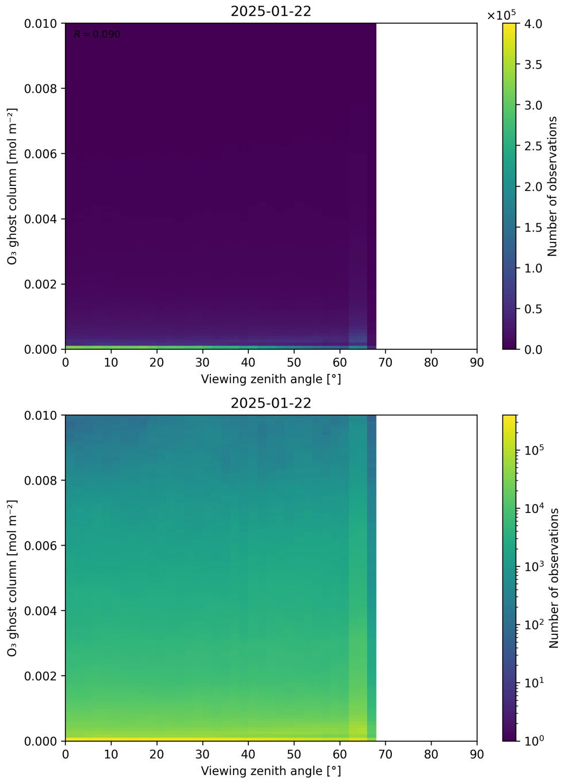
Figure 51: Scatter density plot of “Viewing zenith angle” against “O 3 ghost column” for 2025-01-21 to 2025-01-23.
