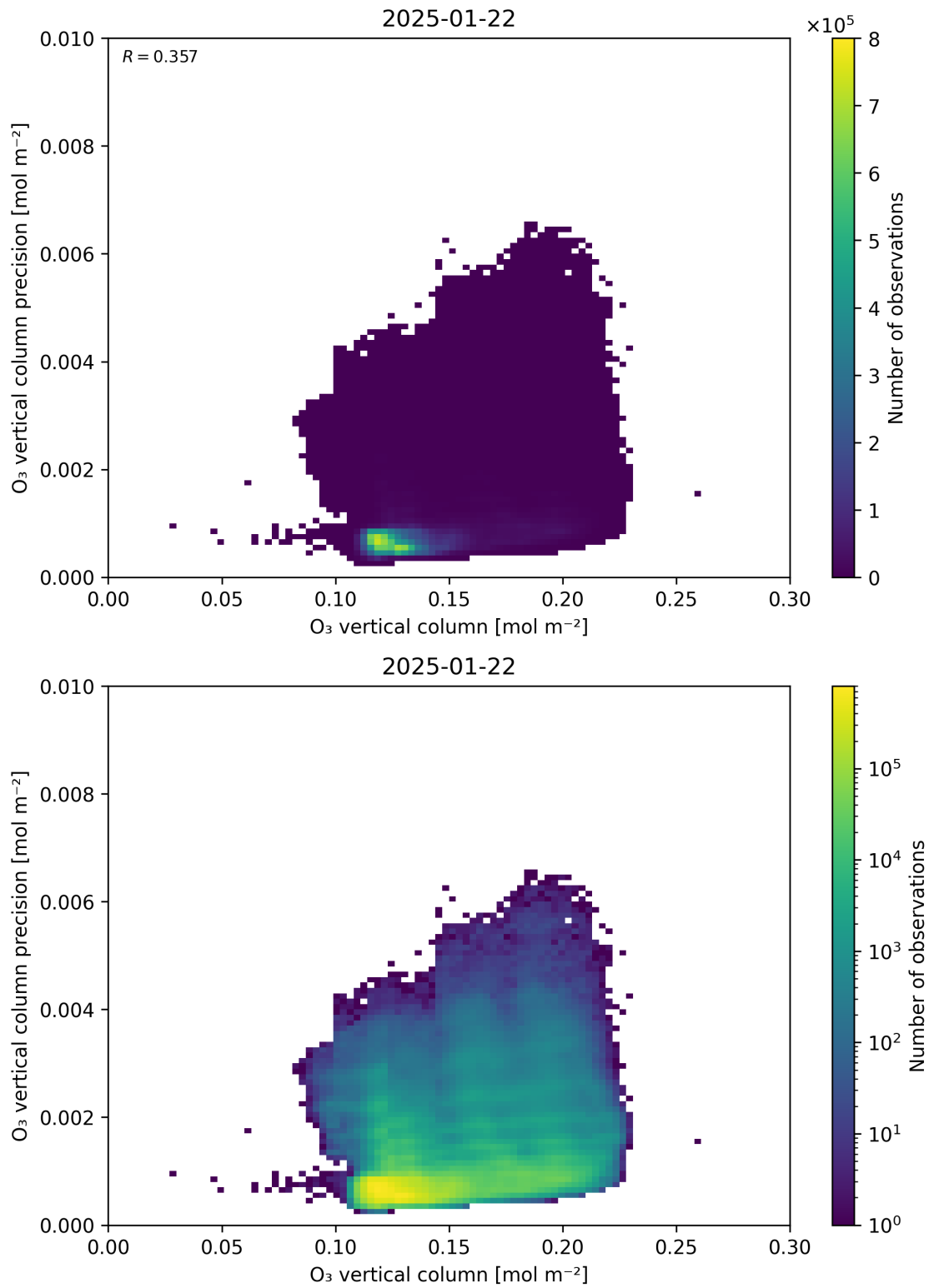
Figure 41: Scatter density plot of “O 3 vertical column” against “O 3 vertical column precision” for 2025-01-21 to 2025-01-23.
