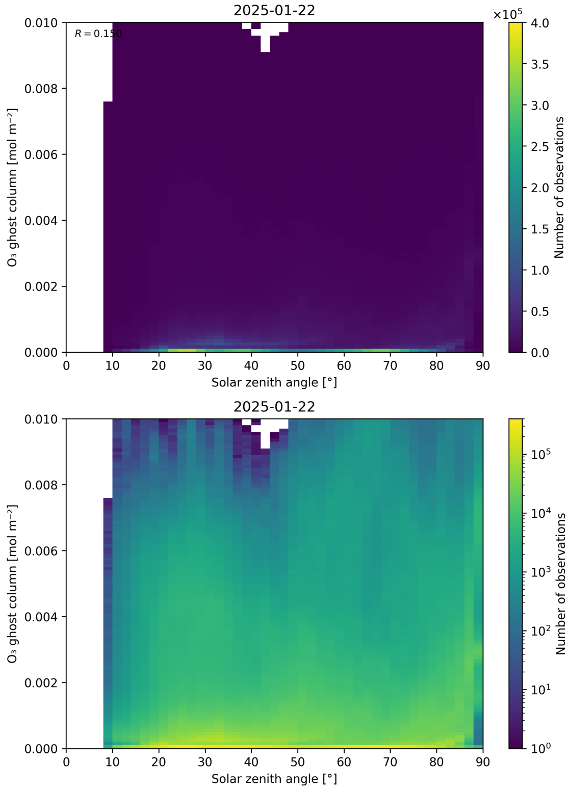
Figure 46: Scatter density plot of “Solar zenith angle” against “O 3 ghost column” for 2025-01-21 to 2025-01-23.
