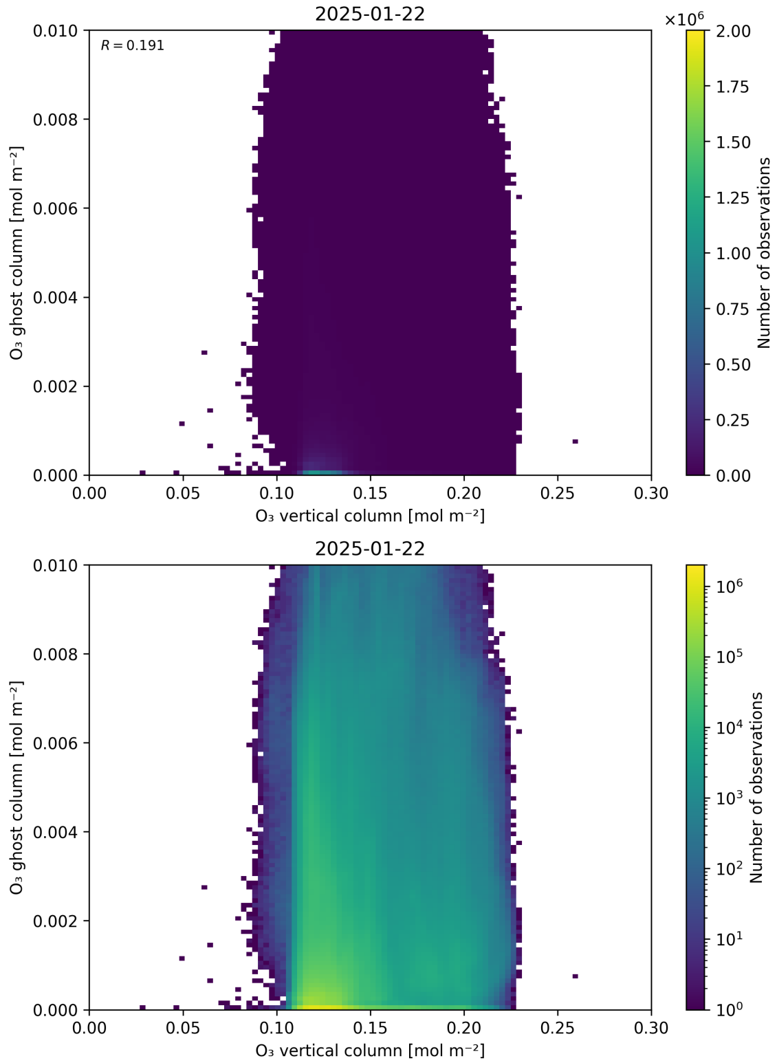
Figure 40: Scatter density plot of “O 3 vertical column” against “O 3 ghost column” for 2025-01-21 to 2025-01-23.
