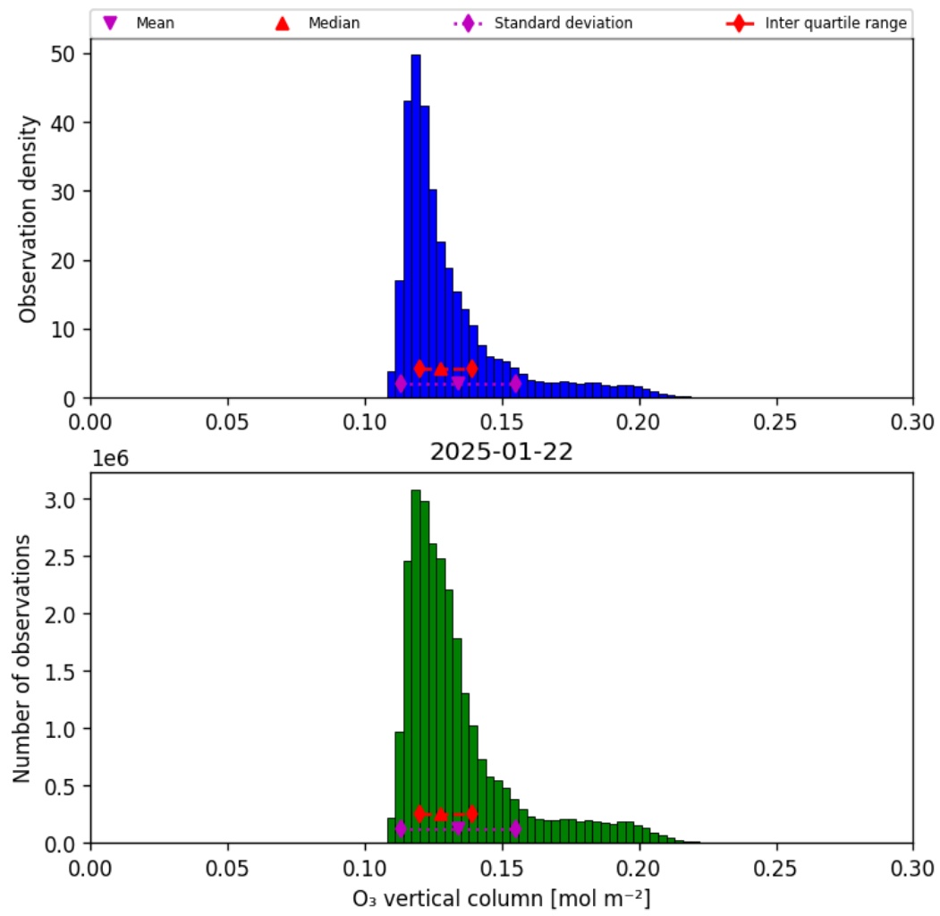
Figure 21: Histogram of “O 3 vertical column” for 2025-01-21 to 2025-01-23
