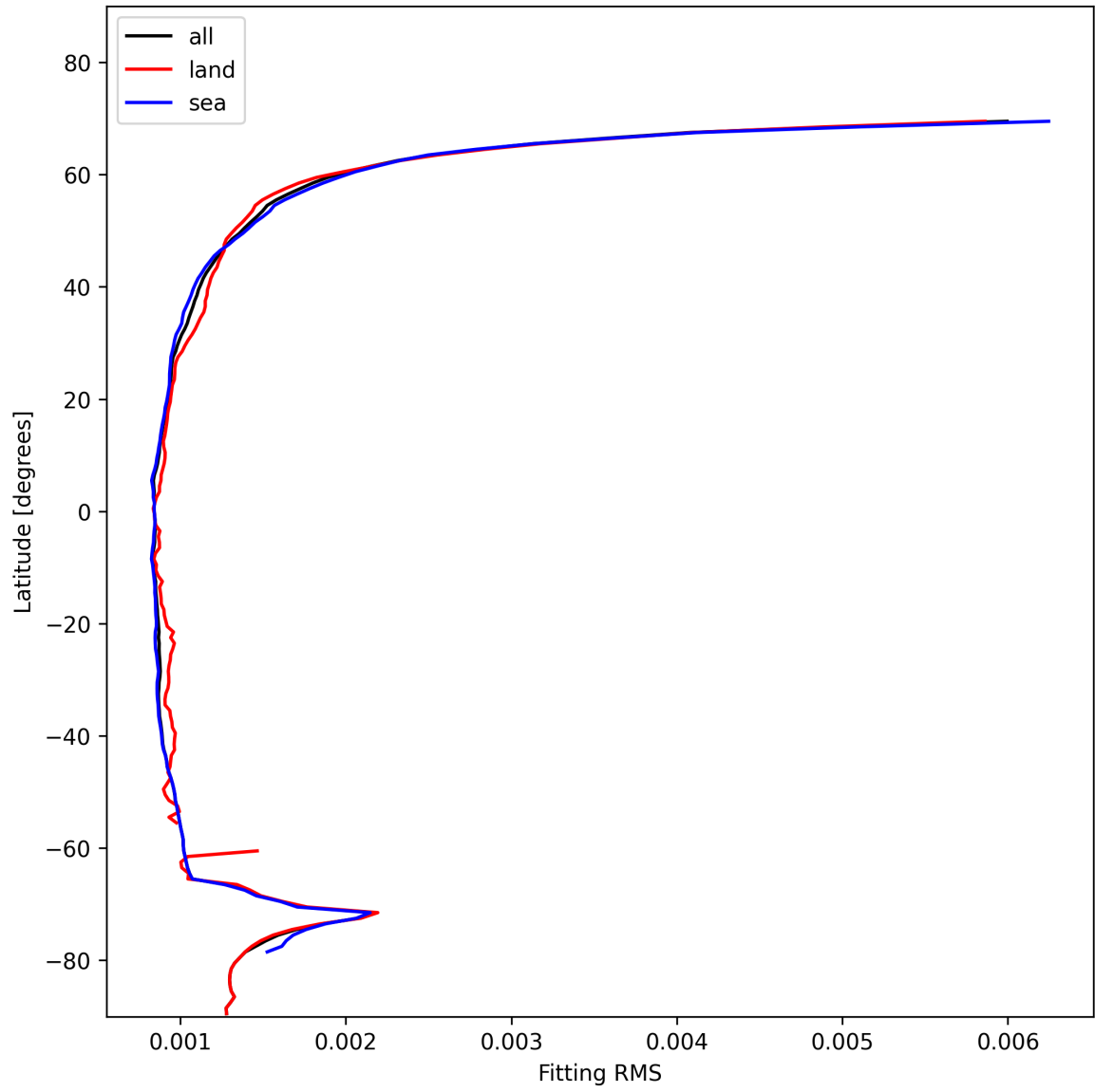
Figure 16: Zonal average of “Fitting RMS” for 2025-01-21 to 2025-01-23.
