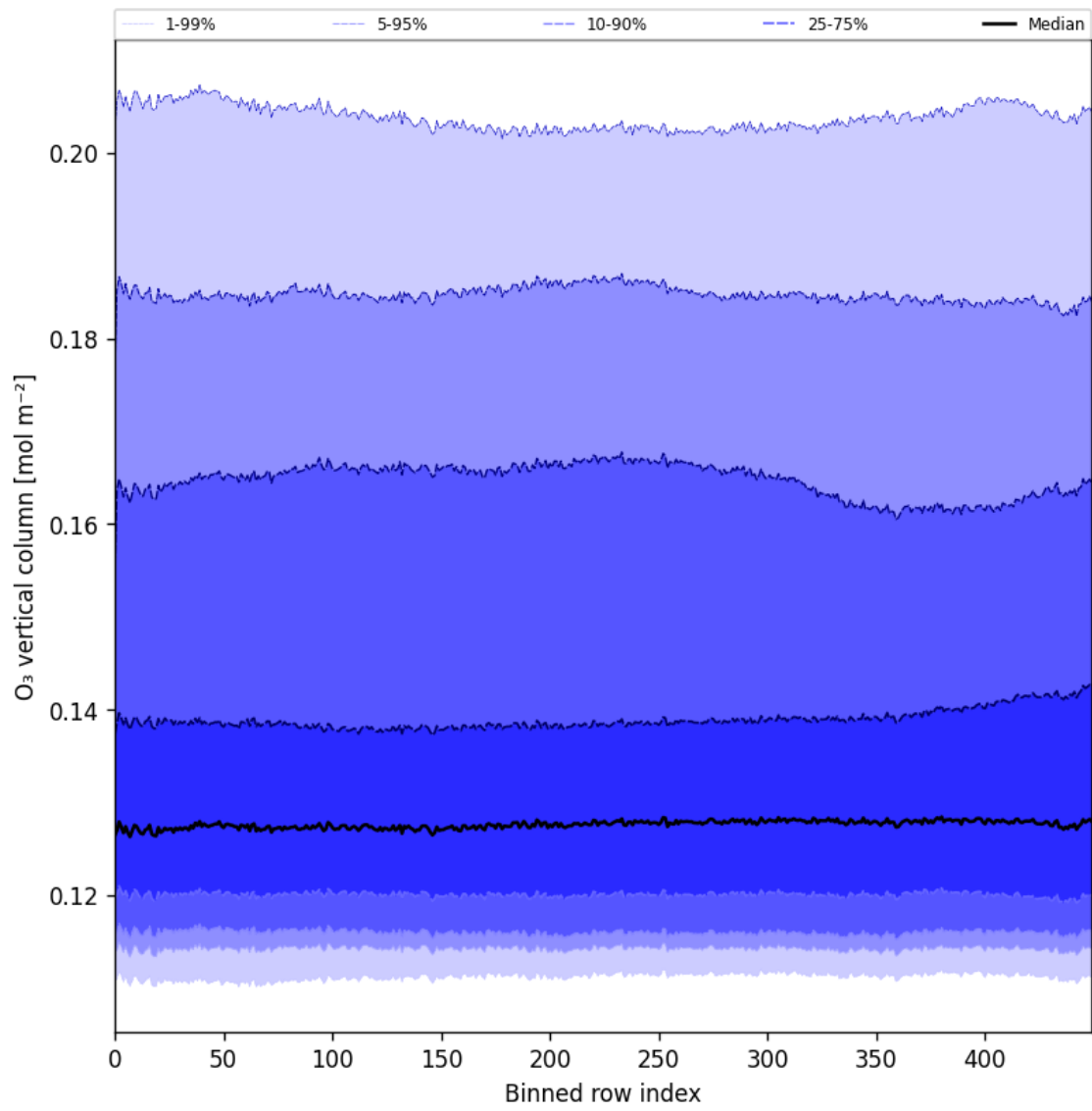
Figure 28: Along track statistics of “O 3 vertical column” for 2025-01-21 to 2025-01-23
