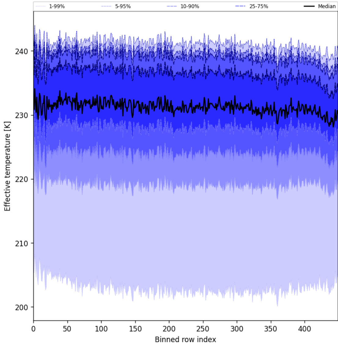
Figure 31: Along track statistics of “Effective temperature” for 2025-01-21 to 2025-01-23
