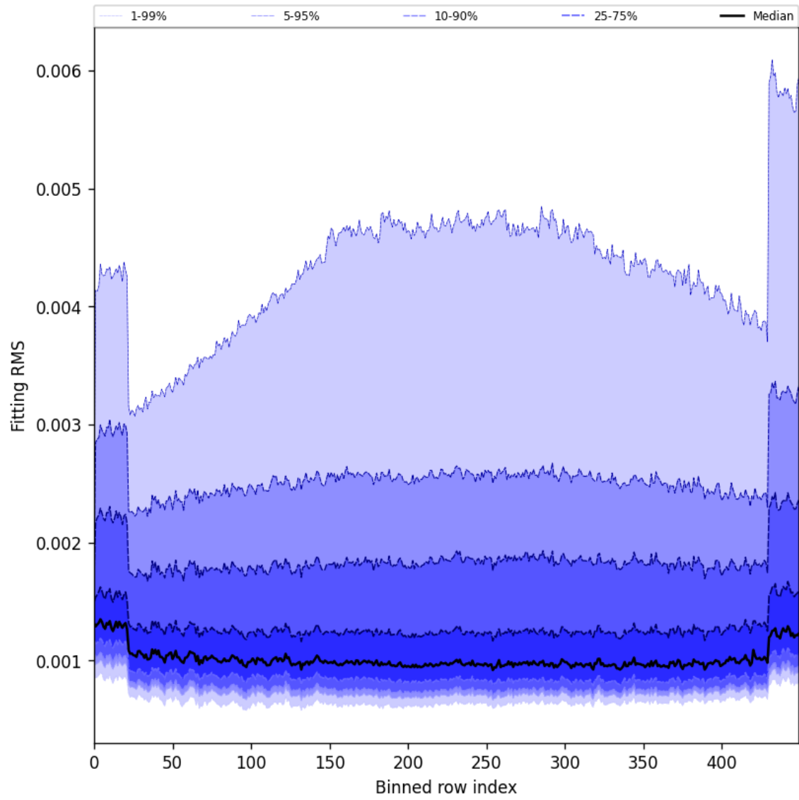
Figure 30: Along track statistics of “Fitting RMS” for 2025-01-21 to 2025-01-23
