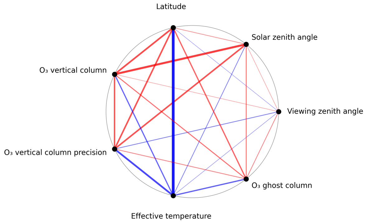
Figure 1: Map of correlation graph for 2025-01-21 to 2025-01-23.
