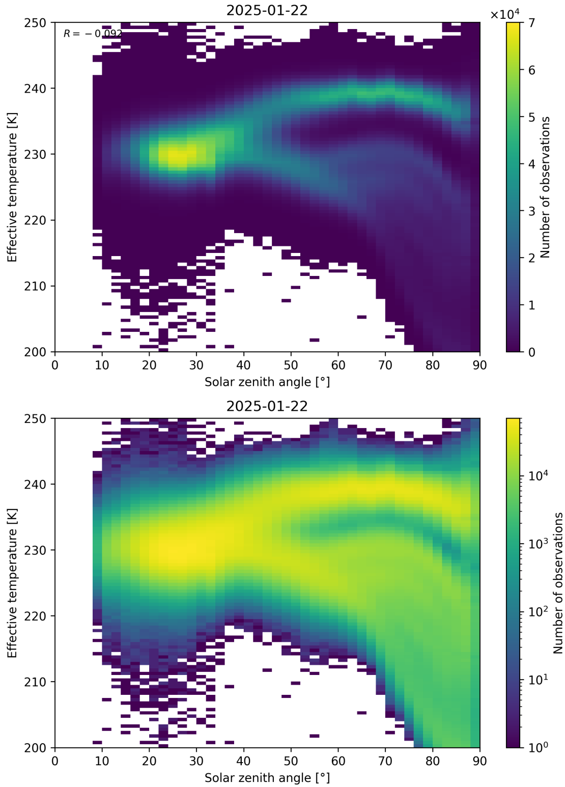
Figure 45: Scatter density plot of “Solar zenith angle” against “Effective temperature” for 2025-01-21 to 2025-01-23.
