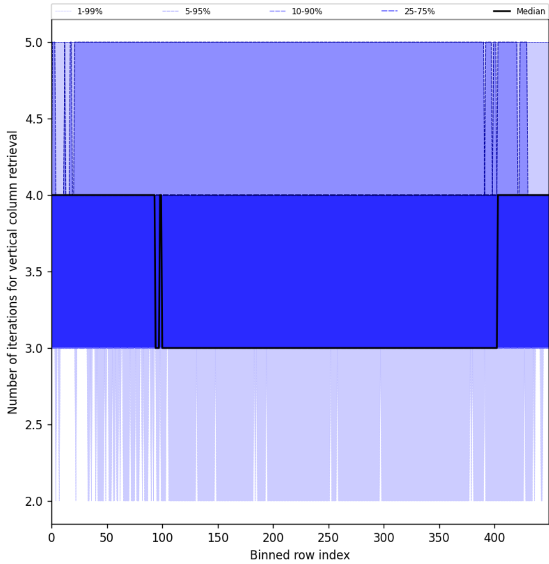
Figure 33: Along track statistics of “Number of iterations for vertical column retrieval” for 2025-01-21 to 2025-01-23
