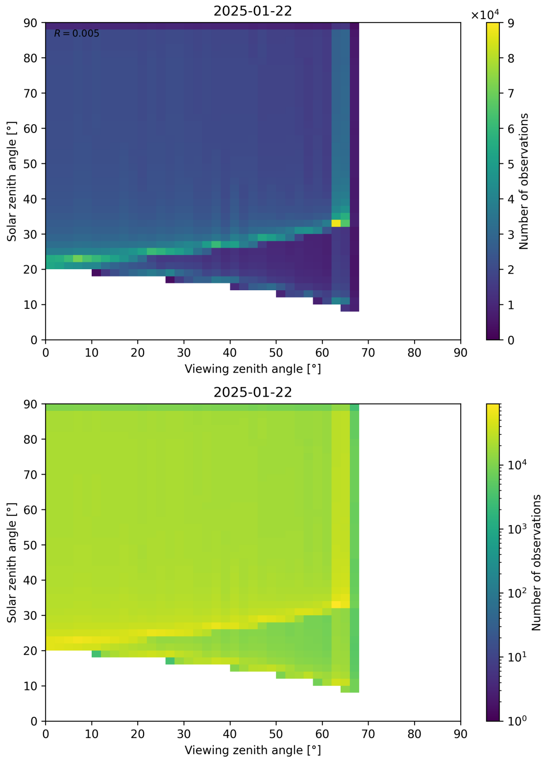
Figure 54: Scatter density plot of “Viewing zenith angle” against “Solar zenith angle” for 2025-01-21 to 2025-01-23.
