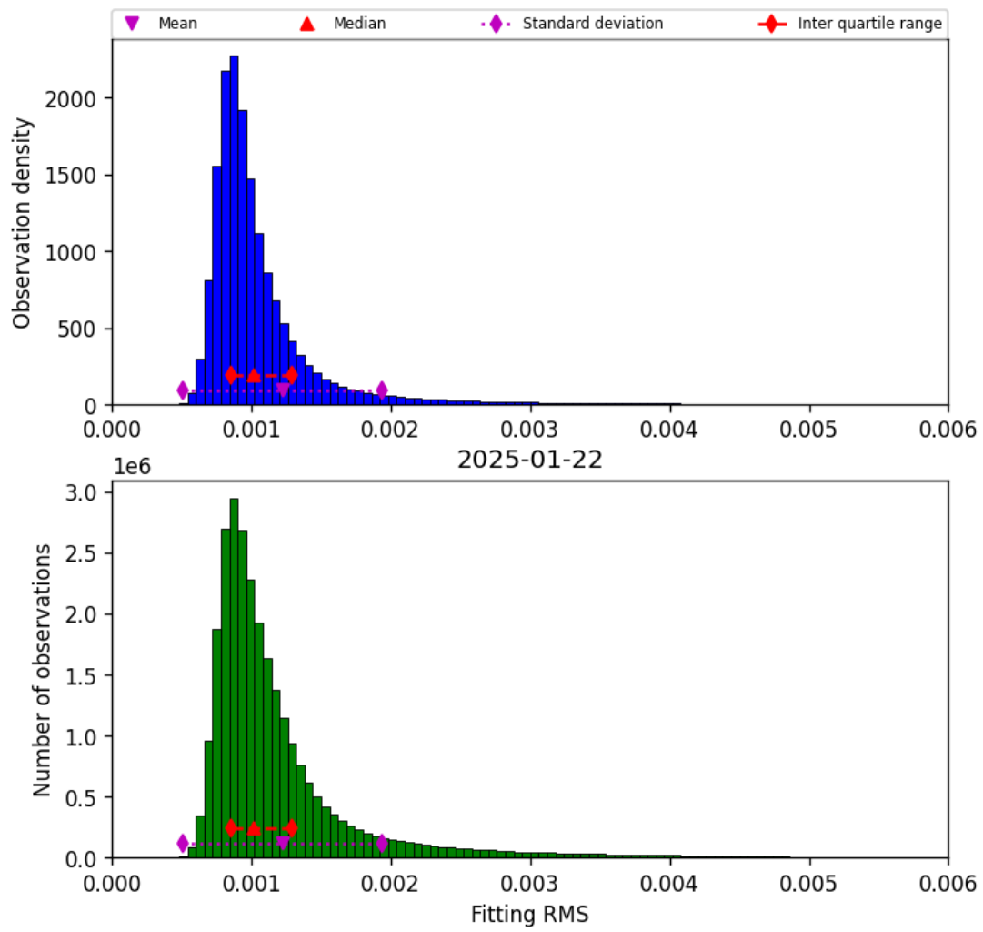
Figure 23: Histogram of “Fitting RMS” for 2025-01-21 to 2025-01-23
