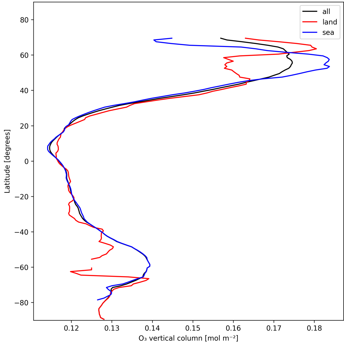
Figure 14: Zonal average of “O 3 vertical column” for 2025-01-21 to 2025-01-23.
