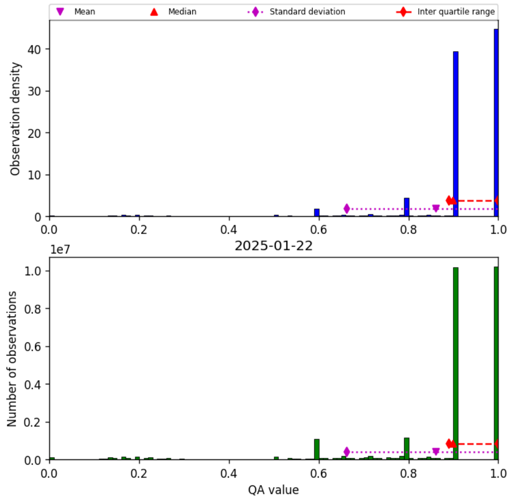
Figure 20: Histogram of “QA value” for 2025-01-21 to 2025-01-23
