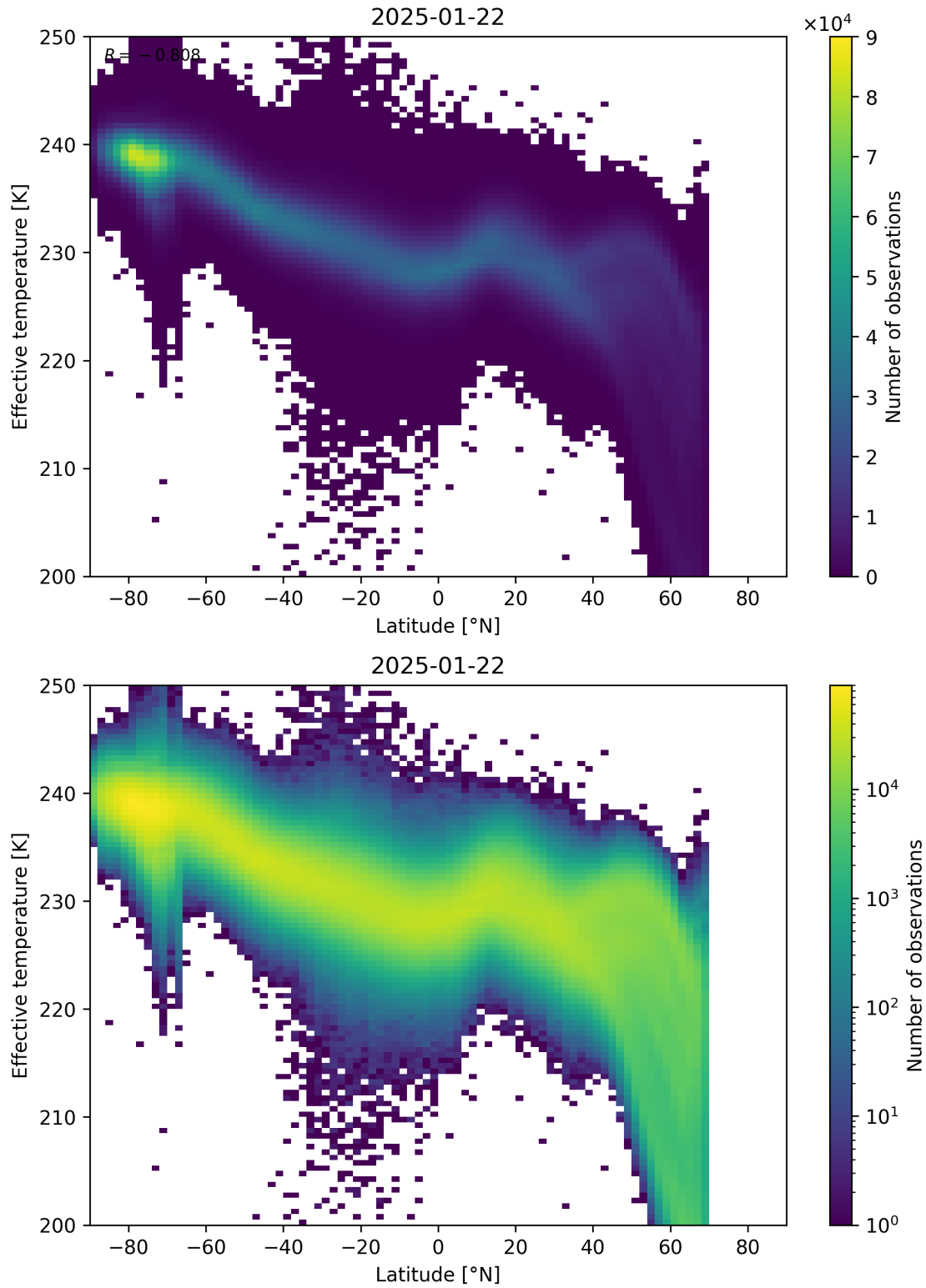
Figure 34: Scatter density plot of “Latitude” against “Effective temperature” for 2025-01-21 to 2025-01-23.
