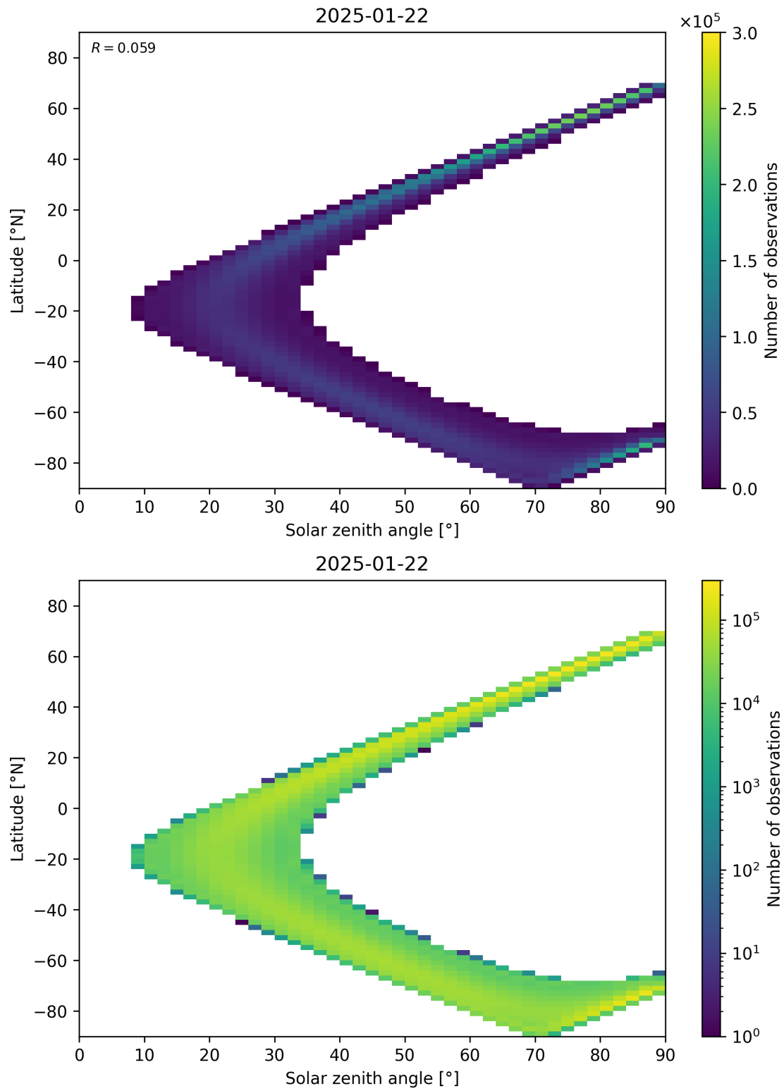
Figure 44: Scatter density plot of “Solar zenith angle” against “Latitude” for 2025-01-21 to 2025-01-23.
