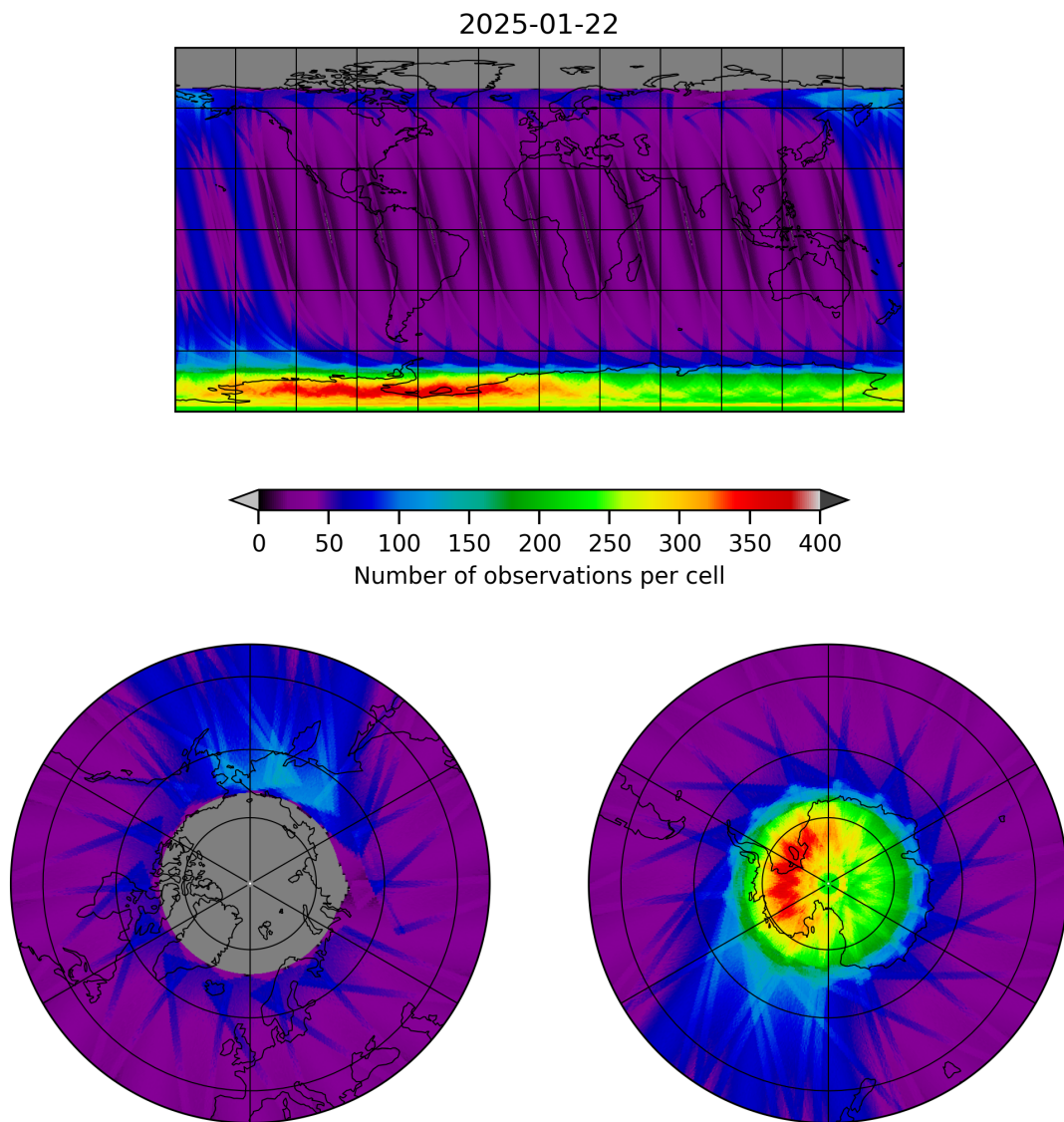
Figure 12: Map of the number of observations for 2025-01-21 to 2025-01-23
