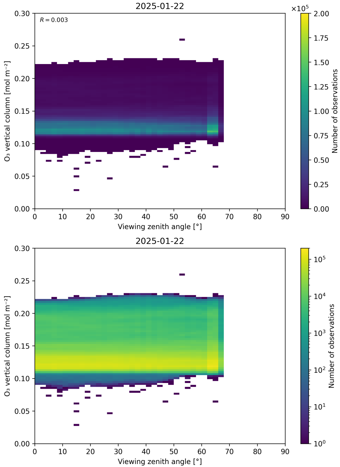
Figure 52: Scatter density plot of “Viewing zenith angle” against “O 3 vertical column” for 2025-01-21 to 2025-01-23.
