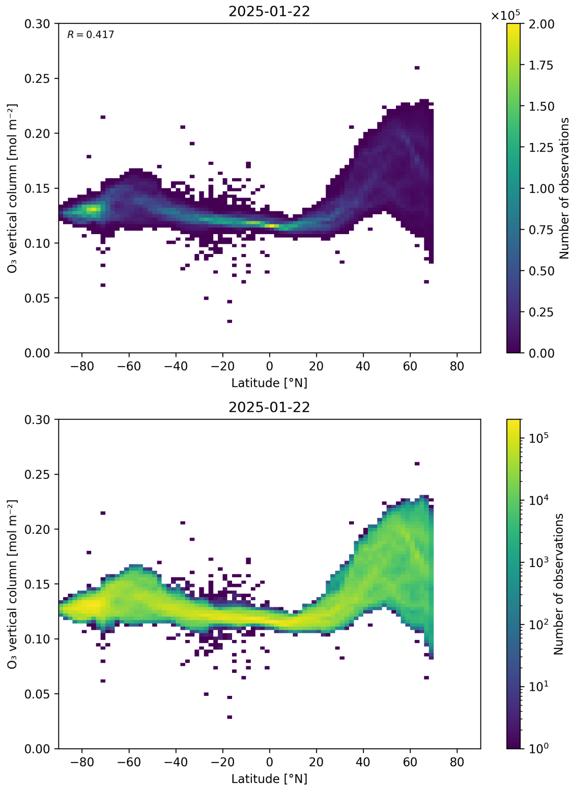
Figure 36: Scatter density plot of “Latitude” against “O 3 vertical column” for 2025-01-21 to 2025-01-23.
