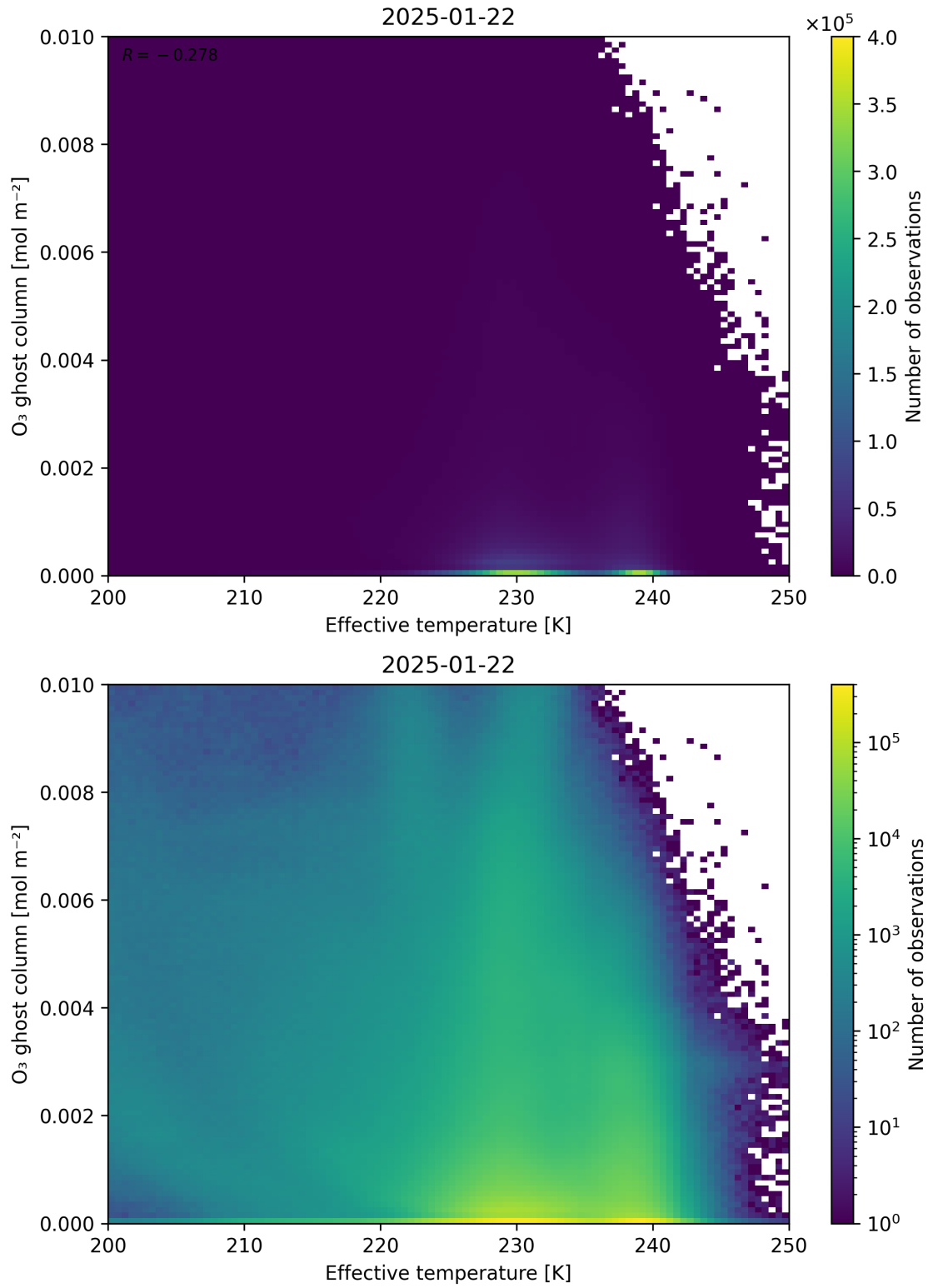
Figure 38: Scatter density plot of “Effective temperature” against “O 3 ghost column” for 2025-01-21 to 2025-01-23.
