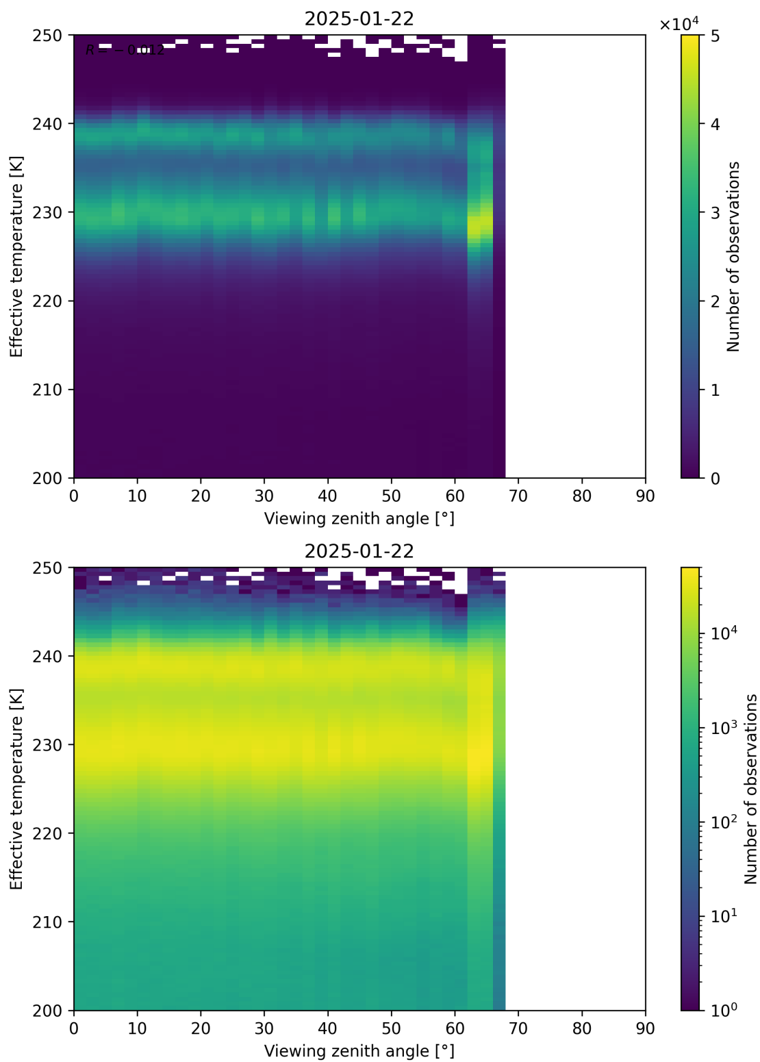
Figure 50: Scatter density plot of “Viewing zenith angle” against “Effective temperature” for 2025-01-21 to 2025-01-23.
