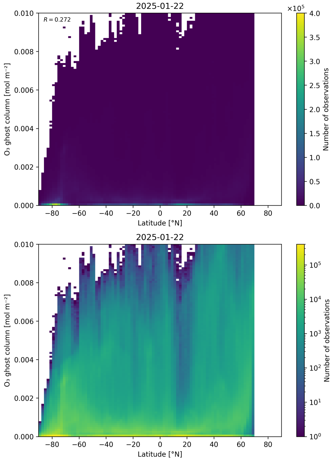
Figure 35: Scatter density plot of “Latitude” against “O 3 ghost column” for 2025-01-21 to 2025-01-23.
