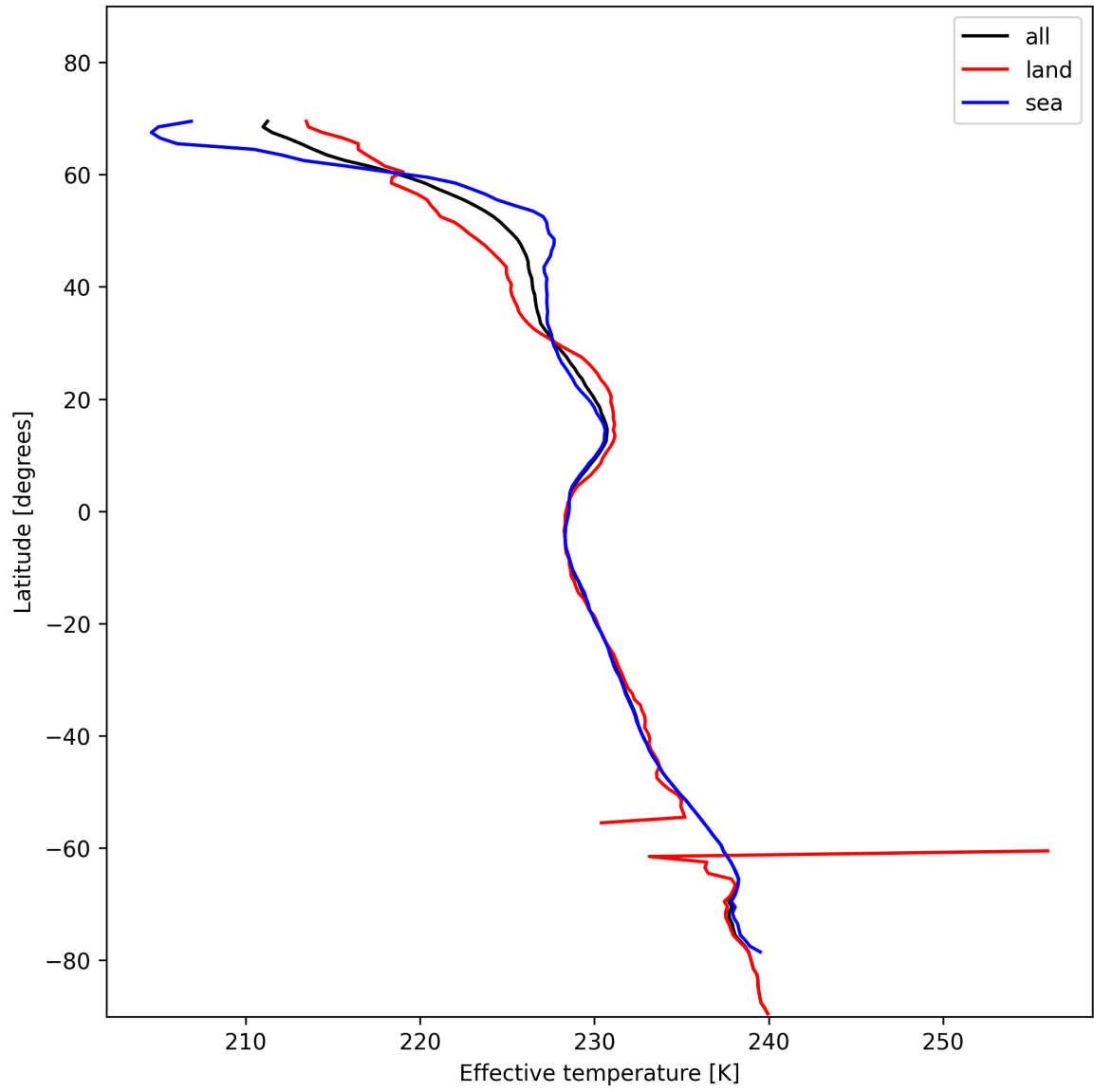
Figure 17: Zonal average of “Effective temperature” for 2025-01-21 to 2025-01-23.
