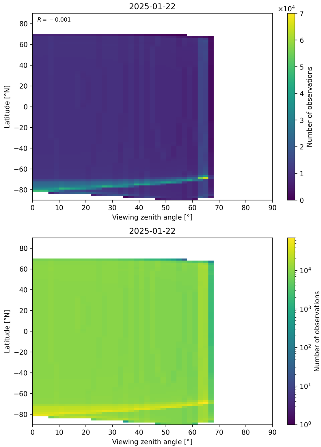
Figure 49: Scatter density plot of “Viewing zenith angle” against “Latitude” for 2025-01-21 to 2025-01-23.
