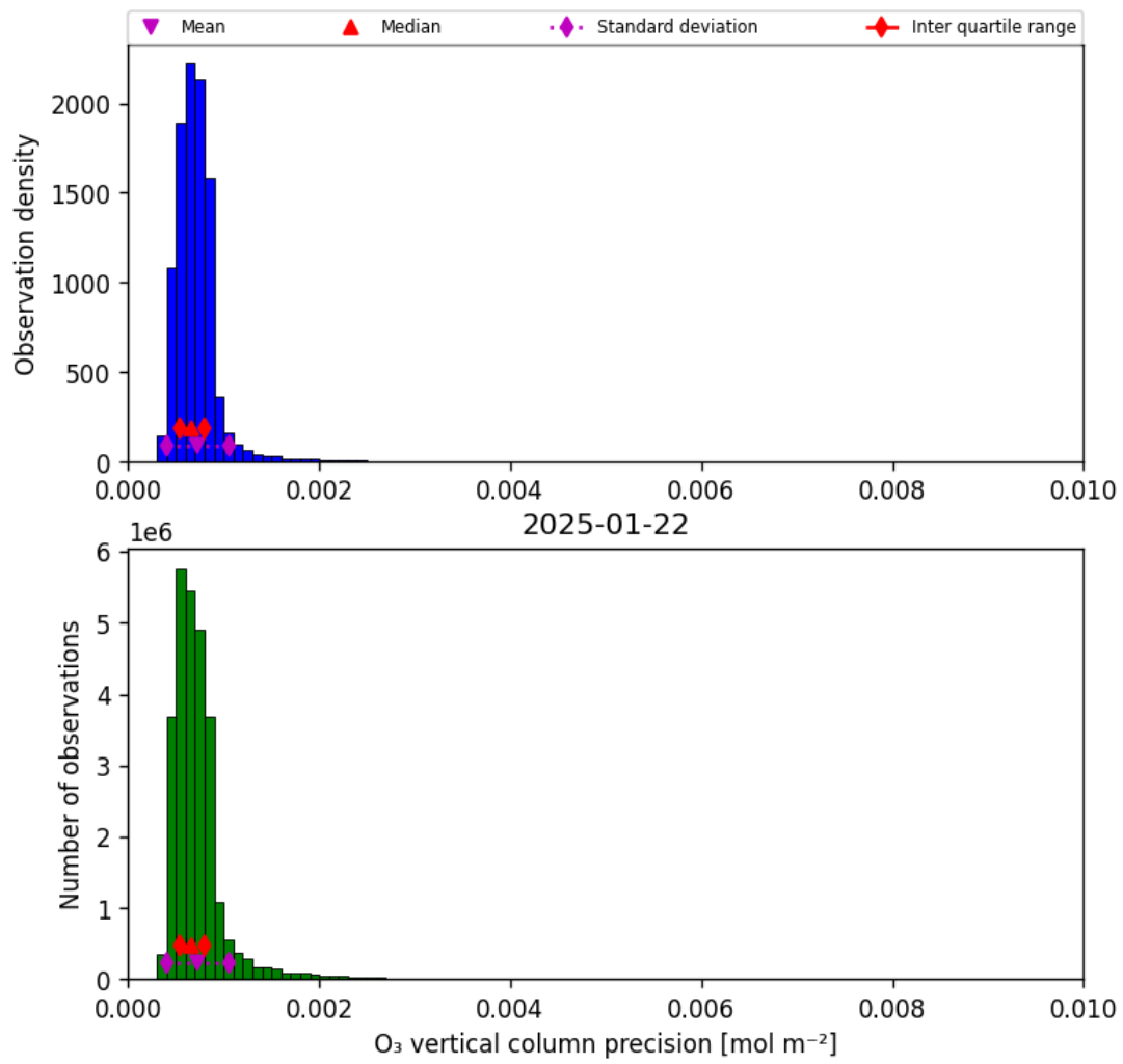
Figure 22: Histogram of “O 3 vertical column precision” for 2025-01-21 to 2025-01-23
