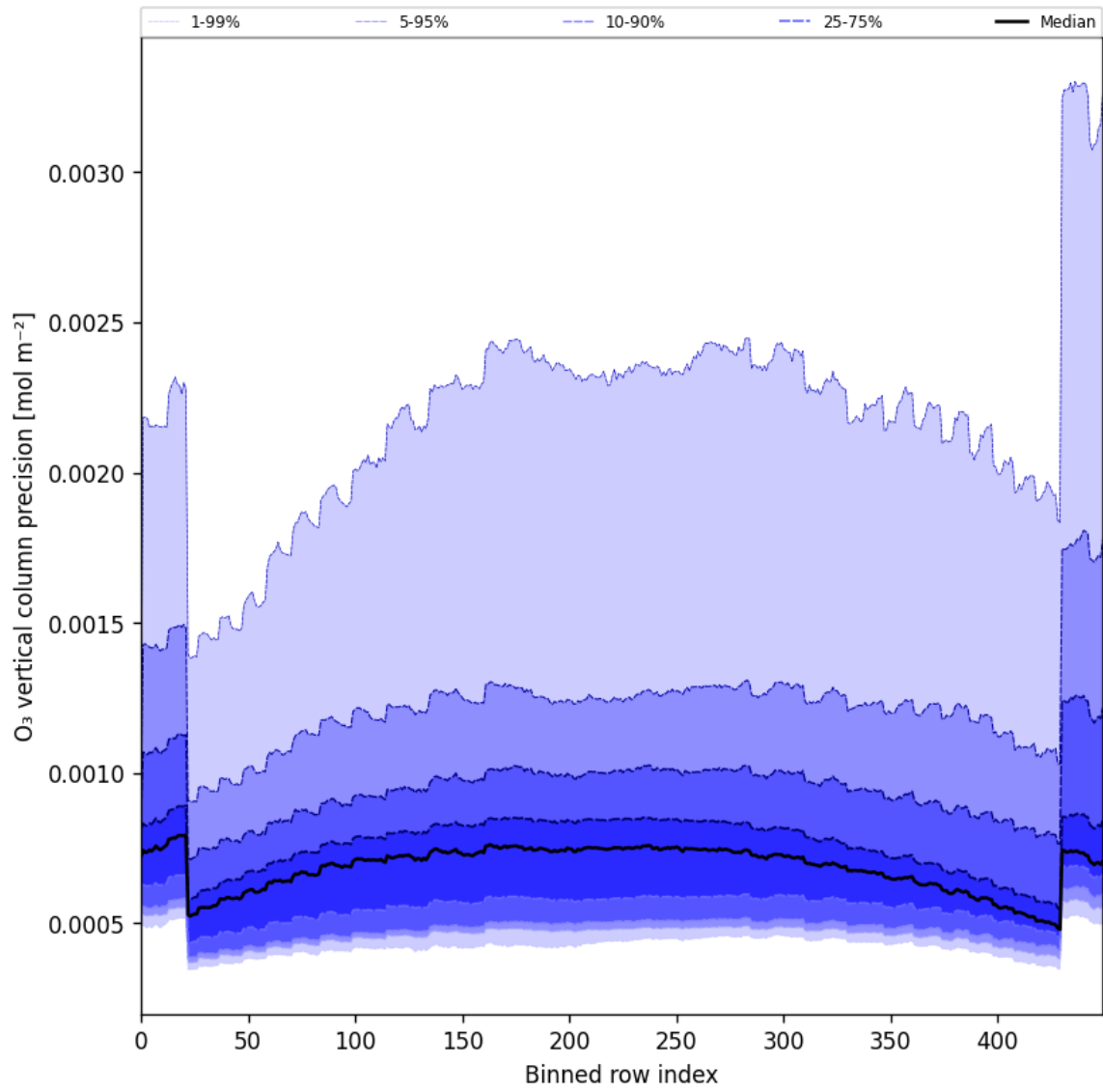
Figure 29: Along track statistics of “O 3 vertical column precision” for 2025-01-21 to 2025-01-23
