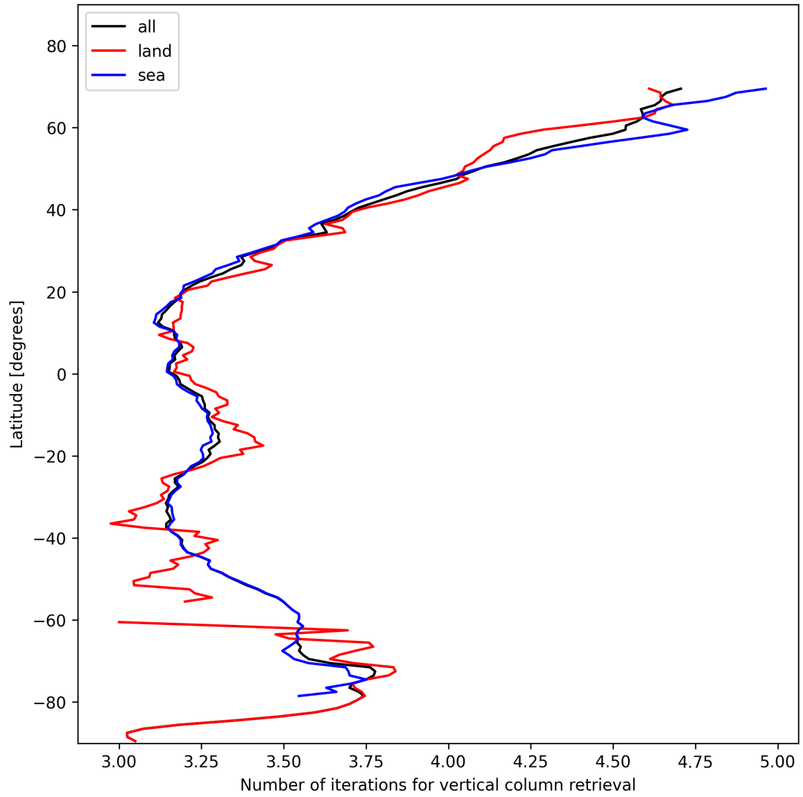
Figure 19: Zonal average of “Number of iterations for vertical column retrieval” for 2025-01-21 to 2025-01-23.
