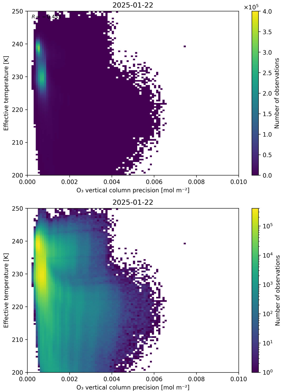
Figure 42: Scatter density plot of “O 3 vertical column precision” against “Effective temperature” for 2025-01-21 to 2025-01-23.
