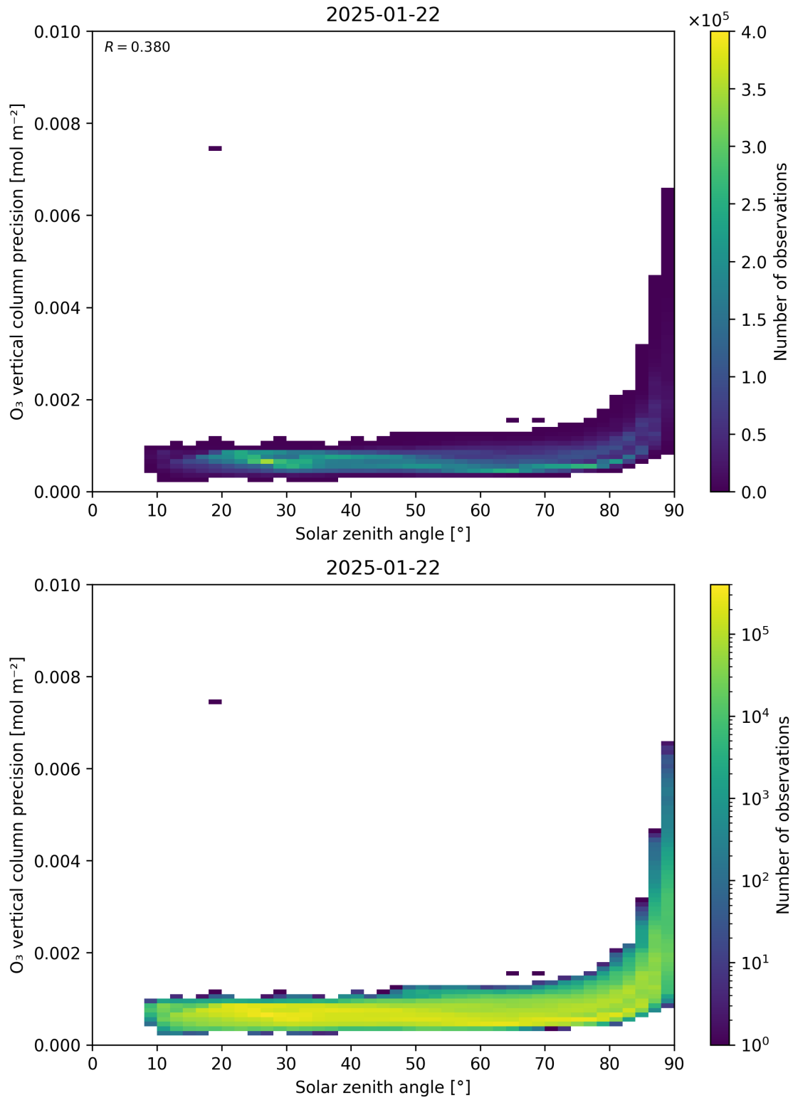
Figure 48: Scatter density plot of “Solar zenith angle” against “O 3 vertical column precision” for 2025-01-21 to 2025-01-23.
