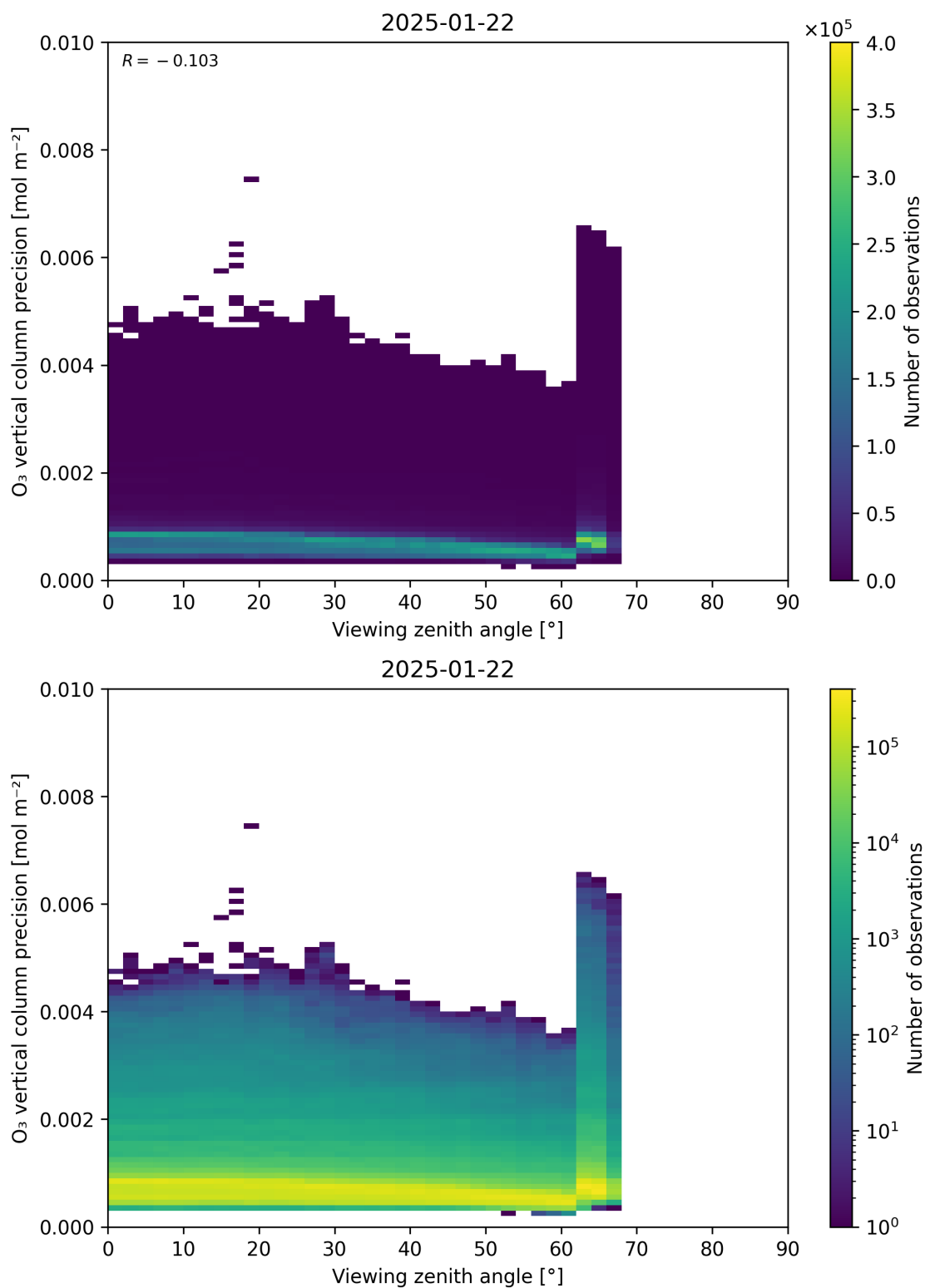
Figure 53: Scatter density plot of “Viewing zenith angle” against “O 3 vertical column precision” for 2025-01-21 to 2025-01-23.
