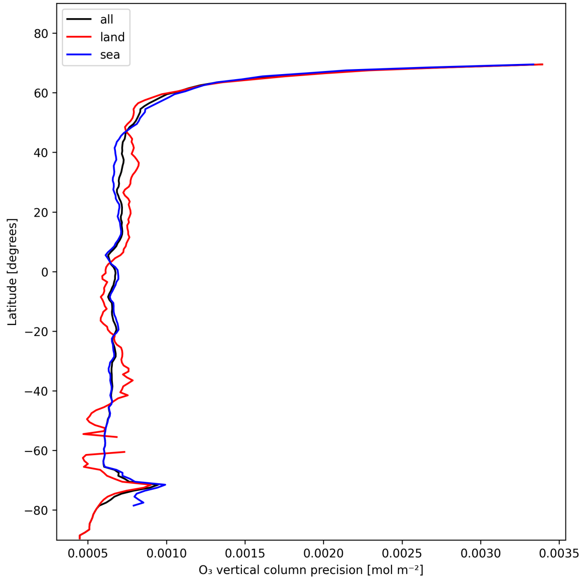
Figure 15: Zonal average of “O 3 vertical column precision” for 2025-01-21 to 2025-01-23.
