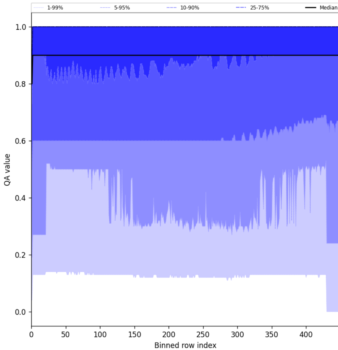
Figure 27: Along track statistics of “QA value” for 2025-01-21 to 2025-01-23
