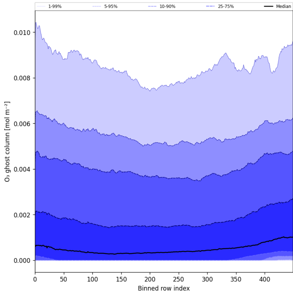
Figure 32: Along track statistics of “O 3 ghost column” for 2025-01-21 to 2025-01-23
