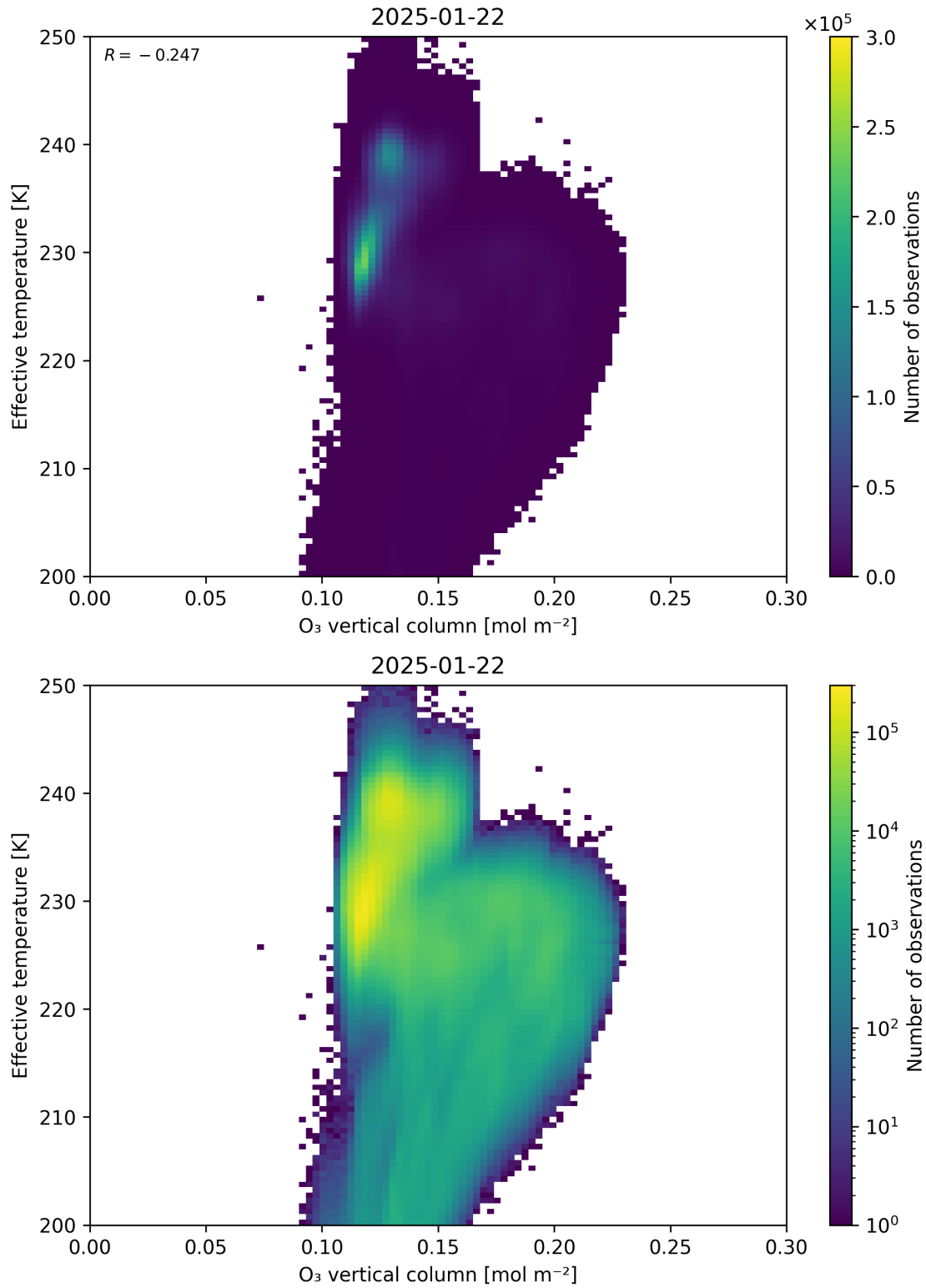
Figure 39: Scatter density plot of “O 3 vertical column” against “Effective temperature” for 2025-01-21 to 2025-01-23.
