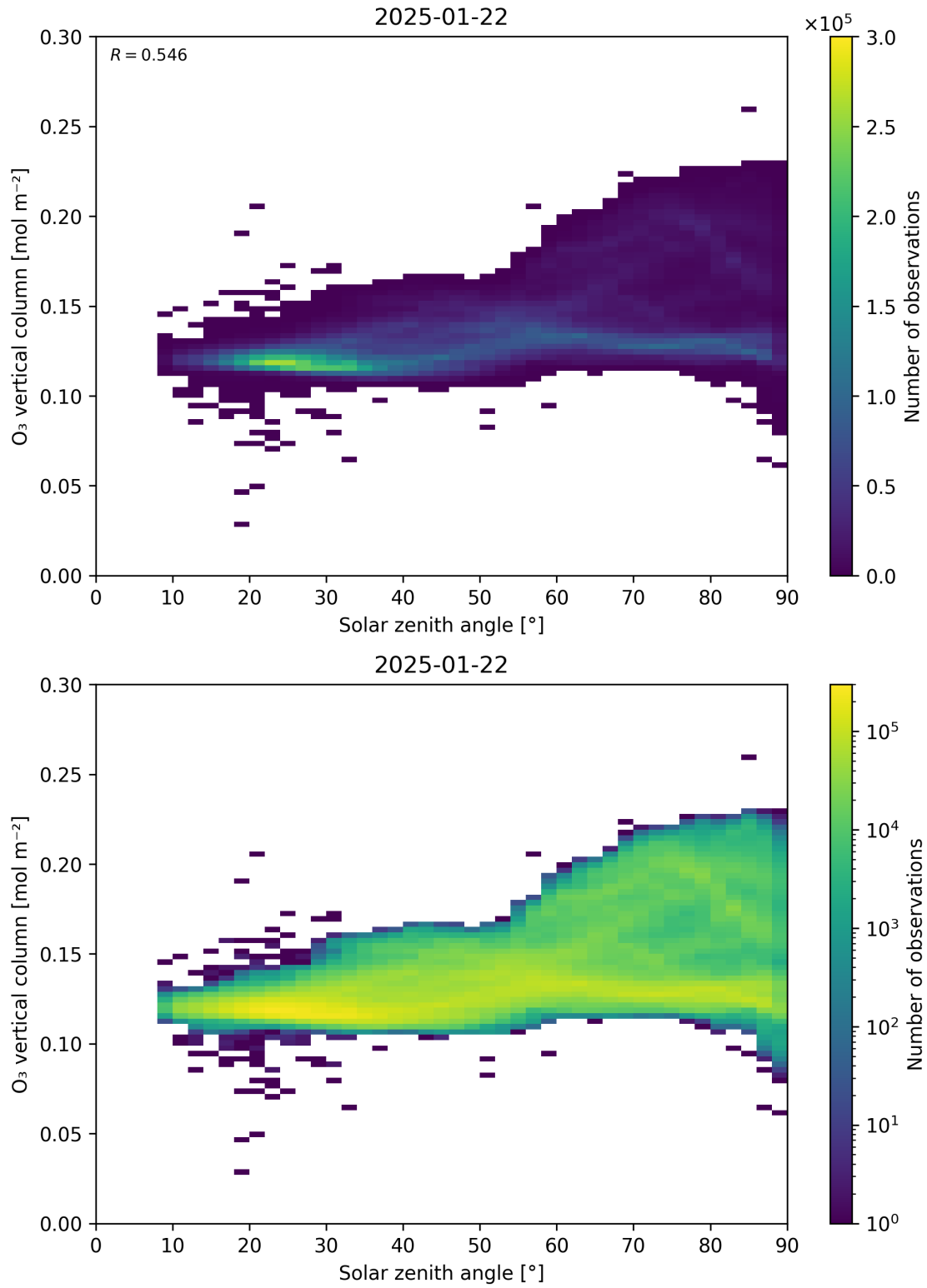
Figure 47: Scatter density plot of “Solar zenith angle” against “O 3 vertical column” for 2025-01-21 to 2025-01-23.
