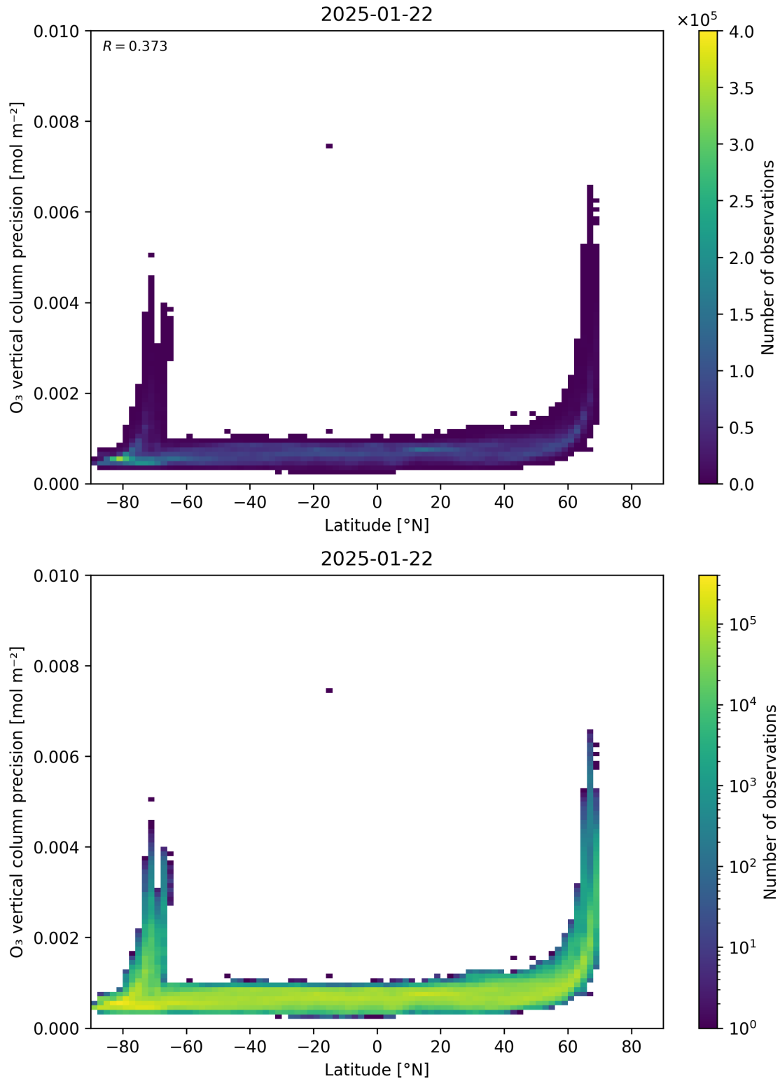
Figure 37: Scatter density plot of “Latitude” against “O 3 vertical column precision” for 2025-01-21 to 2025-01-23.
