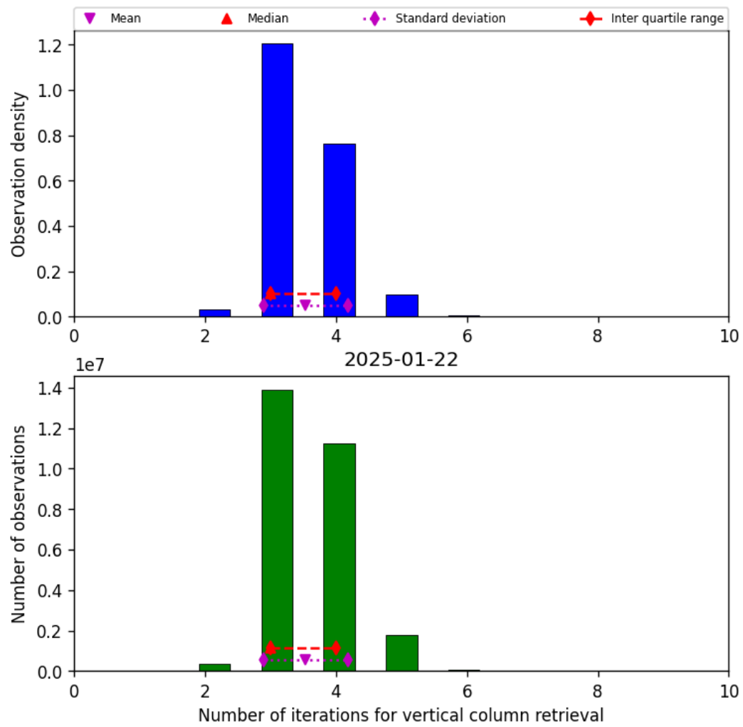
Figure 26: Histogram of “Number of iterations for vertical column retrieval” for 2025-01-21 to 2025-01-23
