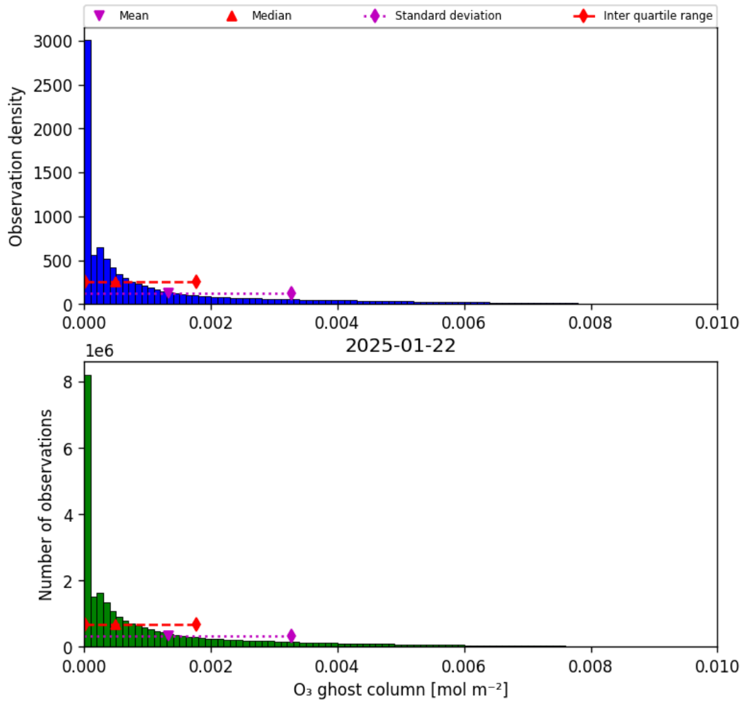
Figure 25: Histogram of “O 3 ghost column” for 2025-01-21 to 2025-01-23
