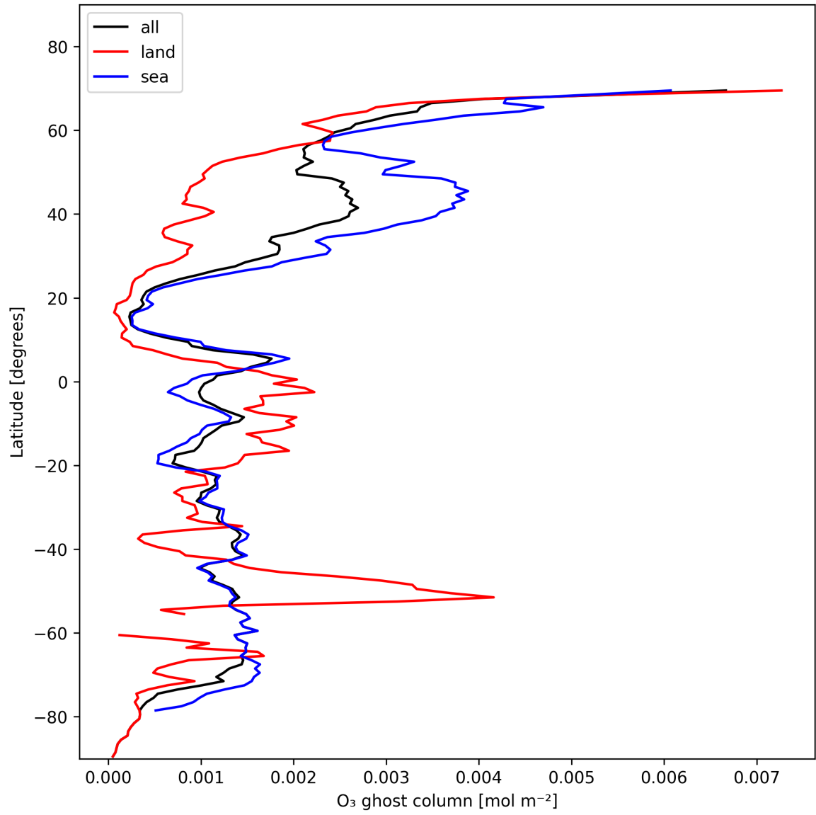
Figure 18: Zonal average of “O 3 ghost column” for 2025-01-21 to 2025-01-23.
