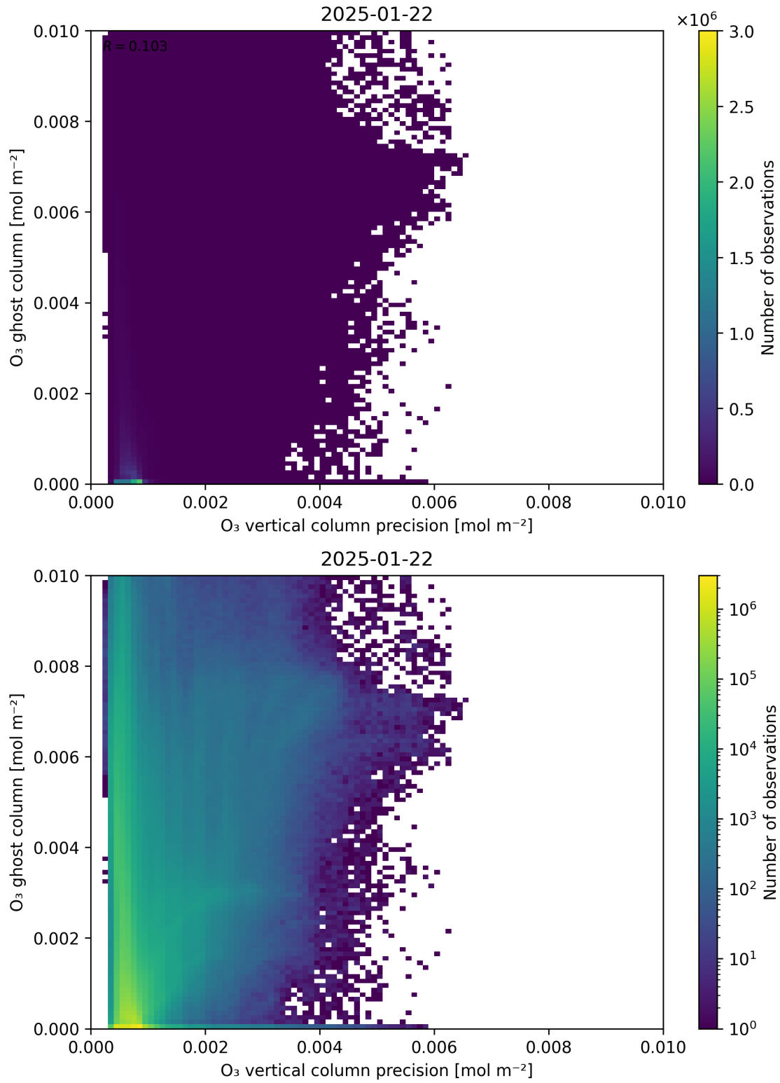
Figure 43: Scatter density plot of “O 3 vertical column precision” against “O 3 ghost column” for 2025-01-21 to 2025-01-23.
