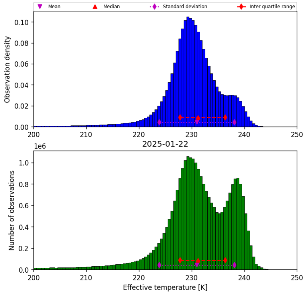
Figure 24: Histogram of “Effective temperature” for 2025-01-21 to 2025-01-23
