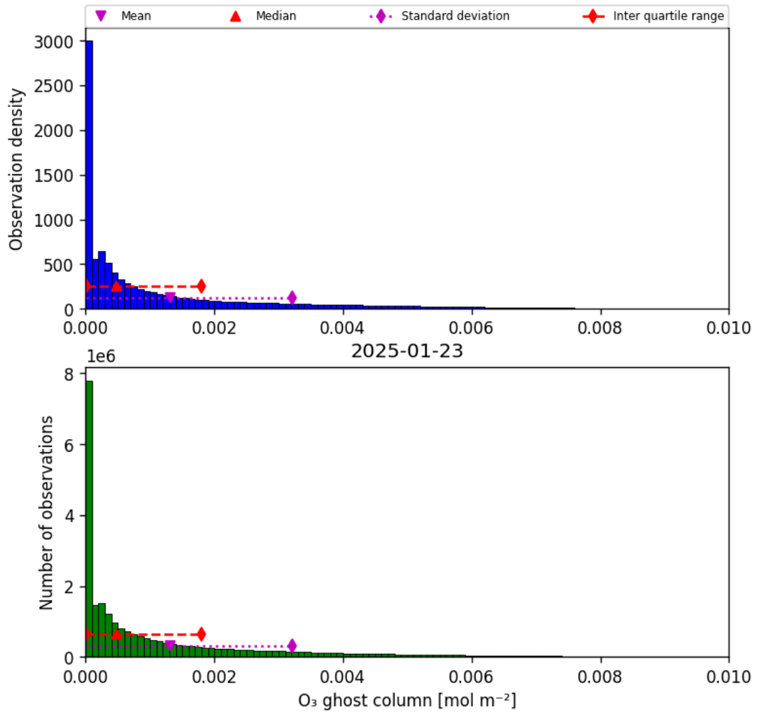
Figure 25: Histogram of “O 3 ghost column” for 2025-01-23 to 2025-01-24
