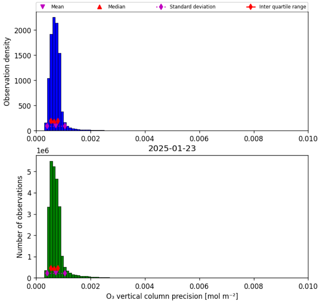
Figure 22: Histogram of “O 3 vertical column precision” for 2025-01-23 to 2025-01-24
