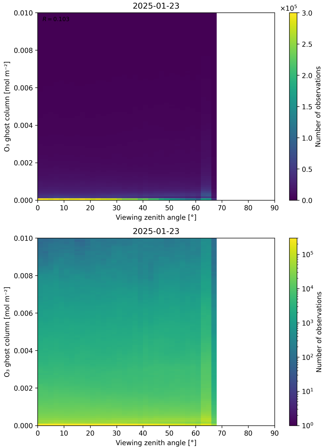
Figure 51: Scatter density plot of “Viewing zenith angle” against “O 3 ghost column” for 2025-01-23 to 2025-01-24.
