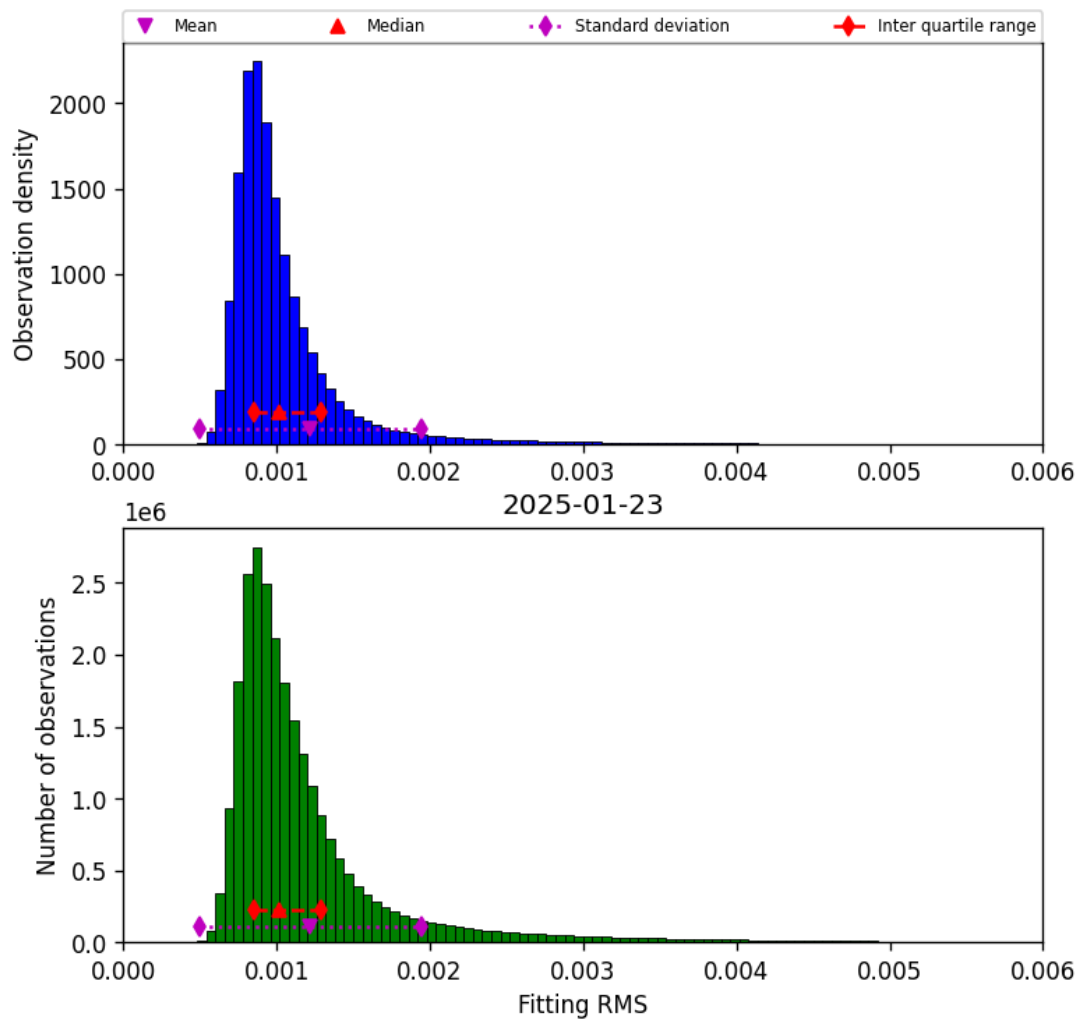
Figure 23: Histogram of “Fitting RMS” for 2025-01-23 to 2025-01-24
