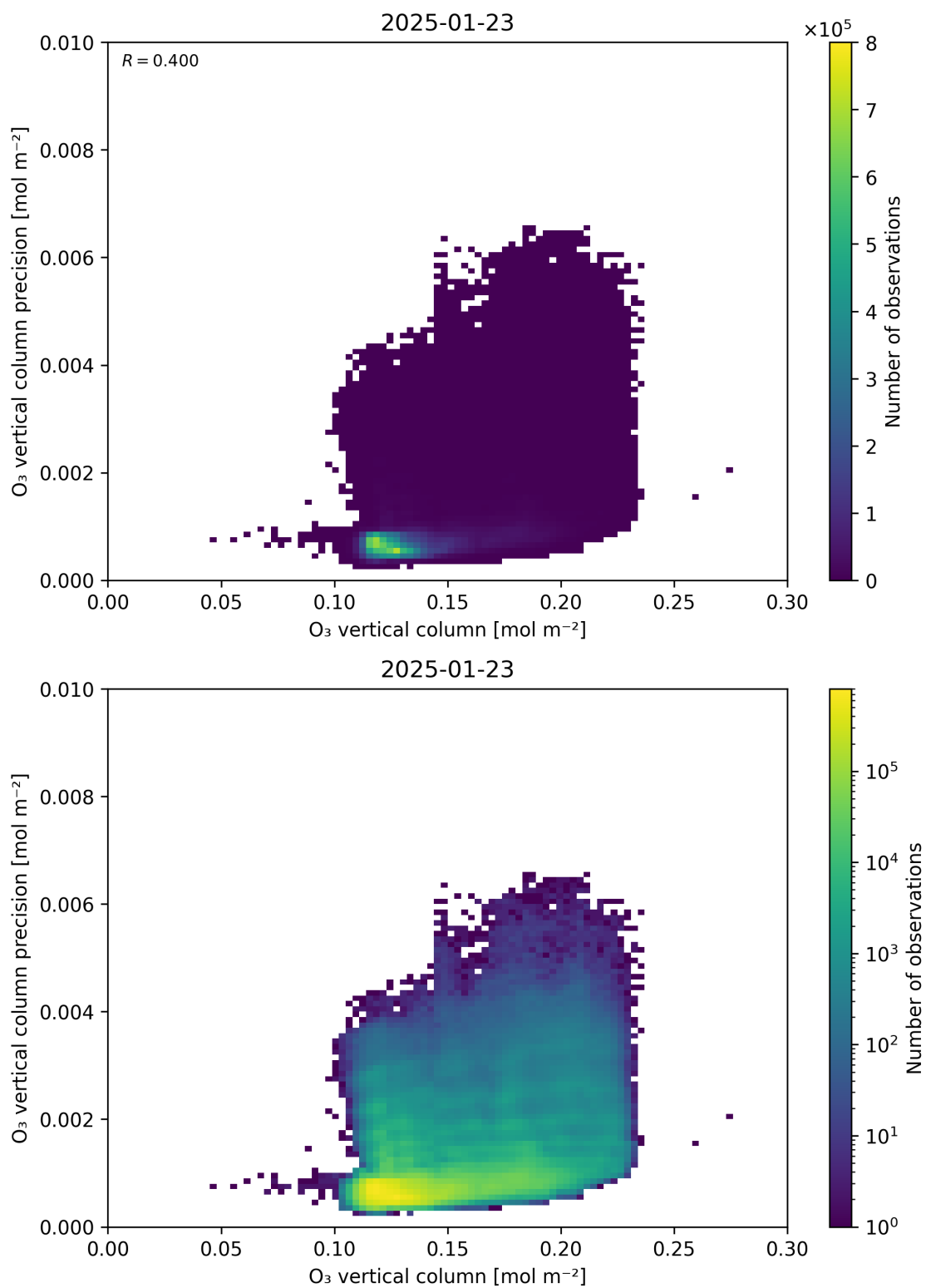
Figure 41: Scatter density plot of “O 3 vertical column” against “O 3 vertical column precision” for 2025-01-23 to 2025-01-24.
