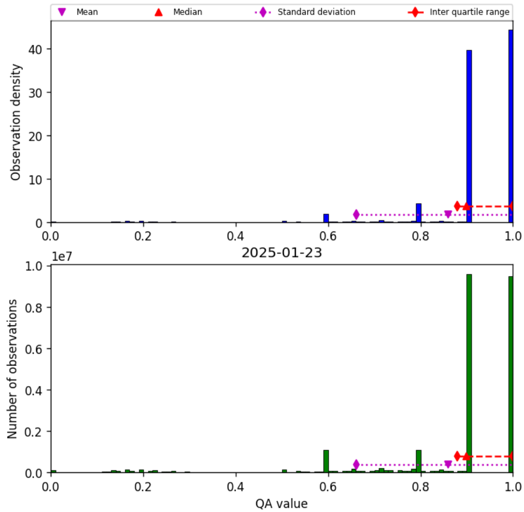
Figure 20: Histogram of “QA value” for 2025-01-23 to 2025-01-24
