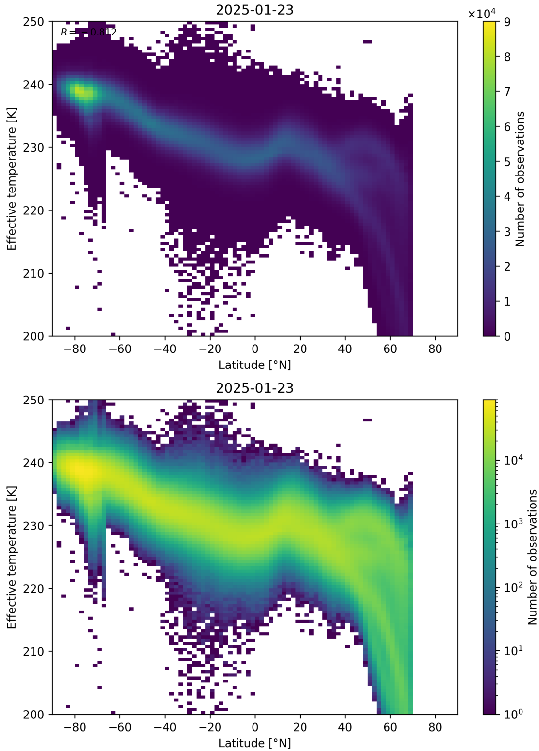
Figure 34: Scatter density plot of “Latitude” against “Effective temperature” for 2025-01-23 to 2025-01-24.
