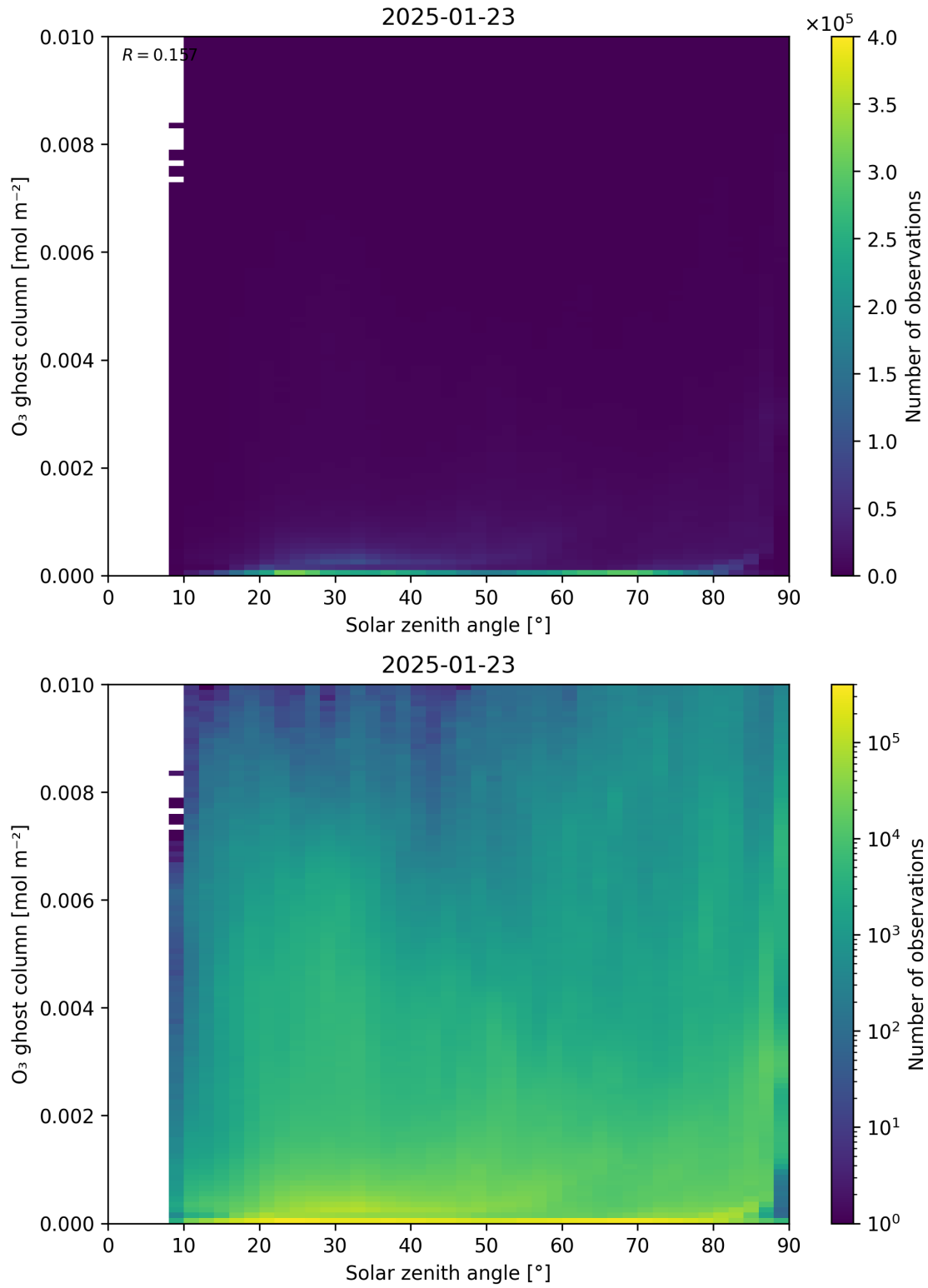
Figure 46: Scatter density plot of “Solar zenith angle” against “O 3 ghost column” for 2025-01-23 to 2025-01-24.
