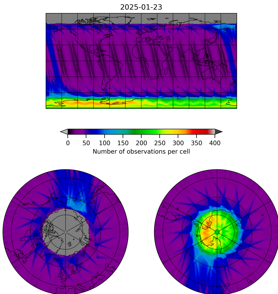
Figure 12: Map of the number of observations for 2025-01-23 to 2025-01-24
