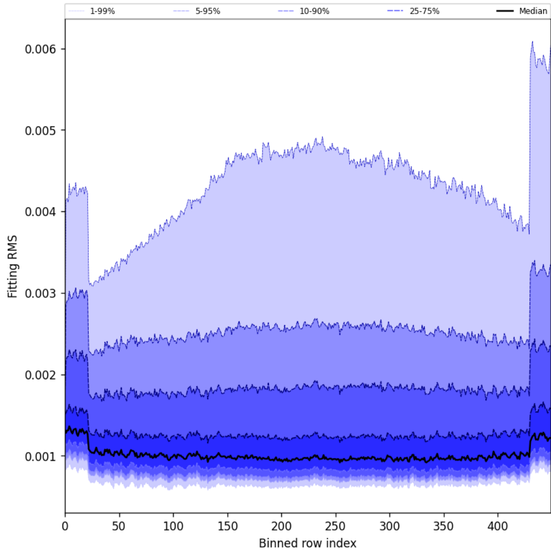
Figure 30: Along track statistics of “Fitting RMS” for 2025-01-23 to 2025-01-24
