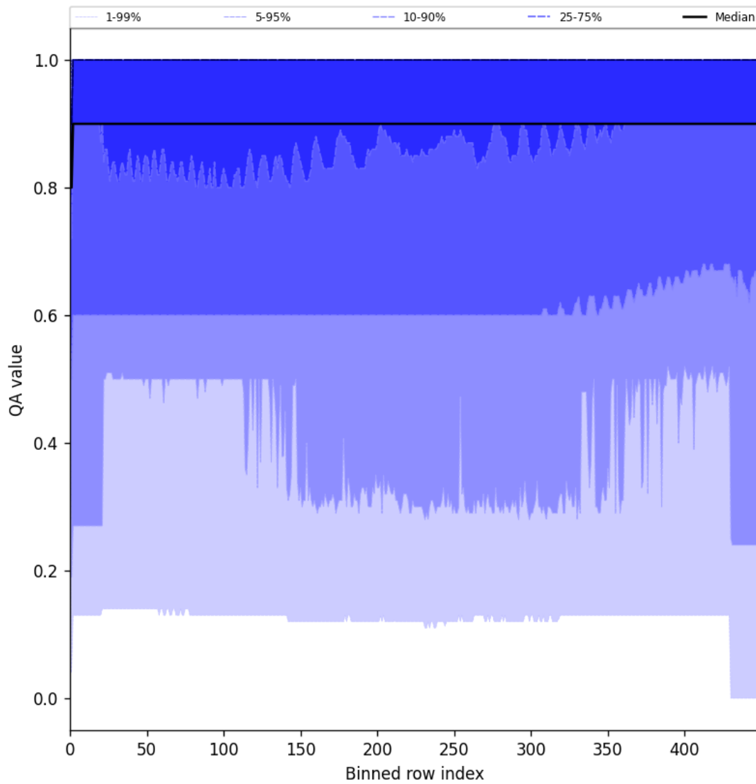
Figure 27: Along track statistics of “QA value” for 2025-01-23 to 2025-01-24
