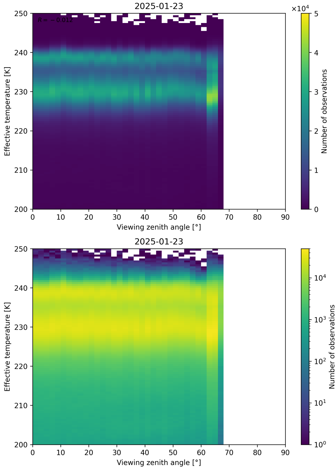
Figure 50: Scatter density plot of “Viewing zenith angle” against “Effective temperature” for 2025-01-23 to 2025-01-24.
