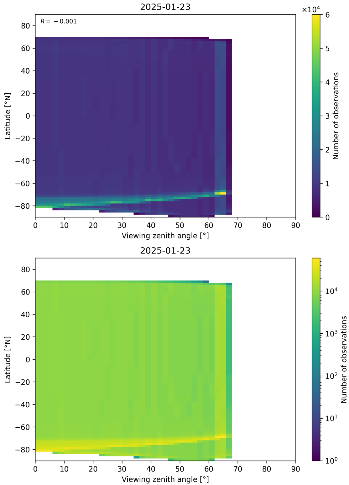
Figure 49: Scatter density plot of “Viewing zenith angle” against “Latitude” for 2025-01-23 to 2025-01-24.
