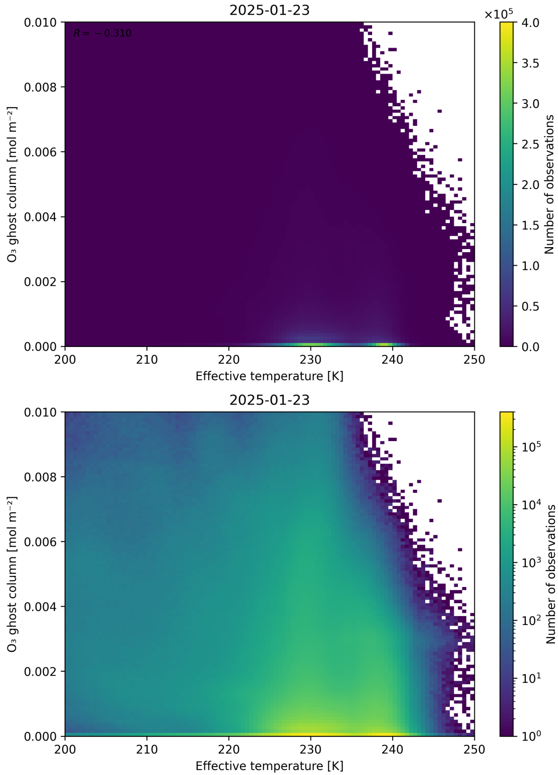
Figure 38: Scatter density plot of “Effective temperature” against “O 3 ghost column” for 2025-01-23 to 2025-01-24.
