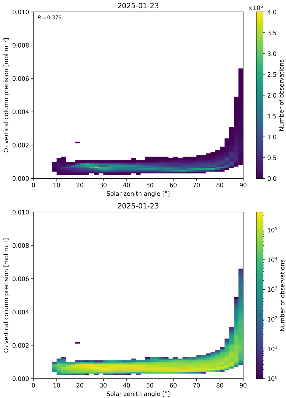
Figure 48: Scatter density plot of “Solar zenith angle” against “O 3 vertical column precision” for 2025-01-23 to 2025-01-24.
