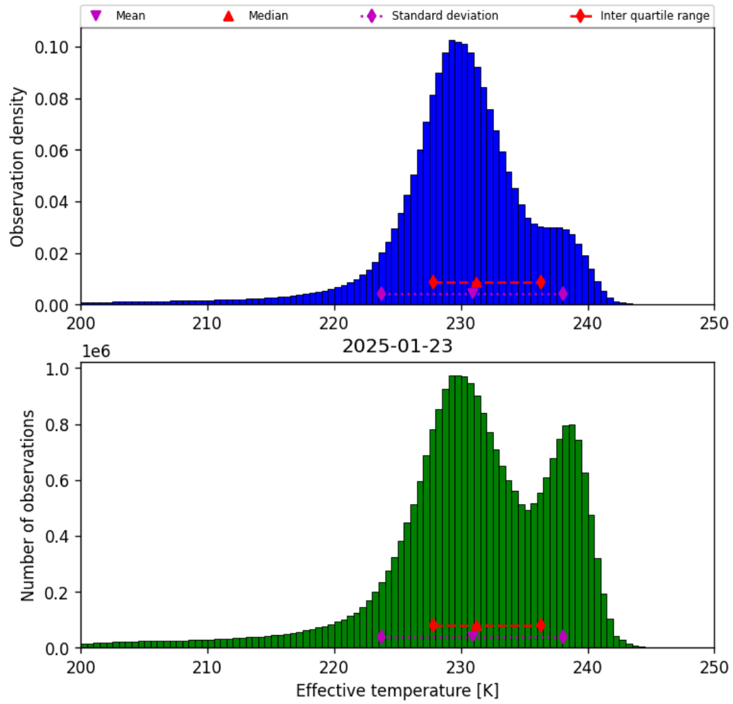
Figure 24: Histogram of “Effective temperature” for 2025-01-23 to 2025-01-24
