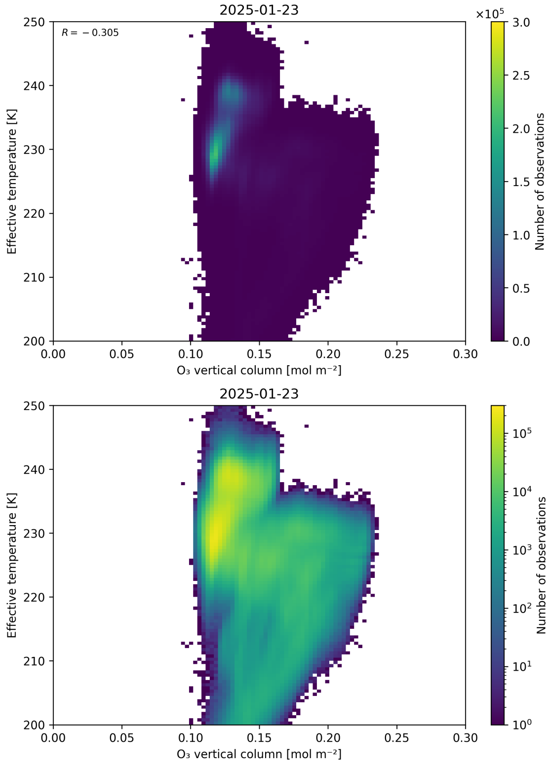
Figure 39: Scatter density plot of “O 3 vertical column” against “Effective temperature” for 2025-01-23 to 2025-01-24.
