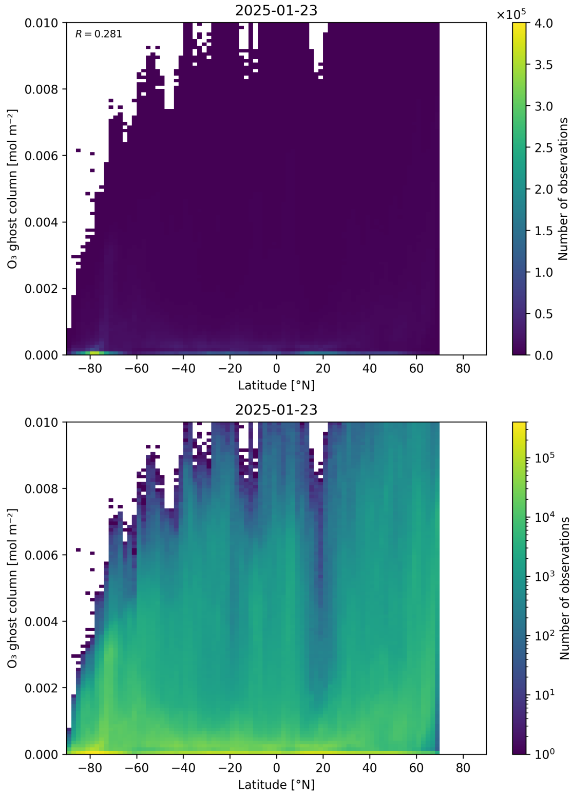
Figure 35: Scatter density plot of “Latitude” against “O 3 ghost column” for 2025-01-23 to 2025-01-24.
