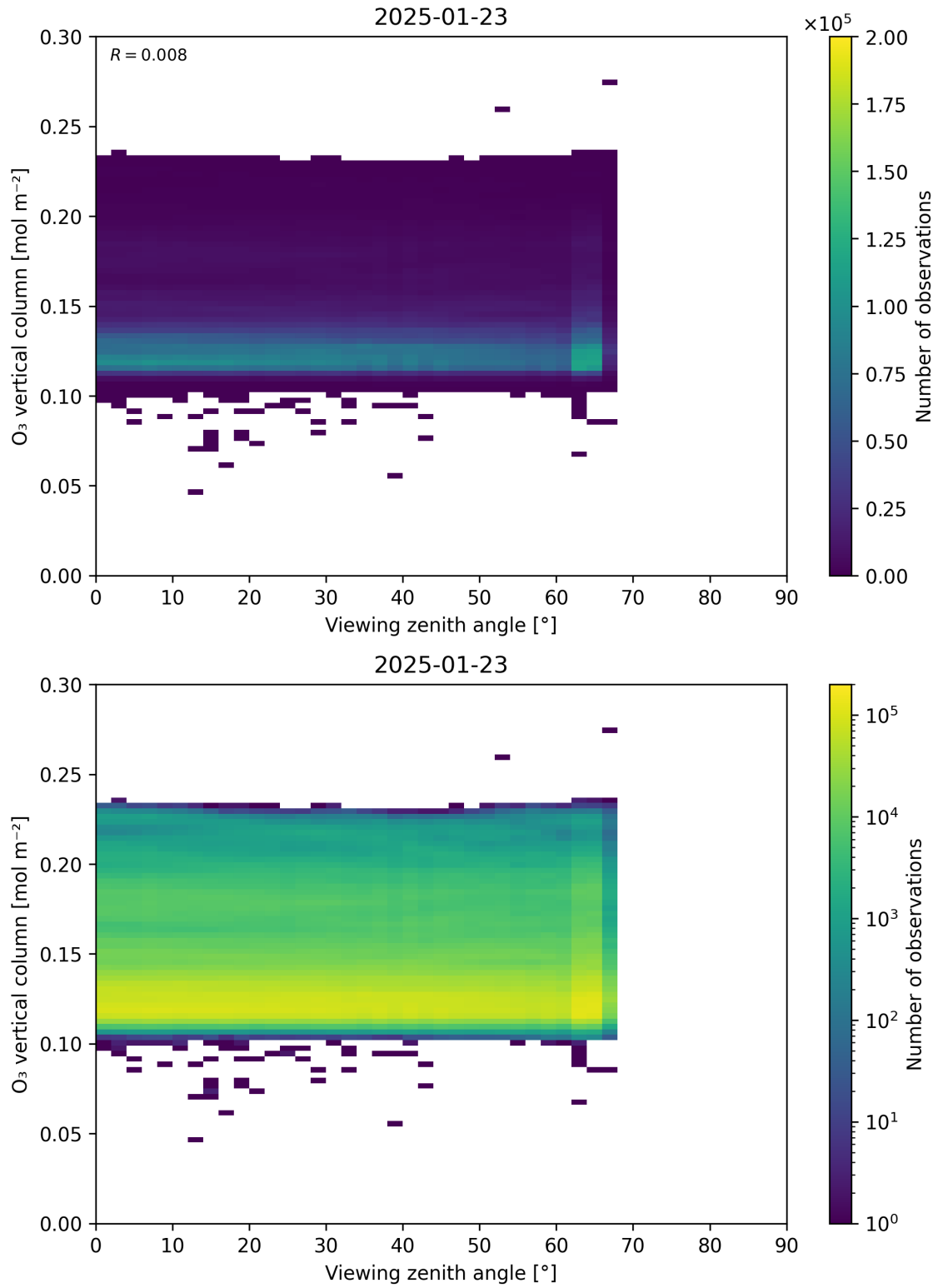
Figure 52: Scatter density plot of “Viewing zenith angle” against “O 3 vertical column” for 2025-01-23 to 2025-01-24.
