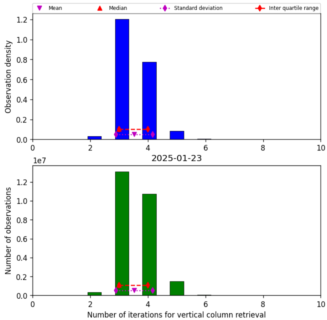
Figure 26: Histogram of “Number of iterations for vertical column retrieval” for 2025-01-23 to 2025-01-24
