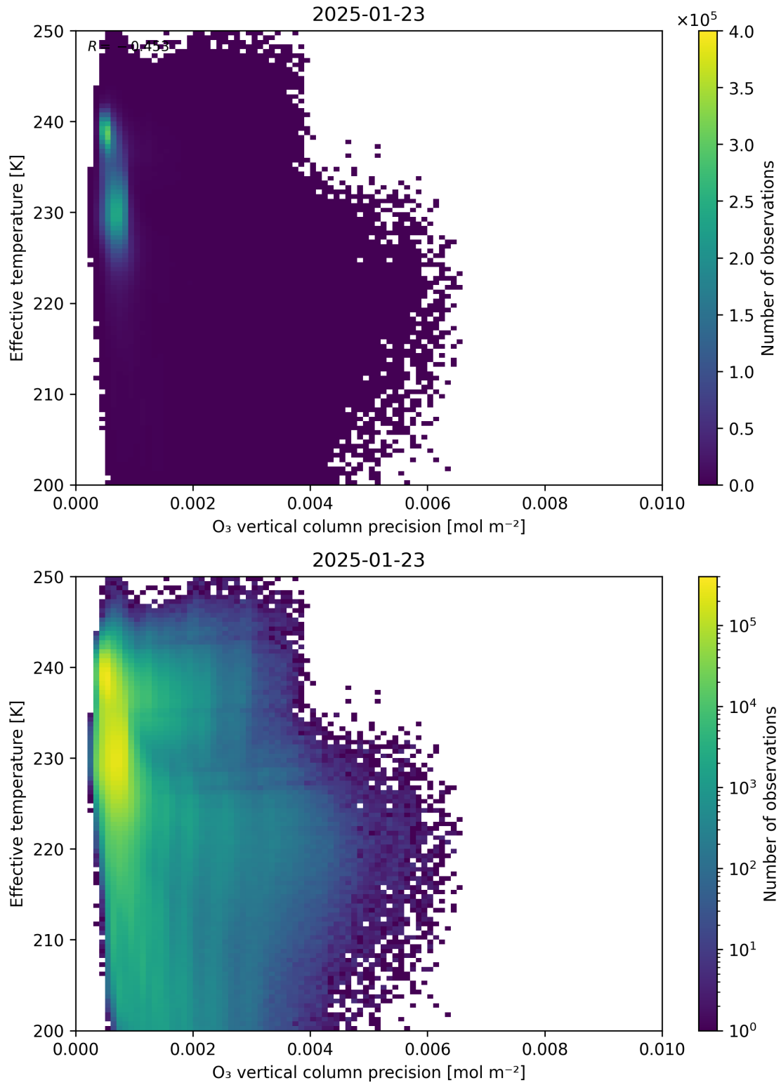
Figure 42: Scatter density plot of “O 3 vertical column precision” against “Effective temperature” for 2025-01-23 to 2025-01-24.
