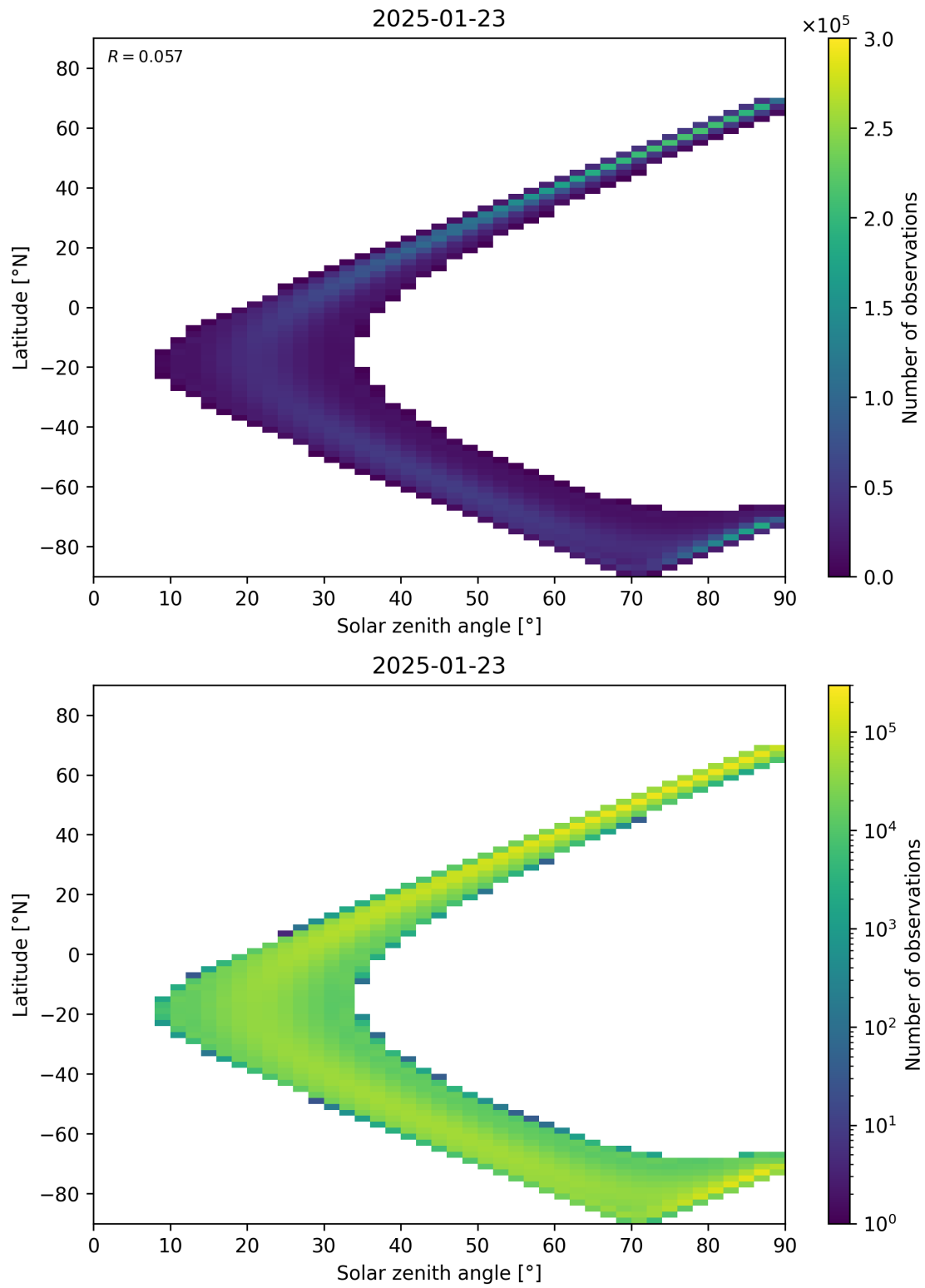
Figure 44: Scatter density plot of “Solar zenith angle” against “Latitude” for 2025-01-23 to 2025-01-24.
