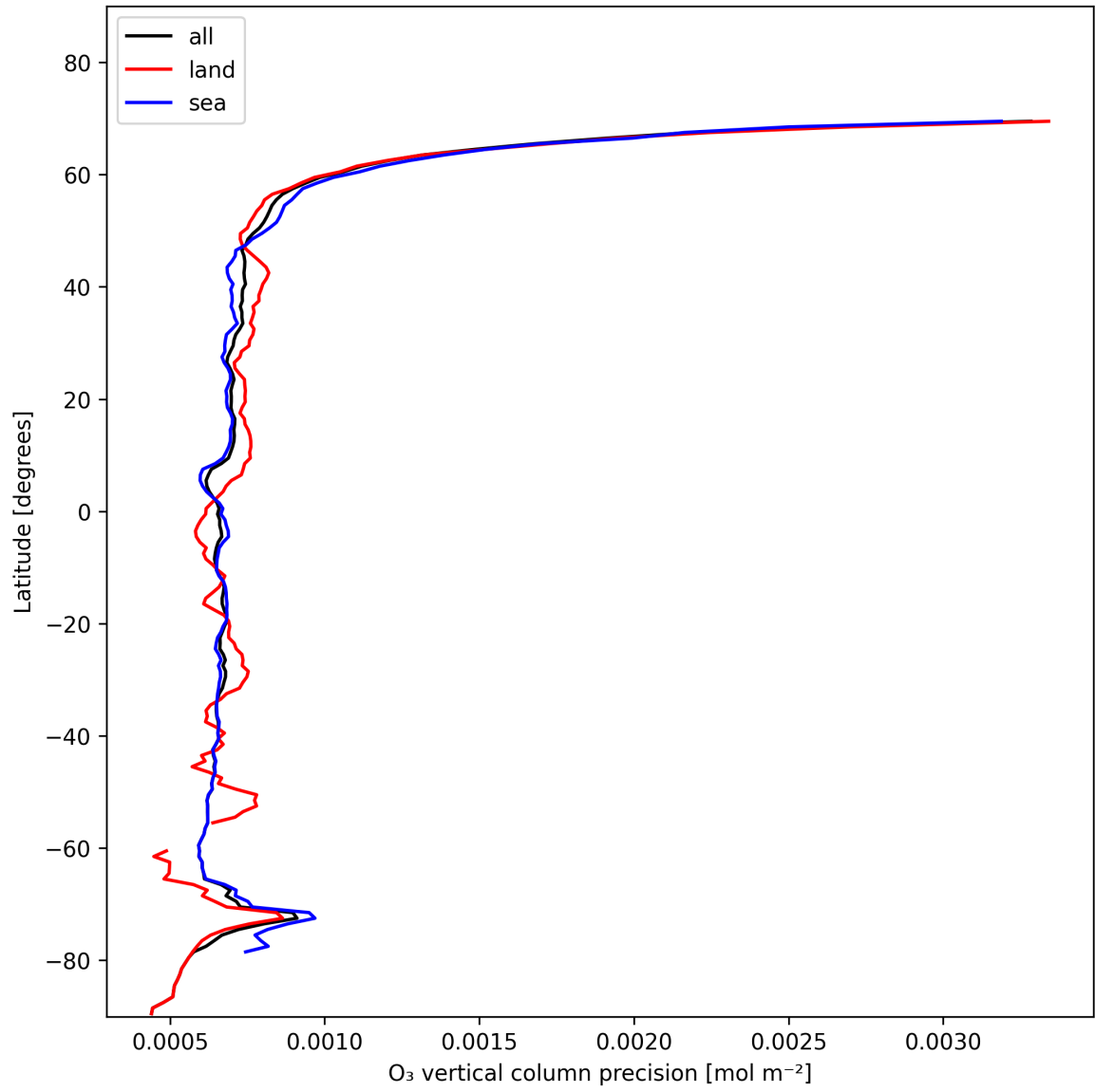
Figure 15: Zonal average of “O 3 vertical column precision” for 2025-01-23 to 2025-01-24.
