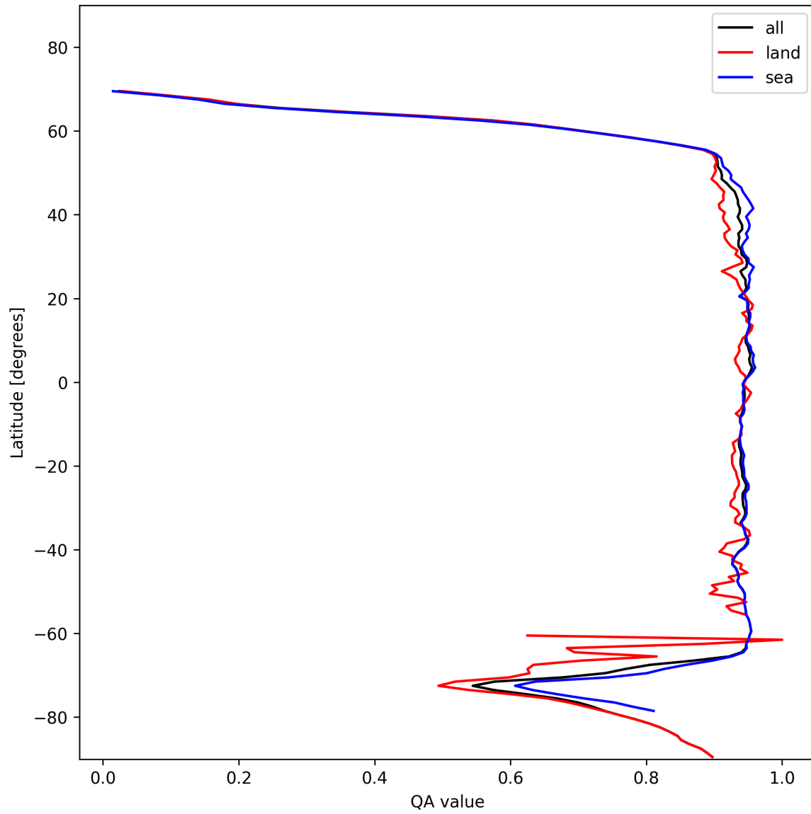
Figure 13: Zonal average of “QA value” for 2025-01-23 to 2025-01-24.
