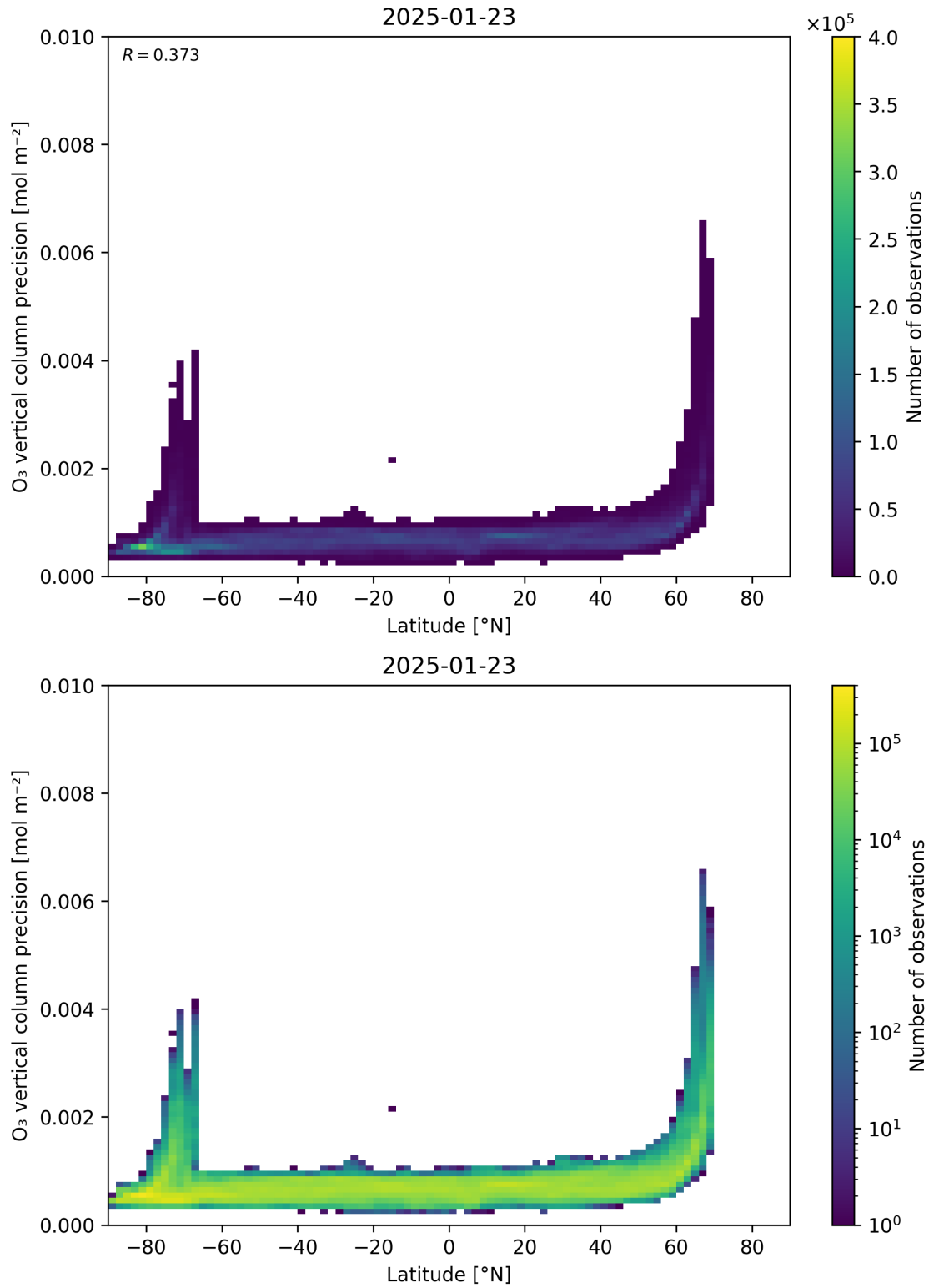
Figure 37: Scatter density plot of “Latitude” against “O 3 vertical column precision” for 2025-01-23 to 2025-01-24.
