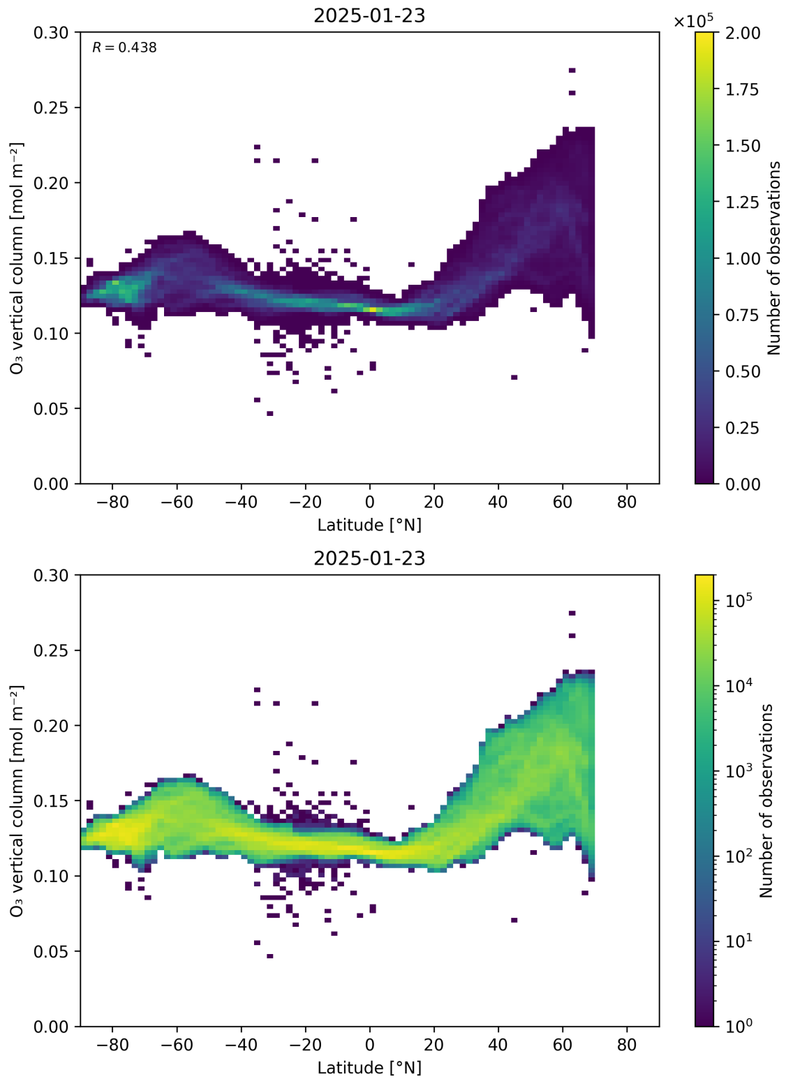
Figure 36: Scatter density plot of “Latitude” against “O 3 vertical column” for 2025-01-23 to 2025-01-24.
