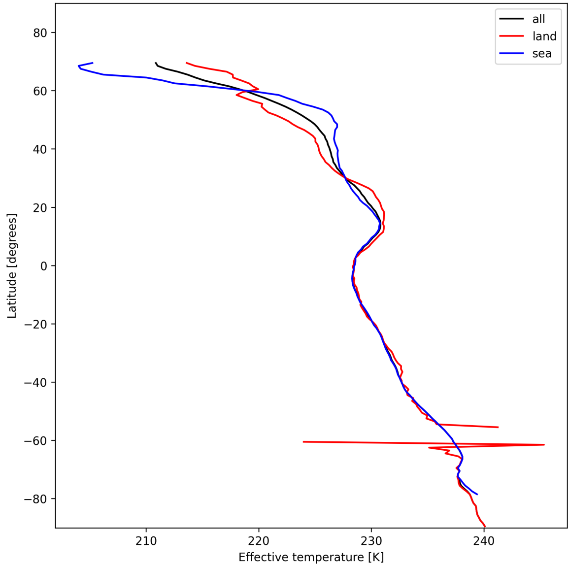
Figure 17: Zonal average of “Effective temperature” for 2025-01-23 to 2025-01-24.
