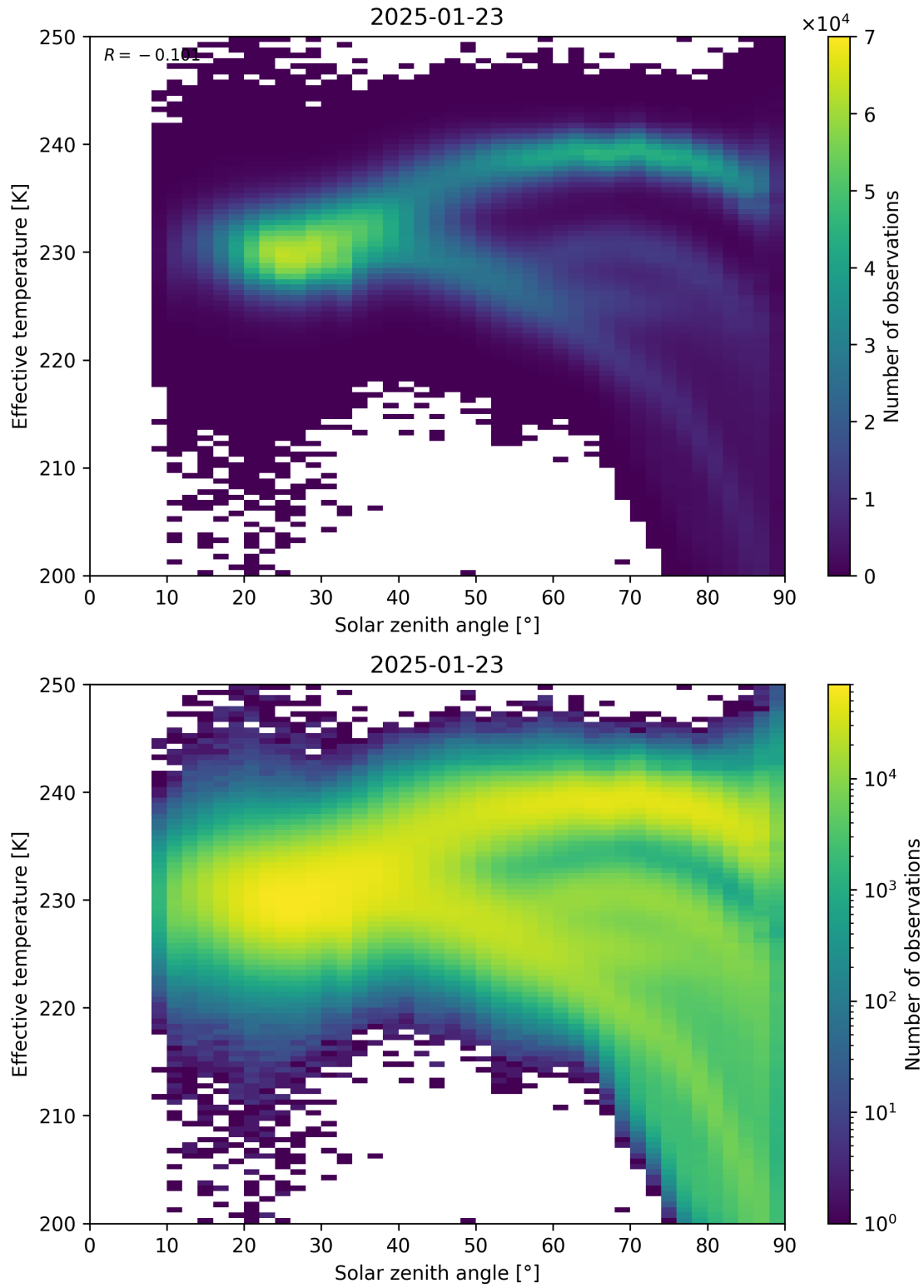
Figure 45: Scatter density plot of “Solar zenith angle” against “Effective temperature” for 2025-01-23 to 2025-01-24.
