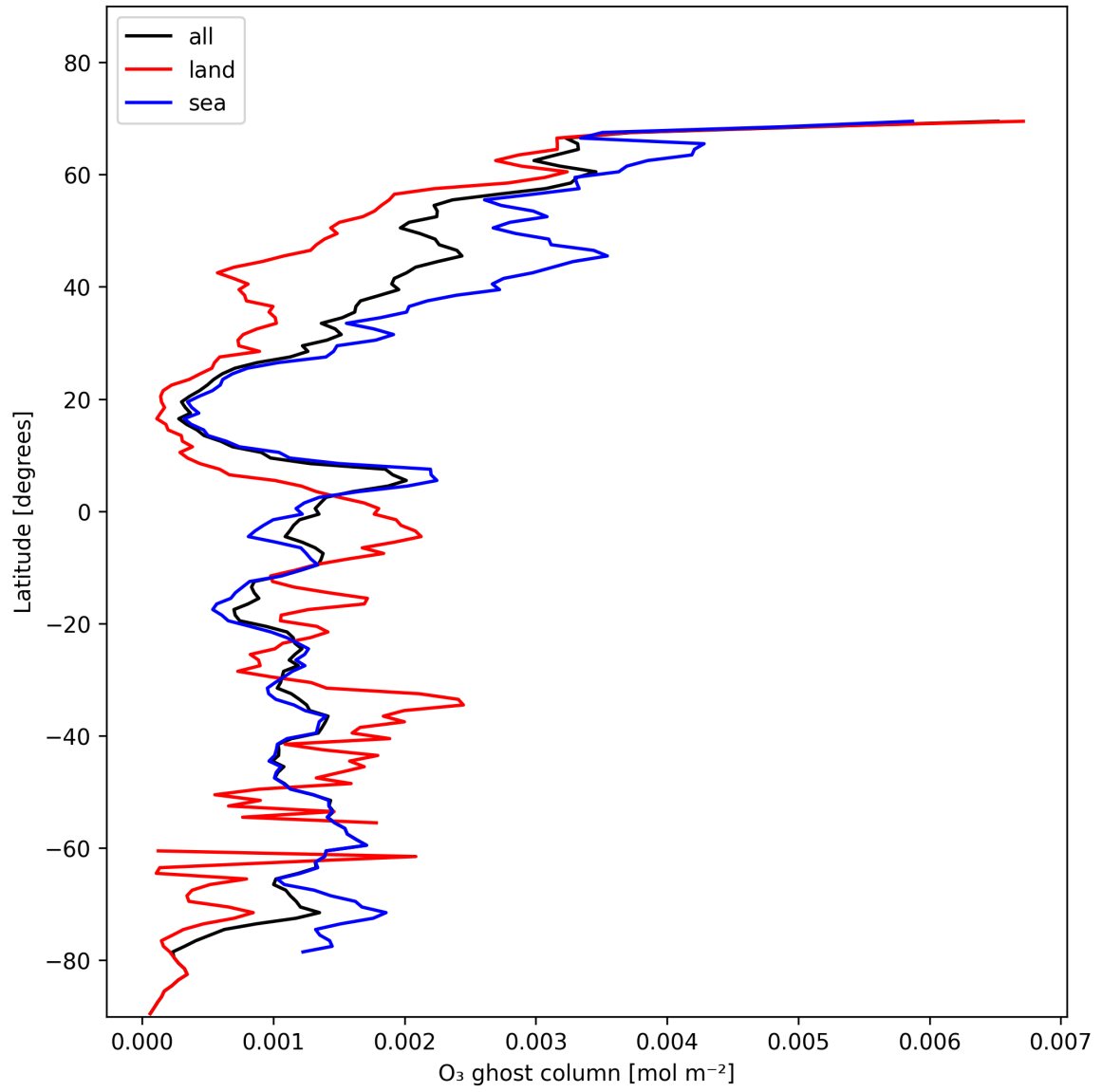
Figure 18: Zonal average of "O 3 ghost column" for 2025-01-23 to 2025-01-24.
