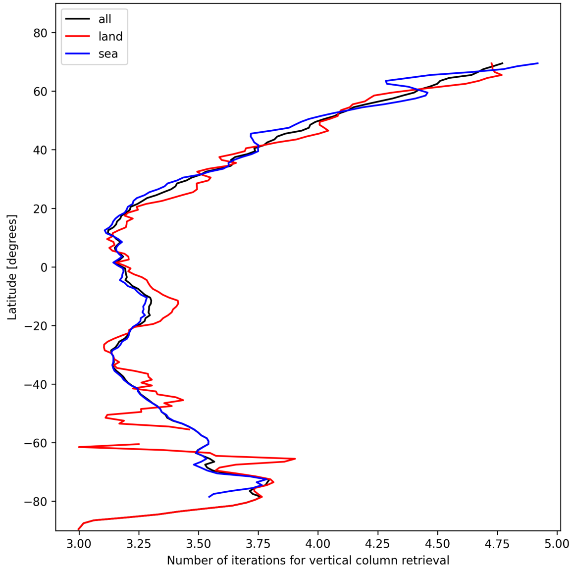
Figure 19: Zonal average of “Number of iterations for vertical column retrieval” for 2025-01-23 to 2025-01-24.
