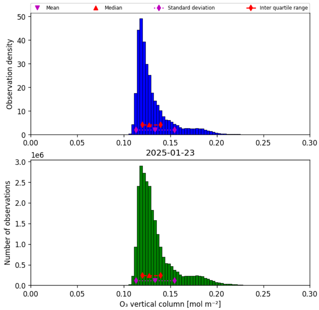
Figure 21: Histogram of “O 3 vertical column” for 2025-01-23 to 2025-01-24
