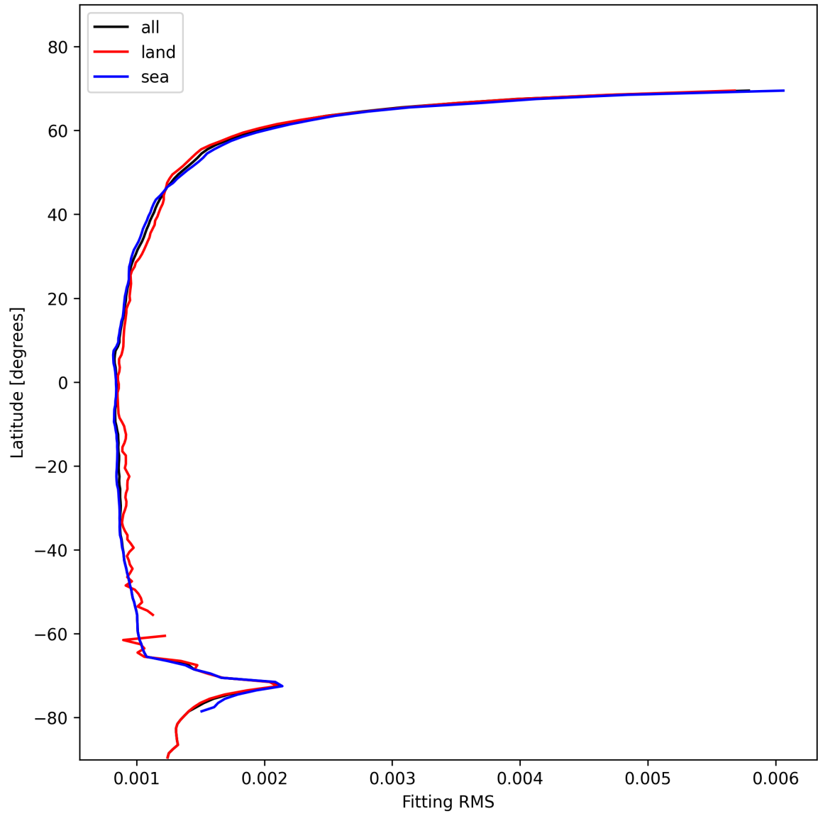
Figure 16: Zonal average of “Fitting RMS” for 2025-01-23 to 2025-01-24.
