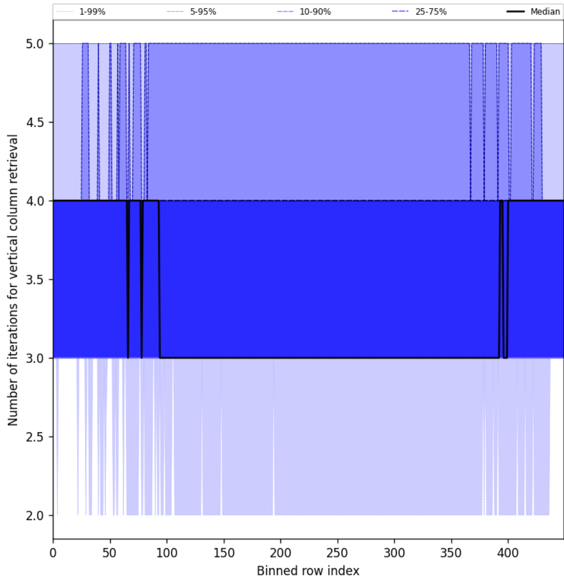
Figure 33: Along track statistics of “Number of iterations for vertical column retrieval” for 2025-01-23 to 2025-01-24
