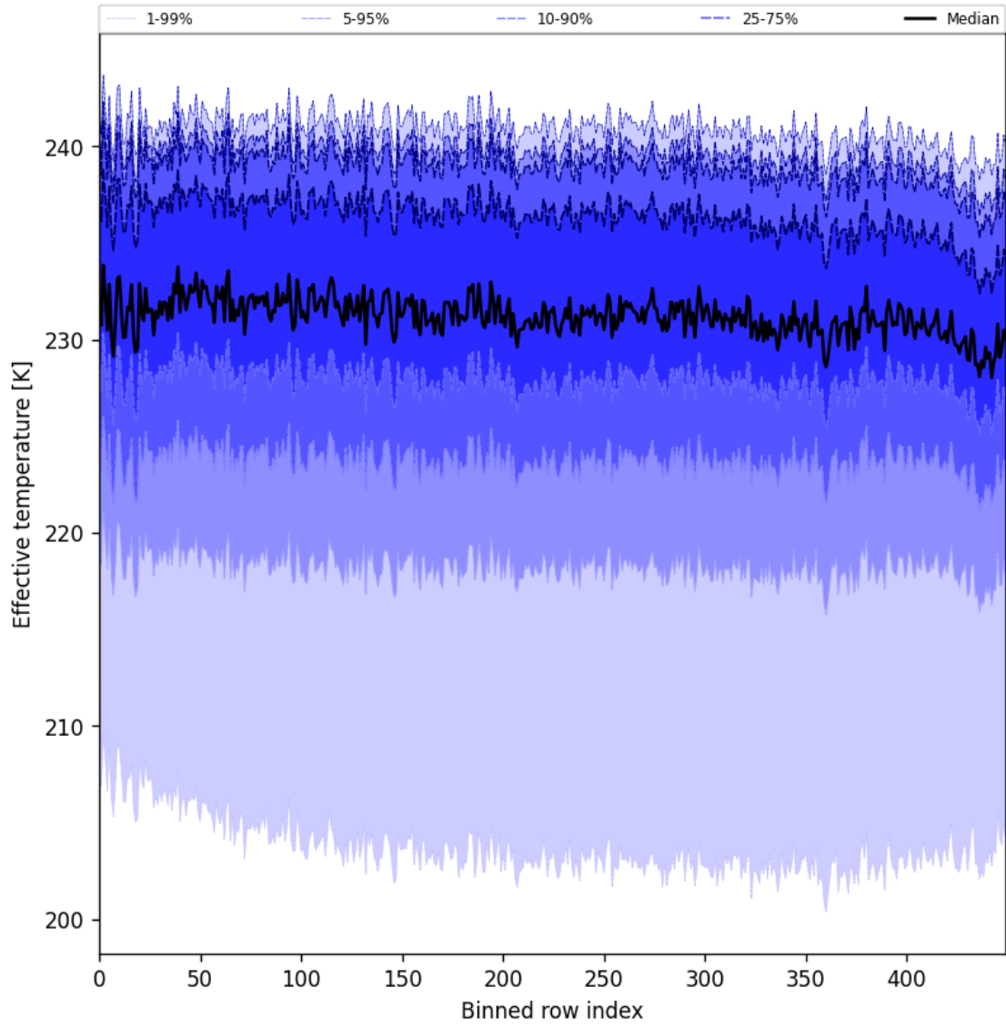
Figure 31: Along track statistics of “Effective temperature” for 2025-01-23 to 2025-01-24
