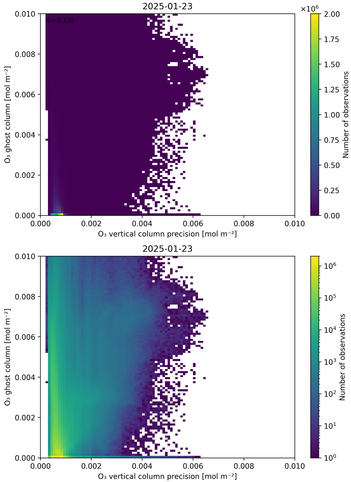
Figure 43: Scatter density plot of “O 3 vertical column precision” against “O 3 ghost column” for 2025-01-23 to 2025-01-24.
