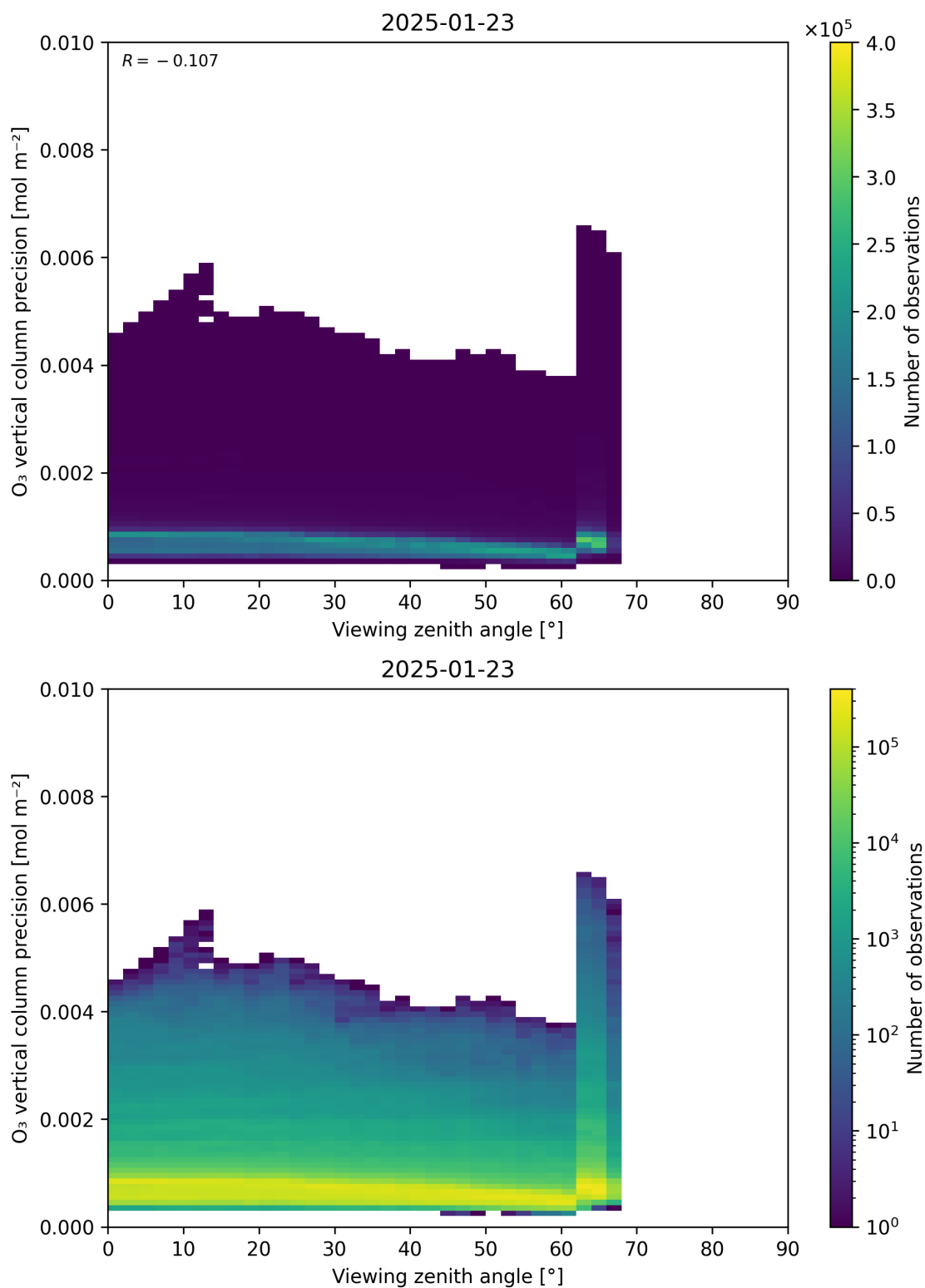
Figure 53: Scatter density plot of “Viewing zenith angle” against “O 3 vertical column precision” for 2025-01-23 to 2025-01-24.
