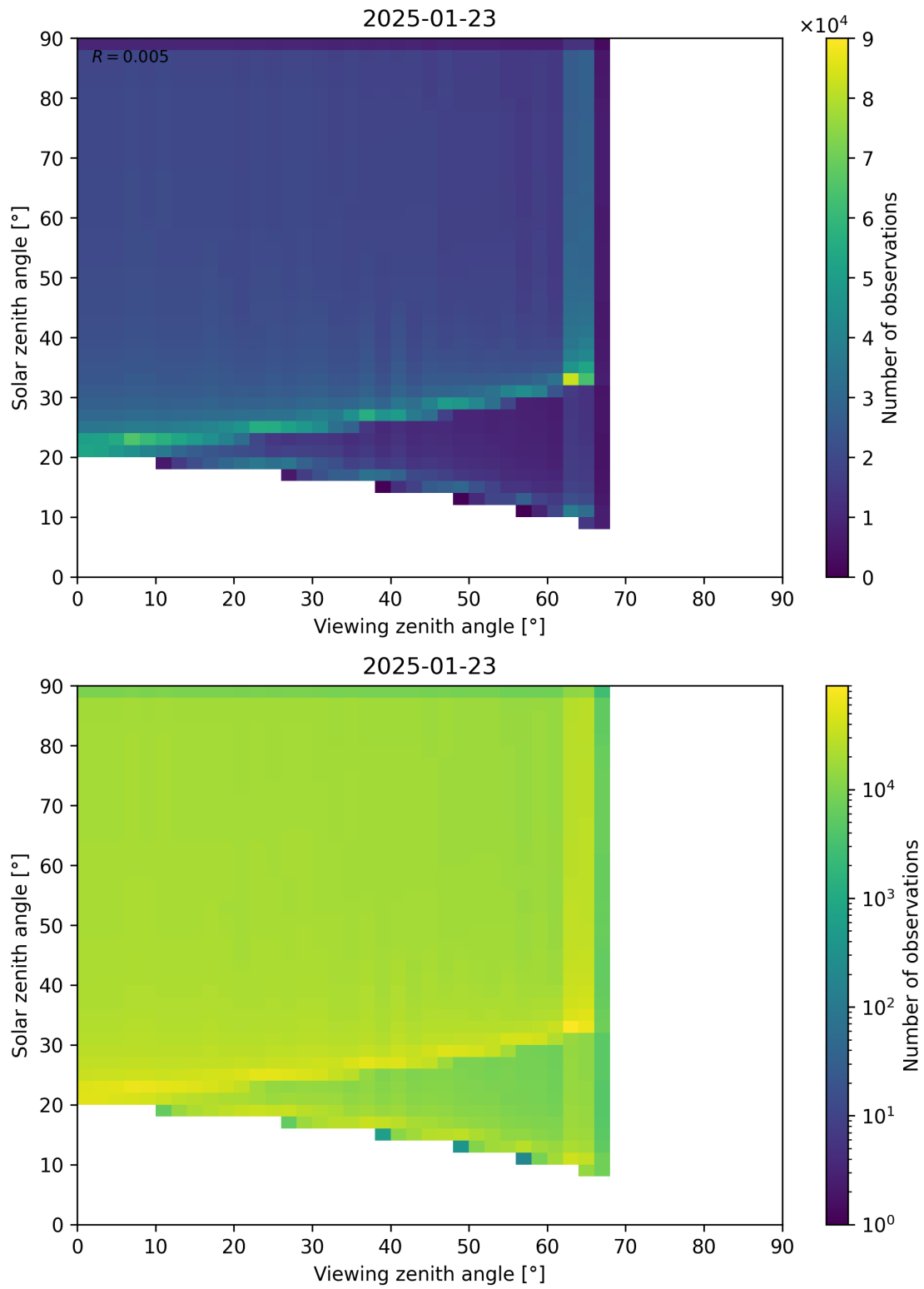
Figure 54: Scatter density plot of “Viewing zenith angle” against “Solar zenith angle” for 2025-01-23 to 2025-01-24.
