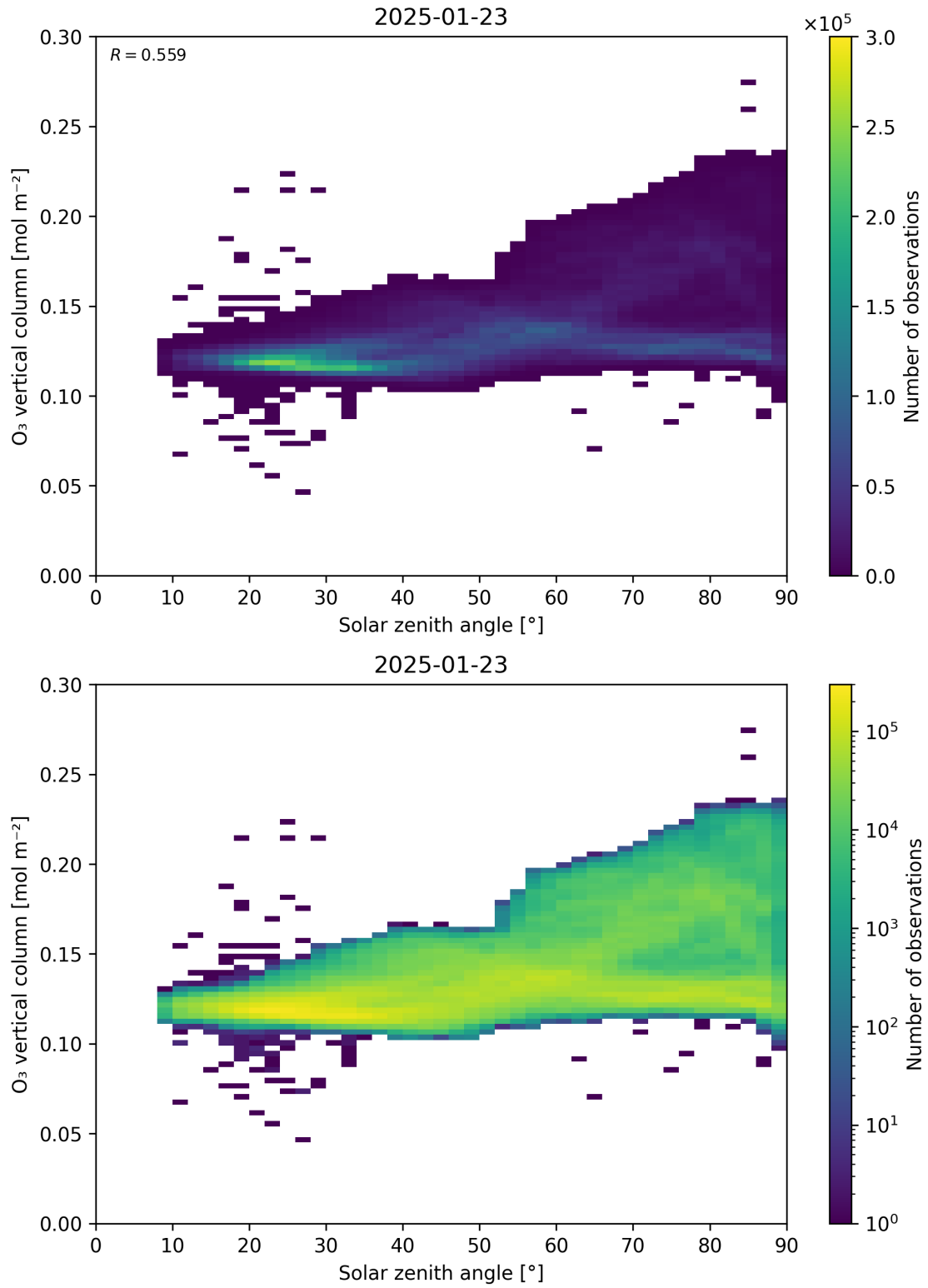
Figure 47: Scatter density plot of “Solar zenith angle” against “O 3 vertical column” for 2025-01-23 to 2025-01-24.
