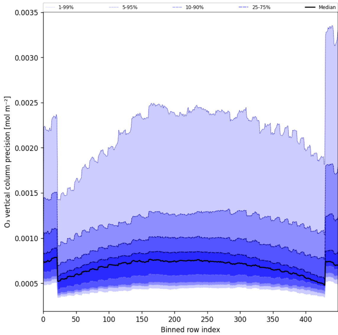
Figure 29: Along track statistics of “O 3 vertical column precision” for 2025-01-23 to 2025-01-24
