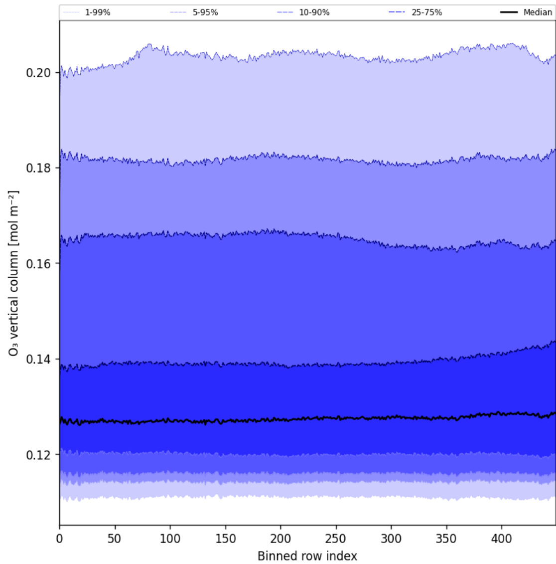
Figure 28: Along track statistics of “O 3 vertical column” for 2025-01-23 to 2025-01-24
