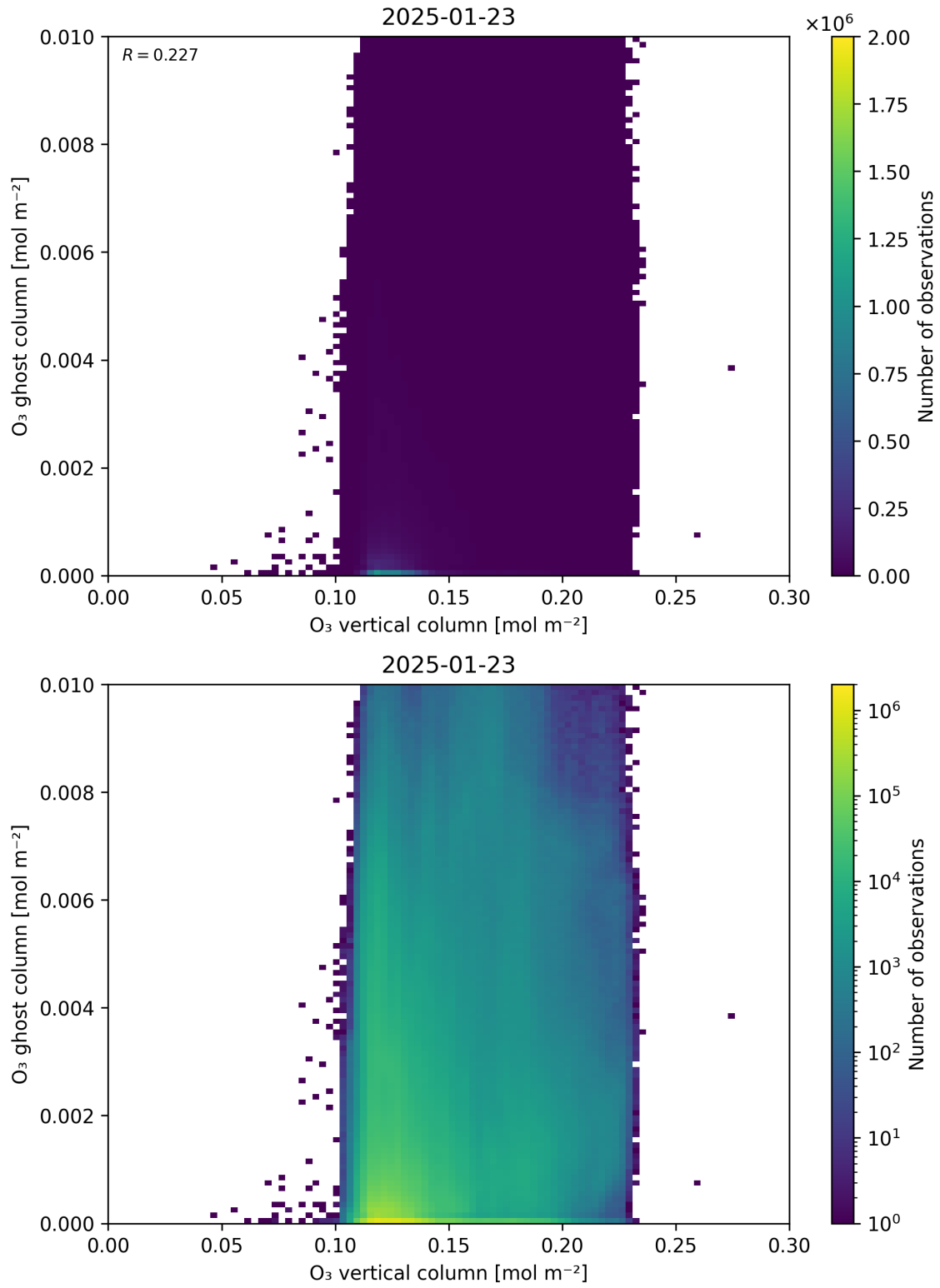
Figure 40: Scatter density plot of “O 3 vertical column” against “O 3 ghost column” for 2025-01-23 to 2025-01-24.
