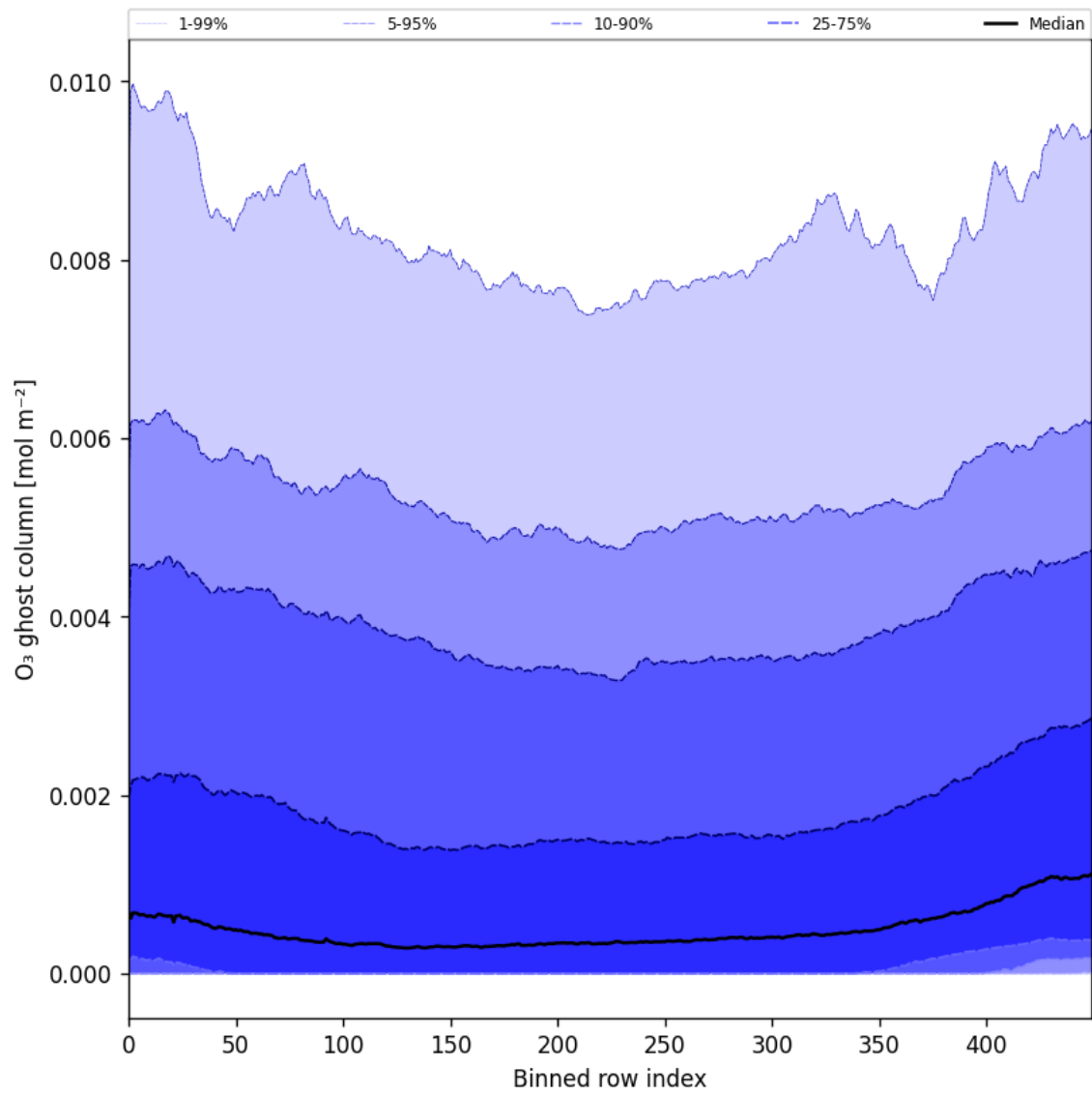
Figure 32: Along track statistics of “O 3 ghost column” for 2025-01-23 to 2025-01-24
