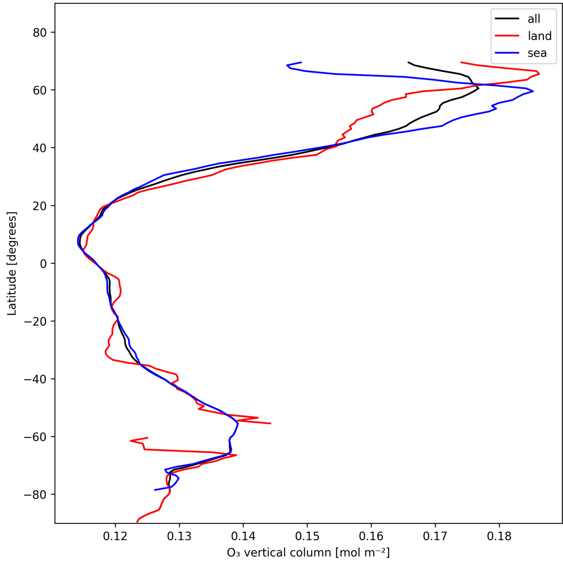
Figure 14: Zonal average of “O 3 vertical column” for 2025-01-23 to 2025-01-24.
