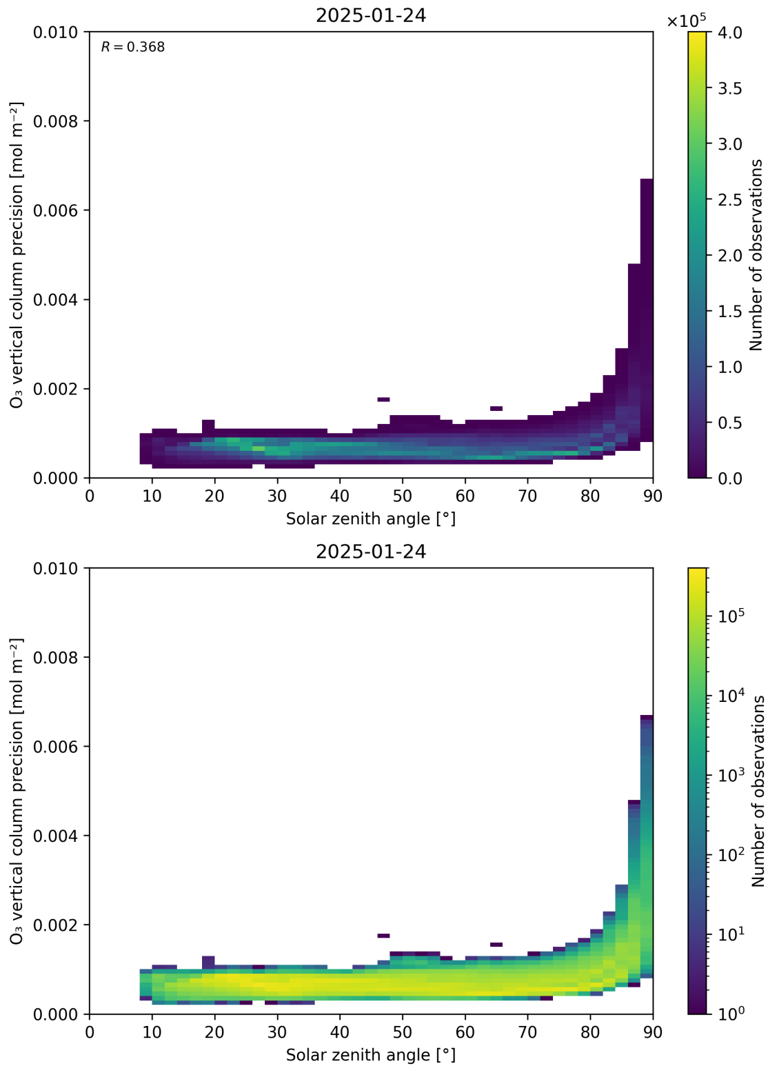
Figure 48: Scatter density plot of “Solar zenith angle” against “O 3 vertical column precision” for 2025-01-23 to 2025-01-25.
