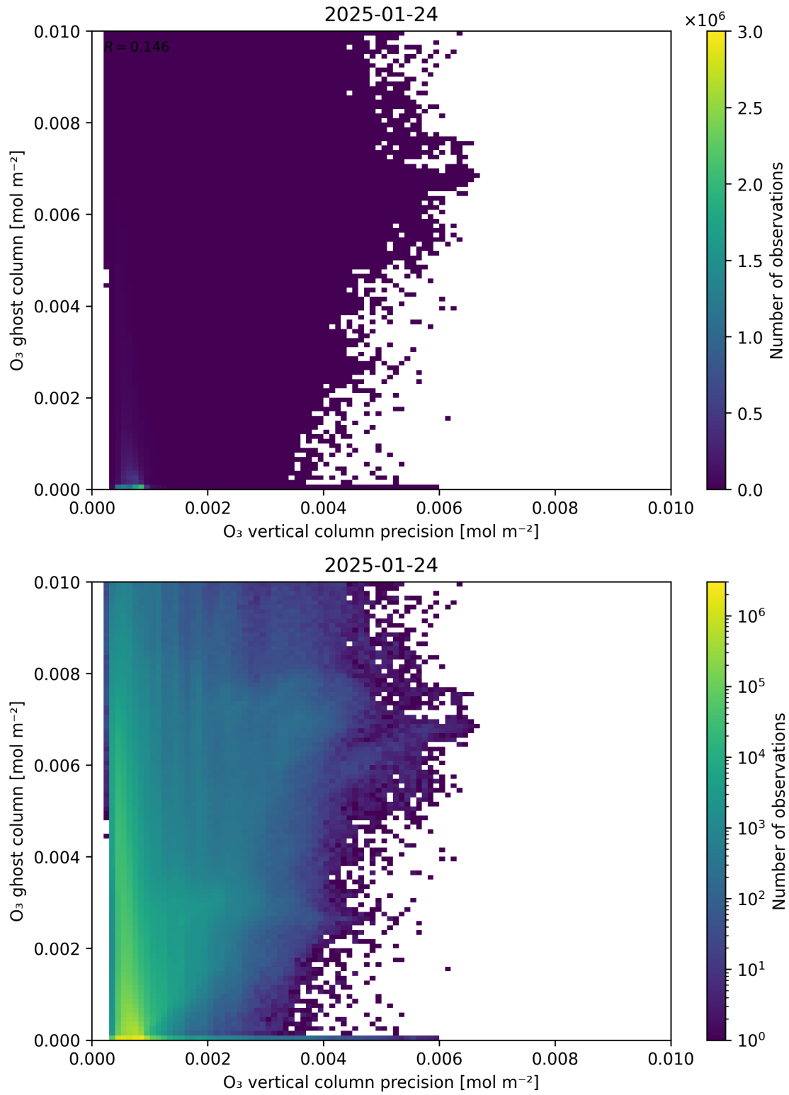
Figure 43: Scatter density plot of “O 3 vertical column precision” against “O 3 ghost column” for 2025-01-23 to 2025-01-25.
