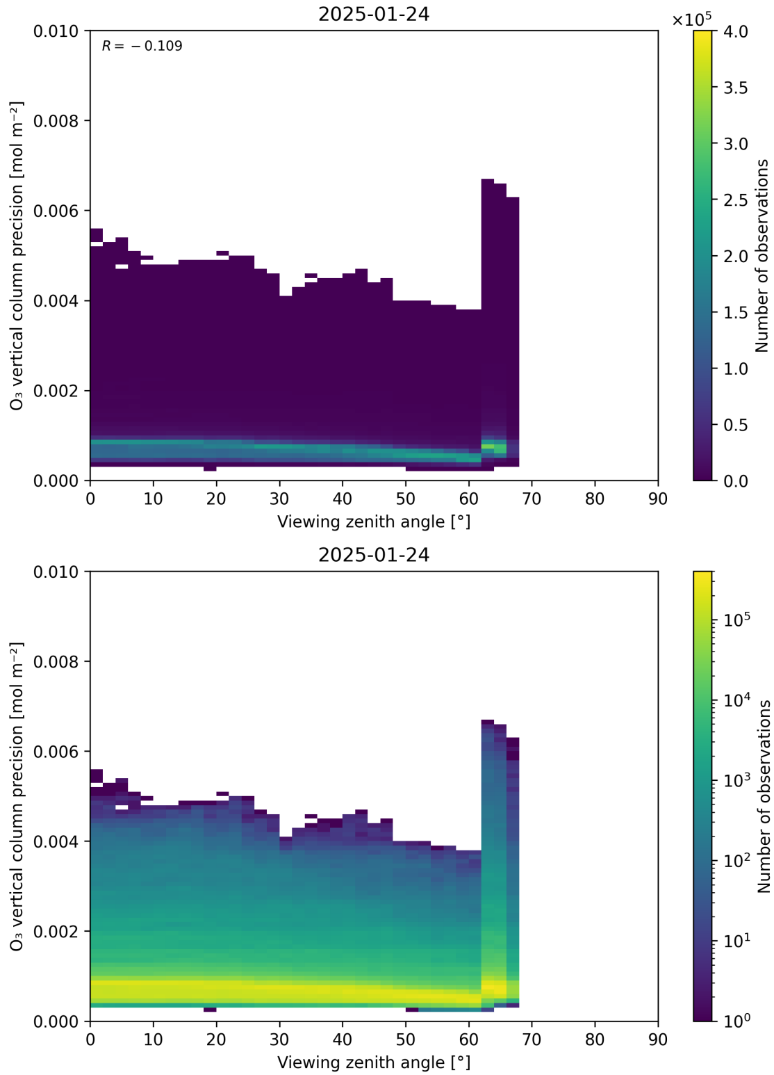
Figure 53: Scatter density plot of “Viewing zenith angle” against “O 3 vertical column precision” for 2025-01-23 to 2025-01-25.
