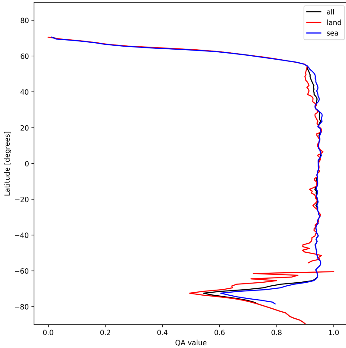
Figure 13: Zonal average of “QA value” for 2025-01-23 to 2025-01-25.
