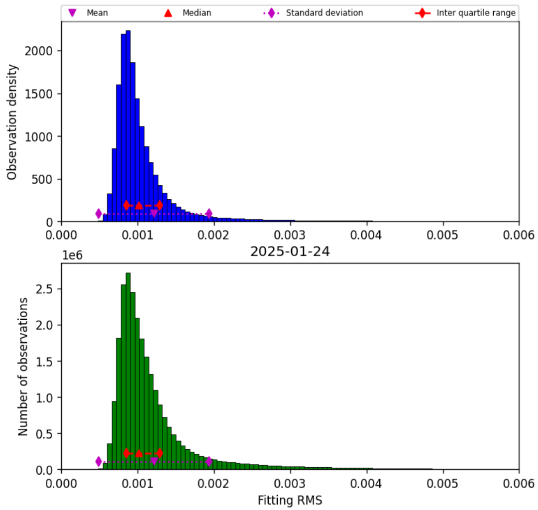
Figure 23: Histogram of “Fitting RMS” for 2025-01-23 to 2025-01-25
