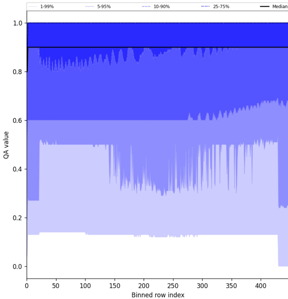
Figure 27: Along track statistics of “QA value” for 2025-01-23 to 2025-01-25
