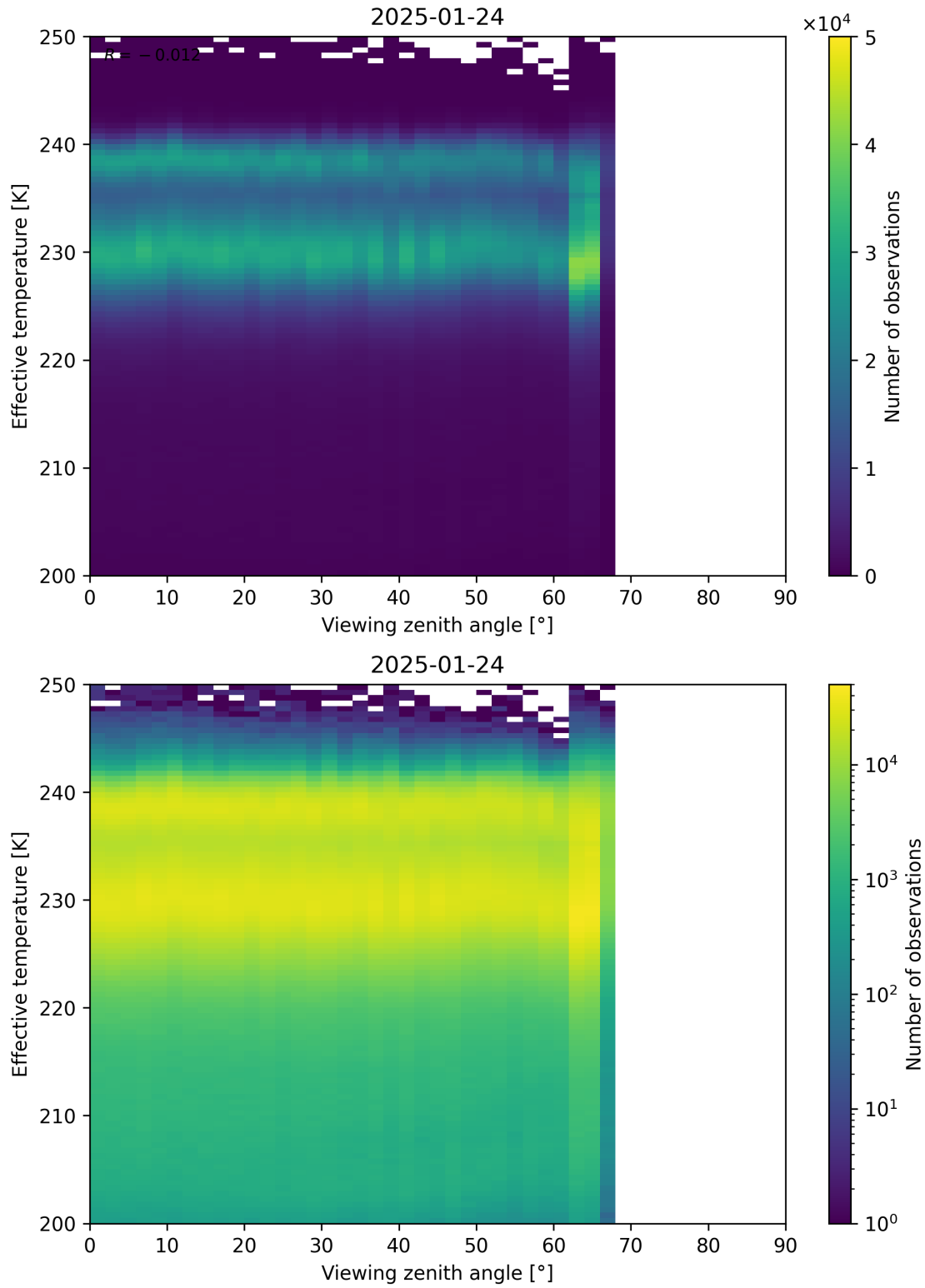
Figure 50: Scatter density plot of “Viewing zenith angle” against “Effective temperature” for 2025-01-23 to 2025-01-25.
