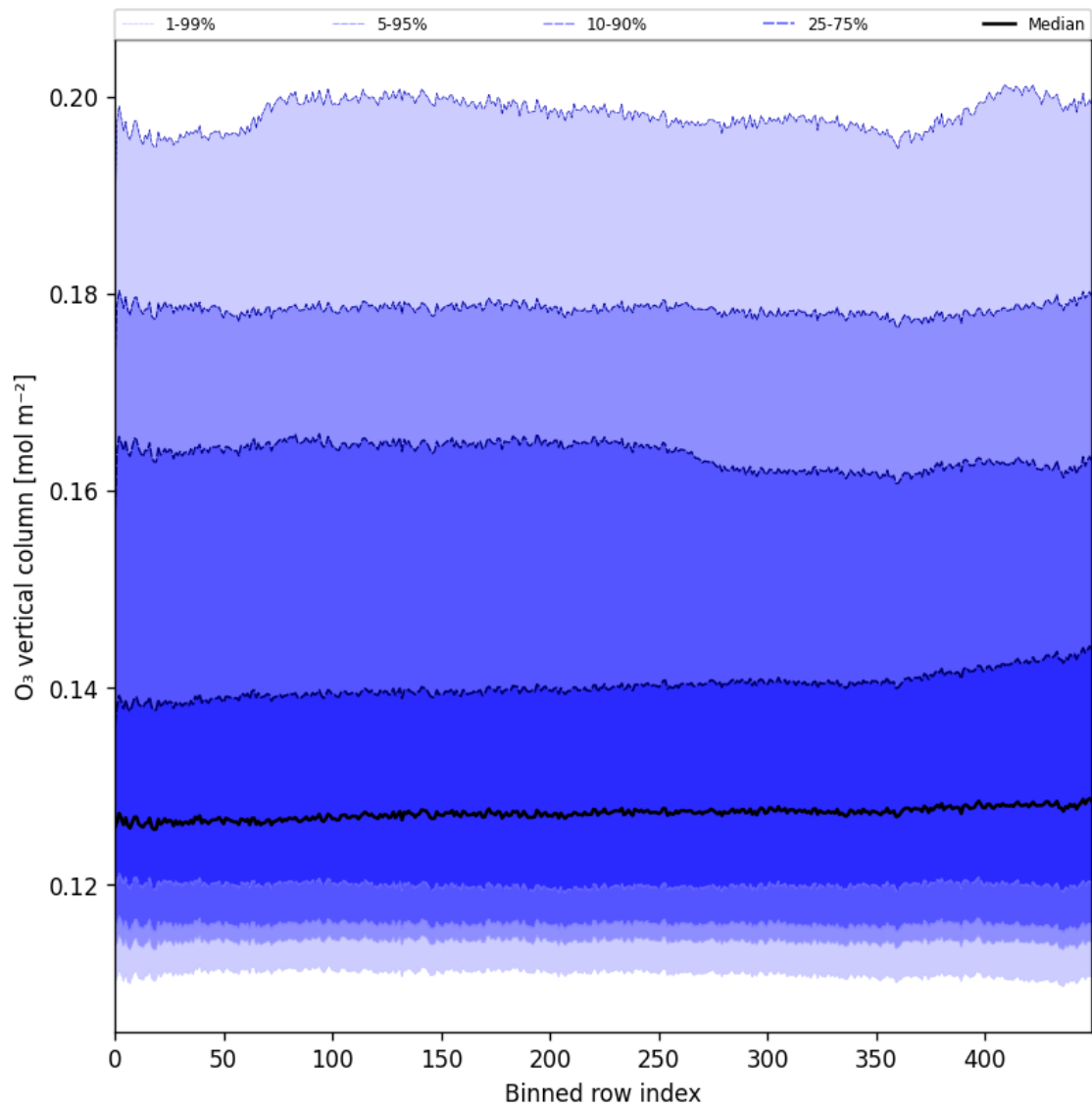
Figure 28: Along track statistics of “ O_3 vertical column” for 2025-01-23 to 2025-01-25
