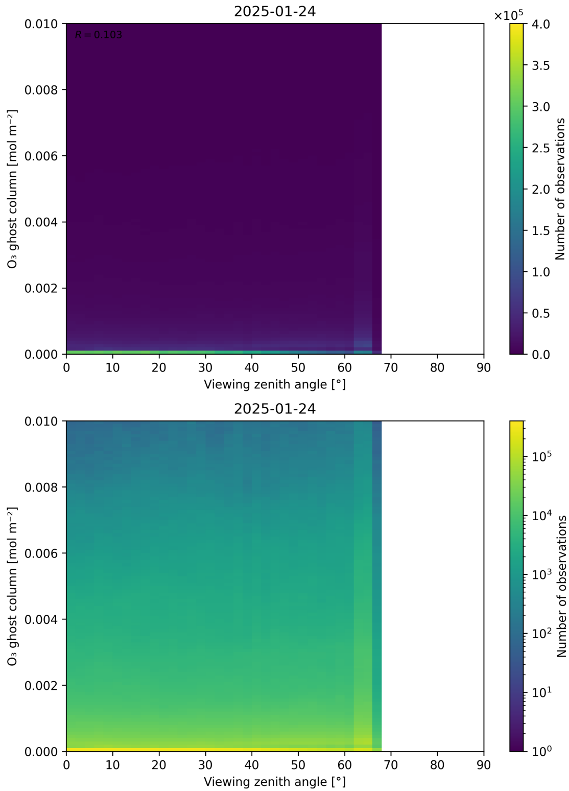
Figure 51: Scatter density plot of “Viewing zenith angle” against “O 3 ghost column” for 2025-01-23 to 2025-01-25.
