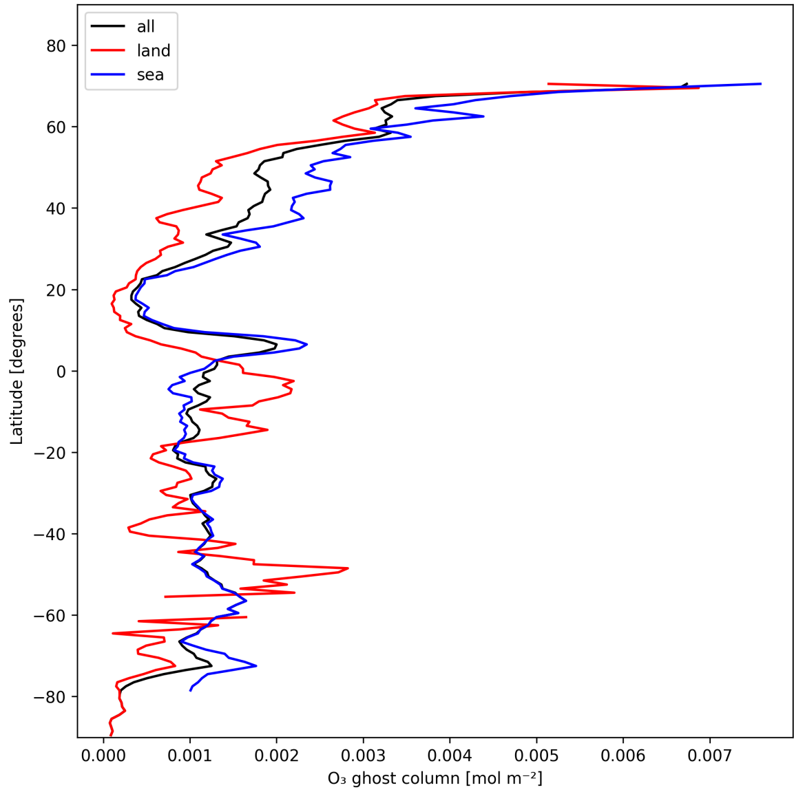
Figure 18: Zonal average of "O 3 ghost column" for 2025-01-23 to 2025-01-25.
