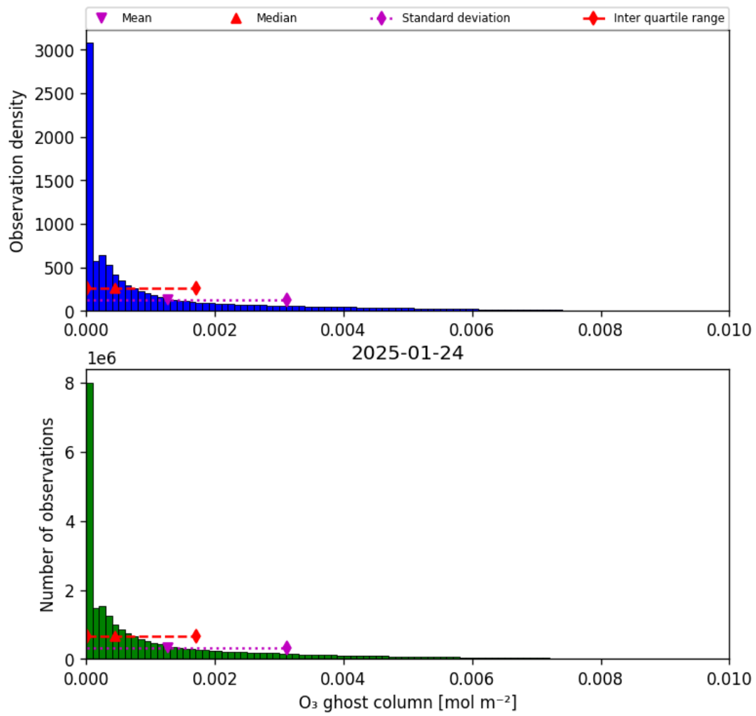
Figure 25: Histogram of “O 3 ghost column” for 2025-01-23 to 2025-01-25
