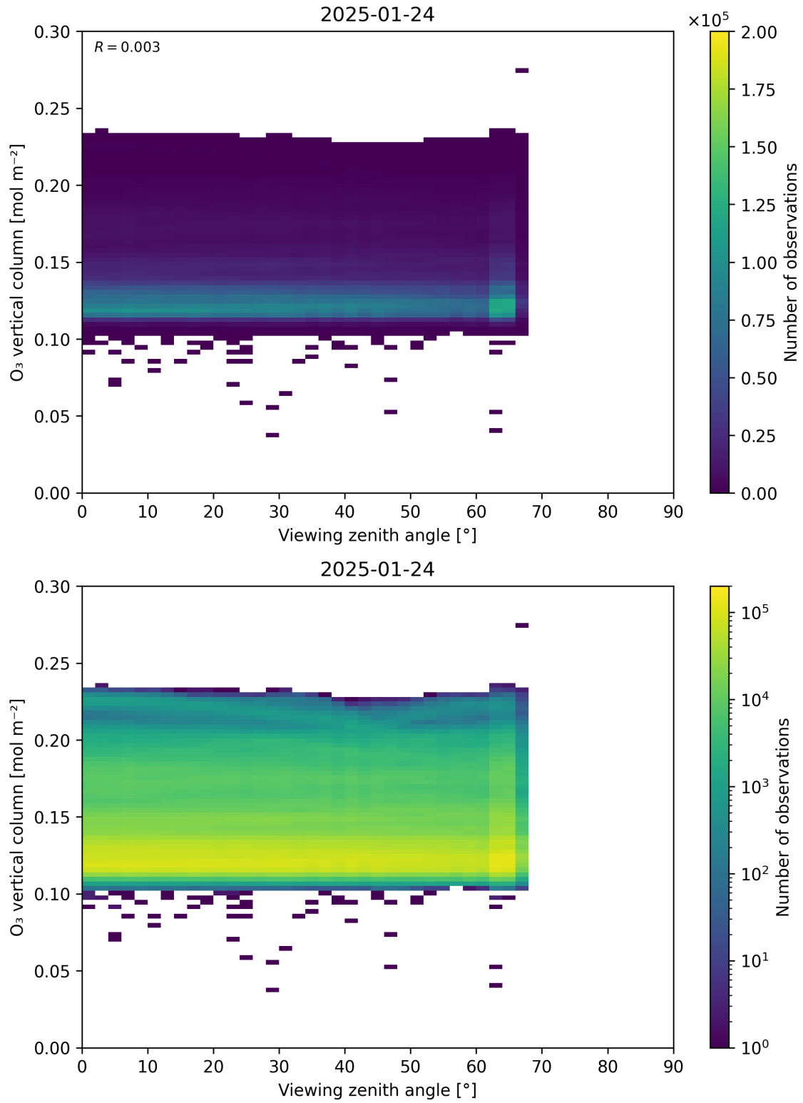
Figure 52: Scatter density plot of “Viewing zenith angle” against “O 3 vertical column” for 2025-01-23 to 2025-01-25.
