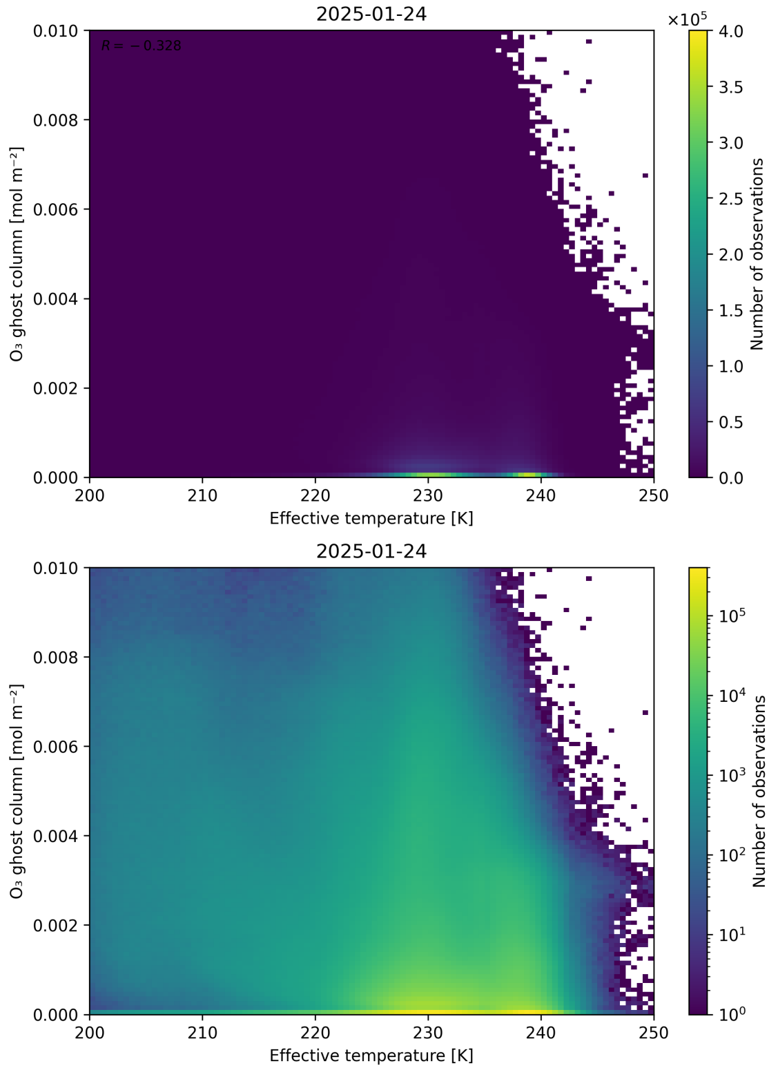
Figure 38: Scatter density plot of “Effective temperature” against “O 3 ghost column” for 2025-01-23 to 2025-01-25.
