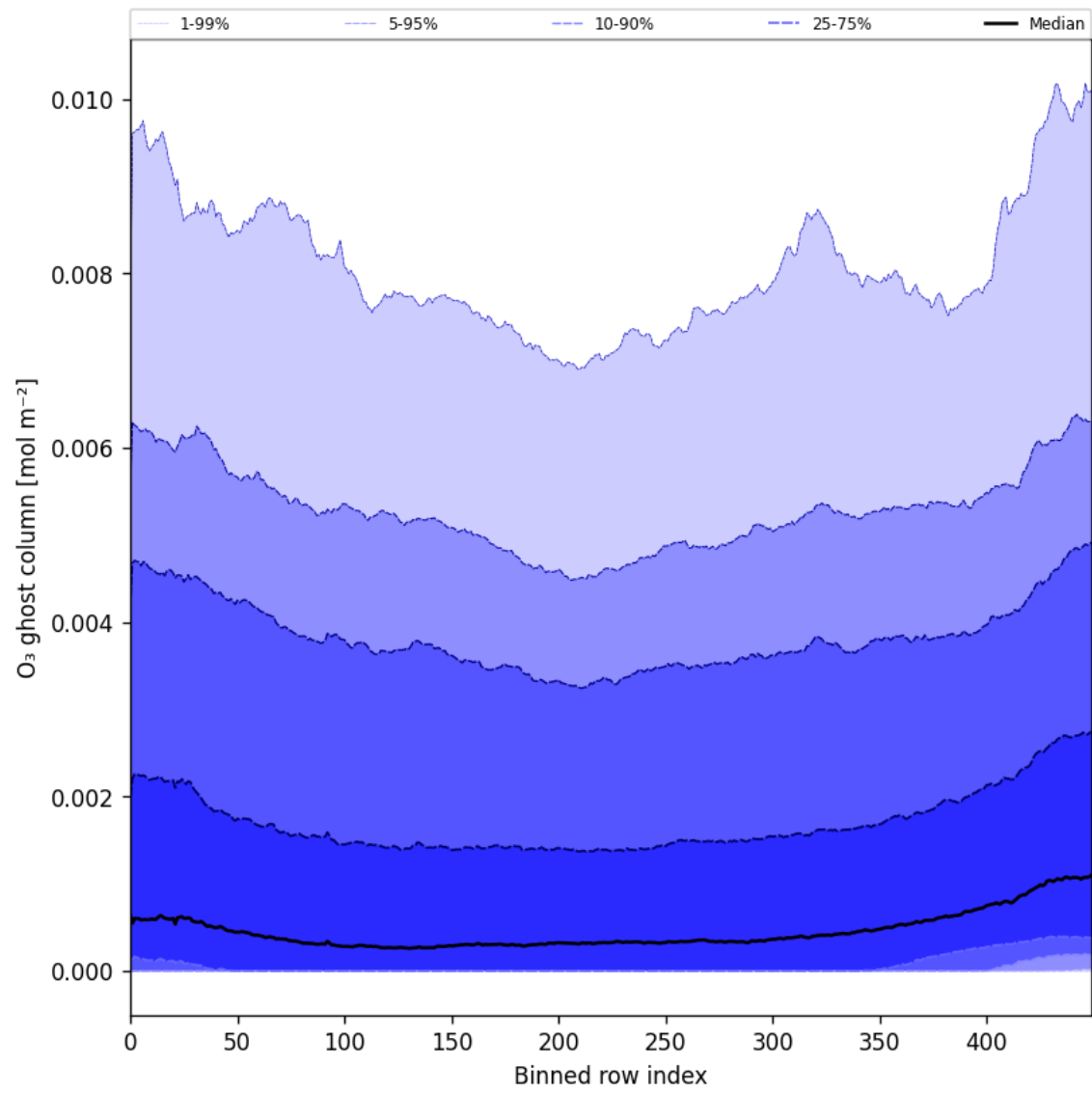
Figure 32: Along track statistics of “O 3 ghost column” for 2025-01-23 to 2025-01-25
