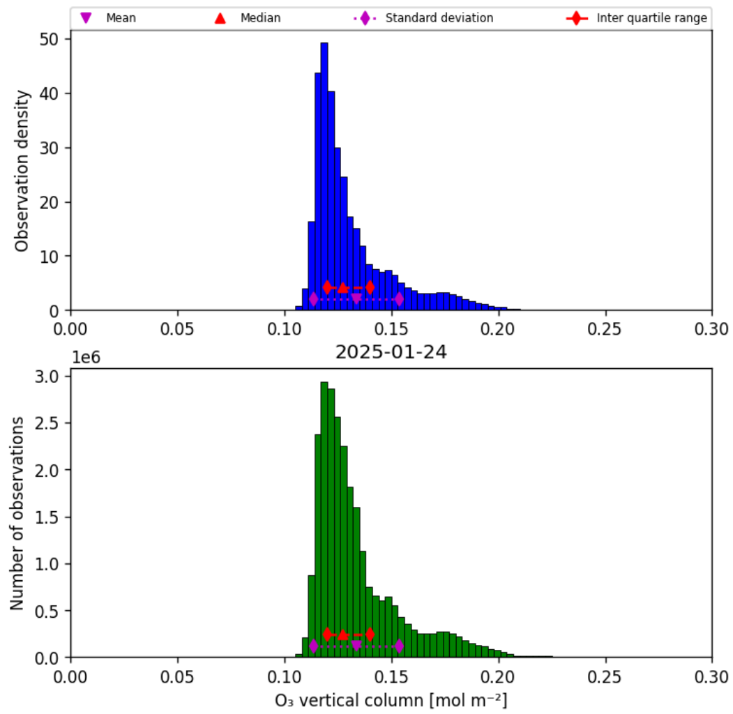
Figure 21: Histogram of “O 3 vertical column” for 2025-01-23 to 2025-01-25
