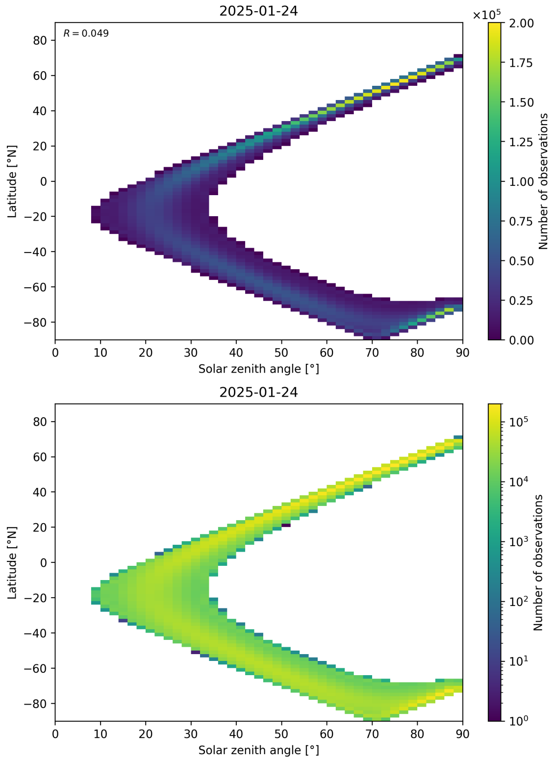
Figure 44: Scatter density plot of “Solar zenith angle” against “Latitude” for 2025-01-23 to 2025-01-25.
