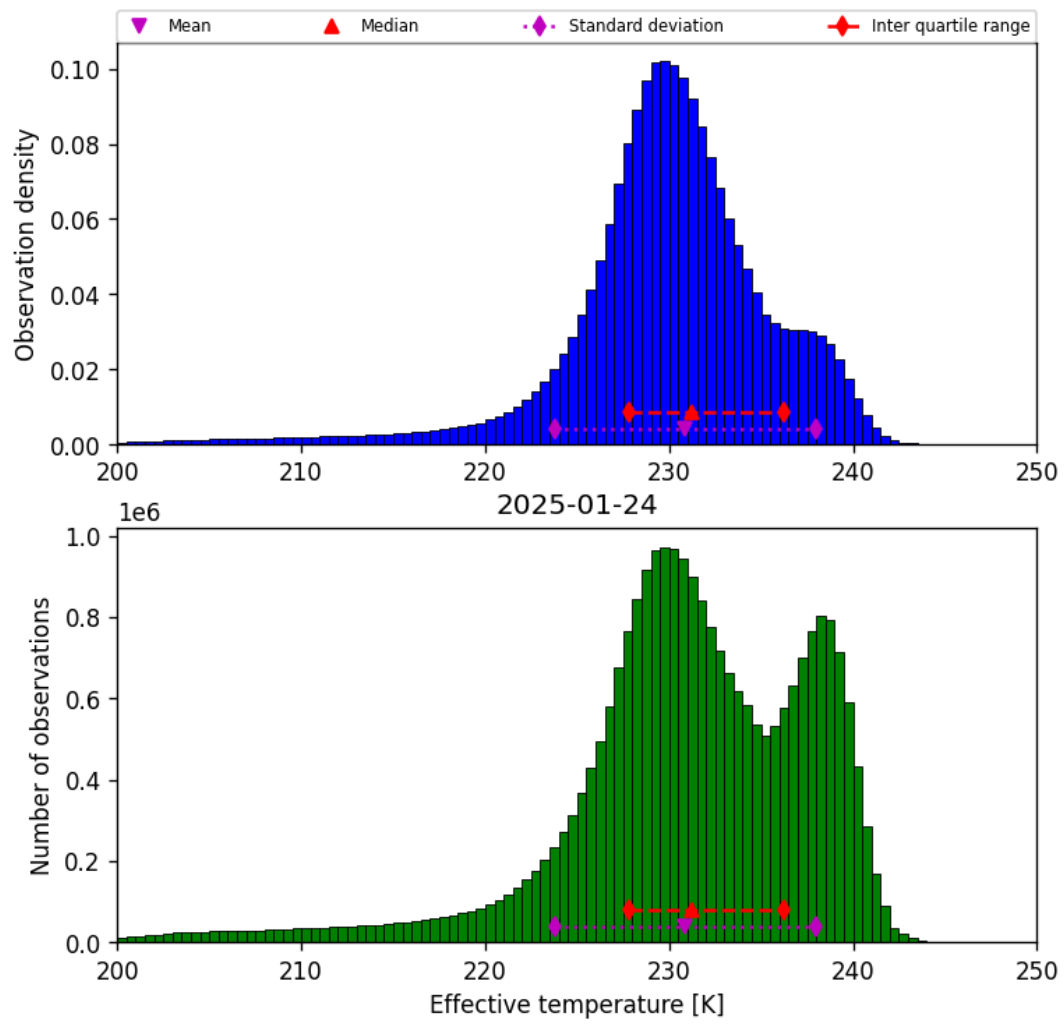
Figure 24: Histogram of “Effective temperature” for 2025-01-23 to 2025-01-25
