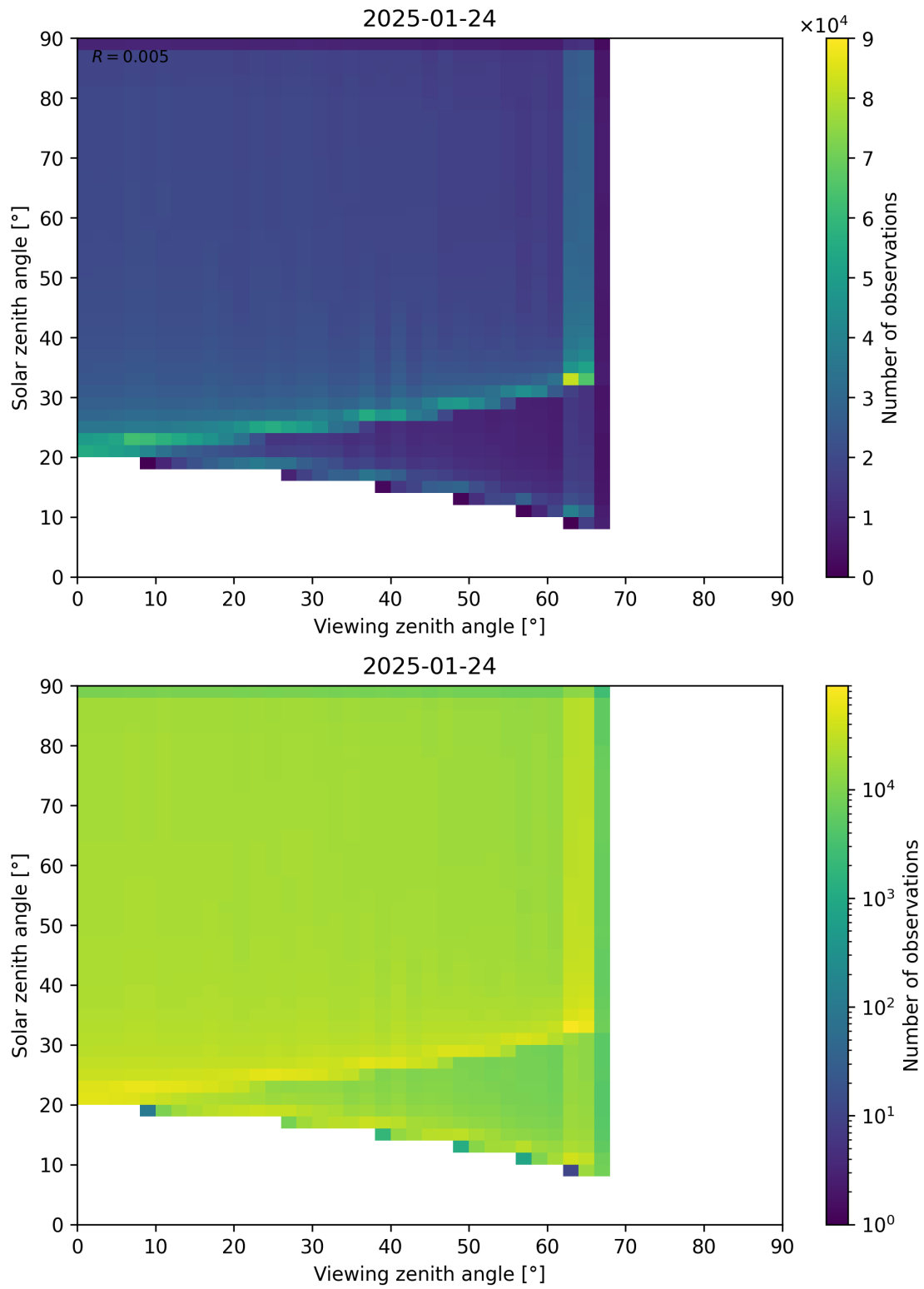
Figure 54: Scatter density plot of “Viewing zenith angle” against “Solar zenith angle” for 2025-01-23 to 2025-01-25.
