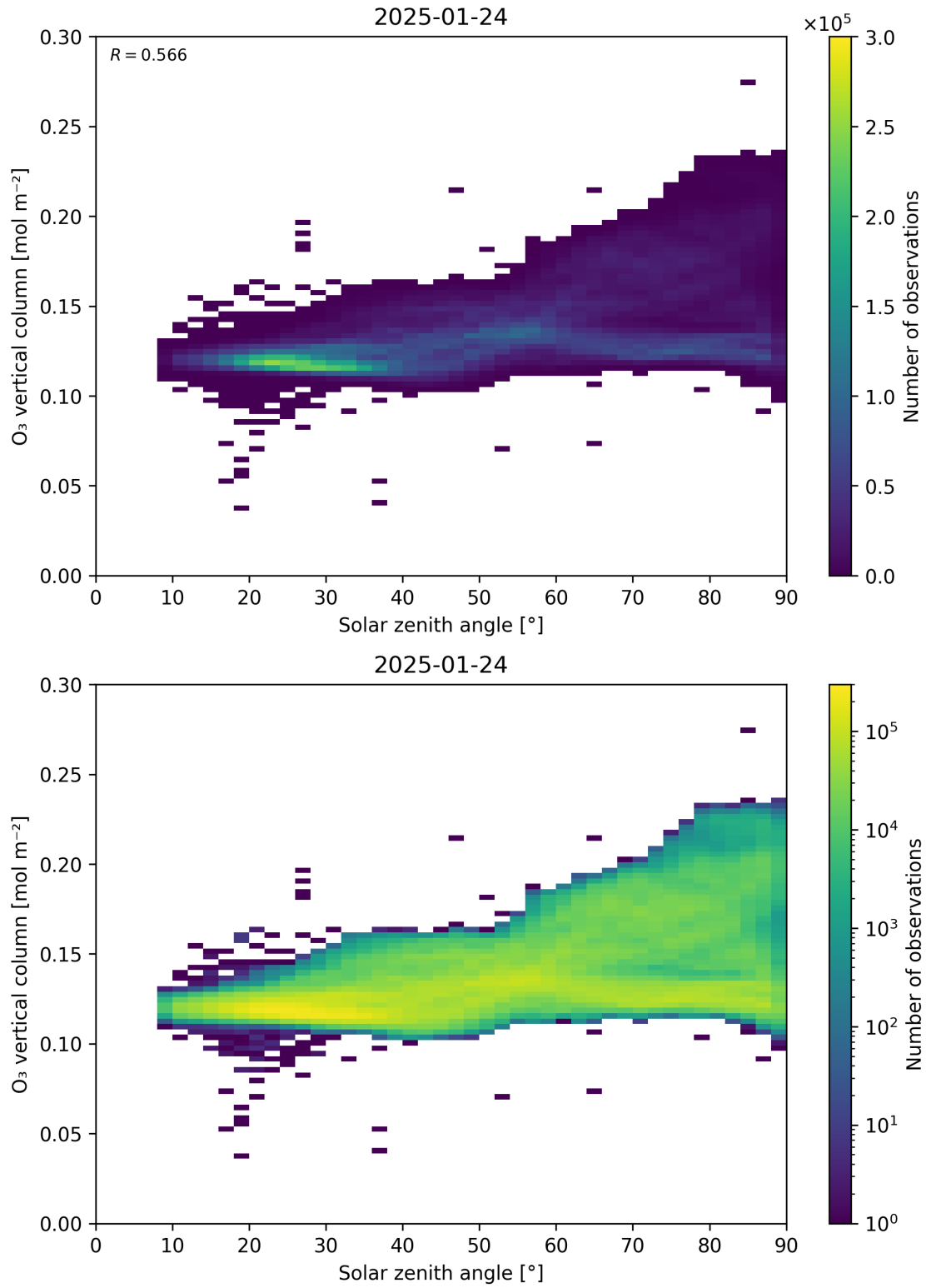
Figure 47: Scatter density plot of “Solar zenith angle” against “O 3 vertical column” for 2025-01-23 to 2025-01-25.
