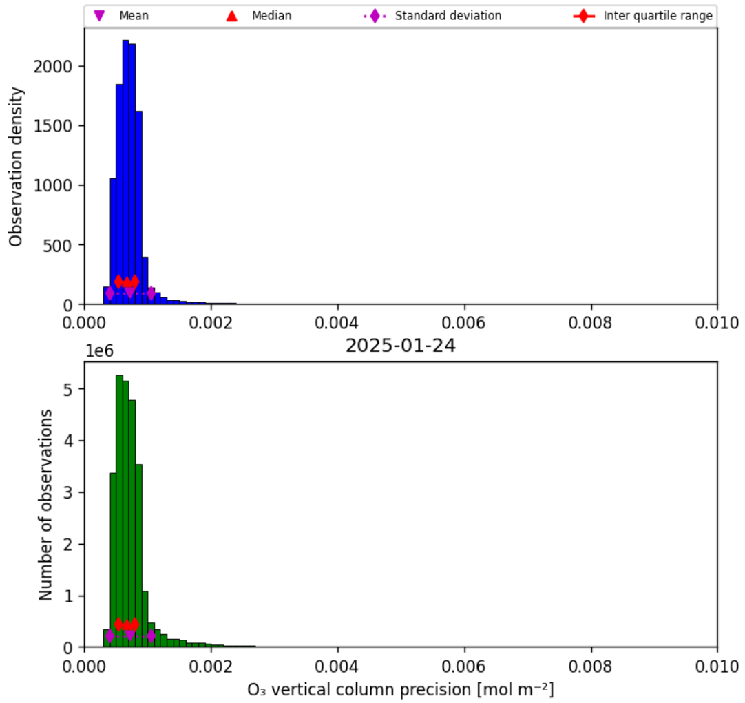
Figure 22: Histogram of “O 3 vertical column precision” for 2025-01-23 to 2025-01-25
