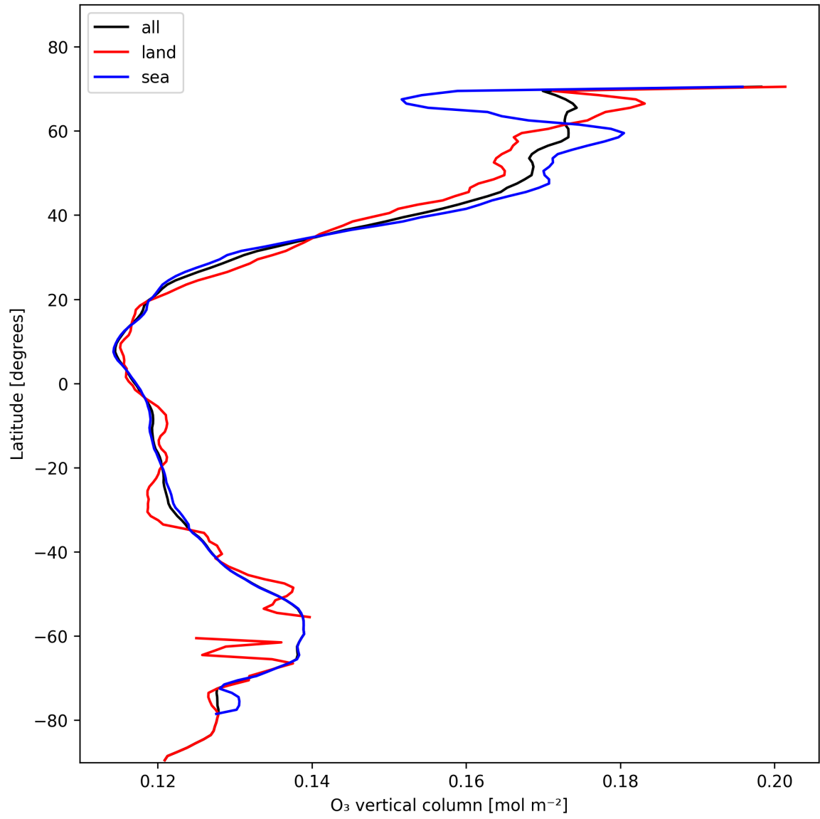
Figure 14: Zonal average of “O 3 vertical column” for 2025-01-23 to 2025-01-25.
