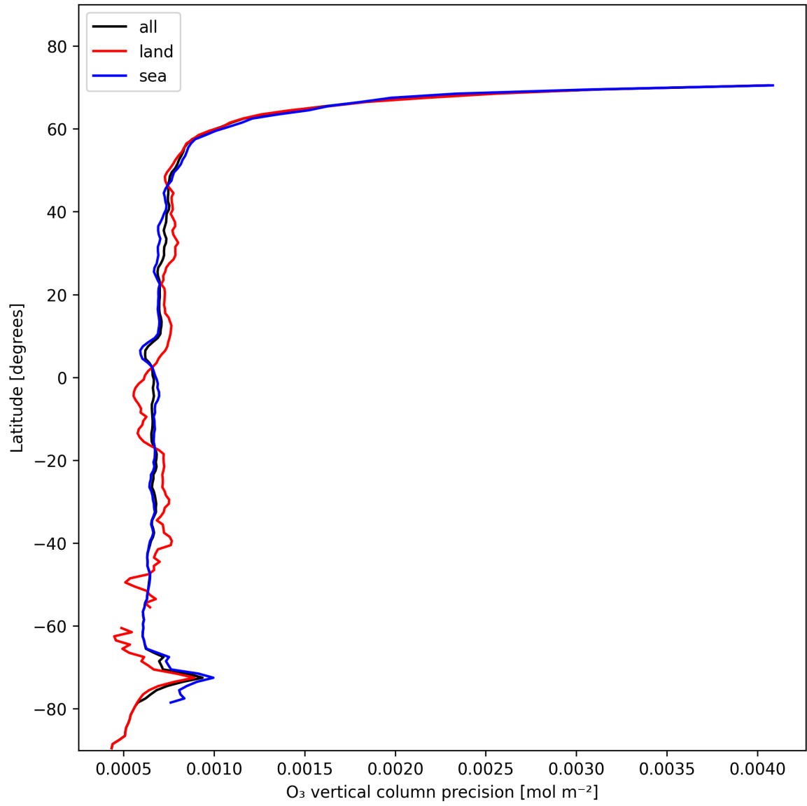
Figure 15: Zonal average of “O 3 vertical column precision” for 2025-01-23 to 2025-01-25.
