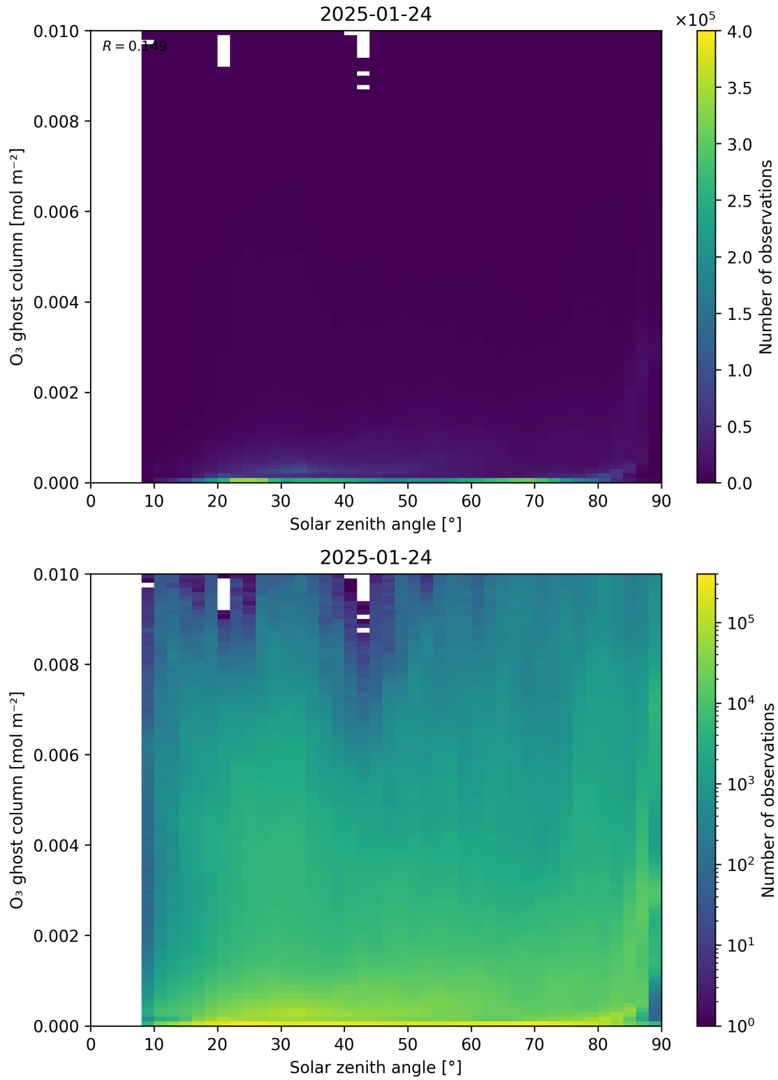
Figure 46: Scatter density plot of “Solar zenith angle” against “O 3 ghost column” for 2025-01-23 to 2025-01-25.
