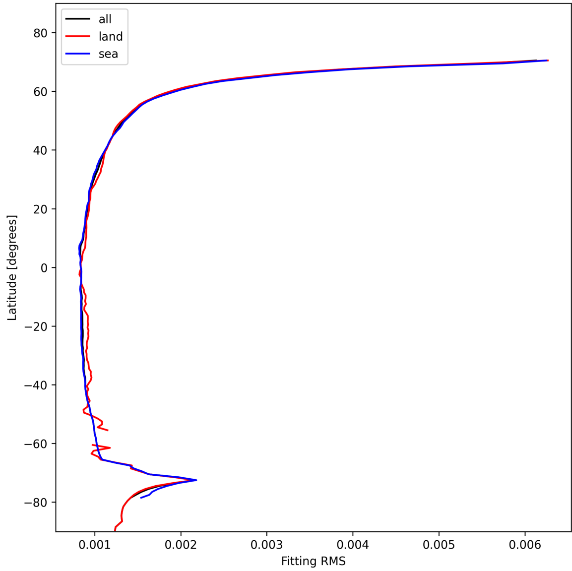
Figure 16: Zonal average of “Fitting RMS” for 2025-01-23 to 2025-01-25.
