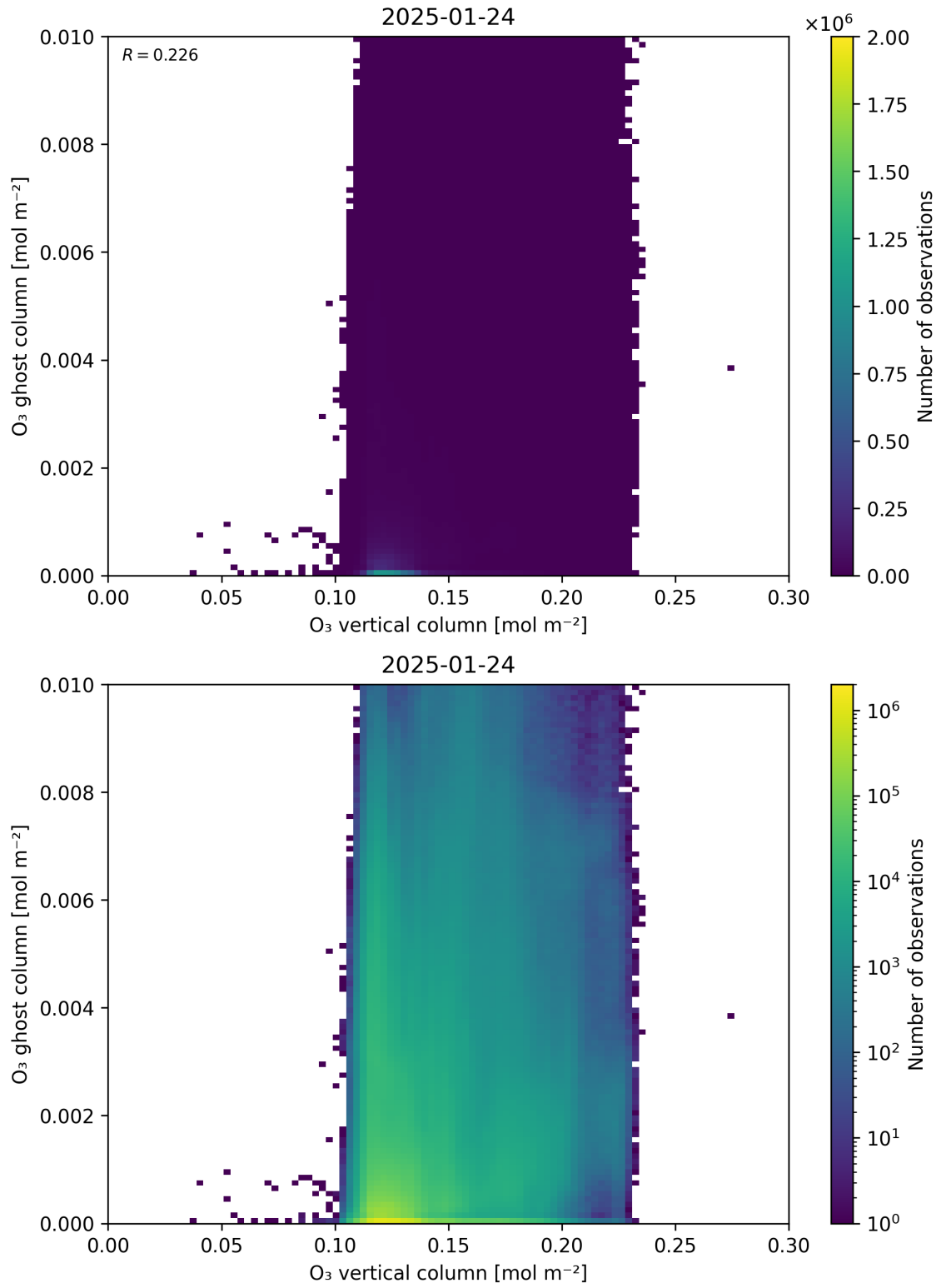
Figure 40: Scatter density plot of “O 3 vertical column” against “O 3 ghost column” for 2025-01-23 to 2025-01-25.
