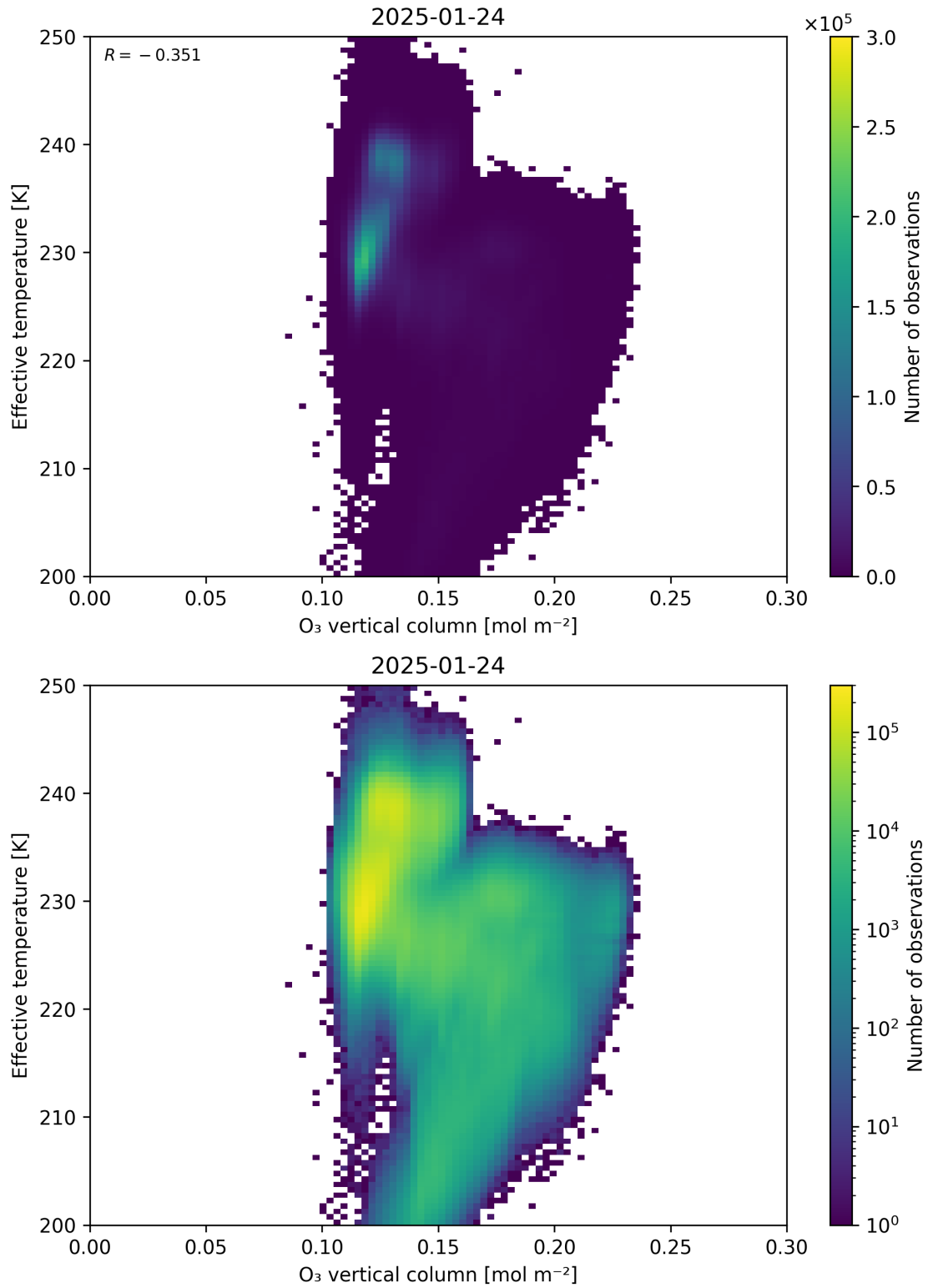
Figure 39: Scatter density plot of “O 3 vertical column” against “Effective temperature” for 2025-01-23 to 2025-01-25.
