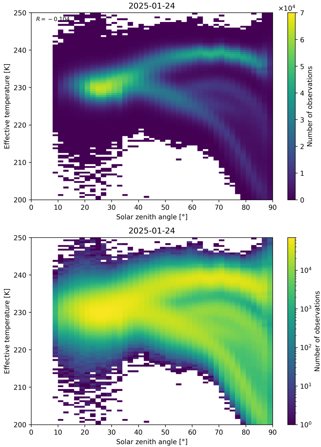
Figure 45: Scatter density plot of “Solar zenith angle” against “Effective temperature” for 2025-01-23 to 2025-01-25.
