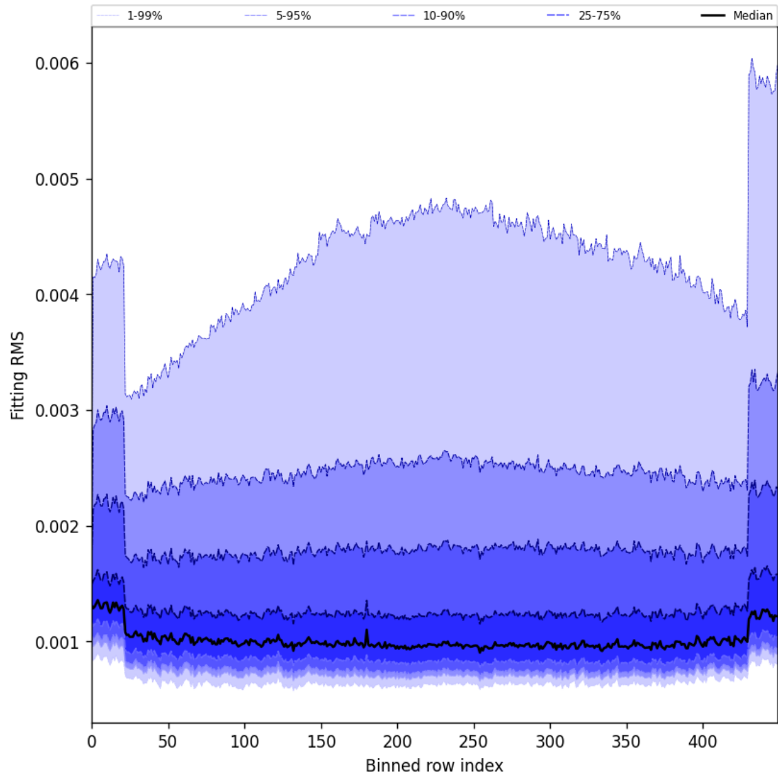
Figure 30: Along track statistics of “Fitting RMS” for 2025-01-23 to 2025-01-25
