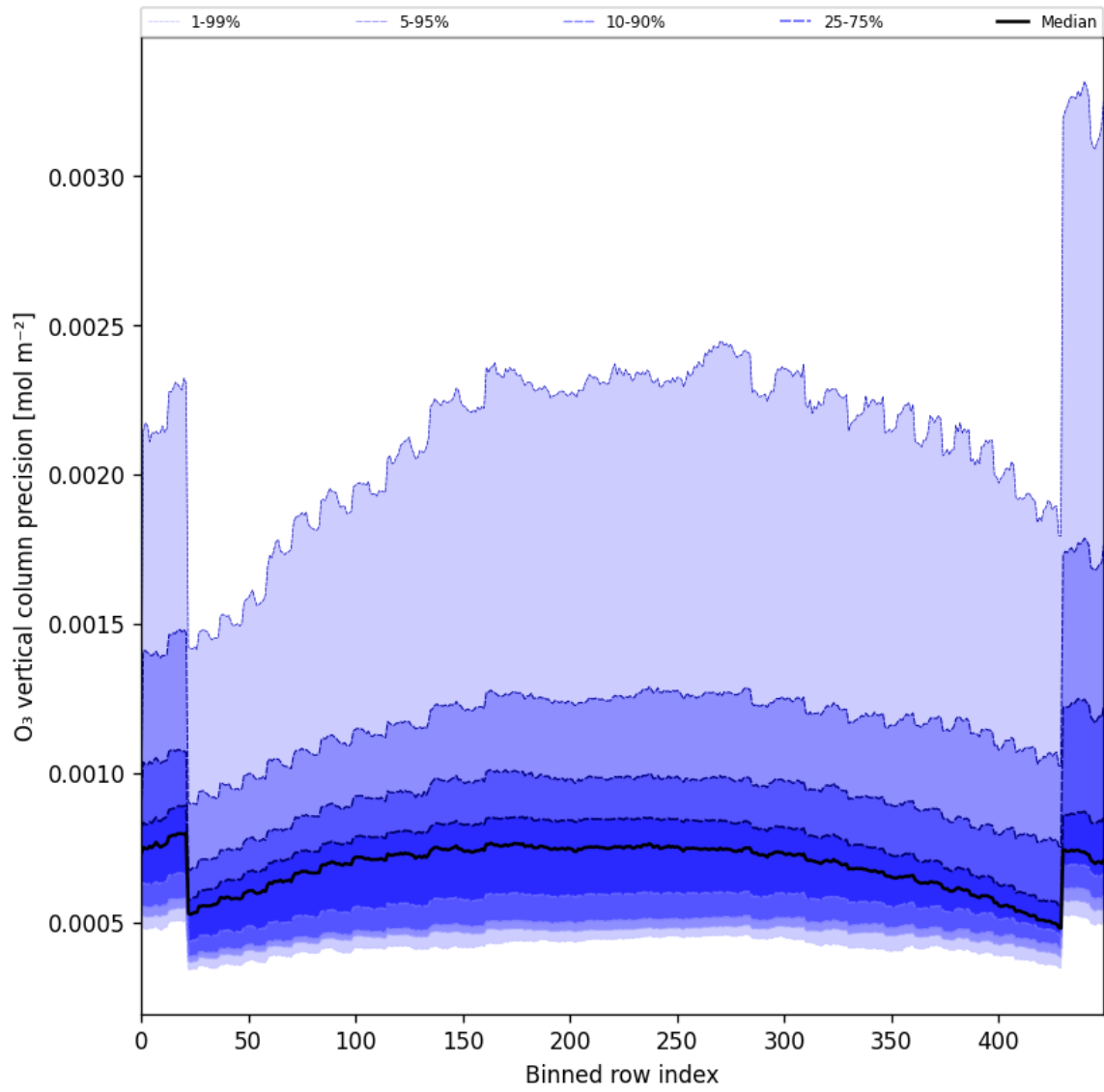
Figure 29: Along track statistics of “O 3 vertical column precision” for 2025-01-23 to 2025-01-25
