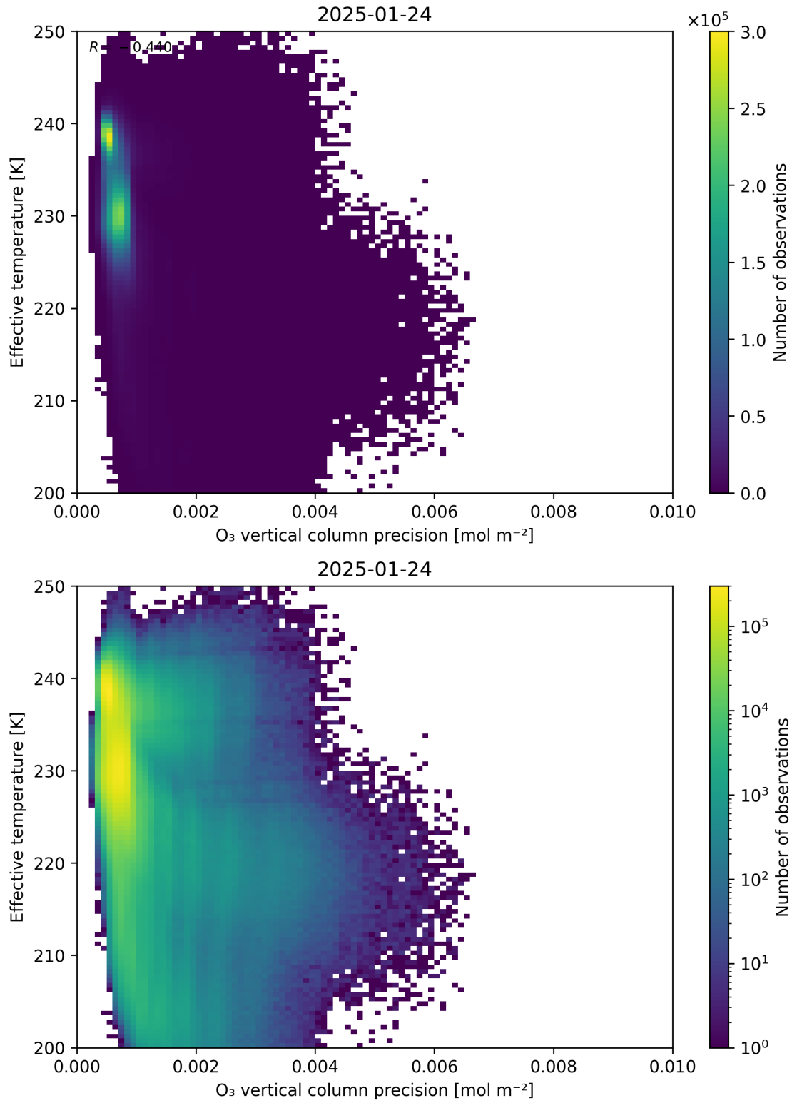
Figure 42: Scatter density plot of “ O_3 vertical column precision” against “Effective temperature” for 2025-01-23 to 2025-01-25.
