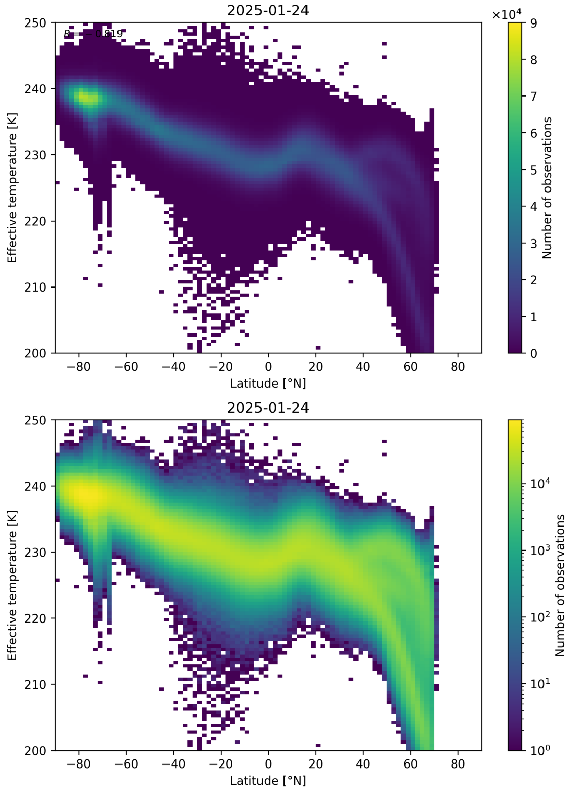
Figure 34: Scatter density plot of “Latitude” against “Effective temperature” for 2025-01-23 to 2025-01-25.
