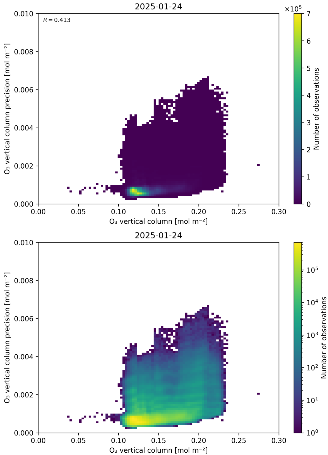
Figure 41: Scatter density plot of “O 3 vertical column” against “O 3 vertical column precision” for 2025-01-23 to 2025-01-25.
