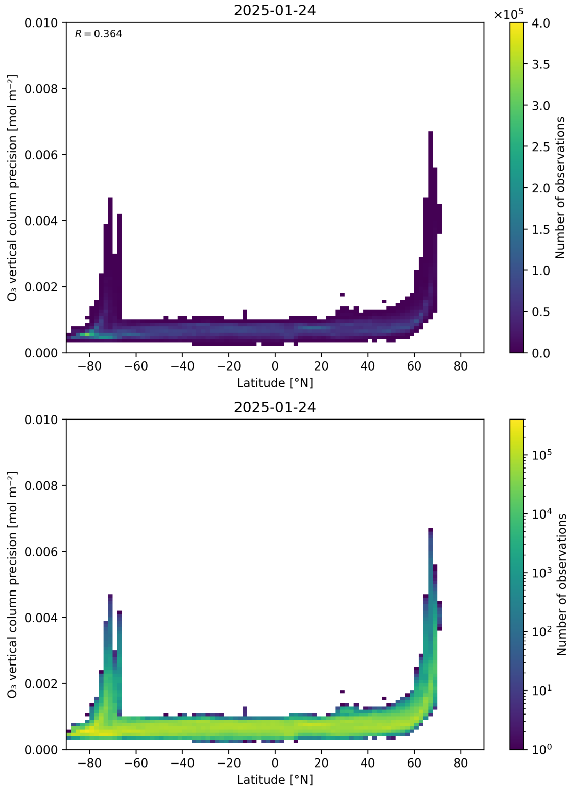
Figure 37: Scatter density plot of “Latitude” against “O 3 vertical column precision” for 2025-01-23 to 2025-01-25.
