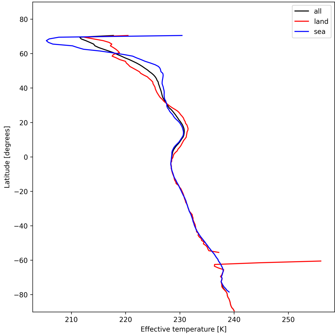
Figure 17: Zonal average of “Effective temperature” for 2025-01-23 to 2025-01-25.
