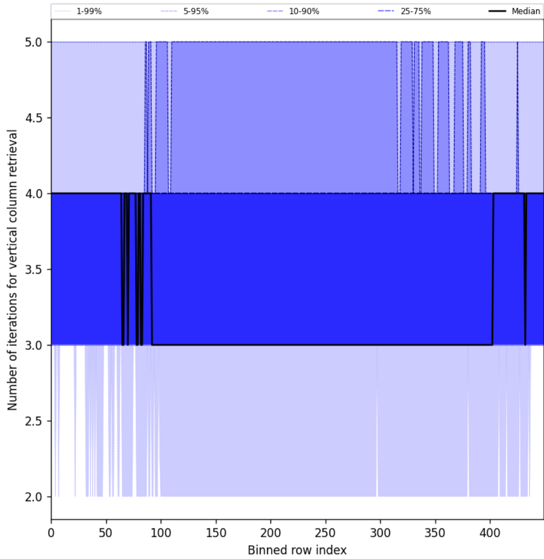
Figure 33: Along track statistics of “Number of iterations for vertical column retrieval” for 2025-01-23 to 2025-01-25
