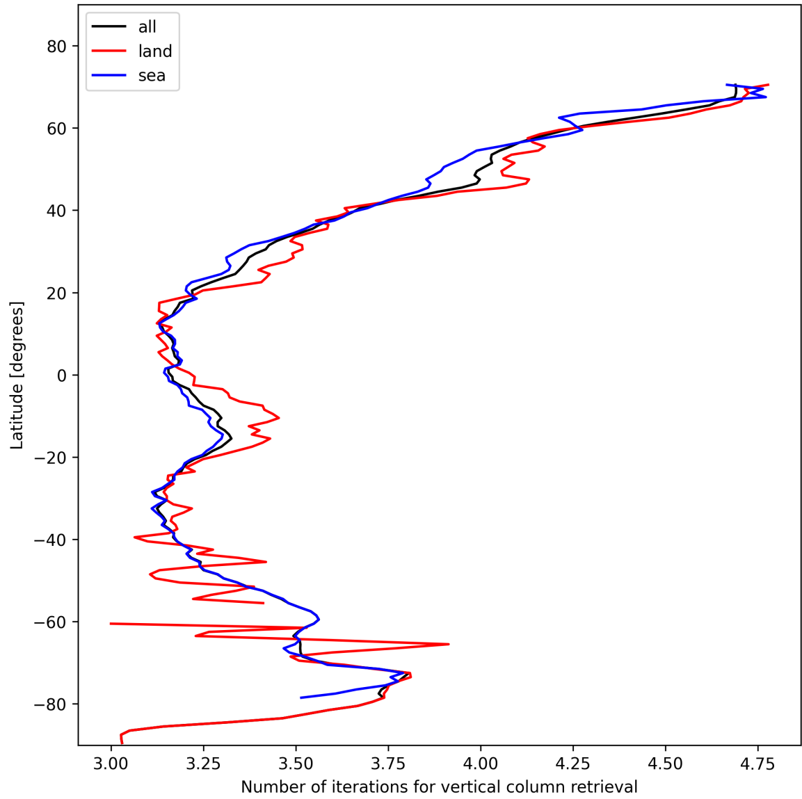
Figure 19: Zonal average of “Number of iterations for vertical column retrieval” for 2025-01-23 to 2025-01-25.
