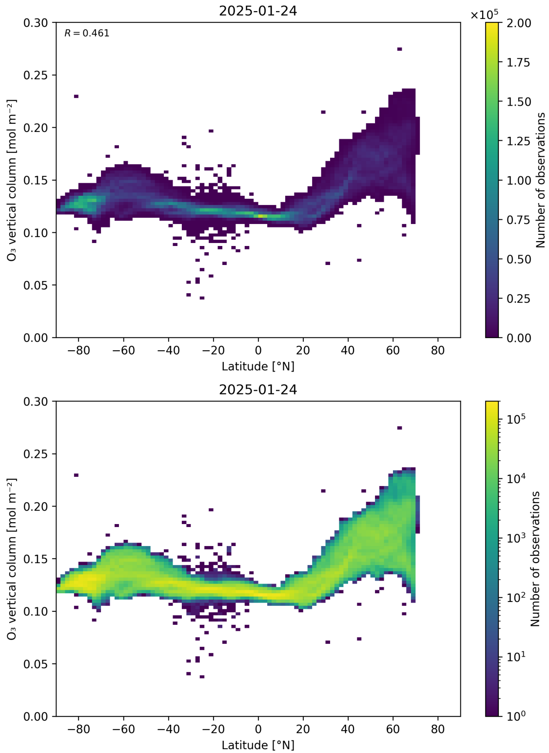
Figure 36: Scatter density plot of “Latitude” against “O 3 vertical column” for 2025-01-23 to 2025-01-25.
