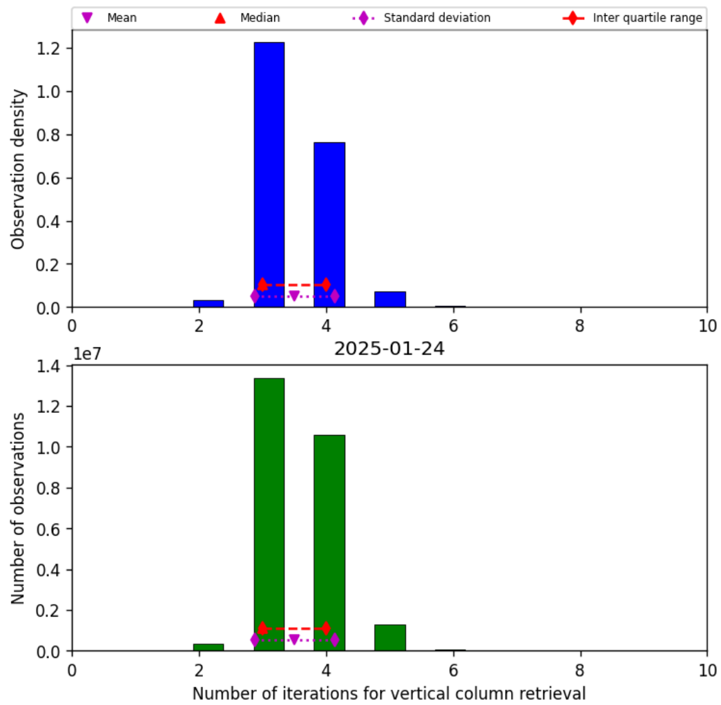
Figure 26: Histogram of “Number of iterations for vertical column retrieval” for 2025-01-23 to 2025-01-25
