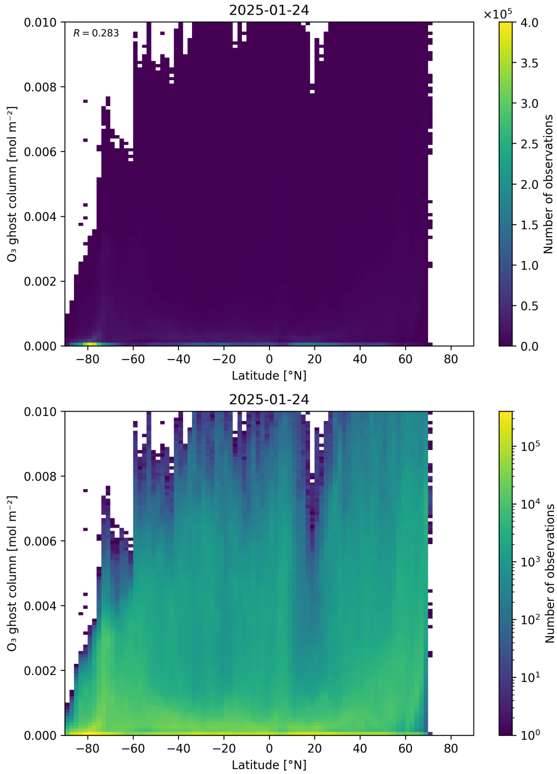
Figure 35: Scatter density plot of “Latitude” against “O 3 ghost column” for 2025-01-23 to 2025-01-25.
