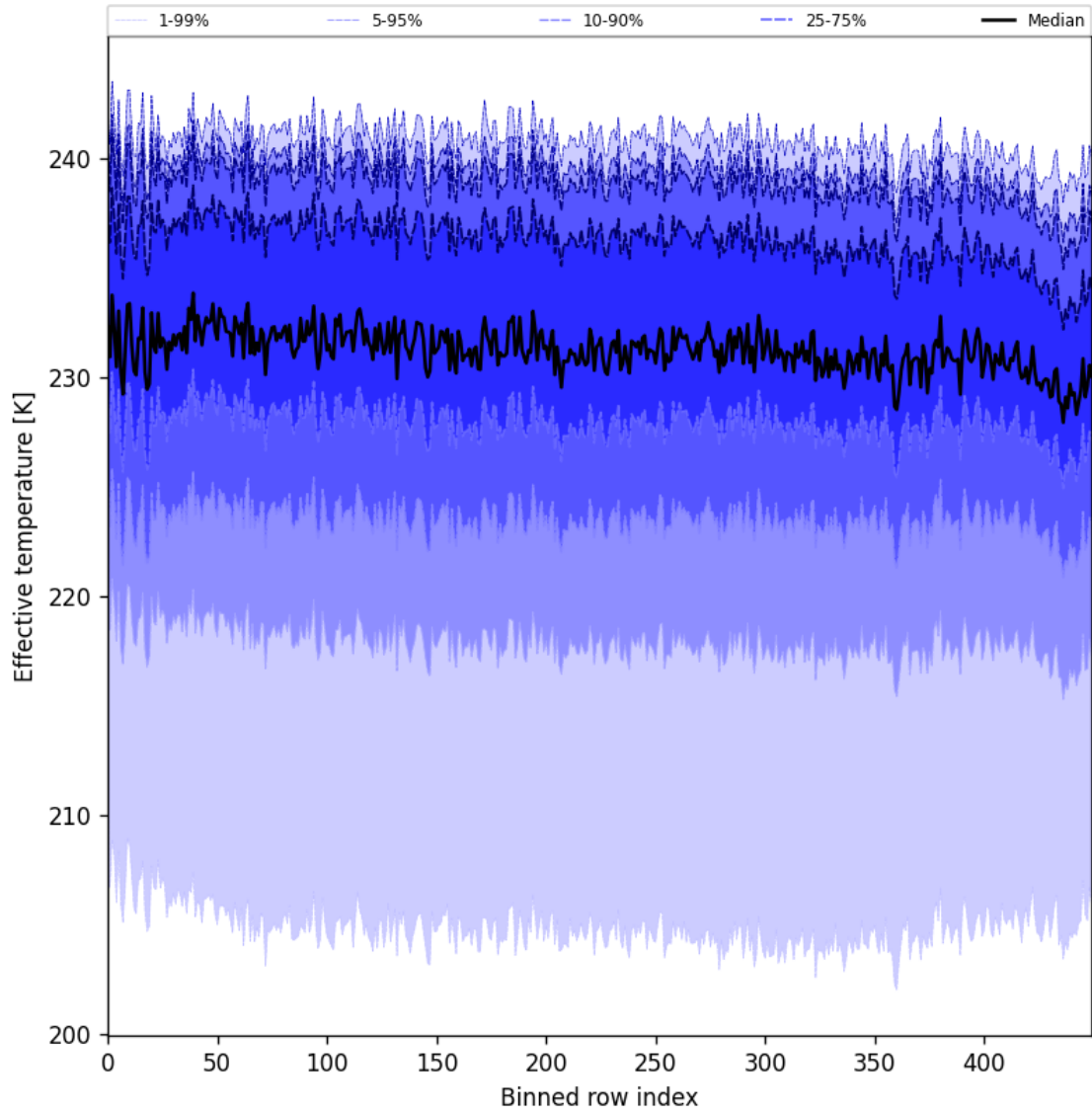
Figure 31: Along track statistics of “Effective temperature” for 2025-01-23 to 2025-01-25
