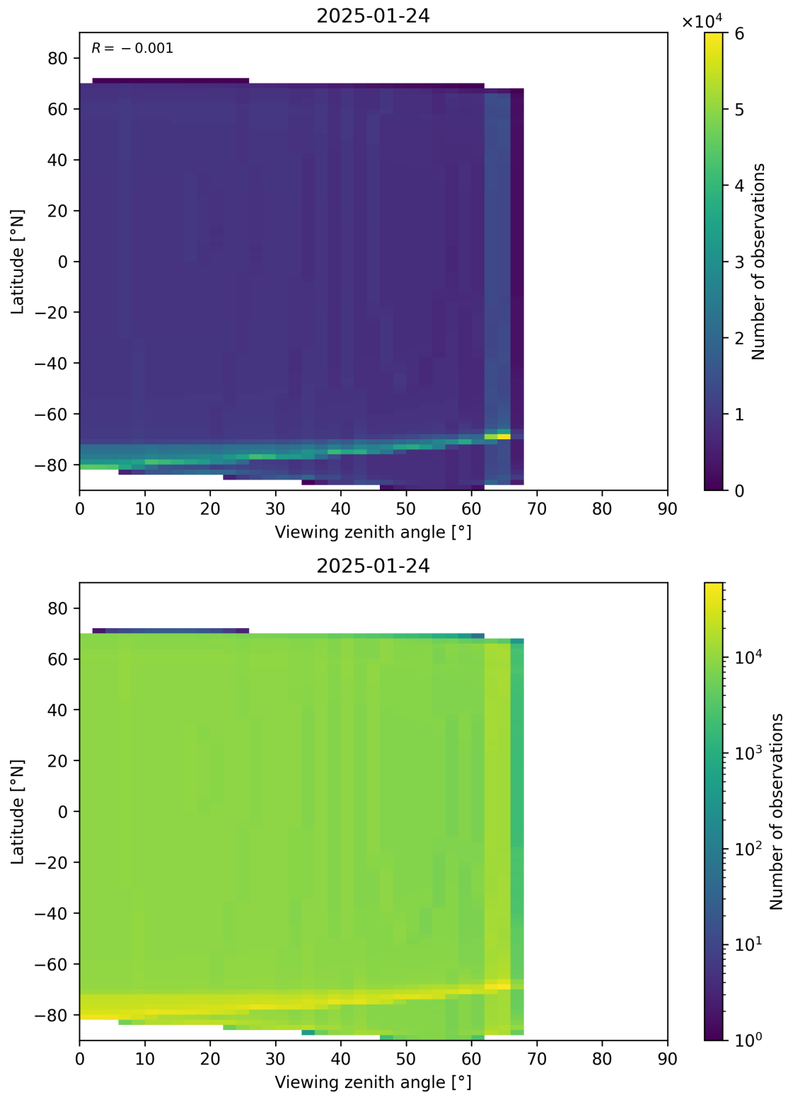
Figure 49: Scatter density plot of “Viewing zenith angle” against “Latitude” for 2025-01-23 to 2025-01-25.
