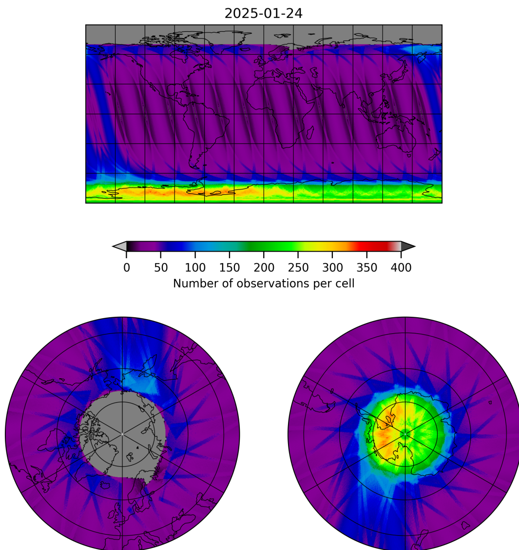
Figure 12: Map of the number of observations for 2025-01-23 to 2025-01-25
