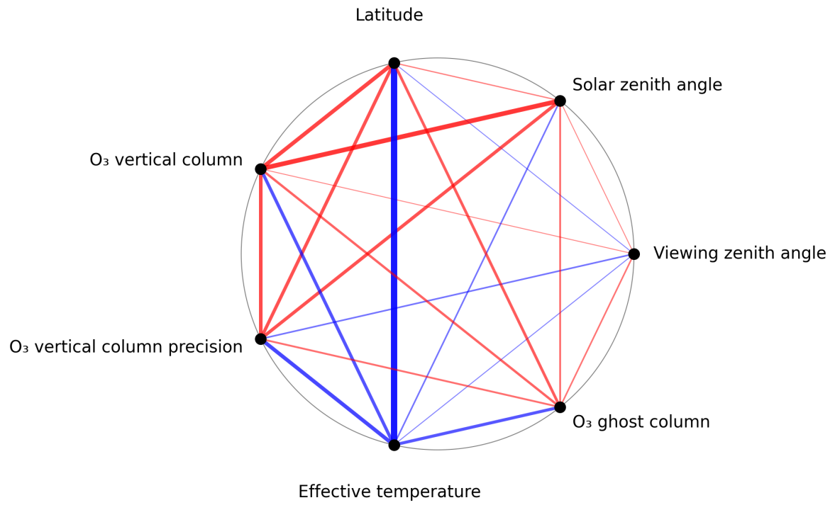
Figure 1: Map of correlation graph for 2025-01-23 to 2025-01-25.
