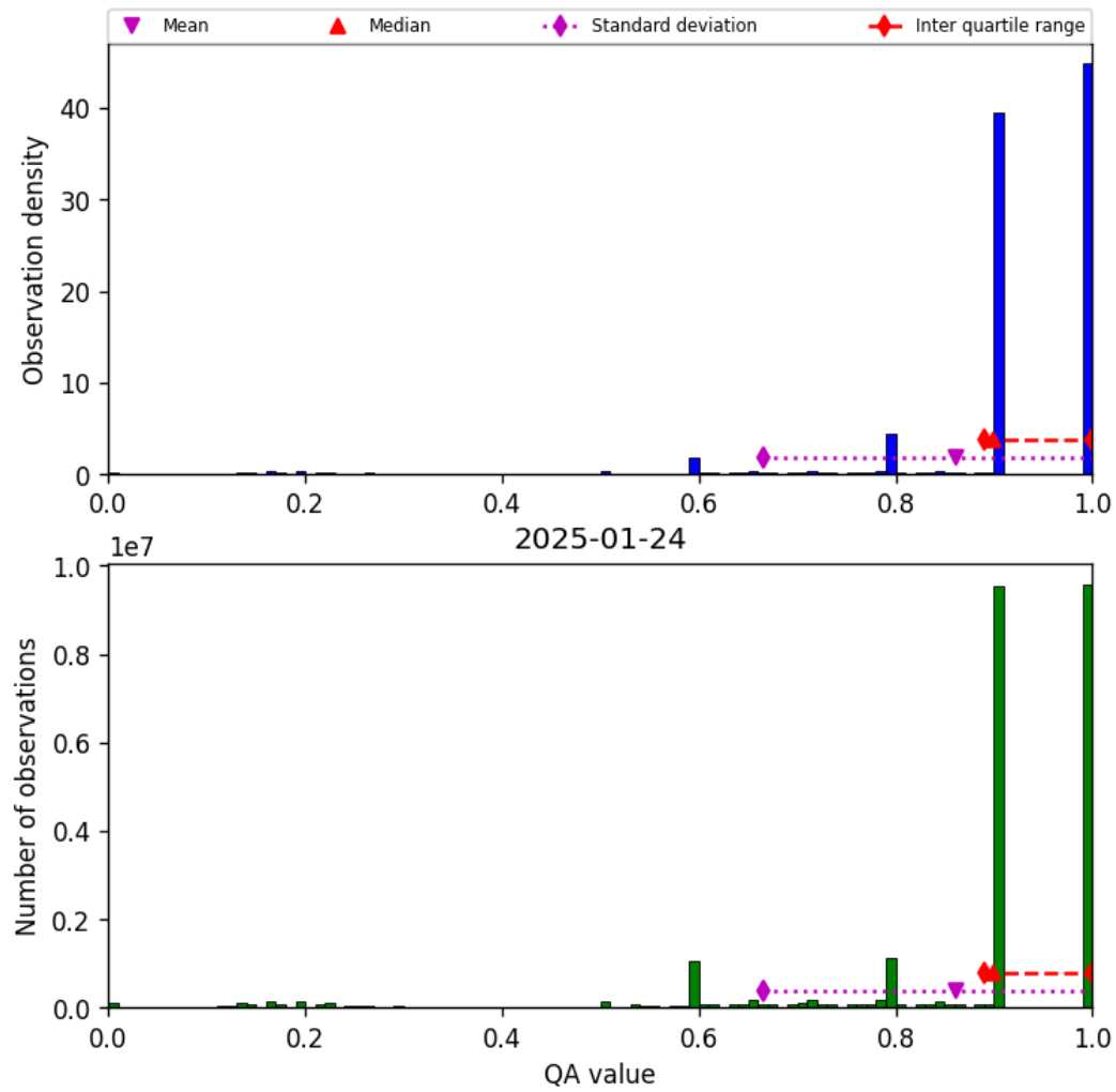
Figure 20: Histogram of “QA value” for 2025-01-23 to 2025-01-25
