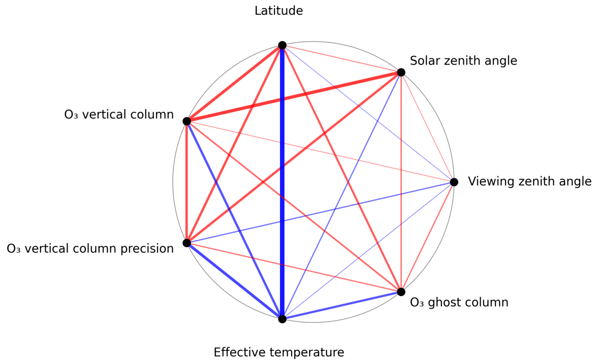
Figure 1: Map of correlation graph for 2025-01-24 to 2025-01-26.
