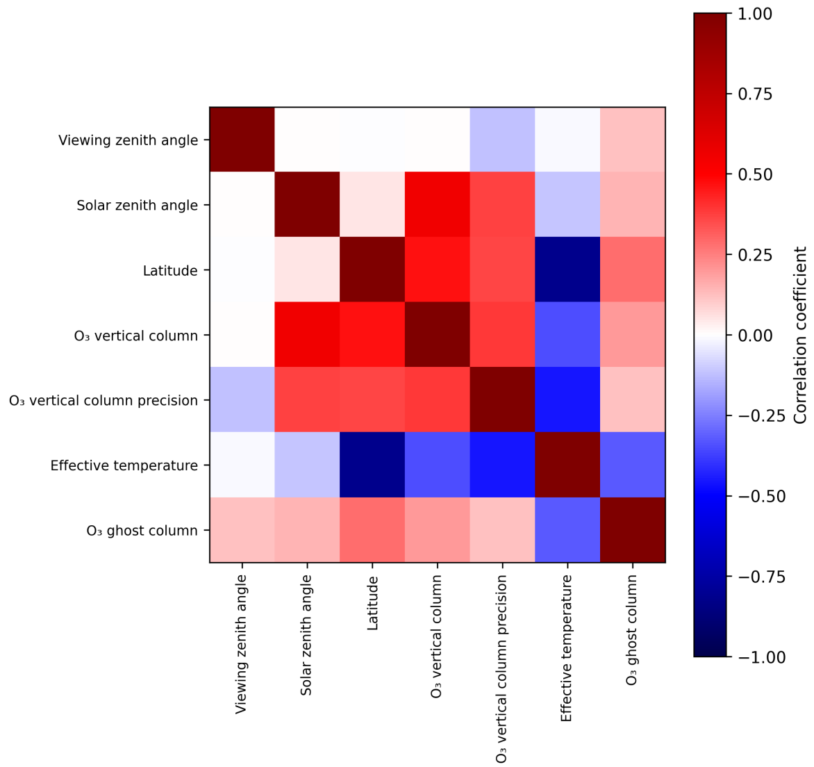
Figure 2: Map of correlation matrix for 2025-01-24 to 2025-01-26.
