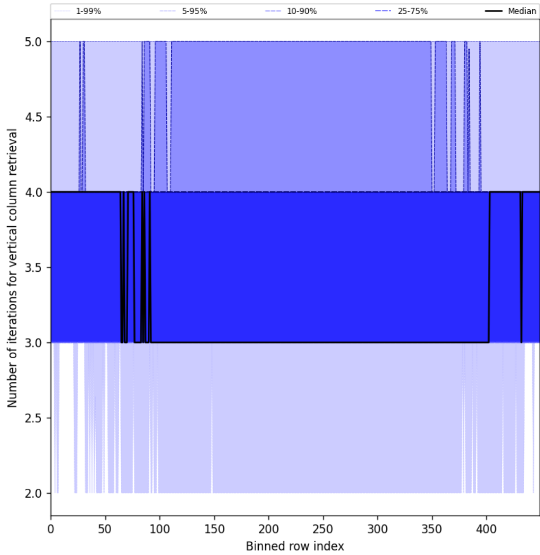
Figure 33: Along track statistics of “Number of iterations for vertical column retrieval” for 2025-01-24 to 2025-01-26
