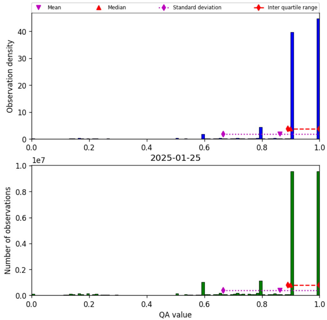
Figure 20: Histogram of “QA value” for 2025-01-24 to 2025-01-26
