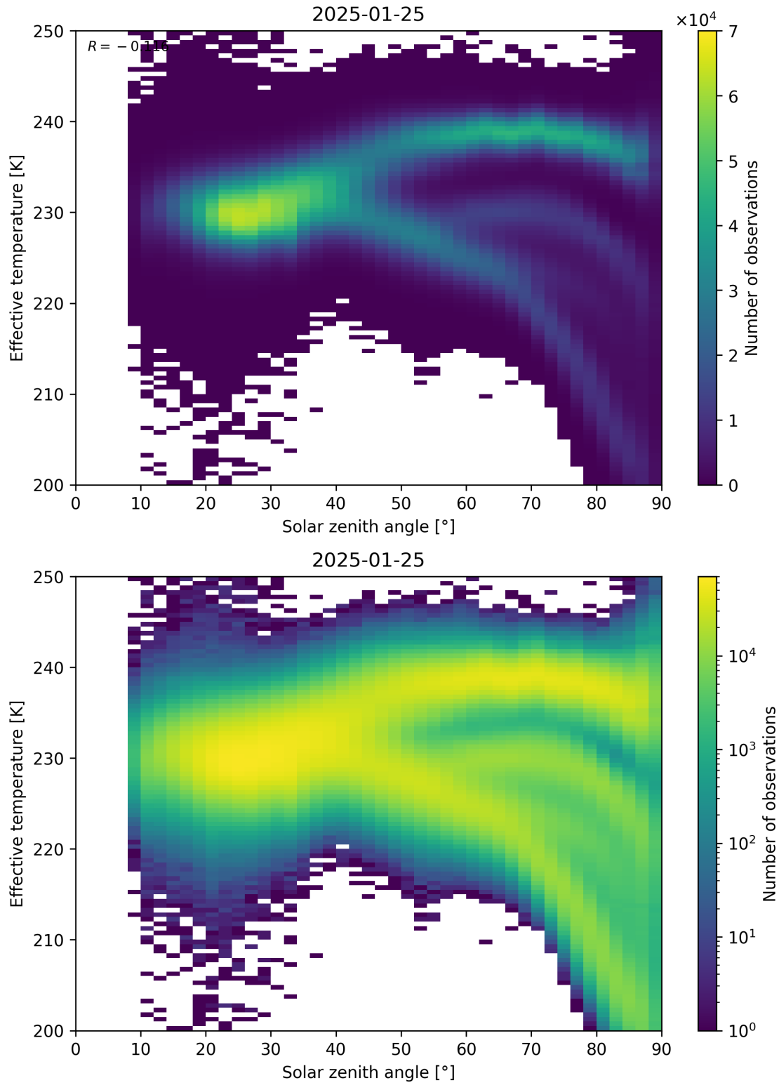
Figure 45: Scatter density plot of “Solar zenith angle” against “Effective temperature” for 2025-01-24 to 2025-01-26.
