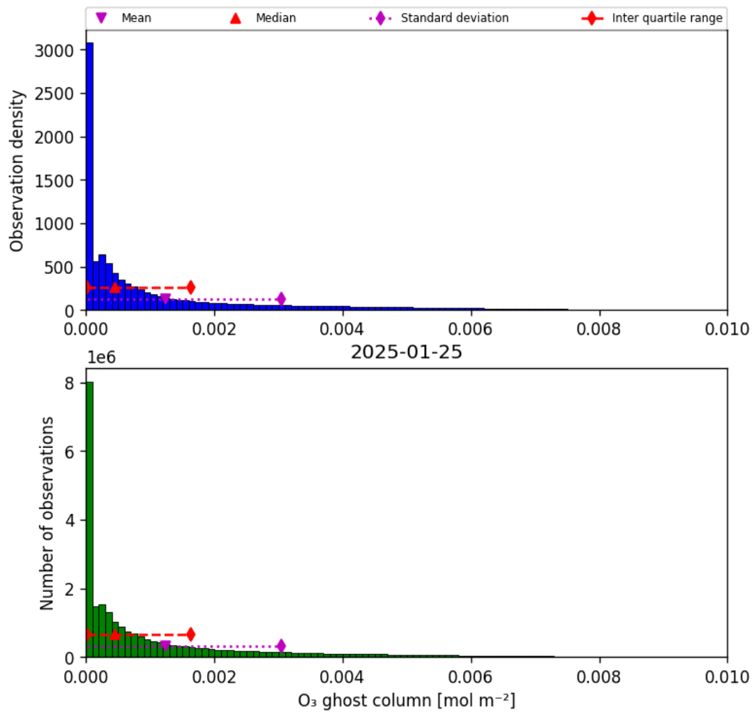
Figure 25: Histogram of “O 3 ghost column” for 2025-01-24 to 2025-01-26
