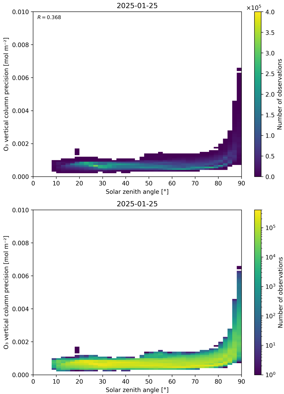
Figure 48: Scatter density plot of “Solar zenith angle” against “O 3 vertical column precision” for 2025-01-24 to 2025-01-26.
