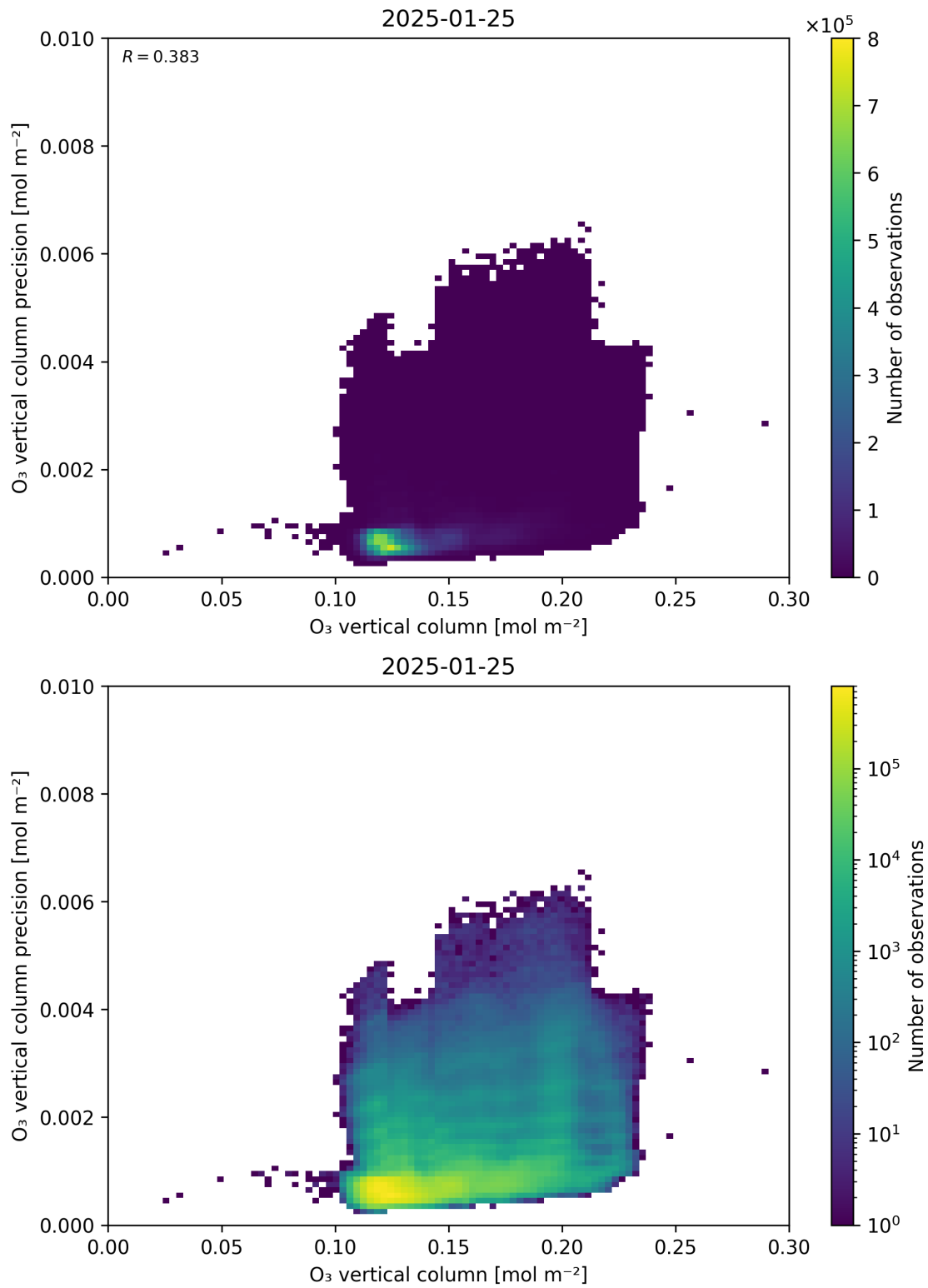
Figure 41: Scatter density plot of “O 3 vertical column” against “O 3 vertical column precision” for 2025-01-24 to 2025-01-26.
