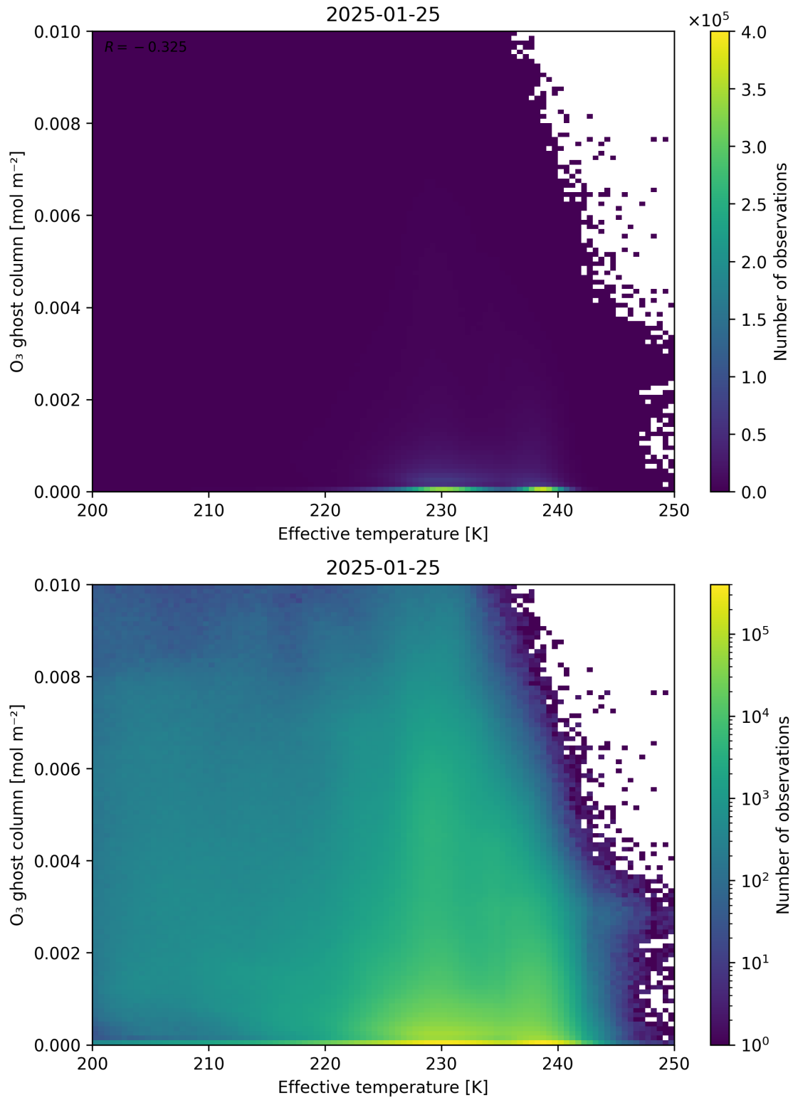
Figure 38: Scatter density plot of “Effective temperature” against “O 3 ghost column” for 2025-01-24 to 2025-01-26.
