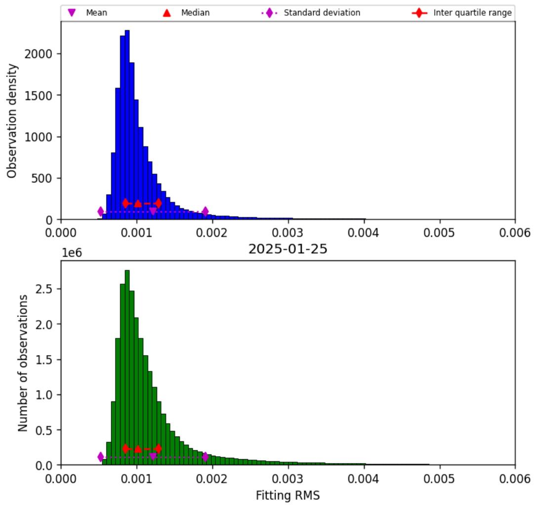
Figure 23: Histogram of “Fitting RMS” for 2025-01-24 to 2025-01-26
