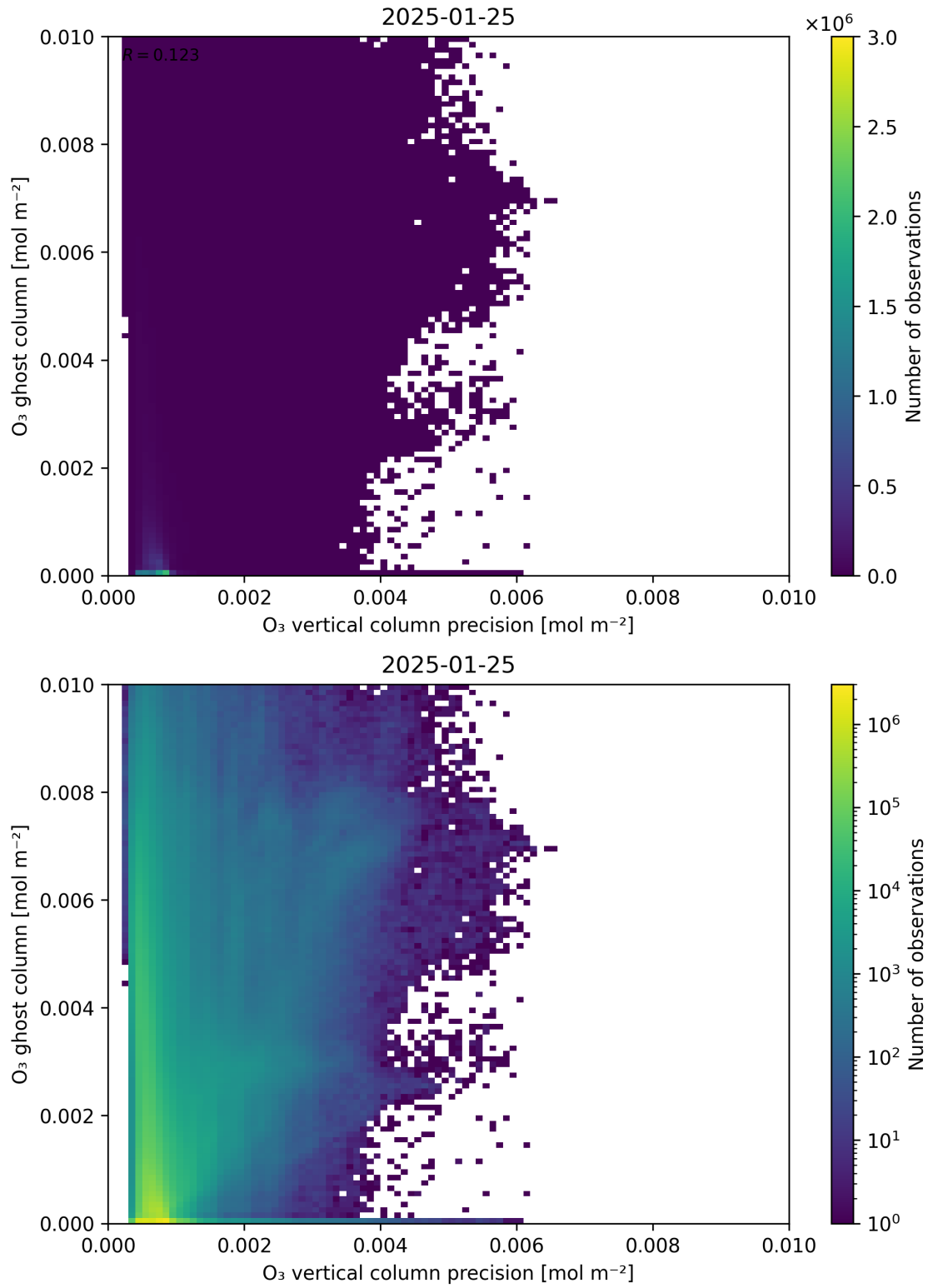
Figure 43: Scatter density plot of “O 3 vertical column precision” against “O 3 ghost column” for 2025-01-24 to 2025-01-26.
