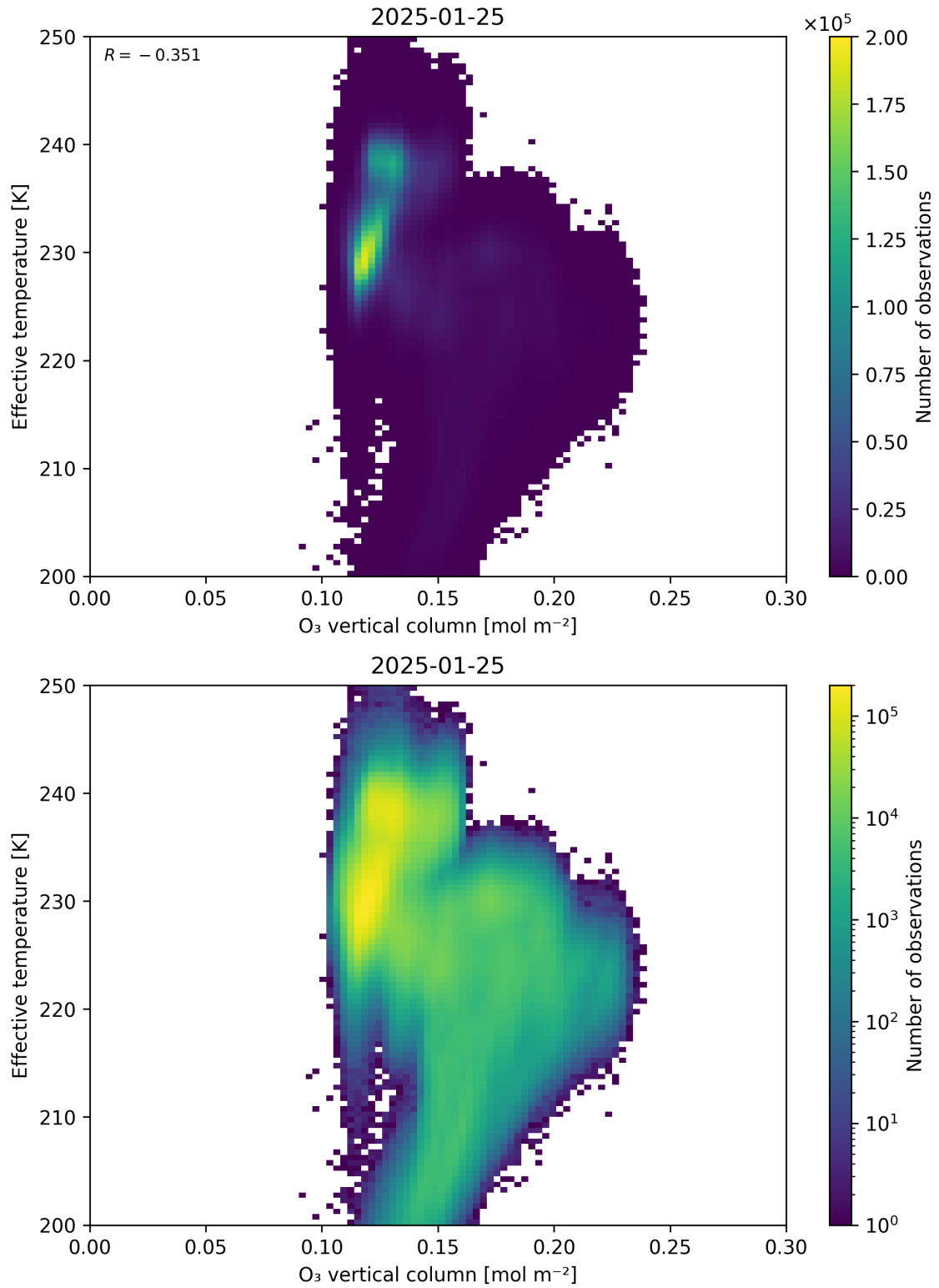
Figure 39: Scatter density plot of “O 3 vertical column” against “Effective temperature” for 2025-01-24 to 2025-01-26.
