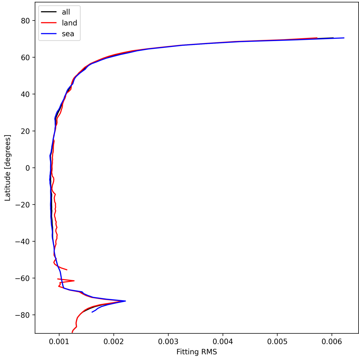
Figure 16: Zonal average of “Fitting RMS” for 2025-01-24 to 2025-01-26.
