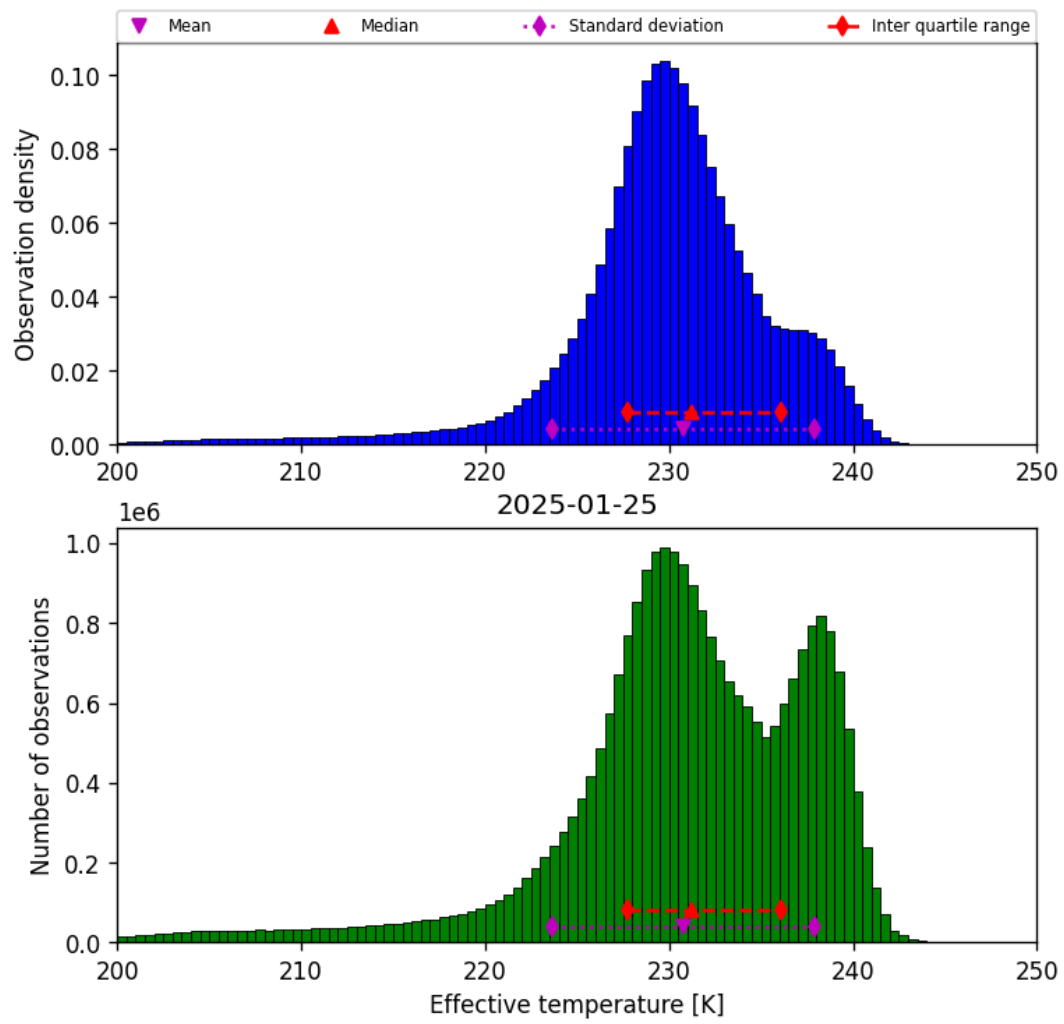
Figure 24: Histogram of “Effective temperature” for 2025-01-24 to 2025-01-26
