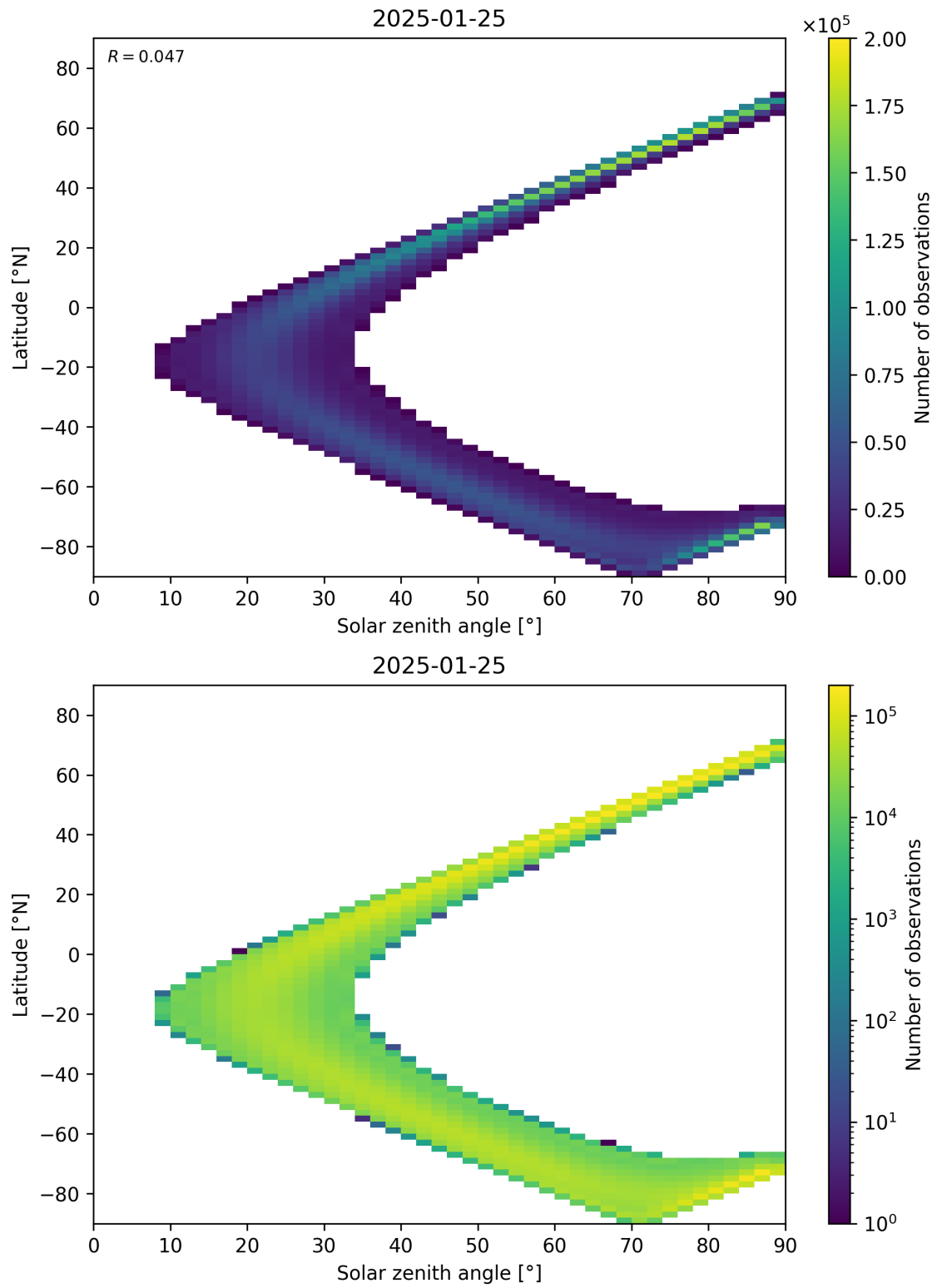
Figure 44: Scatter density plot of “Solar zenith angle” against “Latitude” for 2025-01-24 to 2025-01-26.
