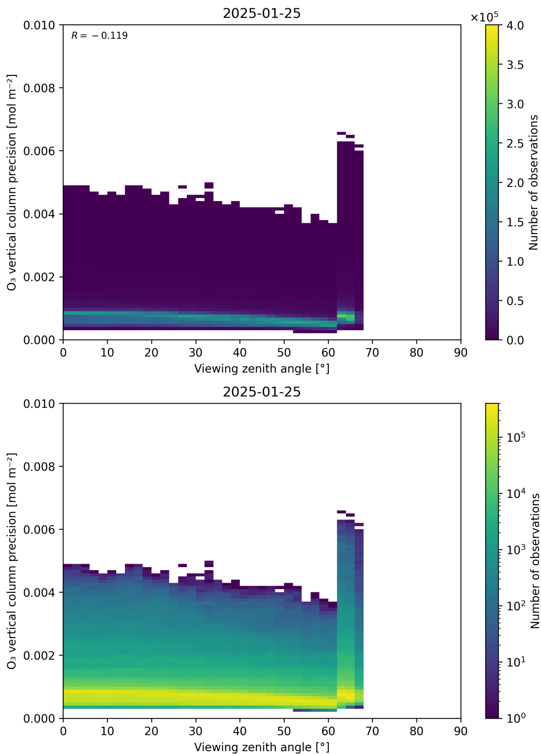
Figure 53: Scatter density plot of “Viewing zenith angle” against “O 3 vertical column precision” for 2025-01-24 to 2025-01-26.
