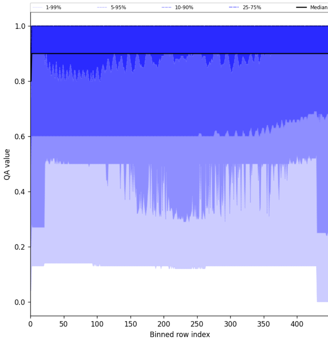
Figure 27: Along track statistics of “QA value” for 2025-01-24 to 2025-01-26
