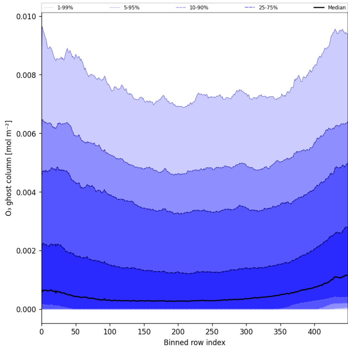
Figure 32: Along track statistics of “O 3 ghost column” for 2025-01-24 to 2025-01-26
