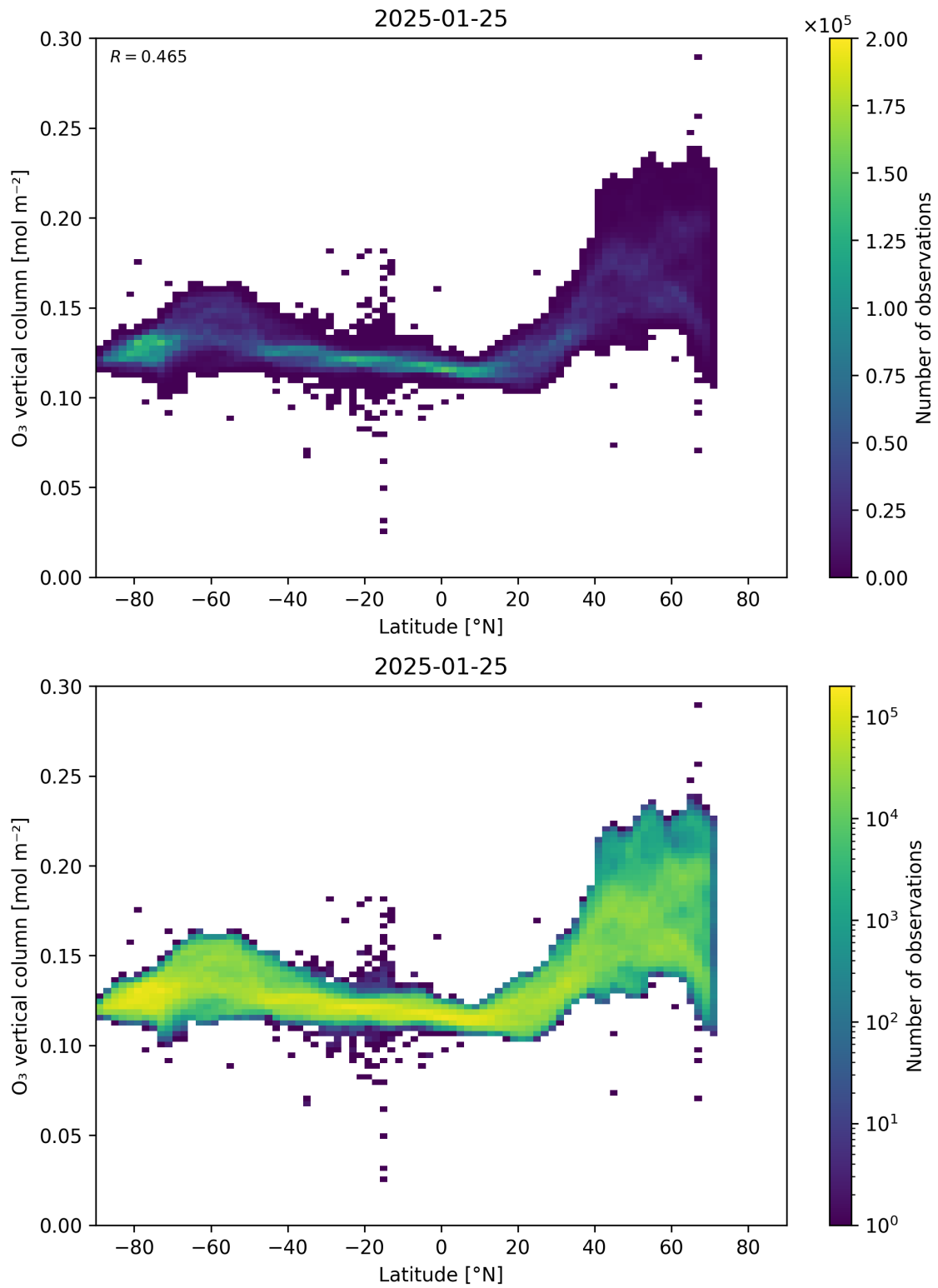
Figure 36: Scatter density plot of “Latitude” against “O 3 vertical column” for 2025-01-24 to 2025-01-26.
