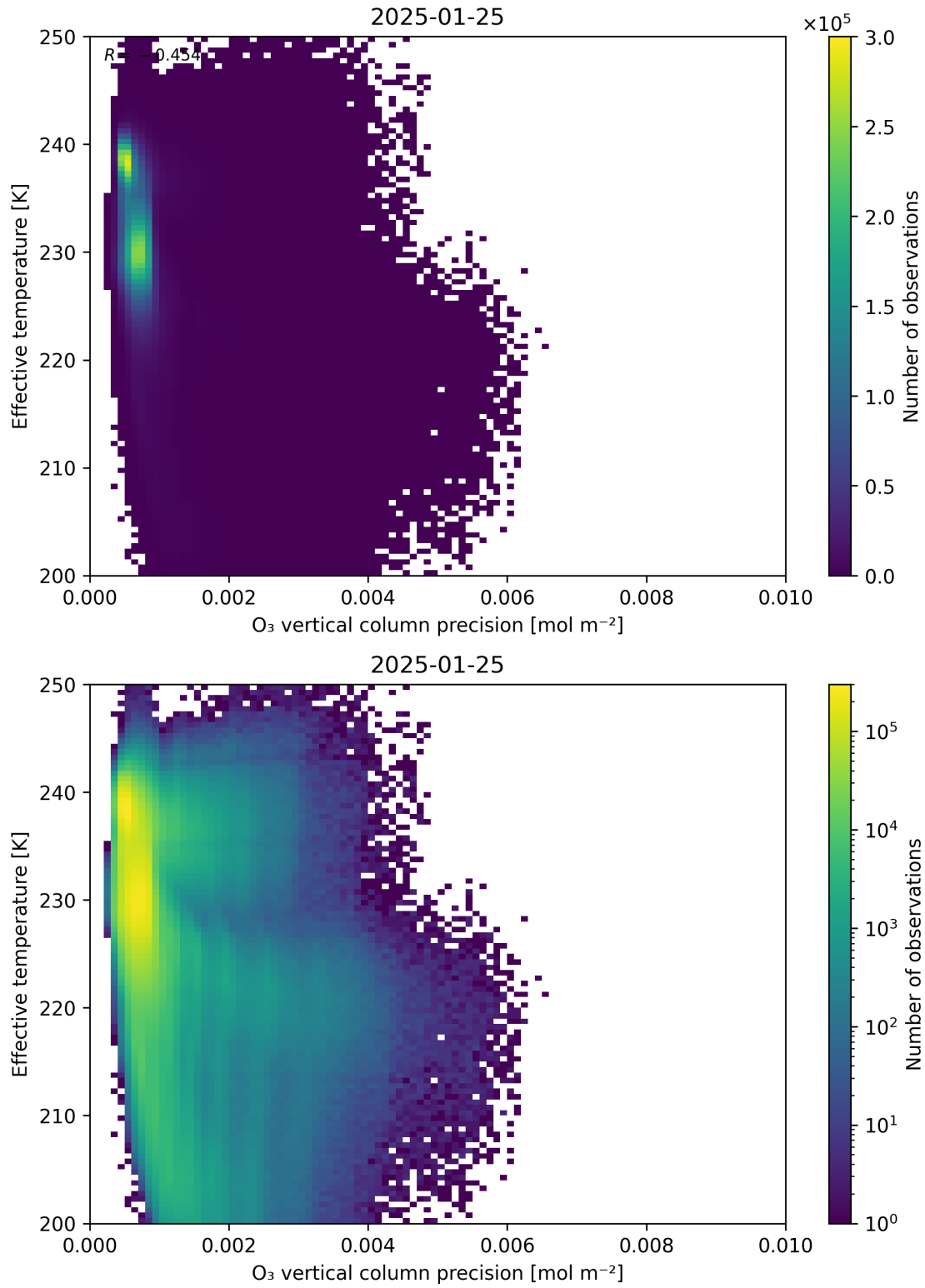
Figure 42: Scatter density plot of “O 3 vertical column precision” against “Effective temperature” for 2025-01-24 to 2025-01-26.
