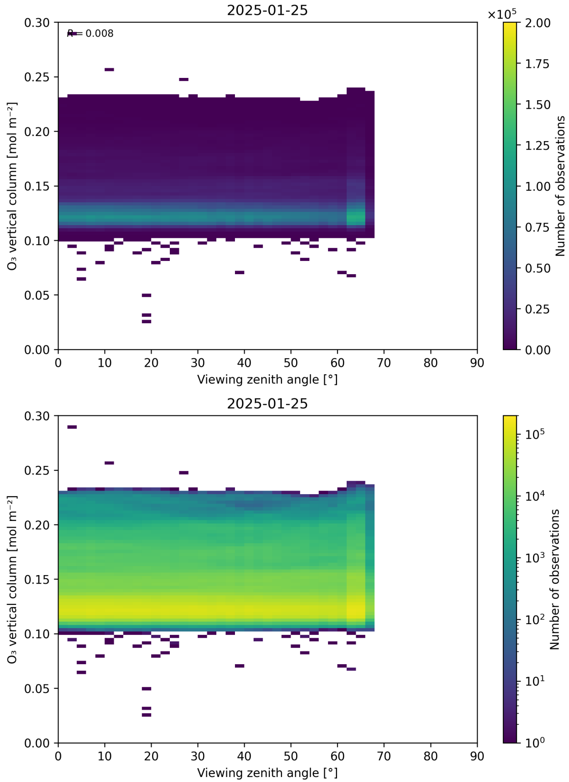
Figure 52: Scatter density plot of “Viewing zenith angle” against “O 3 vertical column” for 2025-01-24 to 2025-01-26.
