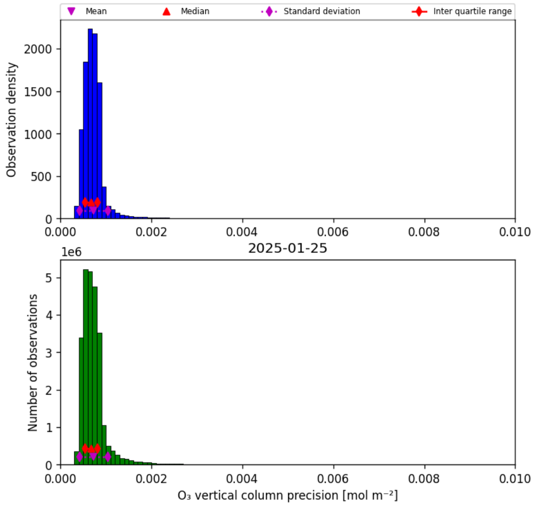
Figure 22: Histogram of “O 3 vertical column precision” for 2025-01-24 to 2025-01-26
