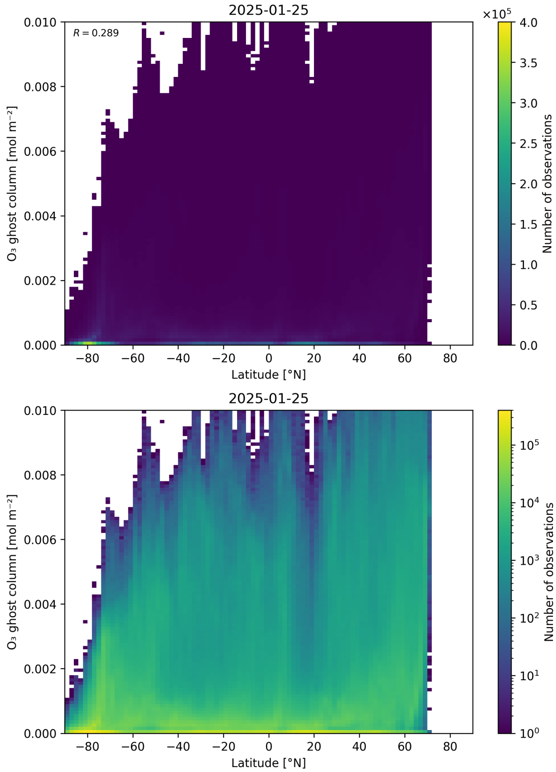
Figure 35: Scatter density plot of “Latitude” against “O 3 ghost column” for 2025-01-24 to 2025-01-26.
