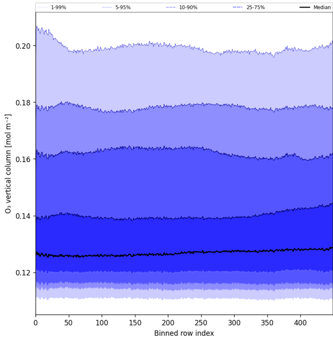
Figure 28: Along track statistics of “ O_3 vertical column” for 2025-01-24 to 2025-01-26
