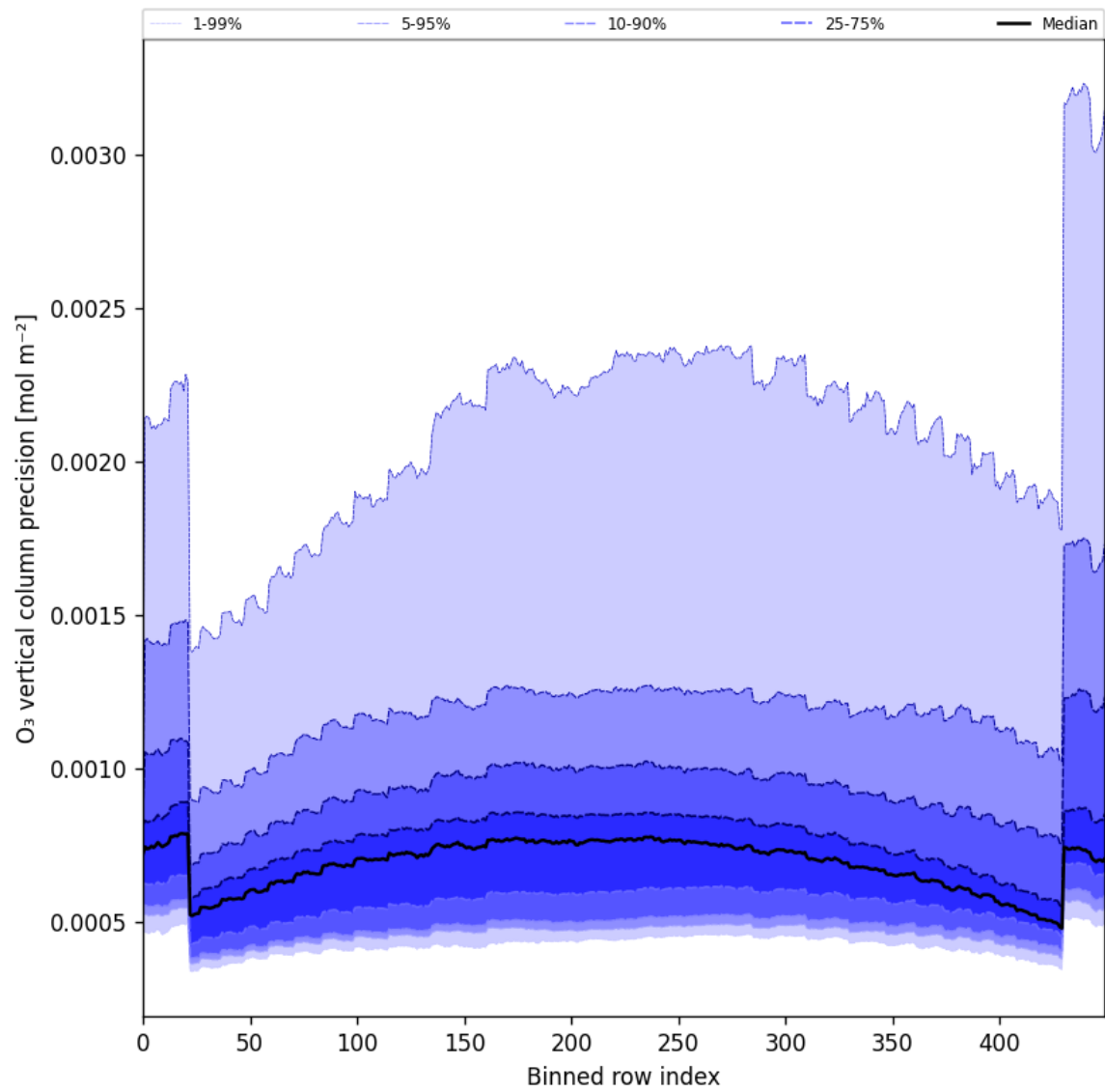
Figure 29: Along track statistics of “O 3 vertical column precision” for 2025-01-24 to 2025-01-26
