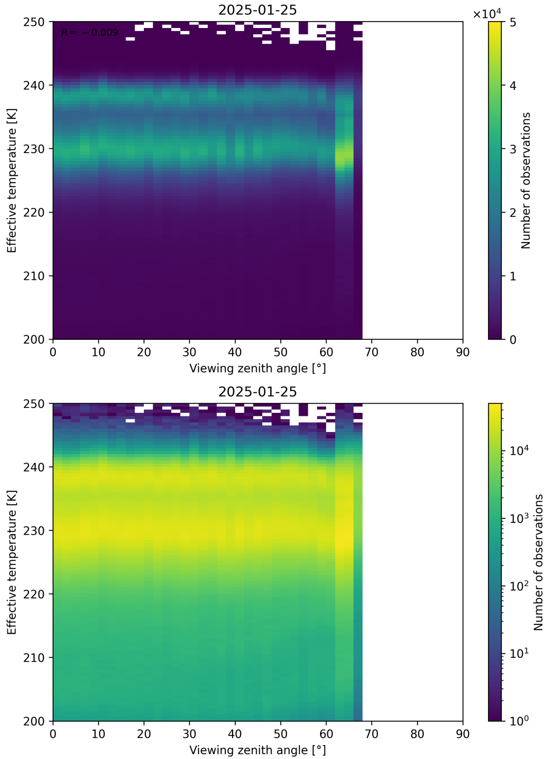
Figure 50: Scatter density plot of “Viewing zenith angle” against “Effective temperature” for 2025-01-24 to 2025-01-26.
