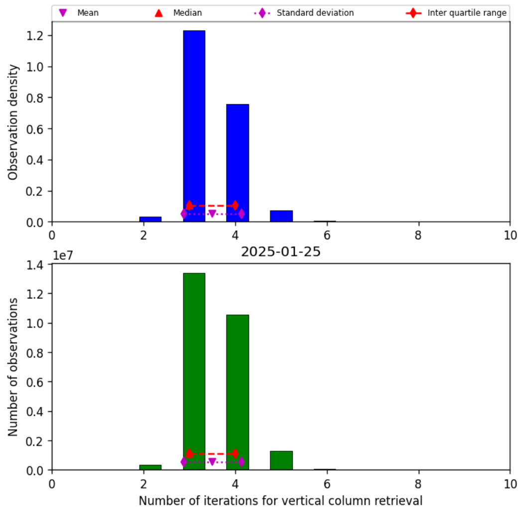
Figure 26: Histogram of “Number of iterations for vertical column retrieval” for 2025-01-24 to 2025-01-26
