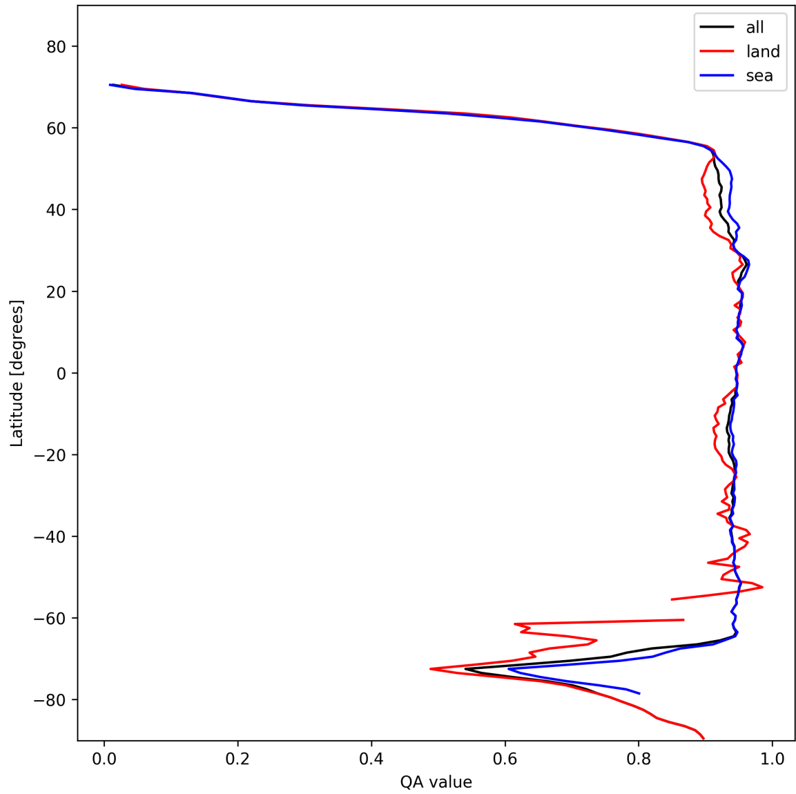
Figure 13: Zonal average of “QA value” for 2025-01-24 to 2025-01-26.
