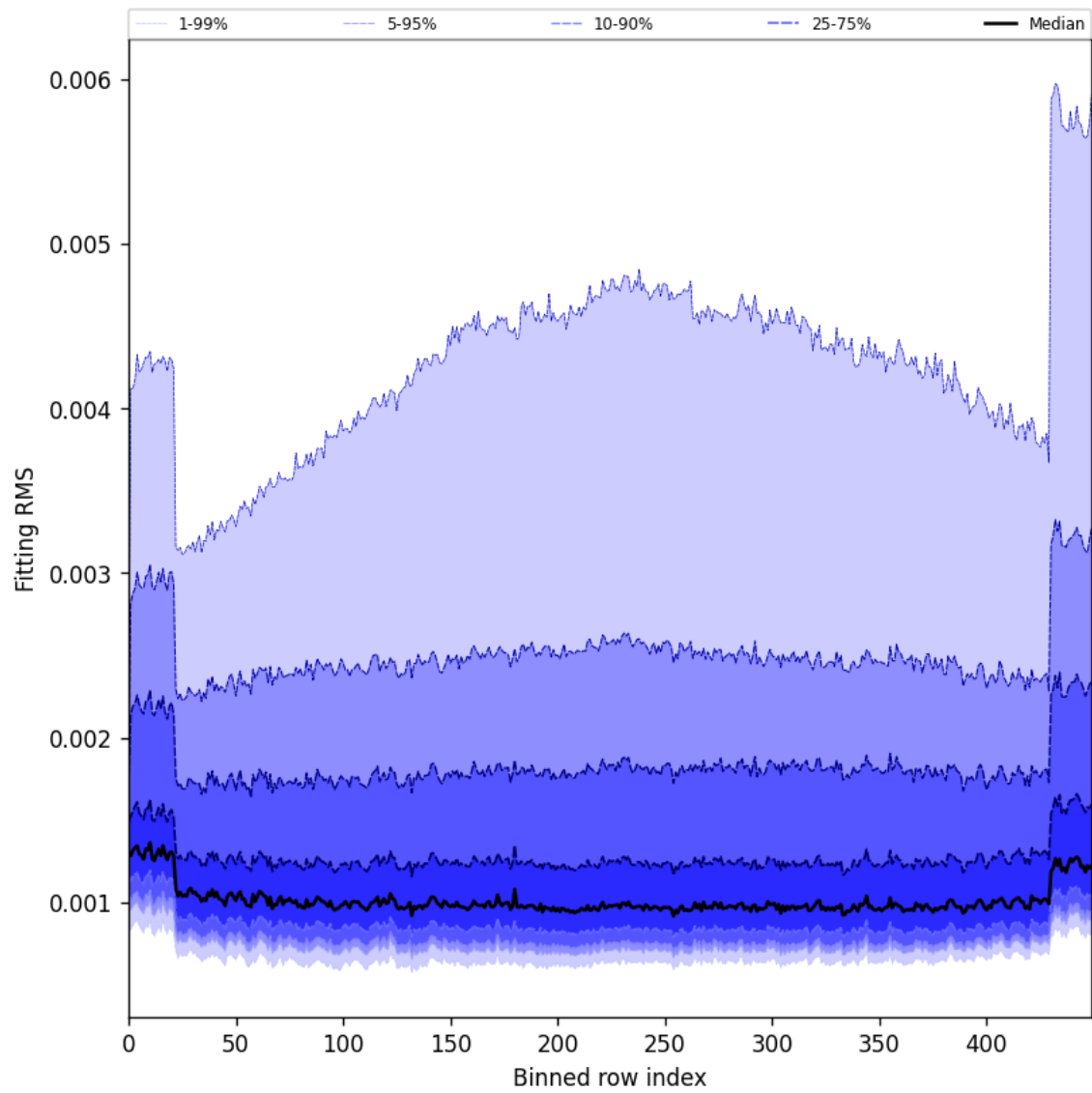
Figure 30: Along track statistics of “Fitting RMS” for 2025-01-24 to 2025-01-26
