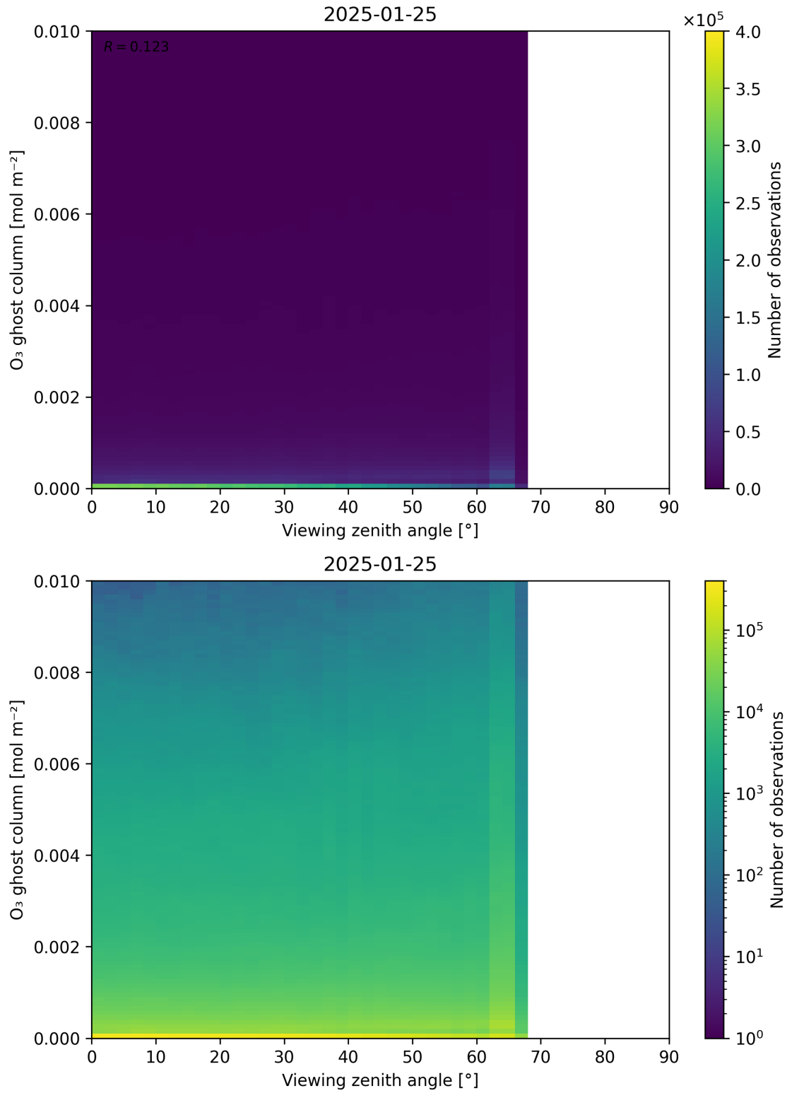
Figure 51: Scatter density plot of “Viewing zenith angle” against “O 3 ghost column” for 2025-01-24 to 2025-01-26.
