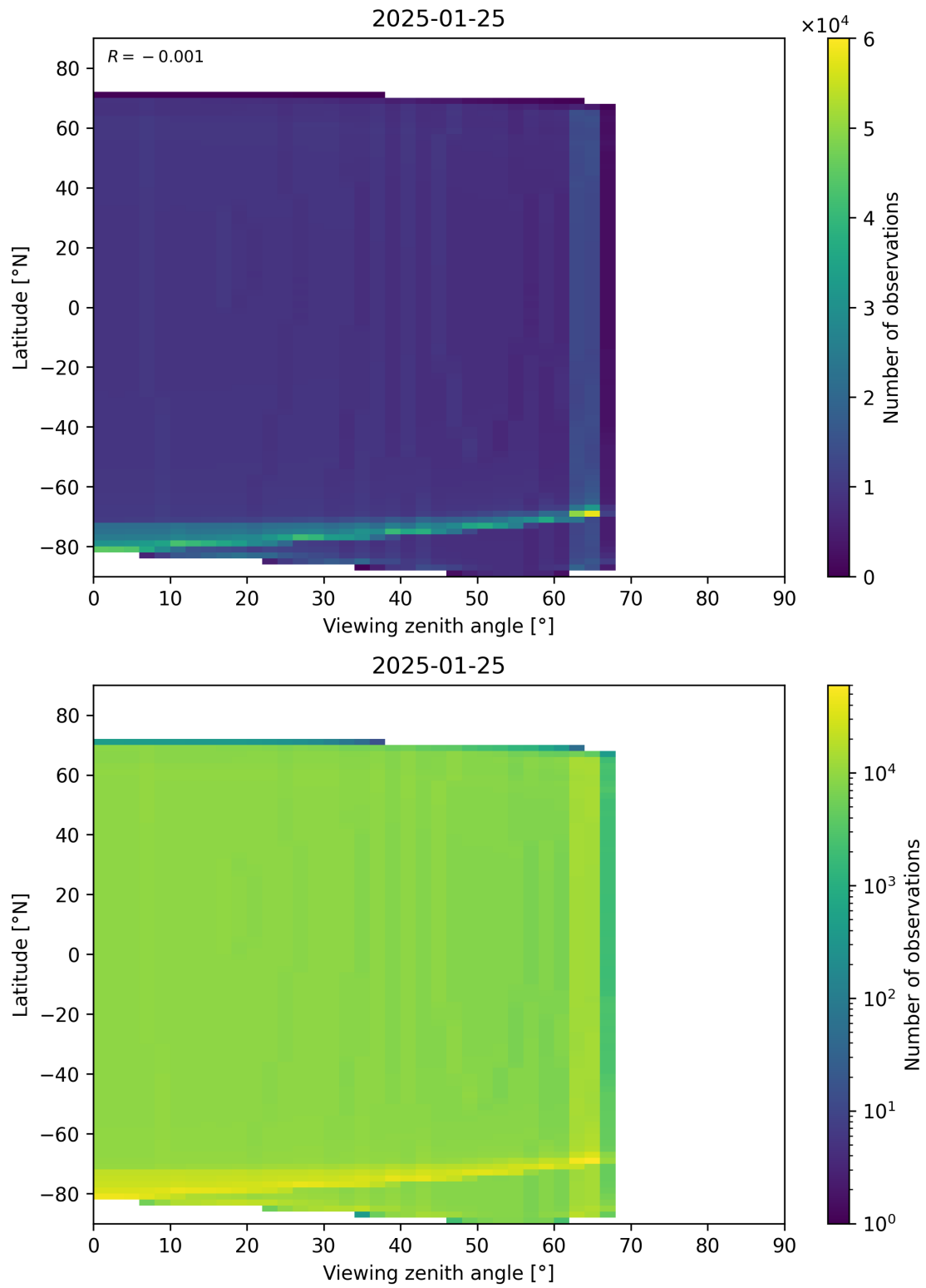
Figure 49: Scatter density plot of “Viewing zenith angle” against “Latitude” for 2025-01-24 to 2025-01-26.
