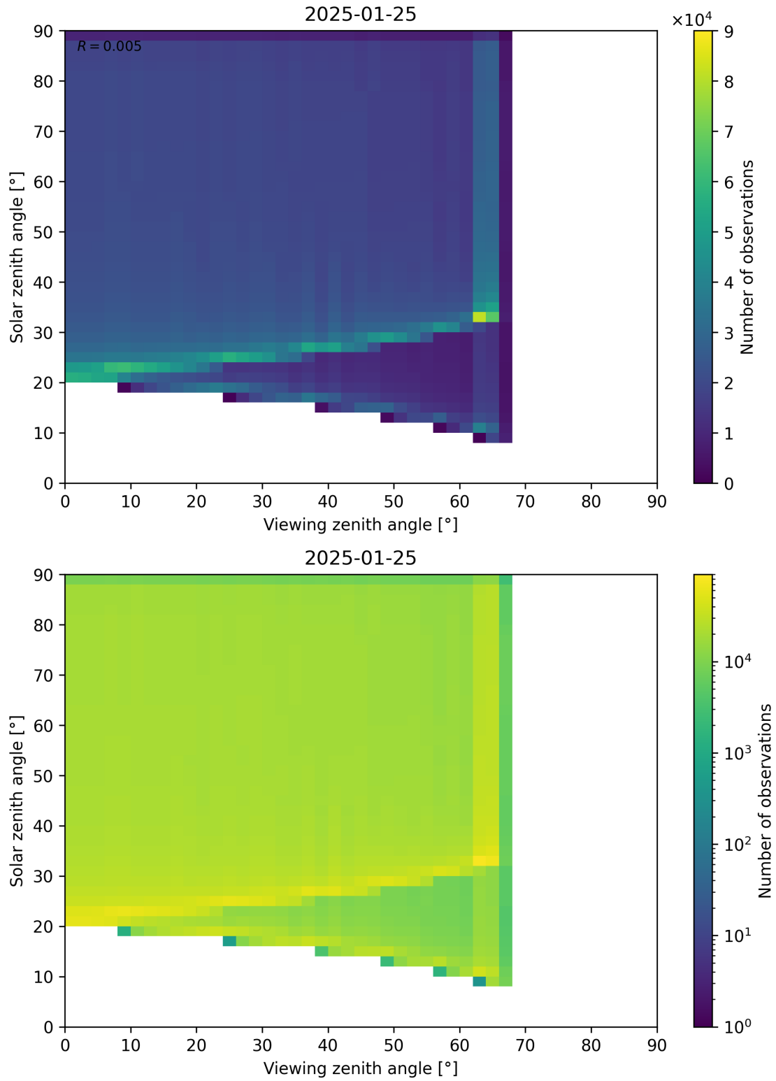
Figure 54: Scatter density plot of “Viewing zenith angle” against “Solar zenith angle” for 2025-01-24 to 2025-01-26.
