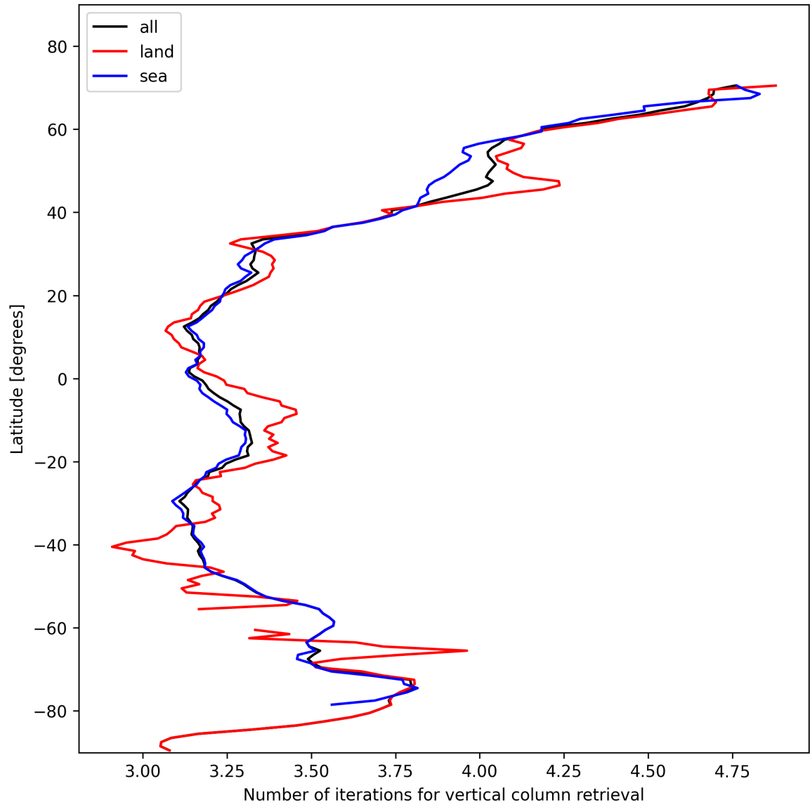
Figure 19: Zonal average of “Number of iterations for vertical column retrieval” for 2025-01-24 to 2025-01-26.
