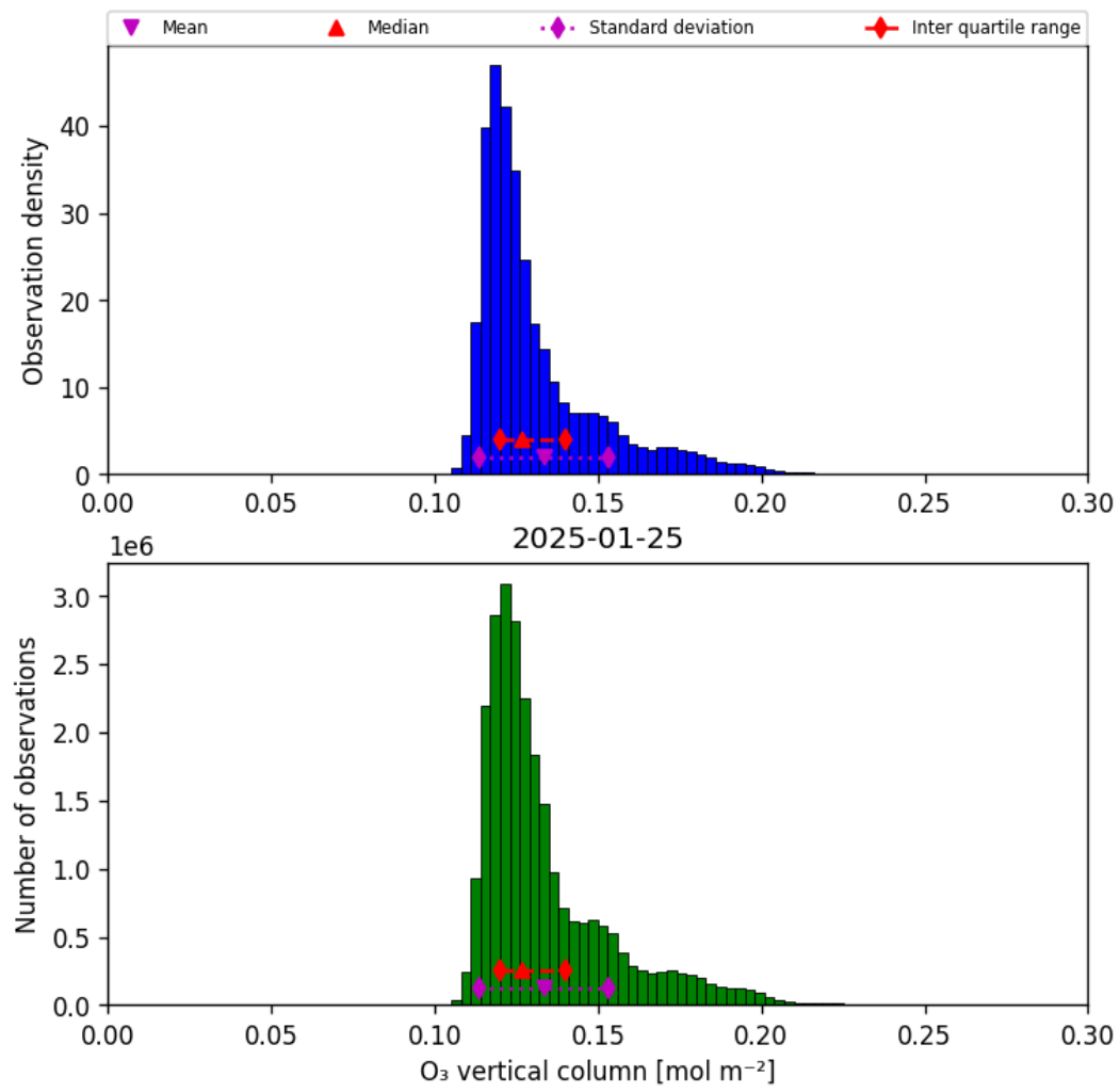
Figure 21: Histogram of “O 3 vertical column” for 2025-01-24 to 2025-01-26
