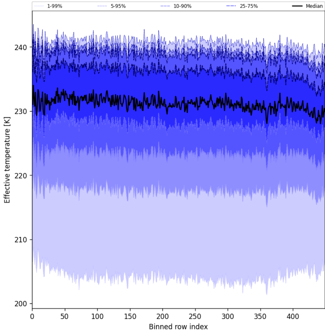
Figure 31: Along track statistics of “Effective temperature” for 2025-01-24 to 2025-01-26
