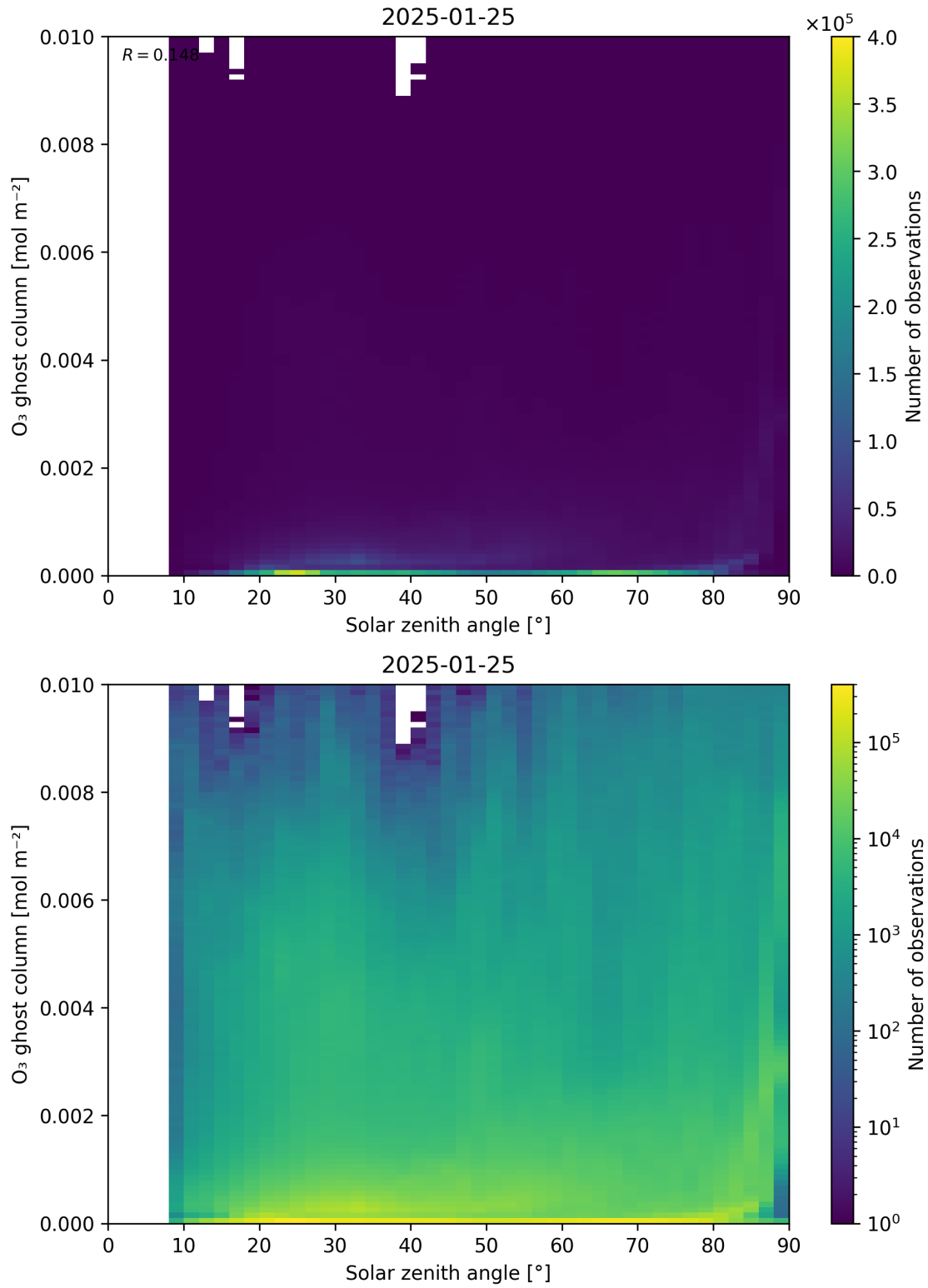
Figure 46: Scatter density plot of “Solar zenith angle” against “O 3 ghost column” for 2025-01-24 to 2025-01-26.
