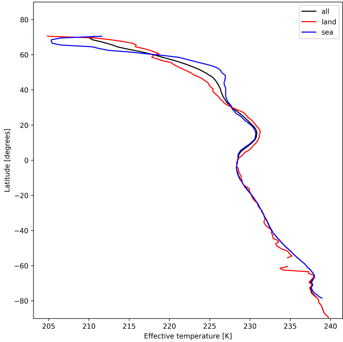
Figure 17: Zonal average of “Effective temperature” for 2025-01-24 to 2025-01-26.
