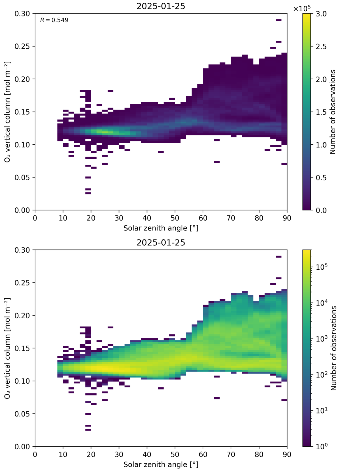
Figure 47: Scatter density plot of “Solar zenith angle” against “O 3 vertical column” for 2025-01-24 to 2025-01-26.
