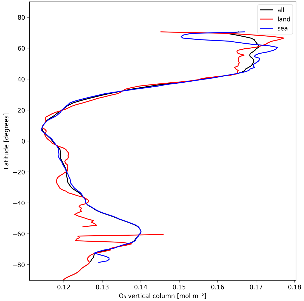
Figure 14: Zonal average of “O 3 vertical column” for 2025-01-24 to 2025-01-26.
