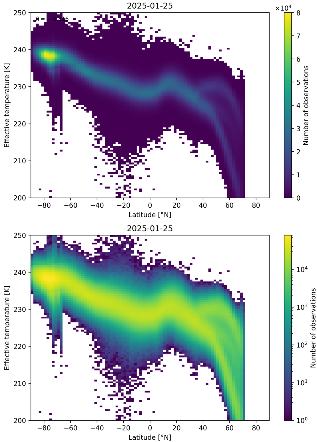
Figure 34: Scatter density plot of “Latitude” against “Effective temperature” for 2025-01-24 to 2025-01-26.
