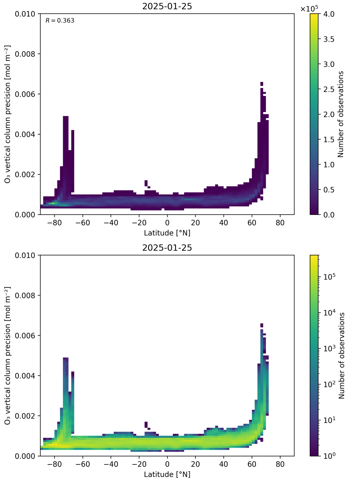
Figure 37: Scatter density plot of “Latitude” against “O 3 vertical column precision” for 2025-01-24 to 2025-01-26.
