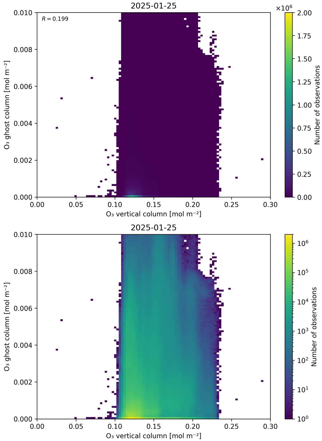
Figure 40: Scatter density plot of “O 3 vertical column” against “O 3 ghost column” for 2025-01-24 to 2025-01-26.
