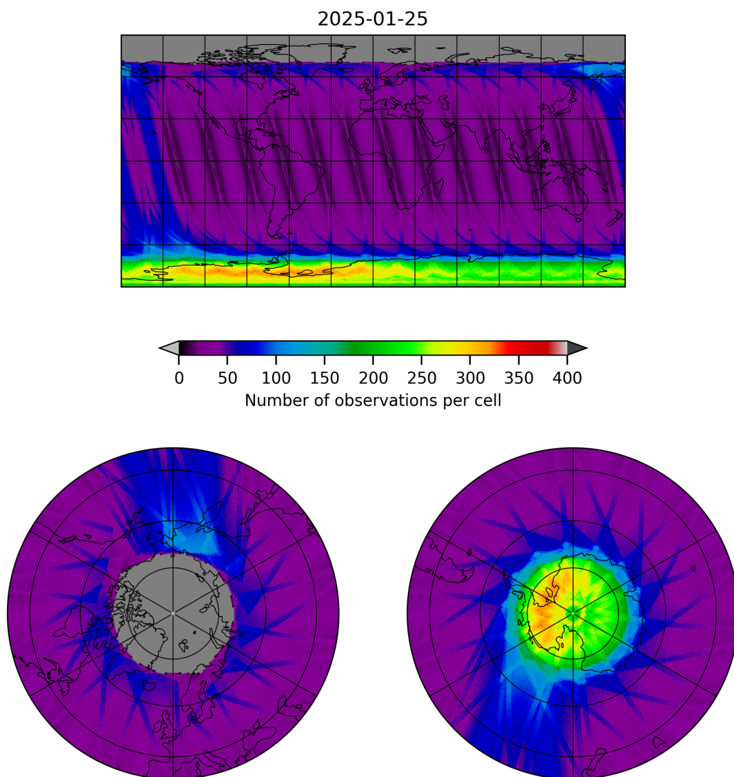
Figure 12: Map of the number of observations for 2025-01-24 to 2025-01-26
