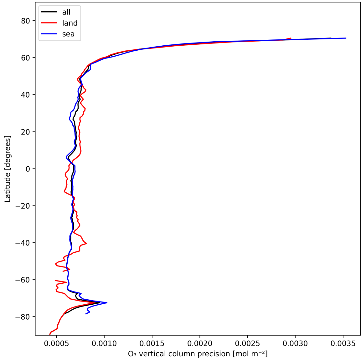
Figure 15: Zonal average of “O 3 vertical column precision” for 2025-01-24 to 2025-01-26.
