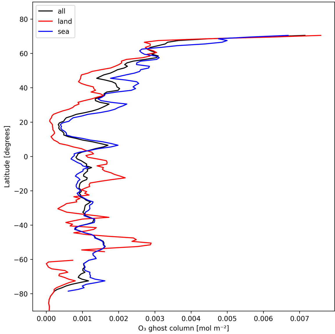
Figure 18: Zonal average of “O 3 ghost column” for 2025-01-24 to 2025-01-26.
