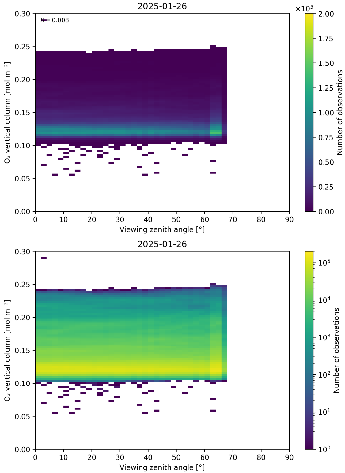
Figure 52: Scatter density plot of “Viewing zenith angle” against “O 3 vertical column” for 2025-01-25 to 2025-01-27.
