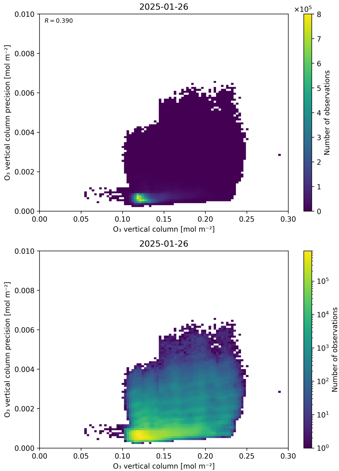
Figure 41: Scatter density plot of “O 3 vertical column” against “O 3 vertical column precision” for 2025-01-25 to 2025-01-27.
