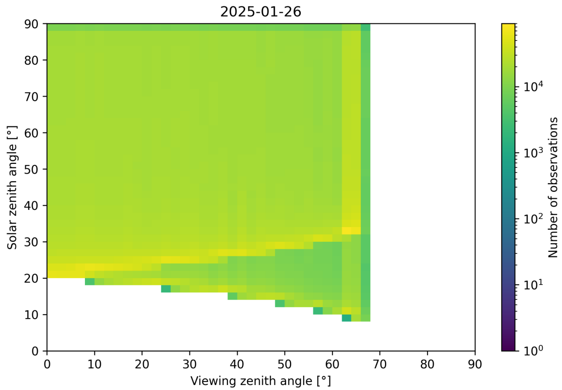
Figure 54: Scatter density plot of “Viewing zenith angle” against “Solar zenith angle” for 2025-01-25 to 2025-01-27.
