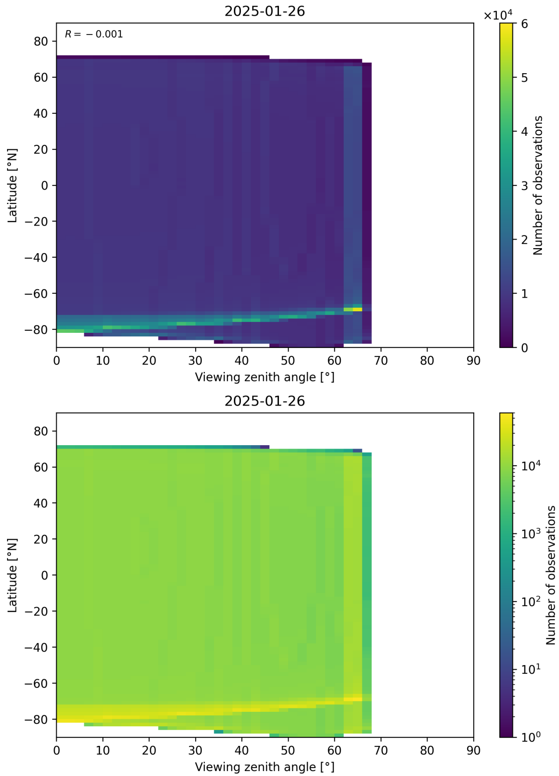
Figure 49: Scatter density plot of “Viewing zenith angle” against “Latitude” for 2025-01-25 to 2025-01-27.
