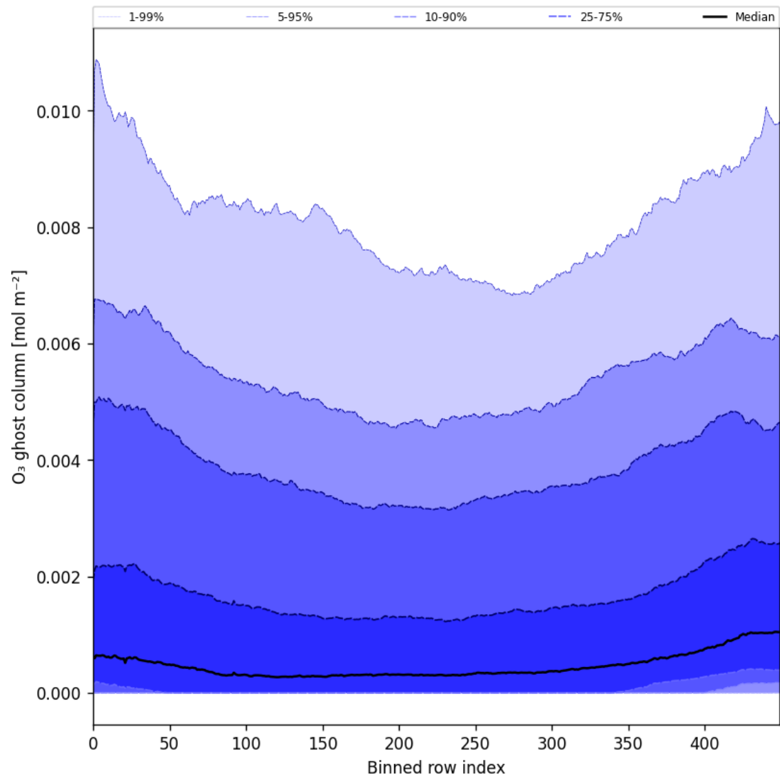
Figure 32: Along track statistics of “O 3 ghost column” for 2025-01-25 to 2025-01-27
