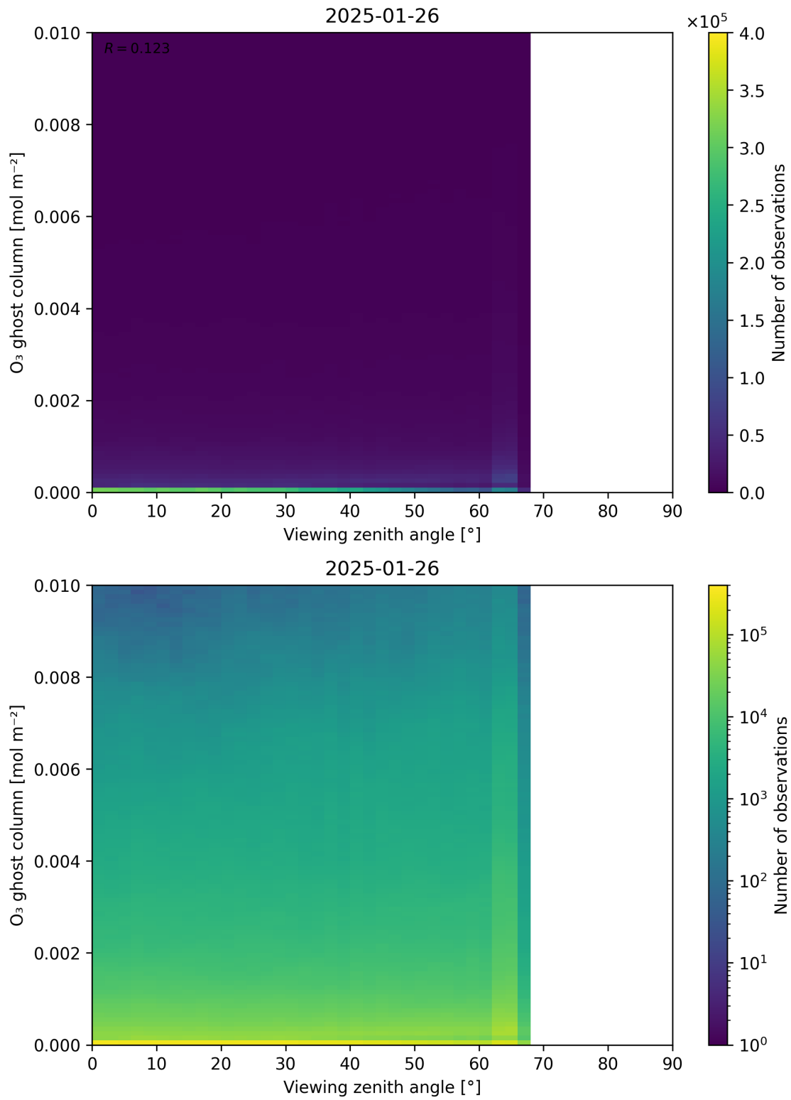
Figure 51: Scatter density plot of “Viewing zenith angle” against “O 3 ghost column” for 2025-01-25 to 2025-01-27.
