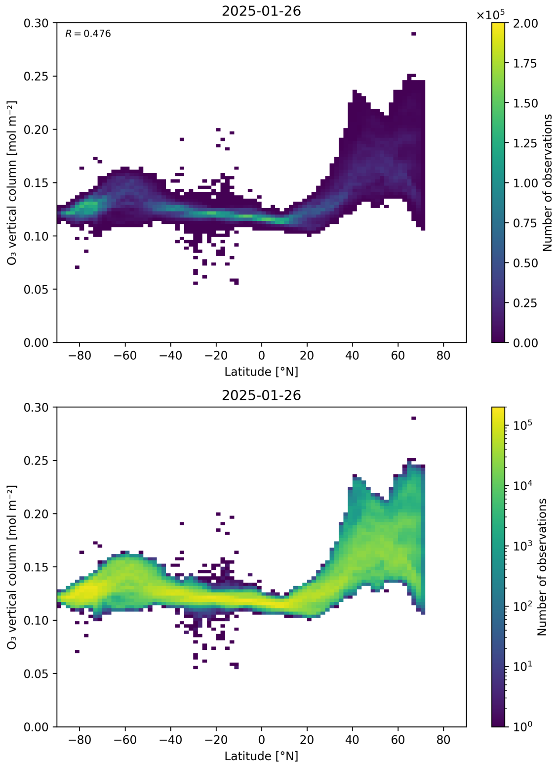
Figure 36: Scatter density plot of “Latitude” against “O 3 vertical column” for 2025-01-25 to 2025-01-27.
