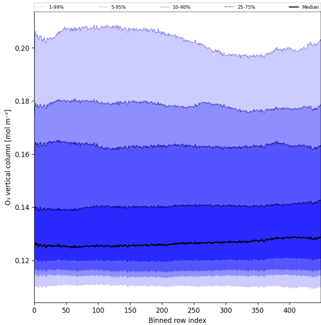
Figure 28: Along track statistics of “O 3 vertical column” for 2025-01-25 to 2025-01-27
