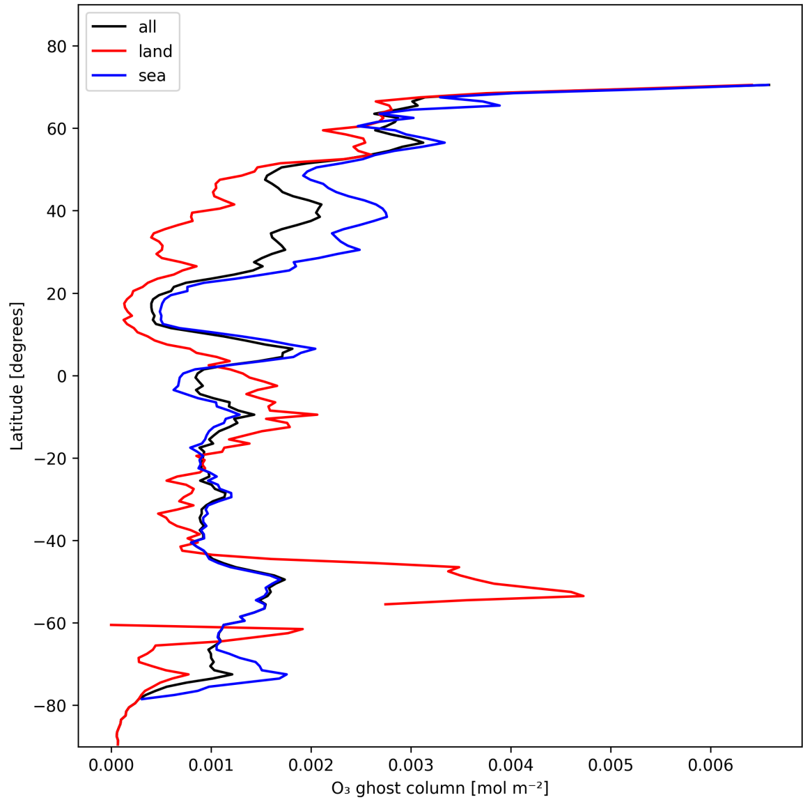
Figure 18: Zonal average of "O 3 ghost column" for 2025-01-25 to 2025-01-27.
