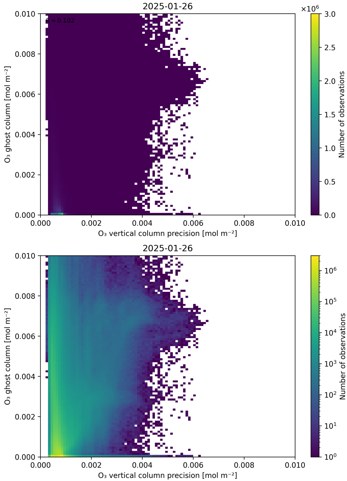
Figure 43: Scatter density plot of “O 3 vertical column precision” against “O 3 ghost column” for 2025-01-25 to 2025-01-27.
