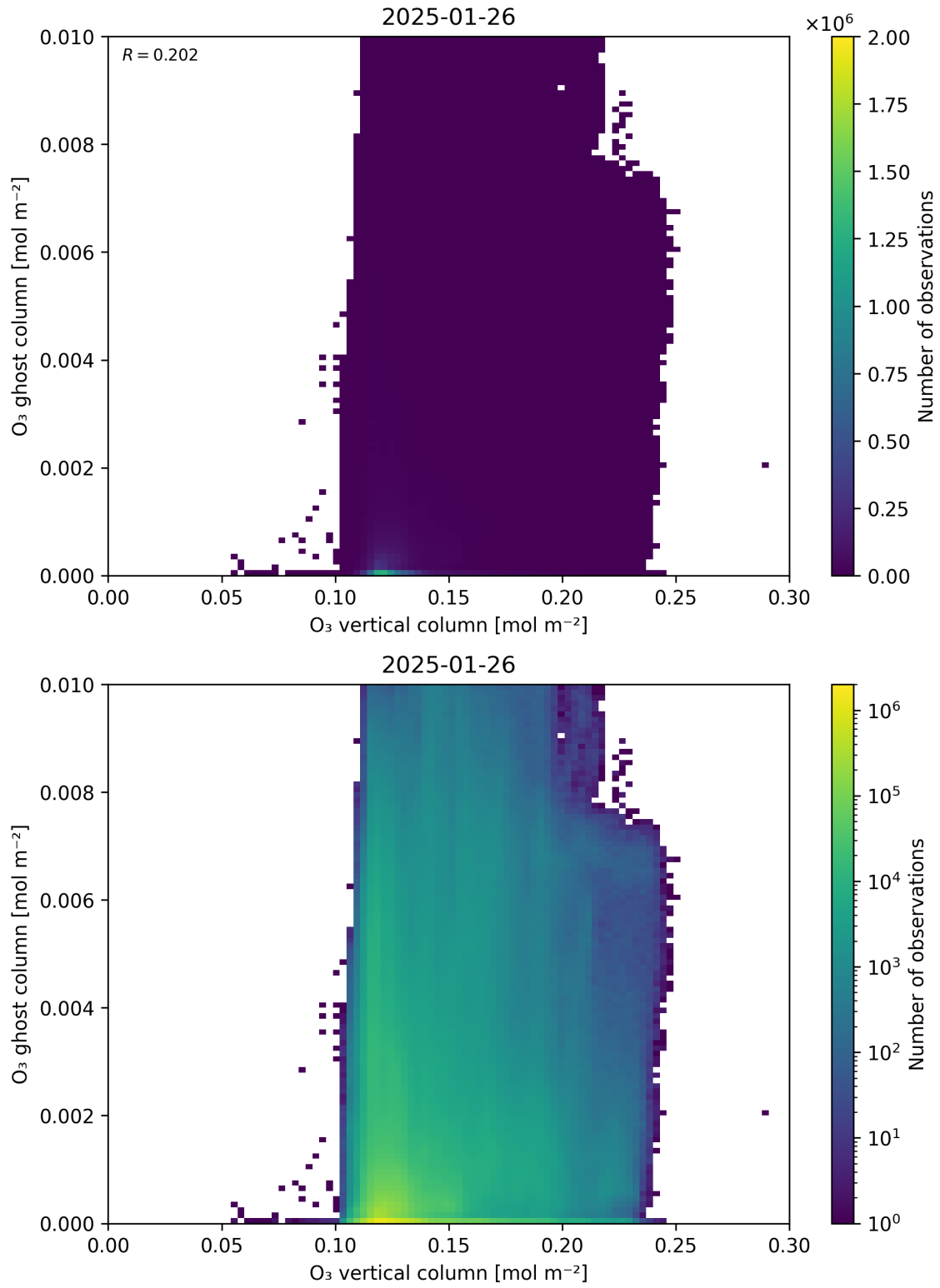
Figure 40: Scatter density plot of “O 3 vertical column” against “O 3 ghost column” for 2025-01-25 to 2025-01-27.
