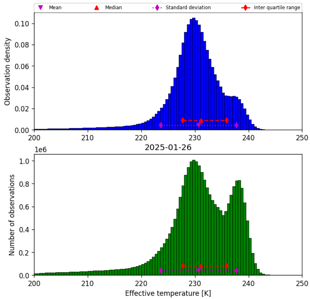
Figure 24: Histogram of “Effective temperature” for 2025-01-25 to 2025-01-27
