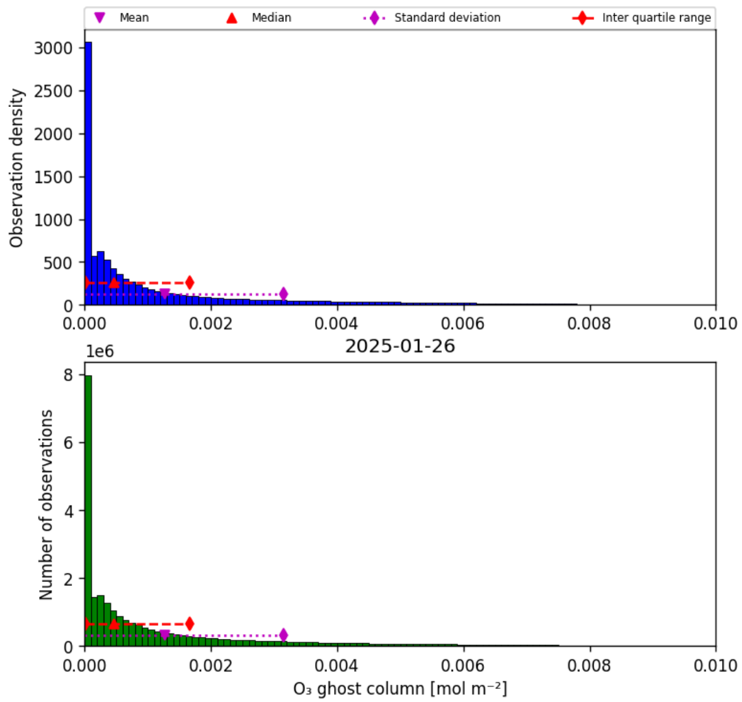
Figure 25: Histogram of “O 3 ghost column” for 2025-01-25 to 2025-01-27
