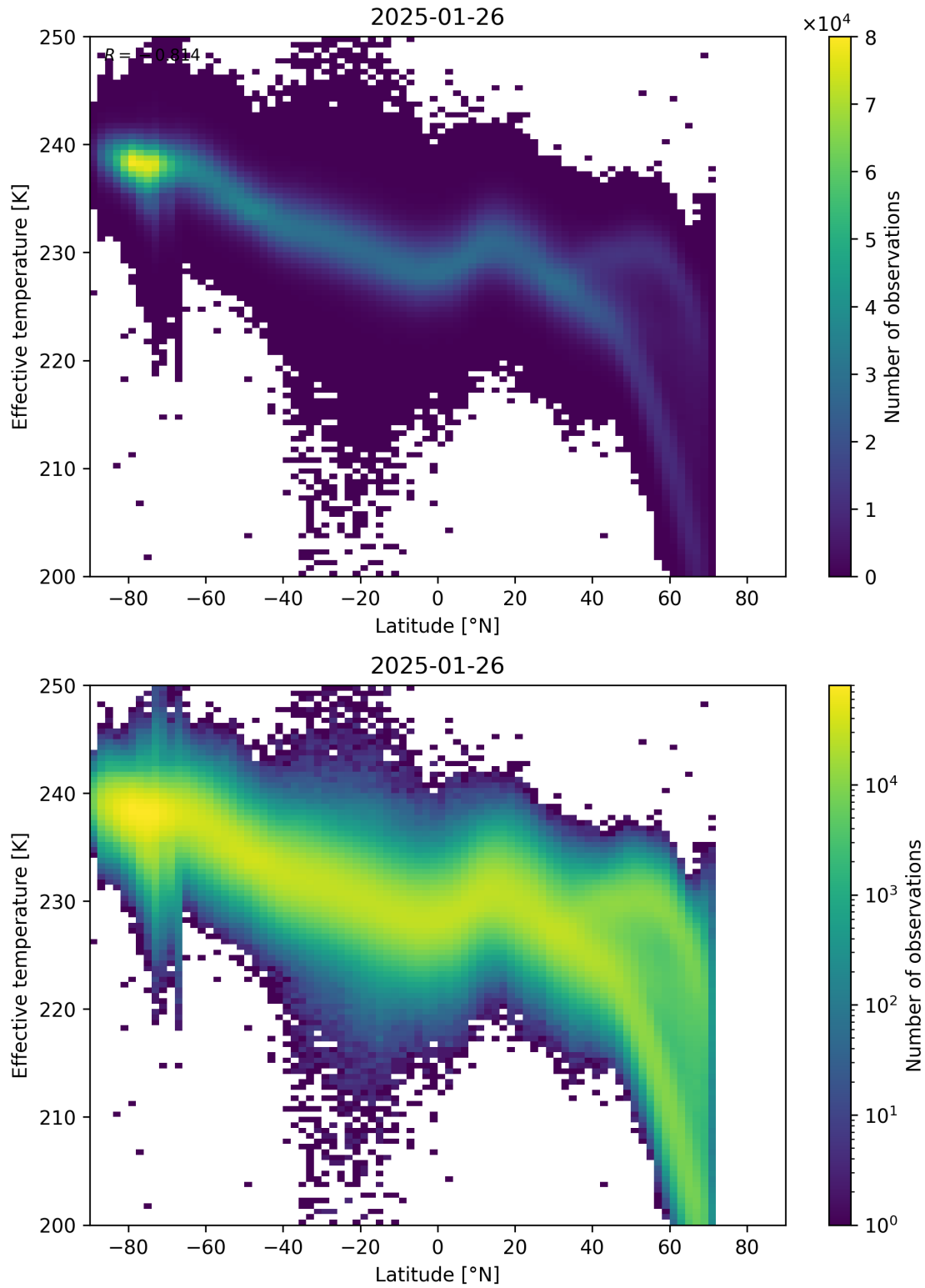
Figure 34: Scatter density plot of “Latitude” against “Effective temperature” for 2025-01-25 to 2025-01-27.
