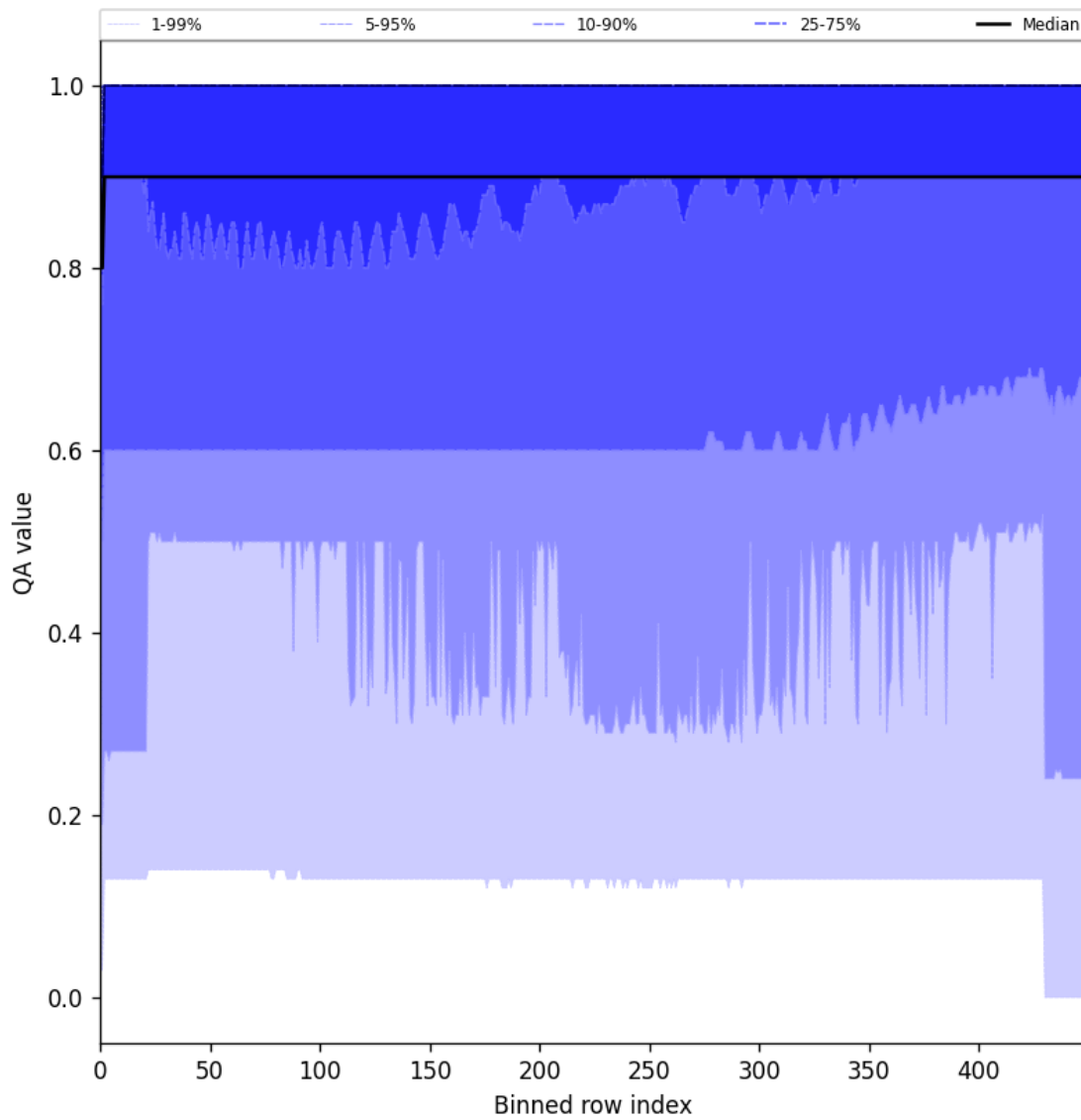
Figure 27: Along track statistics of “QA value” for 2025-01-25 to 2025-01-27
