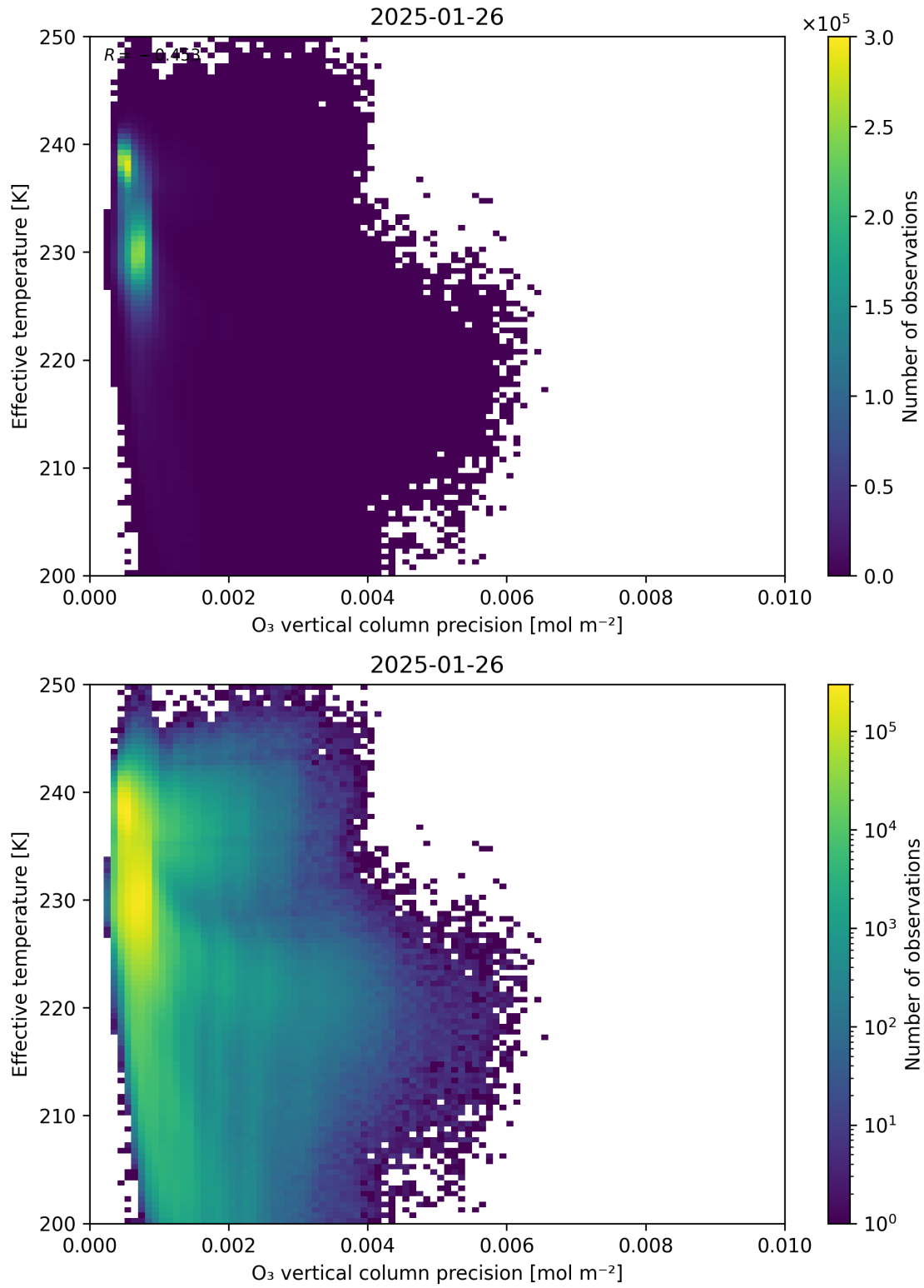
Figure 42: Scatter density plot of “O 3 vertical column precision” against “Effective temperature” for 2025-01-25 to 2025-01-27.
