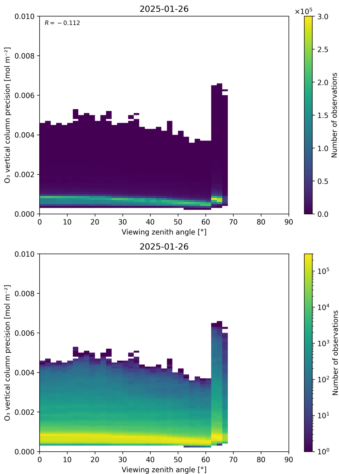
Figure 53: Scatter density plot of “Viewing zenith angle” against “O 3 vertical column precision” for 2025-01-25 to 2025-01-27.
