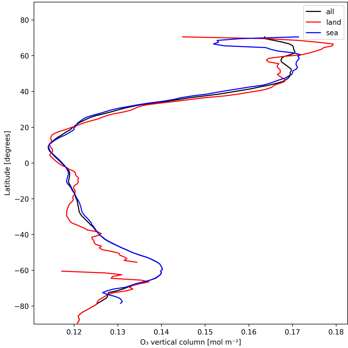
Figure 14: Zonal average of “O 3 vertical column” for 2025-01-25 to 2025-01-27.
