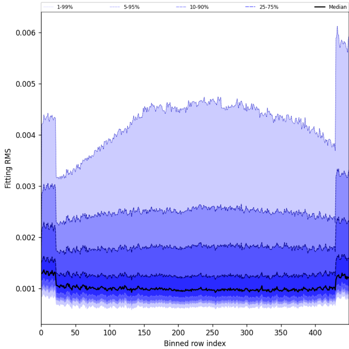
Figure 30: Along track statistics of “Fitting RMS” for 2025-01-25 to 2025-01-27
