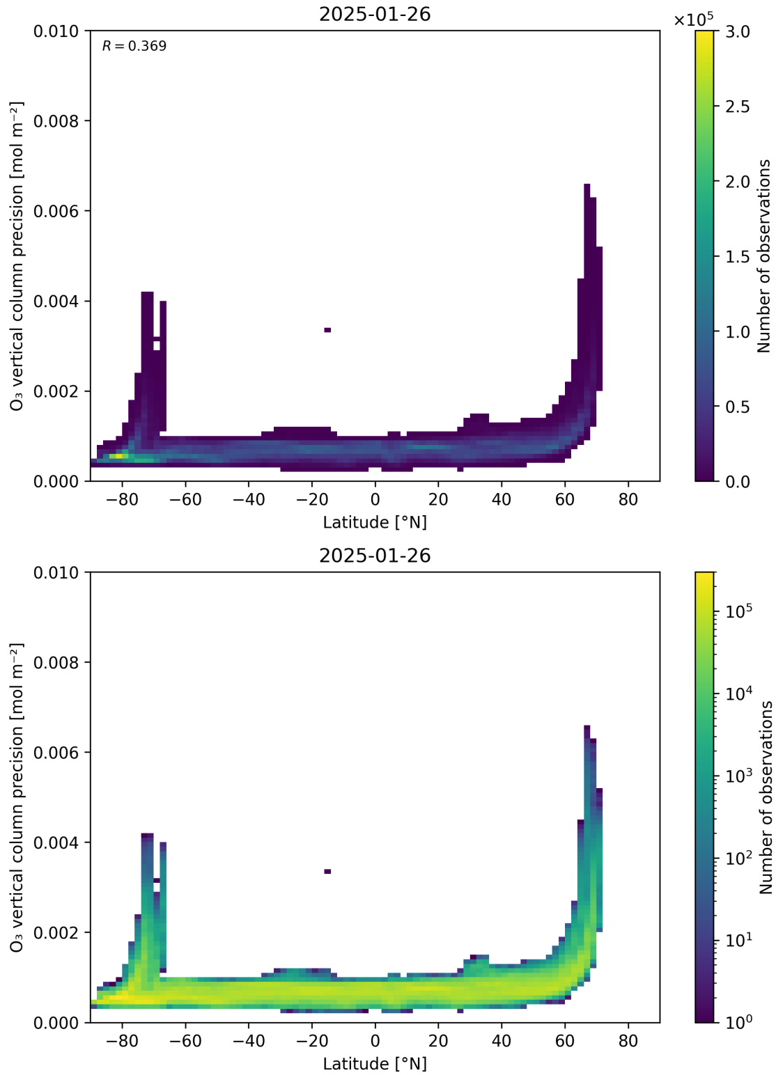
Figure 37: Scatter density plot of “Latitude” against “O 3 vertical column precision” for 2025-01-25 to 2025-01-27.
