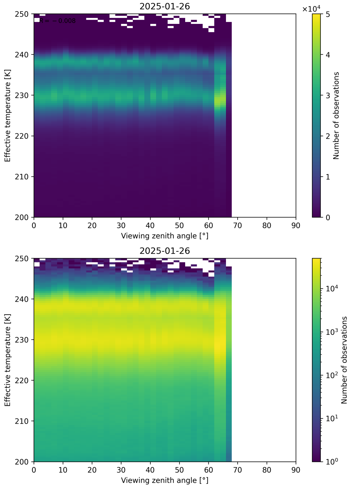
Figure 50: Scatter density plot of “Viewing zenith angle” against “Effective temperature” for 2025-01-25 to 2025-01-27.
