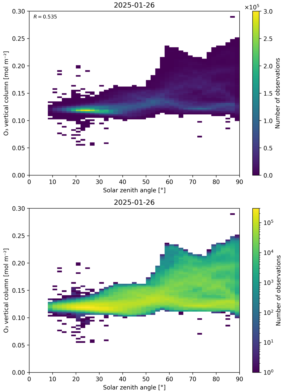
Figure 47: Scatter density plot of “Solar zenith angle” against “O 3 vertical column” for 2025-01-25 to 2025-01-27.
