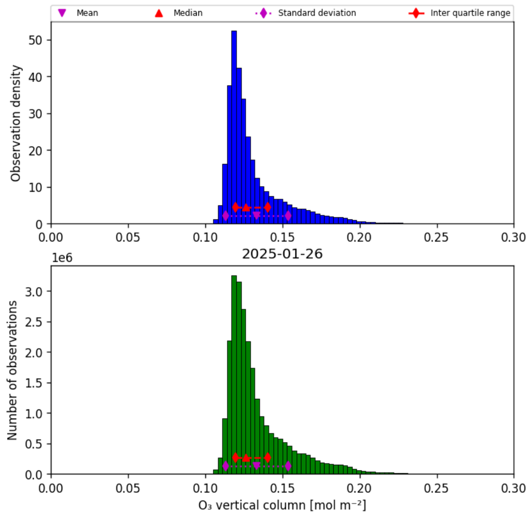
Figure 21: Histogram of “O 3 vertical column” for 2025-01-25 to 2025-01-27
