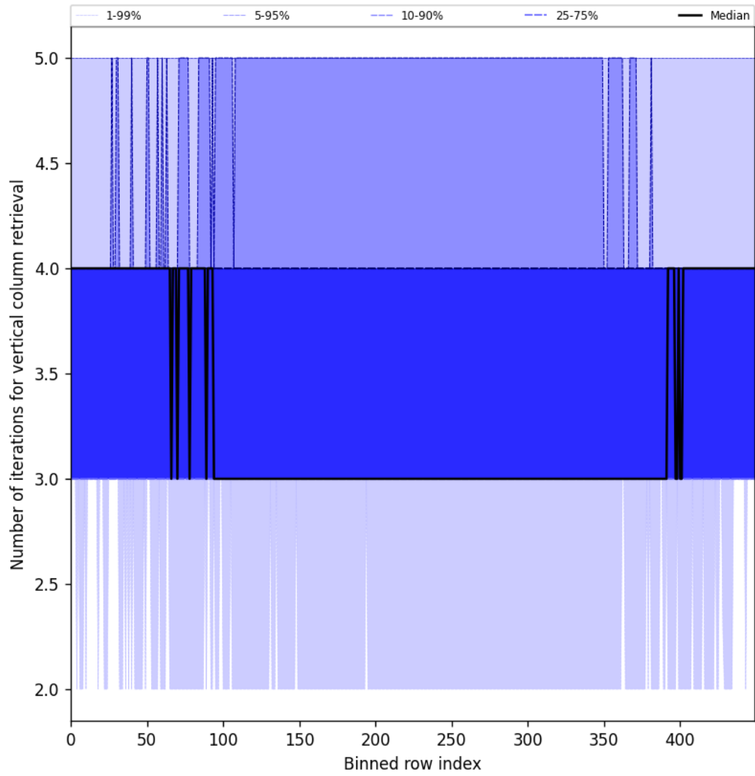
Figure 33: Along track statistics of “Number of iterations for vertical column retrieval” for 2025-01-25 to 2025-01-27
