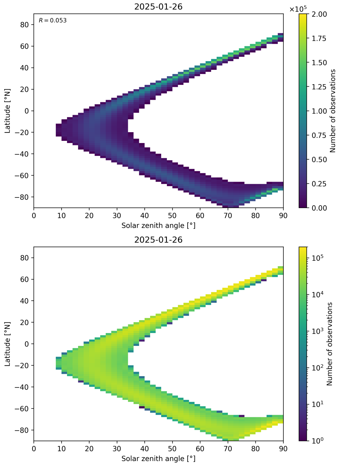
Figure 44: Scatter density plot of “Solar zenith angle” against “Latitude” for 2025-01-25 to 2025-01-27.
