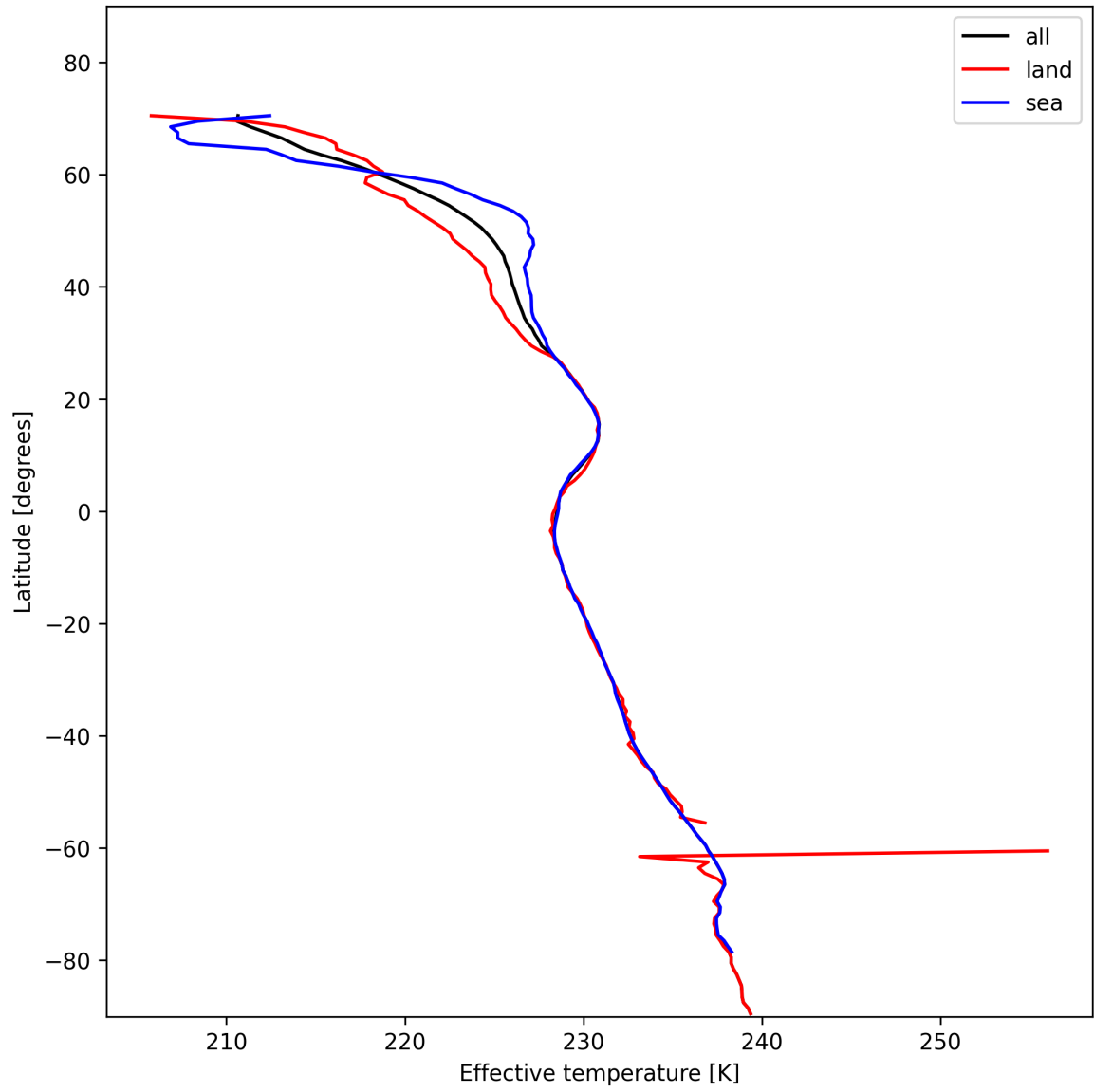
Figure 17: Zonal average of “Effective temperature” for 2025-01-25 to 2025-01-27.
