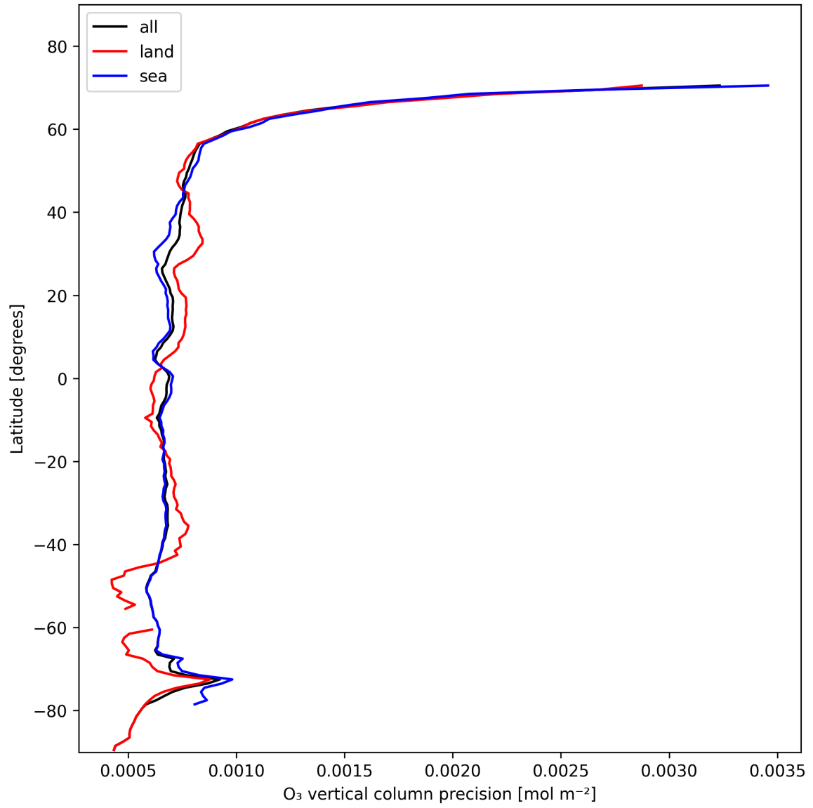
Figure 15: Zonal average of “O 3 vertical column precision” for 2025-01-25 to 2025-01-27.
