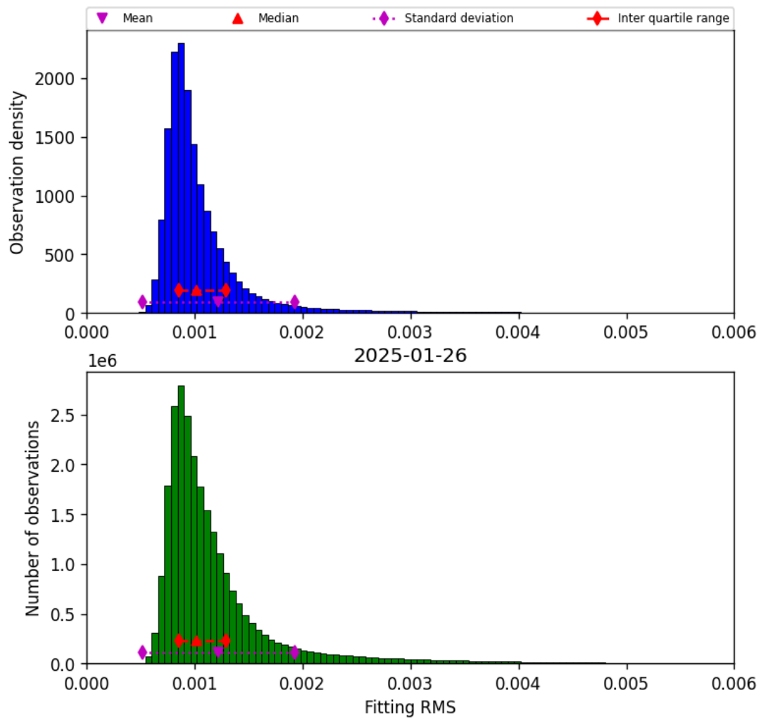
Figure 23: Histogram of “Fitting RMS” for 2025-01-25 to 2025-01-27
