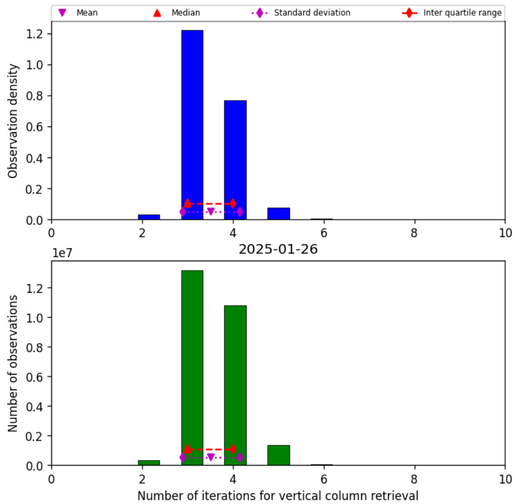
Figure 26: Histogram of “Number of iterations for vertical column retrieval” for 2025-01-25 to 2025-01-27
