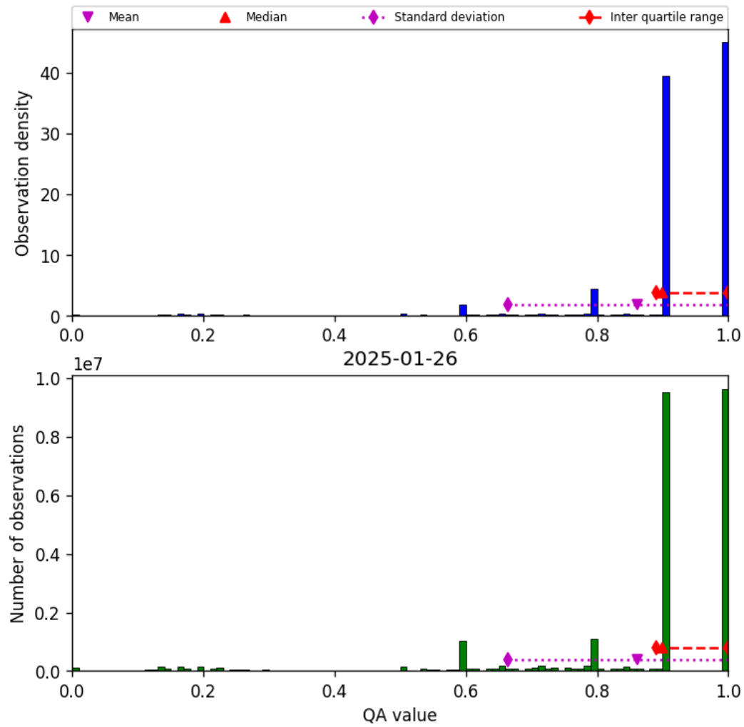
Figure 20: Histogram of “QA value” for 2025-01-25 to 2025-01-27
