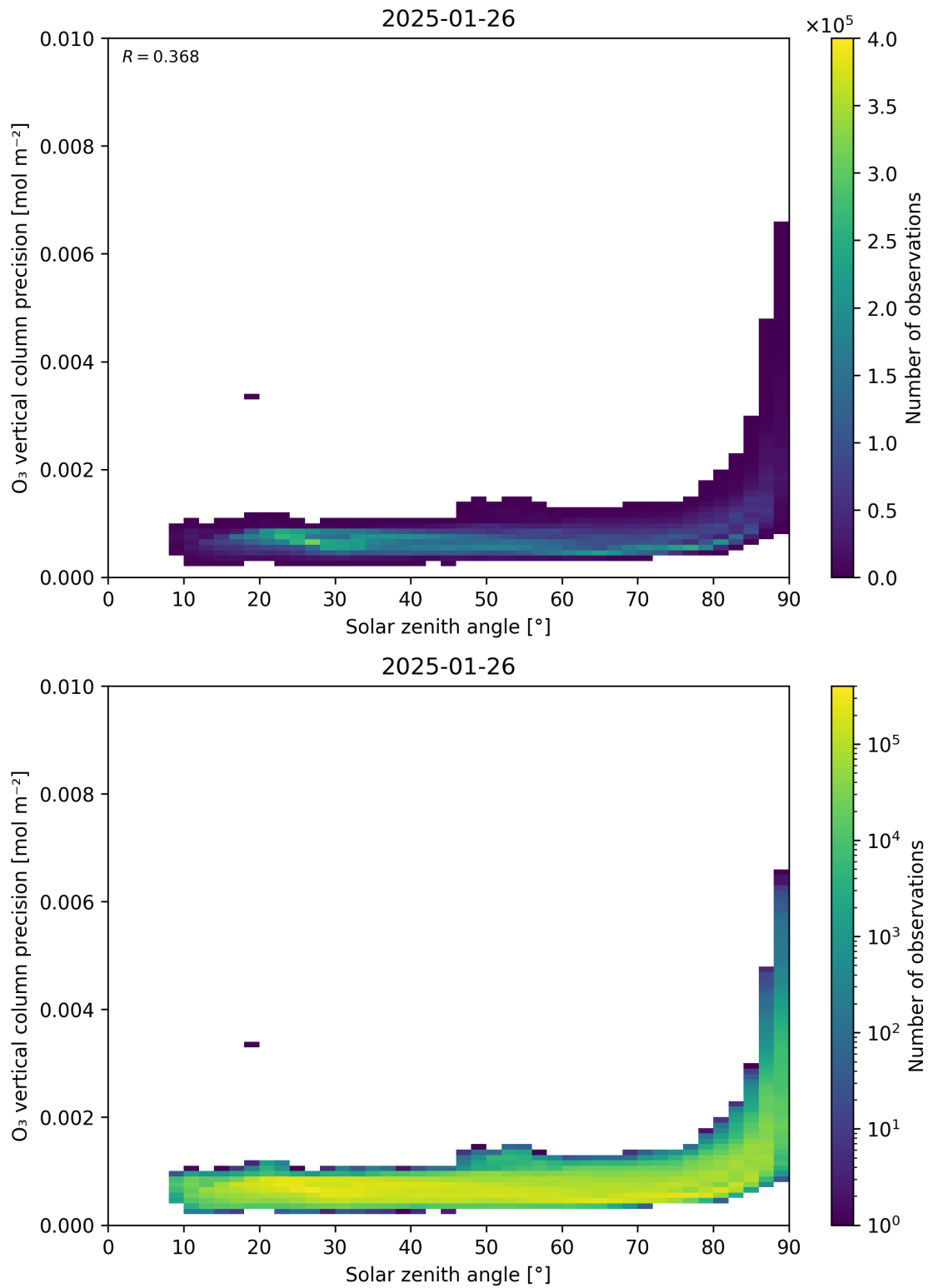
Figure 48: Scatter density plot of “Solar zenith angle” against “O 3 vertical column precision” for 2025-01-25 to 2025-01-27.
