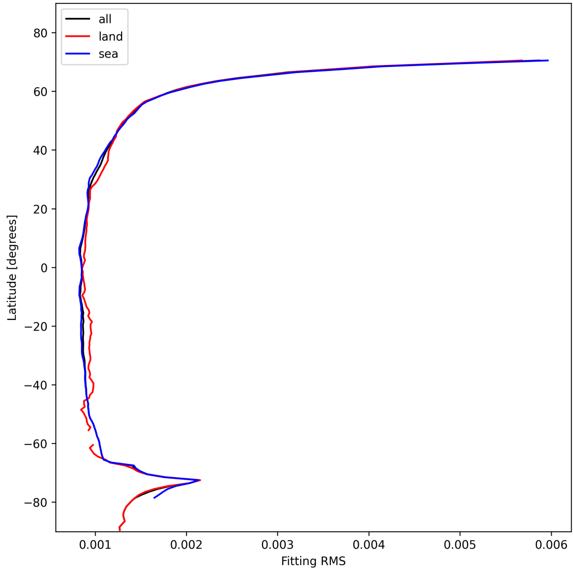
Figure 16: Zonal average of “Fitting RMS” for 2025-01-25 to 2025-01-27.
