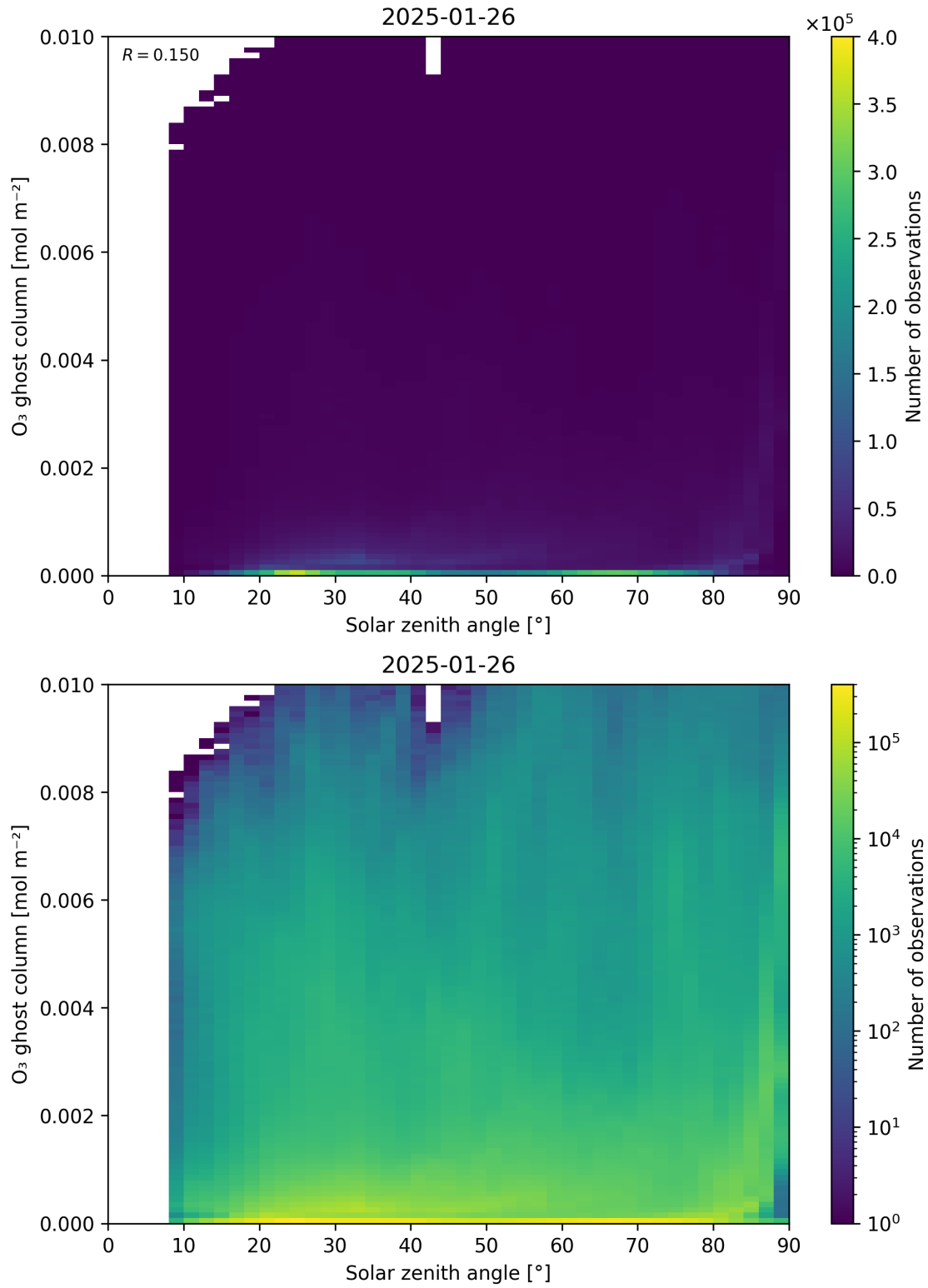
Figure 46: Scatter density plot of “Solar zenith angle” against “O 3 ghost column” for 2025-01-25 to 2025-01-27.
