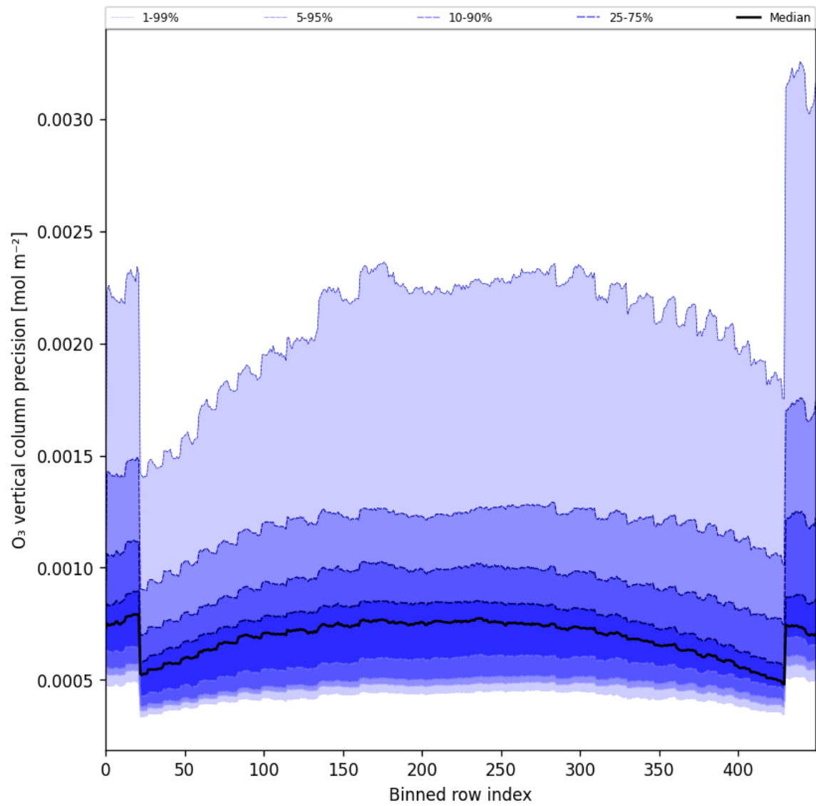
Figure 29: Along track statistics of “O 3 vertical column precision” for 2025-01-25 to 2025-01-27
