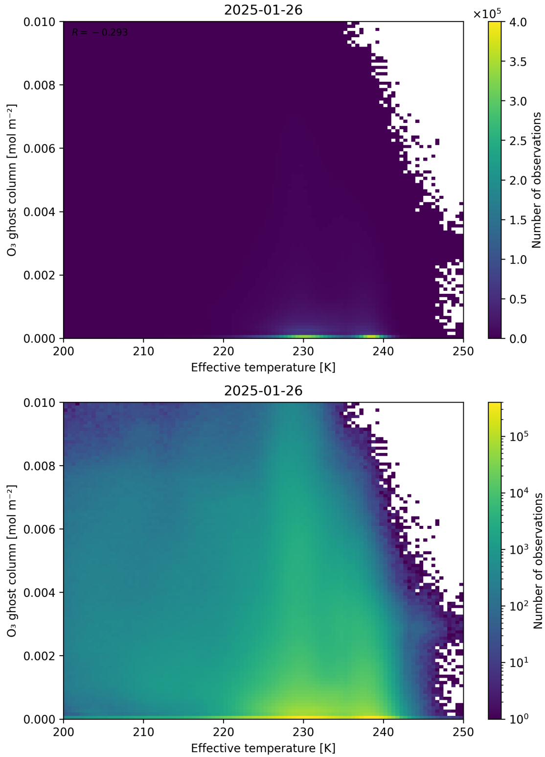
Figure 38: Scatter density plot of “Effective temperature” against “O 3 ghost column” for 2025-01-25 to 2025-01-27.
