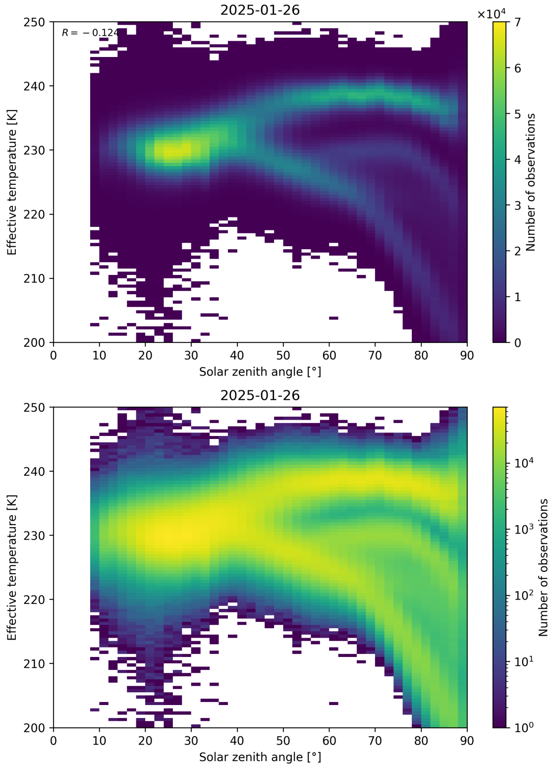
Figure 45: Scatter density plot of “Solar zenith angle” against “Effective temperature” for 2025-01-25 to 2025-01-27.
