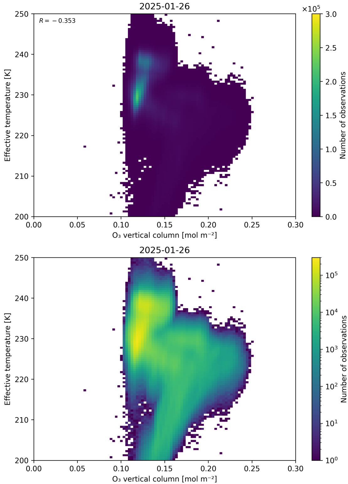
Figure 39: Scatter density plot of “O 3 vertical column” against “Effective temperature” for 2025-01-25 to 2025-01-27.
