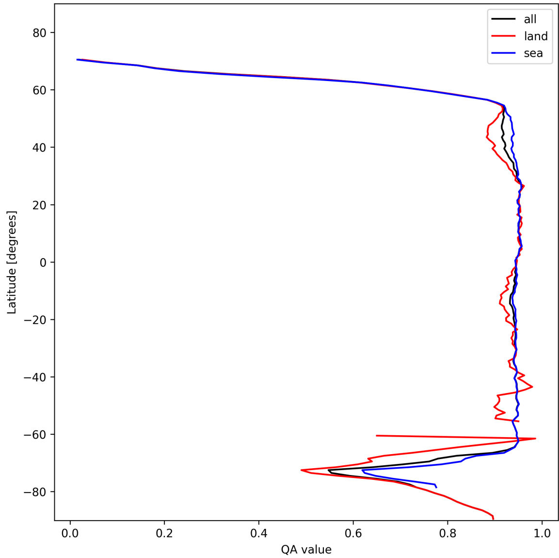
Figure 13: Zonal average of “QA value” for 2025-01-25 to 2025-01-27.
