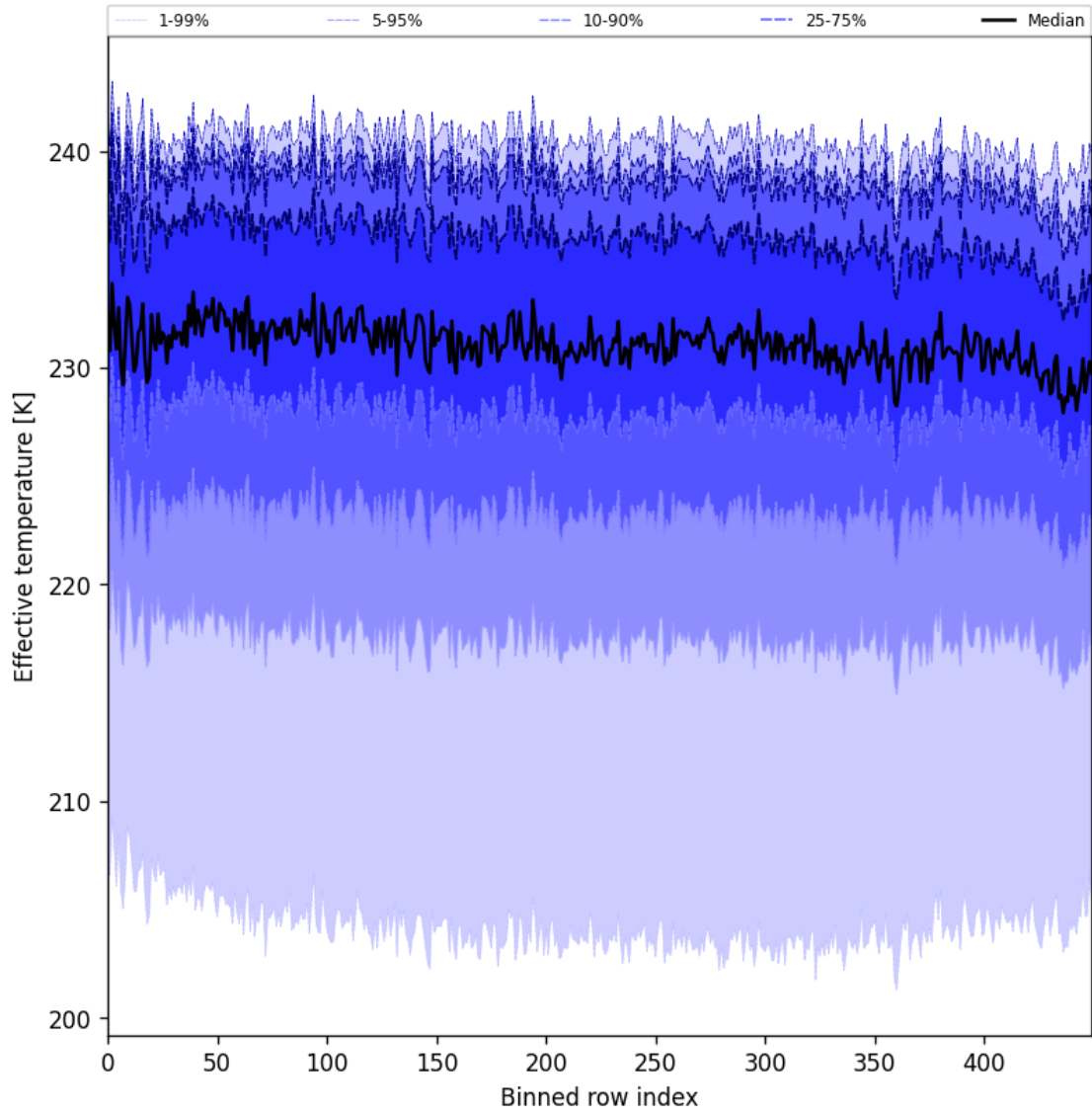
Figure 31: Along track statistics of "Effective temperature" for 2025-01-25 to 2025-01-27
