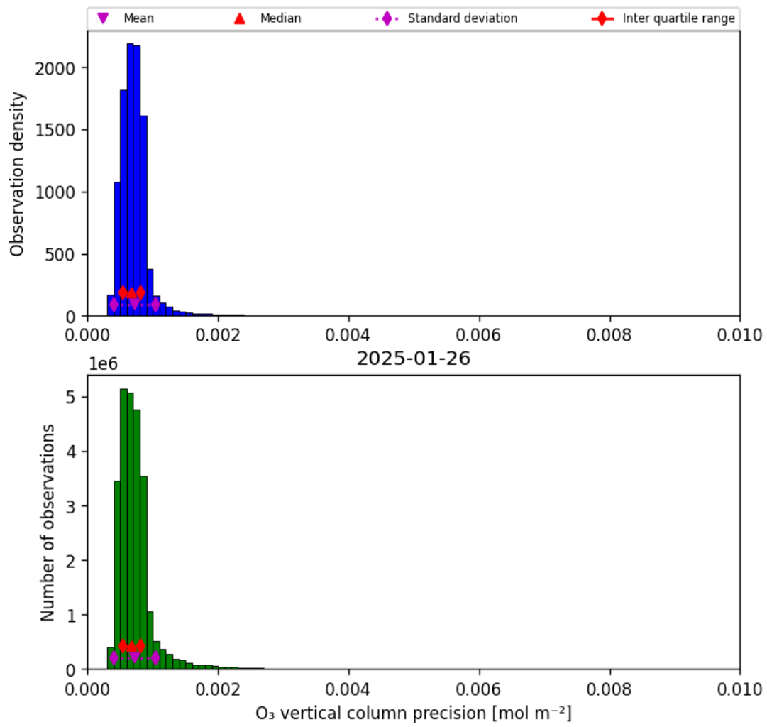
Figure 22: Histogram of “O 3 vertical column precision” for 2025-01-25 to 2025-01-27
