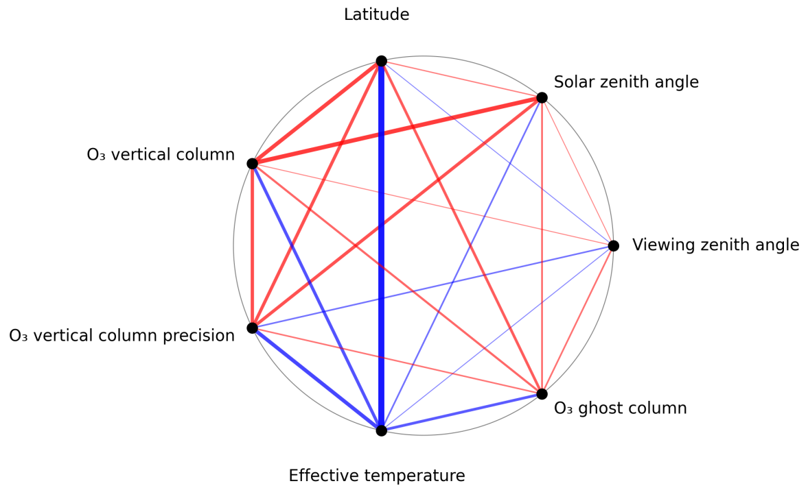
Figure 1: Map of correlation graph for 2025-01-25 to 2025-01-27.
