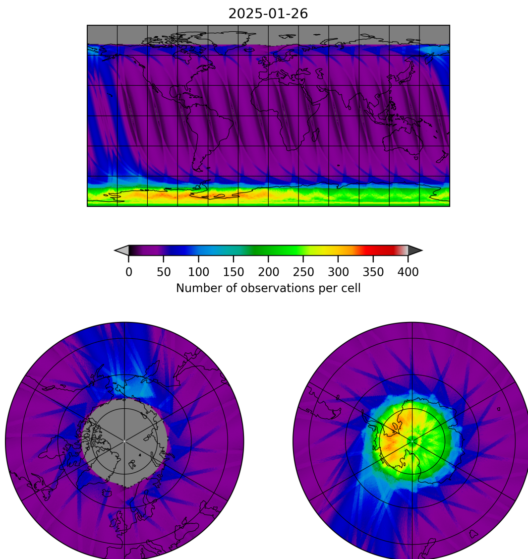
Figure 12: Map of the number of observations for 2025-01-25 to 2025-01-27
