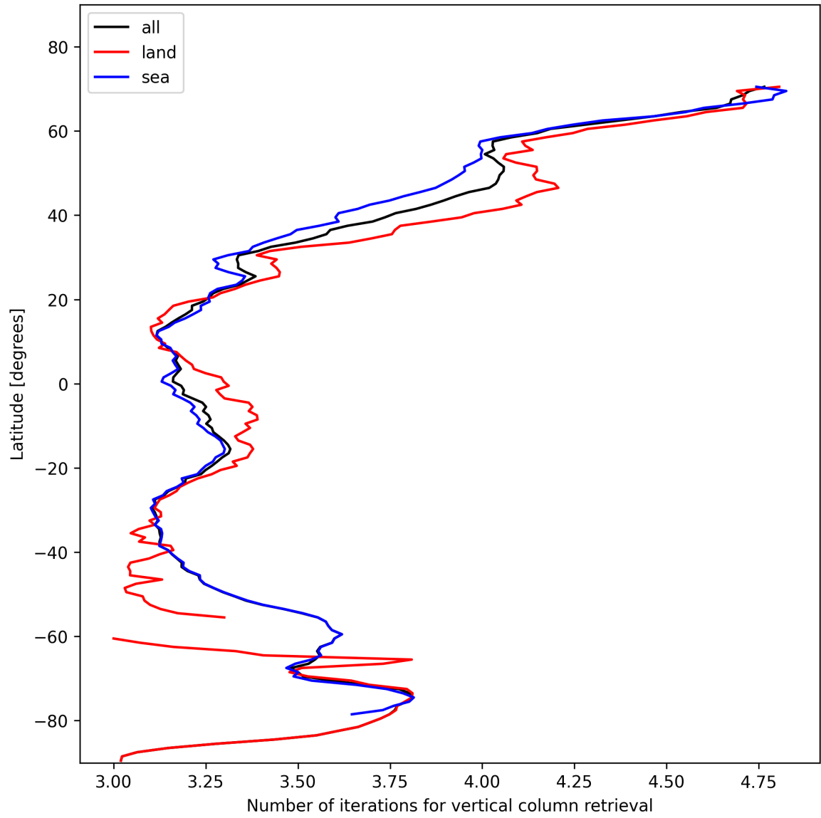
Figure 19: Zonal average of “Number of iterations for vertical column retrieval” for 2025-01-25 to 2025-01-27.
