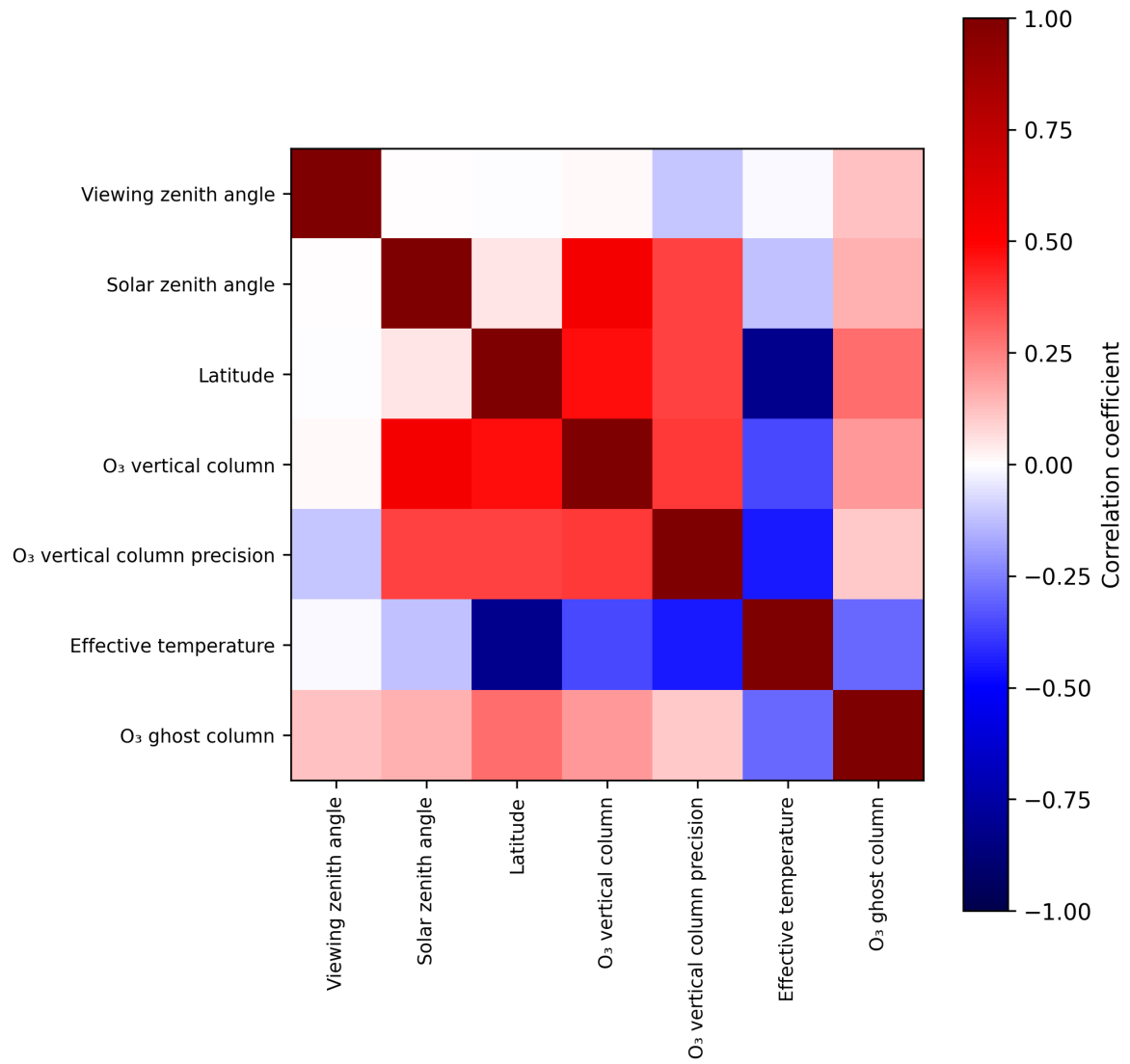
Figure 2: Map of correlation matrix for 2025-01-25 to 2025-01-27.
