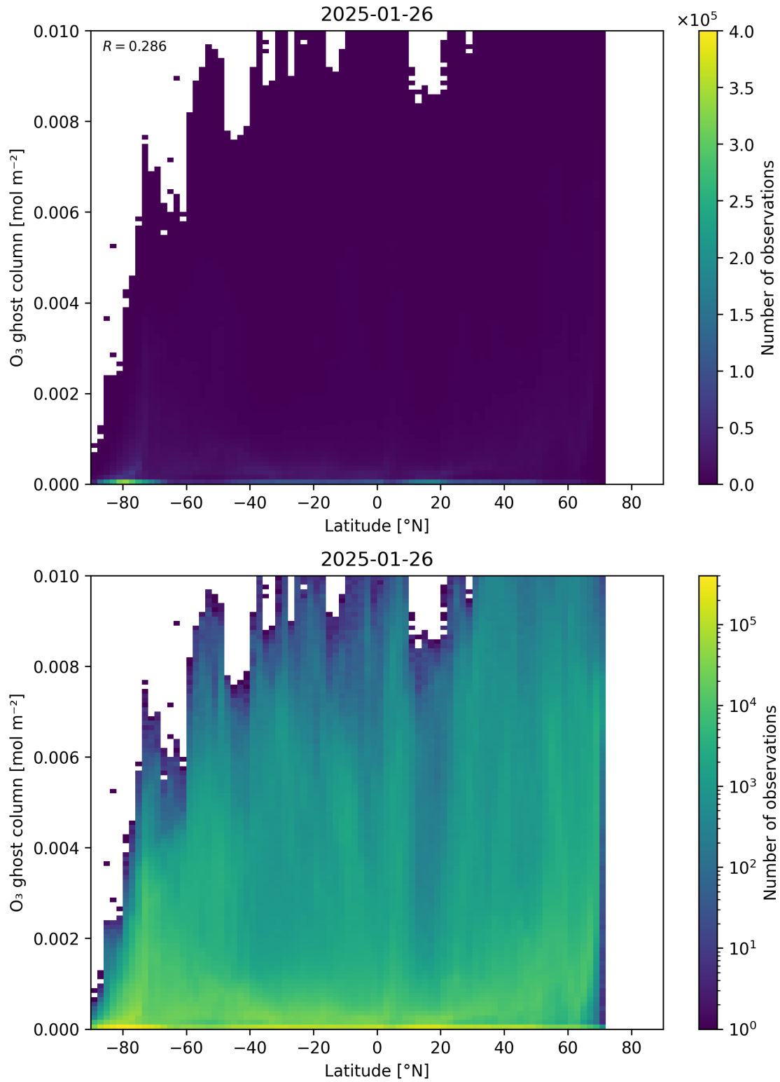
Figure 35: Scatter density plot of “Latitude” against “O 3 ghost column” for 2025-01-25 to 2025-01-27.
