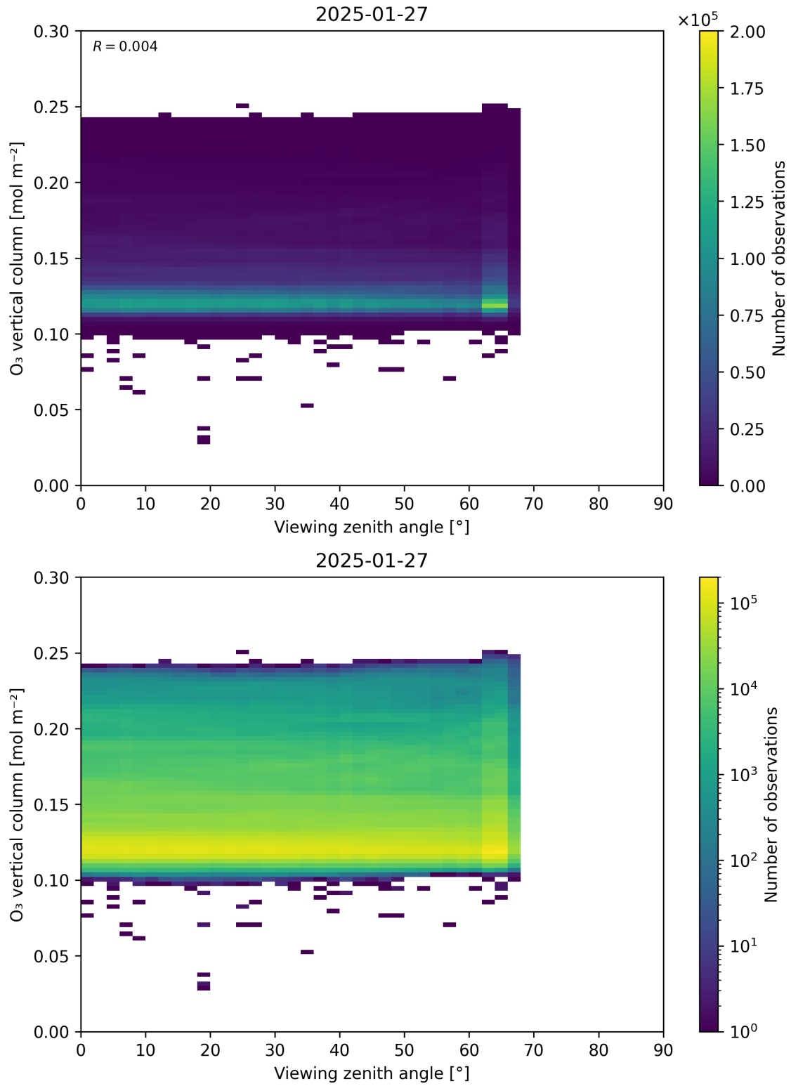
Figure 52: Scatter density plot of “Viewing zenith angle” against “O 3 vertical column” for 2025-01-26 to 2025-01-28.
