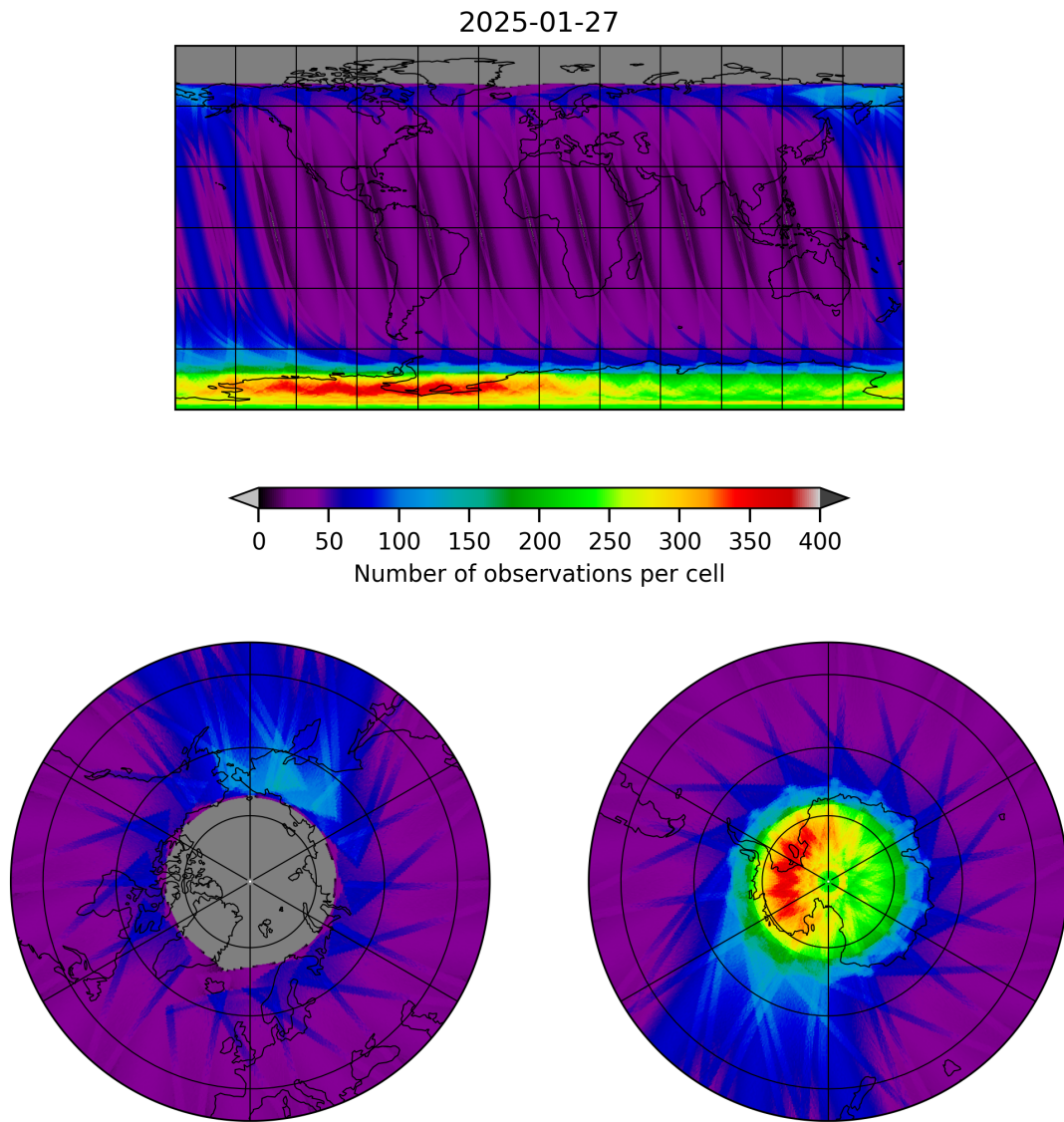
Figure 12: Map of the number of observations for 2025-01-26 to 2025-01-28
