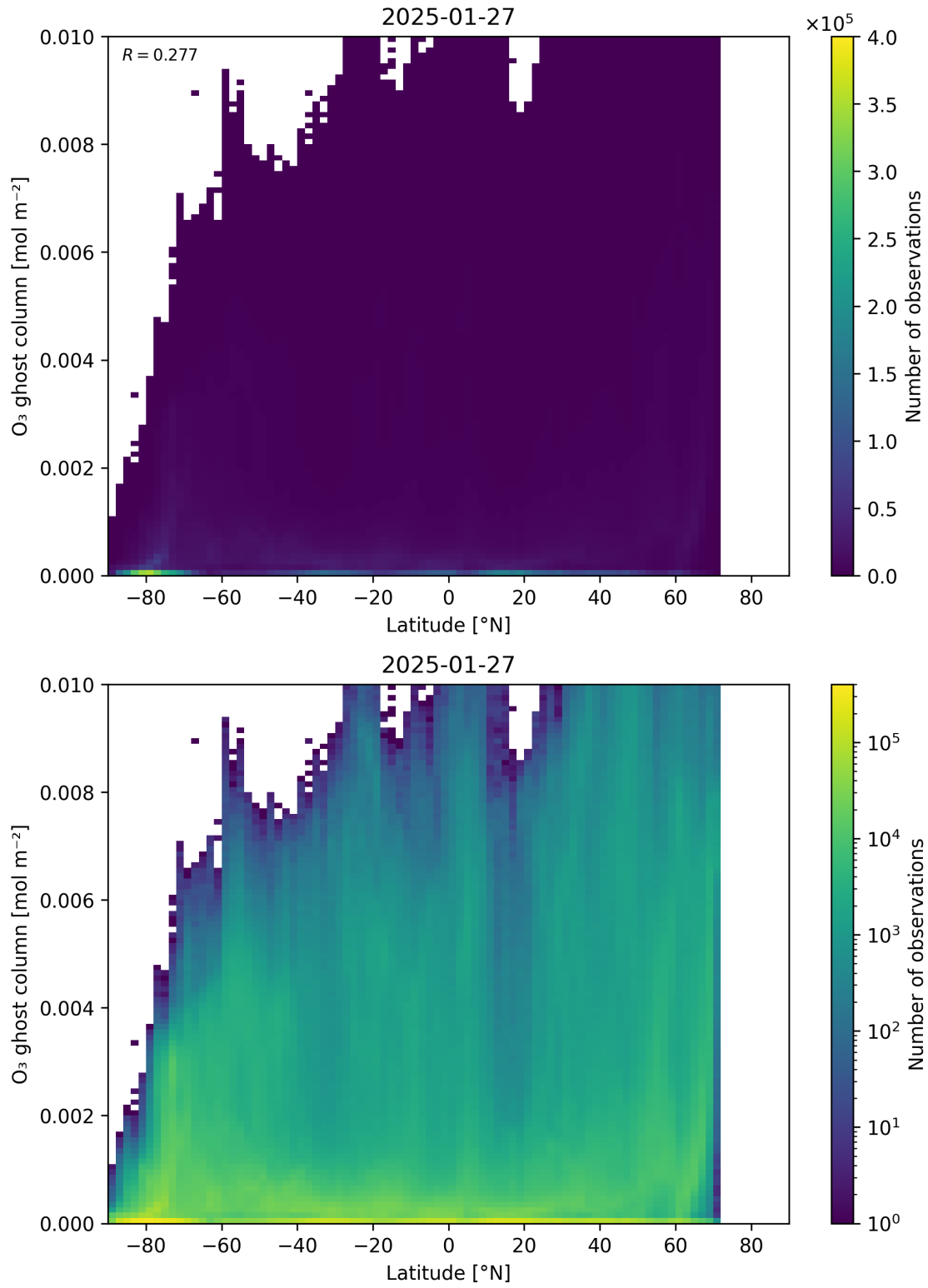
Figure 35: Scatter density plot of “Latitude” against “O 3 ghost column” for 2025-01-26 to 2025-01-28.
