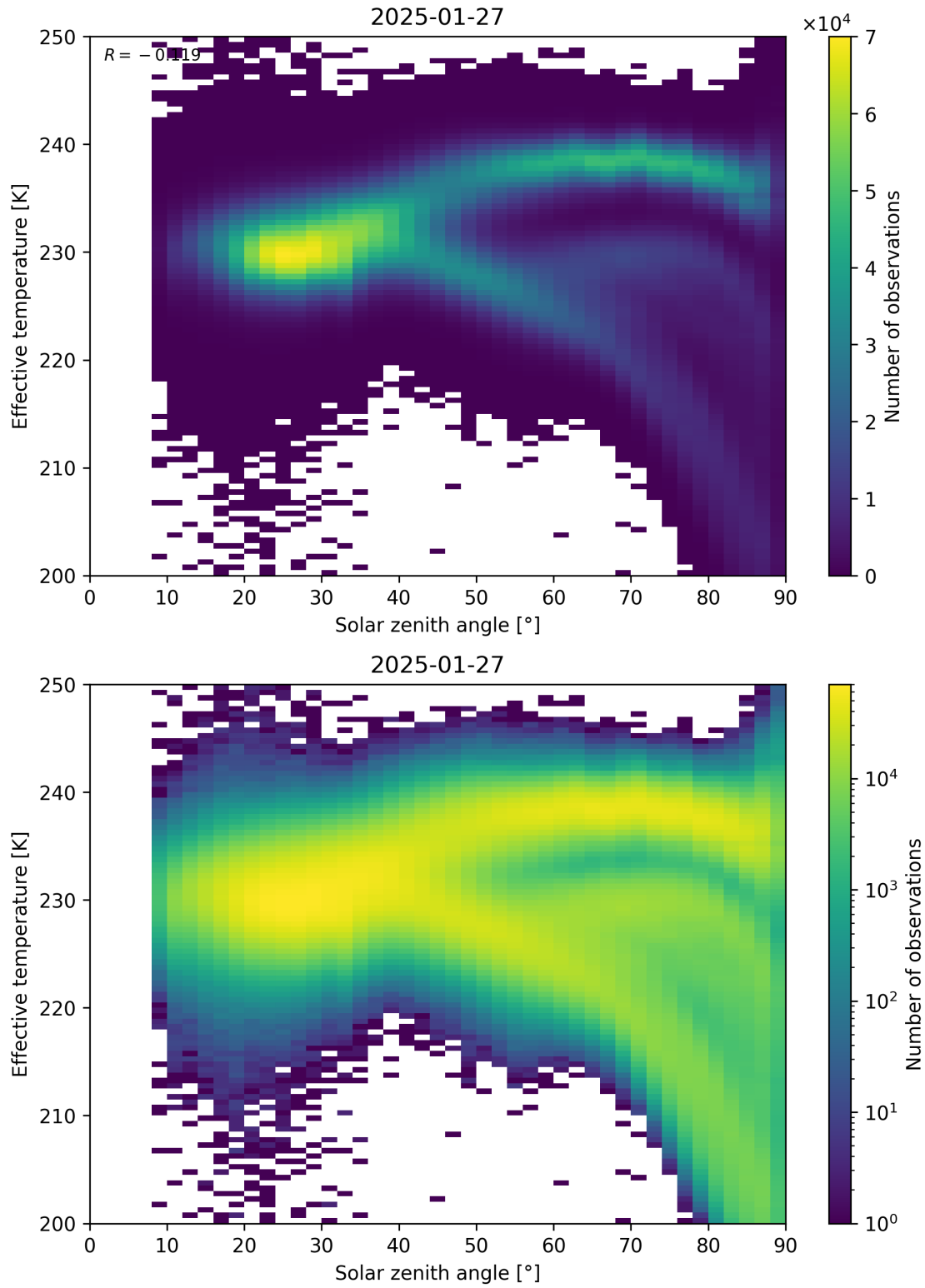
Figure 45: Scatter density plot of “Solar zenith angle” against “Effective temperature” for 2025-01-26 to 2025-01-28.
