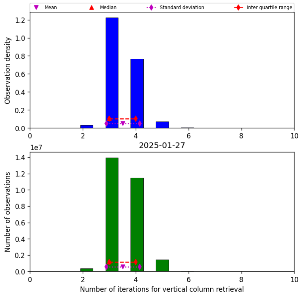
Figure 26: Histogram of “Number of iterations for vertical column retrieval” for 2025-01-26 to 2025-01-28
