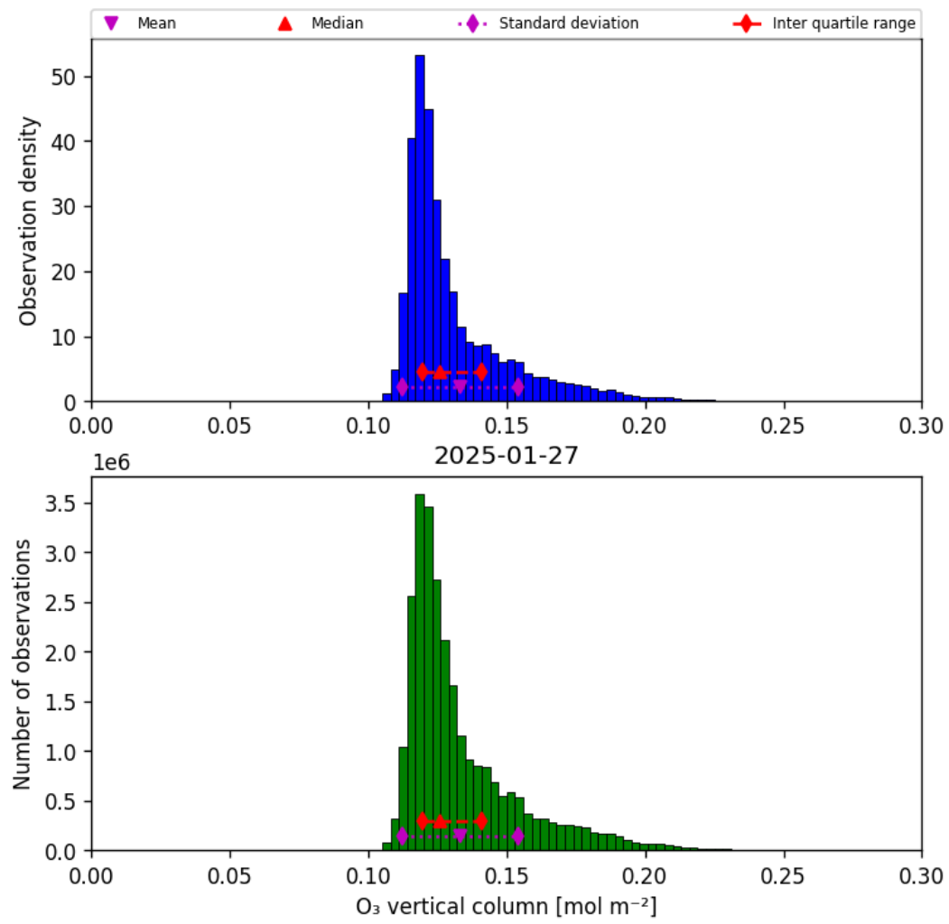
Figure 21: Histogram of “O 3 vertical column” for 2025-01-26 to 2025-01-28
