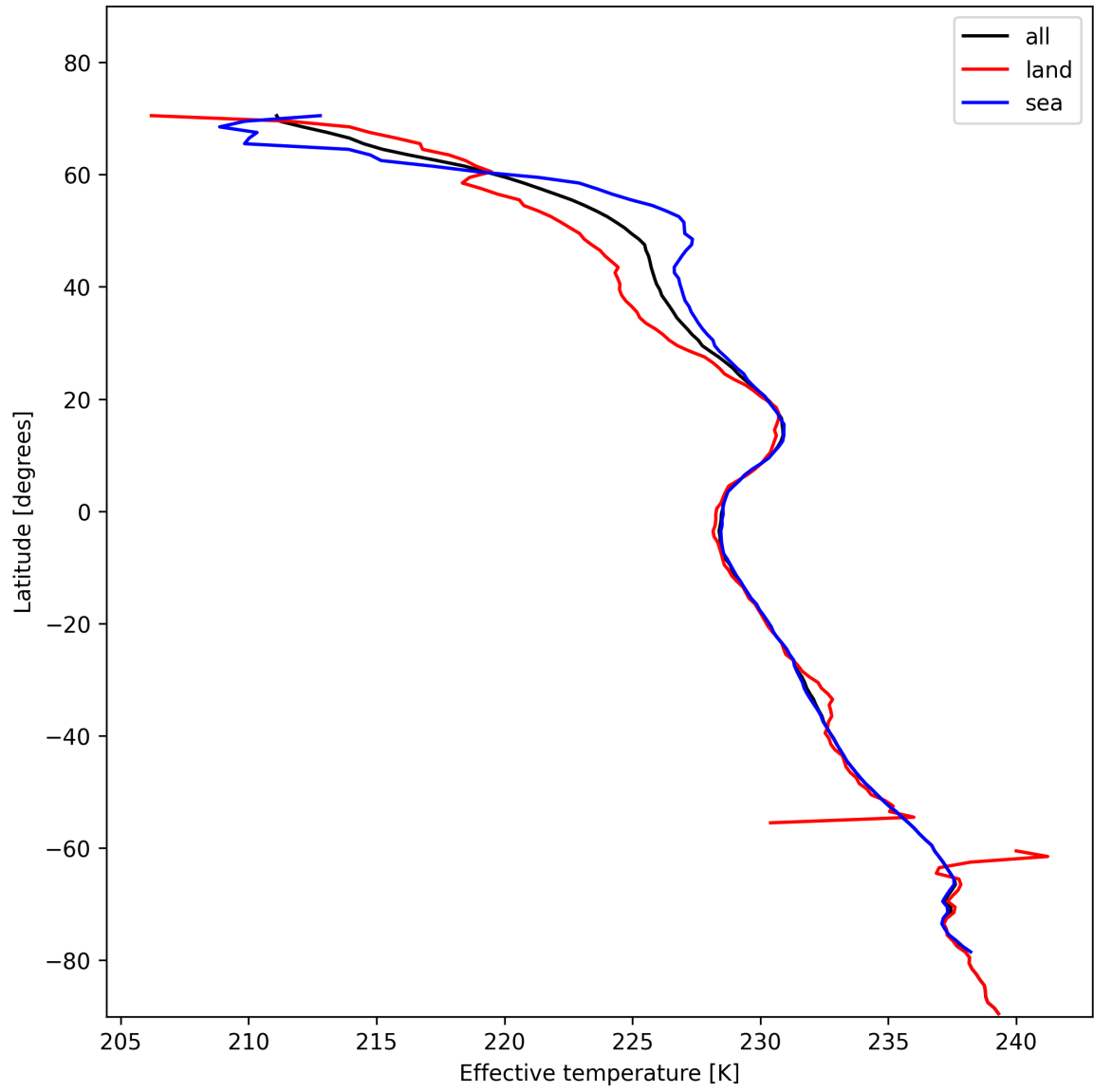
Figure 17: Zonal average of “Effective temperature” for 2025-01-26 to 2025-01-28.
