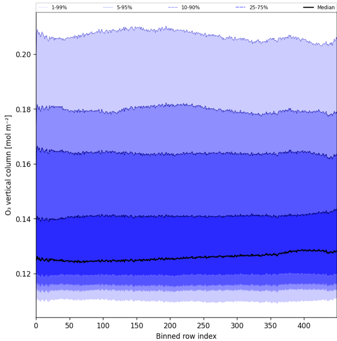
Figure 28: Along track statistics of “O 3 vertical column” for 2025-01-26 to 2025-01-28
