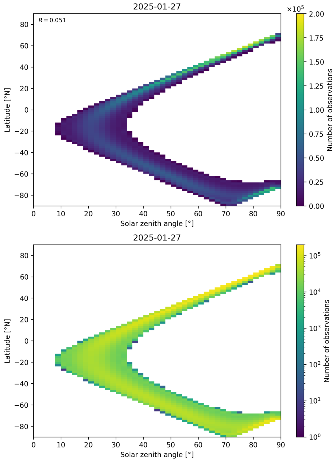
Figure 44: Scatter density plot of “Solar zenith angle” against “Latitude” for 2025-01-26 to 2025-01-28.
