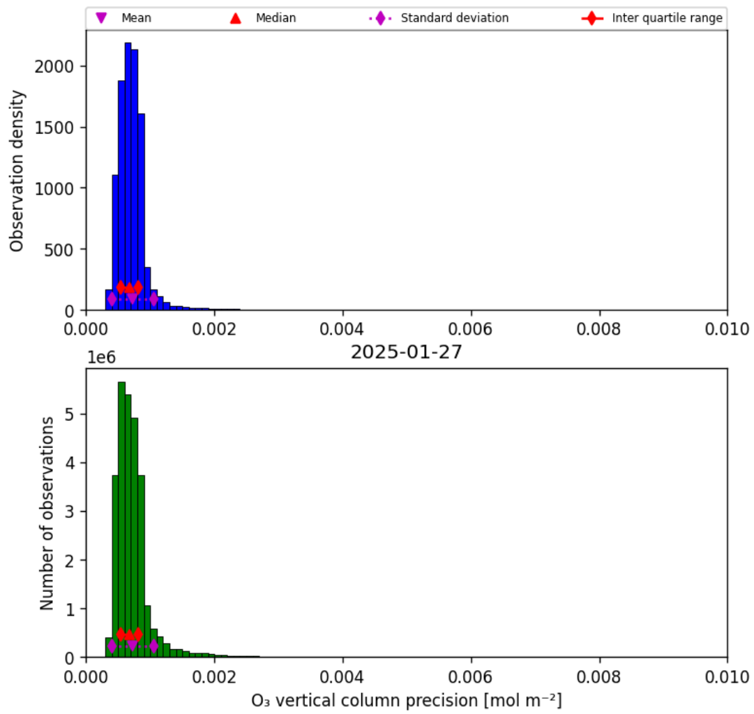
Figure 22: Histogram of “O 3 vertical column precision” for 2025-01-26 to 2025-01-28
