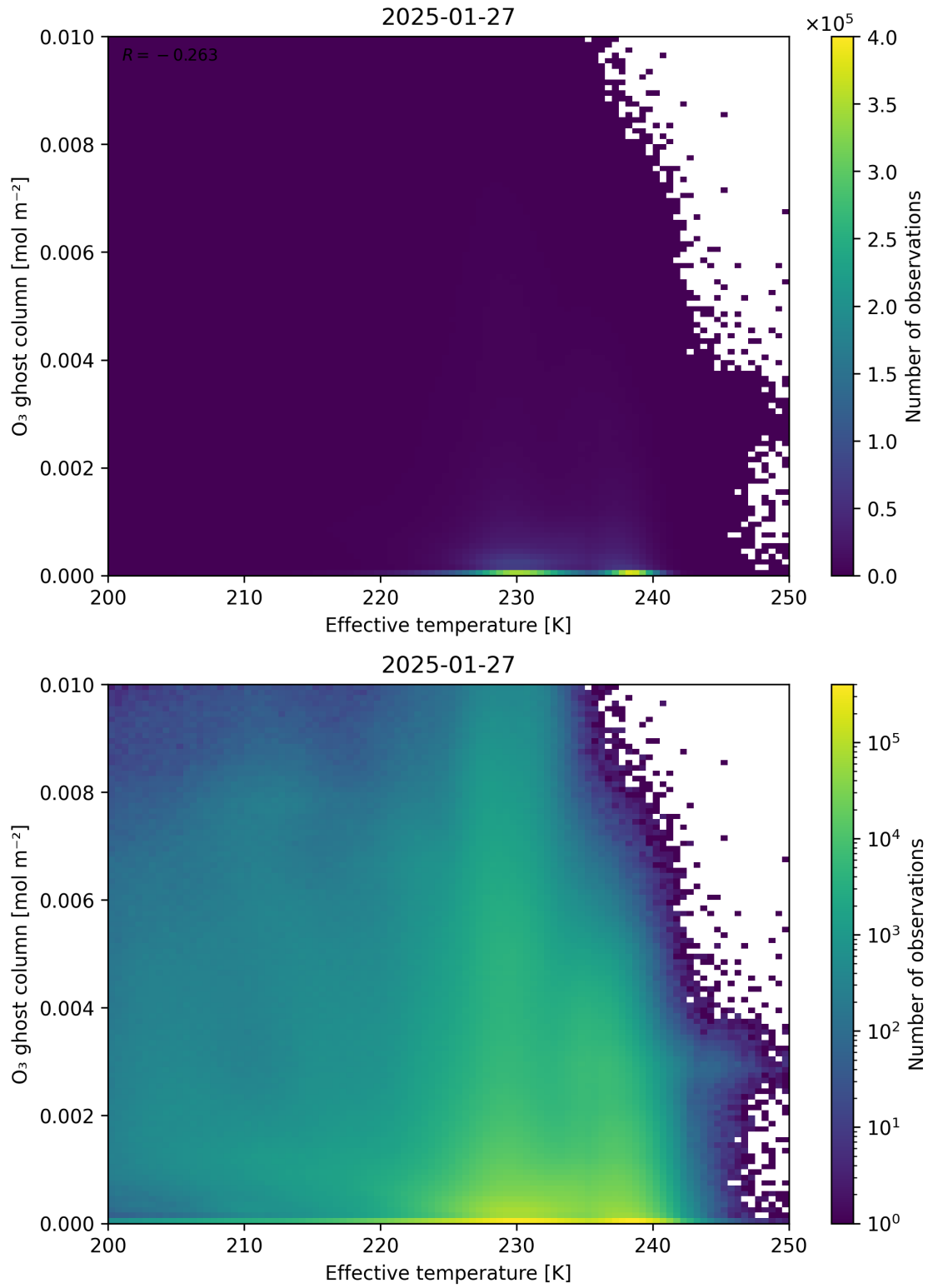
Figure 38: Scatter density plot of “Effective temperature” against “O 3 ghost column” for 2025-01-26 to 2025-01-28.
