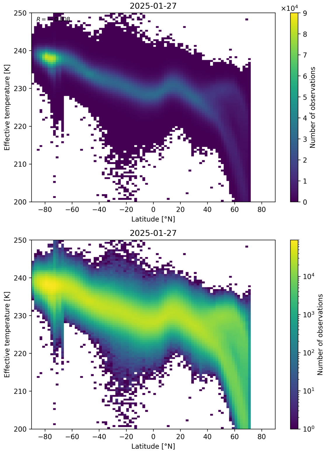
Figure 34: Scatter density plot of “Latitude” against “Effective temperature” for 2025-01-26 to 2025-01-28.
