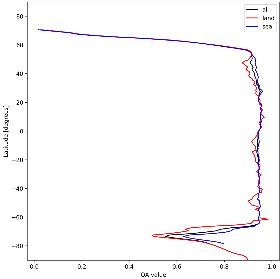
Figure 13: Zonal average of “QA value” for 2025-01-26 to 2025-01-28.
