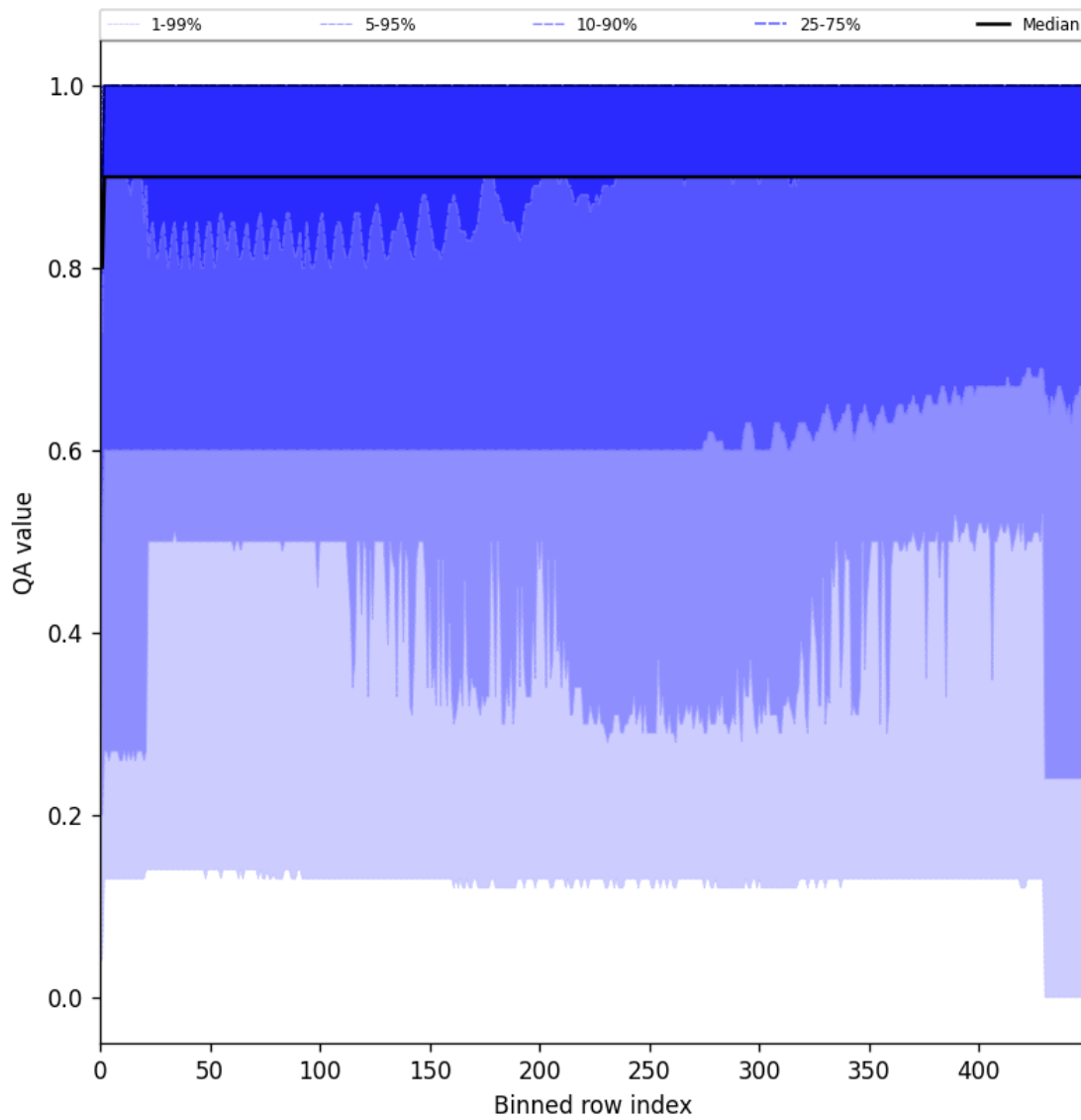
Figure 27: Along track statistics of “QA value” for 2025-01-26 to 2025-01-28
