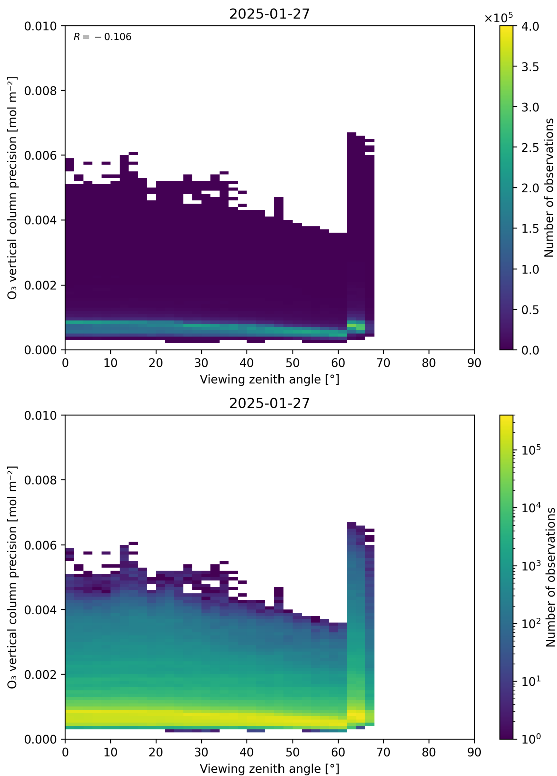
Figure 53: Scatter density plot of “Viewing zenith angle” against “O 3 vertical column precision” for 2025-01-26 to 2025-01-28.
