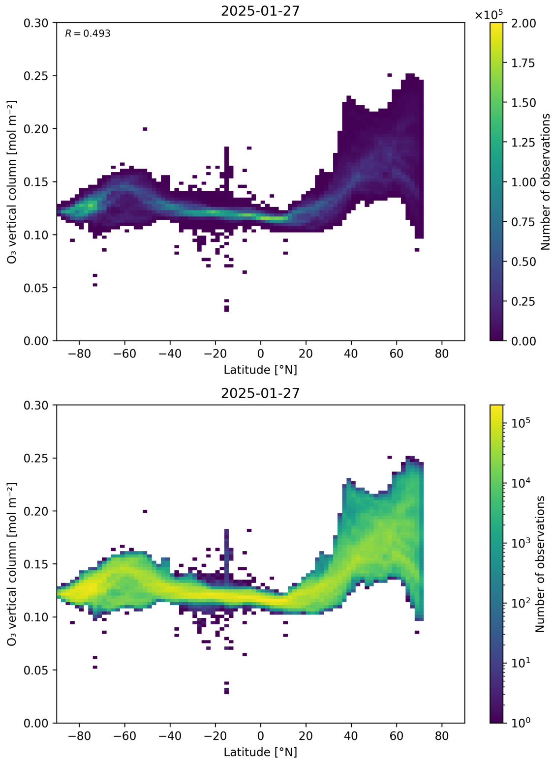
Figure 36: Scatter density plot of “Latitude” against “O 3 vertical column” for 2025-01-26 to 2025-01-28.
