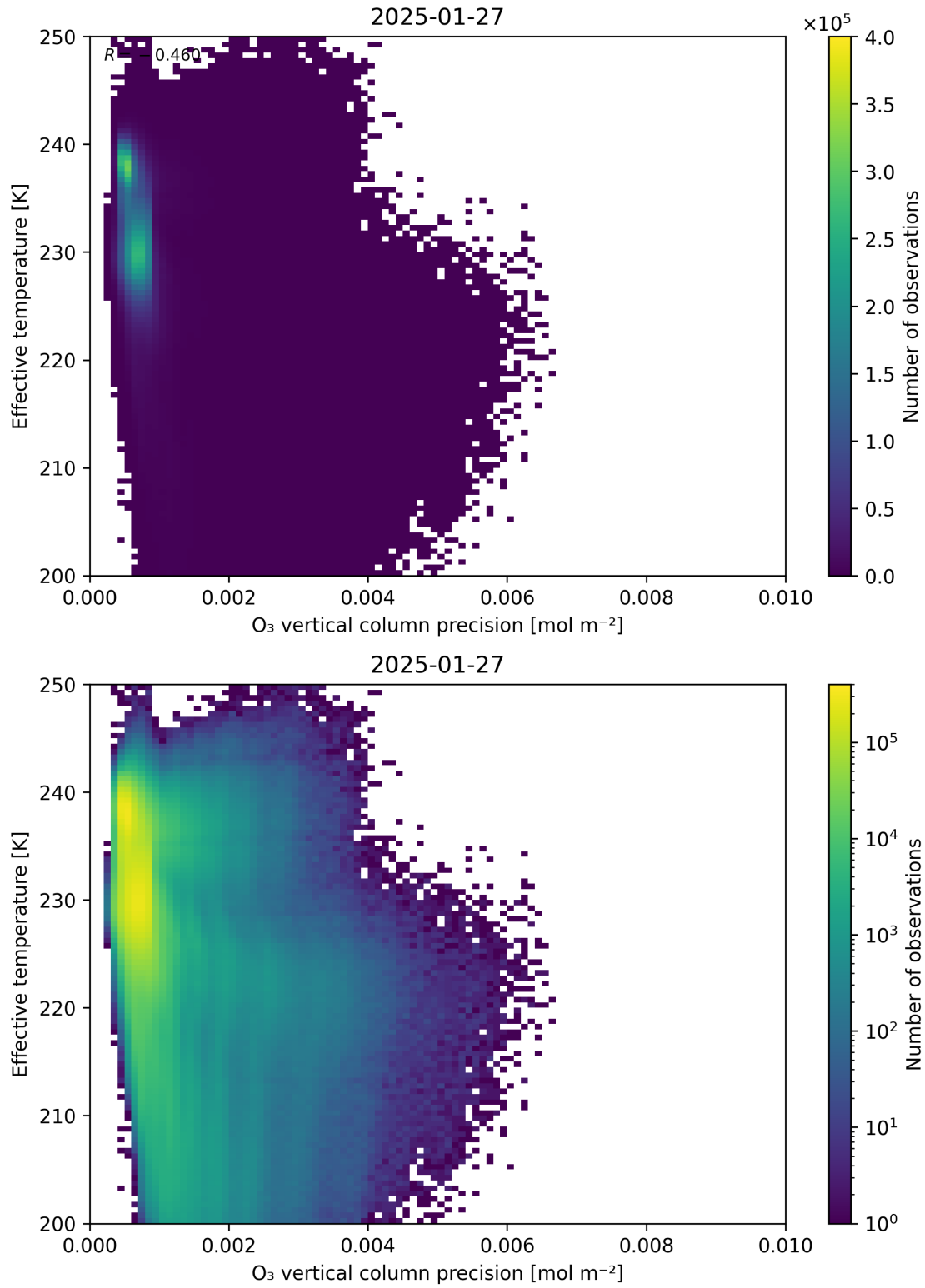
Figure 42: Scatter density plot of “O 3 vertical column precision” against “Effective temperature” for 2025-01-26 to 2025-01-28.
