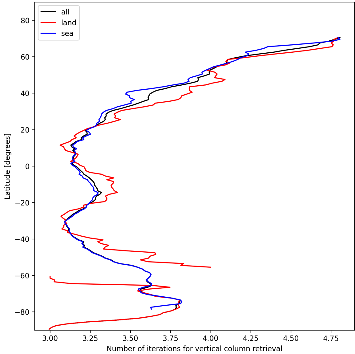
Figure 19: Zonal average of “Number of iterations for vertical column retrieval” for 2025-01-26 to 2025-01-28.
