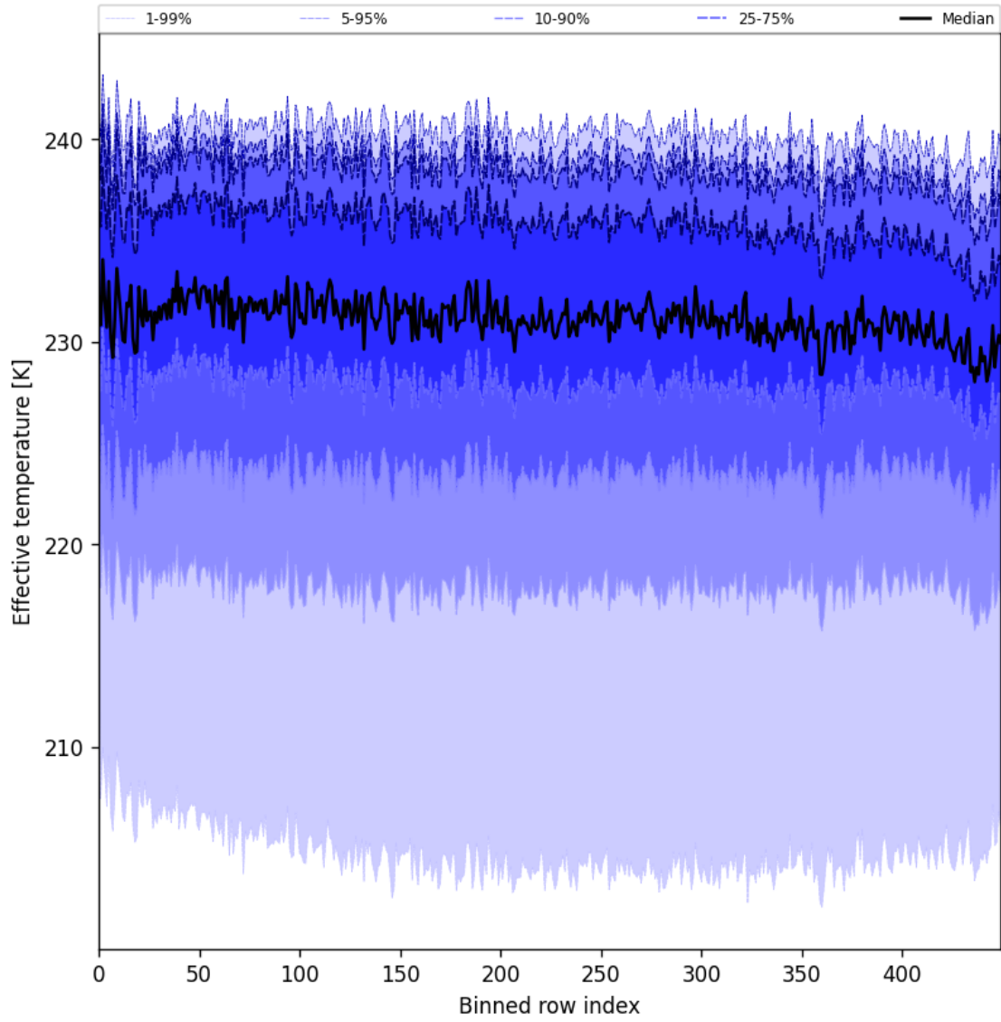
Figure 31: Along track statistics of "Effective temperature" for 2025-01-26 to 2025-01-28
