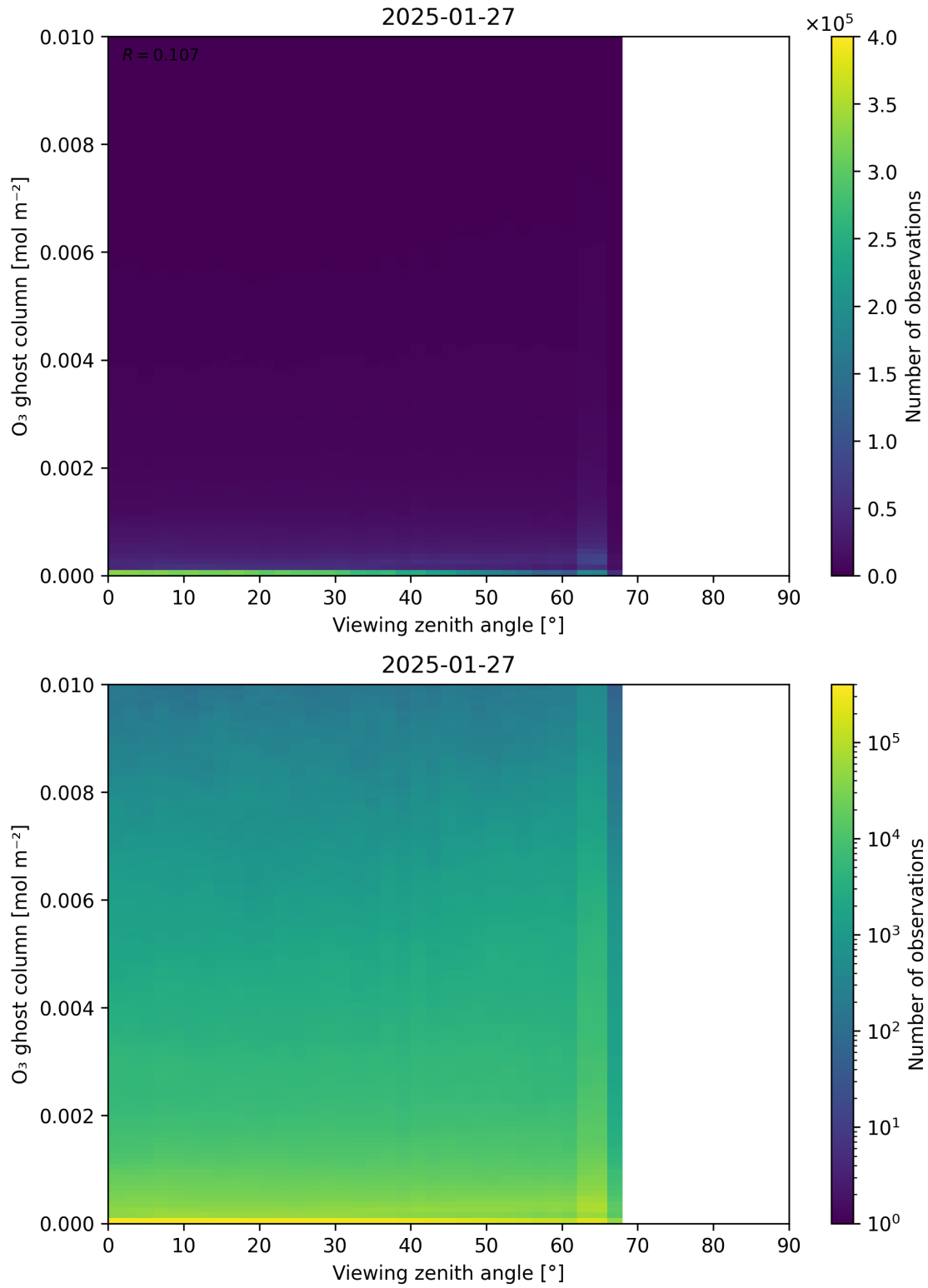
Figure 51: Scatter density plot of “Viewing zenith angle” against “O 3 ghost column” for 2025-01-26 to 2025-01-28.
