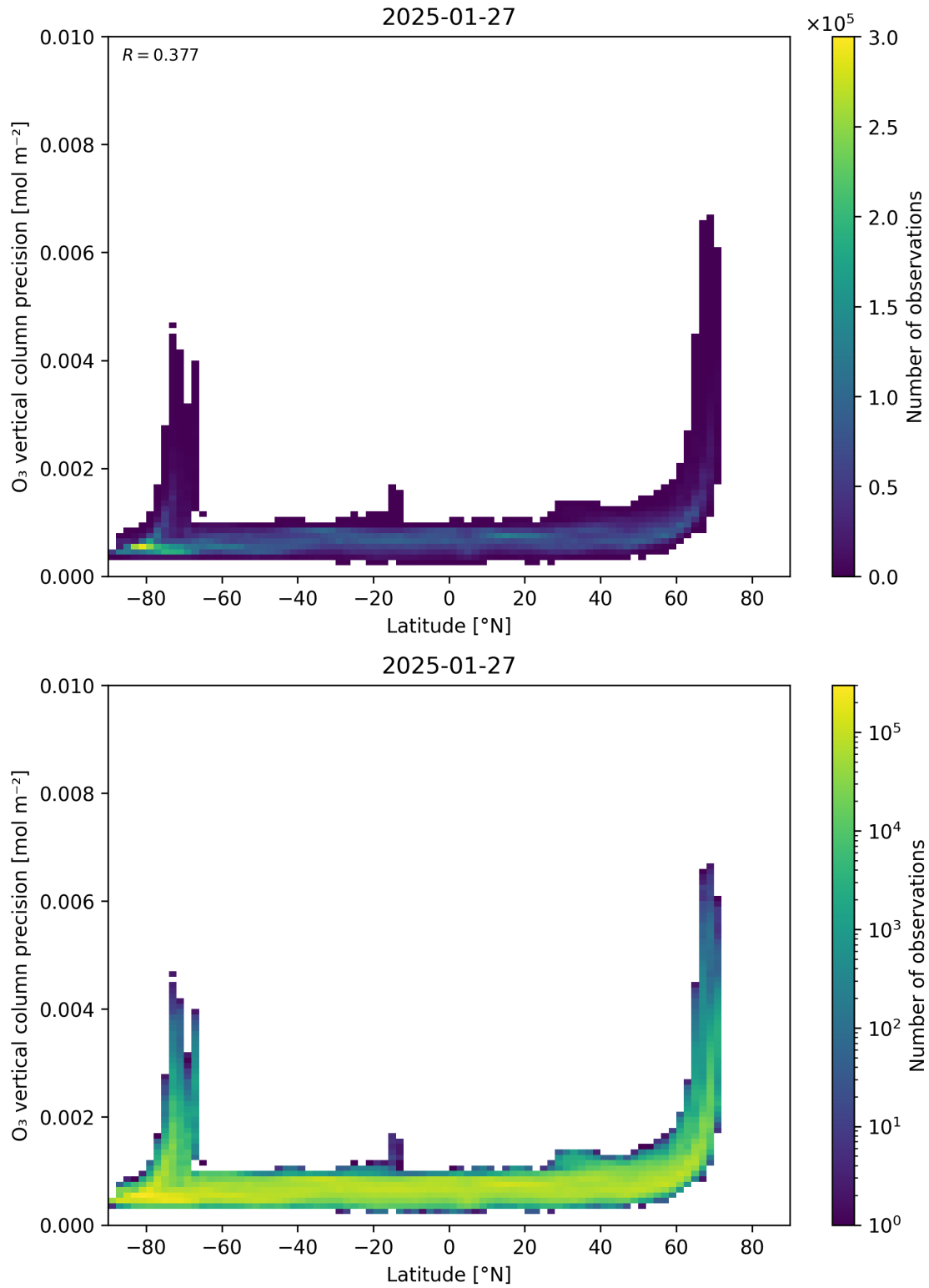
Figure 37: Scatter density plot of “Latitude” against “O 3 vertical column precision” for 2025-01-26 to 2025-01-28.
