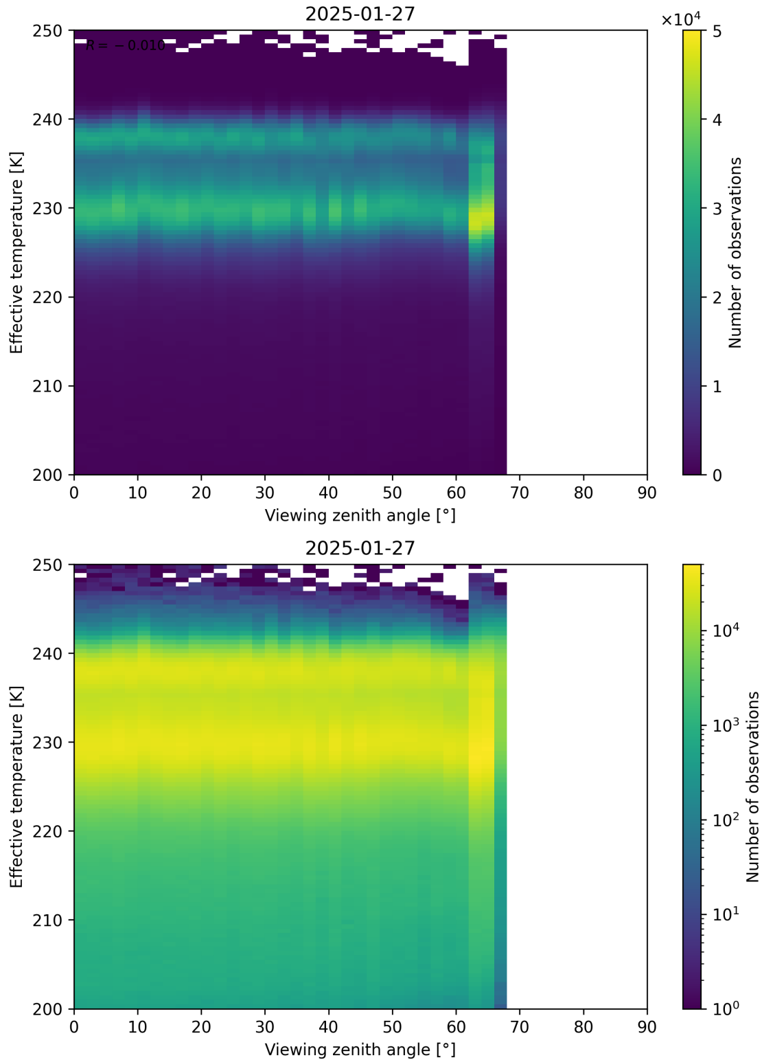
Figure 50: Scatter density plot of “Viewing zenith angle” against “Effective temperature” for 2025-01-26 to 2025-01-28.
