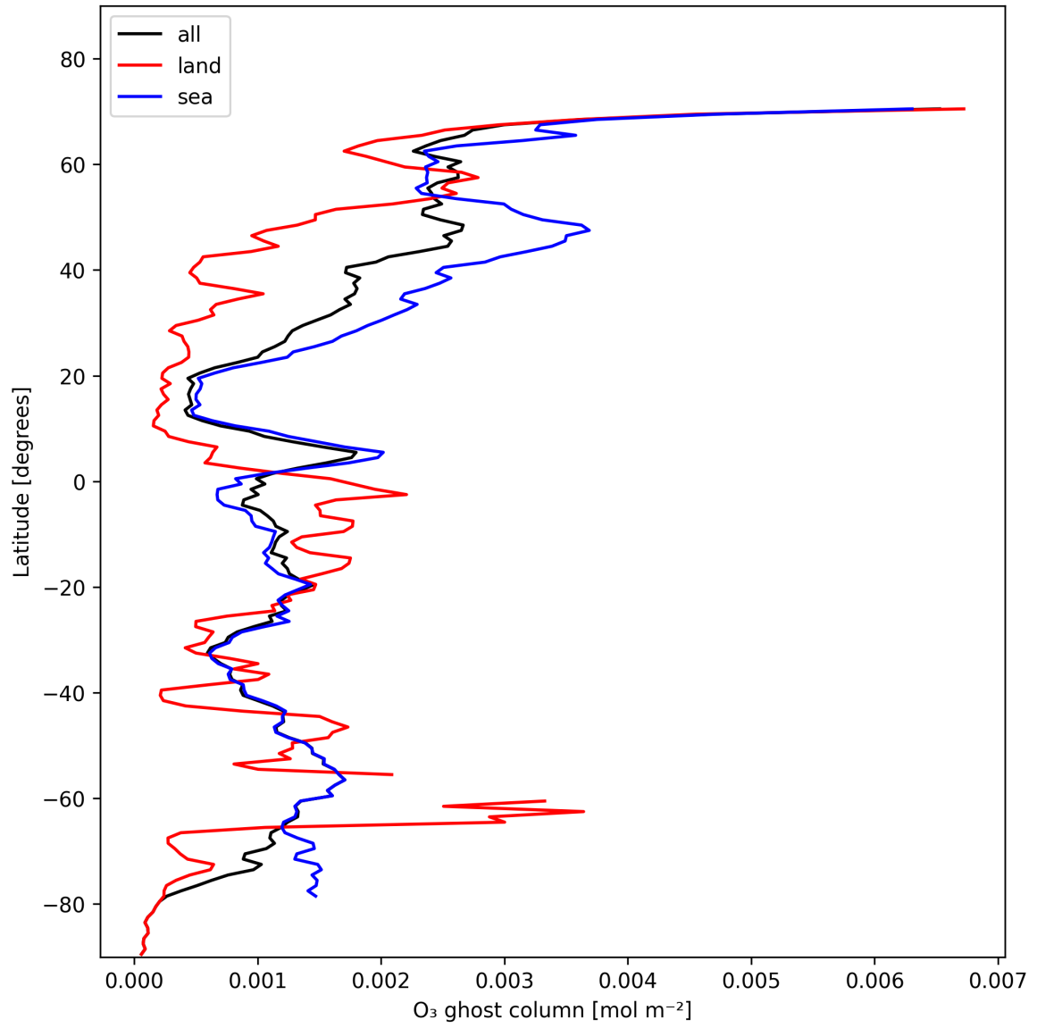
Figure 18: Zonal average of "O 3 ghost column" for 2025-01-26 to 2025-01-28.
