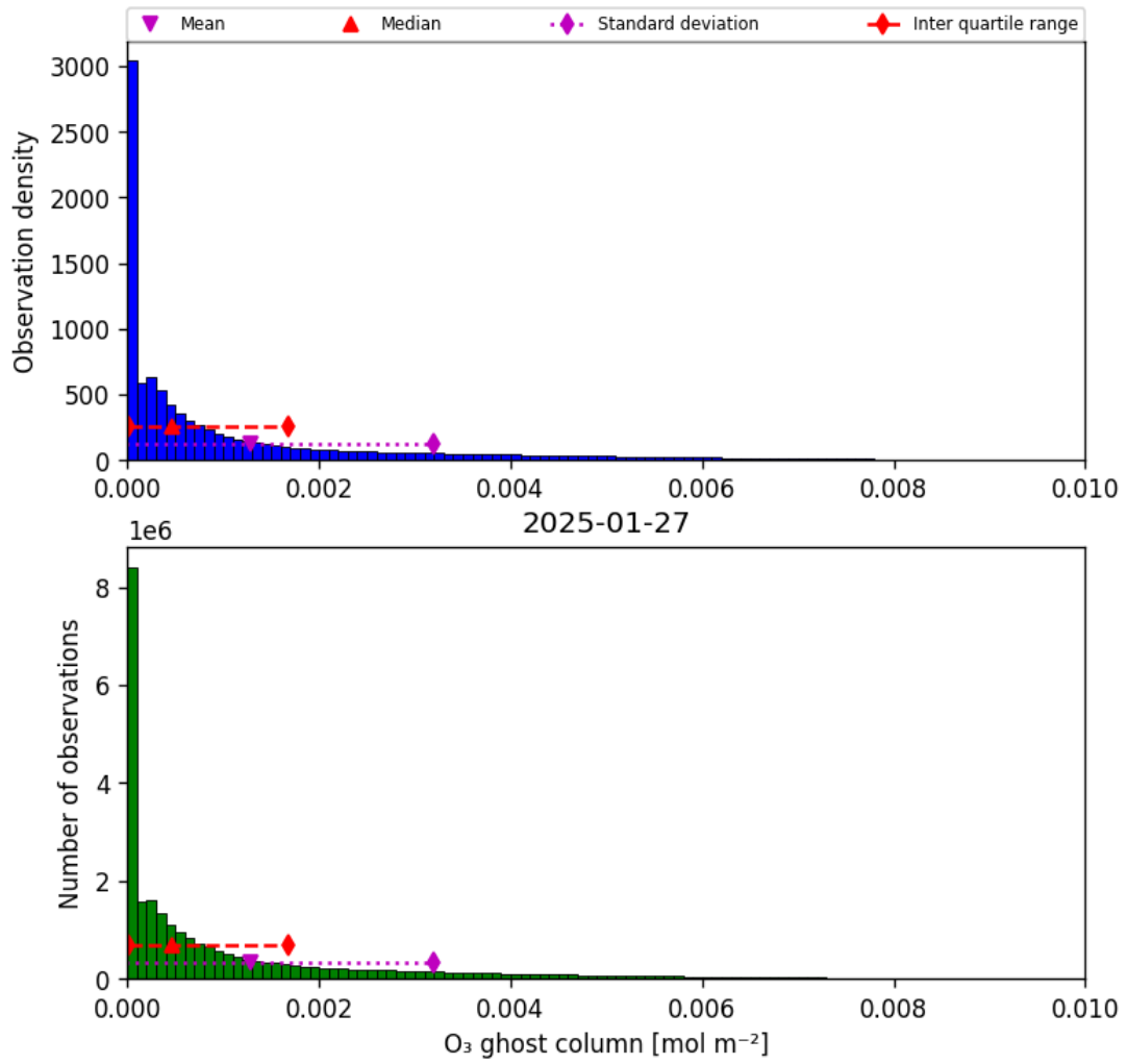
Figure 25: Histogram of “O 3 ghost column” for 2025-01-26 to 2025-01-28
