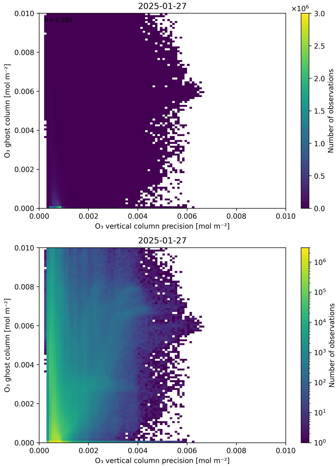
Figure 43: Scatter density plot of “ \text{O}_3 vertical column precision” against “ \text{O}_3 ghost column” for 2025-01-26 to 2025-01-28.
