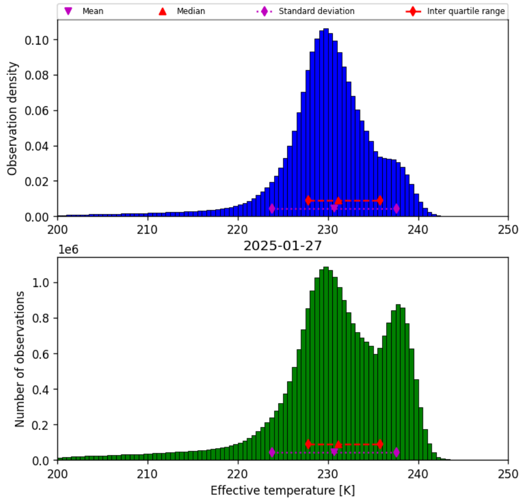
Figure 24: Histogram of “Effective temperature” for 2025-01-26 to 2025-01-28
