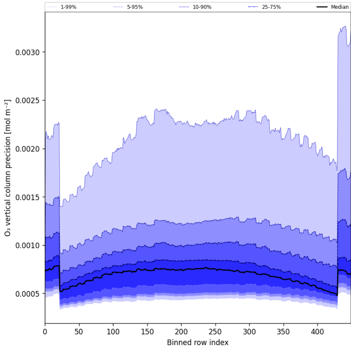
Figure 29: Along track statistics of “O 3 vertical column precision” for 2025-01-26 to 2025-01-28
