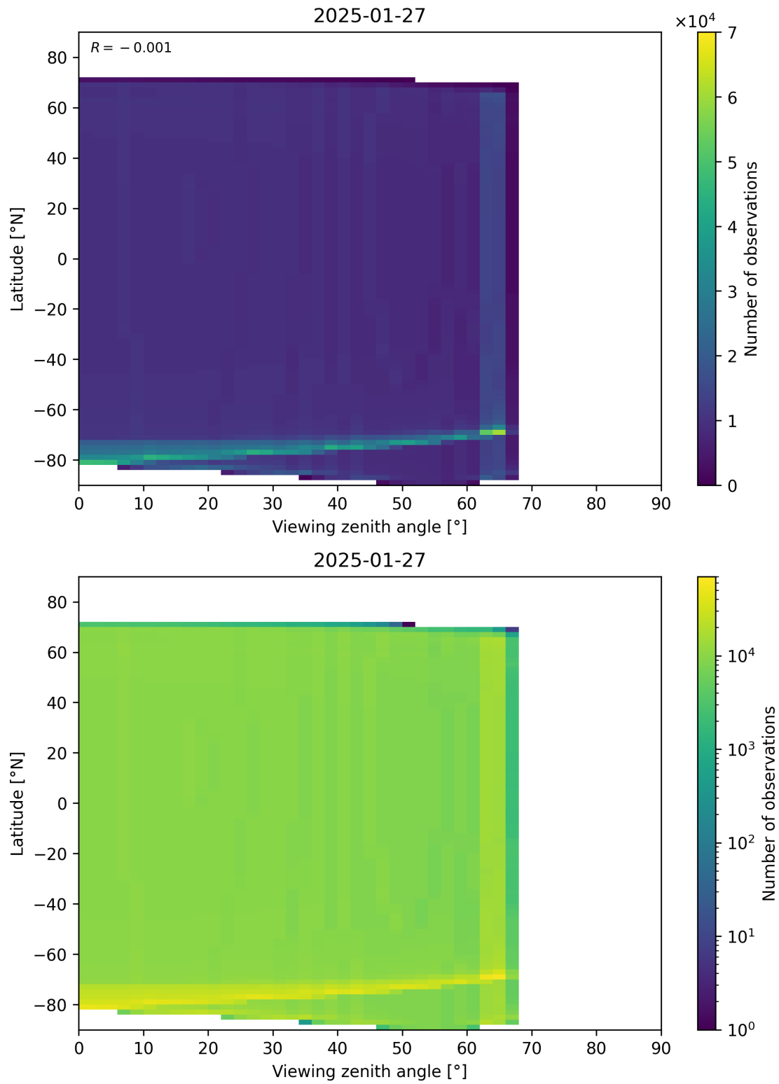
Figure 49: Scatter density plot of “Viewing zenith angle” against “Latitude” for 2025-01-26 to 2025-01-28.
