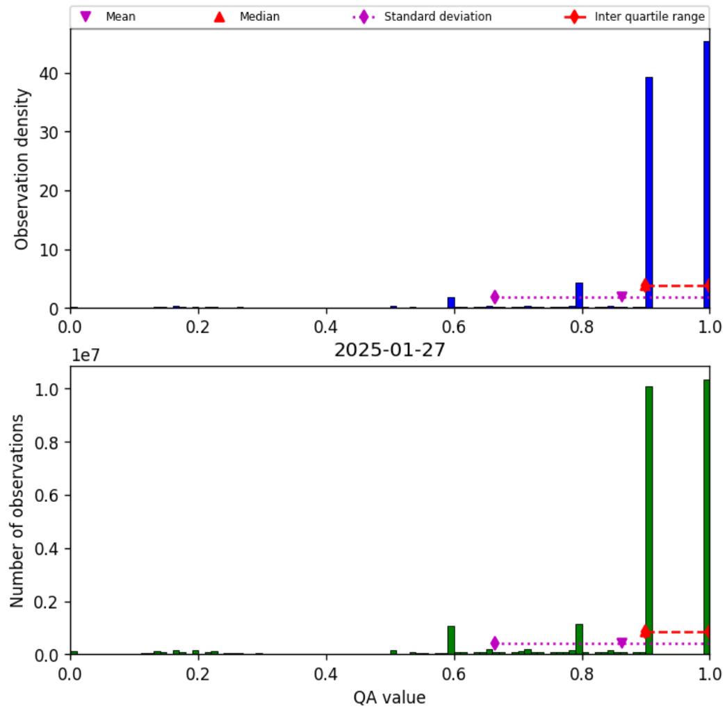
Figure 20: Histogram of “QA value” for 2025-01-26 to 2025-01-28
