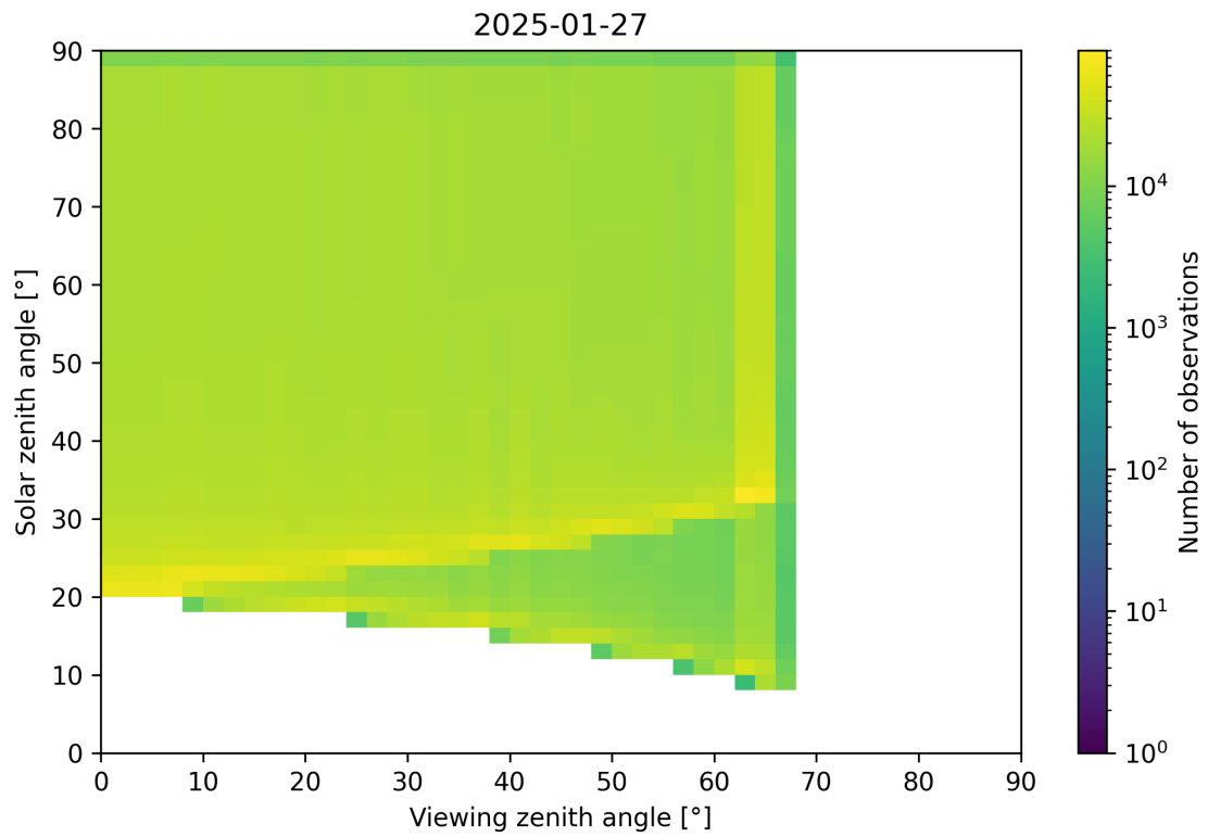
Figure 54: Scatter density plot of “Viewing zenith angle” against “Solar zenith angle” for 2025-01-26 to 2025-01-28.
