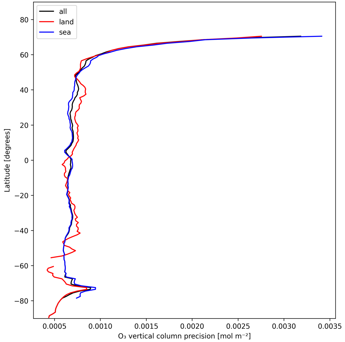
Figure 15: Zonal average of “O 3 vertical column precision” for 2025-01-26 to 2025-01-28.
