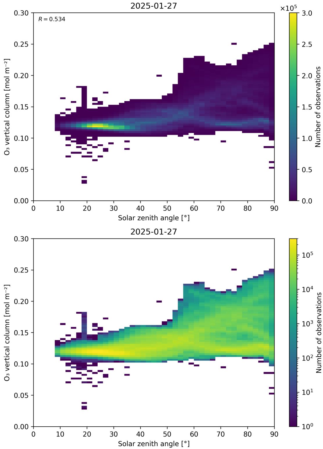
Figure 47: Scatter density plot of “Solar zenith angle” against “O 3 vertical column” for 2025-01-26 to 2025-01-28.
