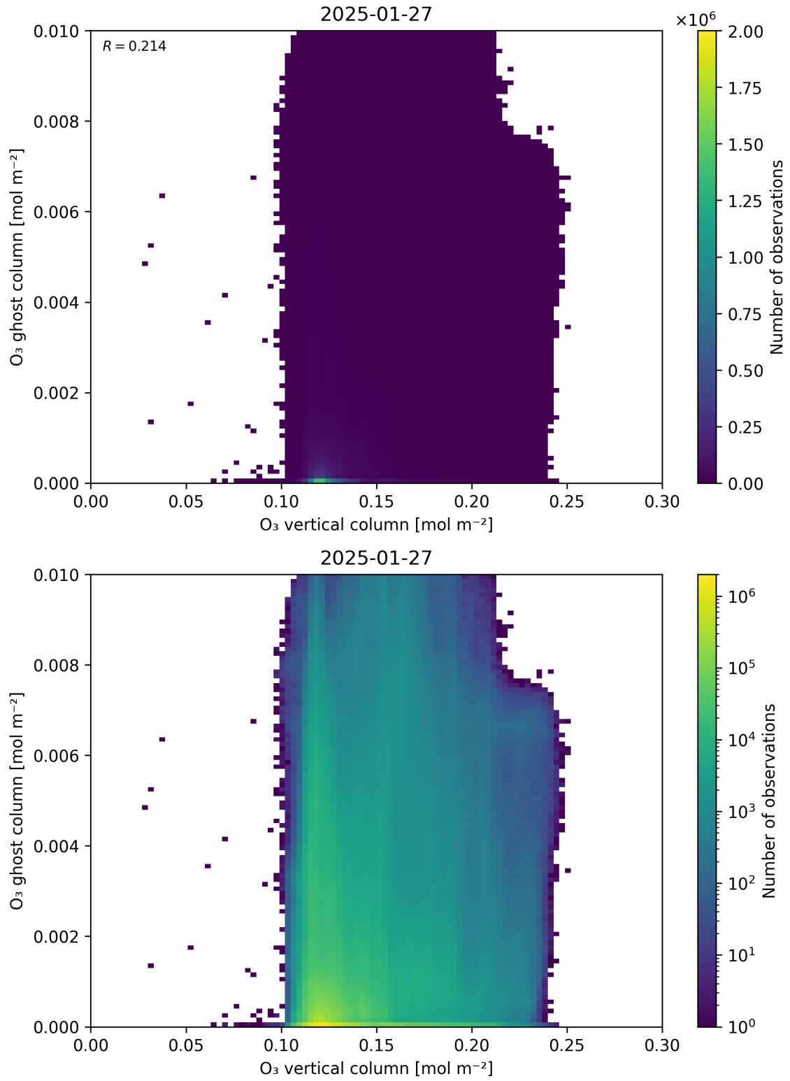
Figure 40: Scatter density plot of “O 3 vertical column” against “O 3 ghost column” for 2025-01-26 to 2025-01-28.
