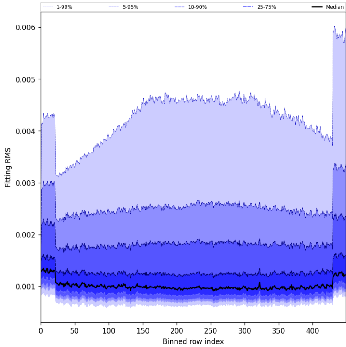
Figure 30: Along track statistics of “Fitting RMS” for 2025-01-26 to 2025-01-28
