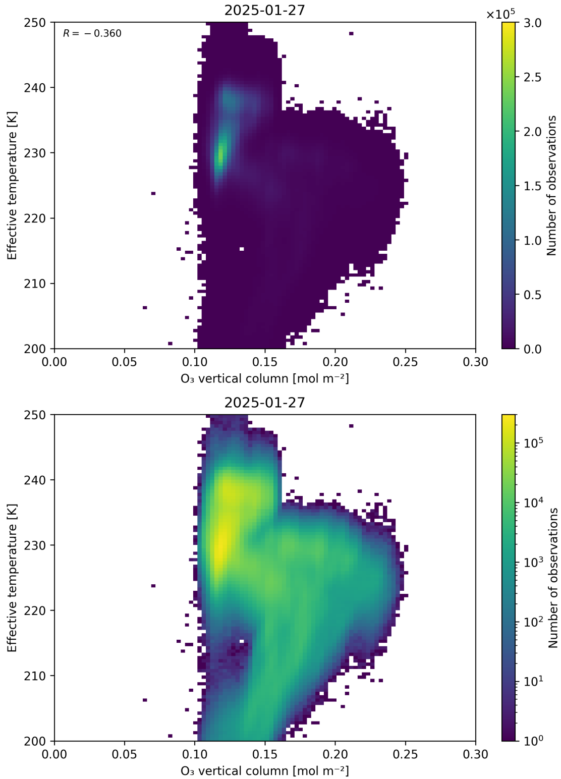
Figure 39: Scatter density plot of “O 3 vertical column” against “Effective temperature” for 2025-01-26 to 2025-01-28.
