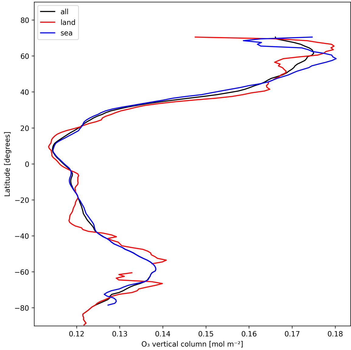
Figure 14: Zonal average of “O 3 vertical column” for 2025-01-26 to 2025-01-28.
