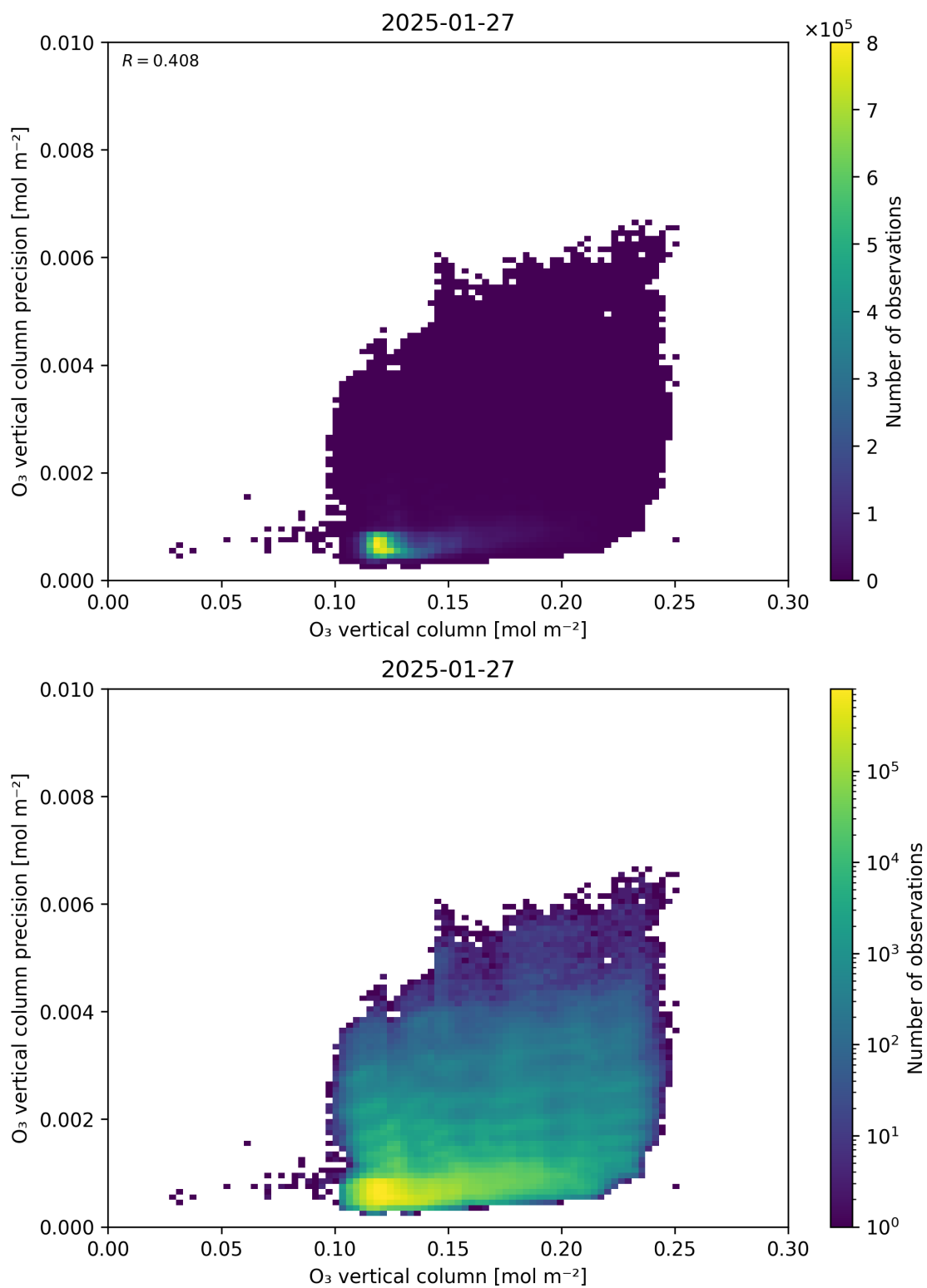
Figure 41: Scatter density plot of “O 3 vertical column” against “O 3 vertical column precision” for 2025-01-26 to 2025-01-28.
