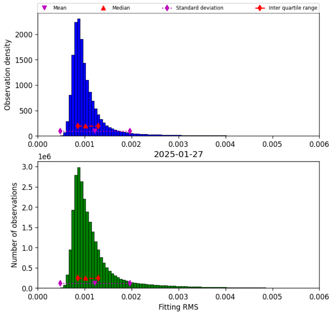
Figure 23: Histogram of “Fitting RMS” for 2025-01-26 to 2025-01-28
