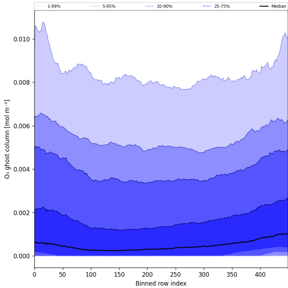
Figure 32: Along track statistics of “O 3 ghost column” for 2025-01-26 to 2025-01-28
