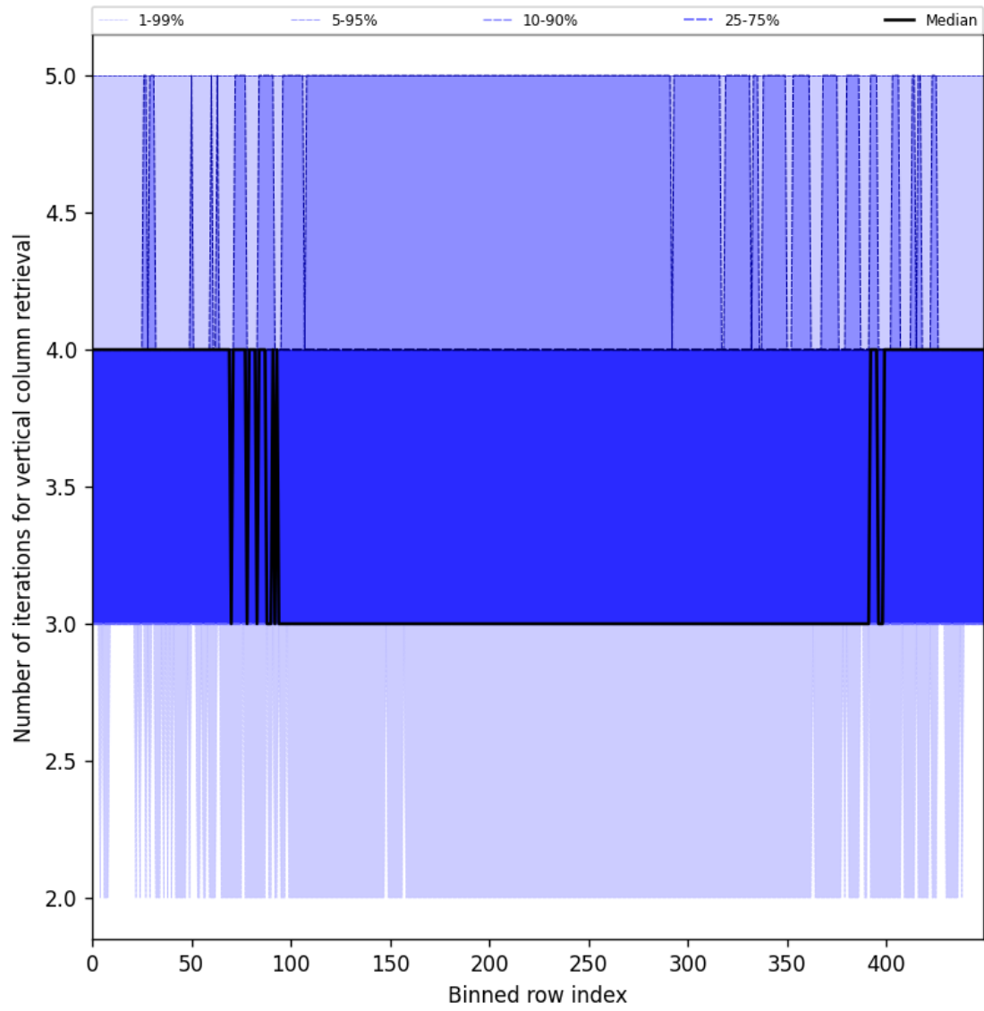
Figure 33: Along track statistics of “Number of iterations for vertical column retrieval” for 2025-01-26 to 2025-01-28
