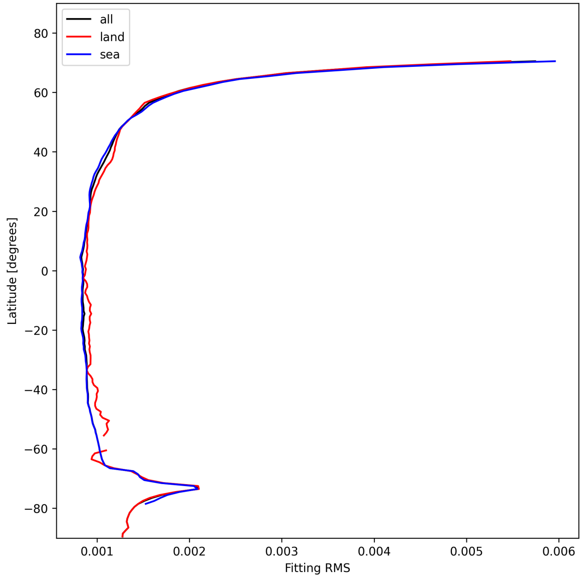
Figure 16: Zonal average of “Fitting RMS” for 2025-01-26 to 2025-01-28.
