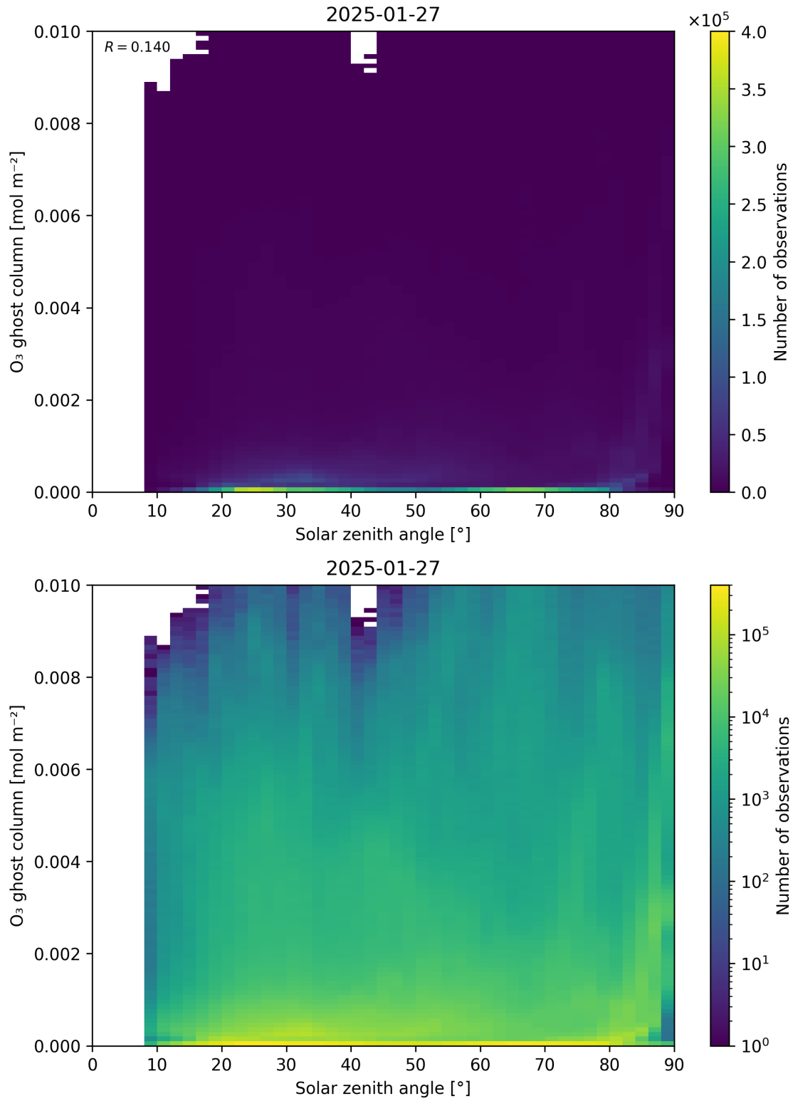
Figure 46: Scatter density plot of “Solar zenith angle” against “O 3 ghost column” for 2025-01-26 to 2025-01-28.
