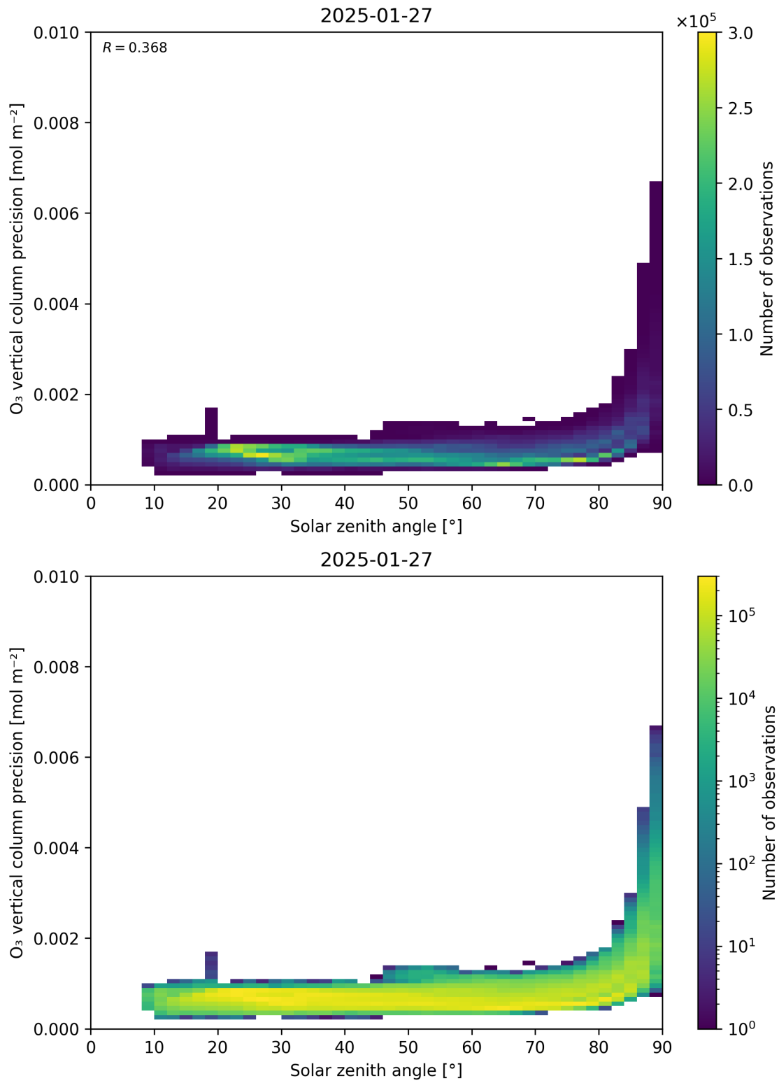
Figure 48: Scatter density plot of “Solar zenith angle” against “O 3 vertical column precision” for 2025-01-26 to 2025-01-28.
