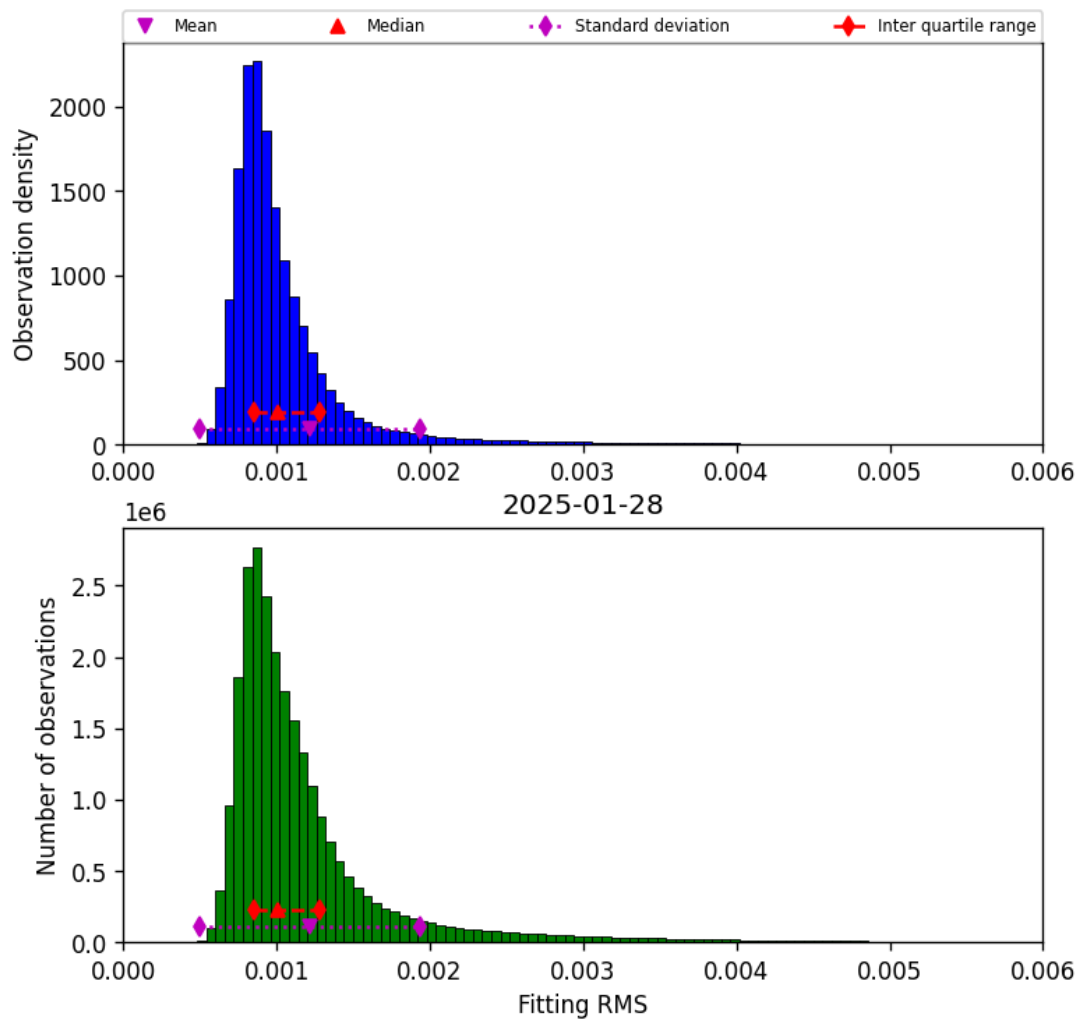
Figure 23: Histogram of “Fitting RMS” for 2025-01-28 to 2025-01-29
