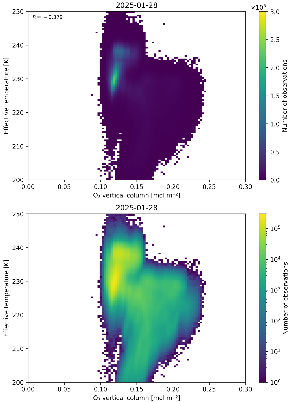
Figure 39: Scatter density plot of “O 3 vertical column” against “Effective temperature” for 2025-01-28 to 2025-01-29.
