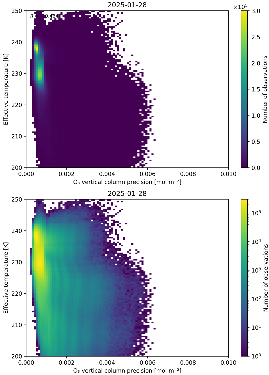
Figure 42: Scatter density plot of “O 3 vertical column precision” against “Effective temperature” for 2025-01-28 to 2025-01-29.
