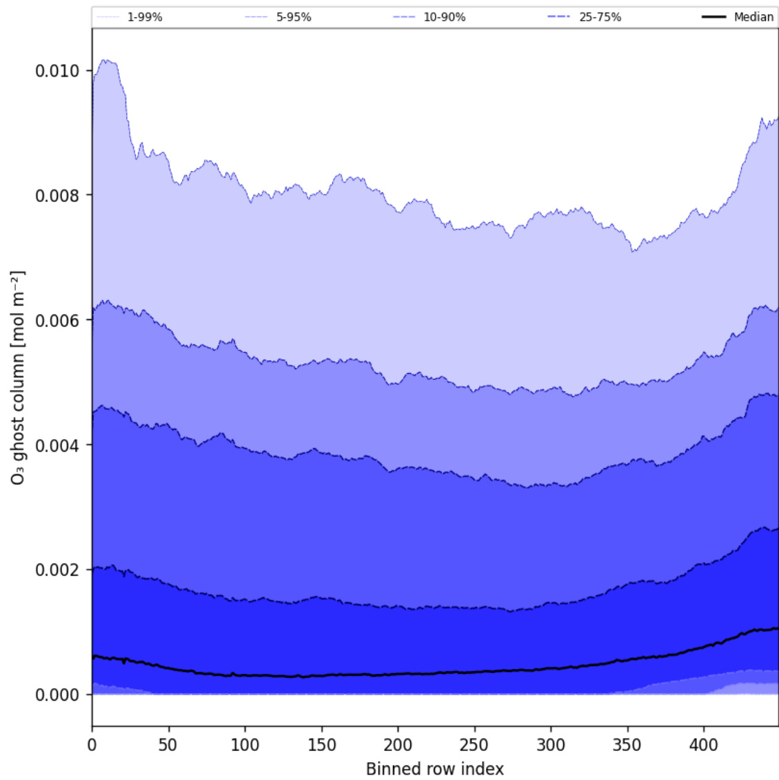
Figure 32: Along track statistics of “O 3 ghost column” for 2025-01-28 to 2025-01-29
