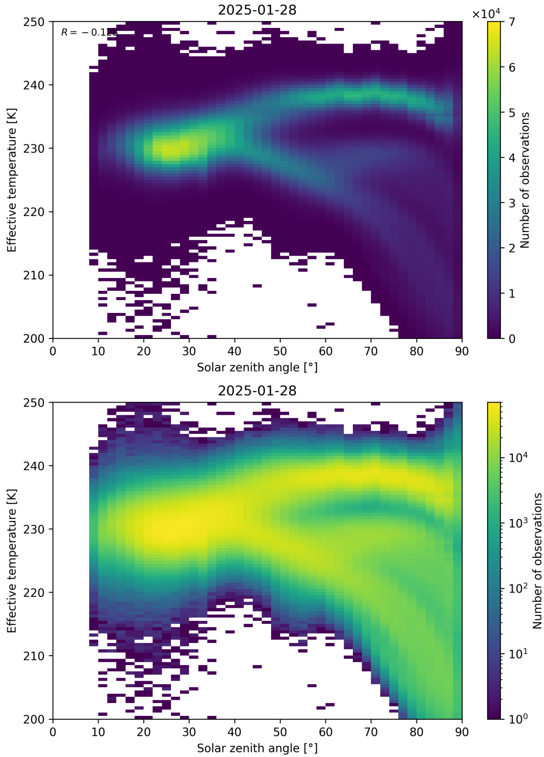
Figure 45: Scatter density plot of “Solar zenith angle” against “Effective temperature” for 2025-01-28 to 2025-01-29.
