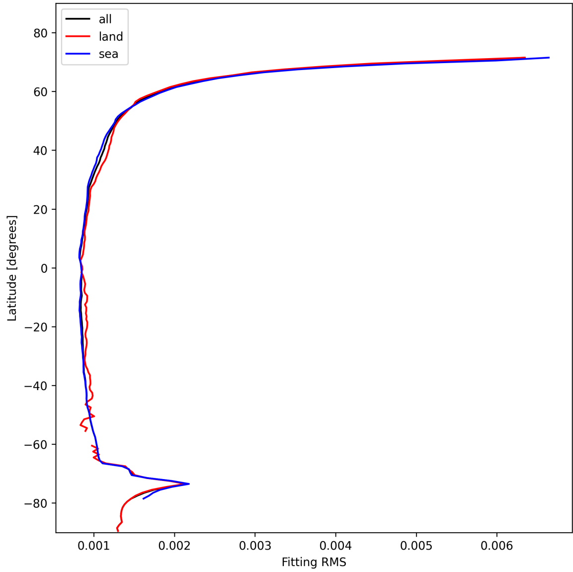
Figure 16: Zonal average of “Fitting RMS” for 2025-01-28 to 2025-01-29.
