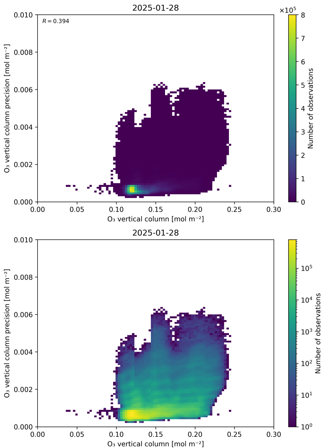
Figure 41: Scatter density plot of “O 3 vertical column” against “O 3 vertical column precision” for 2025-01-28 to 2025-01-29.
