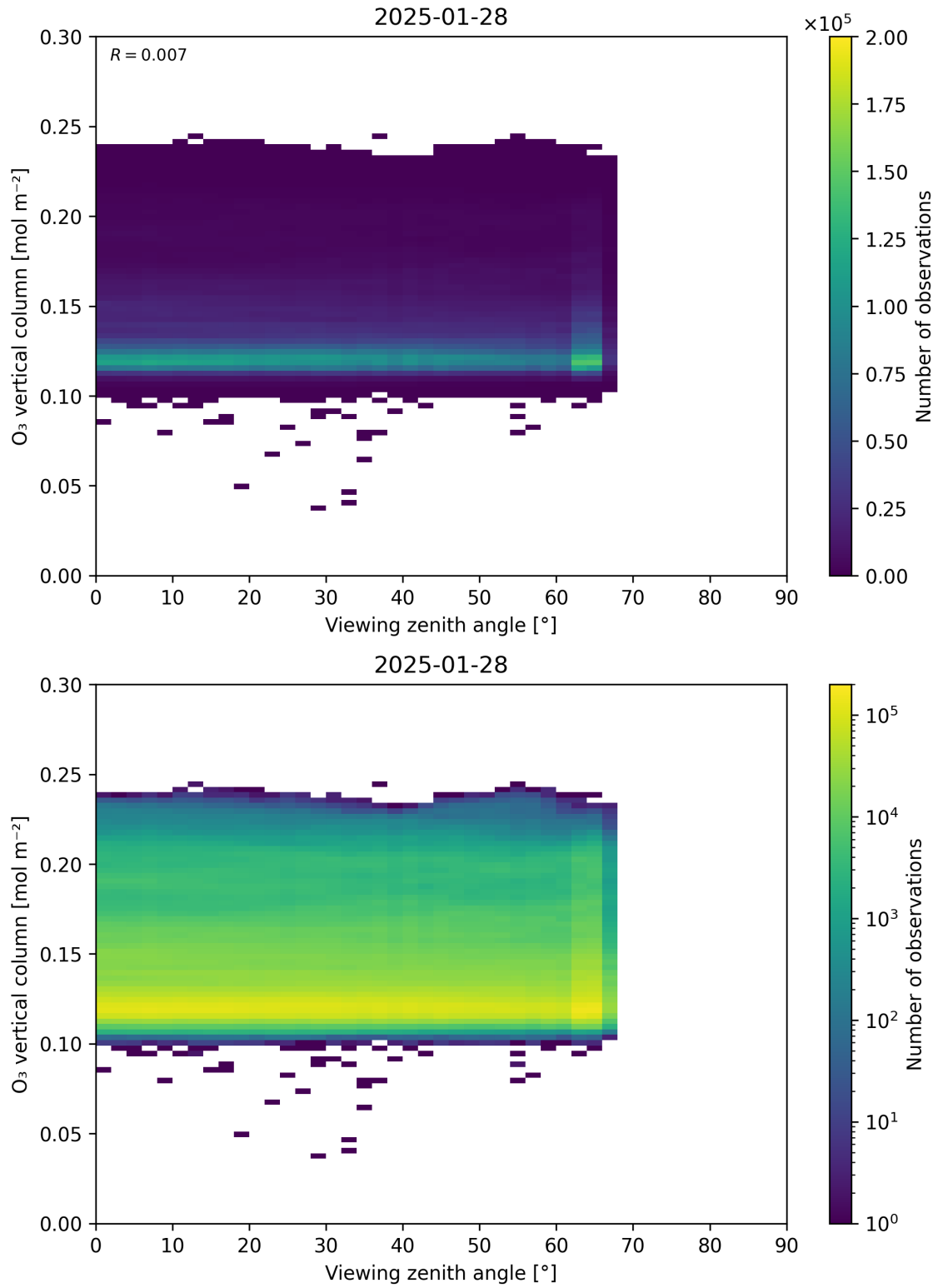
Figure 52: Scatter density plot of “Viewing zenith angle” against “O 3 vertical column” for 2025-01-28 to 2025-01-29.
