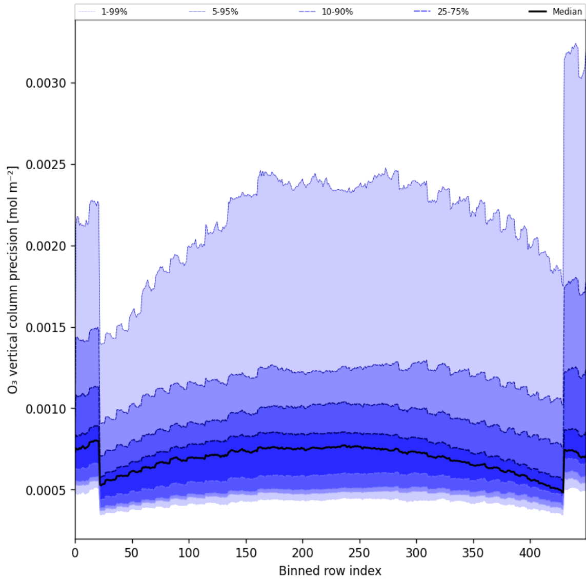
Figure 29: Along track statistics of “O 3 vertical column precision” for 2025-01-28 to 2025-01-29
