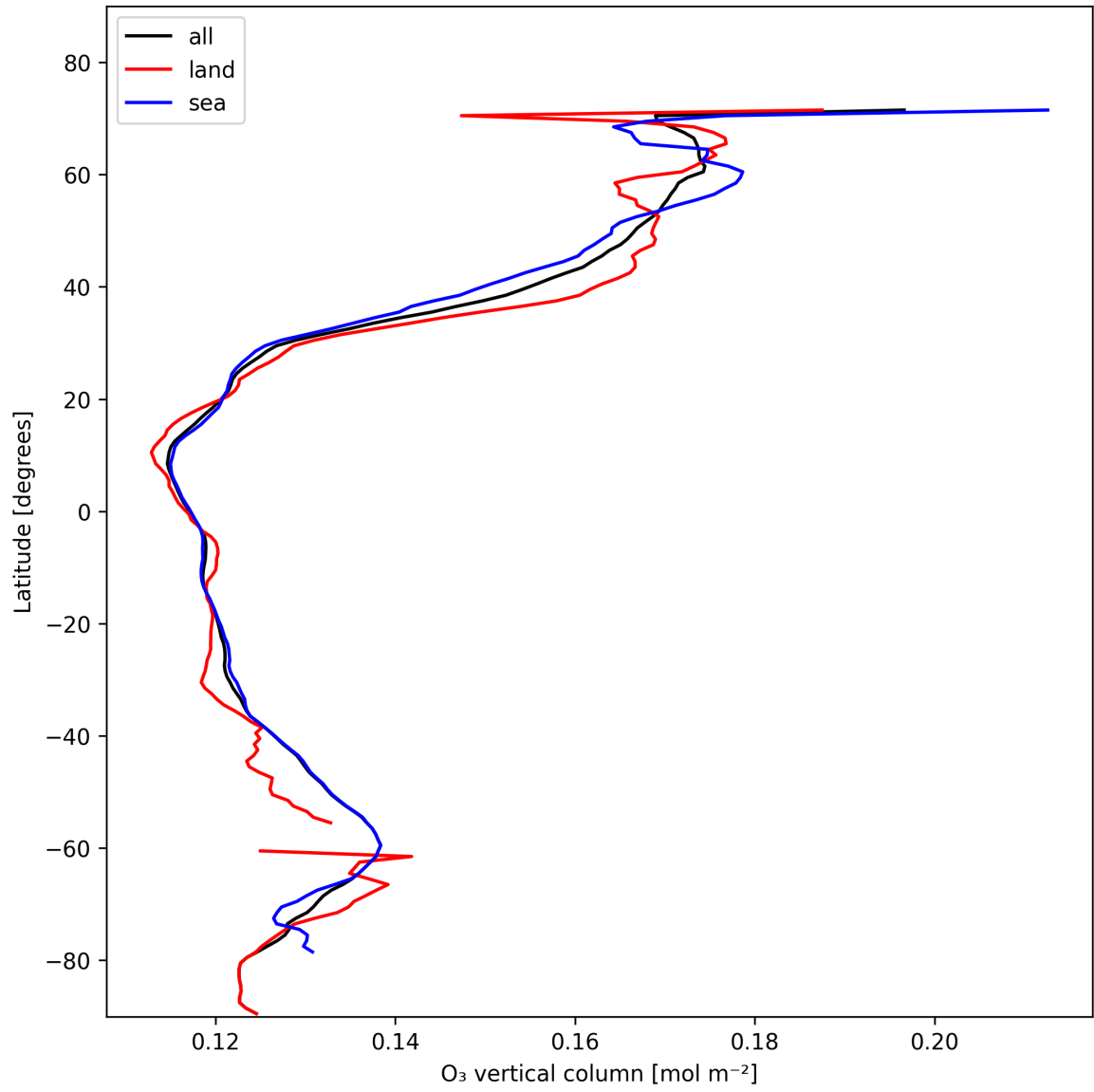
Figure 14: Zonal average of “O 3 vertical column” for 2025-01-28 to 2025-01-29.
