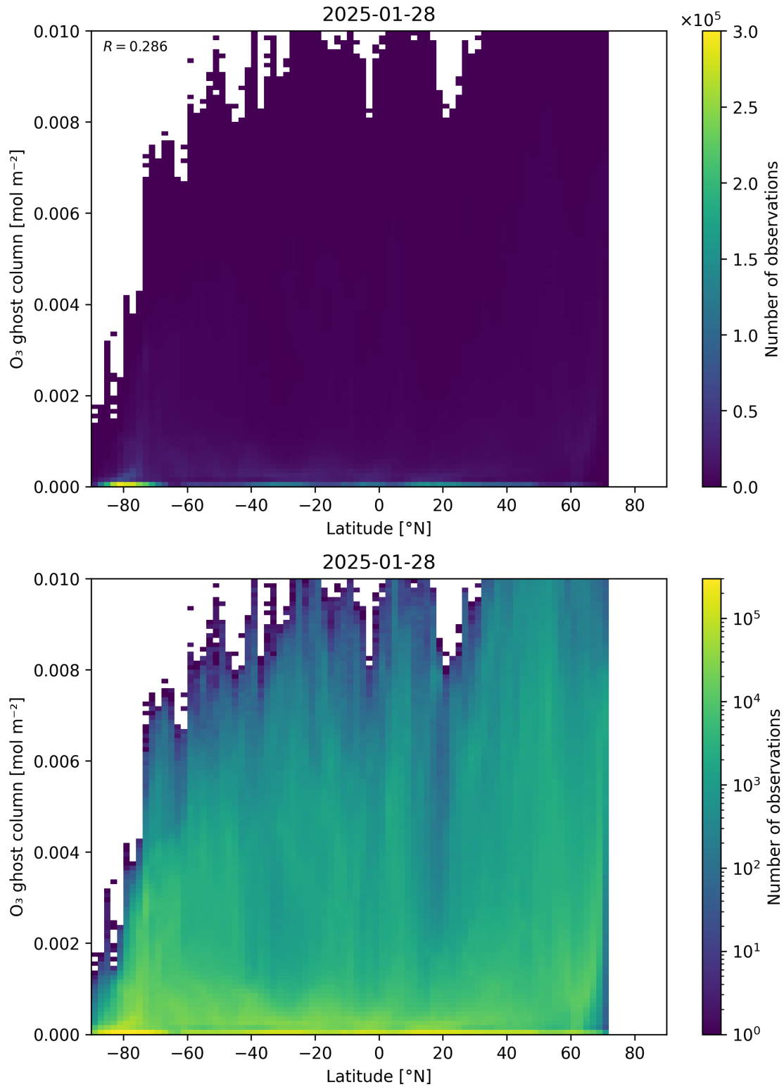
Figure 35: Scatter density plot of “Latitude” against “O 3 ghost column” for 2025-01-28 to 2025-01-29.
