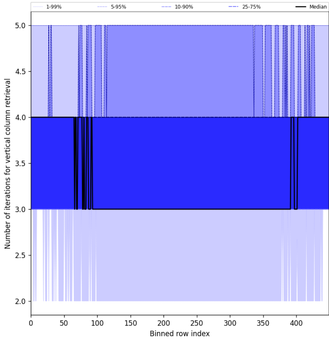
Figure 33: Along track statistics of “Number of iterations for vertical column retrieval” for 2025-01-28 to 2025-01-29
