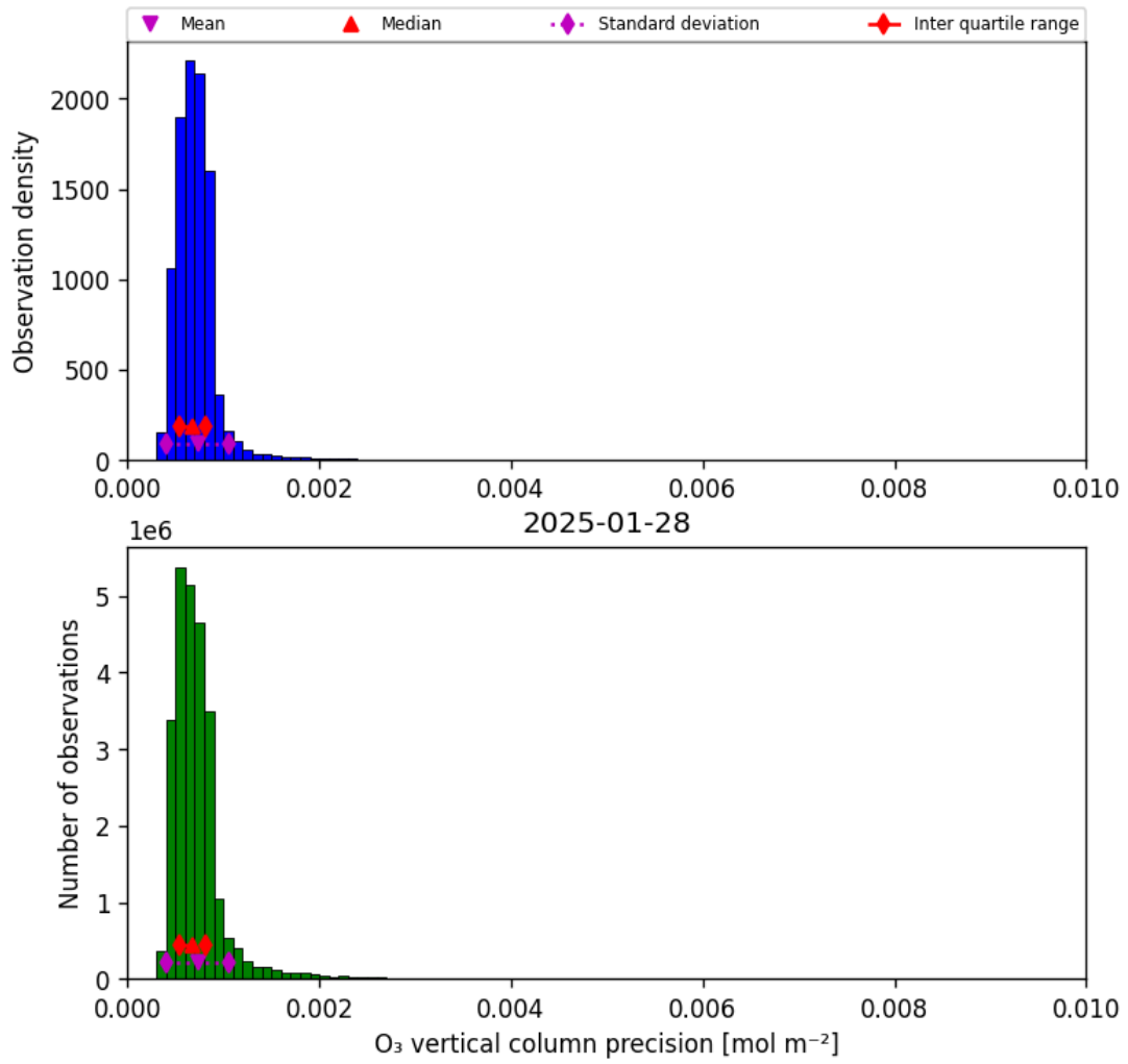
Figure 22: Histogram of “O 3 vertical column precision” for 2025-01-28 to 2025-01-29
