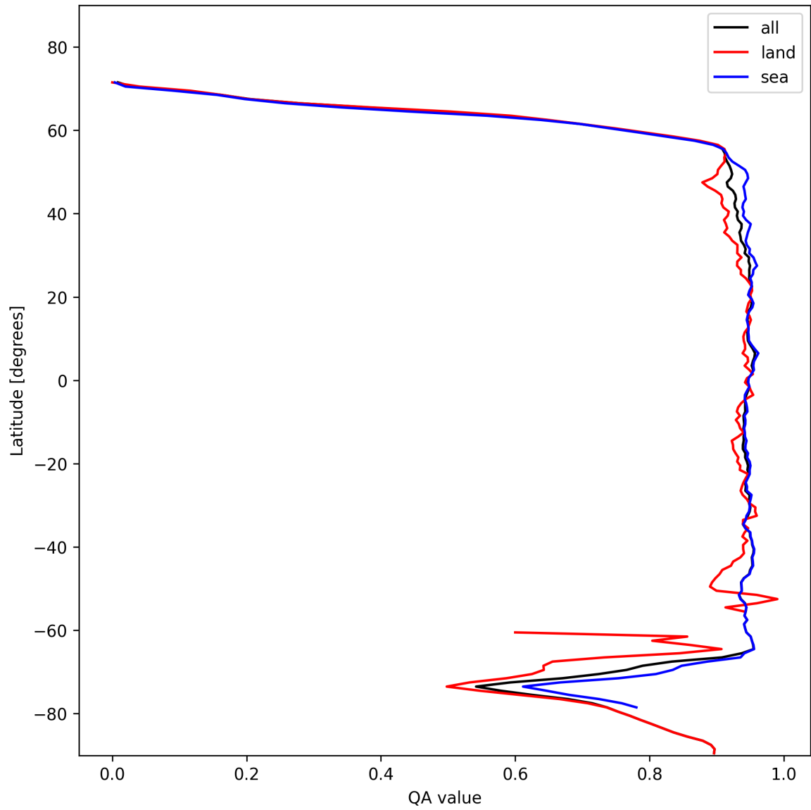
Figure 13: Zonal average of “QA value” for 2025-01-28 to 2025-01-29.
