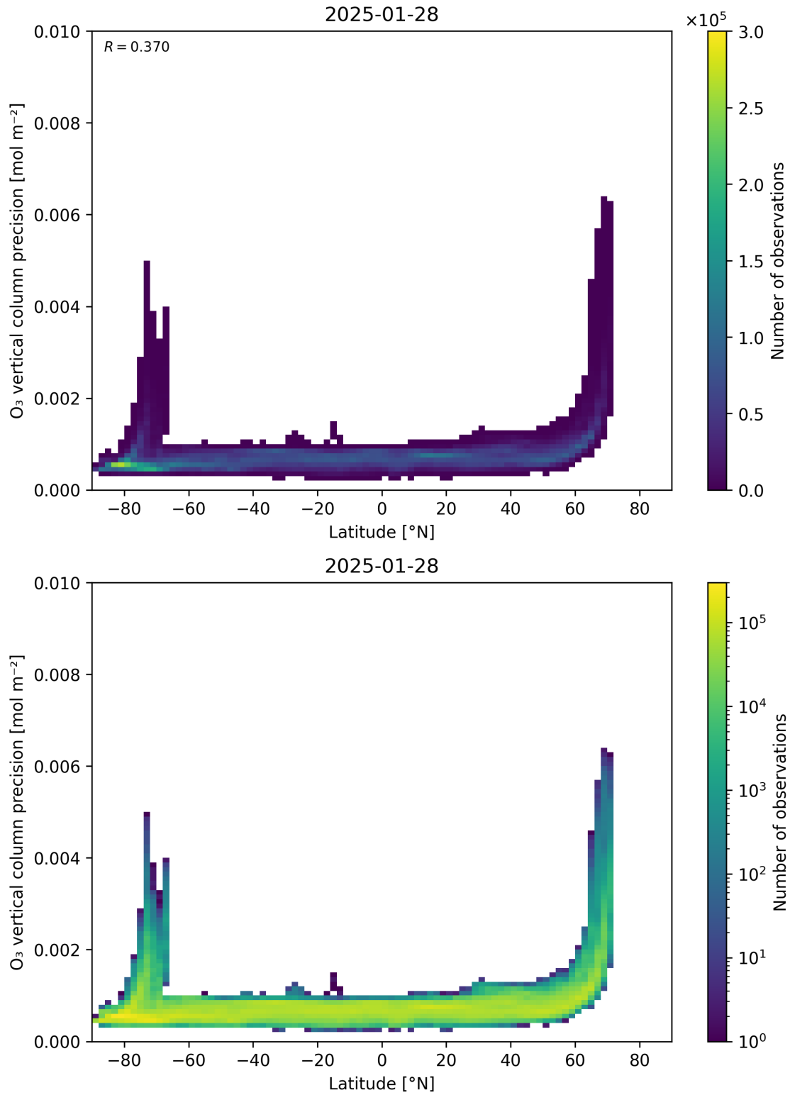
Figure 37: Scatter density plot of “Latitude” against “O 3 vertical column precision” for 2025-01-28 to 2025-01-29.
