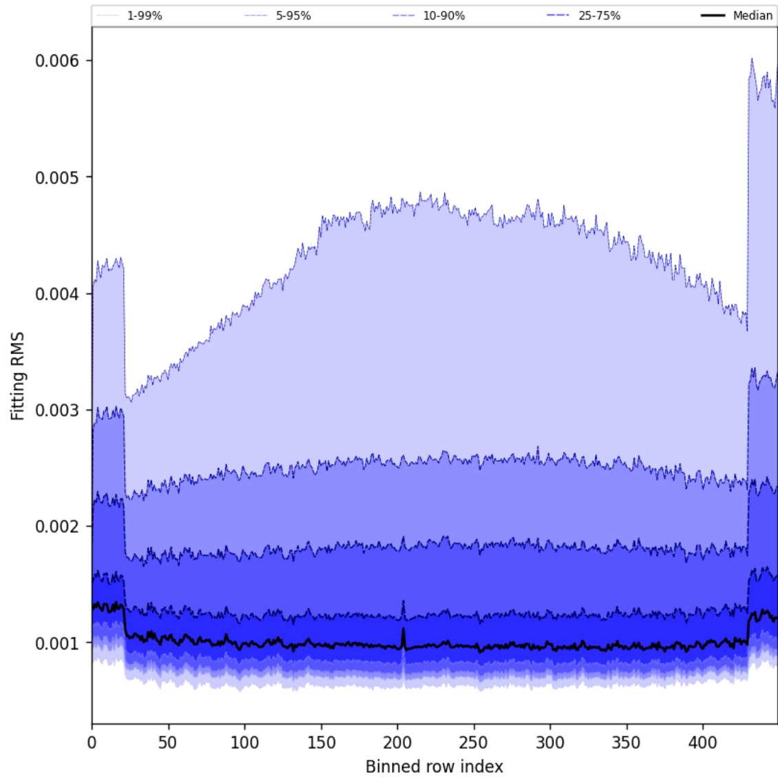
Figure 30: Along track statistics of “Fitting RMS” for 2025-01-28 to 2025-01-29
