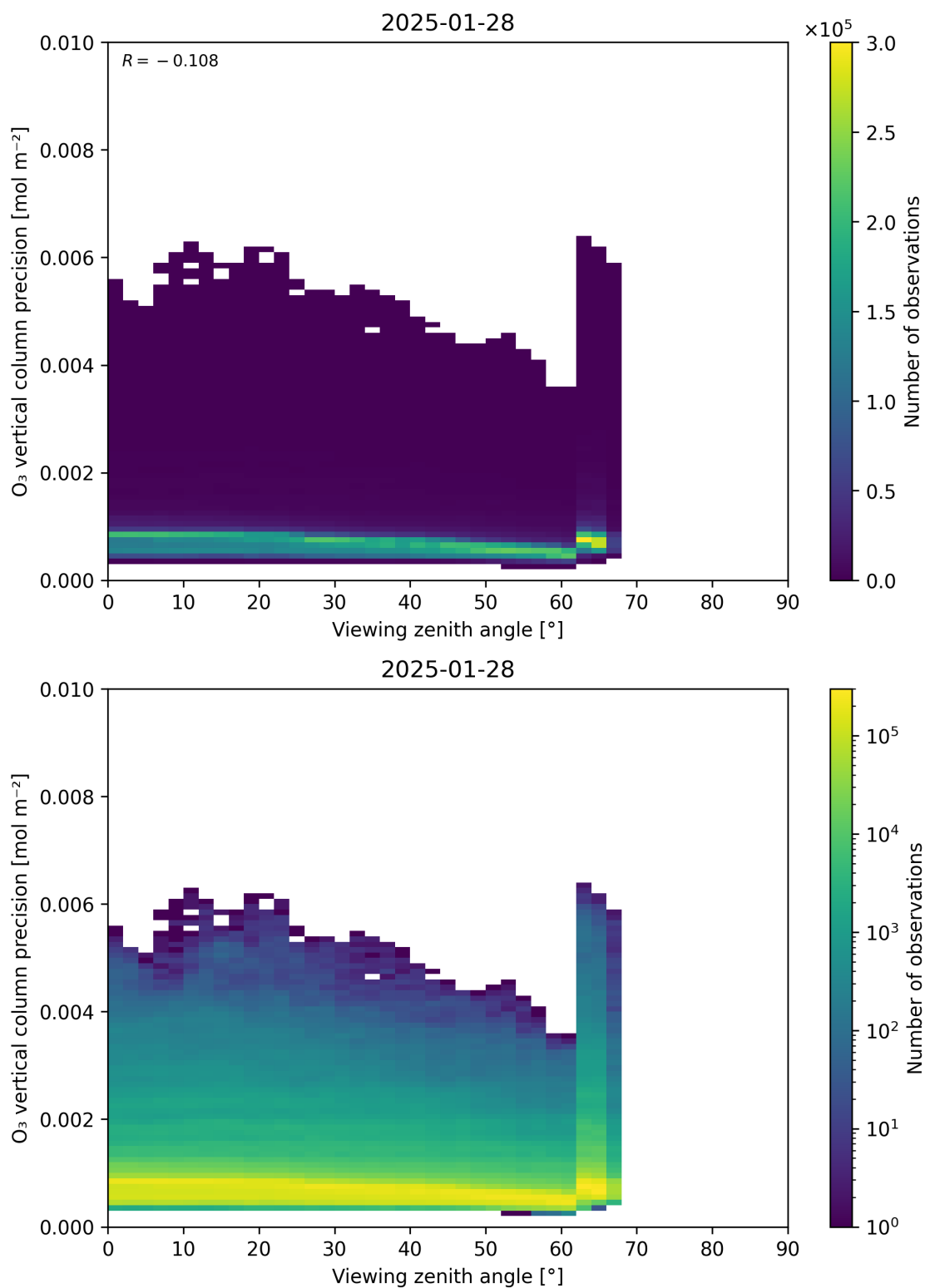
Figure 53: Scatter density plot of “Viewing zenith angle” against “O 3 vertical column precision” for 2025-01-28 to 2025-01-29.
