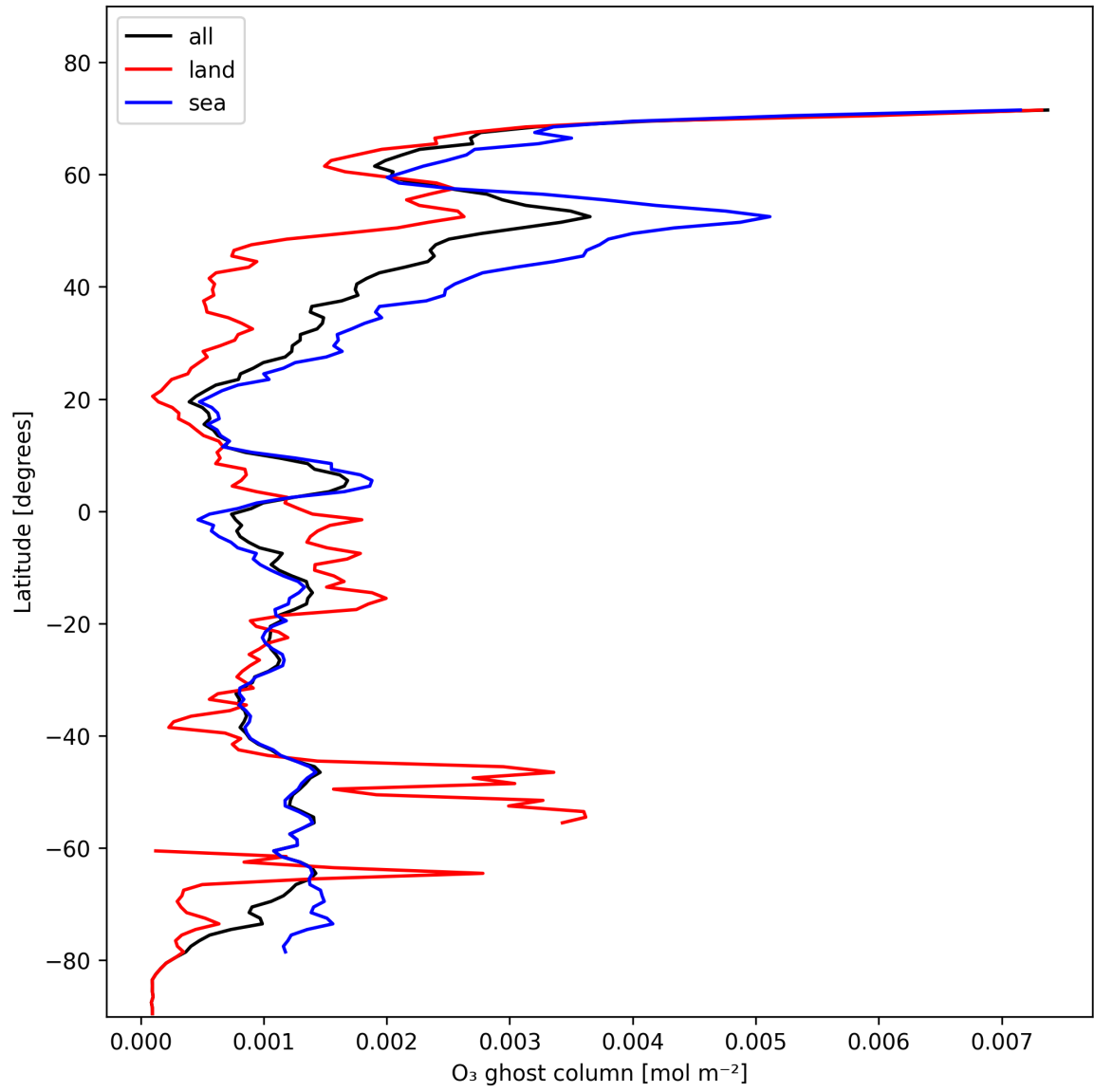
Figure 18: Zonal average of "O 3 ghost column" for 2025-01-28 to 2025-01-29.
