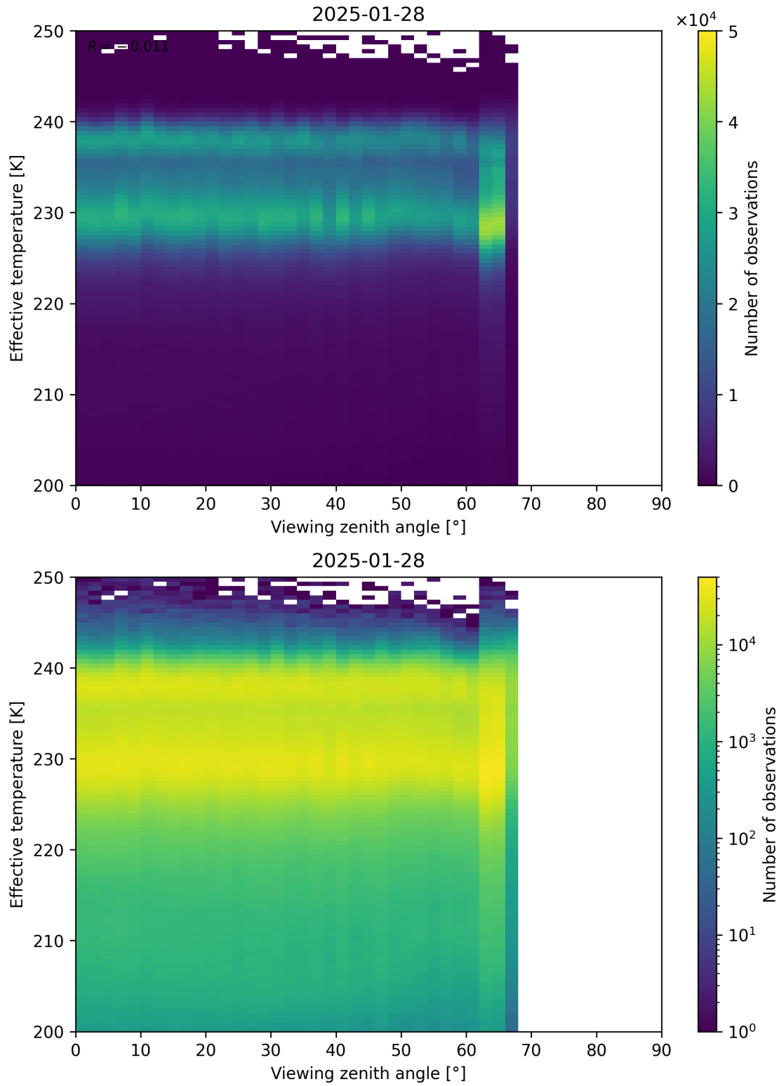
Figure 50: Scatter density plot of “Viewing zenith angle” against “Effective temperature” for 2025-01-28 to 2025-01-29.
