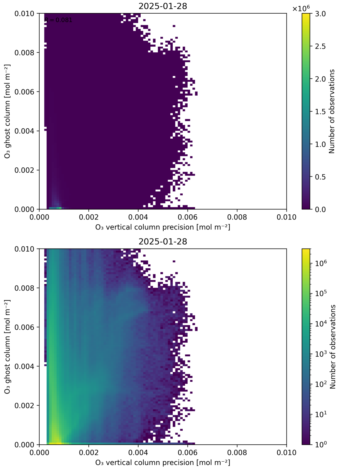
Figure 43: Scatter density plot of “O 3 vertical column precision” against “O 3 ghost column” for 2025-01-28 to 2025-01-29.
