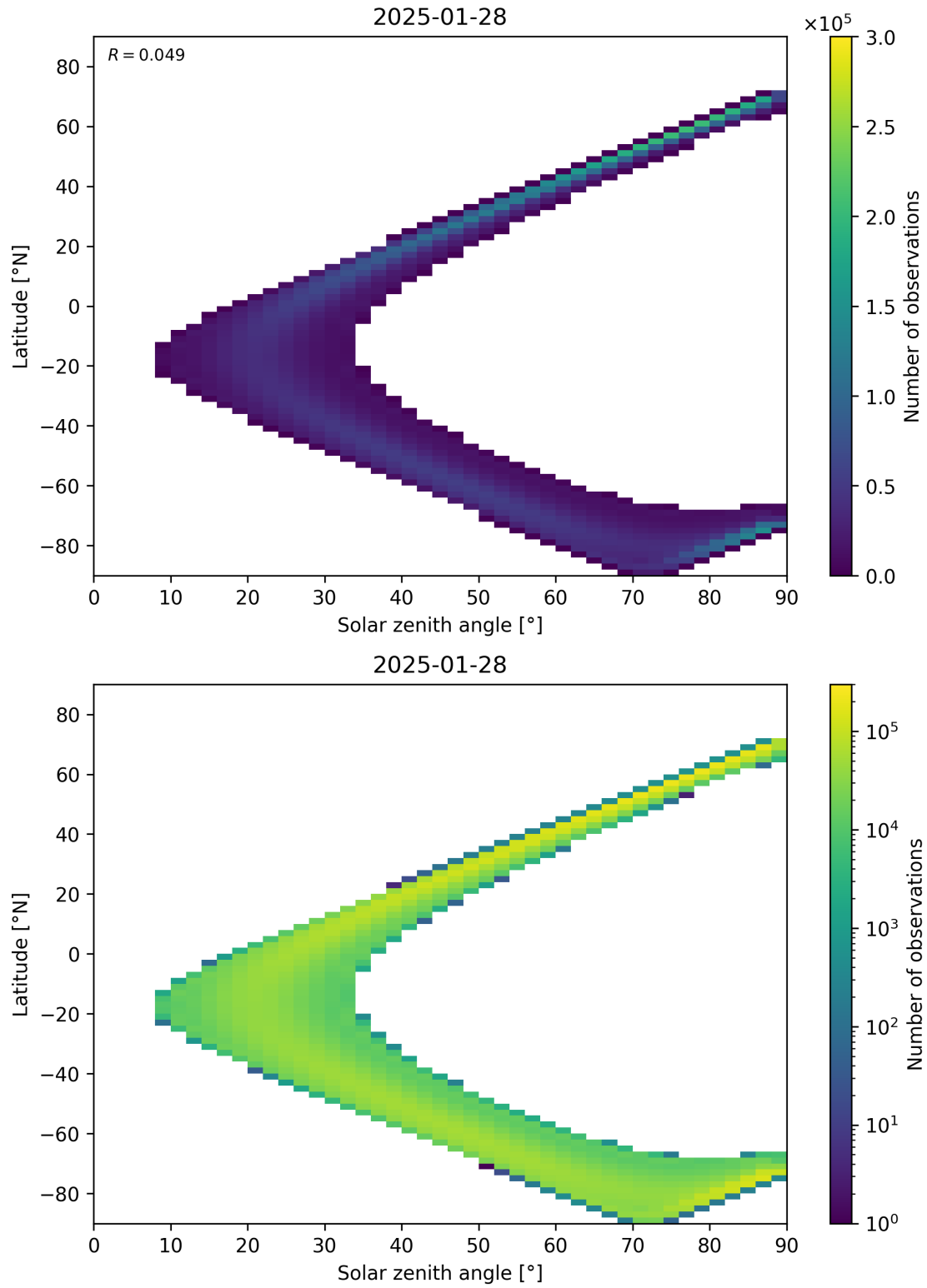
Figure 44: Scatter density plot of “Solar zenith angle” against “Latitude” for 2025-01-28 to 2025-01-29.
