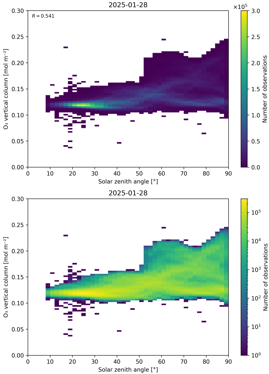
Figure 47: Scatter density plot of “Solar zenith angle” against “O 3 vertical column” for 2025-01-28 to 2025-01-29.
