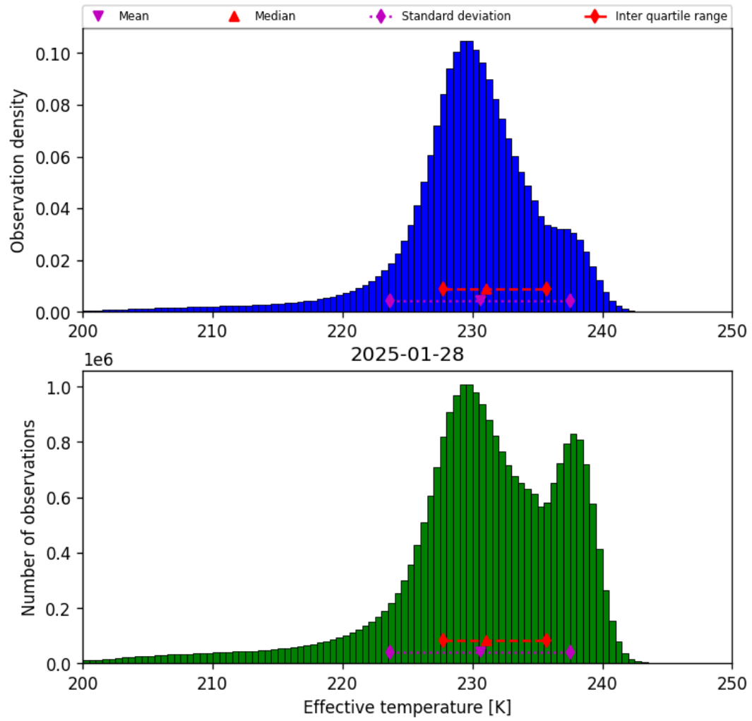
Figure 24: Histogram of “Effective temperature” for 2025-01-28 to 2025-01-29
