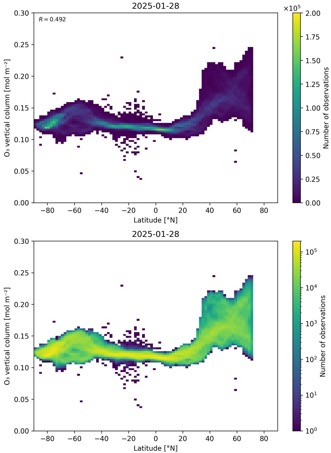
Figure 36: Scatter density plot of “Latitude” against “O 3 vertical column” for 2025-01-28 to 2025-01-29.
