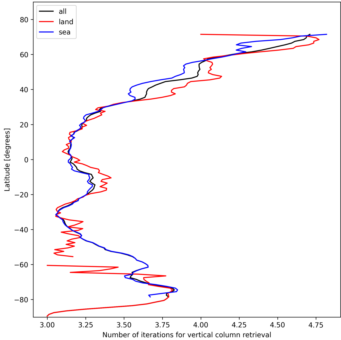
Figure 19: Zonal average of “Number of iterations for vertical column retrieval” for 2025-01-28 to 2025-01-29.
