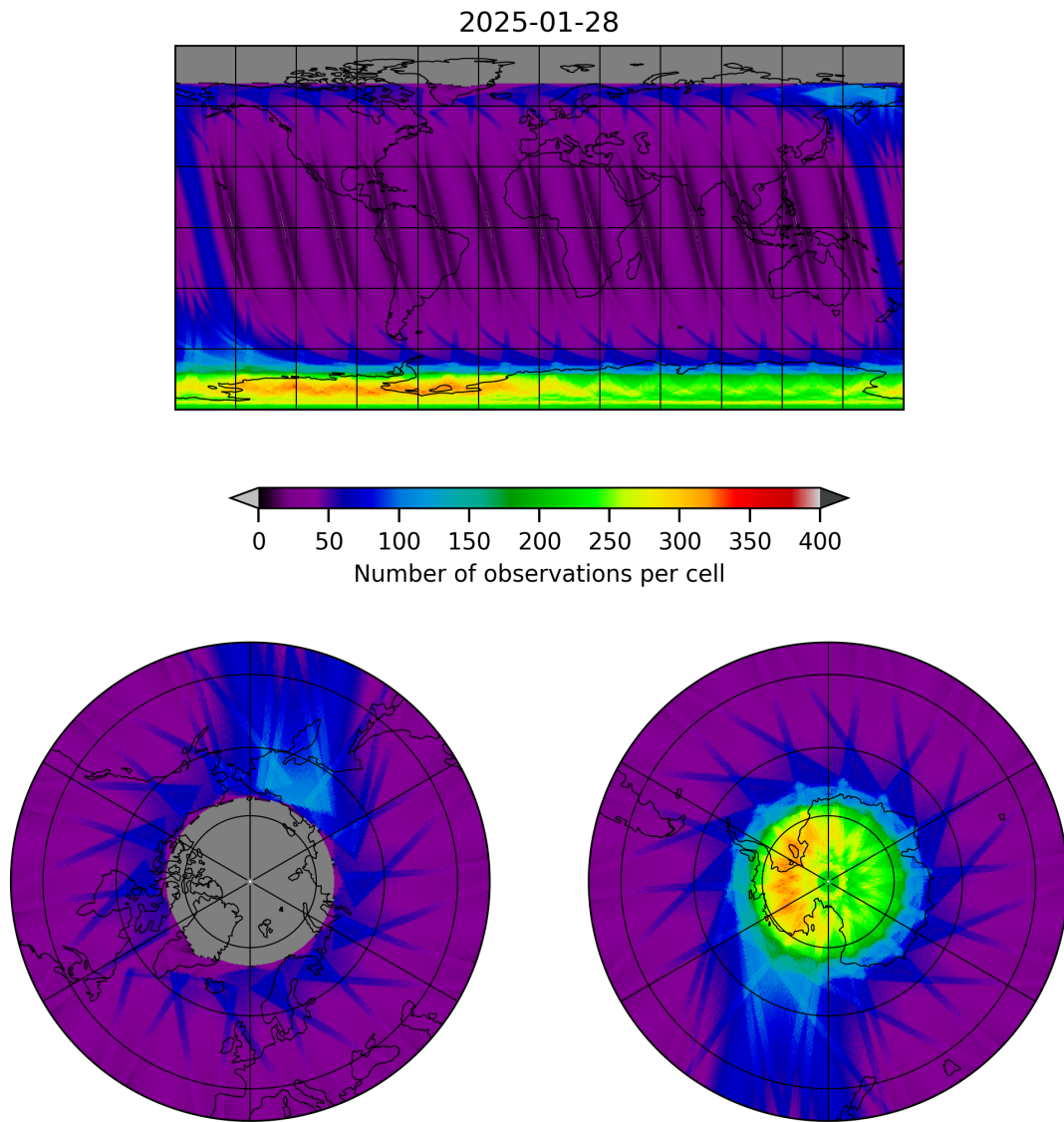
Figure 12: Map of the number of observations for 2025-01-28 to 2025-01-29
