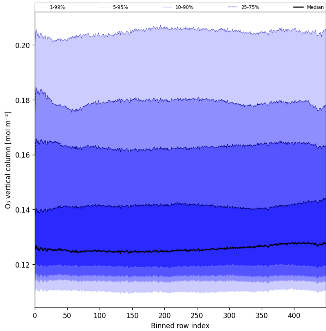
Figure 28: Along track statistics of “O 3 vertical column” for 2025-01-28 to 2025-01-29
