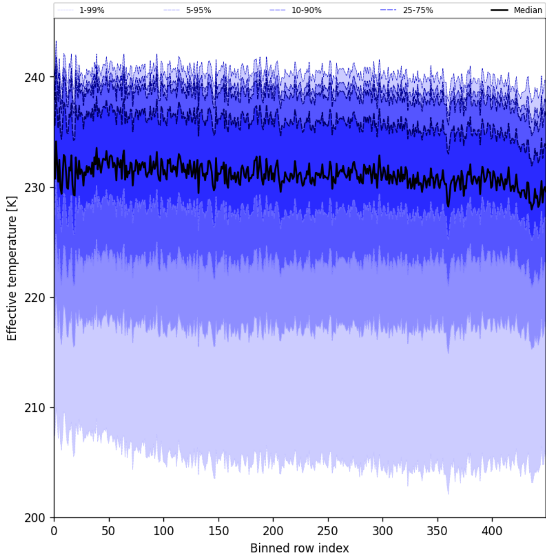
Figure 31: Along track statistics of “Effective temperature” for 2025-01-28 to 2025-01-29
