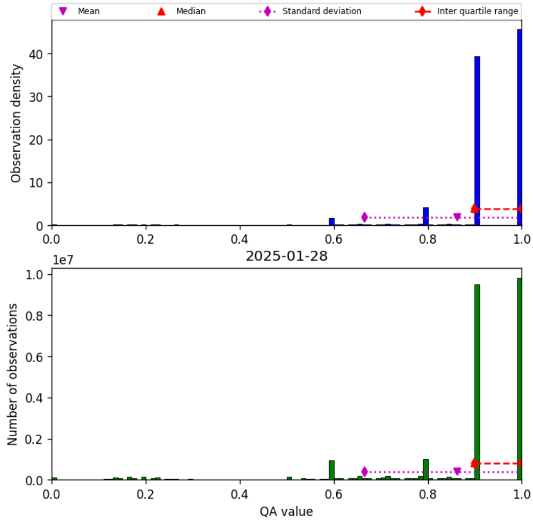
Figure 20: Histogram of “QA value” for 2025-01-28 to 2025-01-29
