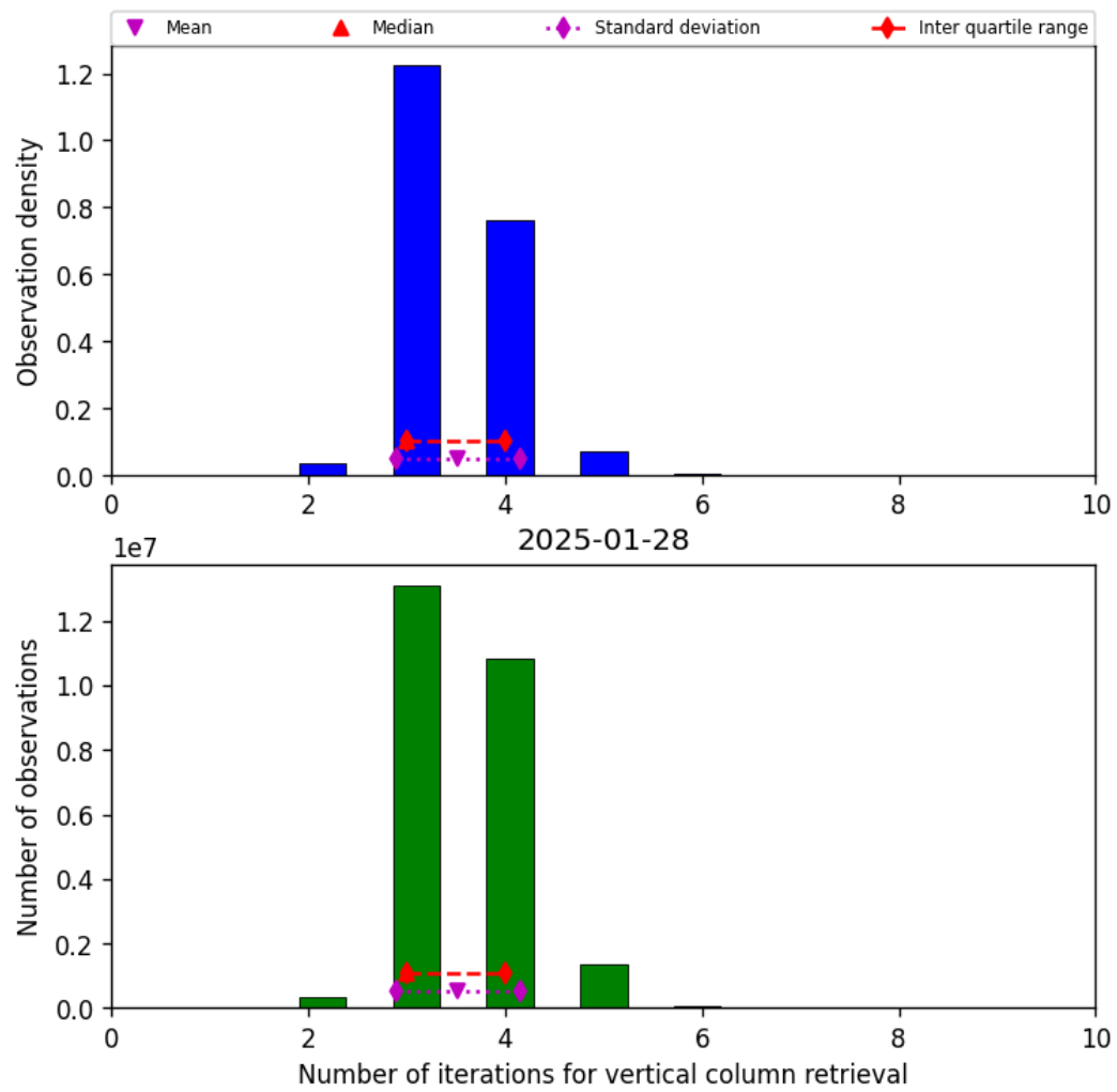
Figure 26: Histogram of “Number of iterations for vertical column retrieval” for 2025-01-28 to 2025-01-29
