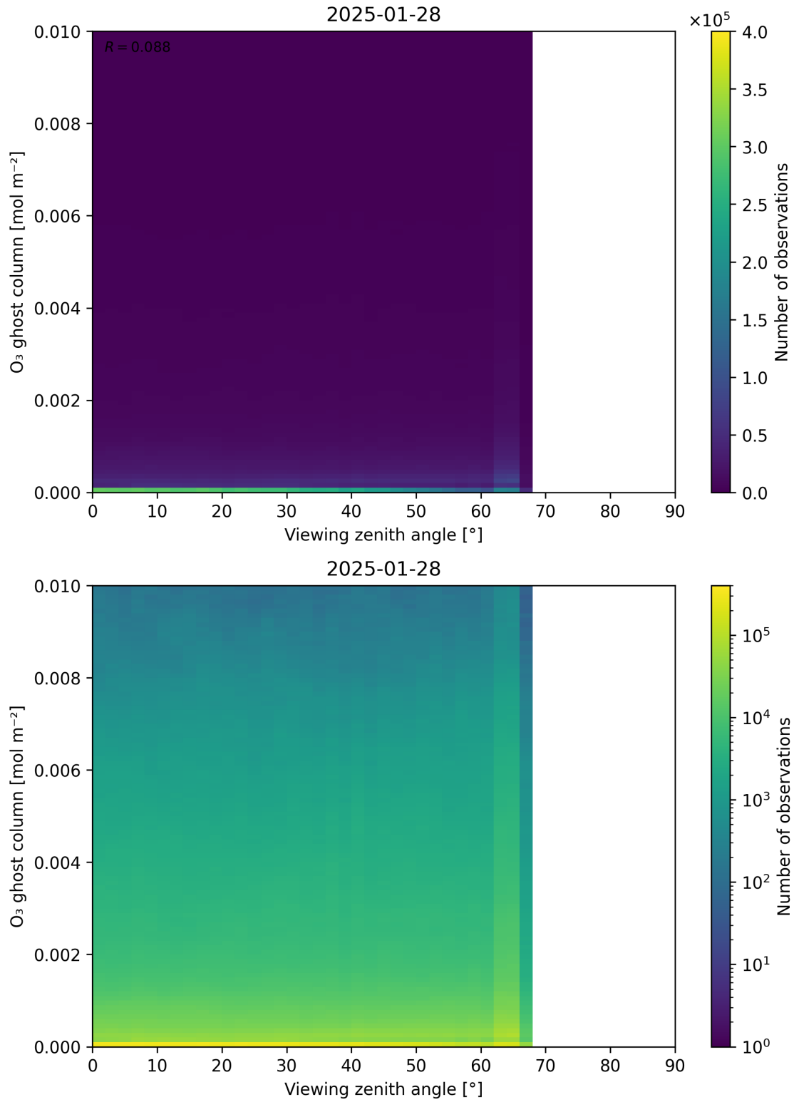
Figure 51: Scatter density plot of “Viewing zenith angle” against “O 3 ghost column” for 2025-01-28 to 2025-01-29.
