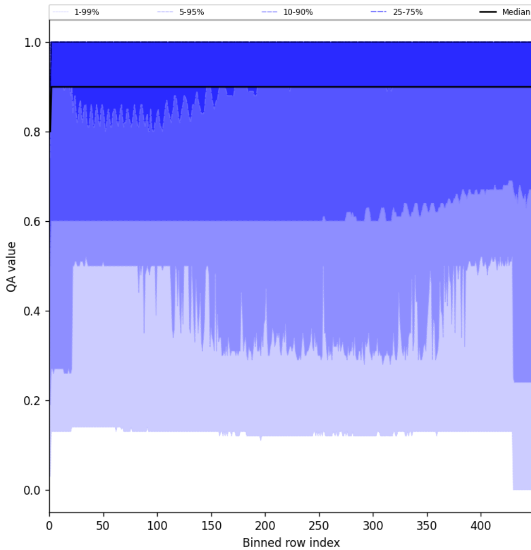
Figure 27: Along track statistics of “QA value” for 2025-01-28 to 2025-01-29
