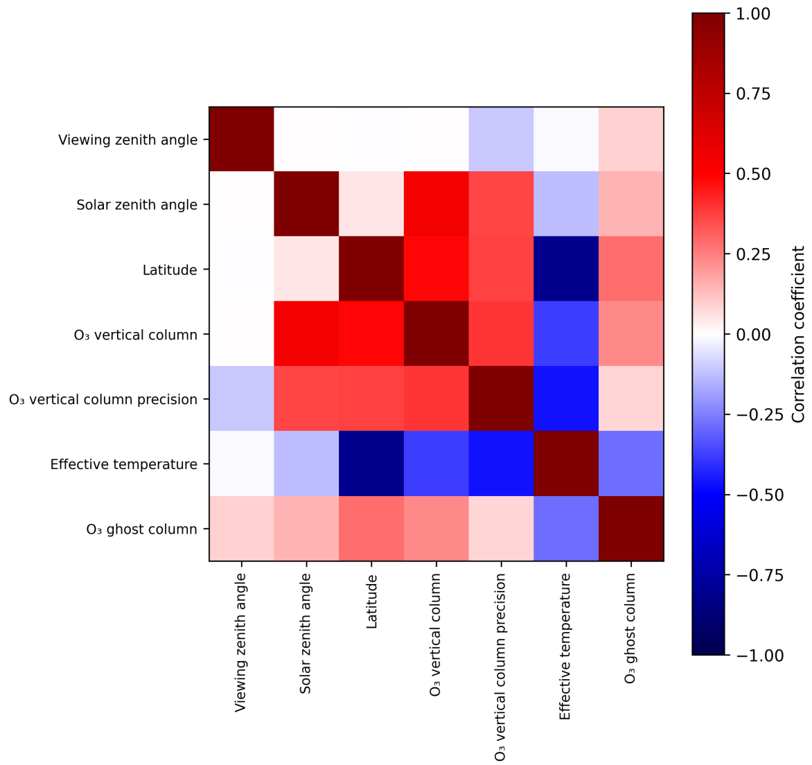
Figure 2: Map of correlation matrix for 2025-01-28 to 2025-01-29.
