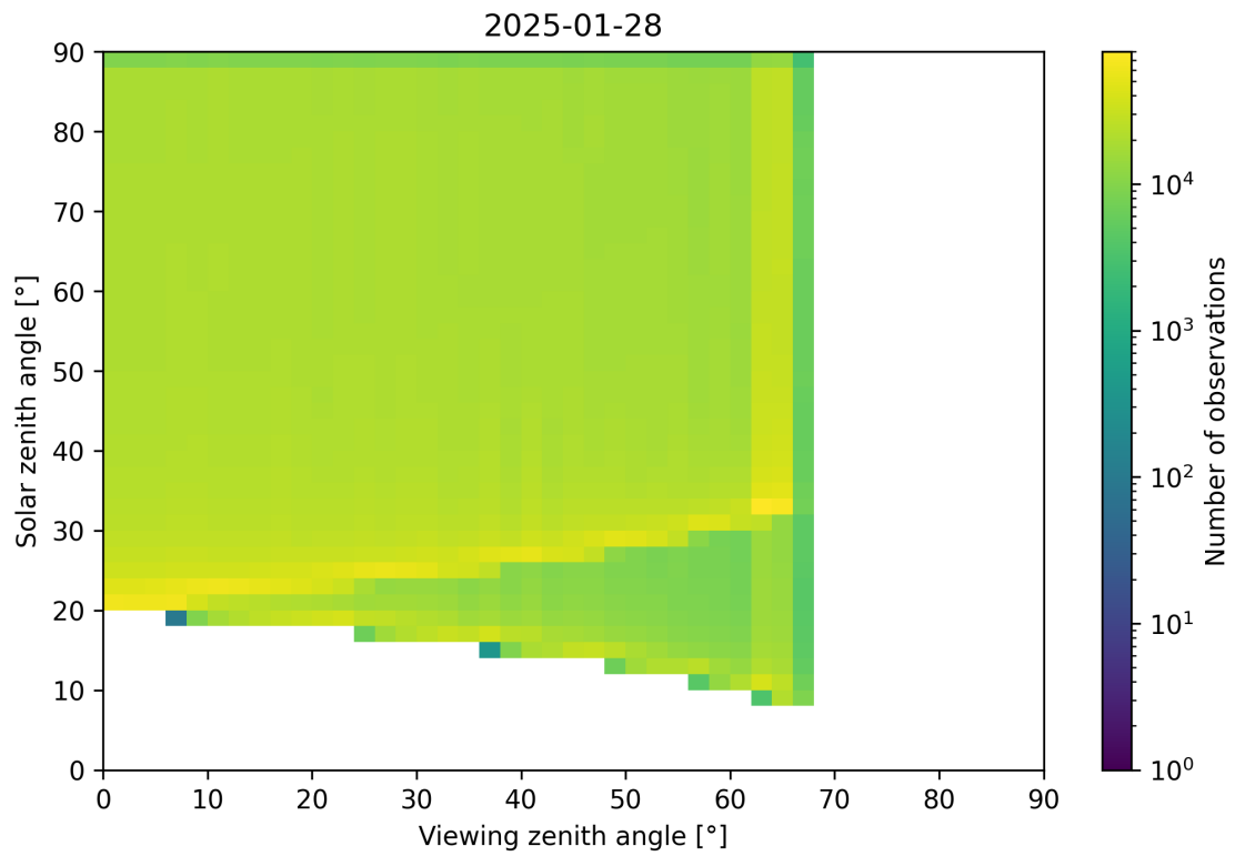
Figure 54: Scatter density plot of “Viewing zenith angle” against “Solar zenith angle” for 2025-01-28 to 2025-01-29.
