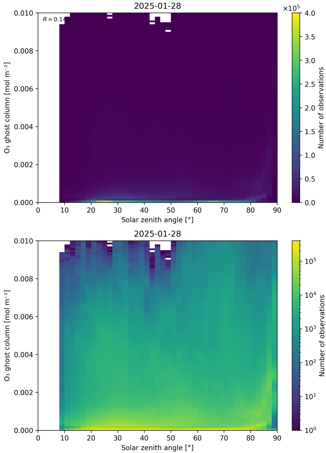
Figure 46: Scatter density plot of “Solar zenith angle” against “O 3 ghost column” for 2025-01-28 to 2025-01-29.
