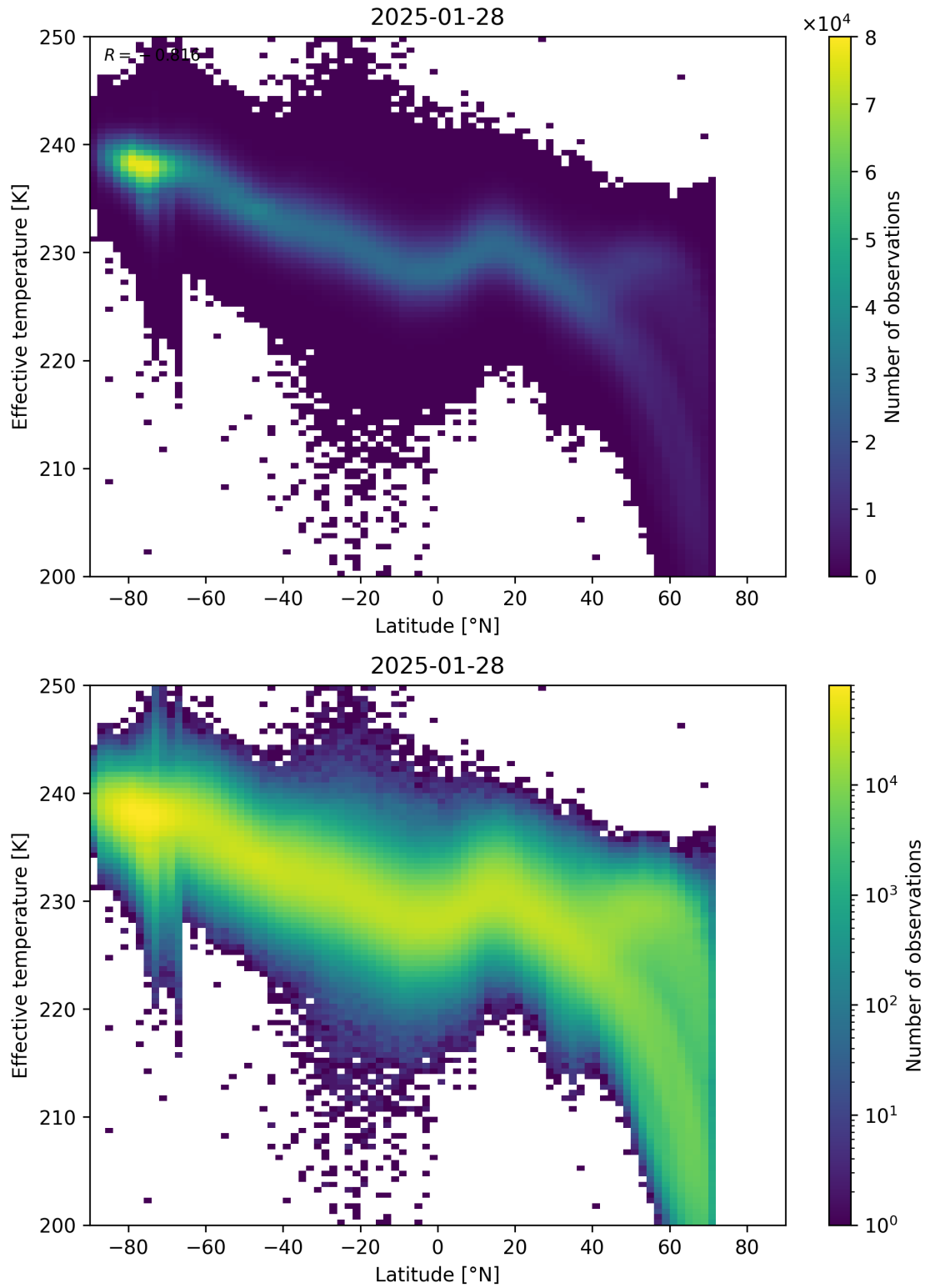
Figure 34: Scatter density plot of “Latitude” against “Effective temperature” for 2025-01-28 to 2025-01-29.
