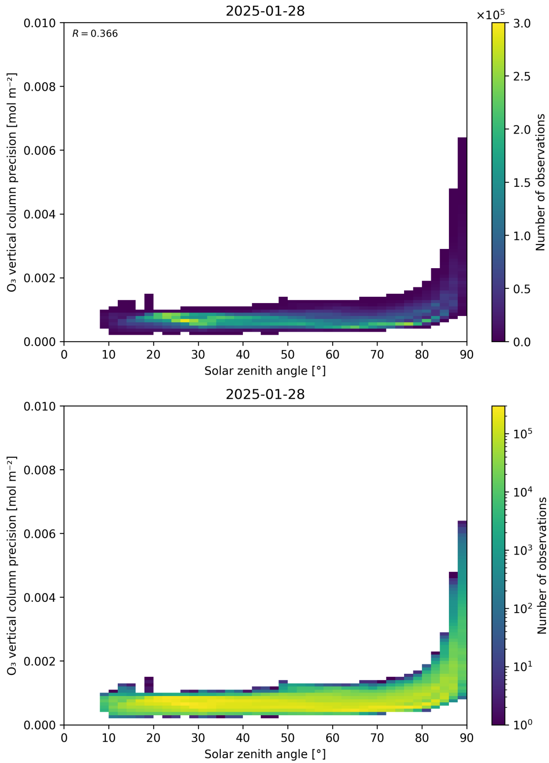
Figure 48: Scatter density plot of “Solar zenith angle” against “O 3 vertical column precision” for 2025-01-28 to 2025-01-29.
