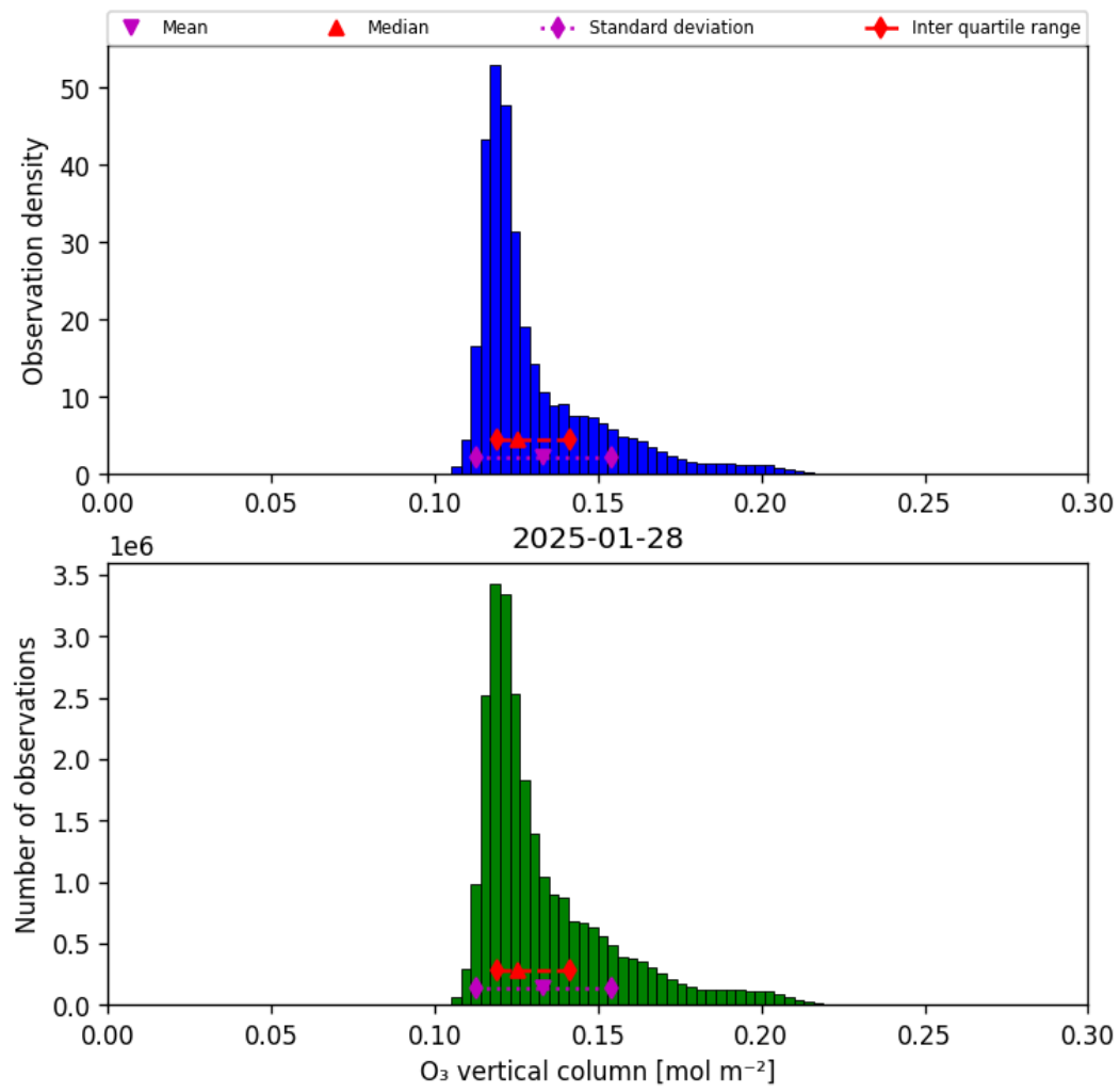
Figure 21: Histogram of “O 3 vertical column” for 2025-01-28 to 2025-01-29
