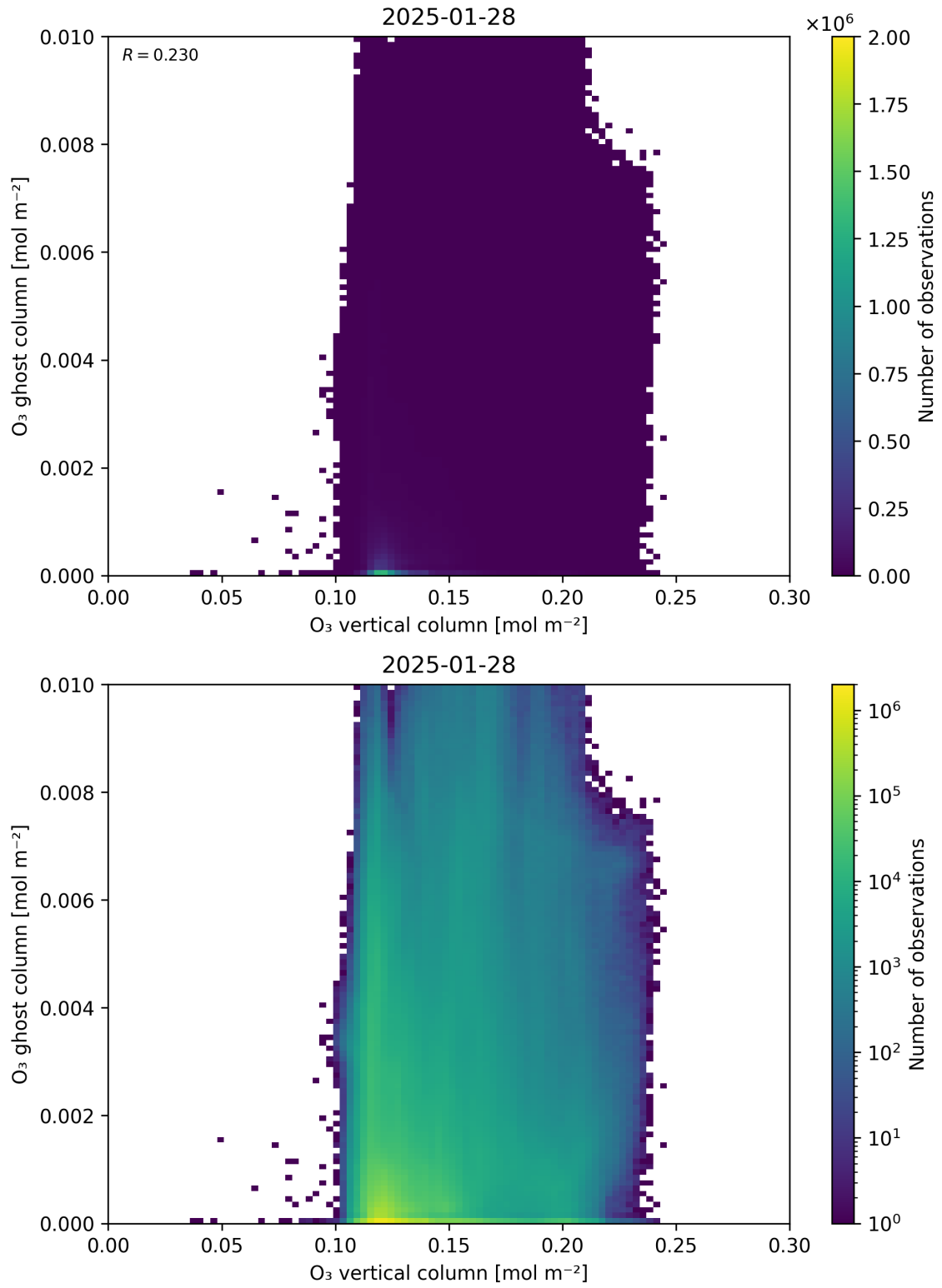
Figure 40: Scatter density plot of “O 3 vertical column” against “O 3 ghost column” for 2025-01-28 to 2025-01-29.
