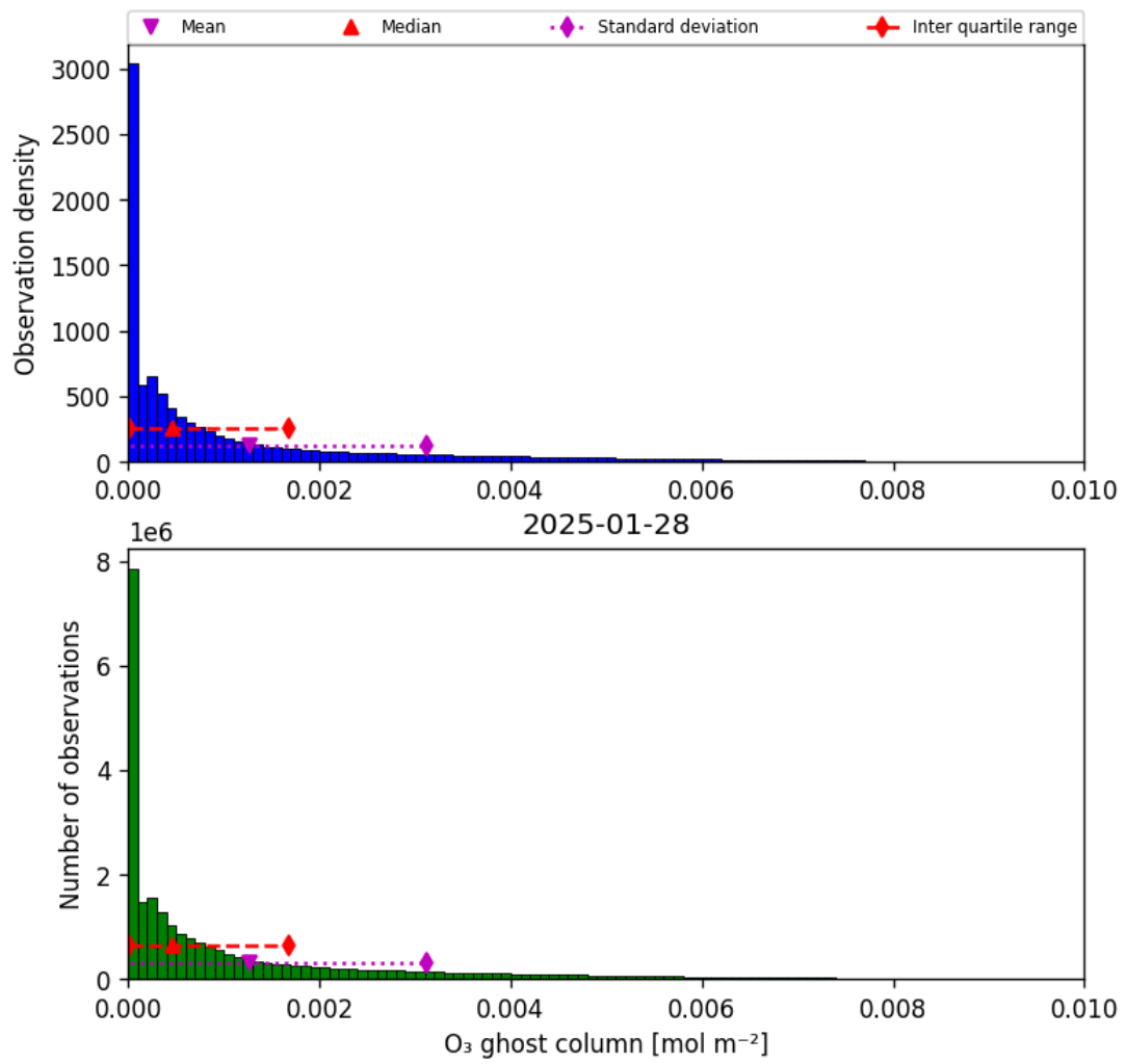
Figure 25: Histogram of “O 3 ghost column” for 2025-01-28 to 2025-01-29
