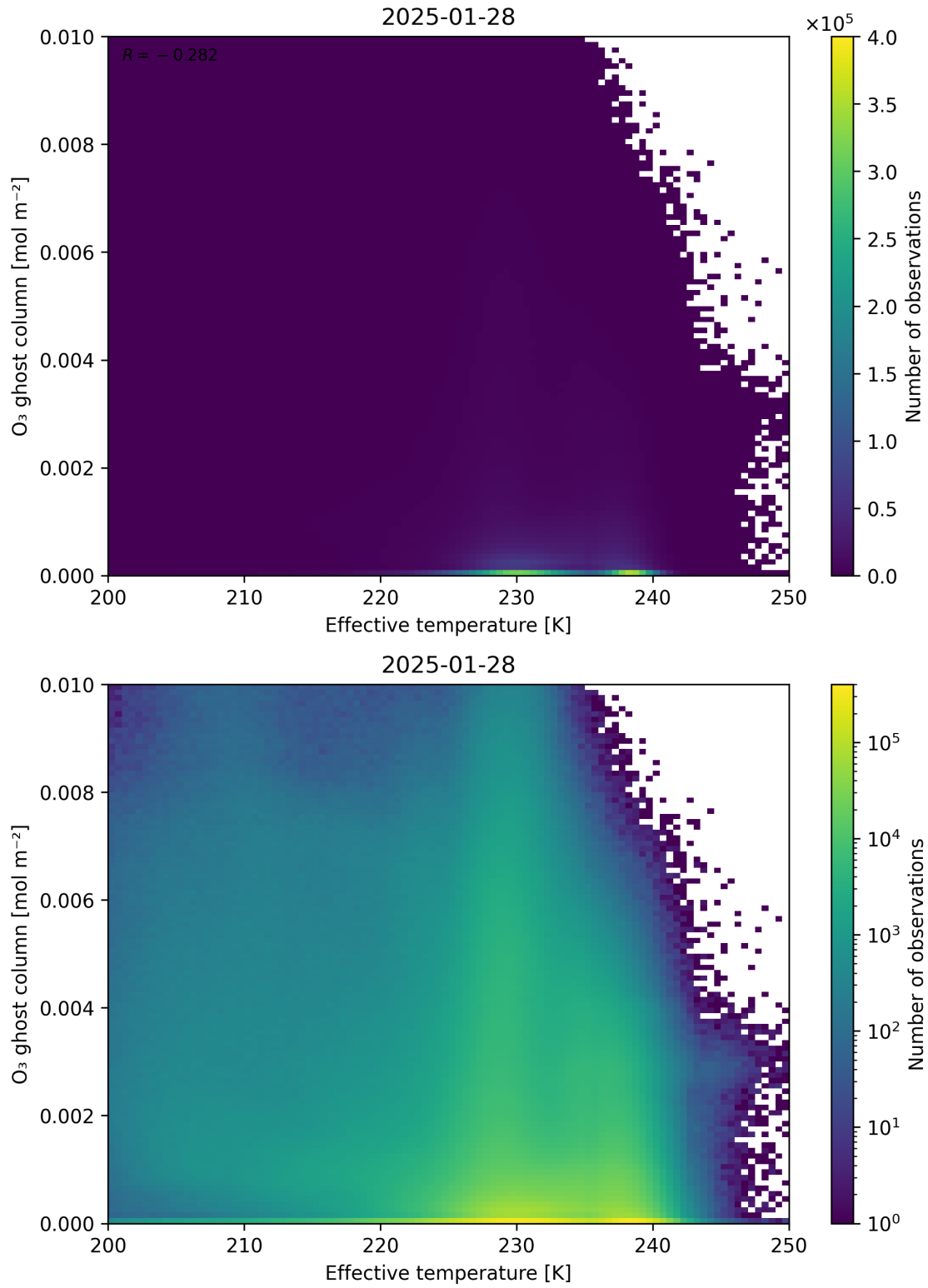
Figure 38: Scatter density plot of “Effective temperature” against “O 3 ghost column” for 2025-01-28 to 2025-01-29.
