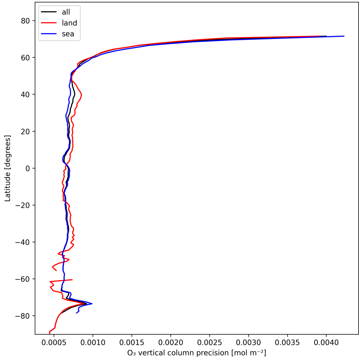
Figure 15: Zonal average of “O 3 vertical column precision” for 2025-01-28 to 2025-01-29.
