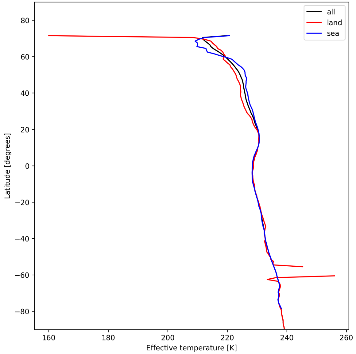
Figure 17: Zonal average of “Effective temperature” for 2025-01-28 to 2025-01-29.
