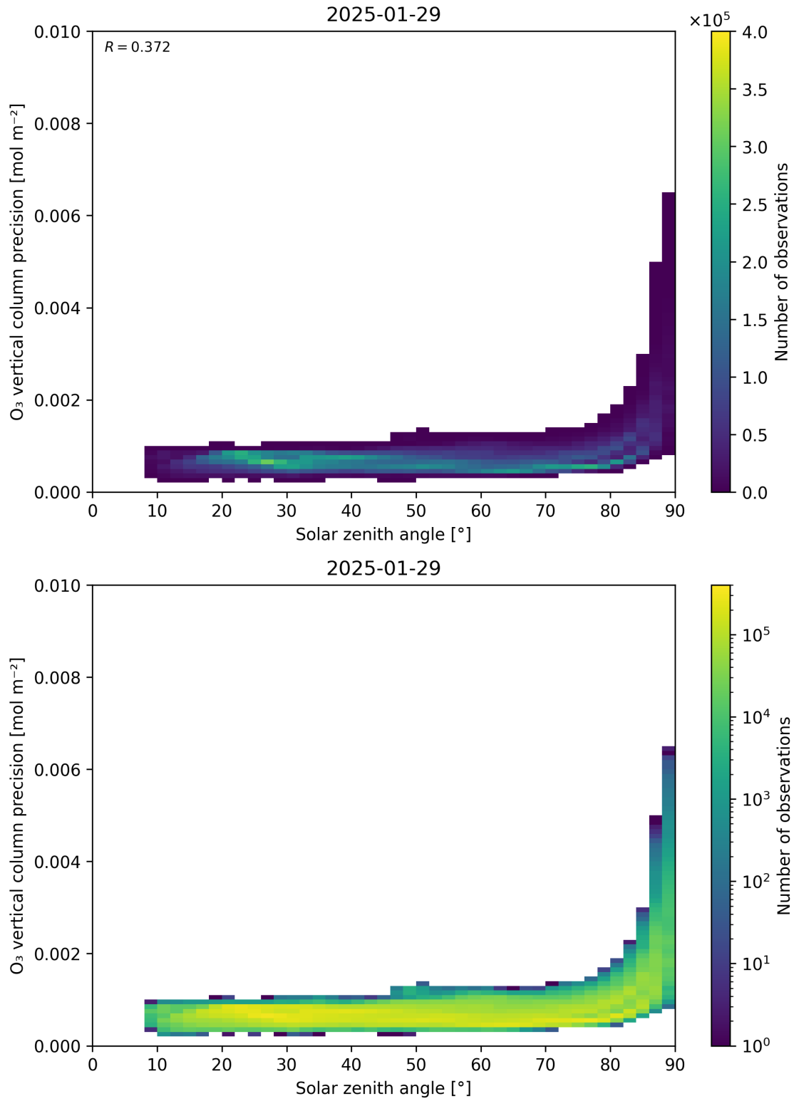
Figure 48: Scatter density plot of “Solar zenith angle” against “O 3 vertical column precision” for 2025-01-28 to 2025-01-30.
