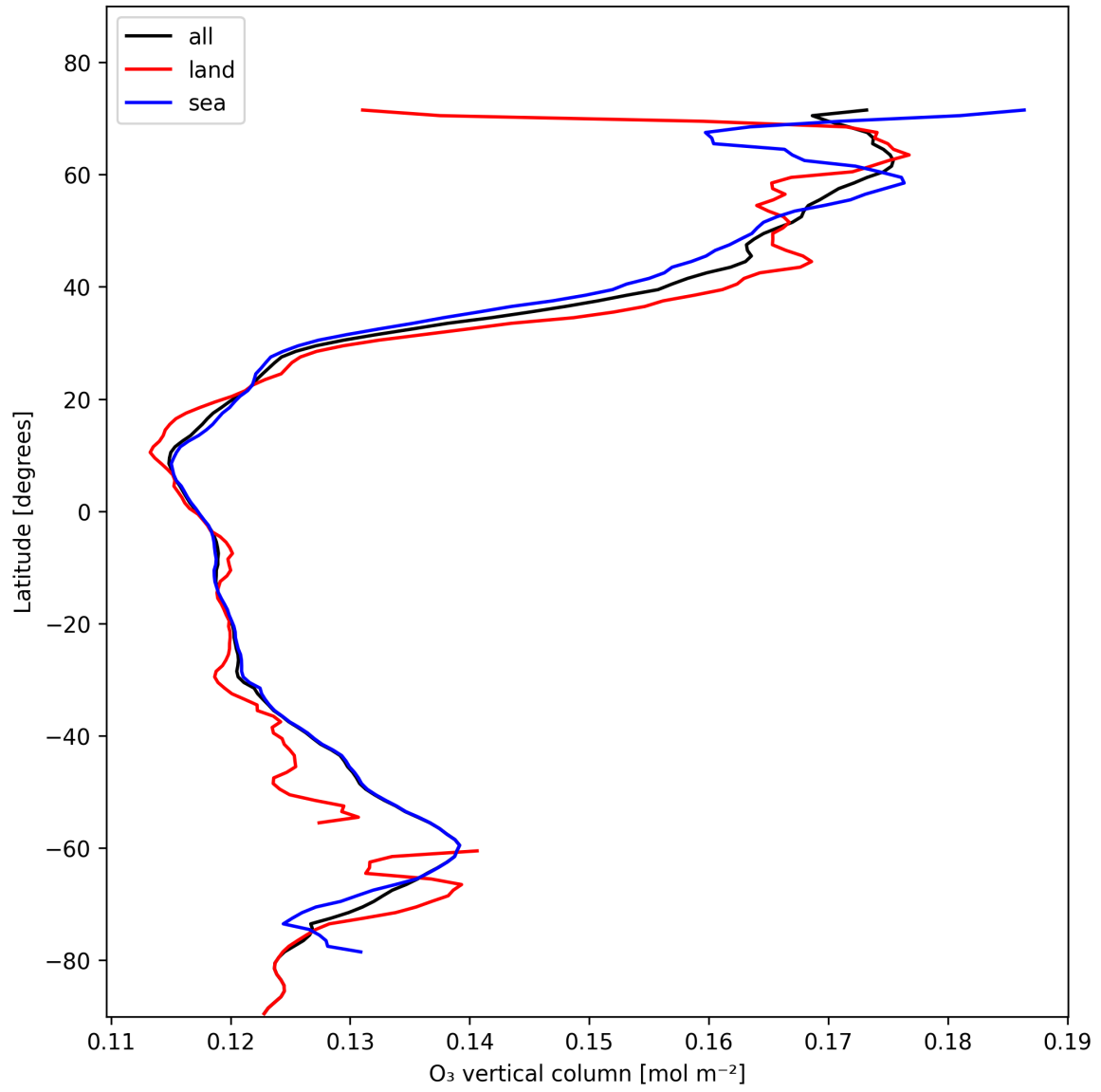
Figure 14: Zonal average of “O 3 vertical column” for 2025-01-28 to 2025-01-30.
