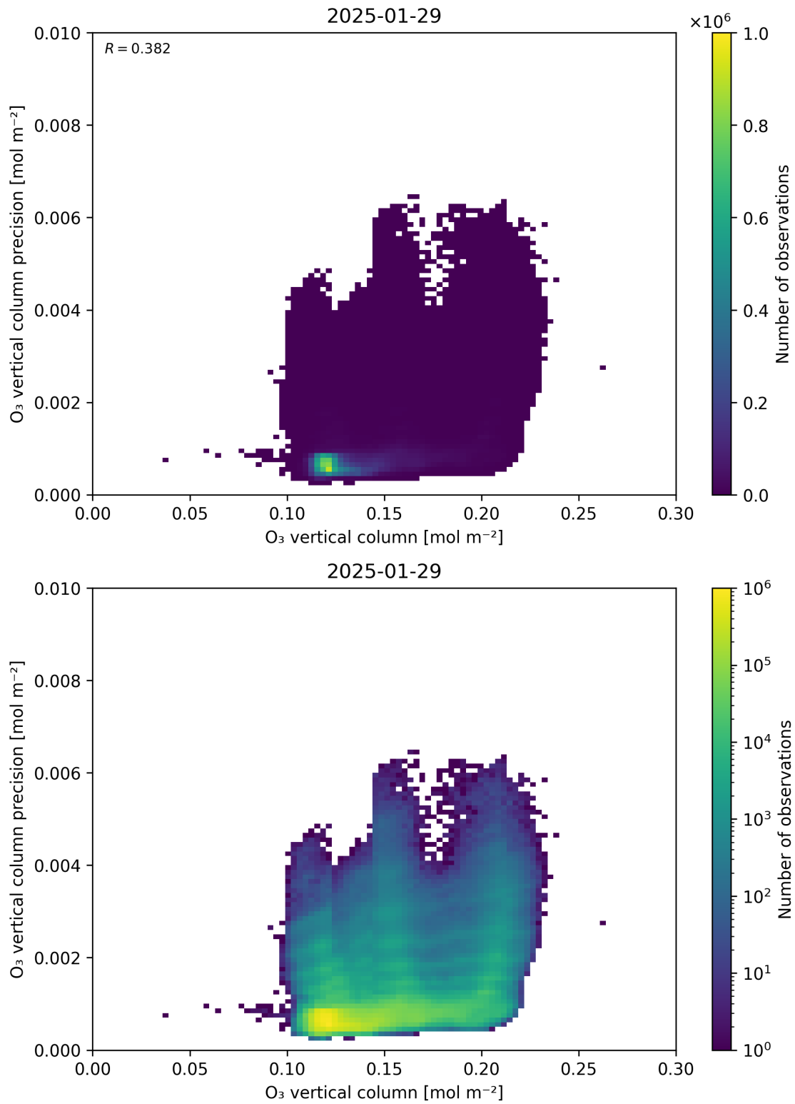
Figure 41: Scatter density plot of “O 3 vertical column” against “O 3 vertical column precision” for 2025-01-28 to 2025-01-30.
