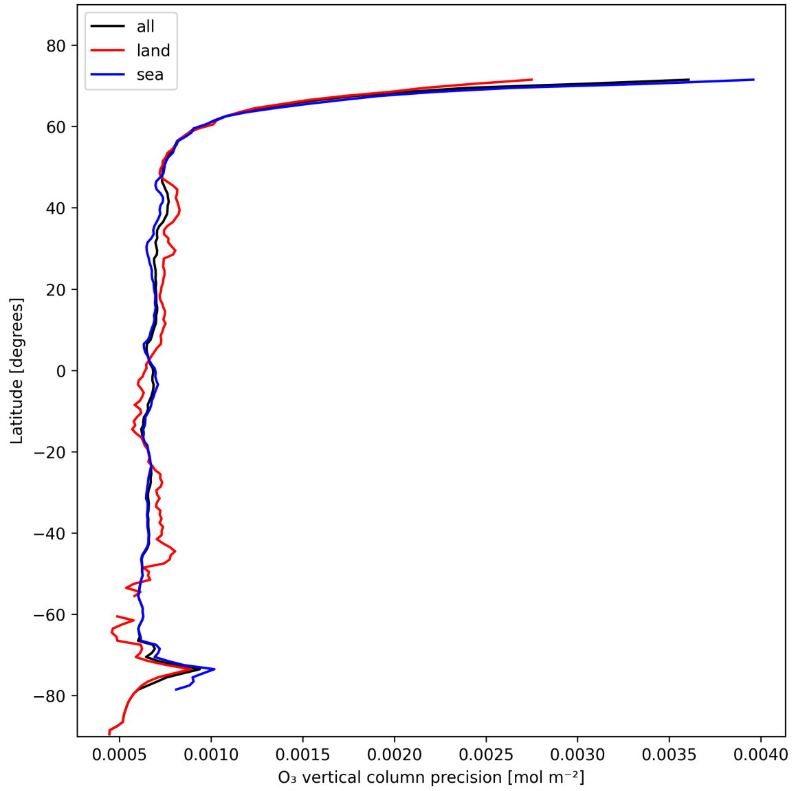
Figure 15: Zonal average of “O 3 vertical column precision” for 2025-01-28 to 2025-01-30.
