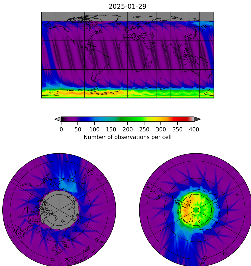
Figure 12: Map of the number of observations for 2025-01-28 to 2025-01-30
