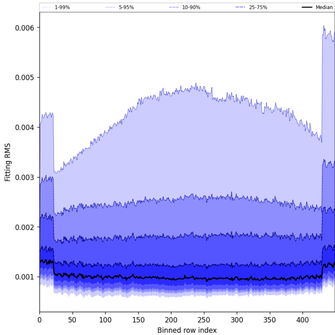
Figure 30: Along track statistics of “Fitting RMS” for 2025-01-28 to 2025-01-30
