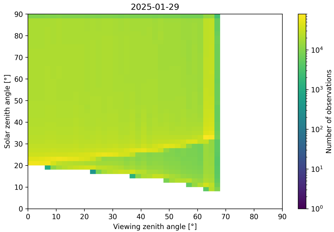
Figure 54: Scatter density plot of “Viewing zenith angle” against “Solar zenith angle” for 2025-01-28 to 2025-01-30.
