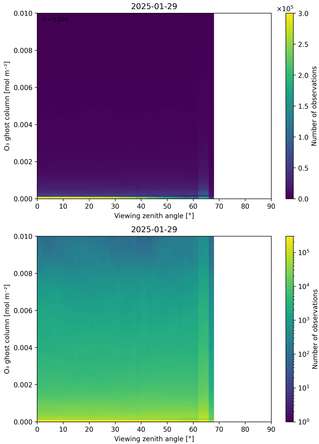
Figure 51: Scatter density plot of “Viewing zenith angle” against “O 3 ghost column” for 2025-01-28 to 2025-01-30.
