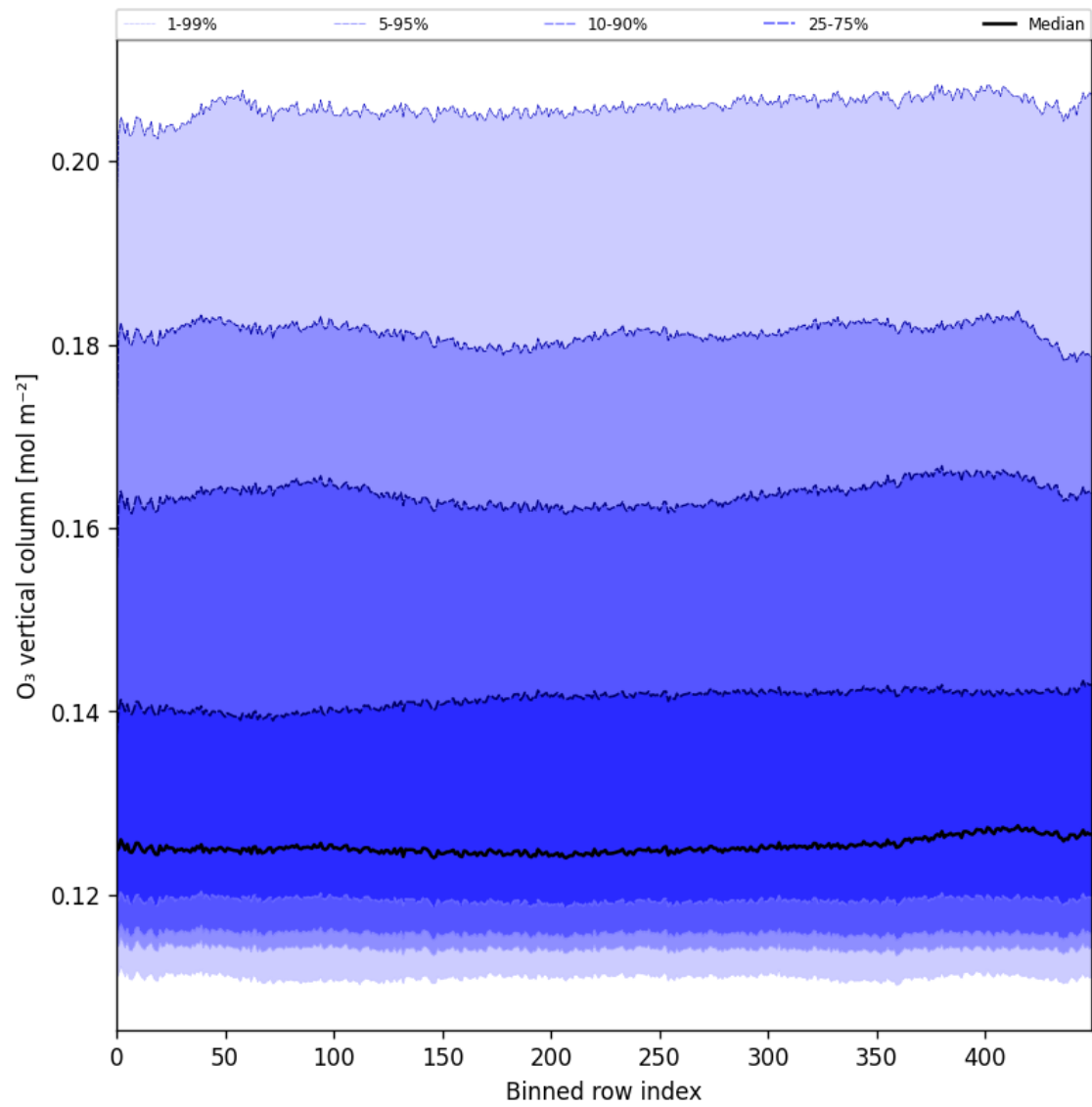
Figure 28: Along track statistics of “O 3 vertical column” for 2025-01-28 to 2025-01-30
