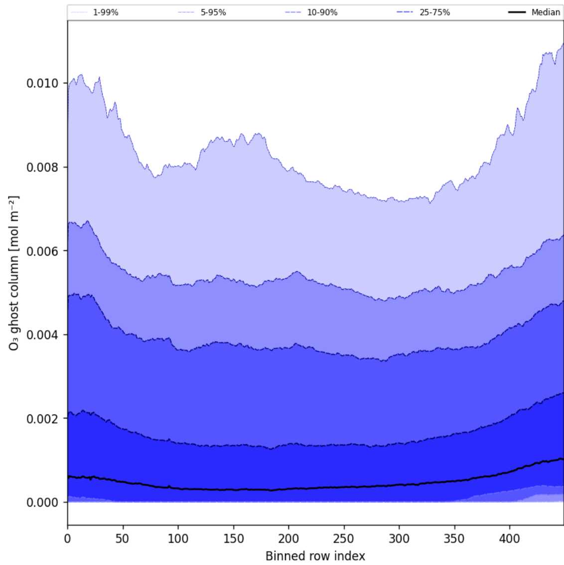
Figure 32: Along track statistics of “O 3 ghost column” for 2025-01-28 to 2025-01-30
