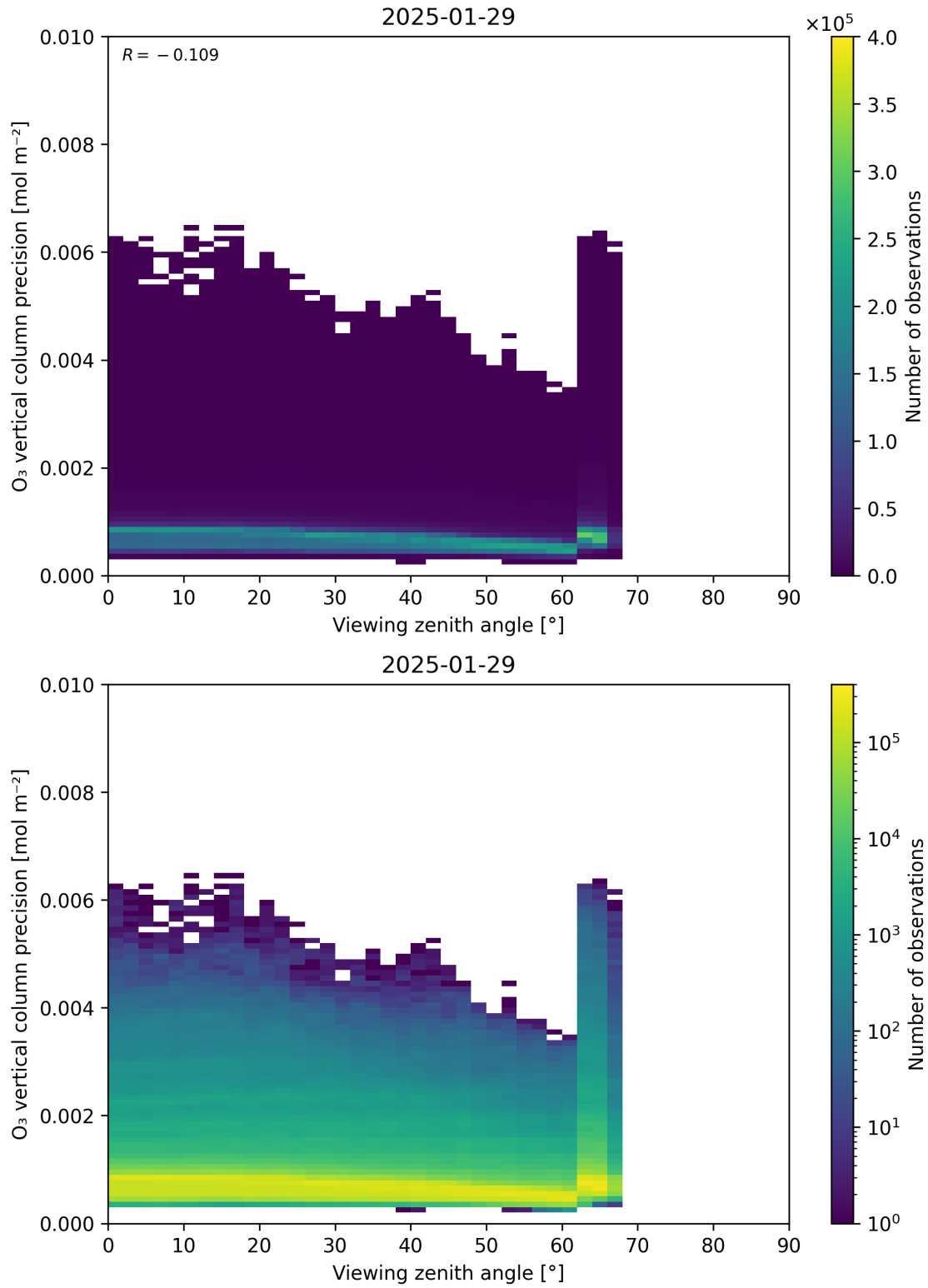
Figure 53: Scatter density plot of “Viewing zenith angle” against “O 3 vertical column precision” for 2025-01-28 to 2025-01-30.
