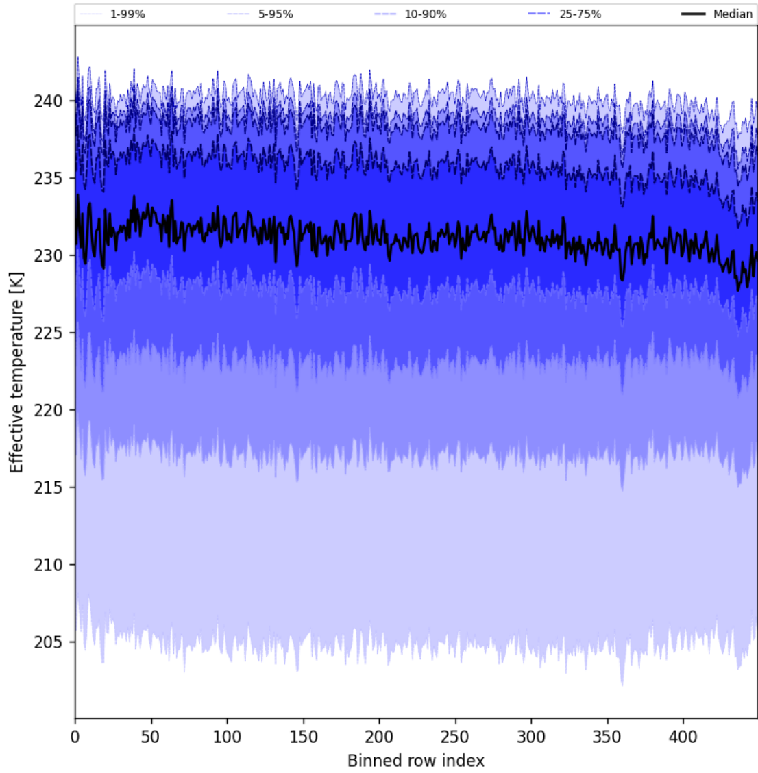
Figure 31: Along track statistics of “Effective temperature” for 2025-01-28 to 2025-01-30
