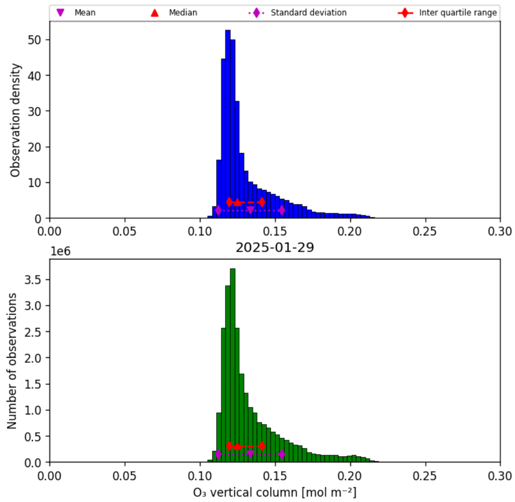
Figure 21: Histogram of “O 3 vertical column” for 2025-01-28 to 2025-01-30
