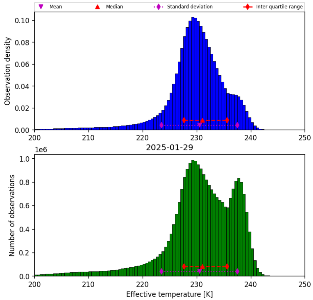
Figure 24: Histogram of “Effective temperature” for 2025-01-28 to 2025-01-30
