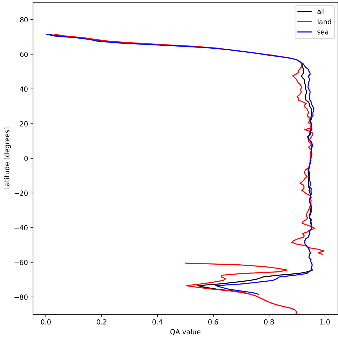
Figure 13: Zonal average of “QA value” for 2025-01-28 to 2025-01-30.
