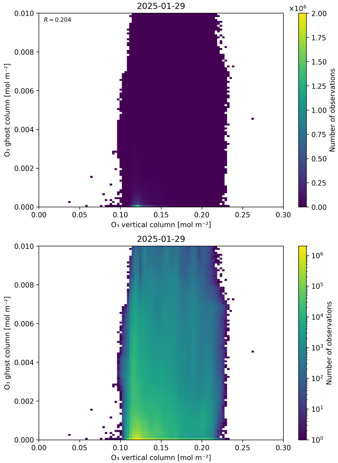
Figure 40: Scatter density plot of “O 3 vertical column” against “O 3 ghost column” for 2025-01-28 to 2025-01-30.
