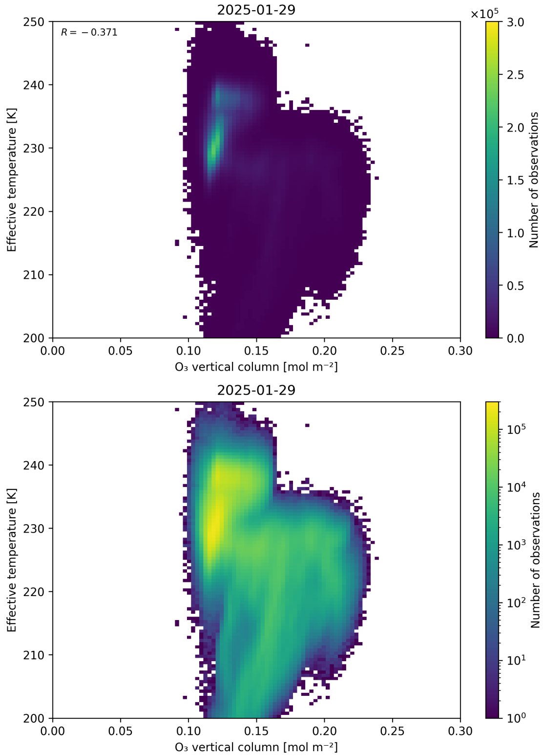
Figure 39: Scatter density plot of “O 3 vertical column” against “Effective temperature” for 2025-01-28 to 2025-01-30.
