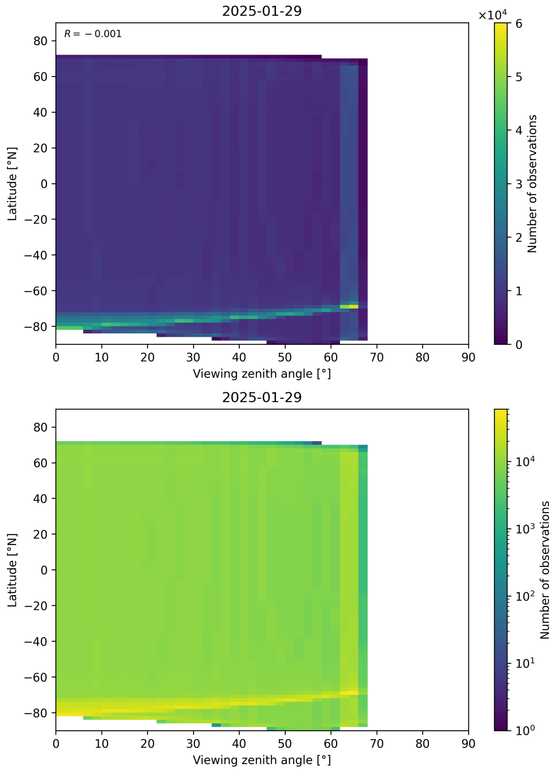
Figure 49: Scatter density plot of “Viewing zenith angle” against “Latitude” for 2025-01-28 to 2025-01-30.
