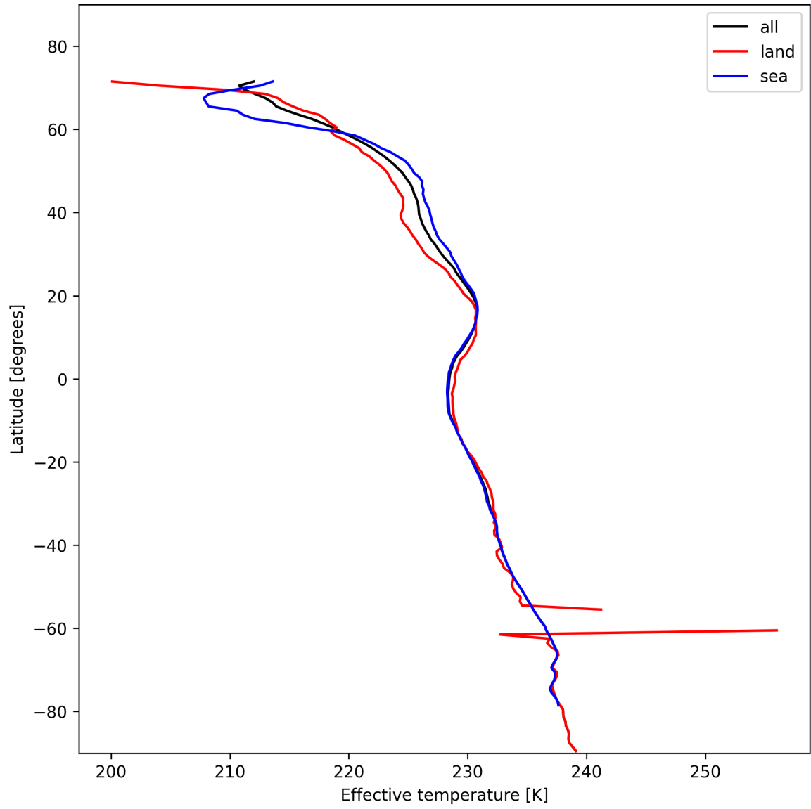
Figure 17: Zonal average of “Effective temperature” for 2025-01-28 to 2025-01-30.
