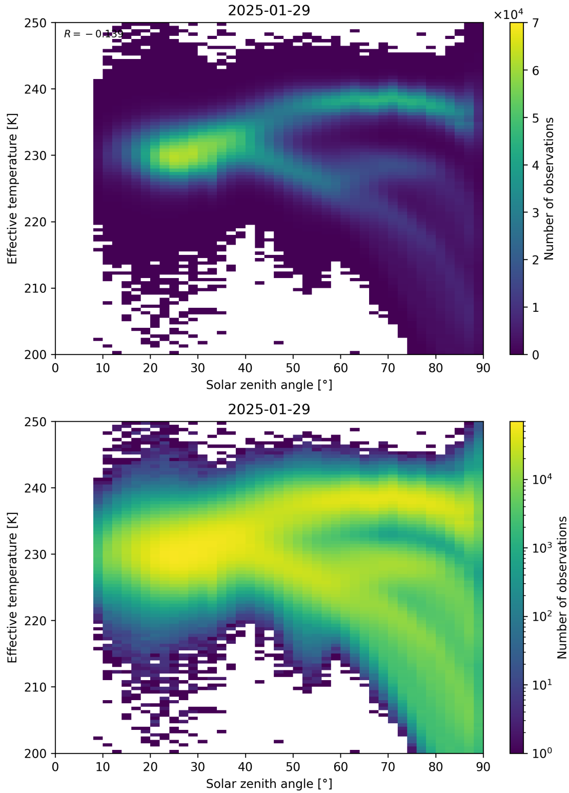
Figure 45: Scatter density plot of “Solar zenith angle” against “Effective temperature” for 2025-01-28 to 2025-01-30.
