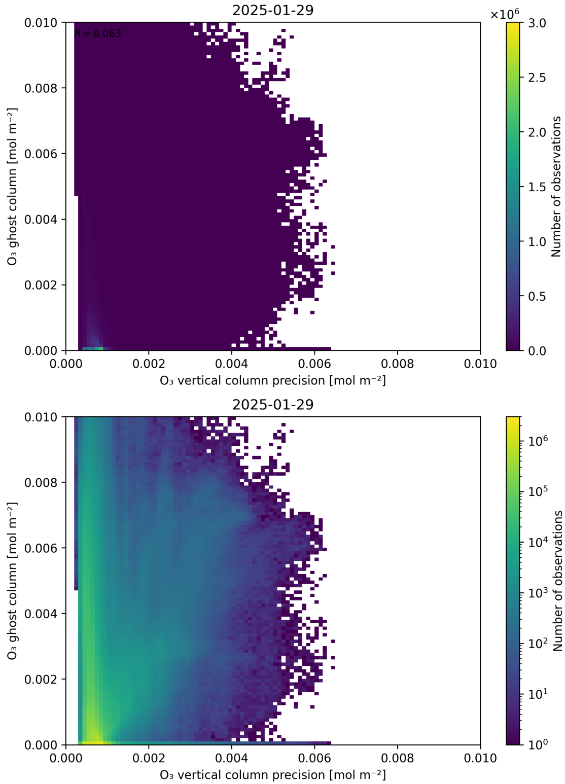
Figure 43: Scatter density plot of “O 3 vertical column precision” against “O 3 ghost column” for 2025-01-28 to 2025-01-30.
