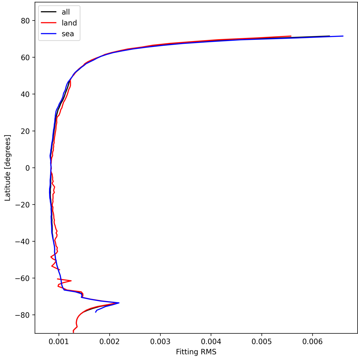
Figure 16: Zonal average of “Fitting RMS” for 2025-01-28 to 2025-01-30.
