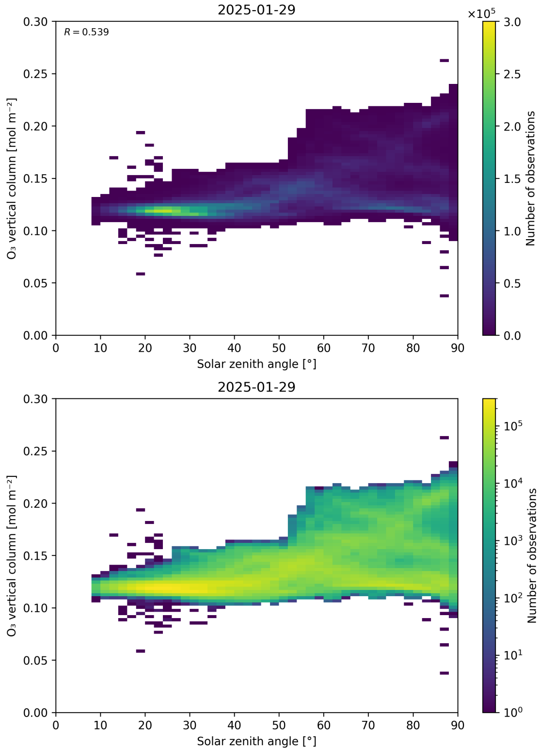
Figure 47: Scatter density plot of “Solar zenith angle” against “O 3 vertical column” for 2025-01-28 to 2025-01-30.
