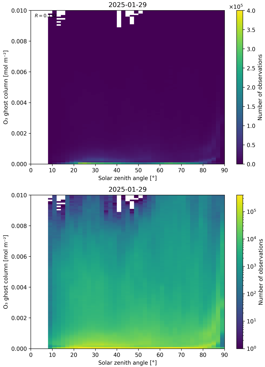
Figure 46: Scatter density plot of “Solar zenith angle” against “O 3 ghost column” for 2025-01-28 to 2025-01-30.
