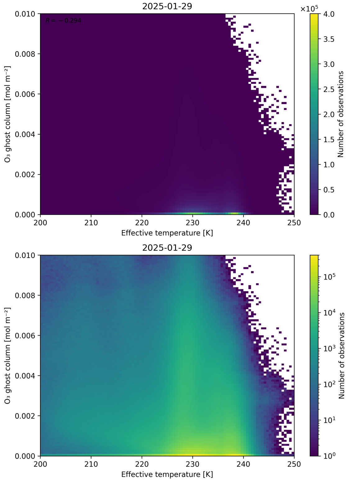
Figure 38: Scatter density plot of “Effective temperature” against “O 3 ghost column” for 2025-01-28 to 2025-01-30.
