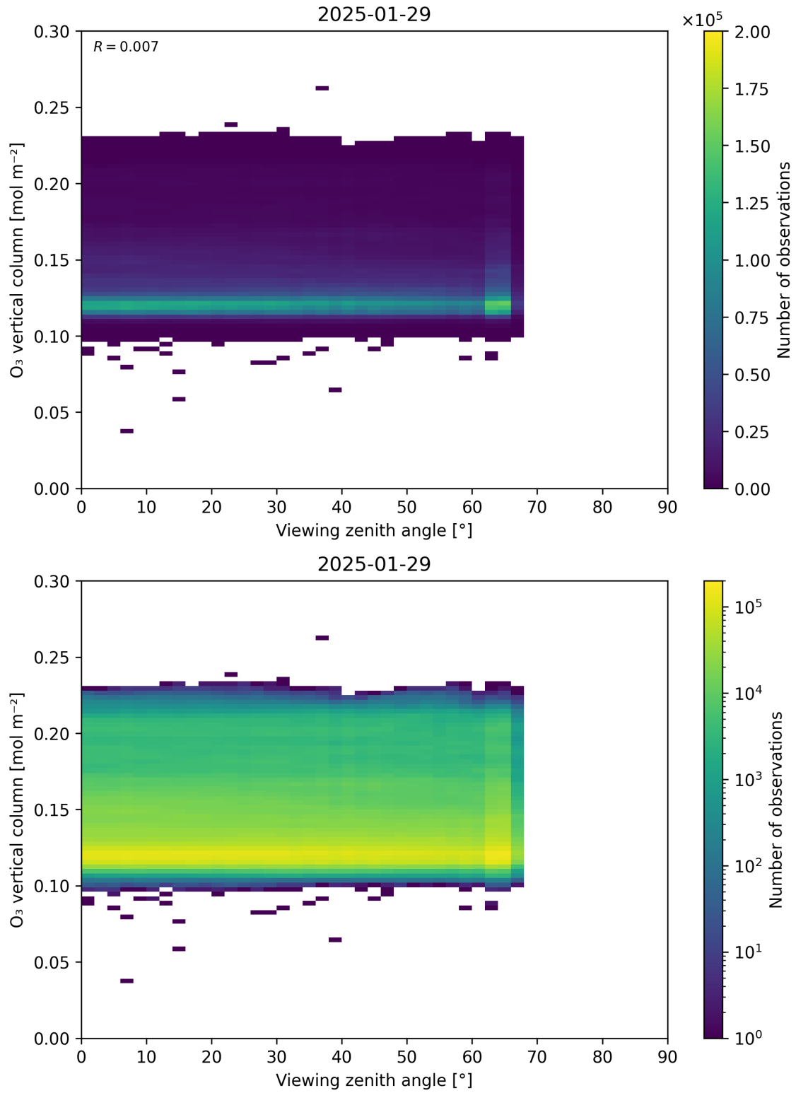
Figure 52: Scatter density plot of “Viewing zenith angle” against “O 3 vertical column” for 2025-01-28 to 2025-01-30.
