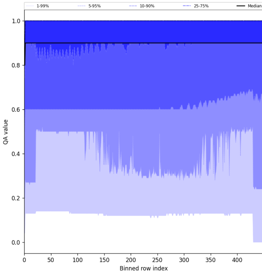
Figure 27: Along track statistics of “QA value” for 2025-01-28 to 2025-01-30
