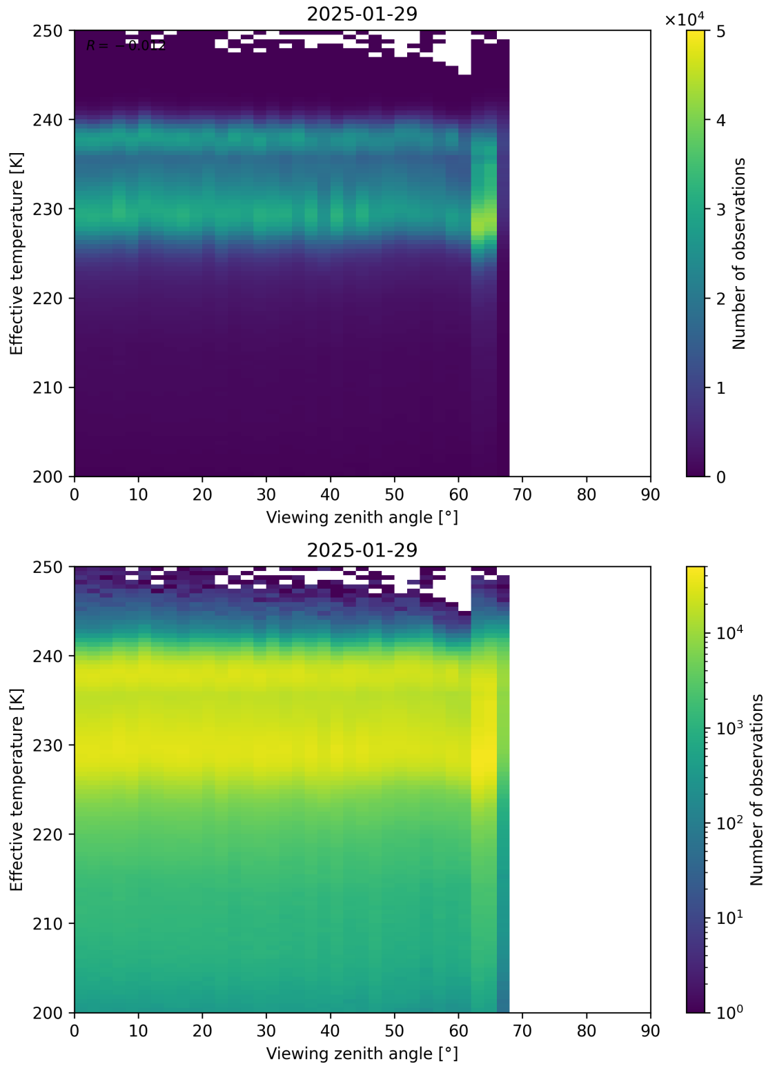
Figure 50: Scatter density plot of “Viewing zenith angle” against “Effective temperature” for 2025-01-28 to 2025-01-30.
