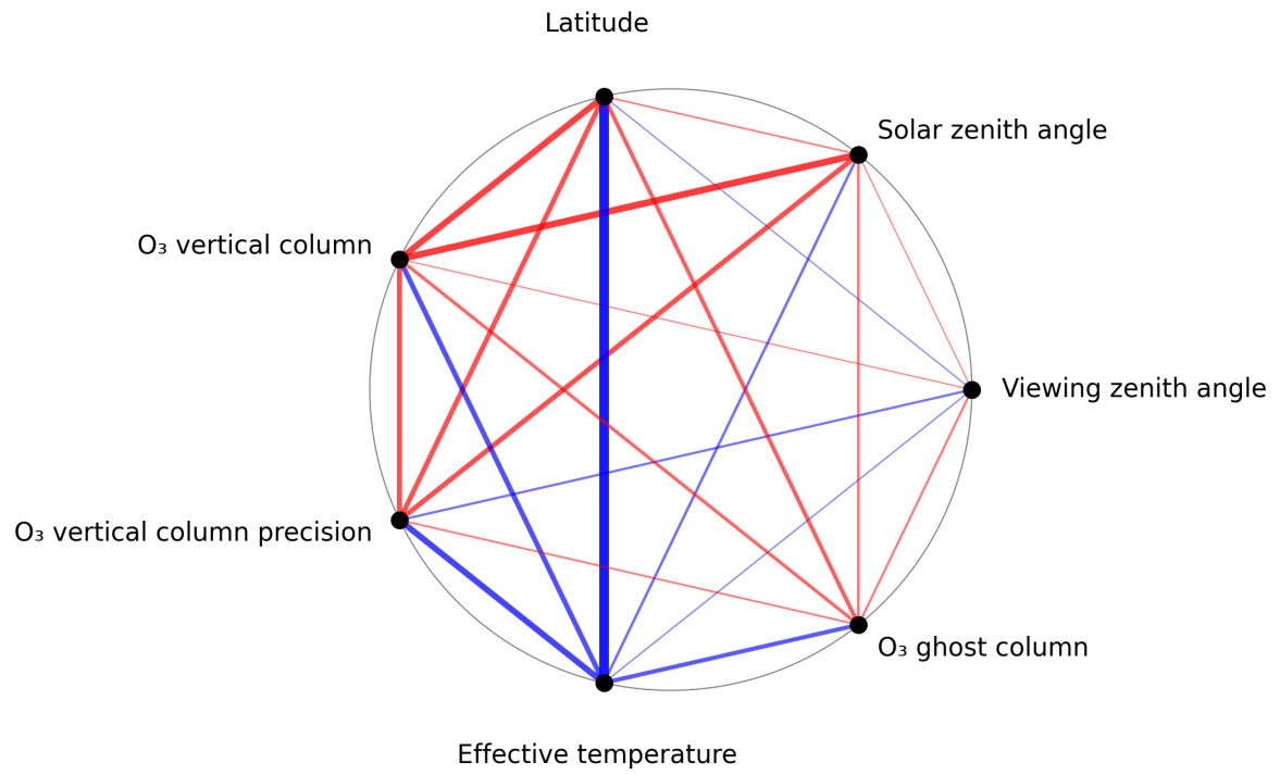
Figure 1: Map of correlation graph for 2025-01-28 to 2025-01-30.
