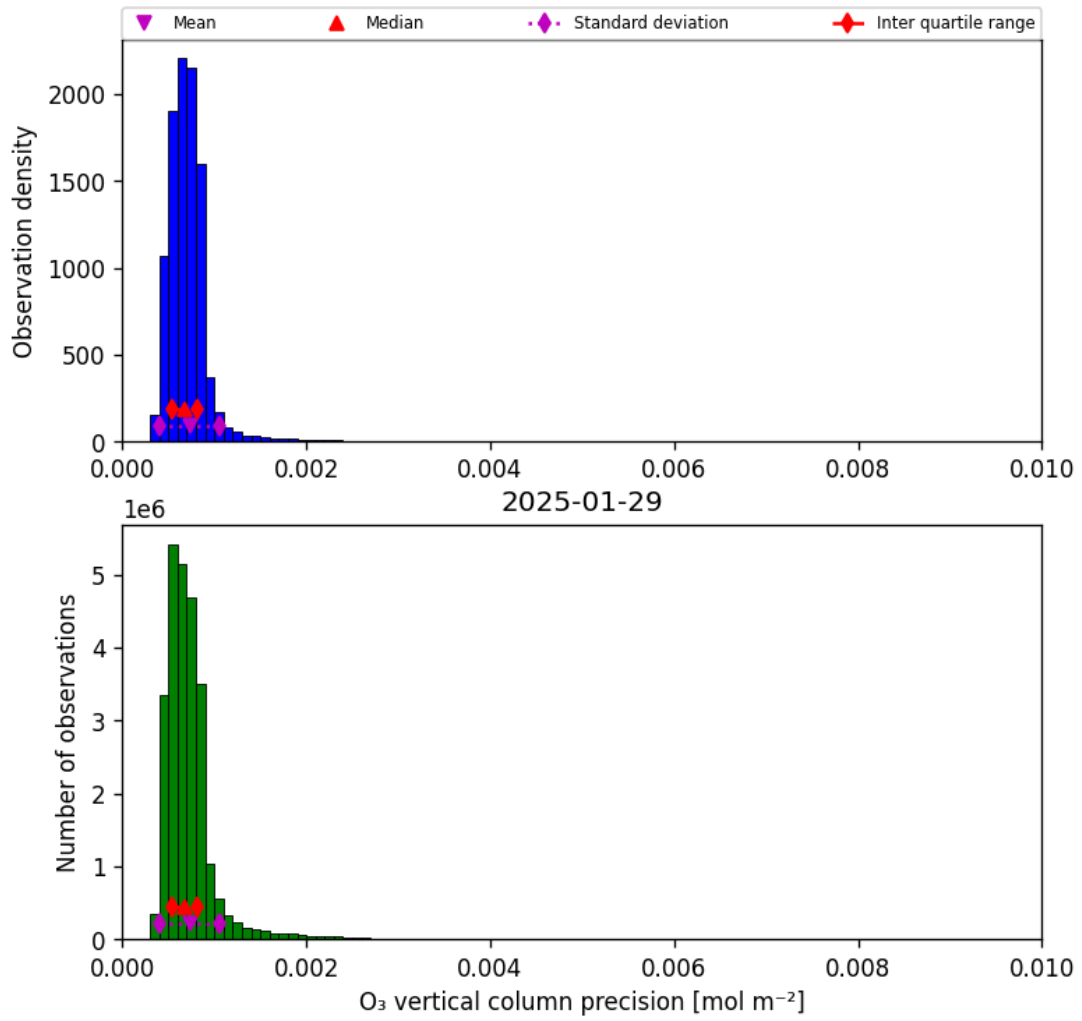
Figure 22: Histogram of “O 3 vertical column precision” for 2025-01-28 to 2025-01-30
