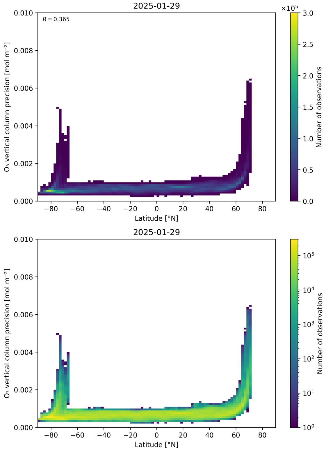
Figure 37: Scatter density plot of “Latitude” against “O 3 vertical column precision” for 2025-01-28 to 2025-01-30.
