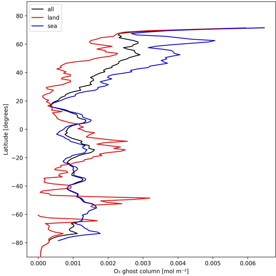
Figure 18: Zonal average of "O 3 ghost column" for 2025-01-28 to 2025-01-30.
