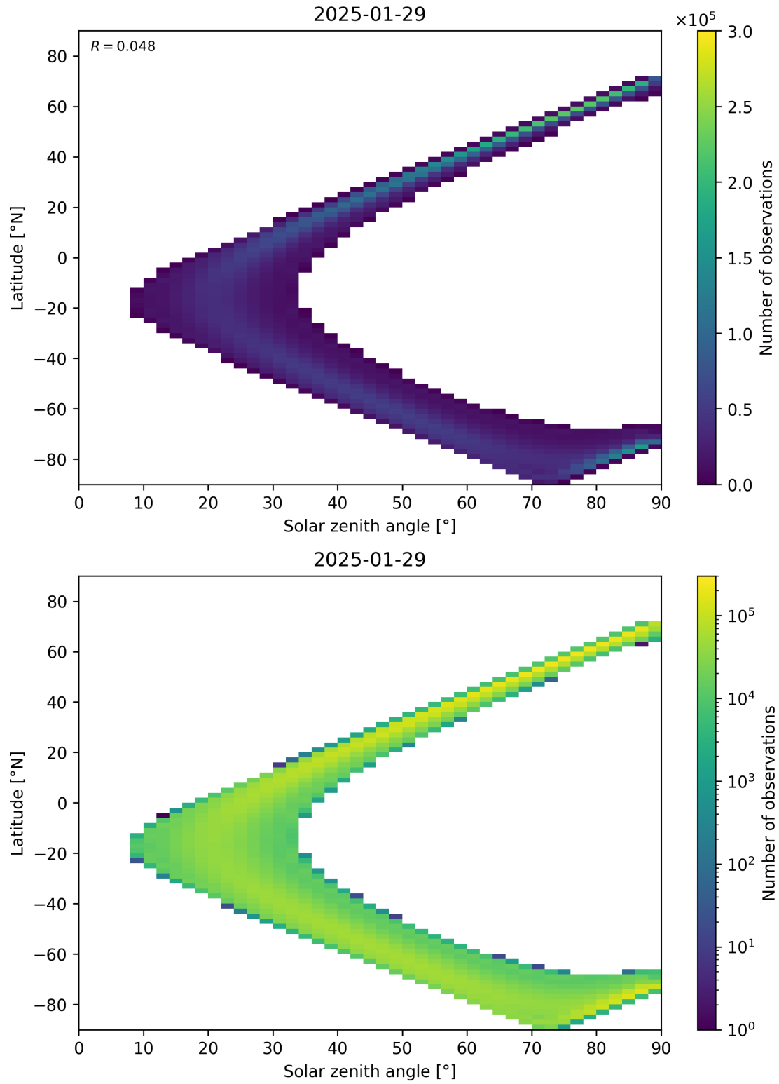
Figure 44: Scatter density plot of “Solar zenith angle” against “Latitude” for 2025-01-28 to 2025-01-30.
