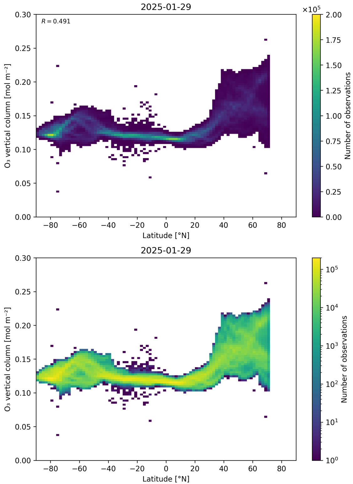
Figure 36: Scatter density plot of “Latitude” against “O 3 vertical column” for 2025-01-28 to 2025-01-30.
