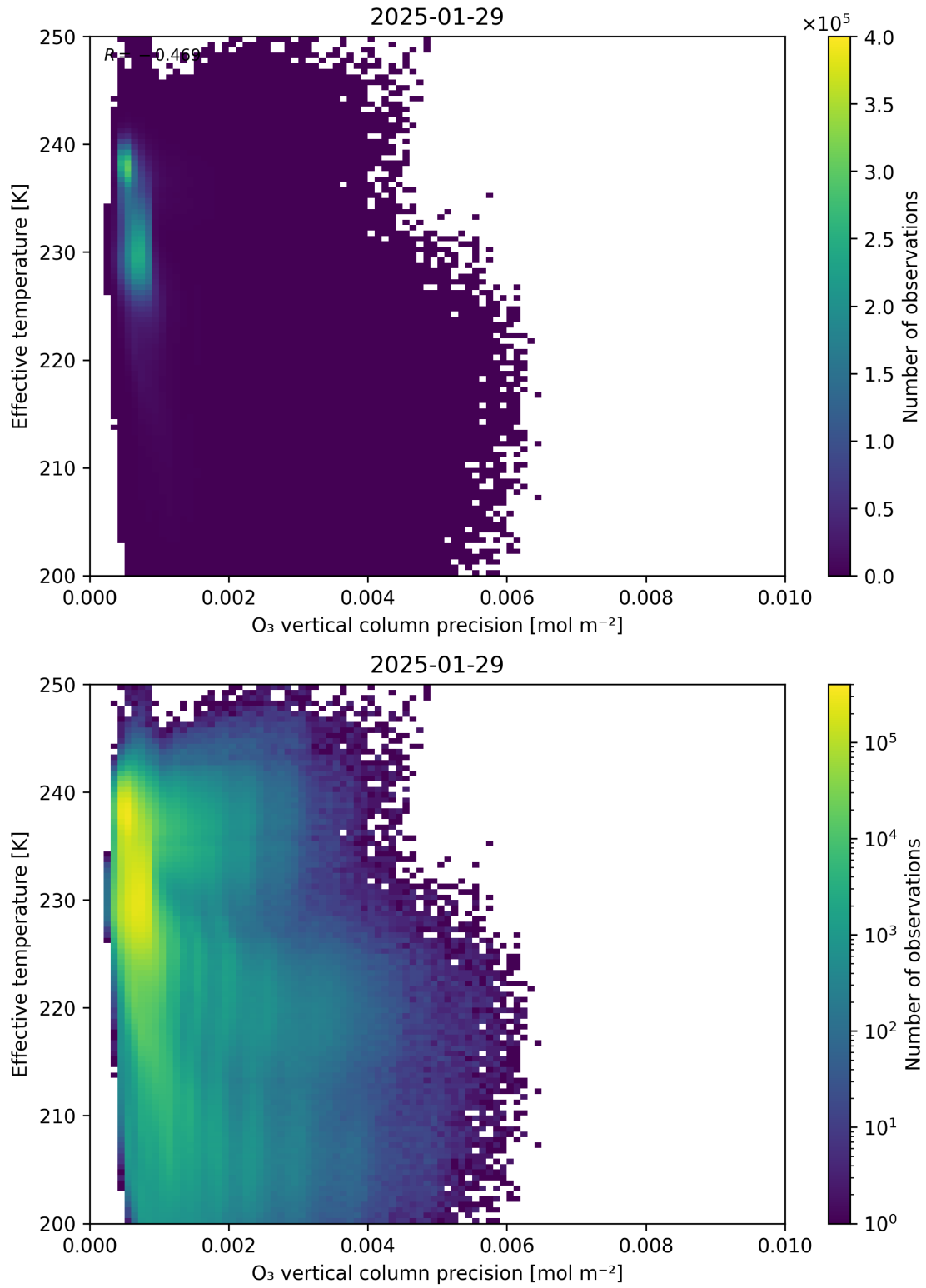
Figure 42: Scatter density plot of “O 3 vertical column precision” against “Effective temperature” for 2025-01-28 to 2025-01-30.
