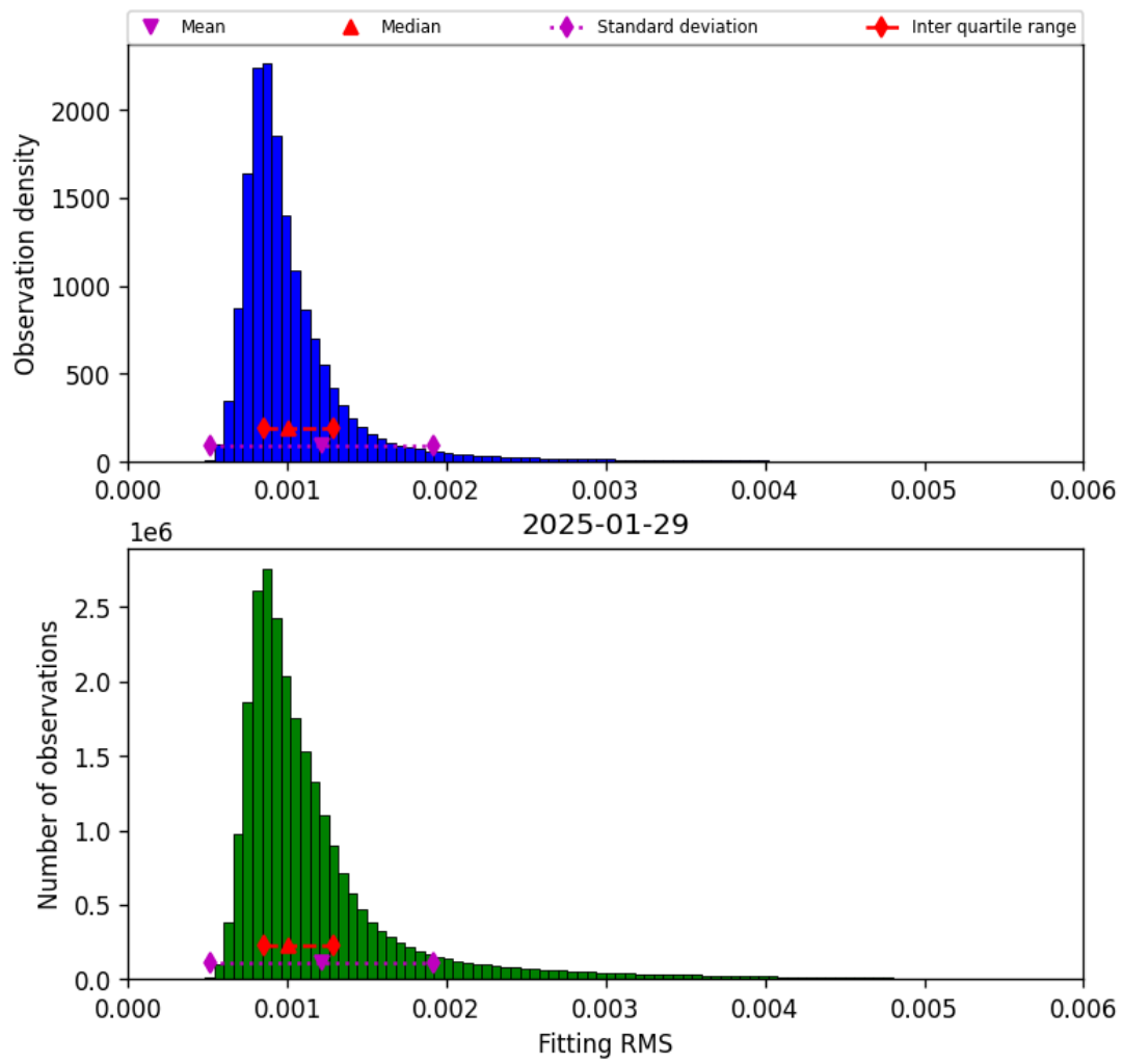
Figure 23: Histogram of “Fitting RMS” for 2025-01-28 to 2025-01-30
