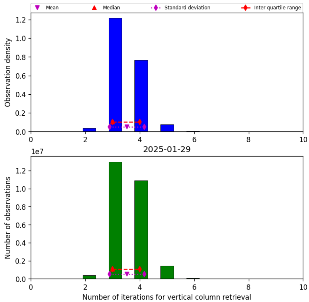
Figure 26: Histogram of “Number of iterations for vertical column retrieval” for 2025-01-28 to 2025-01-30
