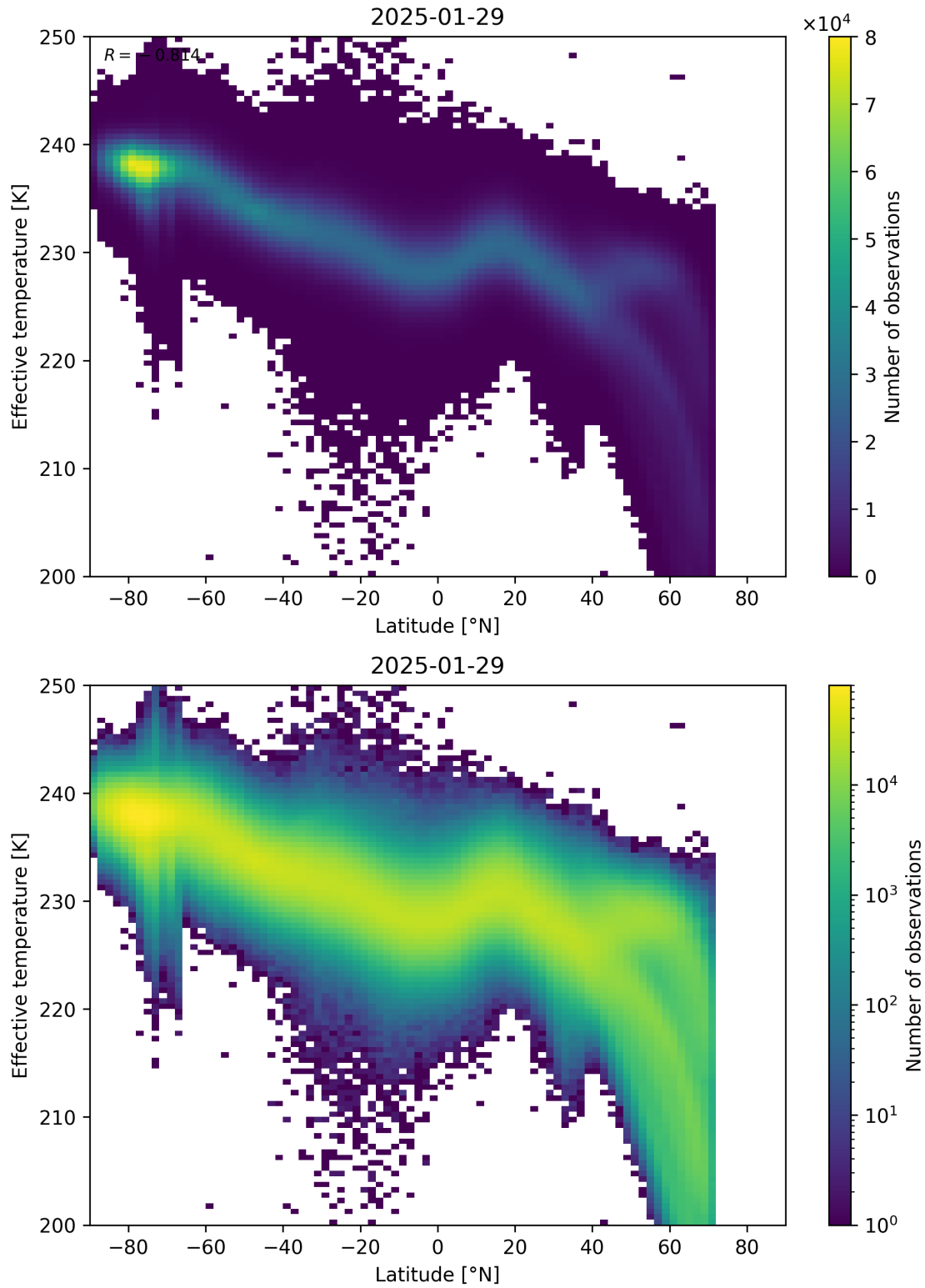
Figure 34: Scatter density plot of “Latitude” against “Effective temperature” for 2025-01-28 to 2025-01-30.
