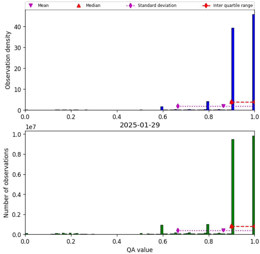
Figure 20: Histogram of “QA value” for 2025-01-28 to 2025-01-30
