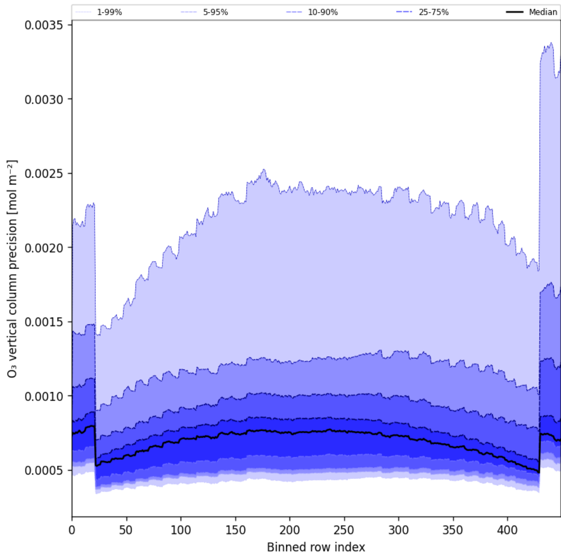
Figure 29: Along track statistics of “O 3 vertical column precision” for 2025-01-28 to 2025-01-30
