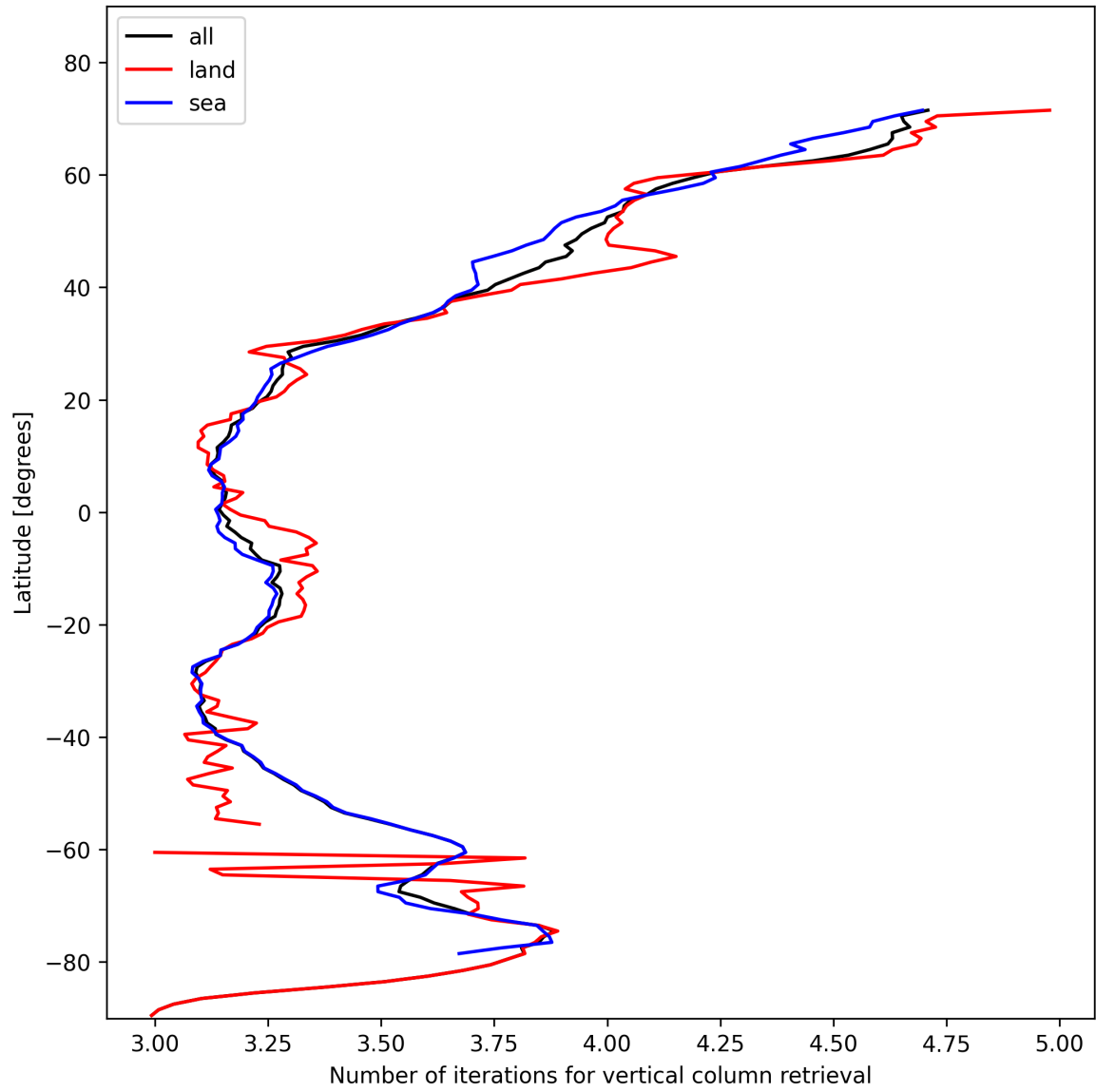
Figure 19: Zonal average of “Number of iterations for vertical column retrieval” for 2025-01-28 to 2025-01-30.
