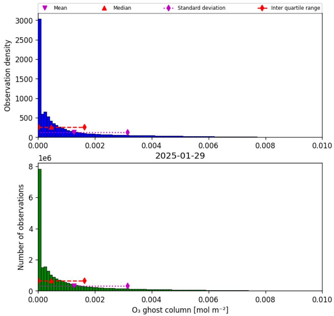
Figure 25: Histogram of “O 3 ghost column” for 2025-01-28 to 2025-01-30
