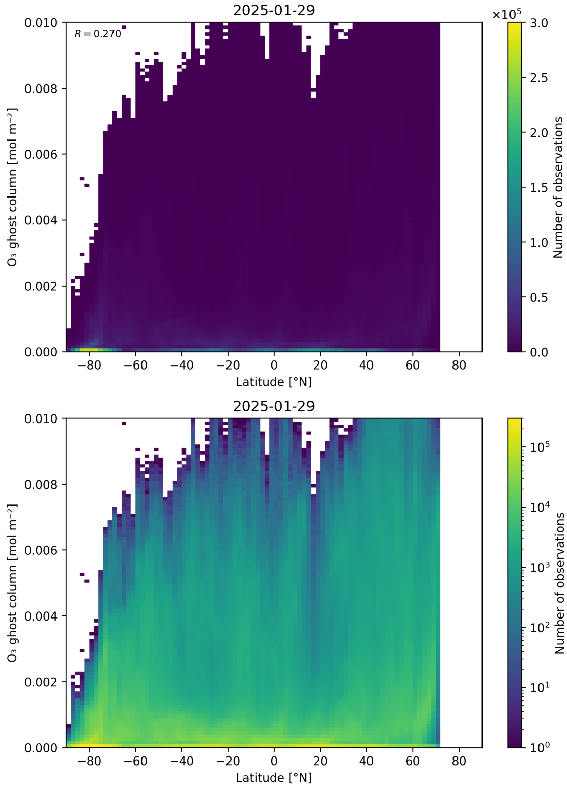
Figure 35: Scatter density plot of “Latitude” against “O 3 ghost column” for 2025-01-28 to 2025-01-30.
