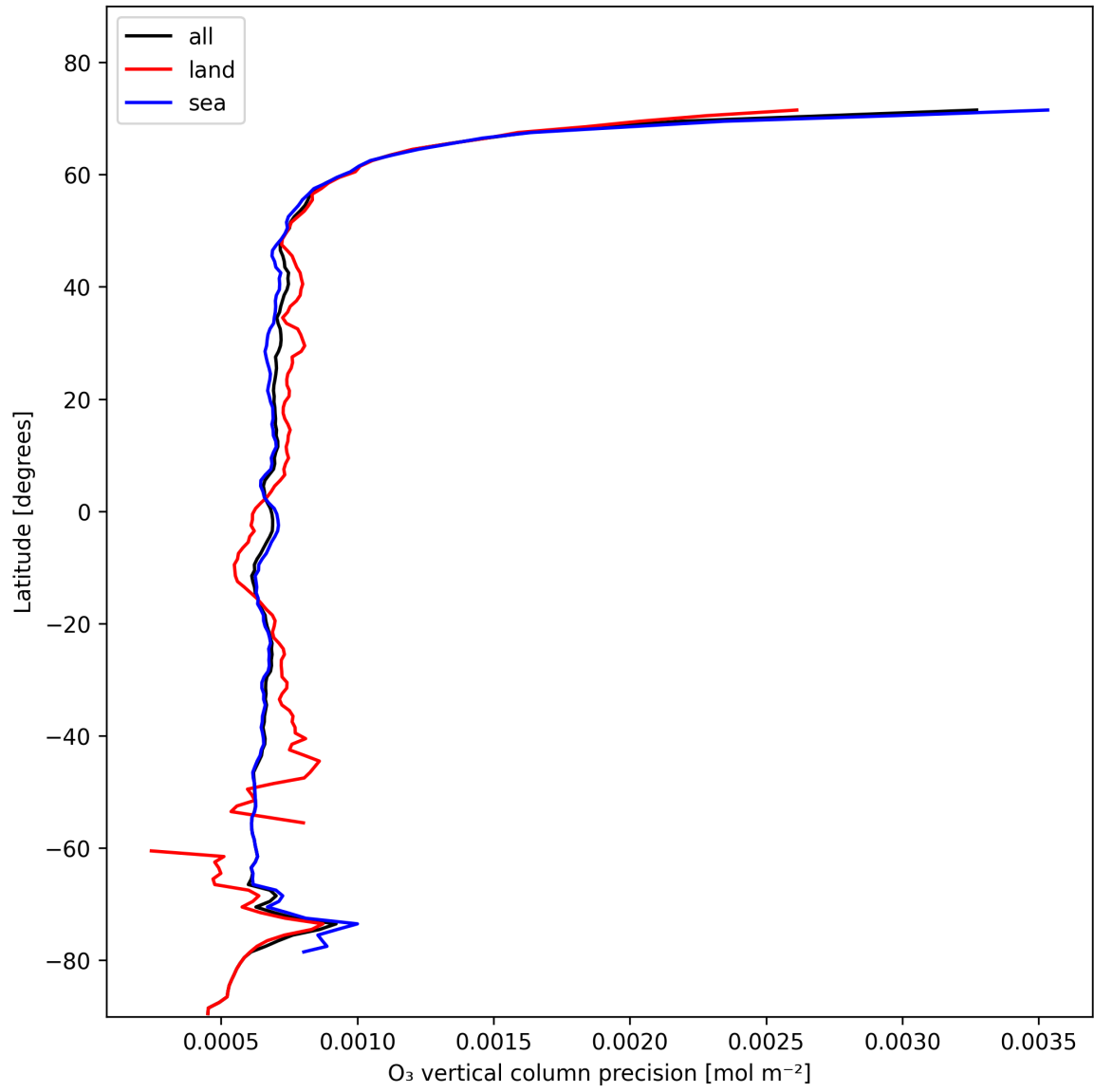
Figure 15: Zonal average of “O 3 vertical column precision” for 2025-01-29 to 2025-01-31.
