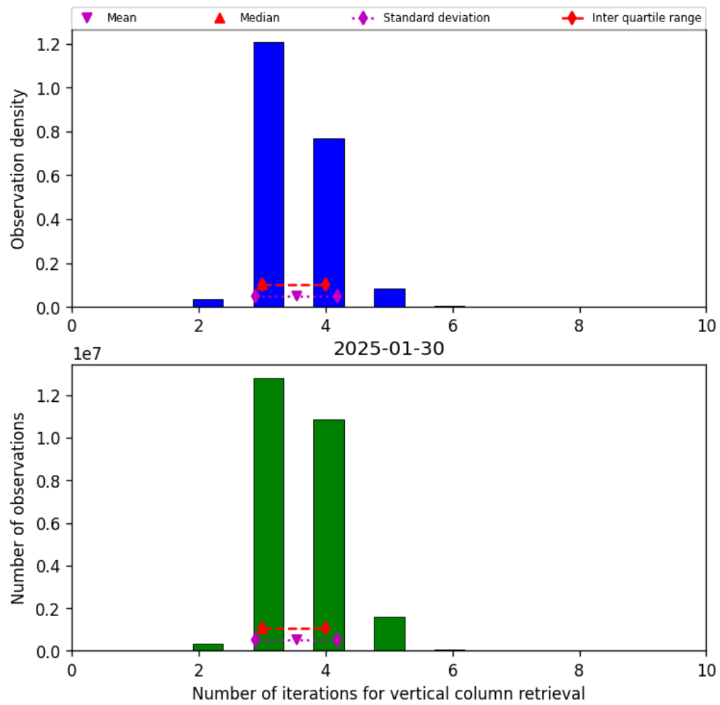
Figure 26: Histogram of “Number of iterations for vertical column retrieval” for 2025-01-29 to 2025-01-31
