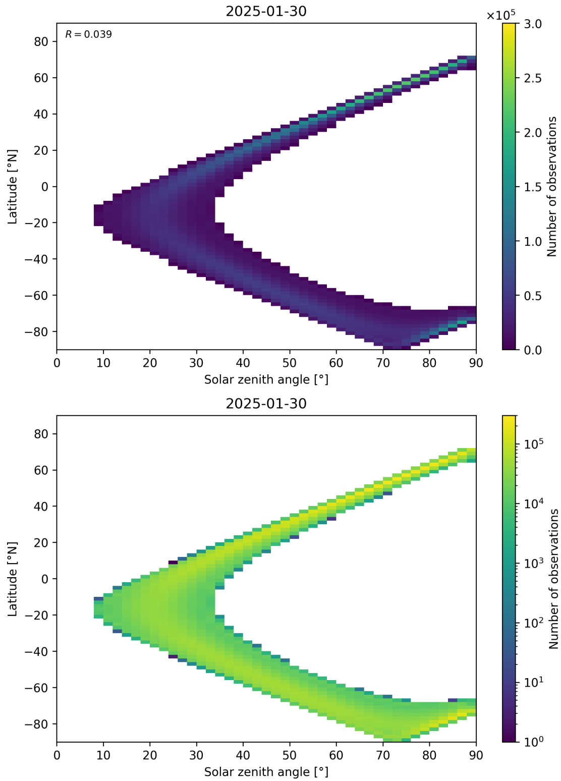
Figure 44: Scatter density plot of “Solar zenith angle” against “Latitude” for 2025-01-29 to 2025-01-31.
