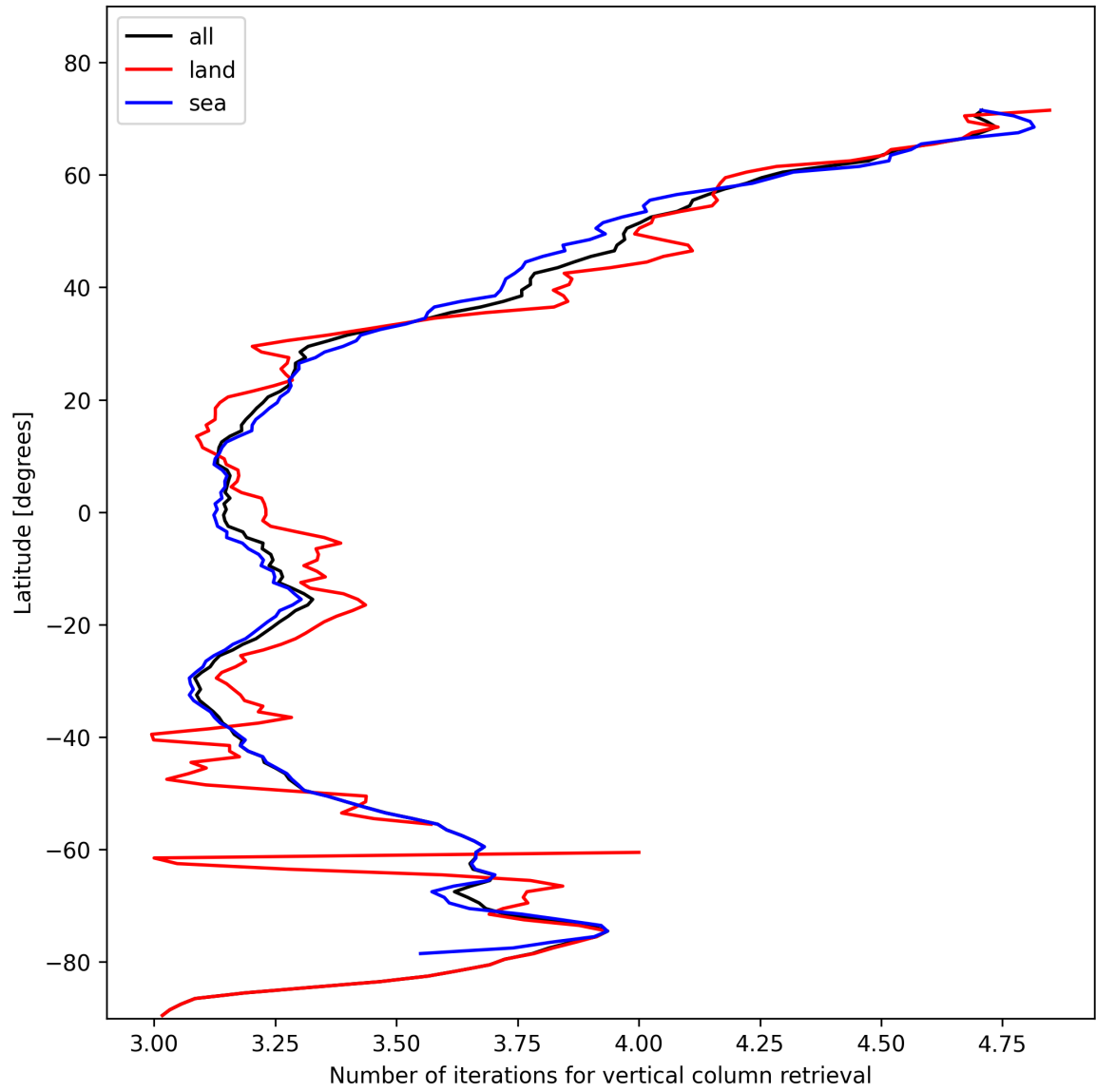
Figure 19: Zonal average of “Number of iterations for vertical column retrieval” for 2025-01-29 to 2025-01-31.
