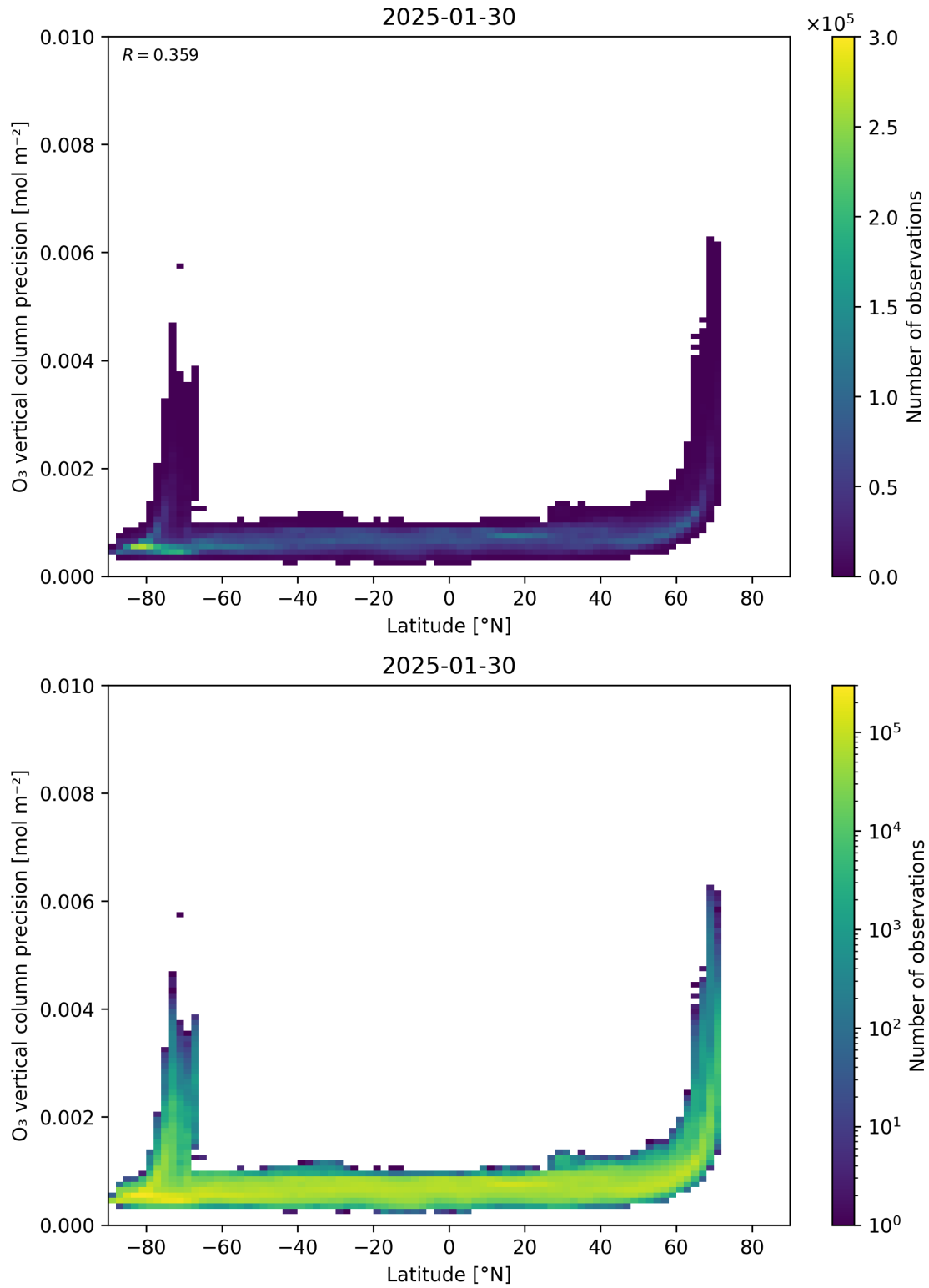
Figure 37: Scatter density plot of “Latitude” against “O 3 vertical column precision” for 2025-01-29 to 2025-01-31.
