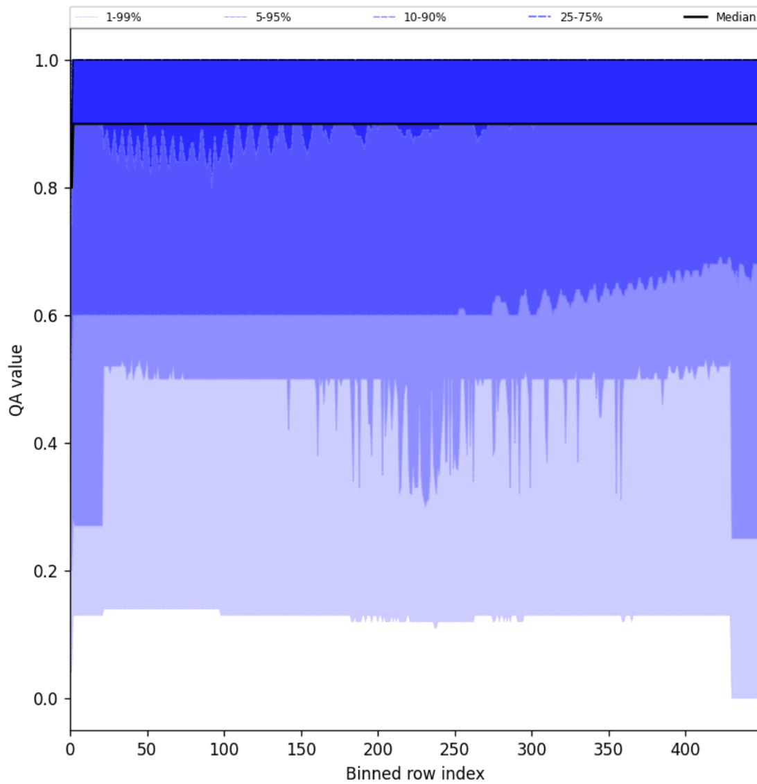
Figure 27: Along track statistics of “QA value” for 2025-01-29 to 2025-01-31
