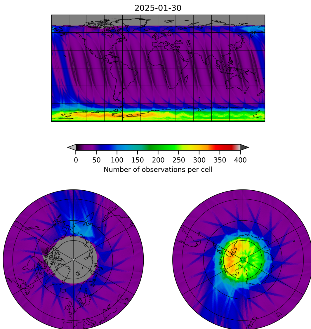
Figure 12: Map of the number of observations for 2025-01-29 to 2025-01-31
