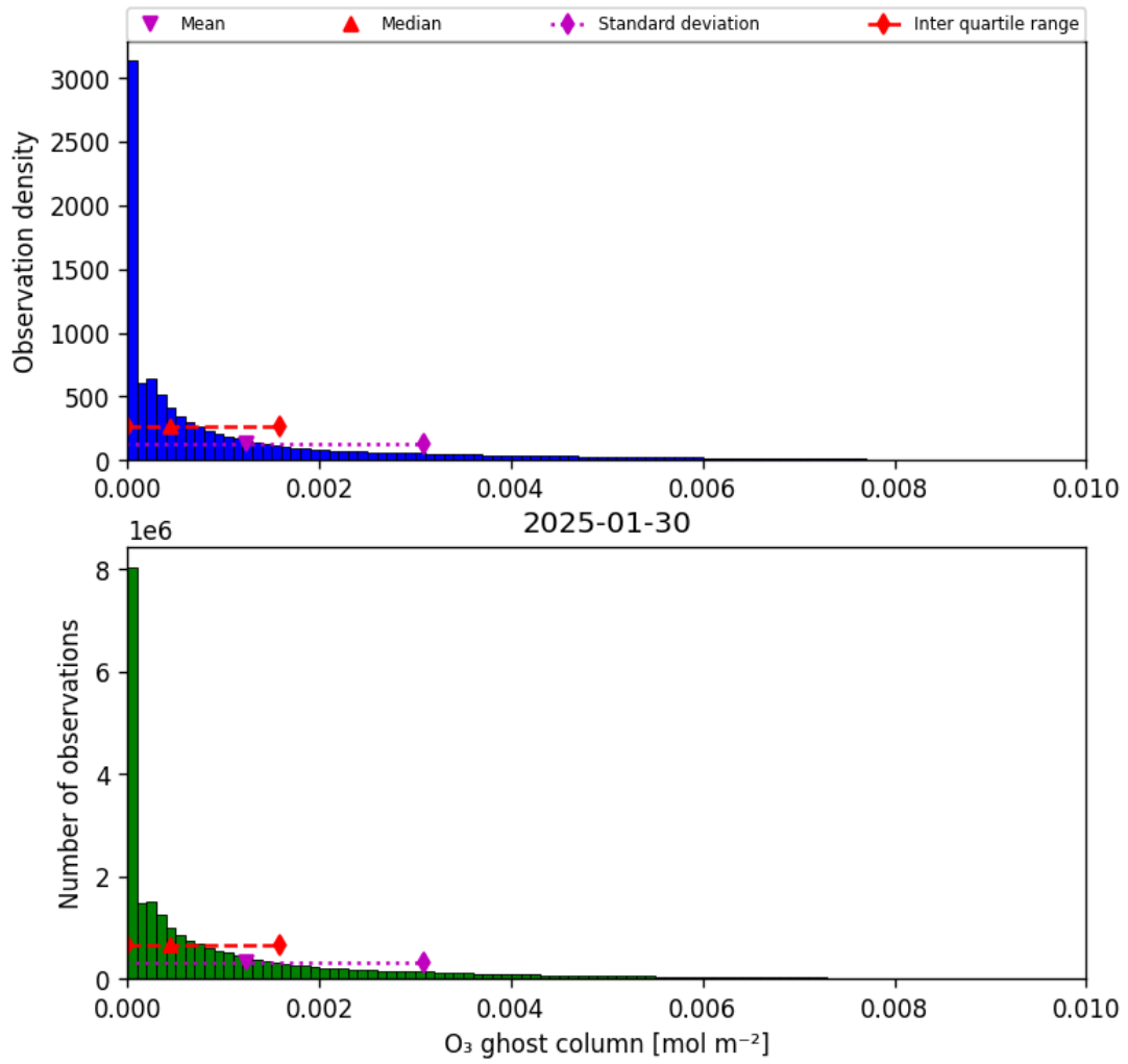
Figure 25: Histogram of “O 3 ghost column” for 2025-01-29 to 2025-01-31
