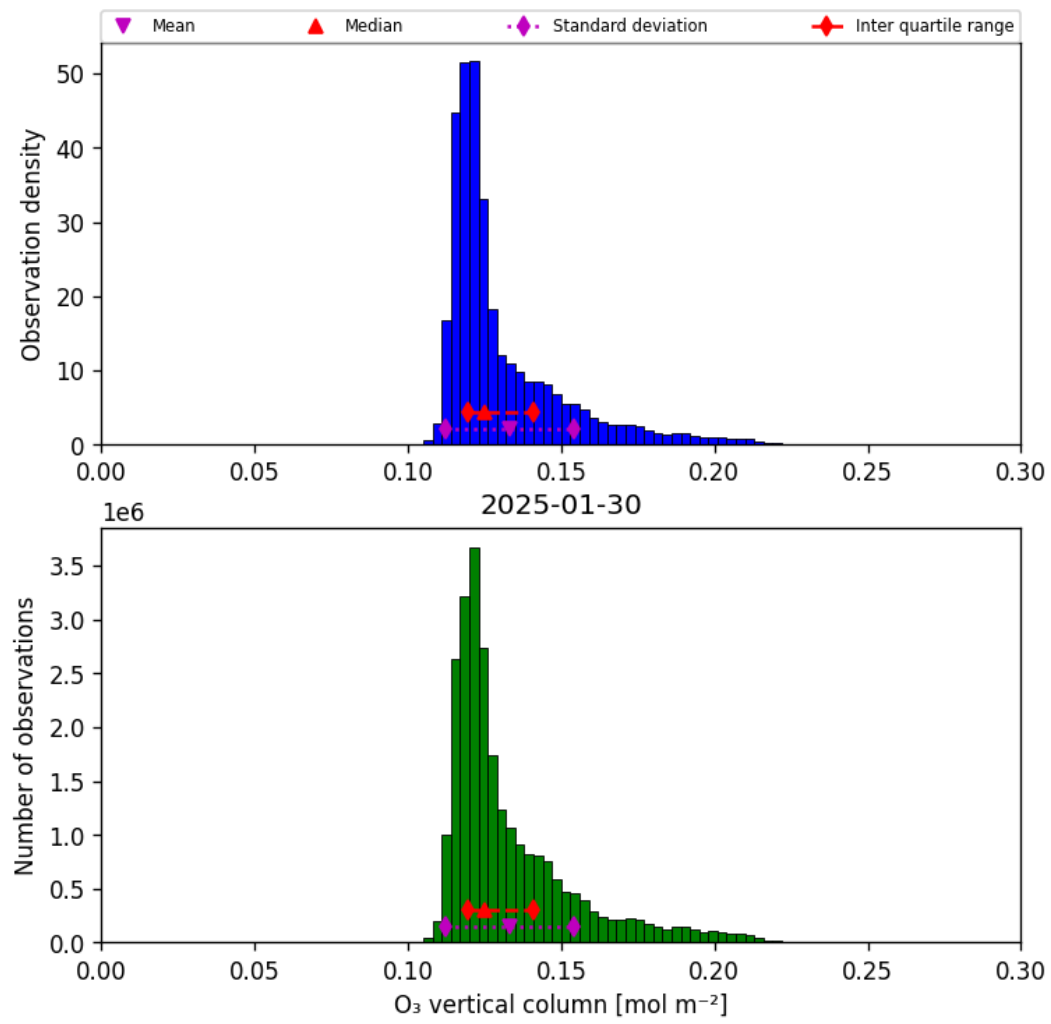
Figure 21: Histogram of “O 3 vertical column” for 2025-01-29 to 2025-01-31
