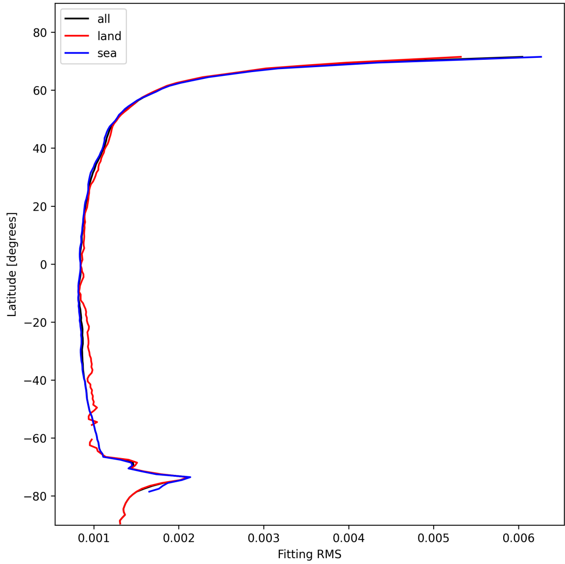
Figure 16: Zonal average of “Fitting RMS” for 2025-01-29 to 2025-01-31.
