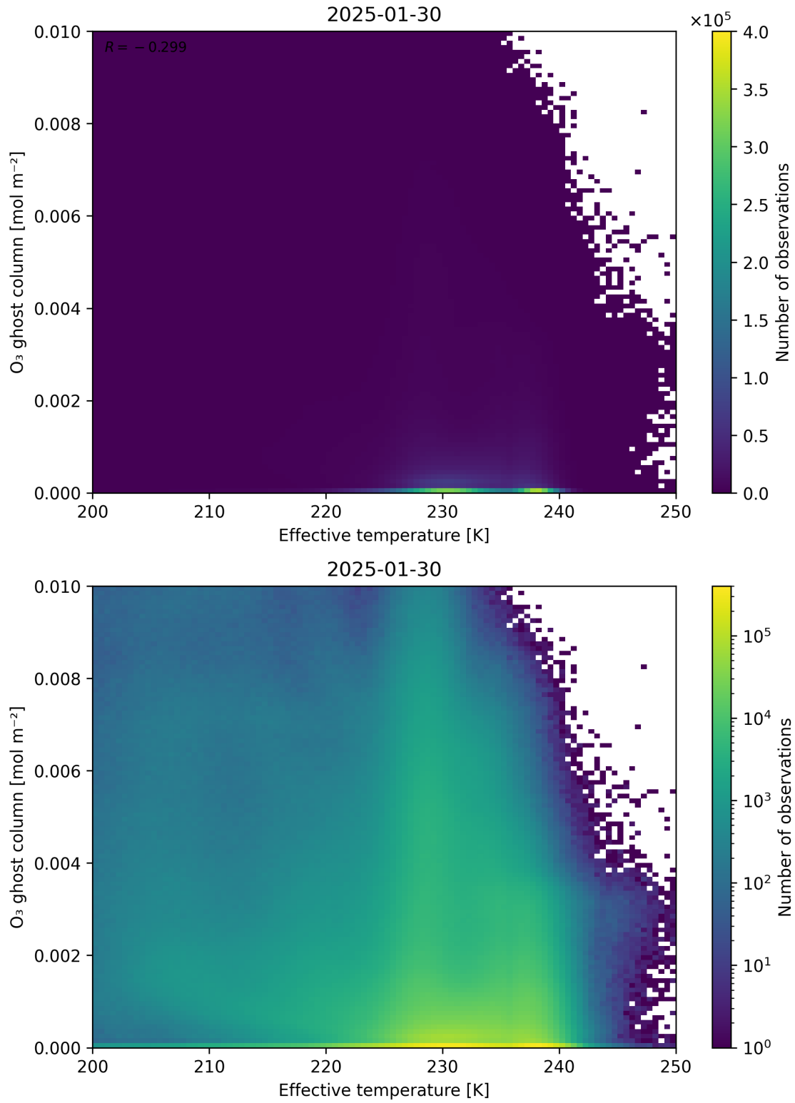
Figure 38: Scatter density plot of “Effective temperature” against “O 3 ghost column” for 2025-01-29 to 2025-01-31.
