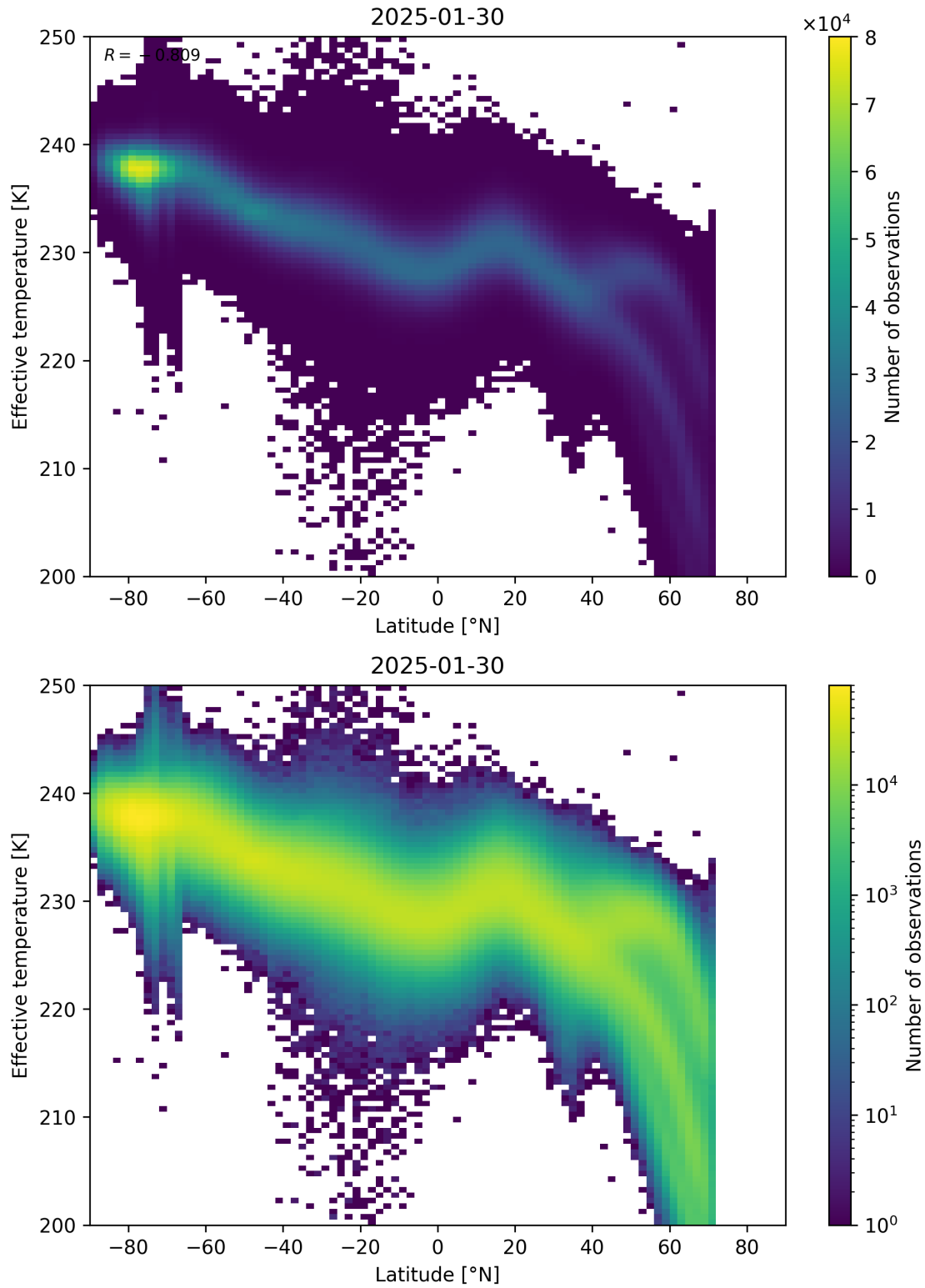
Figure 34: Scatter density plot of “Latitude” against “Effective temperature” for 2025-01-29 to 2025-01-31.
