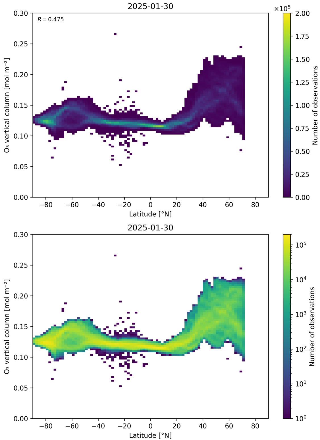
Figure 36: Scatter density plot of “Latitude” against “O 3 vertical column” for 2025-01-29 to 2025-01-31.
