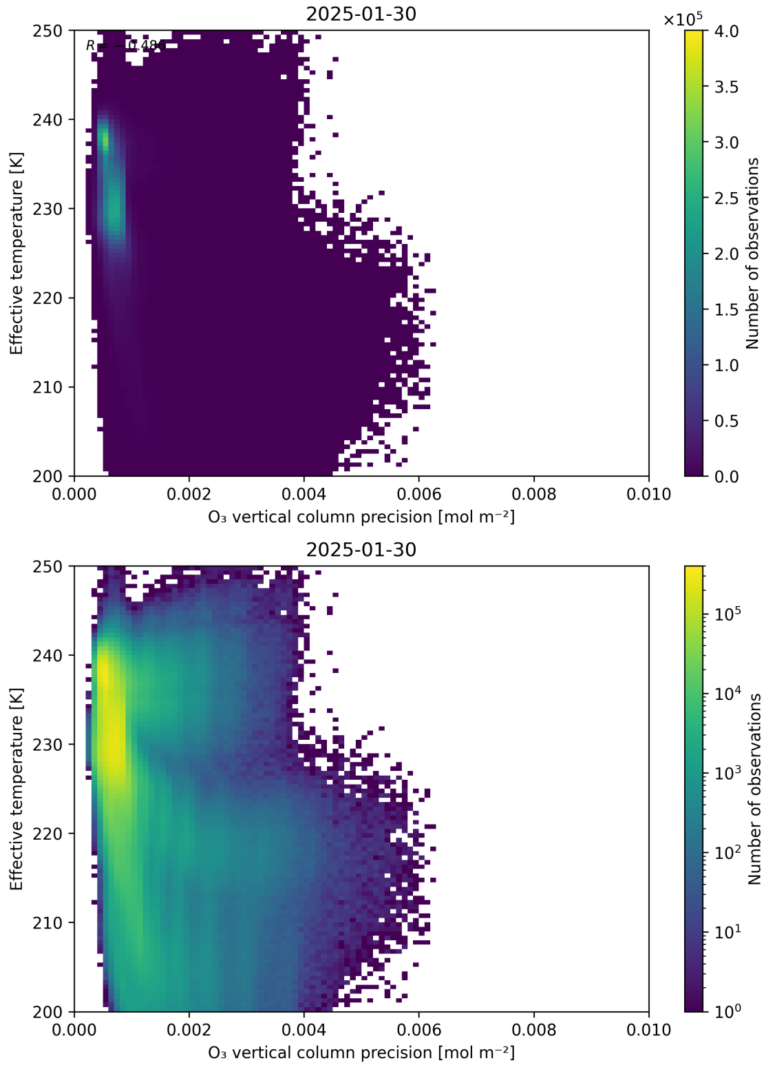
Figure 42: Scatter density plot of “O 3 vertical column precision” against “Effective temperature” for 2025-01-29 to 2025-01-31.
