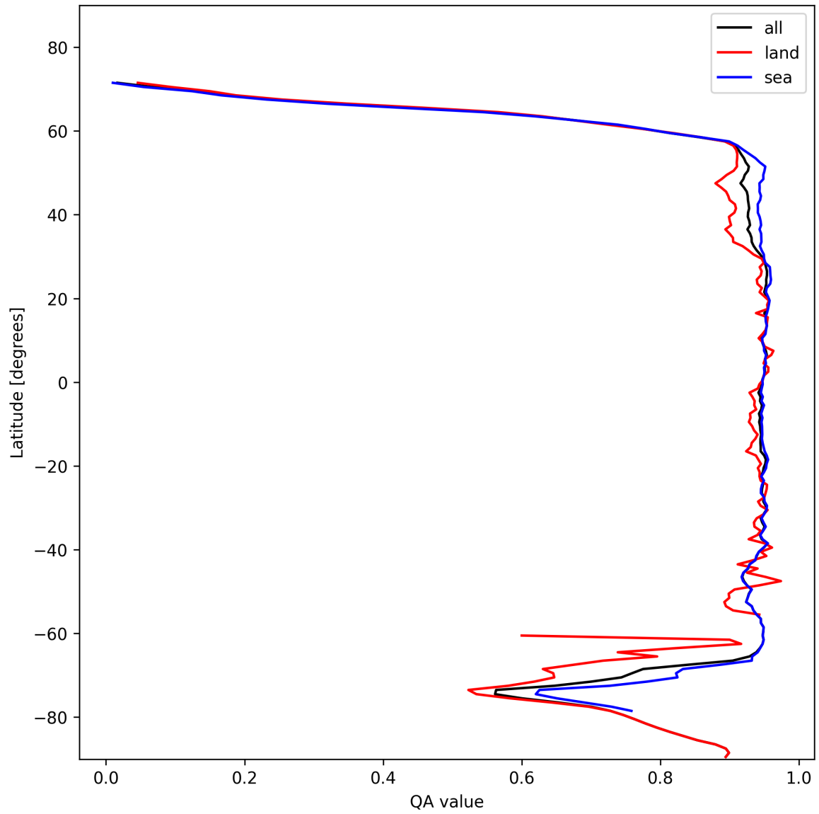
Figure 13: Zonal average of “QA value” for 2025-01-29 to 2025-01-31.
