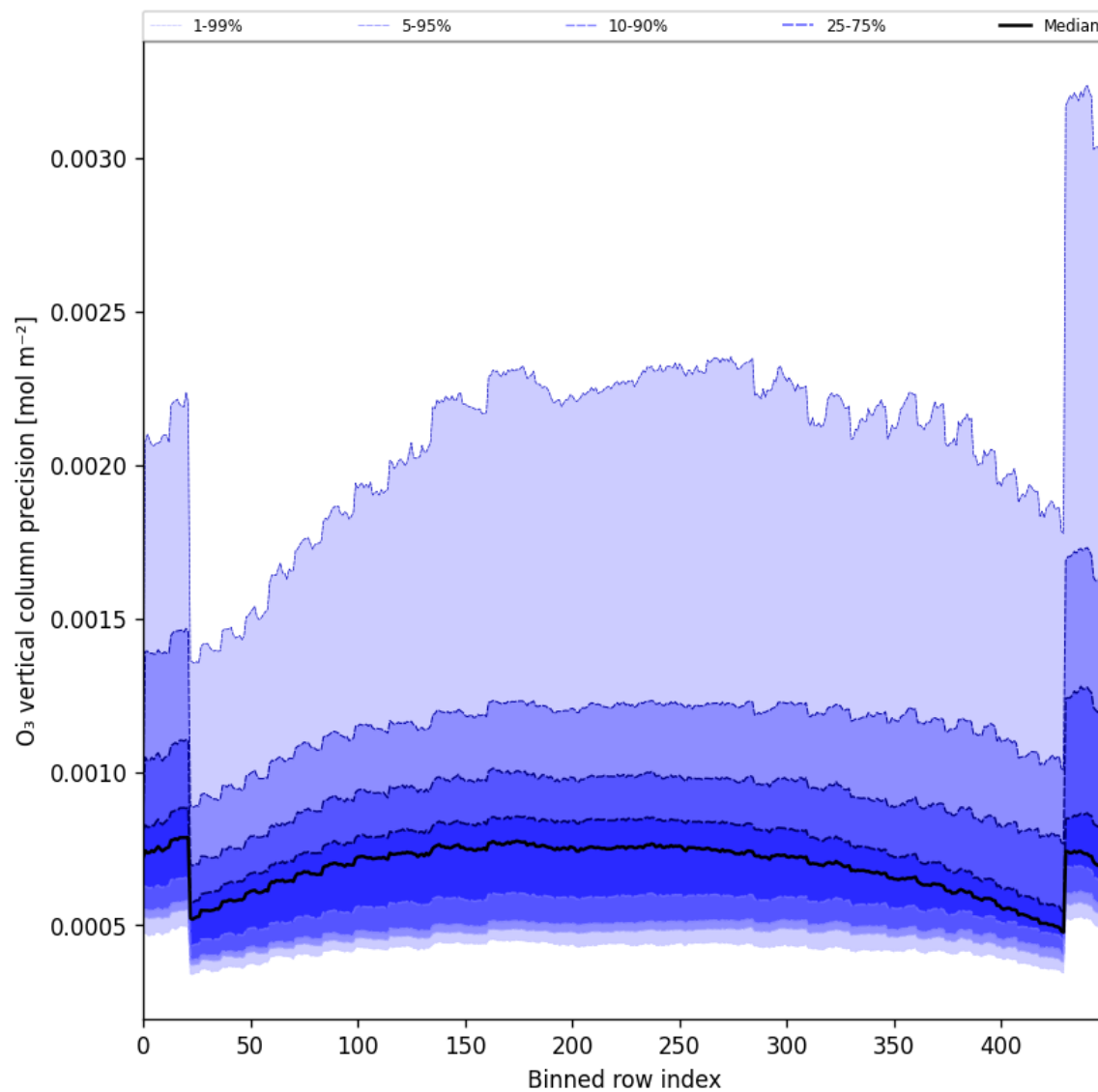
Figure 29: Along track statistics of “O 3 vertical column precision” for 2025-01-29 to 2025-01-31
