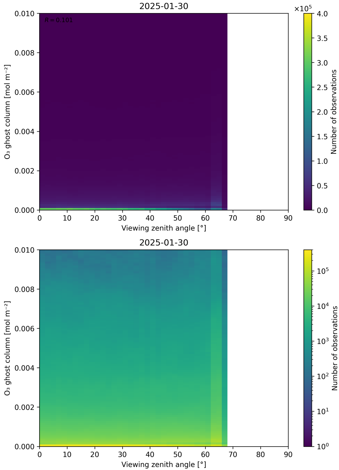
Figure 51: Scatter density plot of “Viewing zenith angle” against “O 3 ghost column” for 2025-01-29 to 2025-01-31.
