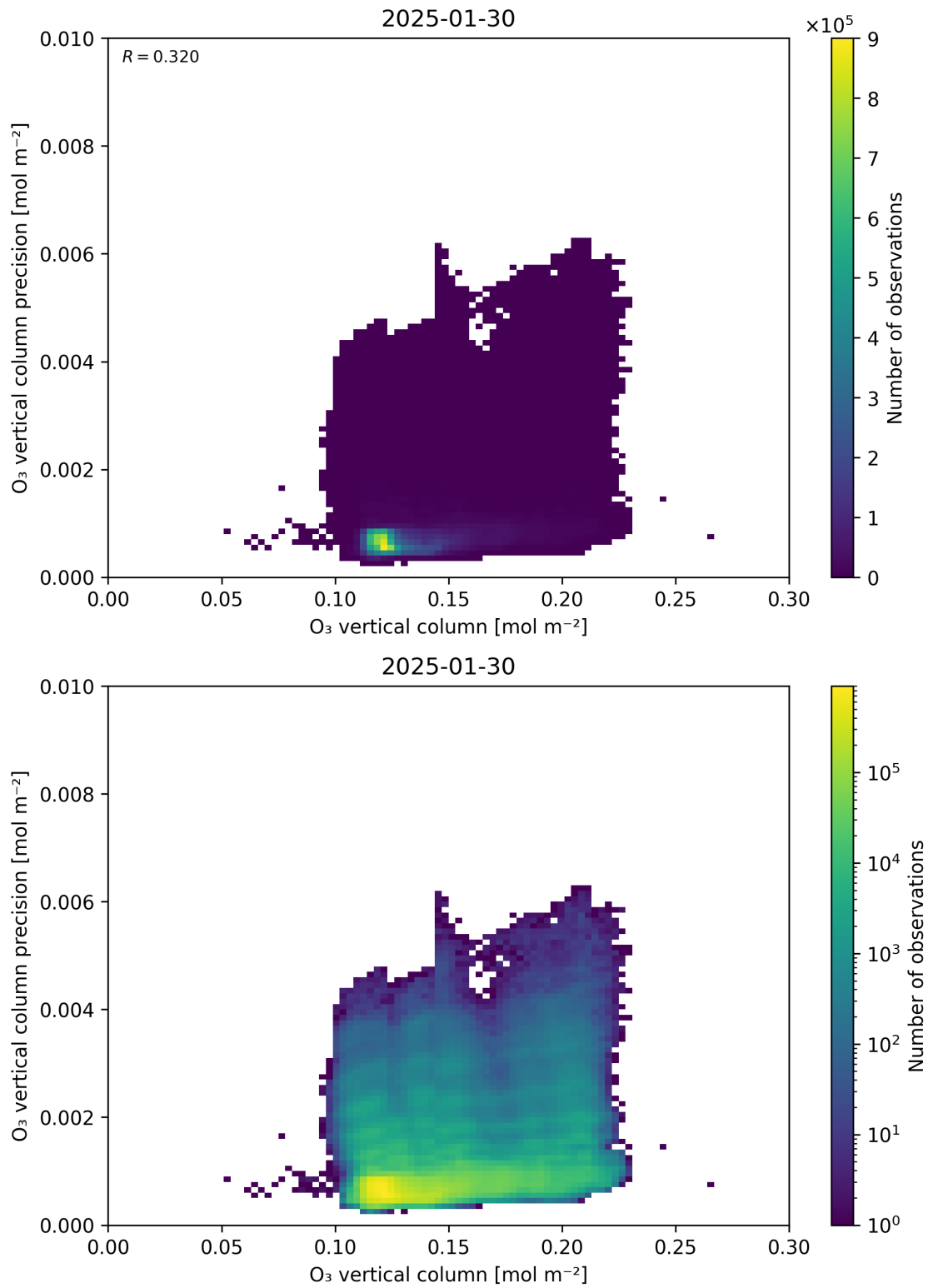
Figure 41: Scatter density plot of “O 3 vertical column” against “O 3 vertical column precision” for 2025-01-29 to 2025-01-31.
