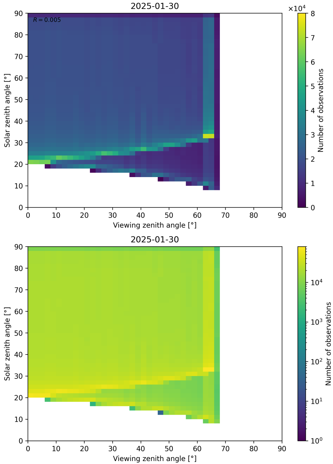
Figure 54: Scatter density plot of “Viewing zenith angle” against “Solar zenith angle” for 2025-01-29 to 2025-01-31.
