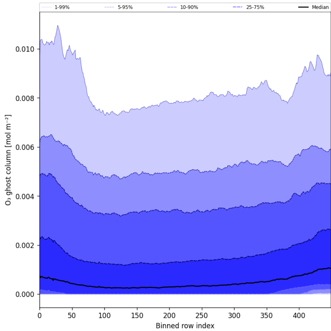
Figure 32: Along track statistics of “O 3 ghost column” for 2025-01-29 to 2025-01-31
