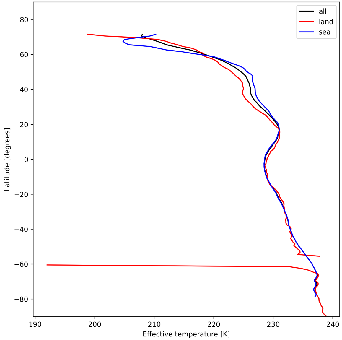
Figure 17: Zonal average of "Effective temperature" for 2025-01-29 to 2025-01-31.
