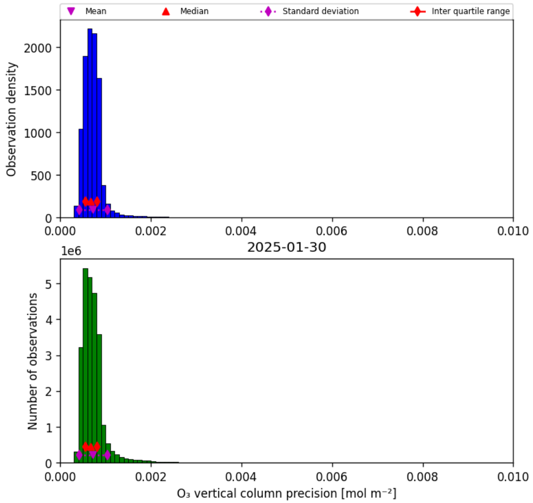
Figure 22: Histogram of “O 3 vertical column precision” for 2025-01-29 to 2025-01-31
