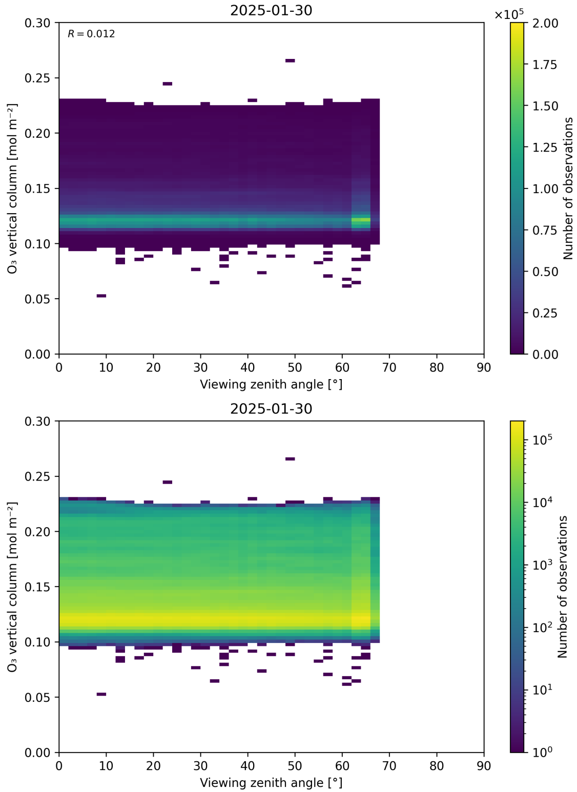
Figure 52: Scatter density plot of “Viewing zenith angle” against “O 3 vertical column” for 2025-01-29 to 2025-01-31.
