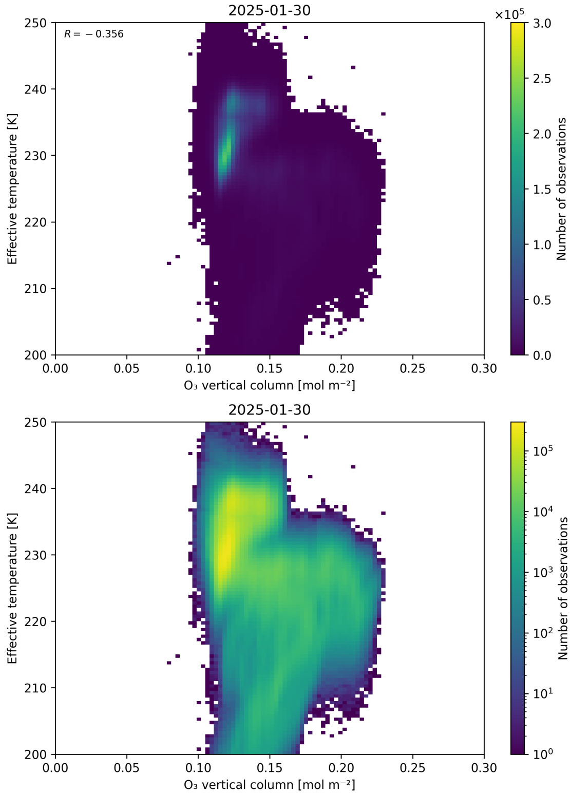
Figure 39: Scatter density plot of “O 3 vertical column” against “Effective temperature” for 2025-01-29 to 2025-01-31.
