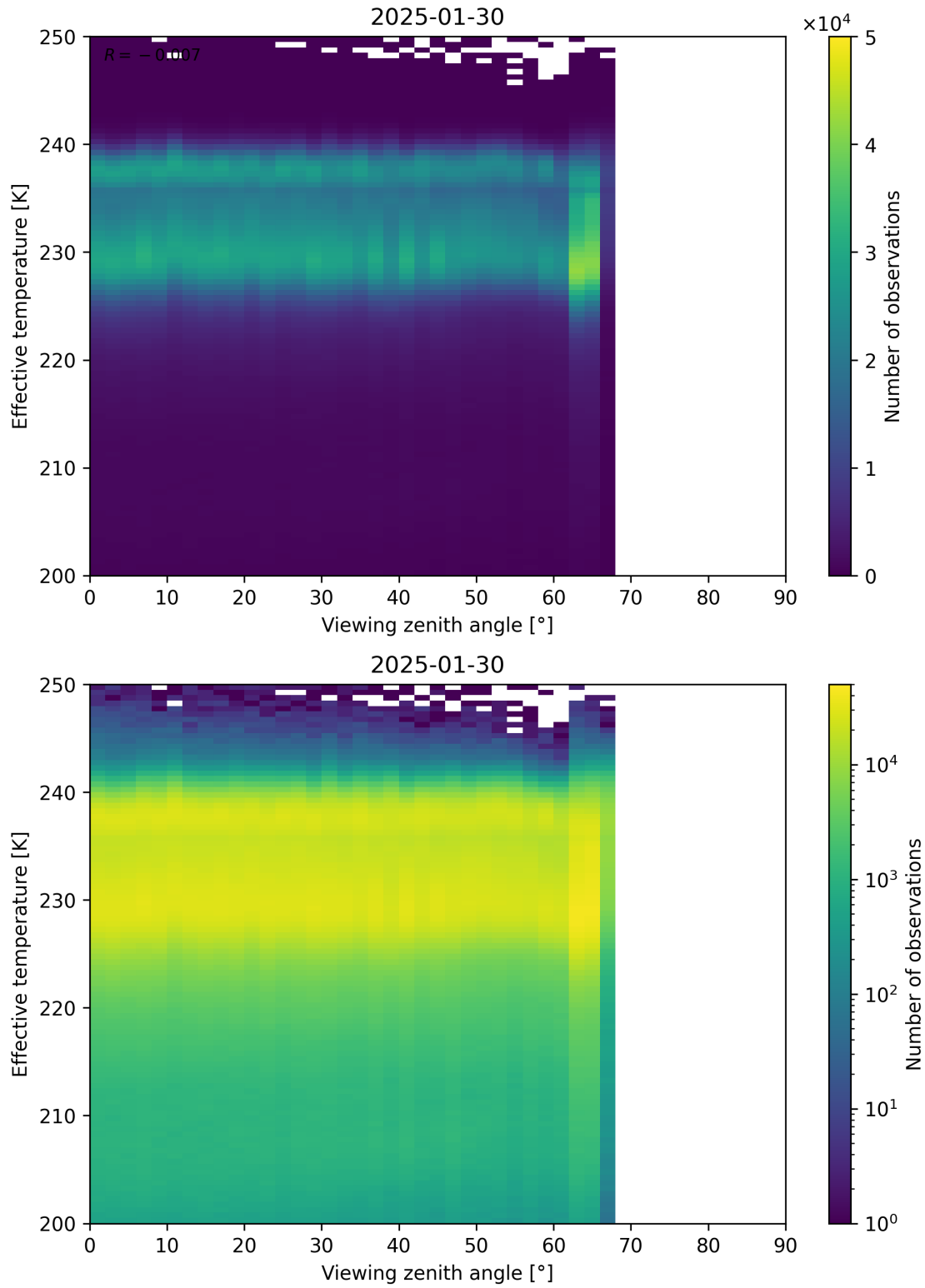
Figure 50: Scatter density plot of “Viewing zenith angle” against “Effective temperature” for 2025-01-29 to 2025-01-31.
