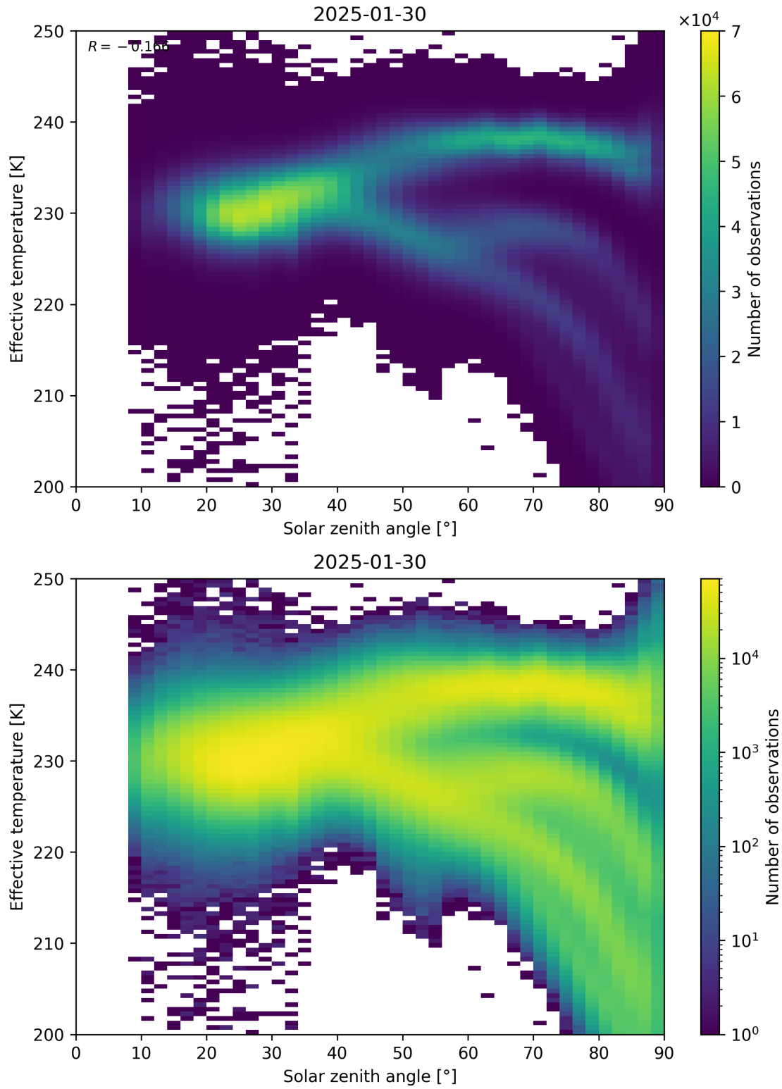
Figure 45: Scatter density plot of “Solar zenith angle” against “Effective temperature” for 2025-01-29 to 2025-01-31.
