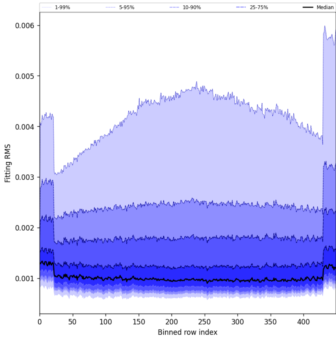
Figure 30: Along track statistics of “Fitting RMS” for 2025-01-29 to 2025-01-31
