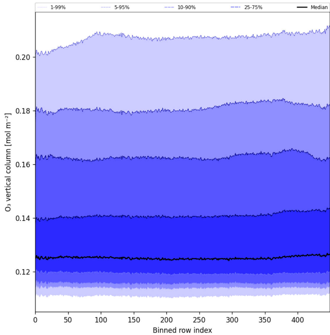
Figure 28: Along track statistics of “O 3 vertical column” for 2025-01-29 to 2025-01-31
