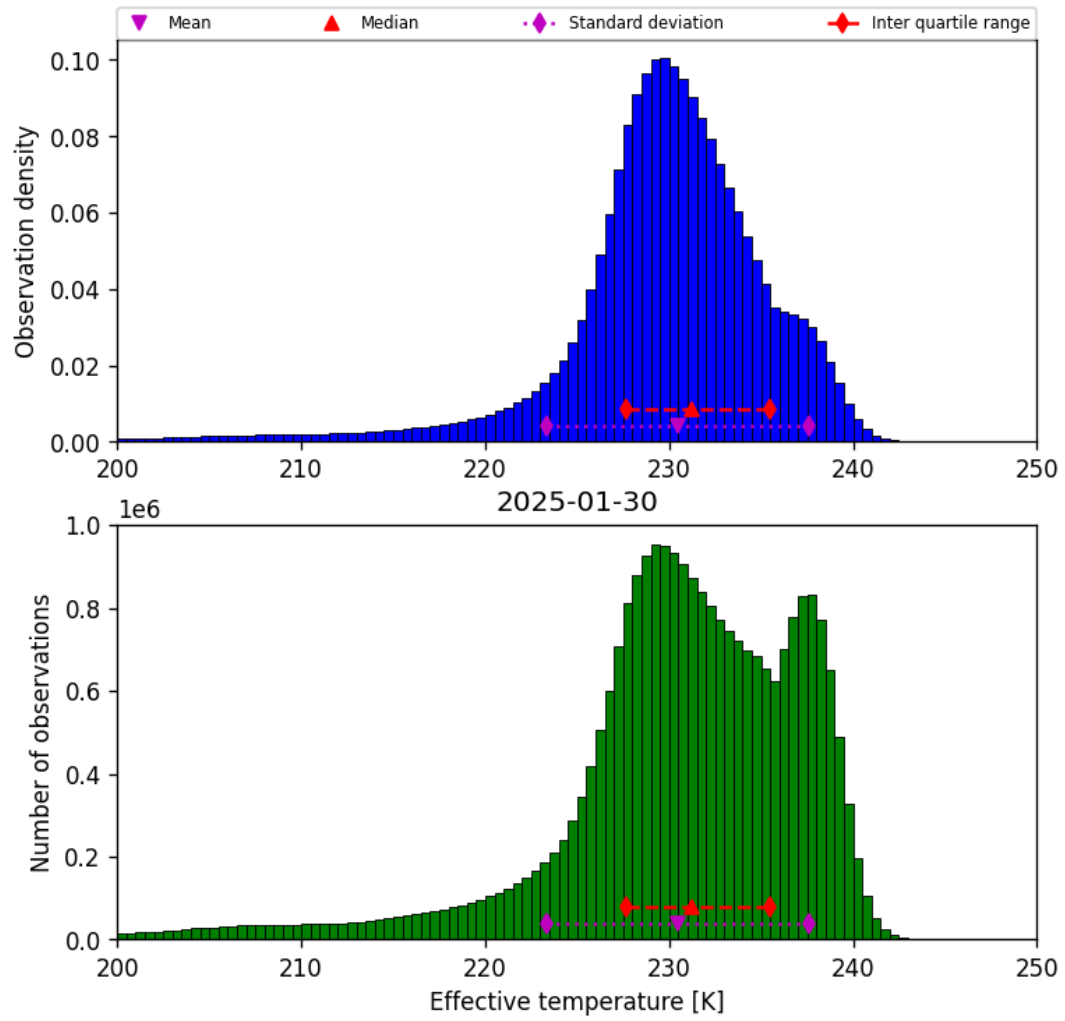
Figure 24: Histogram of “Effective temperature” for 2025-01-29 to 2025-01-31
