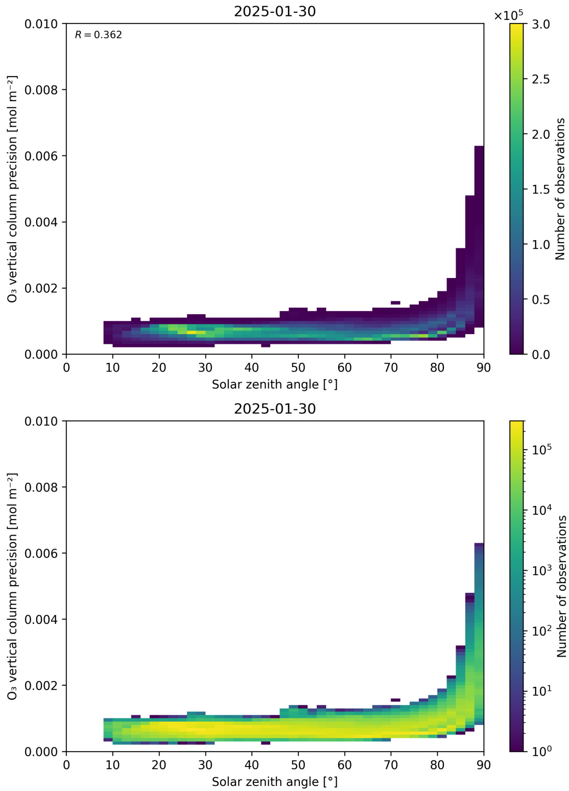
Figure 48: Scatter density plot of “Solar zenith angle” against “O 3 vertical column precision” for 2025-01-29 to 2025-01-31.
