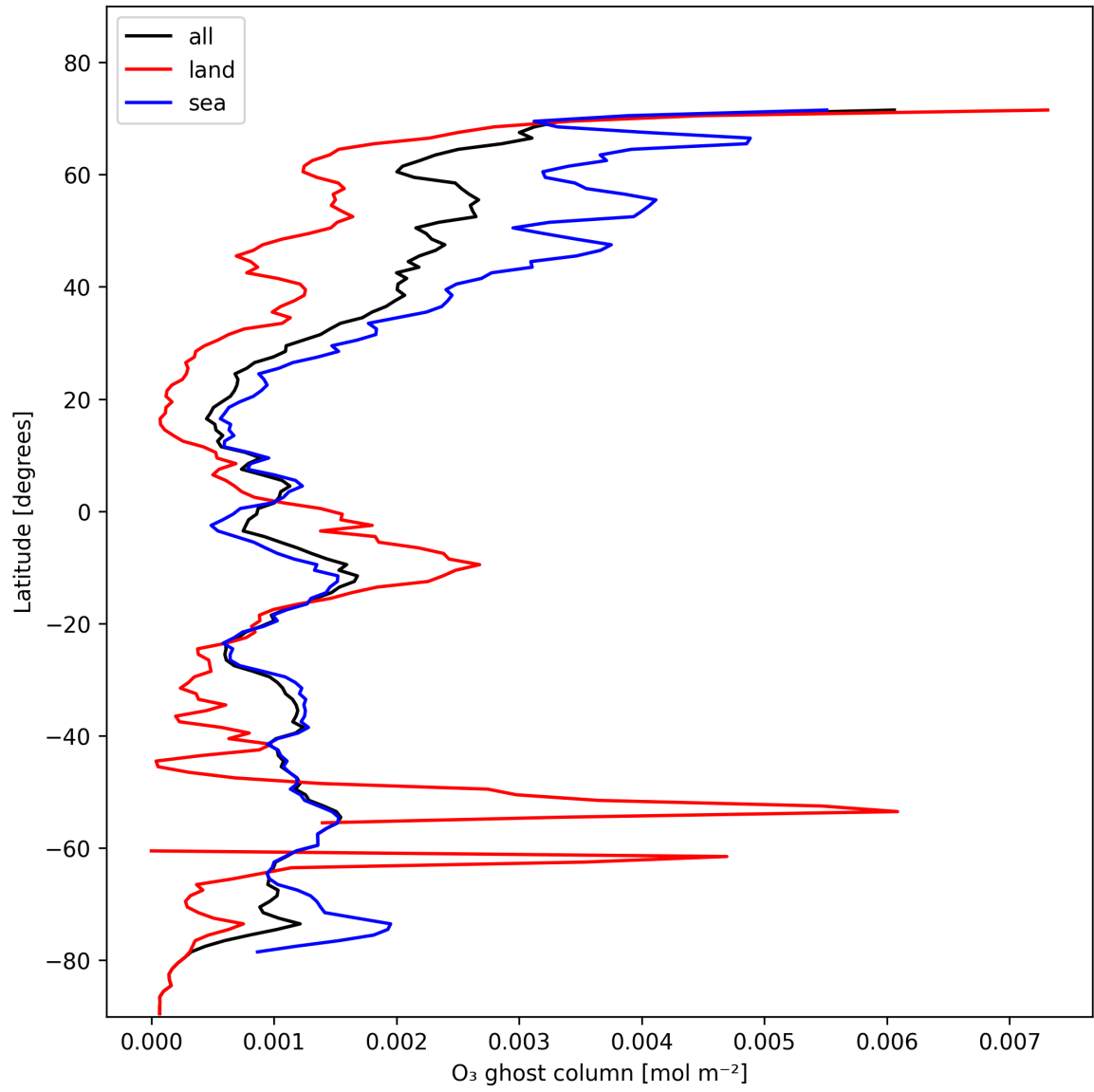
Figure 18: Zonal average of “O 3 ghost column” for 2025-01-29 to 2025-01-31.
