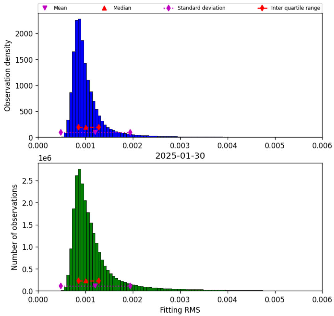
Figure 23: Histogram of “Fitting RMS” for 2025-01-29 to 2025-01-31
