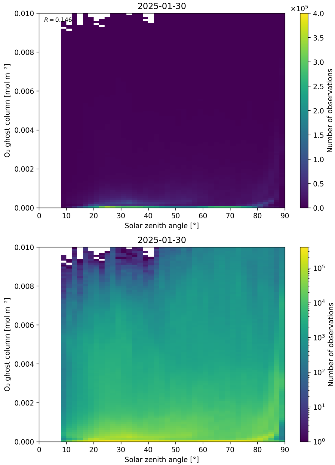
Figure 46: Scatter density plot of “Solar zenith angle” against “O 3 ghost column” for 2025-01-29 to 2025-01-31.
