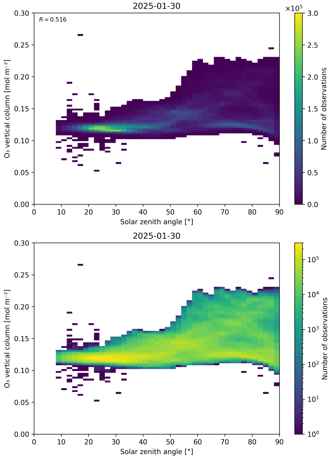
Figure 47: Scatter density plot of “Solar zenith angle” against “O 3 vertical column” for 2025-01-29 to 2025-01-31.
