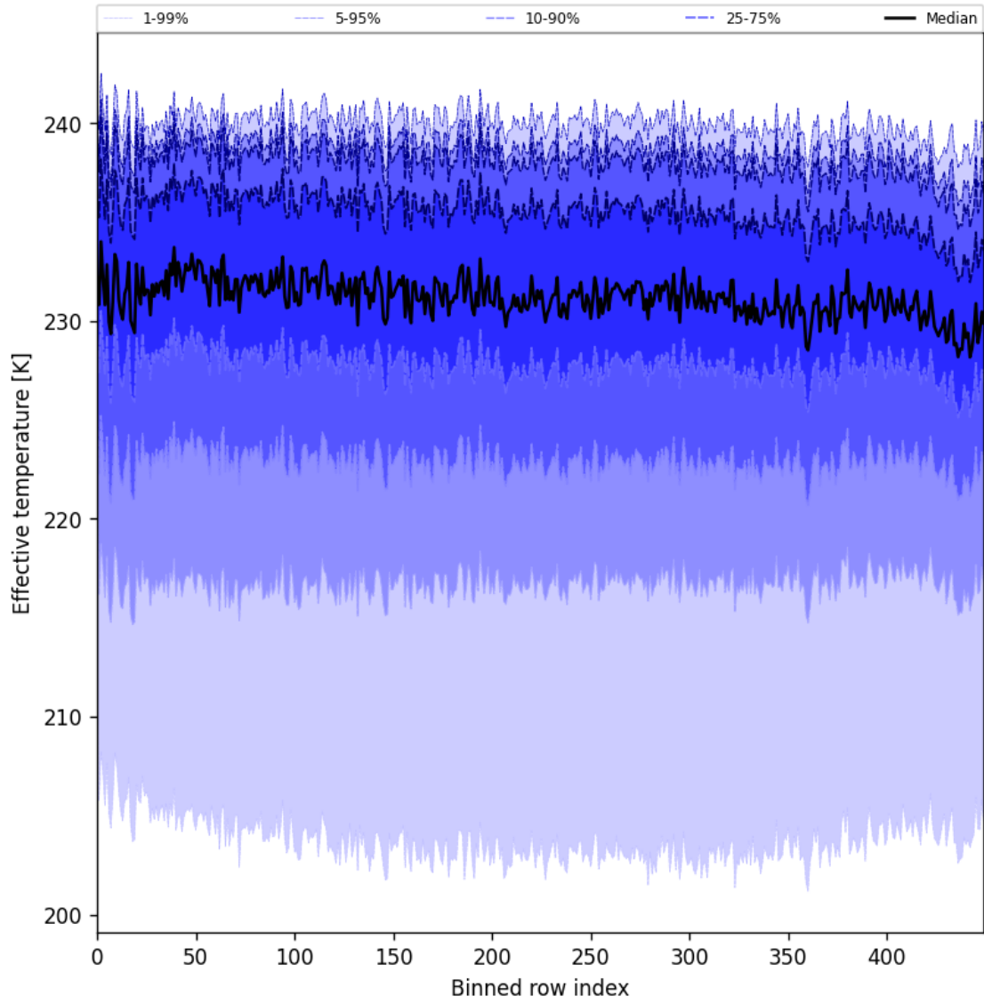
Figure 31: Along track statistics of “Effective temperature” for 2025-01-29 to 2025-01-31
