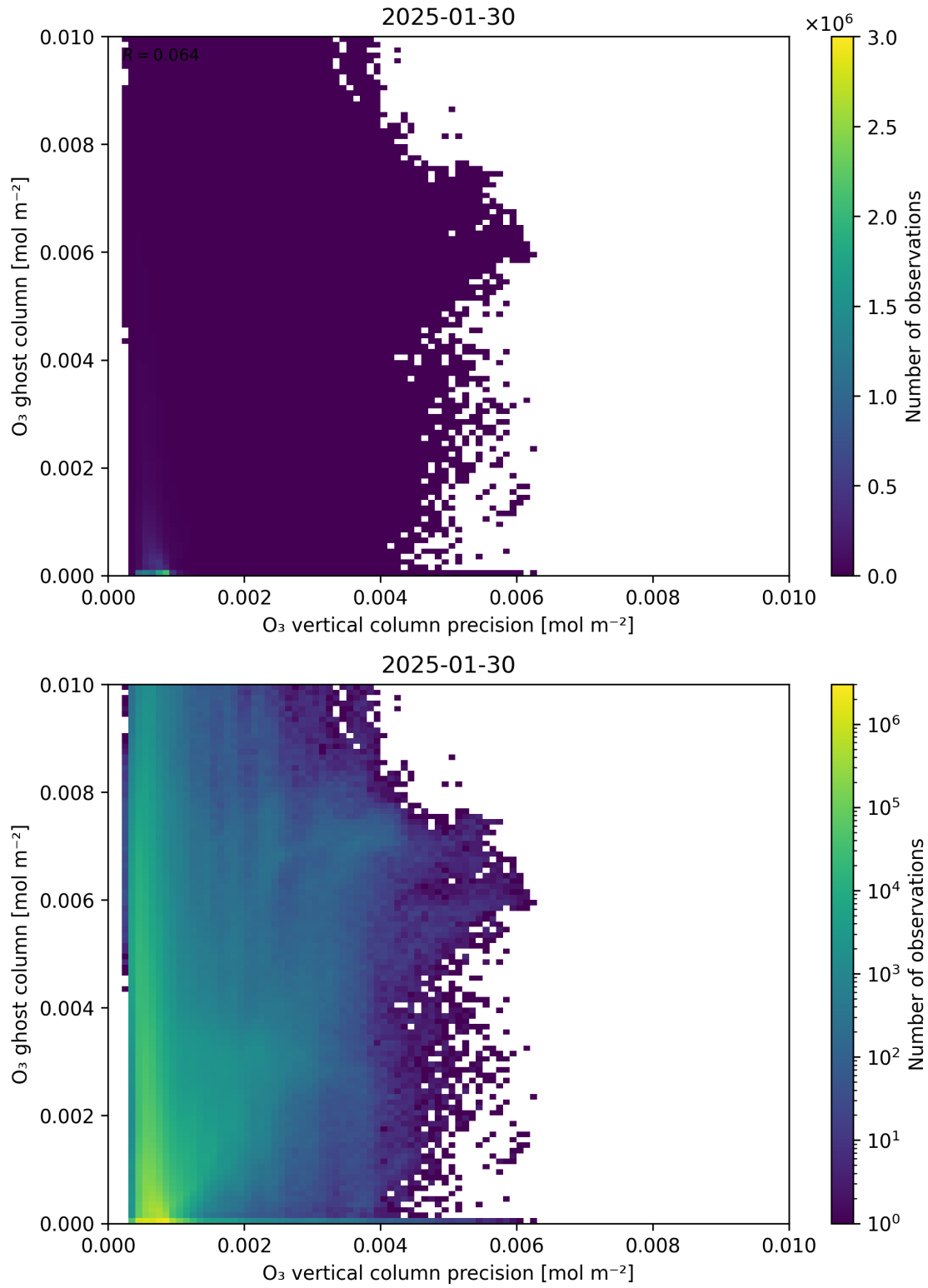
Figure 43: Scatter density plot of “O 3 vertical column precision” against “O 3 ghost column” for 2025-01-29 to 2025-01-31.
