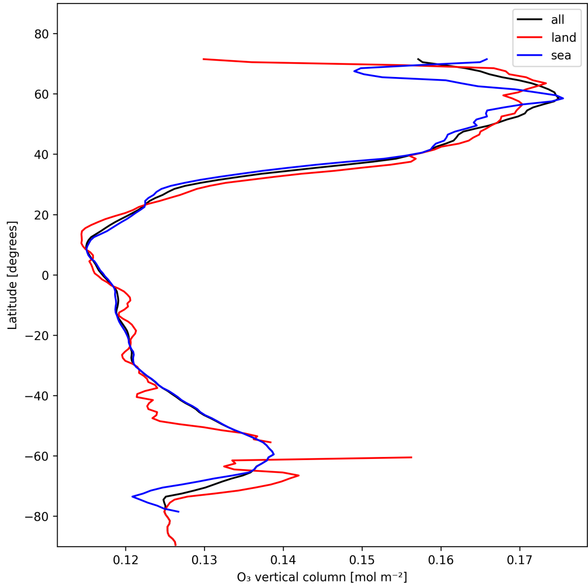
Figure 14: Zonal average of “O 3 vertical column” for 2025-01-29 to 2025-01-31.
