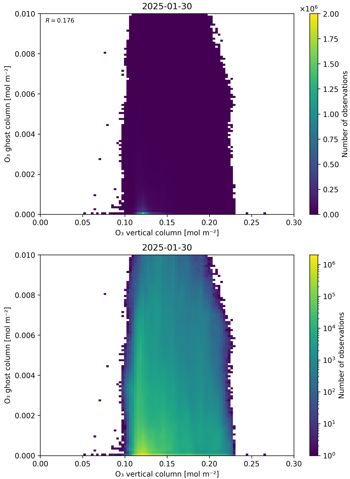
Figure 40: Scatter density plot of “O 3 vertical column” against “O 3 ghost column” for 2025-01-29 to 2025-01-31.
