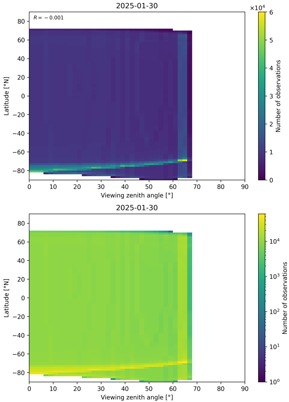
Figure 49: Scatter density plot of “Viewing zenith angle” against “Latitude” for 2025-01-29 to 2025-01-31.
