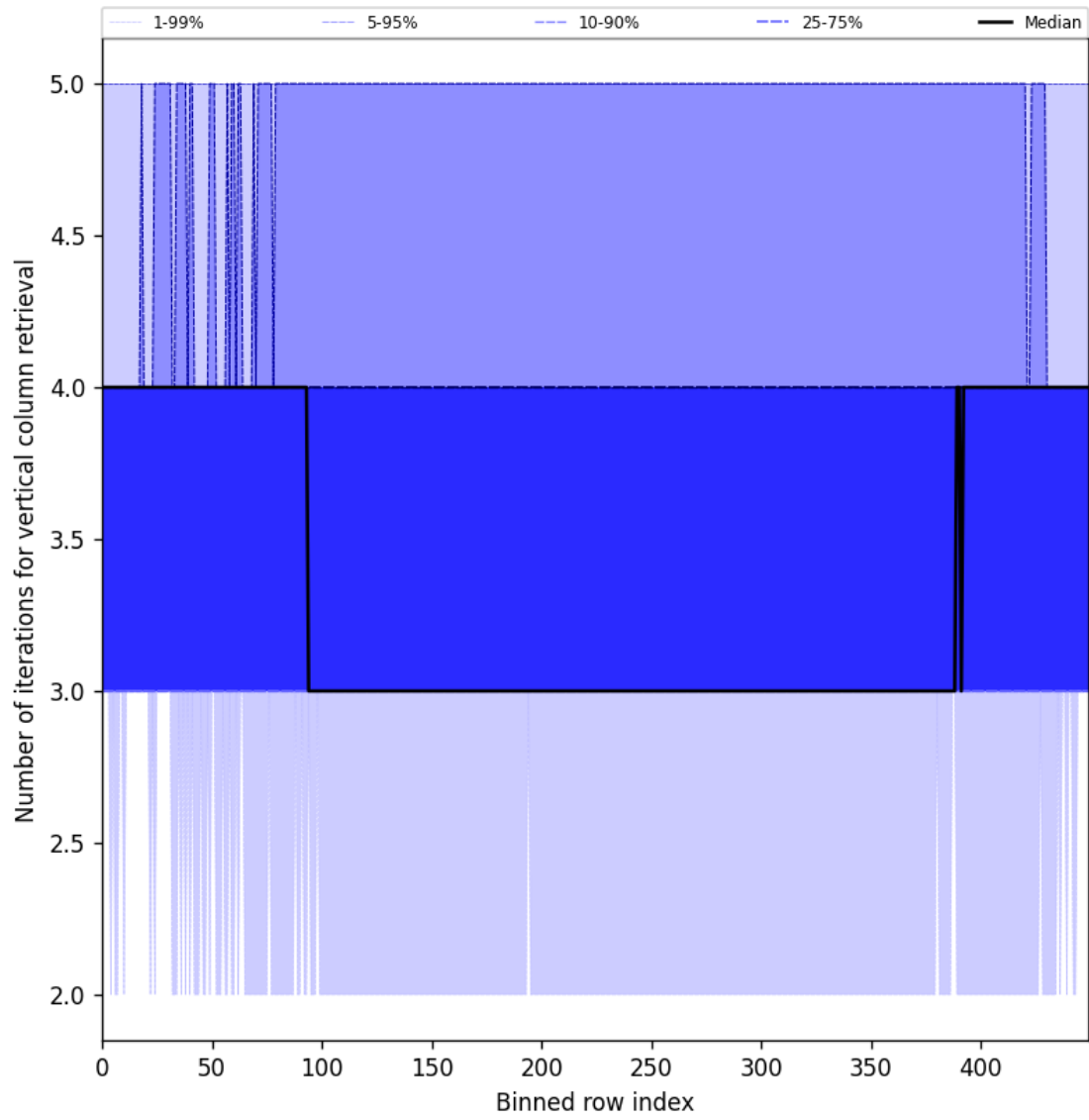
Figure 33: Along track statistics of “Number of iterations for vertical column retrieval” for 2025-01-29 to 2025-01-31
