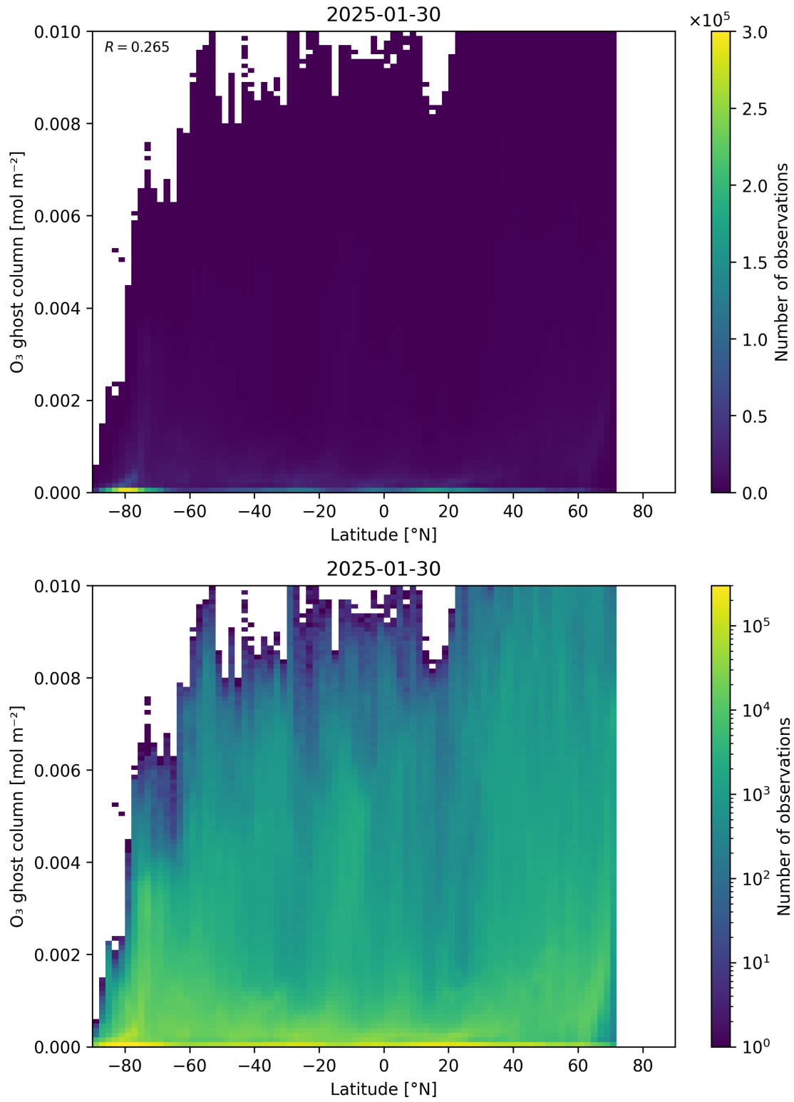
Figure 35: Scatter density plot of “Latitude” against “O 3 ghost column” for 2025-01-29 to 2025-01-31.
