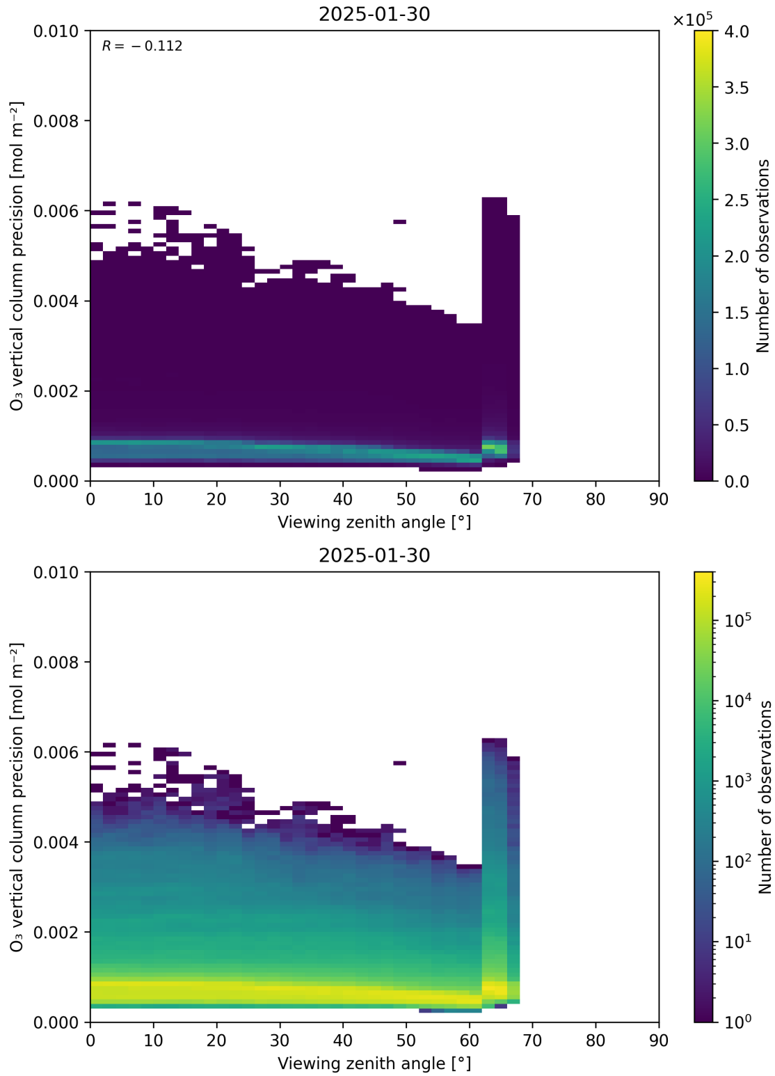
Figure 53: Scatter density plot of “Viewing zenith angle” against “O 3 vertical column precision” for 2025-01-29 to 2025-01-31.
