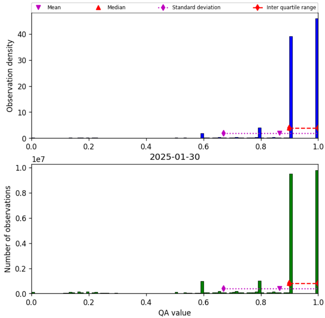
Figure 20: Histogram of “QA value” for 2025-01-29 to 2025-01-31
