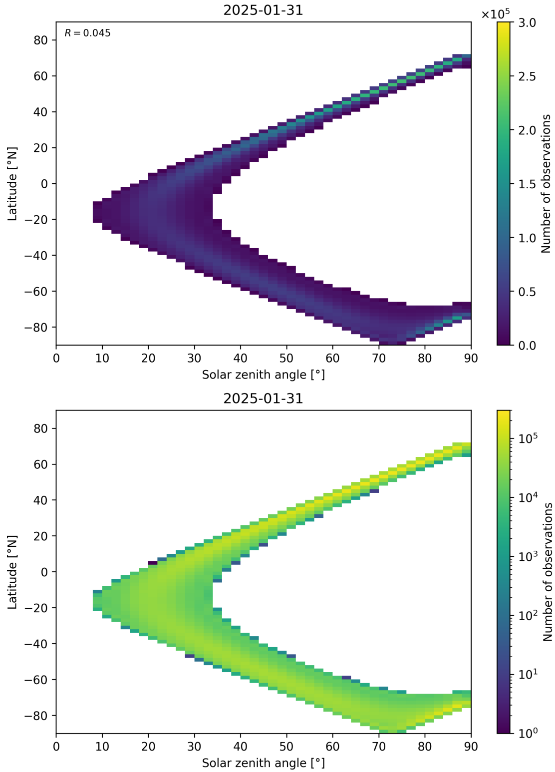
Figure 44: Scatter density plot of “Solar zenith angle” against “Latitude” for 2025-01-30 to 2025-02-01.
