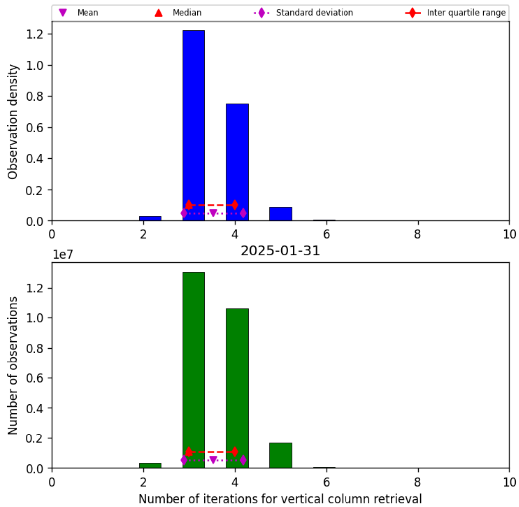
Figure 26: Histogram of “Number of iterations for vertical column retrieval” for 2025-01-30 to 2025-02-01
