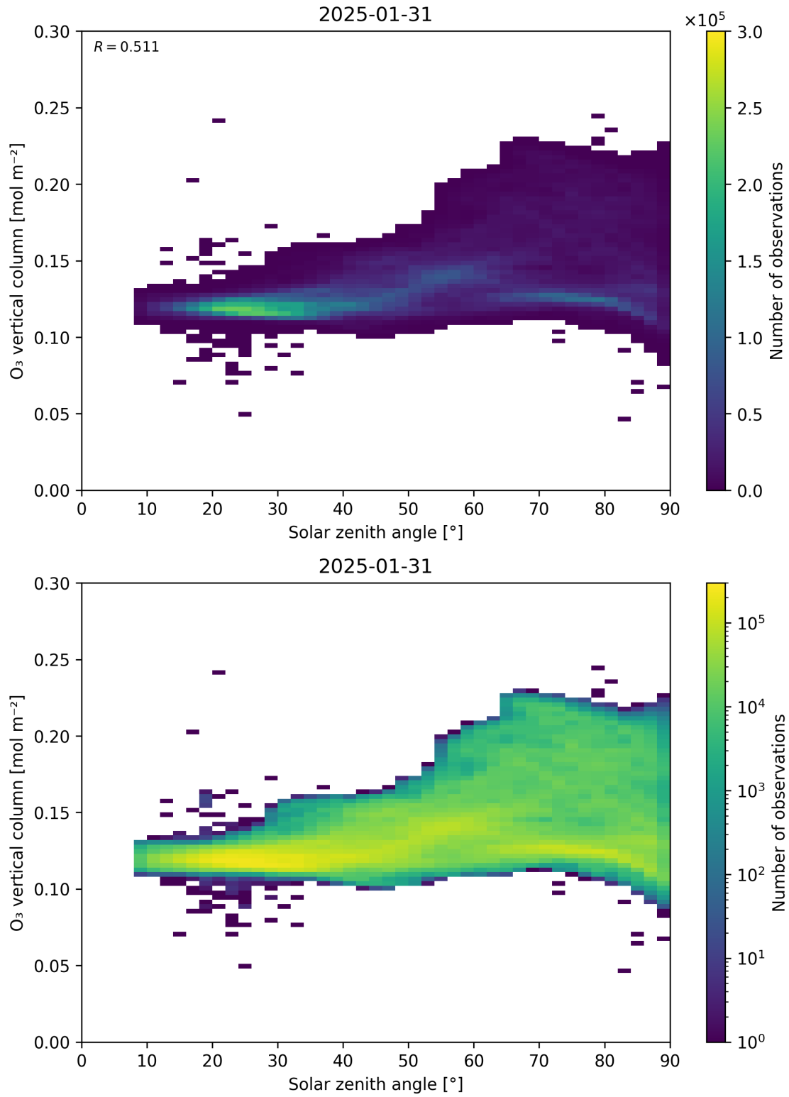
Figure 47: Scatter density plot of “Solar zenith angle” against “O 3 vertical column” for 2025-01-30 to 2025-02-01.
