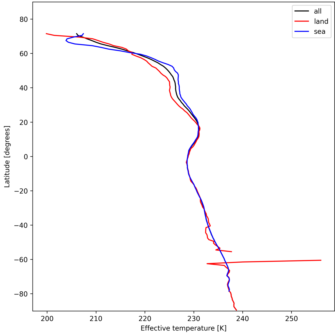
Figure 17: Zonal average of “Effective temperature” for 2025-01-30 to 2025-02-01.
