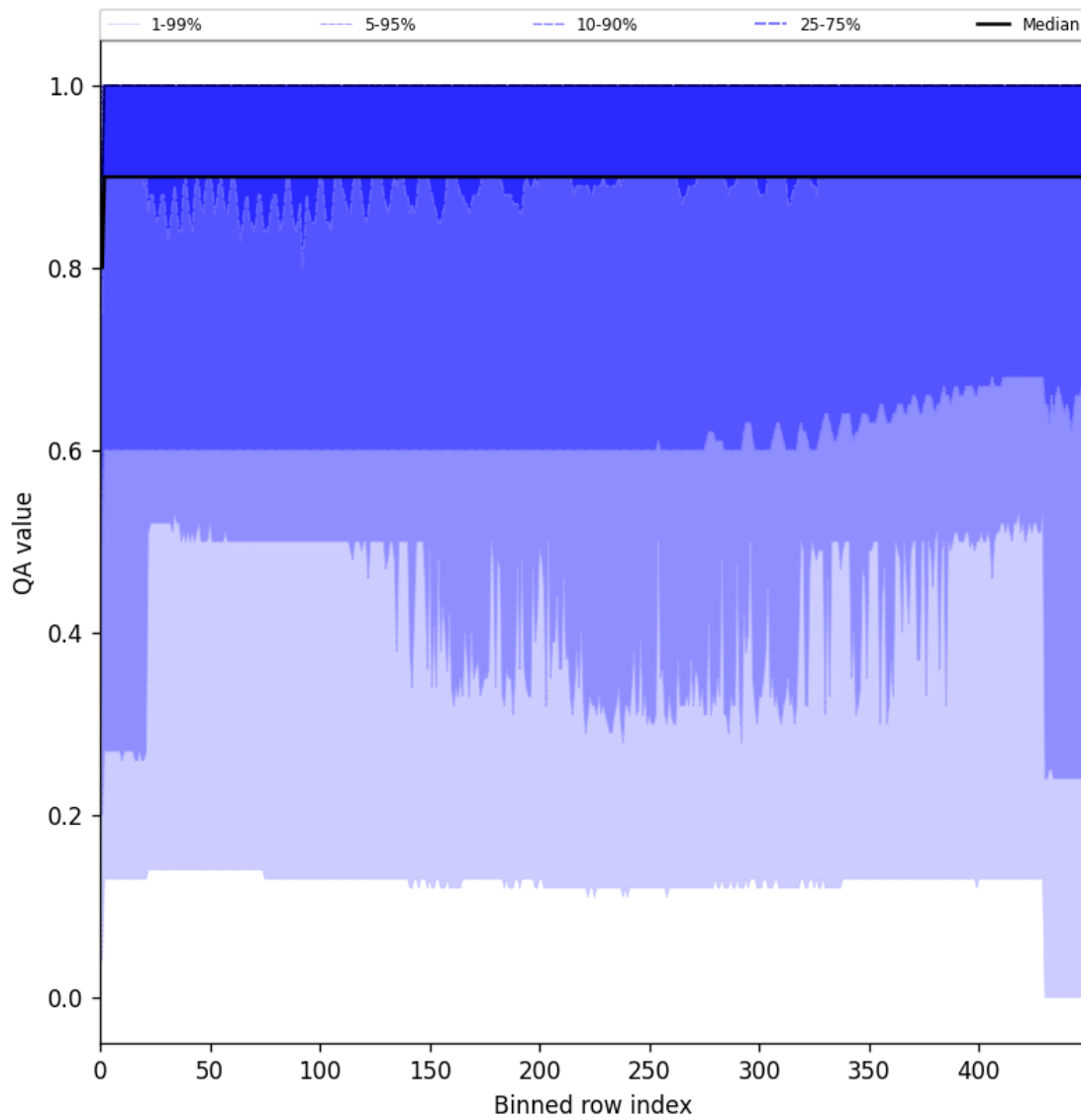
Figure 27: Along track statistics of “QA value” for 2025-01-30 to 2025-02-01
