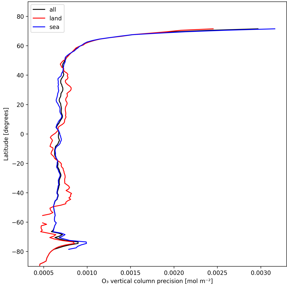
Figure 15: Zonal average of “O 3 vertical column precision” for 2025-01-30 to 2025-02-01.
