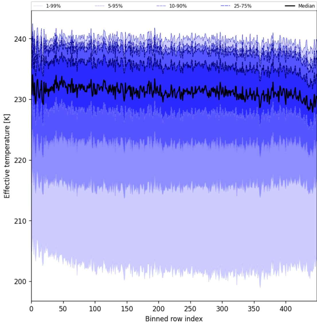
Figure 31: Along track statistics of “Effective temperature” for 2025-01-30 to 2025-02-01
