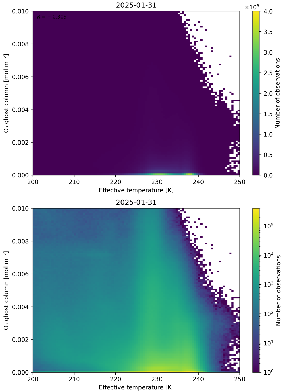
Figure 38: Scatter density plot of “Effective temperature” against “O 3 ghost column” for 2025-01-30 to 2025-02-01.
