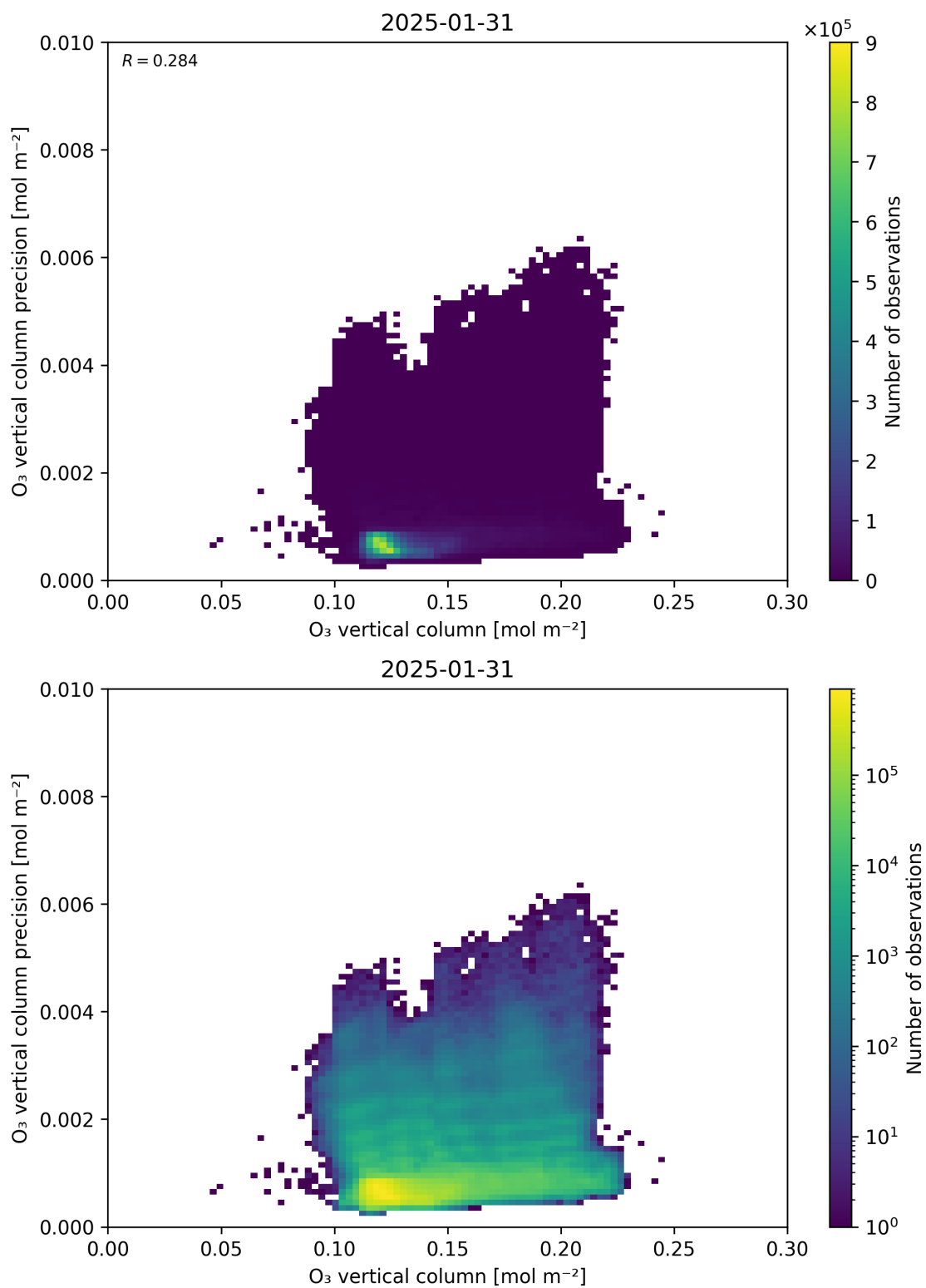
Figure 41: Scatter density plot of “O 3 vertical column” against “O 3 vertical column precision” for 2025-01-30 to 2025-02-01.
