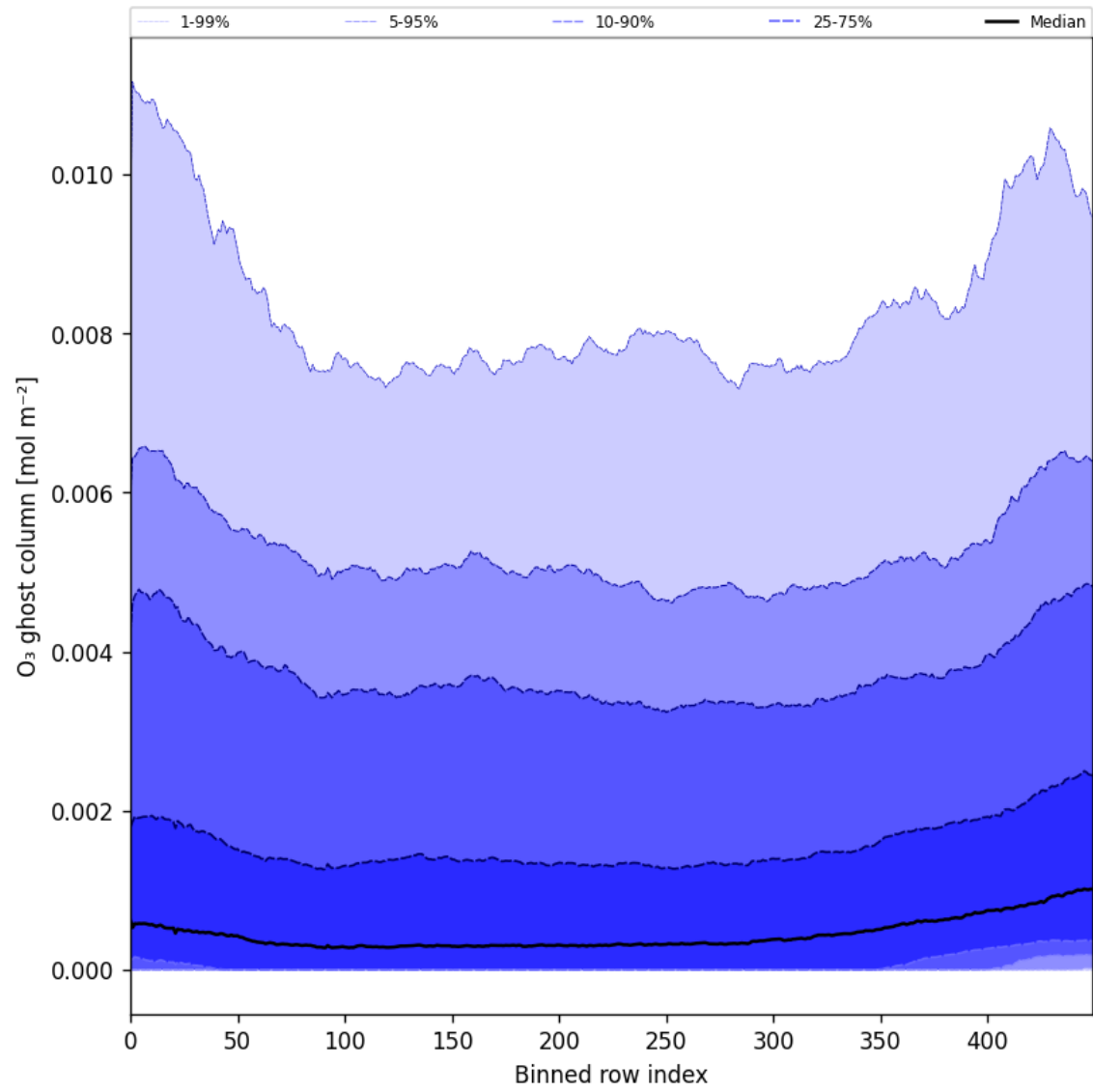
Figure 32: Along track statistics of “O 3 ghost column” for 2025-01-30 to 2025-02-01
