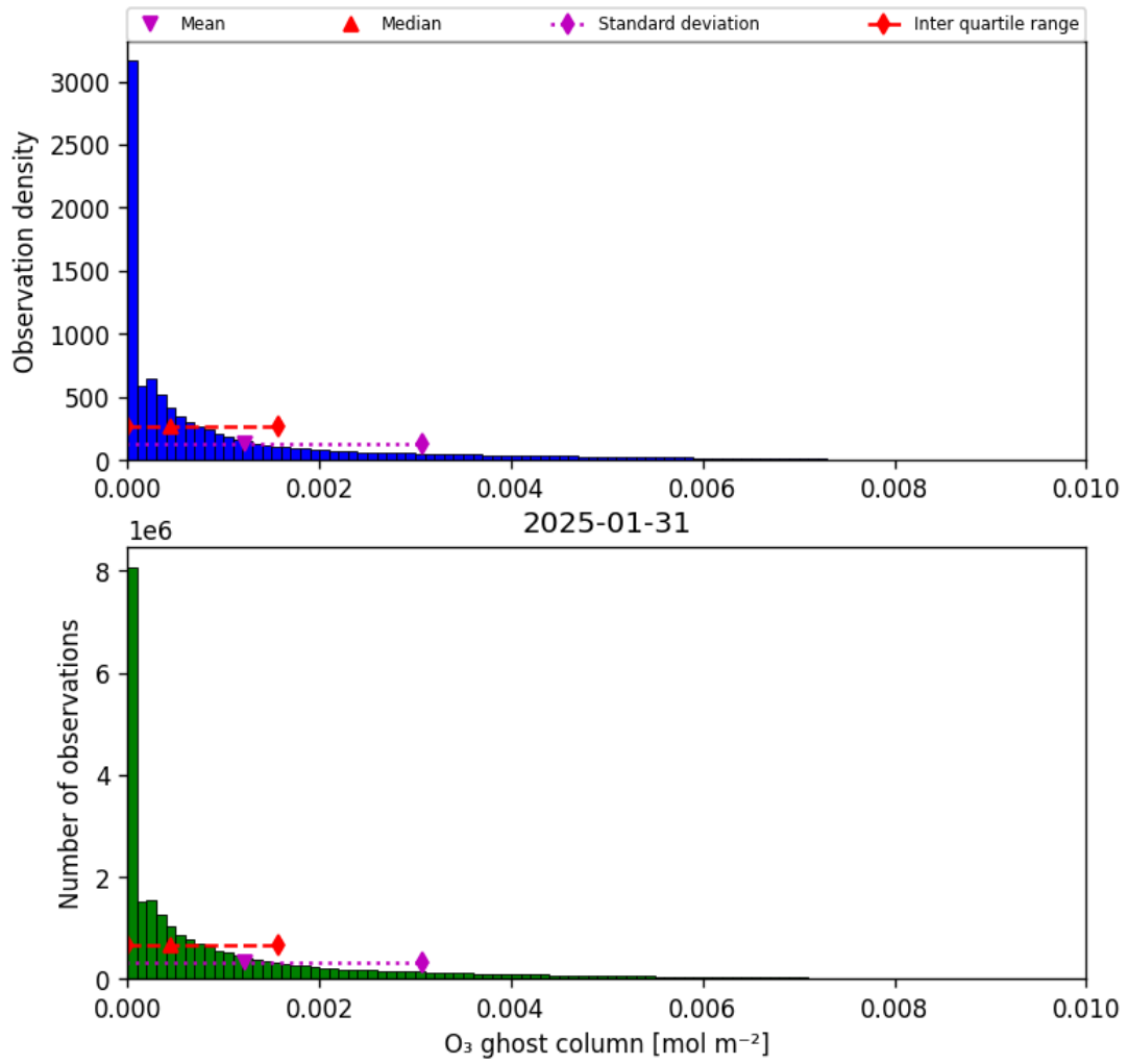
Figure 25: Histogram of "O 3 ghost column" for 2025-01-30 to 2025-02-01
