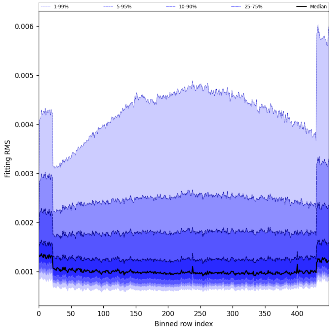
Figure 30: Along track statistics of “Fitting RMS” for 2025-01-30 to 2025-02-01
