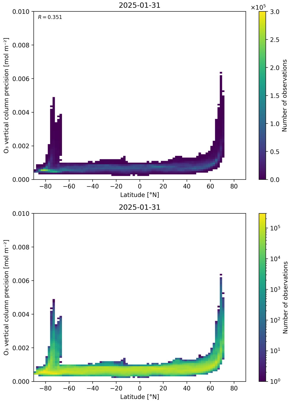
Figure 37: Scatter density plot of “Latitude” against “O 3 vertical column precision” for 2025-01-30 to 2025-02-01.
