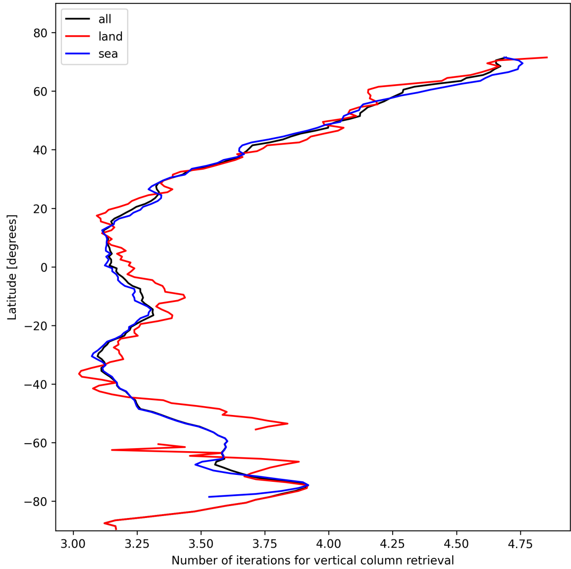
Figure 19: Zonal average of “Number of iterations for vertical column retrieval” for 2025-01-30 to 2025-02-01.
