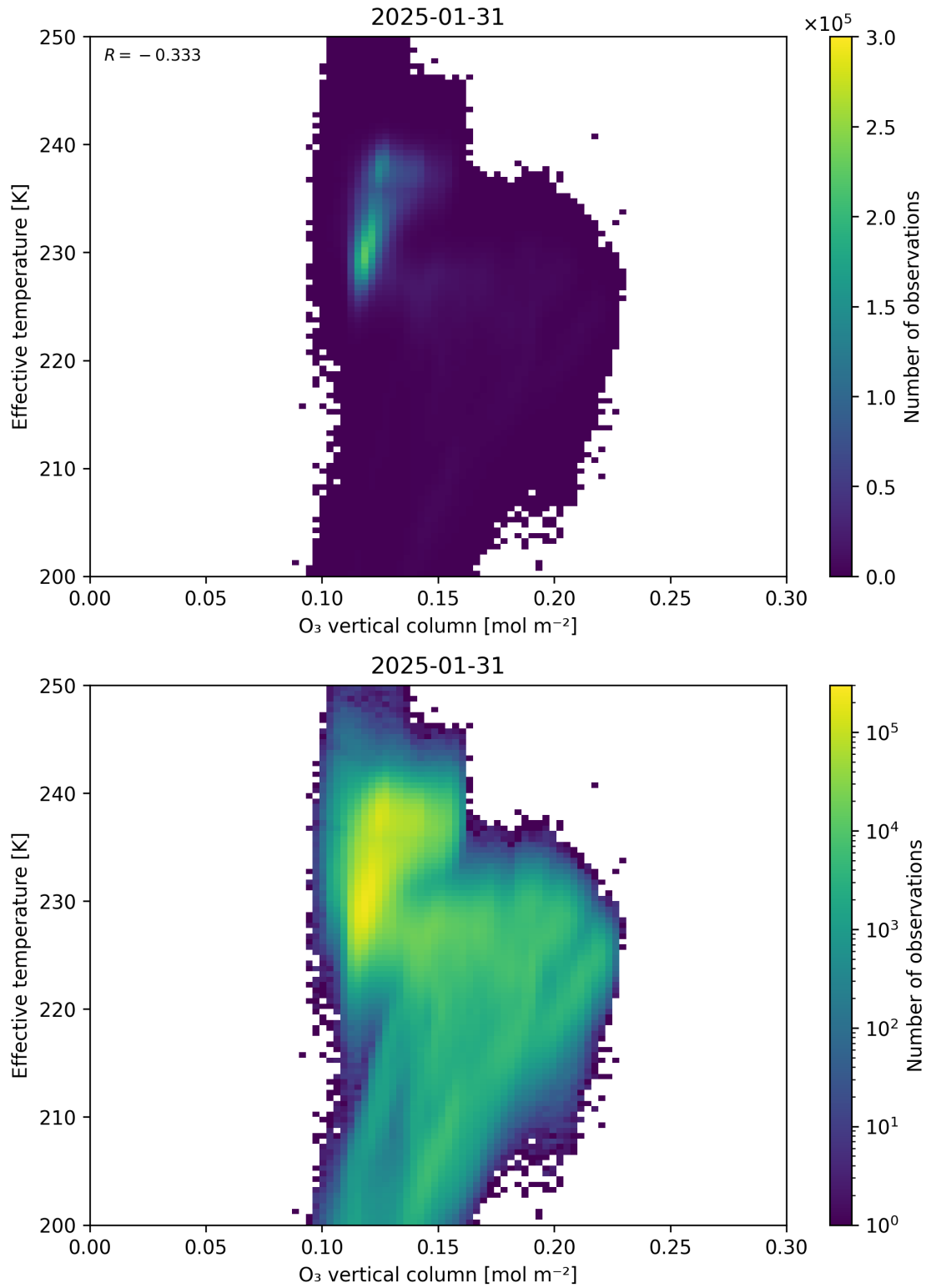
Figure 39: Scatter density plot of “O 3 vertical column” against “Effective temperature” for 2025-01-30 to 2025-02-01.
