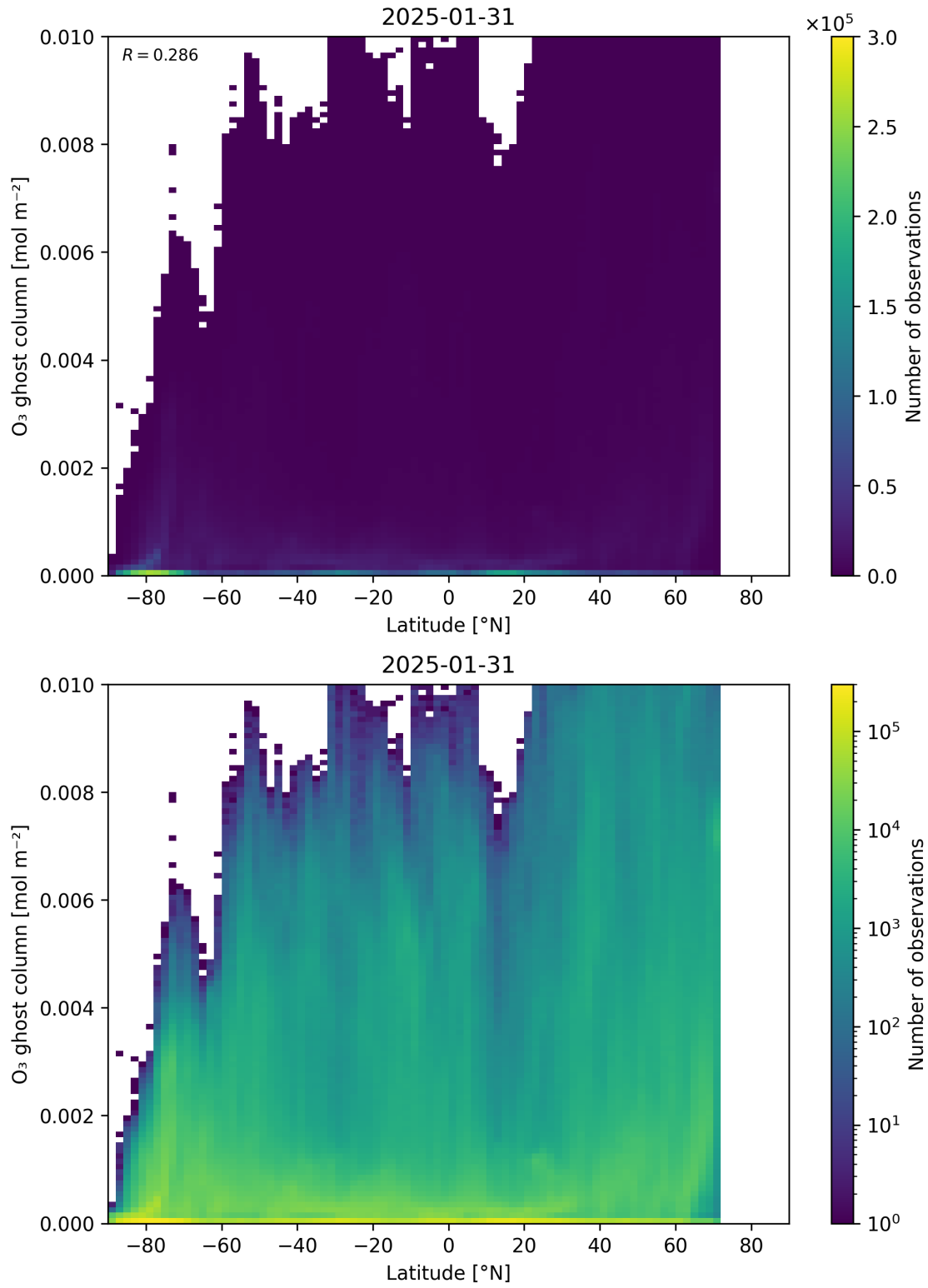
Figure 35: Scatter density plot of “Latitude” against “O 3 ghost column” for 2025-01-30 to 2025-02-01.
