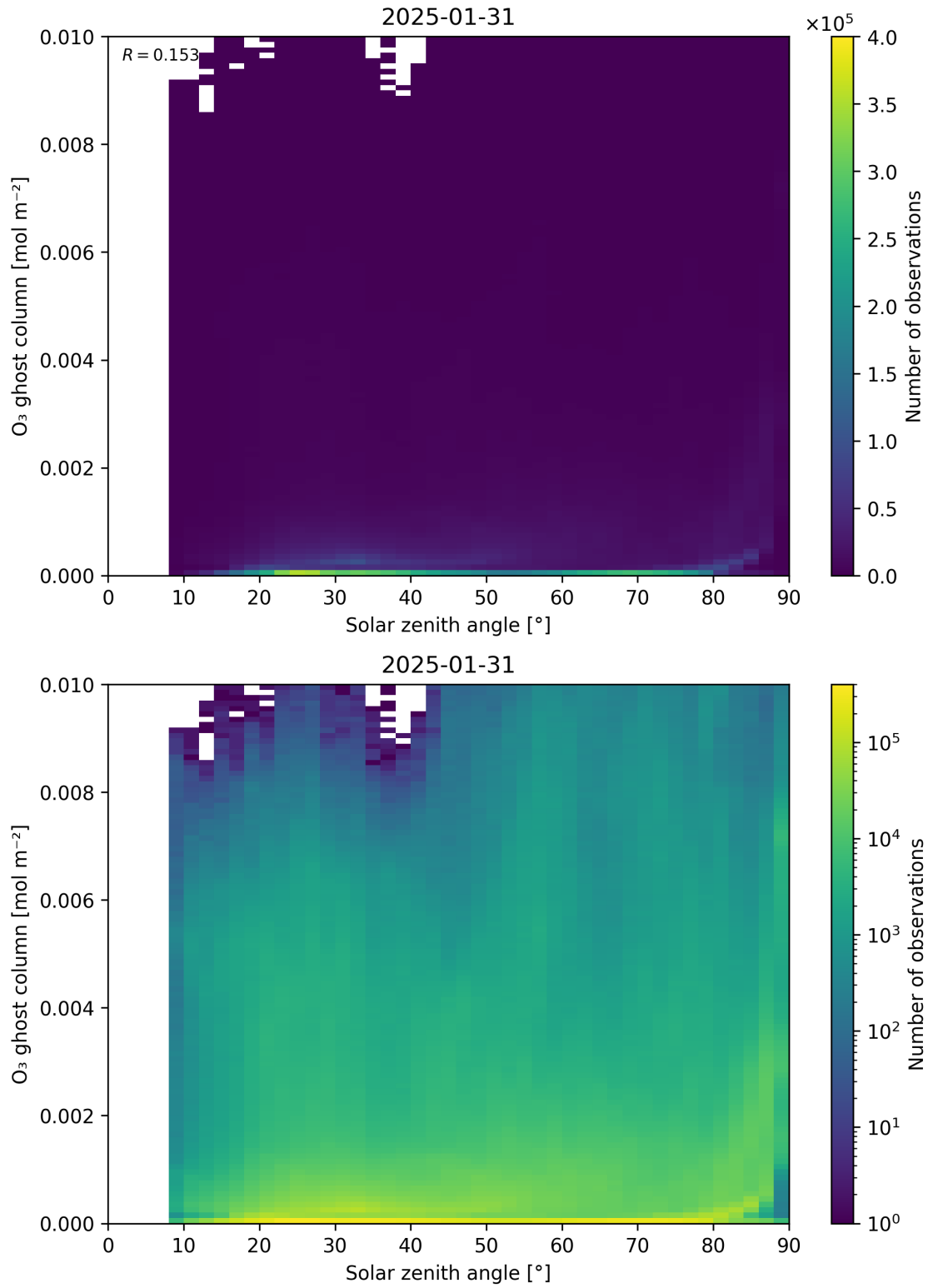
Figure 46: Scatter density plot of “Solar zenith angle” against “O 3 ghost column” for 2025-01-30 to 2025-02-01.
