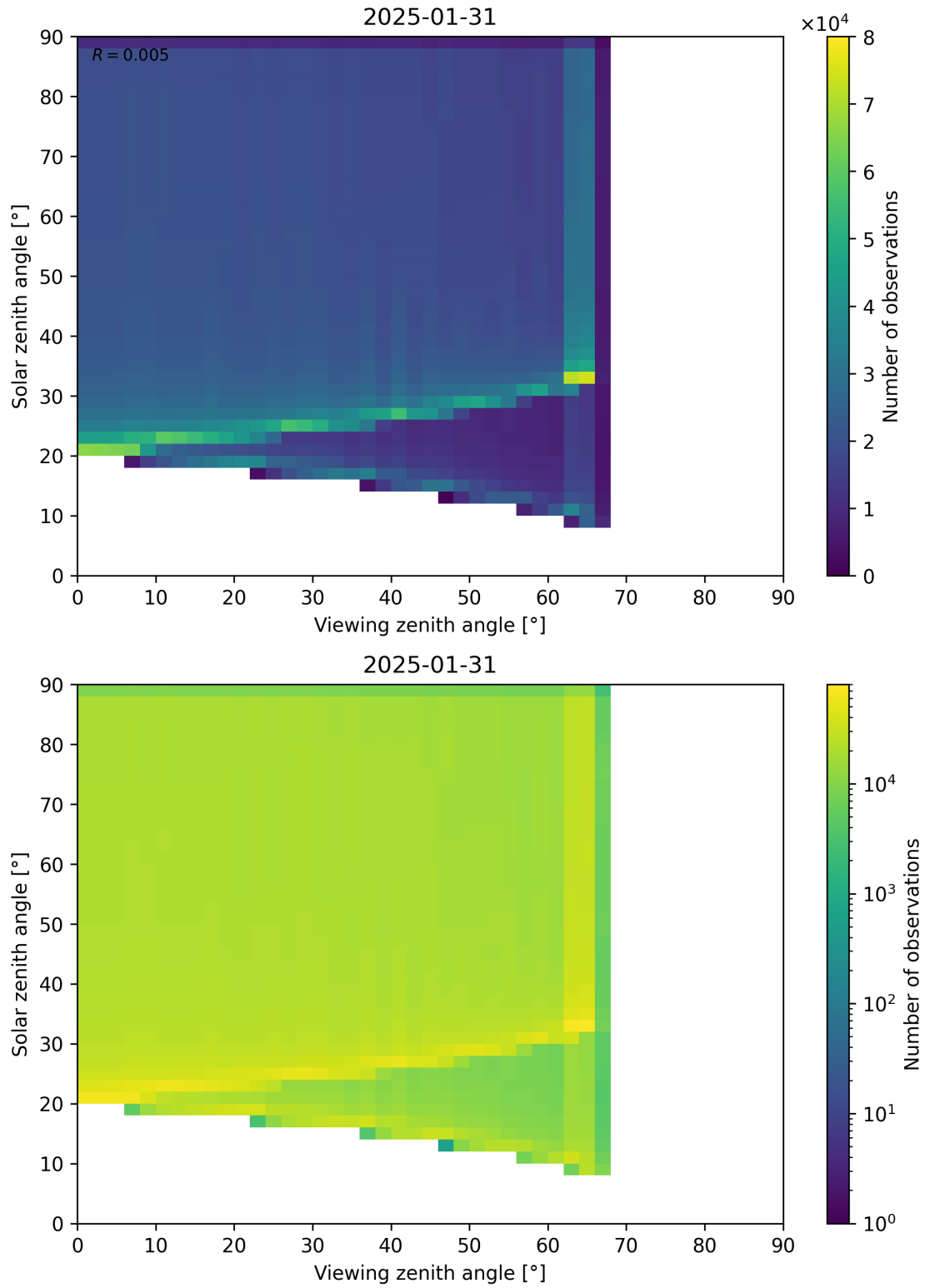
Figure 54: Scatter density plot of “Viewing zenith angle” against “Solar zenith angle” for 2025-01-30 to 2025-02-01.
