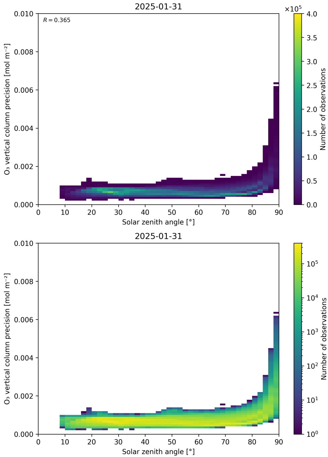
Figure 48: Scatter density plot of “Solar zenith angle” against “O 3 vertical column precision” for 2025-01-30 to 2025-02-01.
