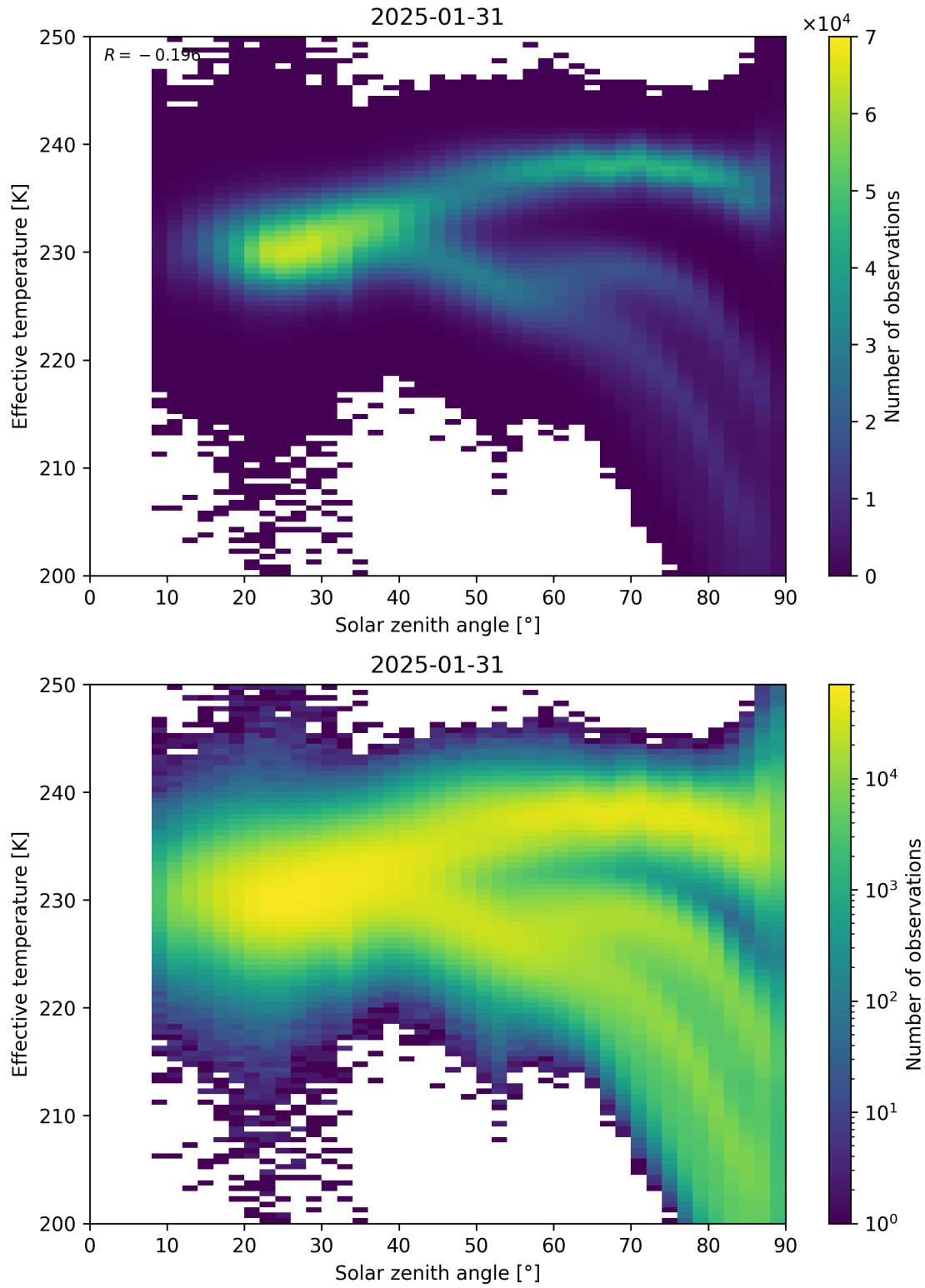
Figure 45: Scatter density plot of “Solar zenith angle” against “Effective temperature” for 2025-01-30 to 2025-02-01.
