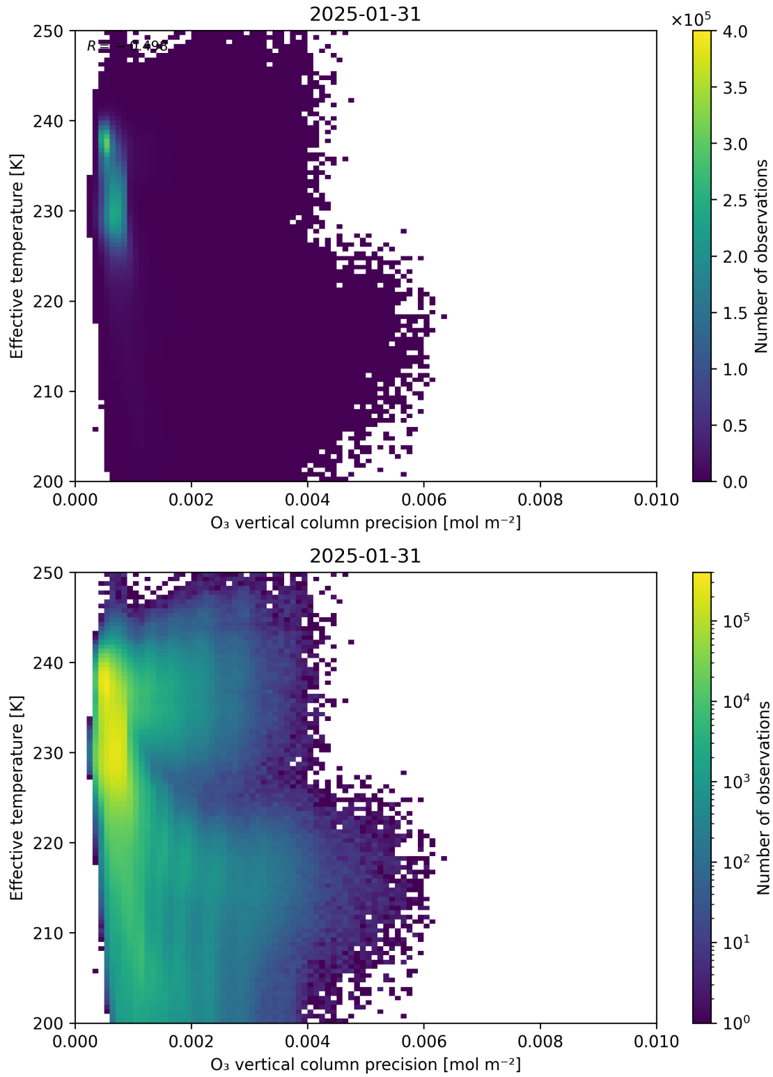
Figure 42: Scatter density plot of “O 3 vertical column precision” against “Effective temperature” for 2025-01-30 to 2025-02-01.
