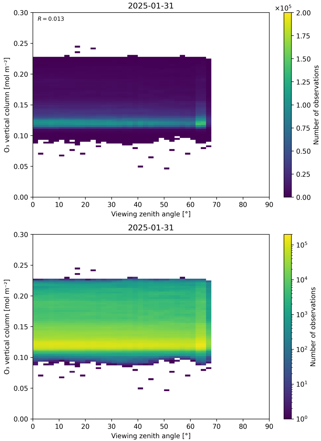
Figure 52: Scatter density plot of “Viewing zenith angle” against “O 3 vertical column” for 2025-01-30 to 2025-02-01.
