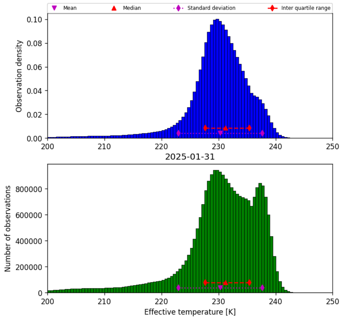
Figure 24: Histogram of “Effective temperature” for 2025-01-30 to 2025-02-01
