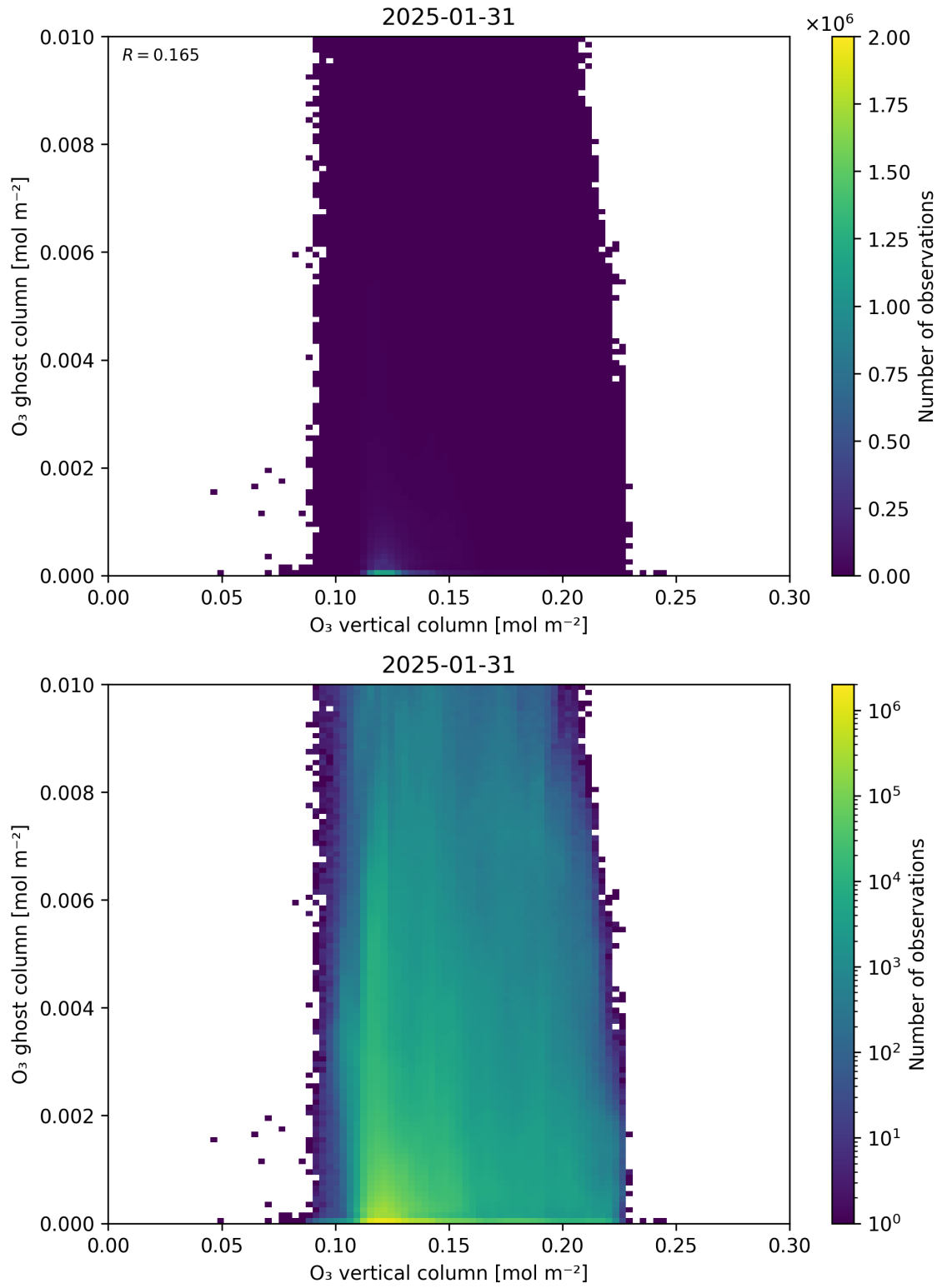
Figure 40: Scatter density plot of “O 3 vertical column” against “O 3 ghost column” for 2025-01-30 to 2025-02-01.
