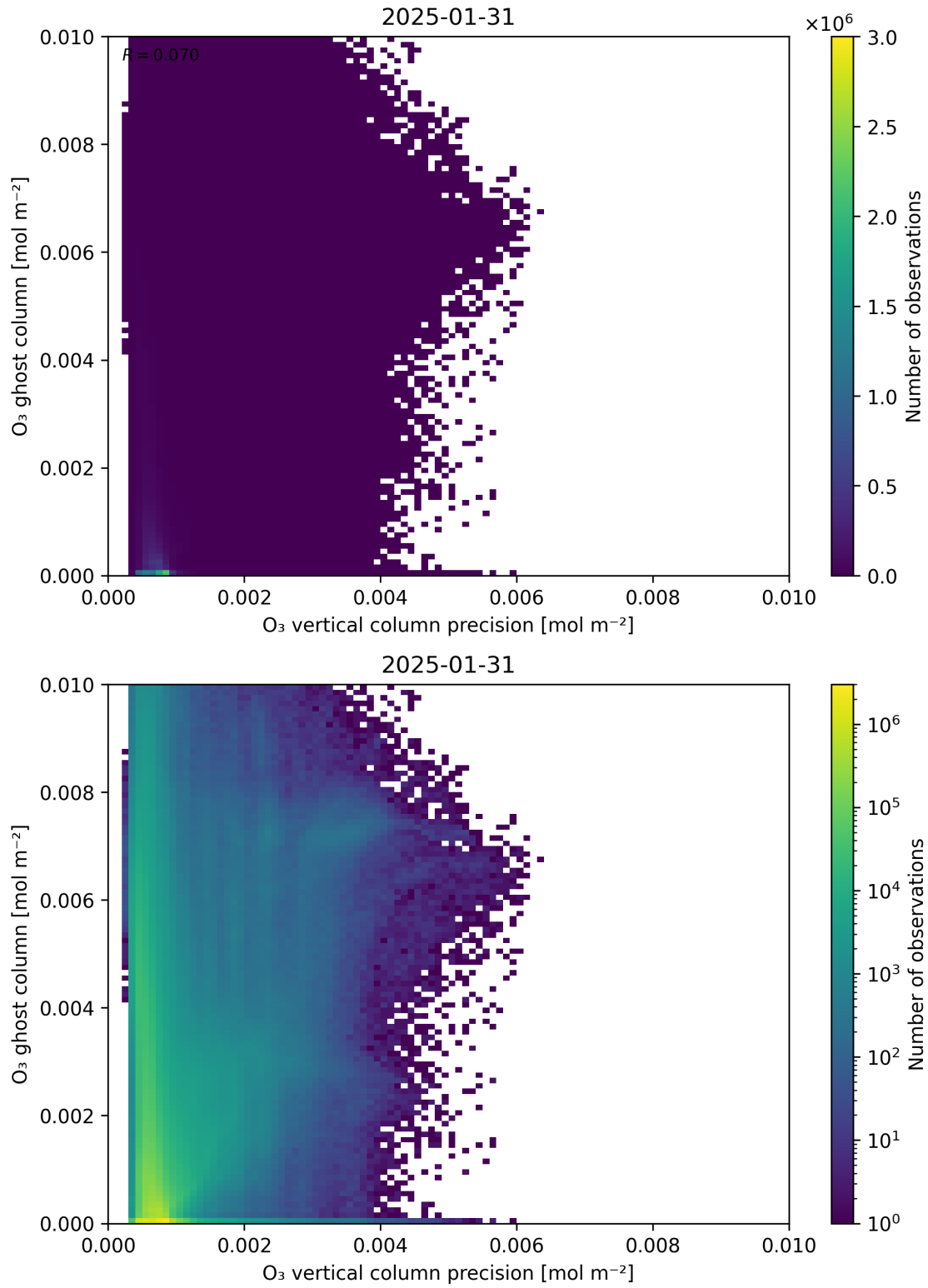
Figure 43: Scatter density plot of “O 3 vertical column precision” against “O 3 ghost column” for 2025-01-30 to 2025-02-01.
