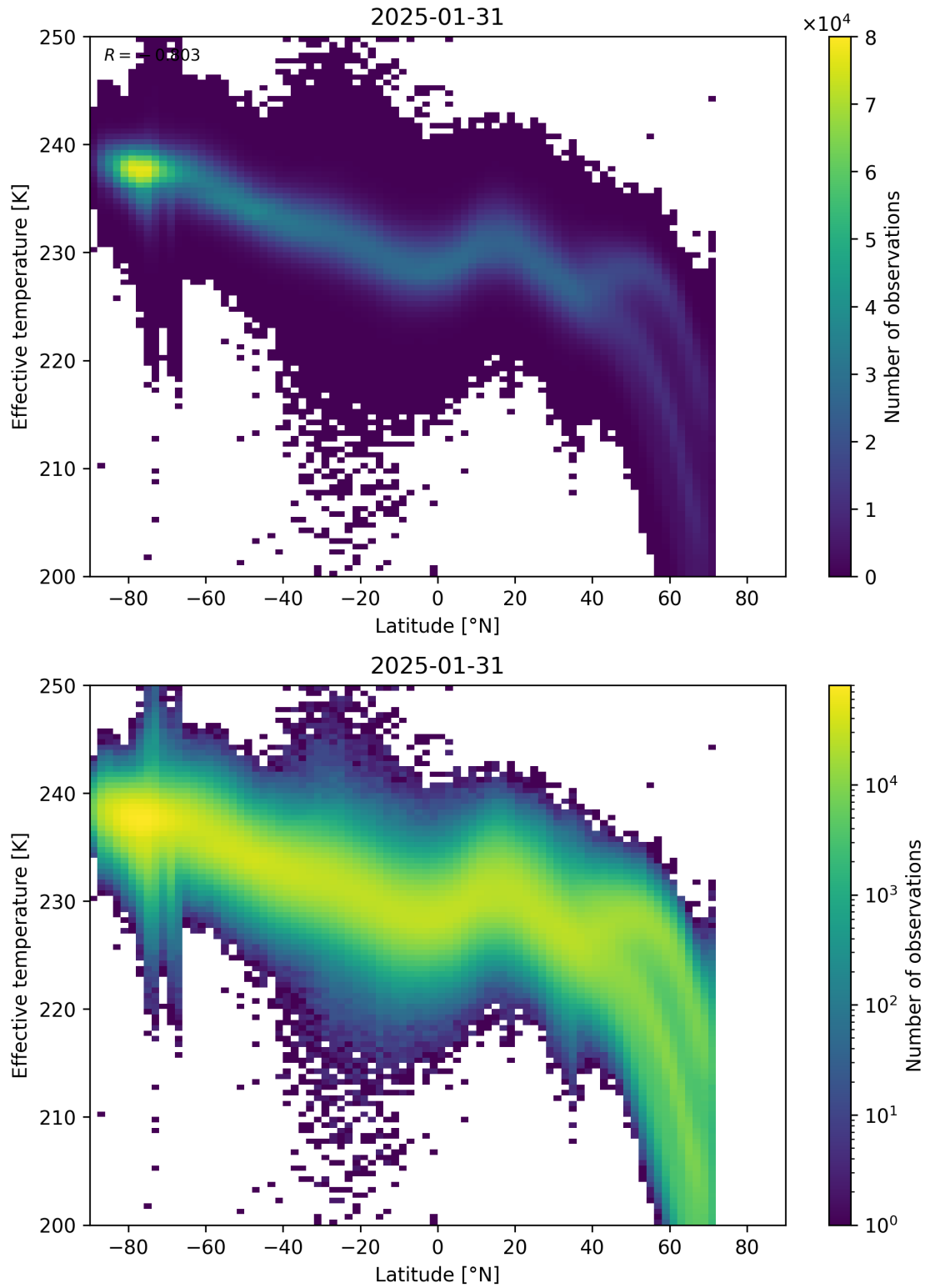
Figure 34: Scatter density plot of “Latitude” against “Effective temperature” for 2025-01-30 to 2025-02-01.
