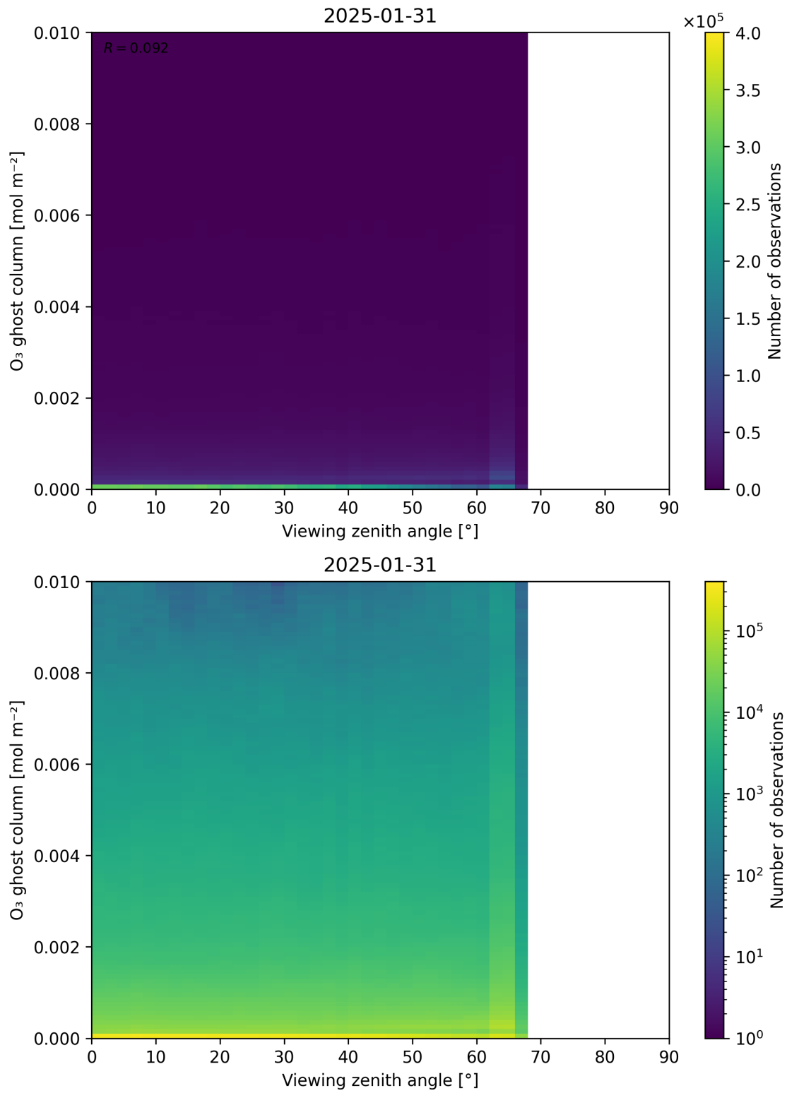
Figure 51: Scatter density plot of “Viewing zenith angle” against “O 3 ghost column” for 2025-01-30 to 2025-02-01.
