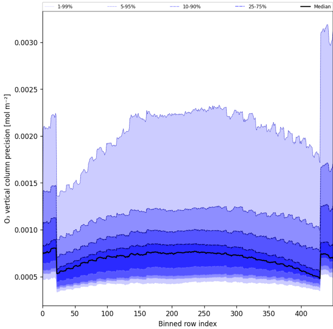
Figure 29: Along track statistics of “O 3 vertical column precision” for 2025-01-30 to 2025-02-01
