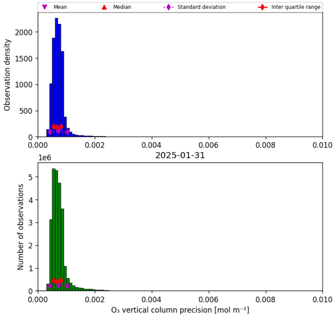
Figure 22: Histogram of “O 3 vertical column precision” for 2025-01-30 to 2025-02-01
