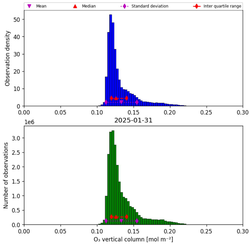
Figure 21: Histogram of “O 3 vertical column” for 2025-01-30 to 2025-02-01
