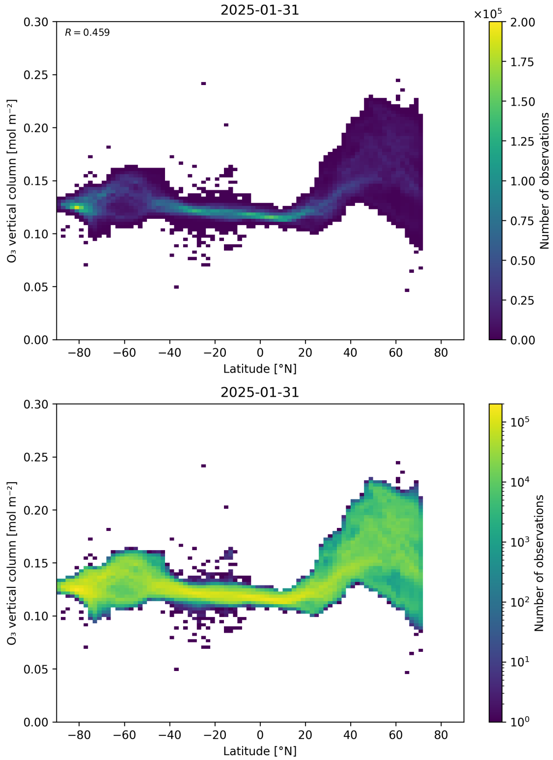
Figure 36: Scatter density plot of “Latitude” against “O 3 vertical column” for 2025-01-30 to 2025-02-01.
