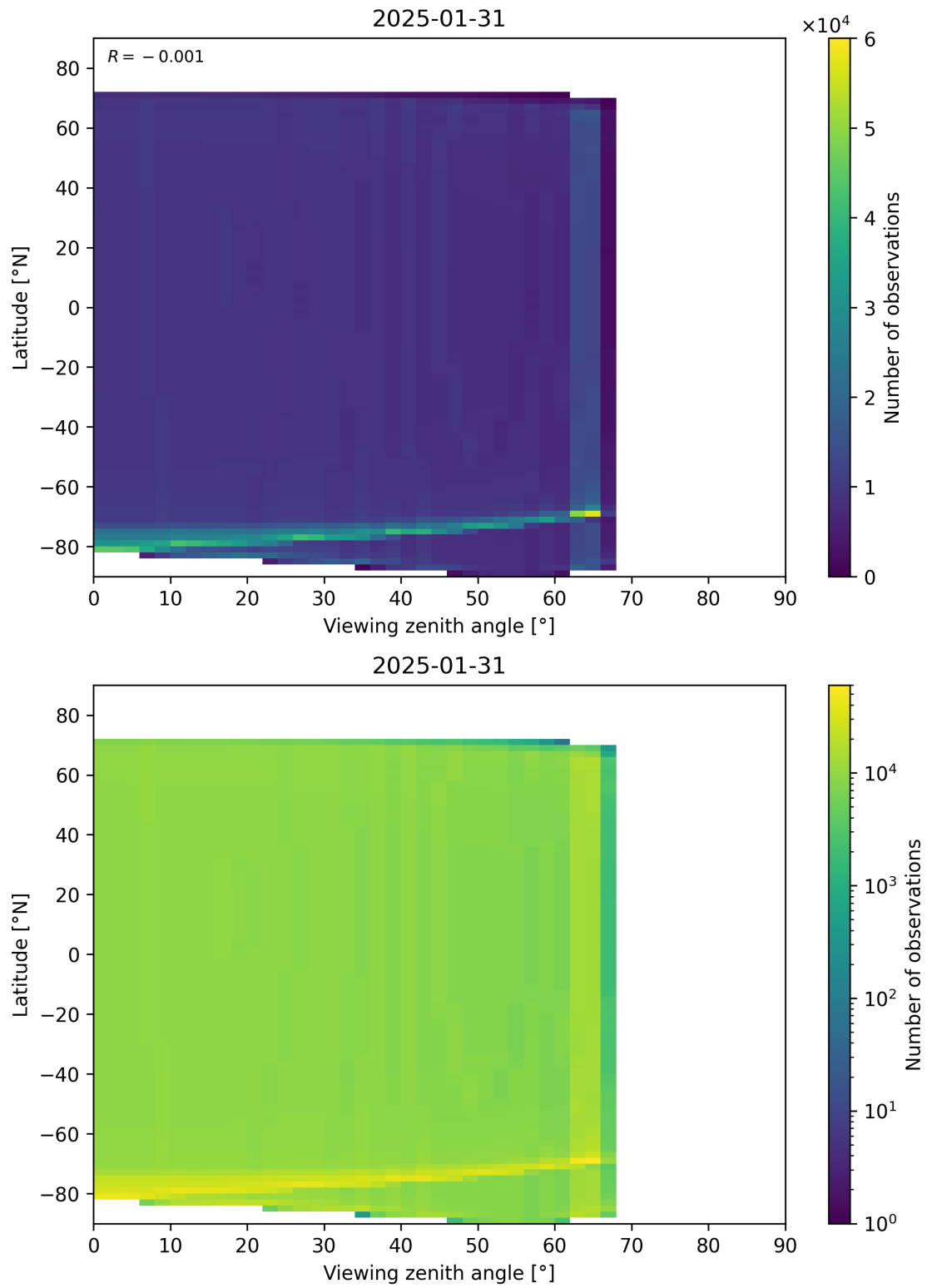
Figure 49: Scatter density plot of “Viewing zenith angle” against “Latitude” for 2025-01-30 to 2025-02-01.
