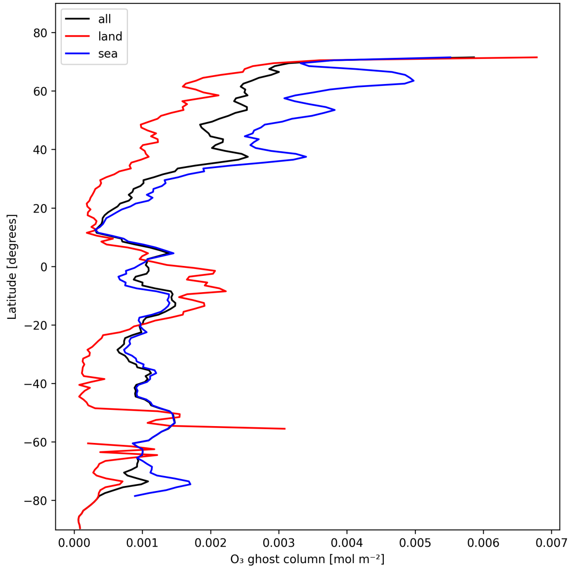
Figure 18: Zonal average of “O 3 ghost column” for 2025-01-30 to 2025-02-01.
