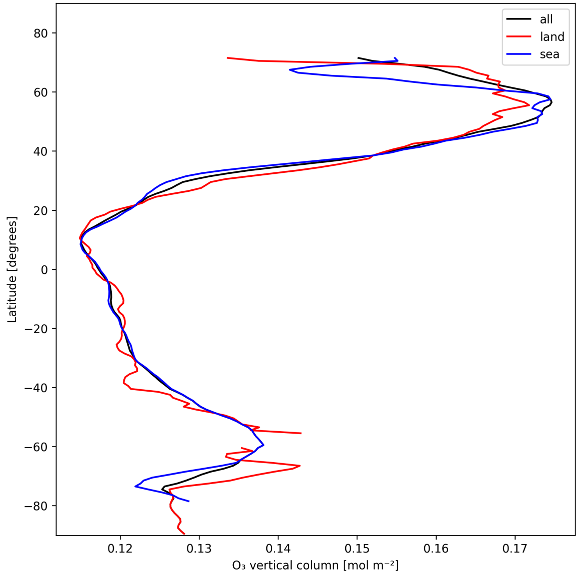
Figure 14: Zonal average of “O 3 vertical column” for 2025-01-30 to 2025-02-01.
