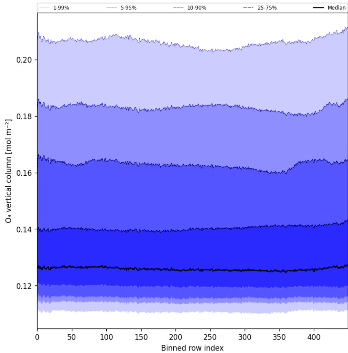
Figure 28: Along track statistics of “O 3 vertical column” for 2025-01-30 to 2025-02-01
