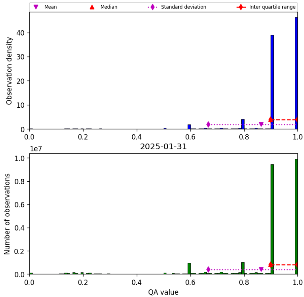
Figure 20: Histogram of “QA value” for 2025-01-30 to 2025-02-01
