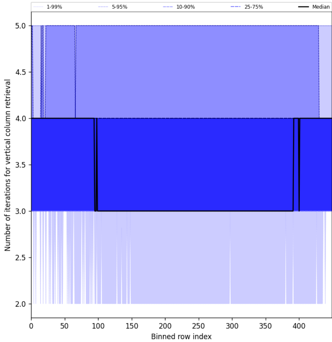
Figure 33: Along track statistics of “Number of iterations for vertical column retrieval” for 2025-01-30 to 2025-02-01
