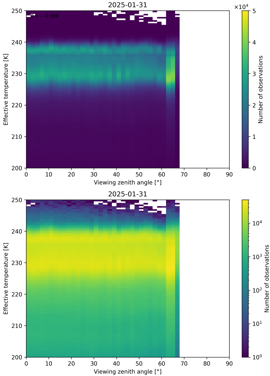
Figure 50: Scatter density plot of “Viewing zenith angle” against “Effective temperature” for 2025-01-30 to 2025-02-01.
