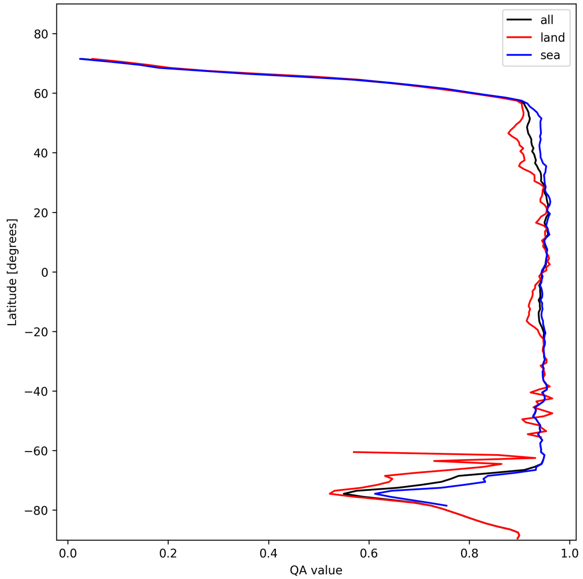
Figure 13: Zonal average of “QA value” for 2025-01-30 to 2025-02-01.
