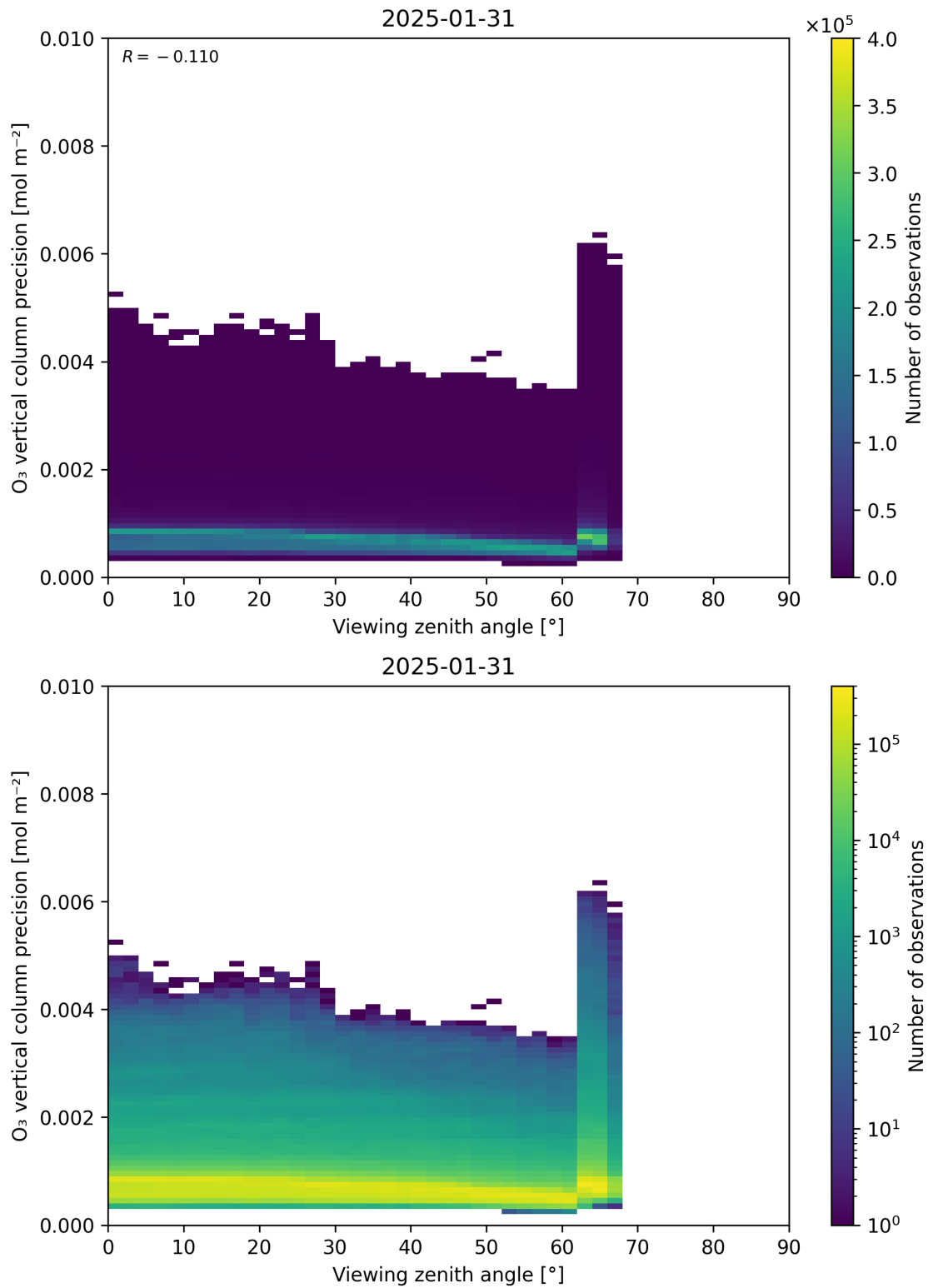
Figure 53: Scatter density plot of “Viewing zenith angle” against “O 3 vertical column precision” for 2025-01-30 to 2025-02-01.
