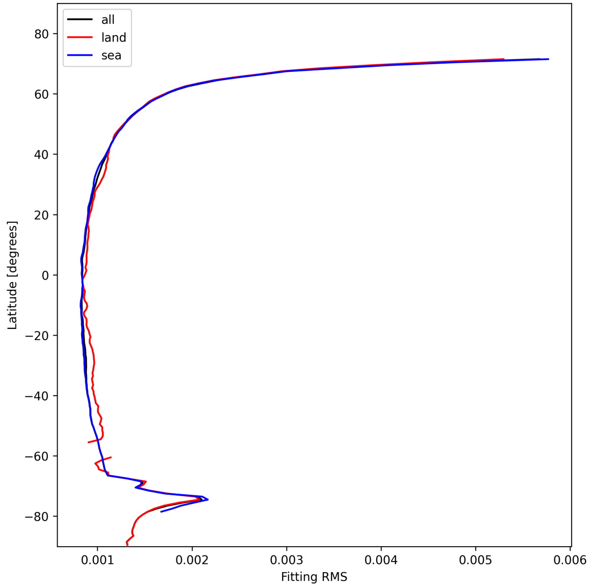
Figure 16: Zonal average of “Fitting RMS” for 2025-01-30 to 2025-02-01.
