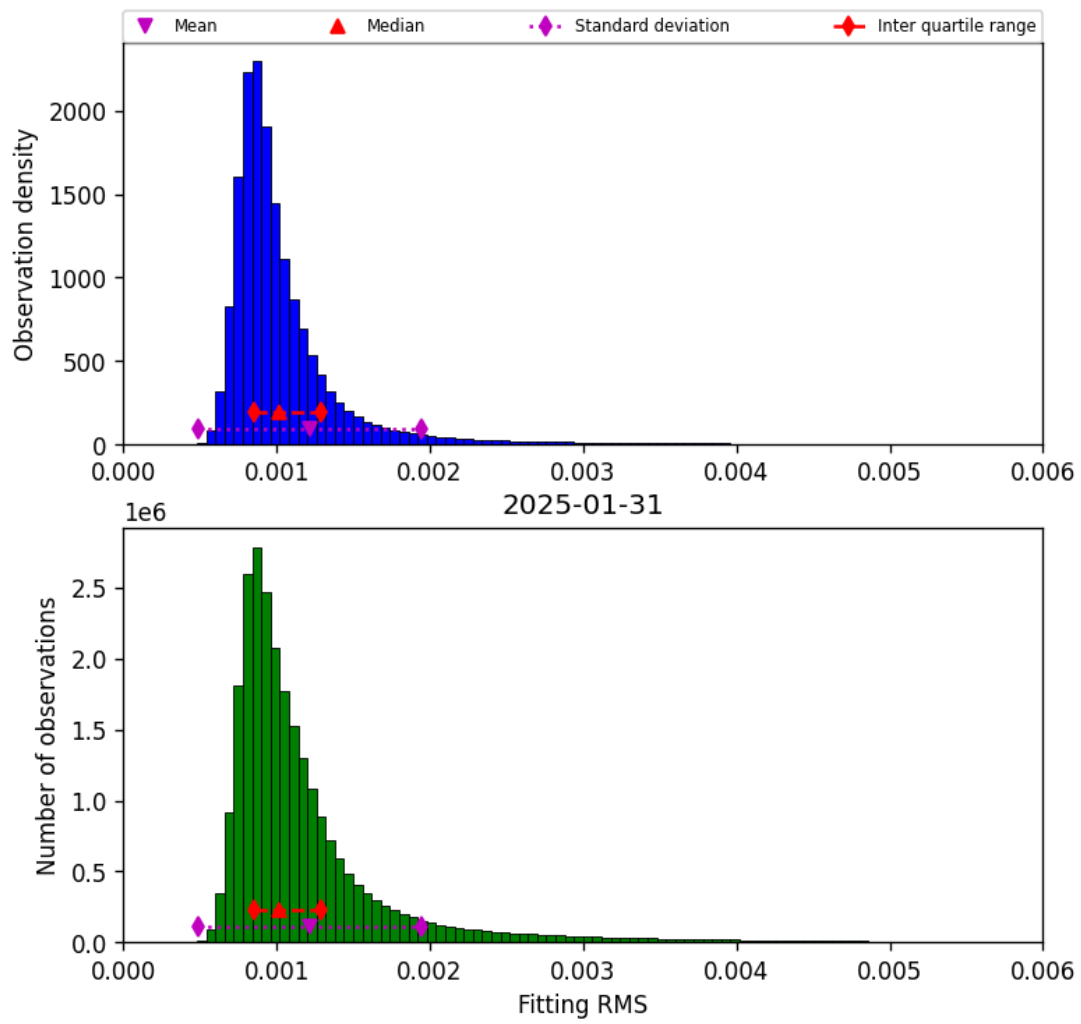
Figure 23: Histogram of “Fitting RMS” for 2025-01-30 to 2025-02-01
