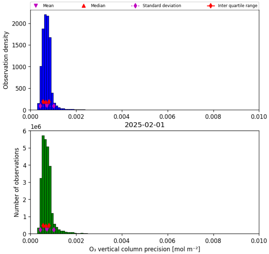
Figure 22: Histogram of “O 3 vertical column precision” for 2025-01-31 to 2025-02-02
