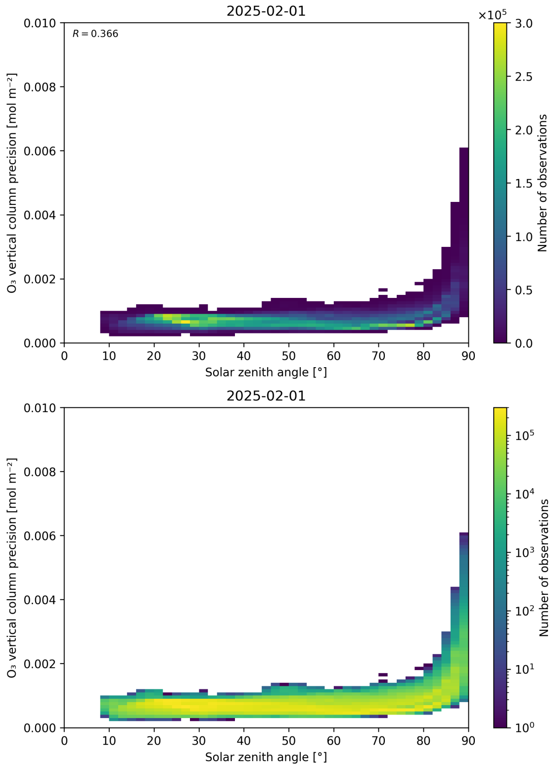
Figure 48: Scatter density plot of “Solar zenith angle” against “O 3 vertical column precision” for 2025-01-31 to 2025-02-02.
