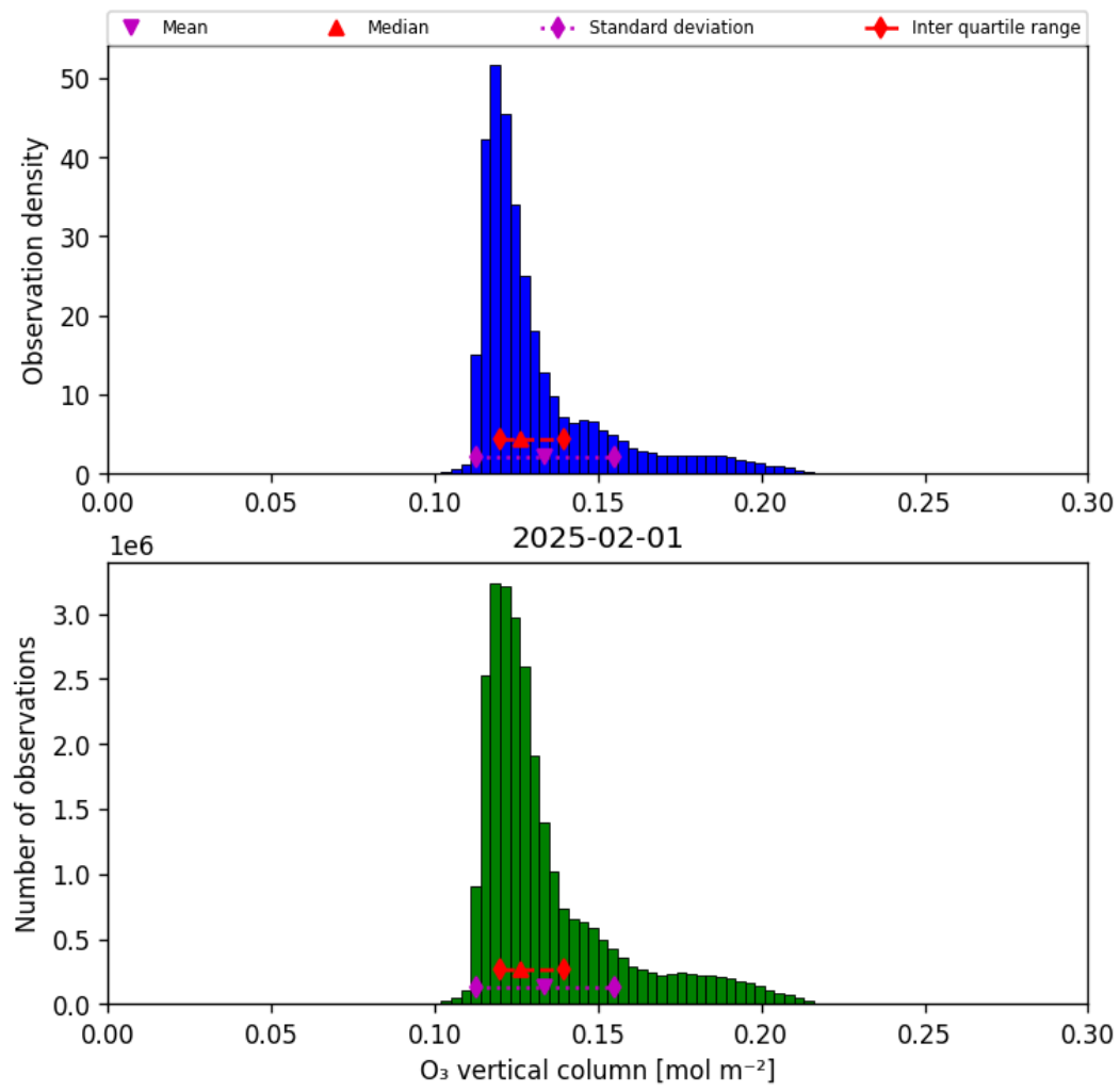
Figure 21: Histogram of “O 3 vertical column” for 2025-01-31 to 2025-02-02
