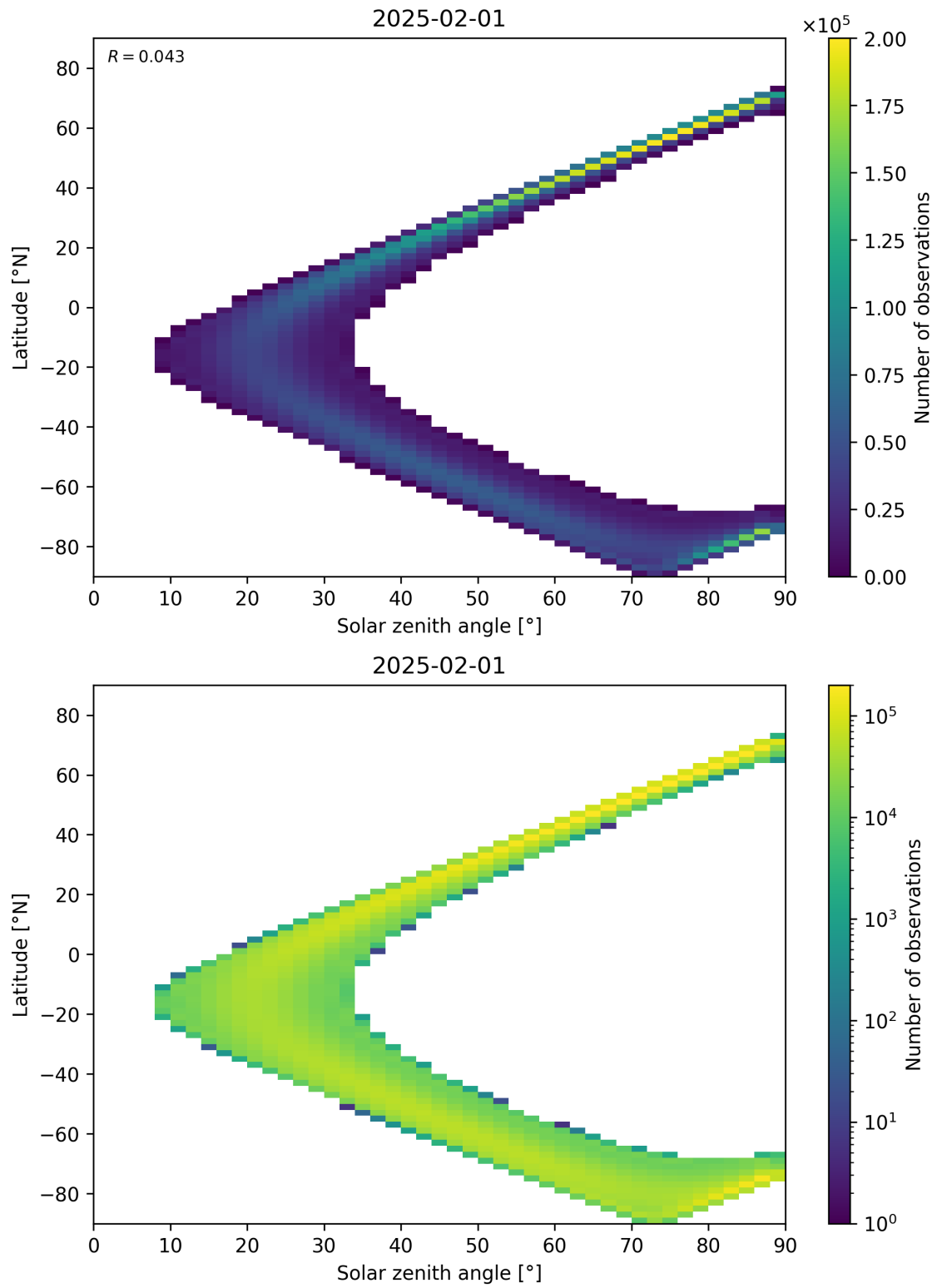
Figure 44: Scatter density plot of “Solar zenith angle” against “Latitude” for 2025-01-31 to 2025-02-02.
