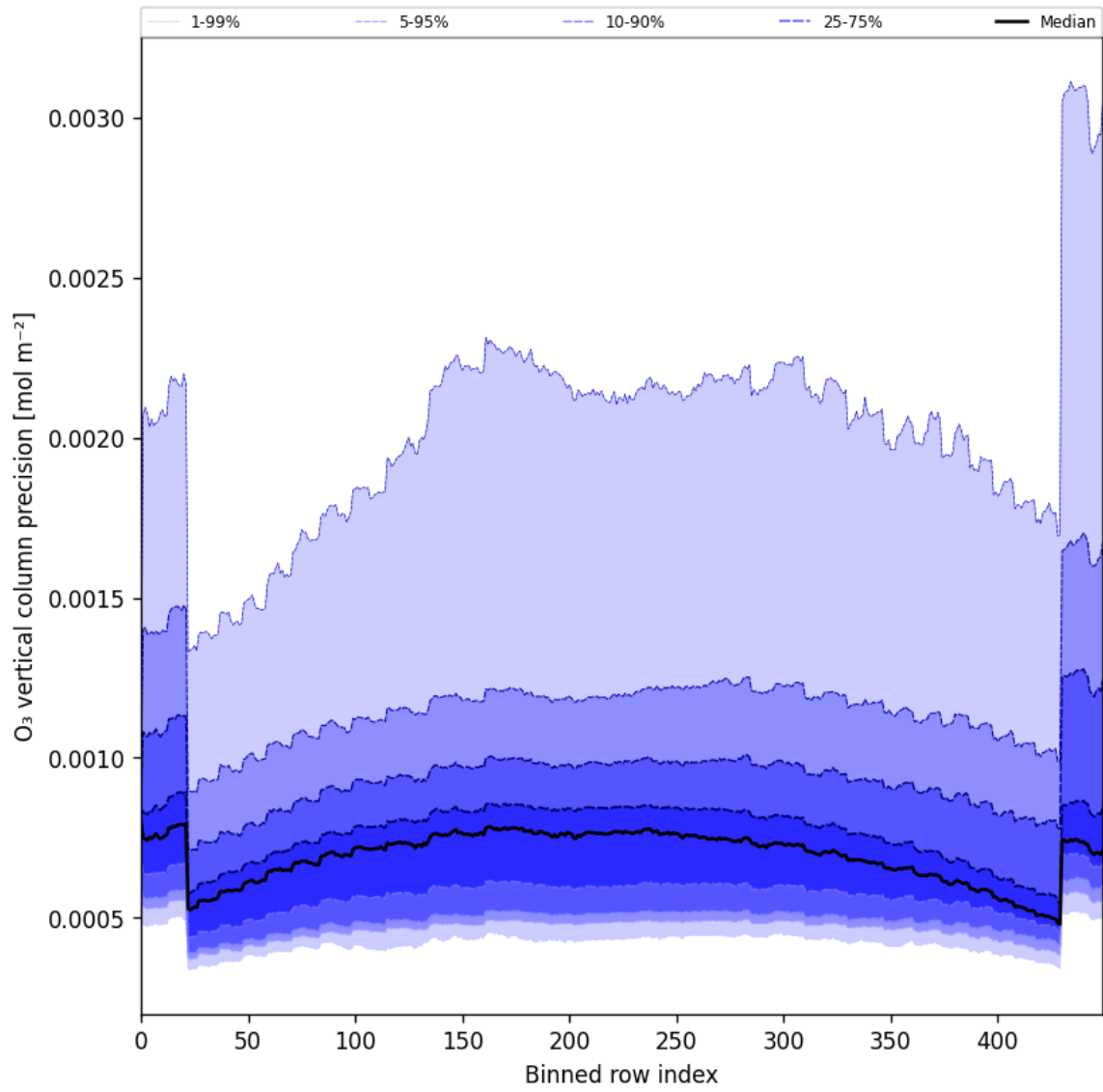
Figure 29: Along track statistics of “O 3 vertical column precision” for 2025-01-31 to 2025-02-02
