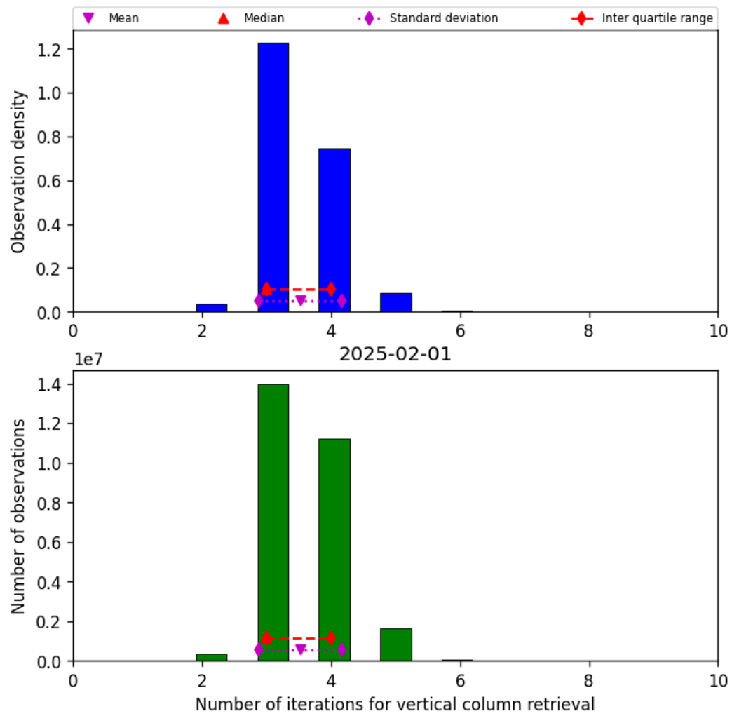
Figure 26: Histogram of “Number of iterations for vertical column retrieval” for 2025-01-31 to 2025-02-02
