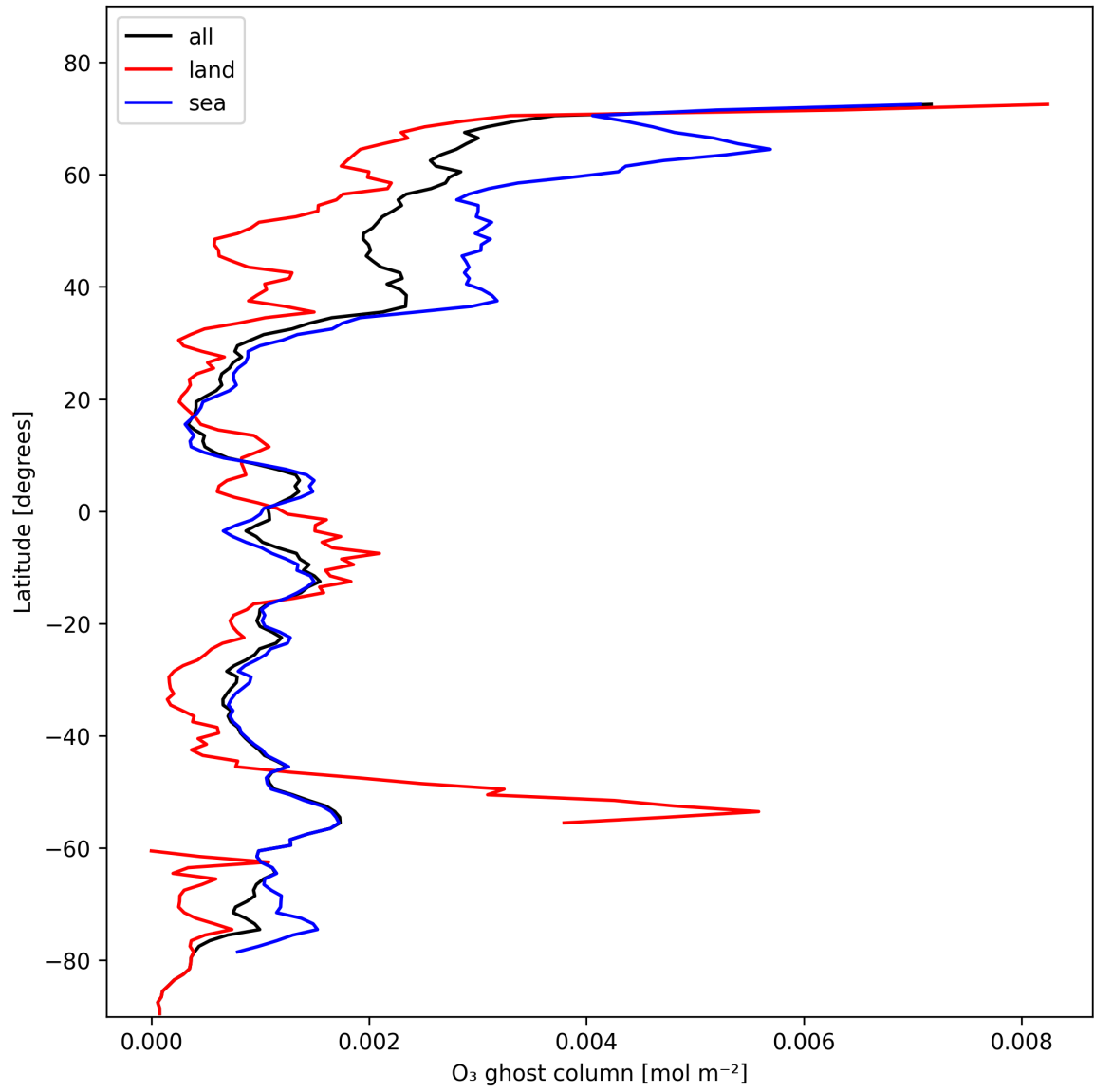
Figure 18: Zonal average of “O 3 ghost column” for 2025-01-31 to 2025-02-02.
