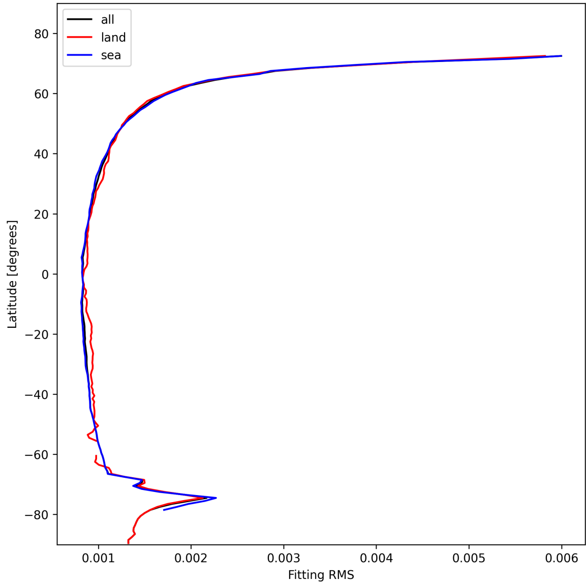
Figure 16: Zonal average of “Fitting RMS” for 2025-01-31 to 2025-02-02.
