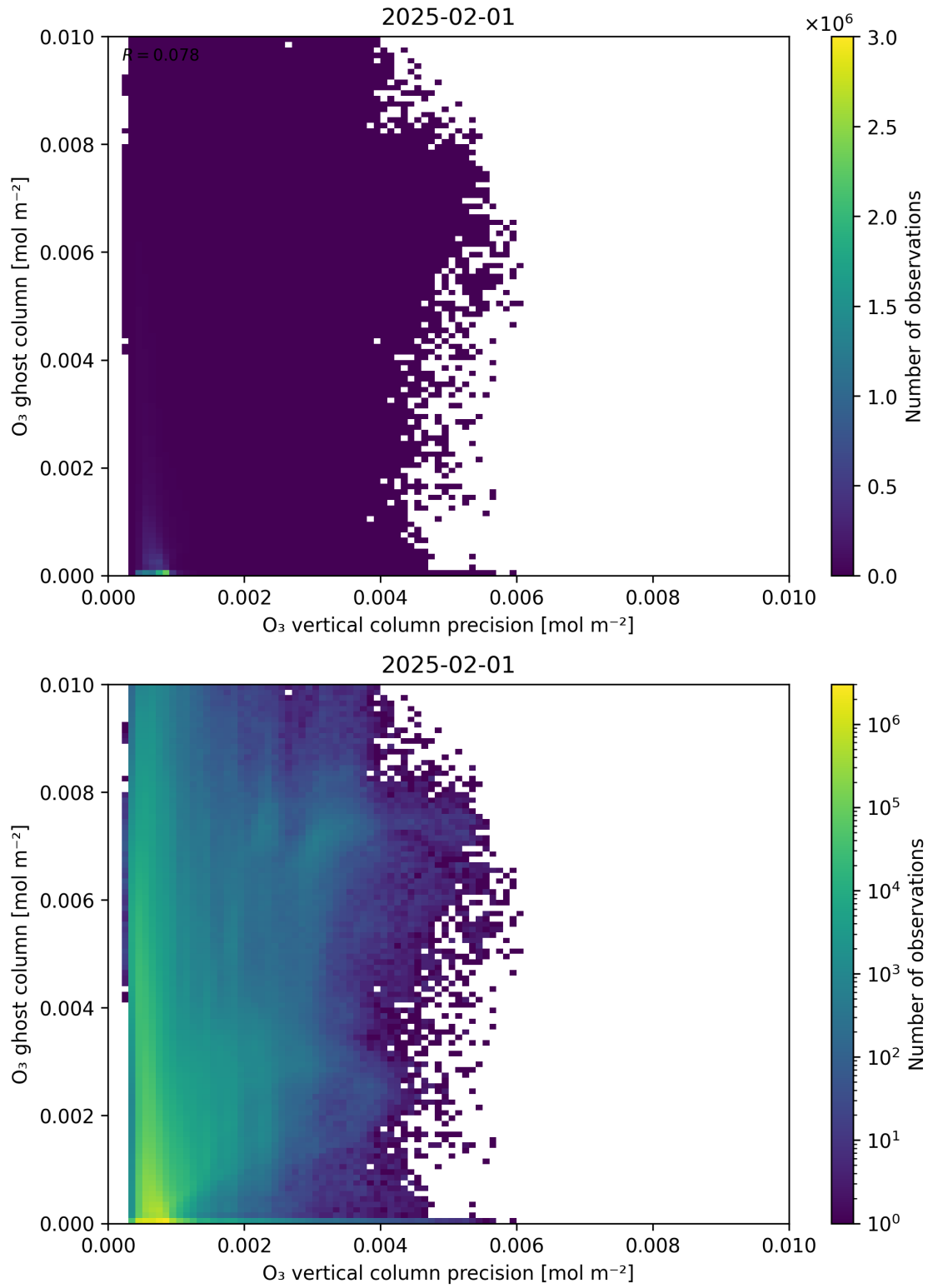
Figure 43: Scatter density plot of “O 3 vertical column precision” against “O 3 ghost column” for 2025-01-31 to 2025-02-02.
