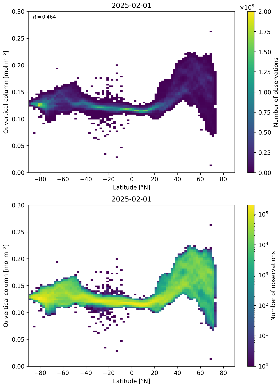
Figure 36: Scatter density plot of “Latitude” against “O 3 vertical column” for 2025-01-31 to 2025-02-02.
