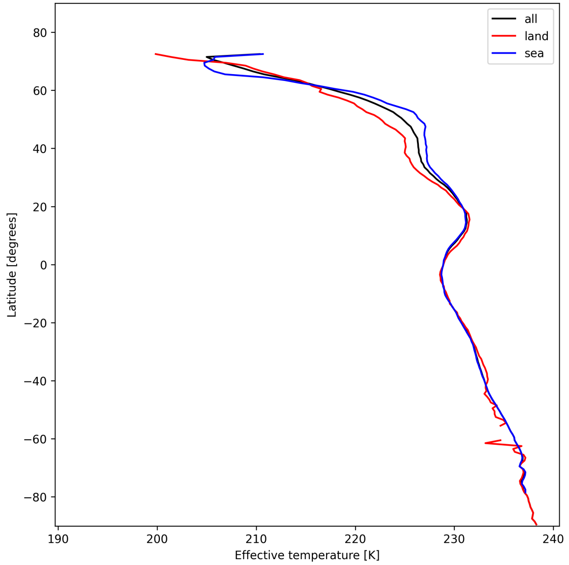
Figure 17: Zonal average of "Effective temperature" for 2025-01-31 to 2025-02-02.
