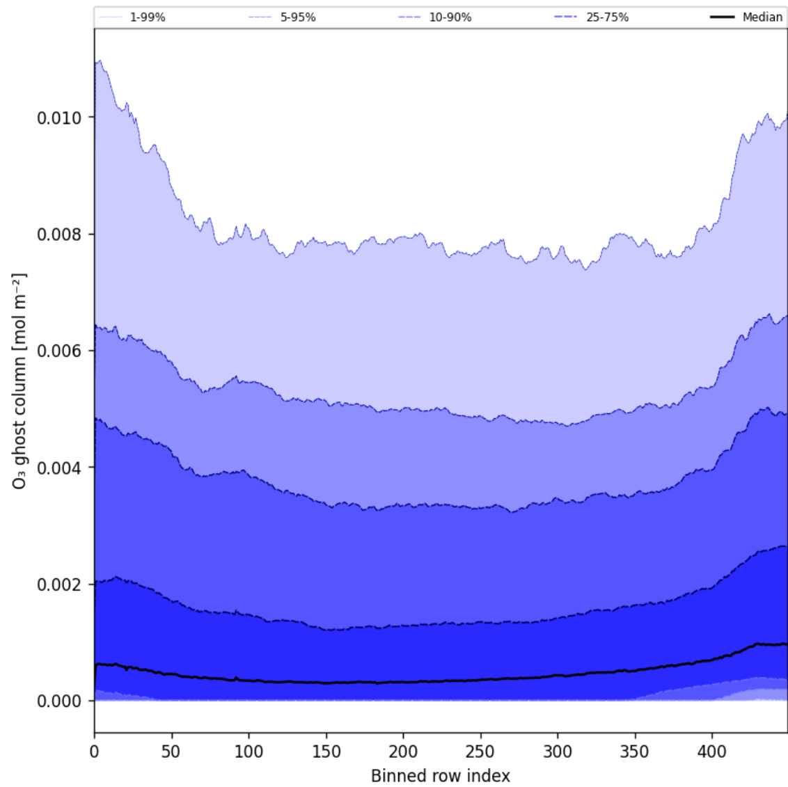
Figure 32: Along track statistics of “O 3 ghost column” for 2025-01-31 to 2025-02-02
