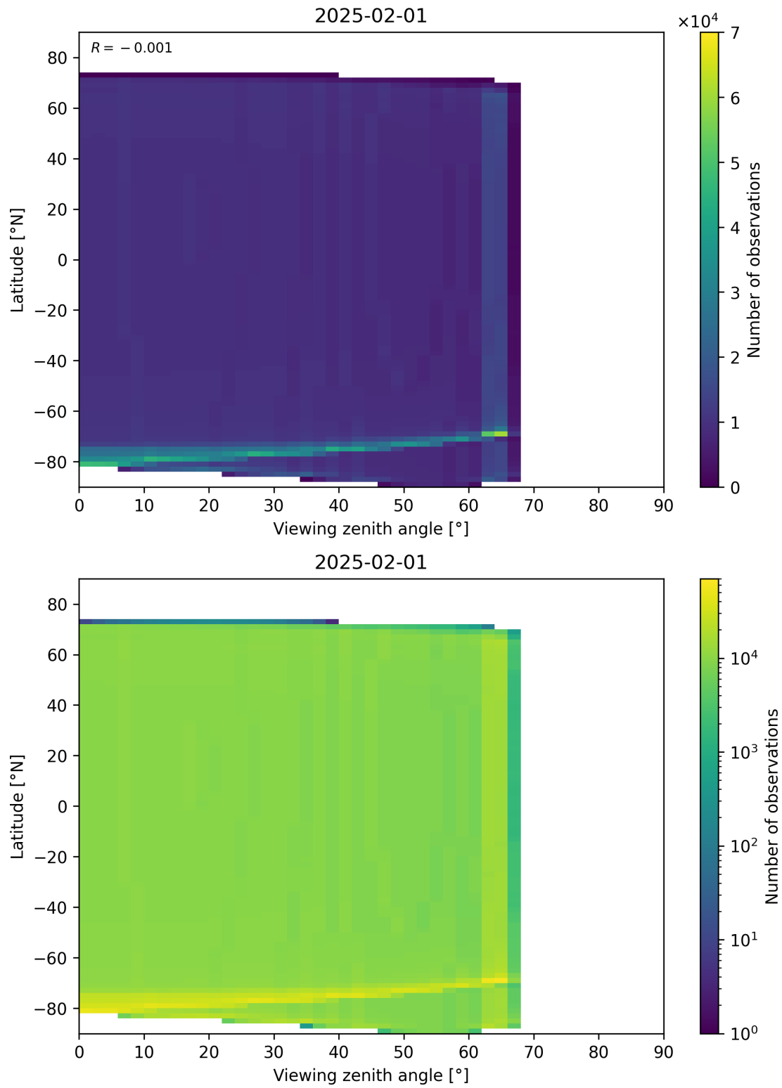
Figure 49: Scatter density plot of “Viewing zenith angle” against “Latitude” for 2025-01-31 to 2025-02-02.
