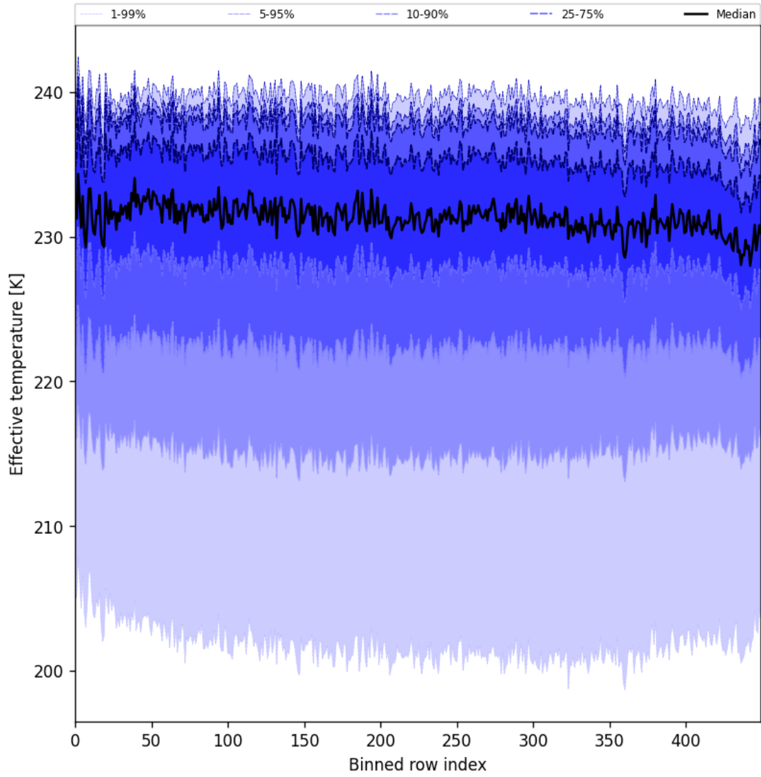
Figure 31: Along track statistics of “Effective temperature” for 2025-01-31 to 2025-02-02
