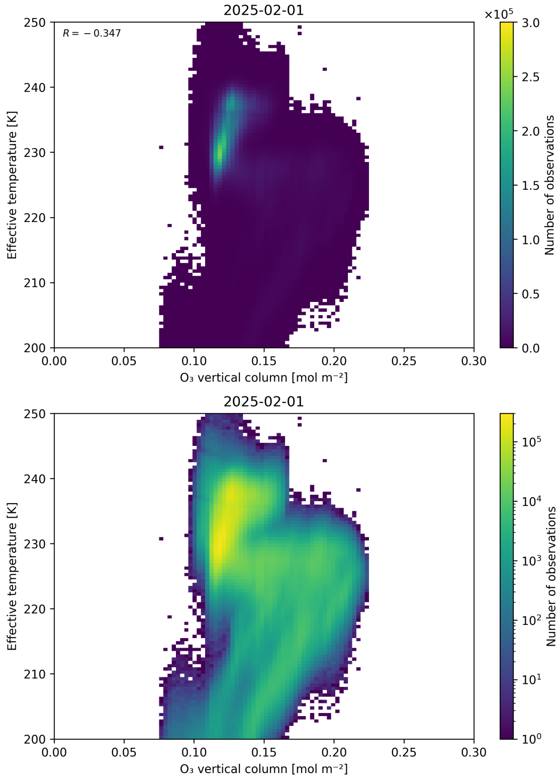
Figure 39: Scatter density plot of “O 3 vertical column” against “Effective temperature” for 2025-01-31 to 2025-02-02.
