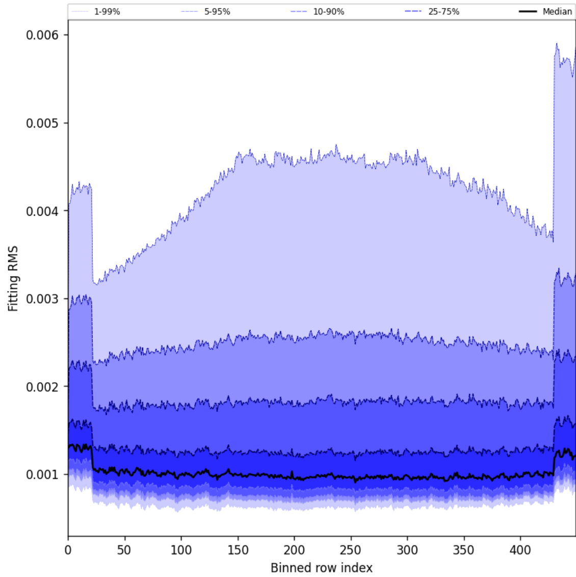
Figure 30: Along track statistics of “Fitting RMS” for 2025-01-31 to 2025-02-02
