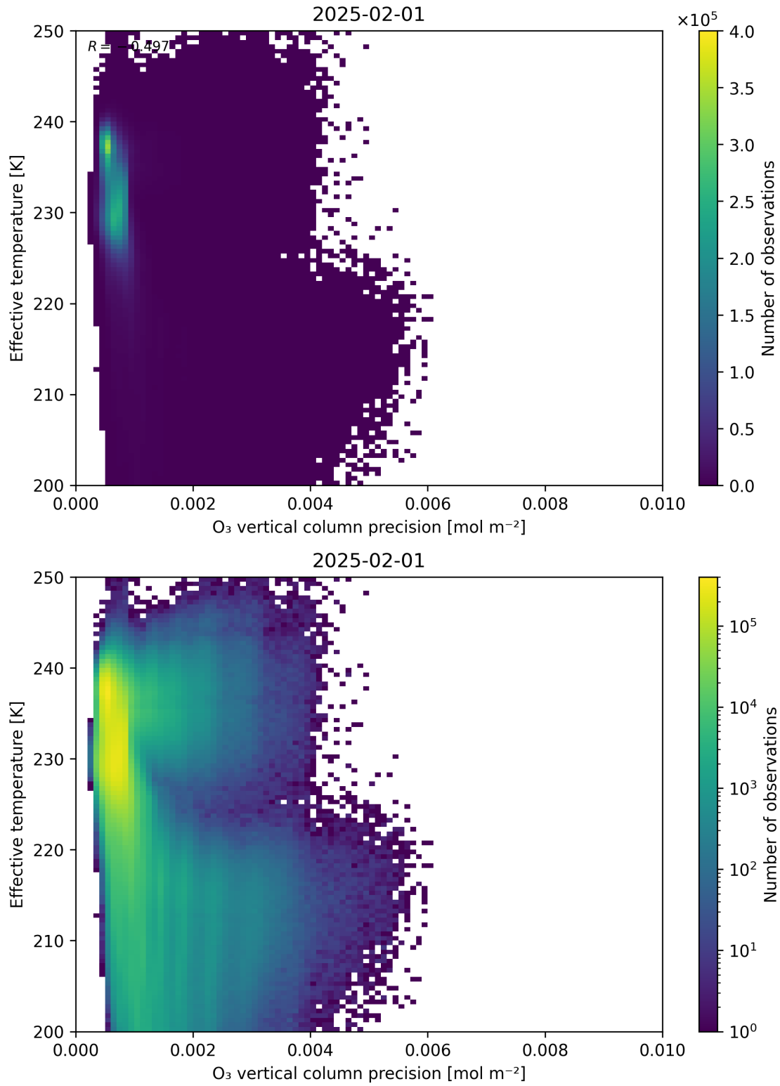
Figure 42: Scatter density plot of “O 3 vertical column precision” against “Effective temperature” for 2025-01-31 to 2025-02-02.
