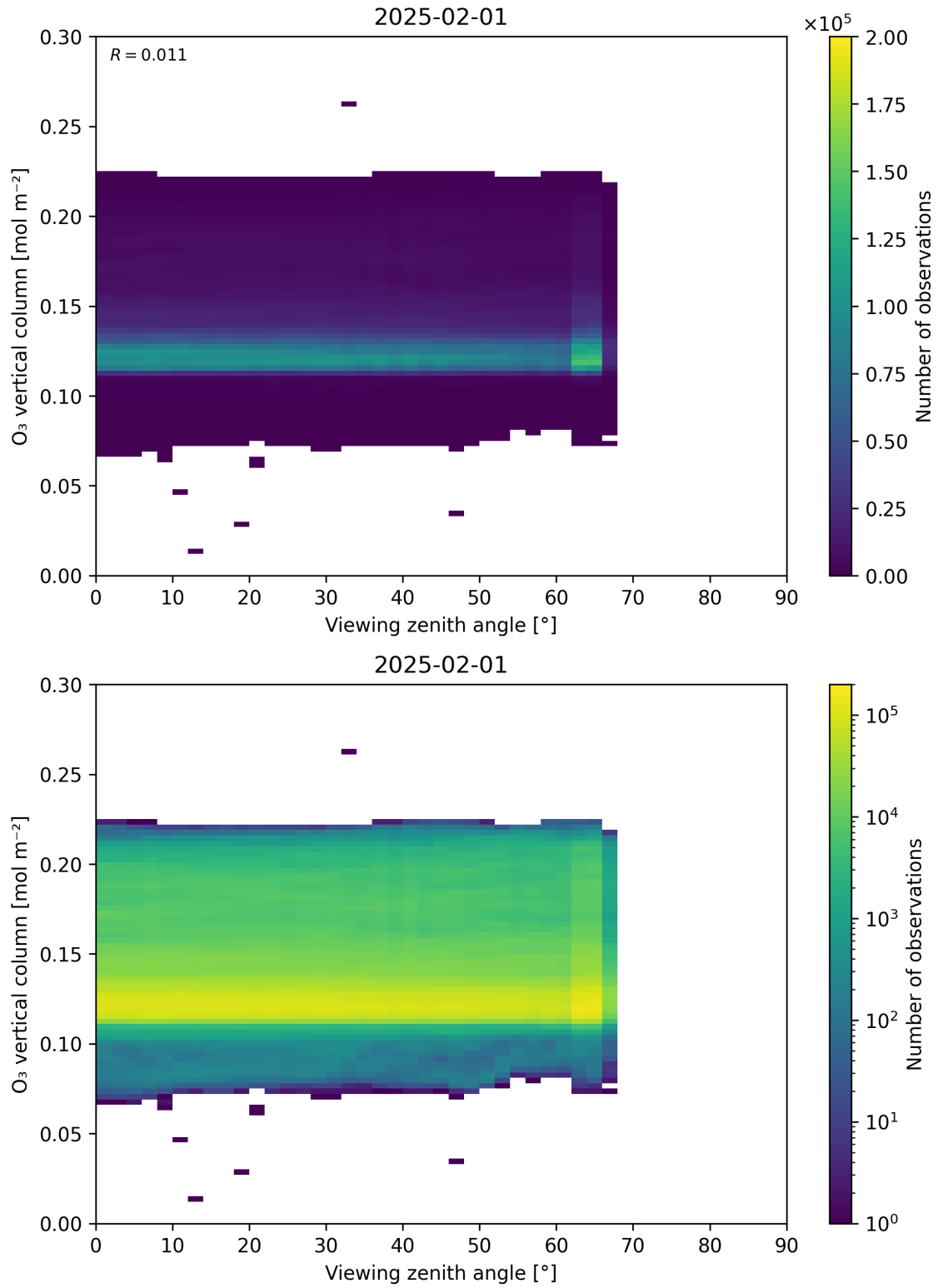
Figure 52: Scatter density plot of “Viewing zenith angle” against “O 3 vertical column” for 2025-01-31 to 2025-02-02.
