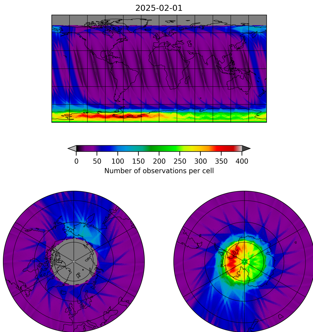
Figure 12: Map of the number of observations for 2025-01-31 to 2025-02-02
