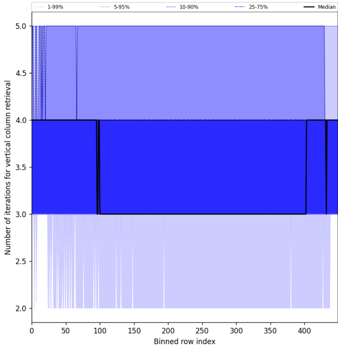
Figure 33: Along track statistics of “Number of iterations for vertical column retrieval” for 2025-01-31 to 2025-02-02
