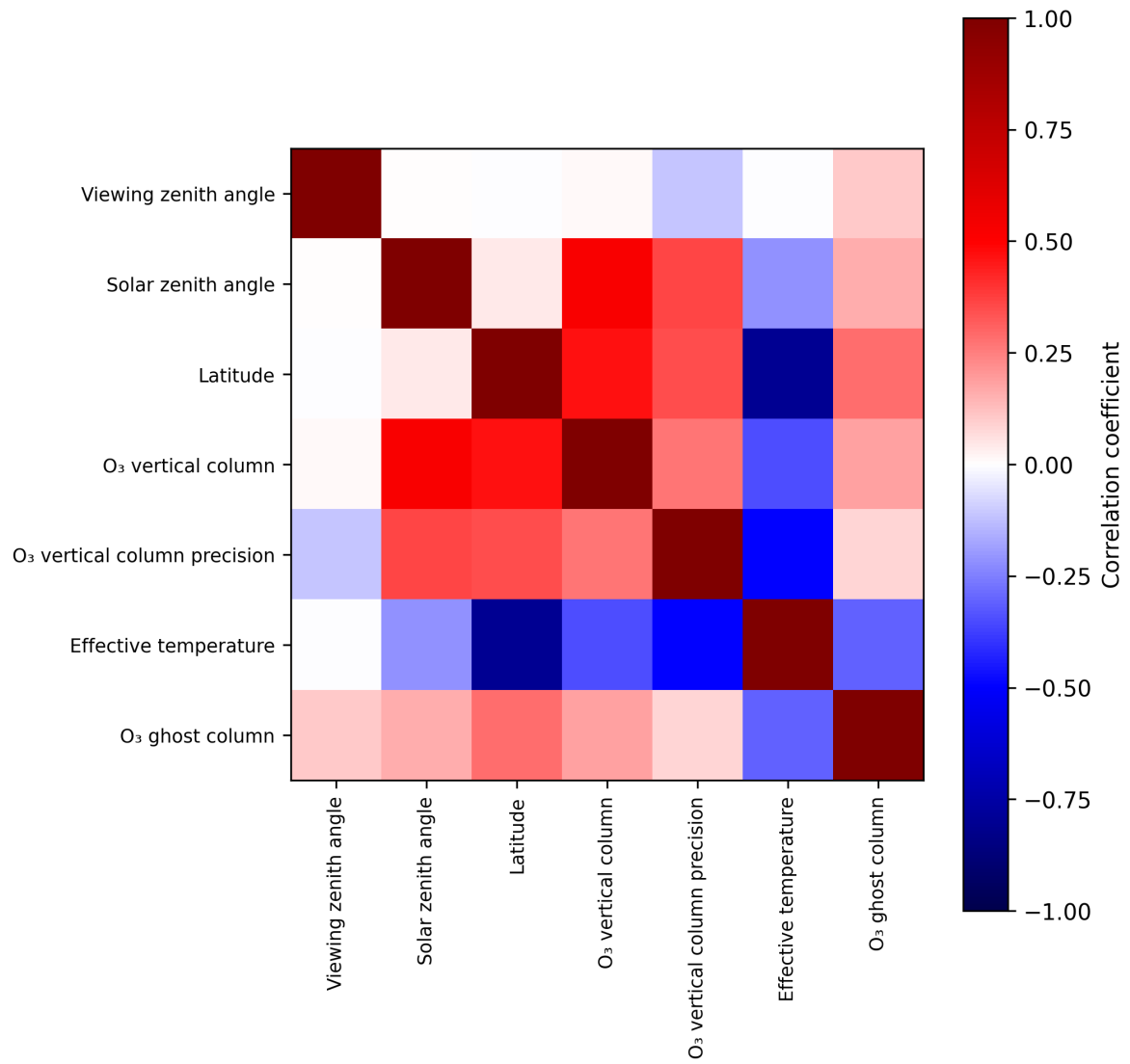
Figure 2: Map of correlation matrix for 2025-01-31 to 2025-02-02.
