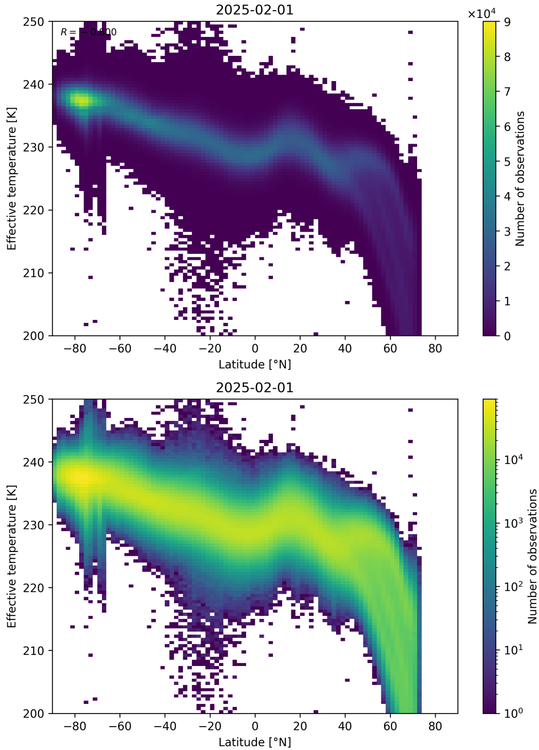
Figure 34: Scatter density plot of “Latitude” against “Effective temperature” for 2025-01-31 to 2025-02-02.
