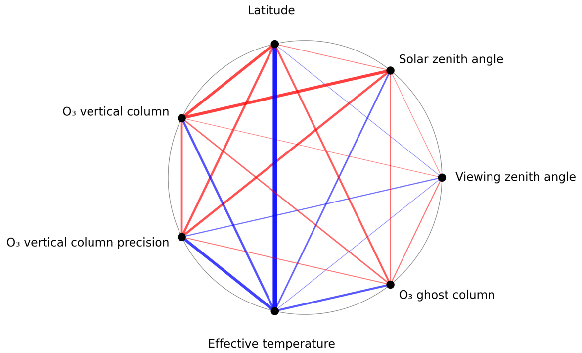
Figure 1: Map of correlation graph for 2025-01-31 to 2025-02-02.
