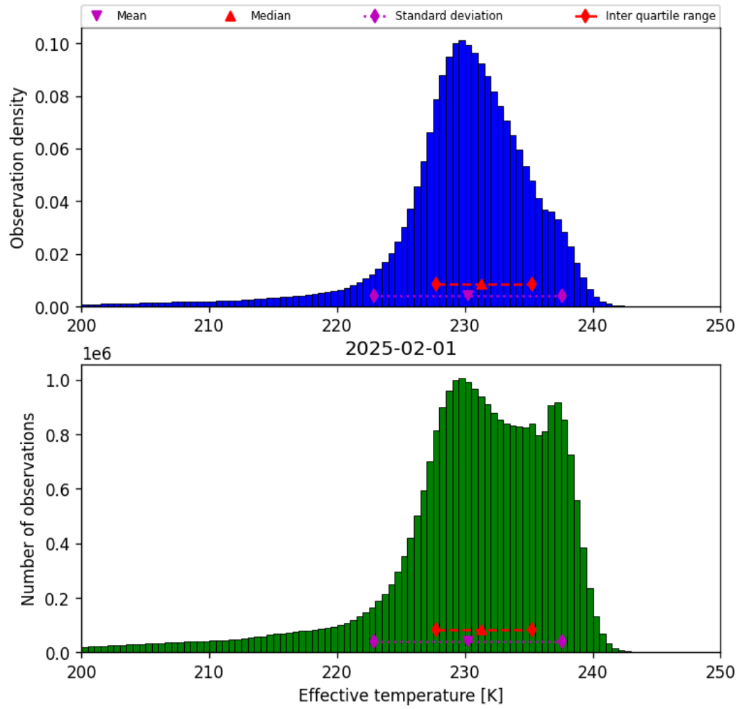
Figure 24: Histogram of “Effective temperature” for 2025-01-31 to 2025-02-02
