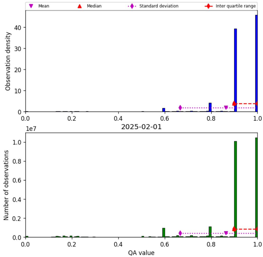
Figure 20: Histogram of “QA value” for 2025-01-31 to 2025-02-02
