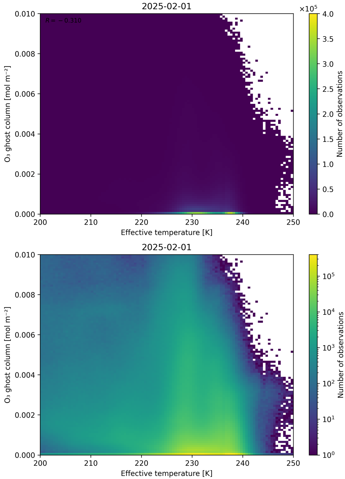
Figure 38: Scatter density plot of “Effective temperature” against “O 3 ghost column” for 2025-01-31 to 2025-02-02.
