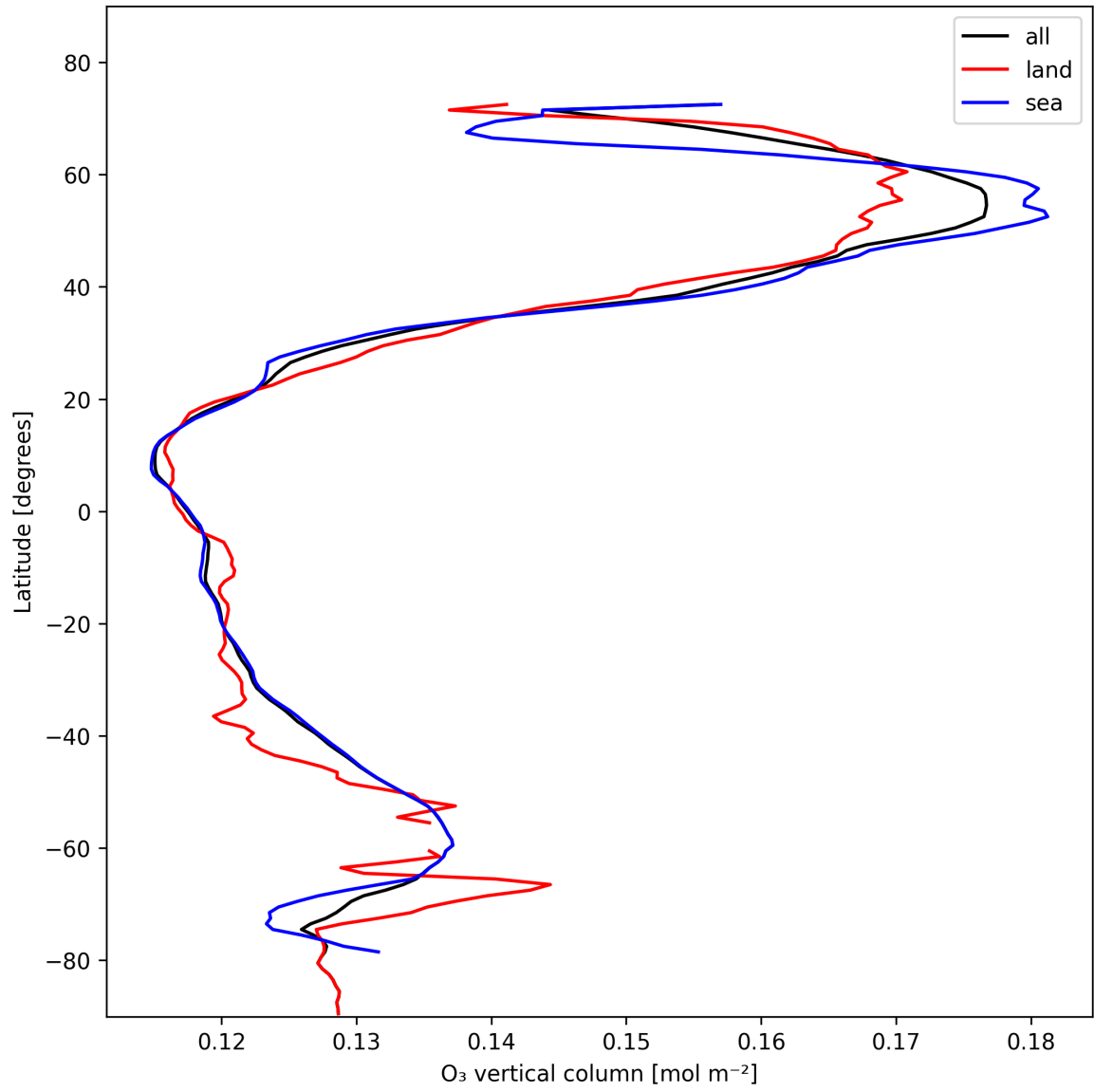
Figure 14: Zonal average of “O 3 vertical column” for 2025-01-31 to 2025-02-02.
