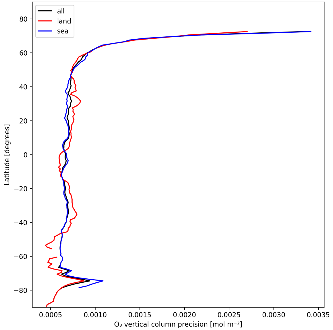
Figure 15: Zonal average of “O 3 vertical column precision” for 2025-01-31 to 2025-02-02.
