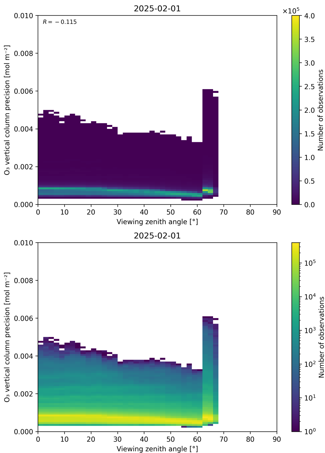
Figure 53: Scatter density plot of “Viewing zenith angle” against “O 3 vertical column precision” for 2025-01-31 to 2025-02-02.
