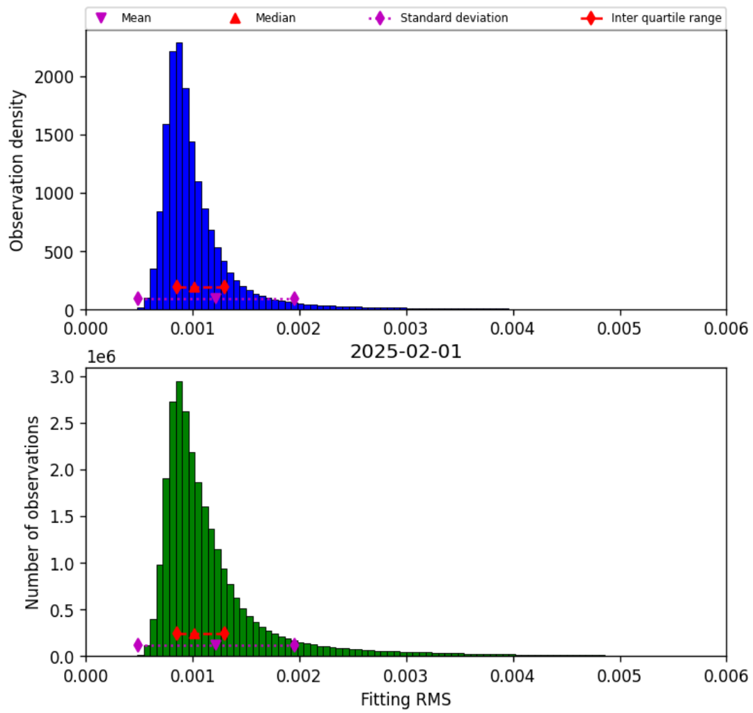
Figure 23: Histogram of “Fitting RMS” for 2025-01-31 to 2025-02-02
