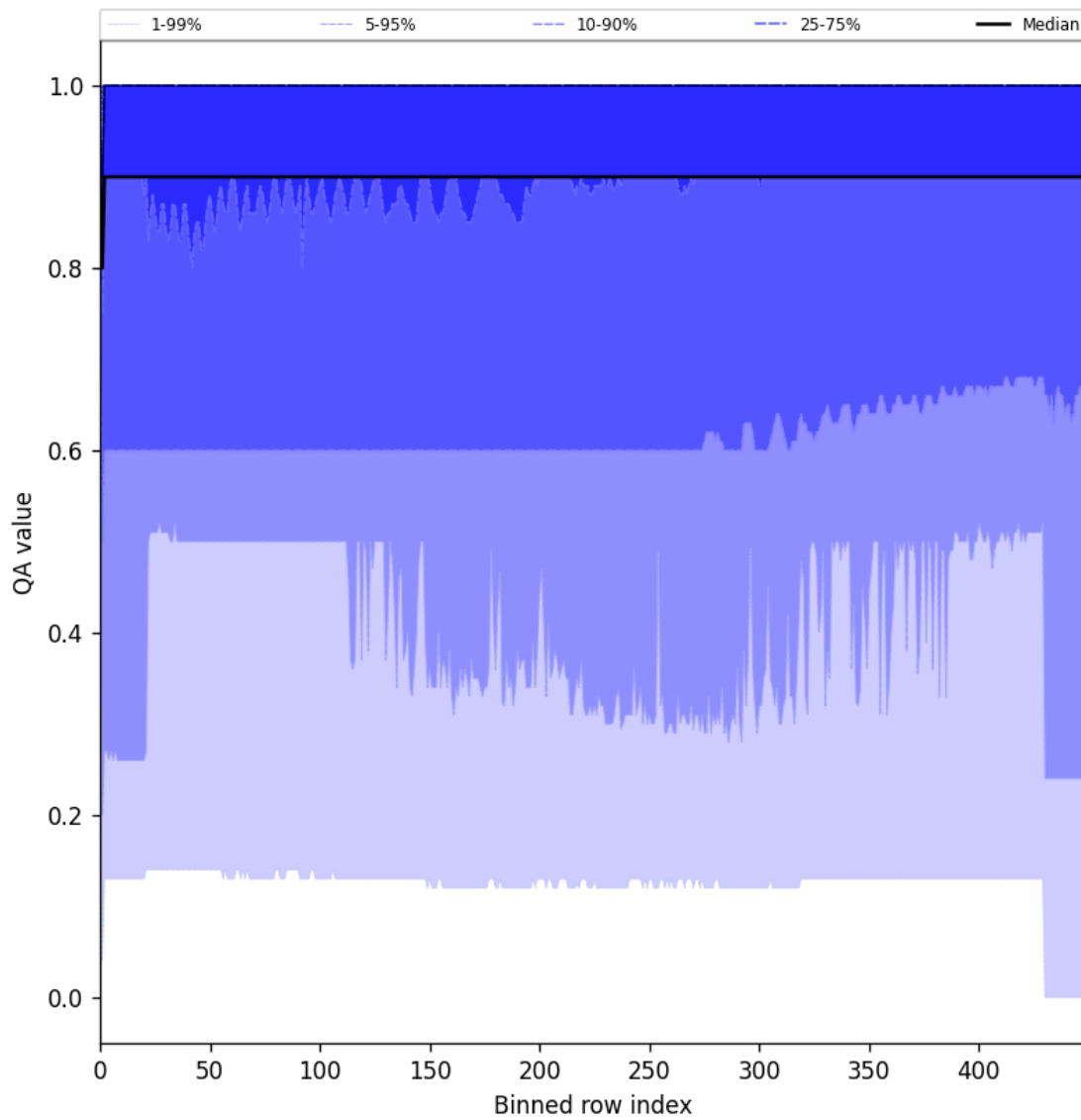
Figure 27: Along track statistics of “QA value” for 2025-01-31 to 2025-02-02
