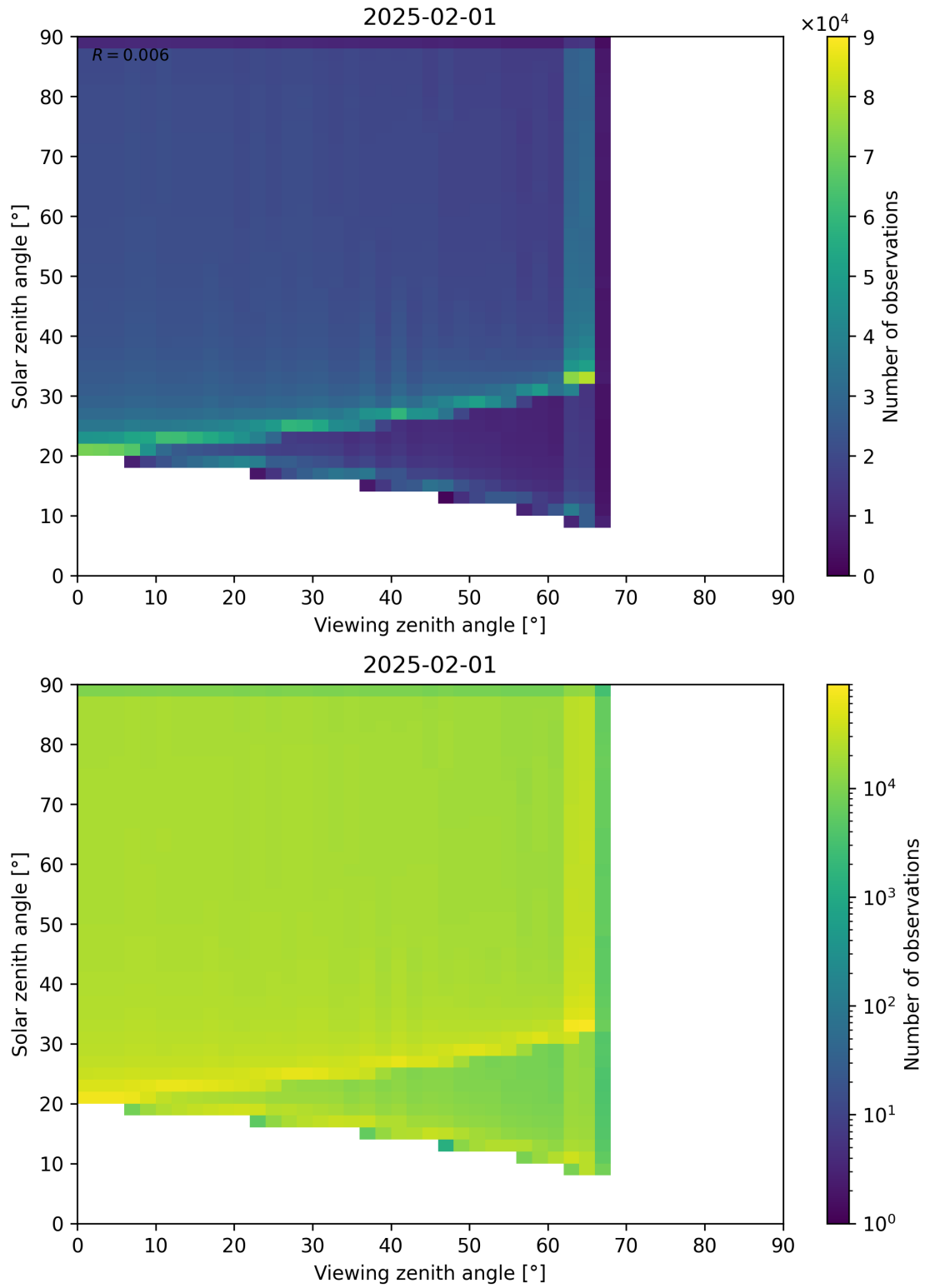
Figure 54: Scatter density plot of “Viewing zenith angle” against “Solar zenith angle” for 2025-01-31 to 2025-02-02.
