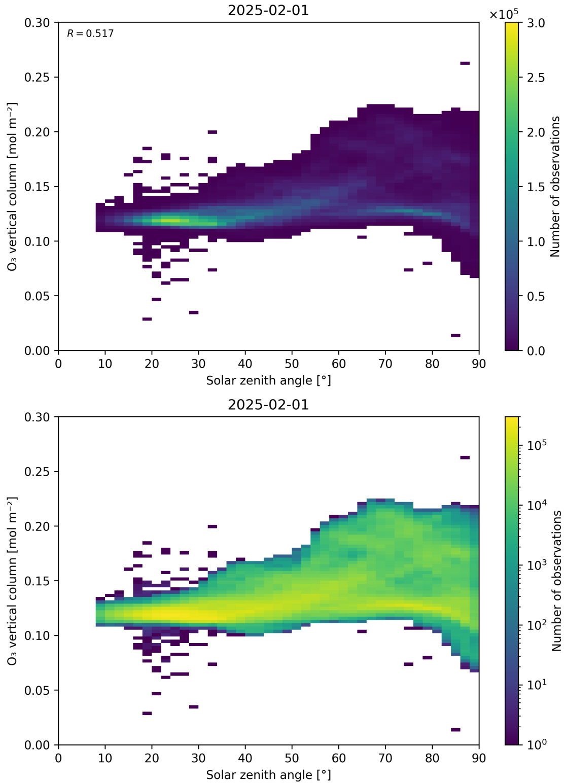
Figure 47: Scatter density plot of “Solar zenith angle” against “O 3 vertical column” for 2025-01-31 to 2025-02-02.
