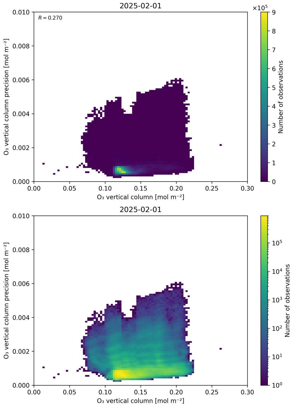
Figure 41: Scatter density plot of “O 3 vertical column” against “O 3 vertical column precision” for 2025-01-31 to 2025-02-02.
