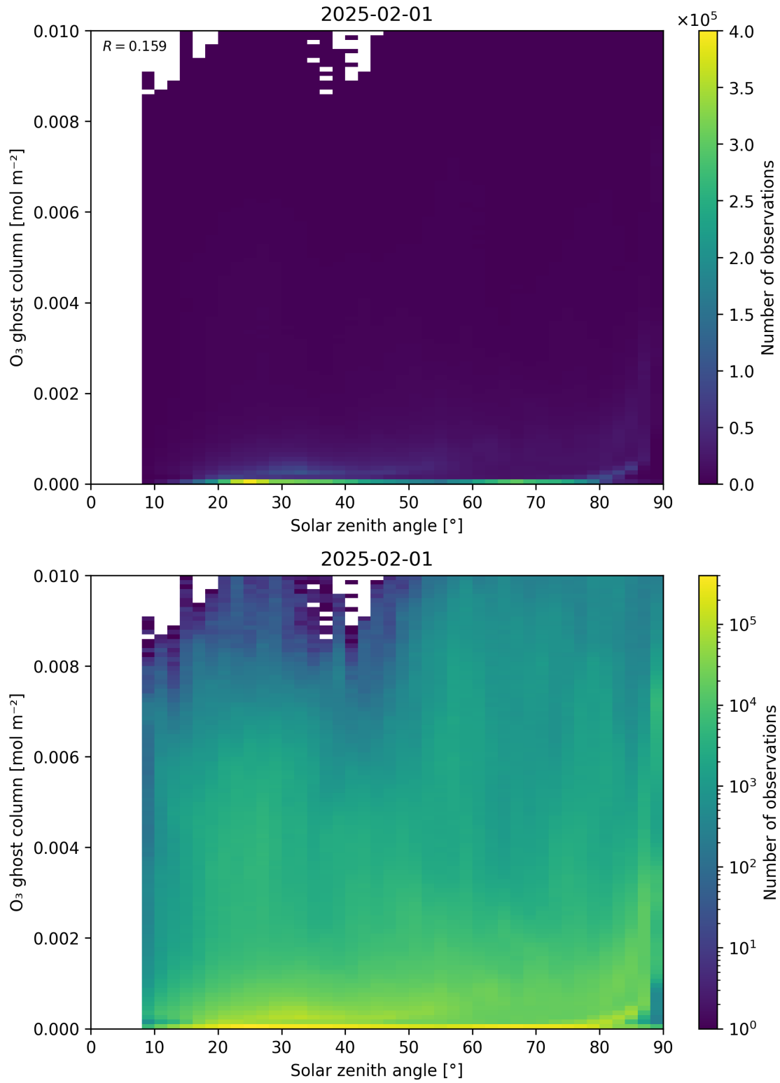
Figure 46: Scatter density plot of “Solar zenith angle” against “O 3 ghost column” for 2025-01-31 to 2025-02-02.
