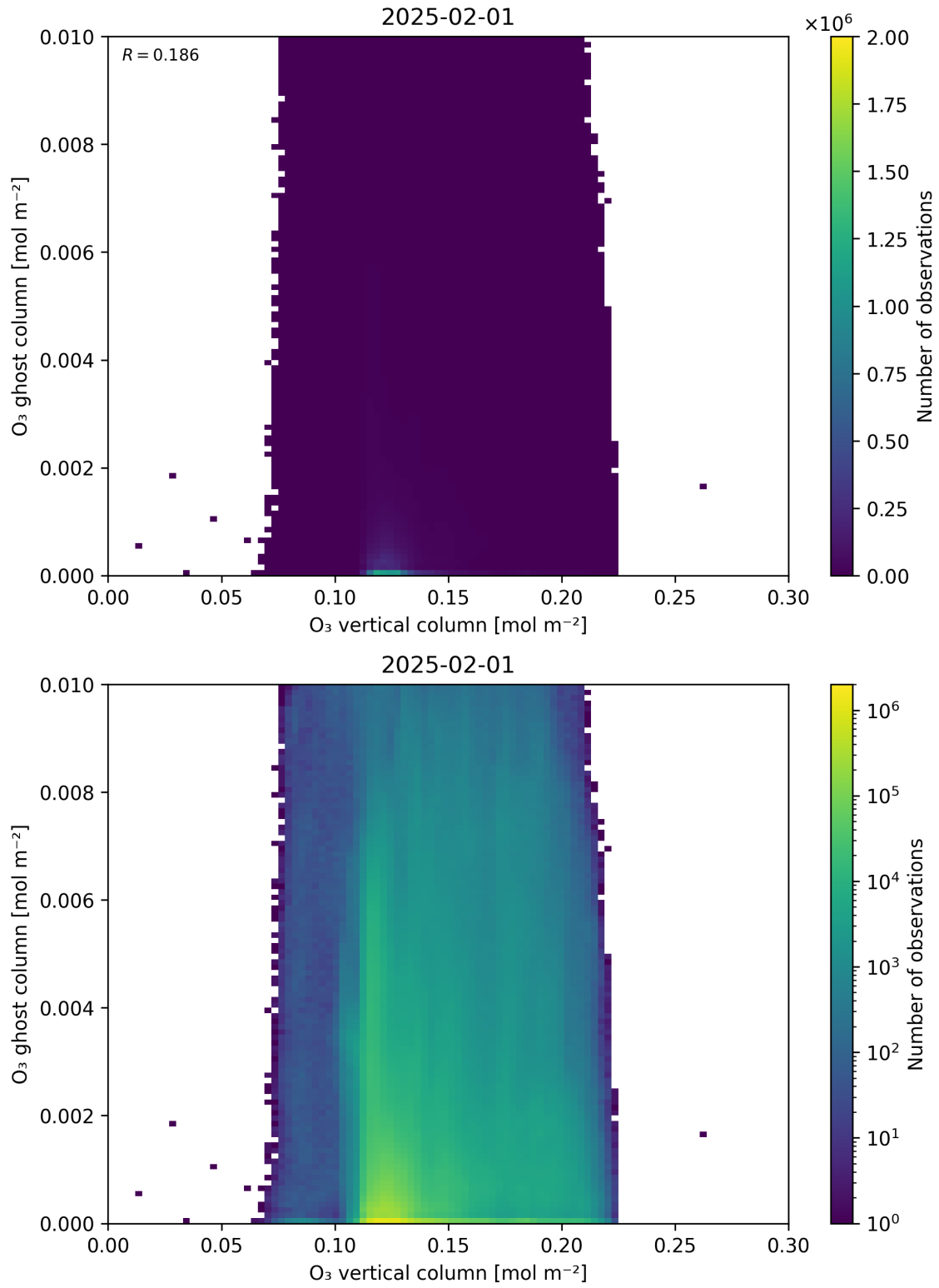
Figure 40: Scatter density plot of “O 3 vertical column” against “O 3 ghost column” for 2025-01-31 to 2025-02-02.
