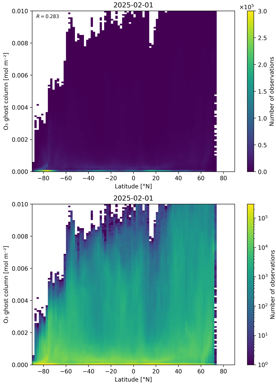
Figure 35: Scatter density plot of “Latitude” against “O 3 ghost column” for 2025-01-31 to 2025-02-02.
