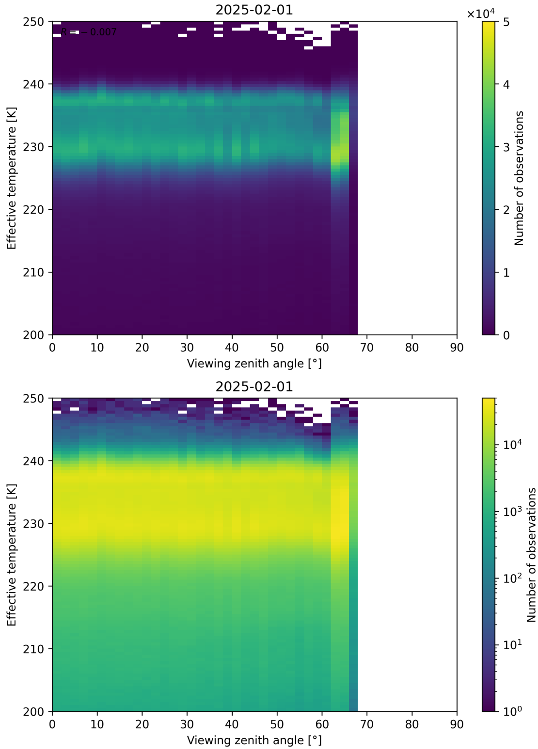
Figure 50: Scatter density plot of “Viewing zenith angle” against “Effective temperature” for 2025-01-31 to 2025-02-02.
