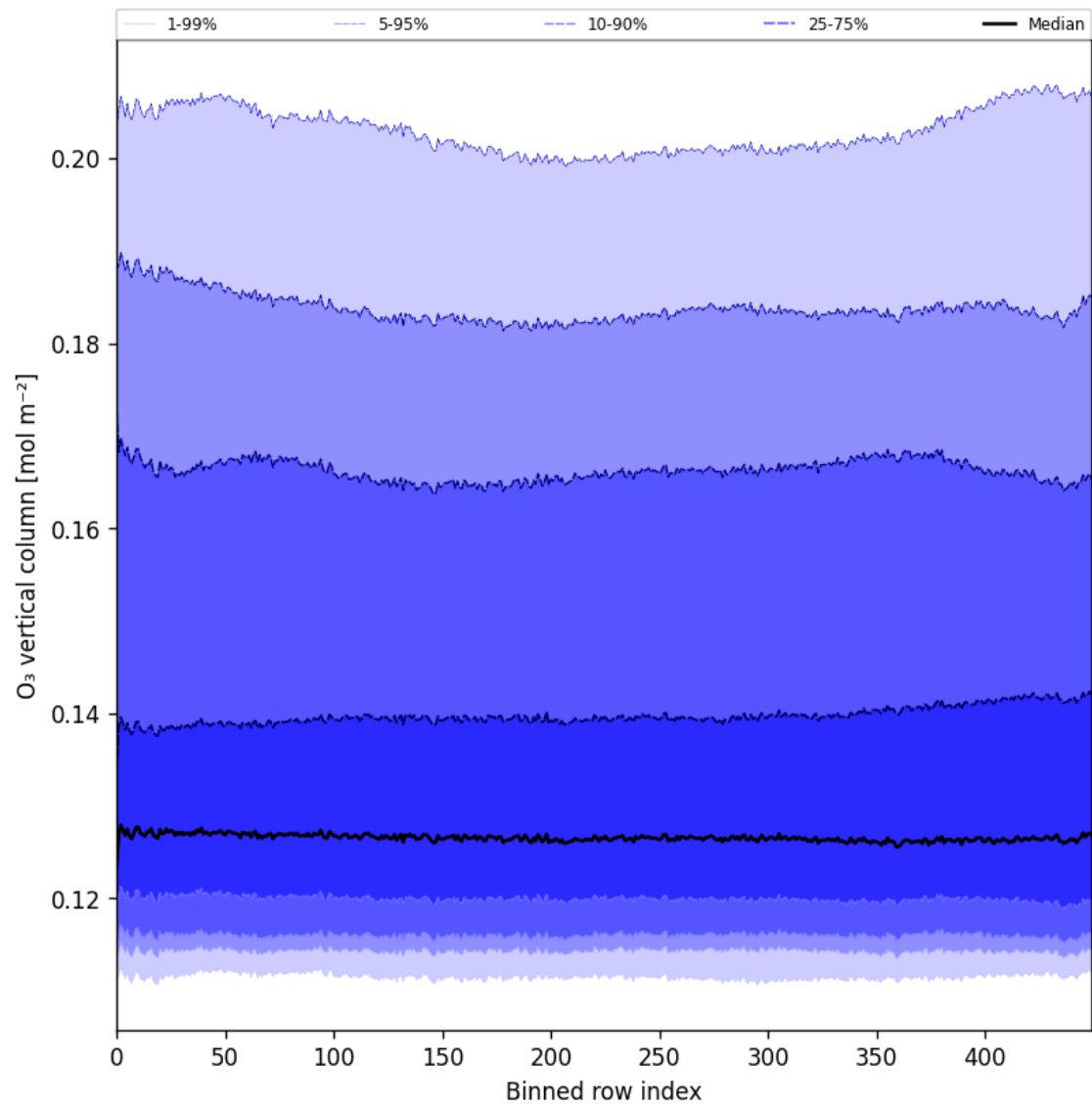
Figure 28: Along track statistics of “O 3 vertical column” for 2025-01-31 to 2025-02-02
