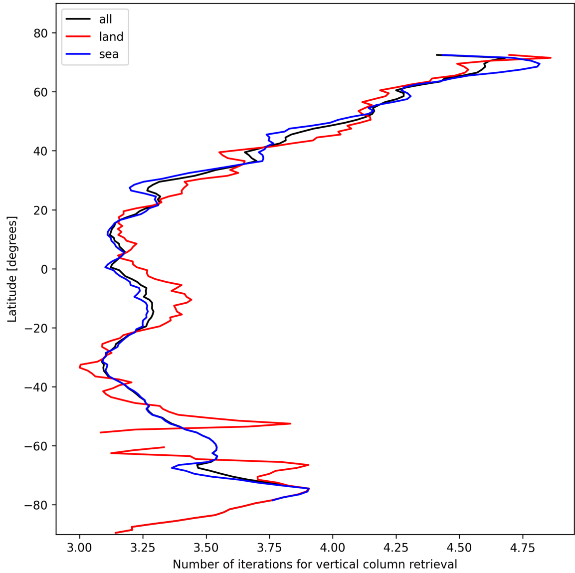
Figure 19: Zonal average of “Number of iterations for vertical column retrieval” for 2025-01-31 to 2025-02-02.
