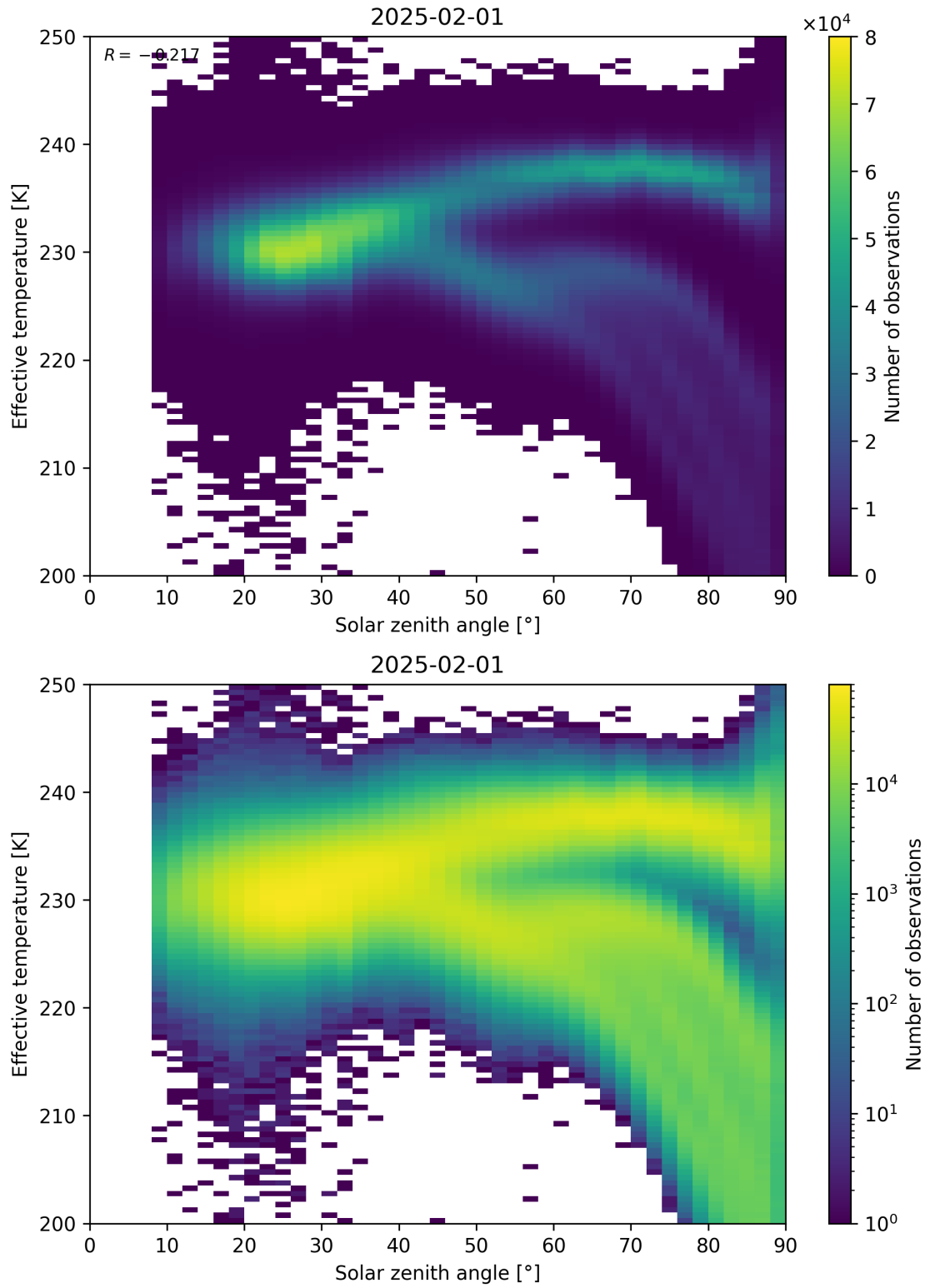
Figure 45: Scatter density plot of “Solar zenith angle” against “Effective temperature” for 2025-01-31 to 2025-02-02.
