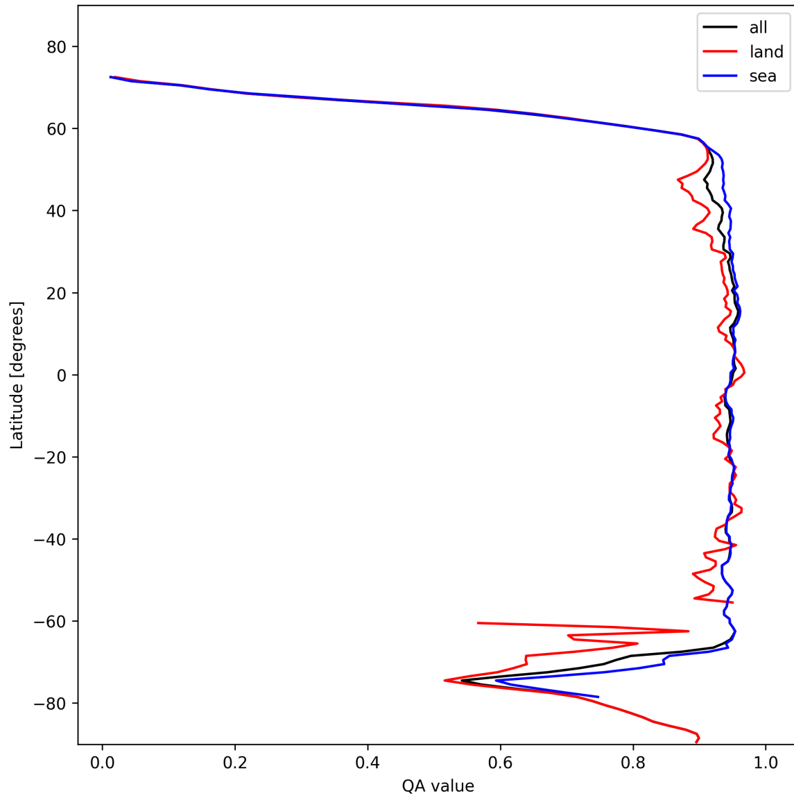
Figure 13: Zonal average of “QA value” for 2025-01-31 to 2025-02-02.
