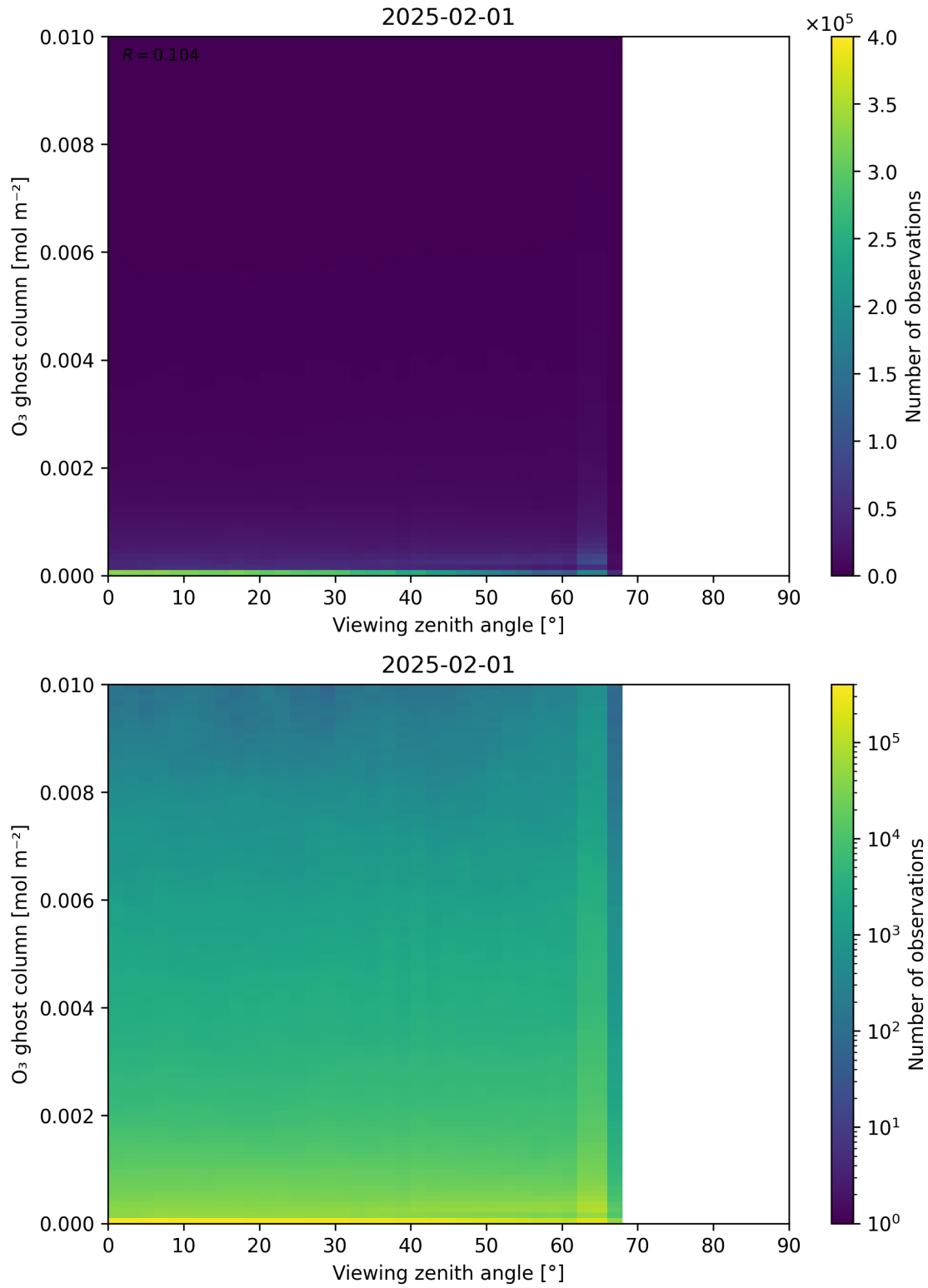
Figure 51: Scatter density plot of “Viewing zenith angle” against “O 3 ghost column” for 2025-01-31 to 2025-02-02.
