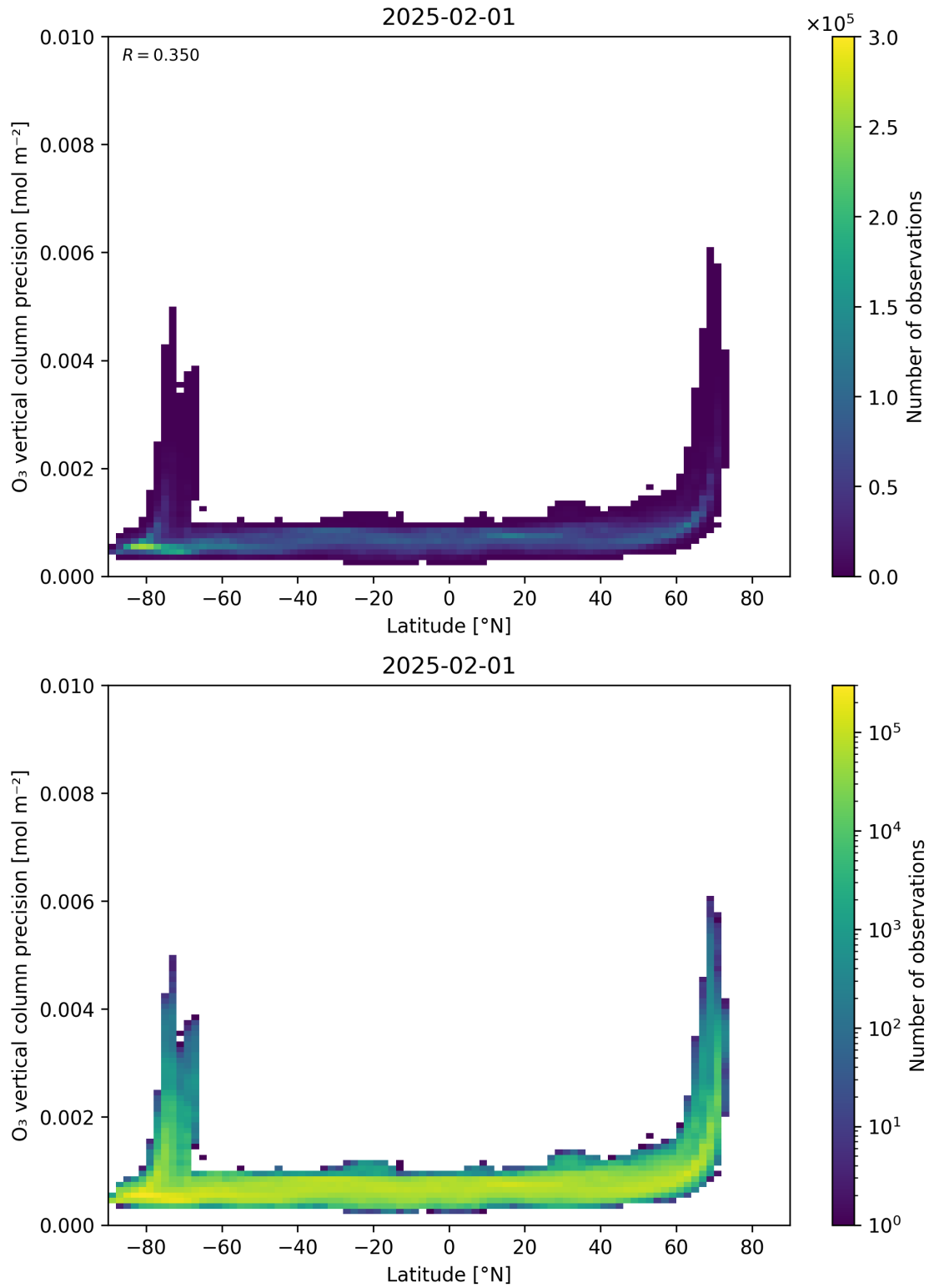
Figure 37: Scatter density plot of “Latitude” against “O 3 vertical column precision” for 2025-01-31 to 2025-02-02.
