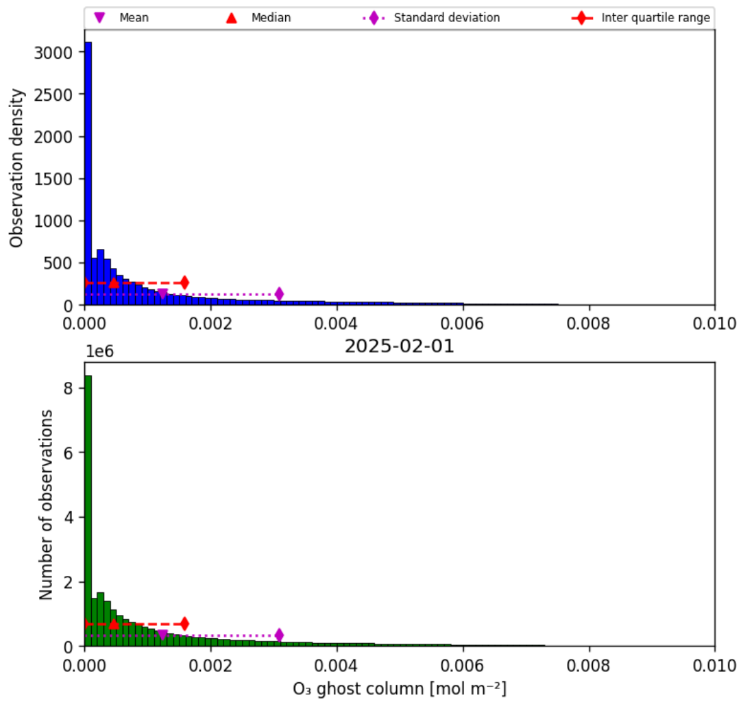
Figure 25: Histogram of “O 3 ghost column” for 2025-01-31 to 2025-02-02
