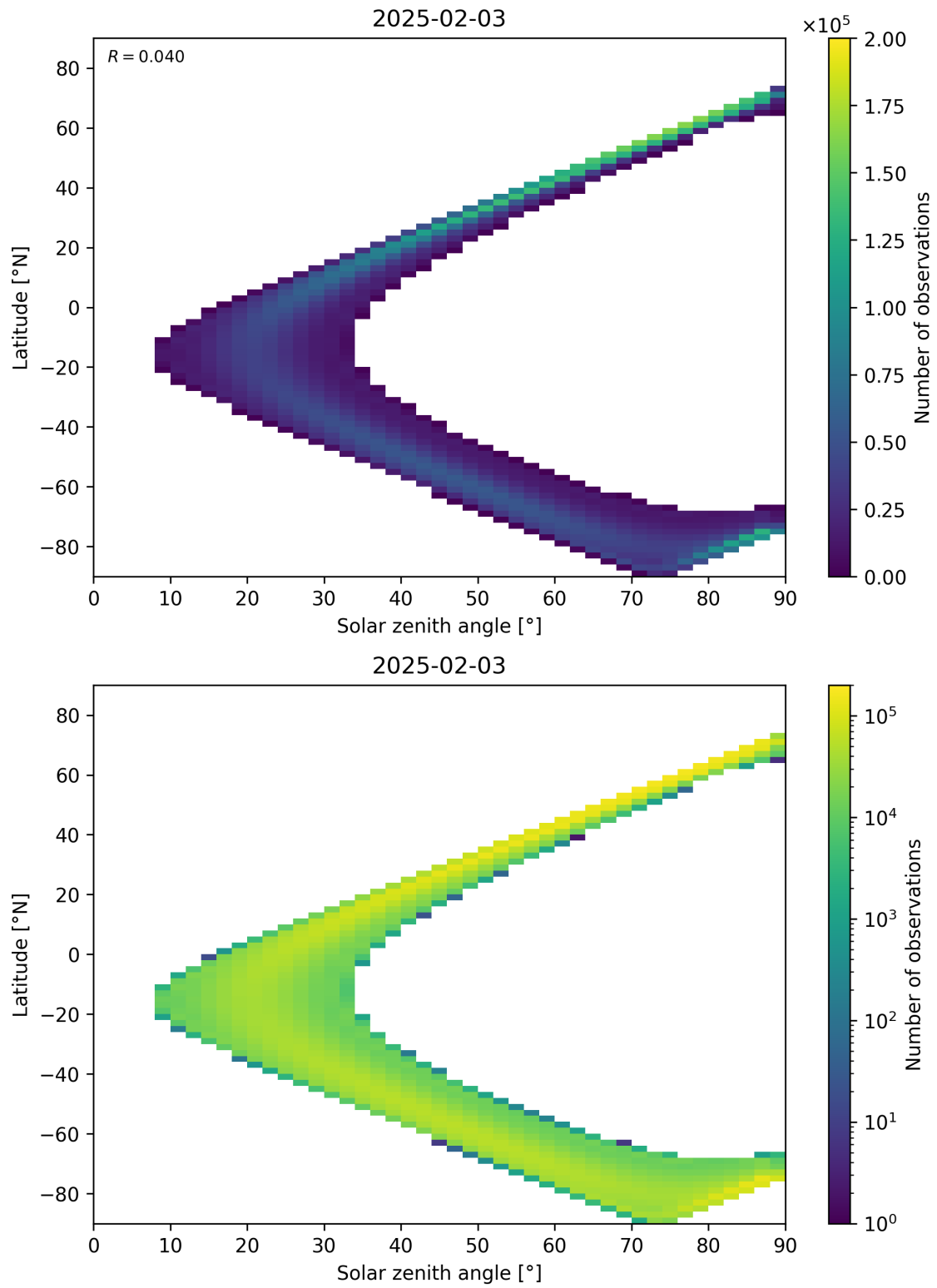
Figure 44: Scatter density plot of “Solar zenith angle” against “Latitude” for 2025-02-03 to 2025-02-04.
