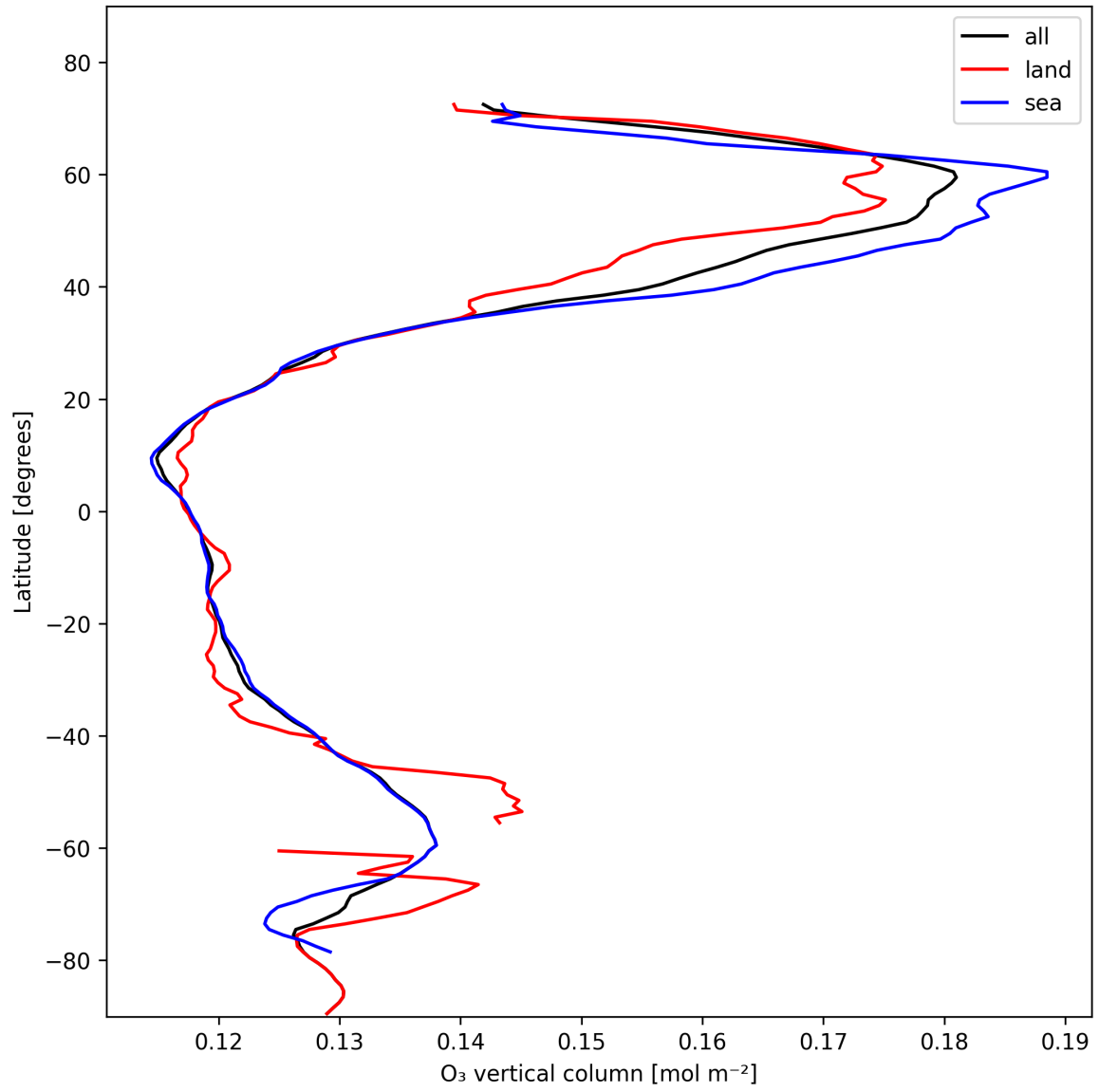
Figure 14: Zonal average of “O 3 vertical column” for 2025-02-03 to 2025-02-04.
