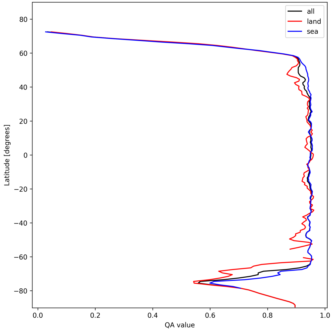
Figure 13: Zonal average of “QA value” for 2025-02-03 to 2025-02-04.
