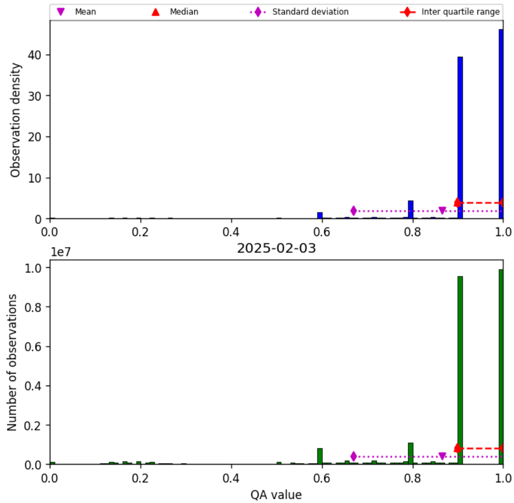
Figure 20: Histogram of “QA value” for 2025-02-03 to 2025-02-04
