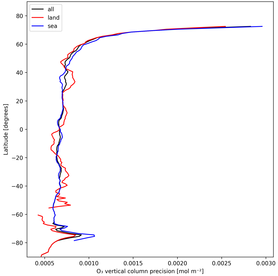
Figure 15: Zonal average of “O 3 vertical column precision” for 2025-02-03 to 2025-02-04.
