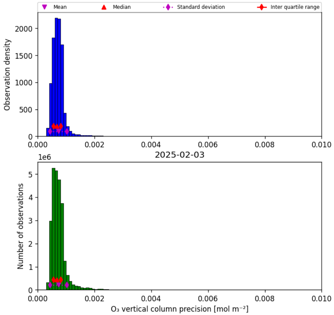
Figure 22: Histogram of “O 3 vertical column precision” for 2025-02-03 to 2025-02-04
