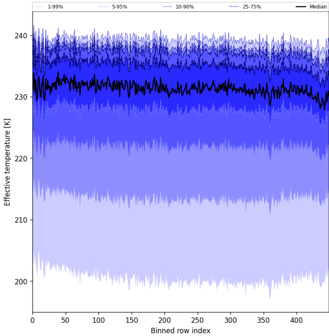
Figure 31: Along track statistics of “Effective temperature” for 2025-02-03 to 2025-02-04
