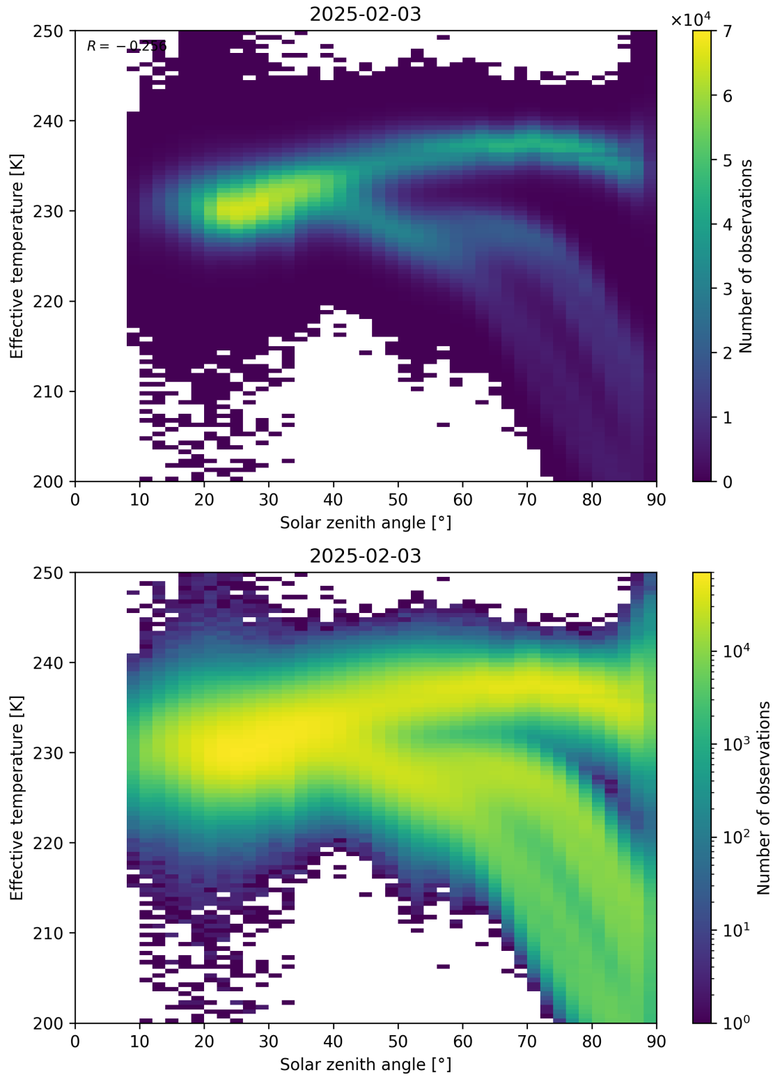
Figure 45: Scatter density plot of “Solar zenith angle” against “Effective temperature” for 2025-02-03 to 2025-02-04.
