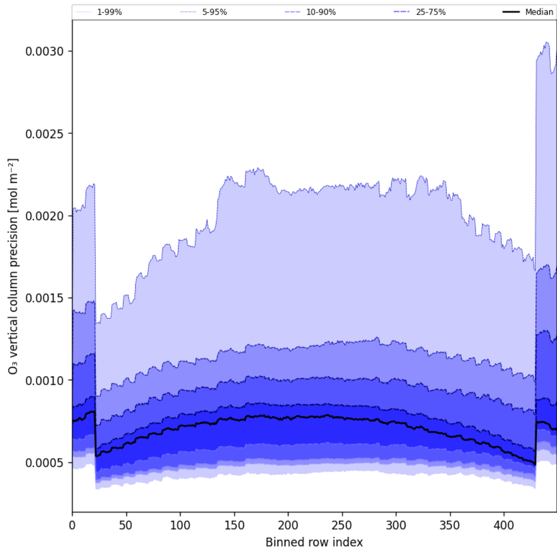
Figure 29: Along track statistics of “O 3 vertical column precision” for 2025-02-03 to 2025-02-04
