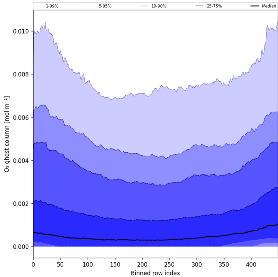
Figure 32: Along track statistics of “O 3 ghost column” for 2025-02-03 to 2025-02-04
