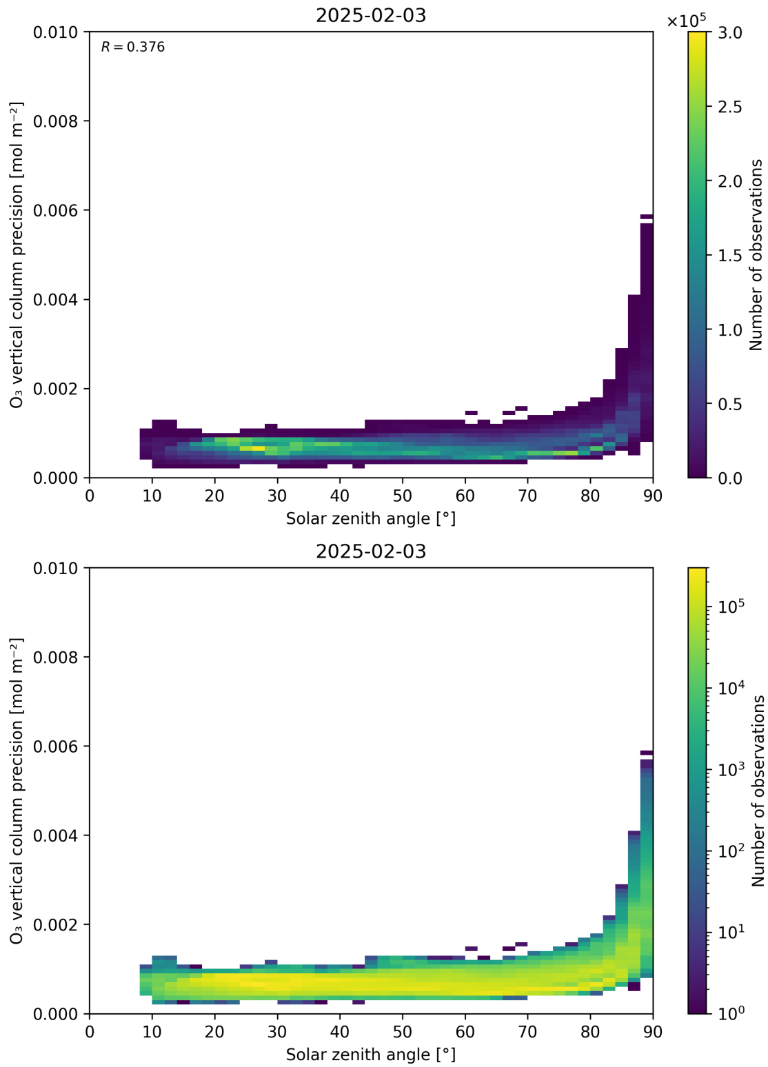
Figure 48: Scatter density plot of “Solar zenith angle” against “O 3 vertical column precision” for 2025-02-03 to 2025-02-04.
