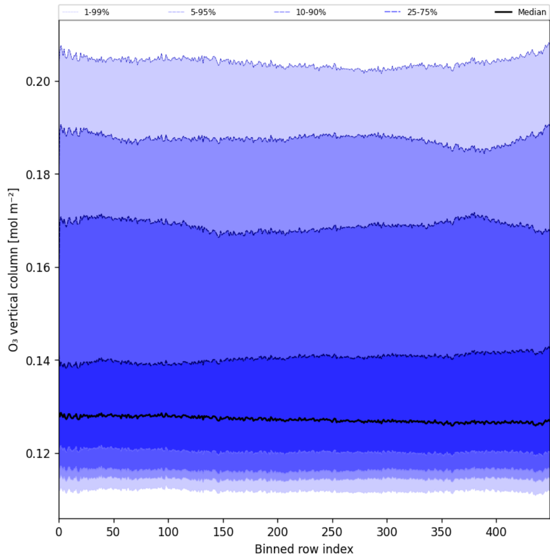
Figure 28: Along track statistics of “O 3 vertical column” for 2025-02-03 to 2025-02-04
