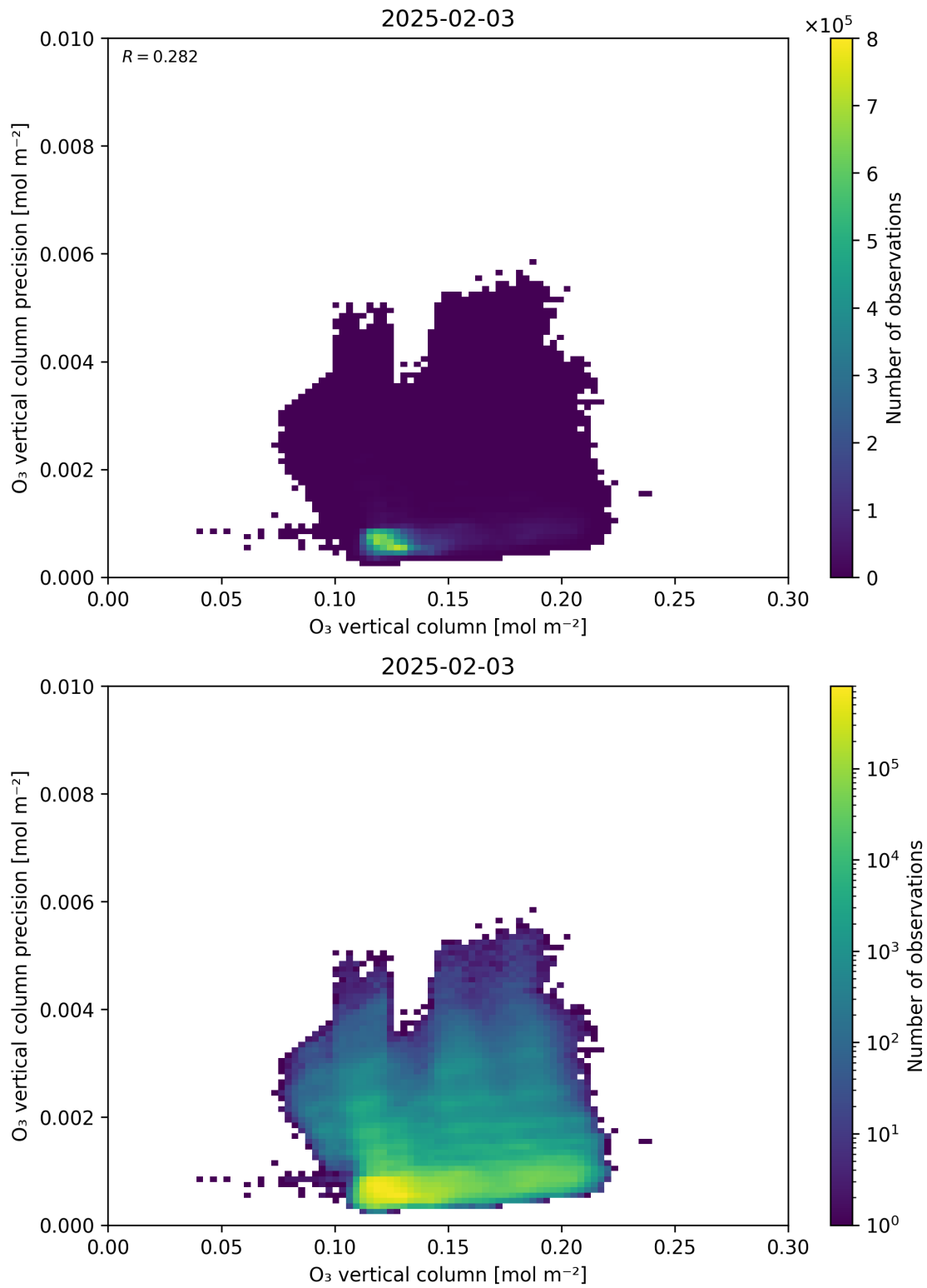
Figure 41: Scatter density plot of “O 3 vertical column” against “O 3 vertical column precision” for 2025-02-03 to 2025-02-04.
