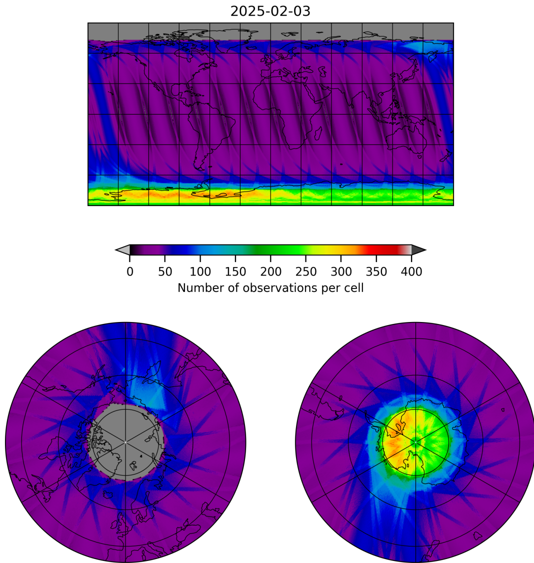
Figure 12: Map of the number of observations for 2025-02-03 to 2025-02-04
