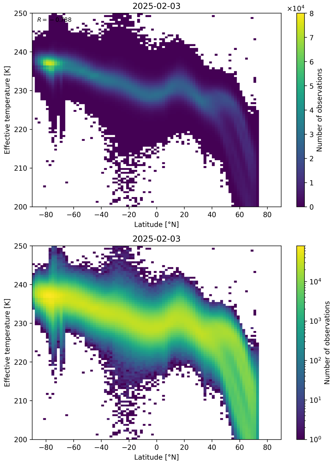
Figure 34: Scatter density plot of “Latitude” against “Effective temperature” for 2025-02-03 to 2025-02-04.
