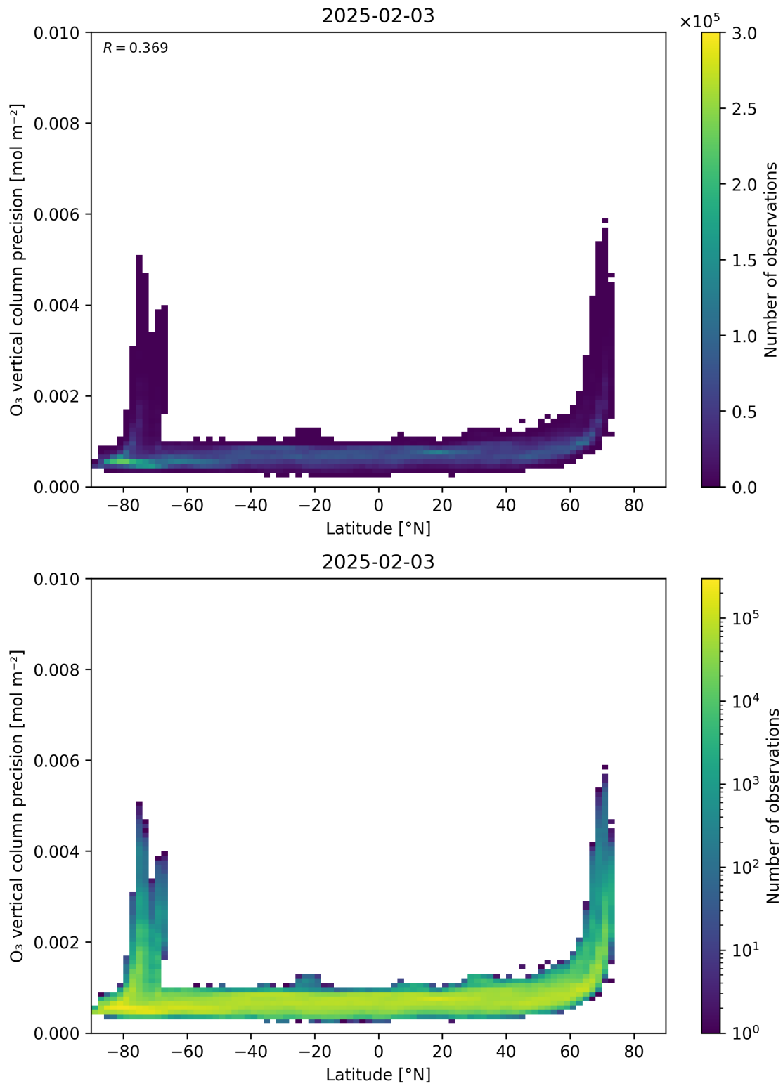
Figure 37: Scatter density plot of “Latitude” against “O 3 vertical column precision” for 2025-02-03 to 2025-02-04.
