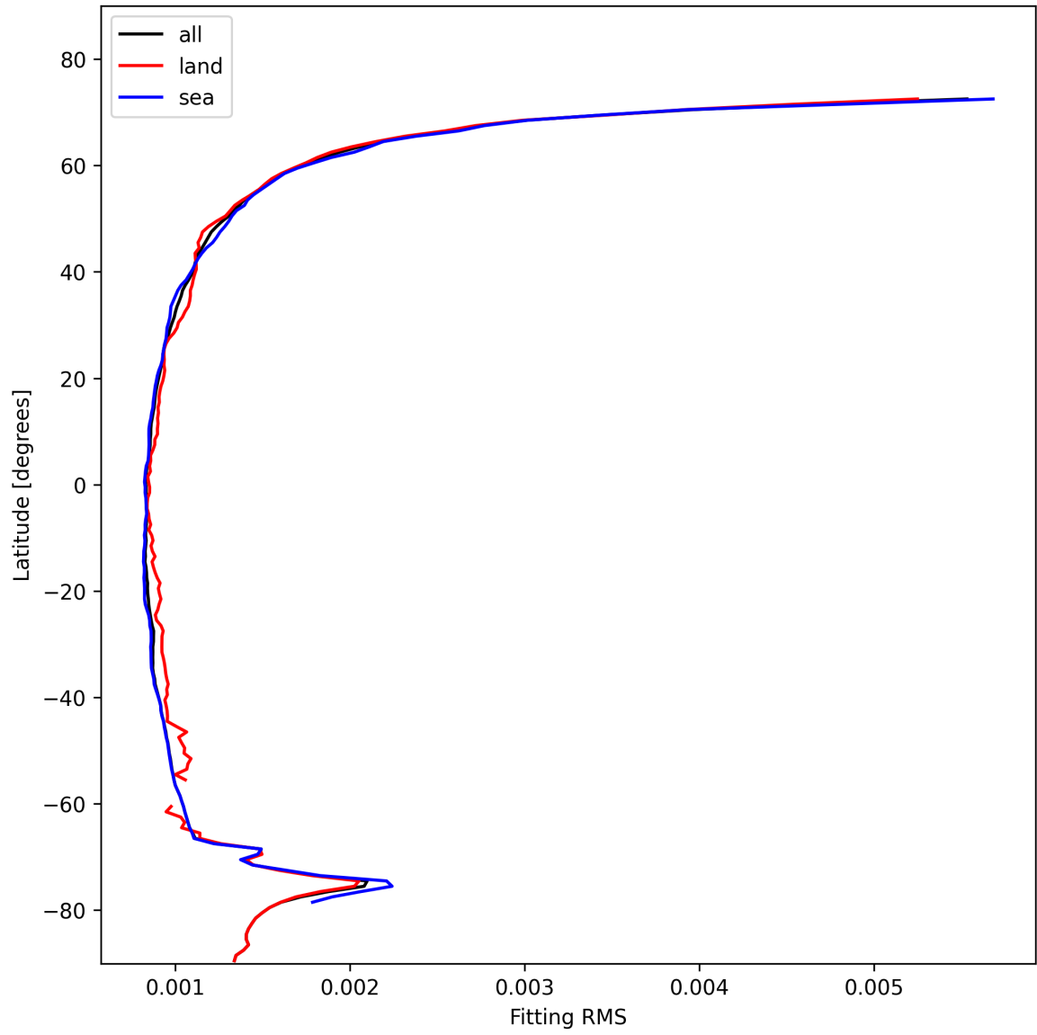
Figure 16: Zonal average of “Fitting RMS” for 2025-02-03 to 2025-02-04.
