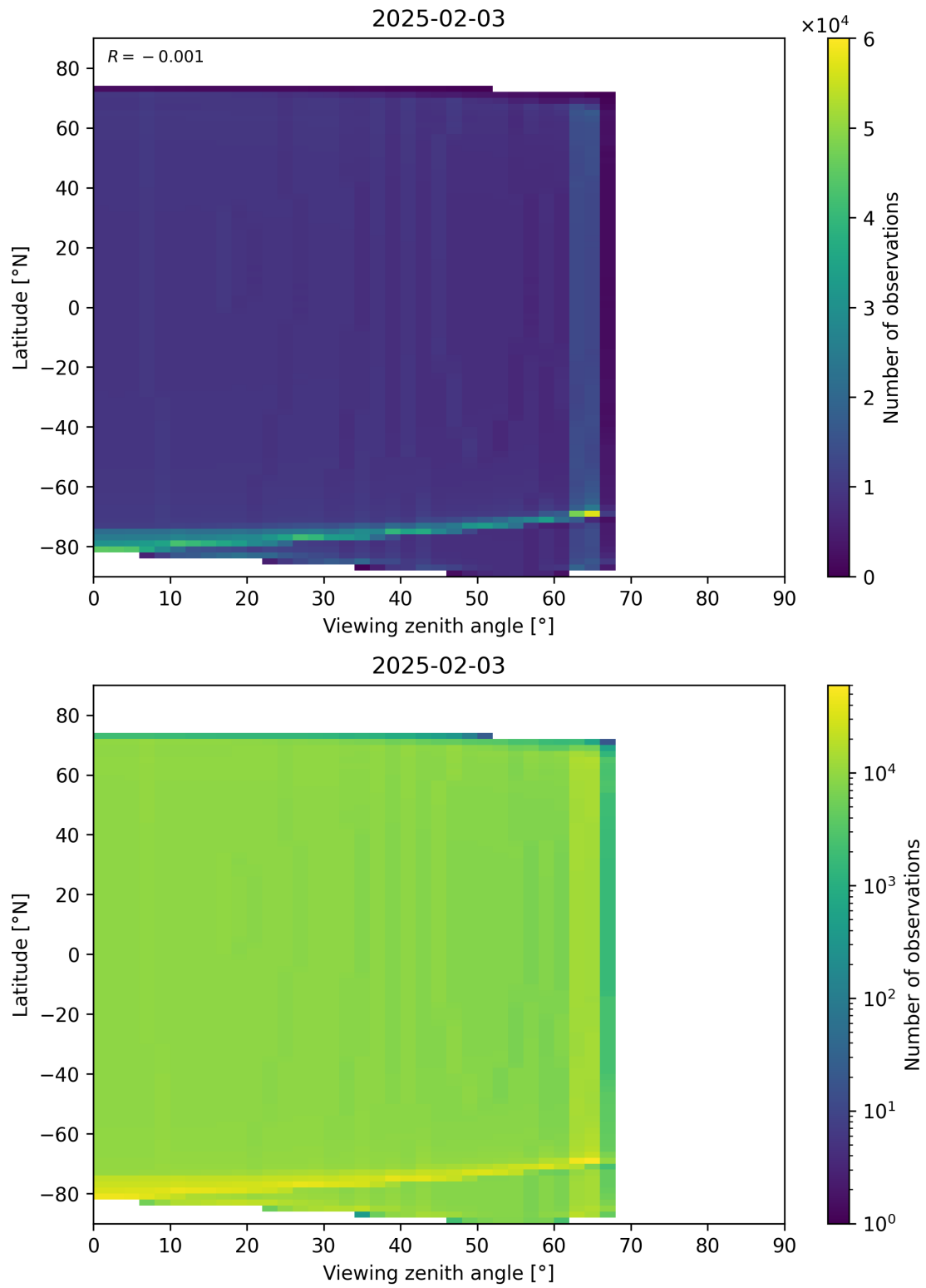
Figure 49: Scatter density plot of “Viewing zenith angle” against “Latitude” for 2025-02-03 to 2025-02-04.
