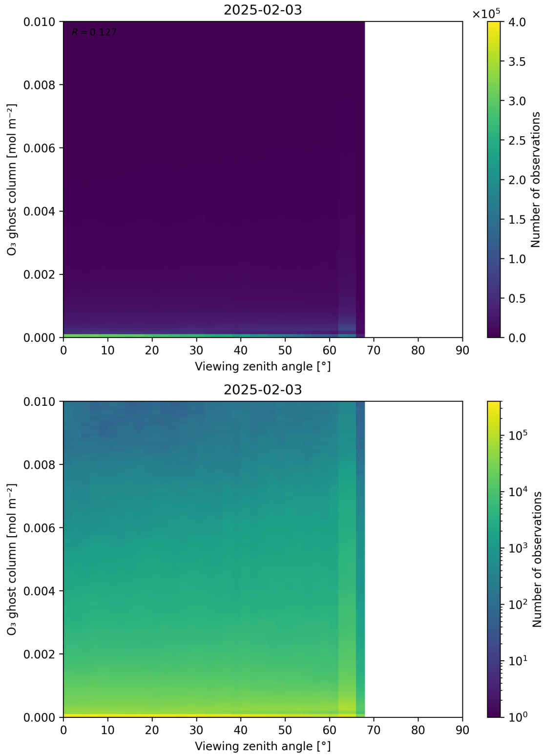
Figure 51: Scatter density plot of “Viewing zenith angle” against “O 3 ghost column” for 2025-02-03 to 2025-02-04.
