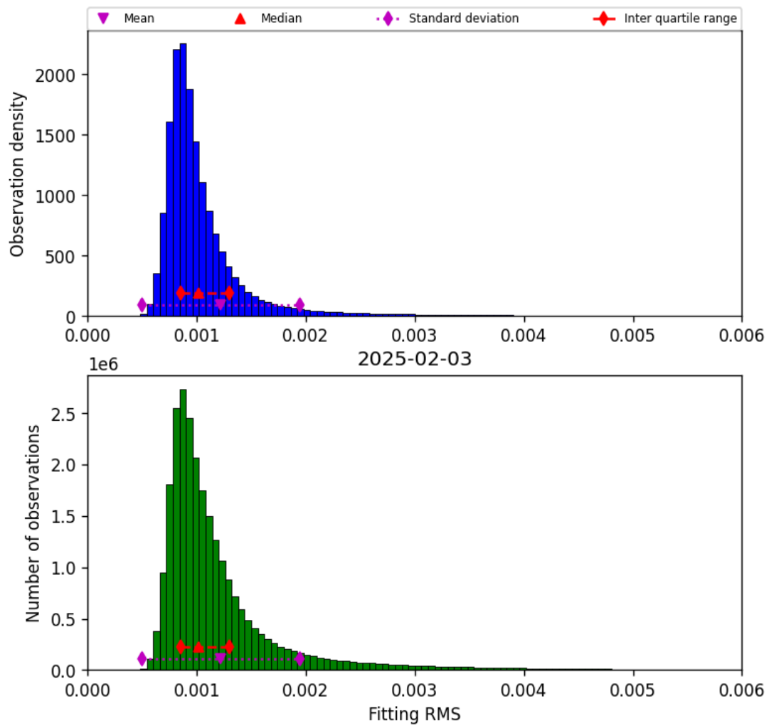
Figure 23: Histogram of “Fitting RMS” for 2025-02-03 to 2025-02-04
