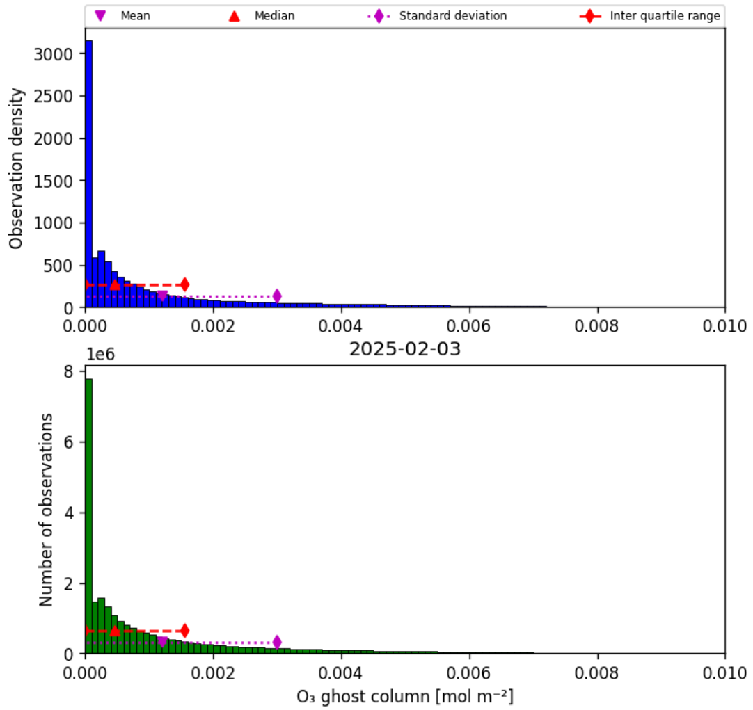
Figure 25: Histogram of “O 3 ghost column” for 2025-02-03 to 2025-02-04
