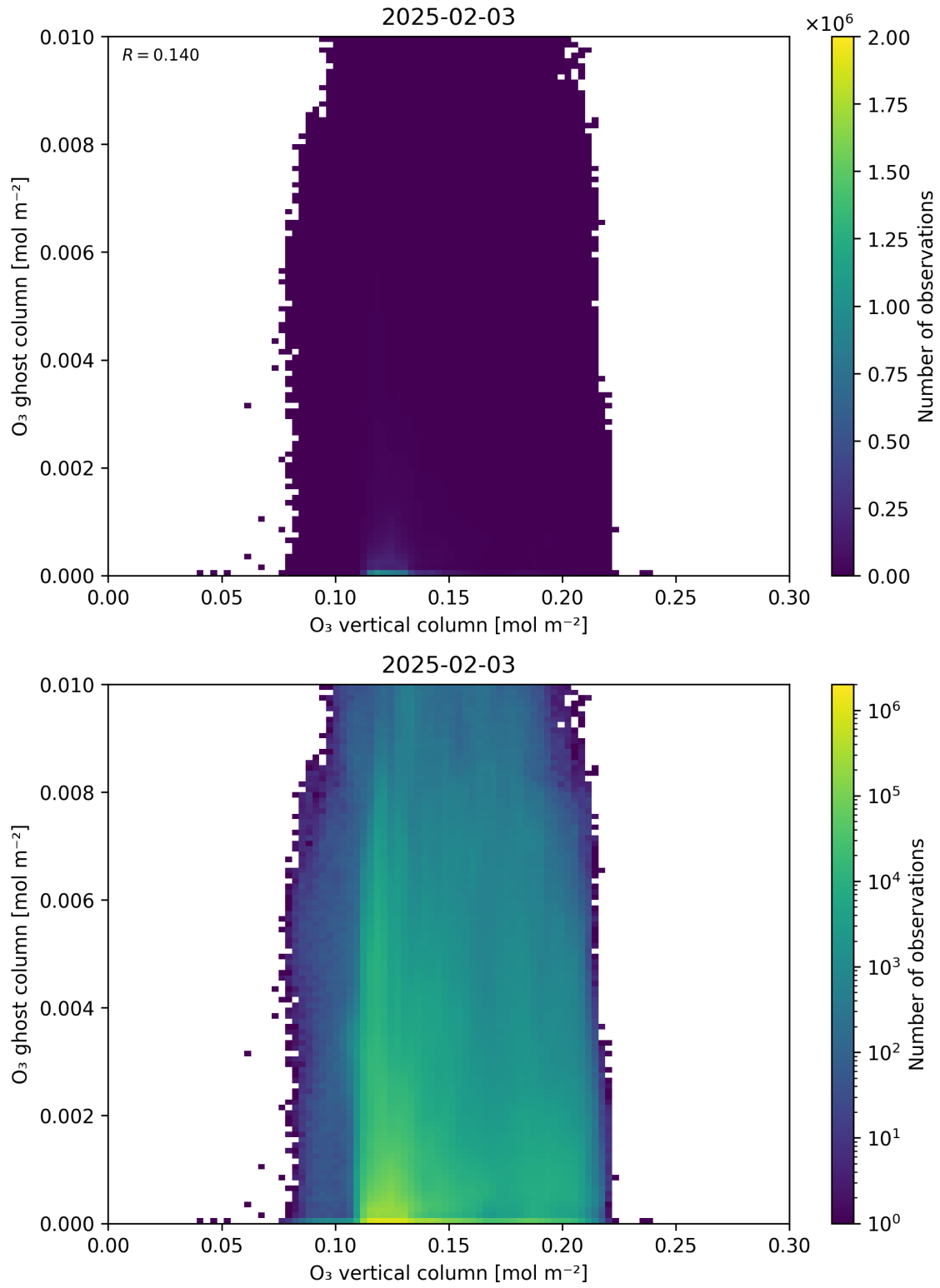
Figure 40: Scatter density plot of “O 3 vertical column” against “O 3 ghost column” for 2025-02-03 to 2025-02-04.
