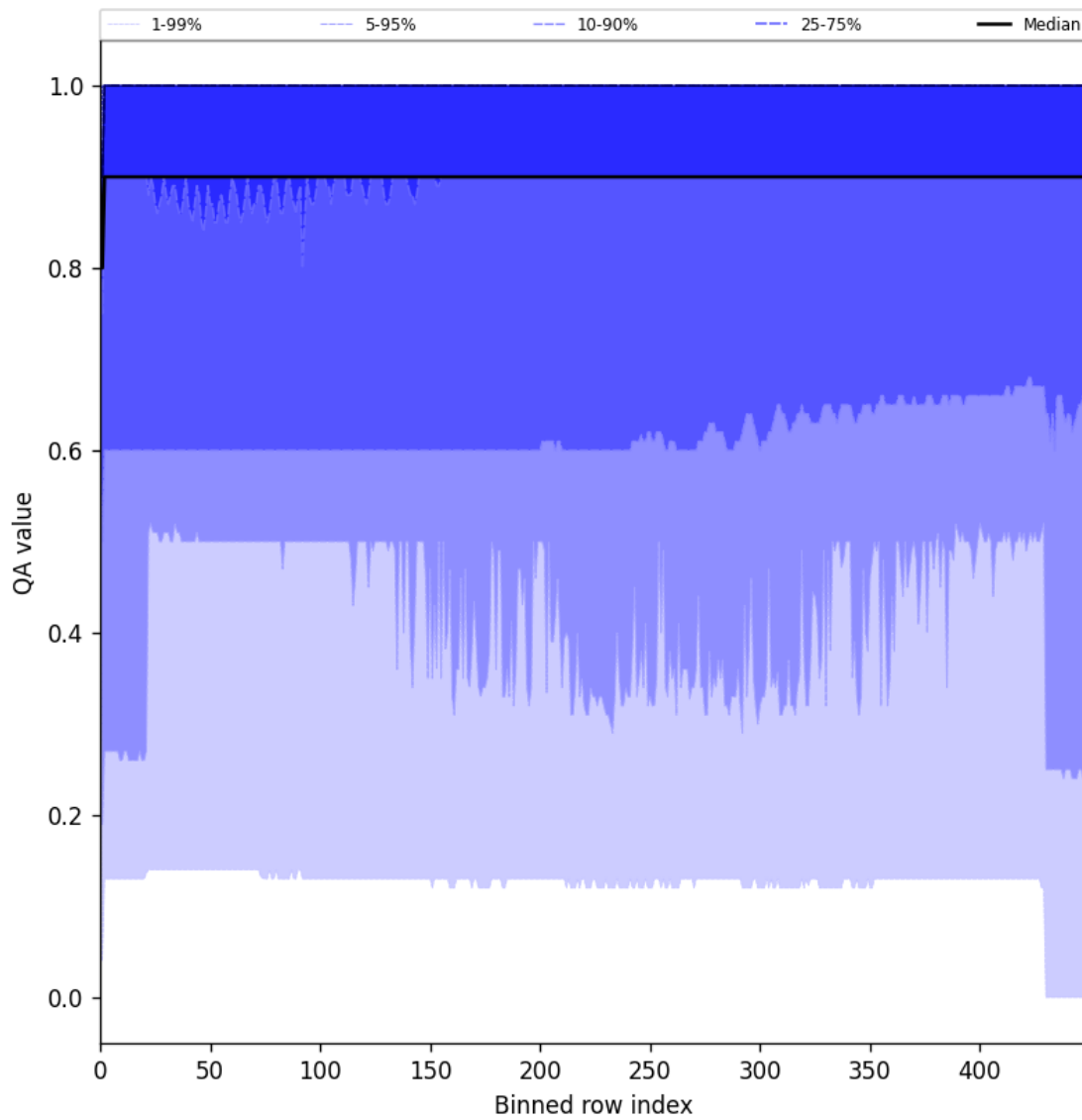
Figure 27: Along track statistics of “QA value” for 2025-02-03 to 2025-02-04
