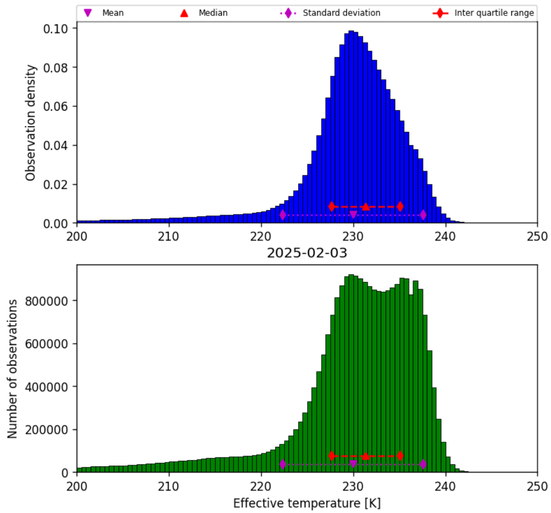
Figure 24: Histogram of “Effective temperature” for 2025-02-03 to 2025-02-04
