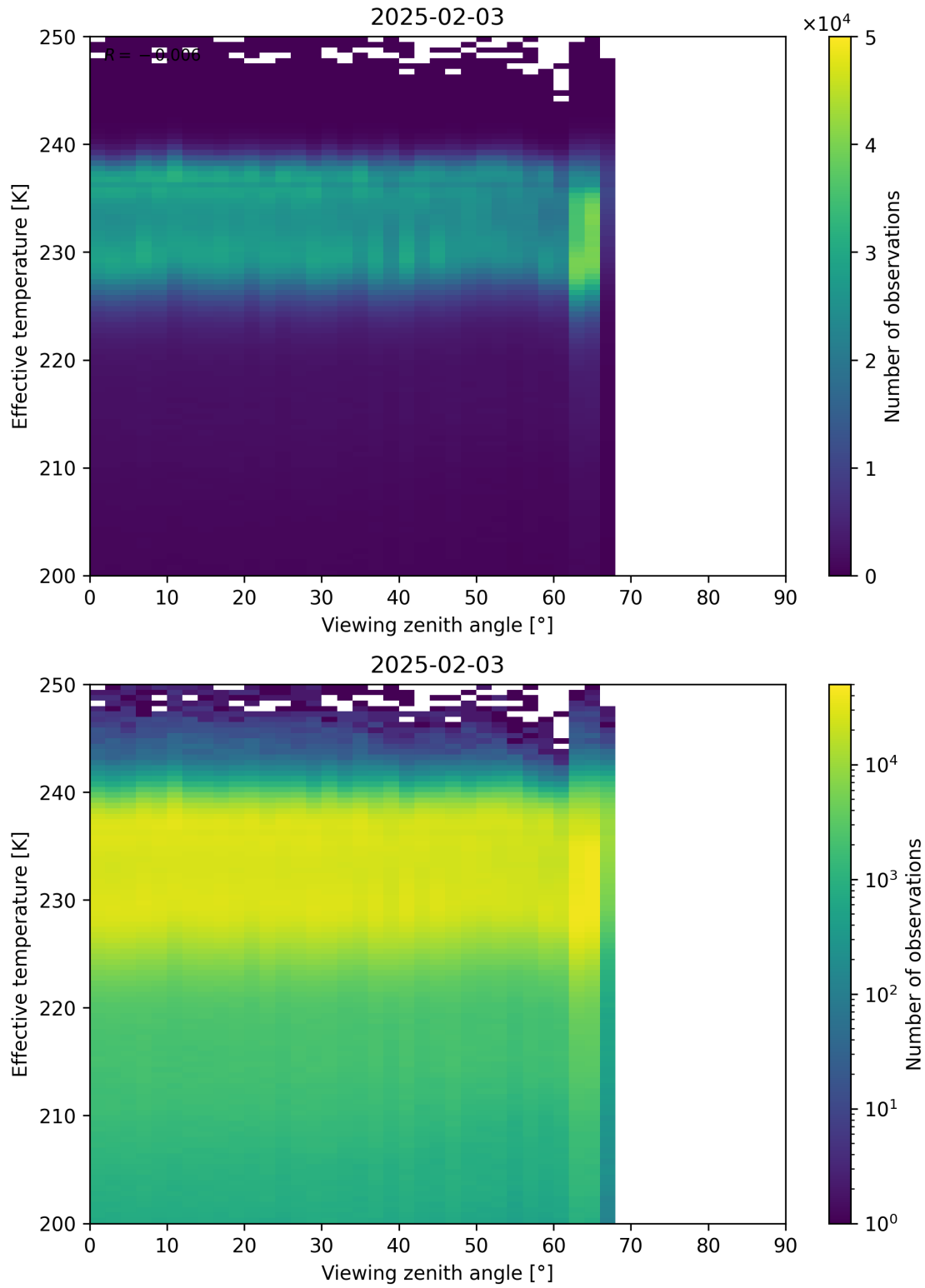
Figure 50: Scatter density plot of “Viewing zenith angle” against “Effective temperature” for 2025-02-03 to 2025-02-04.
