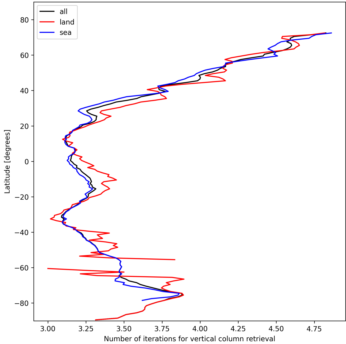
Figure 19: Zonal average of “Number of iterations for vertical column retrieval” for 2025-02-03 to 2025-02-04.
