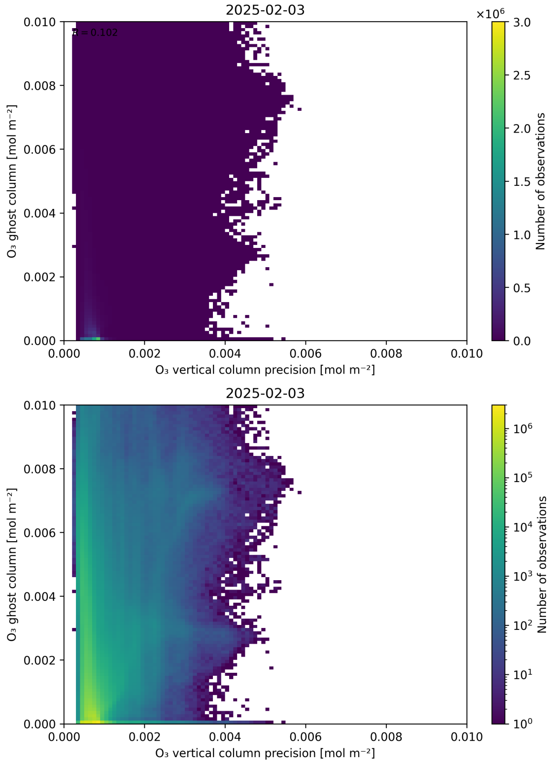
Figure 43: Scatter density plot of “O 3 vertical column precision” against “O 3 ghost column” for 2025-02-03 to 2025-02-04.
