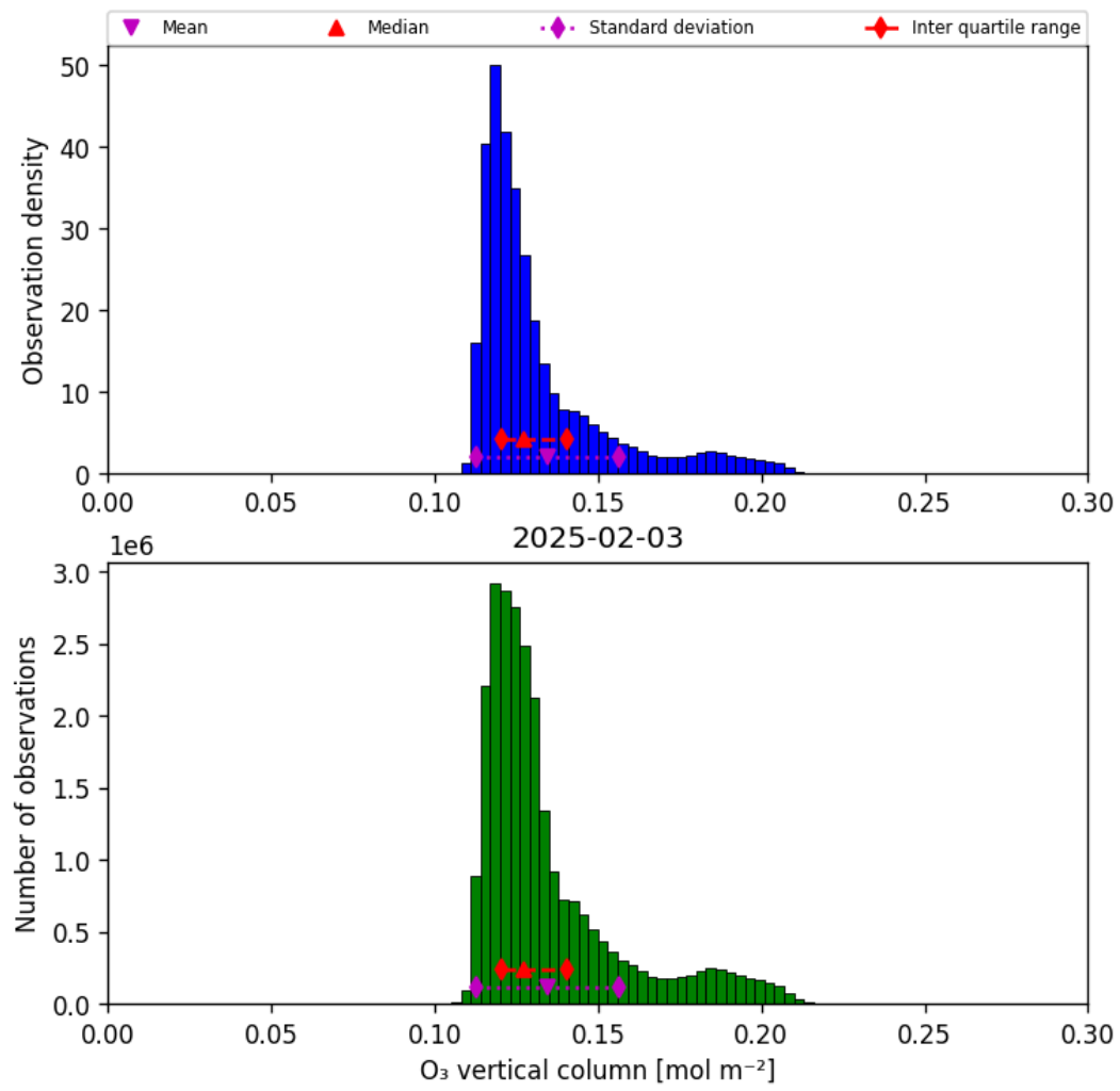
Figure 21: Histogram of “O 3 vertical column” for 2025-02-03 to 2025-02-04
