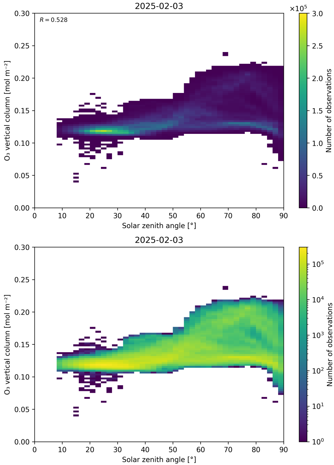
Figure 47: Scatter density plot of “Solar zenith angle” against “O 3 vertical column” for 2025-02-03 to 2025-02-04.
