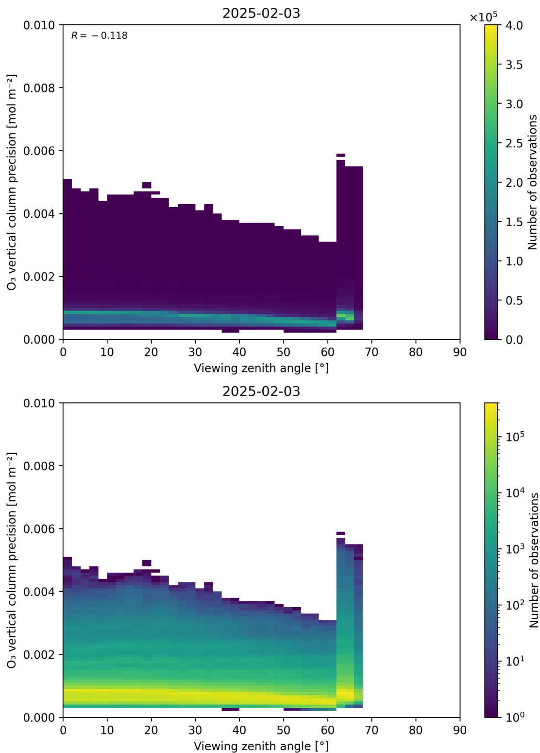
Figure 53: Scatter density plot of “Viewing zenith angle” against “O 3 vertical column precision” for 2025-02-03 to 2025-02-04.
