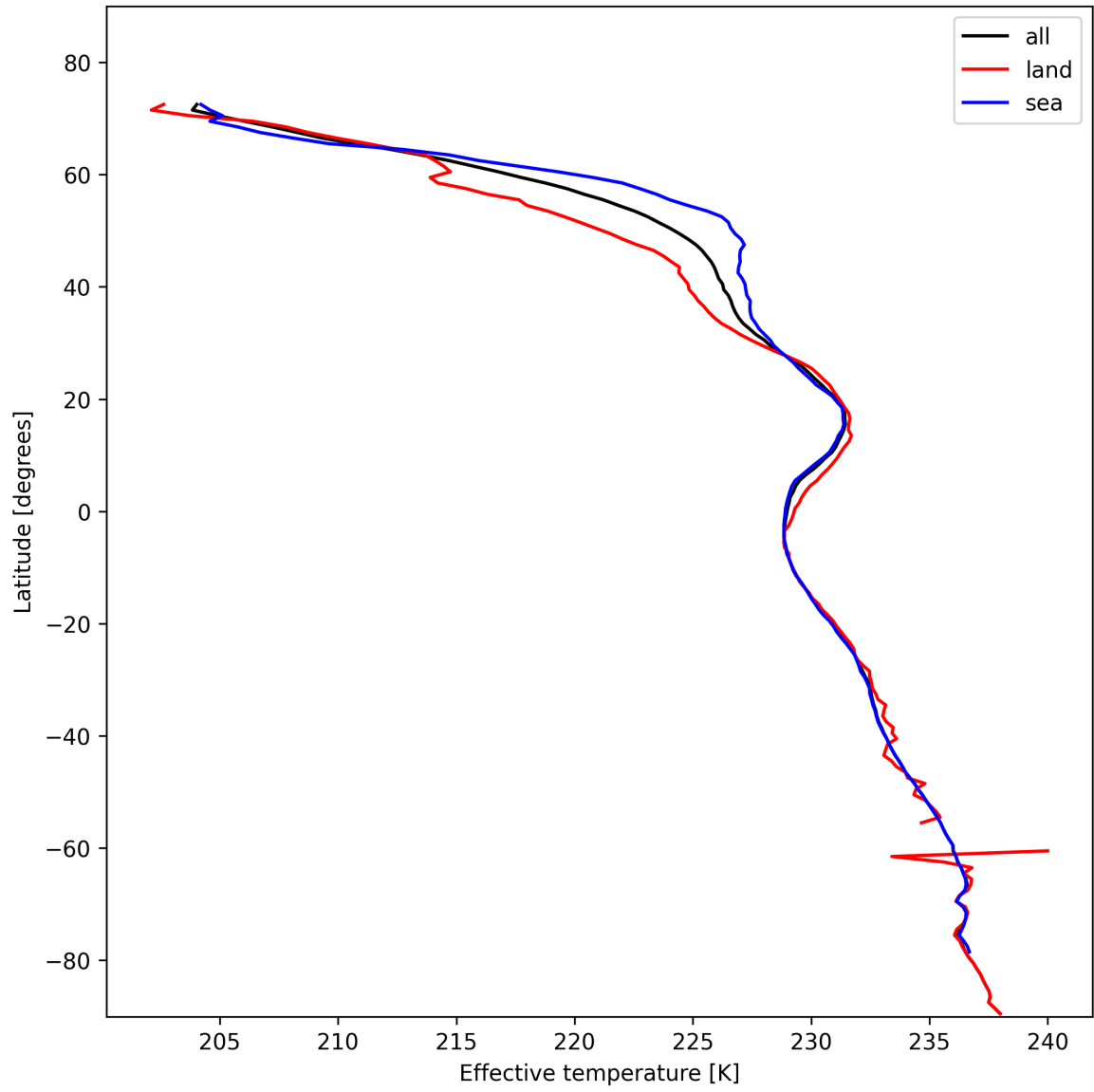
Figure 17: Zonal average of “Effective temperature” for 2025-02-03 to 2025-02-04.
