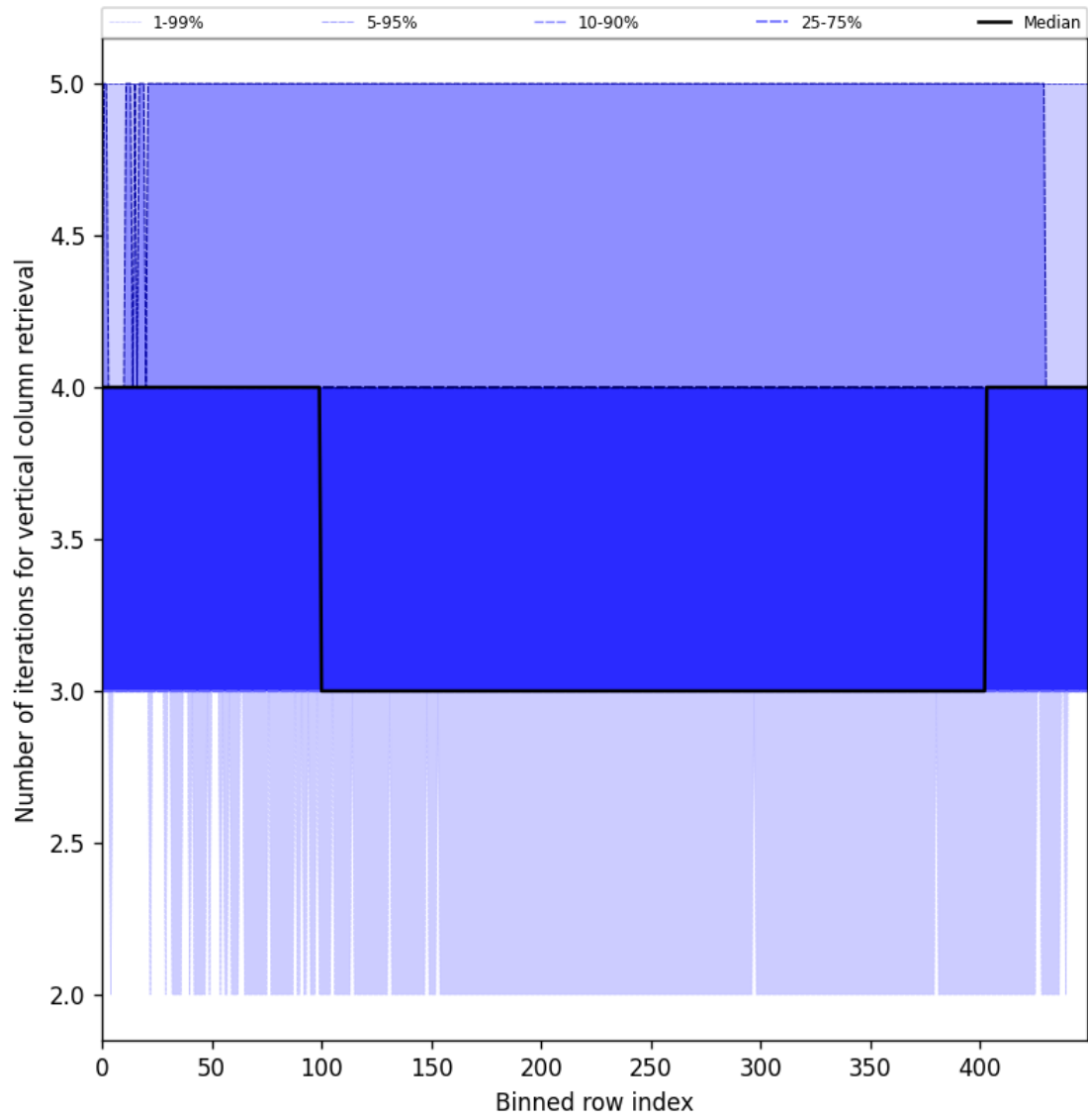
Figure 33: Along track statistics of “Number of iterations for vertical column retrieval” for 2025-02-03 to 2025-02-04
