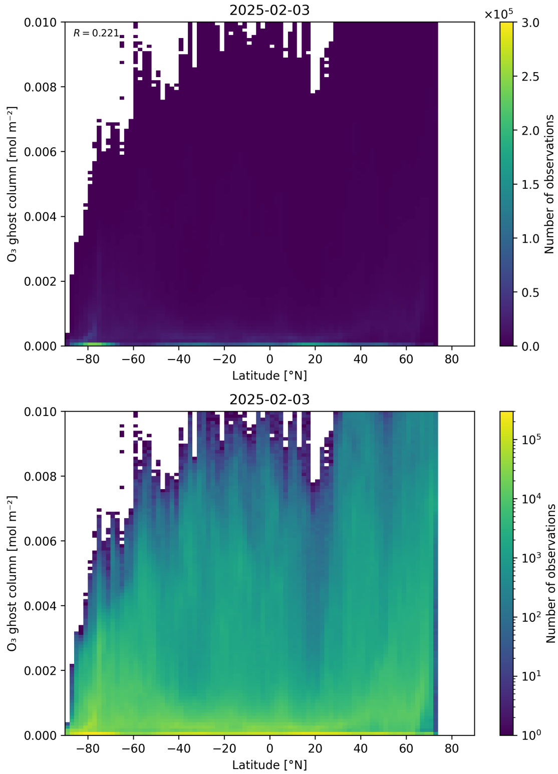
Figure 35: Scatter density plot of “Latitude” against “O 3 ghost column” for 2025-02-03 to 2025-02-04.
