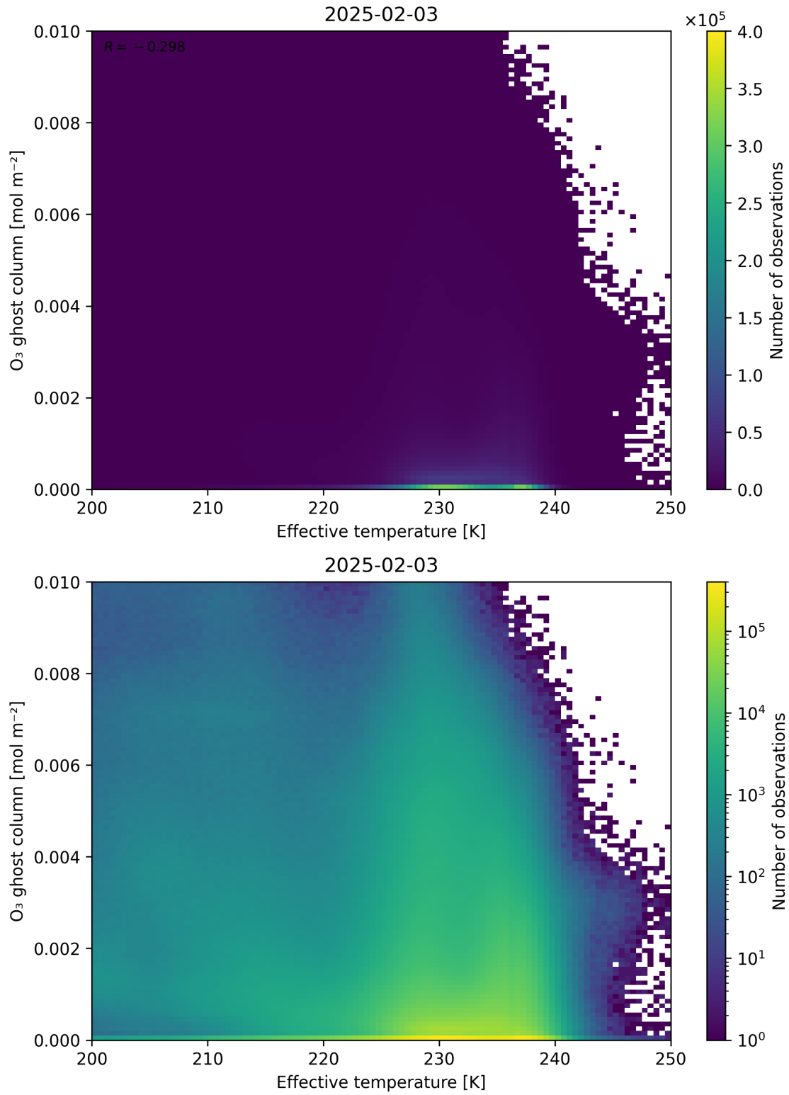
Figure 38: Scatter density plot of “Effective temperature” against “O 3 ghost column” for 2025-02-03 to 2025-02-04.
