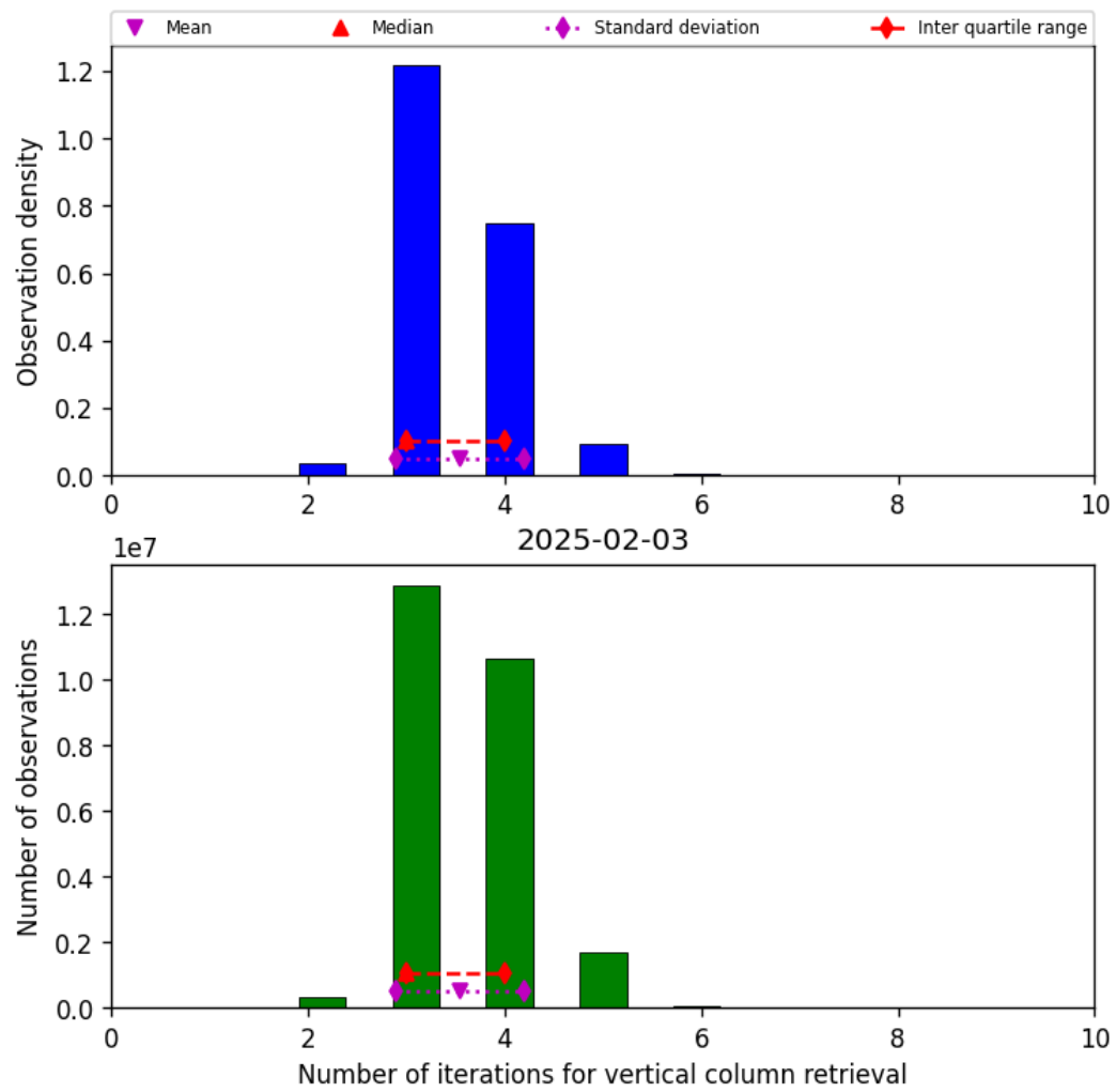
Figure 26: Histogram of “Number of iterations for vertical column retrieval” for 2025-02-03 to 2025-02-04
