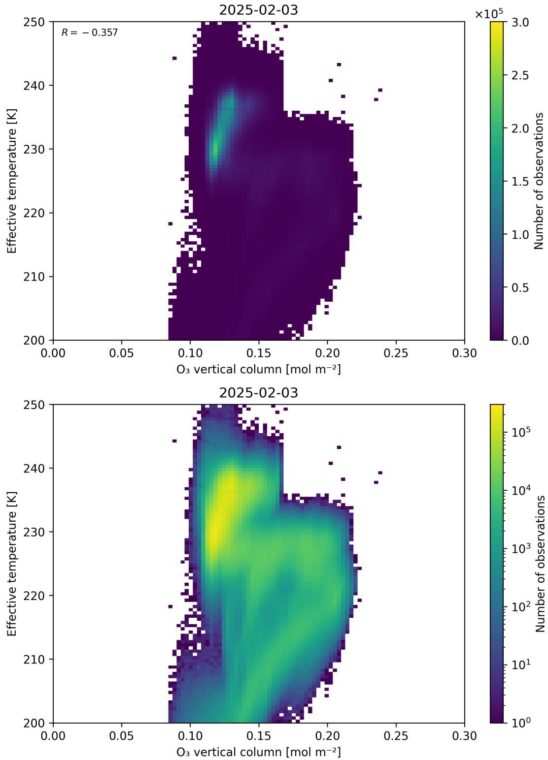
Figure 39: Scatter density plot of “O 3 vertical column” against “Effective temperature” for 2025-02-03 to 2025-02-04.
