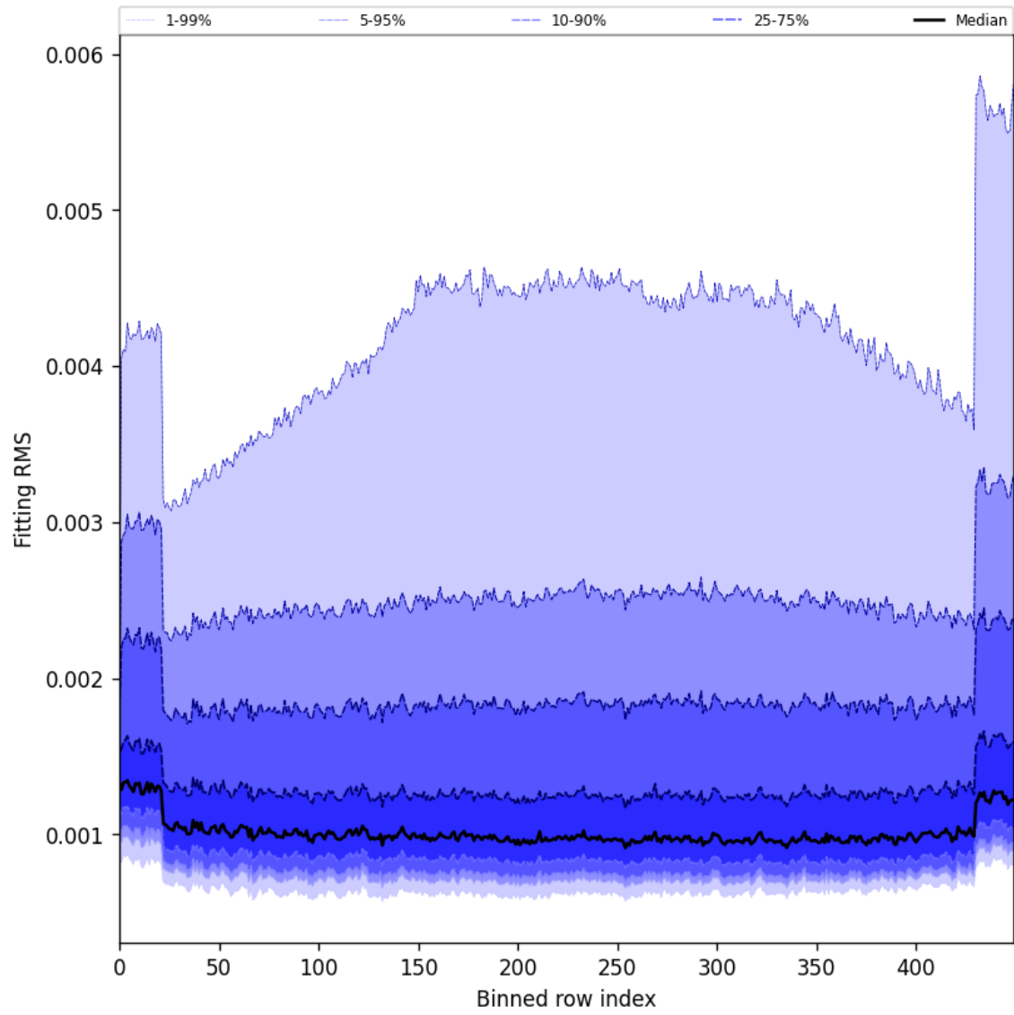
Figure 30: Along track statistics of “Fitting RMS” for 2025-02-03 to 2025-02-04
