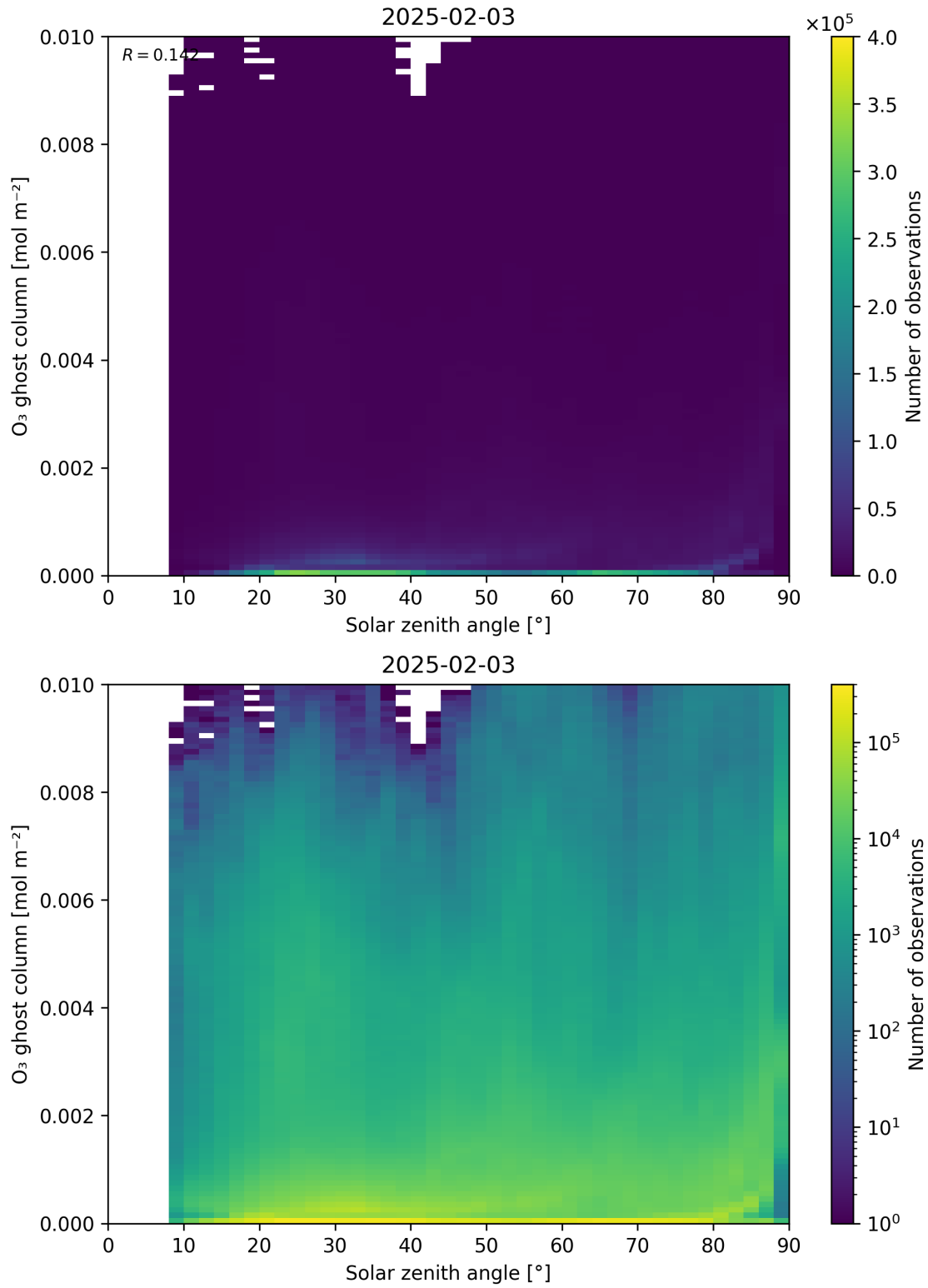
Figure 46: Scatter density plot of “Solar zenith angle” against “O 3 ghost column” for 2025-02-03 to 2025-02-04.
