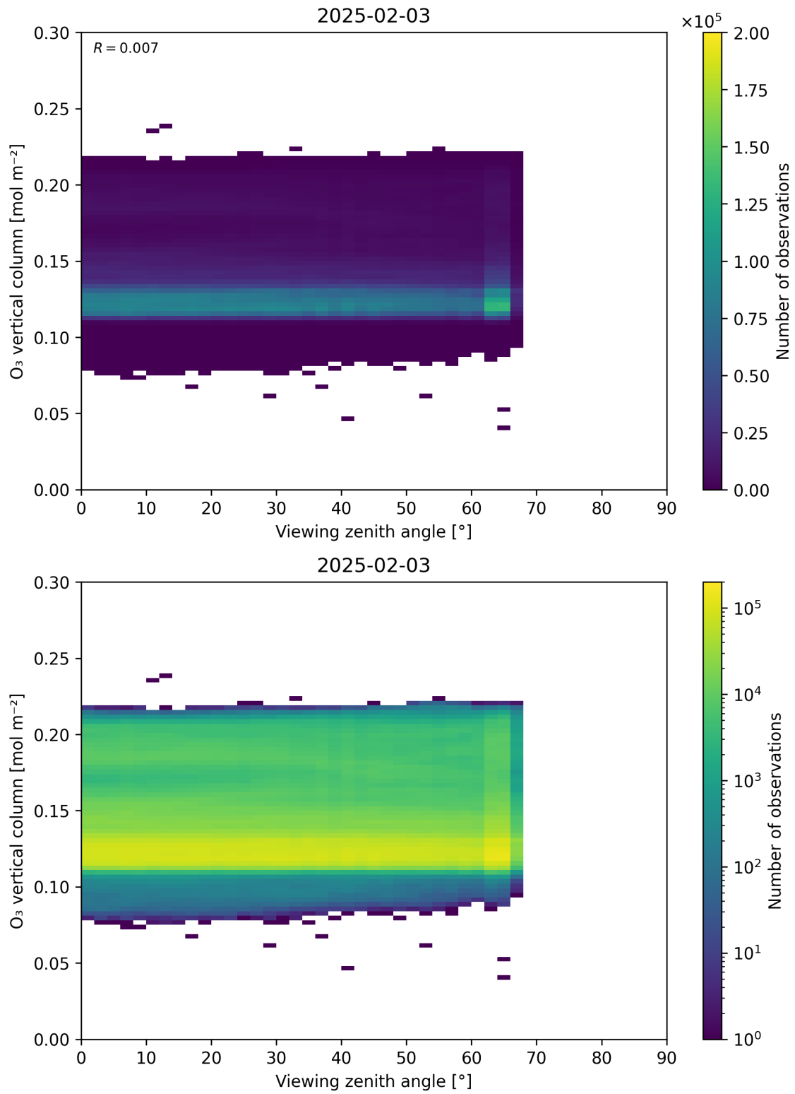
Figure 52: Scatter density plot of “Viewing zenith angle” against “O 3 vertical column” for 2025-02-03 to 2025-02-04.
