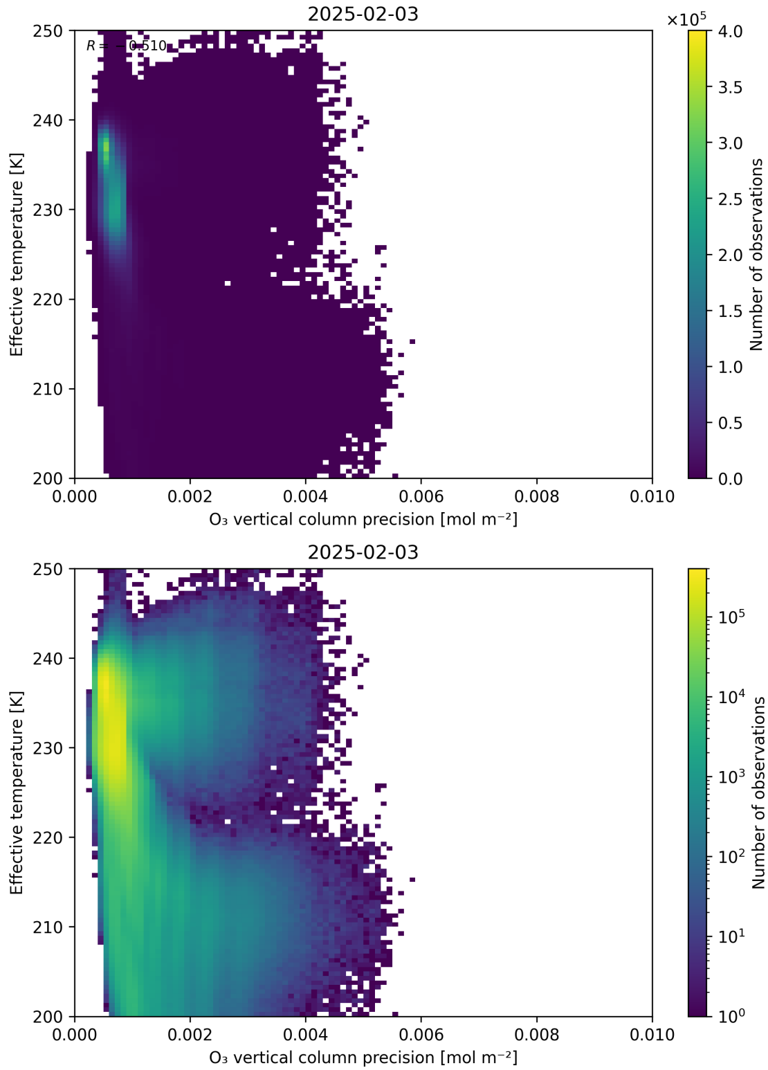
Figure 42: Scatter density plot of “O 3 vertical column precision” against “Effective temperature” for 2025-02-03 to 2025-02-04.
