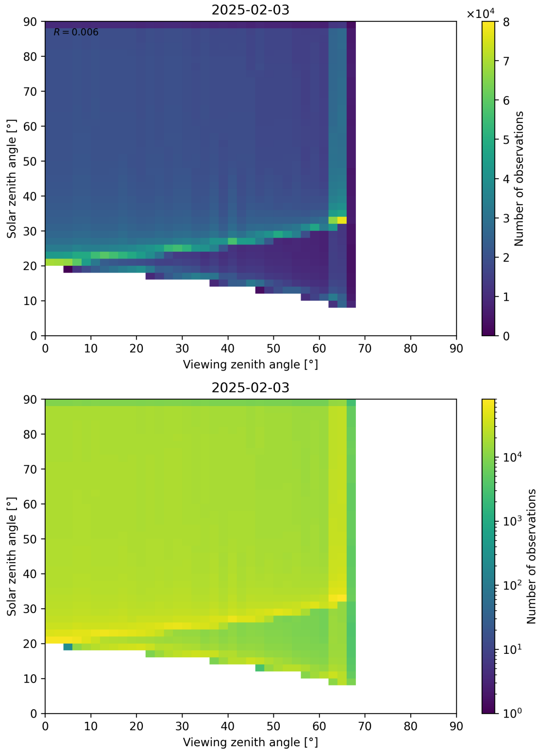
Figure 54: Scatter density plot of “Viewing zenith angle” against “Solar zenith angle” for 2025-02-03 to 2025-02-04.
