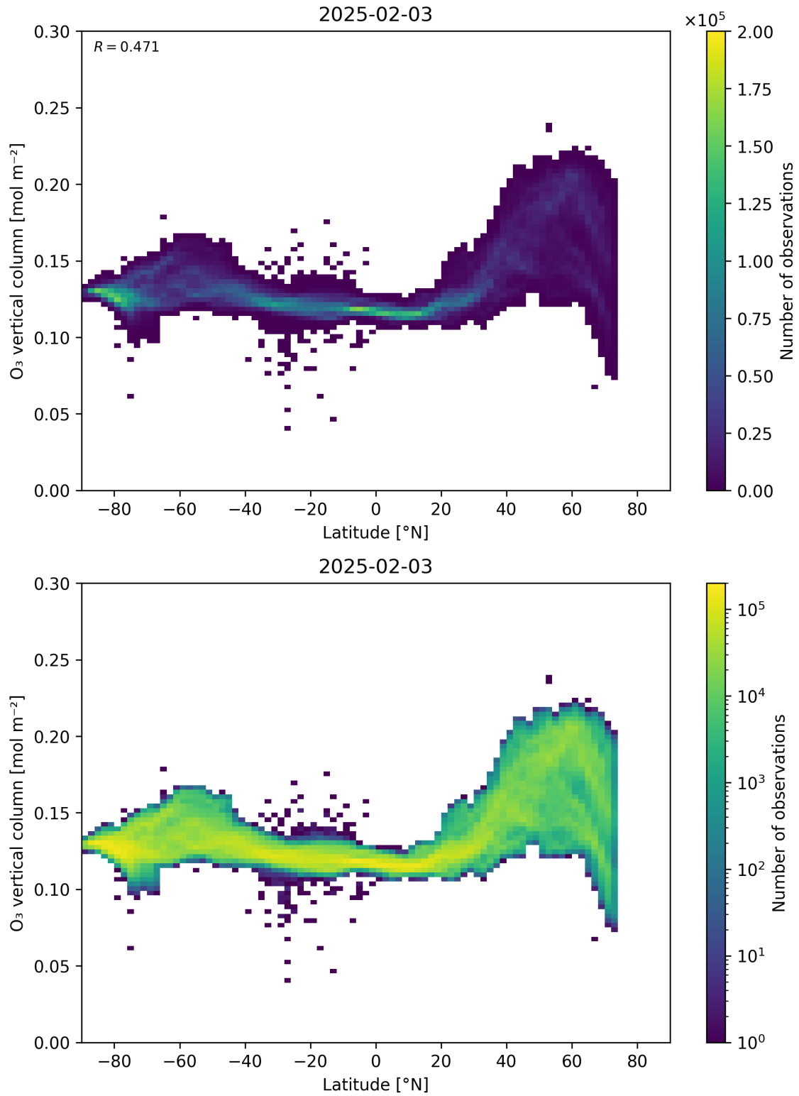
Figure 36: Scatter density plot of “Latitude” against “O 3 vertical column” for 2025-02-03 to 2025-02-04.
