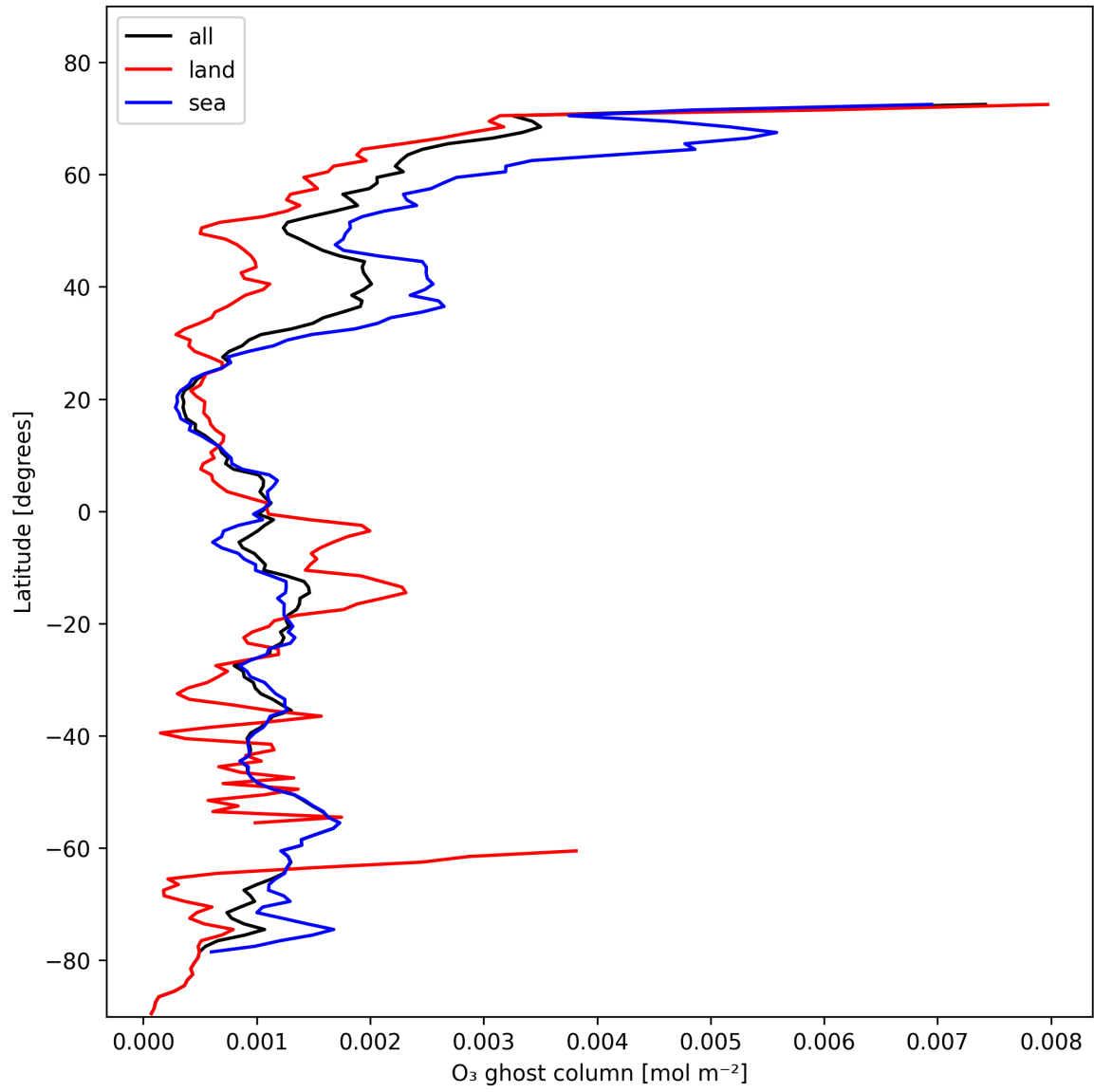
Figure 18: Zonal average of "O 3 ghost column" for 2025-02-03 to 2025-02-04.
