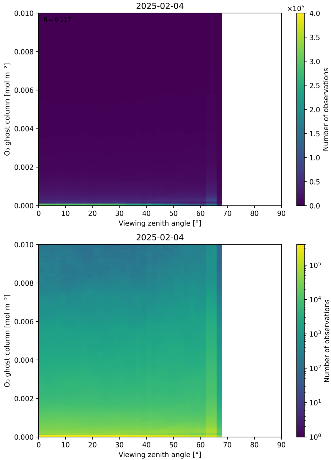
Figure 51: Scatter density plot of “Viewing zenith angle” against “O 3 ghost column” for 2025-02-03 to 2025-02-05.
