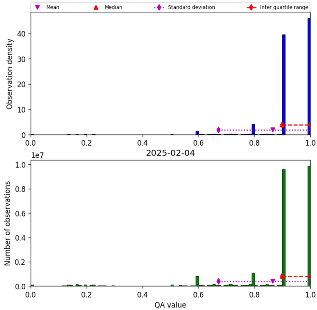
Figure 20: Histogram of “QA value” for 2025-02-03 to 2025-02-05
