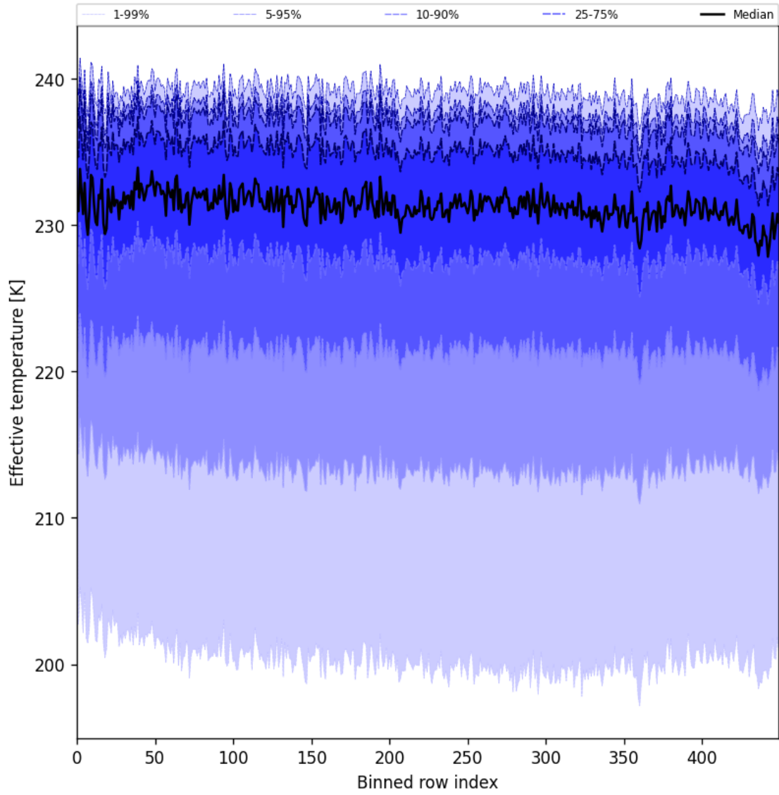
Figure 31: Along track statistics of “Effective temperature” for 2025-02-03 to 2025-02-05
