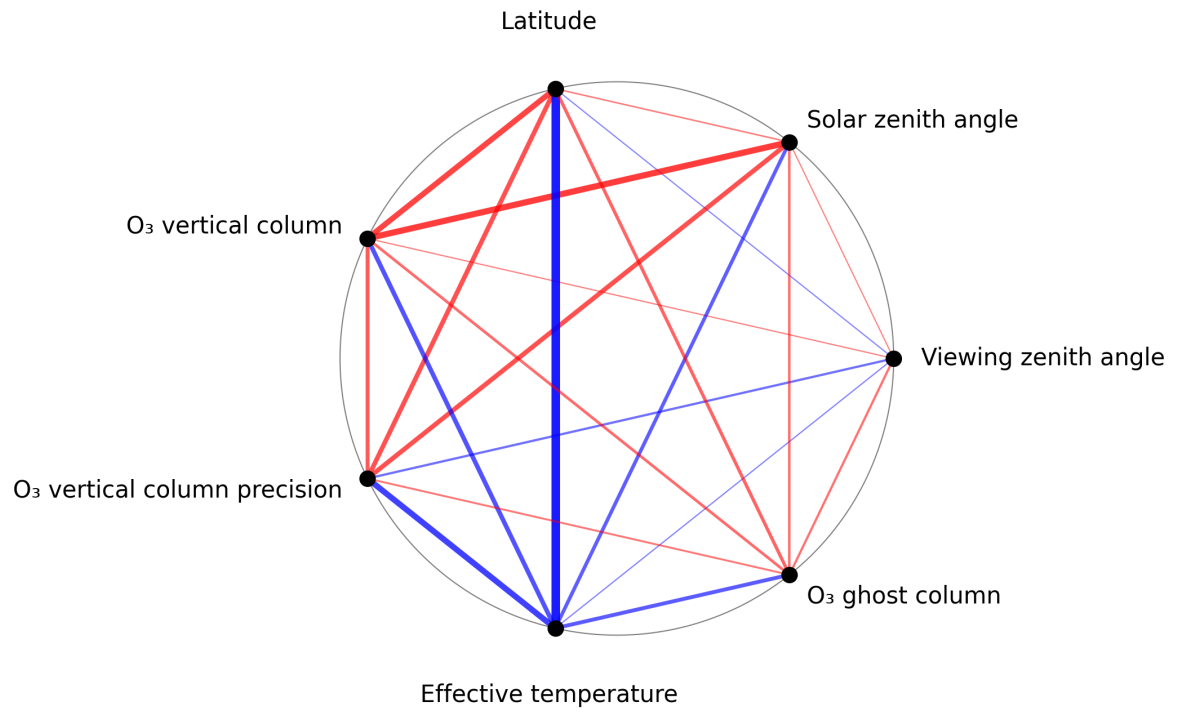
Figure 1: Map of correlation graph for 2025-02-03 to 2025-02-05.
