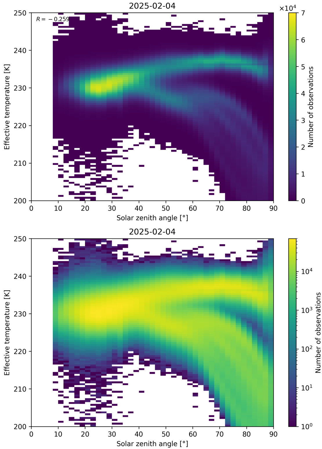
Figure 45: Scatter density plot of “Solar zenith angle” against “Effective temperature” for 2025-02-03 to 2025-02-05.
