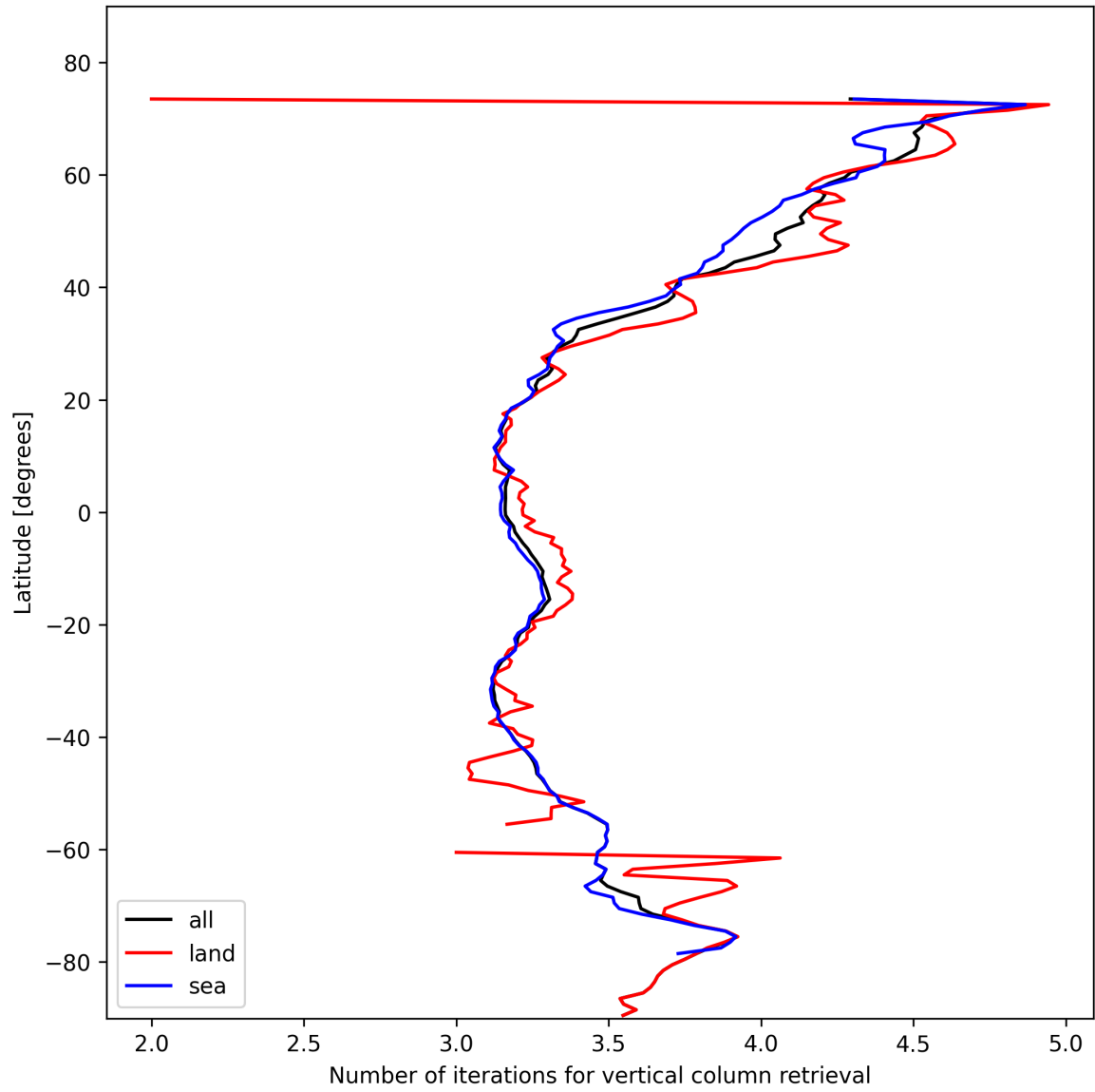
Figure 19: Zonal average of “Number of iterations for vertical column retrieval” for 2025-02-03 to 2025-02-05.
