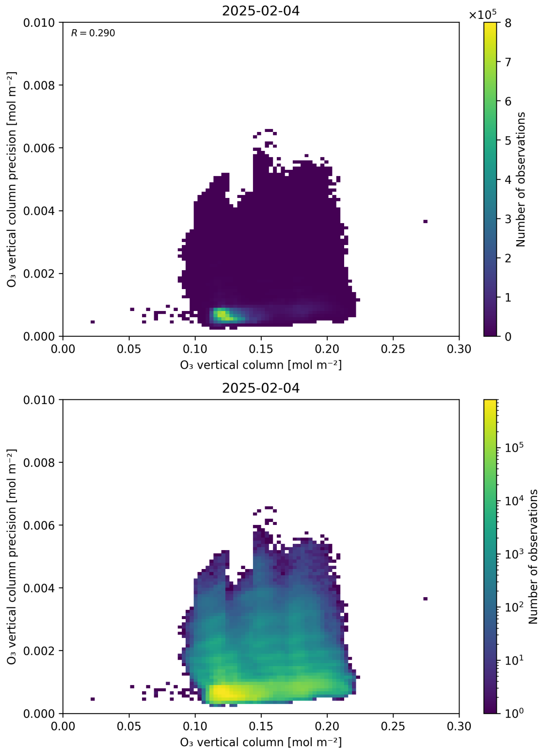
Figure 41: Scatter density plot of “O 3 vertical column” against “O 3 vertical column precision” for 2025-02-03 to 2025-02-05.
