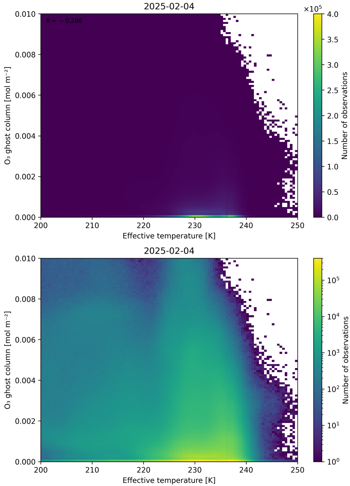
Figure 38: Scatter density plot of “Effective temperature” against “O 3 ghost column” for 2025-02-03 to 2025-02-05.
