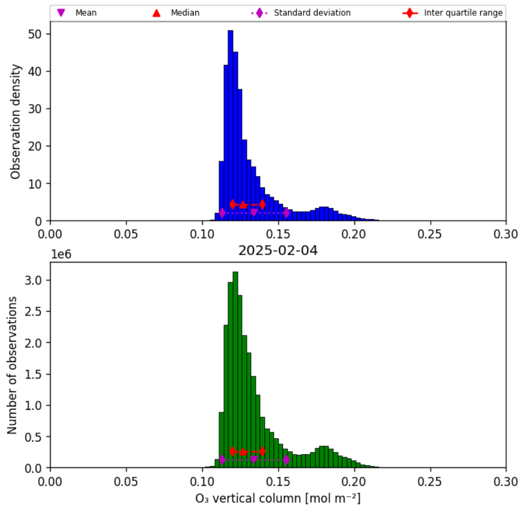
Figure 21: Histogram of “O 3 vertical column” for 2025-02-03 to 2025-02-05
