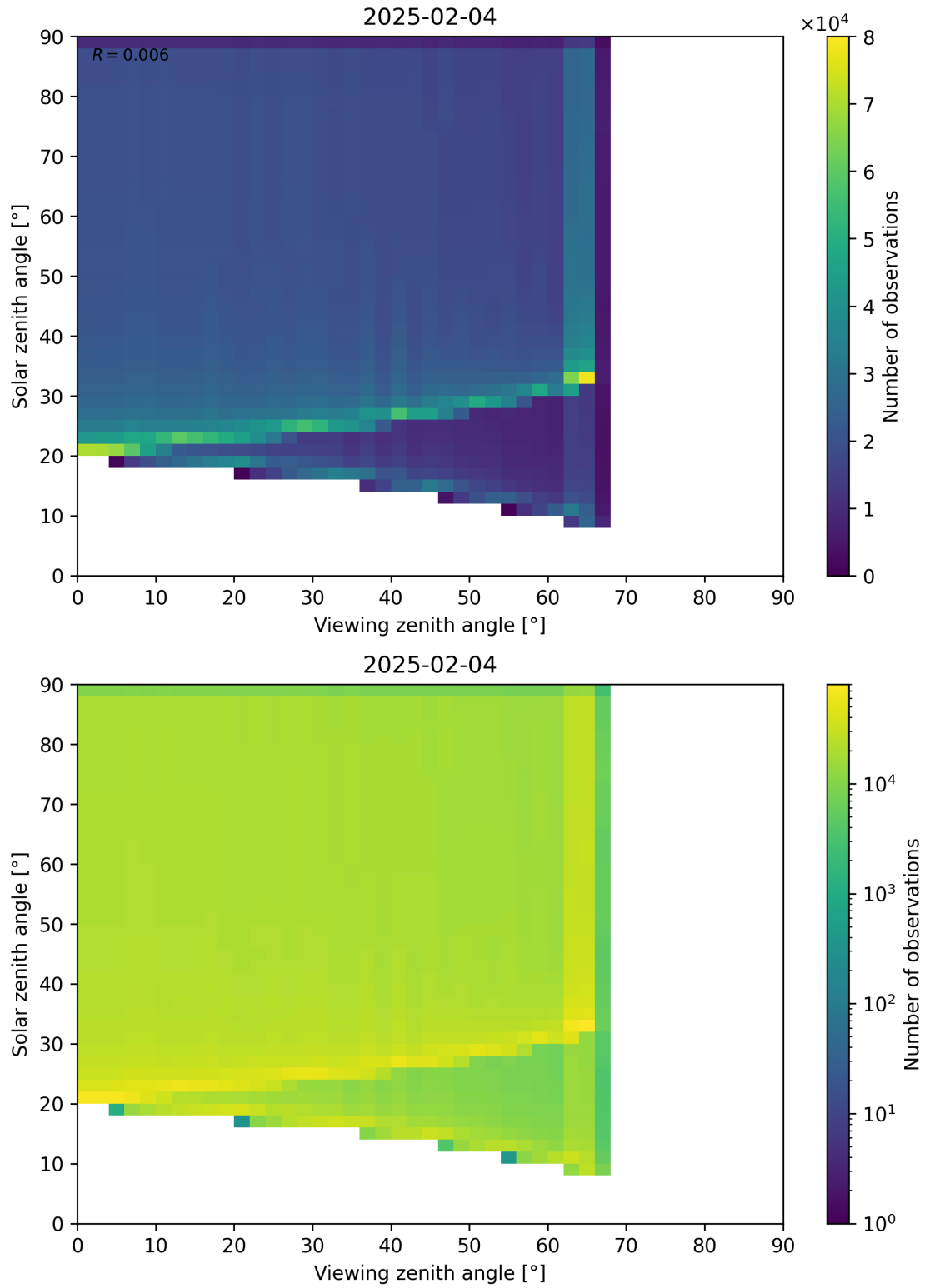
Figure 54: Scatter density plot of “Viewing zenith angle” against “Solar zenith angle” for 2025-02-03 to 2025-02-05.
