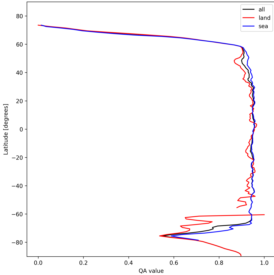
Figure 13: Zonal average of “QA value” for 2025-02-03 to 2025-02-05.
