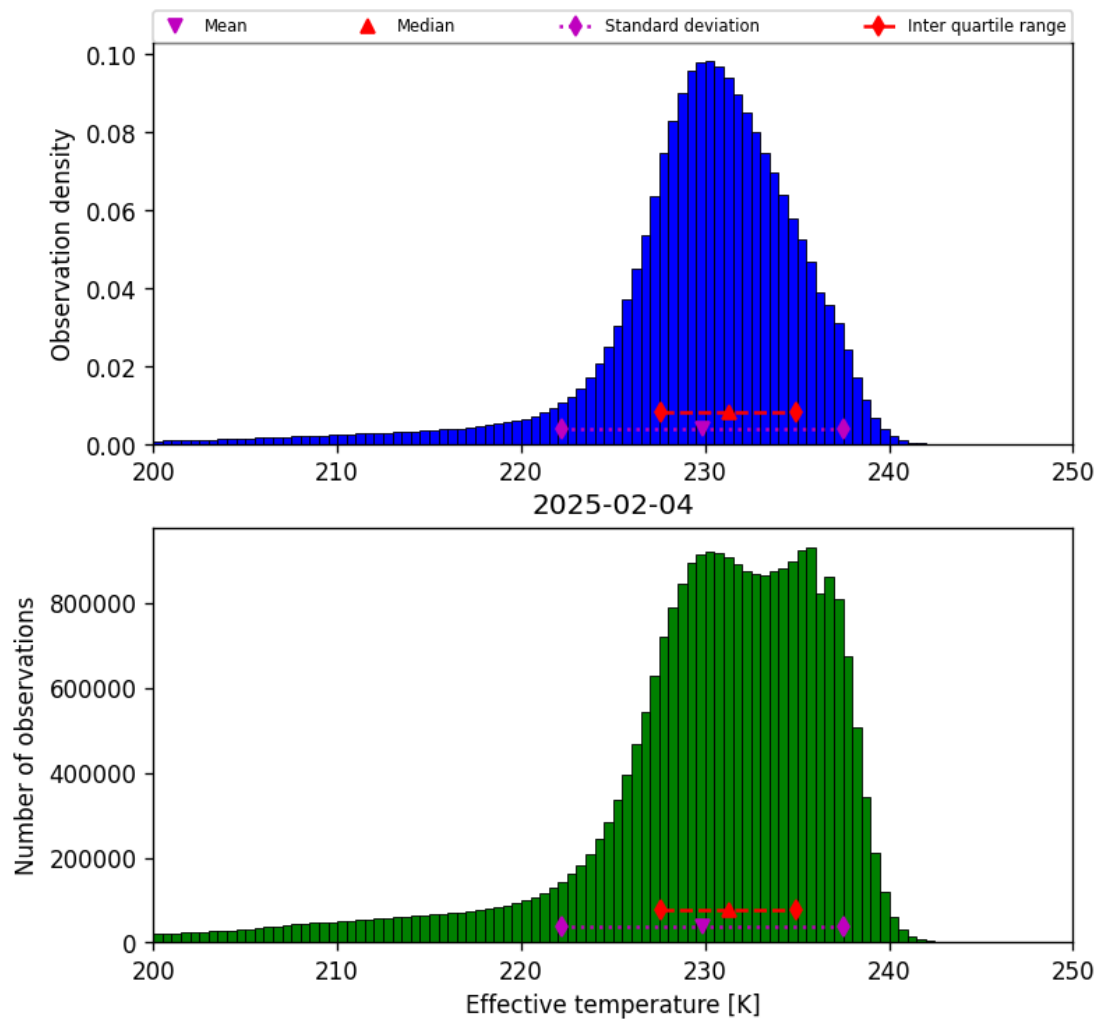
Figure 24: Histogram of “Effective temperature” for 2025-02-03 to 2025-02-05
