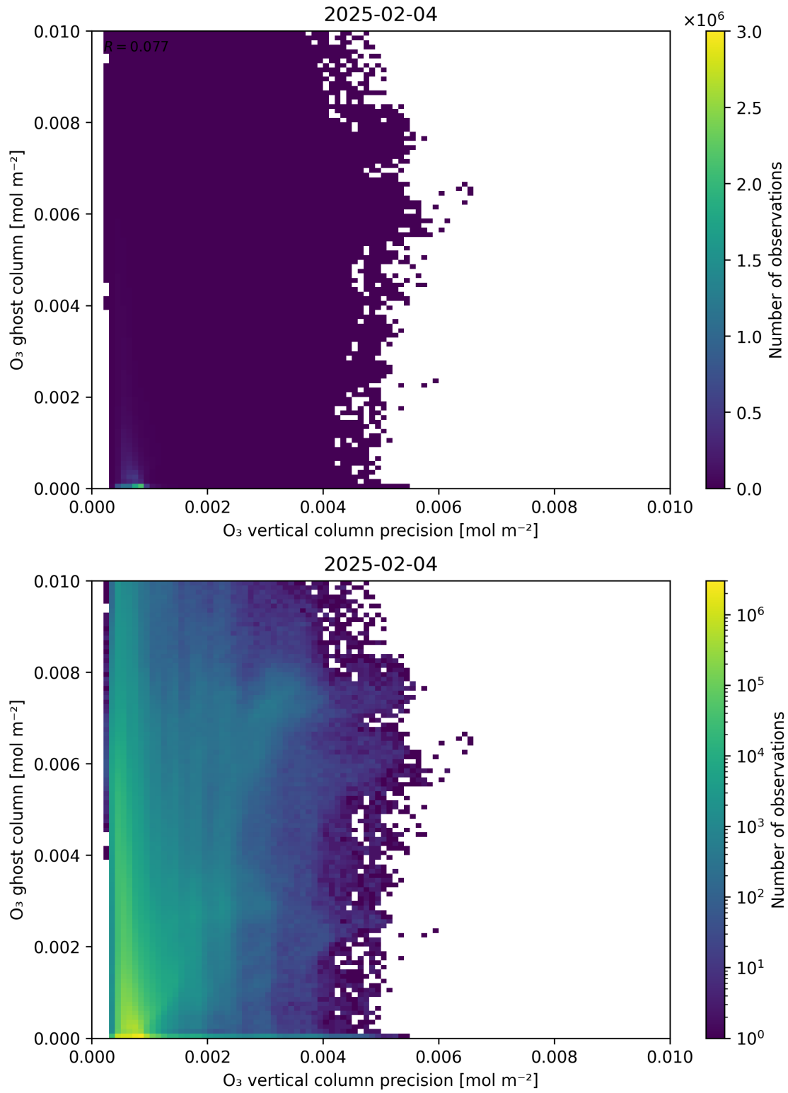
Figure 43: Scatter density plot of “ \text{O}_3 vertical column precision” against “ \text{O}_3 ghost column” for 2025-02-03 to 2025-02-05.
