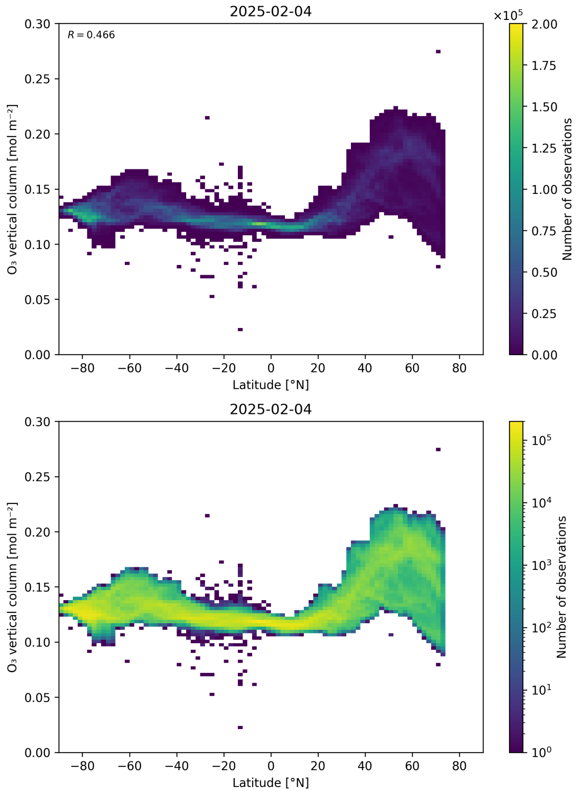
Figure 36: Scatter density plot of “Latitude” against “O 3 vertical column” for 2025-02-03 to 2025-02-05.
