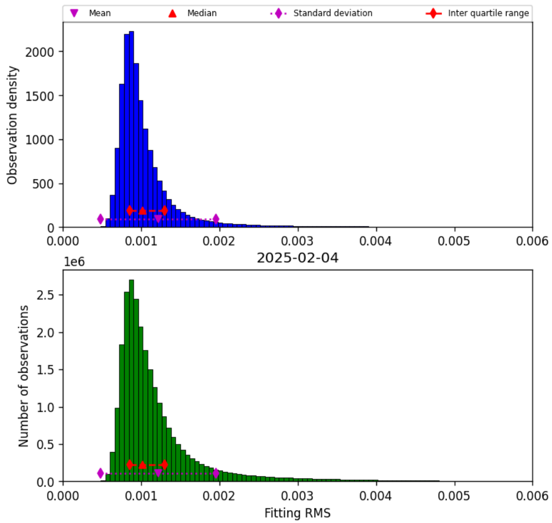
Figure 23: Histogram of “Fitting RMS” for 2025-02-03 to 2025-02-05
