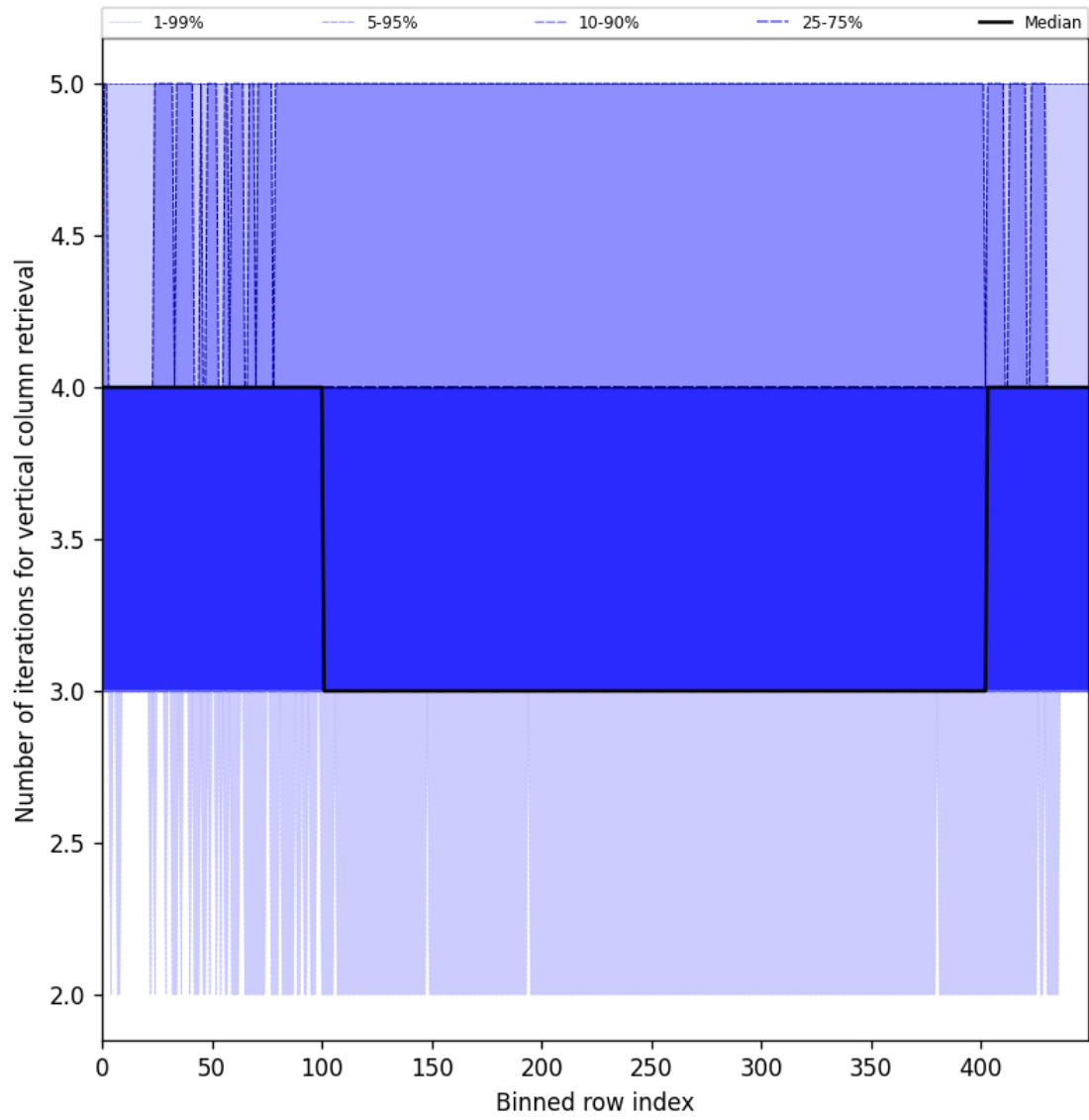
Figure 33: Along track statistics of “Number of iterations for vertical column retrieval” for 2025-02-03 to 2025-02-05
