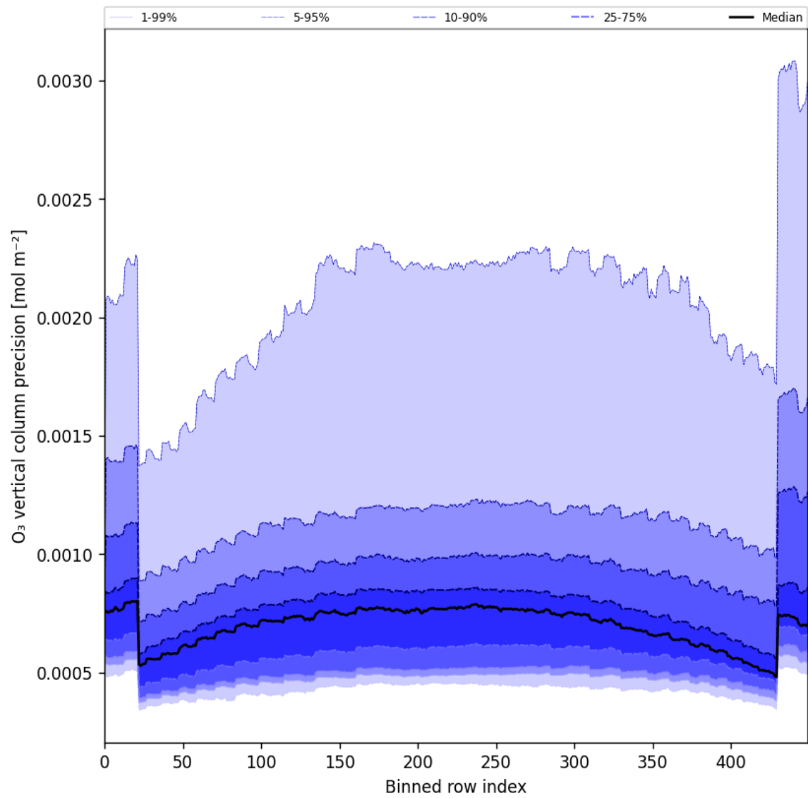
Figure 29: Along track statistics of “O 3 vertical column precision” for 2025-02-03 to 2025-02-05
