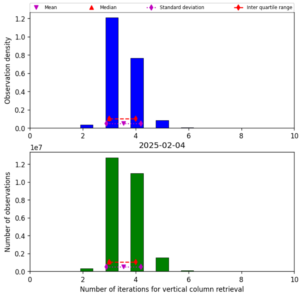
Figure 26: Histogram of “Number of iterations for vertical column retrieval” for 2025-02-03 to 2025-02-05
