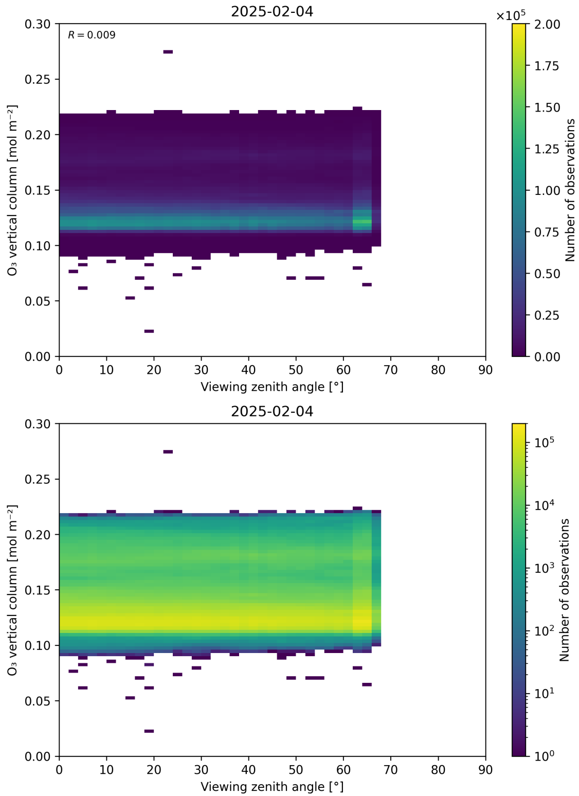
Figure 52: Scatter density plot of “Viewing zenith angle” against “O 3 vertical column” for 2025-02-03 to 2025-02-05.
