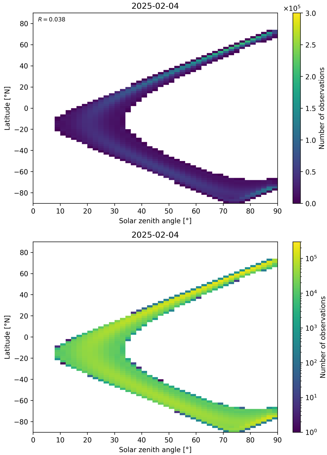
Figure 44: Scatter density plot of “Solar zenith angle” against “Latitude” for 2025-02-03 to 2025-02-05.
