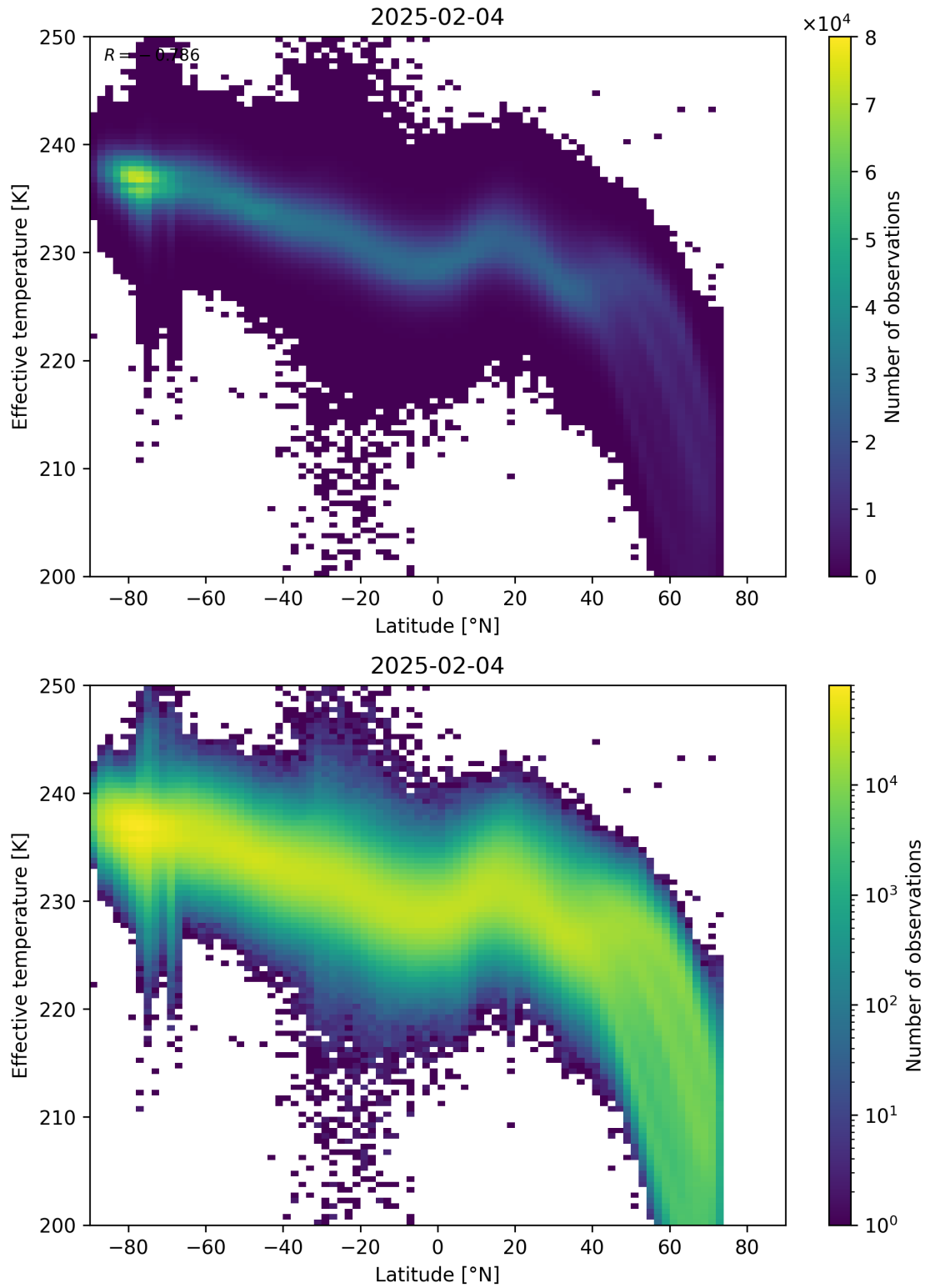
Figure 34: Scatter density plot of “Latitude” against “Effective temperature” for 2025-02-03 to 2025-02-05.
