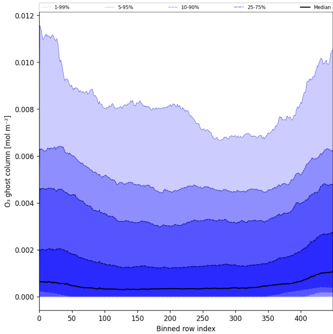
Figure 32: Along track statistics of “O 3 ghost column” for 2025-02-03 to 2025-02-05
