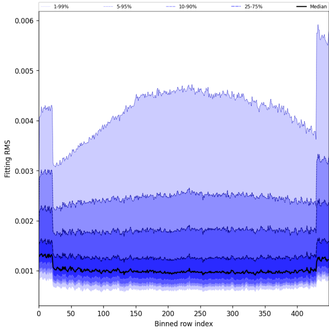
Figure 30: Along track statistics of “Fitting RMS” for 2025-02-03 to 2025-02-05
