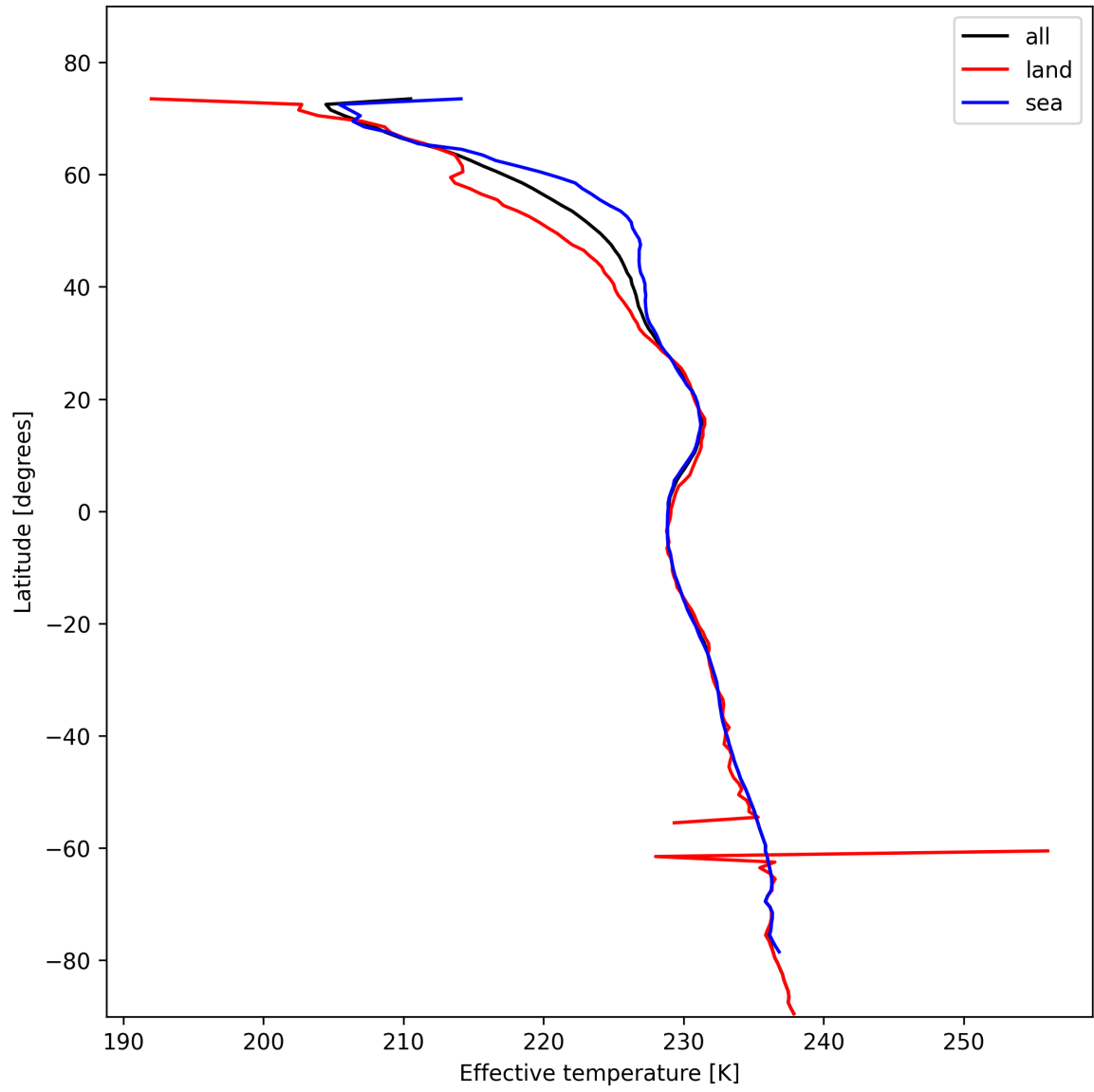
Figure 17: Zonal average of "Effective temperature" for 2025-02-03 to 2025-02-05.
