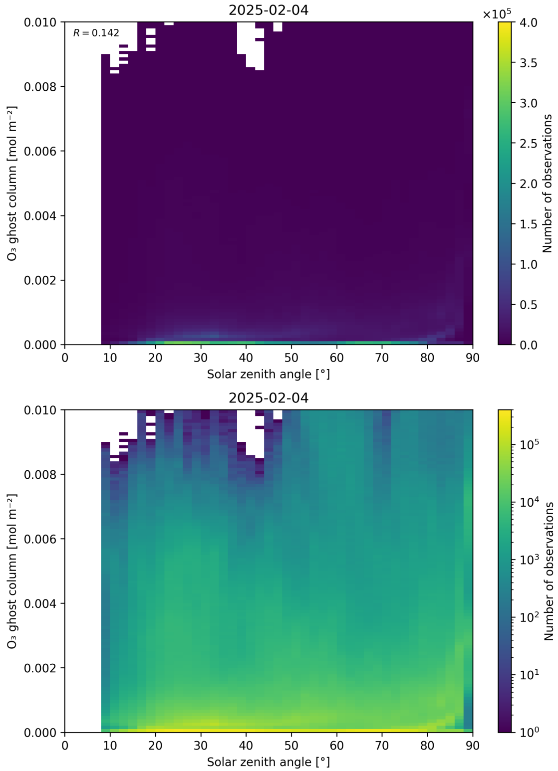
Figure 46: Scatter density plot of “Solar zenith angle” against “O 3 ghost column” for 2025-02-03 to 2025-02-05.
