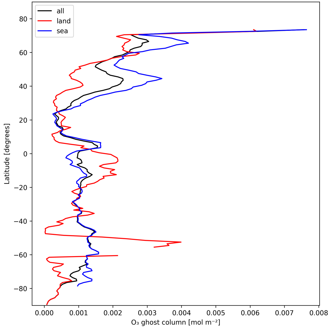
Figure 18: Zonal average of “O 3 ghost column” for 2025-02-03 to 2025-02-05.
