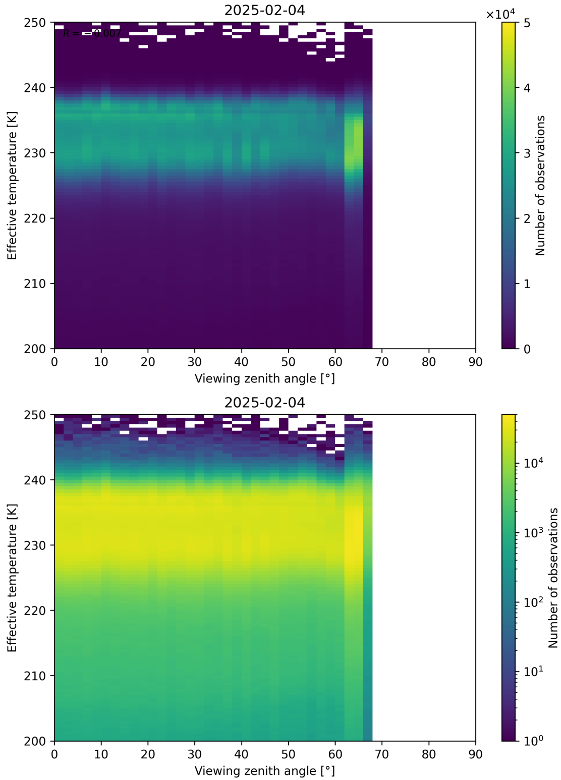
Figure 50: Scatter density plot of “Viewing zenith angle” against “Effective temperature” for 2025-02-03 to 2025-02-05.
