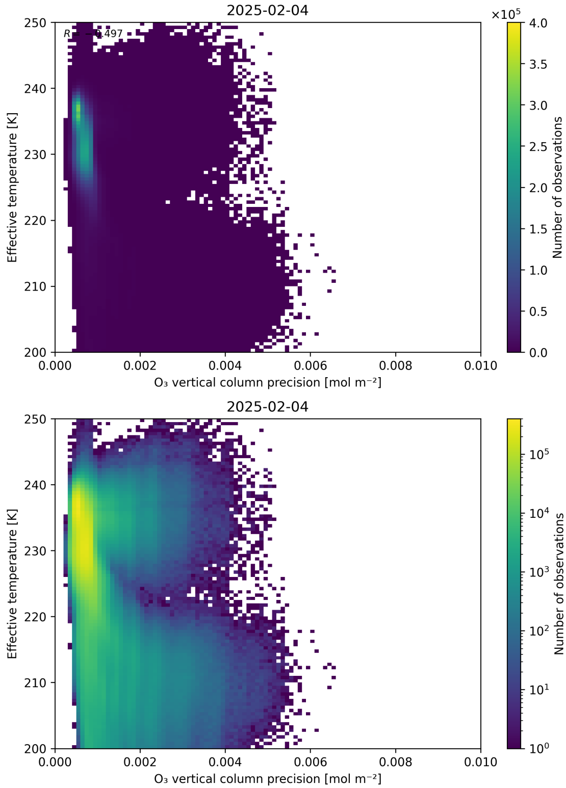
Figure 42: Scatter density plot of “O 3 vertical column precision” against “Effective temperature” for 2025-02-03 to 2025-02-05.
