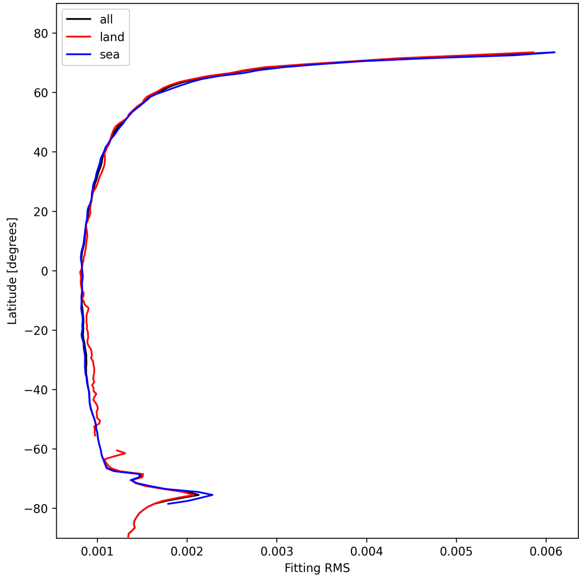
Figure 16: Zonal average of “Fitting RMS” for 2025-02-03 to 2025-02-05.
