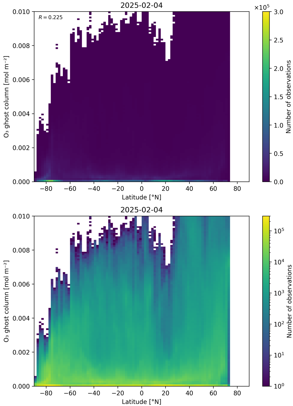
Figure 35: Scatter density plot of “Latitude” against “O 3 ghost column” for 2025-02-03 to 2025-02-05.
