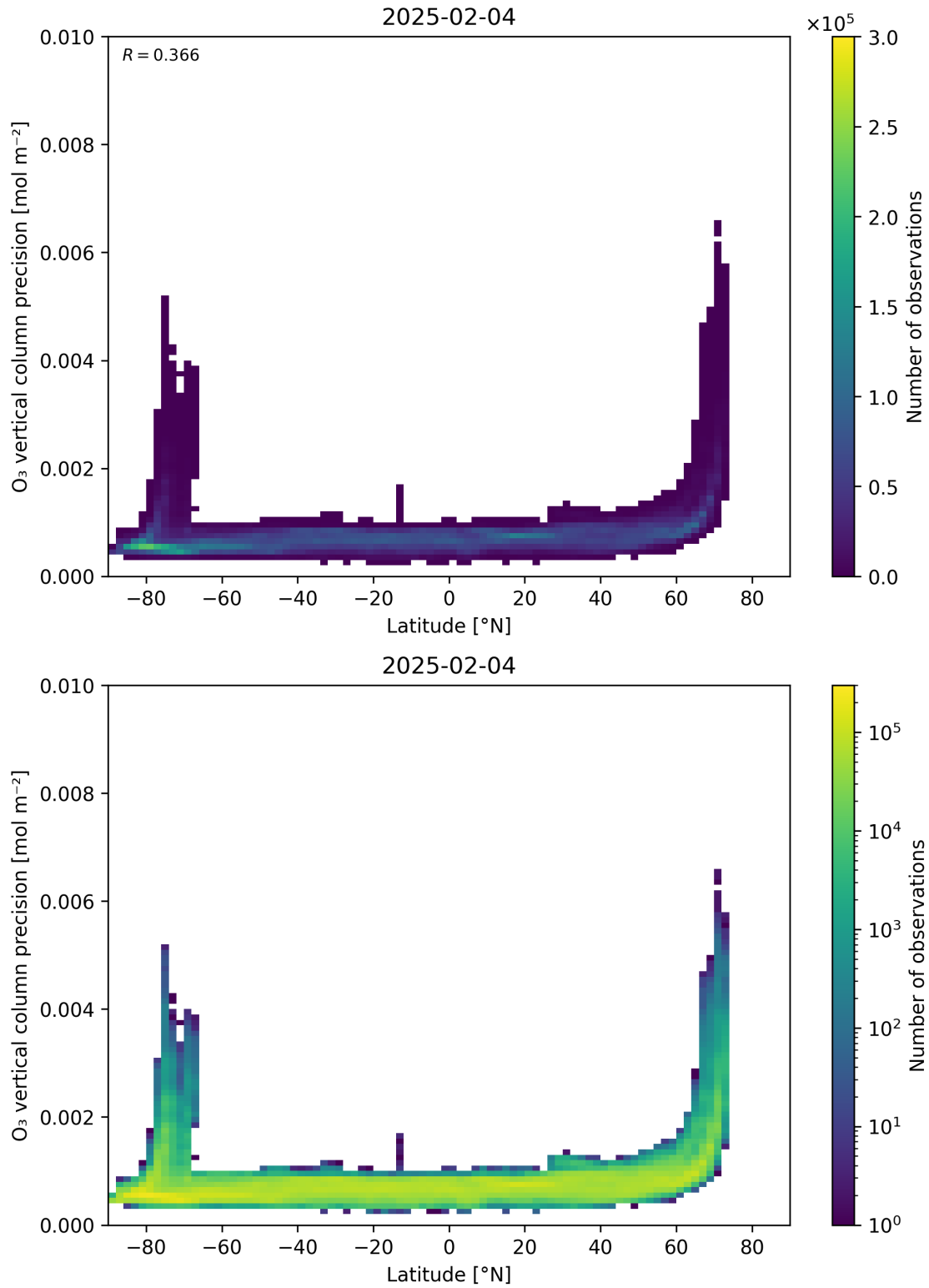
Figure 37: Scatter density plot of “Latitude” against “O 3 vertical column precision” for 2025-02-03 to 2025-02-05.
