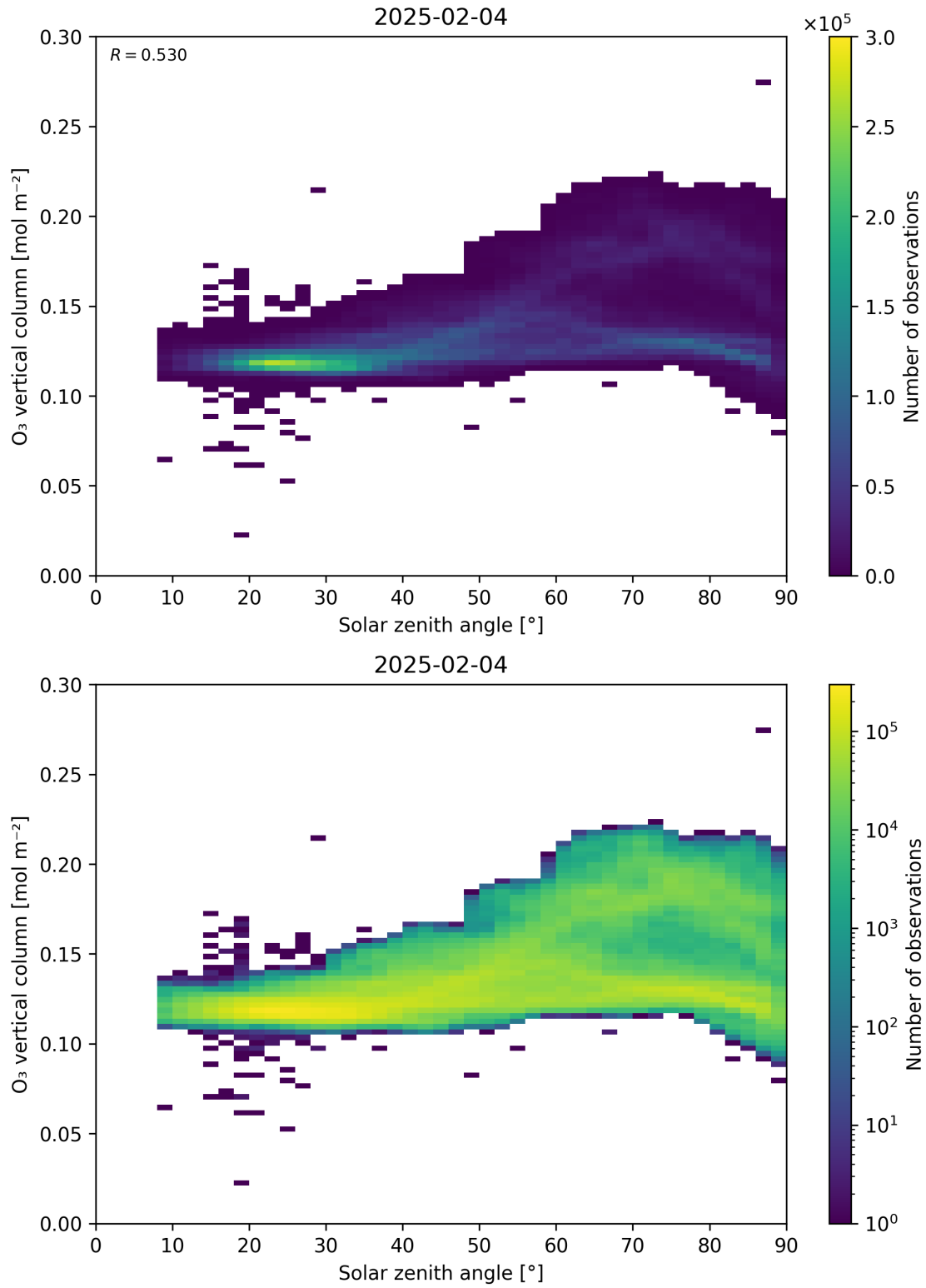
Figure 47: Scatter density plot of “Solar zenith angle” against “O 3 vertical column” for 2025-02-03 to 2025-02-05.
