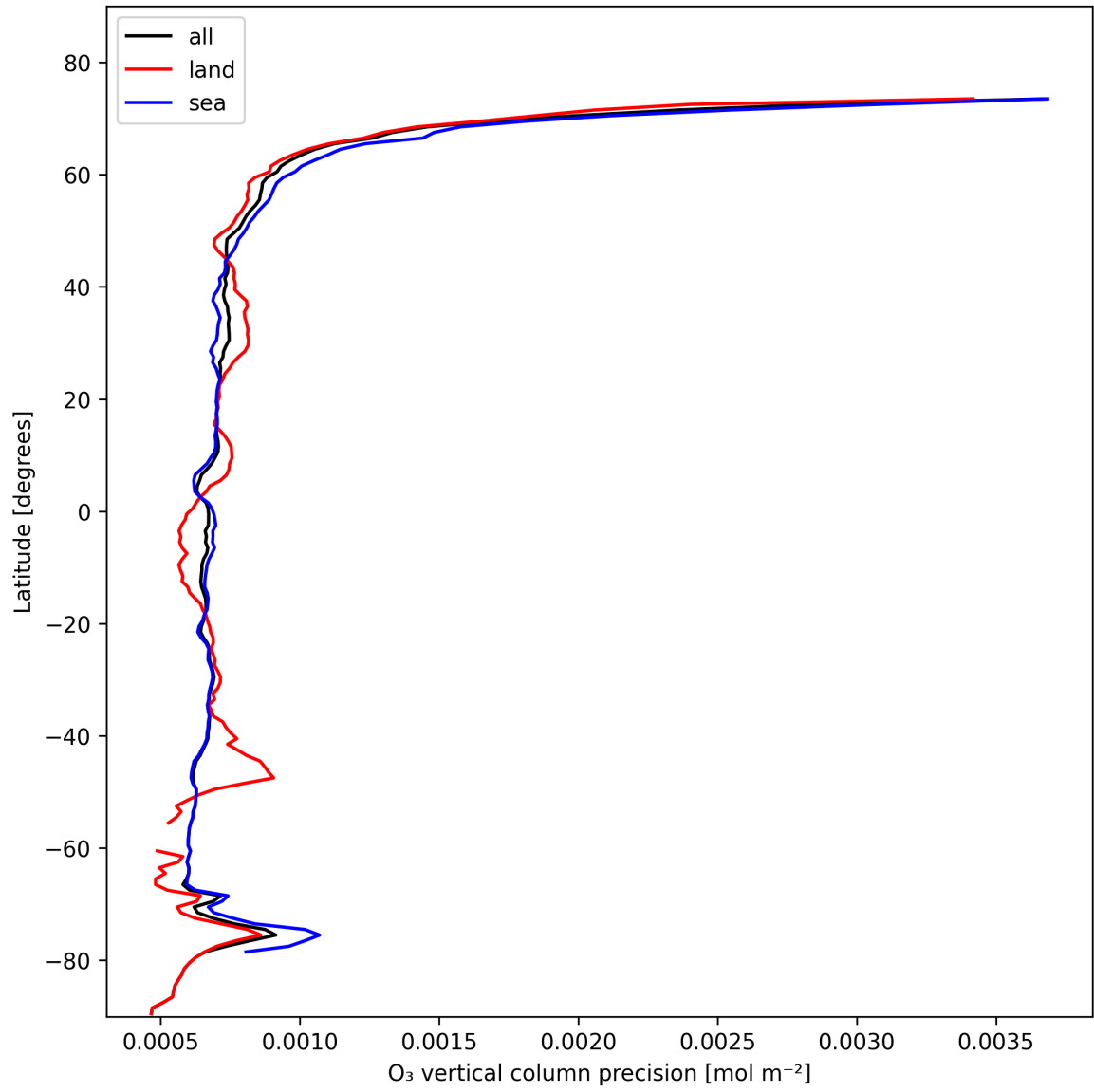
Figure 15: Zonal average of “O 3 vertical column precision” for 2025-02-03 to 2025-02-05.
