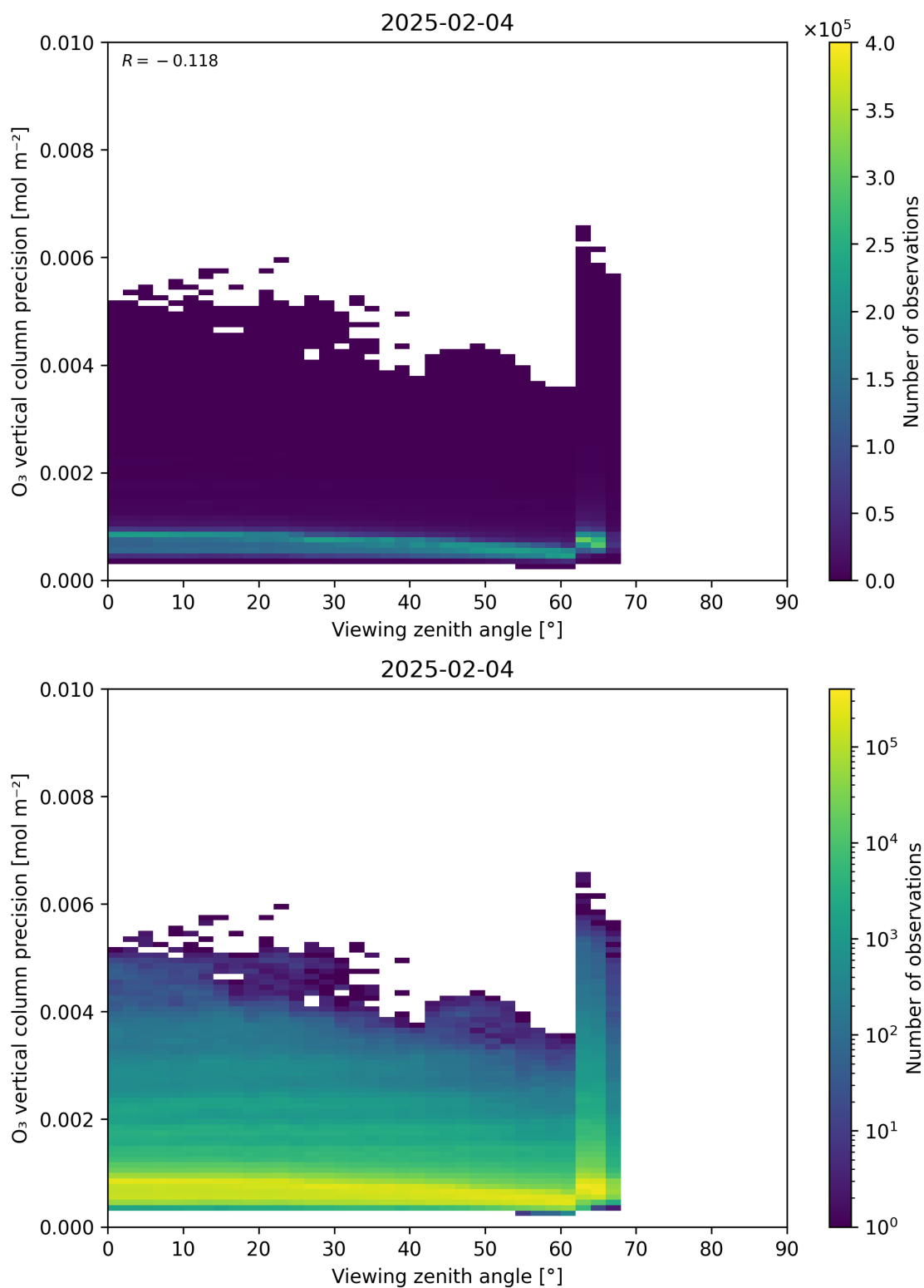
Figure 53: Scatter density plot of “Viewing zenith angle” against “O 3 vertical column precision” for 2025-02-03 to 2025-02-05.
