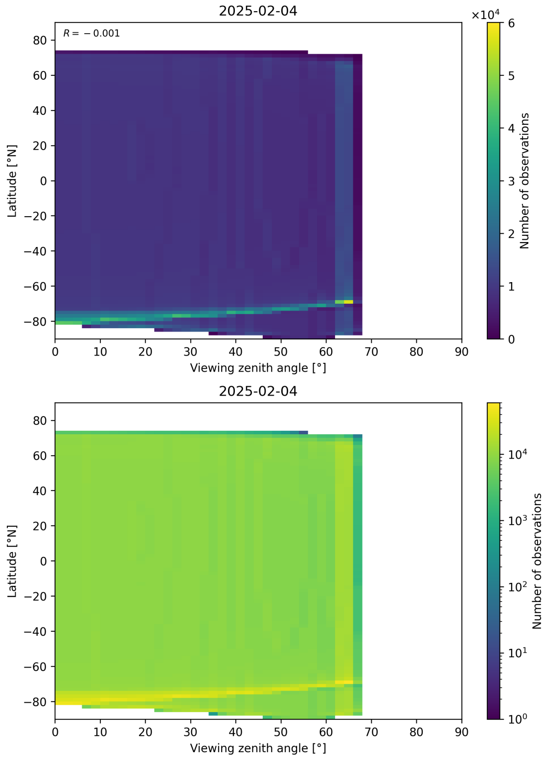
Figure 49: Scatter density plot of “Viewing zenith angle” against “Latitude” for 2025-02-03 to 2025-02-05.
