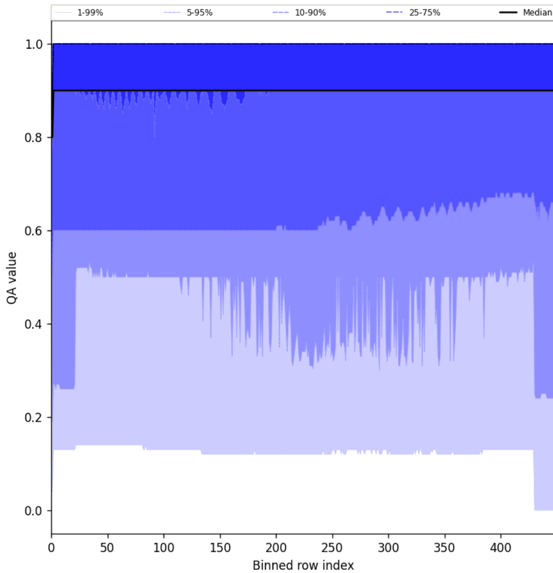
Figure 27: Along track statistics of “QA value” for 2025-02-03 to 2025-02-05
