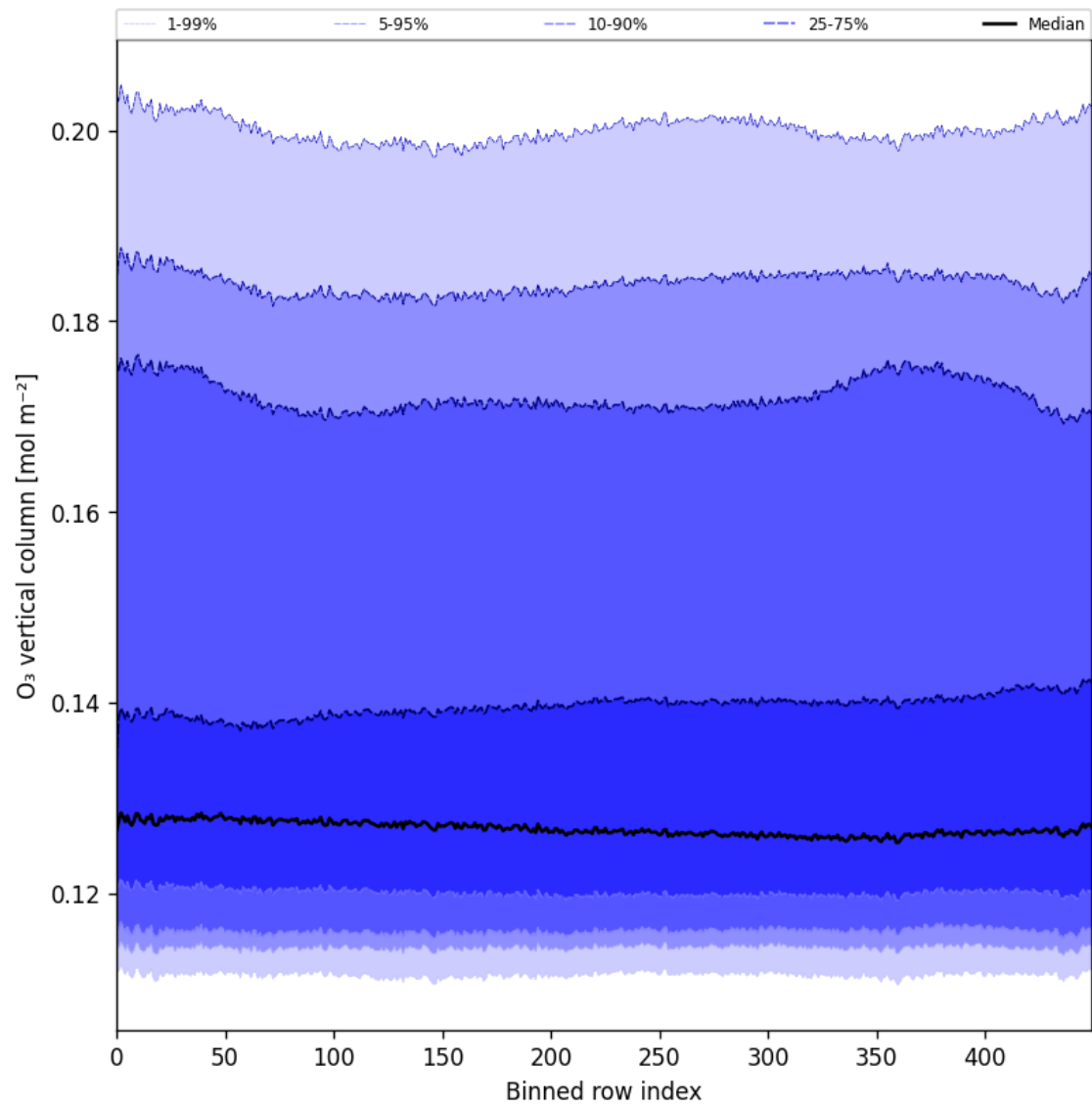
Figure 28: Along track statistics of “O 3 vertical column” for 2025-02-03 to 2025-02-05
