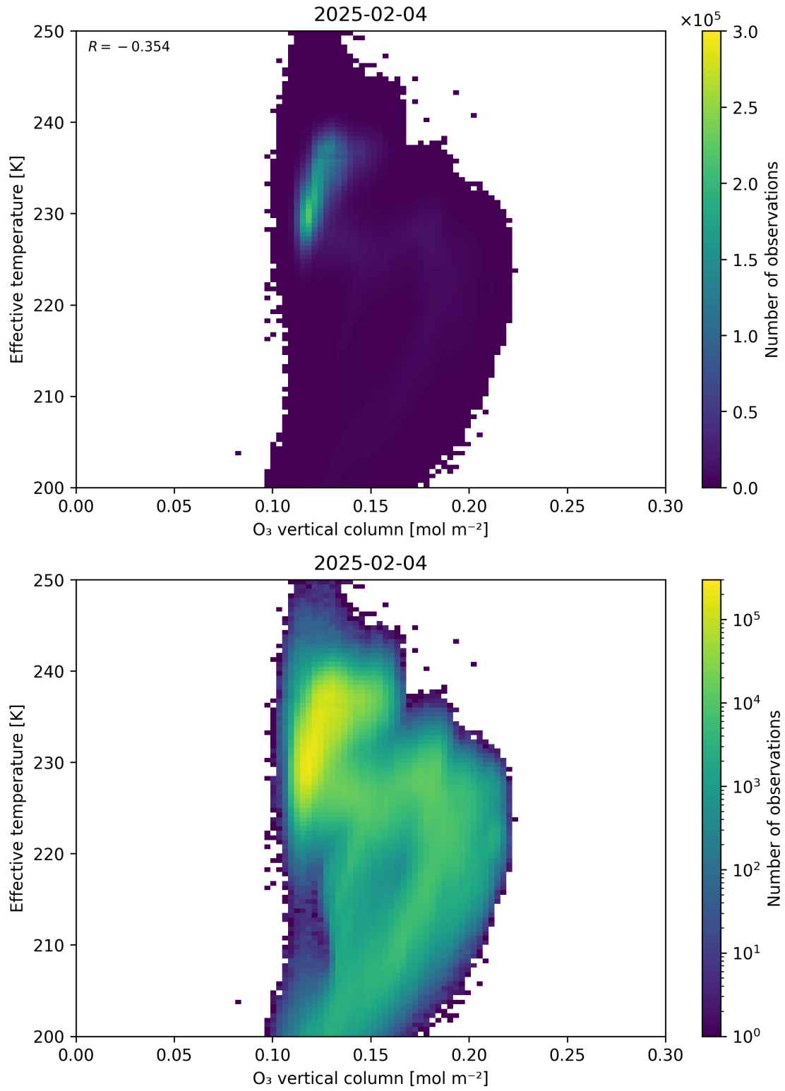
Figure 39: Scatter density plot of “O 3 vertical column” against “Effective temperature” for 2025-02-03 to 2025-02-05.
