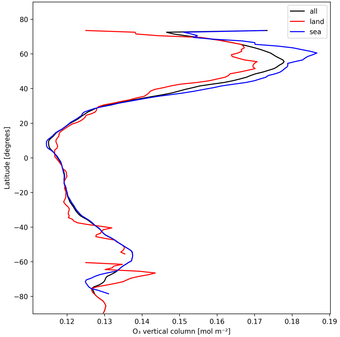
Figure 14: Zonal average of “O 3 vertical column” for 2025-02-03 to 2025-02-05.
