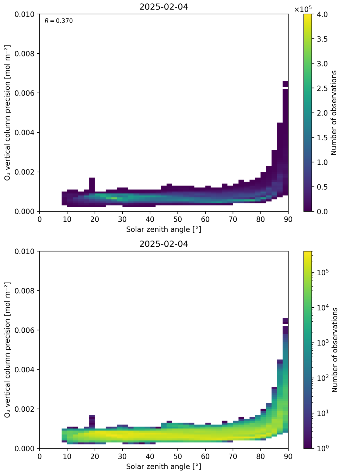
Figure 48: Scatter density plot of “Solar zenith angle” against “O 3 vertical column precision” for 2025-02-03 to 2025-02-05.
