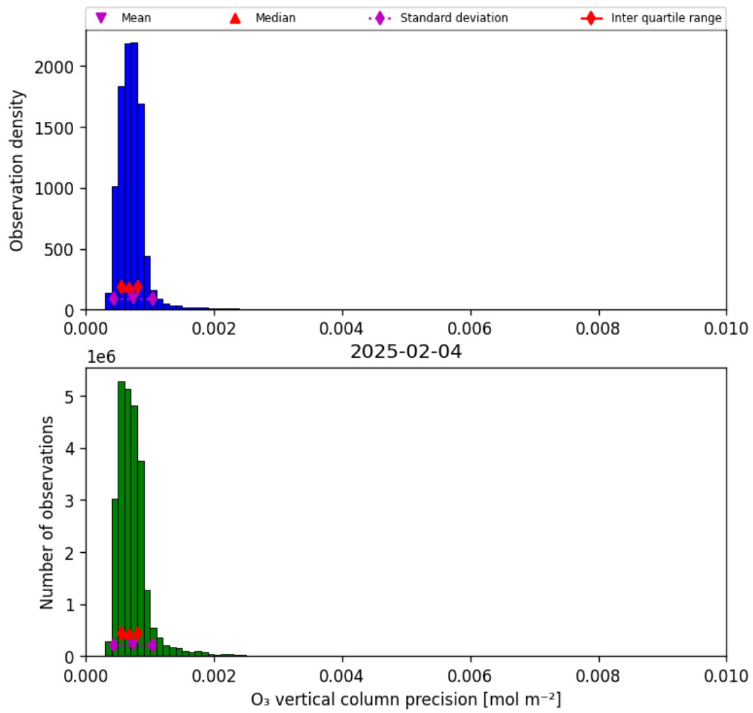
Figure 22: Histogram of “O 3 vertical column precision” for 2025-02-03 to 2025-02-05
