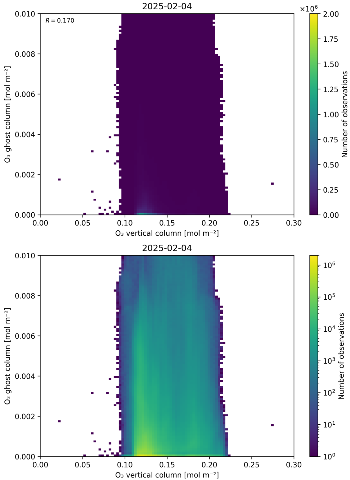
Figure 40: Scatter density plot of “O 3 vertical column” against “O 3 ghost column” for 2025-02-03 to 2025-02-05.
