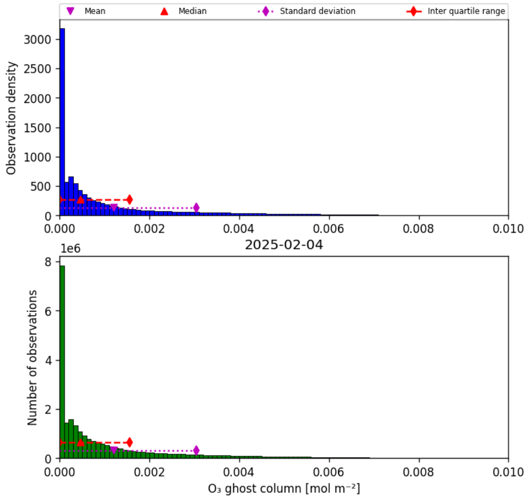
Figure 25: Histogram of “O 3 ghost column” for 2025-02-03 to 2025-02-05
