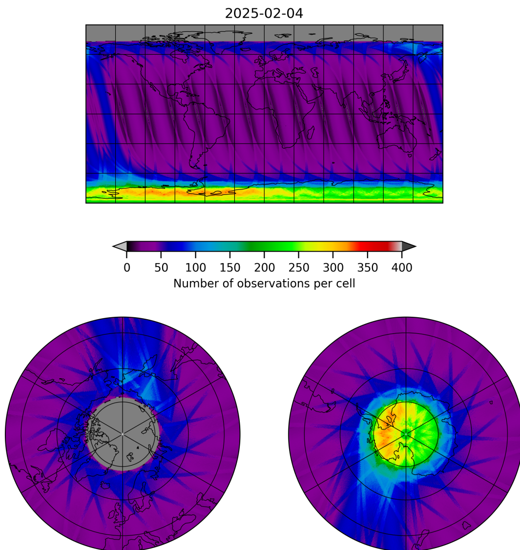
Figure 12: Map of the number of observations for 2025-02-03 to 2025-02-05
