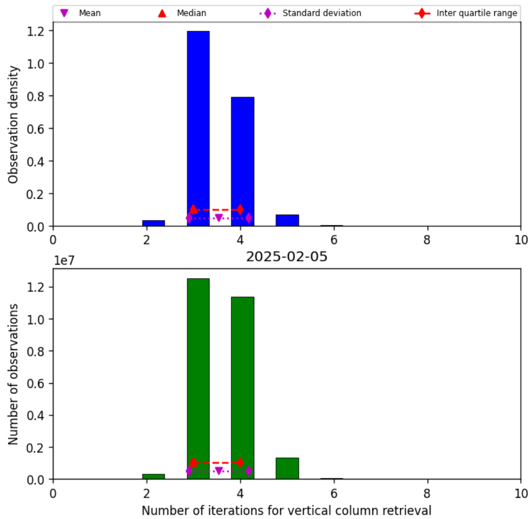
Figure 26: Histogram of “Number of iterations for vertical column retrieval” for 2025-02-04 to 2025-02-06
