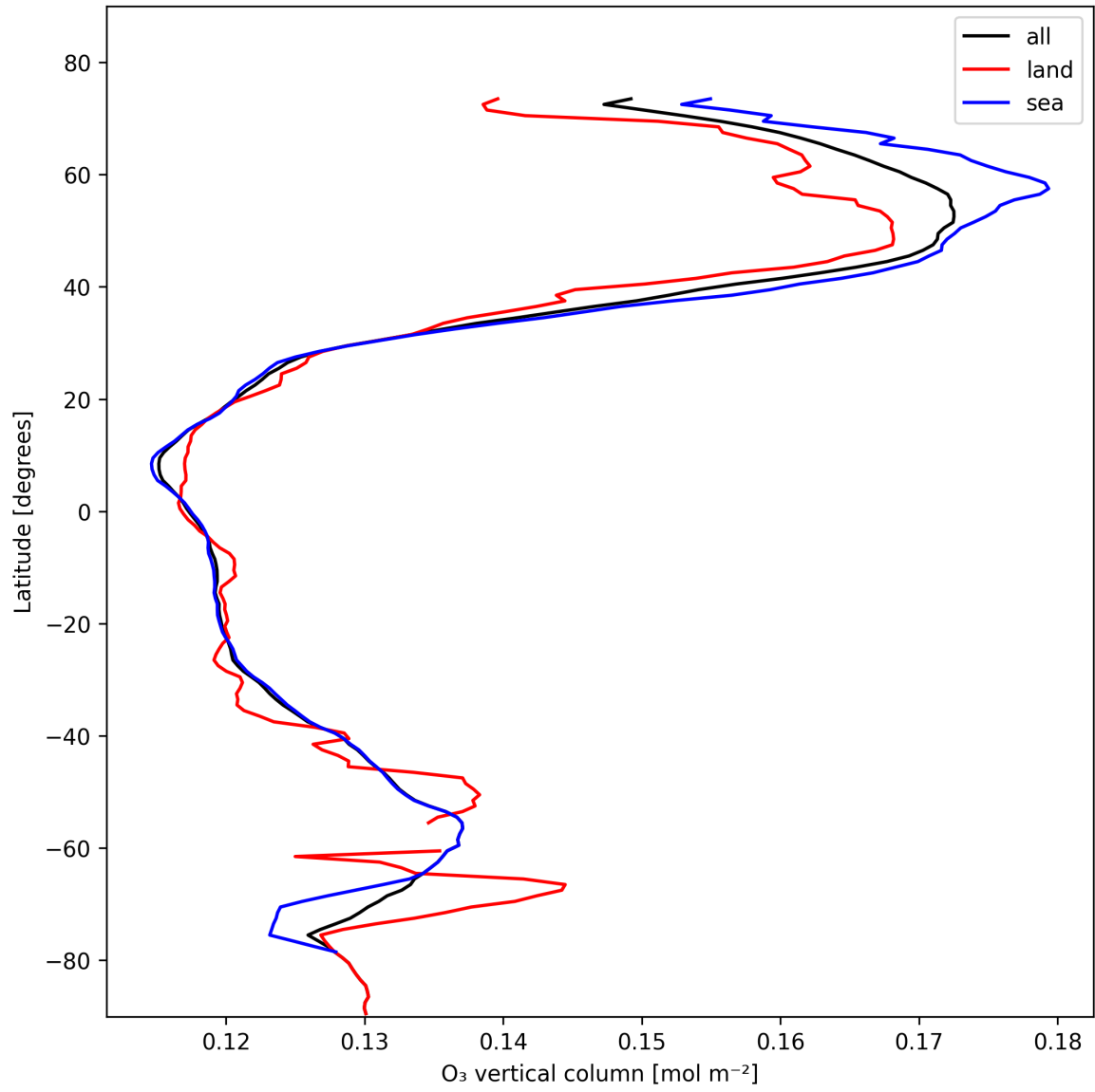
Figure 14: Zonal average of “O 3 vertical column” for 2025-02-04 to 2025-02-06.
