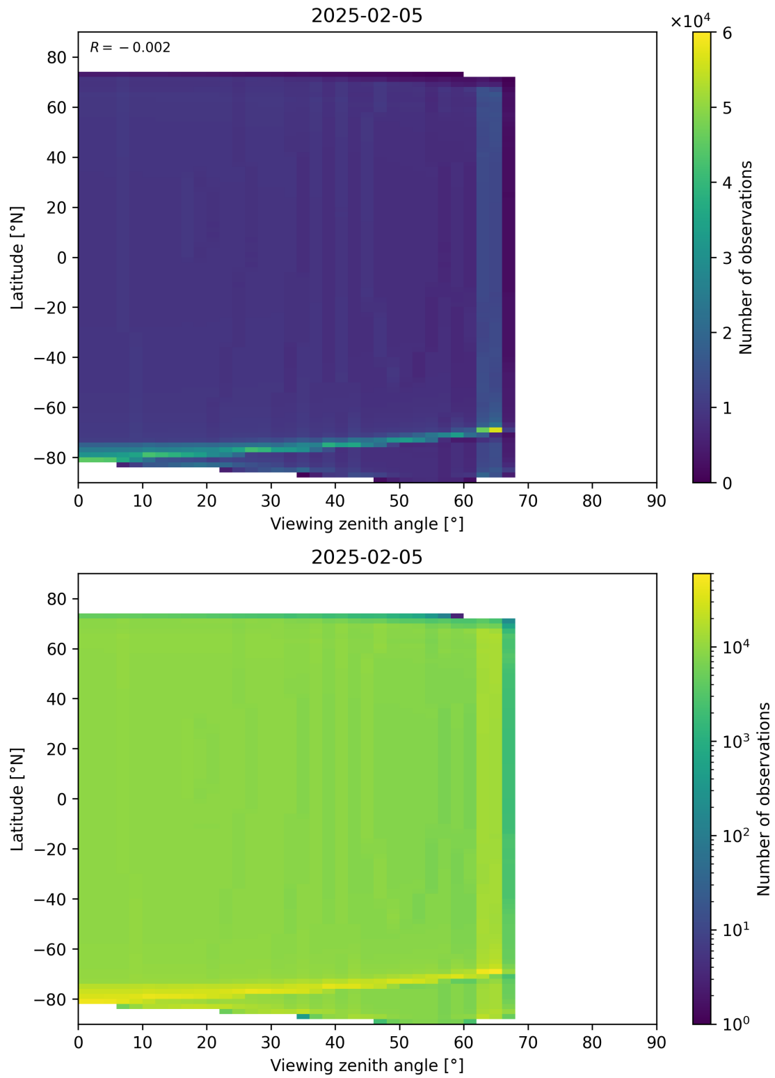
Figure 49: Scatter density plot of “Viewing zenith angle” against “Latitude” for 2025-02-04 to 2025-02-06.
