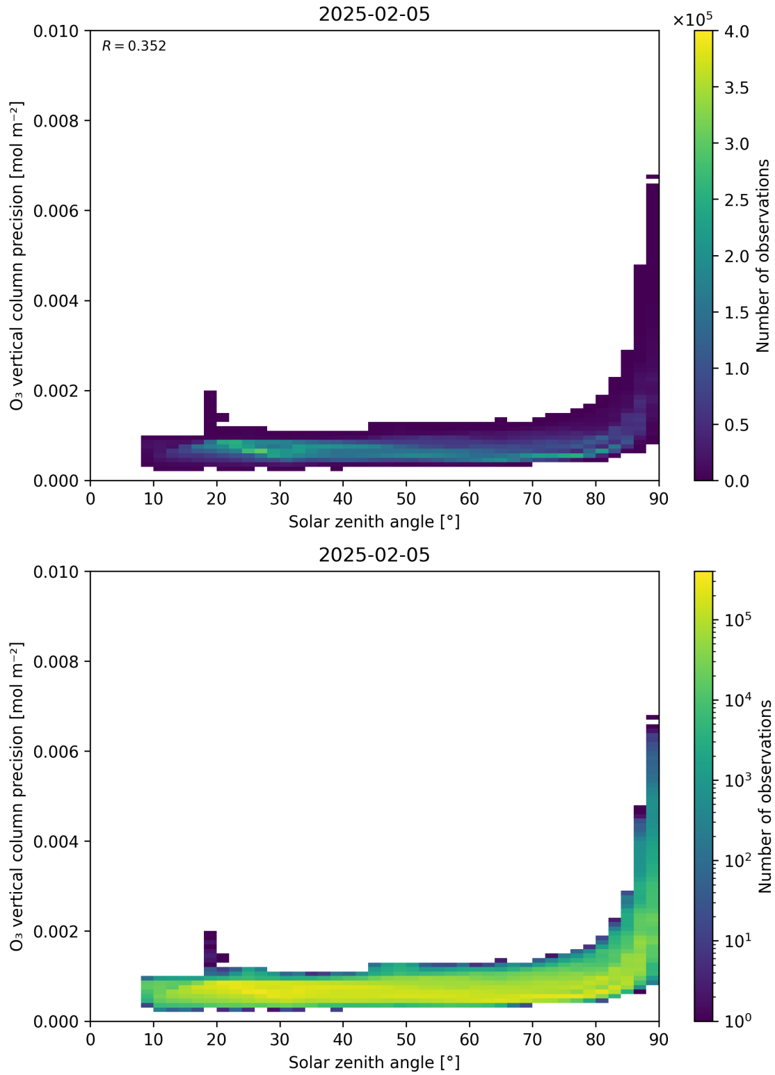
Figure 48: Scatter density plot of “Solar zenith angle” against “O 3 vertical column precision” for 2025-02-04 to 2025-02-06.
