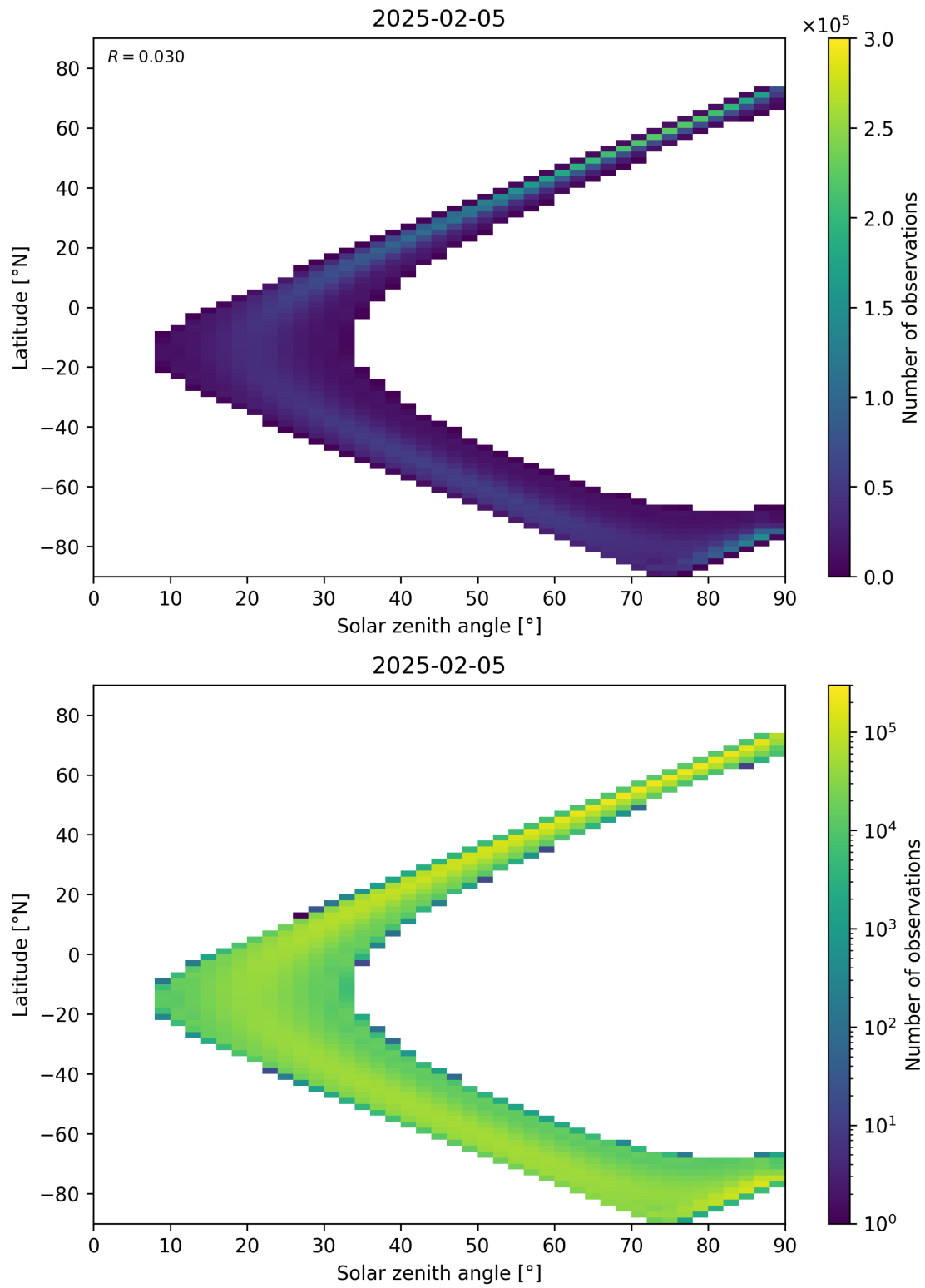
Figure 44: Scatter density plot of “Solar zenith angle” against “Latitude” for 2025-02-04 to 2025-02-06.
