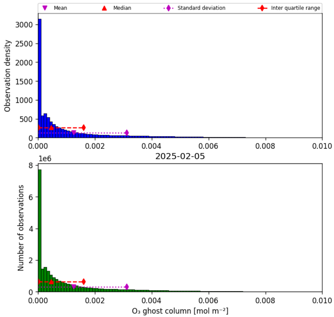
Figure 25: Histogram of “O 3 ghost column” for 2025-02-04 to 2025-02-06
