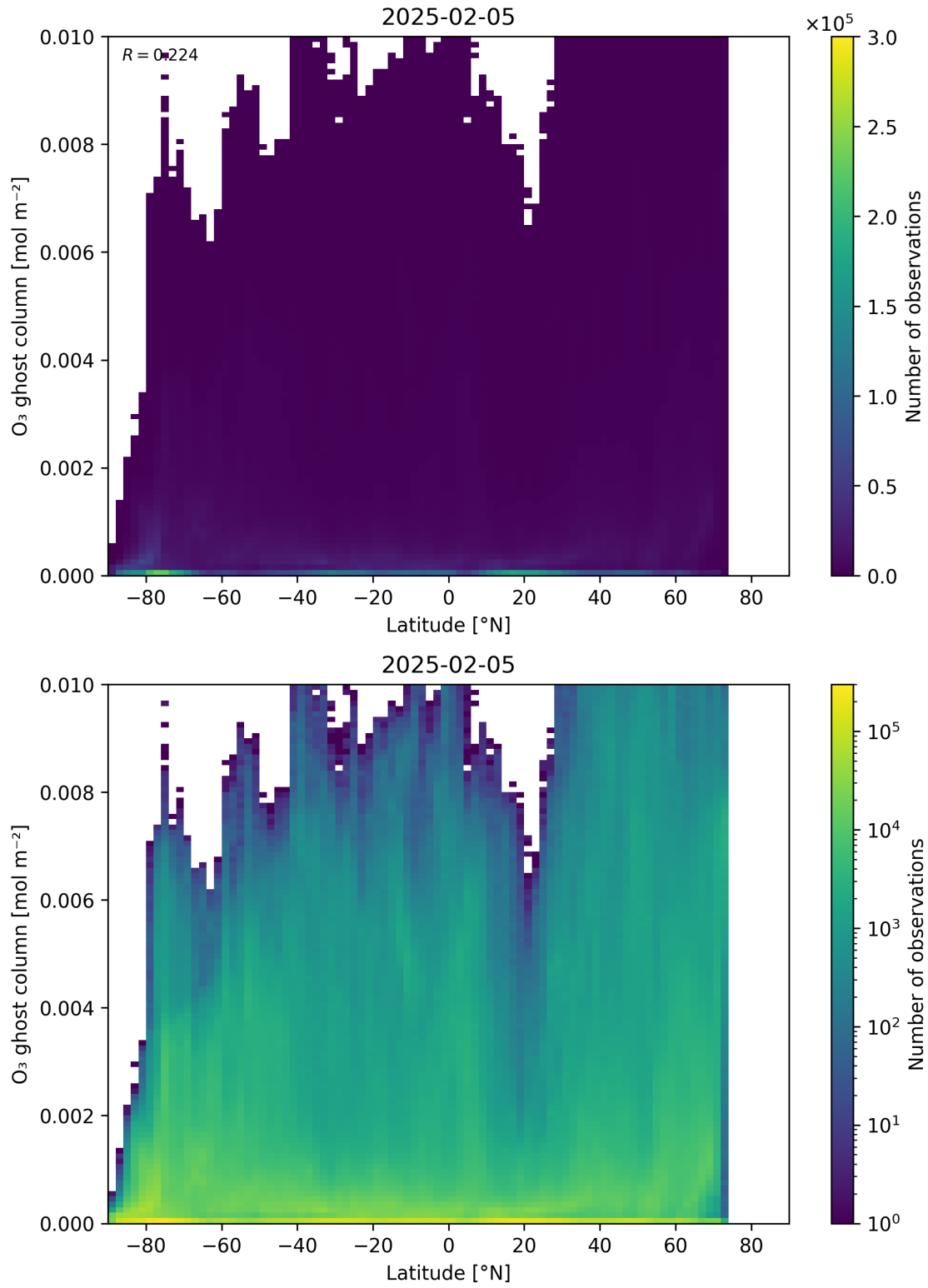
Figure 35: Scatter density plot of “Latitude” against “O 3 ghost column” for 2025-02-04 to 2025-02-06.
