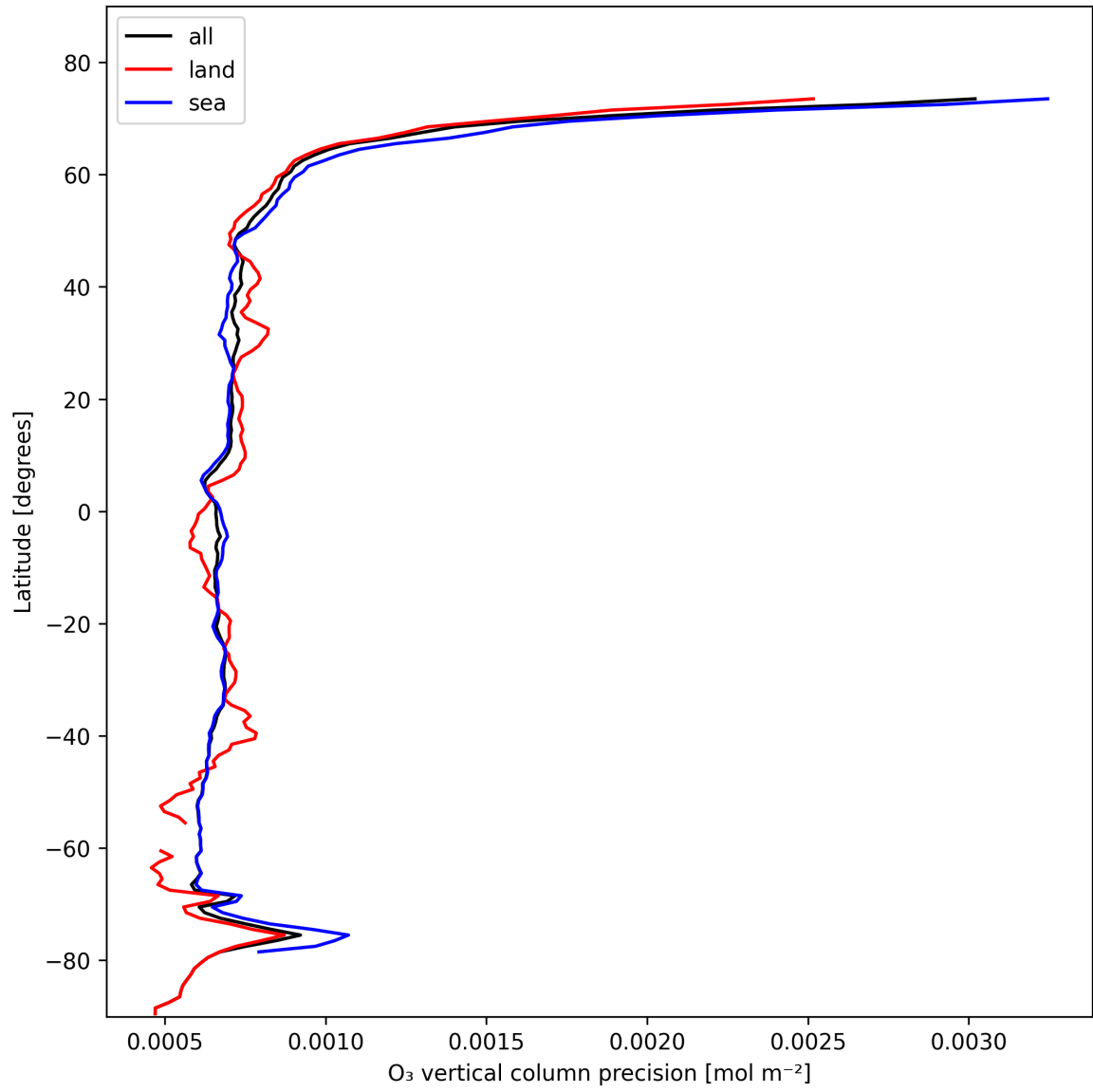
Figure 15: Zonal average of “O 3 vertical column precision” for 2025-02-04 to 2025-02-06.
