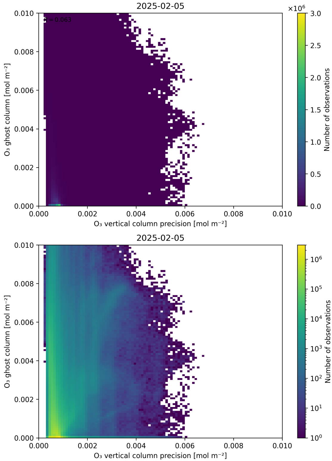
Figure 43: Scatter density plot of “O 3 vertical column precision” against “O 3 ghost column” for 2025-02-04 to 2025-02-06.
