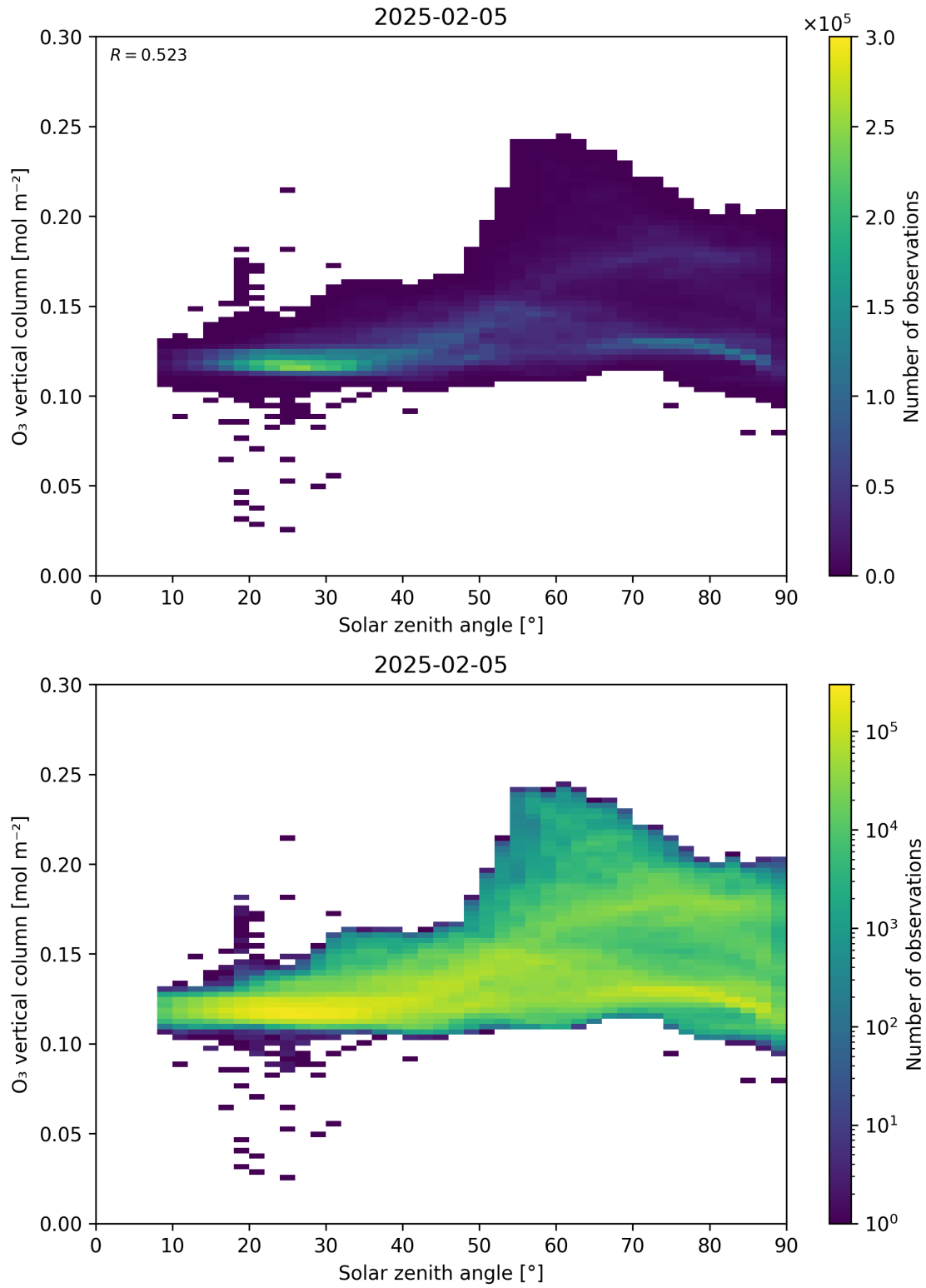
Figure 47: Scatter density plot of “Solar zenith angle” against “O 3 vertical column” for 2025-02-04 to 2025-02-06.
