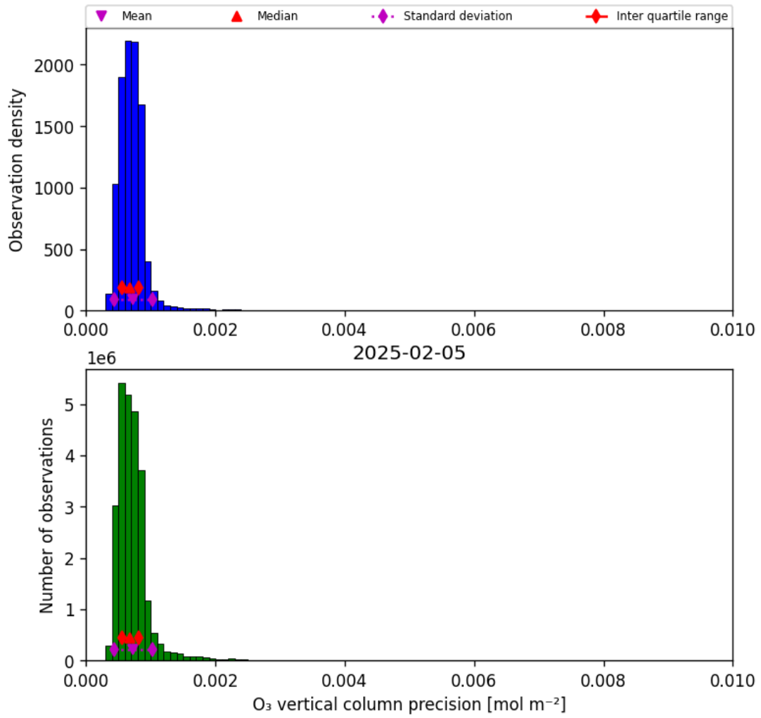
Figure 22: Histogram of “O 3 vertical column precision” for 2025-02-04 to 2025-02-06
