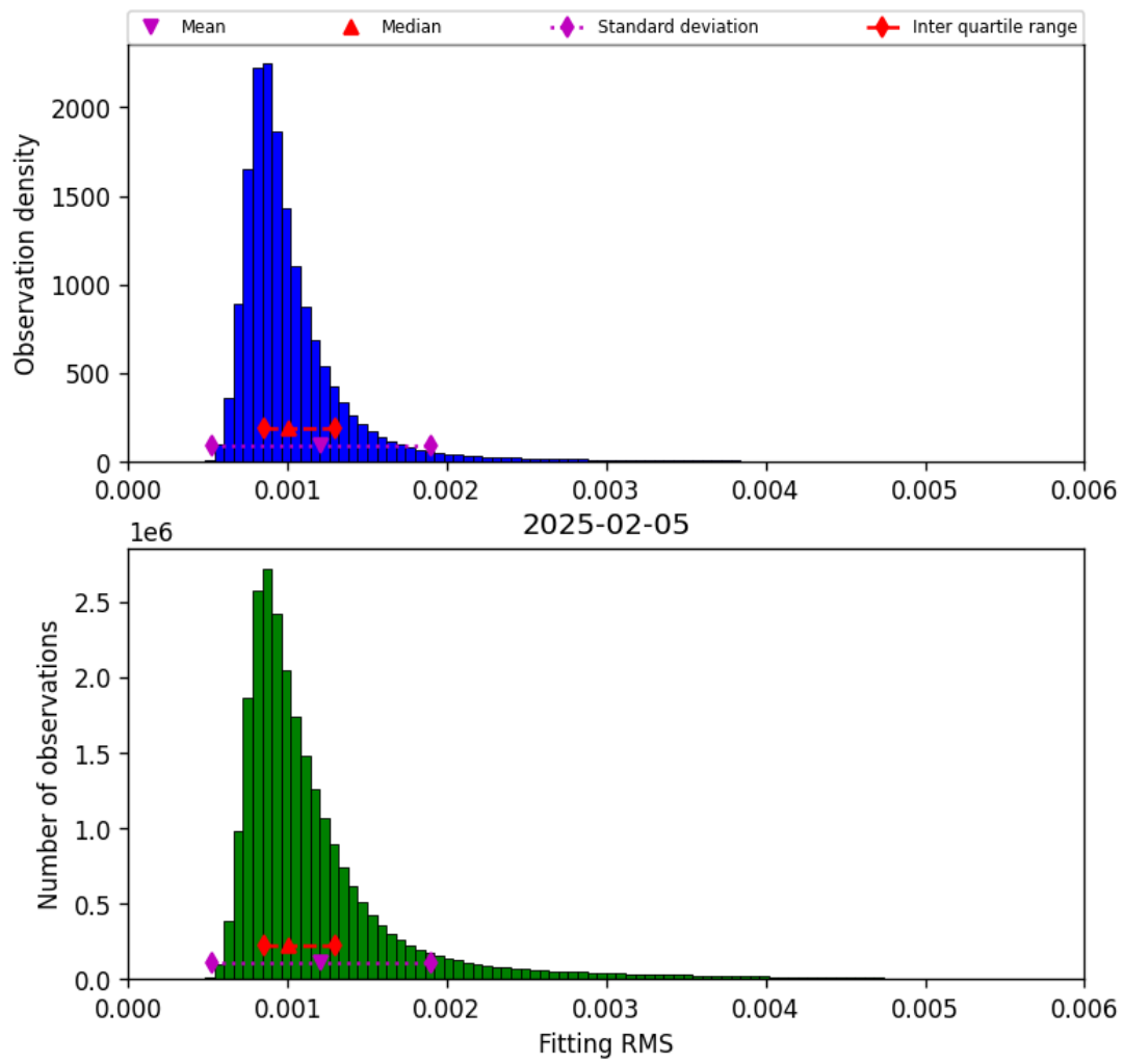
Figure 23: Histogram of “Fitting RMS” for 2025-02-04 to 2025-02-06
