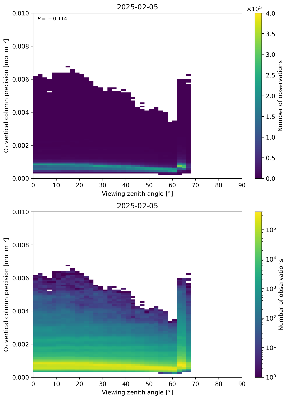
Figure 53: Scatter density plot of “Viewing zenith angle” against “O 3 vertical column precision” for 2025-02-04 to 2025-02-06.
