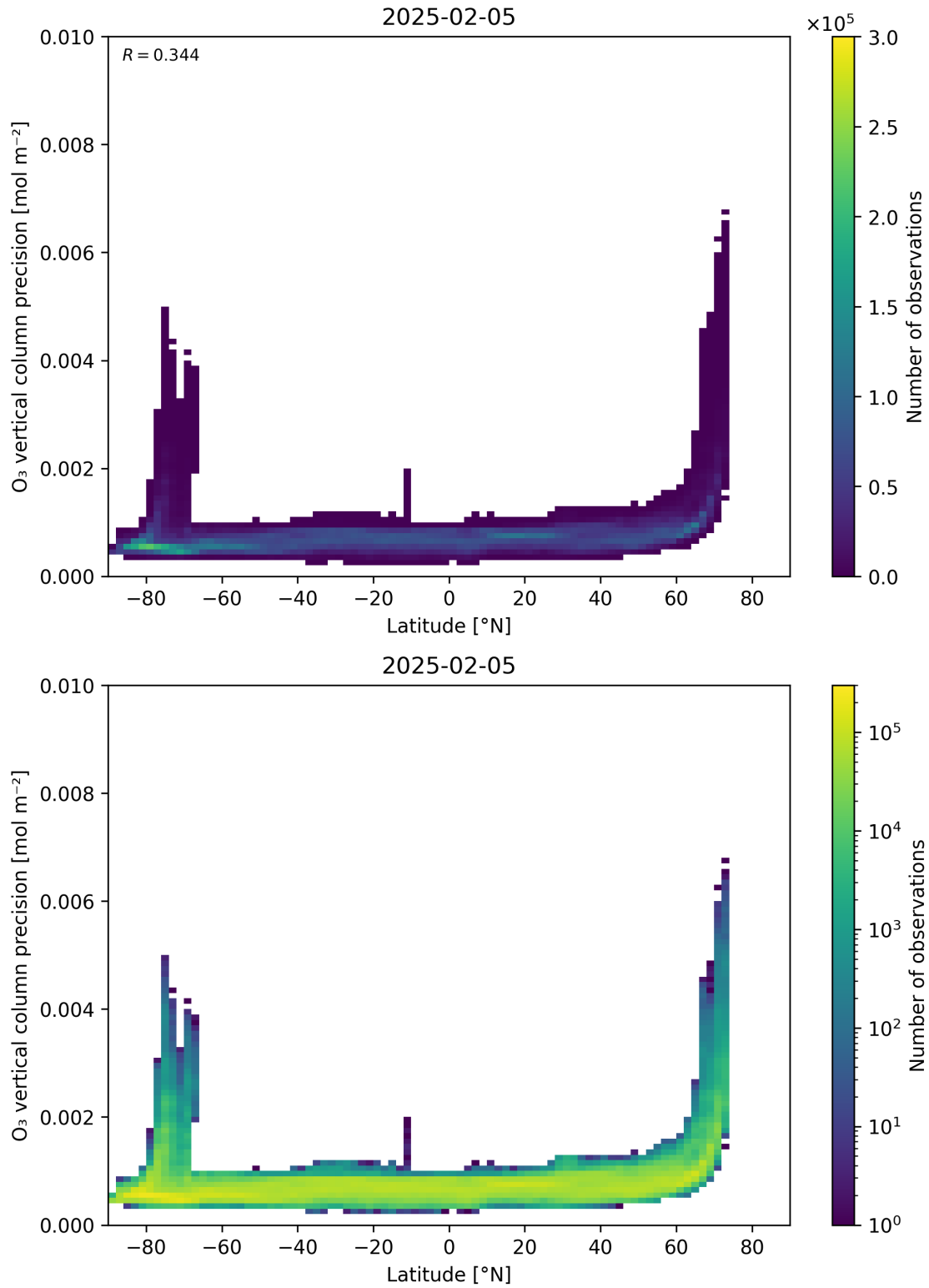
Figure 37: Scatter density plot of “Latitude” against “O 3 vertical column precision” for 2025-02-04 to 2025-02-06.
