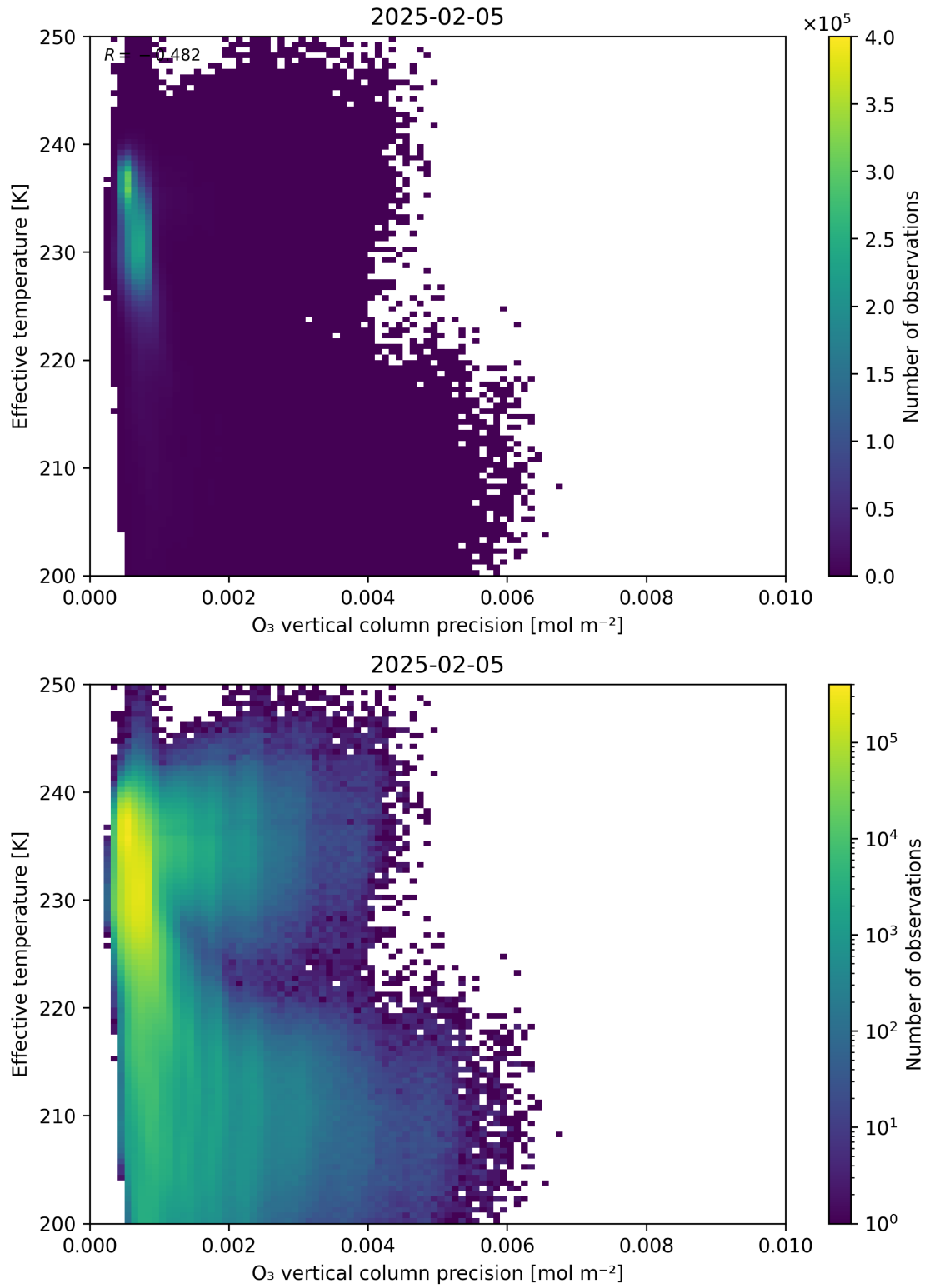
Figure 42: Scatter density plot of “O 3 vertical column precision” against “Effective temperature” for 2025-02-04 to 2025-02-06.
