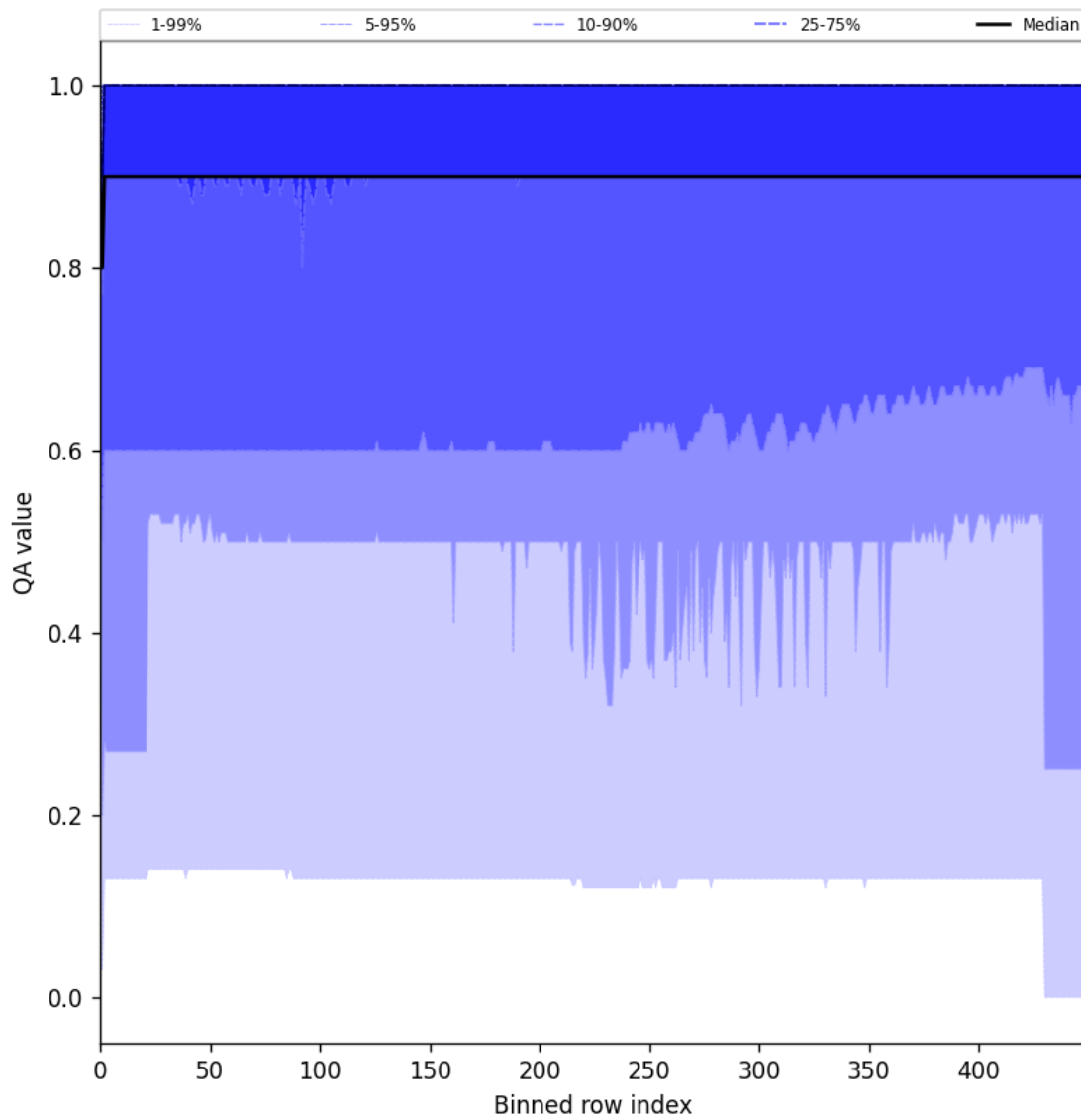
Figure 27: Along track statistics of “QA value” for 2025-02-04 to 2025-02-06
