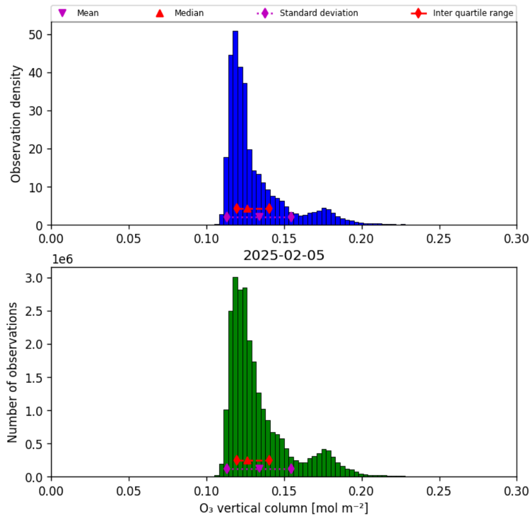
Figure 21: Histogram of “O 3 vertical column” for 2025-02-04 to 2025-02-06
