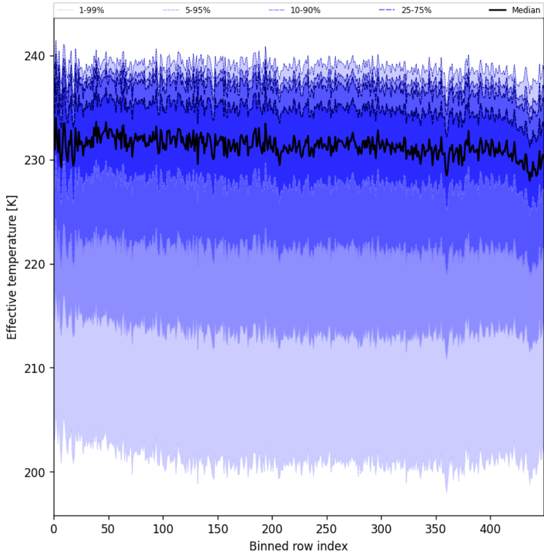
Figure 31: Along track statistics of “Effective temperature” for 2025-02-04 to 2025-02-06
