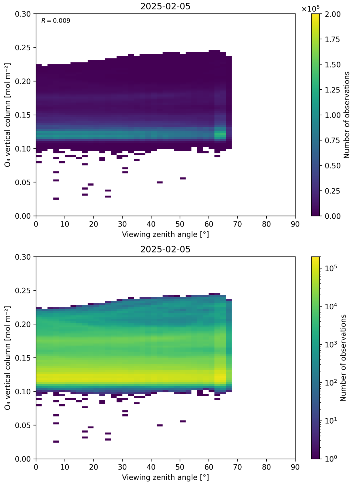
Figure 52: Scatter density plot of “Viewing zenith angle” against “O 3 vertical column” for 2025-02-04 to 2025-02-06.
