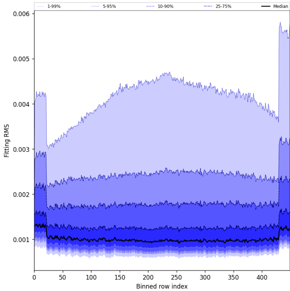
Figure 30: Along track statistics of “Fitting RMS” for 2025-02-04 to 2025-02-06
