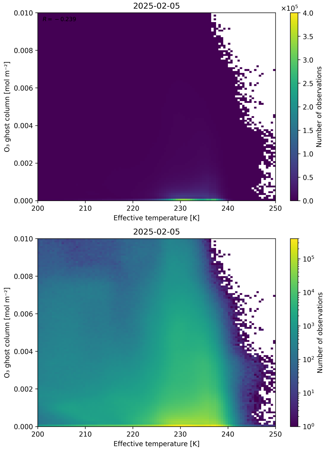
Figure 38: Scatter density plot of “Effective temperature” against “O 3 ghost column” for 2025-02-04 to 2025-02-06.
