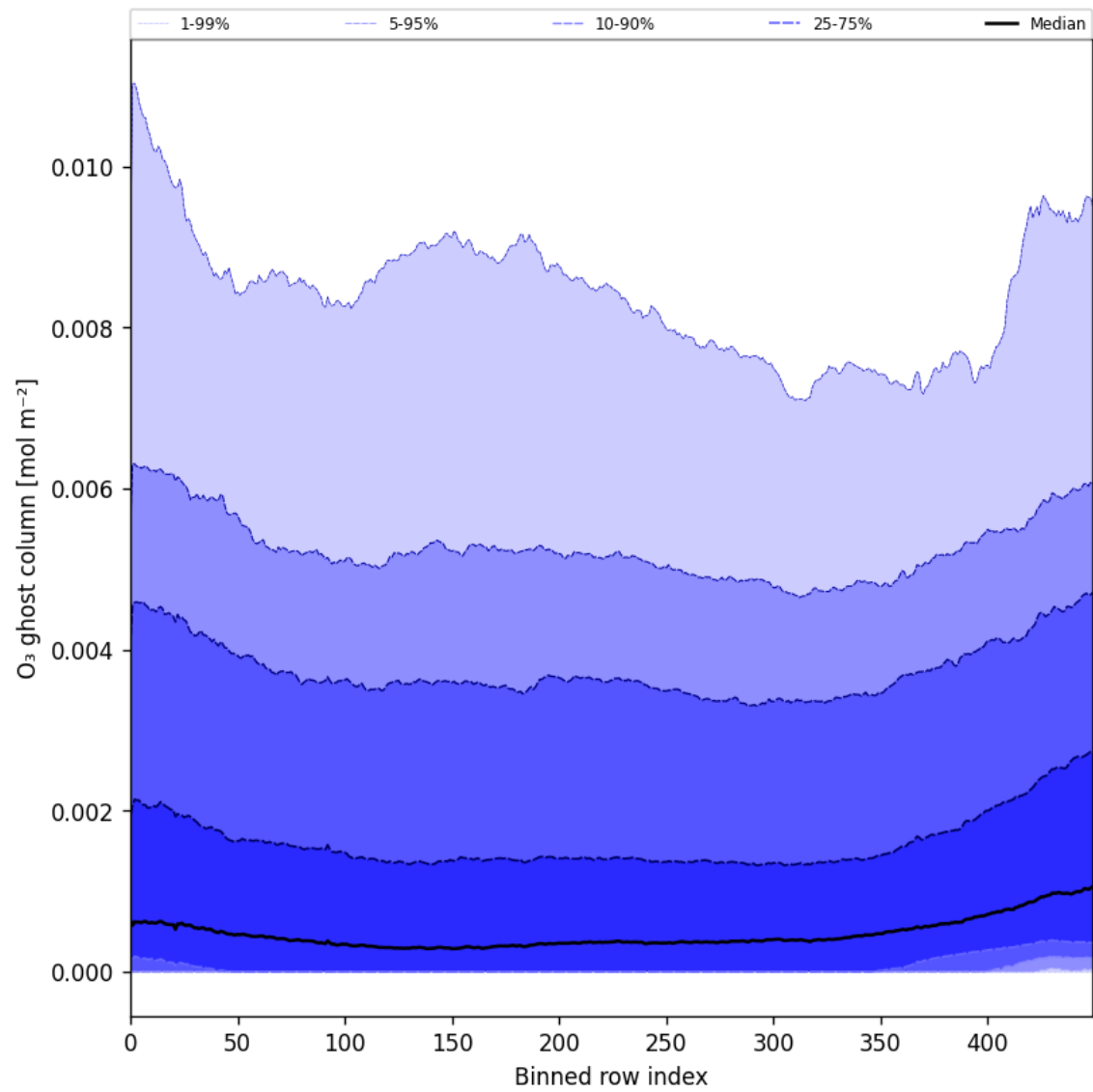
Figure 32: Along track statistics of “O 3 ghost column” for 2025-02-04 to 2025-02-06
