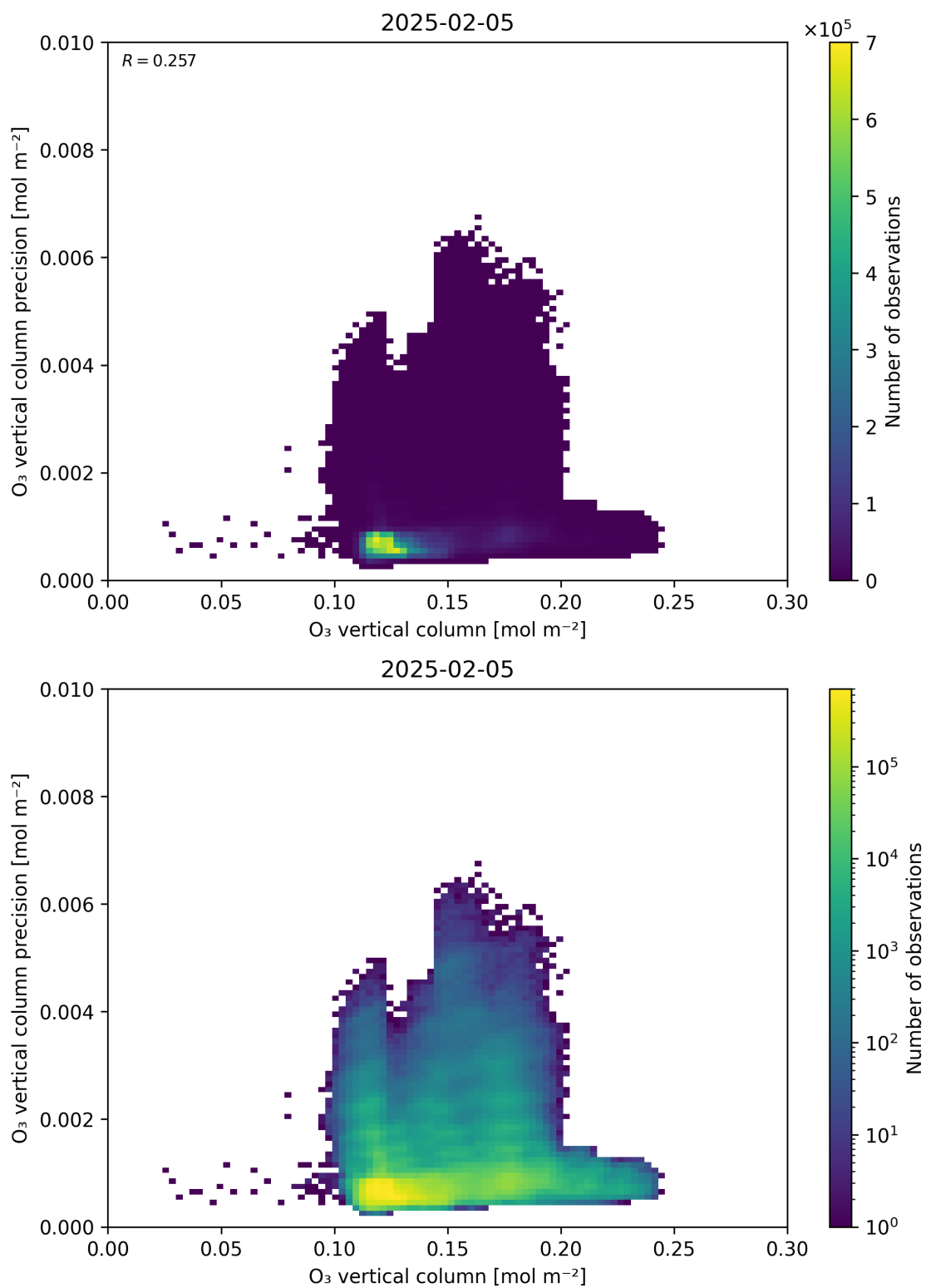
Figure 41: Scatter density plot of “O 3 vertical column” against “O 3 vertical column precision” for 2025-02-04 to 2025-02-06.
