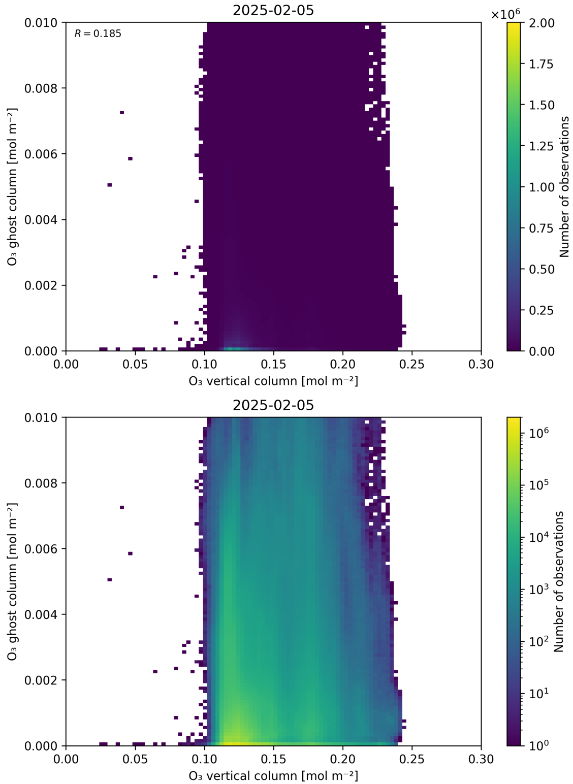
Figure 40: Scatter density plot of “O 3 vertical column” against “O 3 ghost column” for 2025-02-04 to 2025-02-06.
