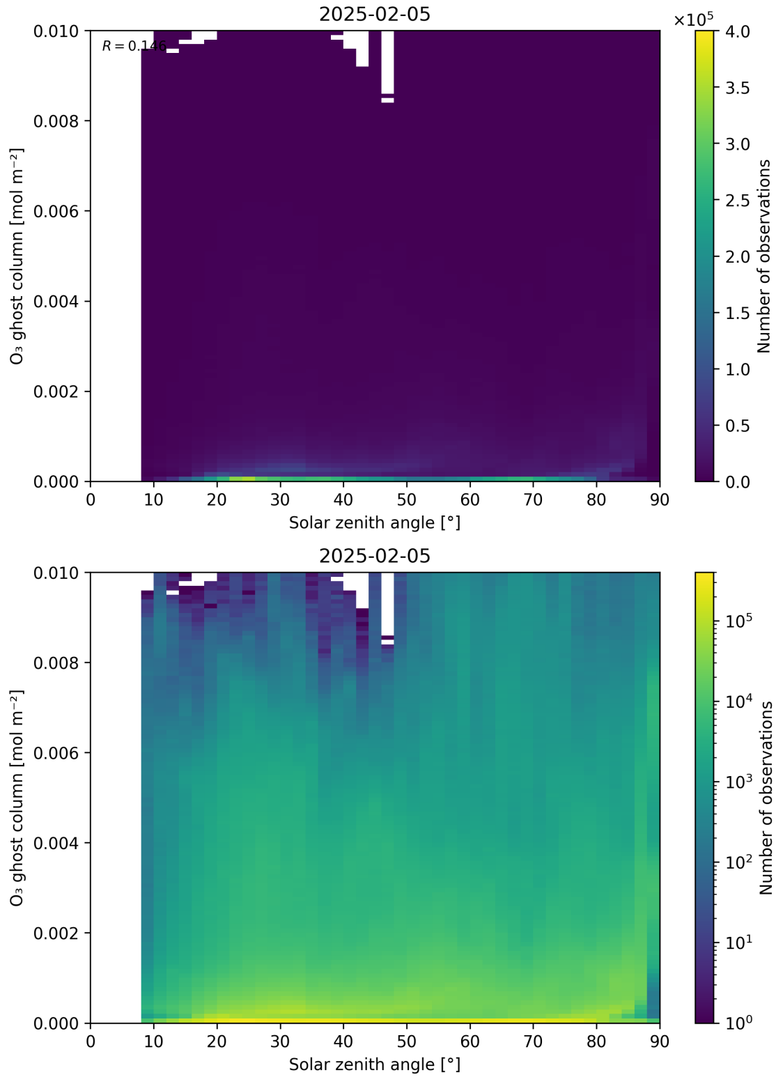
Figure 46: Scatter density plot of “Solar zenith angle” against “O 3 ghost column” for 2025-02-04 to 2025-02-06.
