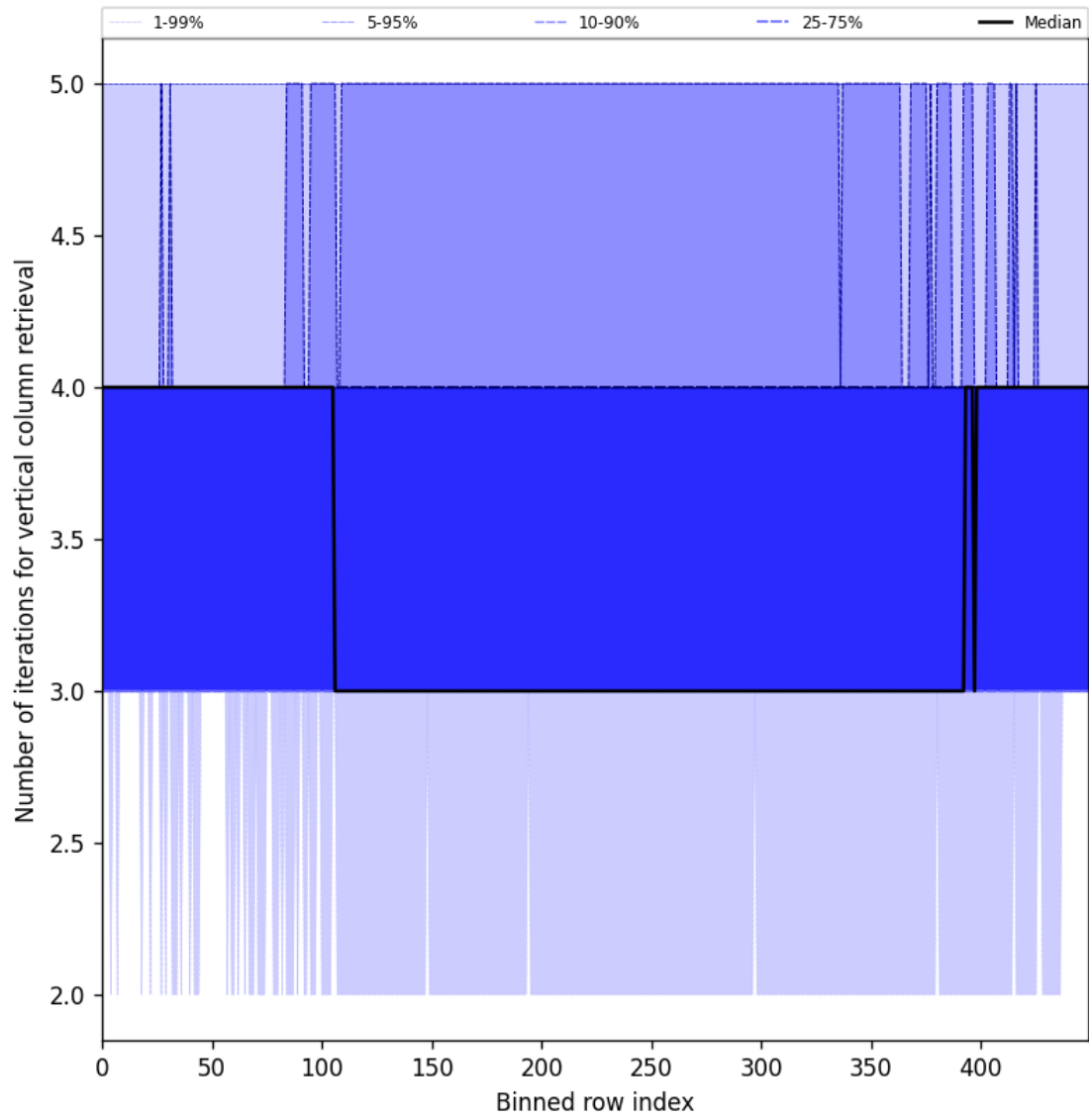
Figure 33: Along track statistics of “Number of iterations for vertical column retrieval” for 2025-02-04 to 2025-02-06
