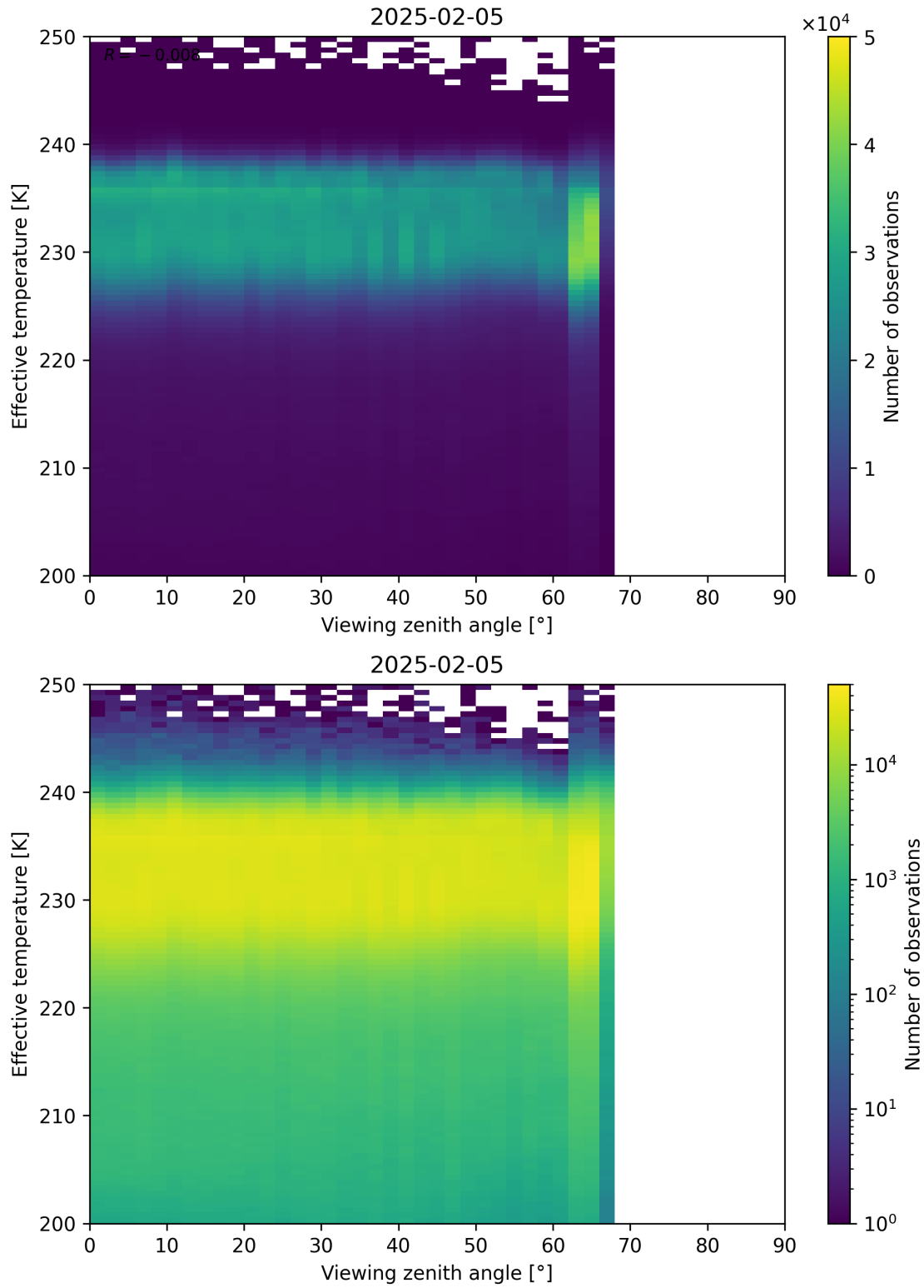
Figure 50: Scatter density plot of “Viewing zenith angle” against “Effective temperature” for 2025-02-04 to 2025-02-06.
