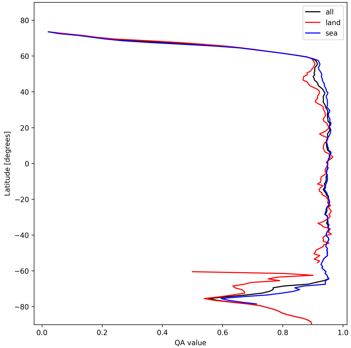
Figure 13: Zonal average of “QA value” for 2025-02-04 to 2025-02-06.
