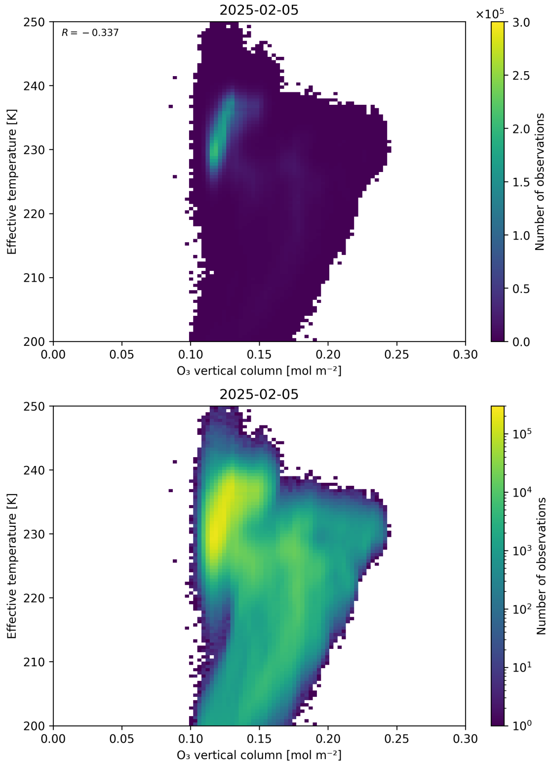
Figure 39: Scatter density plot of “O 3 vertical column” against “Effective temperature” for 2025-02-04 to 2025-02-06.
