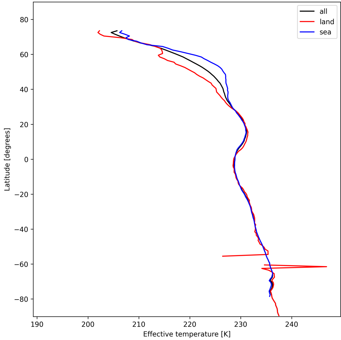
Figure 17: Zonal average of "Effective temperature" for 2025-02-04 to 2025-02-06.
