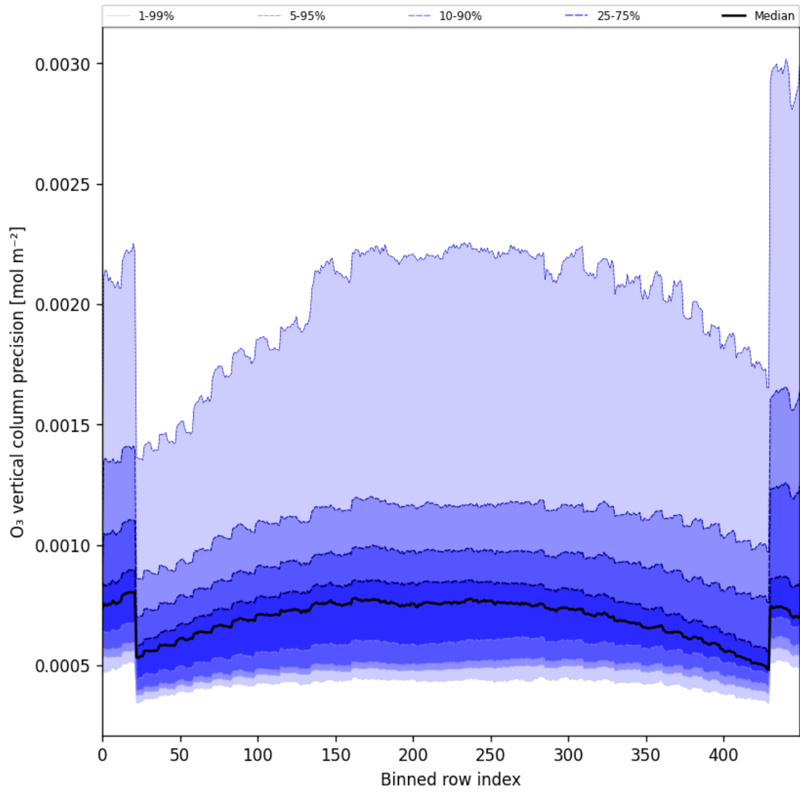
Figure 29: Along track statistics of “O 3 vertical column precision” for 2025-02-04 to 2025-02-06
