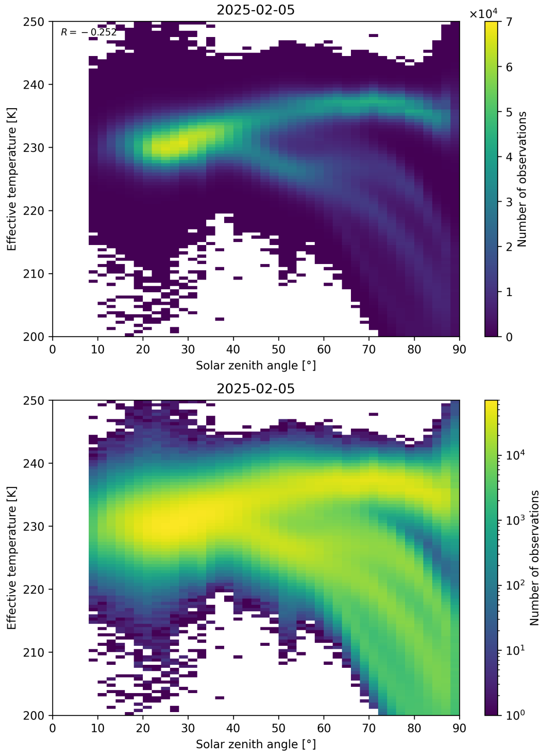
Figure 45: Scatter density plot of “Solar zenith angle” against “Effective temperature” for 2025-02-04 to 2025-02-06.
