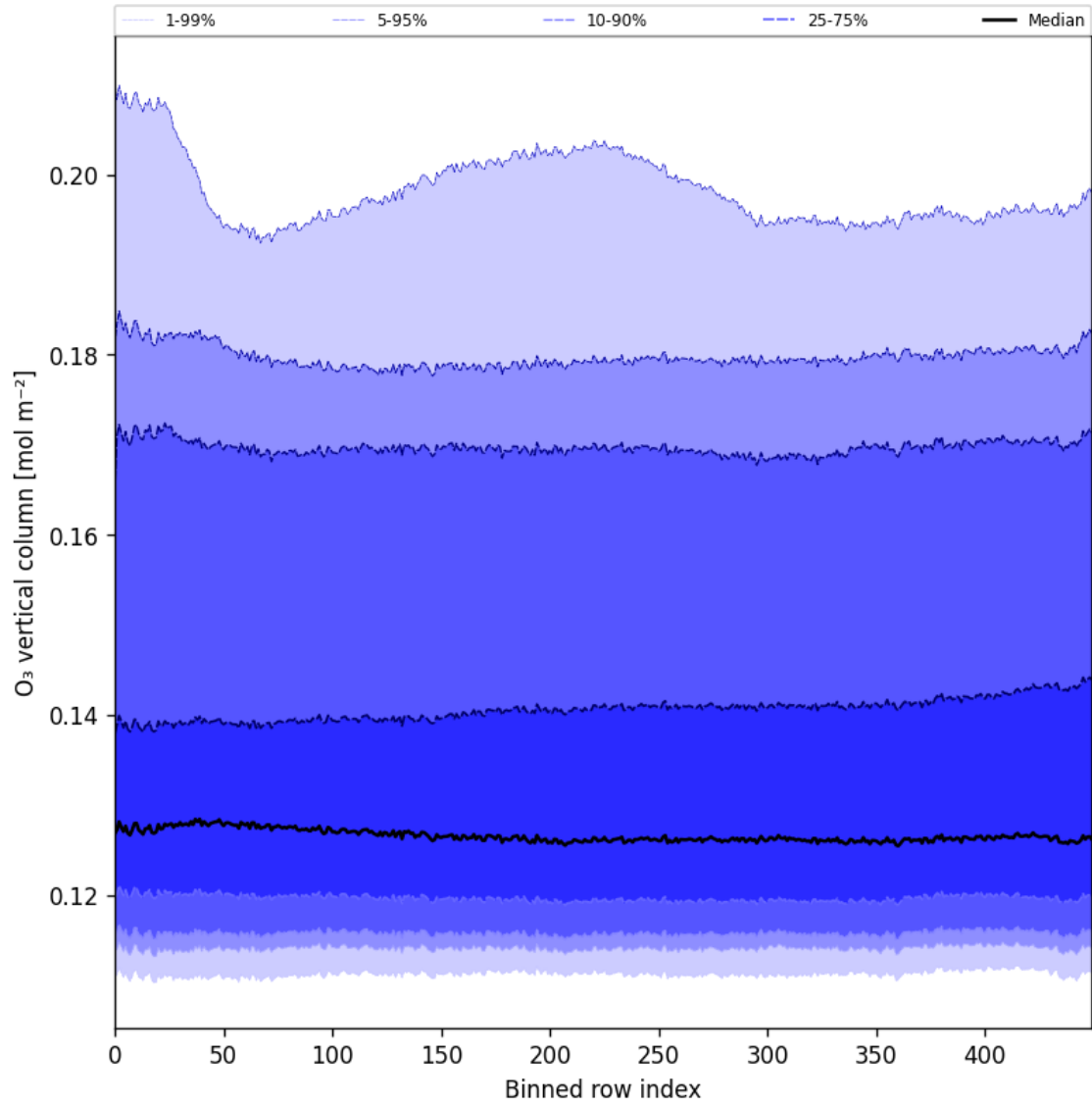
Figure 28: Along track statistics of "O 3 vertical column" for 2025-02-04 to 2025-02-06
