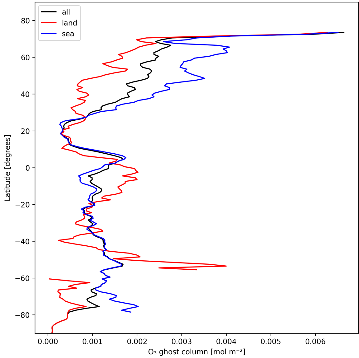
Figure 18: Zonal average of “O 3 ghost column” for 2025-02-04 to 2025-02-06.
