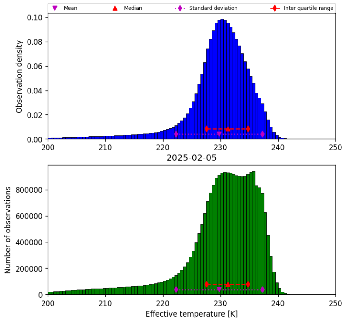
Figure 24: Histogram of “Effective temperature” for 2025-02-04 to 2025-02-06
