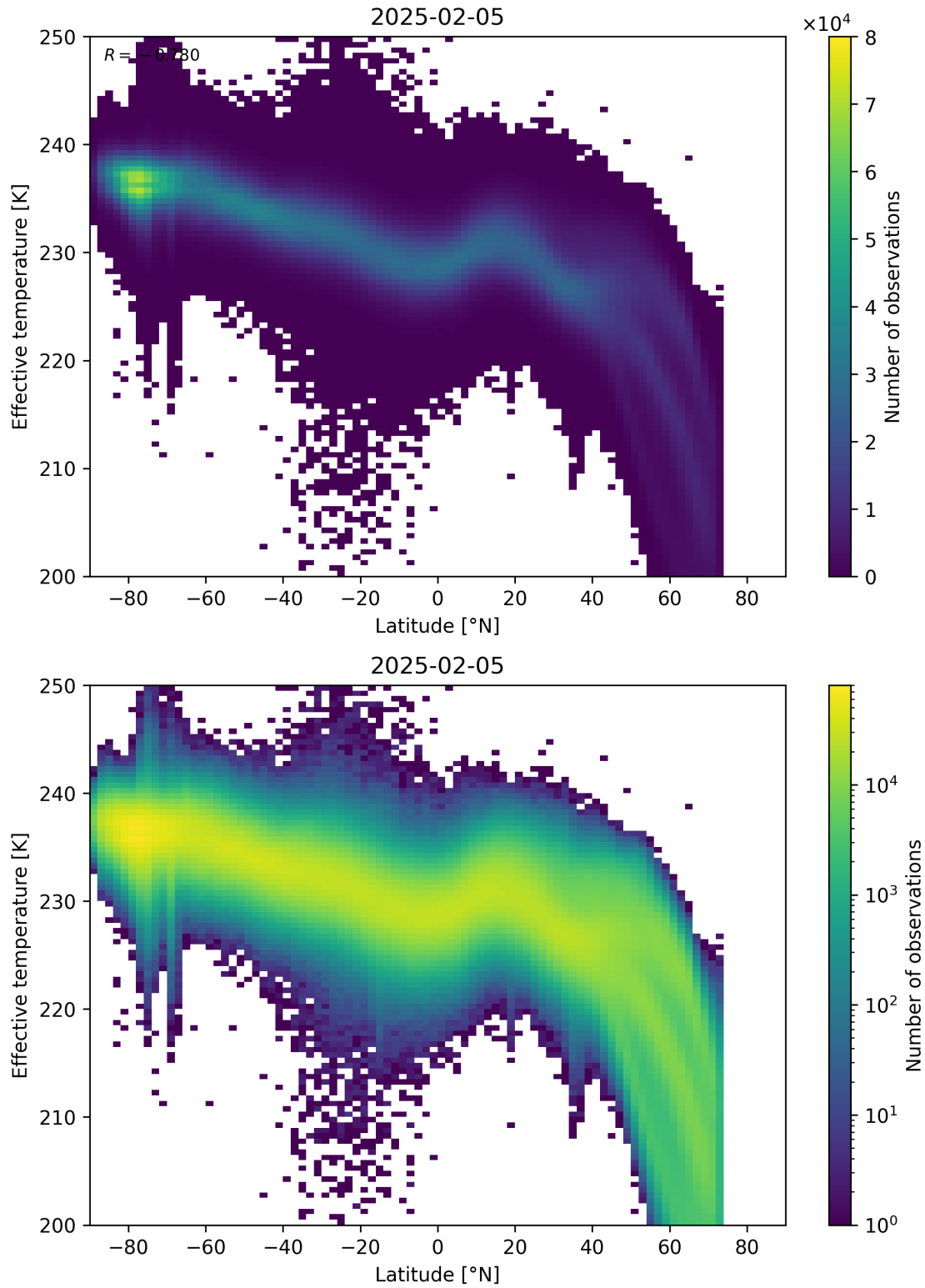
Figure 34: Scatter density plot of “Latitude” against “Effective temperature” for 2025-02-04 to 2025-02-06.
