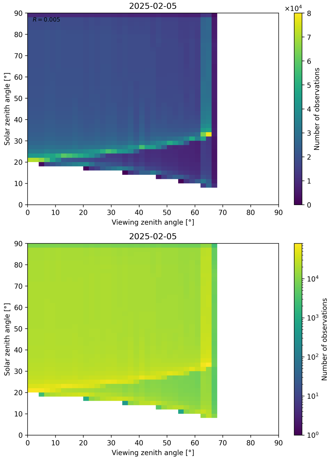
Figure 54: Scatter density plot of “Viewing zenith angle” against “Solar zenith angle” for 2025-02-04 to 2025-02-06.
