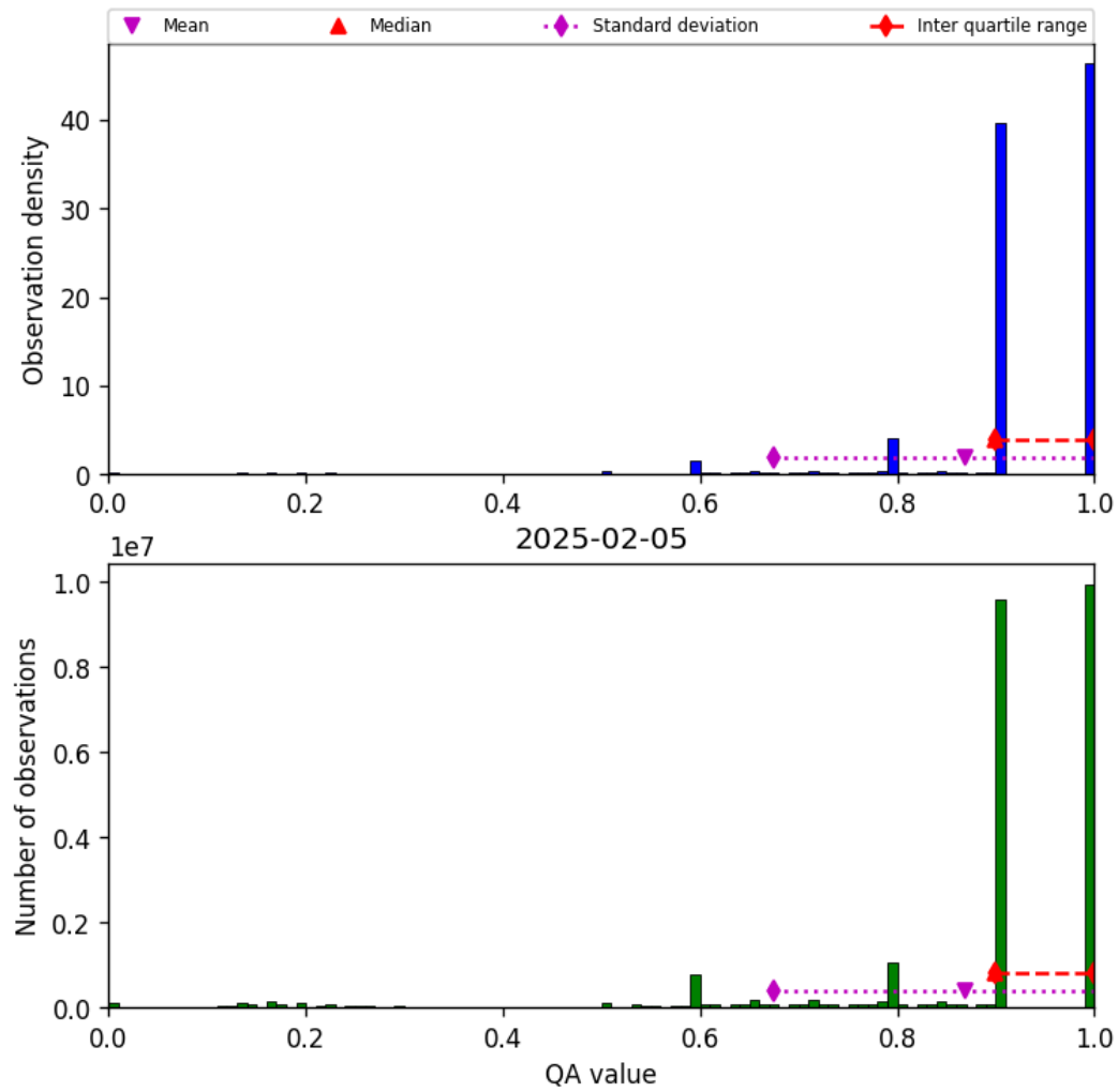
Figure 20: Histogram of “QA value” for 2025-02-04 to 2025-02-06
