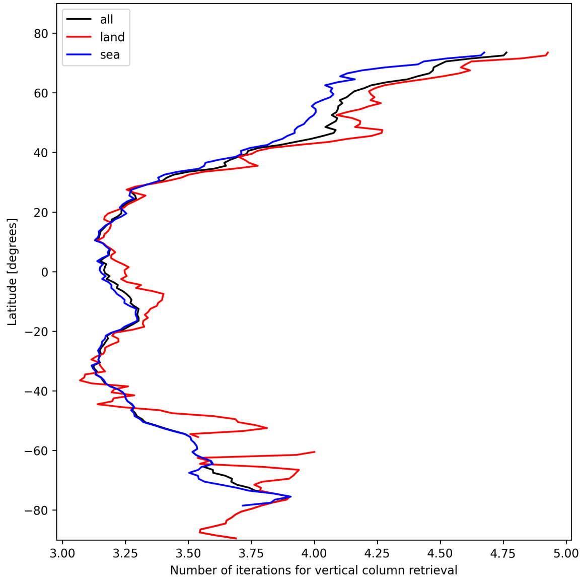
Figure 19: Zonal average of “Number of iterations for vertical column retrieval” for 2025-02-04 to 2025-02-06.
