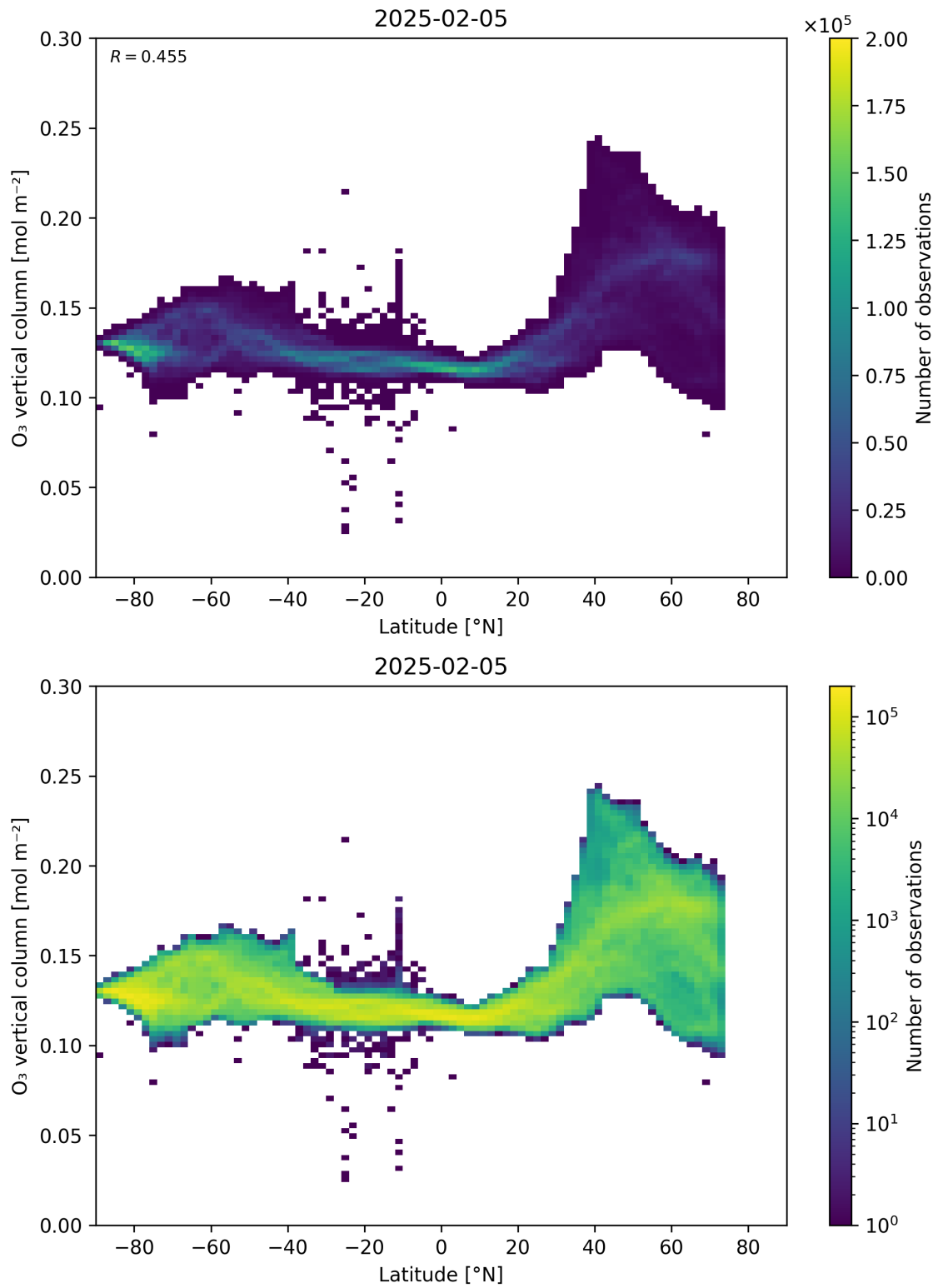
Figure 36: Scatter density plot of “Latitude” against “O 3 vertical column” for 2025-02-04 to 2025-02-06.
