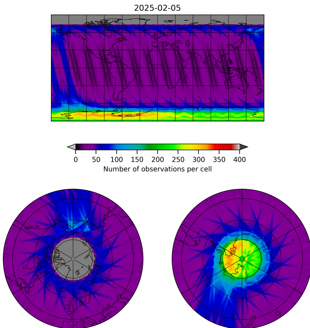
Figure 12: Map of the number of observations for 2025-02-04 to 2025-02-06
