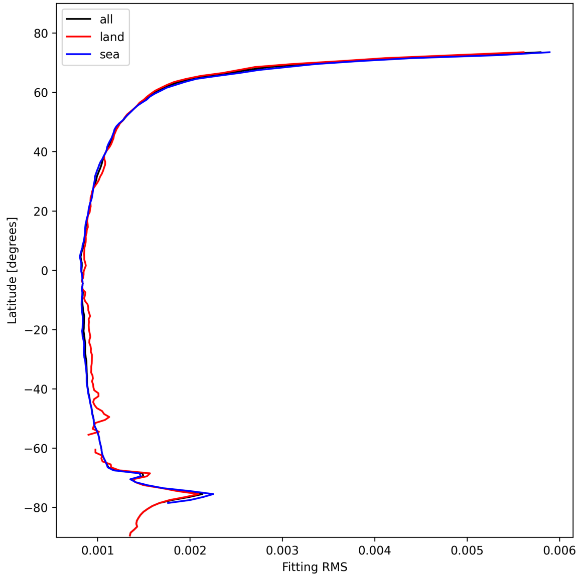
Figure 16: Zonal average of “Fitting RMS” for 2025-02-04 to 2025-02-06.
