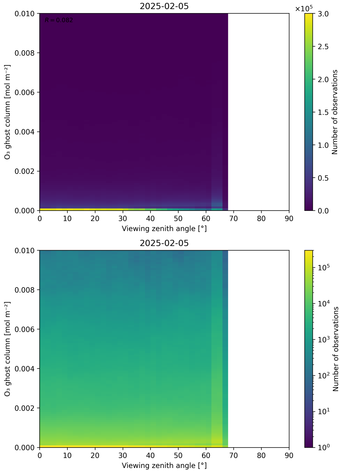
Figure 51: Scatter density plot of “Viewing zenith angle” against “O 3 ghost column” for 2025-02-04 to 2025-02-06.
